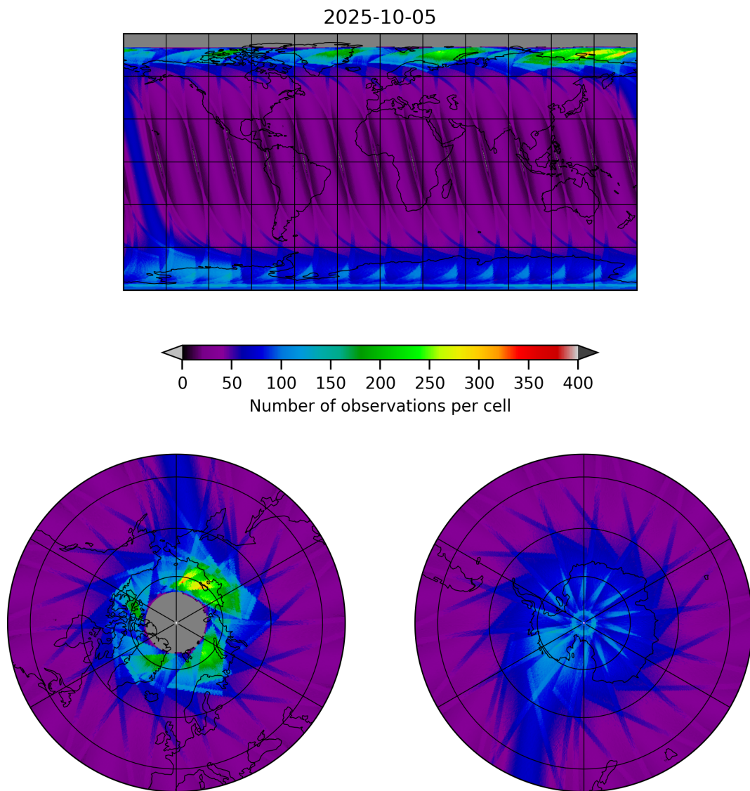
Figure 17: Map of the number of observations for 2025-10-05 to 2025-10-06
