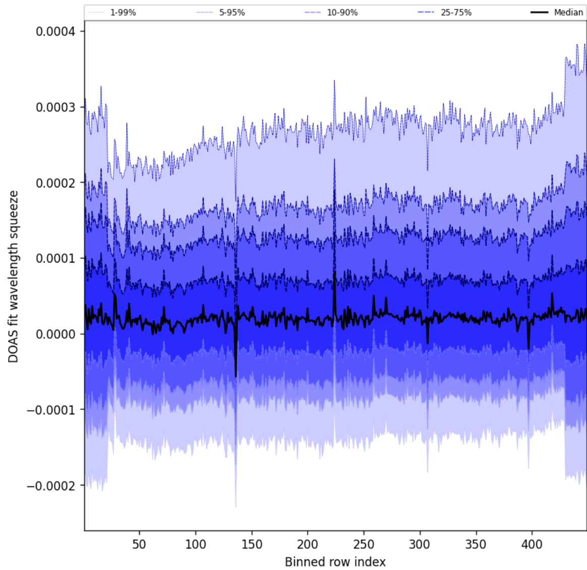
Figure 57: Along track statistics of “DOAS fit wavelength squeeze” for 2025-10-05 to 2025-10-06
