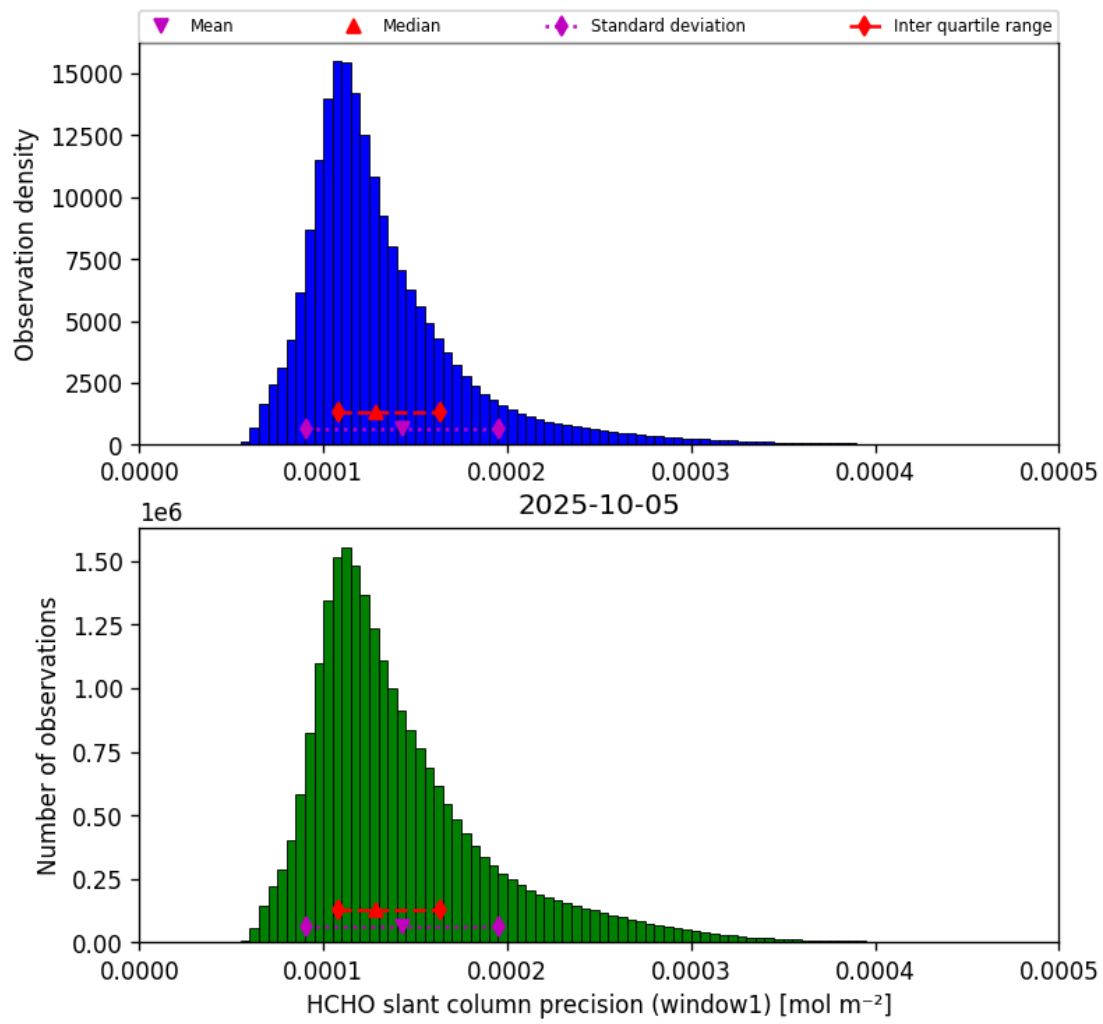
Figure 37: Histogram of “HCHO slant column precision (window1)” for 2025-10-05 to 2025-10-06
