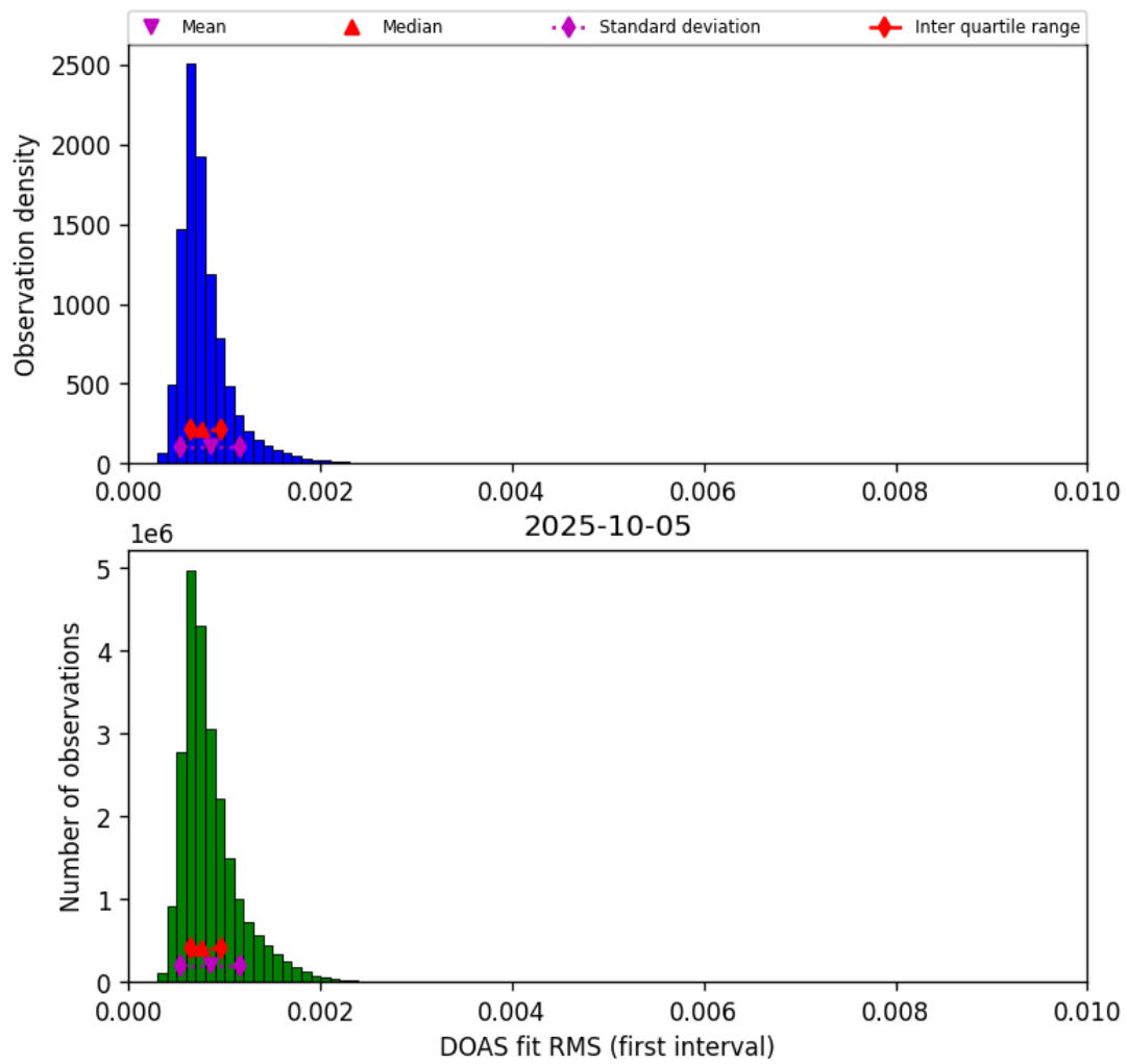
Figure 44: Histogram of “DOAS fit RMS (first interval)” for 2025-10-05 to 2025-10-06
