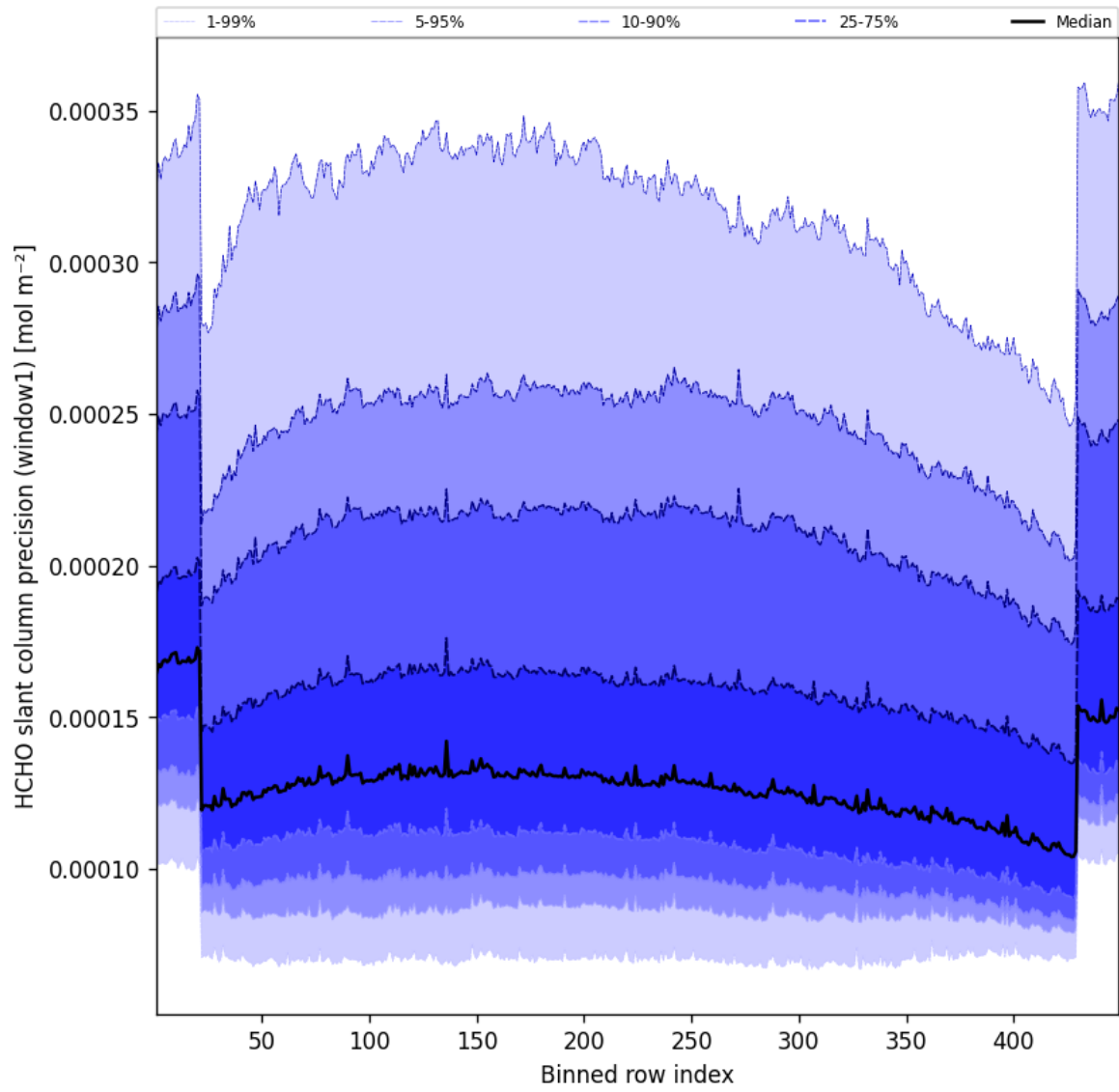
Figure 51: Along track statistics of “HCHO slant column precision (window1)” for 2025-10-05 to 2025-10-06
