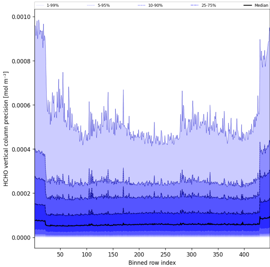
Figure 48: Along track statistics of “HCHO vertical column precision” for 2025-10-05 to 2025-10-06
