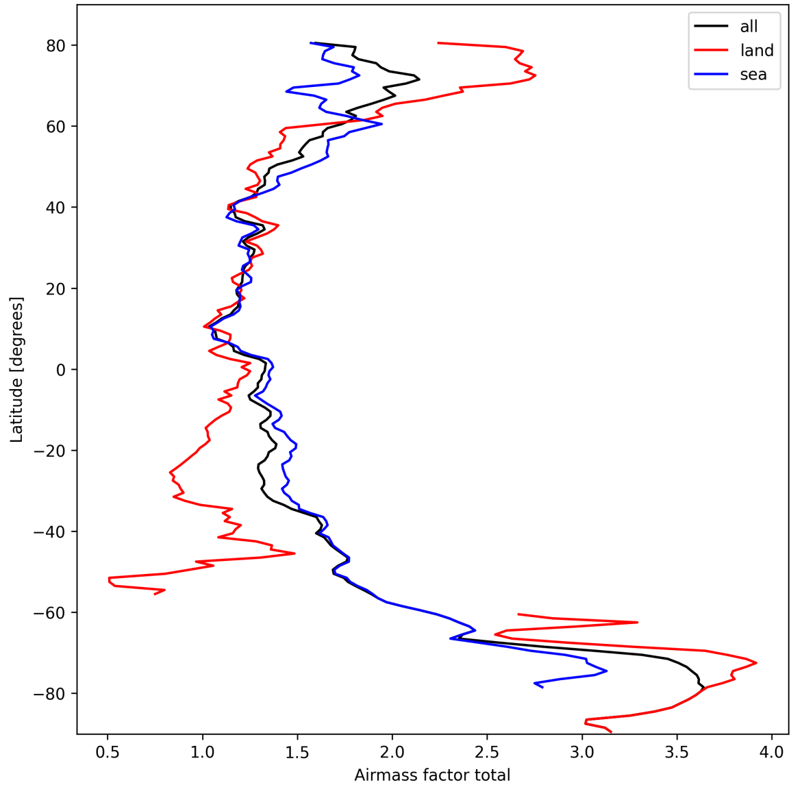
Figure 24: Zonal average of “Airmass factor total” for 2025-10-05 to 2025-10-06.
