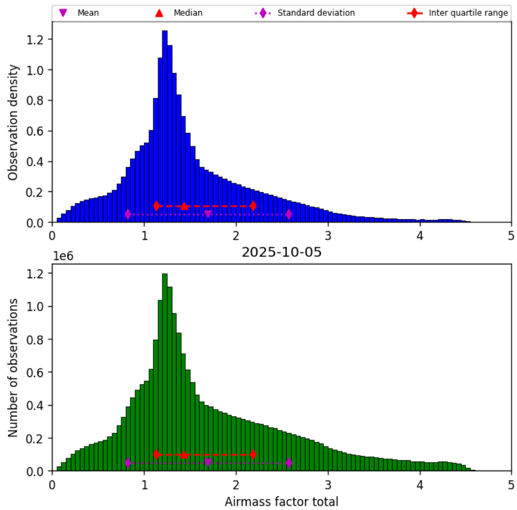
Figure 38: Histogram of “Airmass factor total” for 2025-10-05 to 2025-10-06
