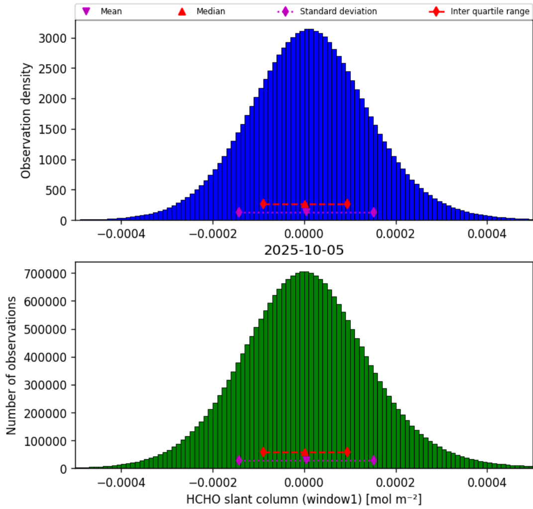
Figure 36: Histogram of “HCHO slant column (window1)” for 2025-10-05 to 2025-10-06
