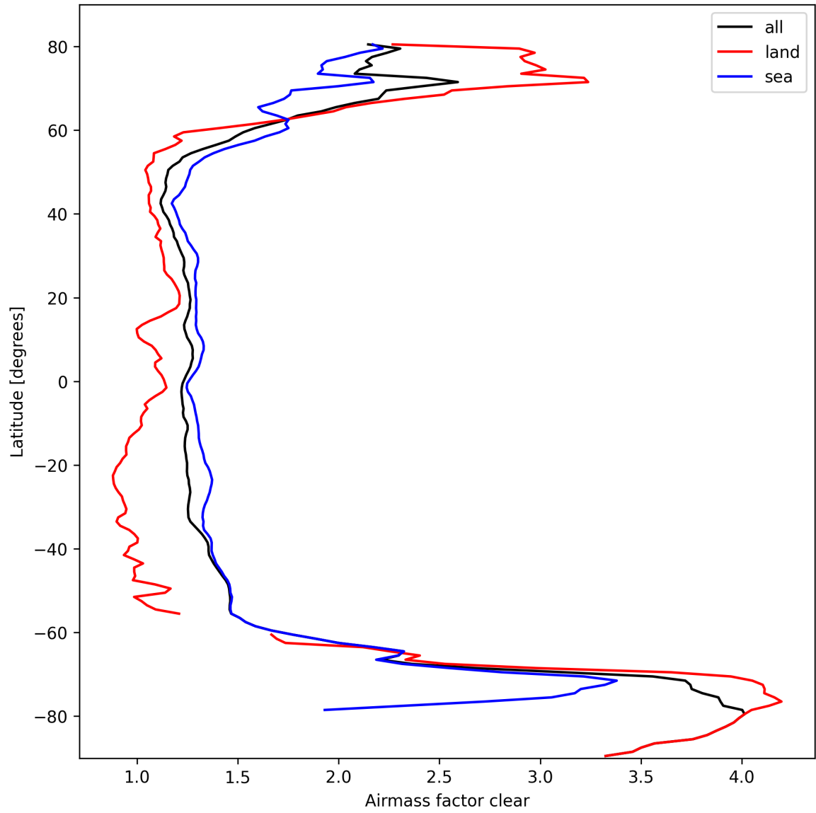
Figure 26: Zonal average of “Airmass factor clear” for 2025-10-05 to 2025-10-06.
