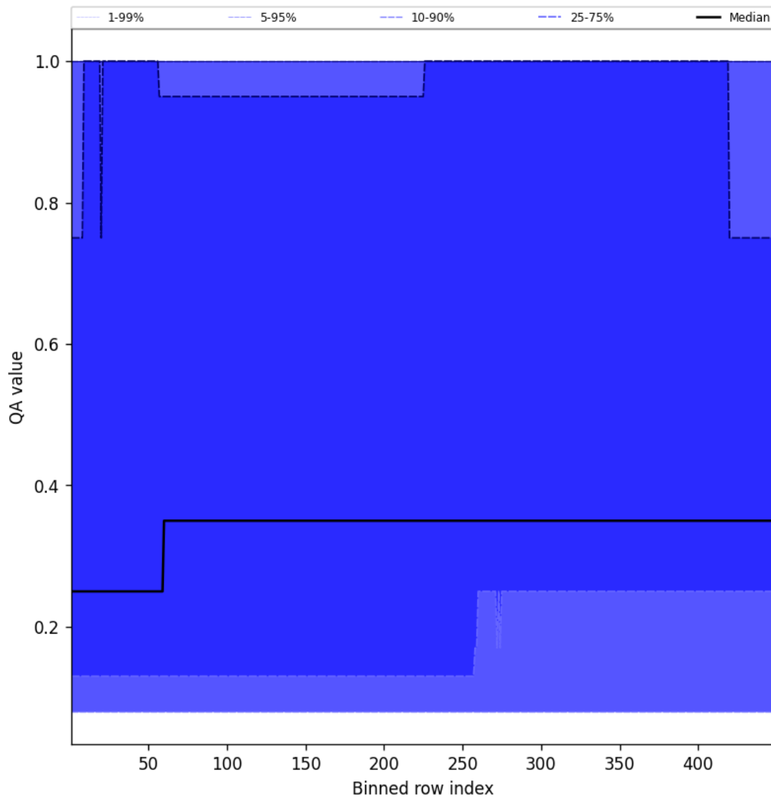
Figure 46: Along track statistics of “QA value” for 2025-10-05 to 2025-10-06
