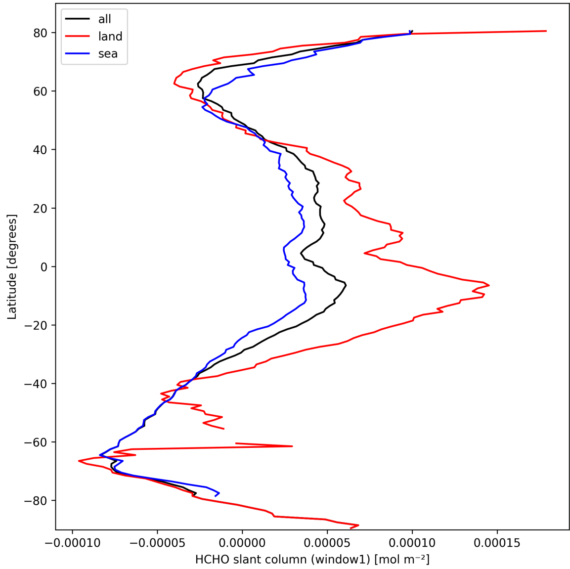
Figure 22: Zonal average of “HCHO slant column (window1)” for 2025-10-05 to 2025-10-06.
