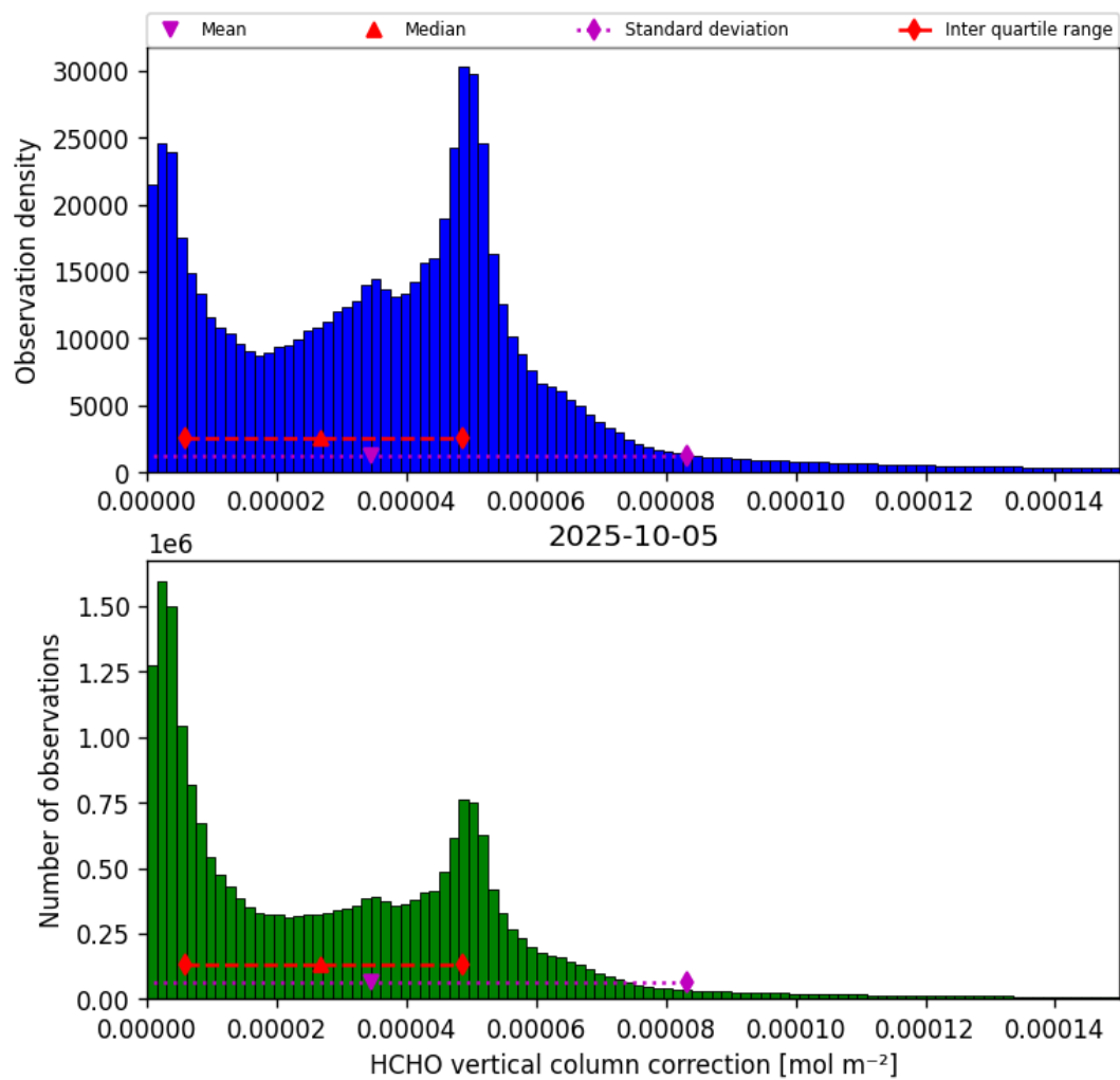
Figure 35: Histogram of “HCHO vertical column correction” for 2025-10-05 to 2025-10-06
