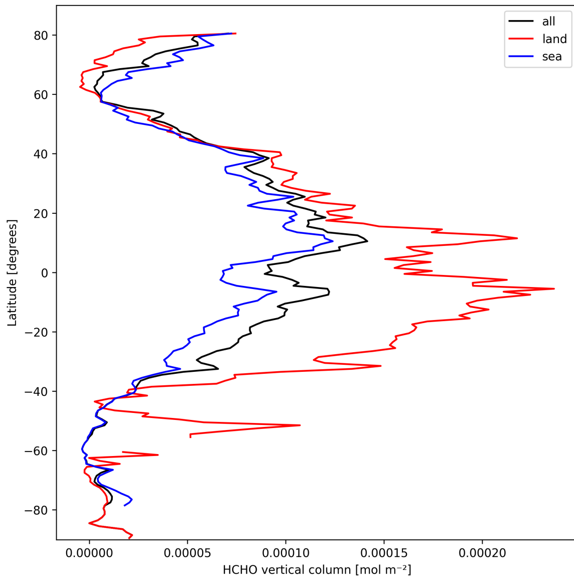
Figure 19: Zonal average of “HCHO vertical column” for 2025-10-05 to 2025-10-06.
