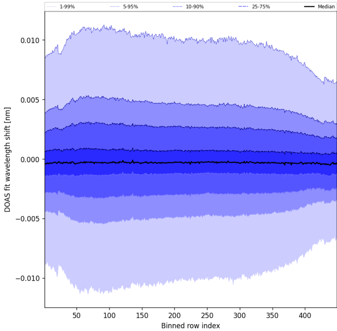
Figure 56: Along track statistics of “DOAS fit wavelength shift” for 2025-10-05 to 2025-10-06
