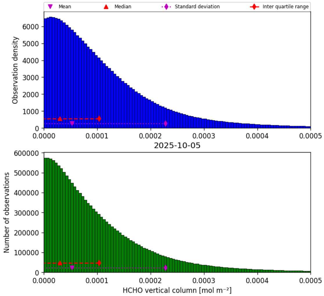
Figure 33: Histogram of “HCHO vertical column” for 2025-10-05 to 2025-10-06
