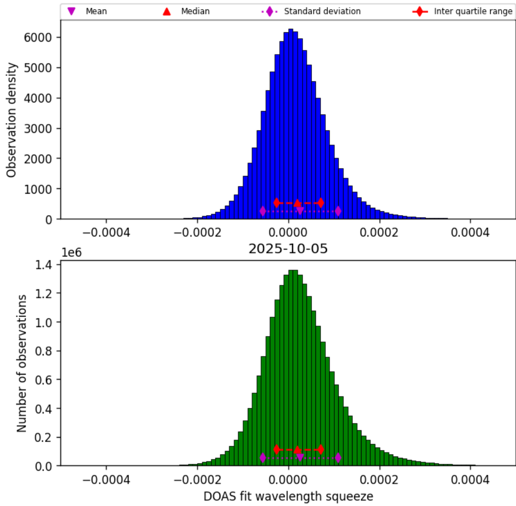
Figure 43: Histogram of “DOAS fit wavelength squeeze” for 2025-10-05 to 2025-10-06
