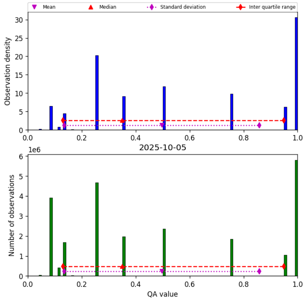
Figure 32: Histogram of “QA value” for 2025-10-05 to 2025-10-06
