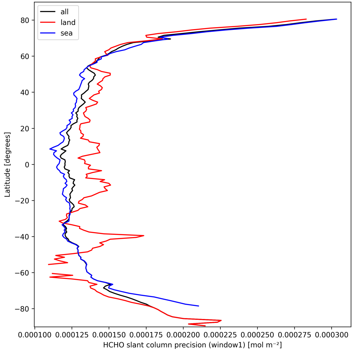
Figure 23: Zonal average of "HCHO slant column precision (window1)" for 2025-10-05 to 2025-10-06.
