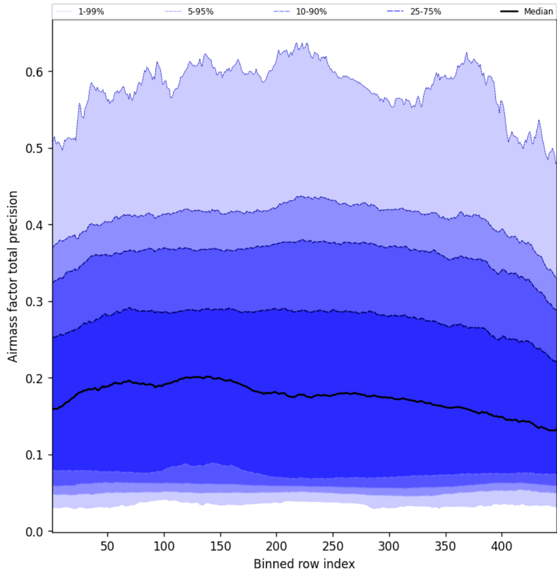
Figure 53: Along track statistics of “Airmass factor total precision” for 2025-10-05 to 2025-10-06
