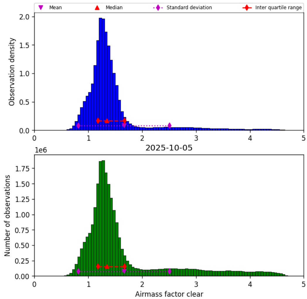
Figure 40: Histogram of “Airmass factor clear” for 2025-10-05 to 2025-10-06
