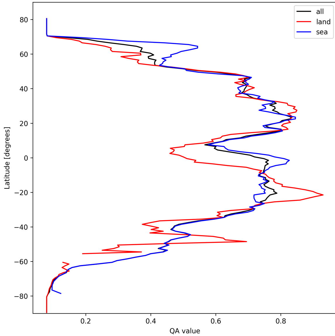
Figure 18: Zonal average of “QA value” for 2025-10-05 to 2025-10-06.
