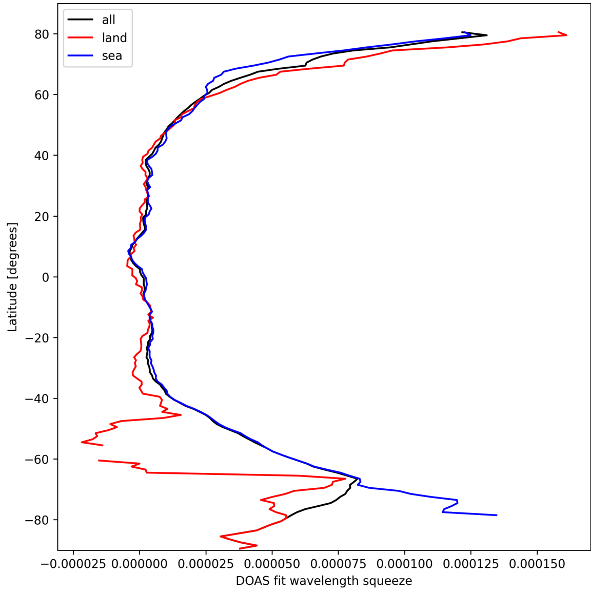
Figure 29: Zonal average of “DOAS fit wavelength squeeze” for 2025-10-05 to 2025-10-06.
