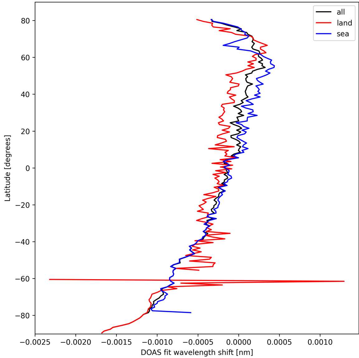
Figure 28: Zonal average of “DOAS fit wavelength shift” for 2025-10-05 to 2025-10-06.
