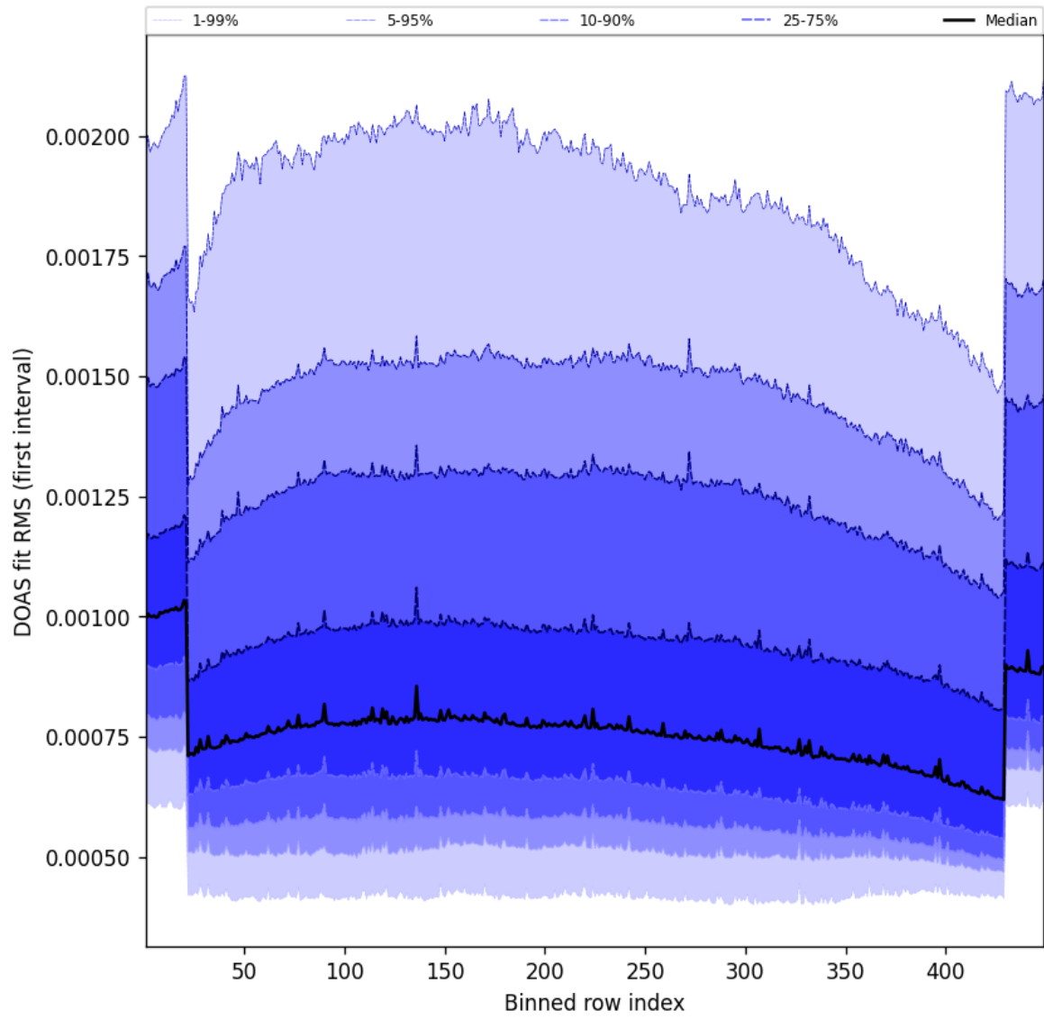
Figure 58: Along track statistics of “DOAS fit RMS (first interval)” for 2025-10-05 to 2025-10-06
