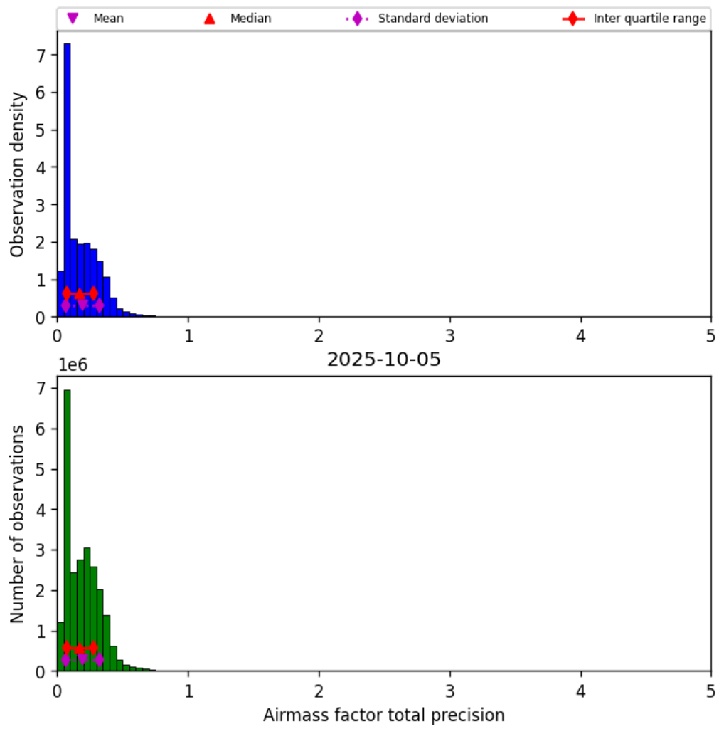
Figure 39: Histogram of “Airmass factor total precision” for 2025-10-05 to 2025-10-06
