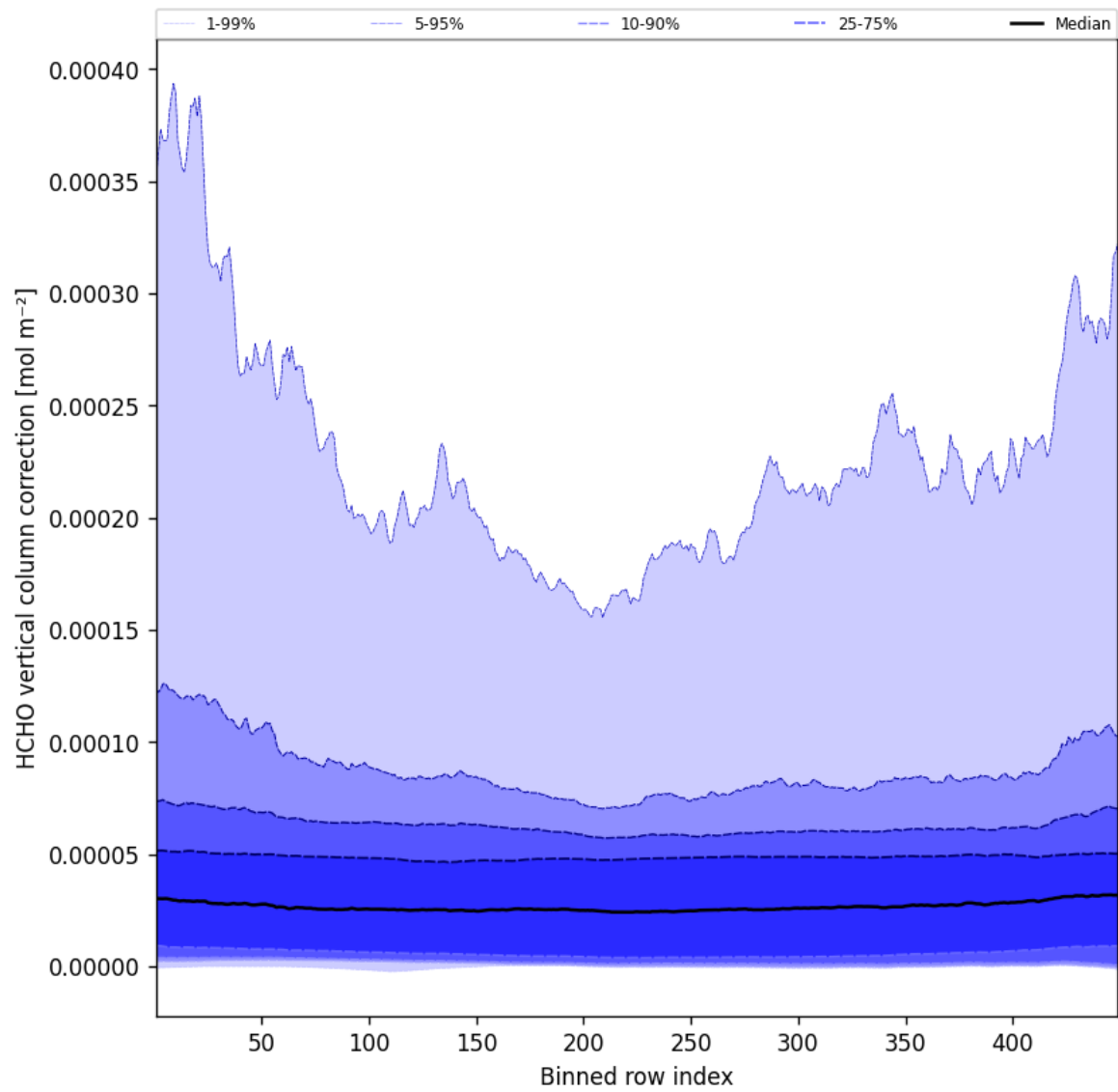
Figure 49: Along track statistics of “HCHO vertical column correction” for 2025-10-05 to 2025-10-06
