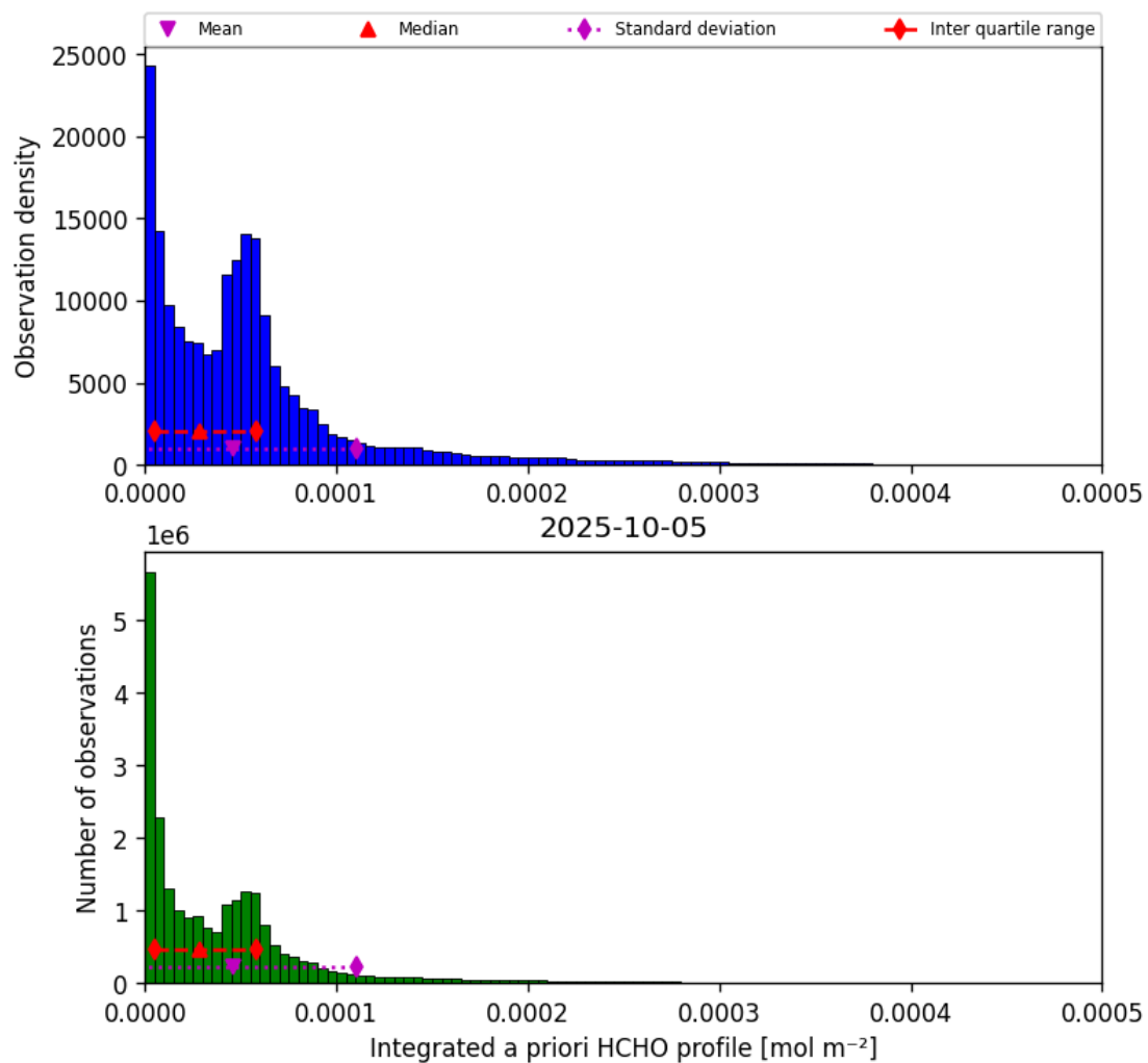
Figure 41: Histogram of “Integrated a priori HCHO profile” for 2025-10-05 to 2025-10-06
