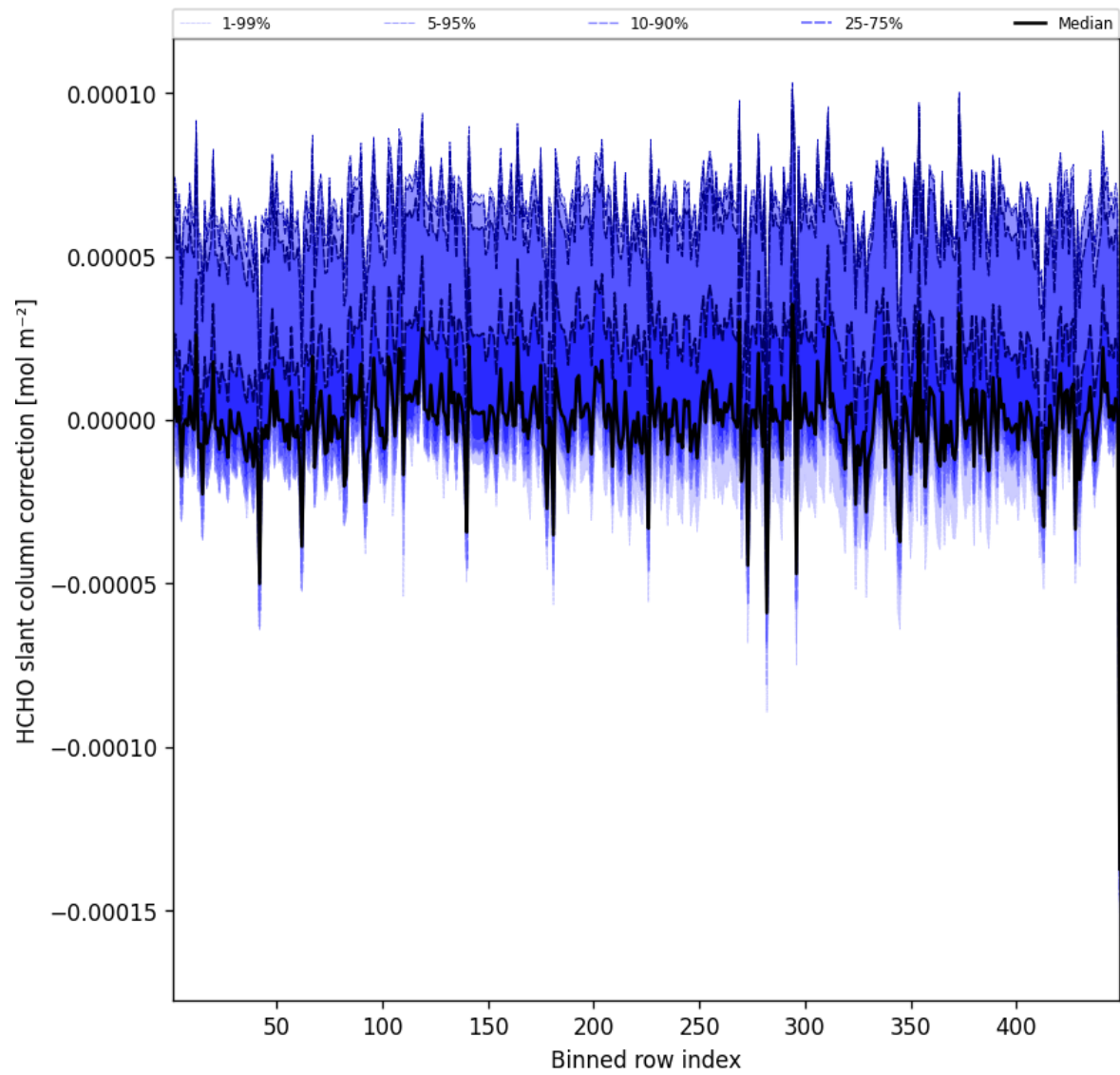
Figure 59: Along track statistics of “HCHO slant column correction” for 2025-10-05 to 2025-10-06
