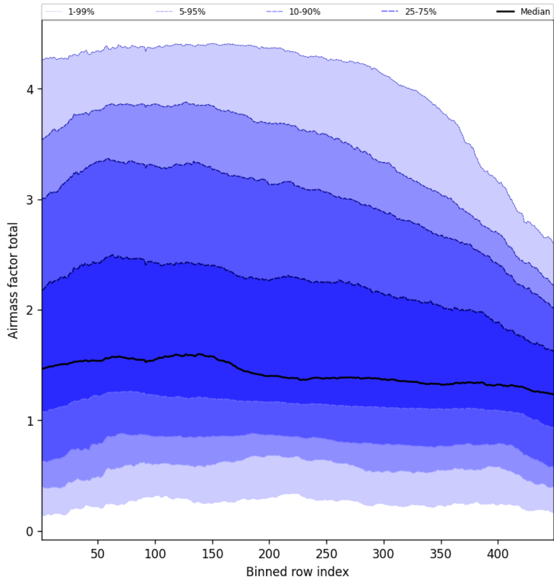
Figure 52: Along track statistics of “Airmass factor total” for 2025-10-05 to 2025-10-06
