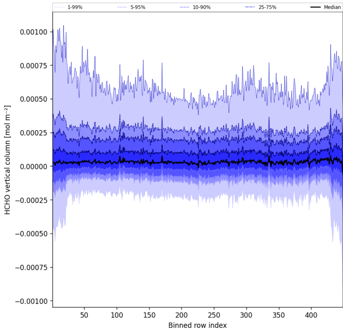
Figure 47: Along track statistics of “HCHO vertical column” for 2025-10-05 to 2025-10-06
