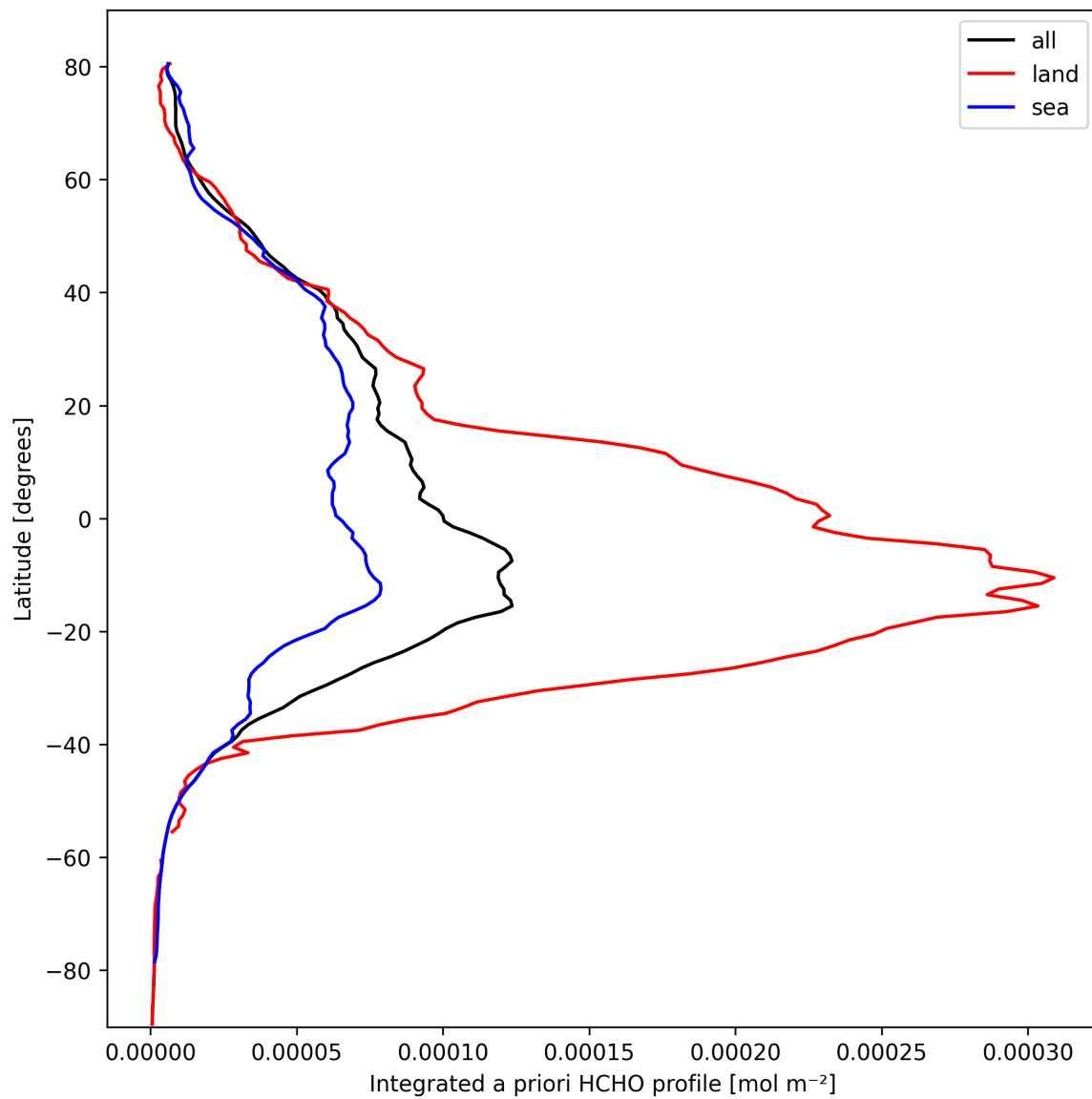
Figure 27: Zonal average of “Integrated a priori HCHO profile” for 2025-10-05 to 2025-10-06.
