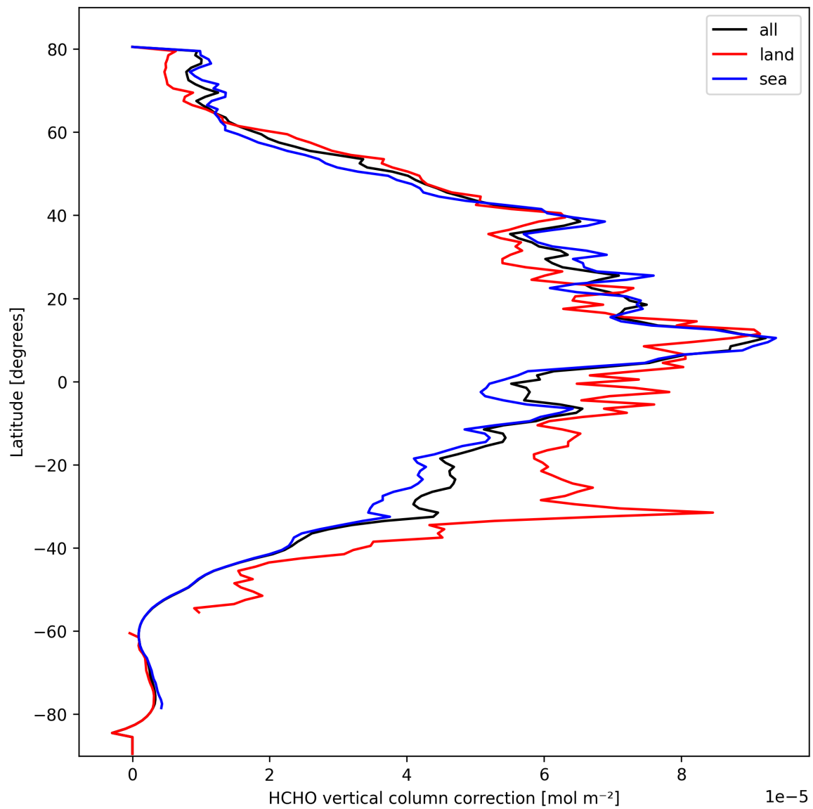
Figure 21: Zonal average of “HCHO vertical column correction” for 2025-10-05 to 2025-10-06.
