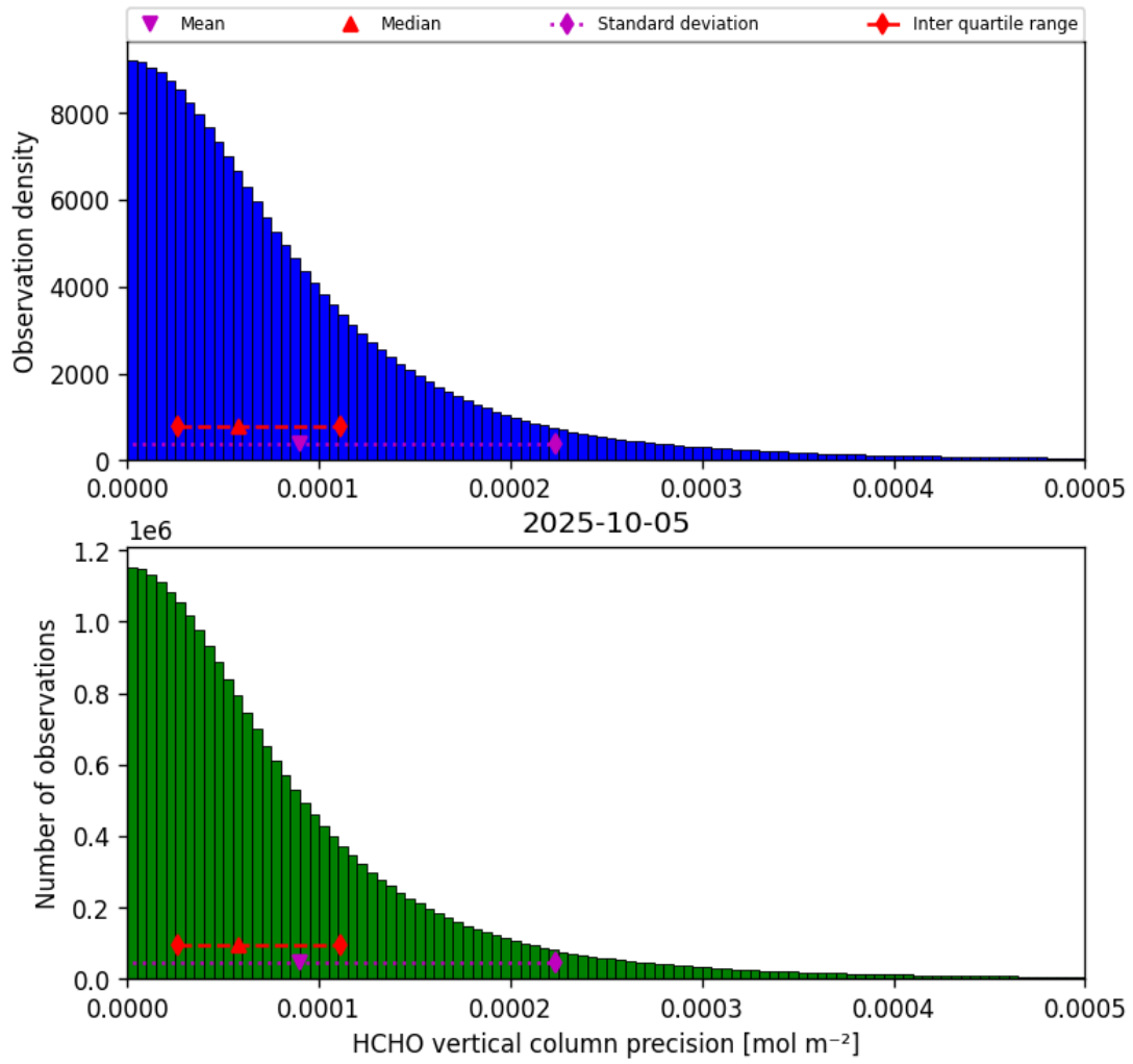
Figure 34: Histogram of “HCHO vertical column precision” for 2025-10-05 to 2025-10-06
