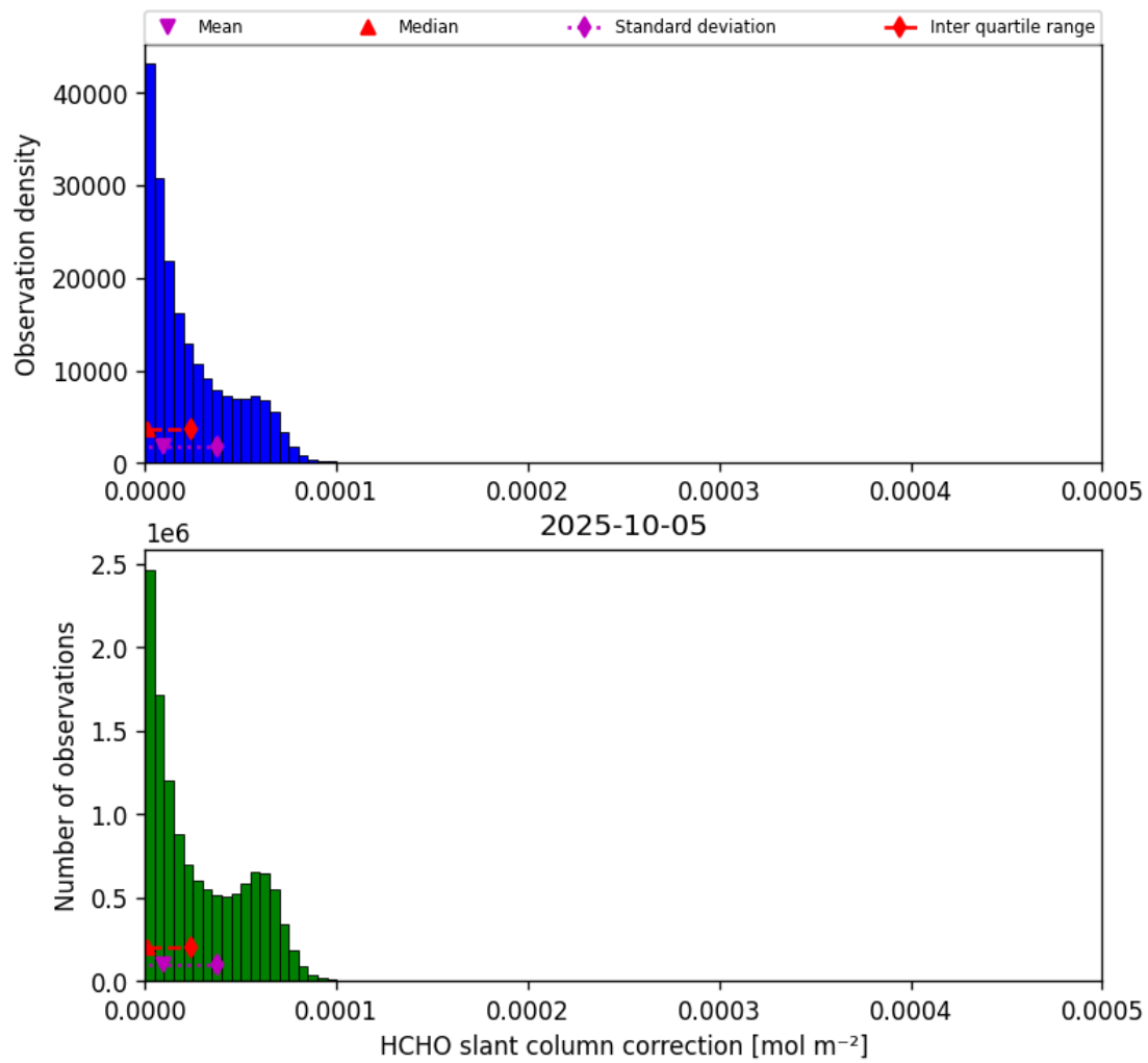
Figure 45: Histogram of “HCHO slant column correction” for 2025-10-05 to 2025-10-06
