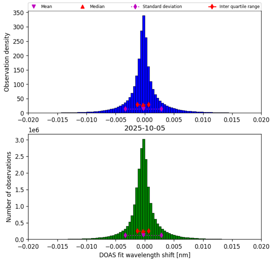
Figure 42: Histogram of “DOAS fit wavelength shift” for 2025-10-05 to 2025-10-06
