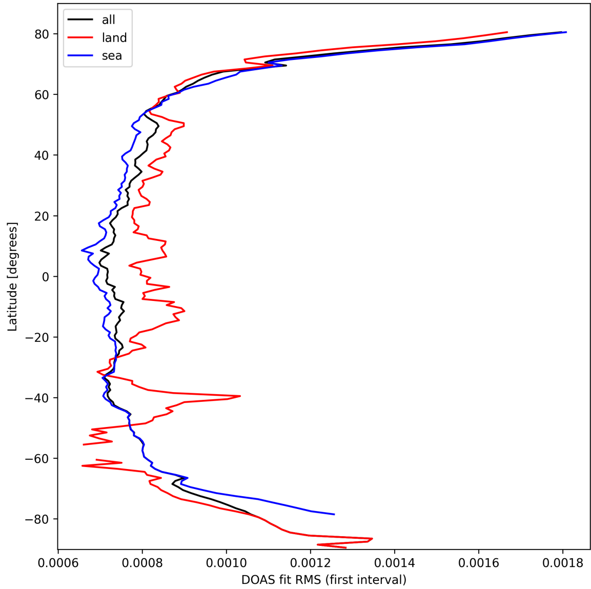
Figure 30: Zonal average of "DOAS fit RMS (first interval)" for 2025-10-05 to 2025-10-06.
