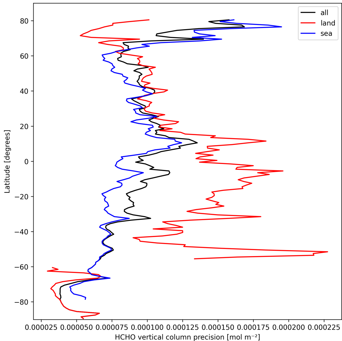
Figure 20: Zonal average of “HCHO vertical column precision” for 2025-10-05 to 2025-10-06.
