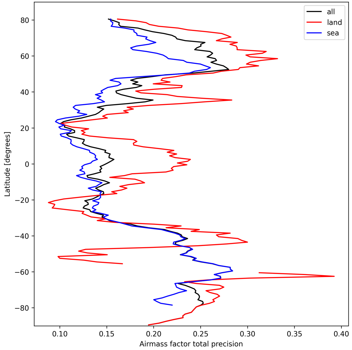
Figure 25: Zonal average of “Airmass factor total precision” for 2025-10-05 to 2025-10-06.
