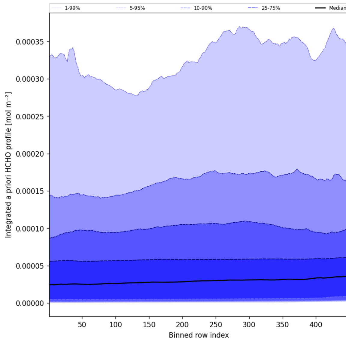
Figure 55: Along track statistics of “Integrated a priori HCHO profile” for 2025-10-05 to 2025-10-06
