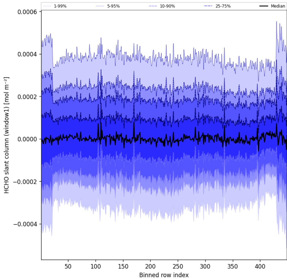
Figure 50: Along track statistics of “HCHO slant column (window1)” for 2025-10-05 to 2025-10-06
