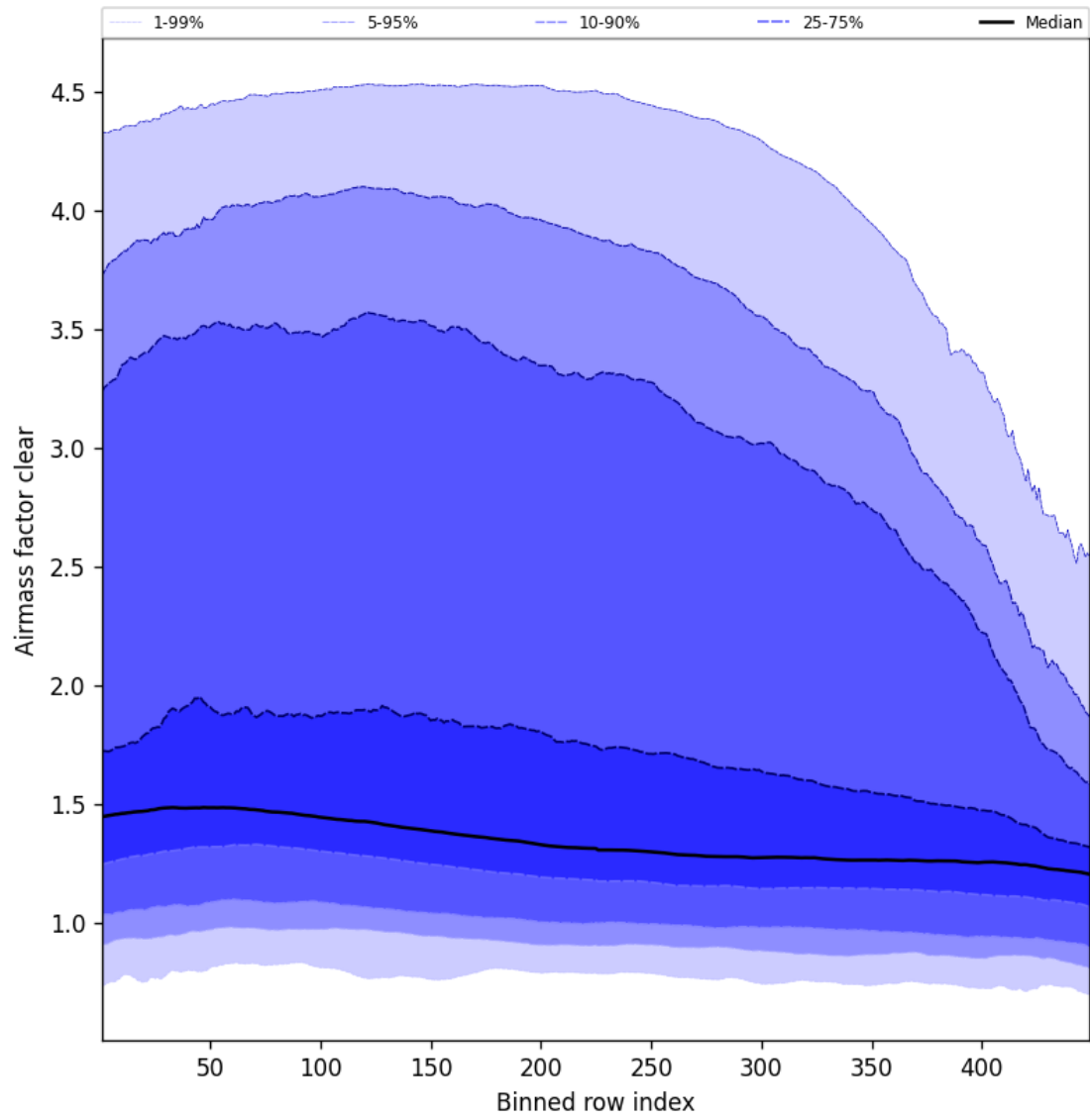
Figure 54: Along track statistics of “Airmass factor clear” for 2025-10-05 to 2025-10-06
