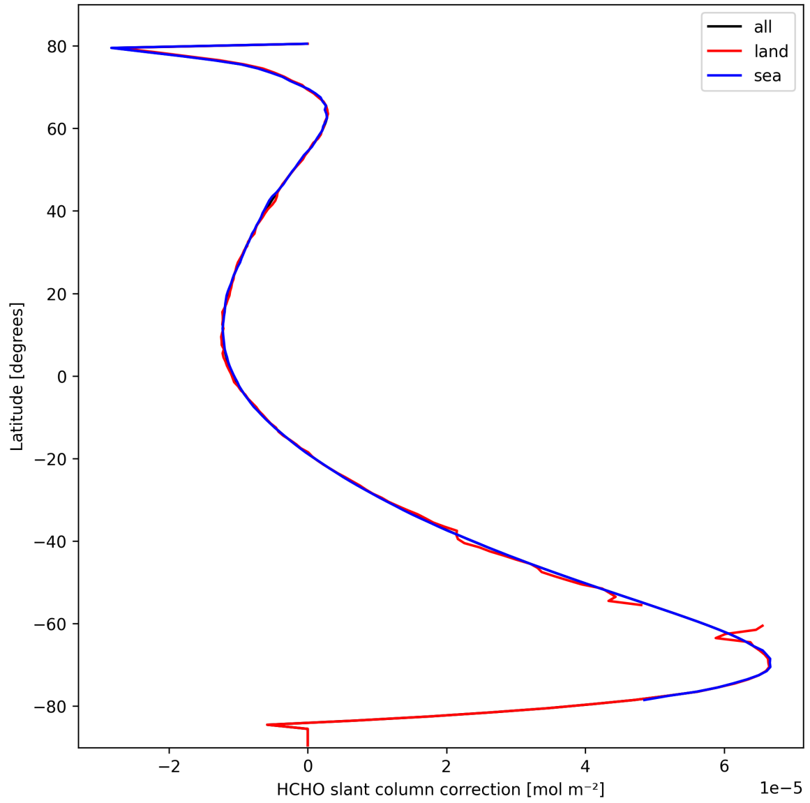
Figure 31: Zonal average of "HCHO slant column correction" for 2025-10-05 to 2025-10-06.
