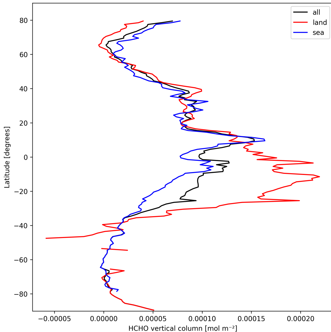
Figure 19: Zonal average of “HCHO vertical column” for 2025-10-07 to 2025-10-07.
