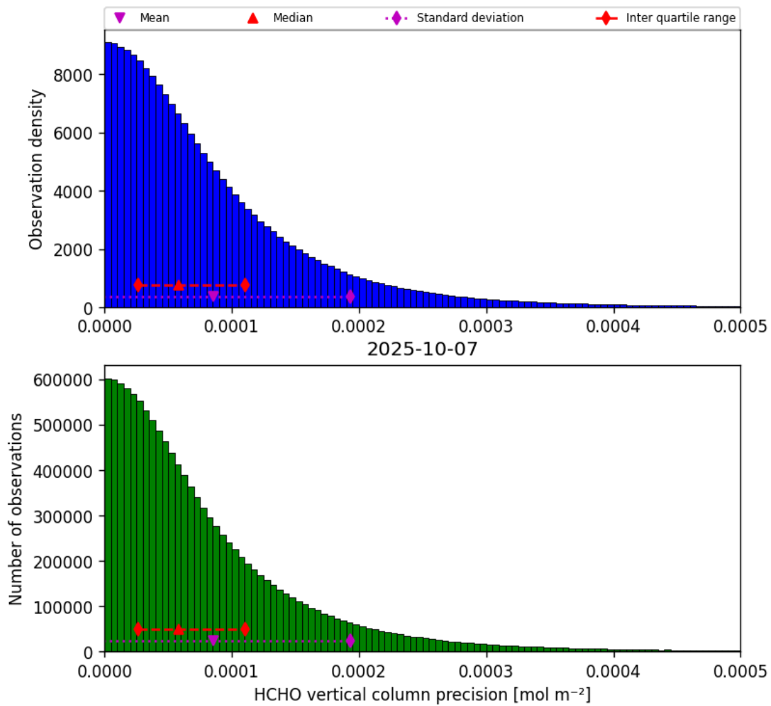
Figure 34: Histogram of “HCHO vertical column precision” for 2025-10-07 to 2025-10-07
