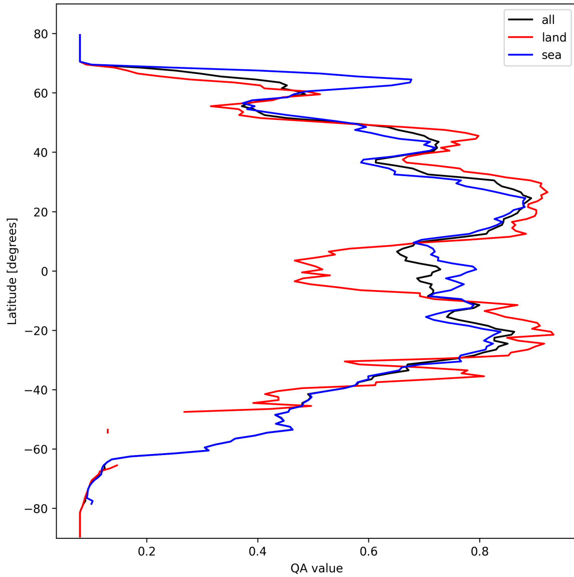
Figure 18: Zonal average of “QA value” for 2025-10-07 to 2025-10-07.
