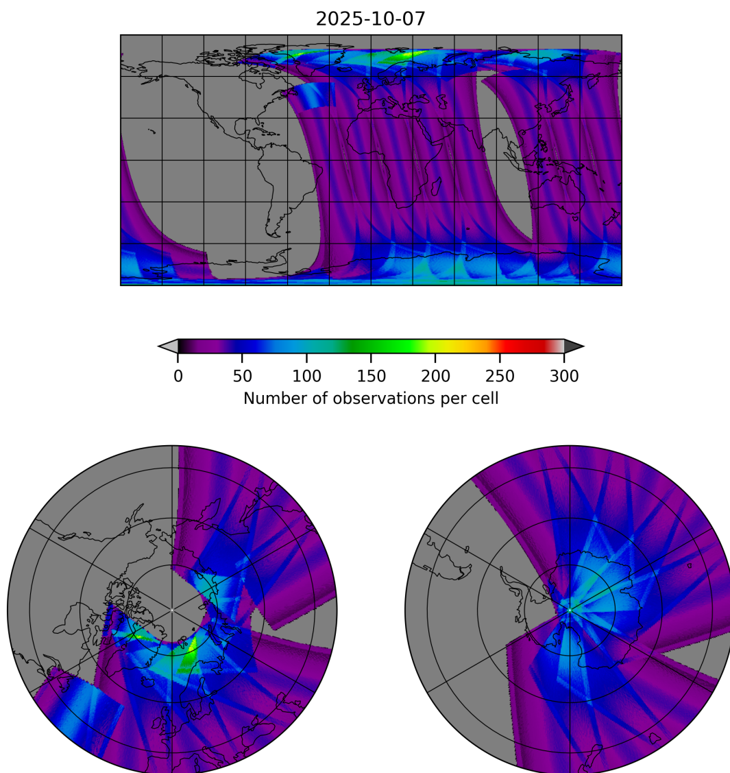
Figure 17: Map of the number of observations for 2025-10-07 to 2025-10-07
