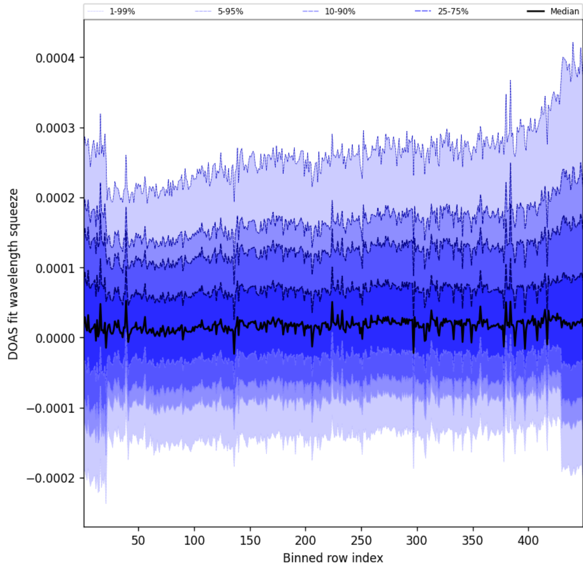
Figure 57: Along track statistics of “DOAS fit wavelength squeeze” for 2025-10-07 to 2025-10-07
