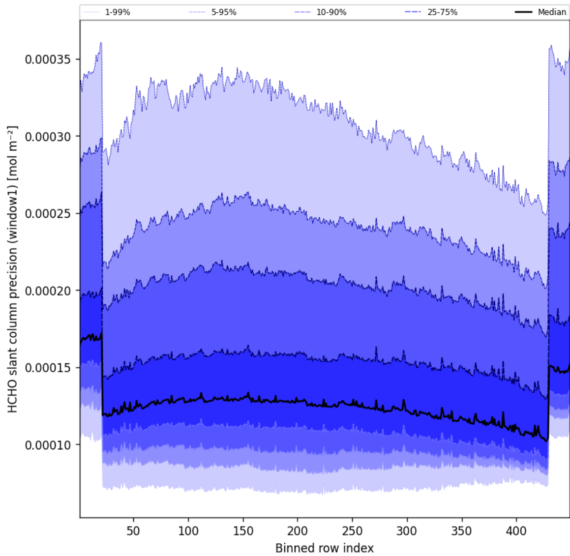
Figure 51: Along track statistics of “HCHO slant column precision (window1)” for 2025-10-07 to 2025-10-07
