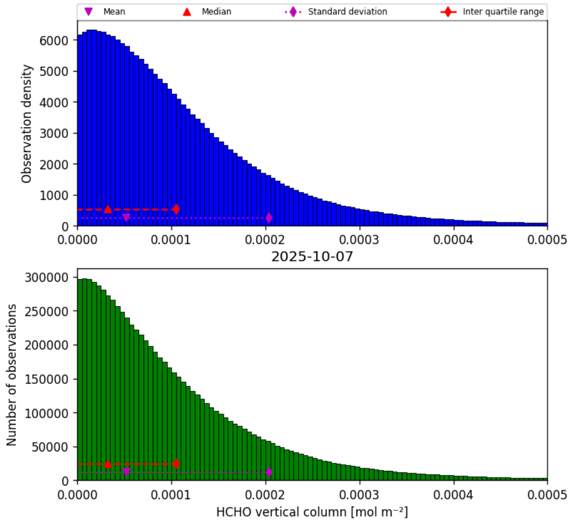
Figure 33: Histogram of “HCHO vertical column” for 2025-10-07 to 2025-10-07
