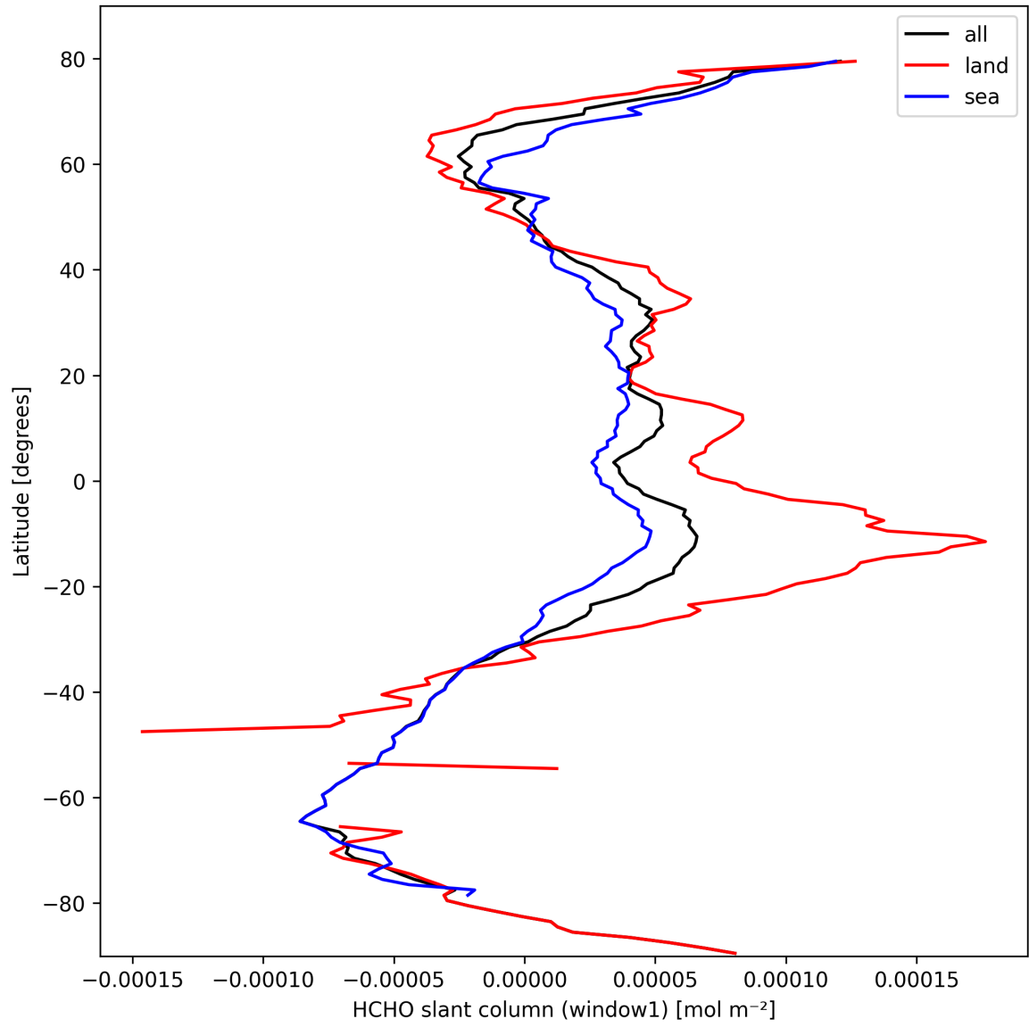
Figure 22: Zonal average of “HCHO slant column (window1)” for 2025-10-07 to 2025-10-07.
