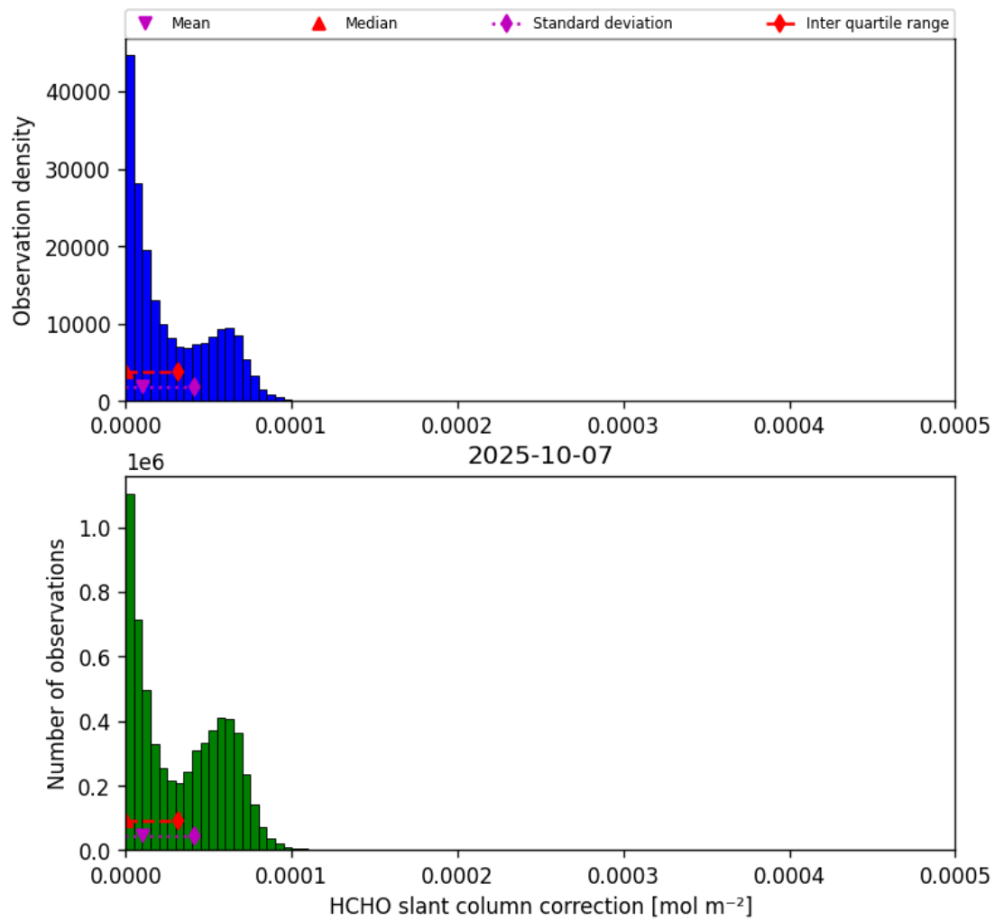
Figure 45: Histogram of “HCHO slant column correction” for 2025-10-07 to 2025-10-07
