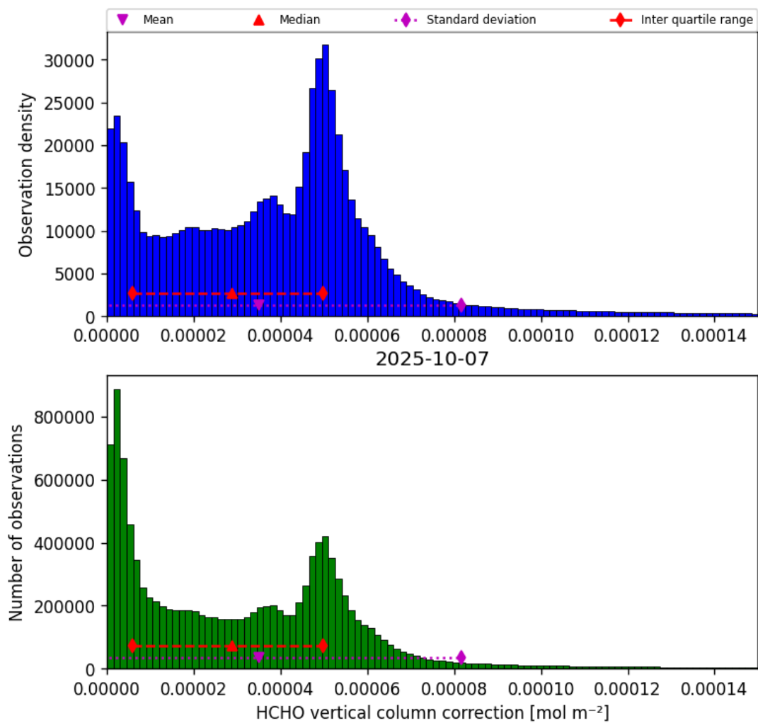
Figure 35: Histogram of “HCHO vertical column correction” for 2025-10-07 to 2025-10-07
