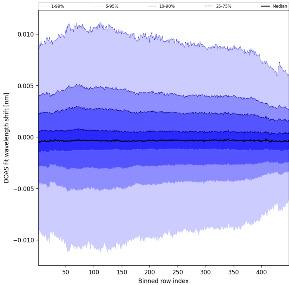
Figure 56: Along track statistics of “DOAS fit wavelength shift” for 2025-10-07 to 2025-10-07
