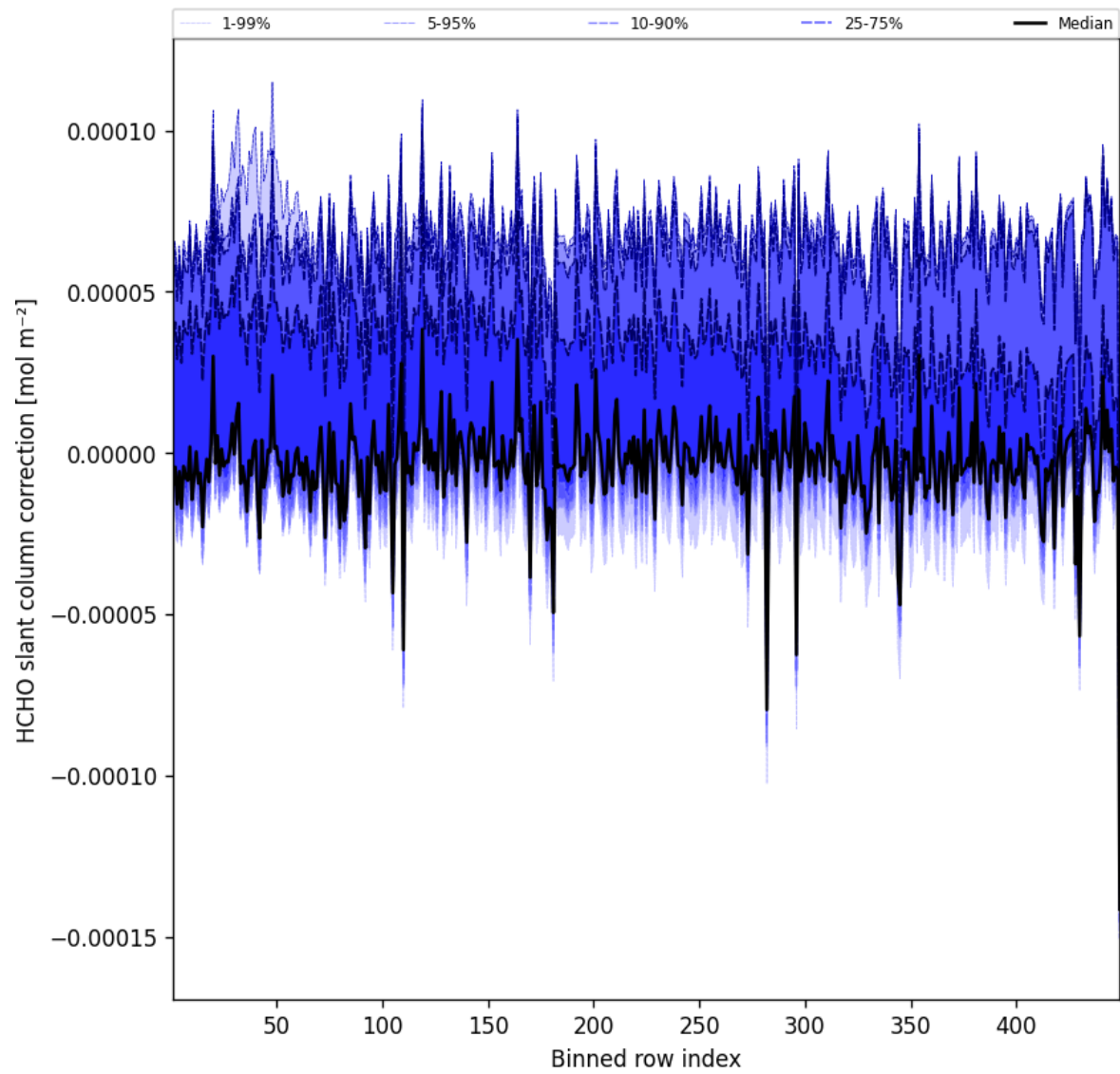
Figure 59: Along track statistics of "HCHO slant column correction" for 2025-10-07 to 2025-10-07
