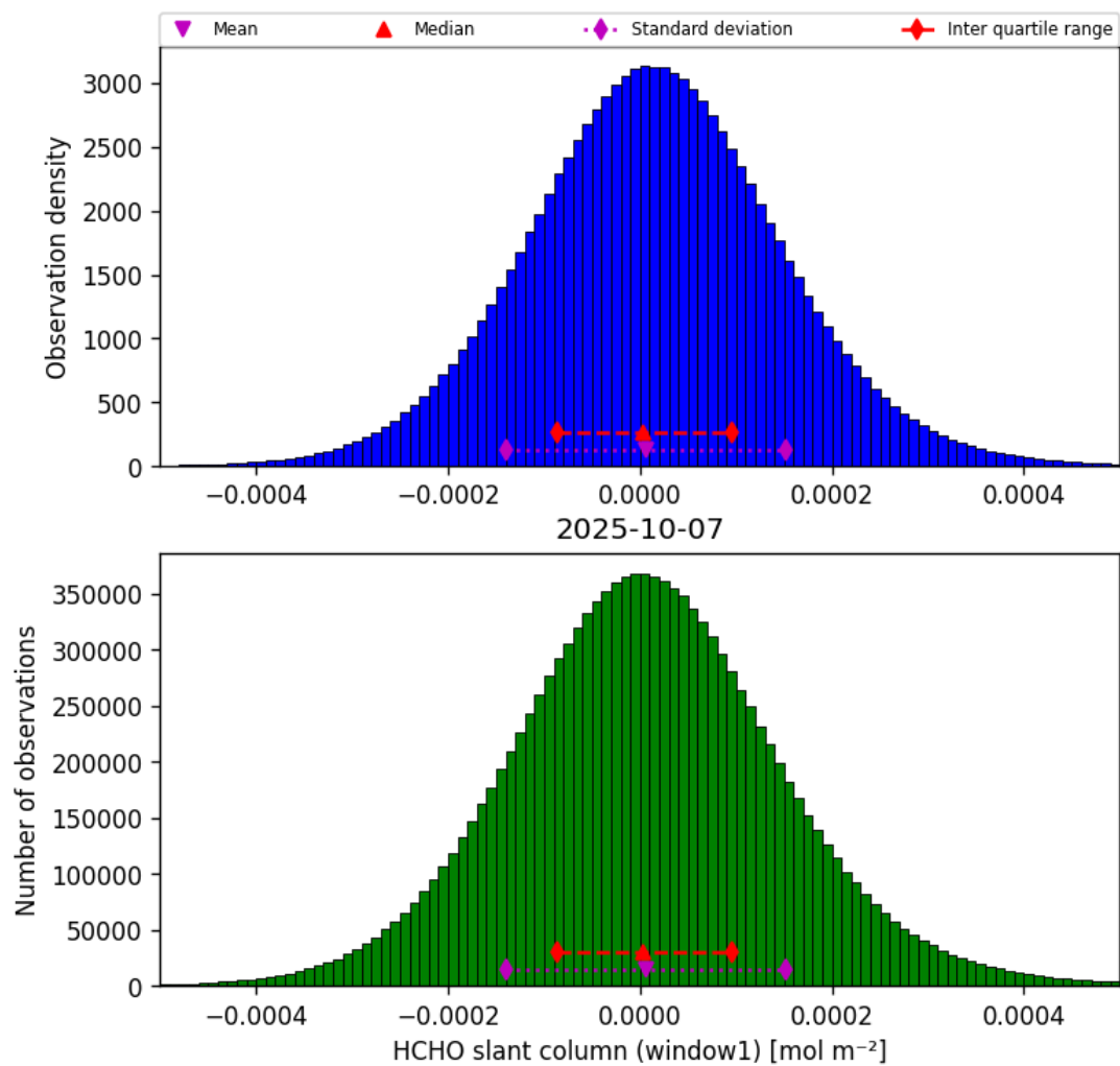
Figure 36: Histogram of “HCHO slant column (window1)” for 2025-10-07 to 2025-10-07
