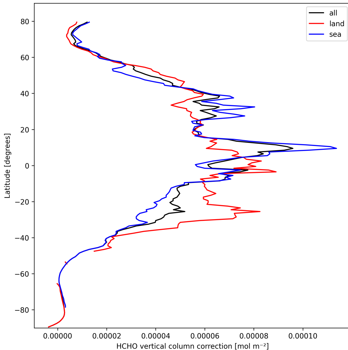
Figure 21: Zonal average of “HCHO vertical column correction” for 2025-10-07 to 2025-10-07.
