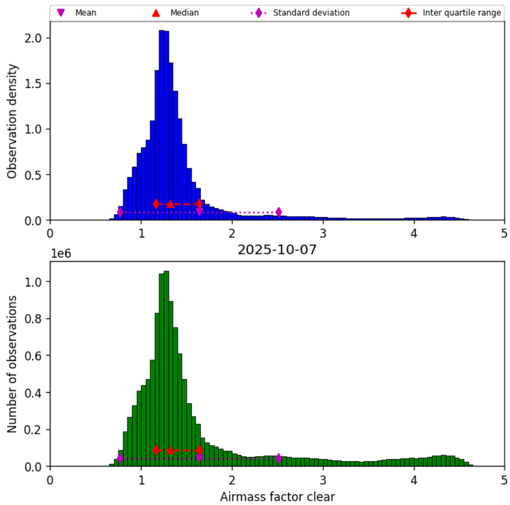
Figure 40: Histogram of “Airmass factor clear” for 2025-10-07 to 2025-10-07
