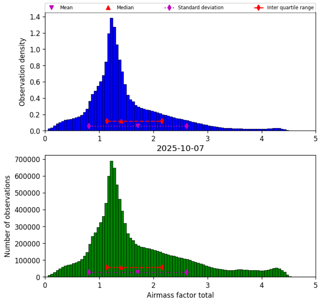
Figure 38: Histogram of “Airmass factor total” for 2025-10-07 to 2025-10-07
