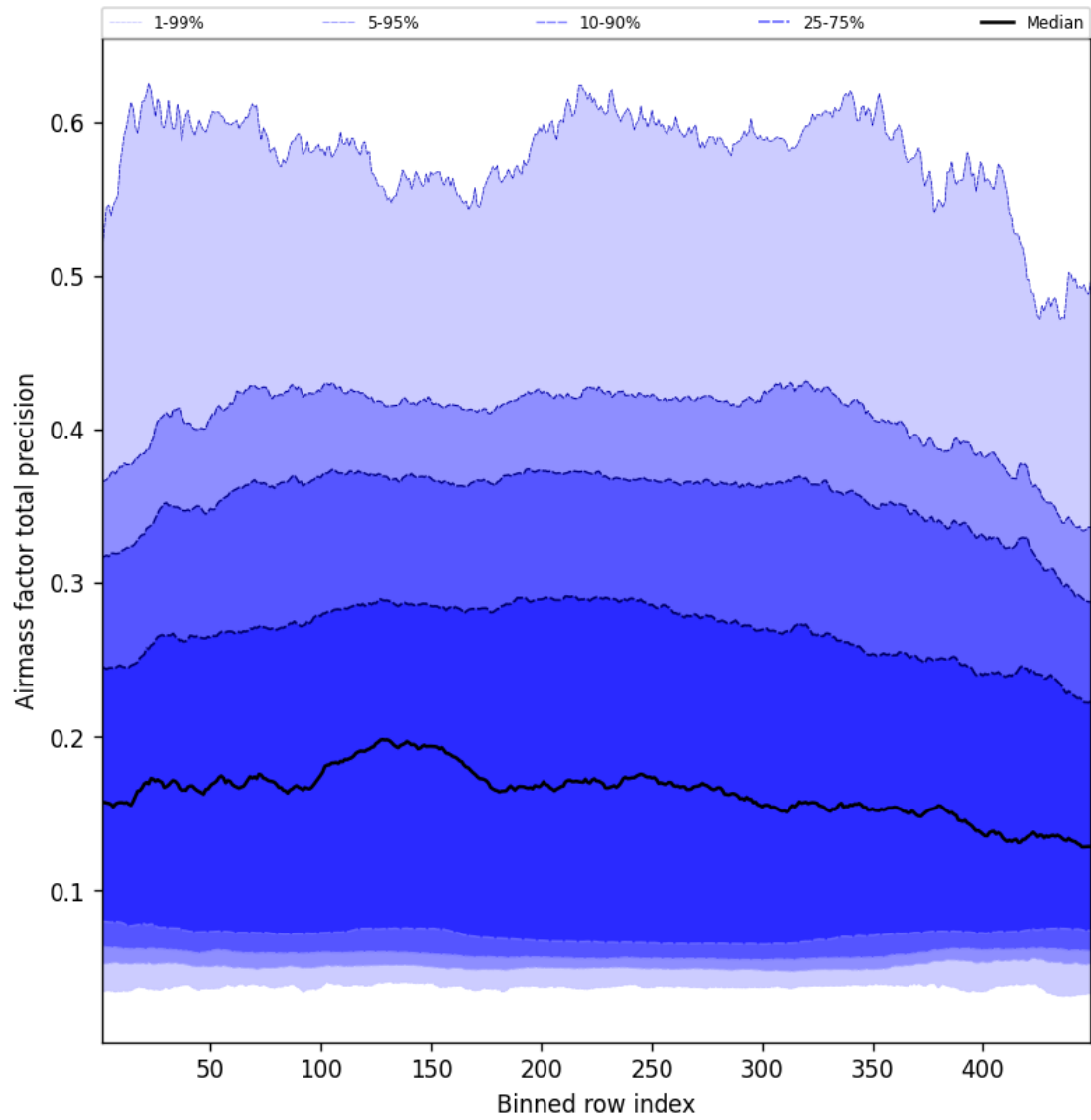
Figure 53: Along track statistics of “Airmass factor total precision” for 2025-10-07 to 2025-10-07
