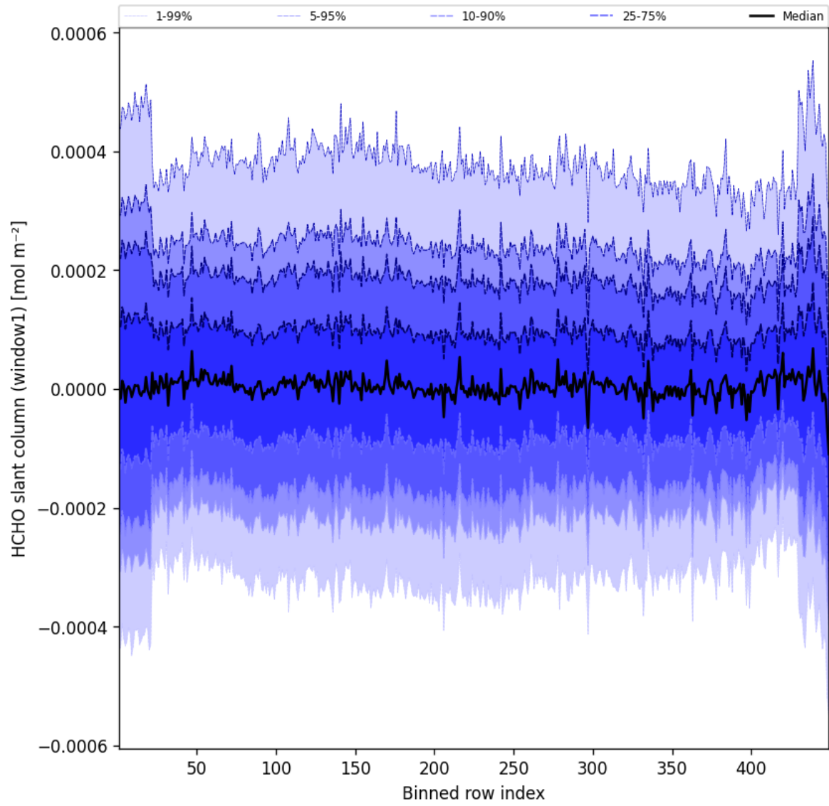
Figure 50: Along track statistics of “HCHO slant column (window1)” for 2025-10-07 to 2025-10-07
