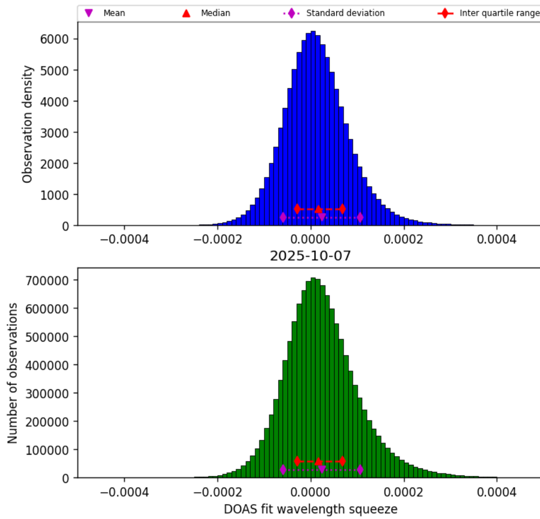
Figure 43: Histogram of “DOAS fit wavelength squeeze” for 2025-10-07 to 2025-10-07
