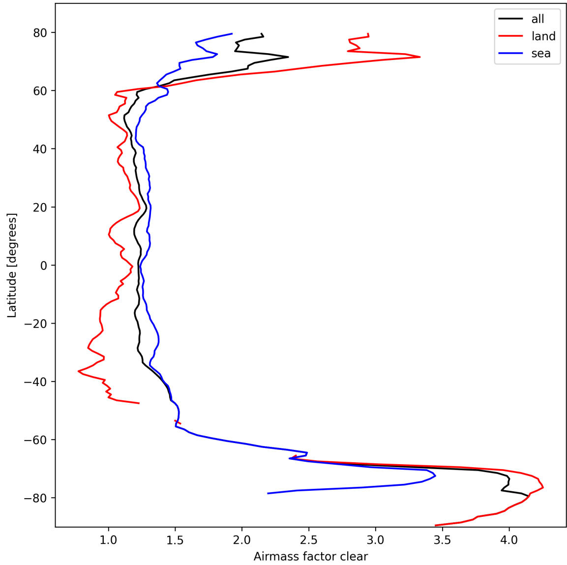
Figure 26: Zonal average of “Airmass factor clear” for 2025-10-07 to 2025-10-07.
