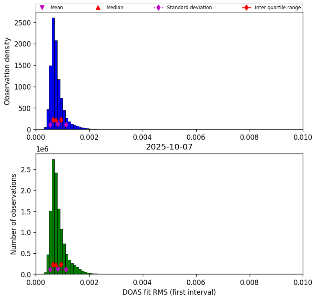
Figure 44: Histogram of “DOAS fit RMS (first interval)” for 2025-10-07 to 2025-10-07
