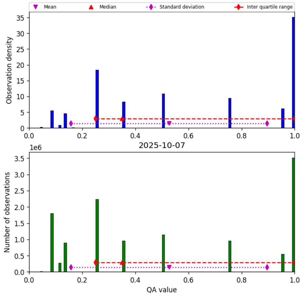
Figure 32: Histogram of “QA value” for 2025-10-07 to 2025-10-07
