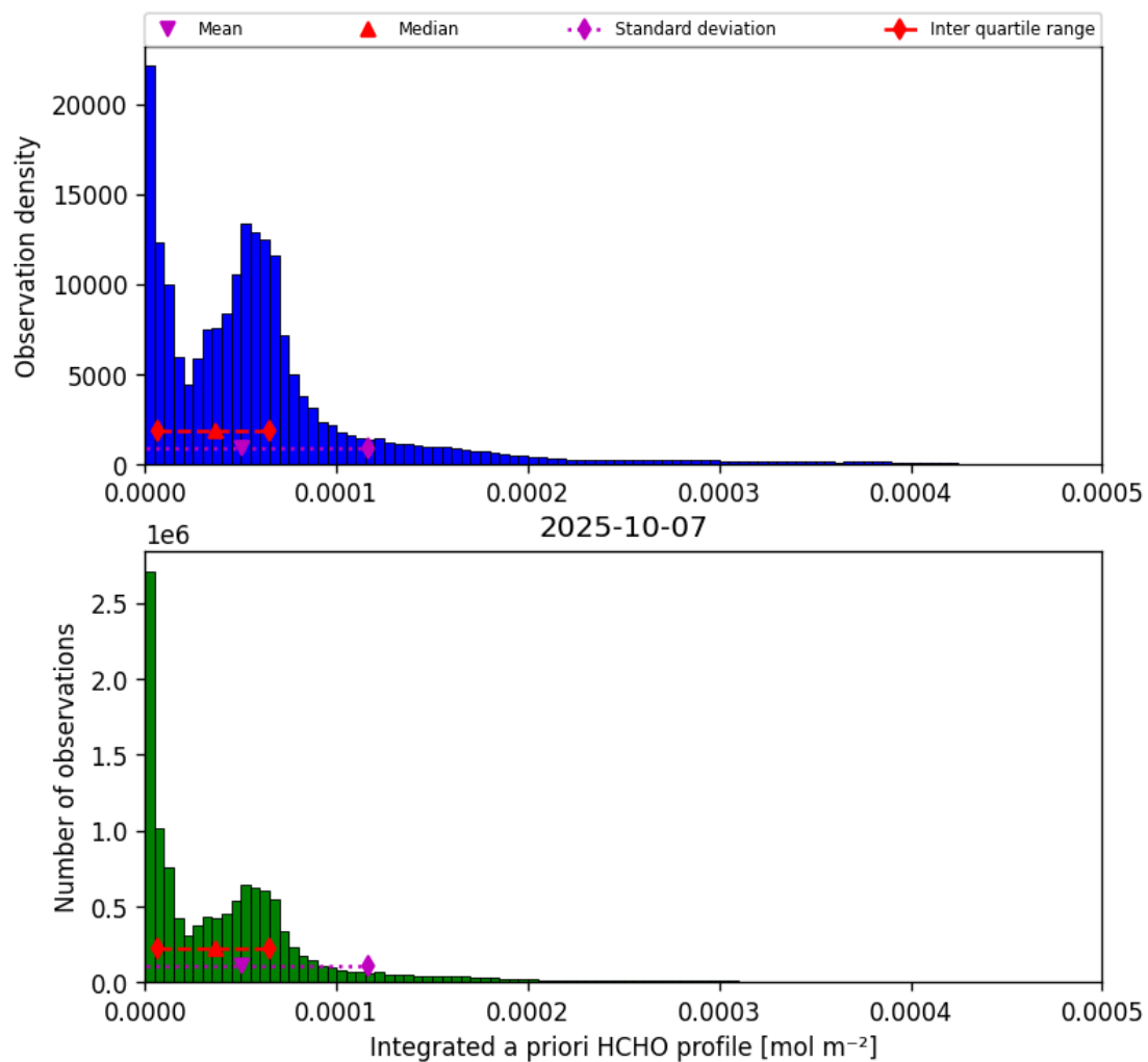
Figure 41: Histogram of “Integrated a priori HCHO profile” for 2025-10-07 to 2025-10-07
