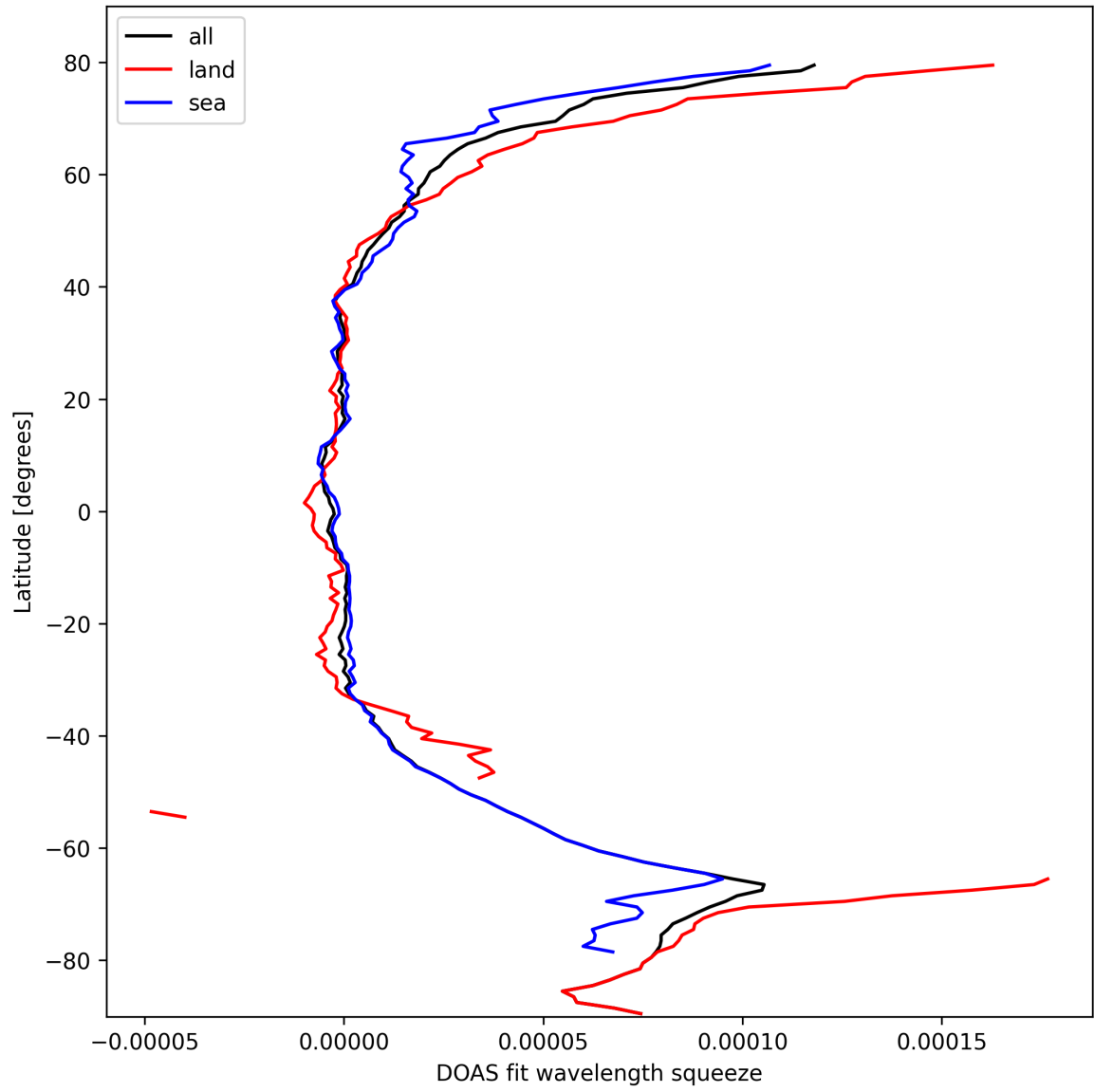
Figure 29: Zonal average of “DOAS fit wavelength squeeze” for 2025-10-07 to 2025-10-07.
