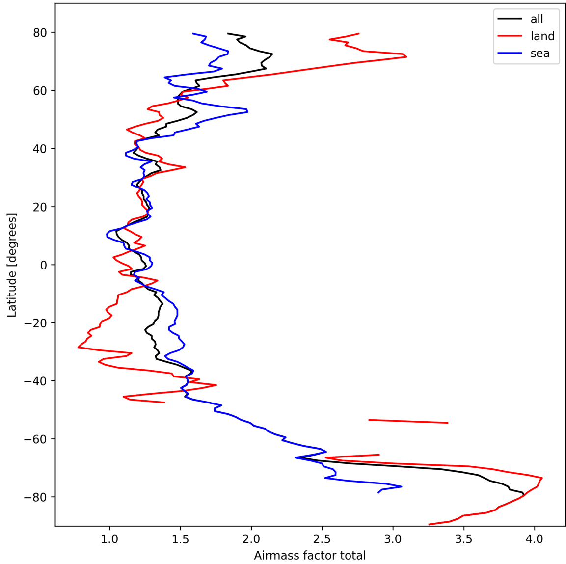
Figure 24: Zonal average of “Airmass factor total” for 2025-10-07 to 2025-10-07.
