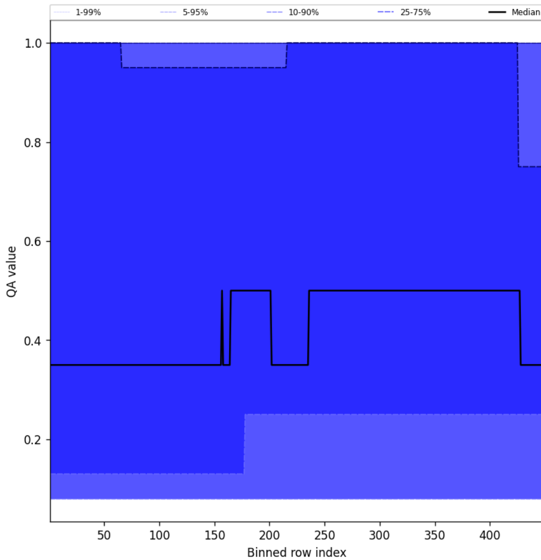
Figure 46: Along track statistics of “QA value” for 2025-10-07 to 2025-10-07
