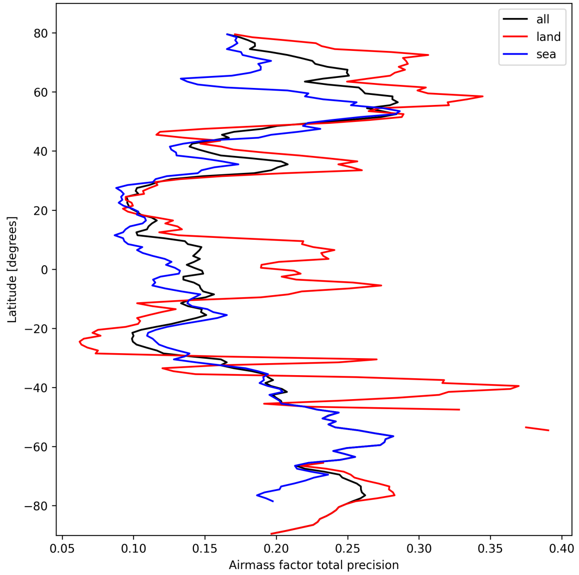
Figure 25: Zonal average of “Airmass factor total precision” for 2025-10-07 to 2025-10-07.
