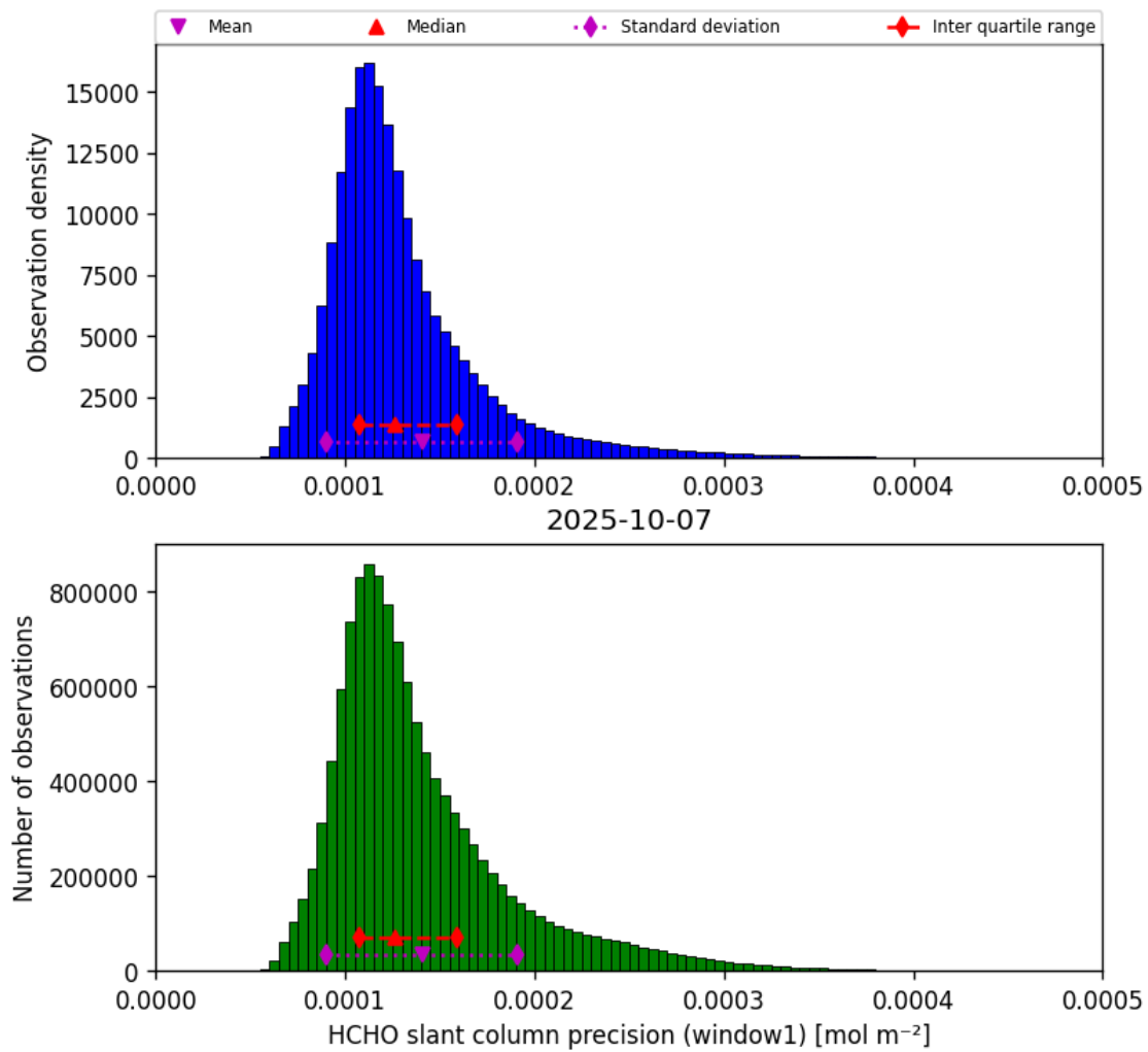
Figure 37: Histogram of “HCHO slant column precision (window1)” for 2025-10-07 to 2025-10-07
