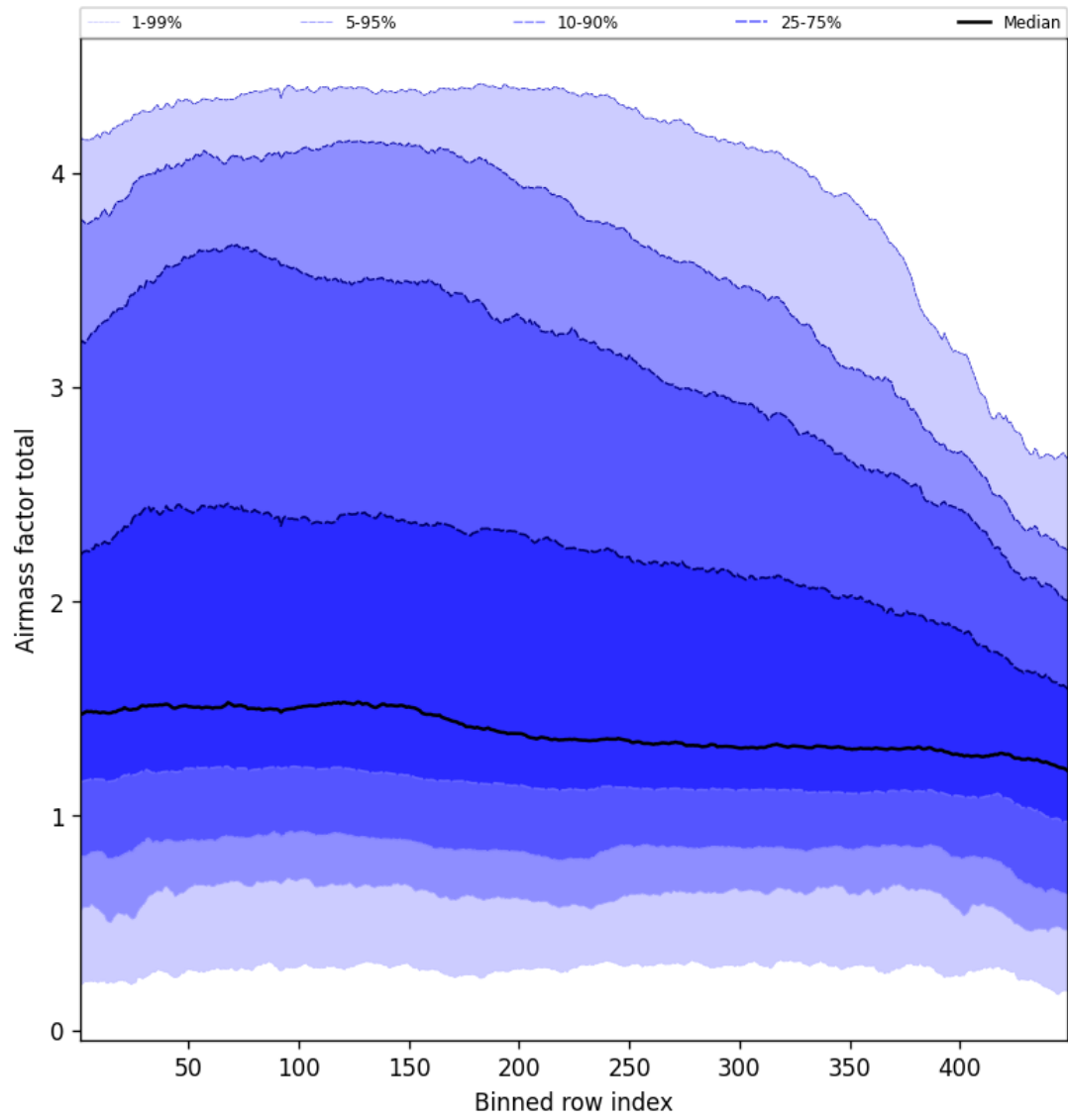
Figure 52: Along track statistics of “Airmass factor total” for 2025-10-07 to 2025-10-07
