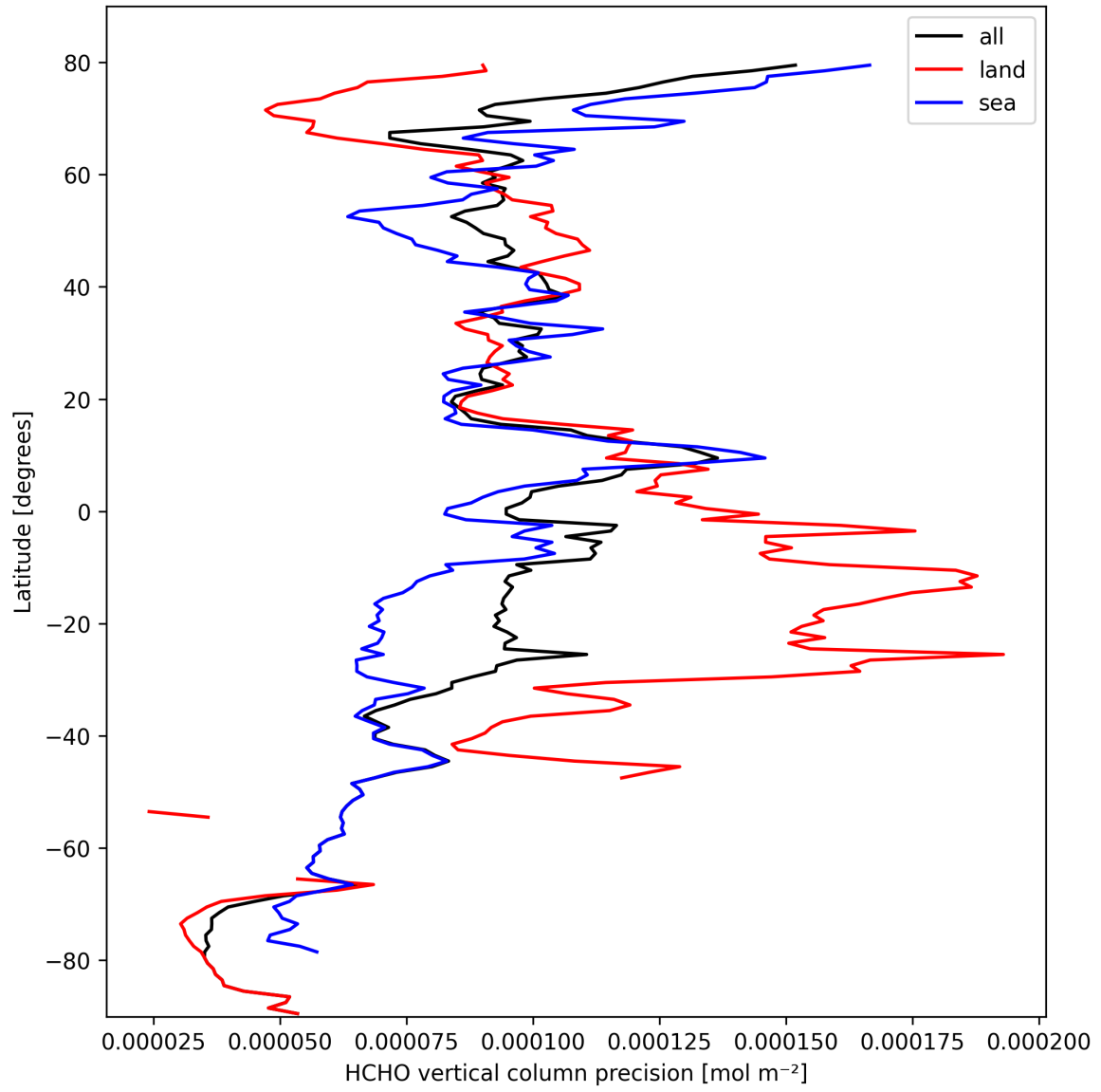
Figure 20: Zonal average of “HCHO vertical column precision” for 2025-10-07 to 2025-10-07.
