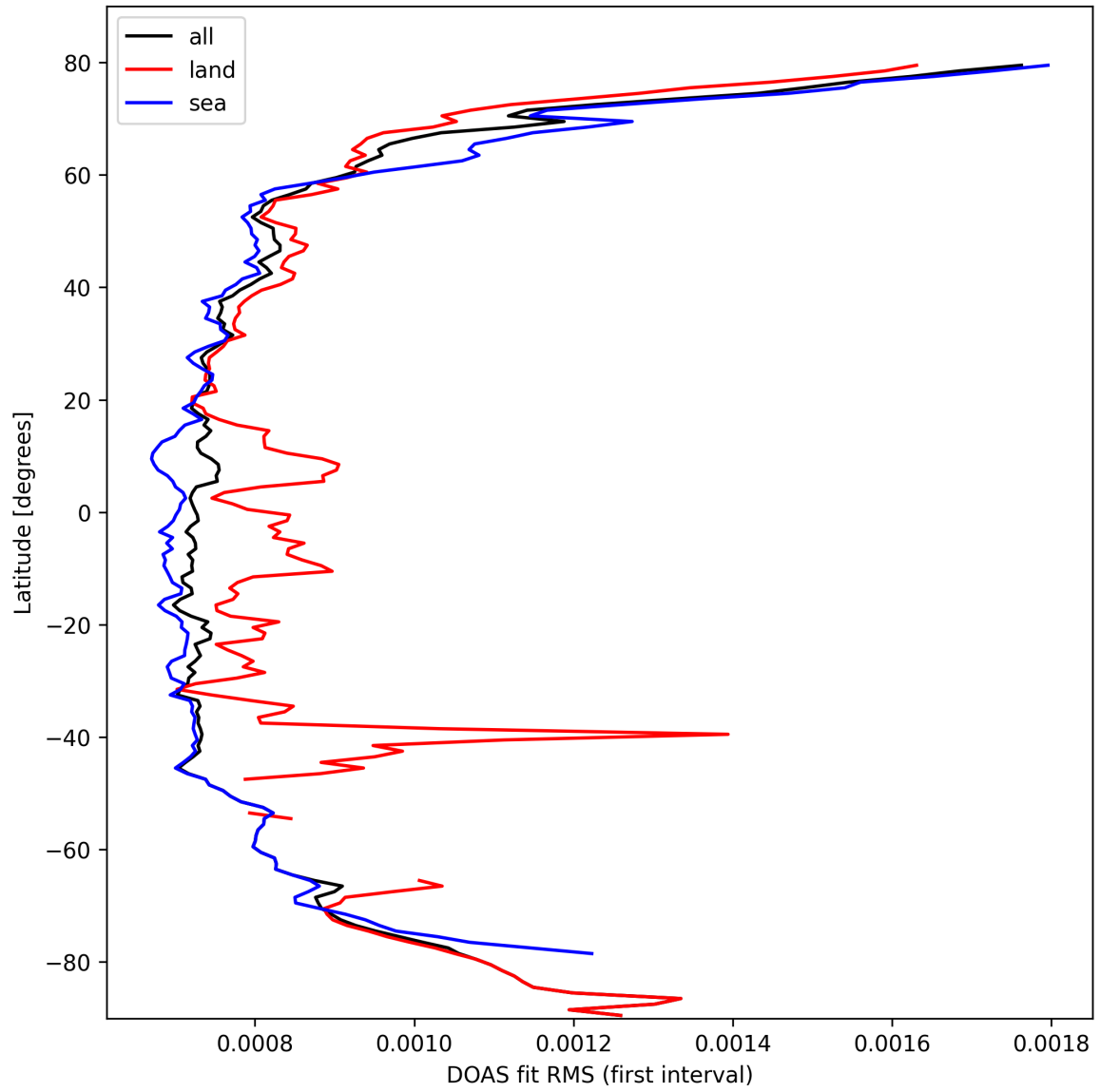
Figure 30: Zonal average of “DOAS fit RMS (first interval)” for 2025-10-07 to 2025-10-07.
