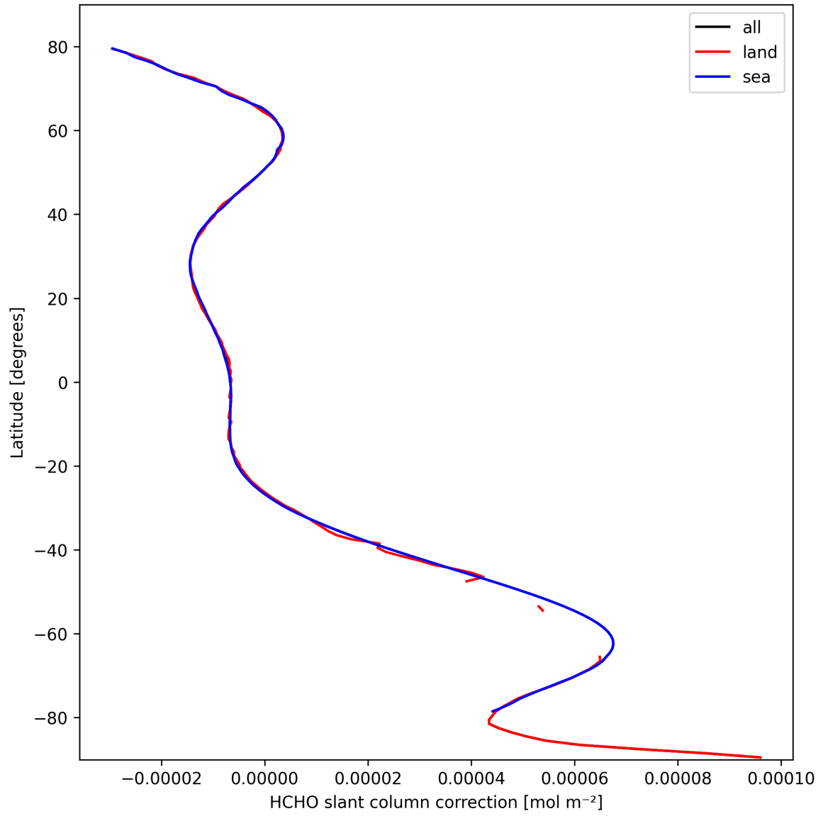
Figure 31: Zonal average of “HCHO slant column correction” for 2025-10-07 to 2025-10-07.
