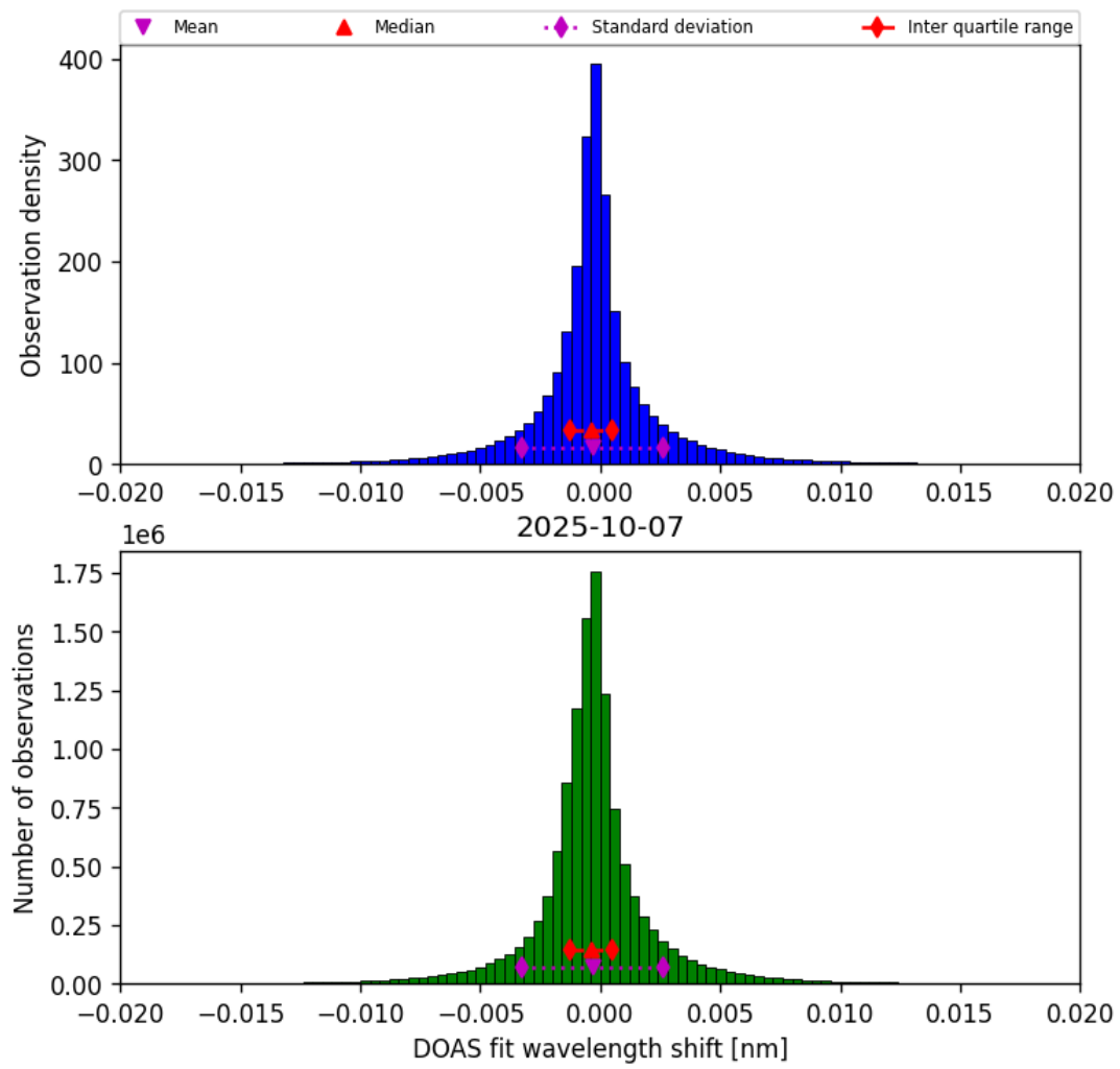
Figure 42: Histogram of “DOAS fit wavelength shift” for 2025-10-07 to 2025-10-07
