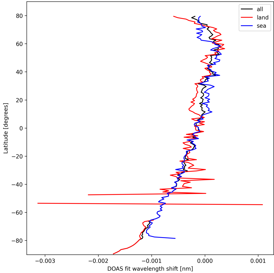
Figure 28: Zonal average of "DOAS fit wavelength shift" for 2025-10-07 to 2025-10-07.
