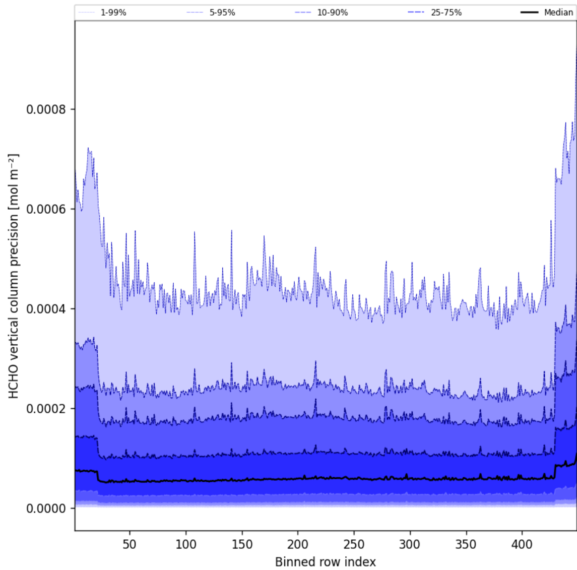
Figure 48: Along track statistics of “HCHO vertical column precision” for 2025-10-07 to 2025-10-07
