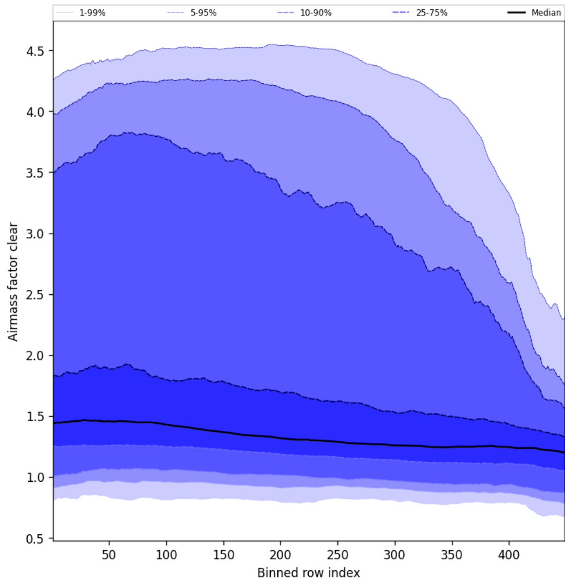
Figure 54: Along track statistics of “Airmass factor clear” for 2025-10-07 to 2025-10-07
