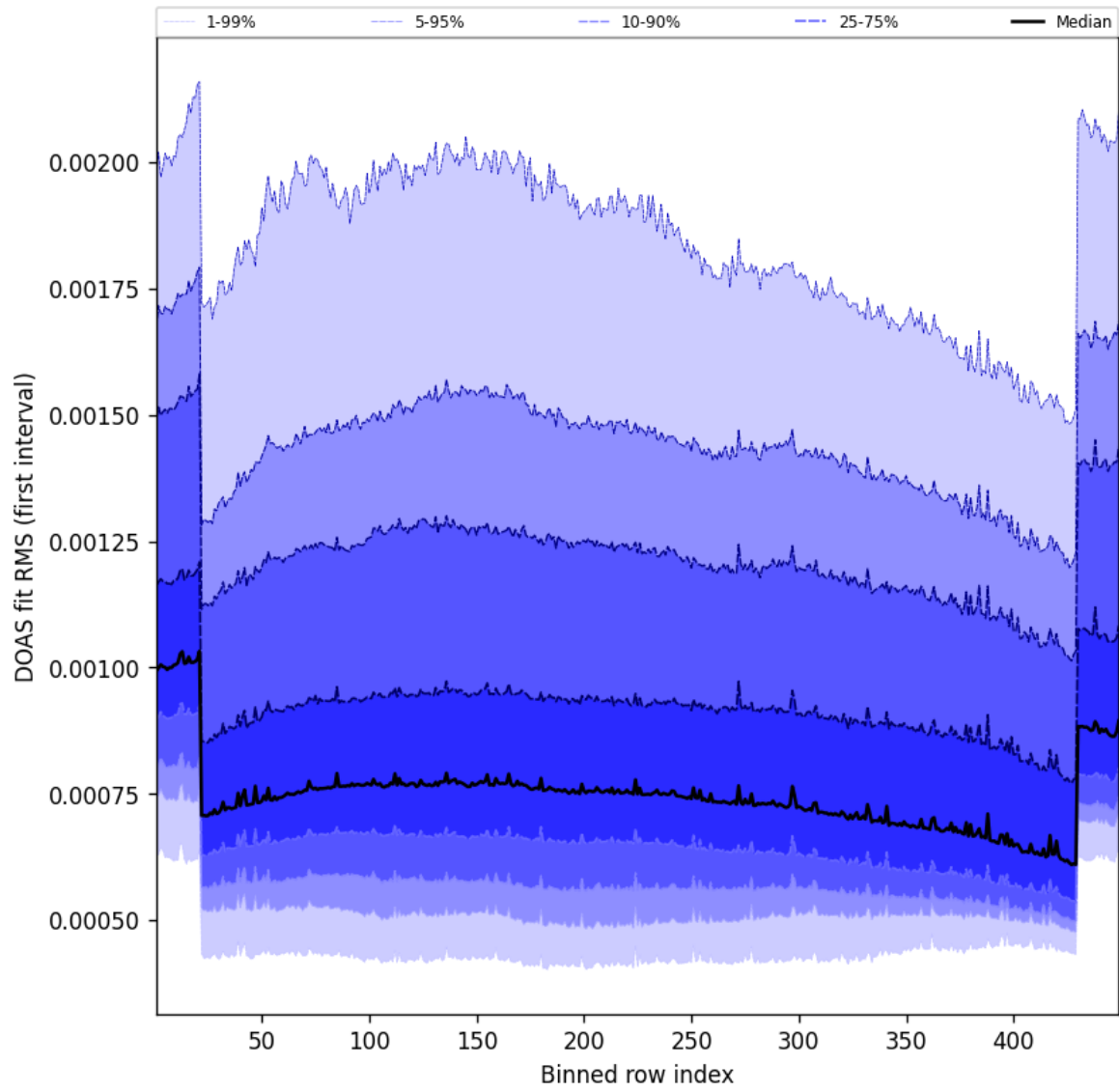
Figure 58: Along track statistics of “DOAS fit RMS (first interval)” for 2025-10-07 to 2025-10-07
