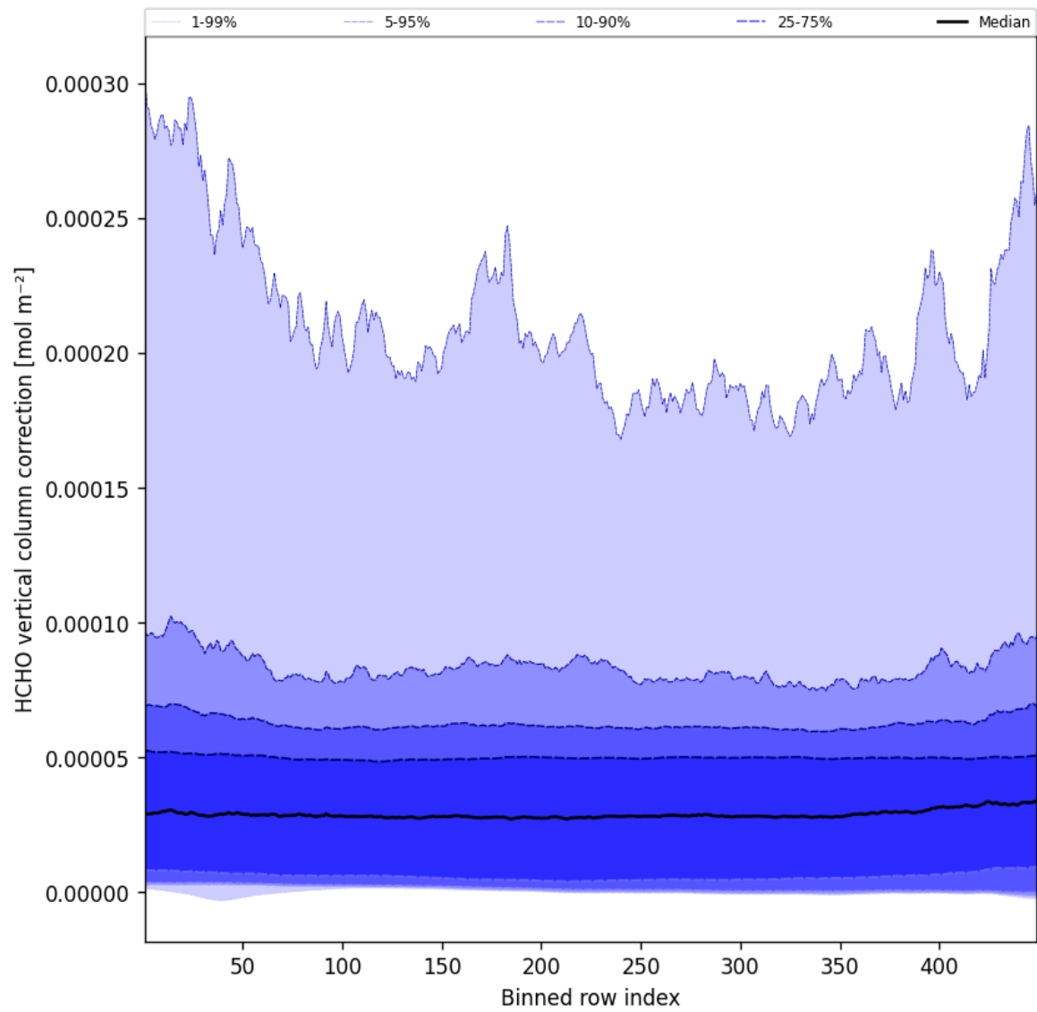
Figure 49: Along track statistics of “HCHO vertical column correction” for 2025-10-07 to 2025-10-07
