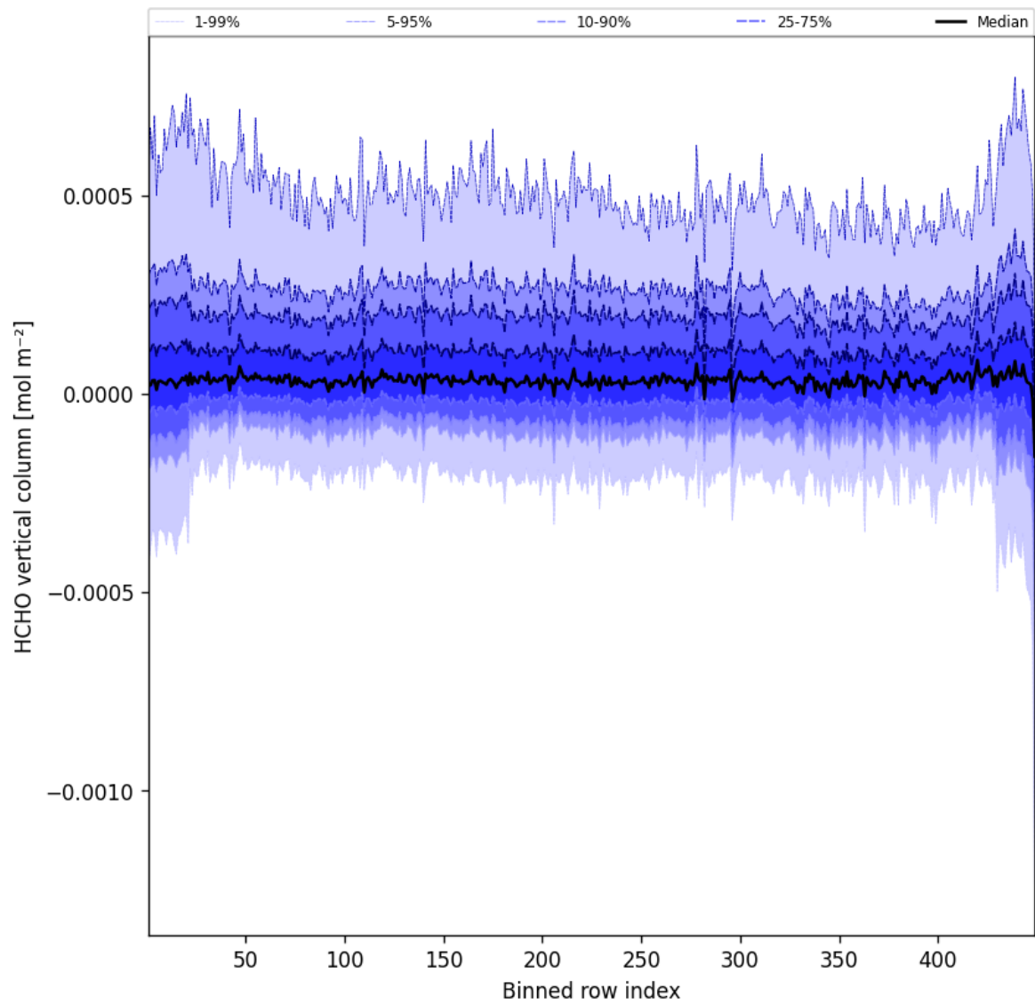
Figure 47: Along track statistics of “HCHO vertical column” for 2025-10-07 to 2025-10-07
