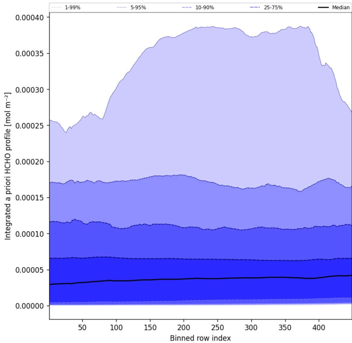
Figure 55: Along track statistics of "Integrated a priori HCHO profile" for 2025-10-07 to 2025-10-07
