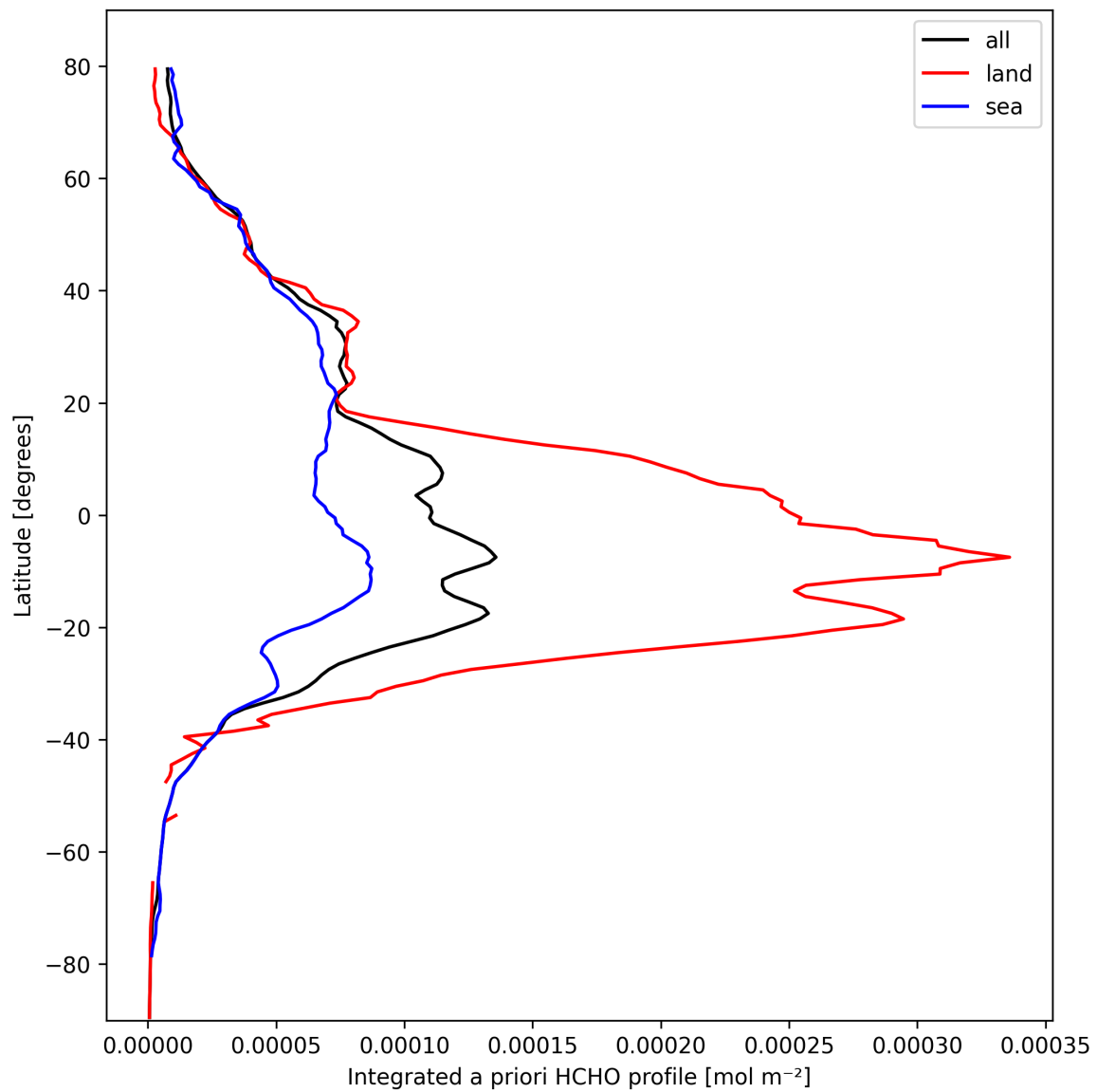
Figure 27: Zonal average of “Integrated a priori HCHO profile” for 2025-10-07 to 2025-10-07.
