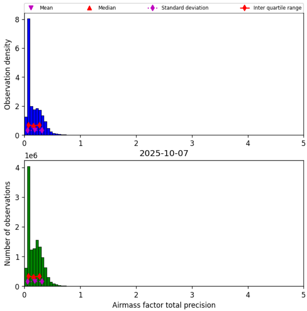
Figure 39: Histogram of “Airmass factor total precision” for 2025-10-07 to 2025-10-07
