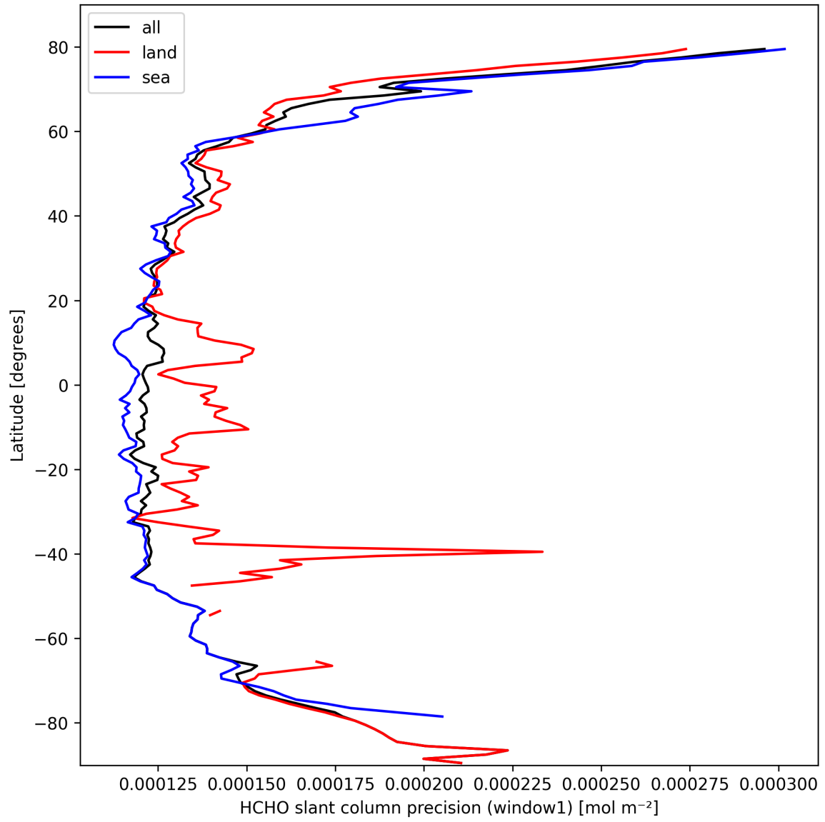
Figure 23: Zonal average of “HCHO slant column precision (window1)” for 2025-10-07 to 2025-10-07.
