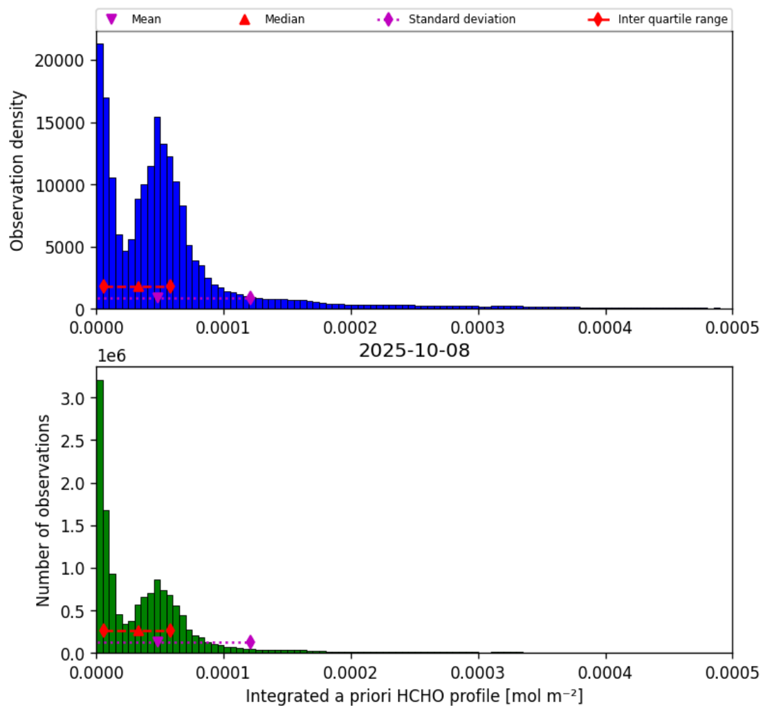
Figure 41: Histogram of “Integrated a priori HCHO profile” for 2025-10-08 to 2025-10-09
