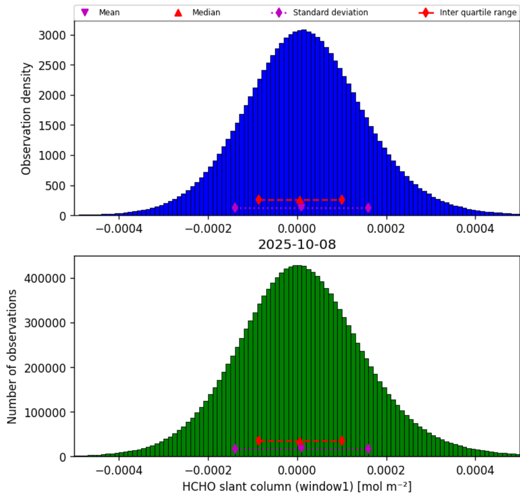
Figure 36: Histogram of “HCHO slant column (window1)” for 2025-10-08 to 2025-10-09
