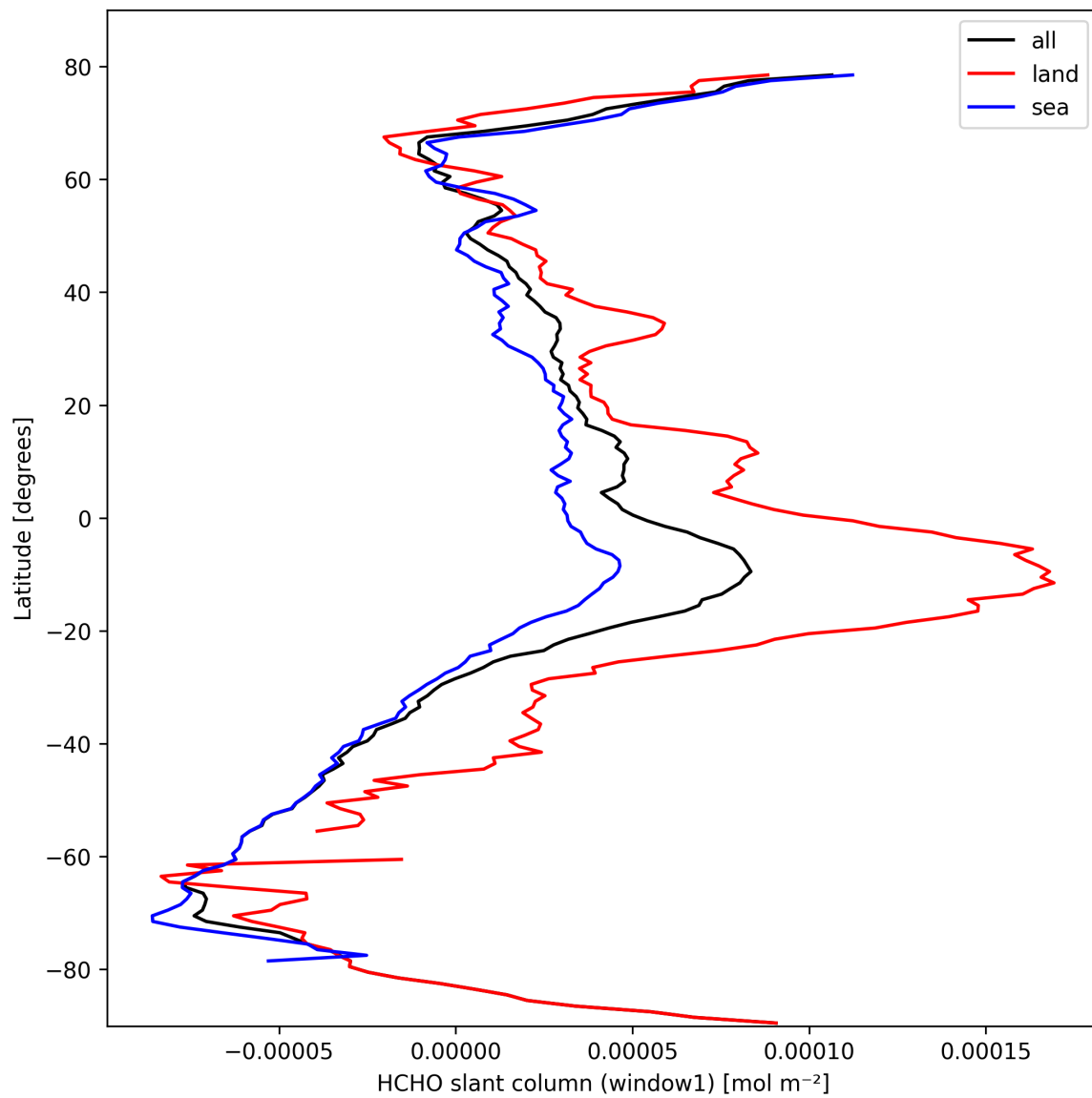
Figure 22: Zonal average of “HCHO slant column (window1)” for 2025-10-08 to 2025-10-09.
