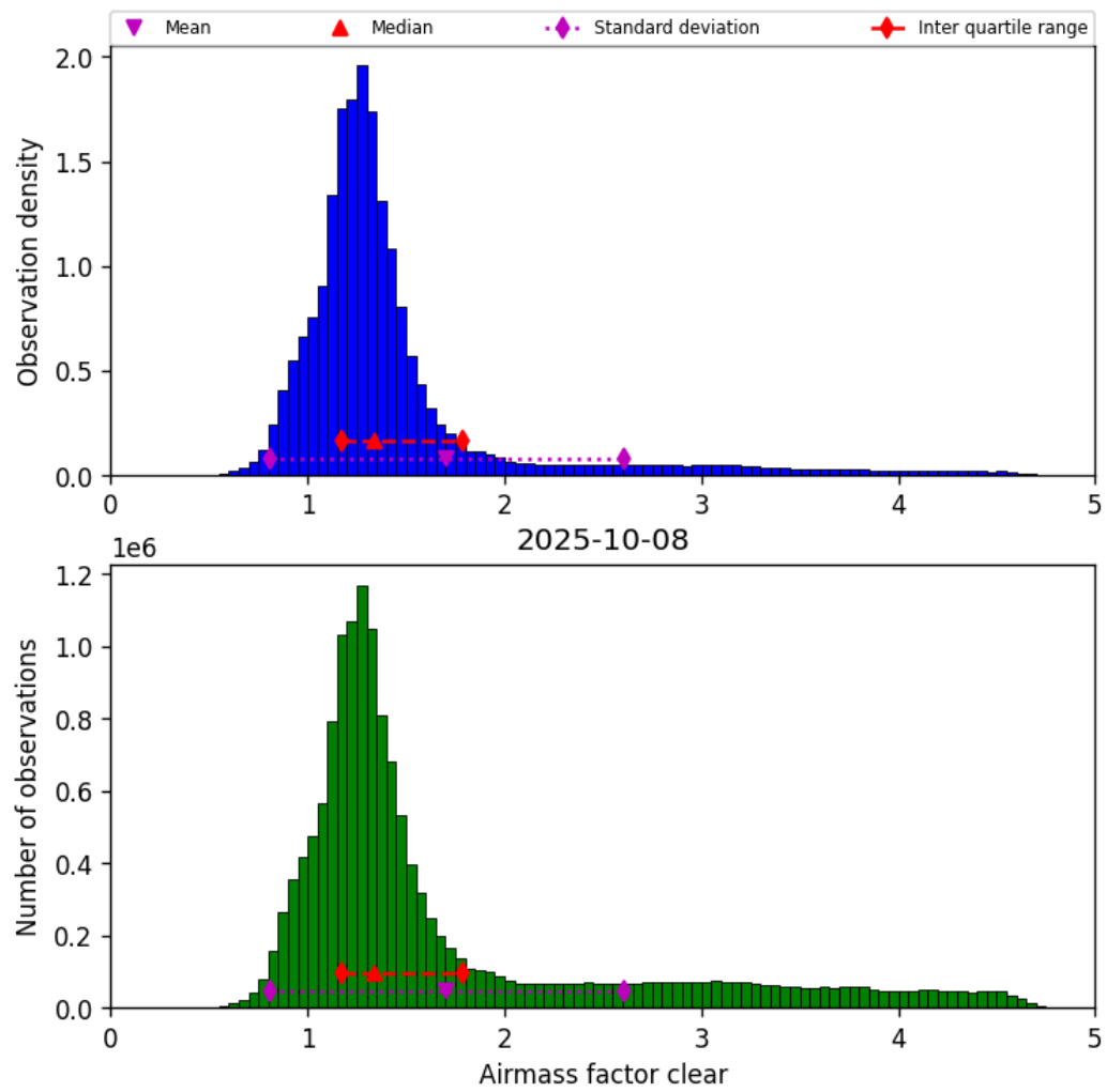
Figure 40: Histogram of “Airmass factor clear” for 2025-10-08 to 2025-10-09
