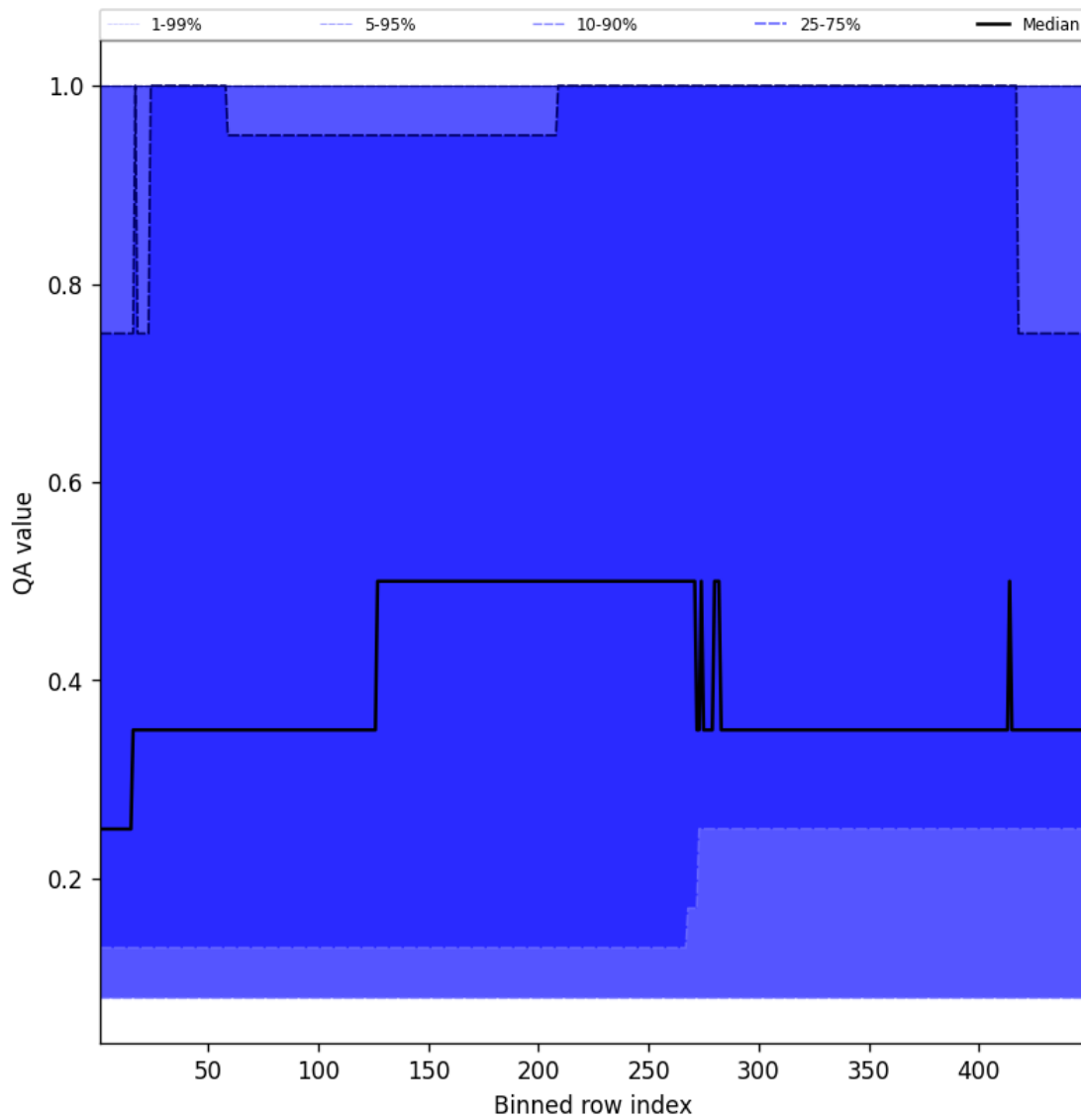
Figure 46: Along track statistics of “QA value” for 2025-10-08 to 2025-10-09
