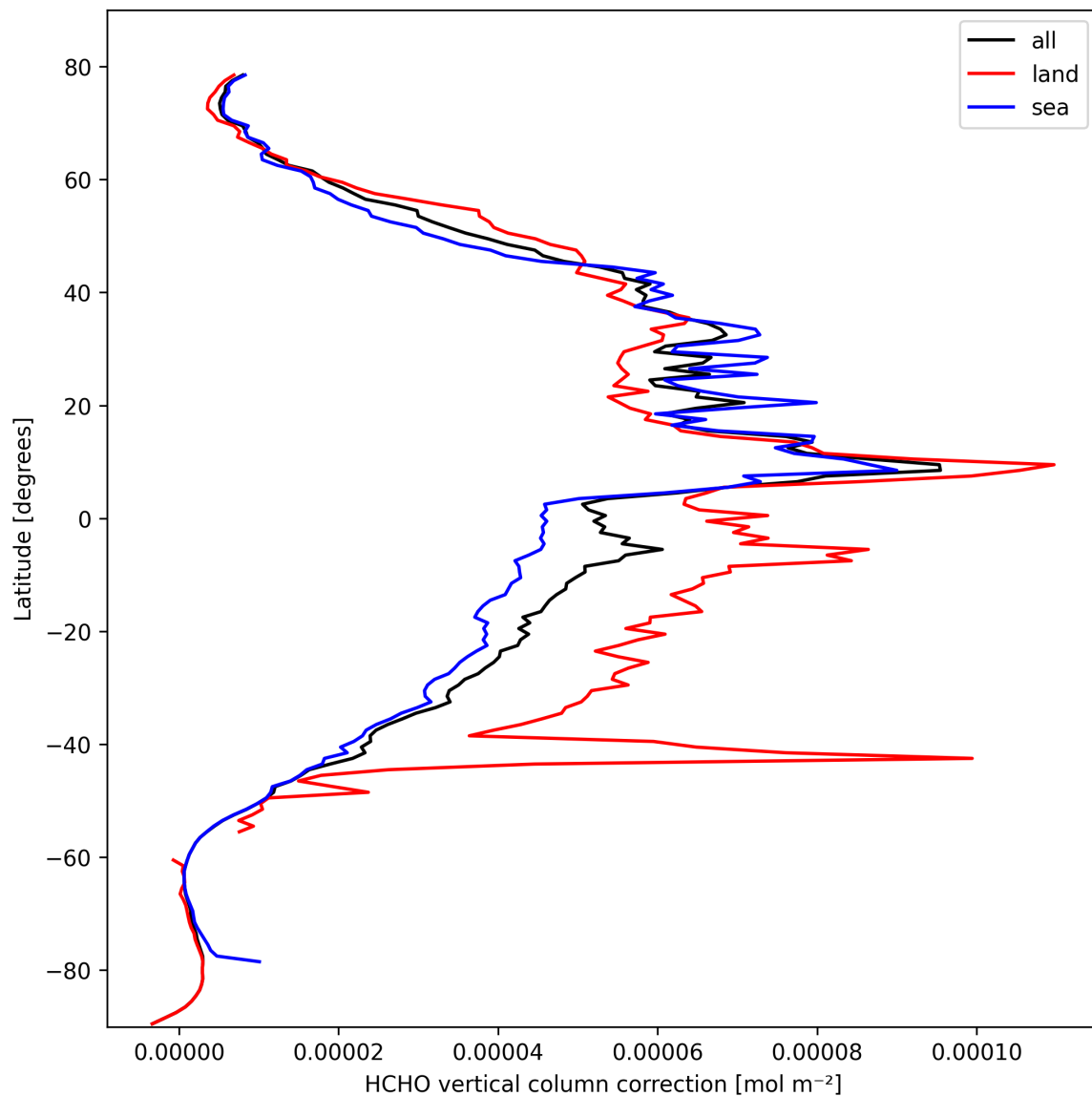
Figure 21: Zonal average of “HCHO vertical column correction” for 2025-10-08 to 2025-10-09.
