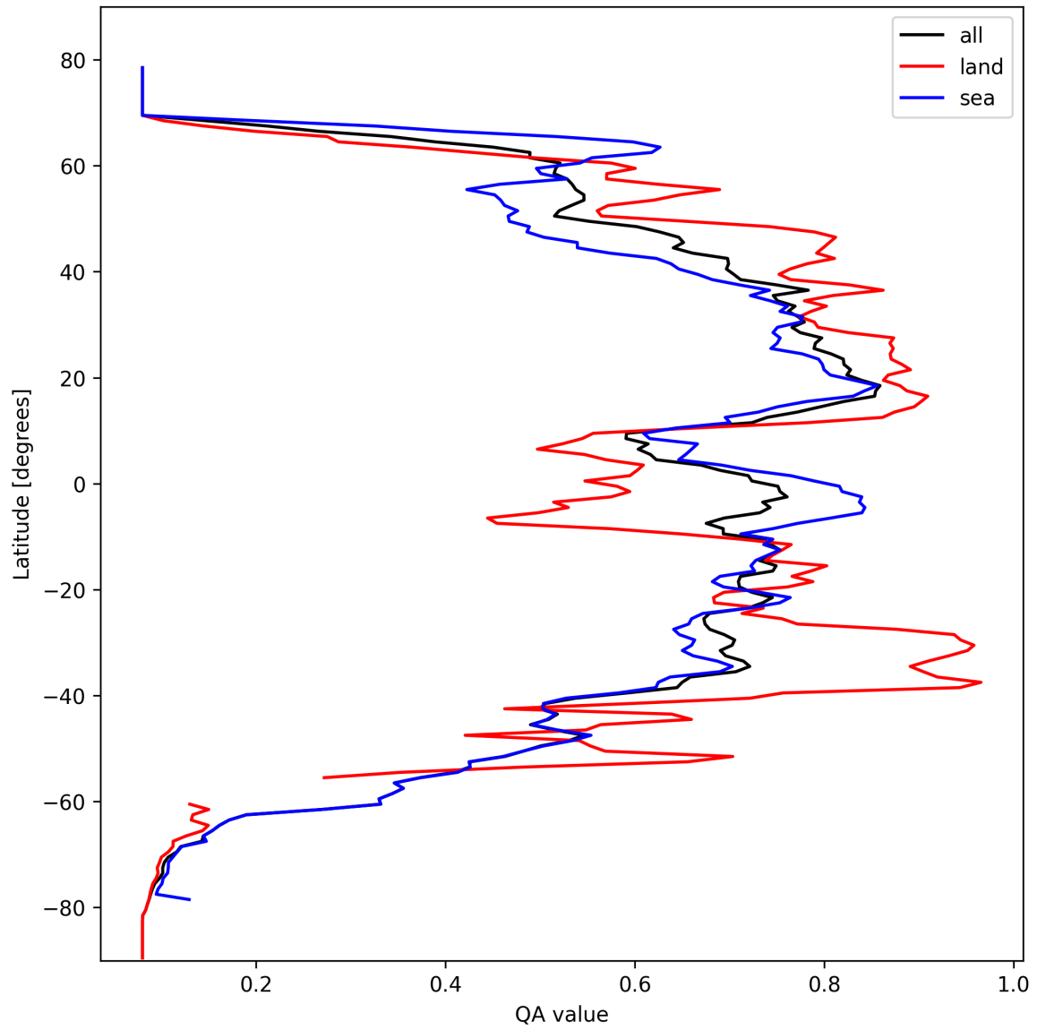
Figure 18: Zonal average of “QA value” for 2025-10-08 to 2025-10-09.
