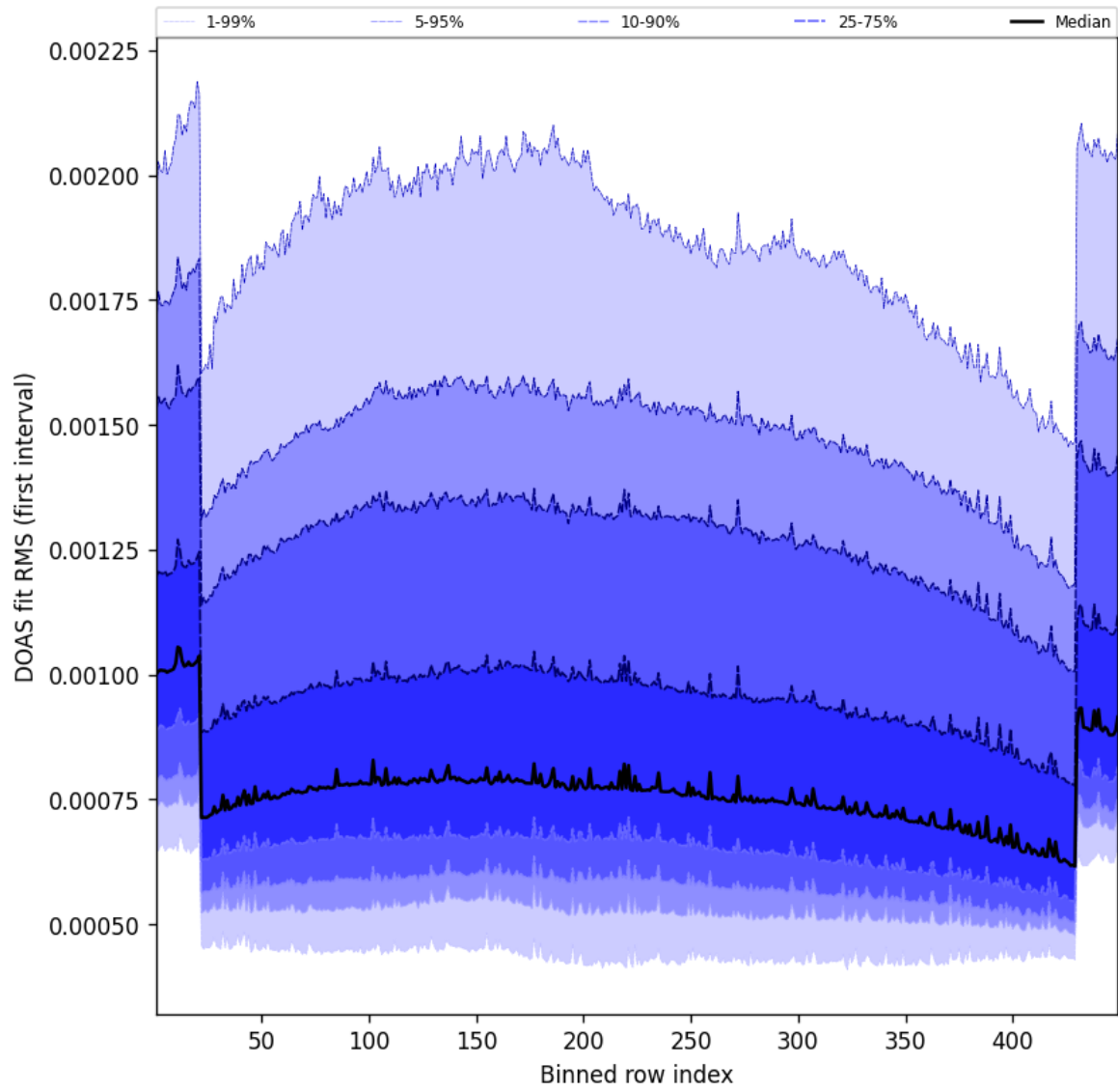
Figure 58: Along track statistics of “DOAS fit RMS (first interval)” for 2025-10-08 to 2025-10-09
