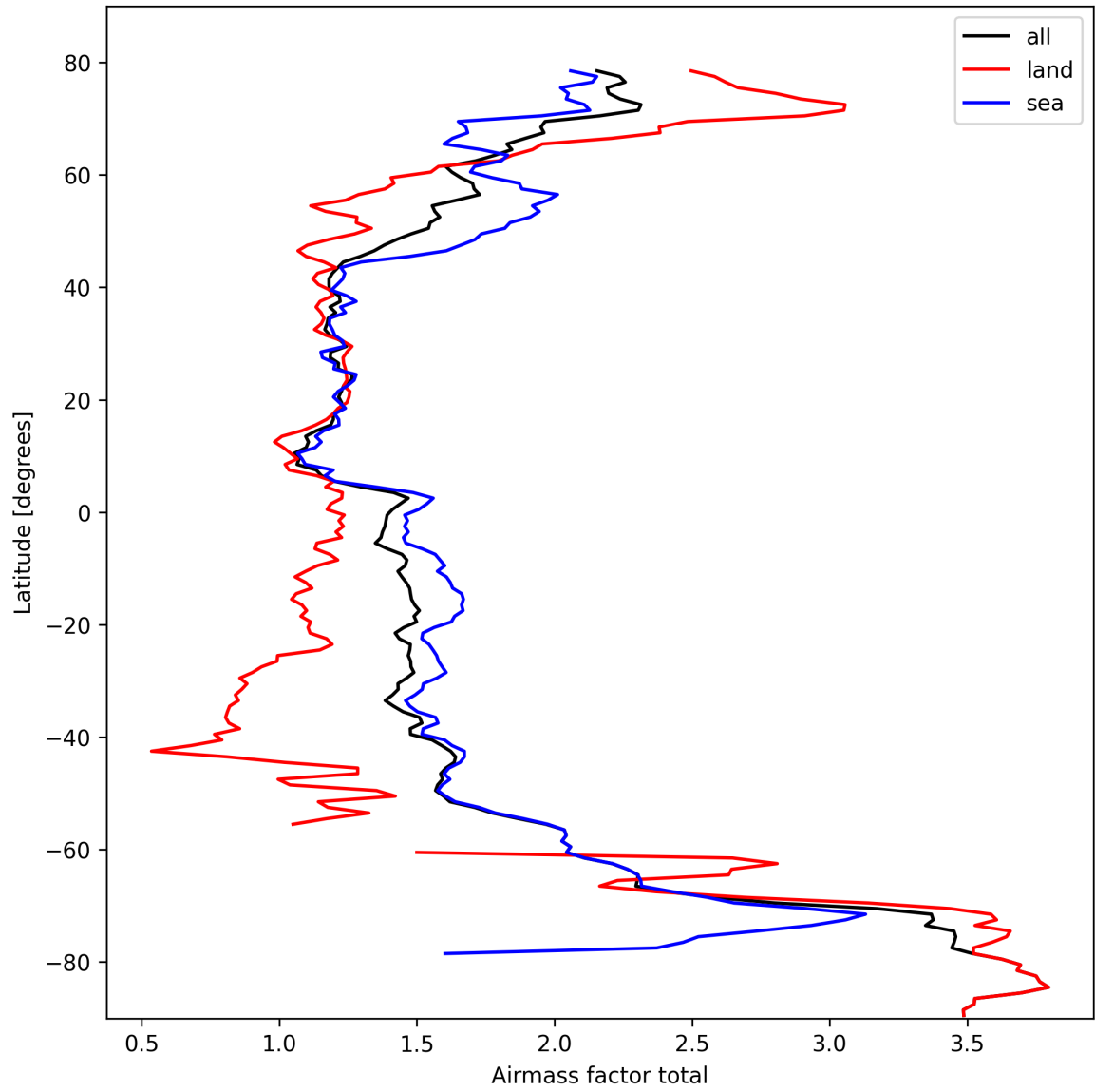
Figure 24: Zonal average of “Airmass factor total” for 2025-10-08 to 2025-10-09.
