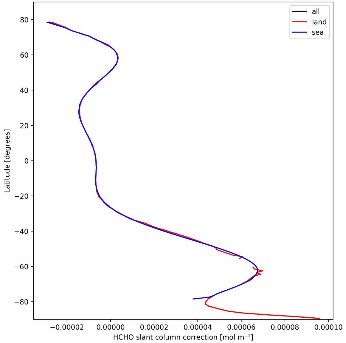
Figure 31: Zonal average of “HCHO slant column correction” for 2025-10-08 to 2025-10-09.
