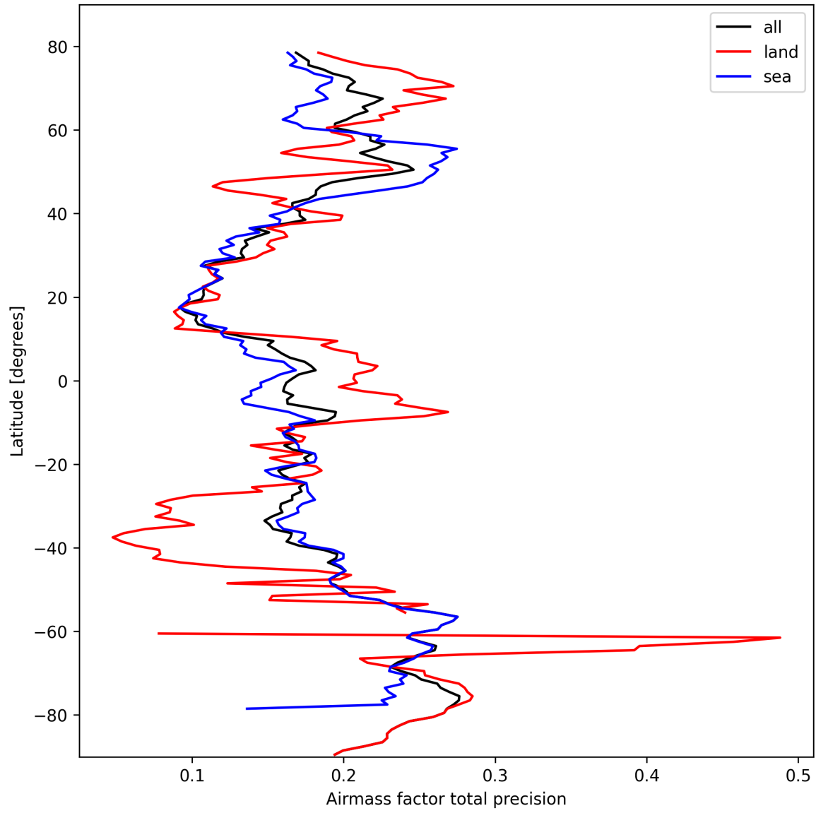
Figure 25: Zonal average of “Airmass factor total precision” for 2025-10-08 to 2025-10-09.
