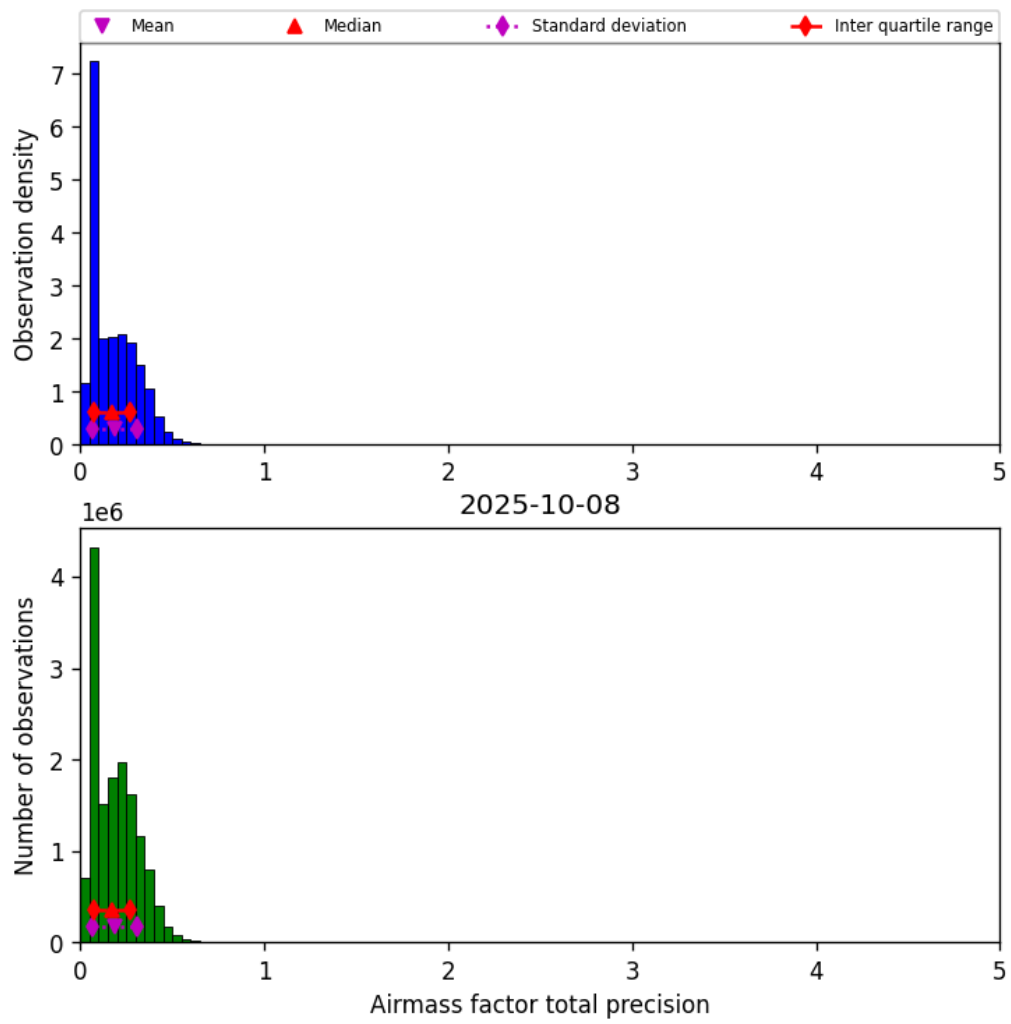
Figure 39: Histogram of “Airmass factor total precision” for 2025-10-08 to 2025-10-09
