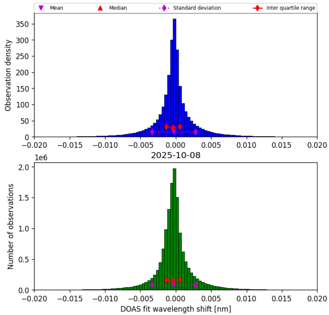
Figure 42: Histogram of “DOAS fit wavelength shift” for 2025-10-08 to 2025-10-09
