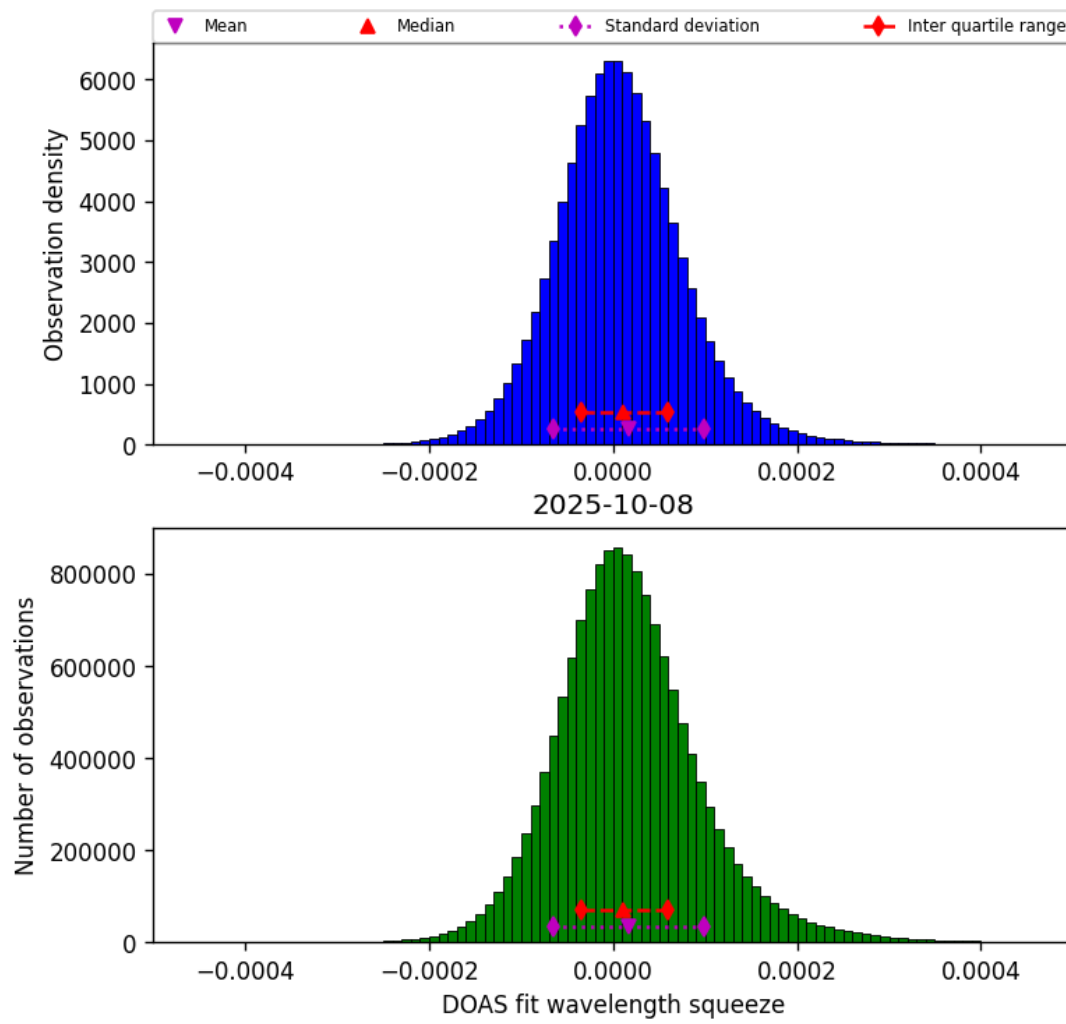
Figure 43: Histogram of “DOAS fit wavelength squeeze” for 2025-10-08 to 2025-10-09
