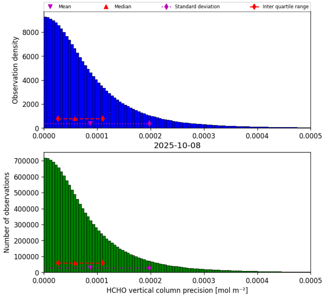
Figure 34: Histogram of “HCHO vertical column precision” for 2025-10-08 to 2025-10-09
