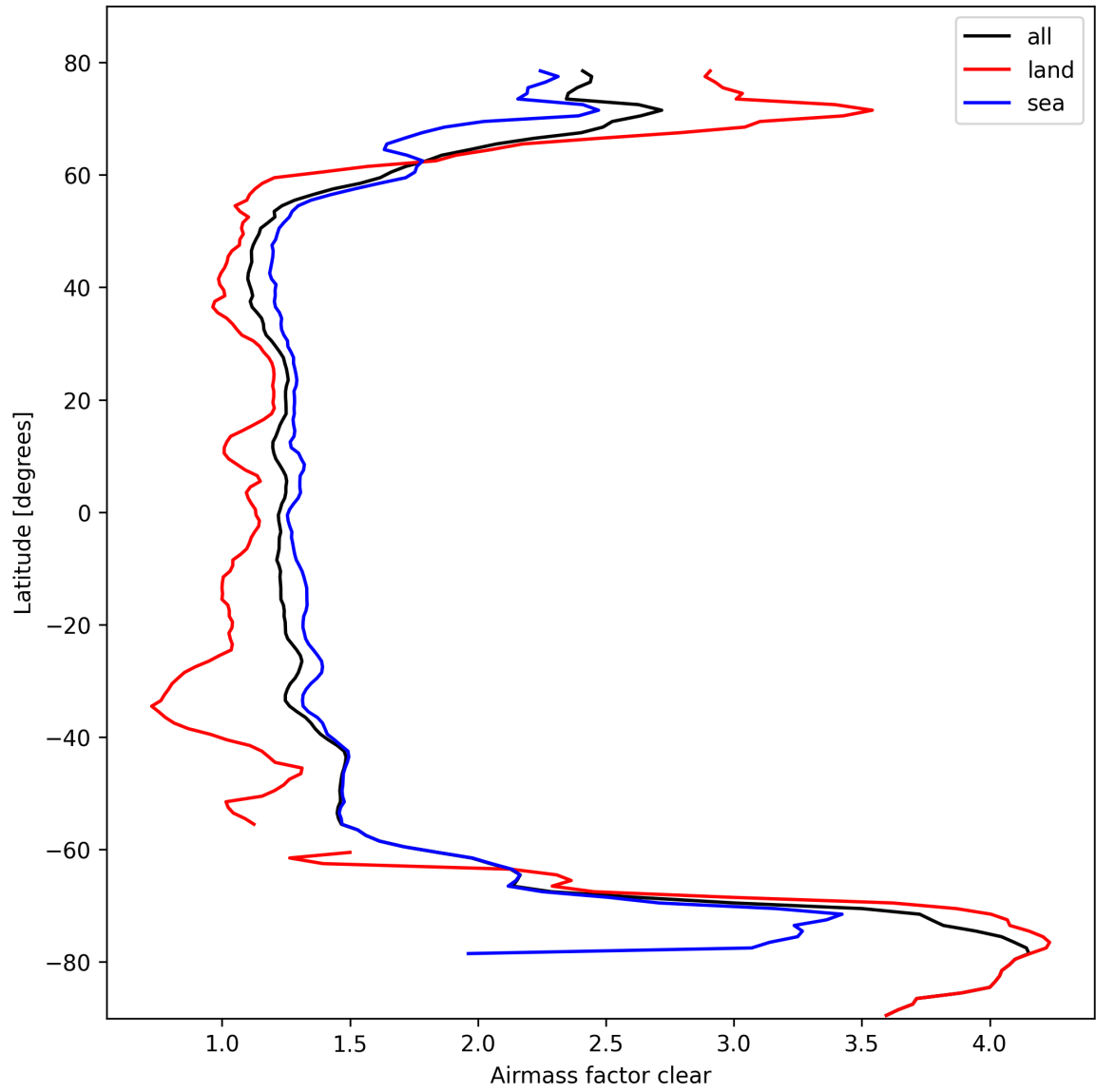
Figure 26: Zonal average of “Airmass factor clear” for 2025-10-08 to 2025-10-09.
