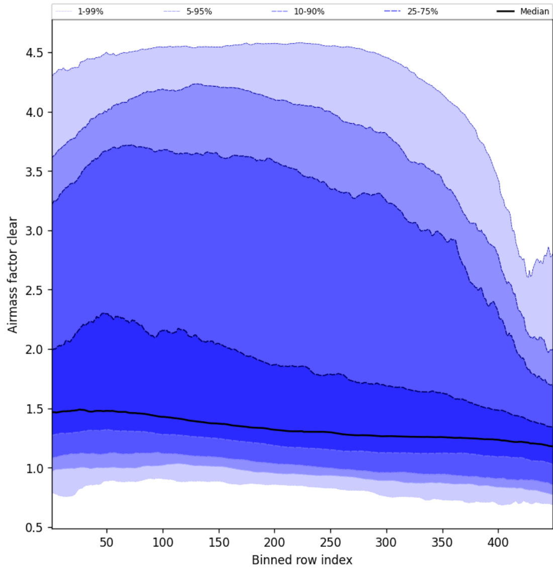
Figure 54: Along track statistics of “Airmass factor clear” for 2025-10-08 to 2025-10-09
