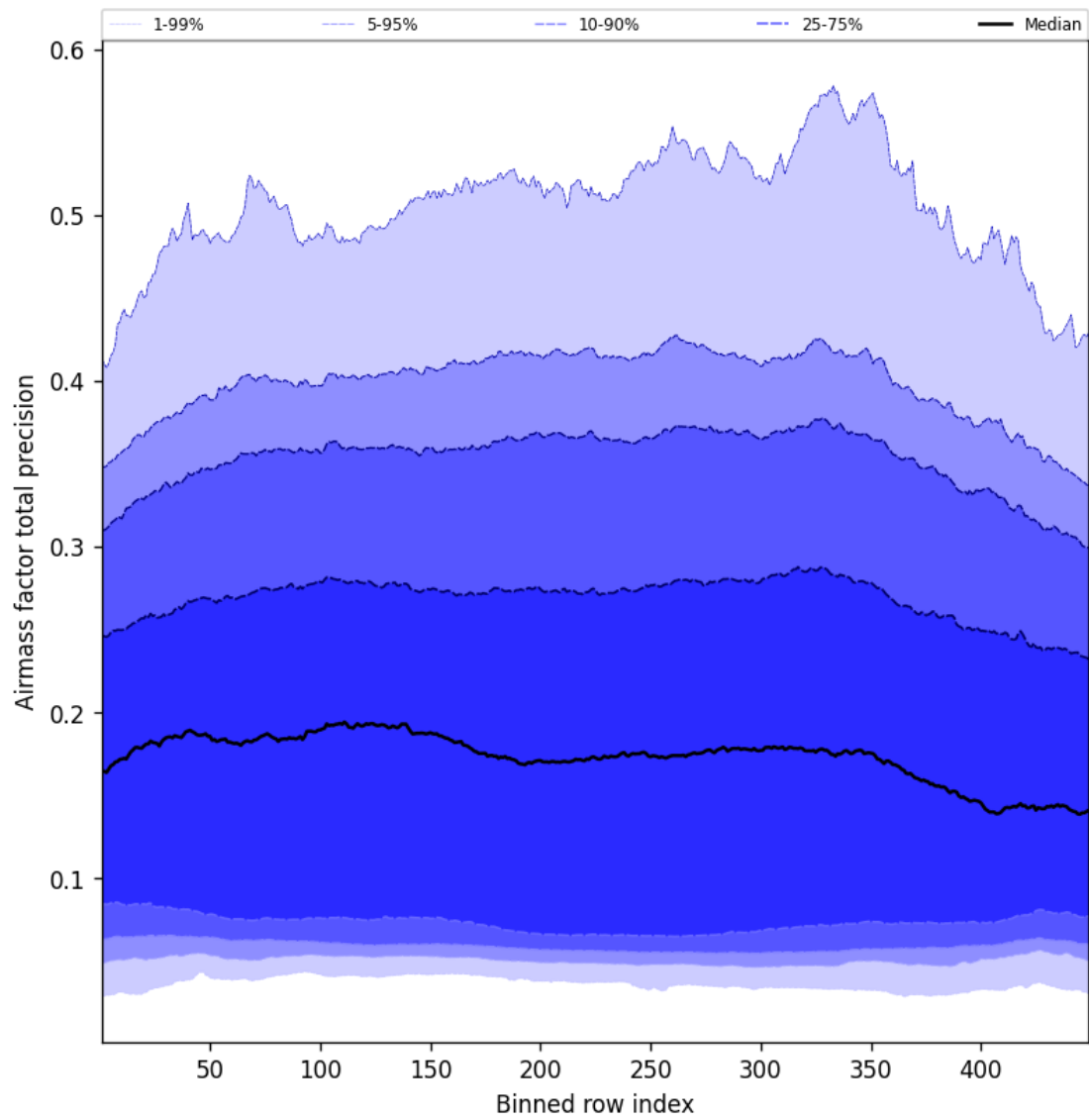
Figure 53: Along track statistics of “Airmass factor total precision” for 2025-10-08 to 2025-10-09
