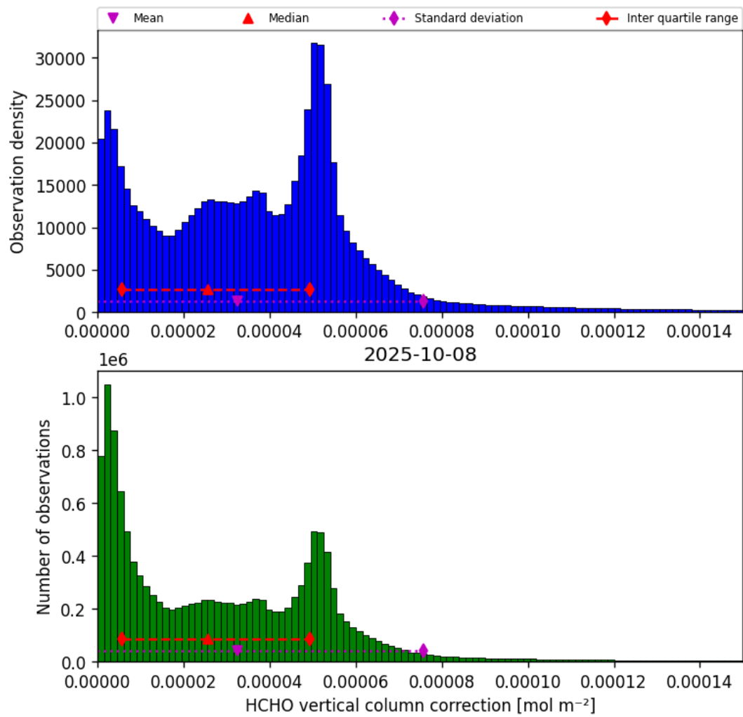
Figure 35: Histogram of “HCHO vertical column correction” for 2025-10-08 to 2025-10-09
