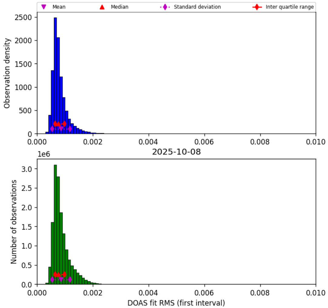
Figure 44: Histogram of “DOAS fit RMS (first interval)” for 2025-10-08 to 2025-10-09
