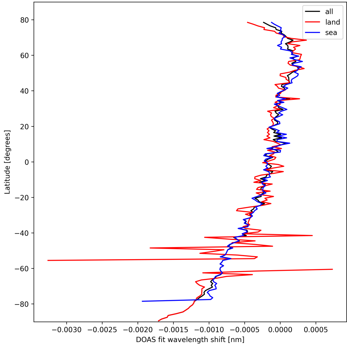
Figure 28: Zonal average of "DOAS fit wavelength shift" for 2025-10-08 to 2025-10-09.
