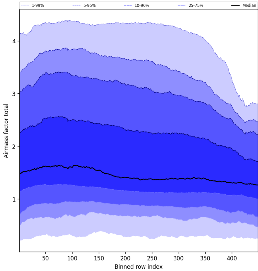
Figure 52: Along track statistics of “Airmass factor total” for 2025-10-08 to 2025-10-09
