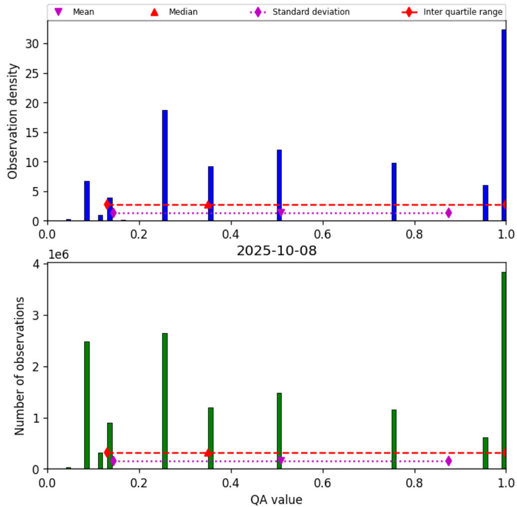
Figure 32: Histogram of “QA value” for 2025-10-08 to 2025-10-09
