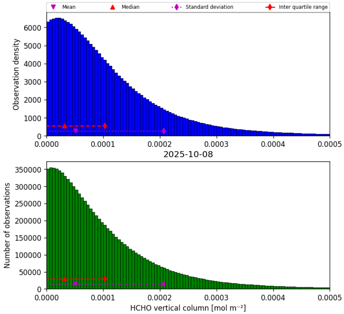
Figure 33: Histogram of “HCHO vertical column” for 2025-10-08 to 2025-10-09
