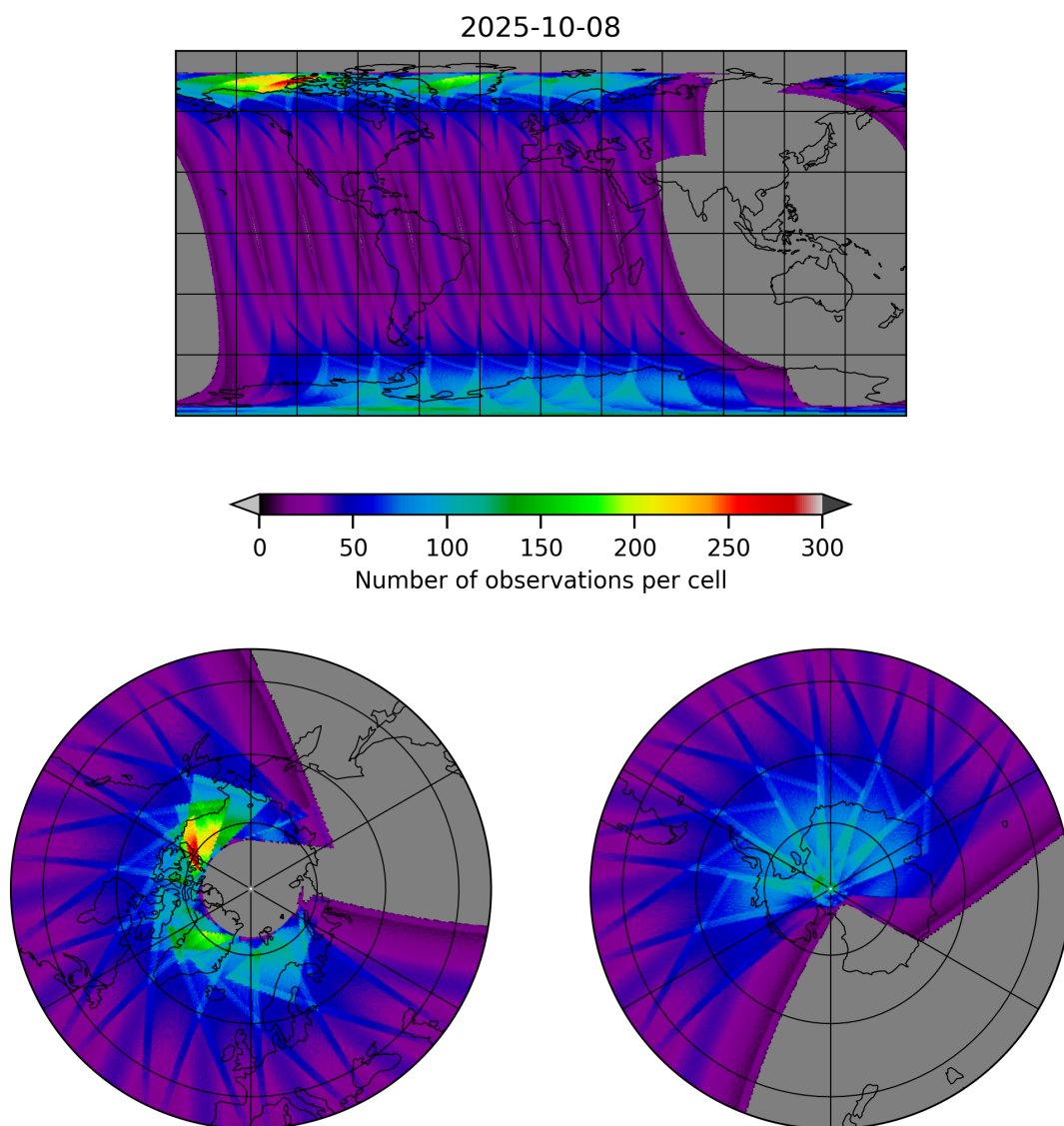
Figure 17: Map of the number of observations for 2025-10-08 to 2025-10-09
