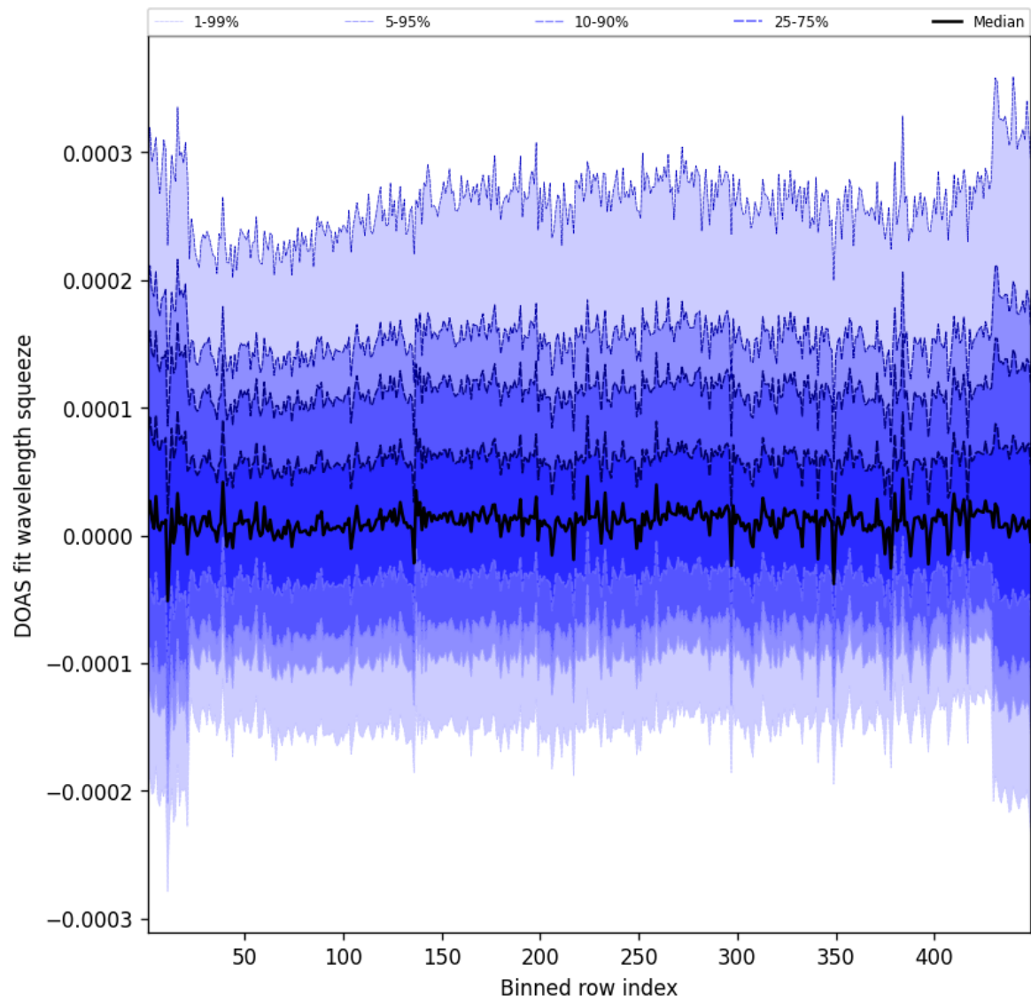
Figure 57: Along track statistics of “DOAS fit wavelength squeeze” for 2025-10-08 to 2025-10-09
