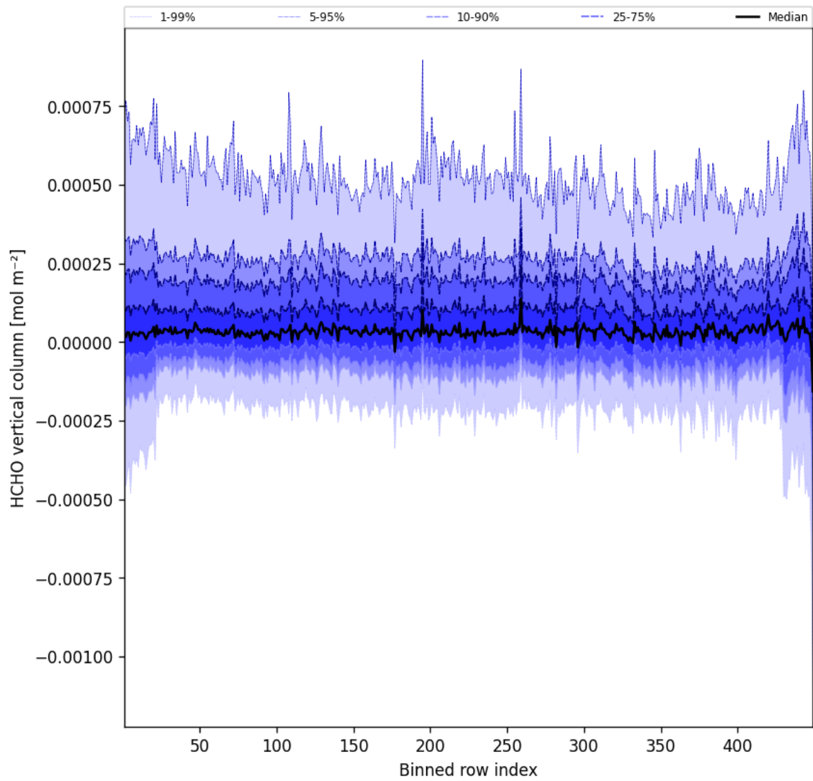
Figure 47: Along track statistics of “HCHO vertical column” for 2025-10-08 to 2025-10-09
