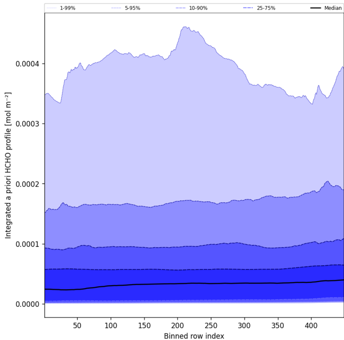
Figure 55: Along track statistics of “Integrated a priori HCHO profile” for 2025-10-08 to 2025-10-09
