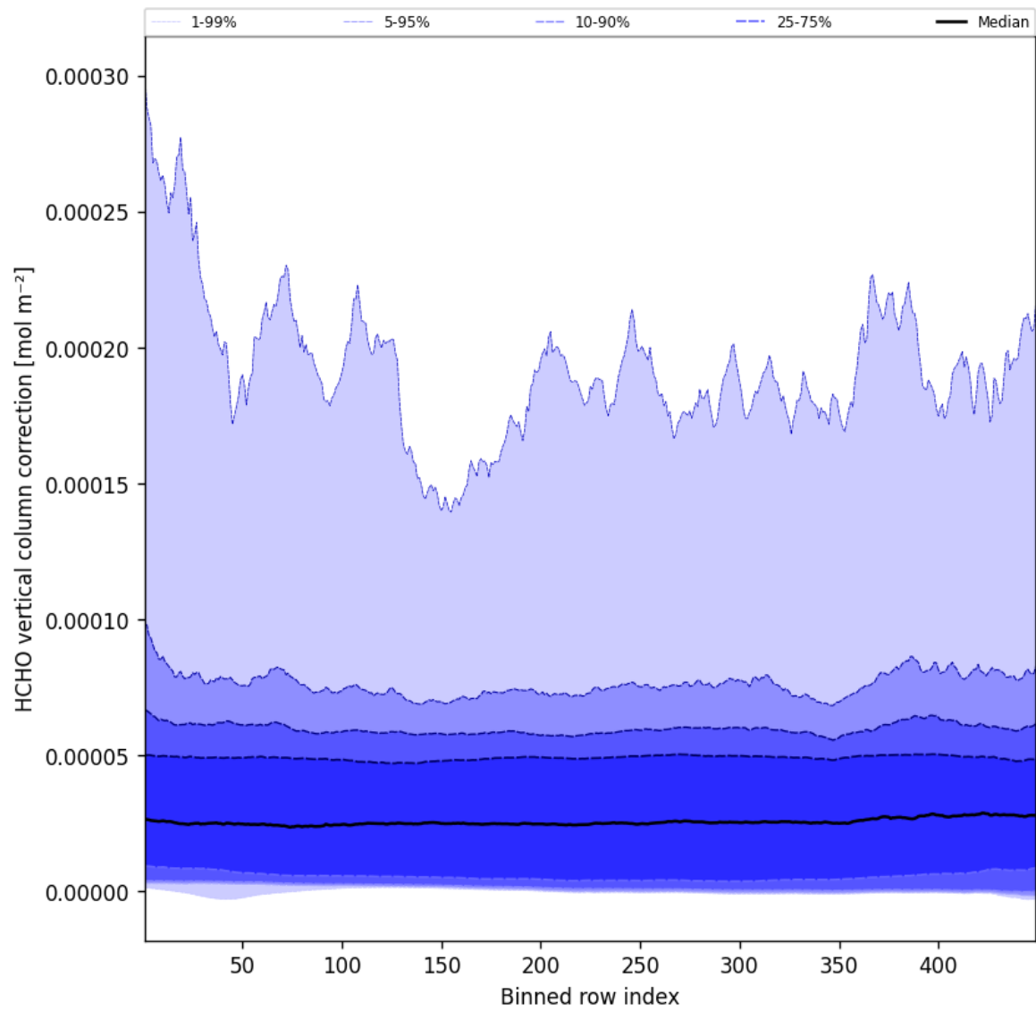
Figure 49: Along track statistics of “HCHO vertical column correction” for 2025-10-08 to 2025-10-09
