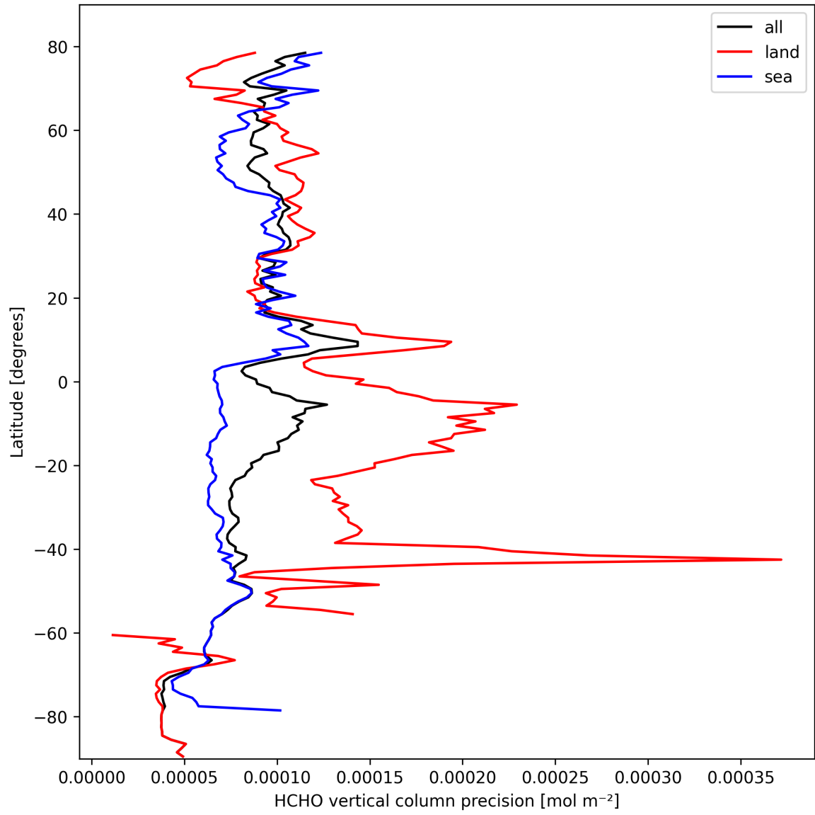
Figure 20: Zonal average of “HCHO vertical column precision” for 2025-10-08 to 2025-10-09.
