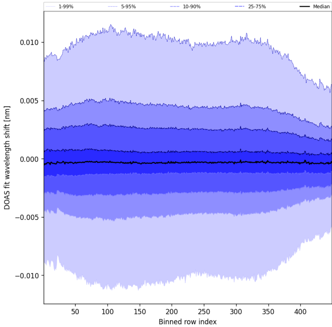
Figure 56: Along track statistics of “DOAS fit wavelength shift” for 2025-10-08 to 2025-10-09
