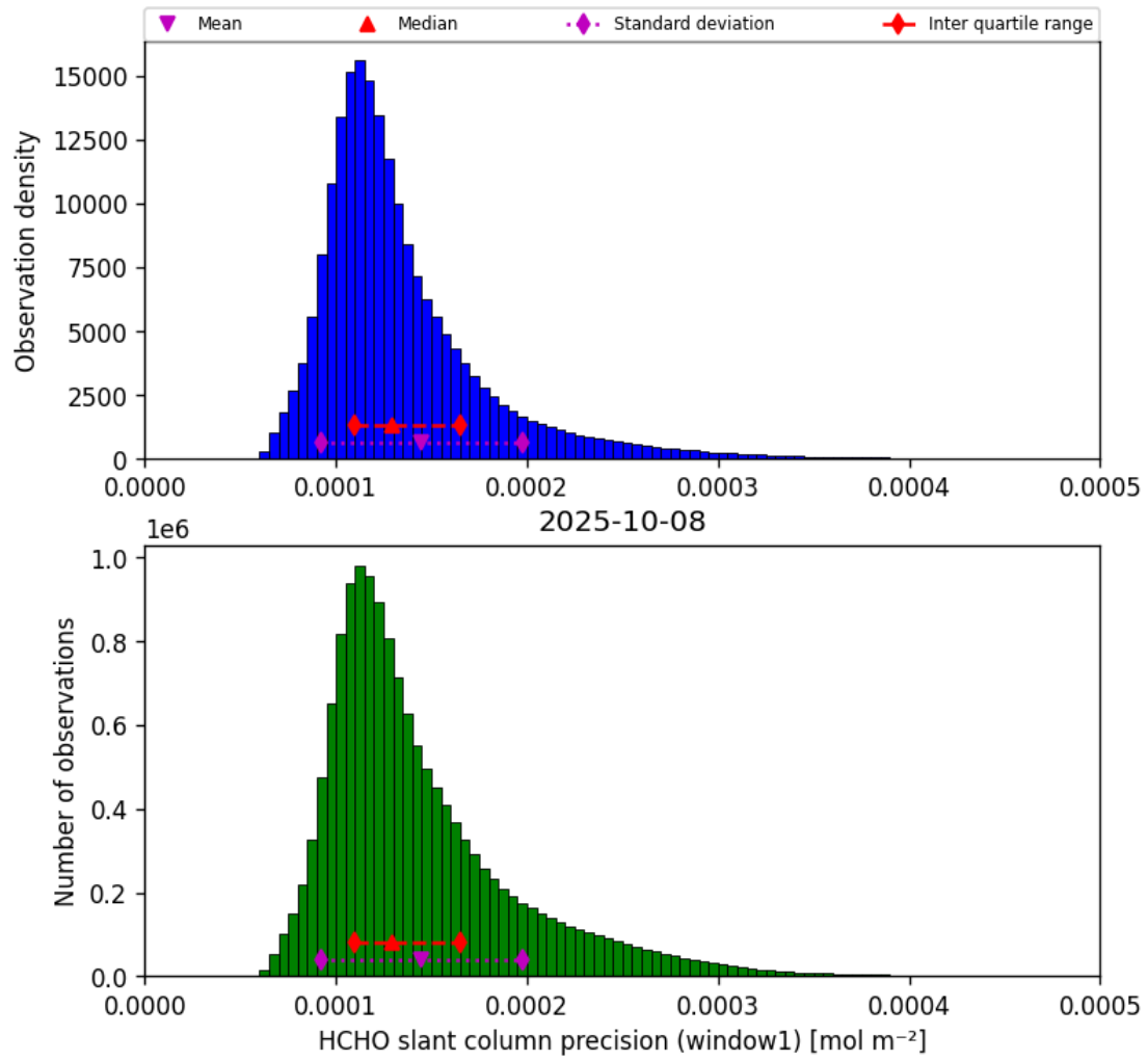
Figure 37: Histogram of “HCHO slant column precision (window1)” for 2025-10-08 to 2025-10-09
