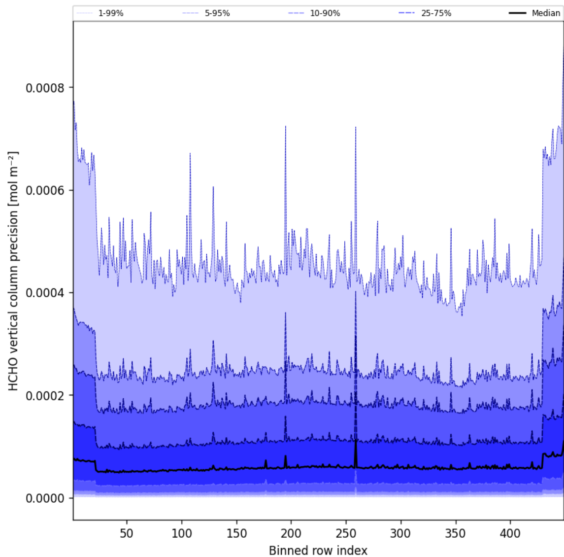
Figure 48: Along track statistics of “HCHO vertical column precision” for 2025-10-08 to 2025-10-09
