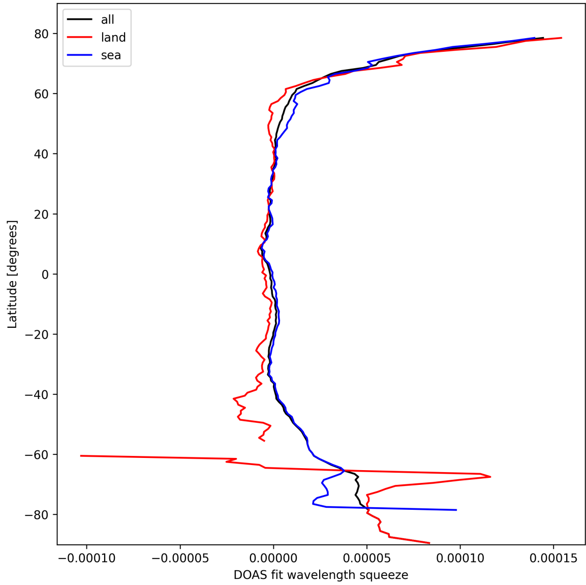
Figure 29: Zonal average of “DOAS fit wavelength squeeze” for 2025-10-08 to 2025-10-09.
