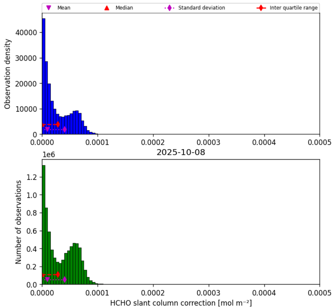
Figure 45: Histogram of “HCHO slant column correction” for 2025-10-08 to 2025-10-09
