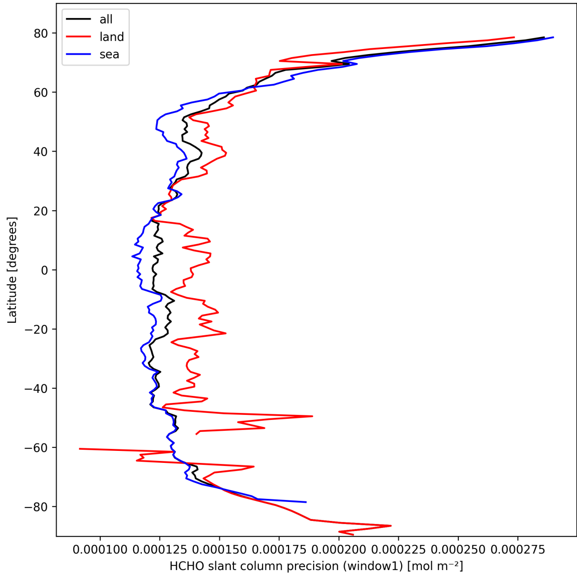
Figure 23: Zonal average of “HCHO slant column precision (window1)” for 2025-10-08 to 2025-10-09.
