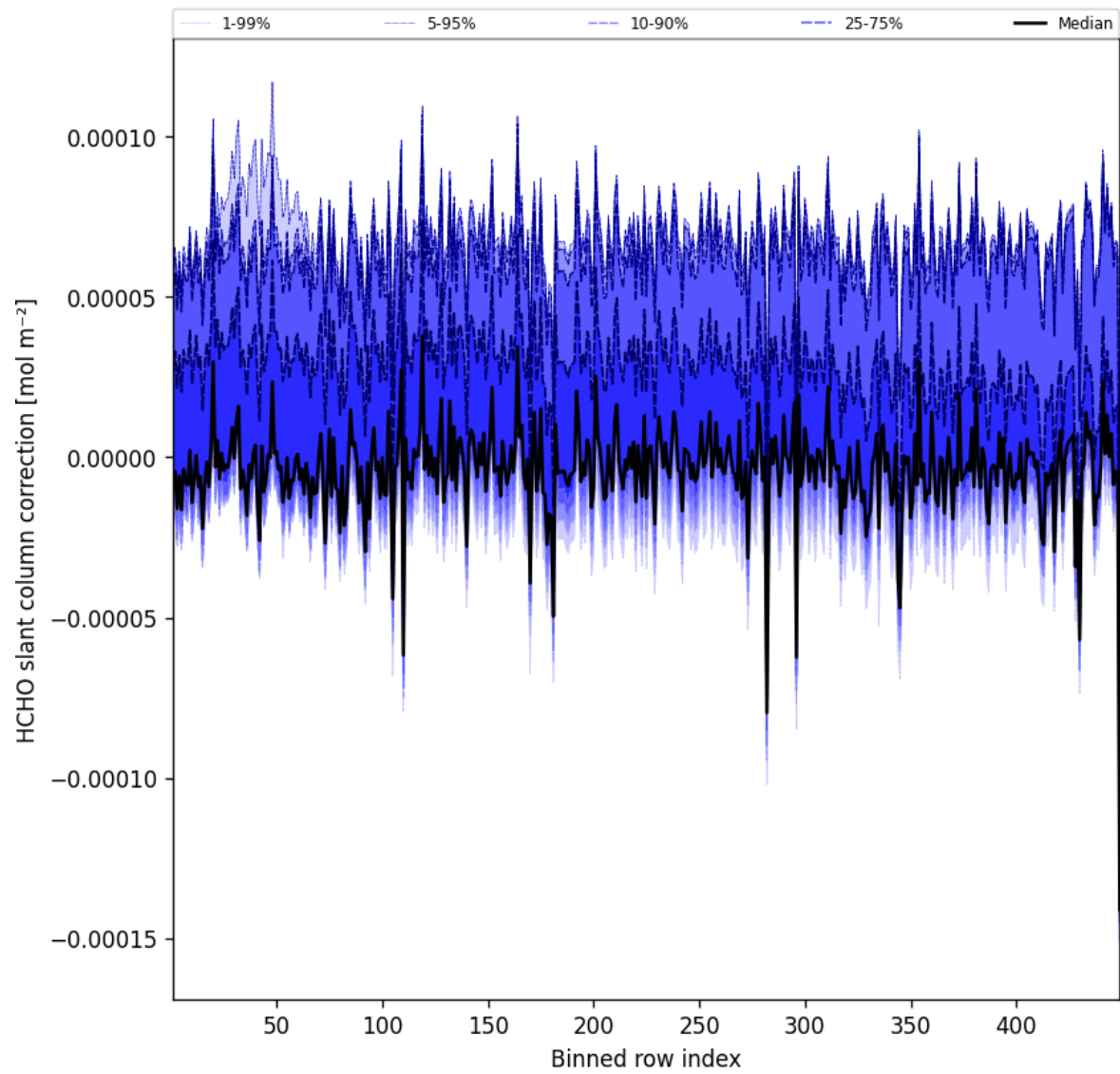
Figure 59: Along track statistics of “HCHO slant column correction” for 2025-10-08 to 2025-10-09
