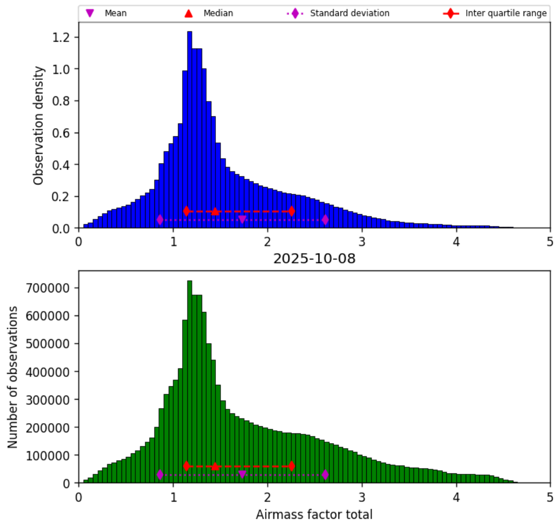
Figure 38: Histogram of “Airmass factor total” for 2025-10-08 to 2025-10-09
