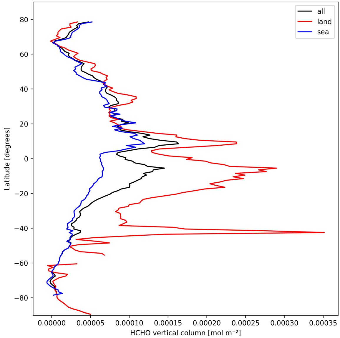
Figure 19: Zonal average of “HCHO vertical column” for 2025-10-08 to 2025-10-09.
