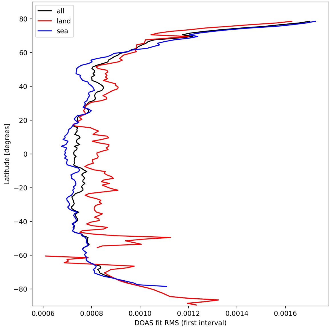
Figure 30: Zonal average of "DOAS fit RMS (first interval)" for 2025-10-08 to 2025-10-09.
