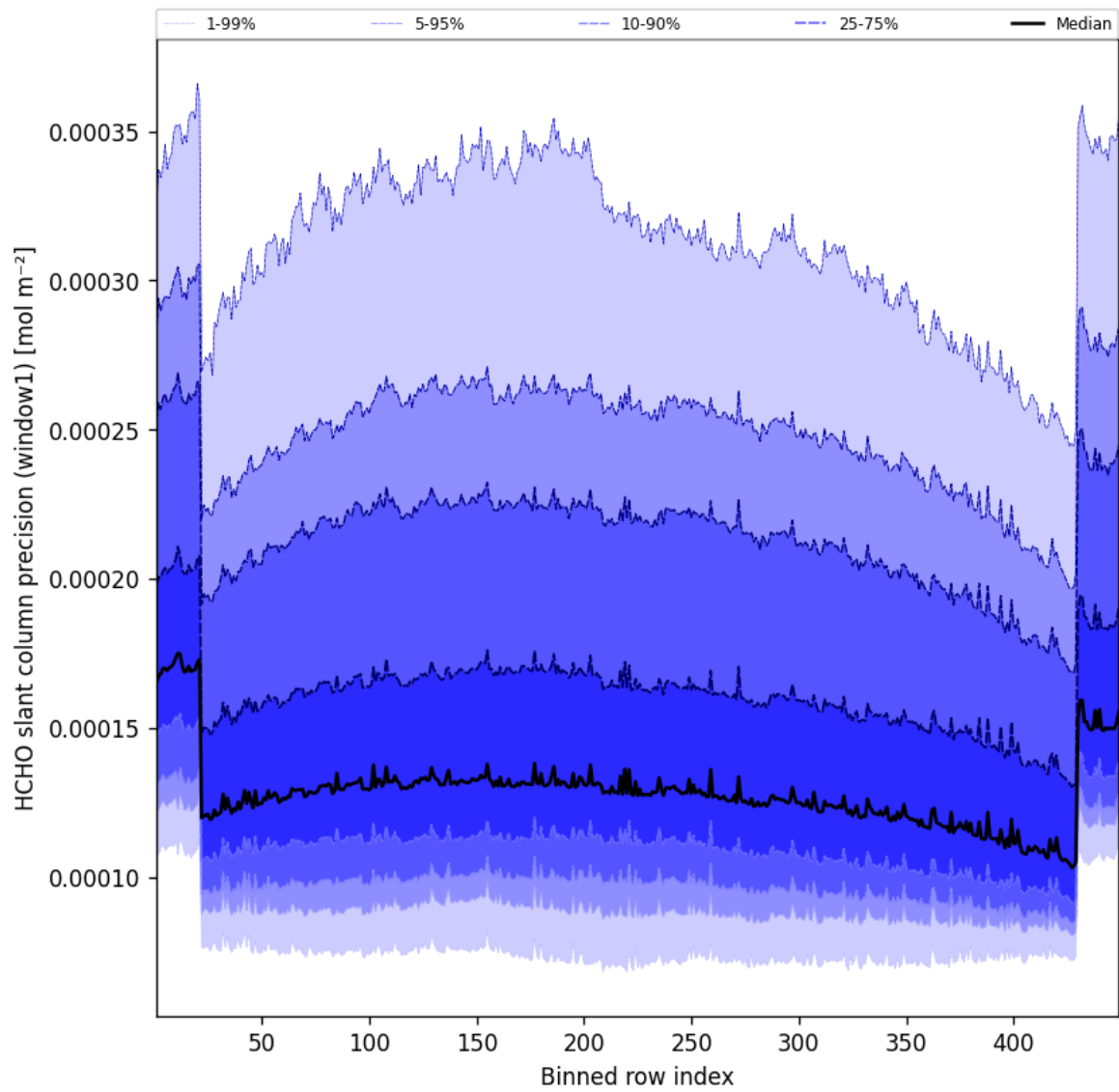
Figure 51: Along track statistics of “HCHO slant column precision (window1)” for 2025-10-08 to 2025-10-09
