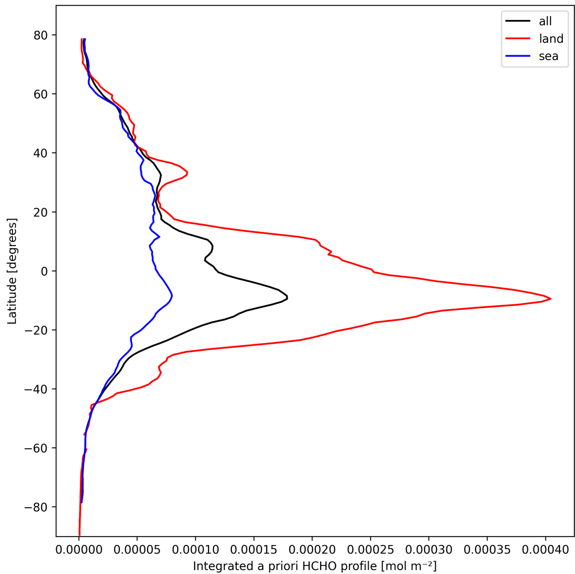
Figure 27: Zonal average of “Integrated a priori HCHO profile” for 2025-10-08 to 2025-10-09.
