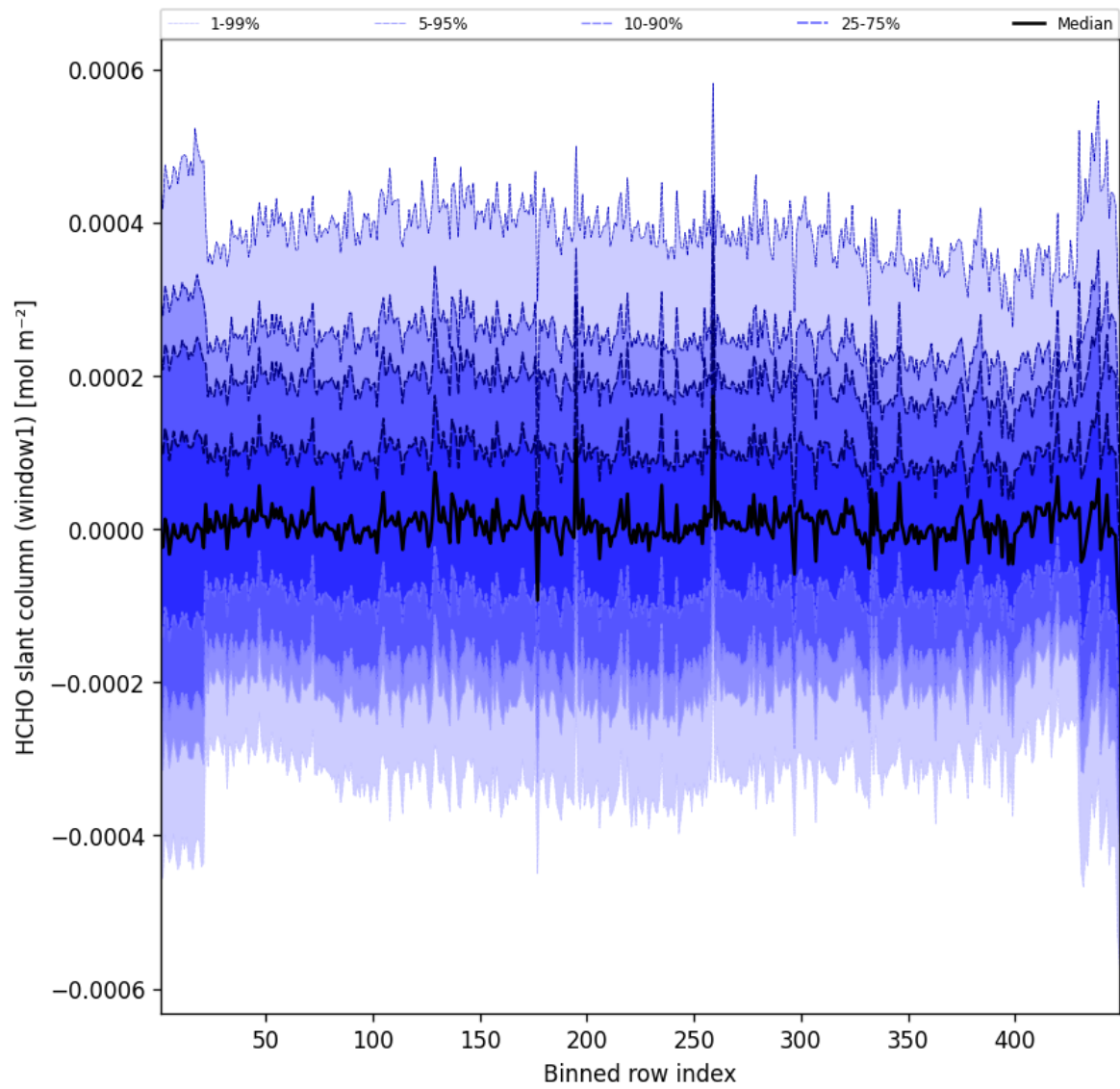
Figure 50: Along track statistics of “HCHO slant column (window1)” for 2025-10-08 to 2025-10-09
