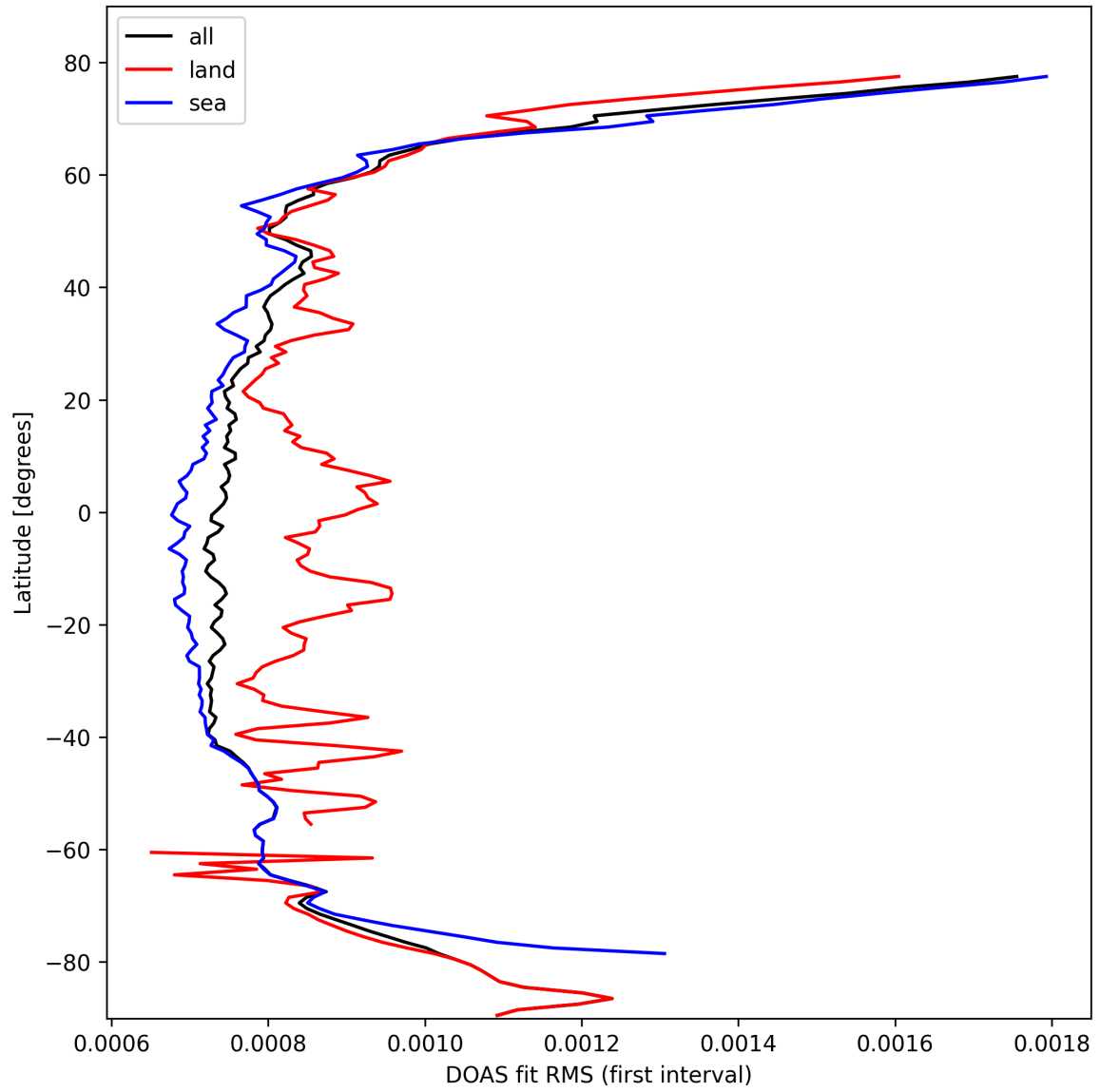
Figure 30: Zonal average of “DOAS fit RMS (first interval)” for 2025-10-11 to 2025-10-12.
