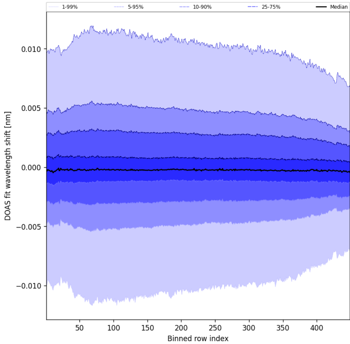
Figure 56: Along track statistics of “DOAS fit wavelength shift” for 2025-10-11 to 2025-10-12
