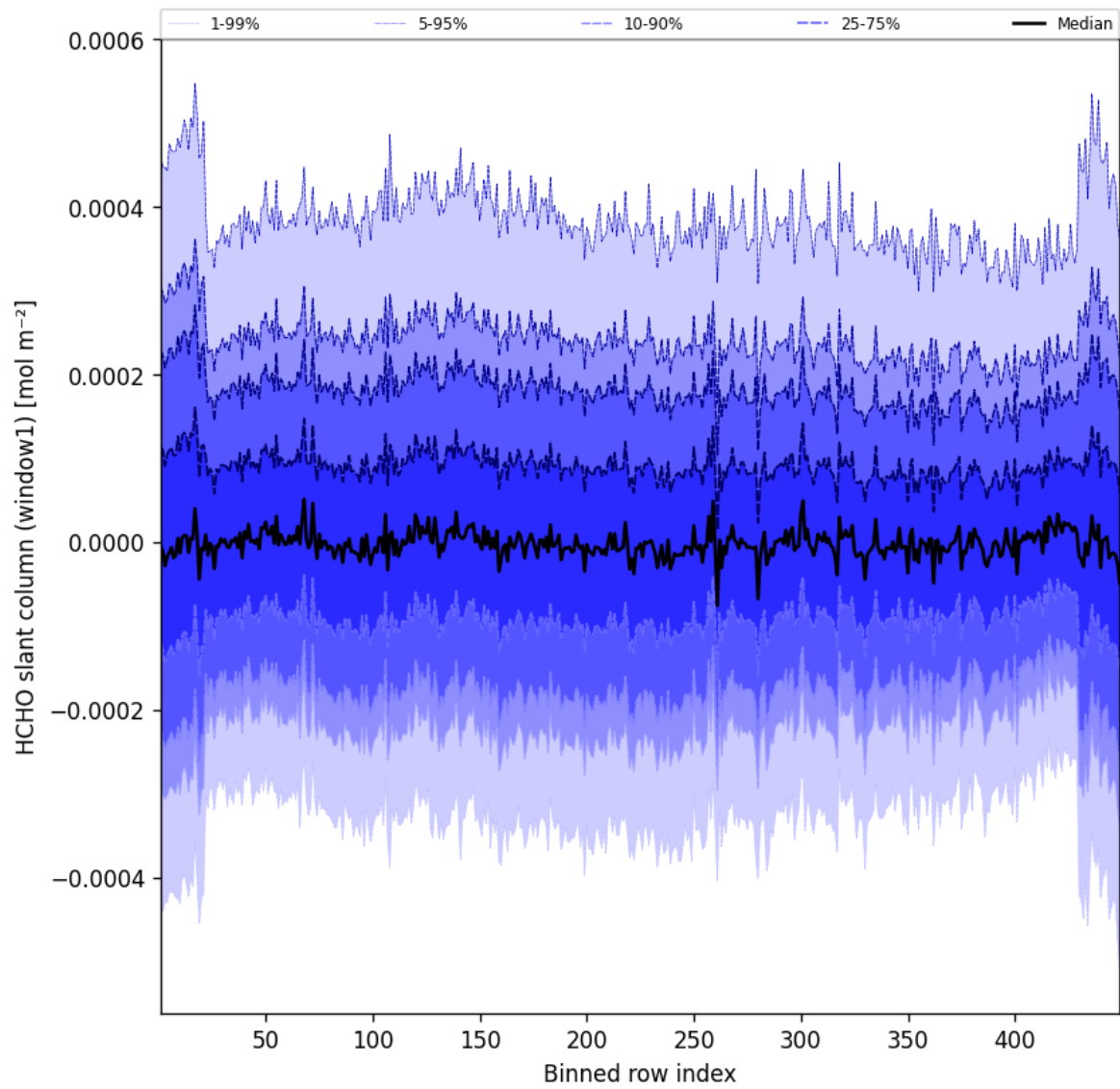
Figure 50: Along track statistics of “HCHO slant column (window1)” for 2025-10-11 to 2025-10-12
