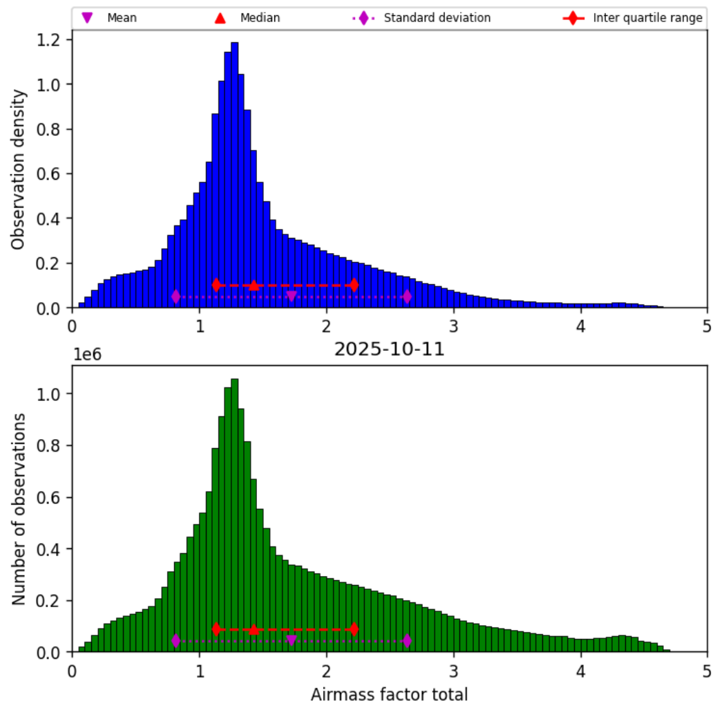
Figure 38: Histogram of “Airmass factor total” for 2025-10-11 to 2025-10-12
