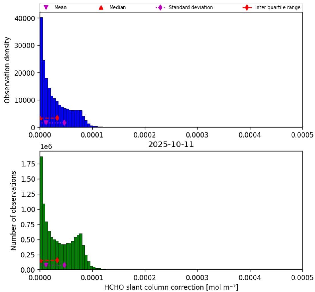
Figure 45: Histogram of “HCHO slant column correction” for 2025-10-11 to 2025-10-12
