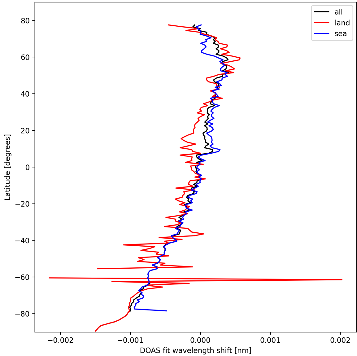
Figure 28: Zonal average of “DOAS fit wavelength shift” for 2025-10-11 to 2025-10-12.
