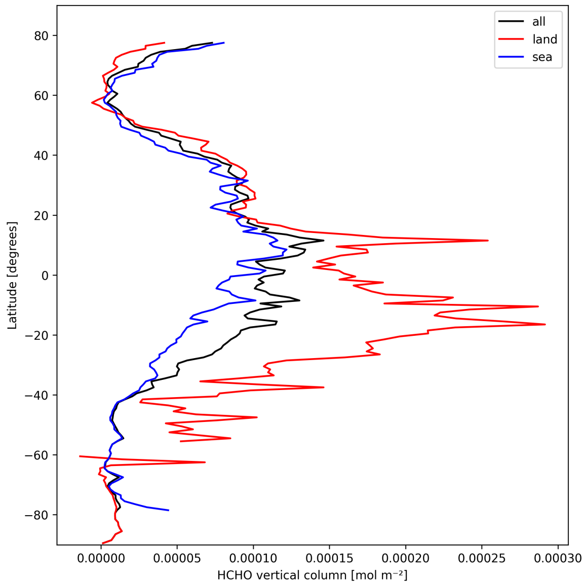
Figure 19: Zonal average of “HCHO vertical column” for 2025-10-11 to 2025-10-12.
