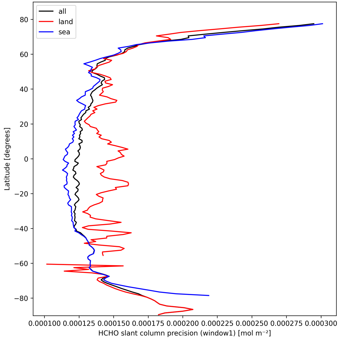
Figure 23: Zonal average of “HCHO slant column precision (window1)” for 2025-10-11 to 2025-10-12.
