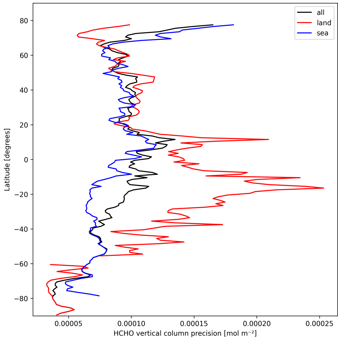
Figure 20: Zonal average of “HCHO vertical column precision” for 2025-10-11 to 2025-10-12.
