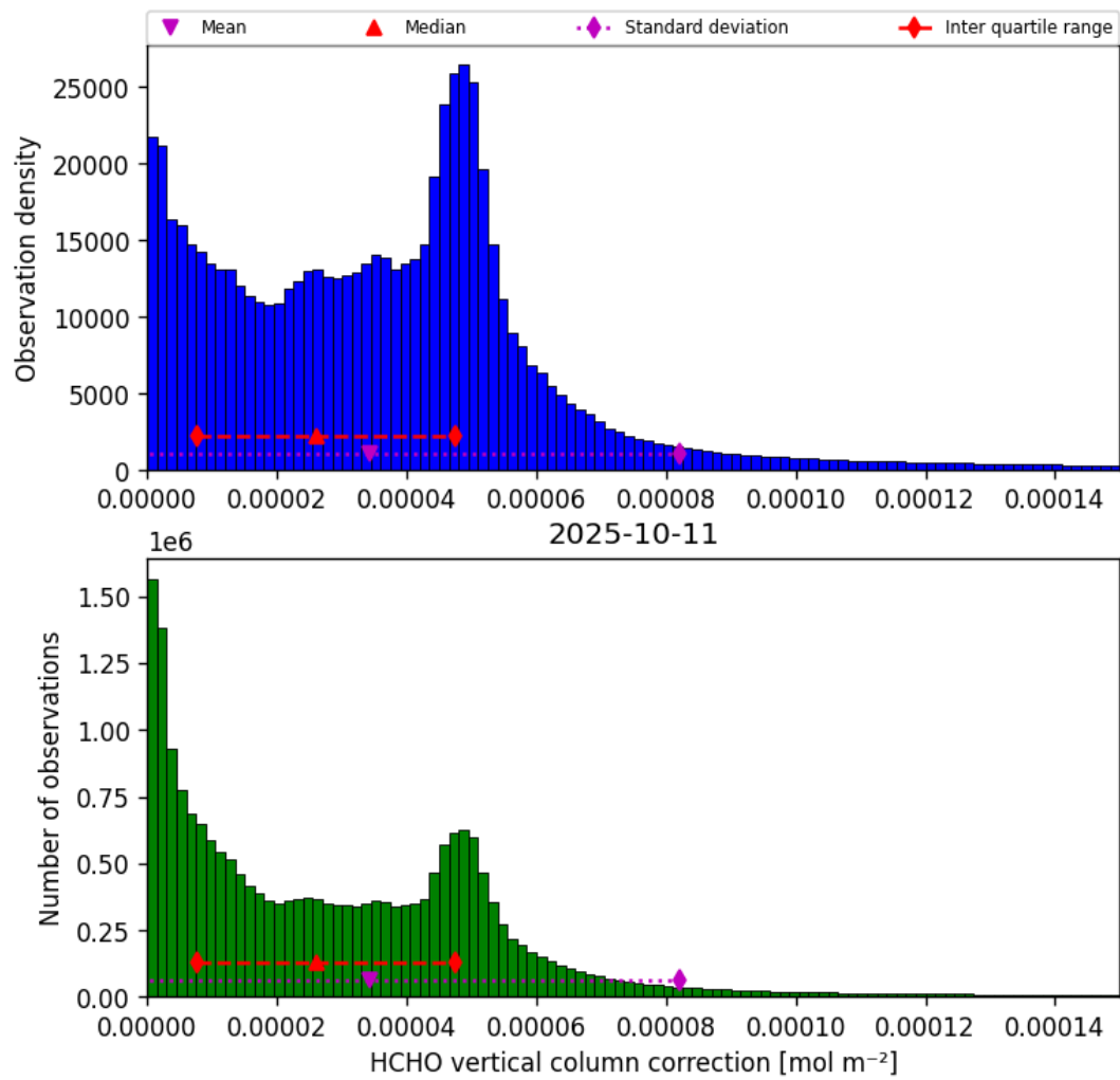
Figure 35: Histogram of “HCHO vertical column correction” for 2025-10-11 to 2025-10-12
