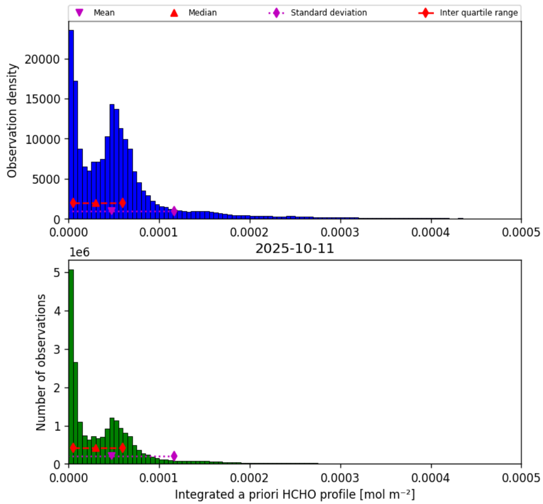
Figure 41: Histogram of “Integrated a priori HCHO profile” for 2025-10-11 to 2025-10-12
