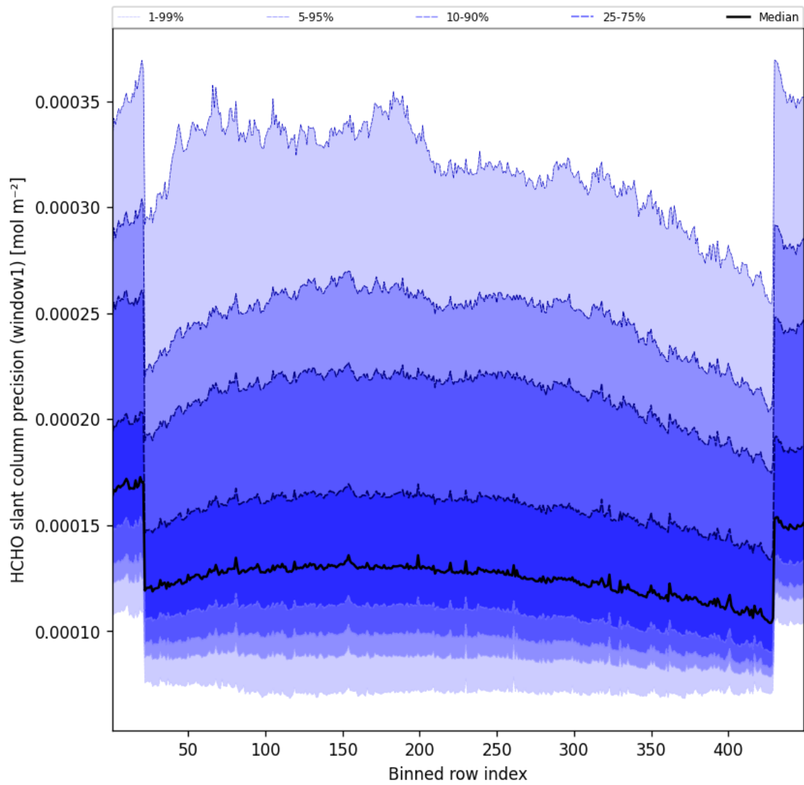
Figure 51: Along track statistics of “HCHO slant column precision (window1)” for 2025-10-11 to 2025-10-12
