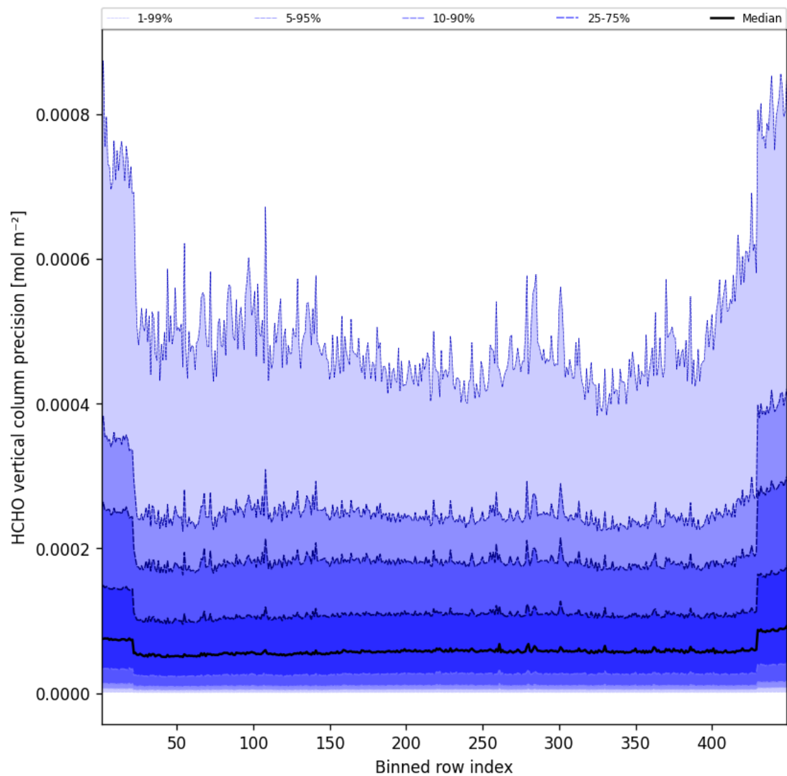
Figure 48: Along track statistics of “HCHO vertical column precision” for 2025-10-11 to 2025-10-12
