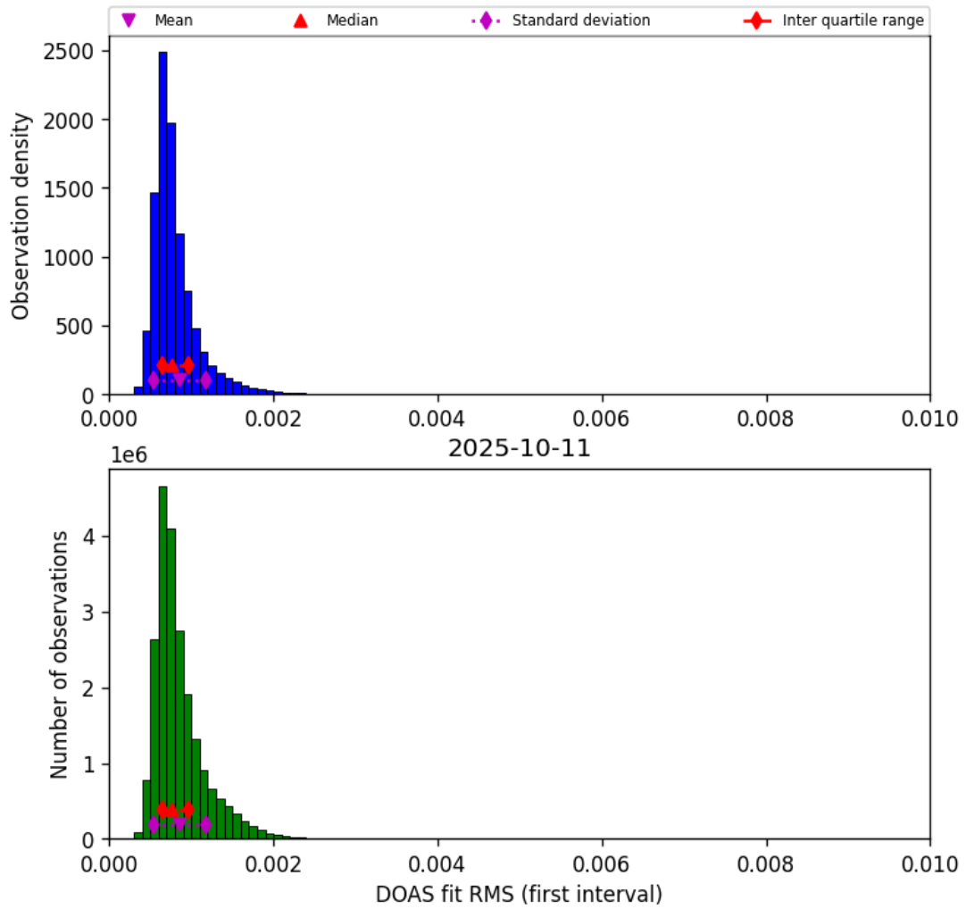
Figure 44: Histogram of “DOAS fit RMS (first interval)” for 2025-10-11 to 2025-10-12
