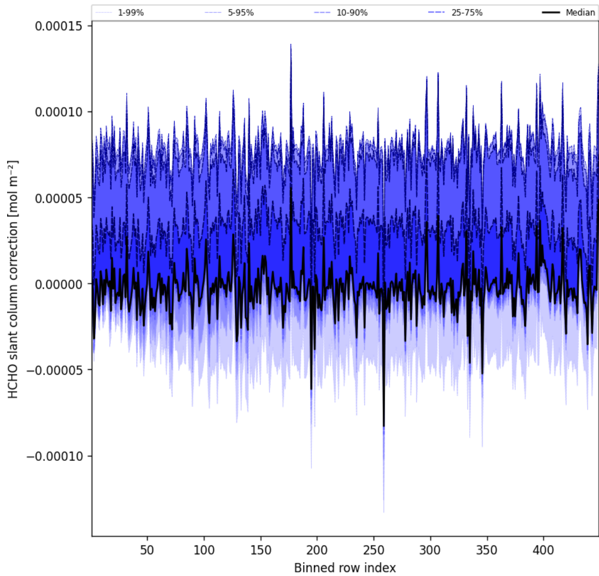
Figure 59: Along track statistics of “HCHO slant column correction” for 2025-10-11 to 2025-10-12
