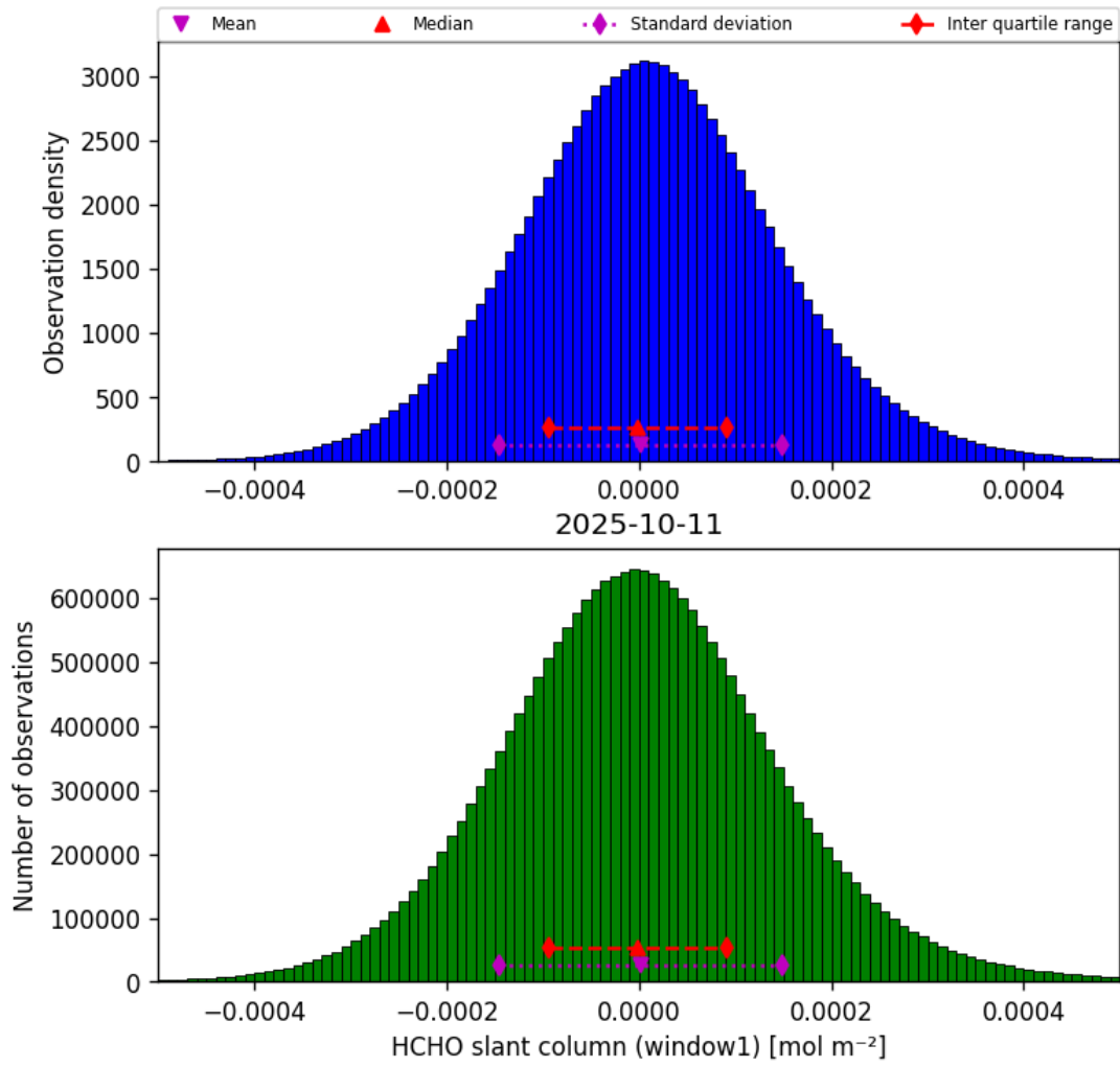
Figure 36: Histogram of “HCHO slant column (window1)” for 2025-10-11 to 2025-10-12
