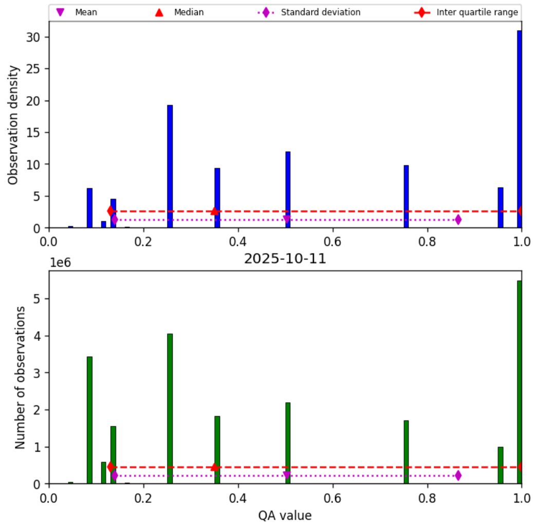
Figure 32: Histogram of “QA value” for 2025-10-11 to 2025-10-12
