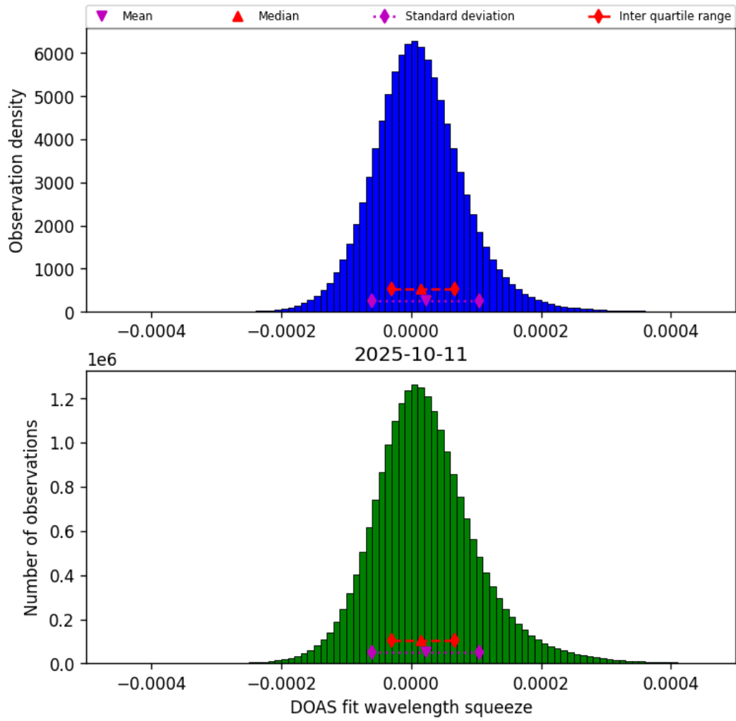
Figure 43: Histogram of “DOAS fit wavelength squeeze” for 2025-10-11 to 2025-10-12
