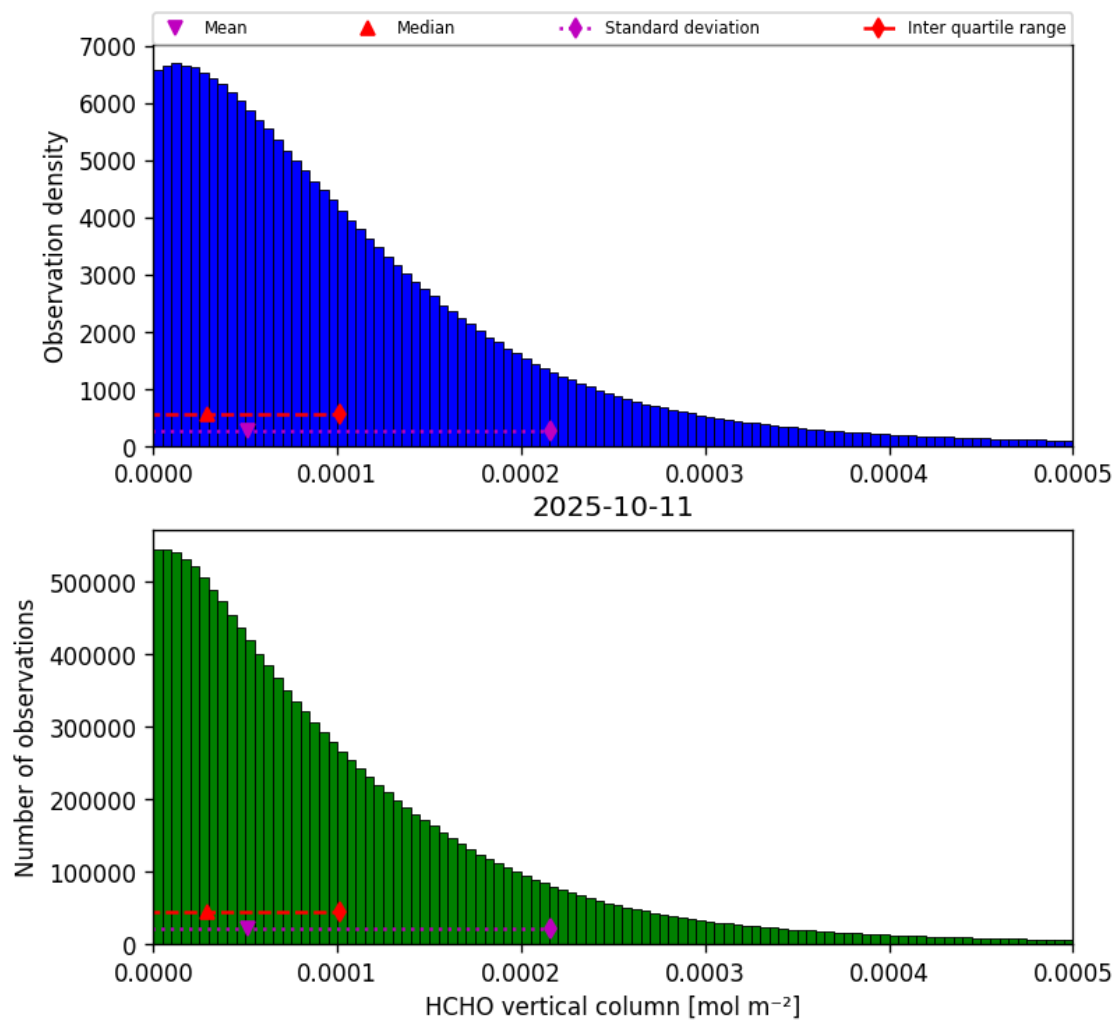
Figure 33: Histogram of “HCHO vertical column” for 2025-10-11 to 2025-10-12
