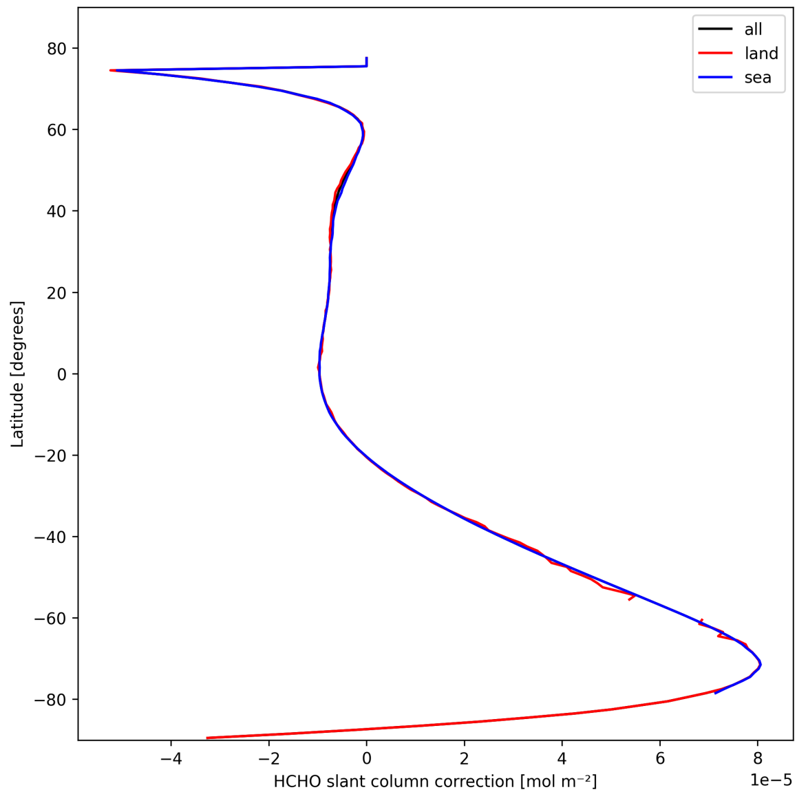
Figure 31: Zonal average of “HCHO slant column correction” for 2025-10-11 to 2025-10-12.
