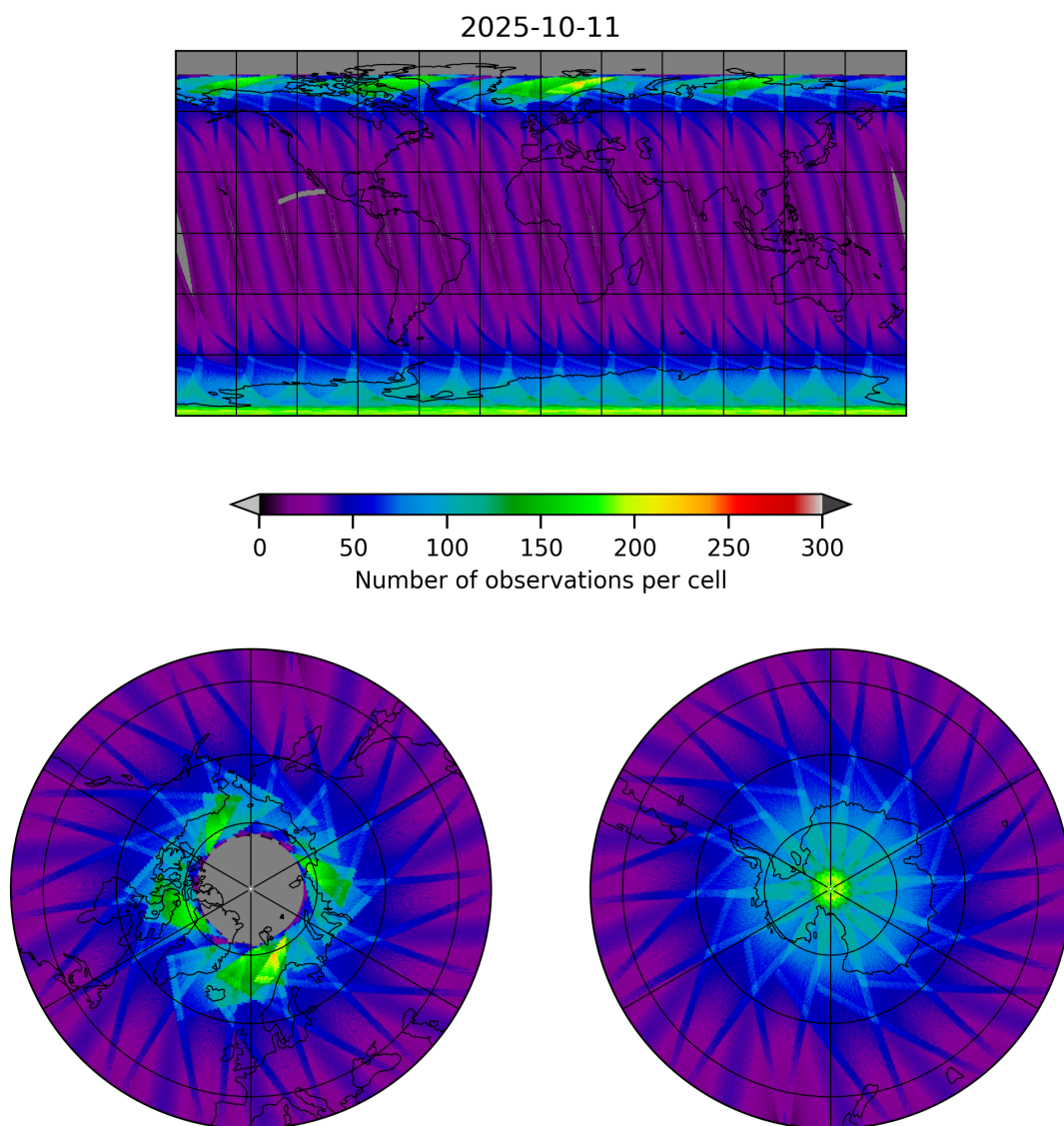
Figure 17: Map of the number of observations for 2025-10-11 to 2025-10-12
