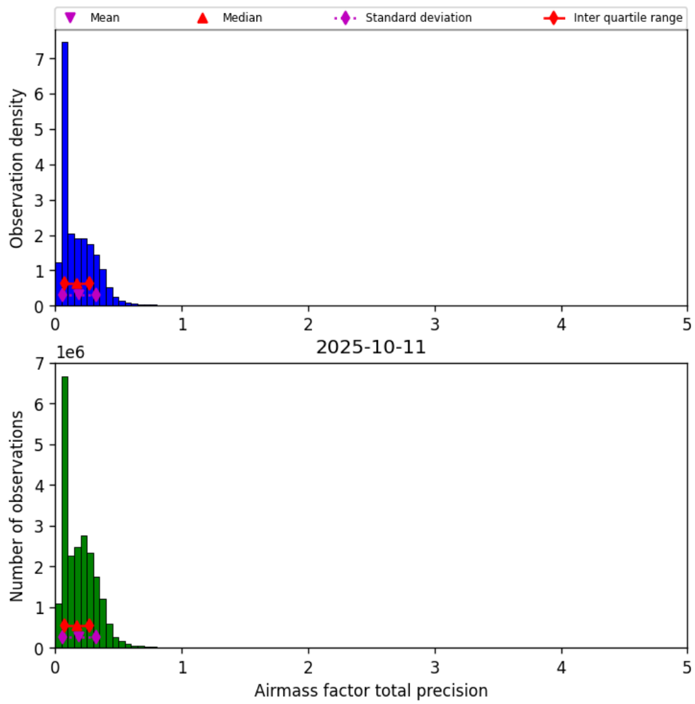
Figure 39: Histogram of “Airmass factor total precision” for 2025-10-11 to 2025-10-12
