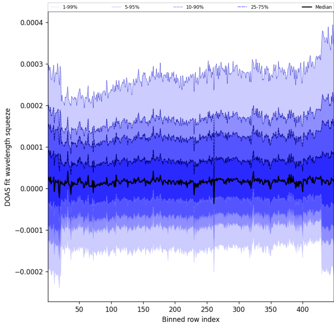
Figure 57: Along track statistics of “DOAS fit wavelength squeeze” for 2025-10-11 to 2025-10-12
