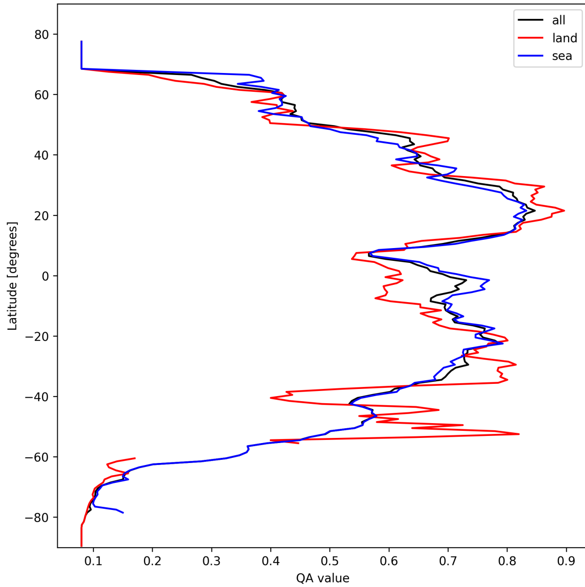
Figure 18: Zonal average of “QA value” for 2025-10-11 to 2025-10-12.
