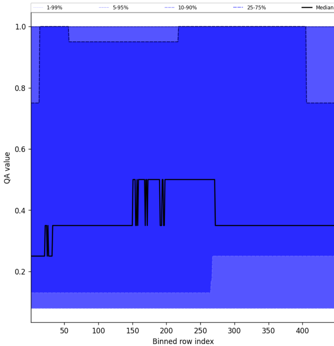
Figure 46: Along track statistics of “QA value” for 2025-10-11 to 2025-10-12
