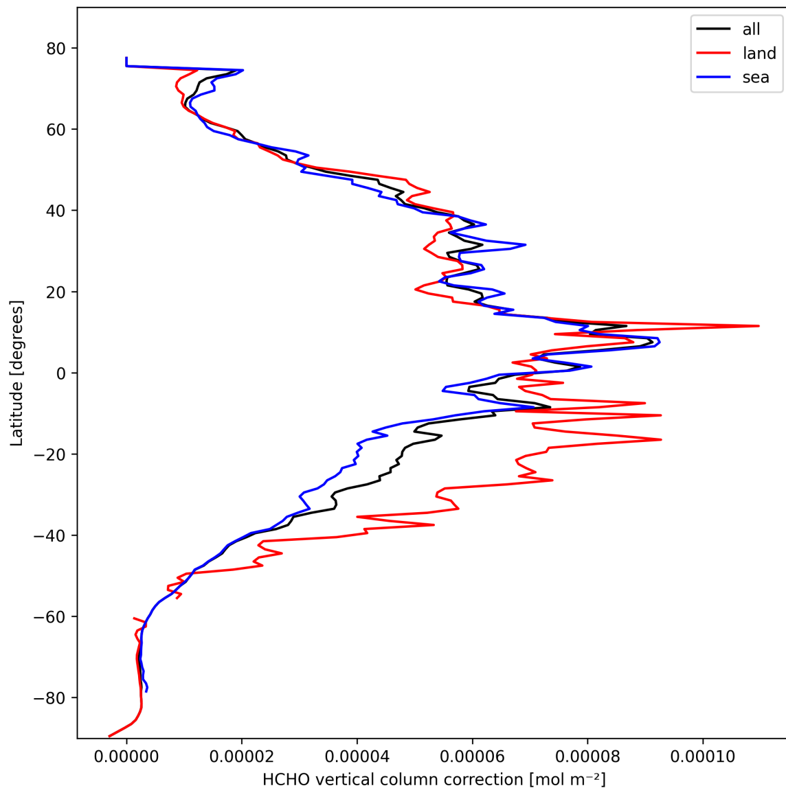
Figure 21: Zonal average of “HCHO vertical column correction” for 2025-10-11 to 2025-10-12.
