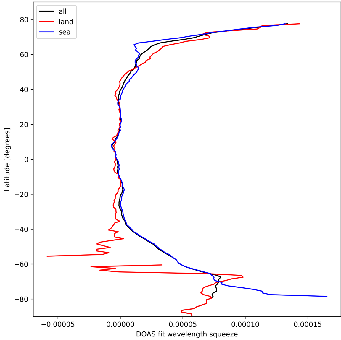
Figure 29: Zonal average of “DOAS fit wavelength squeeze” for 2025-10-11 to 2025-10-12.
