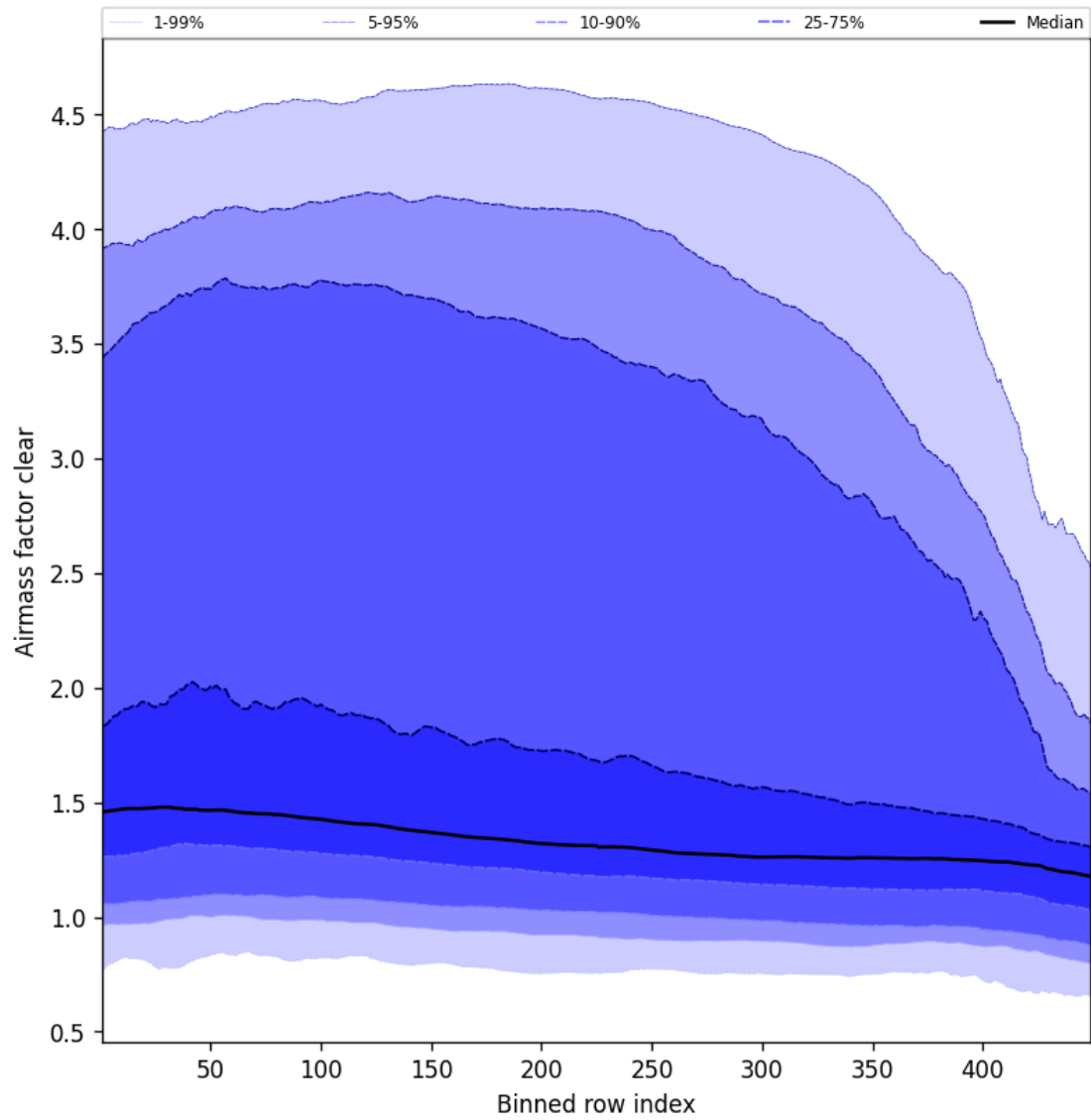
Figure 54: Along track statistics of “Airmass factor clear” for 2025-10-11 to 2025-10-12
