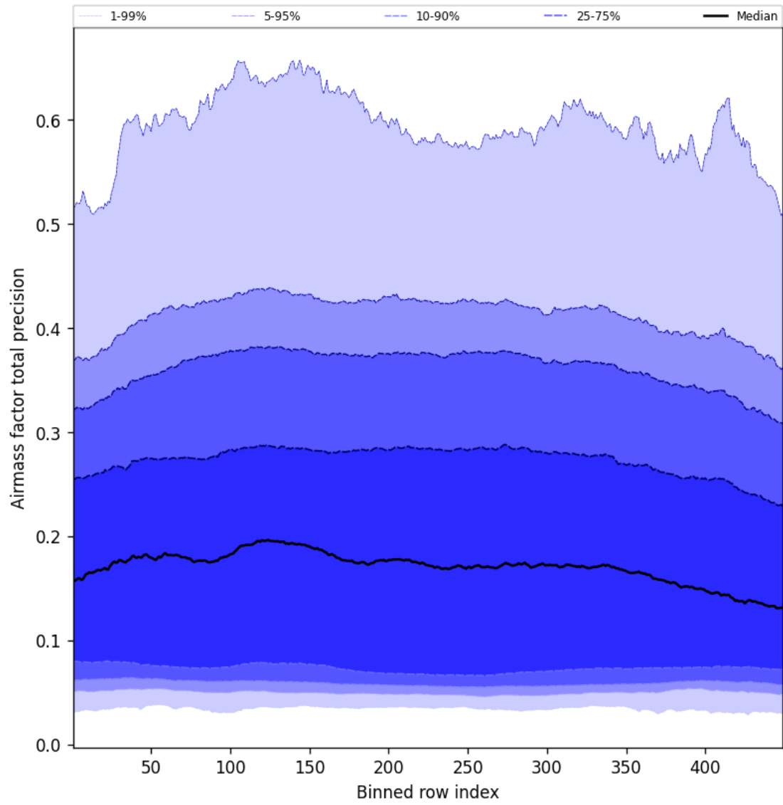
Figure 53: Along track statistics of “Airmass factor total precision” for 2025-10-11 to 2025-10-12
