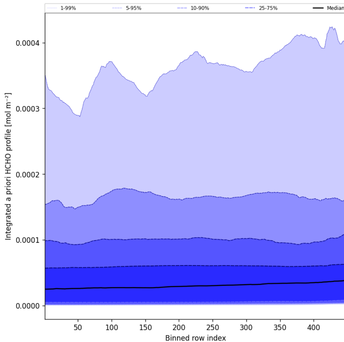
Figure 55: Along track statistics of “Integrated a priori HCHO profile” for 2025-10-11 to 2025-10-12
