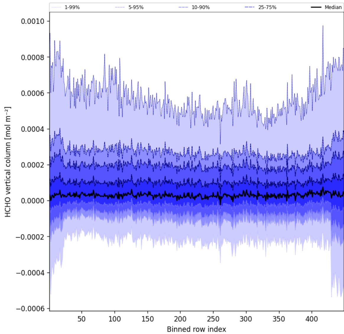
Figure 47: Along track statistics of “HCHO vertical column” for 2025-10-11 to 2025-10-12
