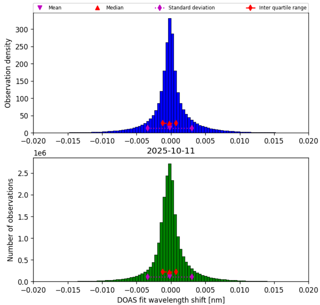
Figure 42: Histogram of “DOAS fit wavelength shift” for 2025-10-11 to 2025-10-12
