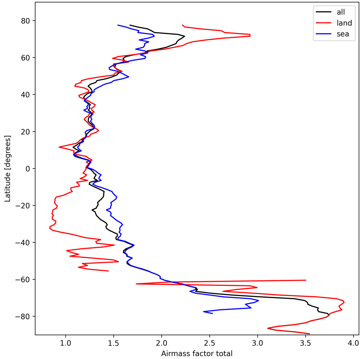
Figure 24: Zonal average of “Airmass factor total” for 2025-10-11 to 2025-10-12.
