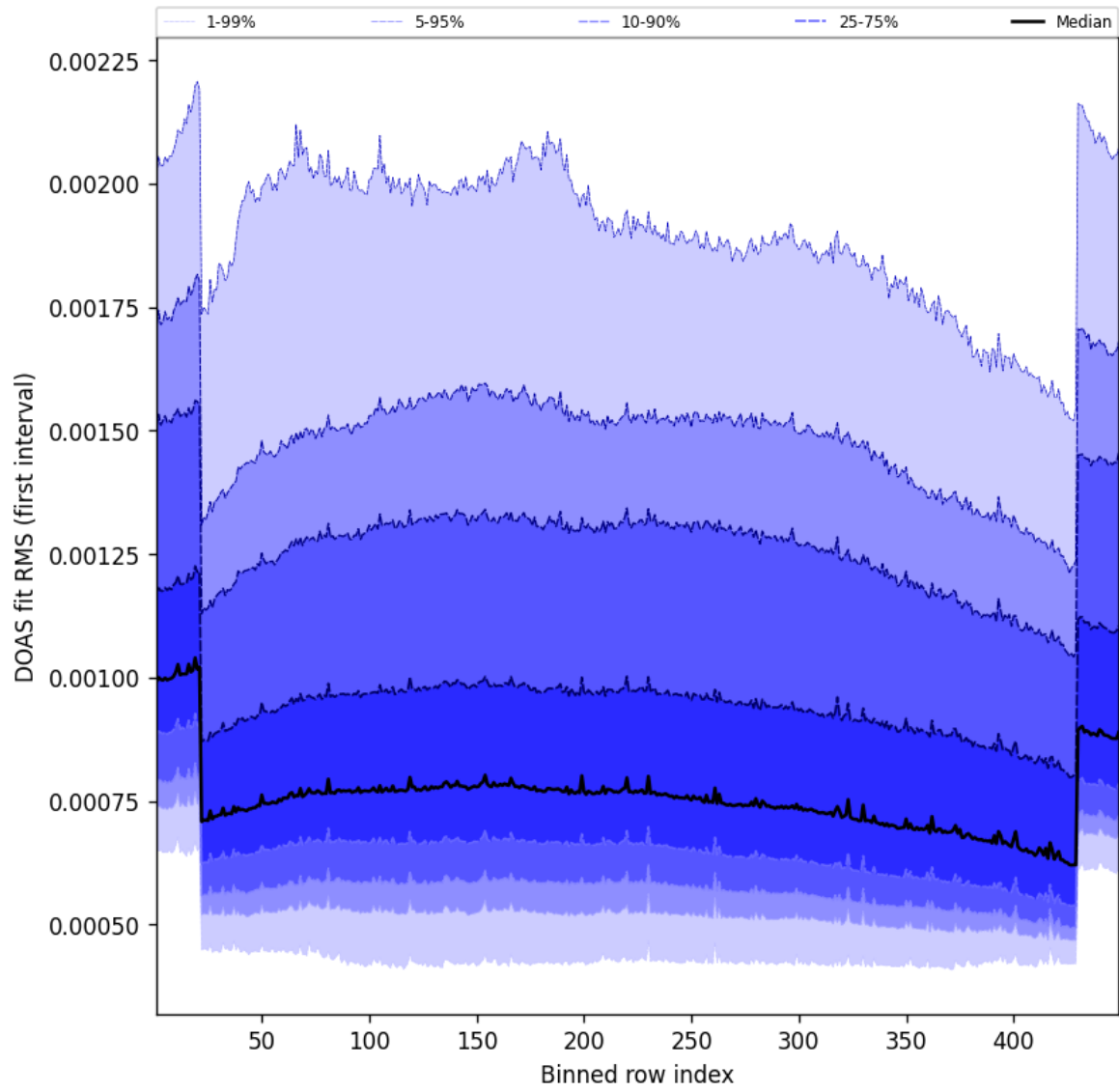
Figure 58: Along track statistics of “DOAS fit RMS (first interval)” for 2025-10-11 to 2025-10-12
