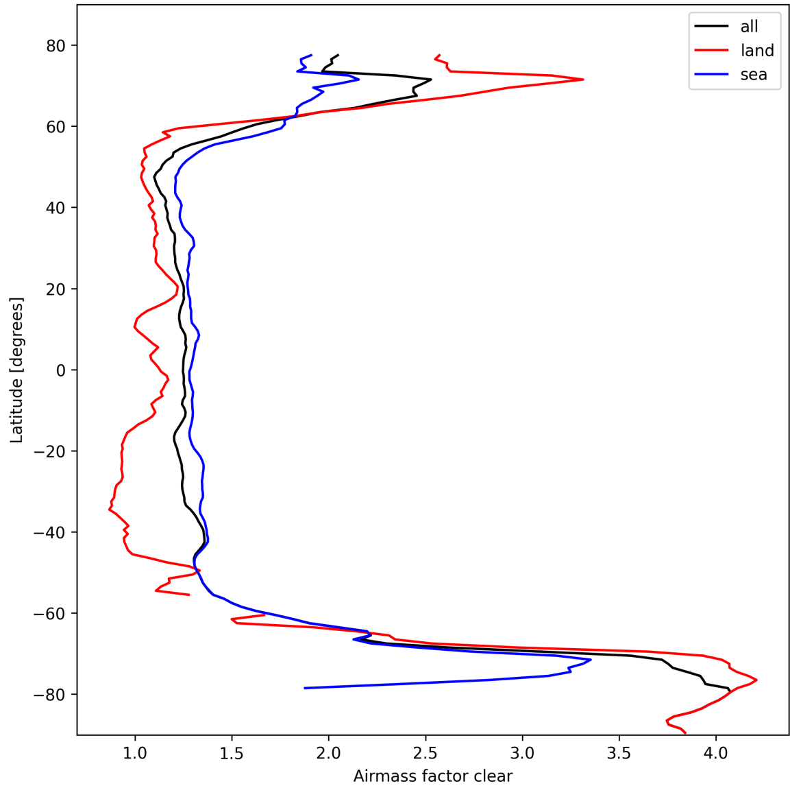
Figure 26: Zonal average of “Airmass factor clear” for 2025-10-11 to 2025-10-12.
