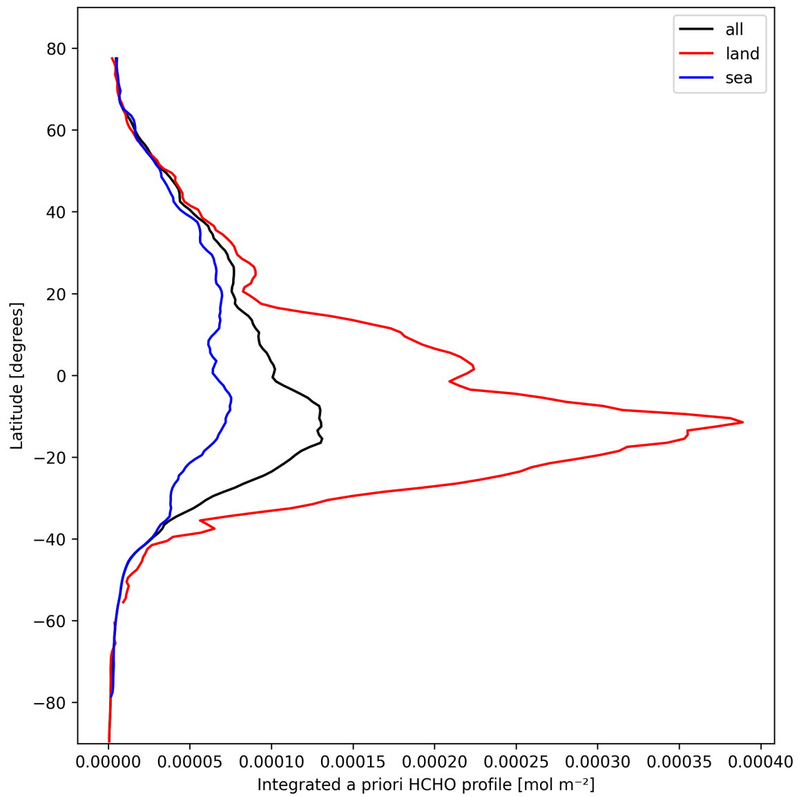
Figure 27: Zonal average of “Integrated a priori HCHO profile” for 2025-10-11 to 2025-10-12.
