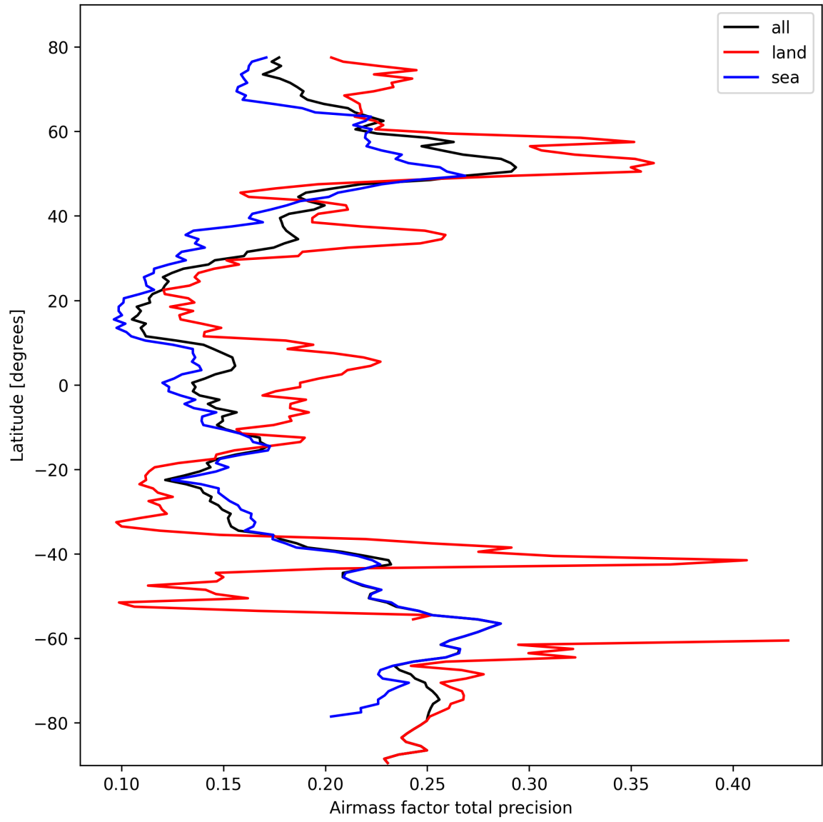
Figure 25: Zonal average of “Airmass factor total precision” for 2025-10-11 to 2025-10-12.
