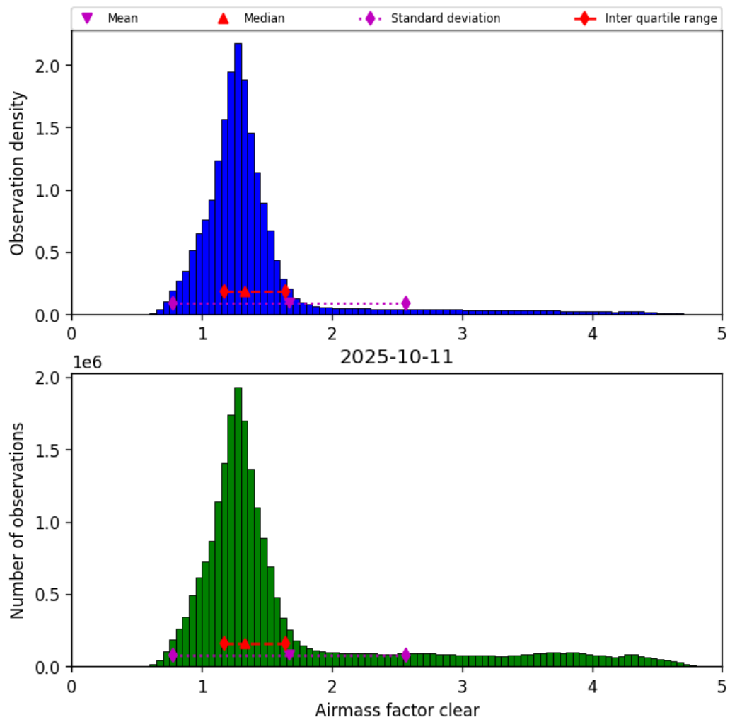
Figure 40: Histogram of “Airmass factor clear” for 2025-10-11 to 2025-10-12
