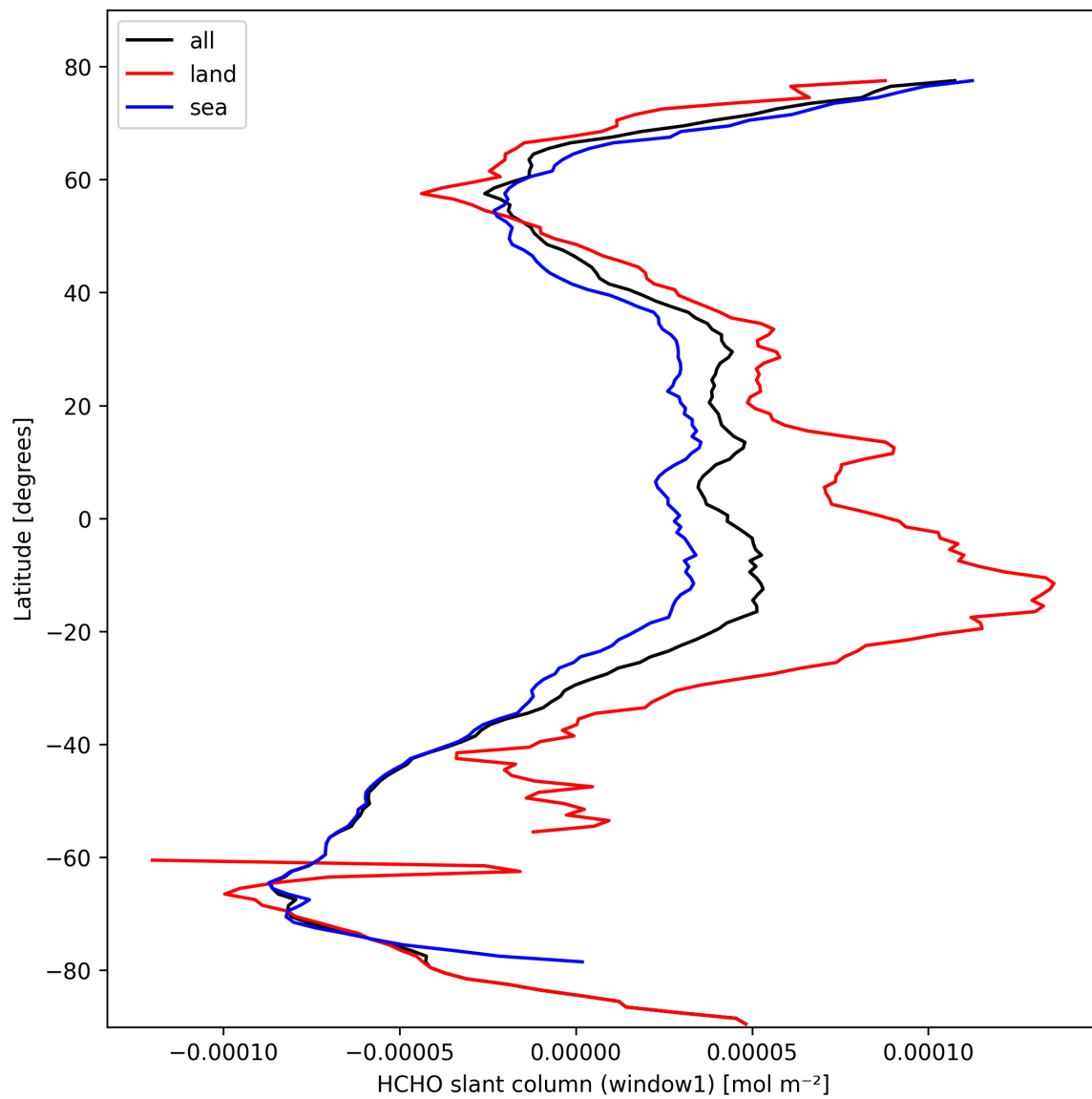
Figure 22: Zonal average of “HCHO slant column (window1)” for 2025-10-11 to 2025-10-12.
