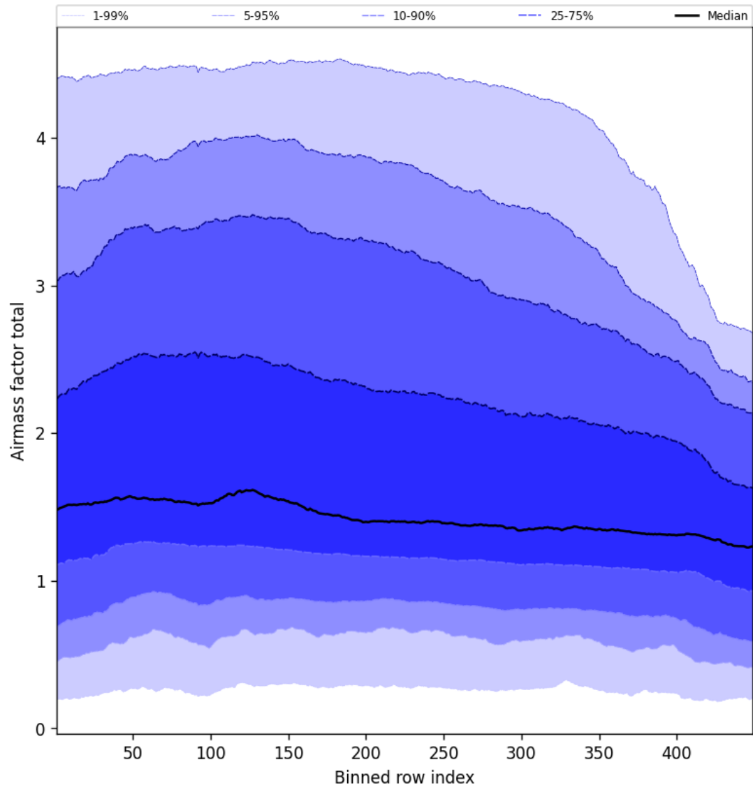
Figure 52: Along track statistics of “Airmass factor total” for 2025-10-11 to 2025-10-12
