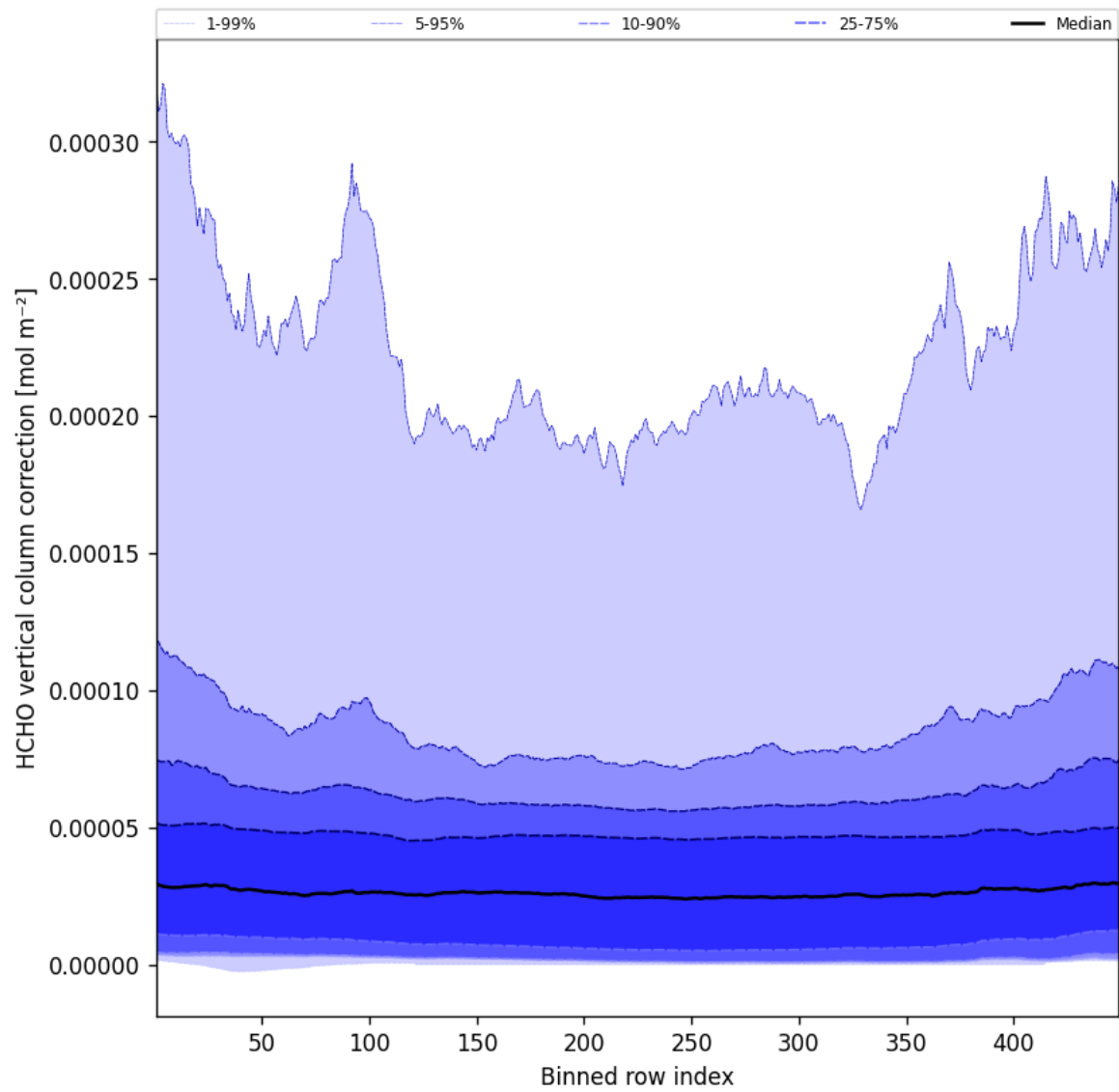
Figure 49: Along track statistics of “HCHO vertical column correction” for 2025-10-11 to 2025-10-12
