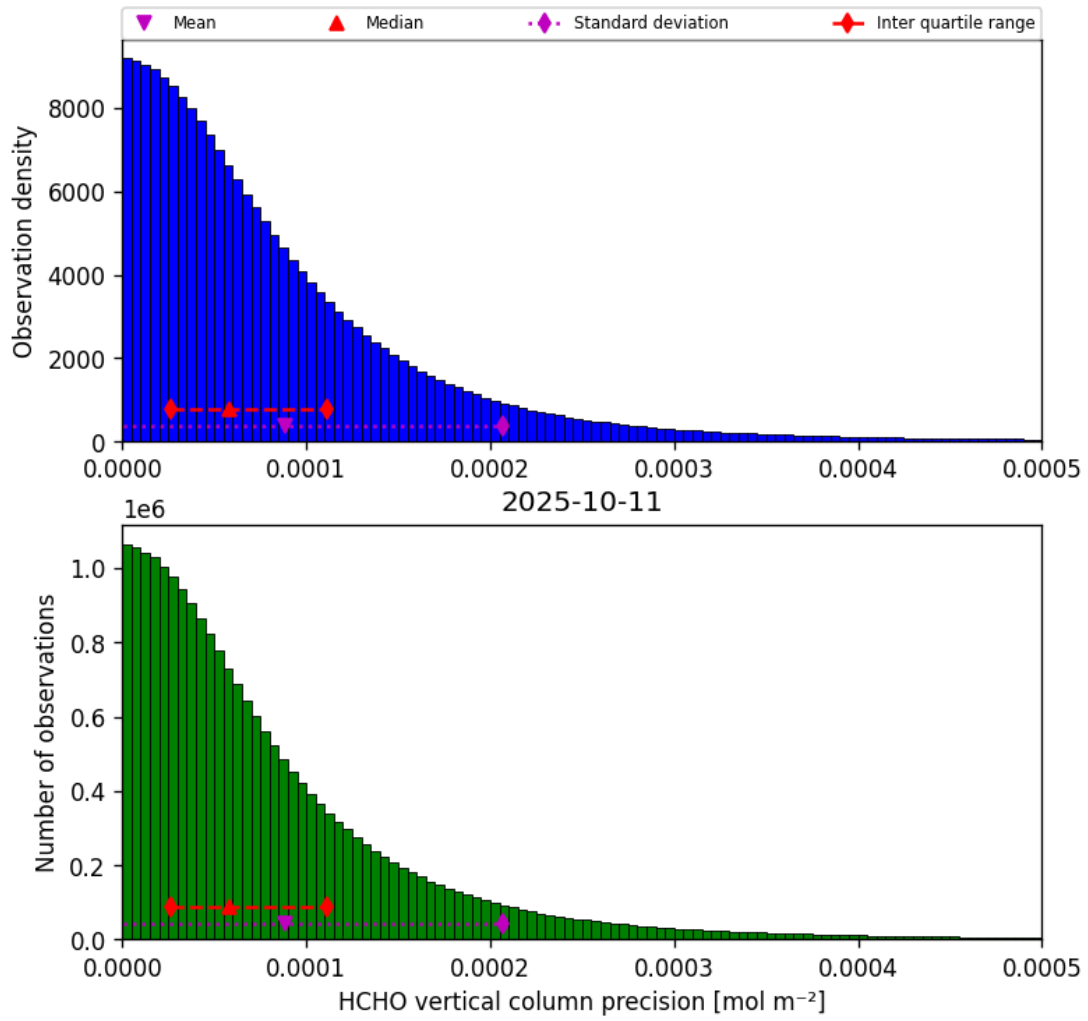
Figure 34: Histogram of “HCHO vertical column precision” for 2025-10-11 to 2025-10-12
