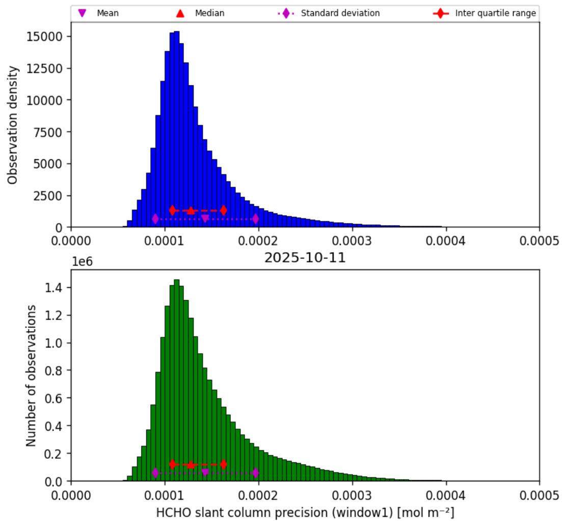
Figure 37: Histogram of “HCHO slant column precision (window1)” for 2025-10-11 to 2025-10-12
