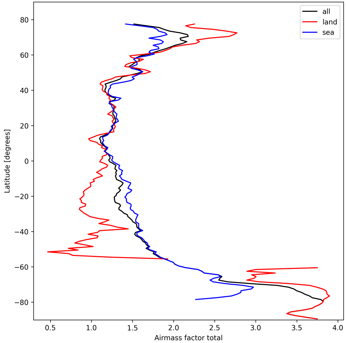
Figure 24: Zonal average of “Airmass factor total” for 2025-10-12 to 2025-10-13.
