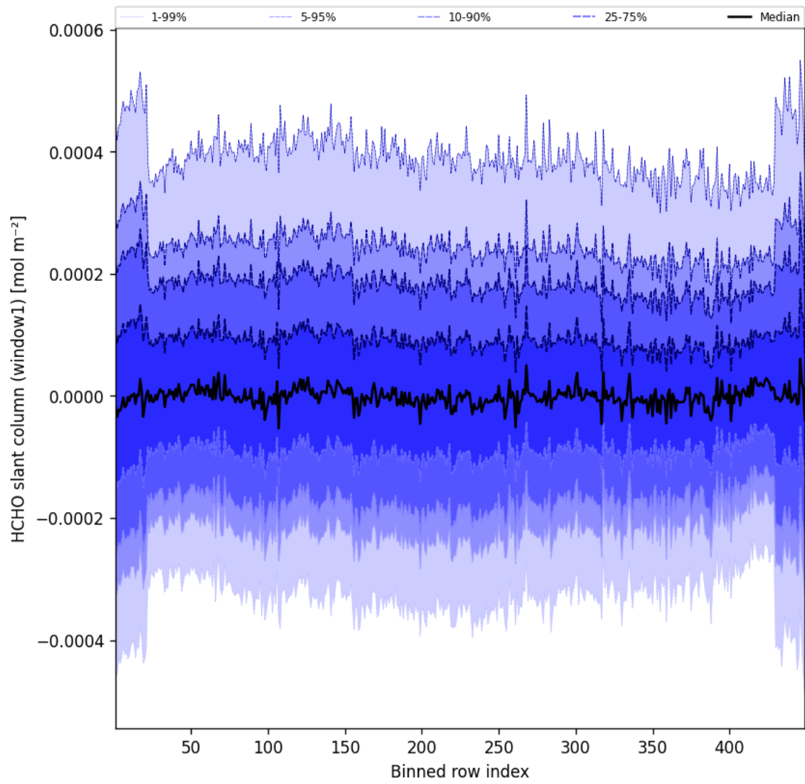
Figure 50: Along track statistics of “HCHO slant column (window1)” for 2025-10-12 to 2025-10-13
