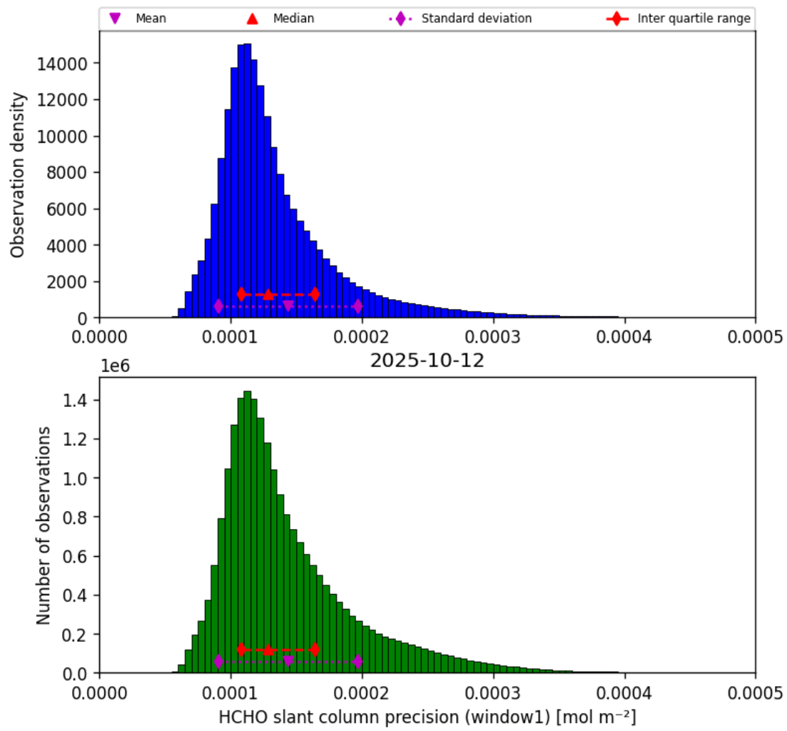
Figure 37: Histogram of “HCHO slant column precision (window1)” for 2025-10-12 to 2025-10-13
