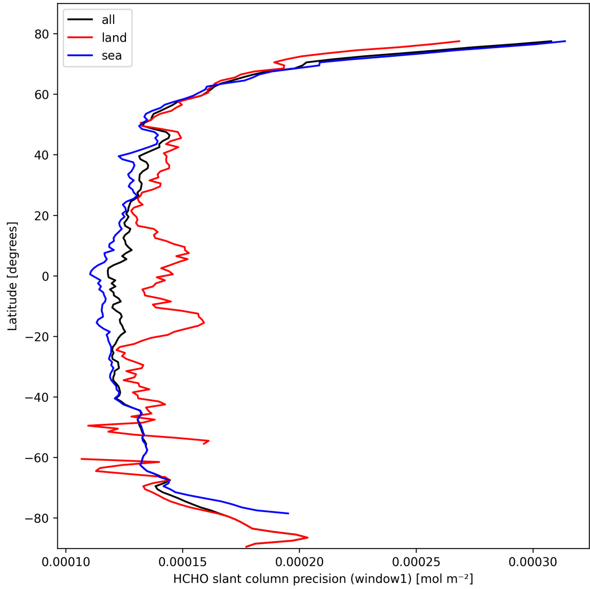
Figure 23: Zonal average of “HCHO slant column precision (window1)” for 2025-10-12 to 2025-10-13.
