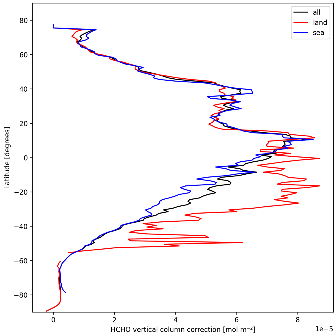
Figure 21: Zonal average of “HCHO vertical column correction” for 2025-10-12 to 2025-10-13.
