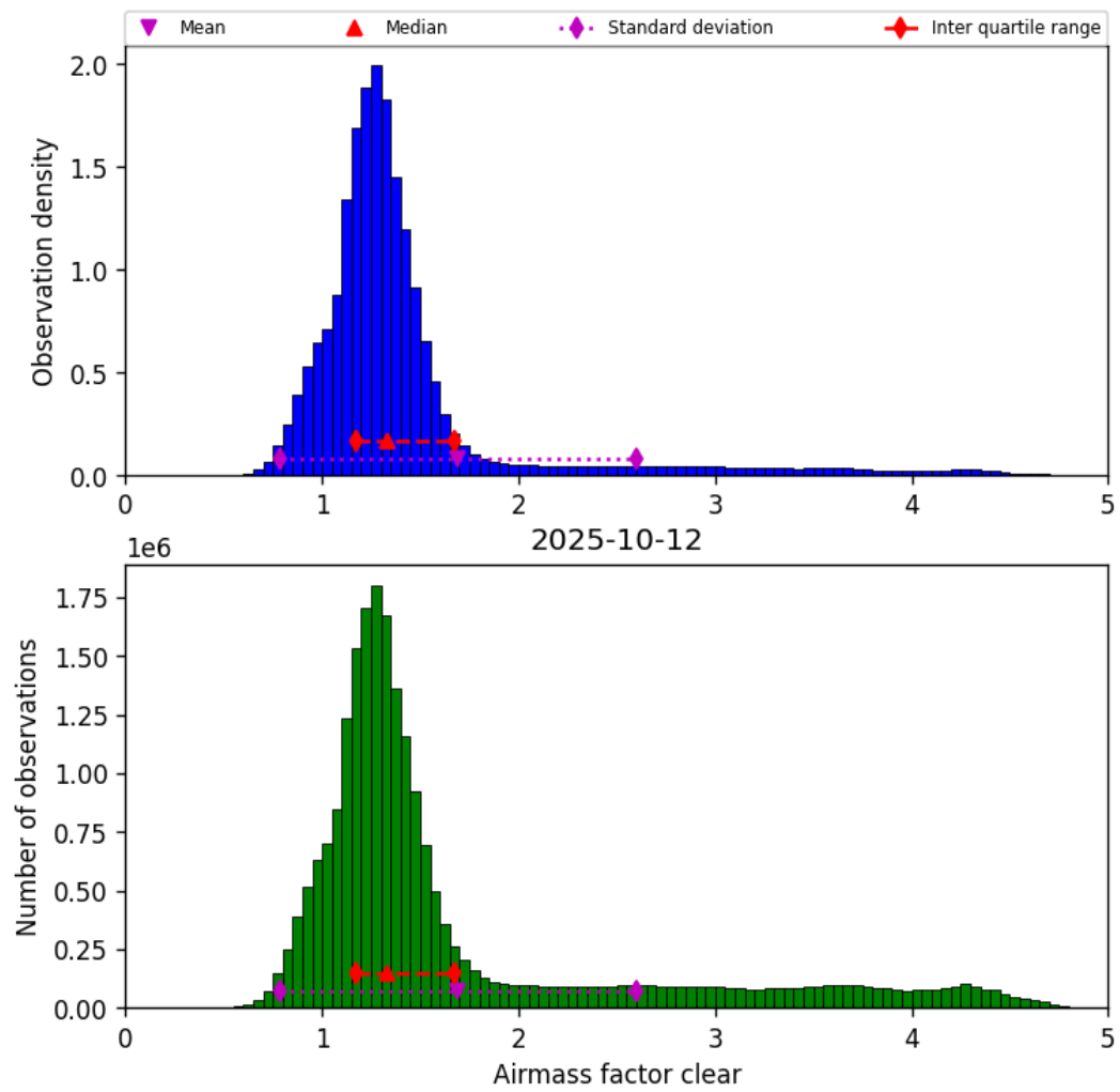
Figure 40: Histogram of “Airmass factor clear” for 2025-10-12 to 2025-10-13
