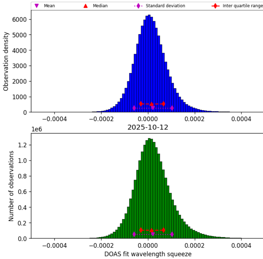
Figure 43: Histogram of “DOAS fit wavelength squeeze” for 2025-10-12 to 2025-10-13
