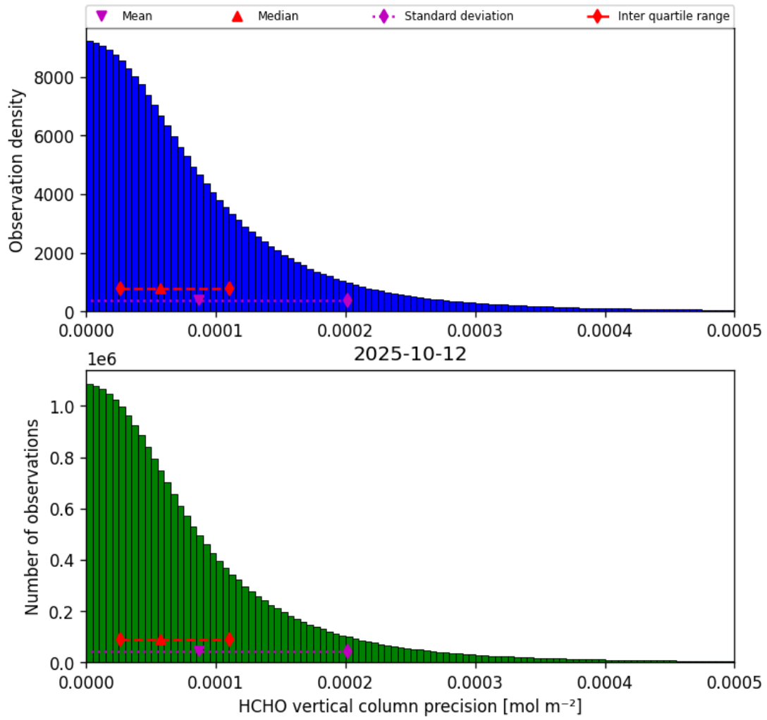
Figure 34: Histogram of “HCHO vertical column precision” for 2025-10-12 to 2025-10-13
