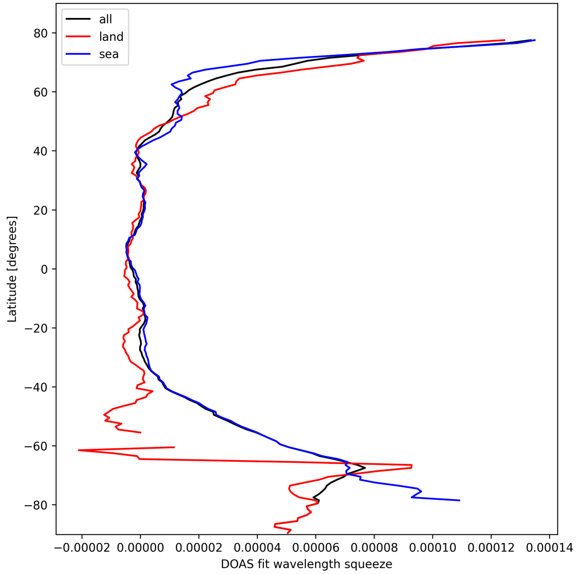
Figure 29: Zonal average of “DOAS fit wavelength squeeze” for 2025-10-12 to 2025-10-13.
