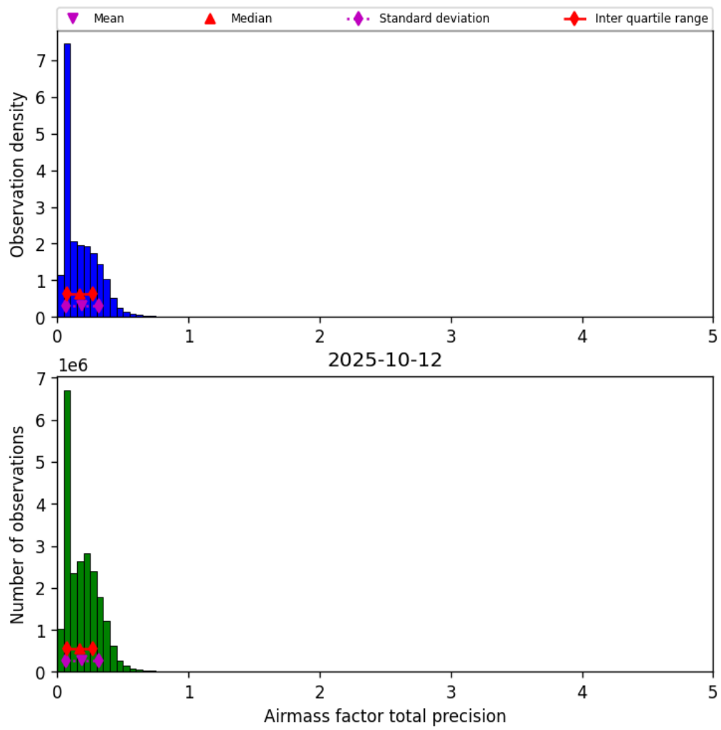
Figure 39: Histogram of “Airmass factor total precision” for 2025-10-12 to 2025-10-13
