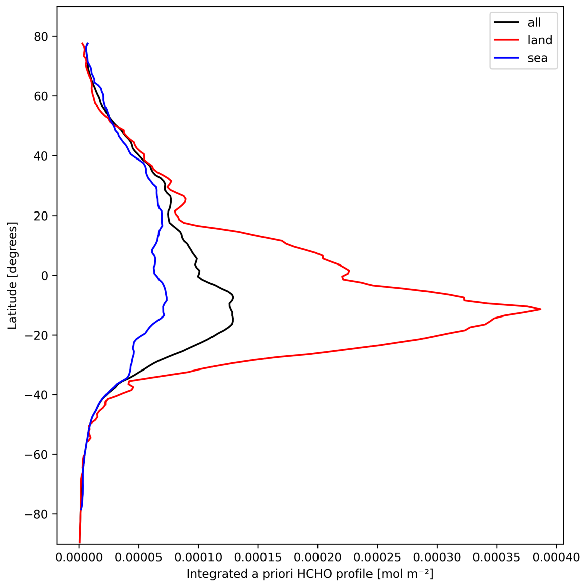
Figure 27: Zonal average of “Integrated a priori HCHO profile” for 2025-10-12 to 2025-10-13.
