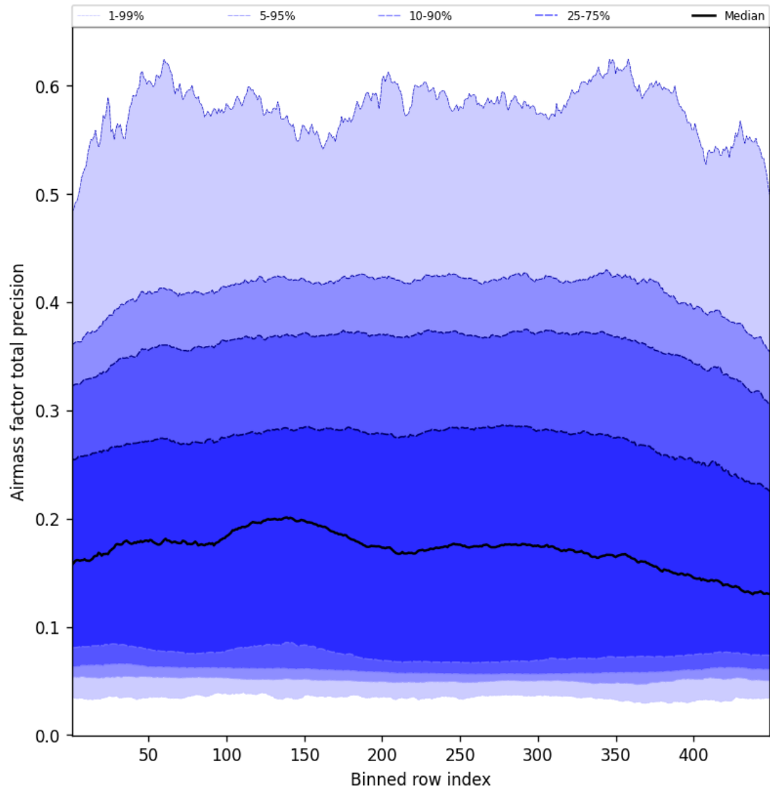
Figure 53: Along track statistics of “Airmass factor total precision” for 2025-10-12 to 2025-10-13
