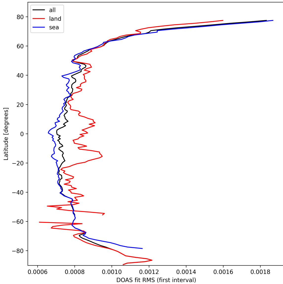
Figure 30: Zonal average of “DOAS fit RMS (first interval)” for 2025-10-12 to 2025-10-13.
