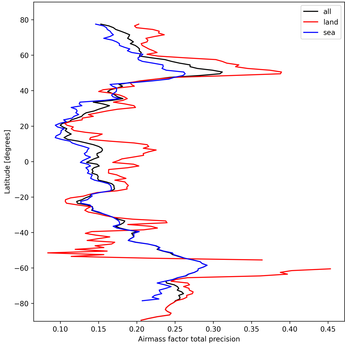
Figure 25: Zonal average of “Airmass factor total precision” for 2025-10-12 to 2025-10-13.
