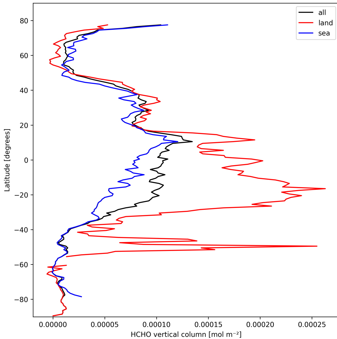
Figure 19: Zonal average of “HCHO vertical column” for 2025-10-12 to 2025-10-13.
