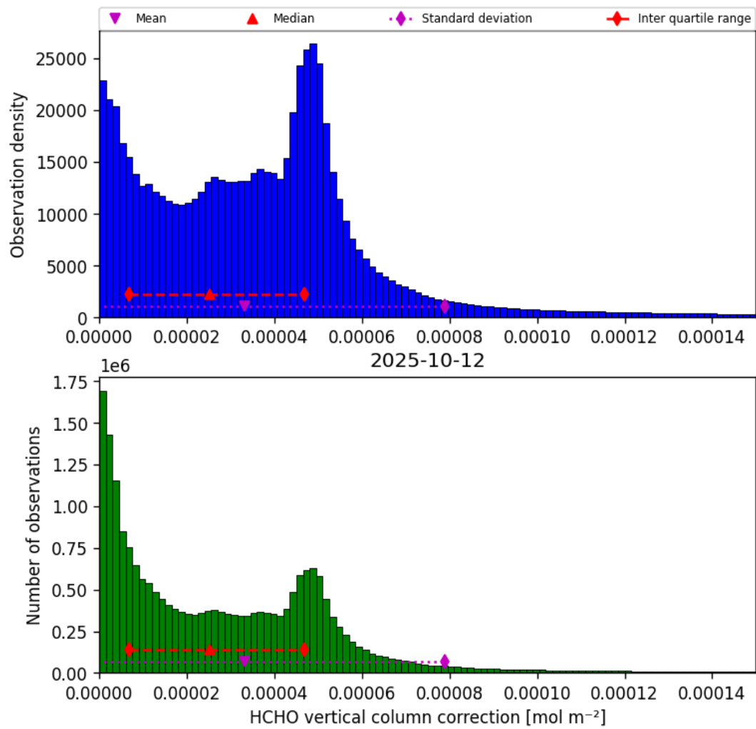
Figure 35: Histogram of “HCHO vertical column correction” for 2025-10-12 to 2025-10-13
