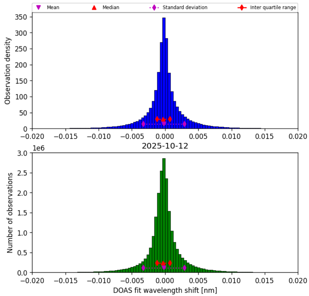
Figure 42: Histogram of “DOAS fit wavelength shift” for 2025-10-12 to 2025-10-13
