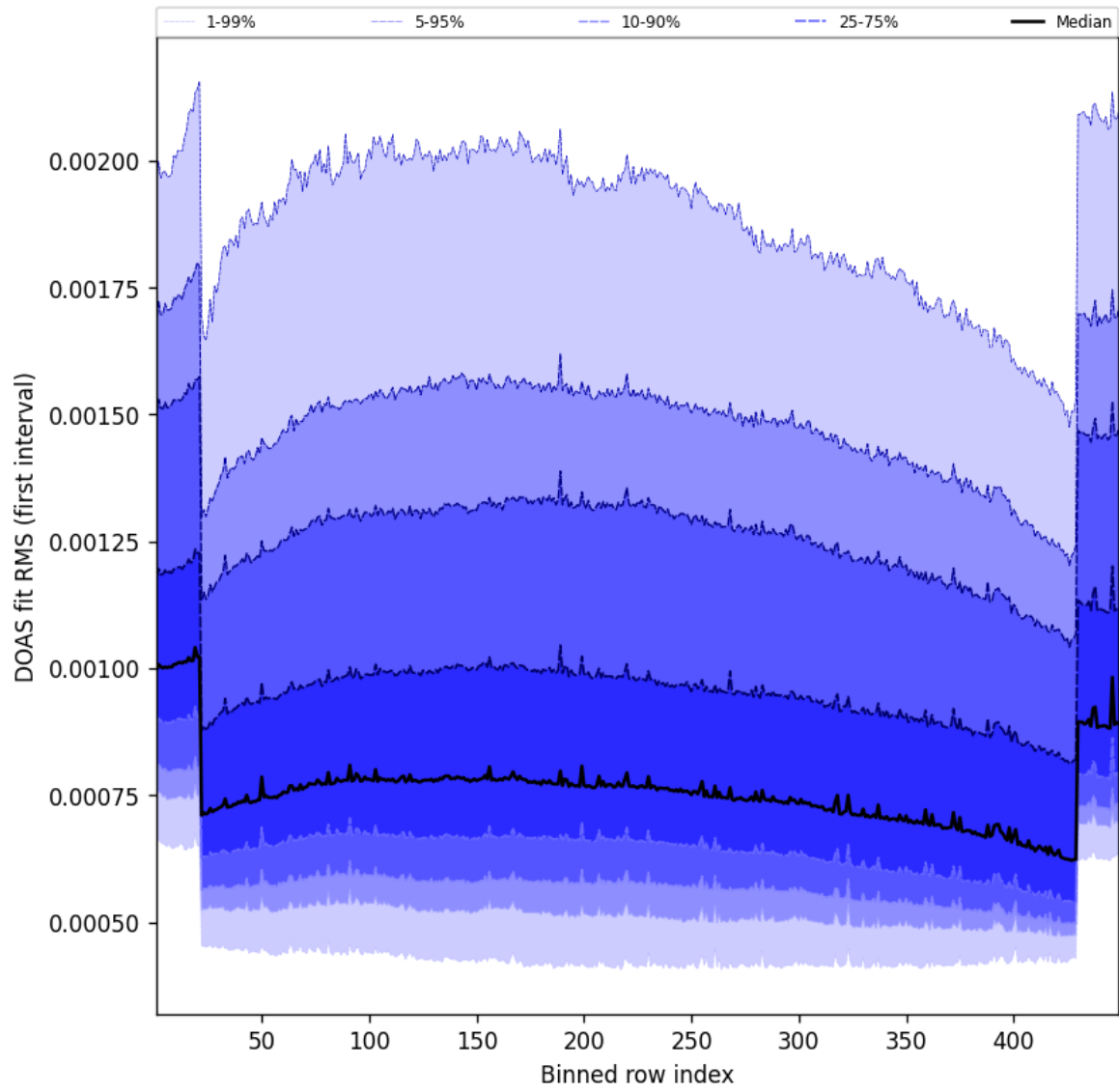
Figure 58: Along track statistics of “DOAS fit RMS (first interval)” for 2025-10-12 to 2025-10-13
