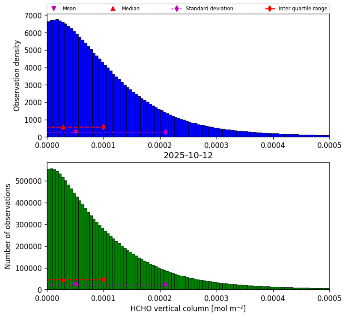
Figure 33: Histogram of “HCHO vertical column” for 2025-10-12 to 2025-10-13
