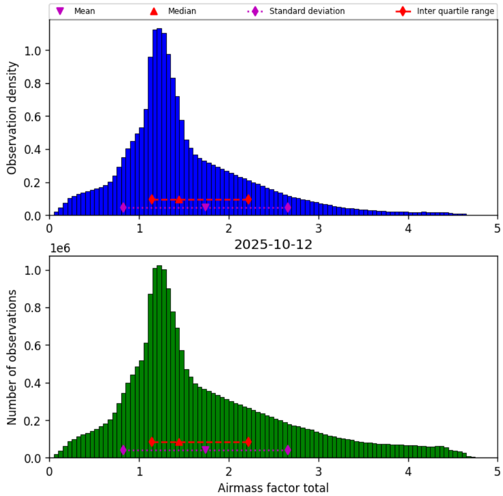
Figure 38: Histogram of “Airmass factor total” for 2025-10-12 to 2025-10-13
