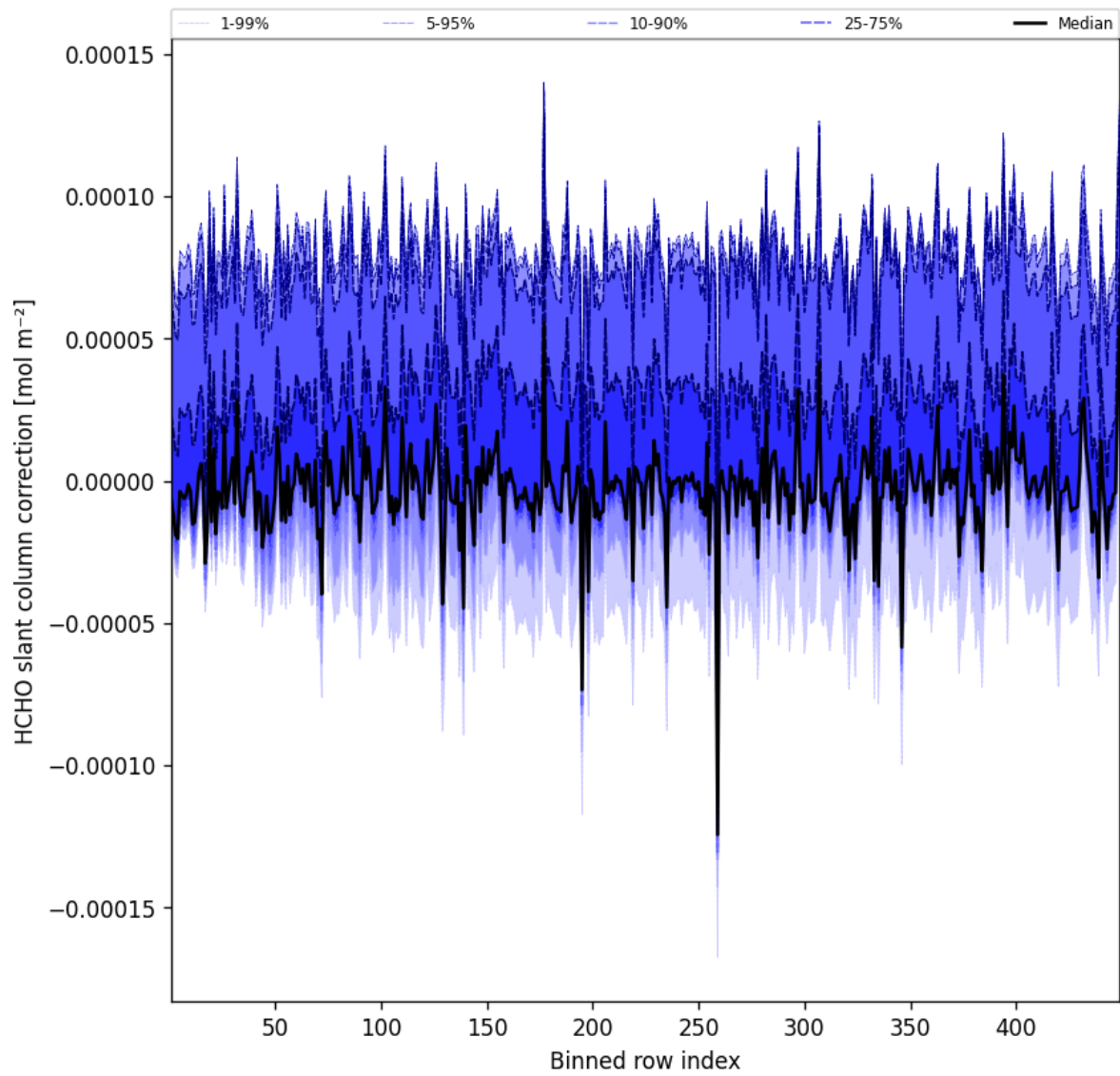
Figure 59: Along track statistics of “HCHO slant column correction” for 2025-10-12 to 2025-10-13
