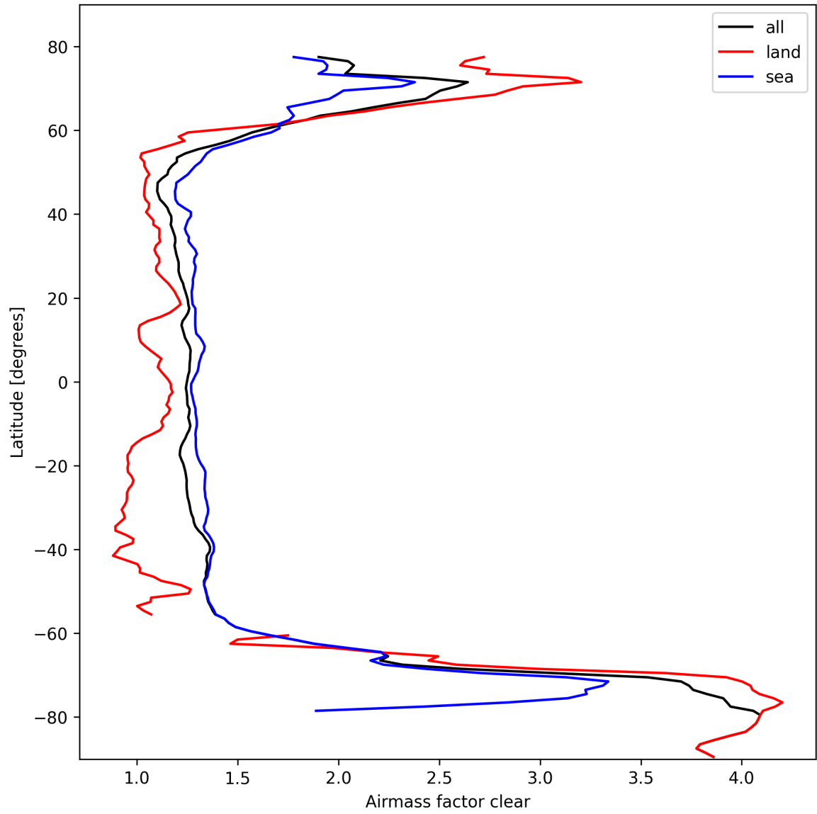
Figure 26: Zonal average of “Airmass factor clear” for 2025-10-12 to 2025-10-13.
