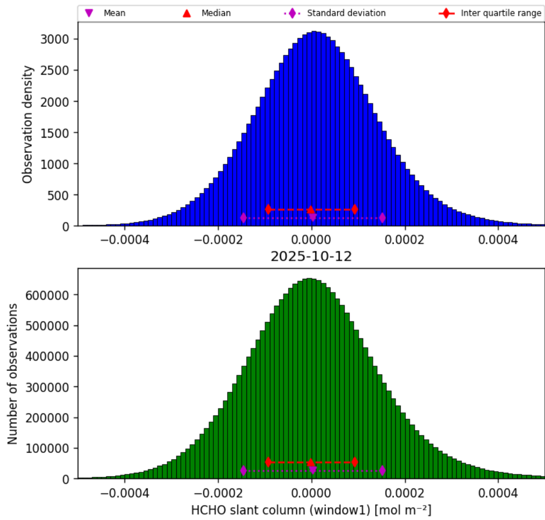
Figure 36: Histogram of “HCHO slant column (window1)” for 2025-10-12 to 2025-10-13
