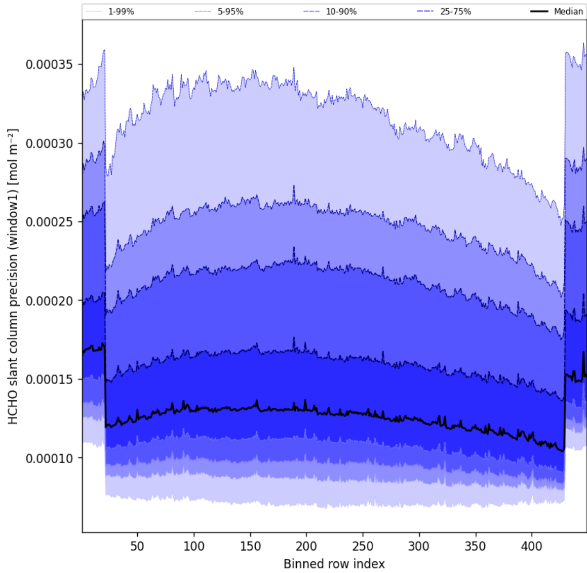
Figure 51: Along track statistics of “HCHO slant column precision (window1)” for 2025-10-12 to 2025-10-13
