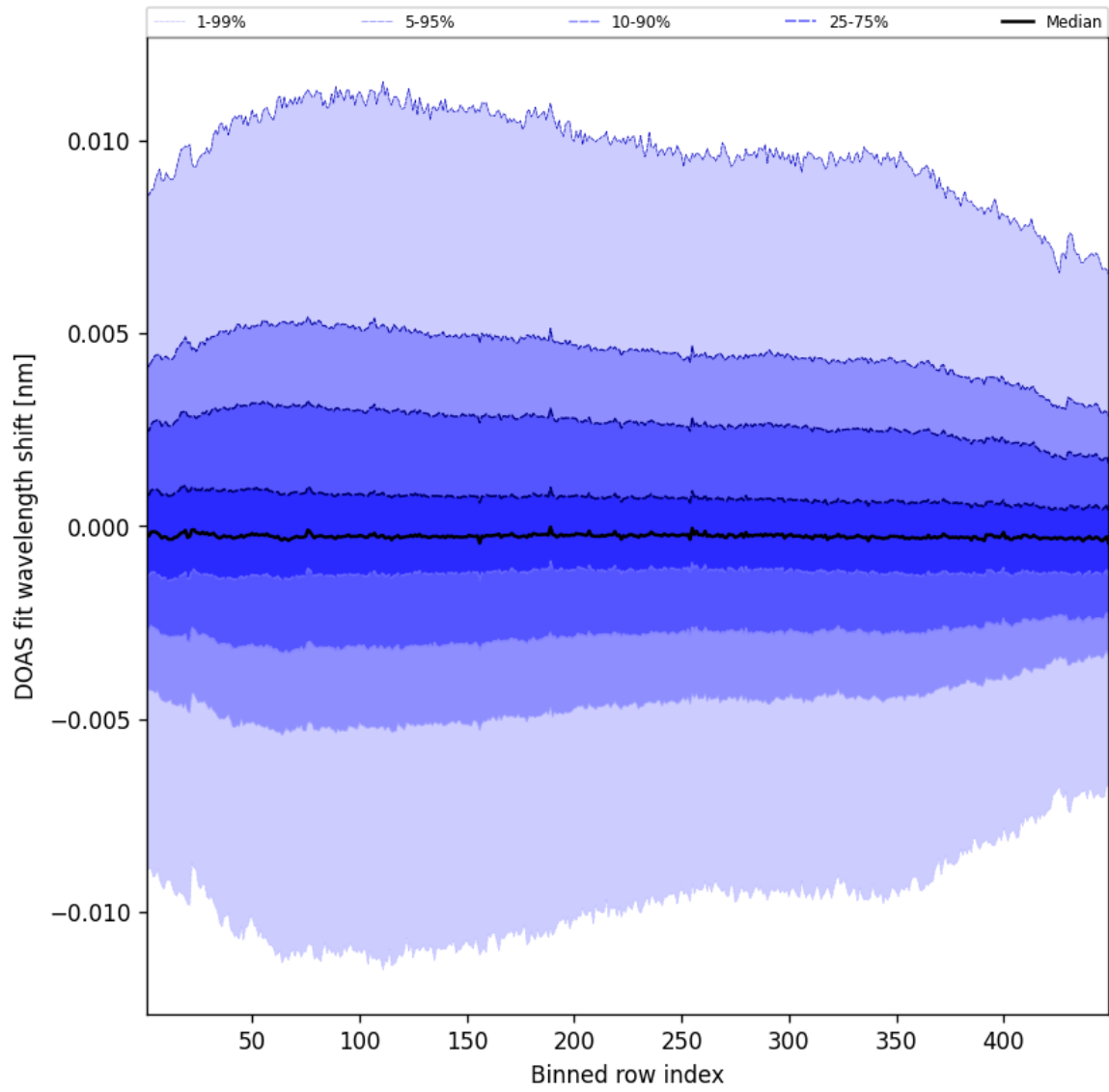
Figure 56: Along track statistics of “DOAS fit wavelength shift” for 2025-10-12 to 2025-10-13
