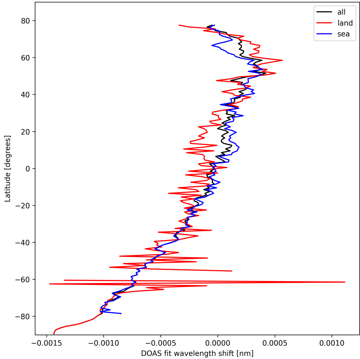
Figure 28: Zonal average of “DOAS fit wavelength shift” for 2025-10-12 to 2025-10-13.
