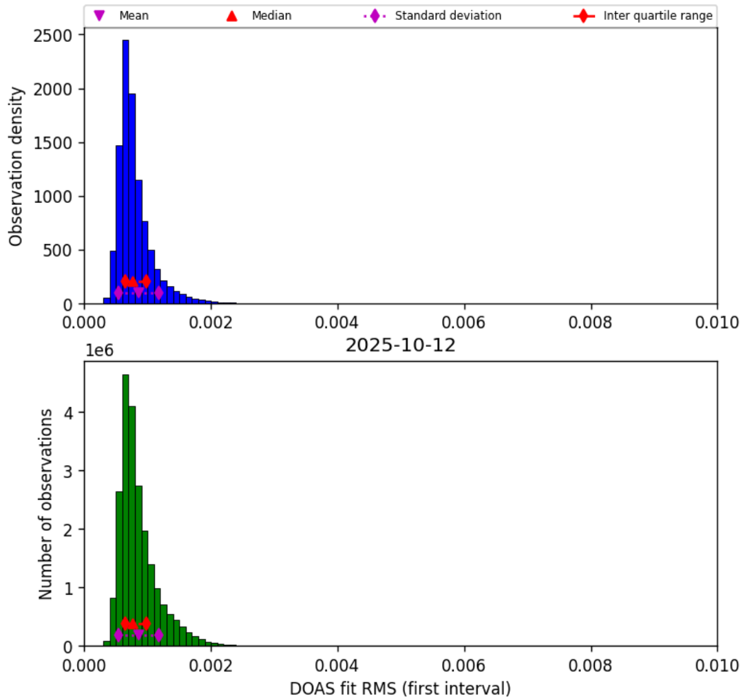
Figure 44: Histogram of “DOAS fit RMS (first interval)” for 2025-10-12 to 2025-10-13
