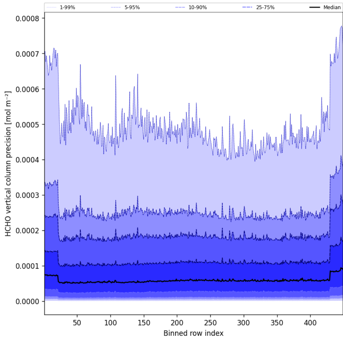
Figure 48: Along track statistics of “HCHO vertical column precision” for 2025-10-12 to 2025-10-13
