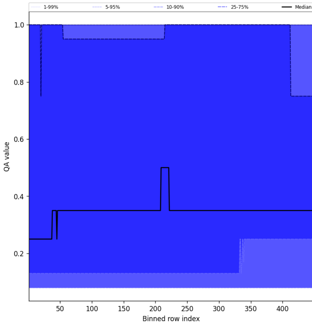
Figure 46: Along track statistics of “QA value” for 2025-10-12 to 2025-10-13
