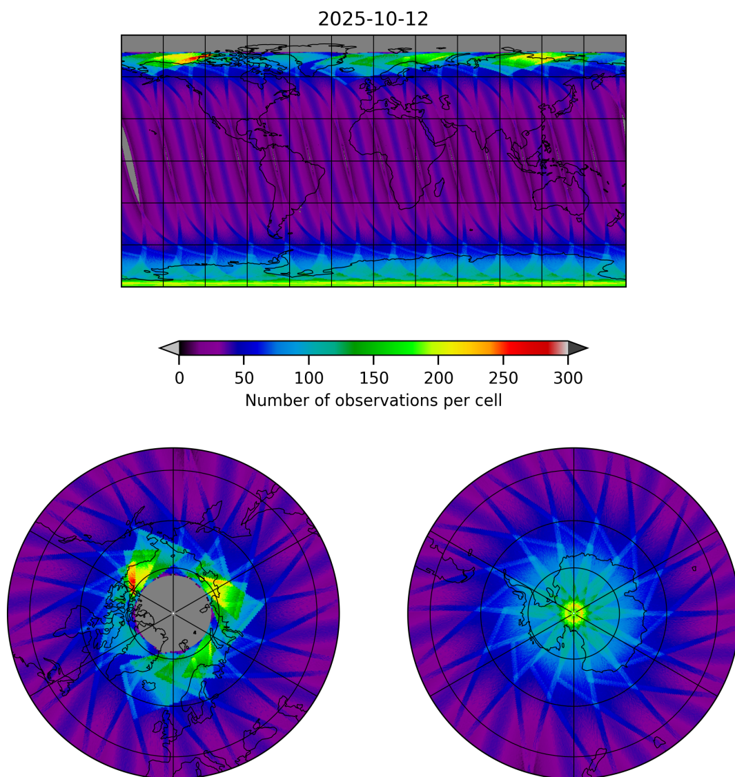
Figure 17: Map of the number of observations for 2025-10-12 to 2025-10-13
