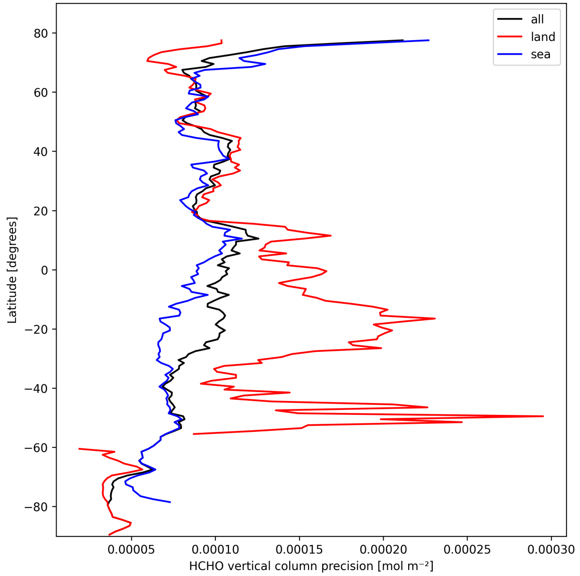
Figure 20: Zonal average of “HCHO vertical column precision” for 2025-10-12 to 2025-10-13.
