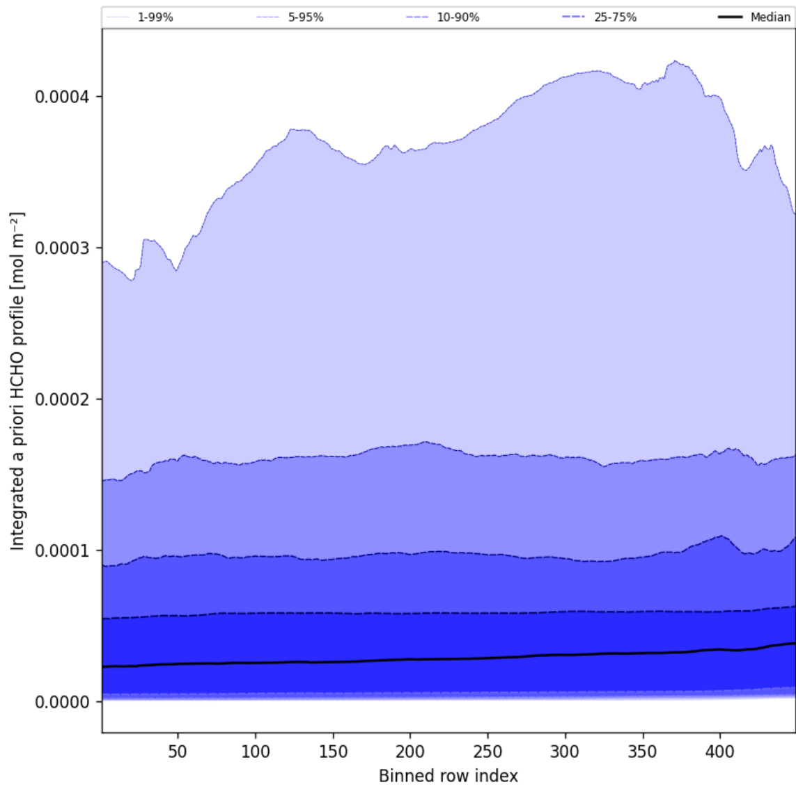
Figure 55: Along track statistics of "Integrated a priori HCHO profile" for 2025-10-12 to 2025-10-13
