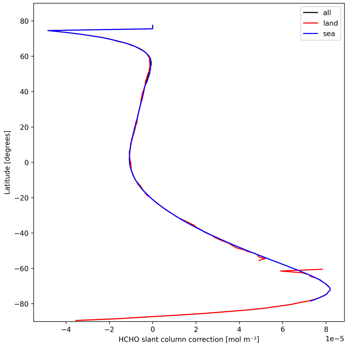
Figure 31: Zonal average of “HCHO slant column correction” for 2025-10-12 to 2025-10-13.
