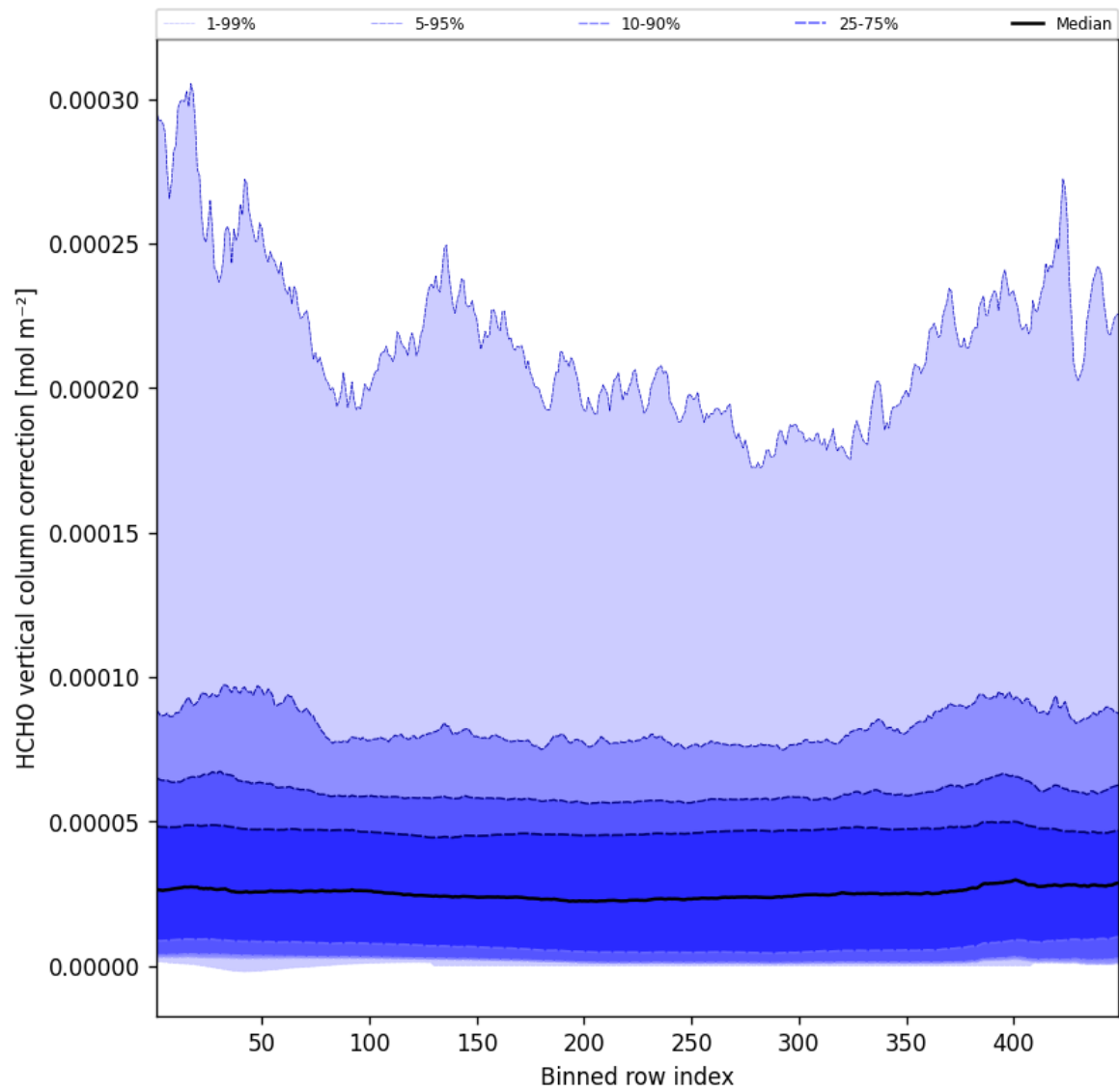
Figure 49: Along track statistics of “HCHO vertical column correction” for 2025-10-12 to 2025-10-13
