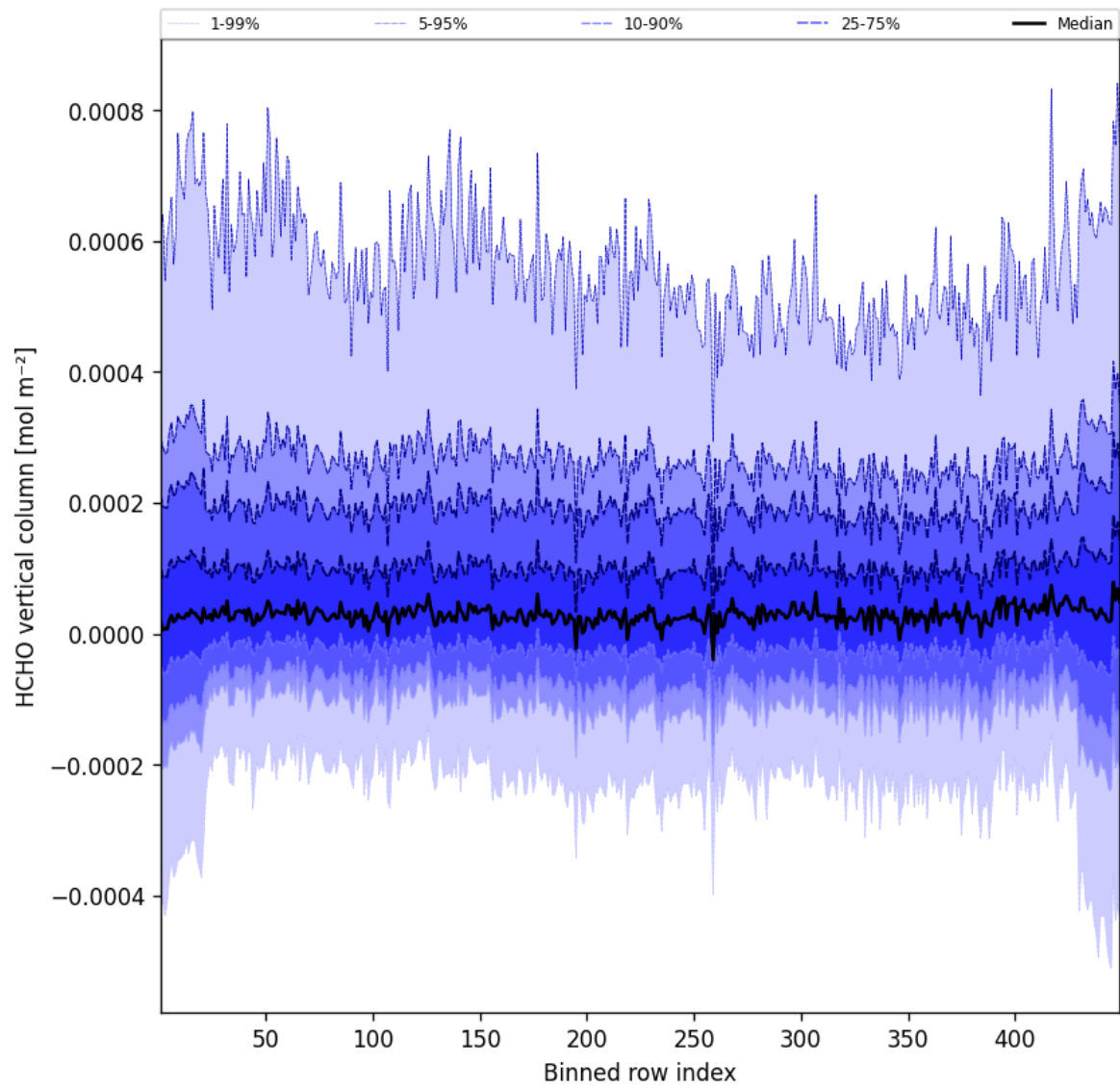
Figure 47: Along track statistics of “HCHO vertical column” for 2025-10-12 to 2025-10-13
