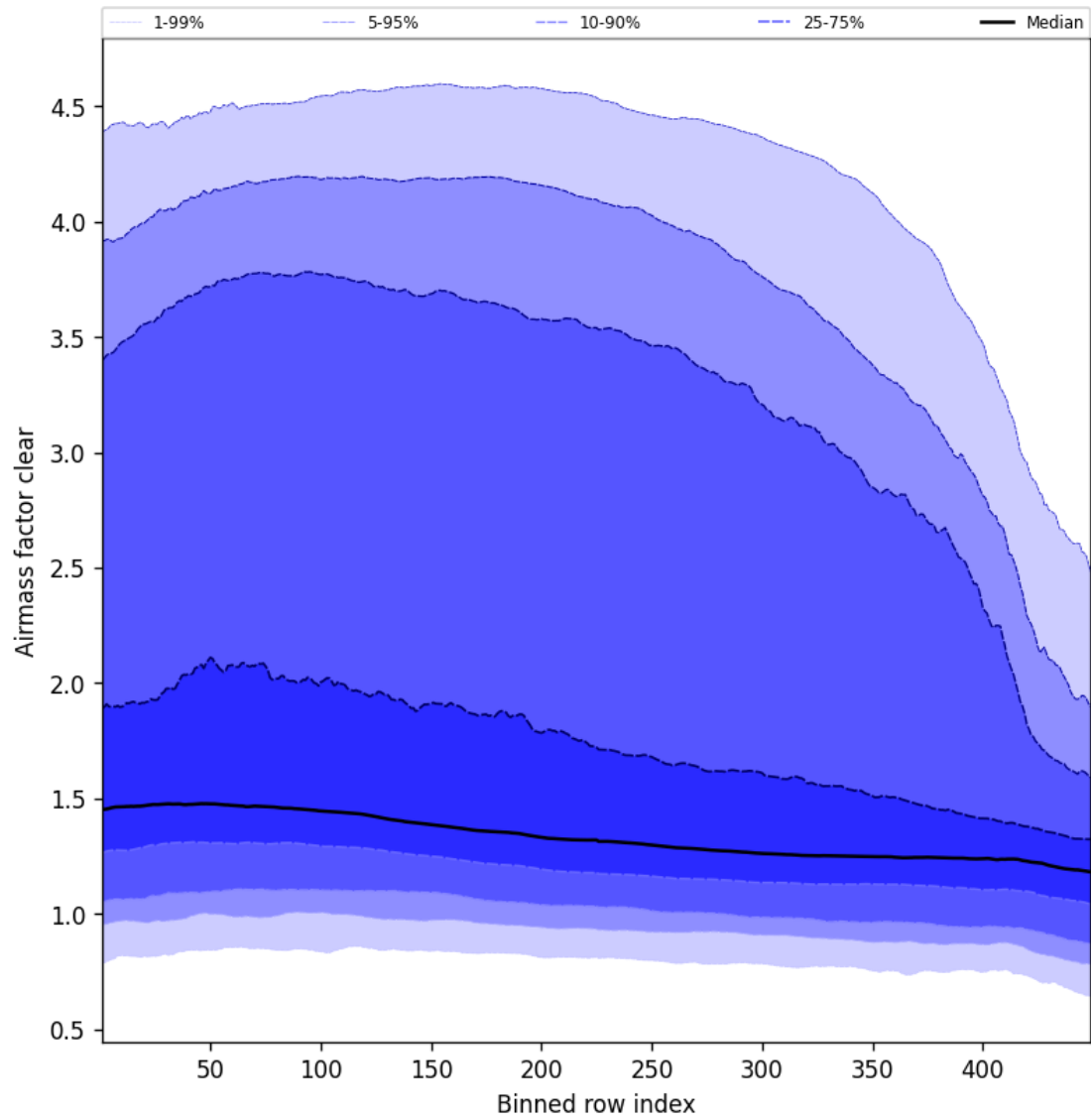
Figure 54: Along track statistics of “Airmass factor clear” for 2025-10-12 to 2025-10-13
