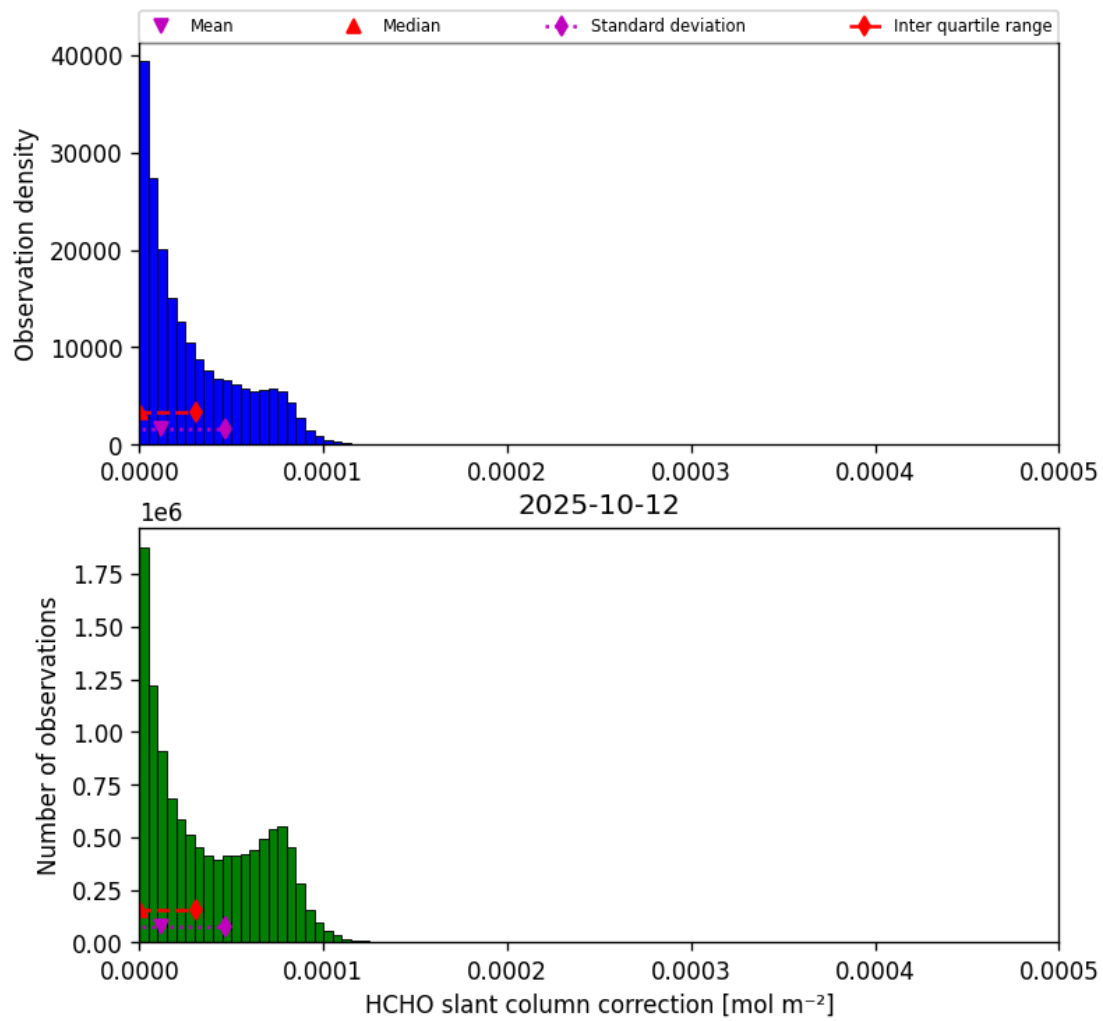
Figure 45: Histogram of “HCHO slant column correction” for 2025-10-12 to 2025-10-13
