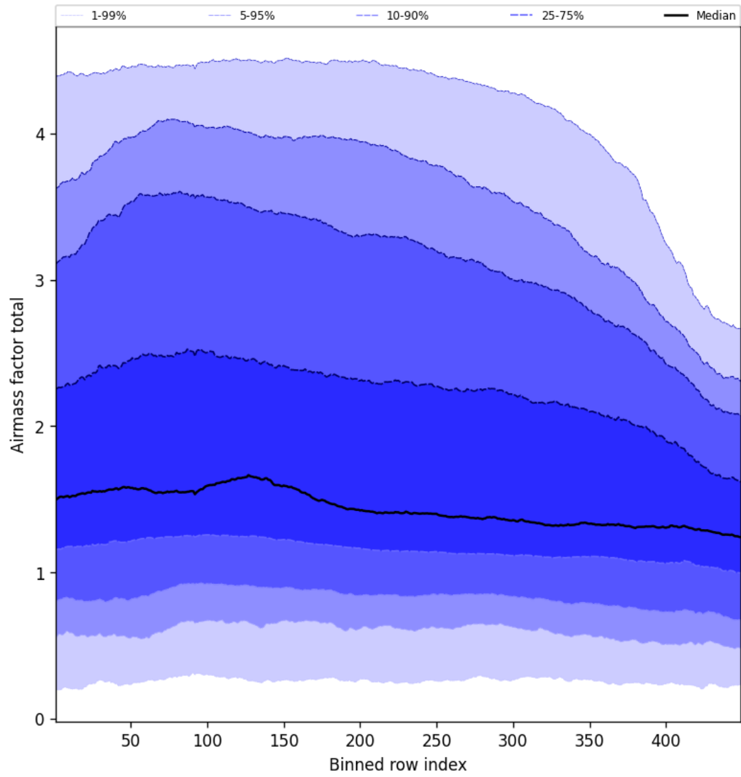
Figure 52: Along track statistics of “Airmass factor total” for 2025-10-12 to 2025-10-13
