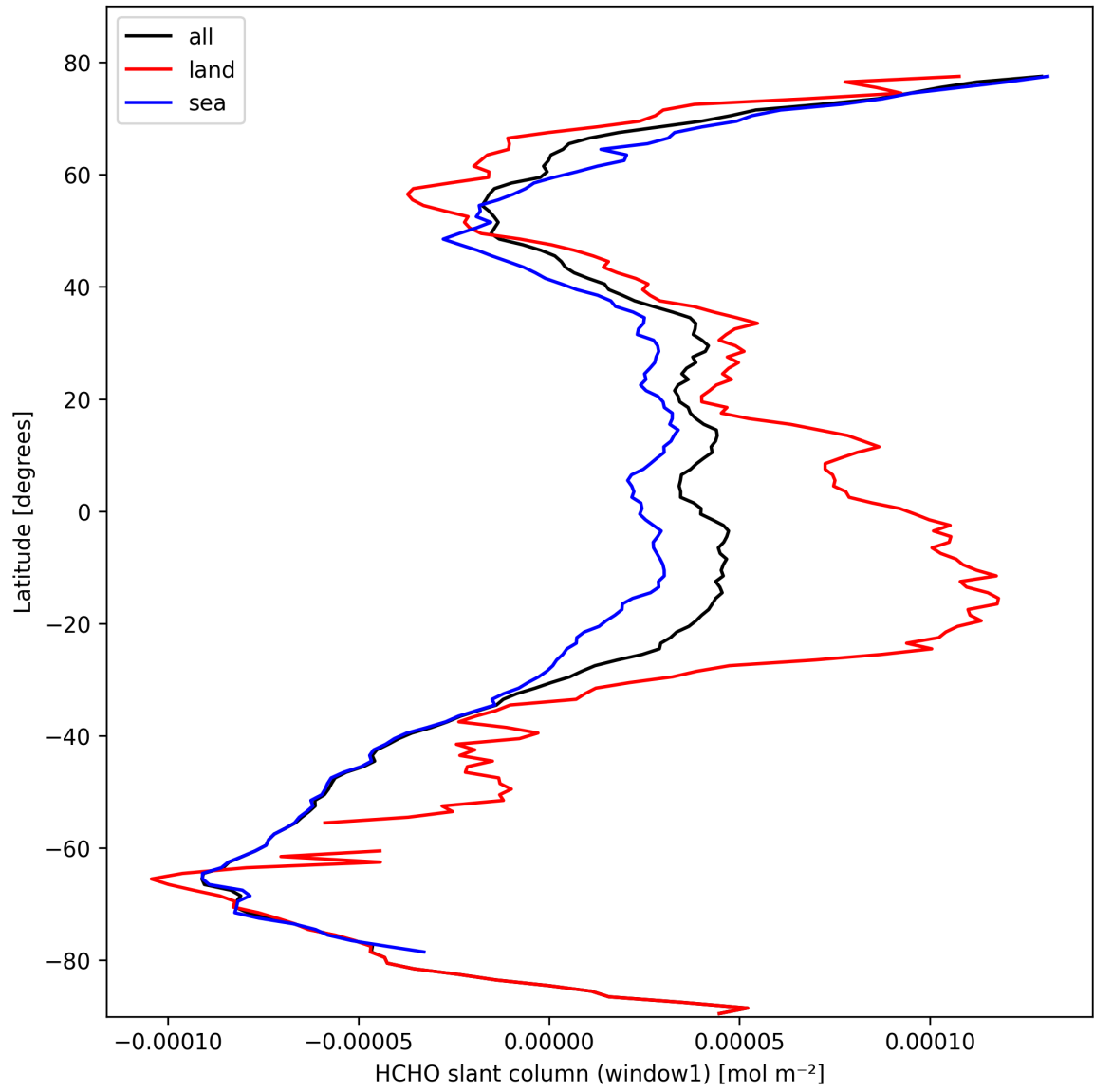
Figure 22: Zonal average of “HCHO slant column (window1)” for 2025-10-12 to 2025-10-13.
