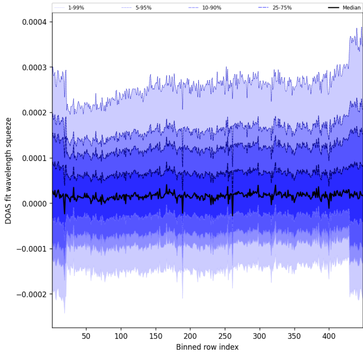
Figure 57: Along track statistics of “DOAS fit wavelength squeeze” for 2025-10-12 to 2025-10-13
