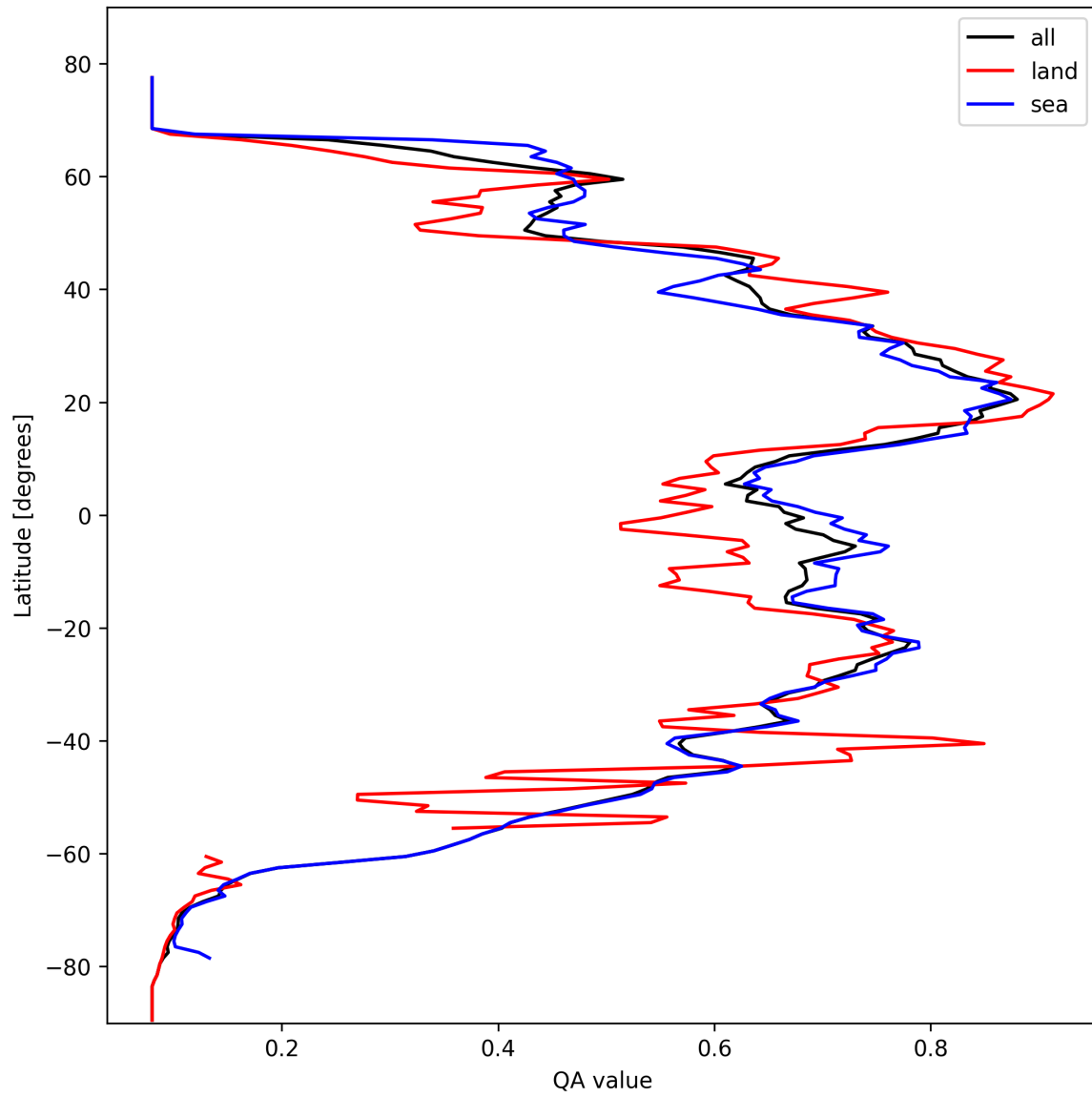
Figure 18: Zonal average of “QA value” for 2025-10-12 to 2025-10-13.
