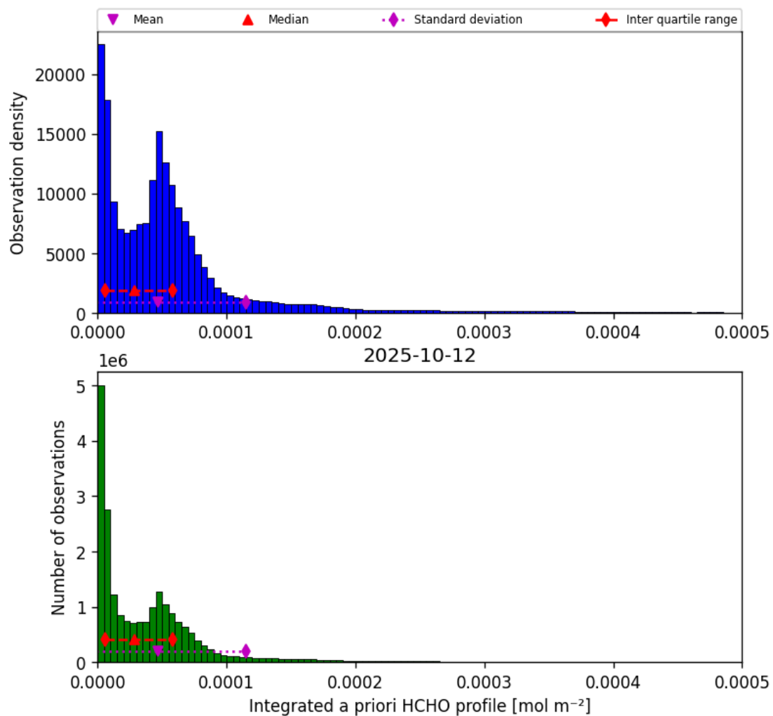
Figure 41: Histogram of “Integrated a priori HCHO profile” for 2025-10-12 to 2025-10-13
