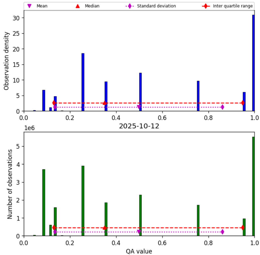
Figure 32: Histogram of “QA value” for 2025-10-12 to 2025-10-13
