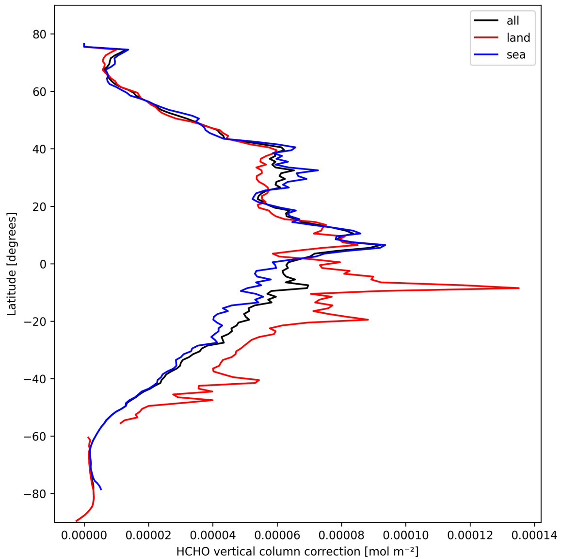
Figure 21: Zonal average of “HCHO vertical column correction” for 2025-10-14 to 2025-10-15.
