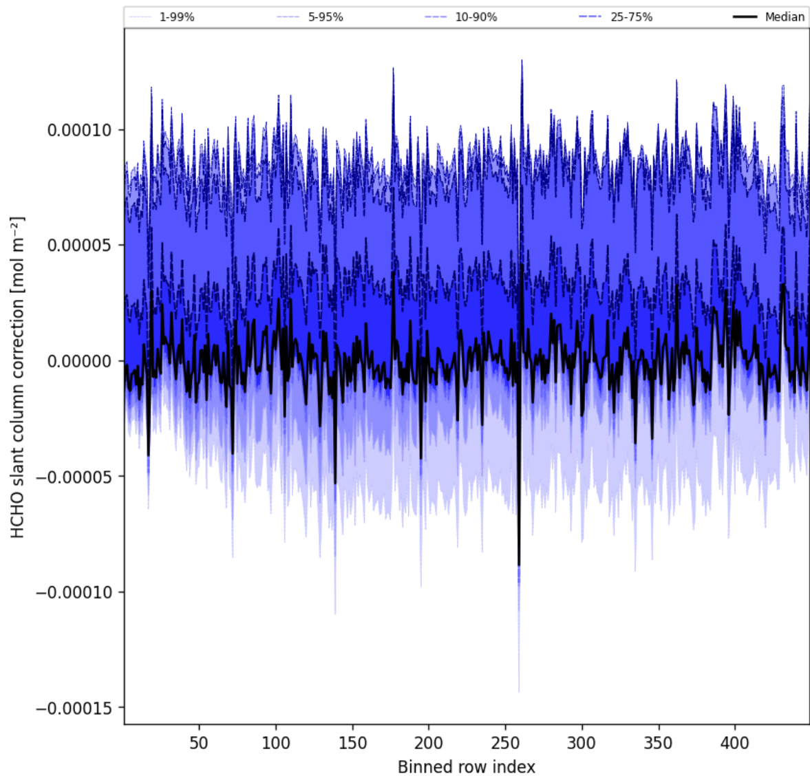
Figure 59: Along track statistics of “HCHO slant column correction” for 2025-10-14 to 2025-10-15
