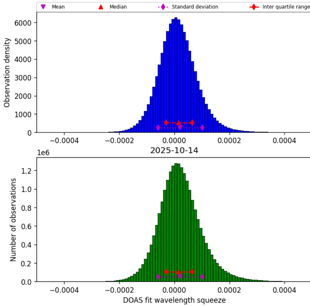
Figure 43: Histogram of “DOAS fit wavelength squeeze” for 2025-10-14 to 2025-10-15
