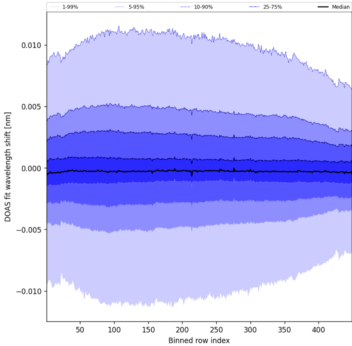
Figure 56: Along track statistics of “DOAS fit wavelength shift” for 2025-10-14 to 2025-10-15
