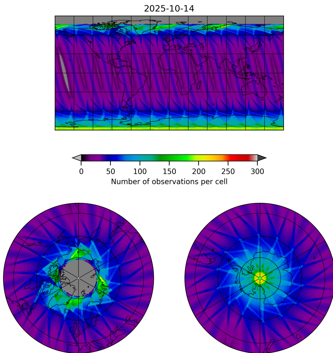
Figure 17: Map of the number of observations for 2025-10-14 to 2025-10-15
