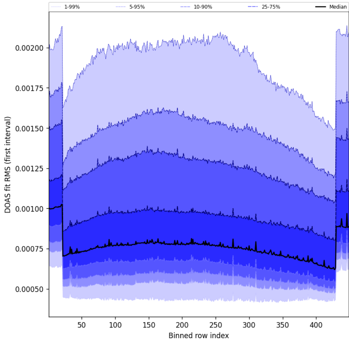
Figure 58: Along track statistics of “DOAS fit RMS (first interval)” for 2025-10-14 to 2025-10-15
