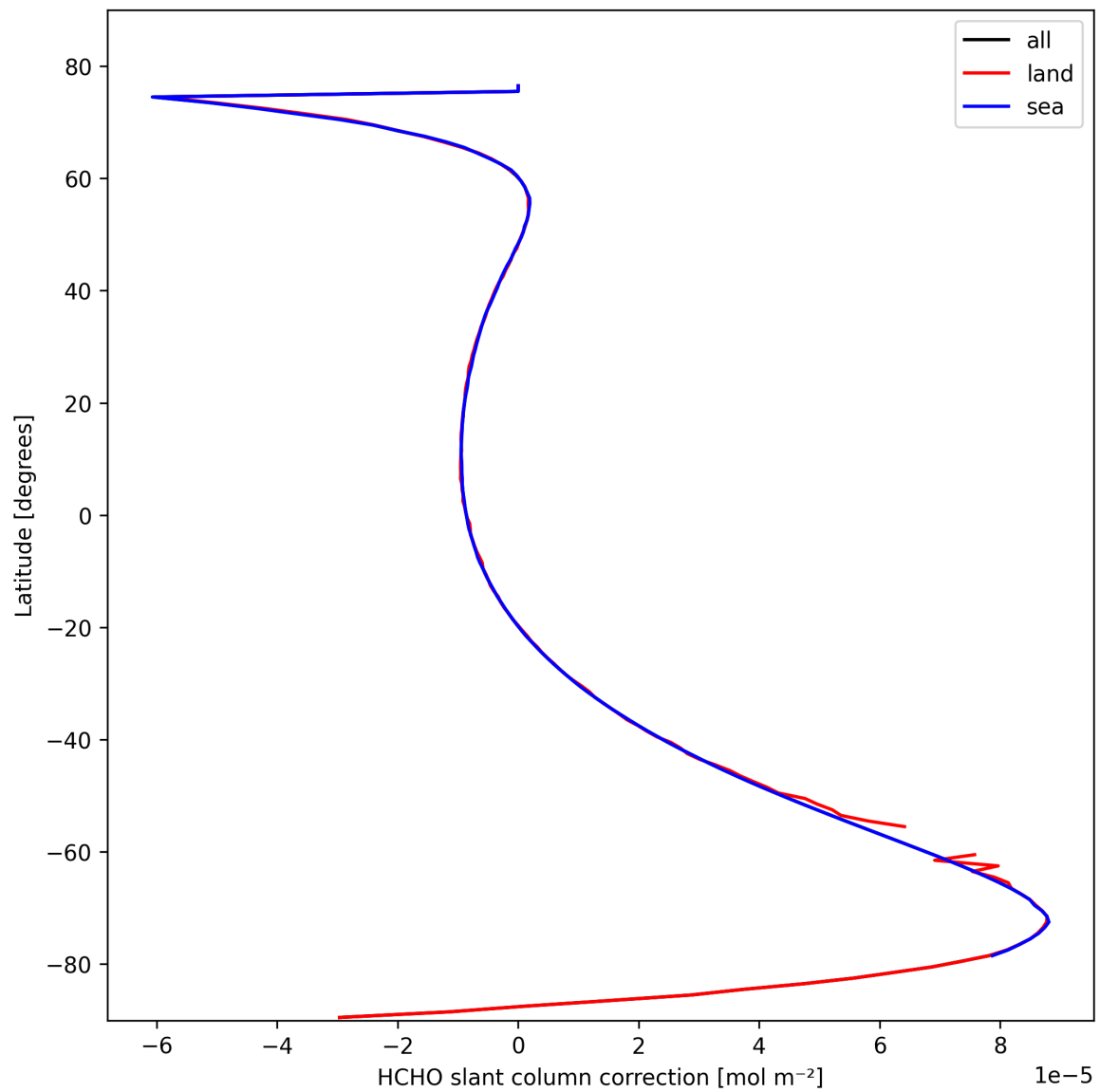
Figure 31: Zonal average of “HCHO slant column correction” for 2025-10-14 to 2025-10-15.
