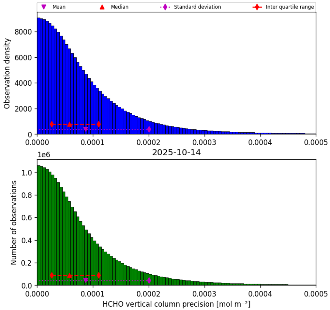
Figure 34: Histogram of “HCHO vertical column precision” for 2025-10-14 to 2025-10-15
