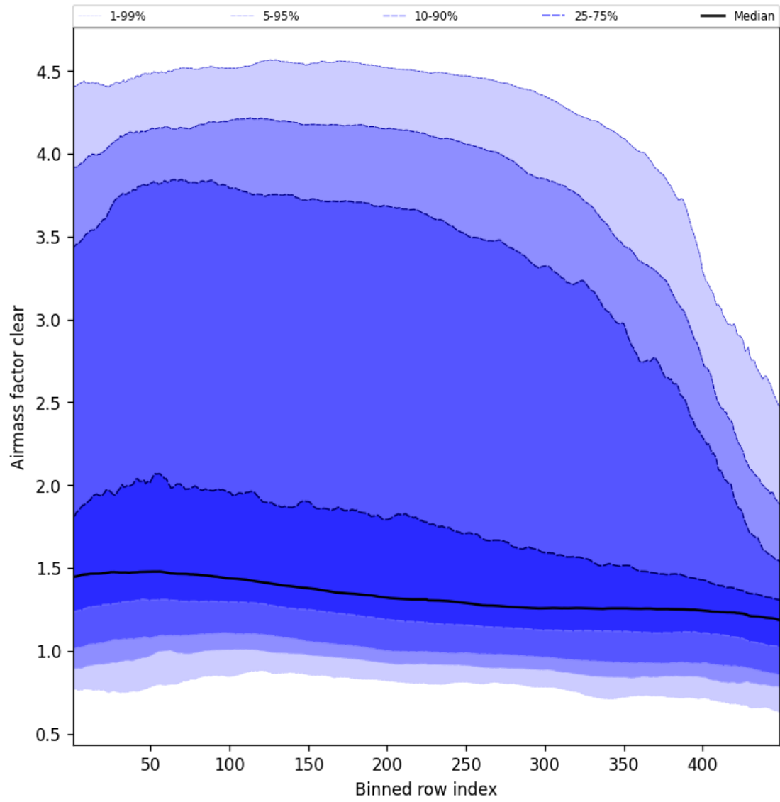
Figure 54: Along track statistics of “Airmass factor clear” for 2025-10-14 to 2025-10-15
