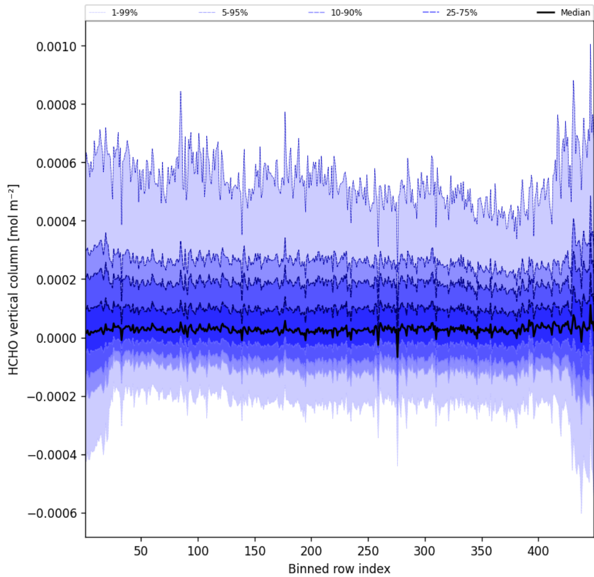
Figure 47: Along track statistics of “HCHO vertical column” for 2025-10-14 to 2025-10-15
