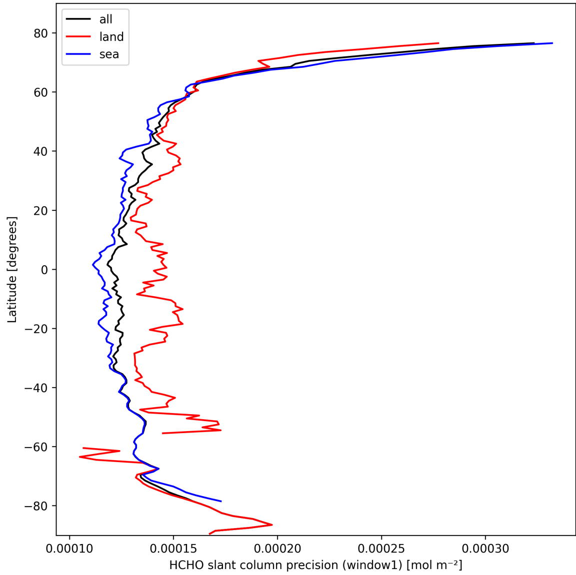
Figure 23: Zonal average of “HCHO slant column precision (window1)” for 2025-10-14 to 2025-10-15.
