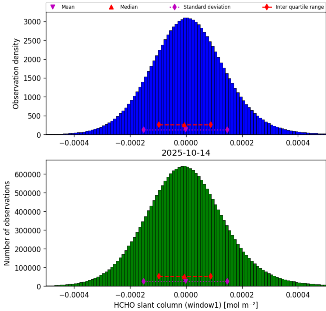
Figure 36: Histogram of “HCHO slant column (window1)” for 2025-10-14 to 2025-10-15
