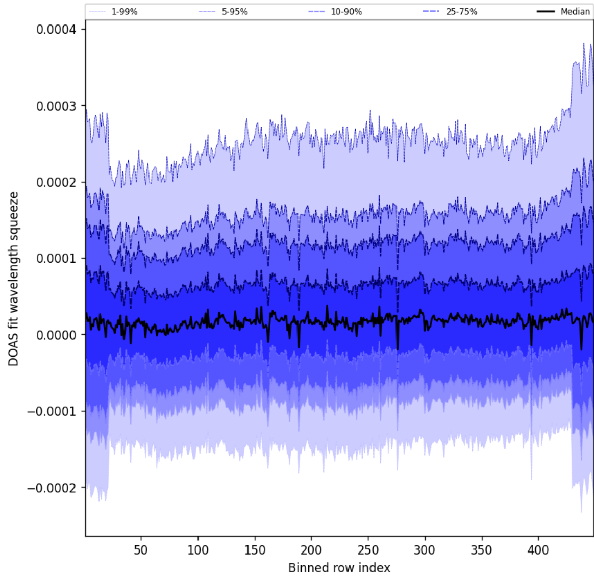
Figure 57: Along track statistics of “DOAS fit wavelength squeeze” for 2025-10-14 to 2025-10-15
