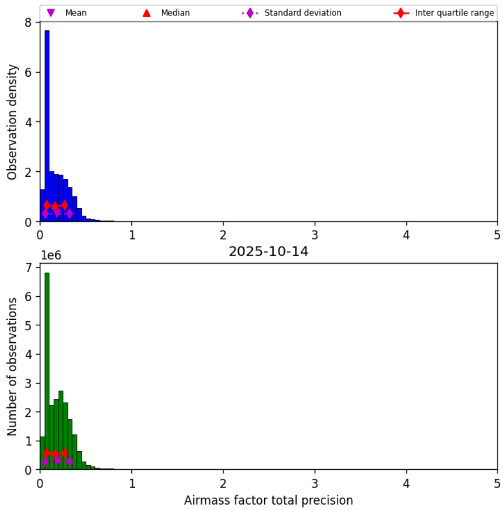
Figure 39: Histogram of “Airmass factor total precision” for 2025-10-14 to 2025-10-15
