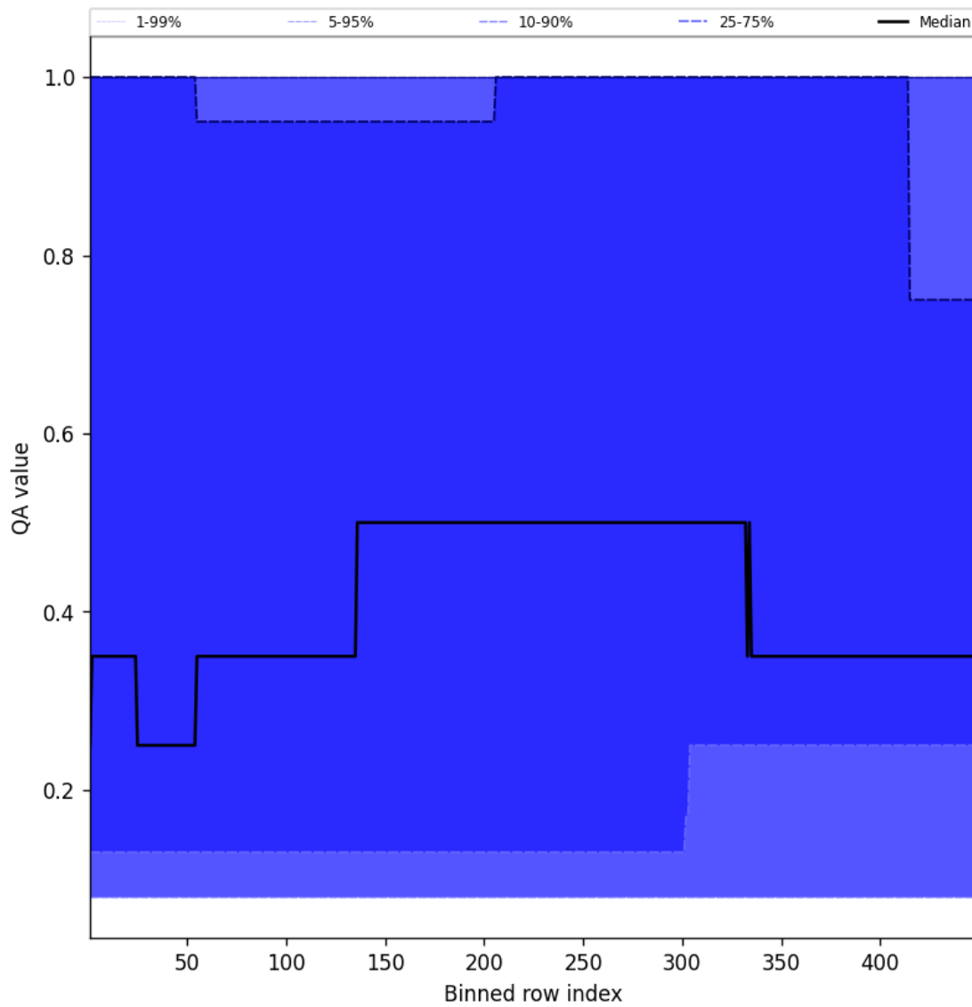
Figure 46: Along track statistics of “QA value” for 2025-10-14 to 2025-10-15
