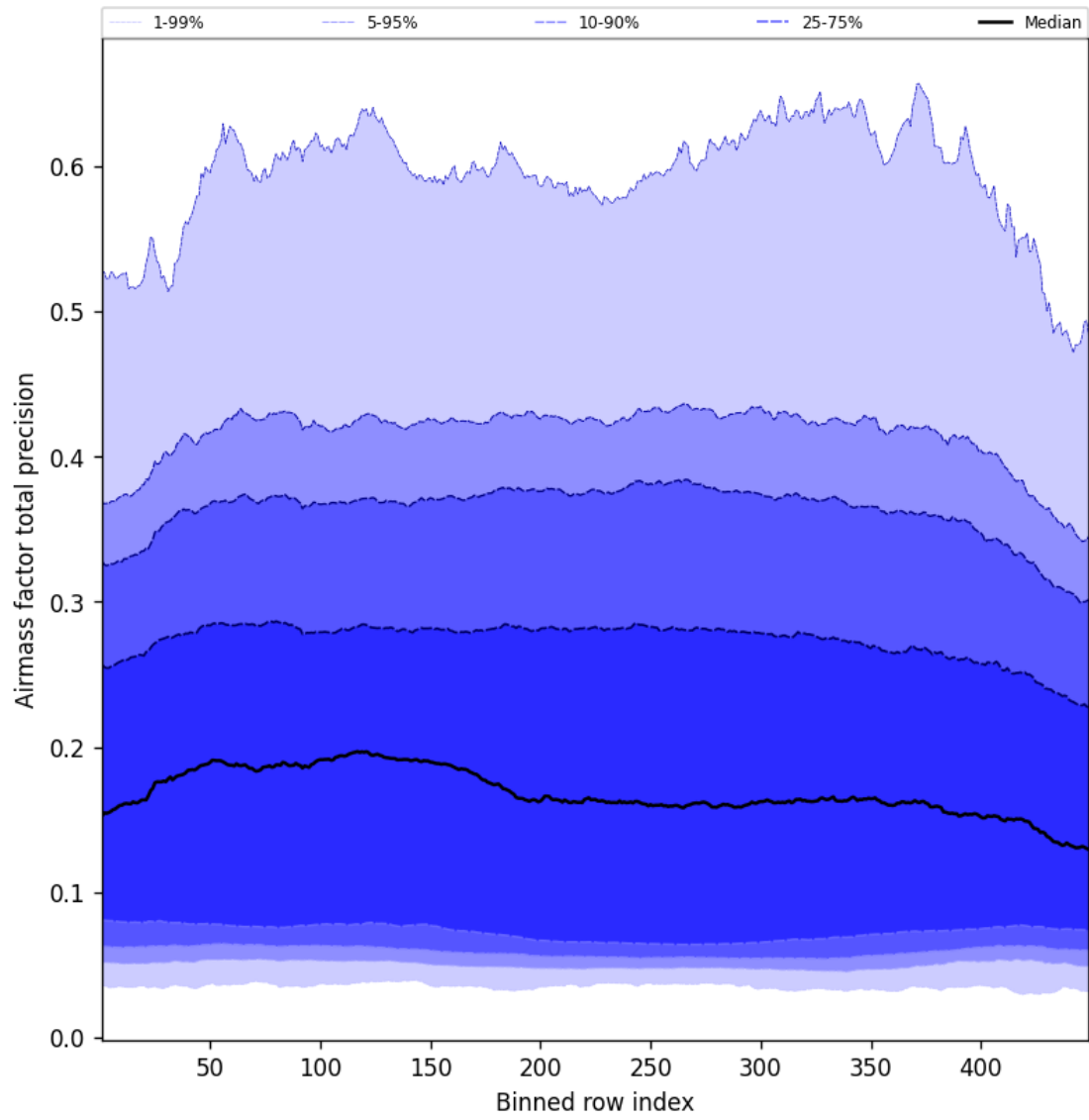
Figure 53: Along track statistics of “Airmass factor total precision” for 2025-10-14 to 2025-10-15
