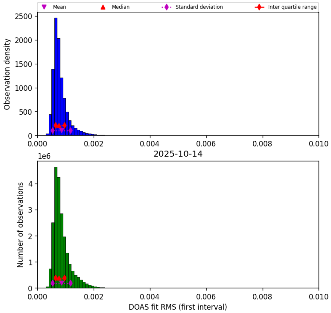
Figure 44: Histogram of "DOAS fit RMS (first interval)" for 2025-10-14 to 2025-10-15
