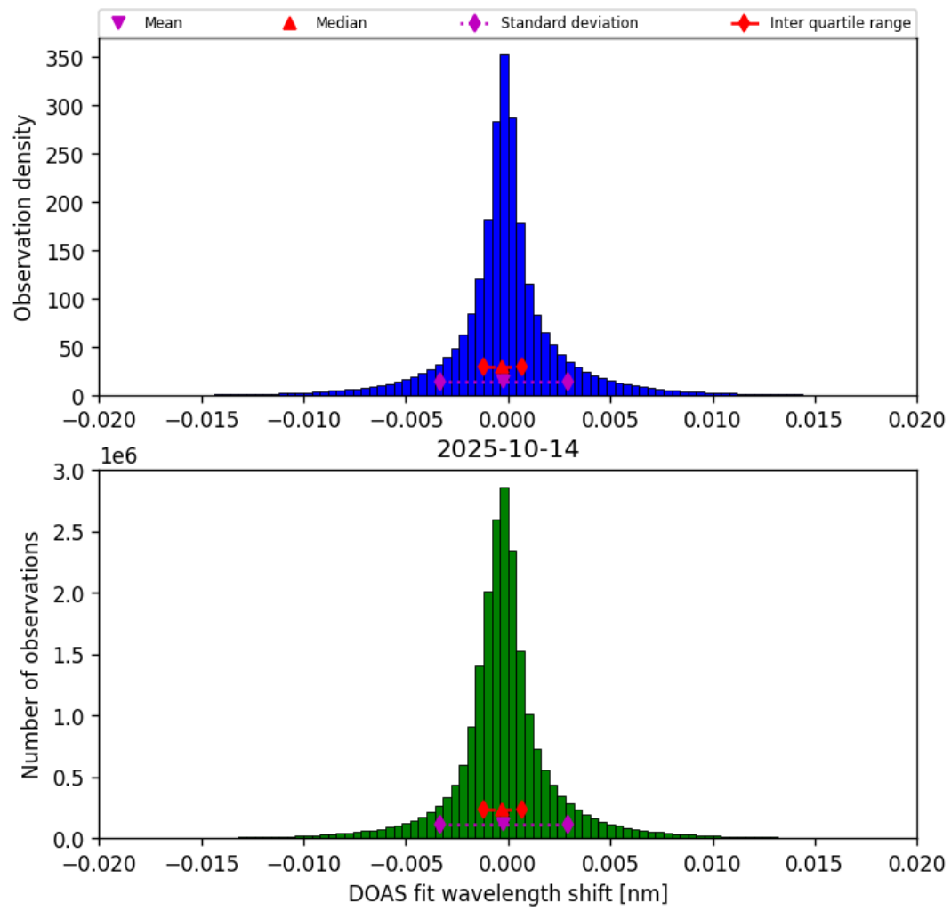
Figure 42: Histogram of “DOAS fit wavelength shift” for 2025-10-14 to 2025-10-15
