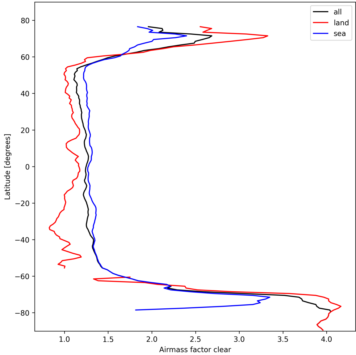
Figure 26: Zonal average of “Airmass factor clear” for 2025-10-14 to 2025-10-15.
