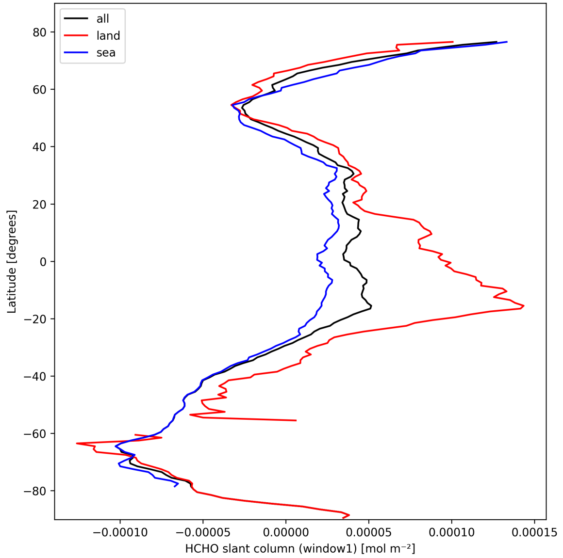
Figure 22: Zonal average of “HCHO slant column (window1)” for 2025-10-14 to 2025-10-15.
