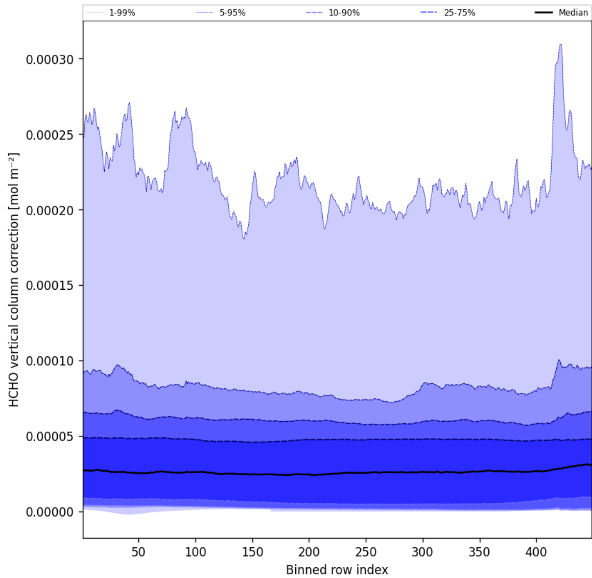
Figure 49: Along track statistics of “HCHO vertical column correction” for 2025-10-14 to 2025-10-15
