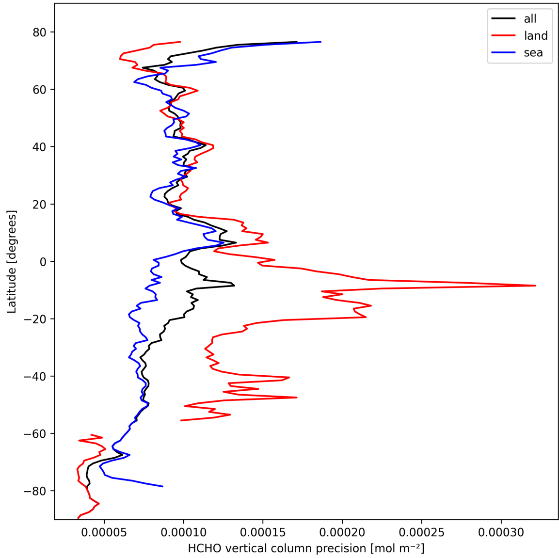
Figure 20: Zonal average of “HCHO vertical column precision” for 2025-10-14 to 2025-10-15.
