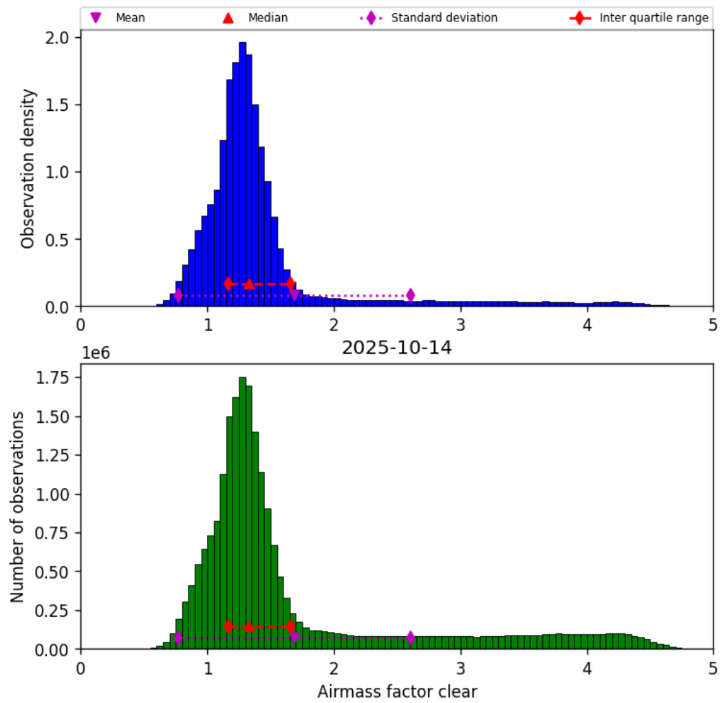
Figure 40: Histogram of “Airmass factor clear” for 2025-10-14 to 2025-10-15
