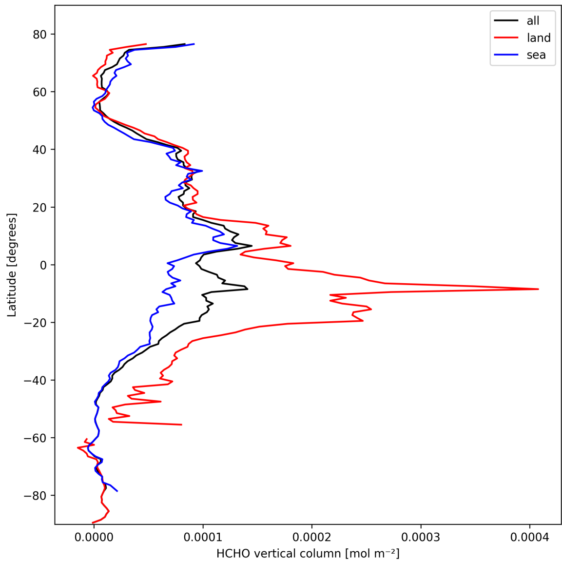
Figure 19: Zonal average of “HCHO vertical column” for 2025-10-14 to 2025-10-15.
