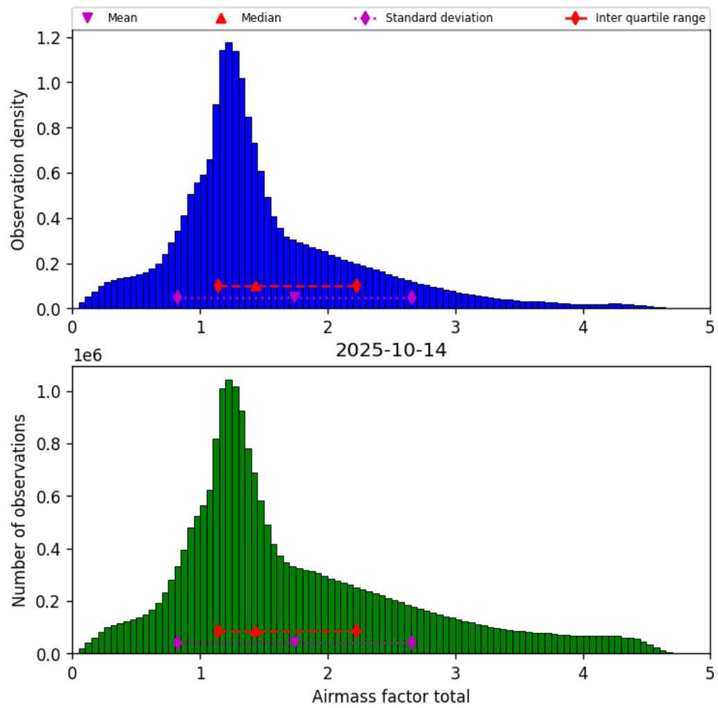
Figure 38: Histogram of “Airmass factor total” for 2025-10-14 to 2025-10-15
