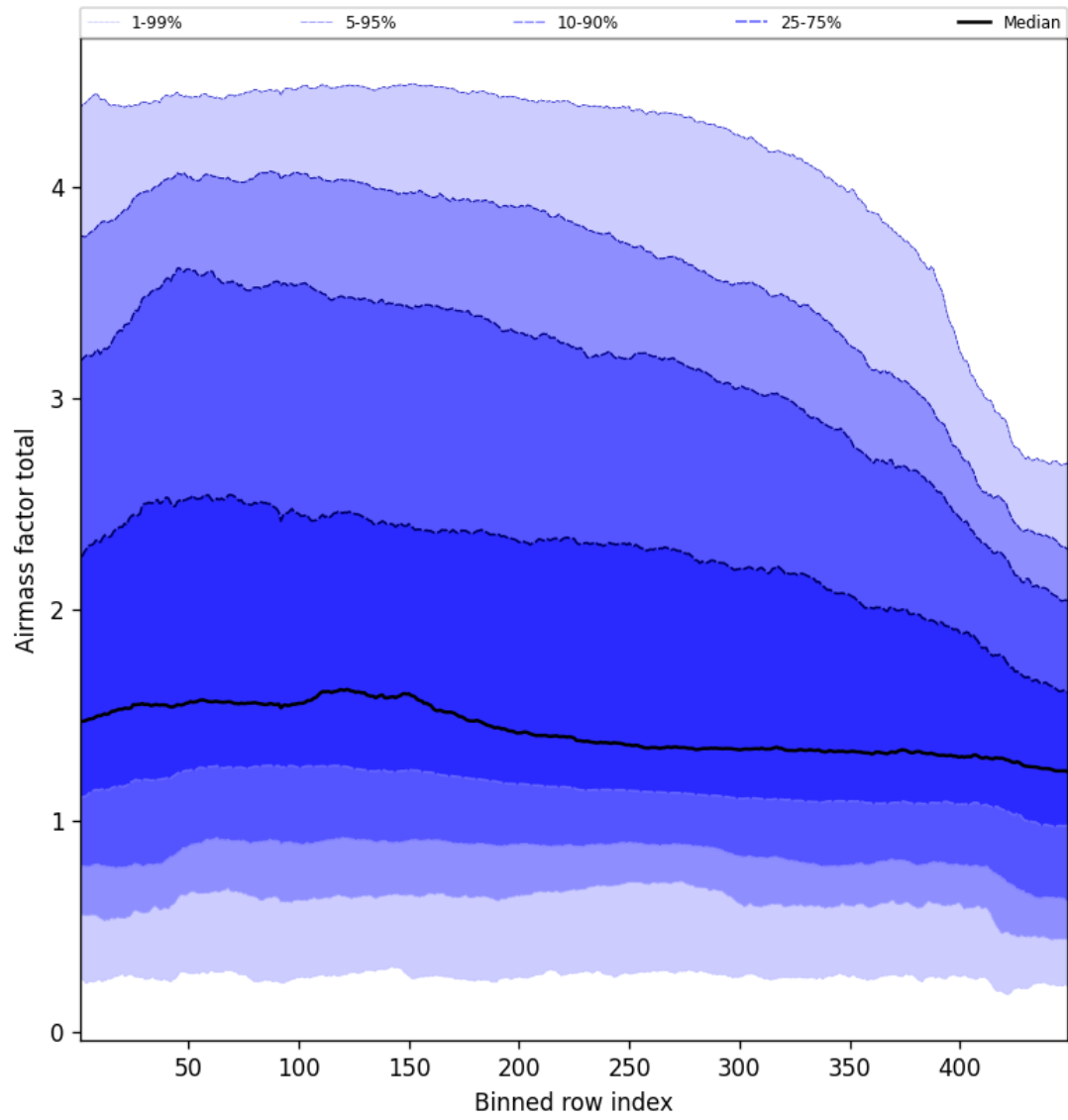
Figure 52: Along track statistics of “Airmass factor total” for 2025-10-14 to 2025-10-15
