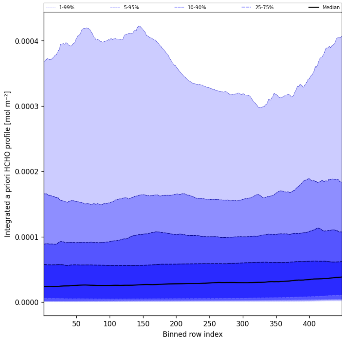
Figure 55: Along track statistics of "Integrated a priori HCHO profile" for 2025-10-14 to 2025-10-15
