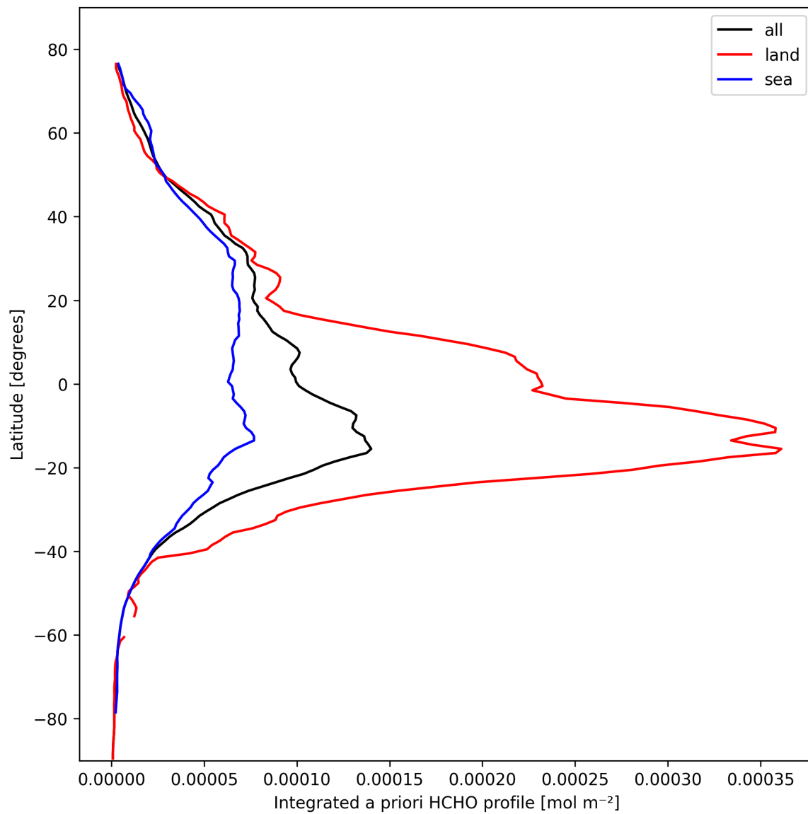
Figure 27: Zonal average of “Integrated a priori HCHO profile” for 2025-10-14 to 2025-10-15.
