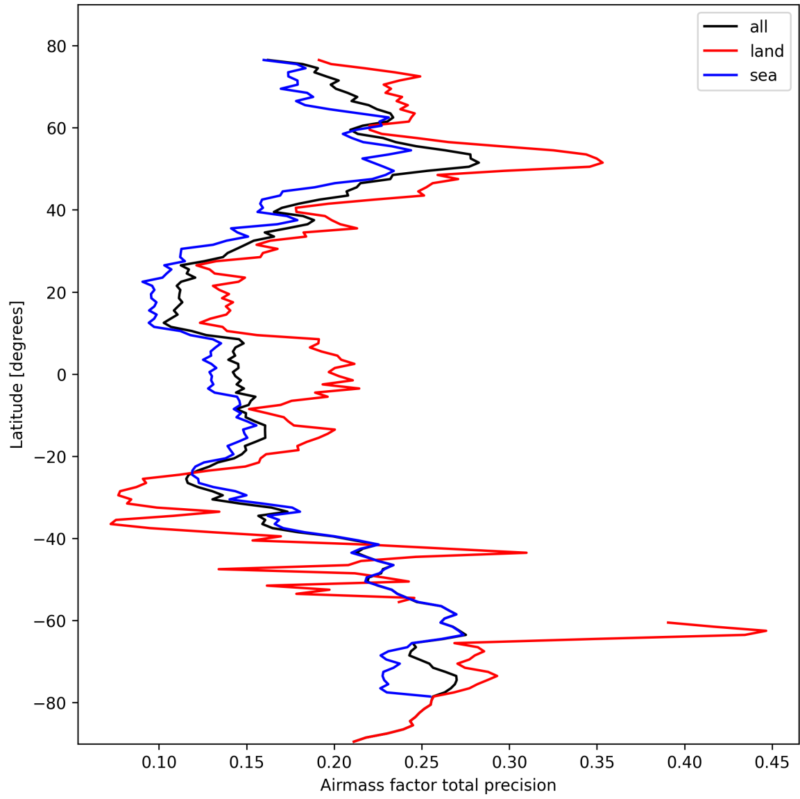
Figure 25: Zonal average of “Airmass factor total precision” for 2025-10-14 to 2025-10-15.
