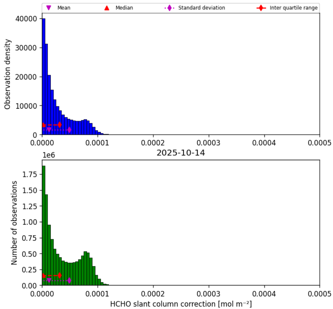
Figure 45: Histogram of “HCHO slant column correction” for 2025-10-14 to 2025-10-15
