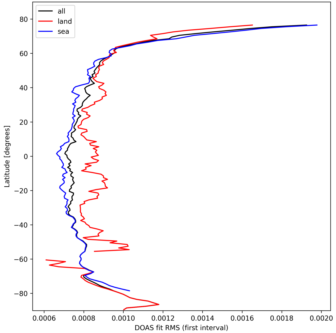
Figure 30: Zonal average of “DOAS fit RMS (first interval)” for 2025-10-14 to 2025-10-15.
