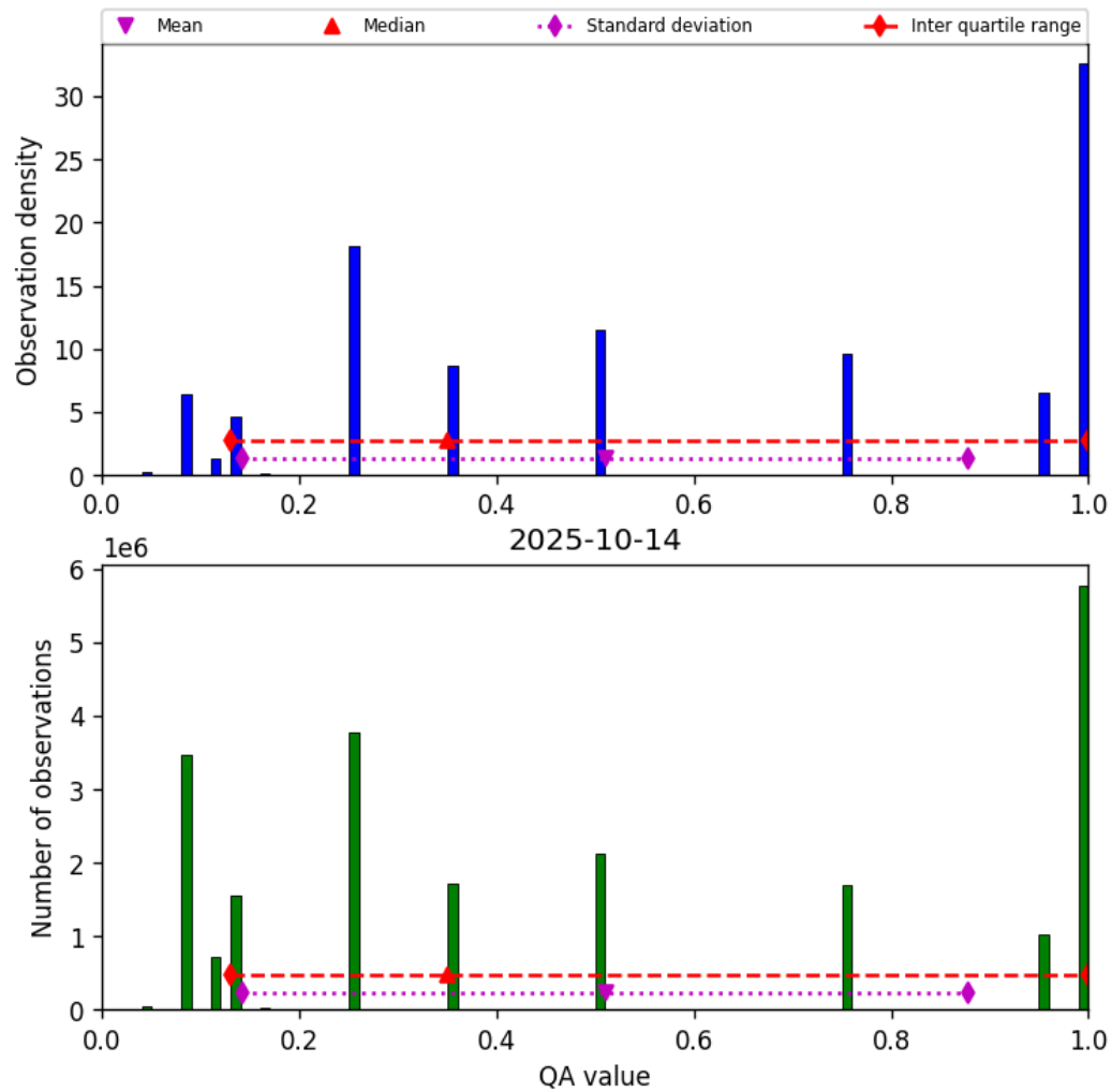
Figure 32: Histogram of “QA value” for 2025-10-14 to 2025-10-15
