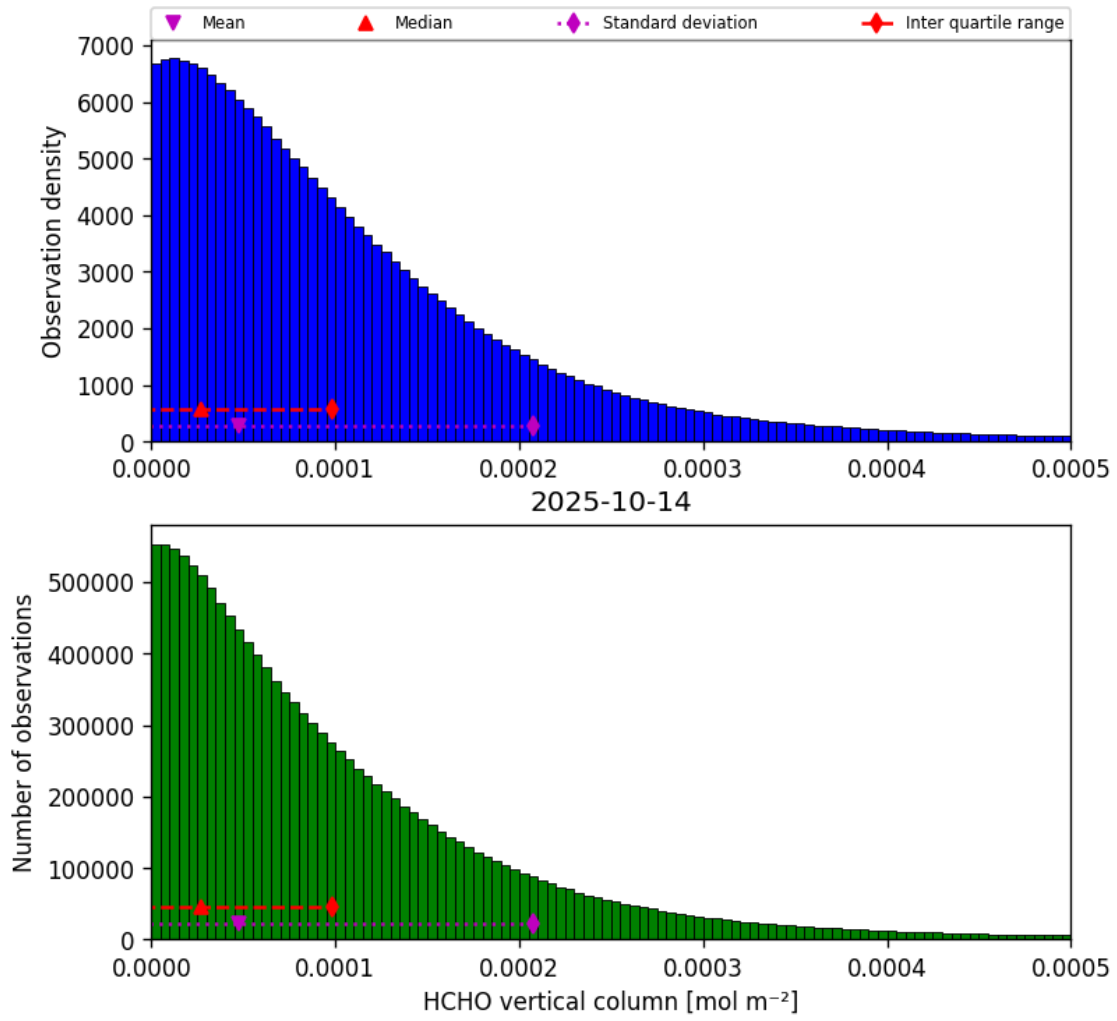
Figure 33: Histogram of “HCHO vertical column” for 2025-10-14 to 2025-10-15
