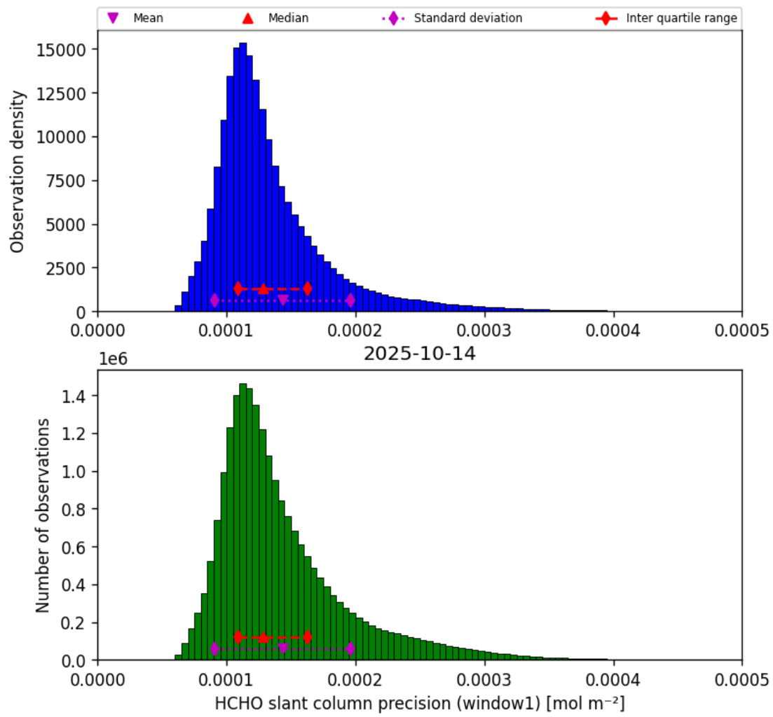
Figure 37: Histogram of “HCHO slant column precision (window1)” for 2025-10-14 to 2025-10-15
