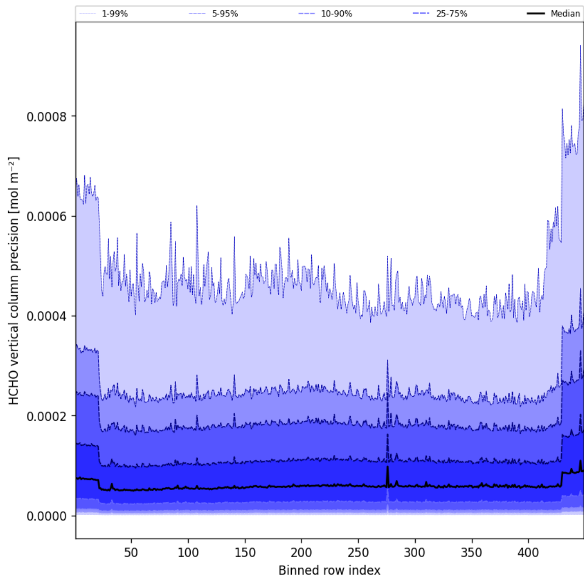
Figure 48: Along track statistics of “HCHO vertical column precision” for 2025-10-14 to 2025-10-15
