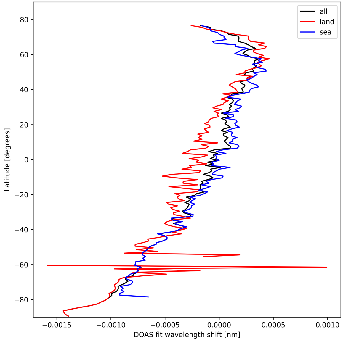
Figure 28: Zonal average of “DOAS fit wavelength shift” for 2025-10-14 to 2025-10-15.
