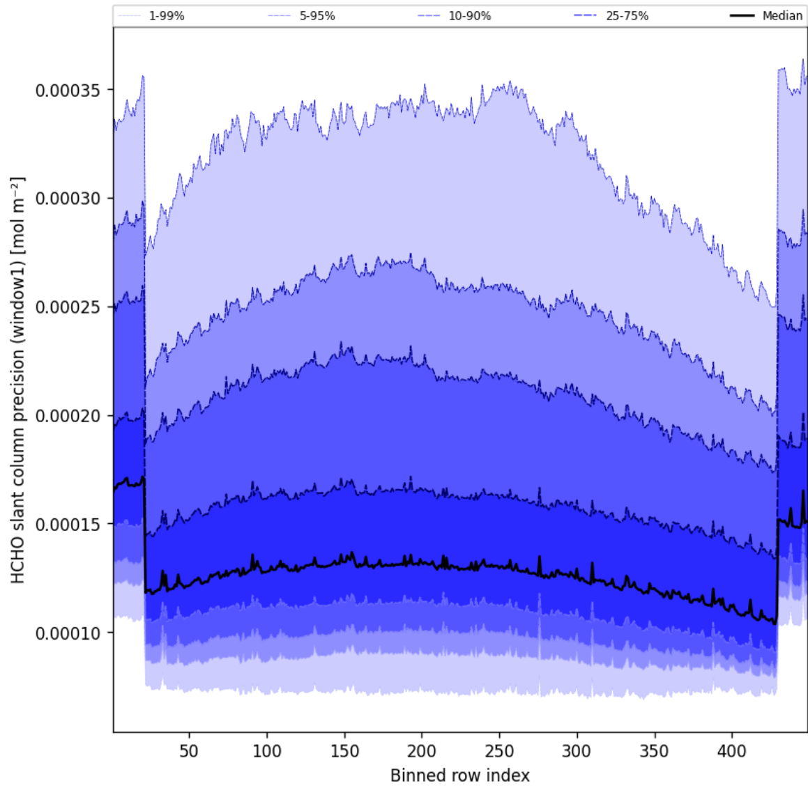
Figure 51: Along track statistics of “HCHO slant column precision (window1)” for 2025-10-14 to 2025-10-15
