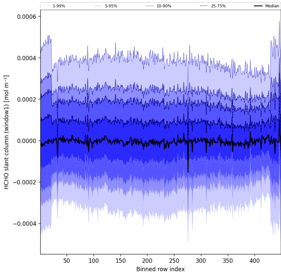
Figure 50: Along track statistics of “HCHO slant column (window1)” for 2025-10-14 to 2025-10-15
