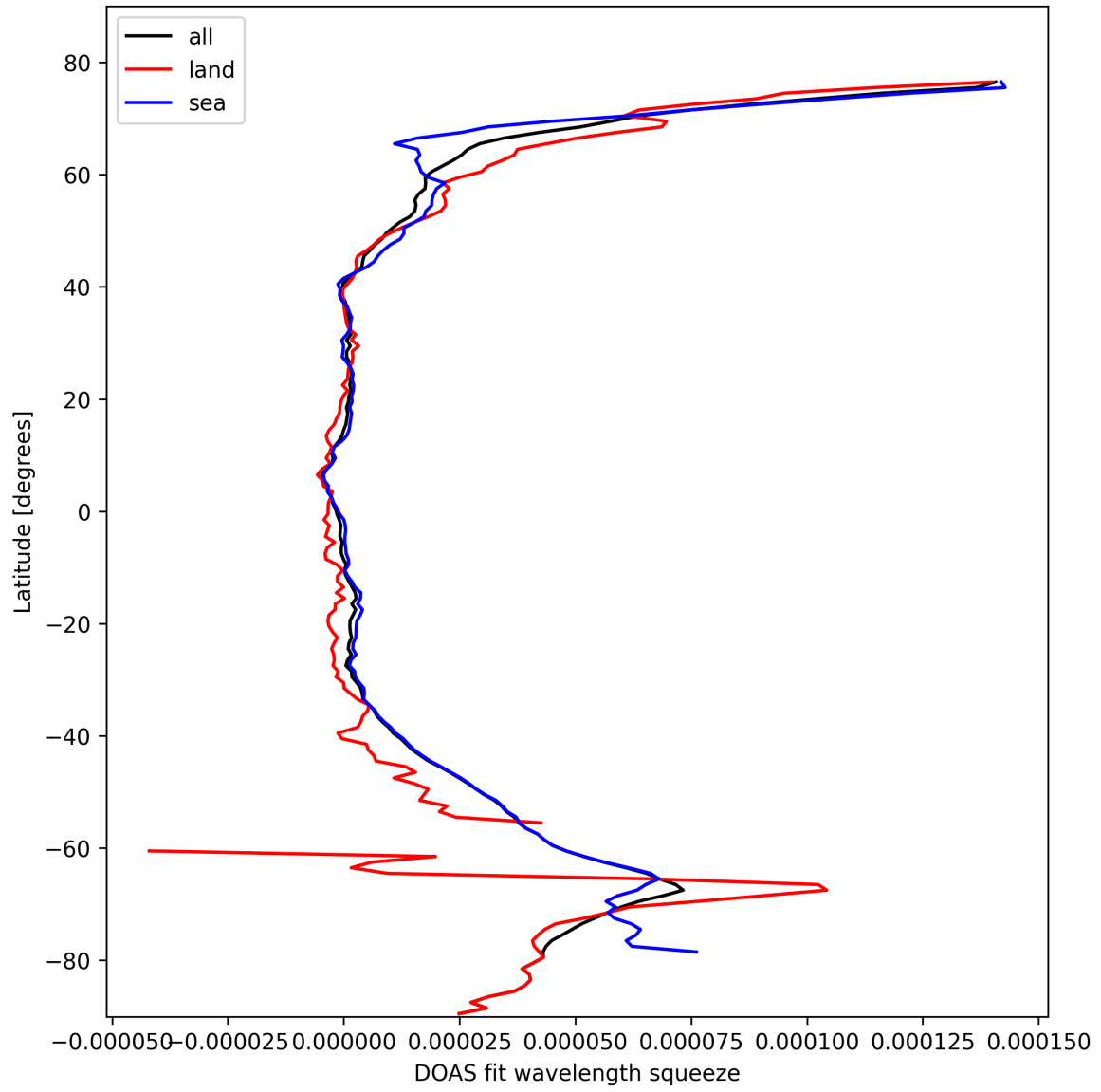
Figure 29: Zonal average of “DOAS fit wavelength squeeze” for 2025-10-14 to 2025-10-15.
