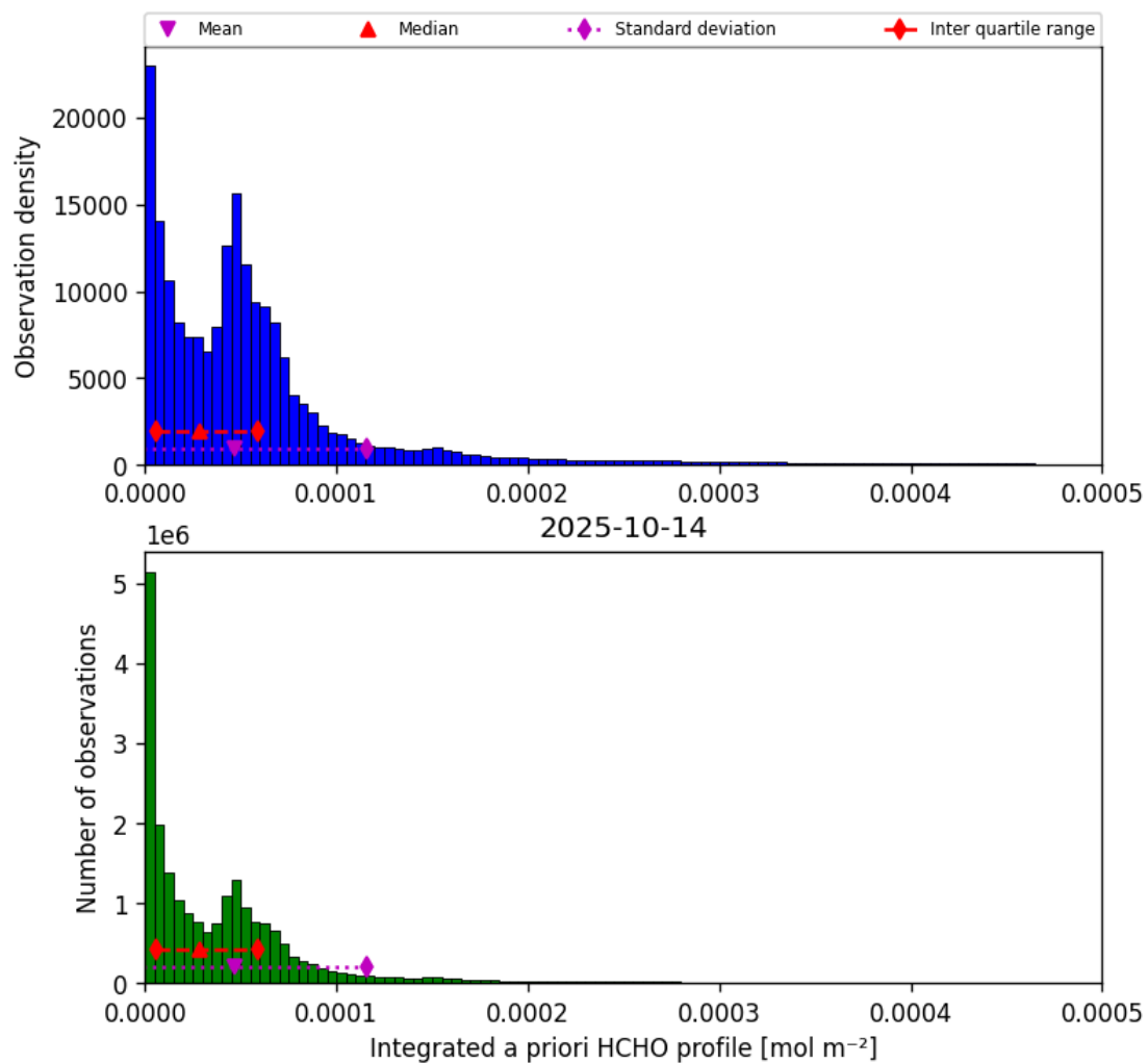
Figure 41: Histogram of “Integrated a priori HCHO profile” for 2025-10-14 to 2025-10-15
