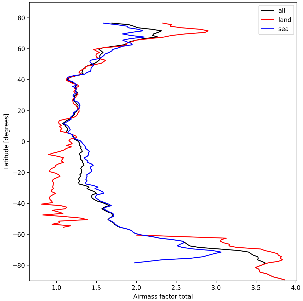
Figure 24: Zonal average of “Airmass factor total” for 2025-10-14 to 2025-10-15.
