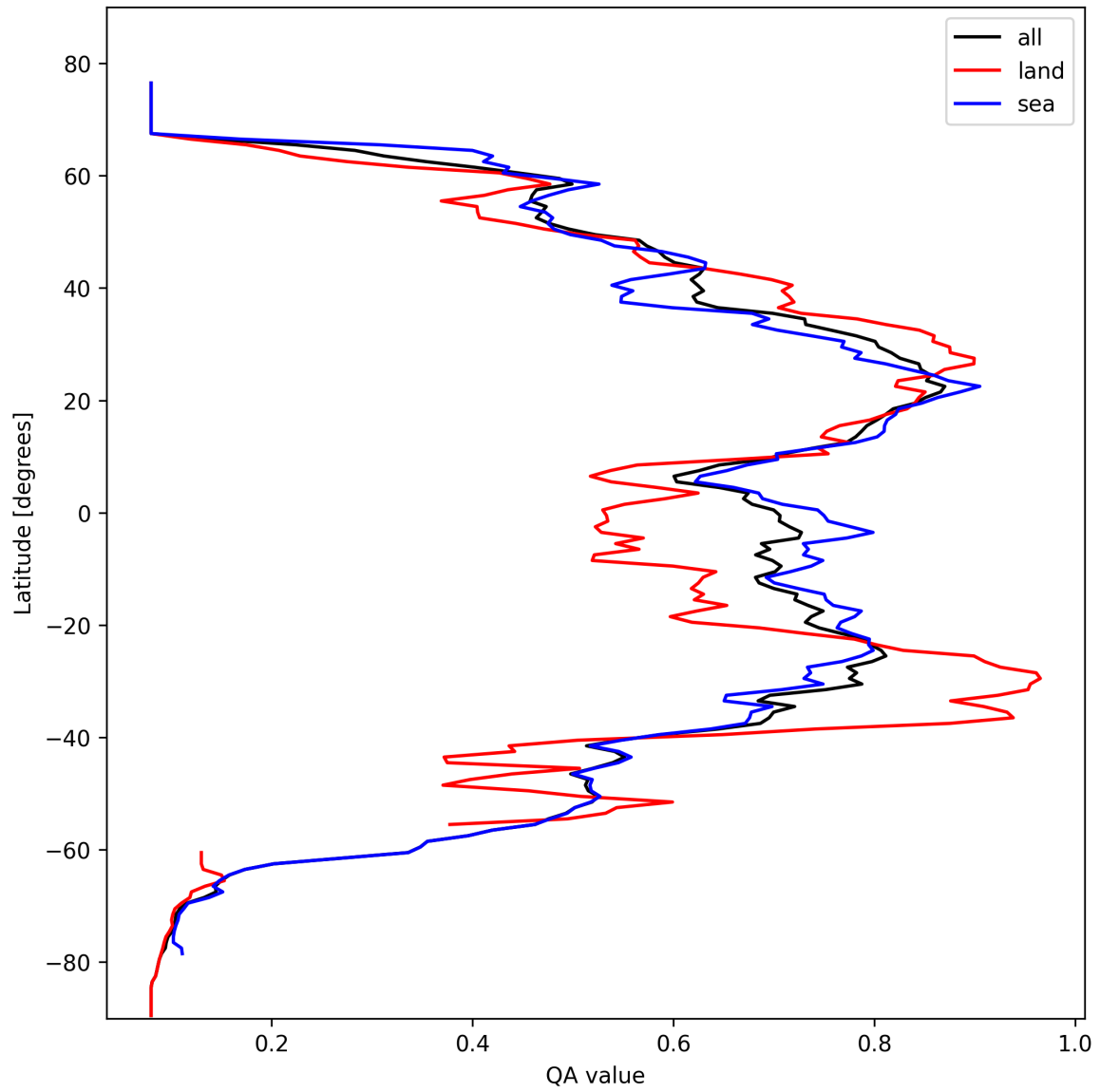
Figure 18: Zonal average of “QA value” for 2025-10-14 to 2025-10-15.
