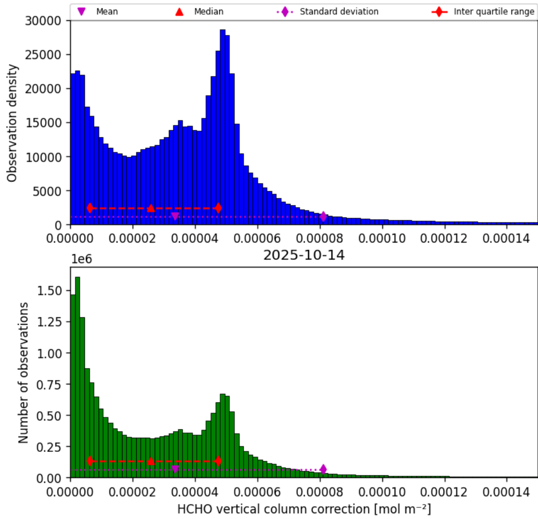
Figure 35: Histogram of “HCHO vertical column correction” for 2025-10-14 to 2025-10-15
