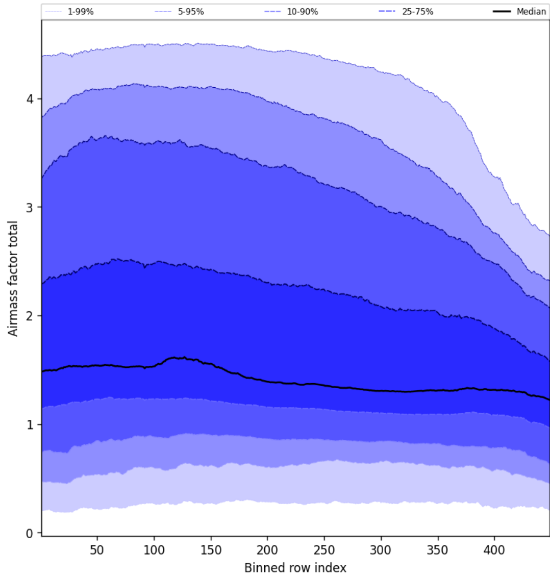
Figure 52: Along track statistics of “Airmass factor total” for 2025-10-15 to 2025-10-15
