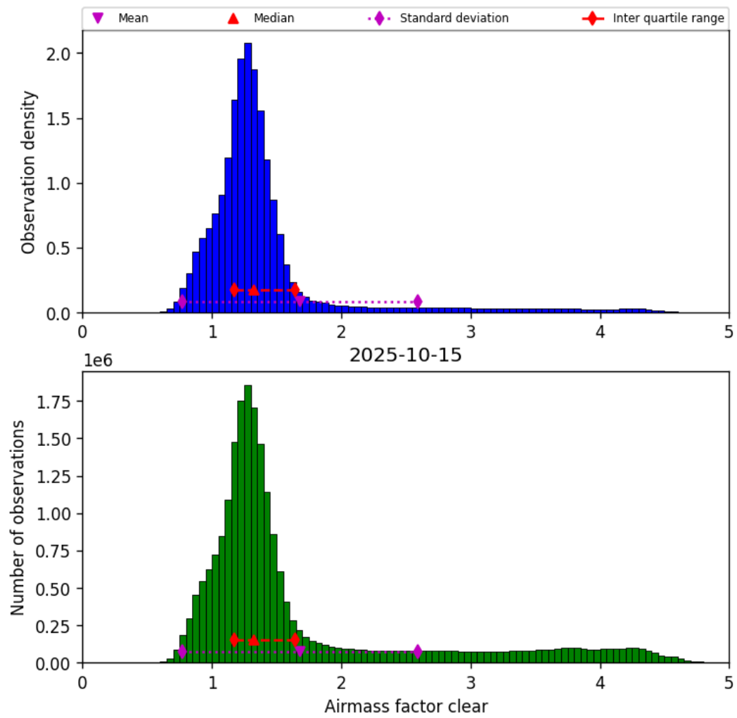
Figure 40: Histogram of “Airmass factor clear” for 2025-10-15 to 2025-10-15
