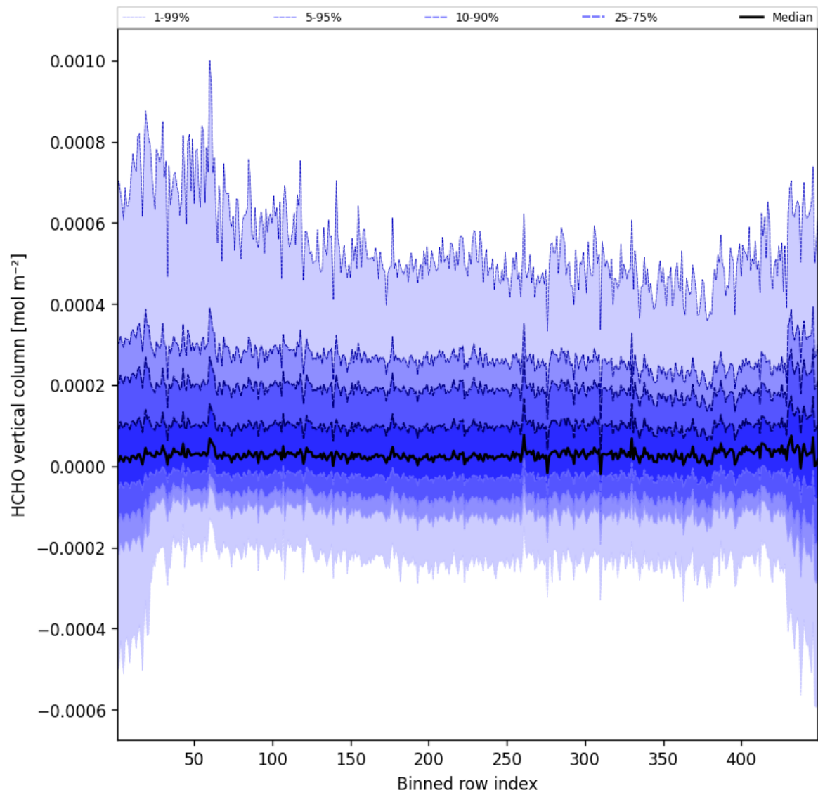
Figure 47: Along track statistics of “HCHO vertical column” for 2025-10-15 to 2025-10-15
