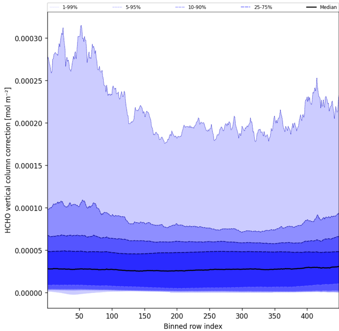
Figure 49: Along track statistics of “HCHO vertical column correction” for 2025-10-15 to 2025-10-15
