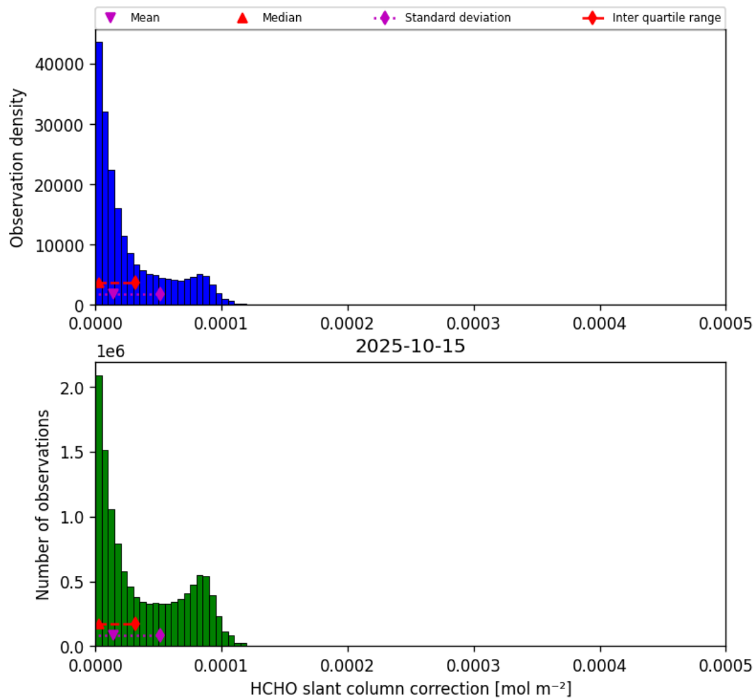
Figure 45: Histogram of “HCHO slant column correction” for 2025-10-15 to 2025-10-15
