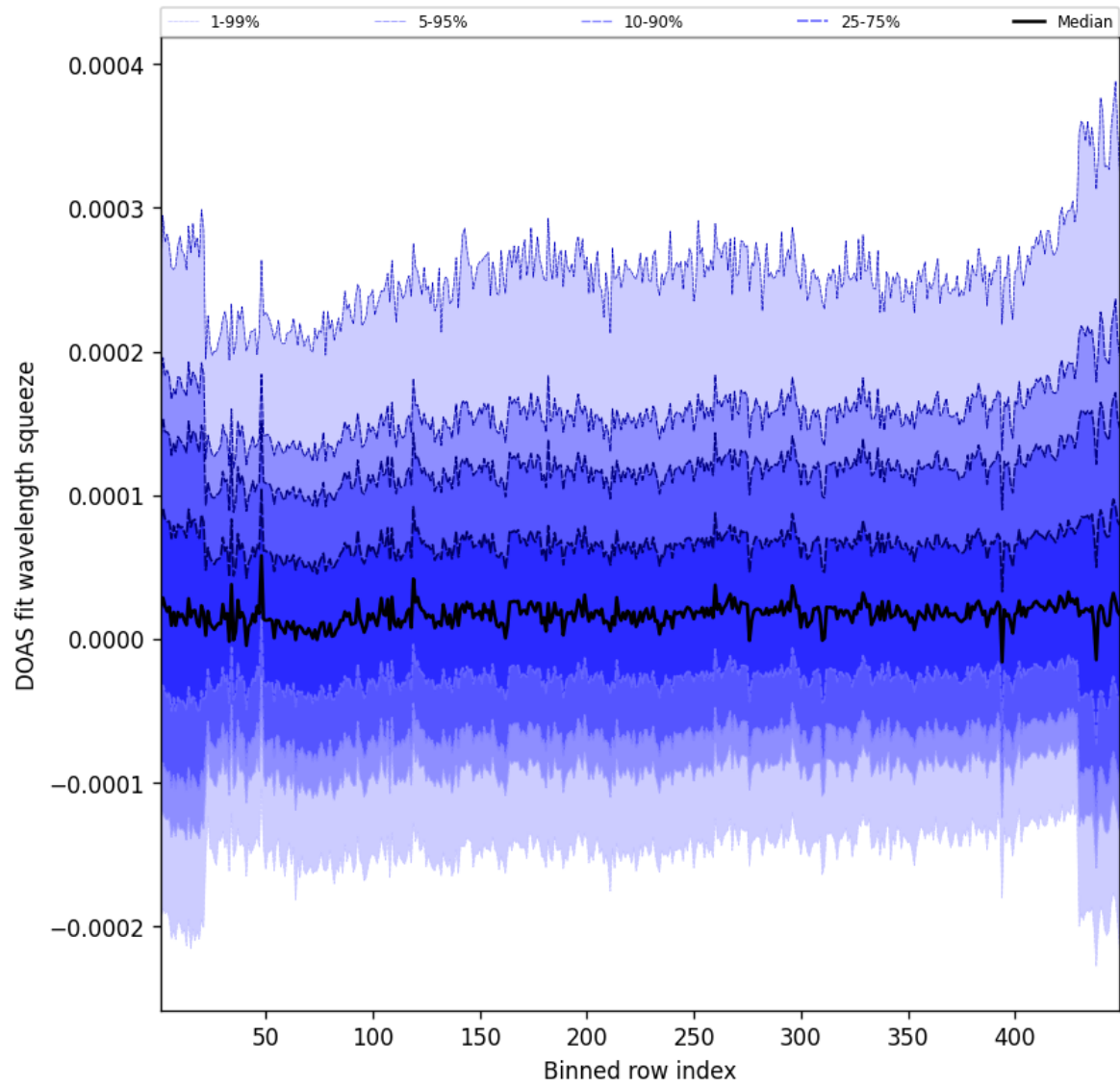
Figure 57: Along track statistics of “DOAS fit wavelength squeeze” for 2025-10-15 to 2025-10-15
