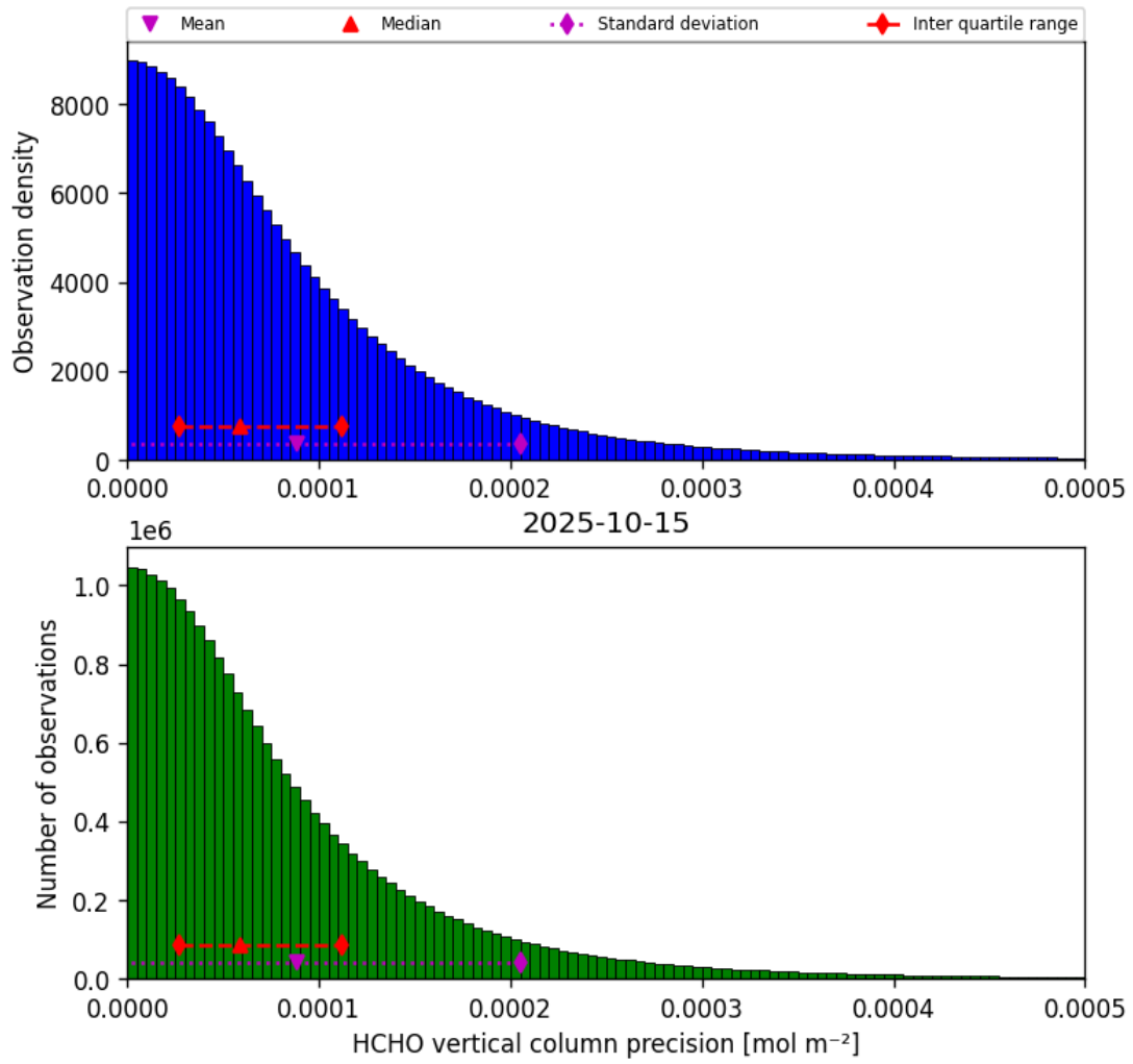
Figure 34: Histogram of “HCHO vertical column precision” for 2025-10-15 to 2025-10-15
