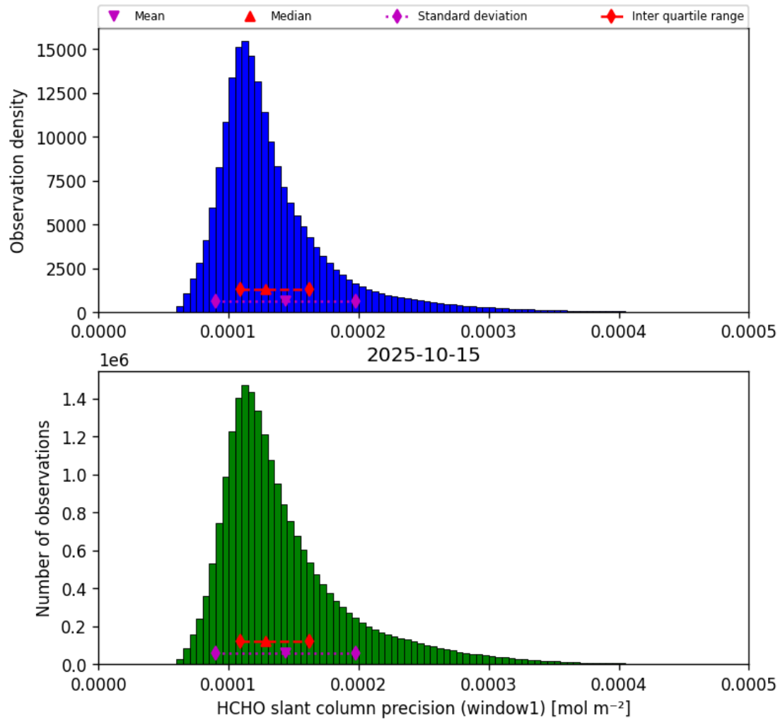
Figure 37: Histogram of “HCHO slant column precision (window1)” for 2025-10-15 to 2025-10-15
