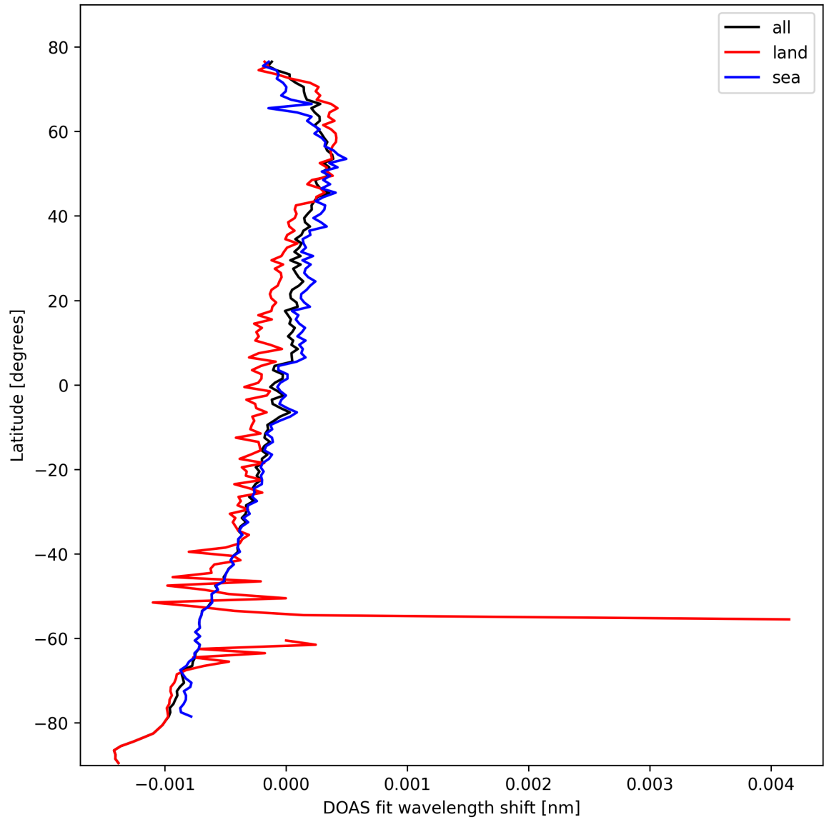
Figure 28: Zonal average of "DOAS fit wavelength shift" for 2025-10-15 to 2025-10-15.
