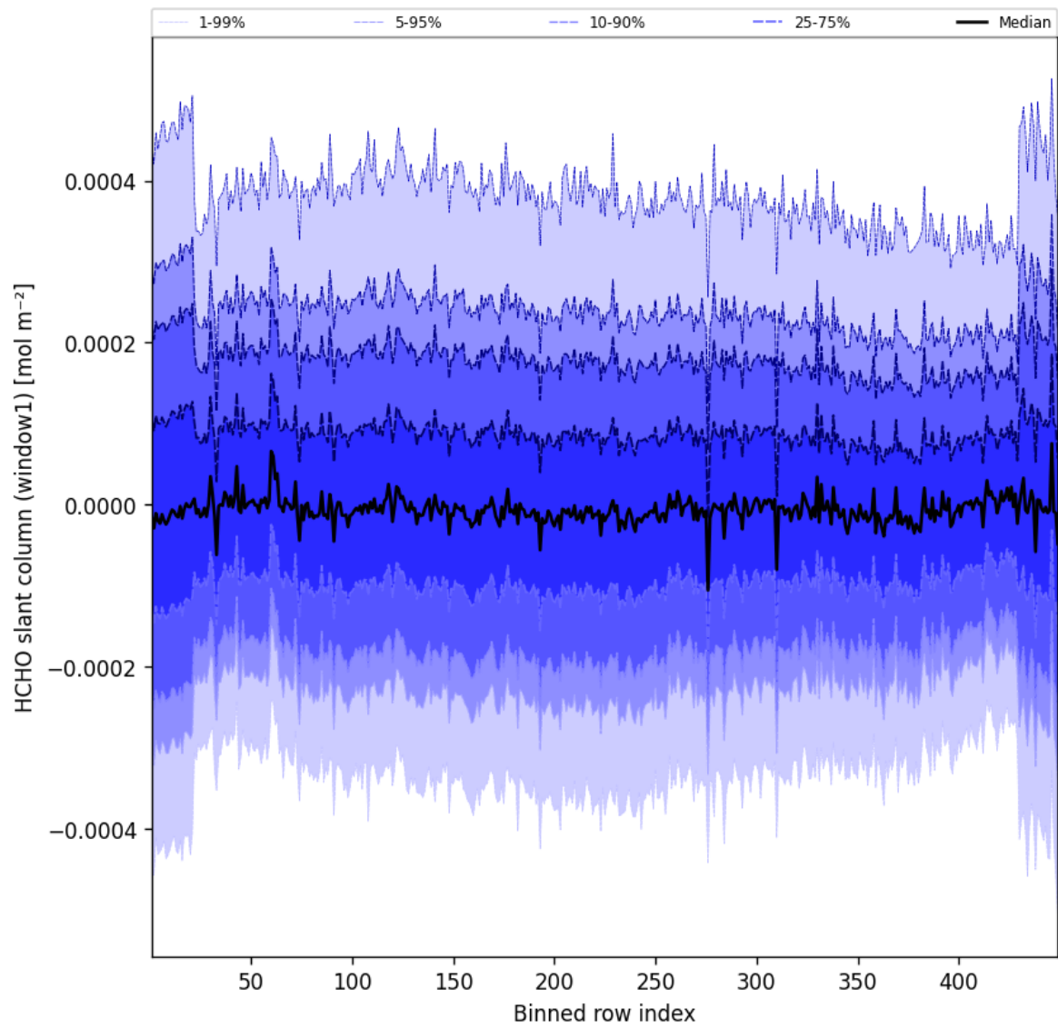
Figure 50: Along track statistics of “HCHO slant column (window1)” for 2025-10-15 to 2025-10-15
