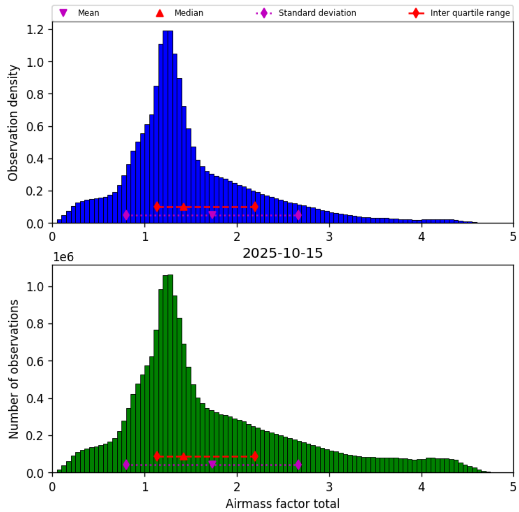
Figure 38: Histogram of “Airmass factor total” for 2025-10-15 to 2025-10-15
