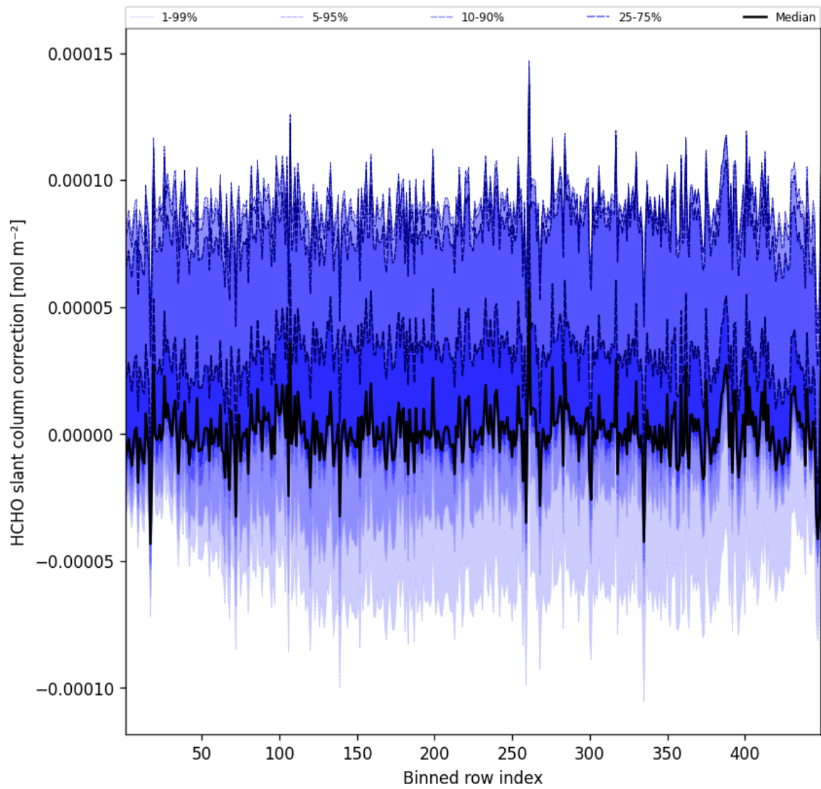
Figure 59: Along track statistics of “HCHO slant column correction” for 2025-10-15 to 2025-10-15
