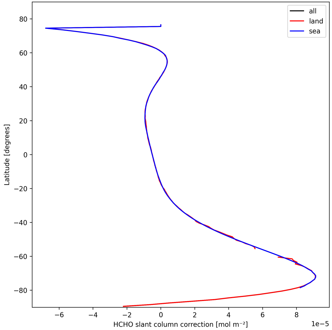
Figure 31: Zonal average of “HCHO slant column correction” for 2025-10-15 to 2025-10-15.
