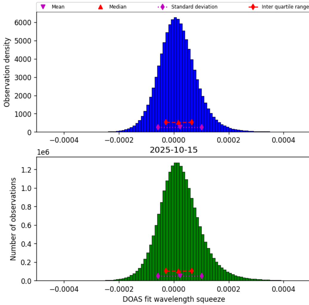
Figure 43: Histogram of “DOAS fit wavelength squeeze” for 2025-10-15 to 2025-10-15
