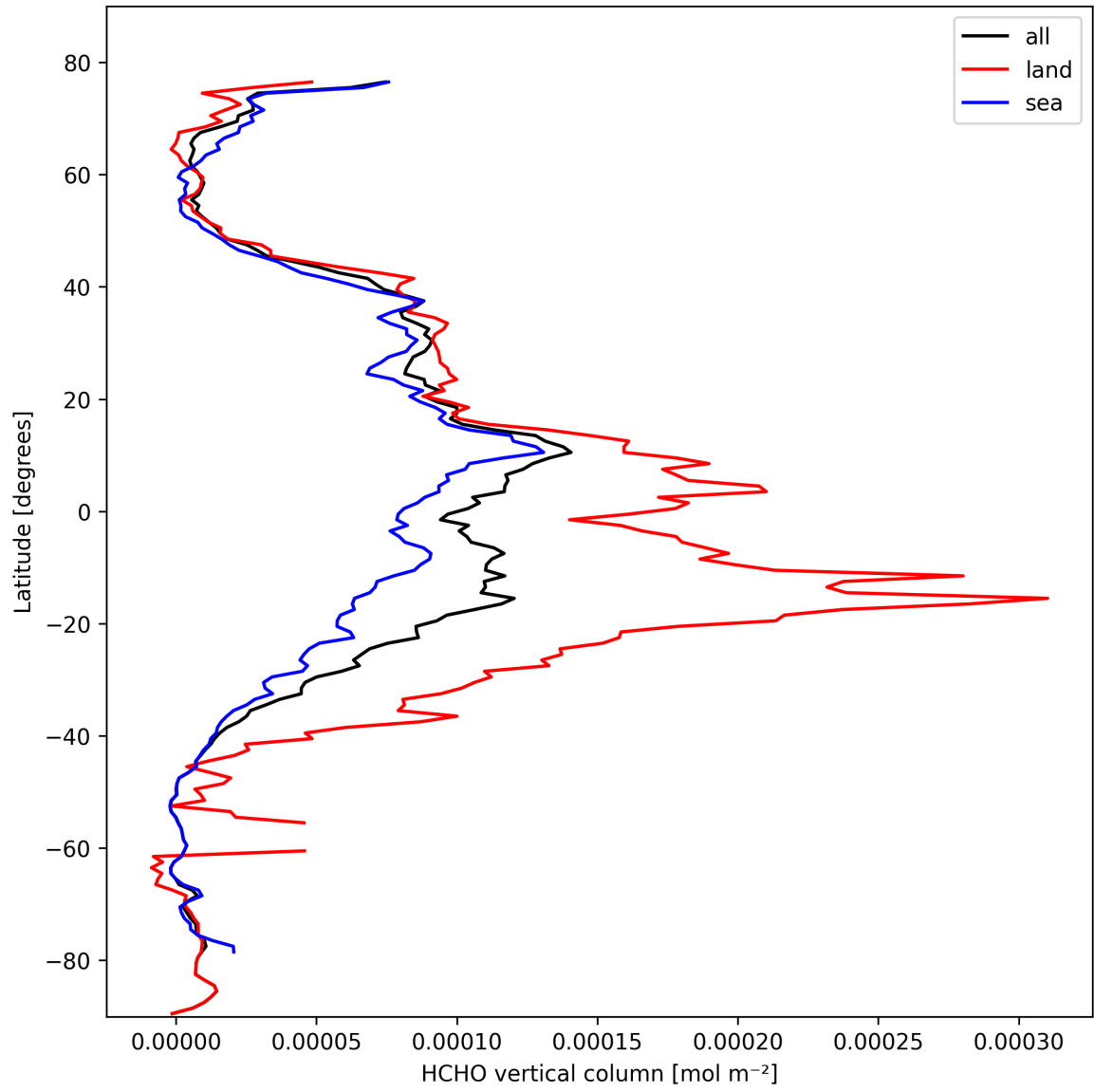
Figure 19: Zonal average of “HCHO vertical column” for 2025-10-15 to 2025-10-15.
