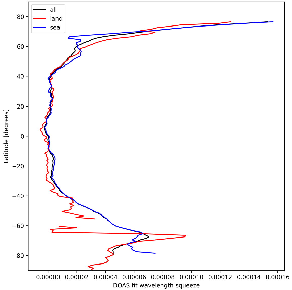
Figure 29: Zonal average of “DOAS fit wavelength squeeze” for 2025-10-15 to 2025-10-15.
