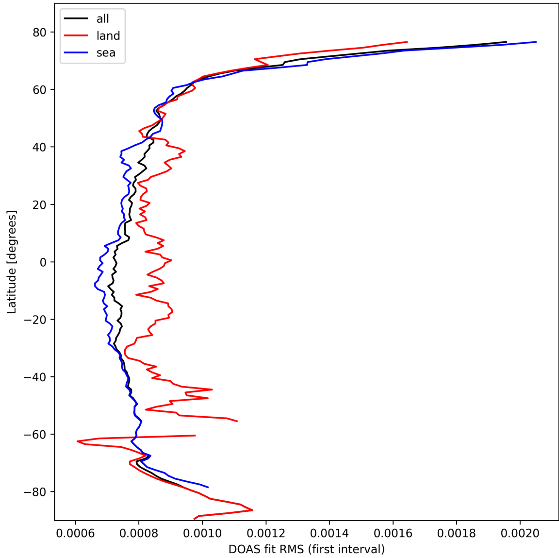
Figure 30: Zonal average of “DOAS fit RMS (first interval)” for 2025-10-15 to 2025-10-15.
