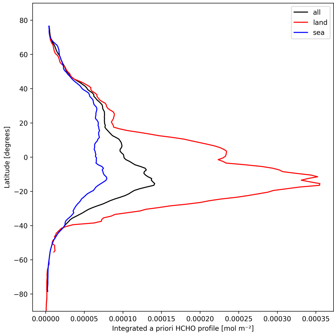
Figure 27: Zonal average of “Integrated a priori HCHO profile” for 2025-10-15 to 2025-10-15.
