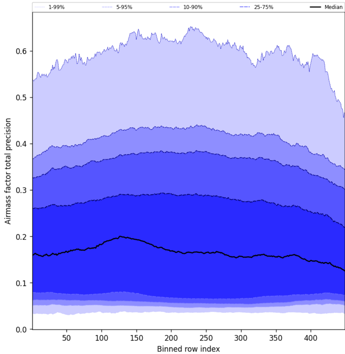
Figure 53: Along track statistics of “Airmass factor total precision” for 2025-10-15 to 2025-10-15
