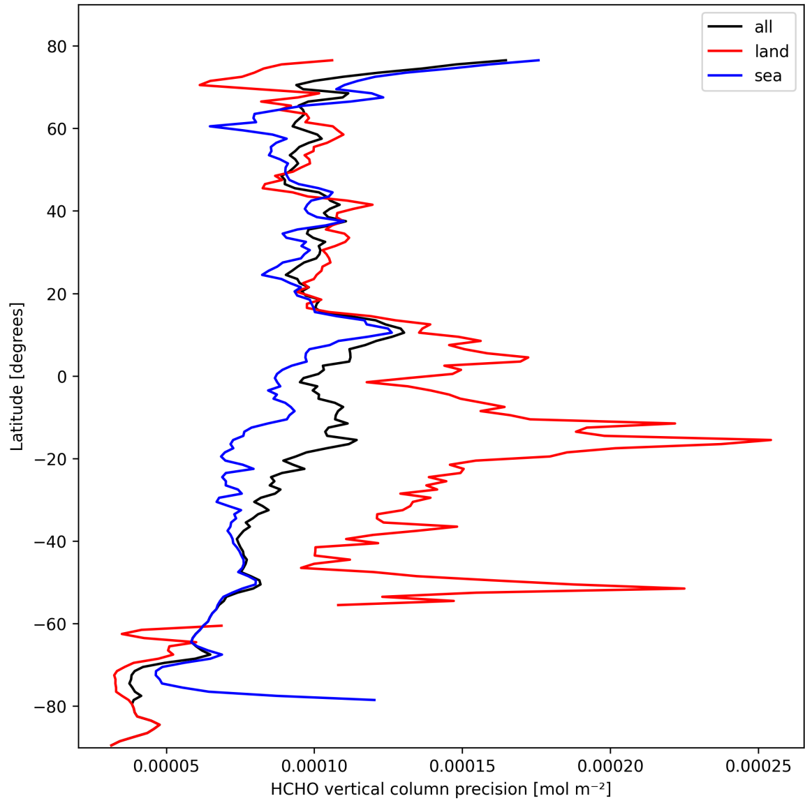
Figure 20: Zonal average of “HCHO vertical column precision” for 2025-10-15 to 2025-10-15.
