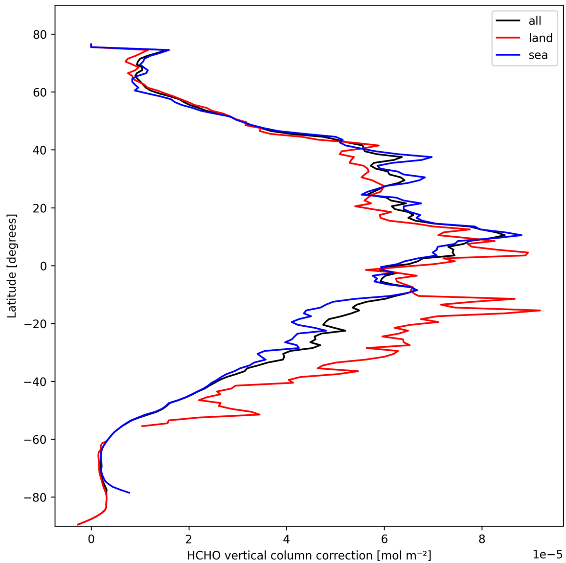
Figure 21: Zonal average of “HCHO vertical column correction” for 2025-10-15 to 2025-10-15.
