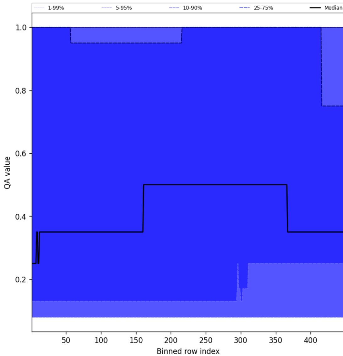
Figure 46: Along track statistics of “QA value” for 2025-10-15 to 2025-10-15
