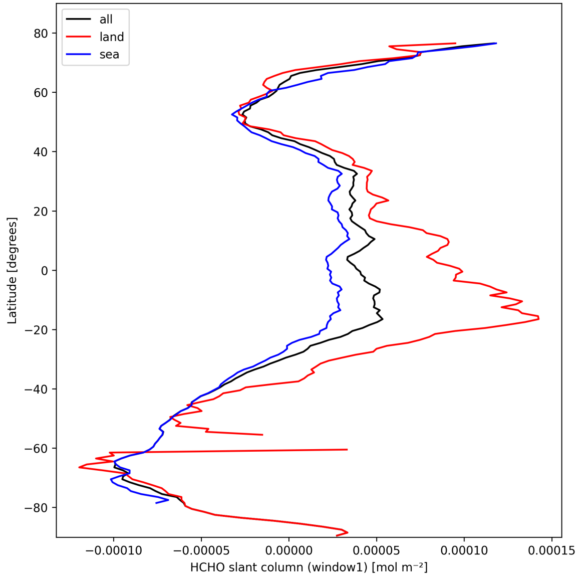
Figure 22: Zonal average of “HCHO slant column (window1)” for 2025-10-15 to 2025-10-15.
