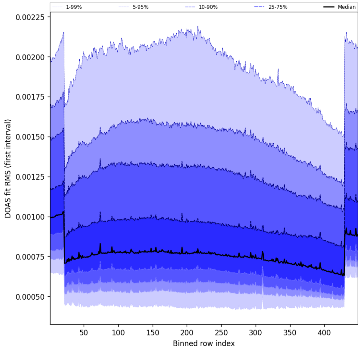
Figure 58: Along track statistics of “DOAS fit RMS (first interval)” for 2025-10-15 to 2025-10-15
