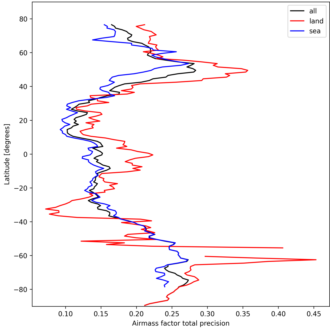
Figure 25: Zonal average of “Airmass factor total precision” for 2025-10-15 to 2025-10-15.
