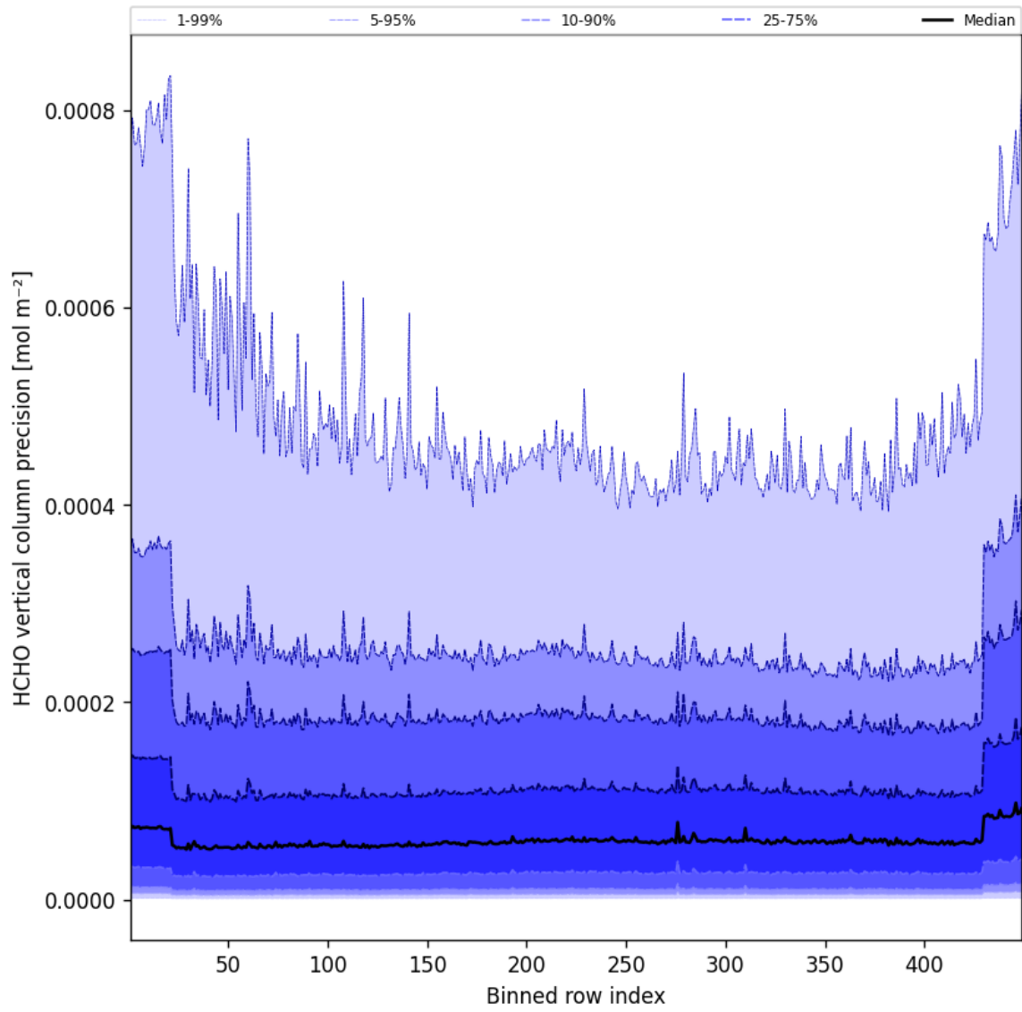
Figure 48: Along track statistics of “HCHO vertical column precision” for 2025-10-15 to 2025-10-15
