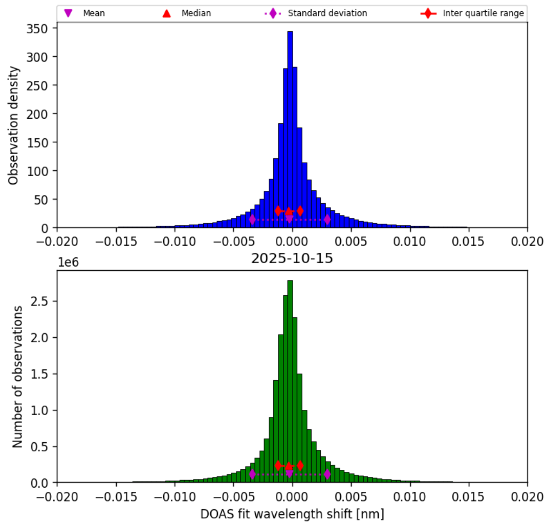
Figure 42: Histogram of “DOAS fit wavelength shift” for 2025-10-15 to 2025-10-15
