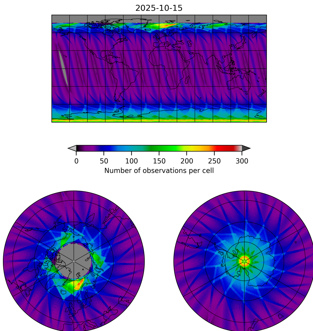
Figure 17: Map of the number of observations for 2025-10-15 to 2025-10-15
