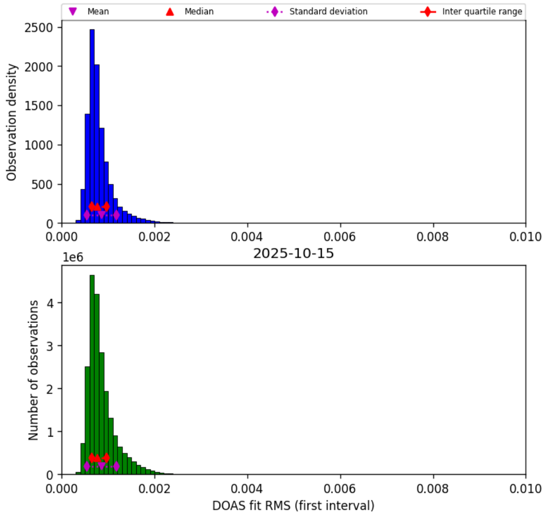
Figure 44: Histogram of “DOAS fit RMS (first interval)” for 2025-10-15 to 2025-10-15
