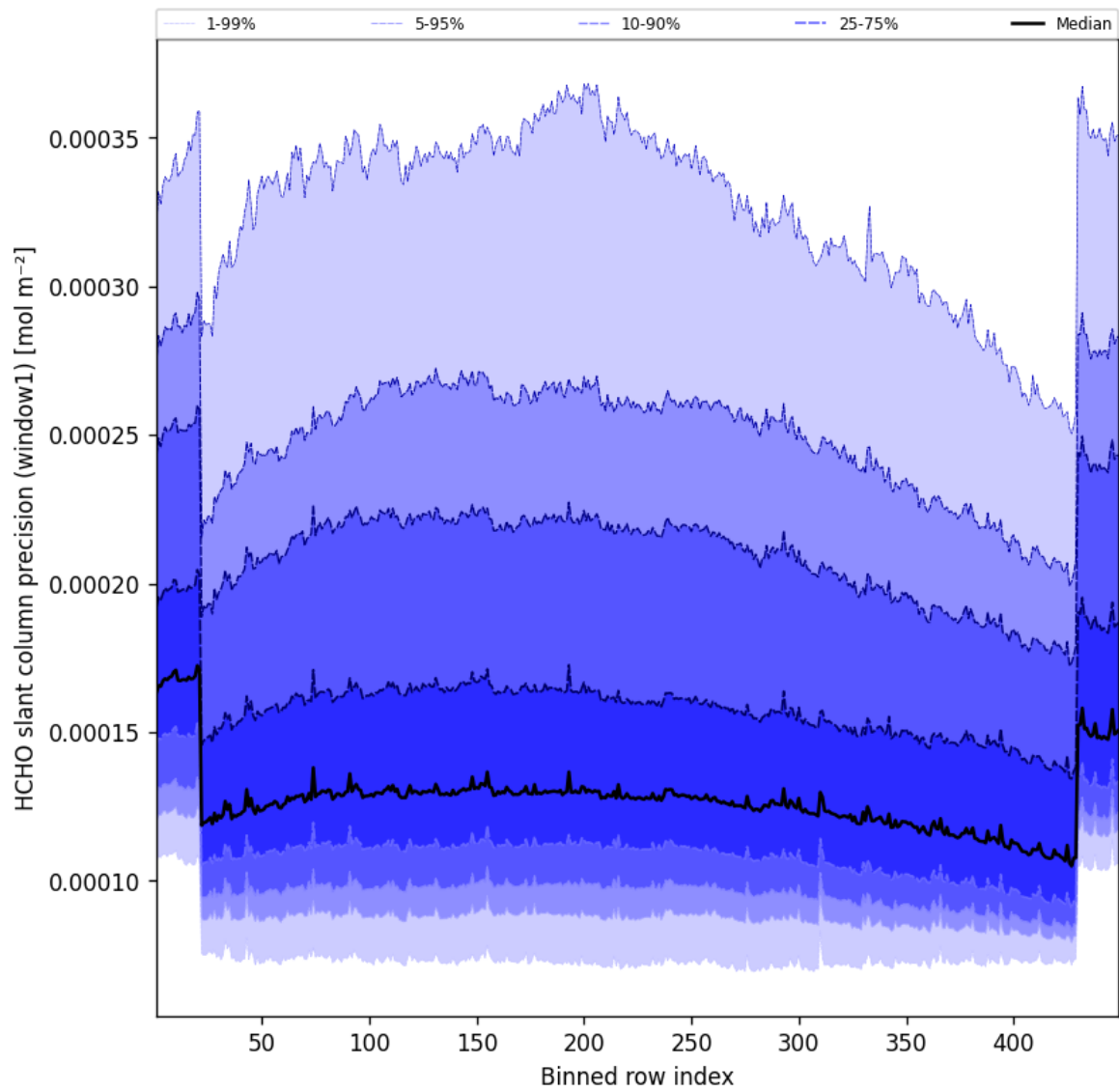
Figure 51: Along track statistics of “HCHO slant column precision (window1)” for 2025-10-15 to 2025-10-15
