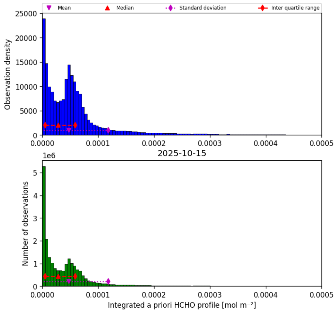
Figure 41: Histogram of “Integrated a priori HCHO profile” for 2025-10-15 to 2025-10-15
