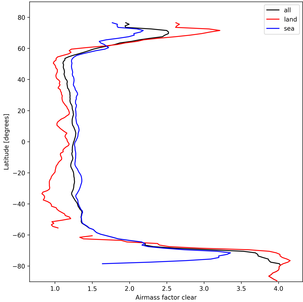
Figure 26: Zonal average of “Airmass factor clear” for 2025-10-15 to 2025-10-15.
