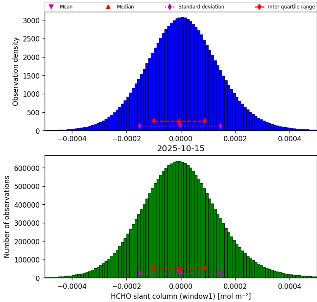
Figure 36: Histogram of "HCHO slant column (window1)" for 2025-10-15 to 2025-10-15
