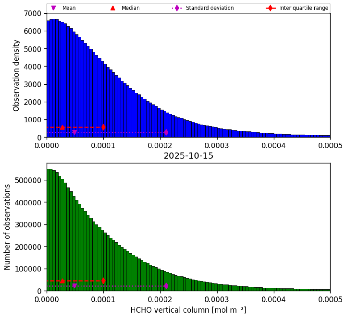
Figure 33: Histogram of “HCHO vertical column” for 2025-10-15 to 2025-10-15
