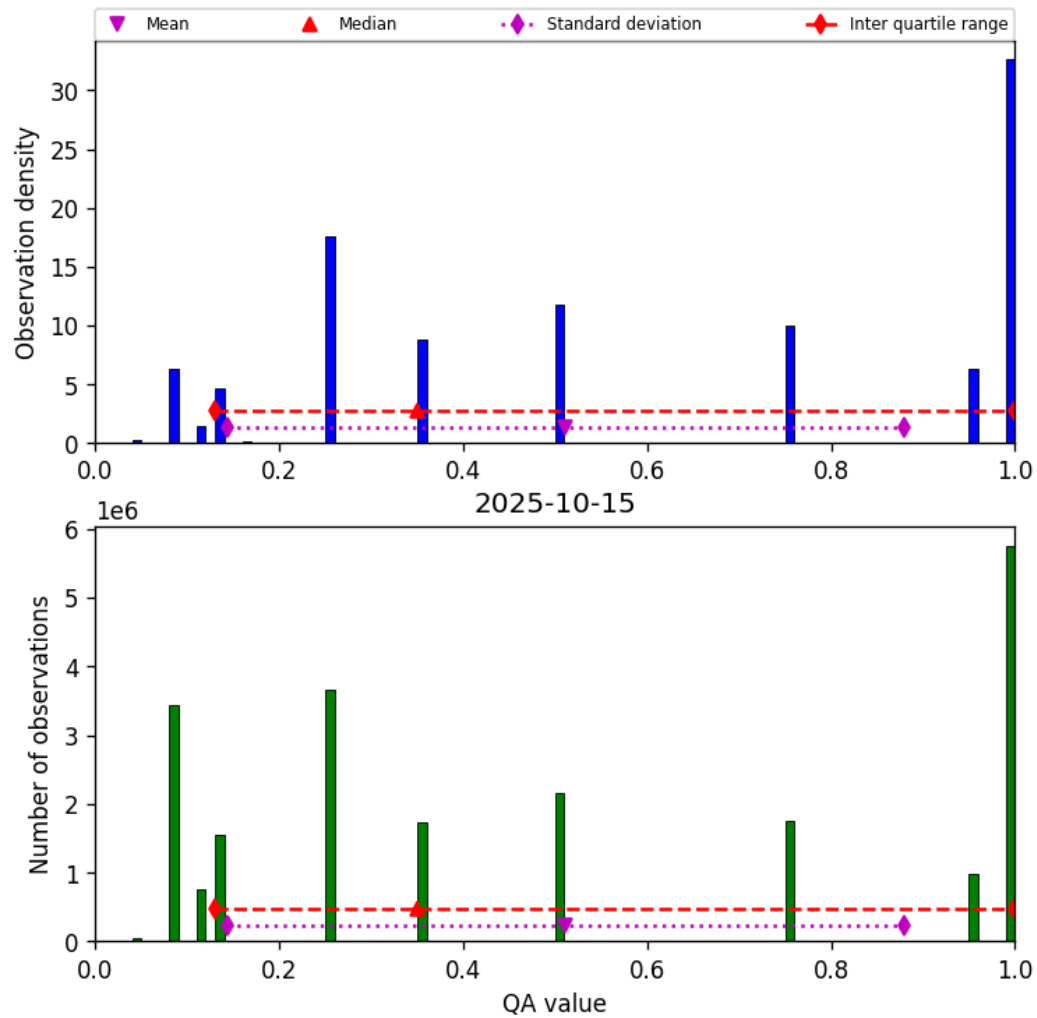
Figure 32: Histogram of “QA value” for 2025-10-15 to 2025-10-15
