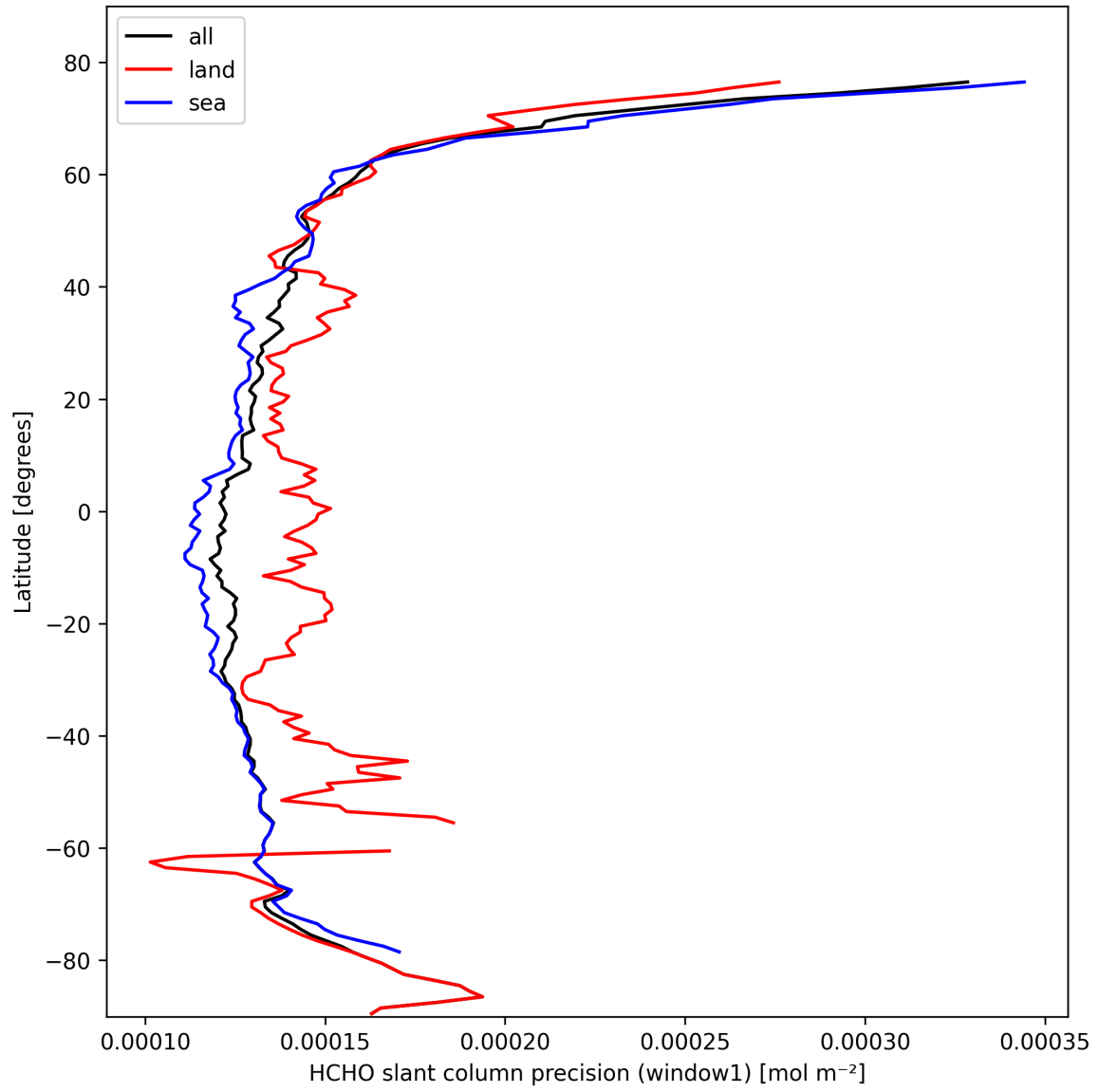
Figure 23: Zonal average of “HCHO slant column precision (window1)” for 2025-10-15 to 2025-10-15.
