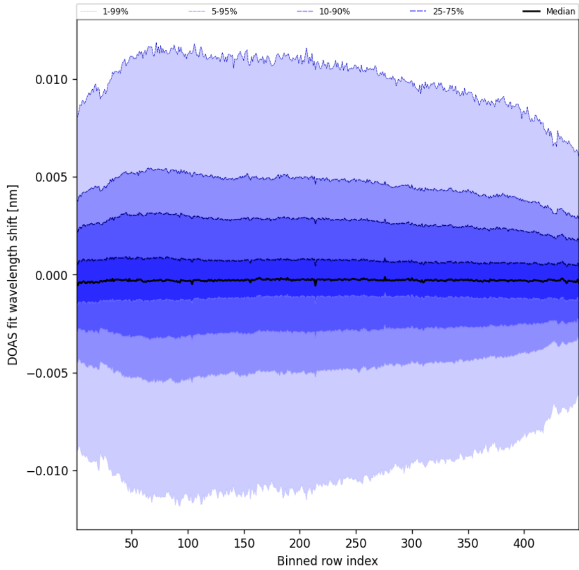
Figure 56: Along track statistics of “DOAS fit wavelength shift” for 2025-10-15 to 2025-10-15
