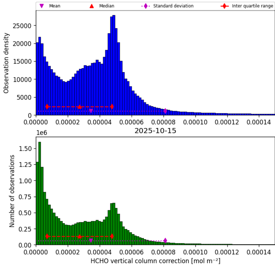
Figure 35: Histogram of “HCHO vertical column correction” for 2025-10-15 to 2025-10-15
