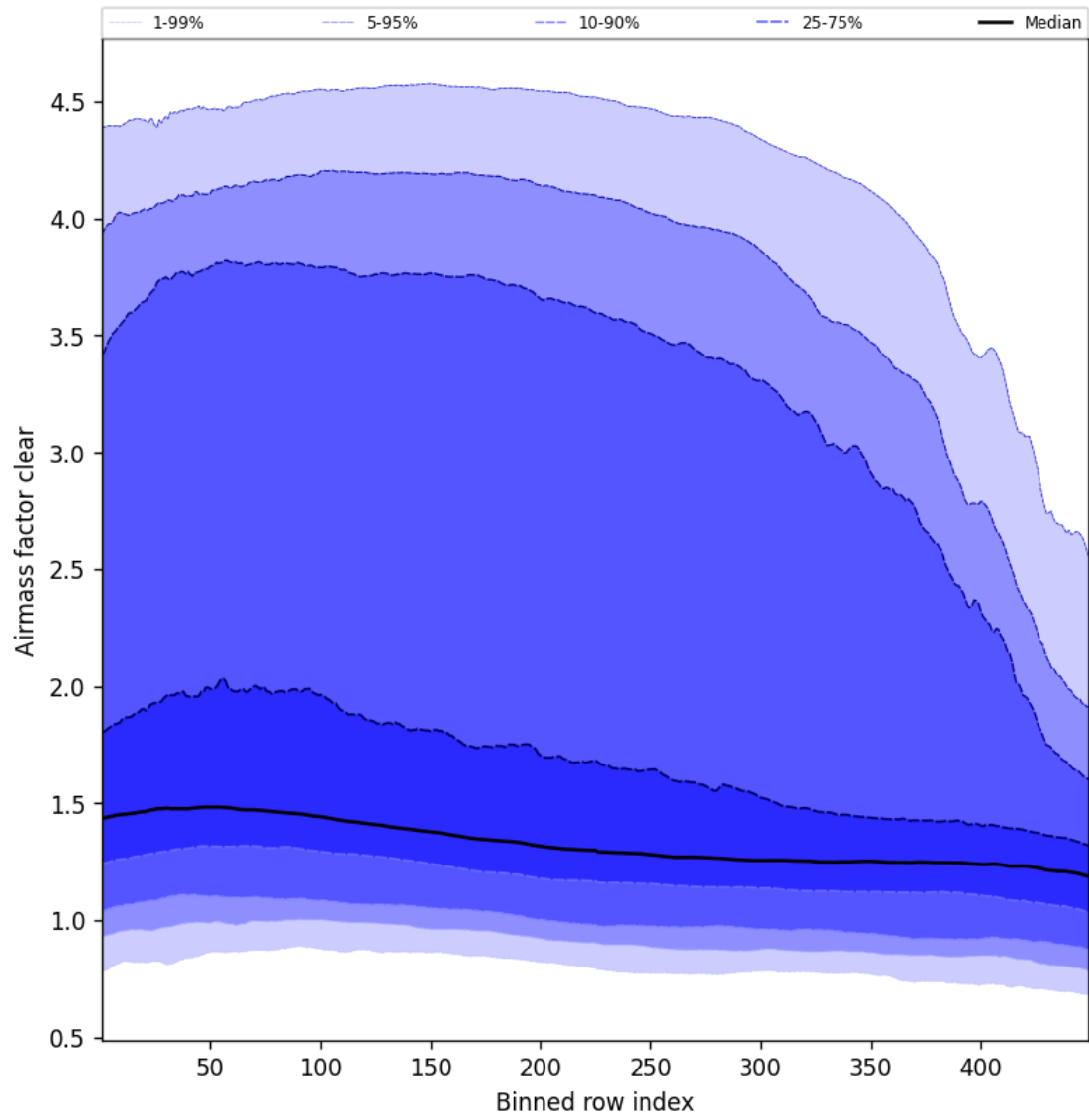
Figure 54: Along track statistics of “Airmass factor clear” for 2025-10-15 to 2025-10-15
