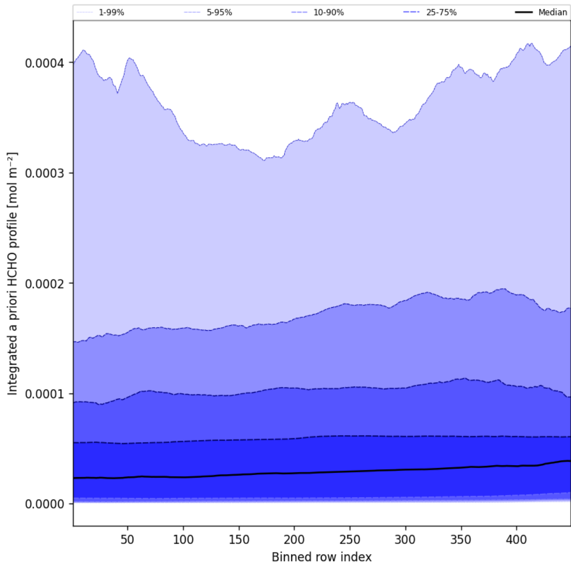
Figure 55: Along track statistics of “Integrated a priori HCHO profile” for 2025-10-15 to 2025-10-15
