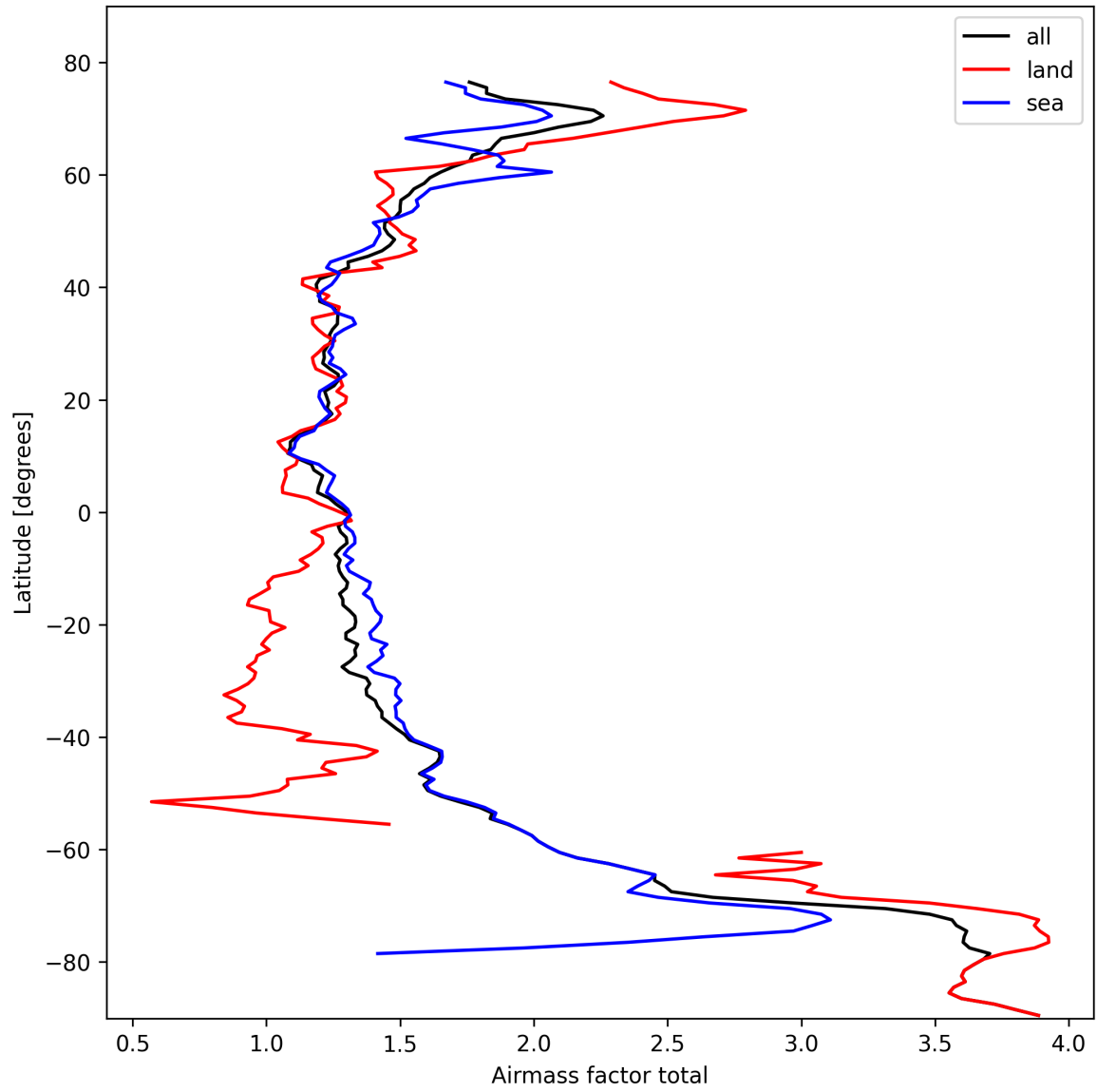
Figure 24: Zonal average of “Airmass factor total” for 2025-10-15 to 2025-10-15.
