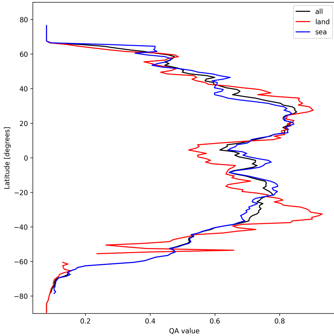
Figure 18: Zonal average of “QA value” for 2025-10-15 to 2025-10-15.
