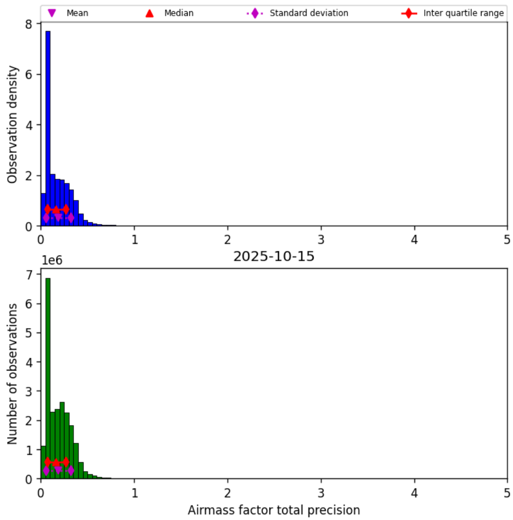
Figure 39: Histogram of “Airmass factor total precision” for 2025-10-15 to 2025-10-15
