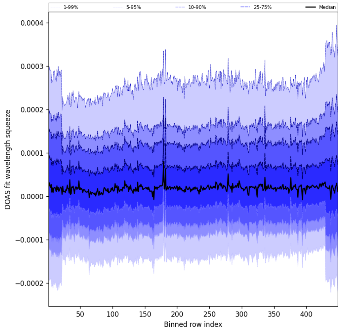
Figure 57: Along track statistics of “DOAS fit wavelength squeeze” for 2025-10-16 to 2025-10-17
