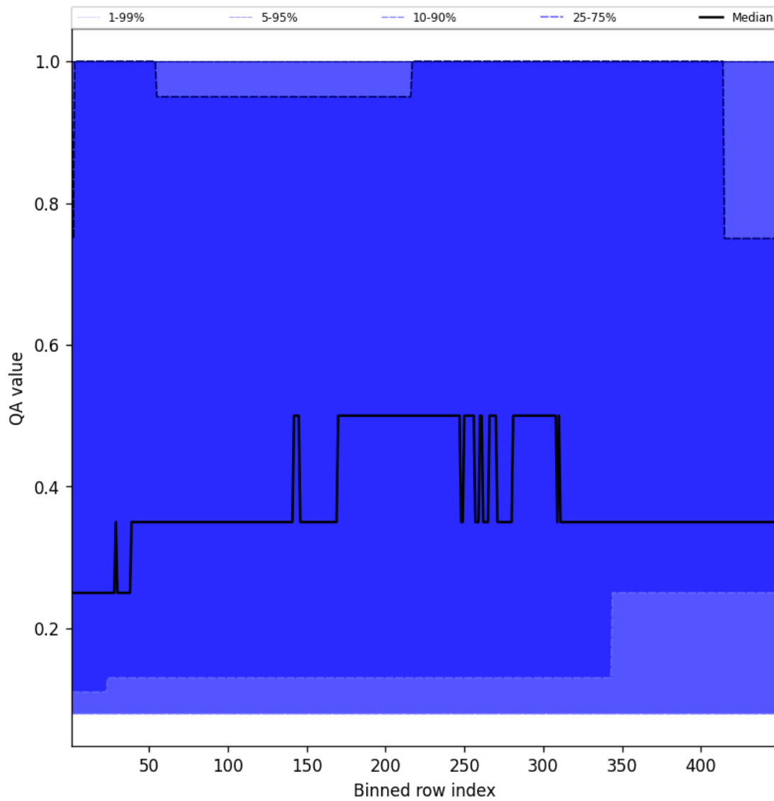
Figure 46: Along track statistics of “QA value” for 2025-10-16 to 2025-10-17
