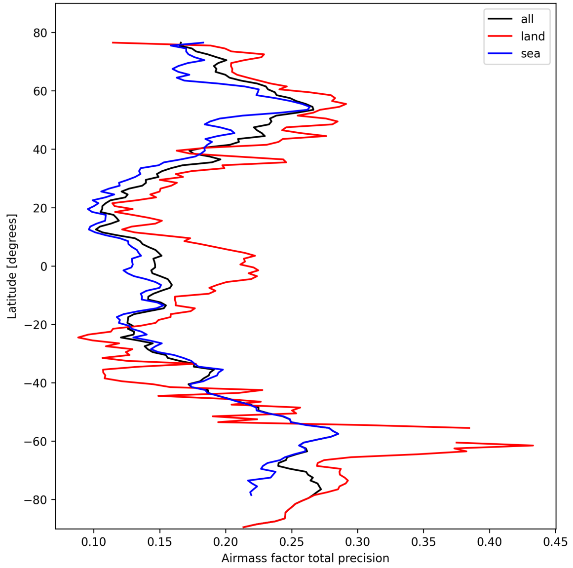
Figure 25: Zonal average of “Airmass factor total precision” for 2025-10-16 to 2025-10-17.
