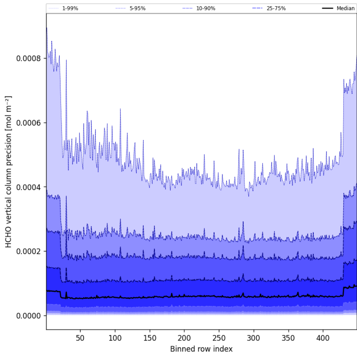
Figure 48: Along track statistics of “HCHO vertical column precision” for 2025-10-16 to 2025-10-17
