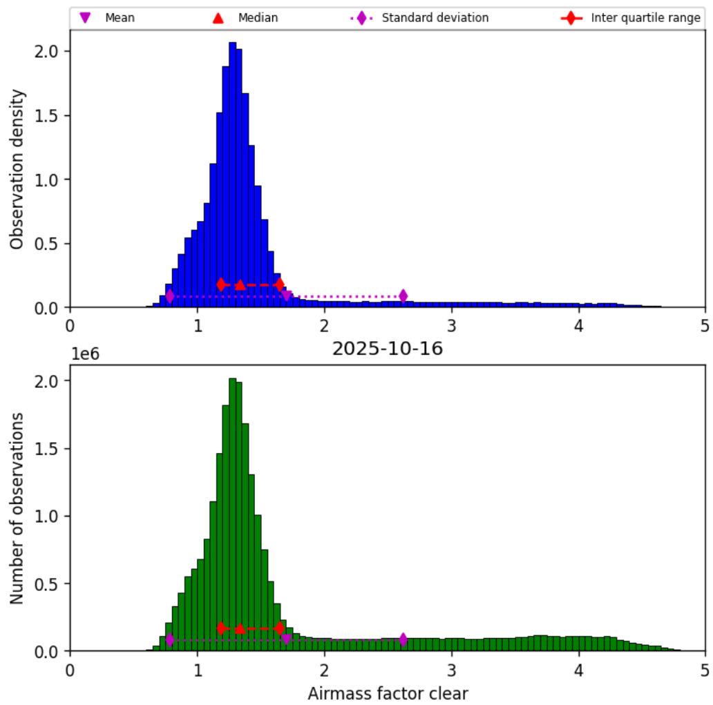
Figure 40: Histogram of “Airmass factor clear” for 2025-10-16 to 2025-10-17
