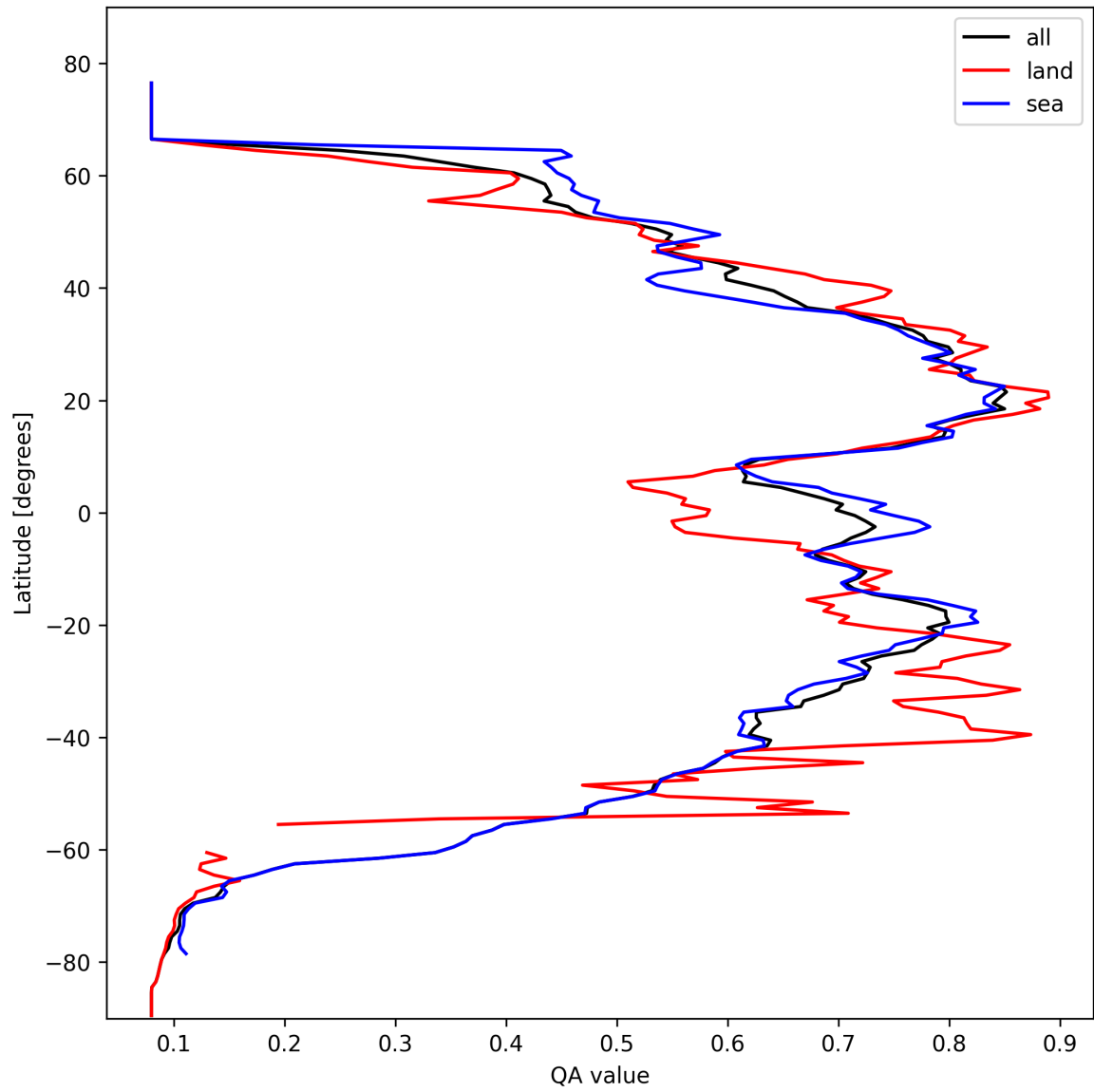
Figure 18: Zonal average of “QA value” for 2025-10-16 to 2025-10-17.
