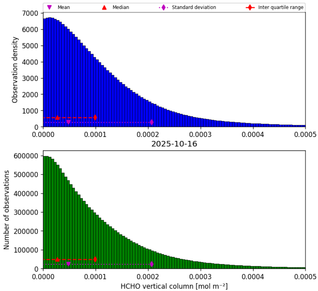
Figure 33: Histogram of “HCHO vertical column” for 2025-10-16 to 2025-10-17
