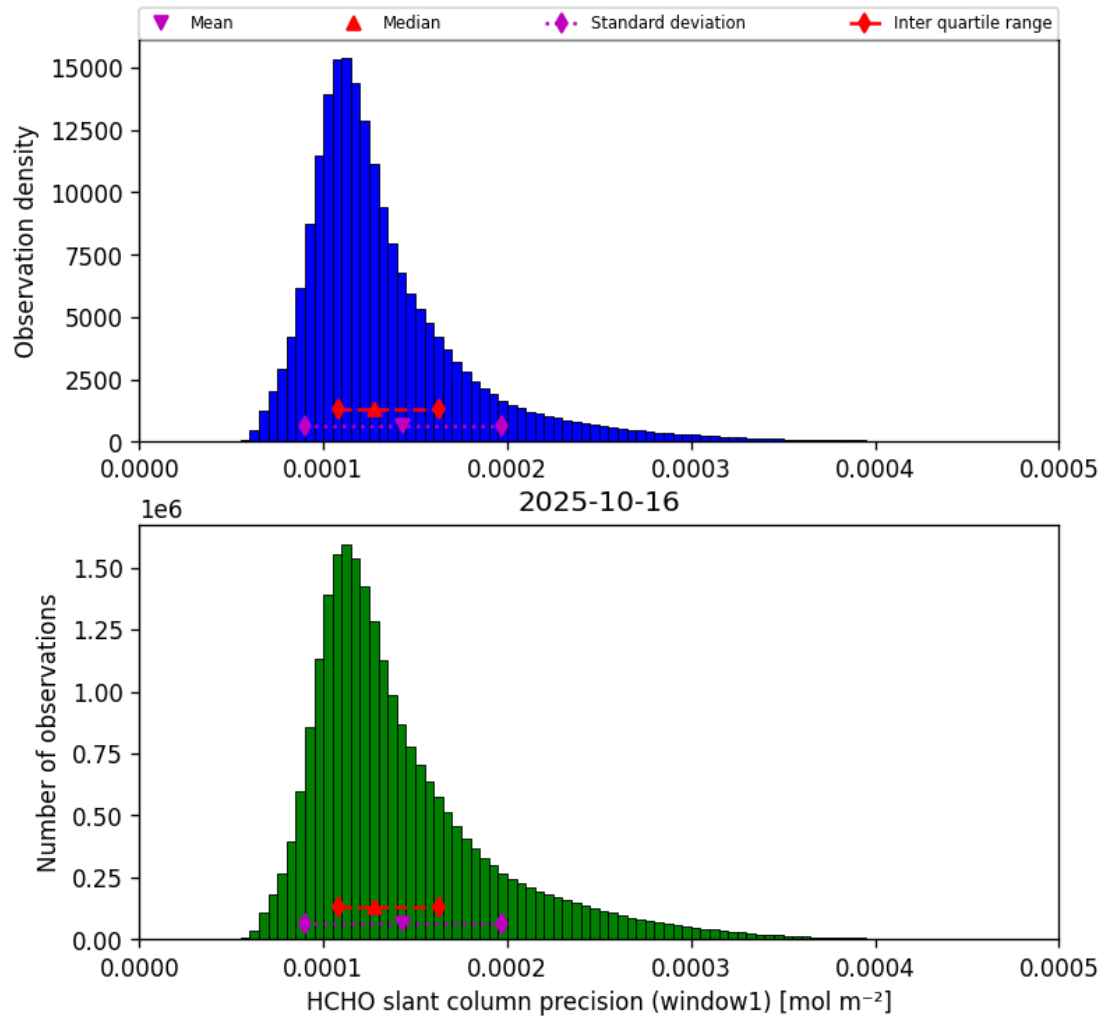
Figure 37: Histogram of “HCHO slant column precision (window1)” for 2025-10-16 to 2025-10-17
