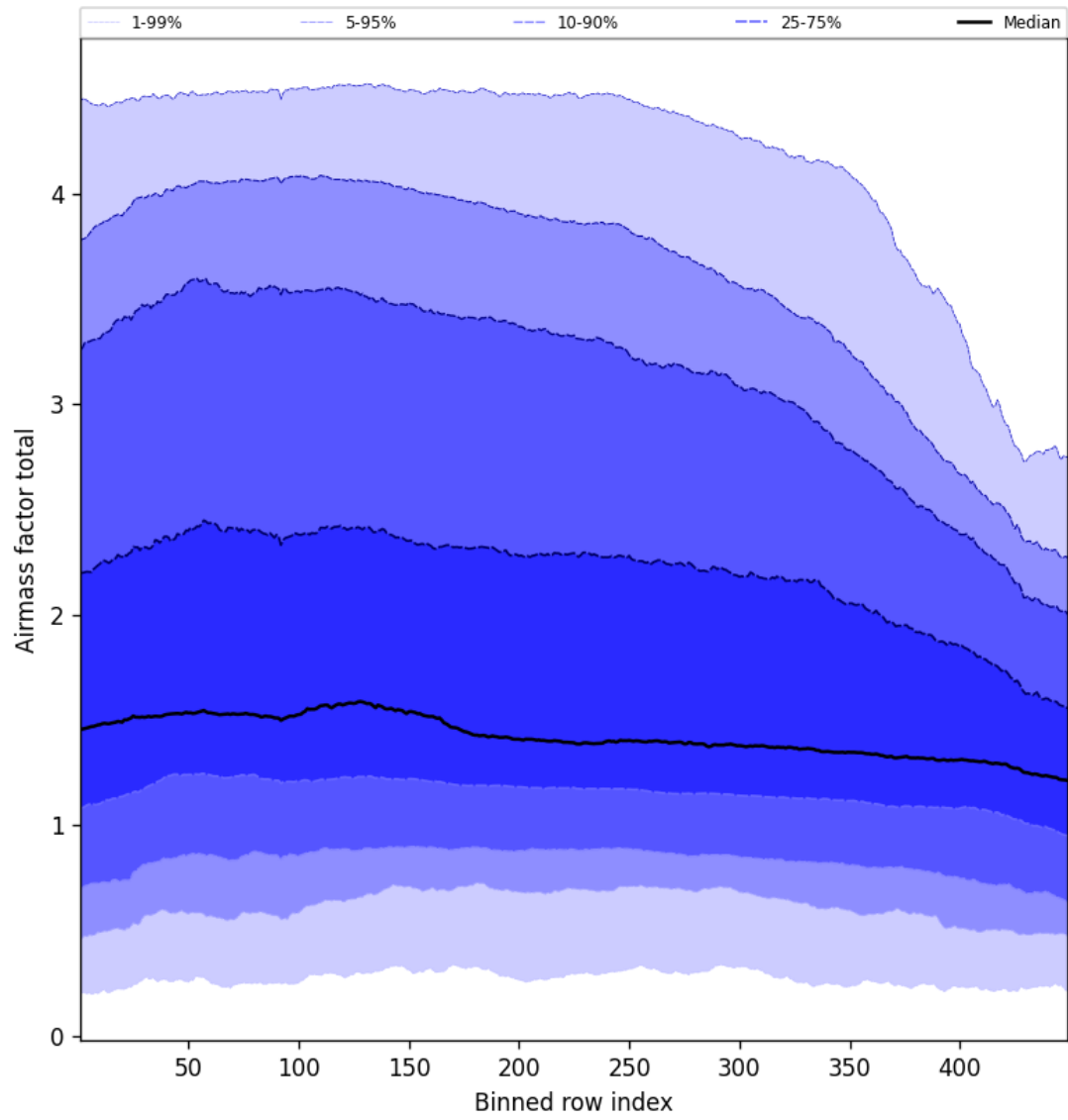
Figure 52: Along track statistics of “Airmass factor total” for 2025-10-16 to 2025-10-17
