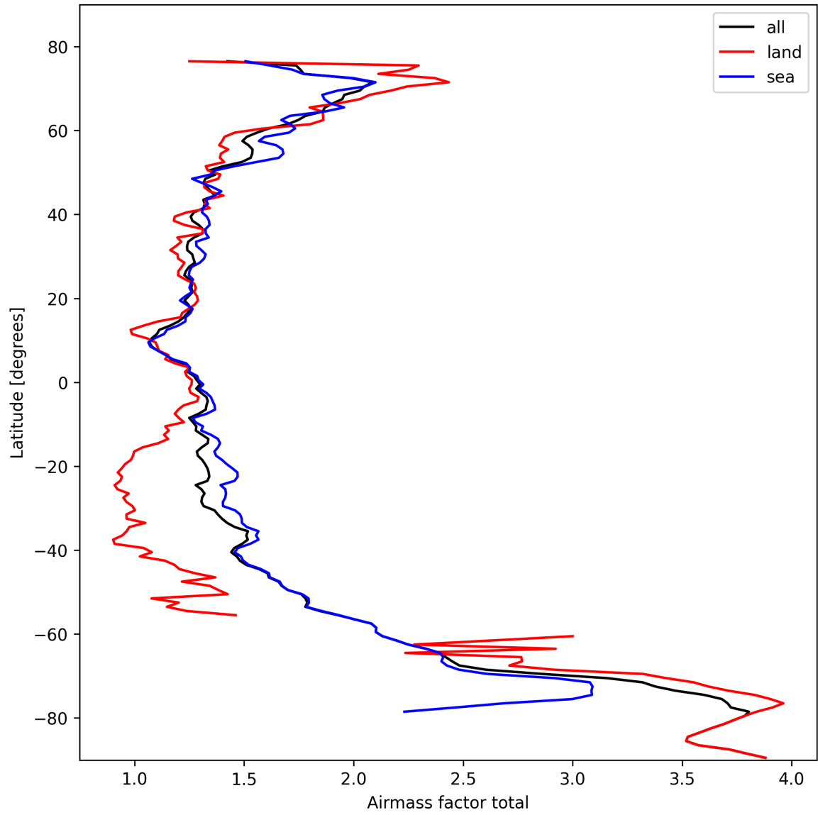
Figure 24: Zonal average of “Airmass factor total” for 2025-10-16 to 2025-10-17.
