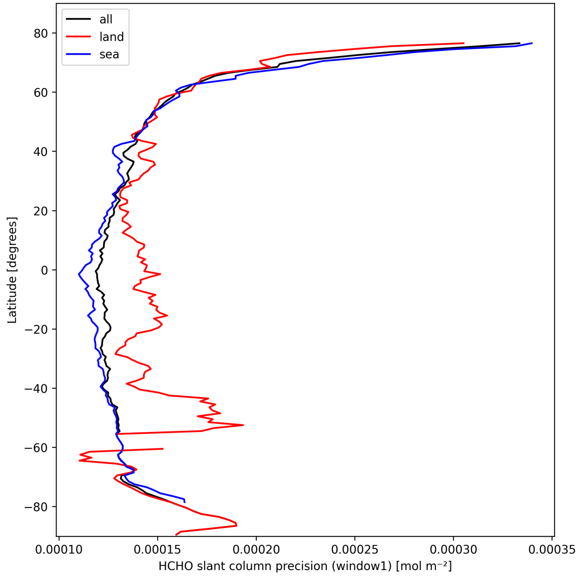
Figure 23: Zonal average of “HCHO slant column precision (window1)” for 2025-10-16 to 2025-10-17.
