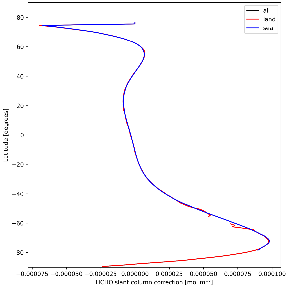
Figure 31: Zonal average of “HCHO slant column correction” for 2025-10-16 to 2025-10-17.
