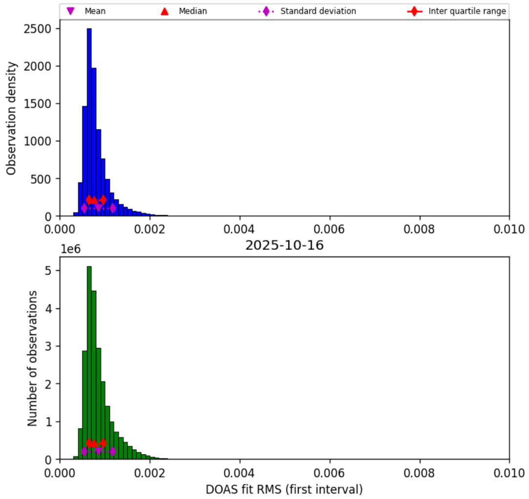
Figure 44: Histogram of “DOAS fit RMS (first interval)” for 2025-10-16 to 2025-10-17
