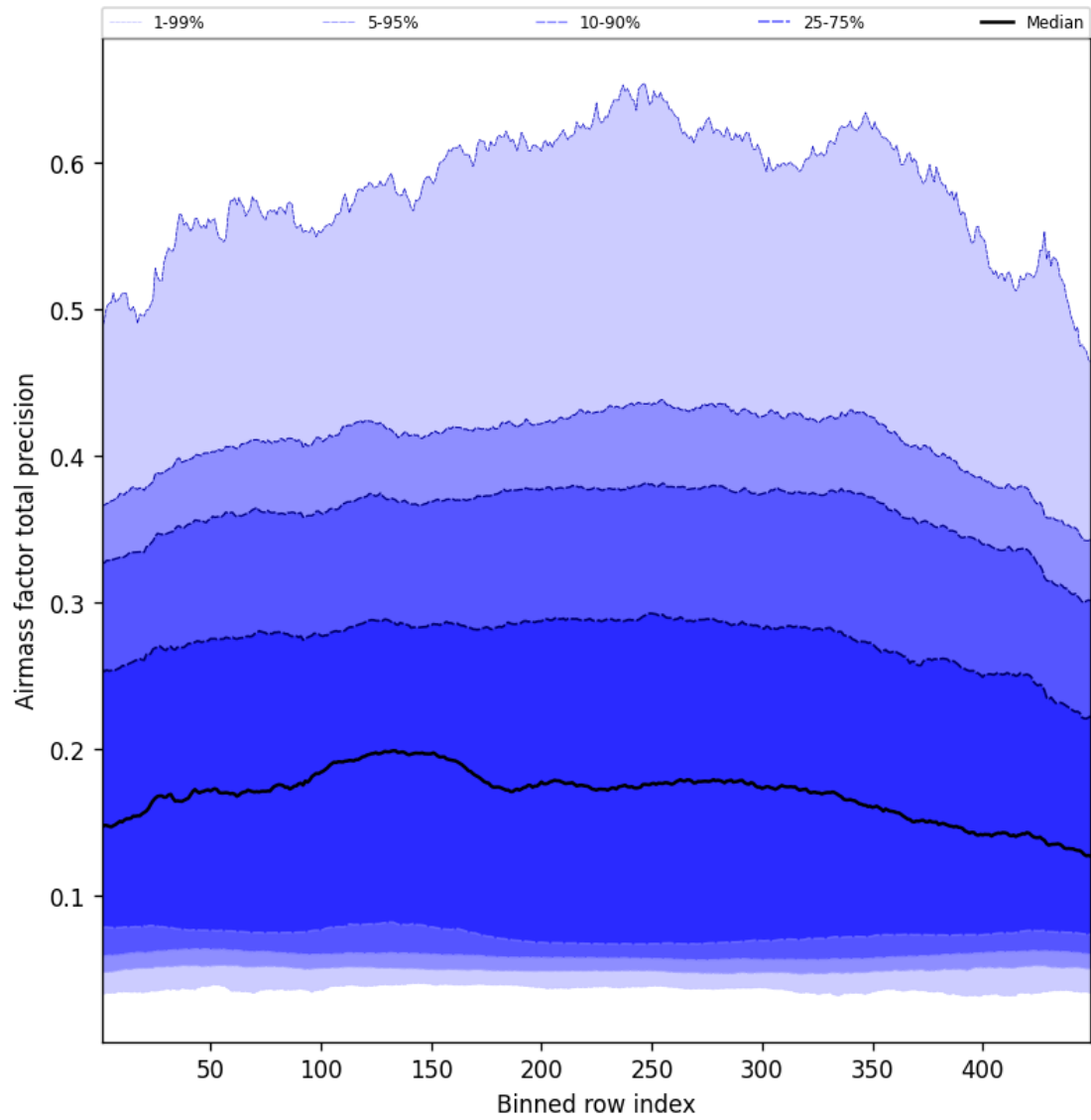
Figure 53: Along track statistics of “Airmass factor total precision” for 2025-10-16 to 2025-10-17
