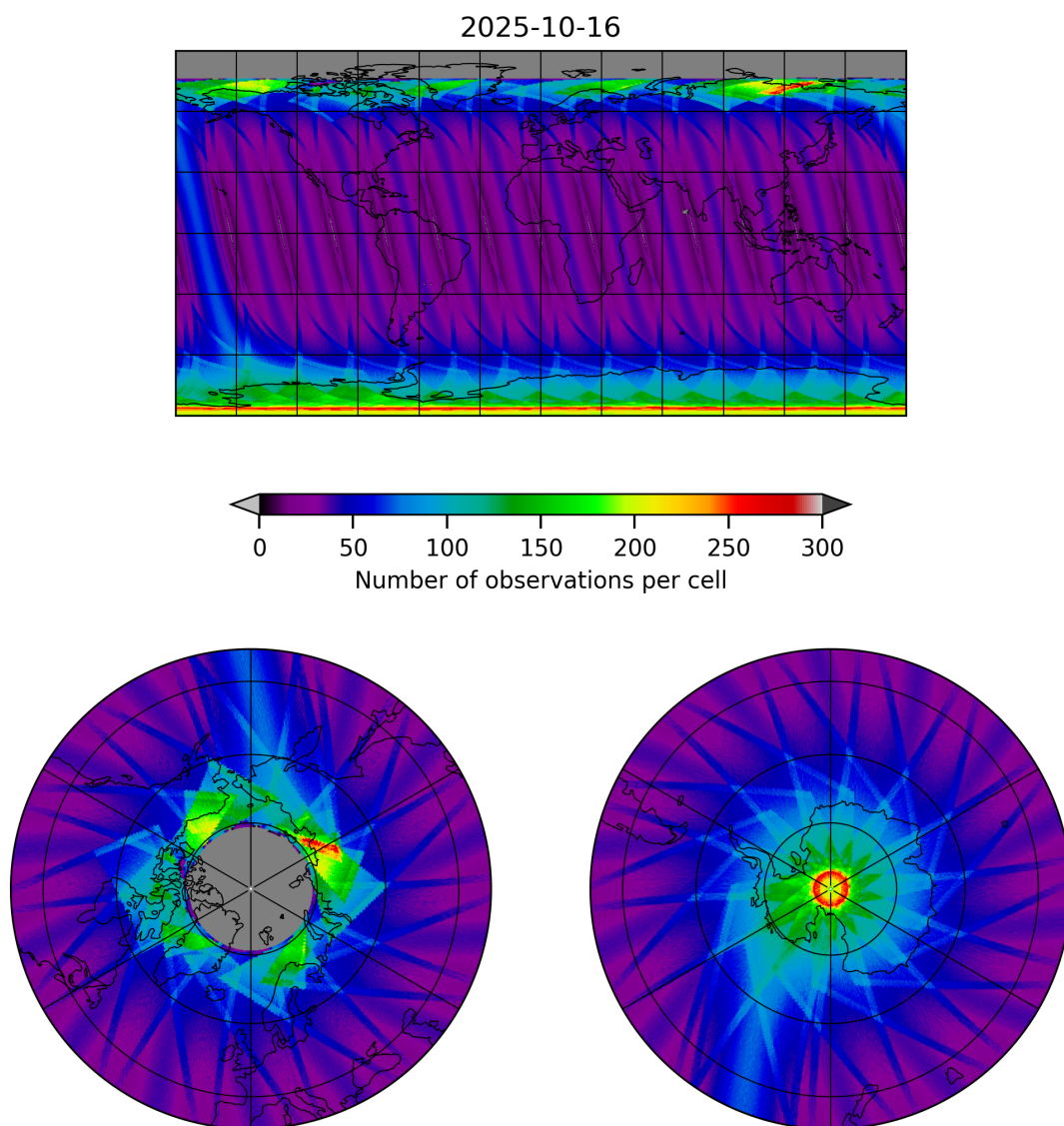
Figure 17: Map of the number of observations for 2025-10-16 to 2025-10-17
