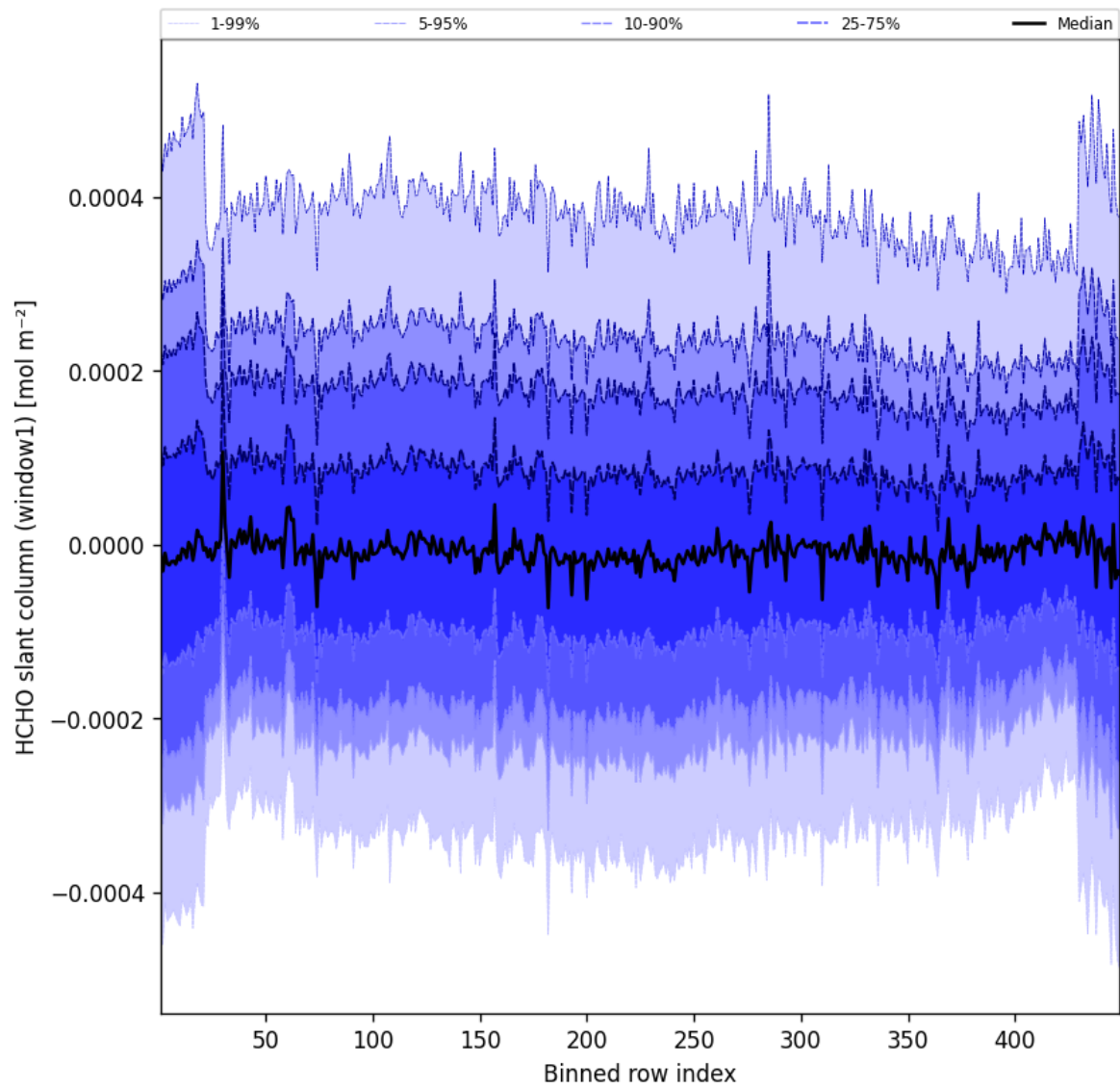
Figure 50: Along track statistics of “HCHO slant column (window1)” for 2025-10-16 to 2025-10-17
