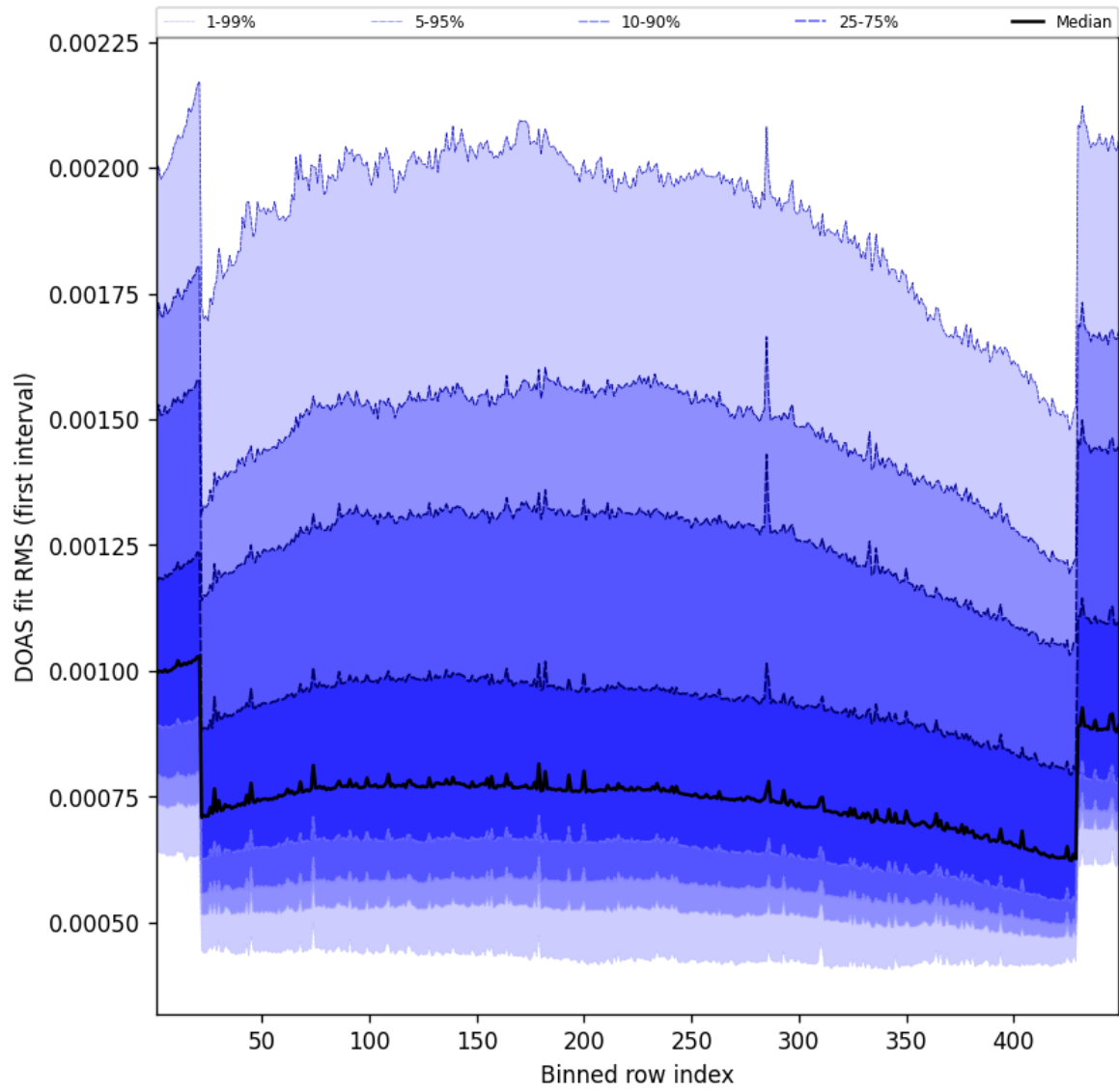
Figure 58: Along track statistics of “DOAS fit RMS (first interval)” for 2025-10-16 to 2025-10-17
