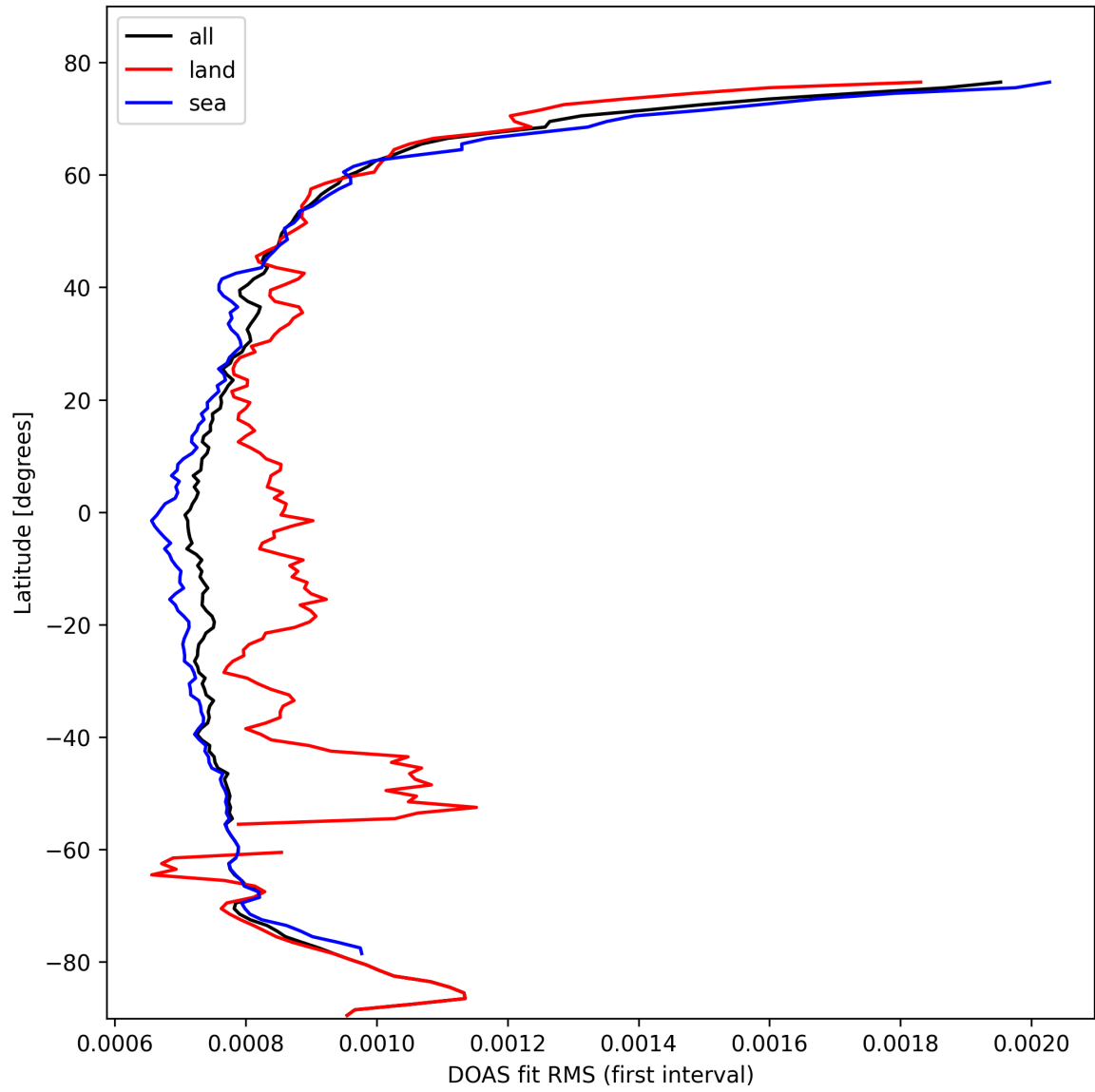
Figure 30: Zonal average of “DOAS fit RMS (first interval)” for 2025-10-16 to 2025-10-17.
