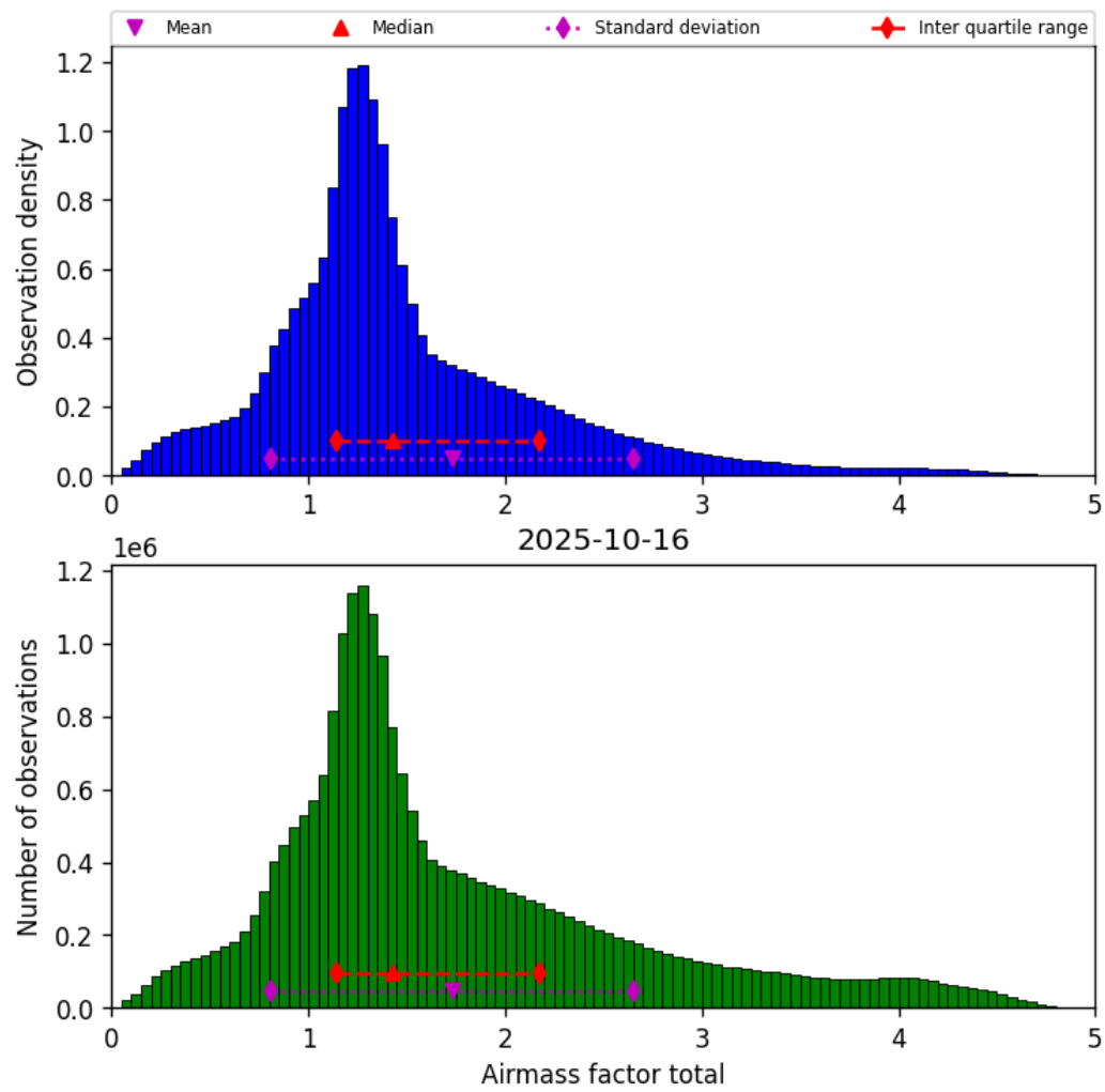
Figure 38: Histogram of “Airmass factor total” for 2025-10-16 to 2025-10-17
