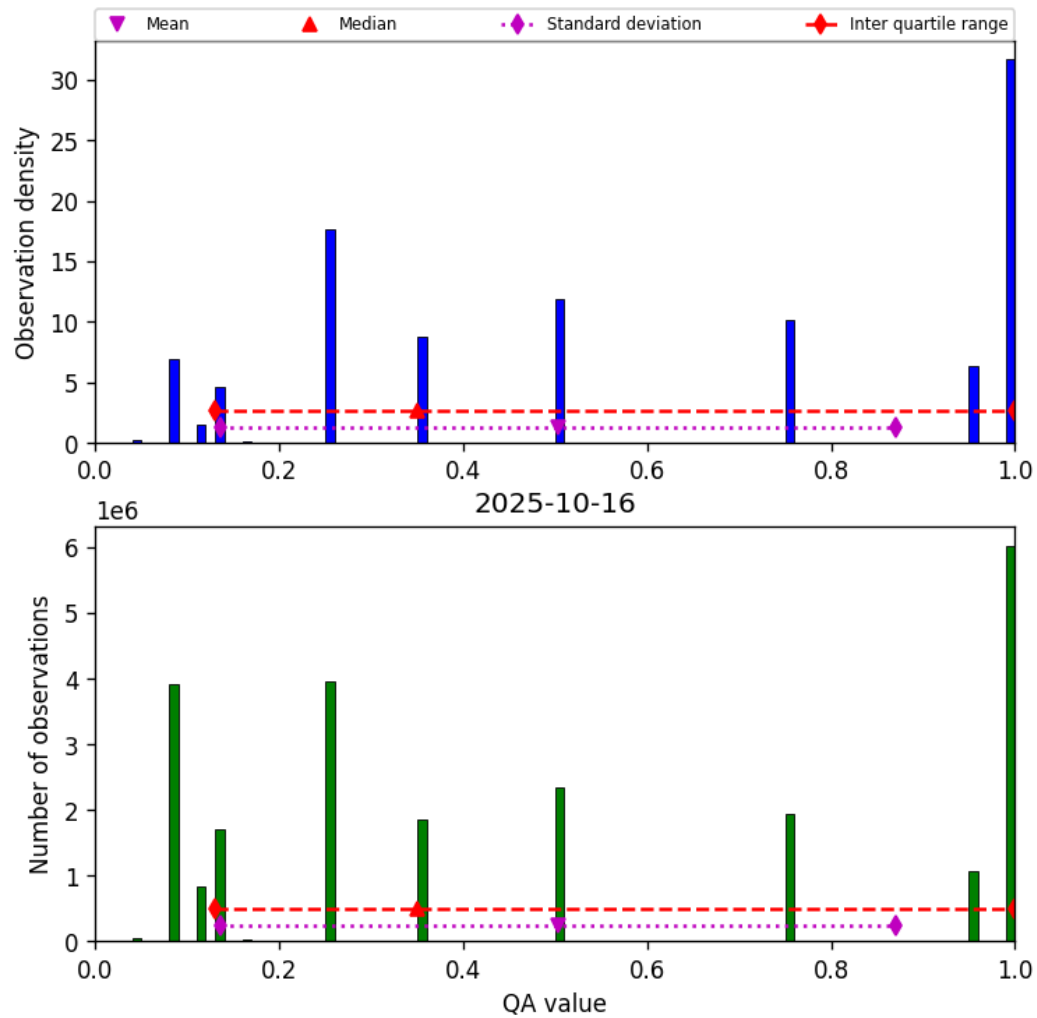
Figure 32: Histogram of “QA value” for 2025-10-16 to 2025-10-17
