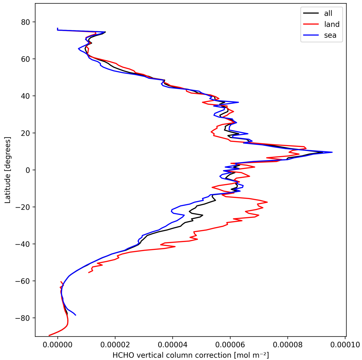
Figure 21: Zonal average of “HCHO vertical column correction” for 2025-10-16 to 2025-10-17.
