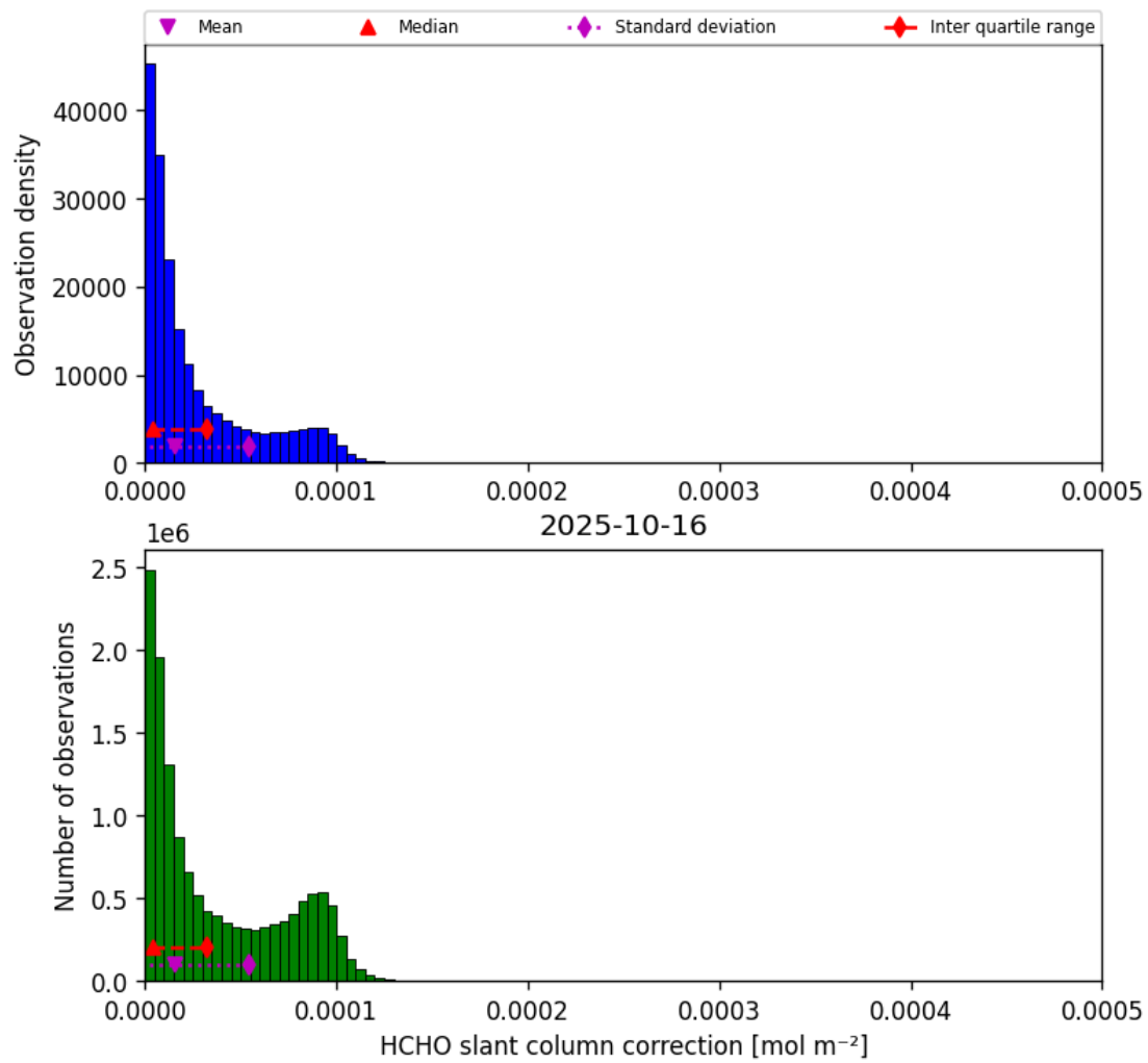
Figure 45: Histogram of “HCHO slant column correction” for 2025-10-16 to 2025-10-17
