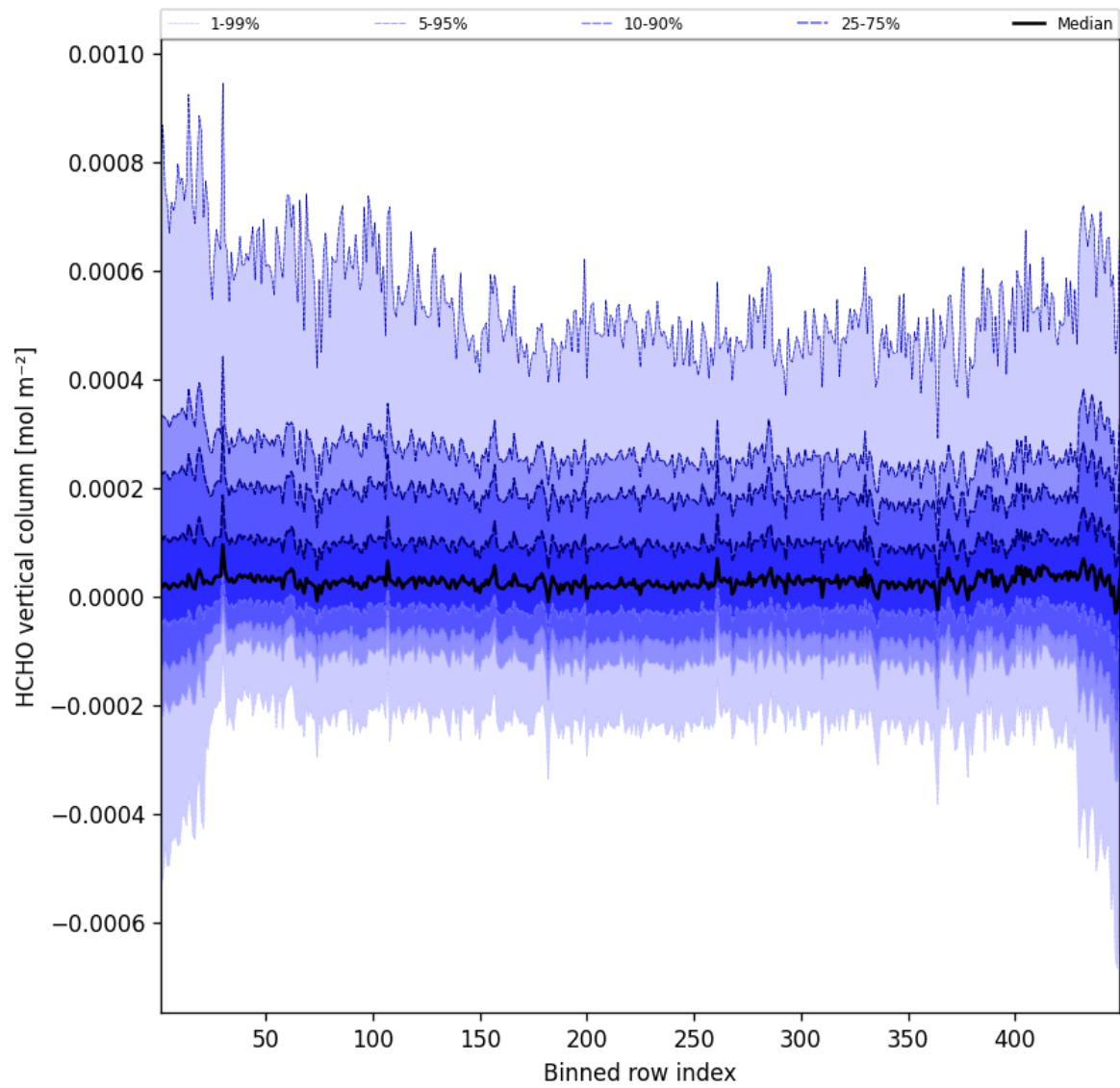
Figure 47: Along track statistics of “HCHO vertical column” for 2025-10-16 to 2025-10-17
