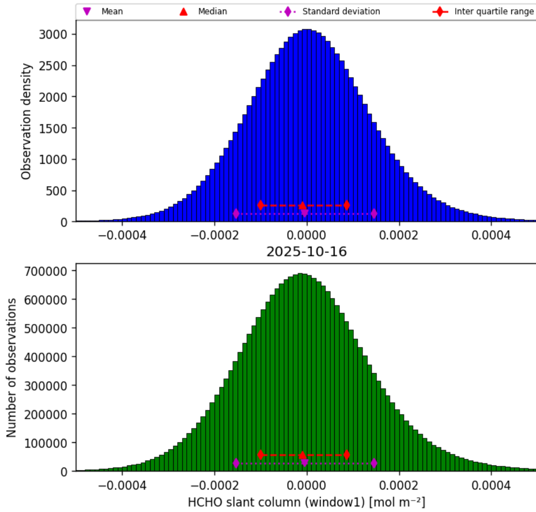
Figure 36: Histogram of “HCHO slant column (window1)” for 2025-10-16 to 2025-10-17
