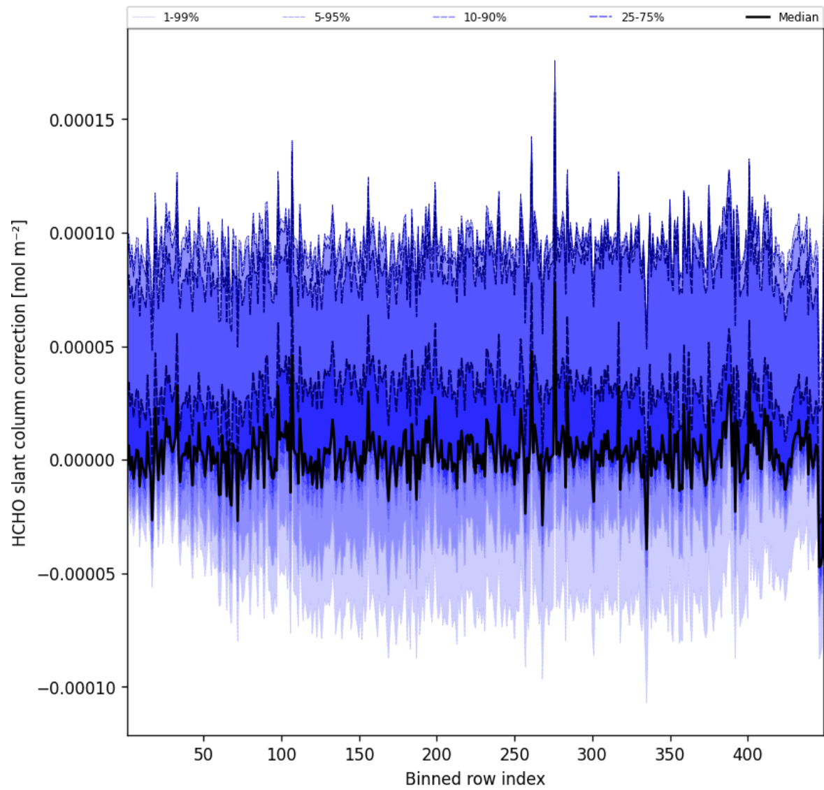
Figure 59: Along track statistics of “HCHO slant column correction” for 2025-10-16 to 2025-10-17
