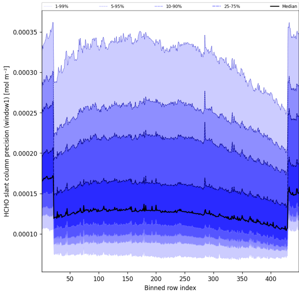
Figure 51: Along track statistics of “HCHO slant column precision (window1)” for 2025-10-16 to 2025-10-17
