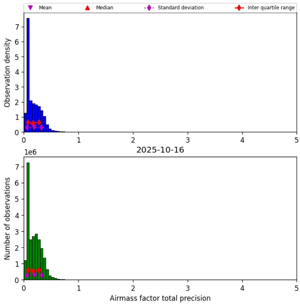
Figure 39: Histogram of “Airmass factor total precision” for 2025-10-16 to 2025-10-17
