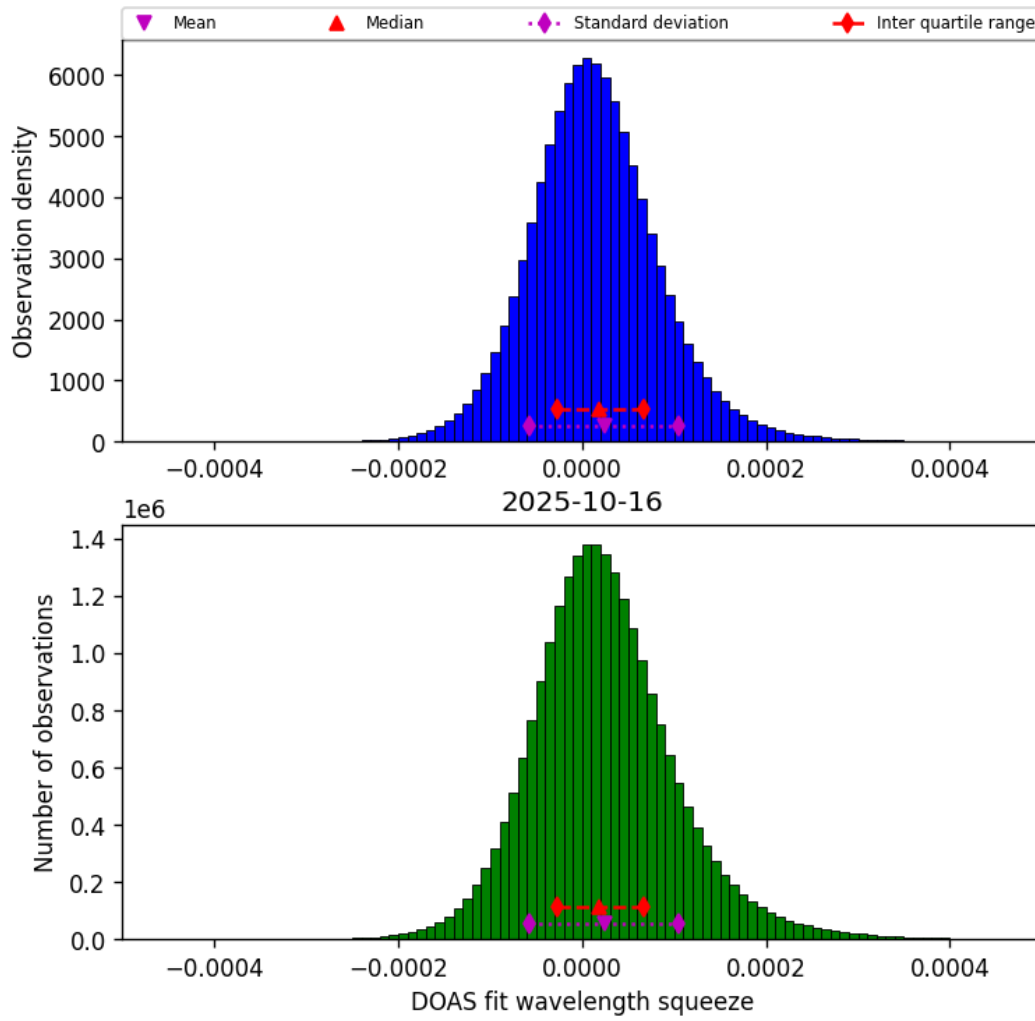
Figure 43: Histogram of “DOAS fit wavelength squeeze” for 2025-10-16 to 2025-10-17
