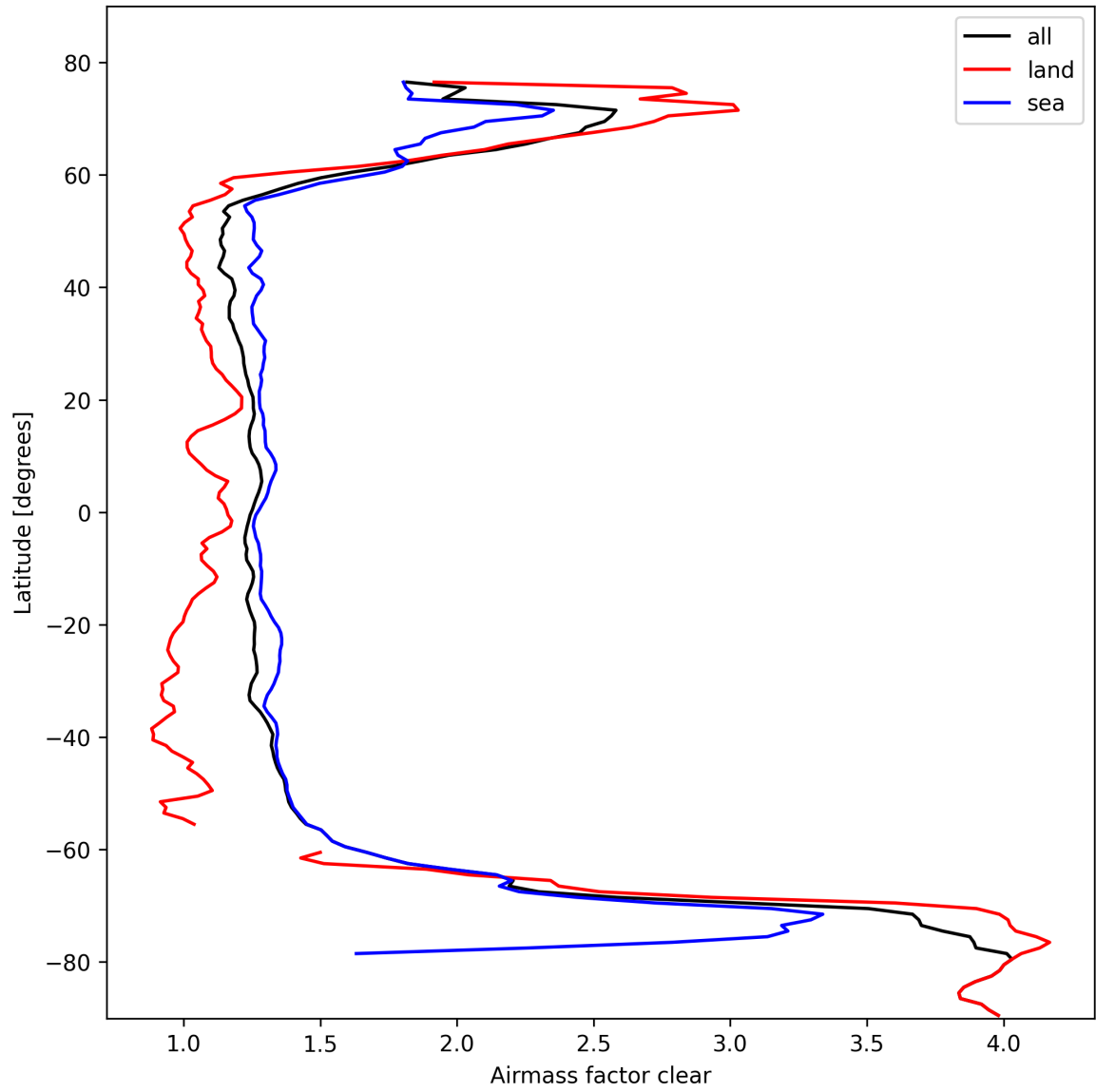
Figure 26: Zonal average of “Airmass factor clear” for 2025-10-16 to 2025-10-17.
