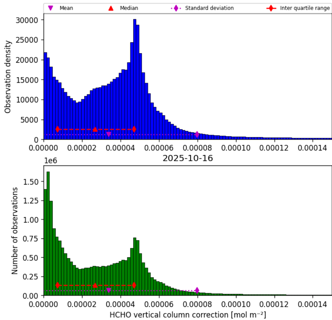
Figure 35: Histogram of “HCHO vertical column correction” for 2025-10-16 to 2025-10-17
