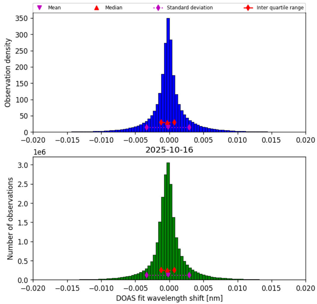
Figure 42: Histogram of “DOAS fit wavelength shift” for 2025-10-16 to 2025-10-17
