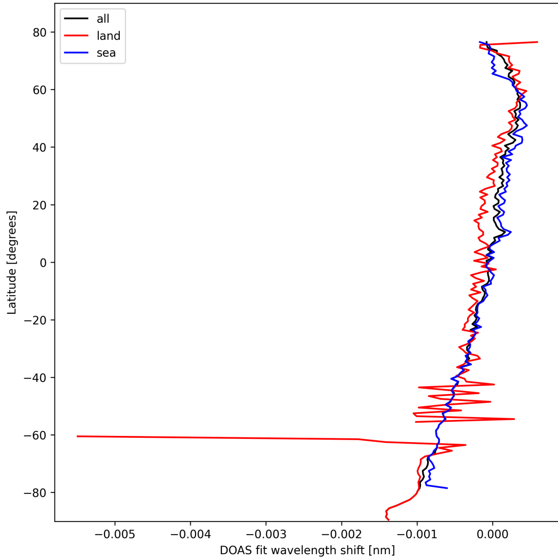
Figure 28: Zonal average of “DOAS fit wavelength shift” for 2025-10-16 to 2025-10-17.
