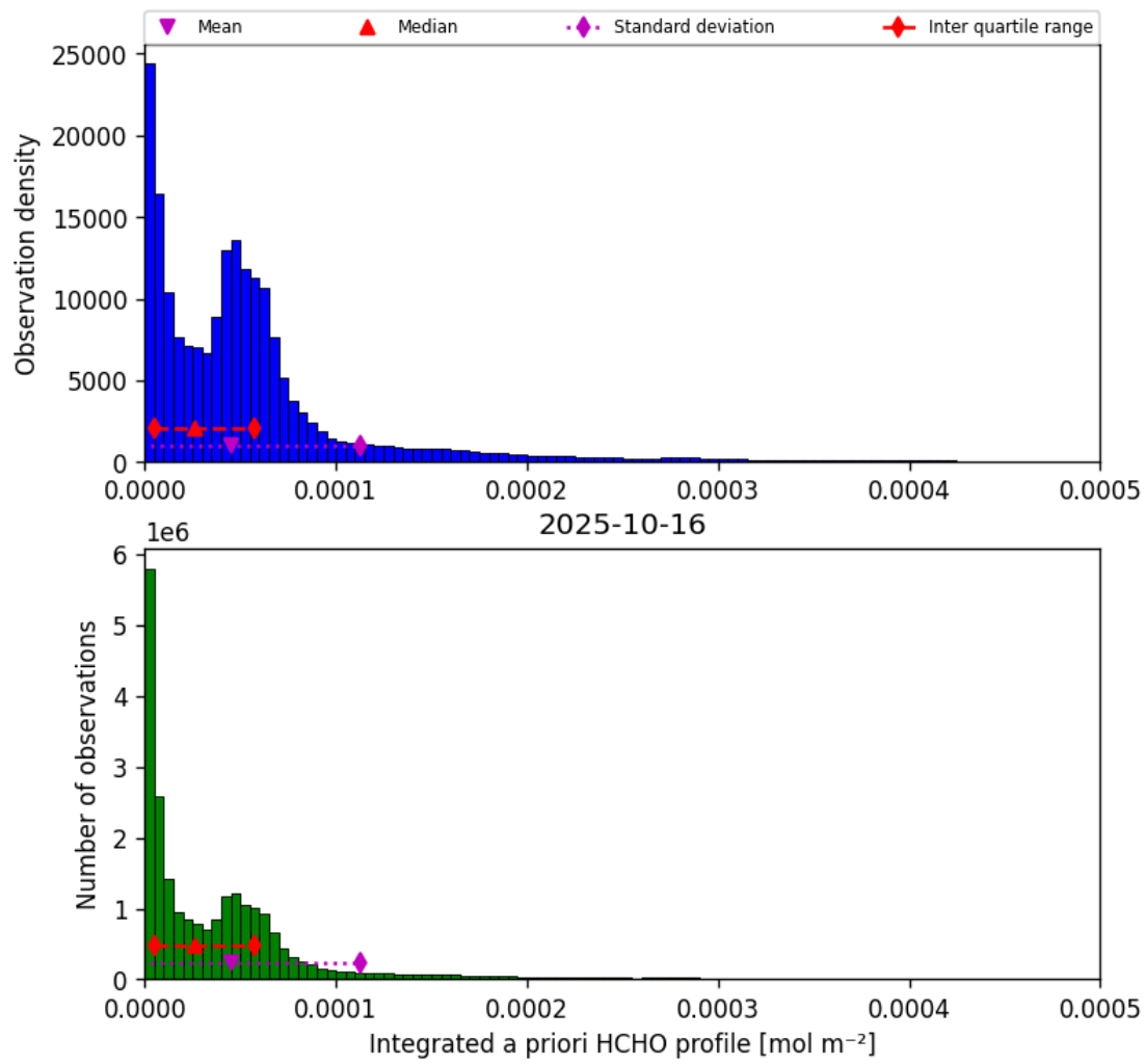
Figure 41: Histogram of “Integrated a priori HCHO profile” for 2025-10-16 to 2025-10-17
