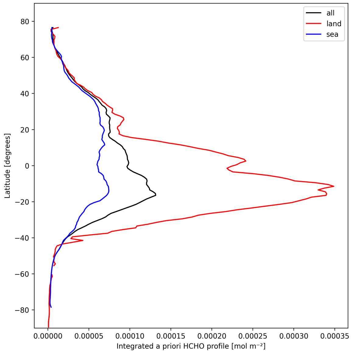
Figure 27: Zonal average of “Integrated a priori HCHO profile” for 2025-10-16 to 2025-10-17.
