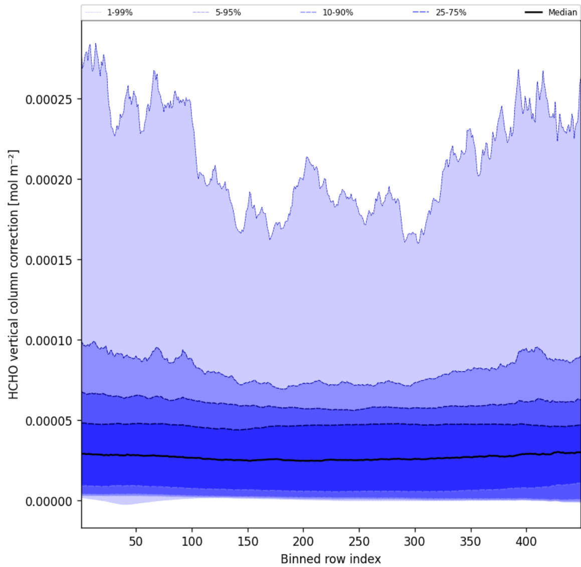
Figure 49: Along track statistics of “HCHO vertical column correction” for 2025-10-16 to 2025-10-17
