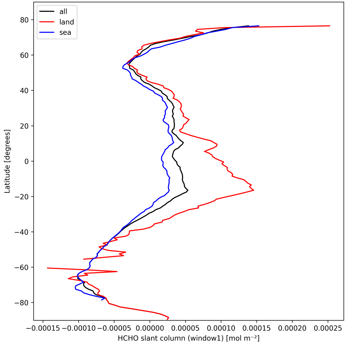
Figure 22: Zonal average of “HCHO slant column (window1)” for 2025-10-16 to 2025-10-17.
