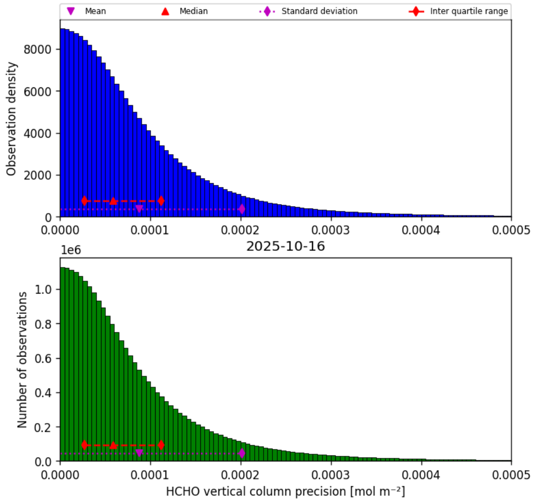
Figure 34: Histogram of “HCHO vertical column precision” for 2025-10-16 to 2025-10-17
