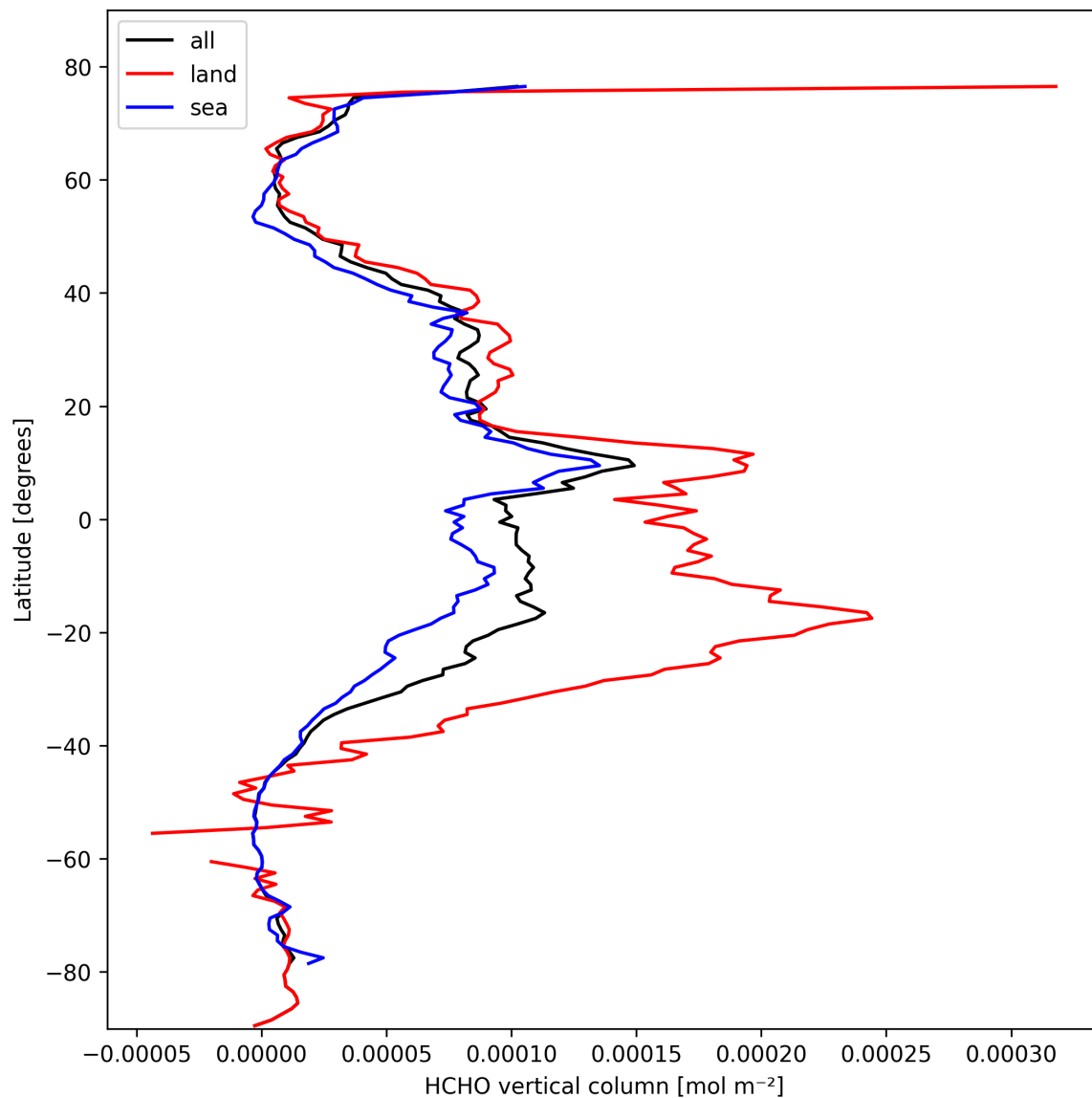
Figure 19: Zonal average of “HCHO vertical column” for 2025-10-16 to 2025-10-17.
