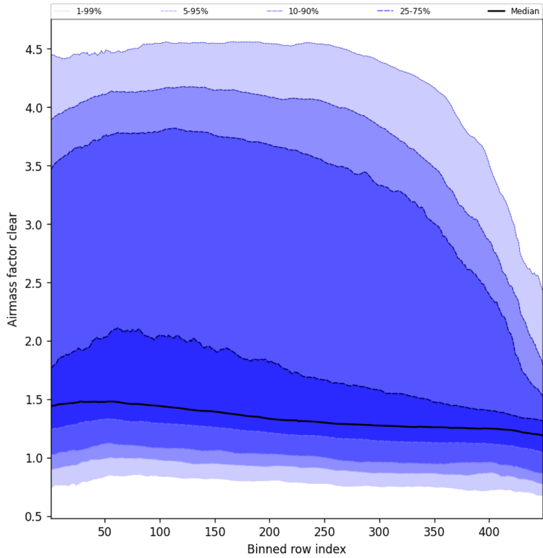
Figure 54: Along track statistics of “Airmass factor clear” for 2025-10-16 to 2025-10-17
