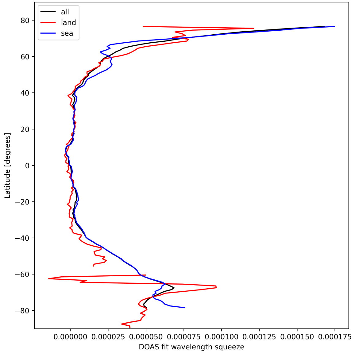
Figure 29: Zonal average of “DOAS fit wavelength squeeze” for 2025-10-16 to 2025-10-17.
