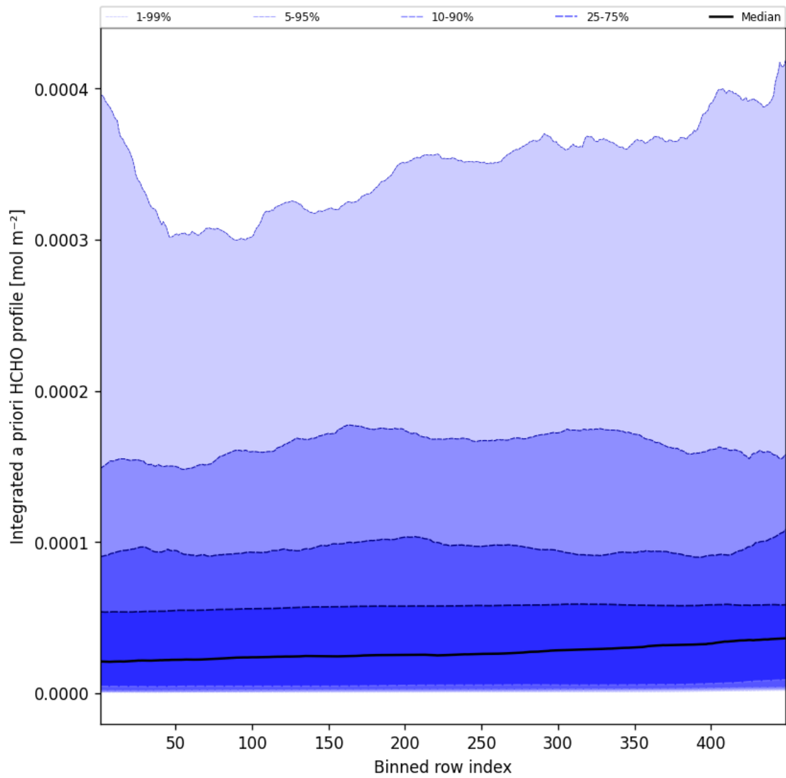
Figure 55: Along track statistics of “Integrated a priori HCHO profile” for 2025-10-16 to 2025-10-17
