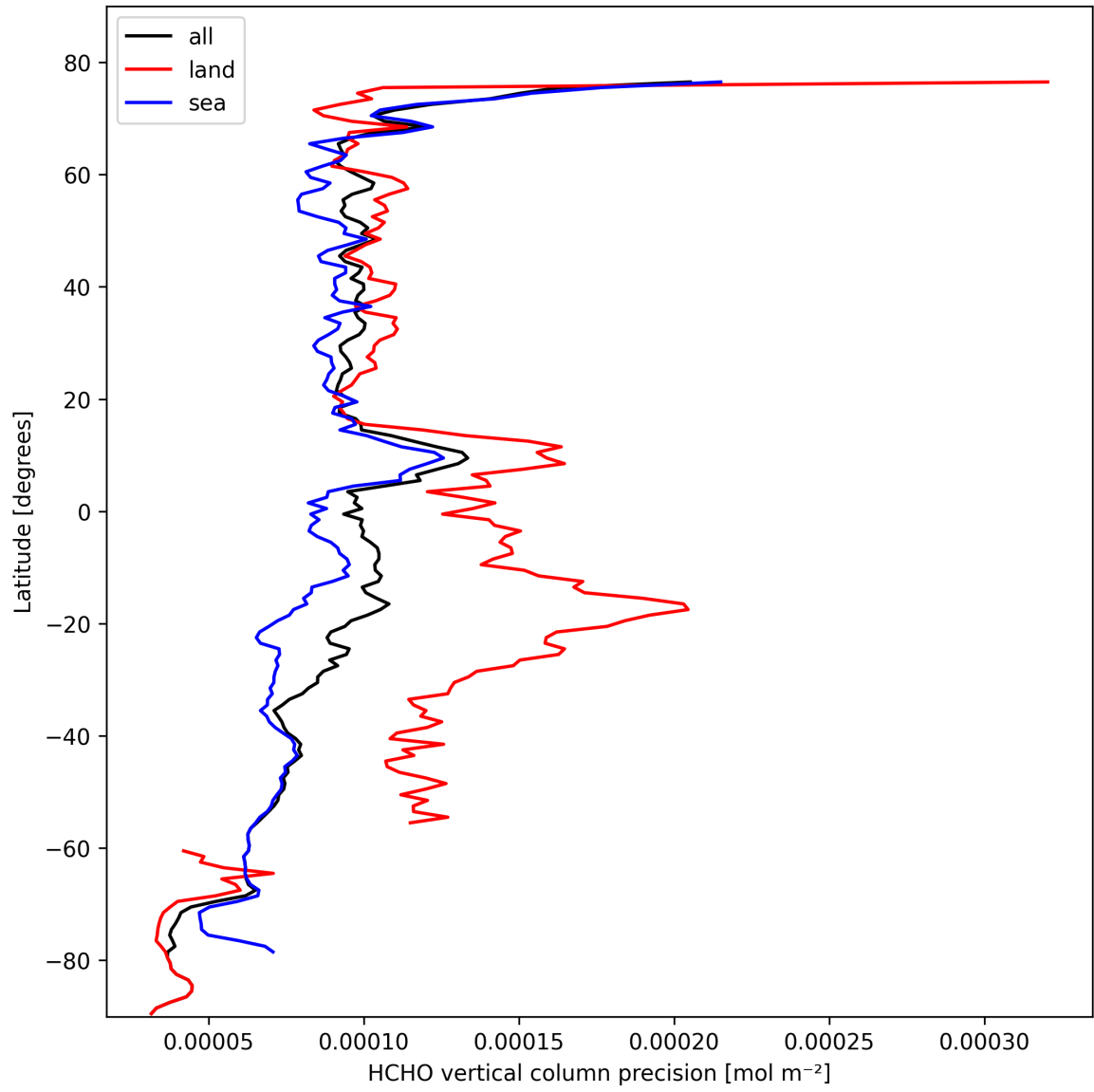
Figure 20: Zonal average of “HCHO vertical column precision” for 2025-10-16 to 2025-10-17.
