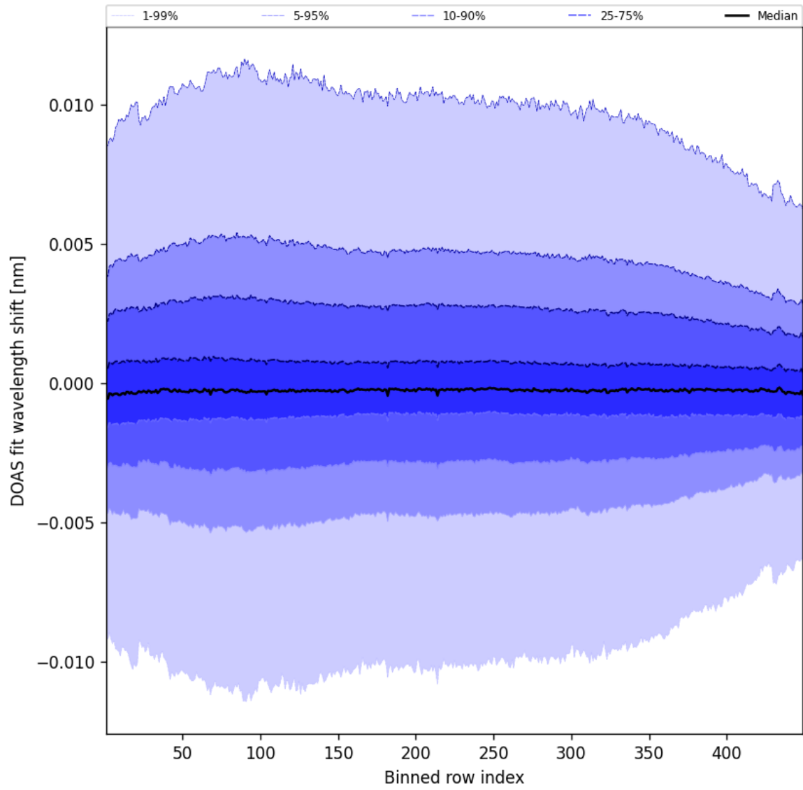
Figure 56: Along track statistics of “DOAS fit wavelength shift” for 2025-10-16 to 2025-10-17
