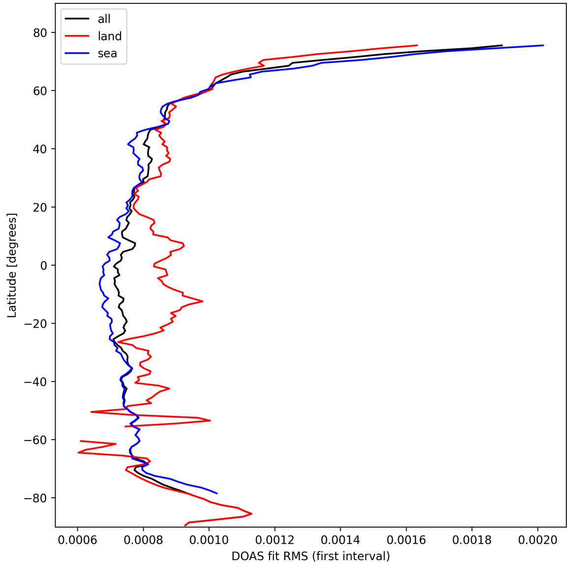
Figure 30: Zonal average of “DOAS fit RMS (first interval)” for 2025-10-17 to 2025-10-18.
