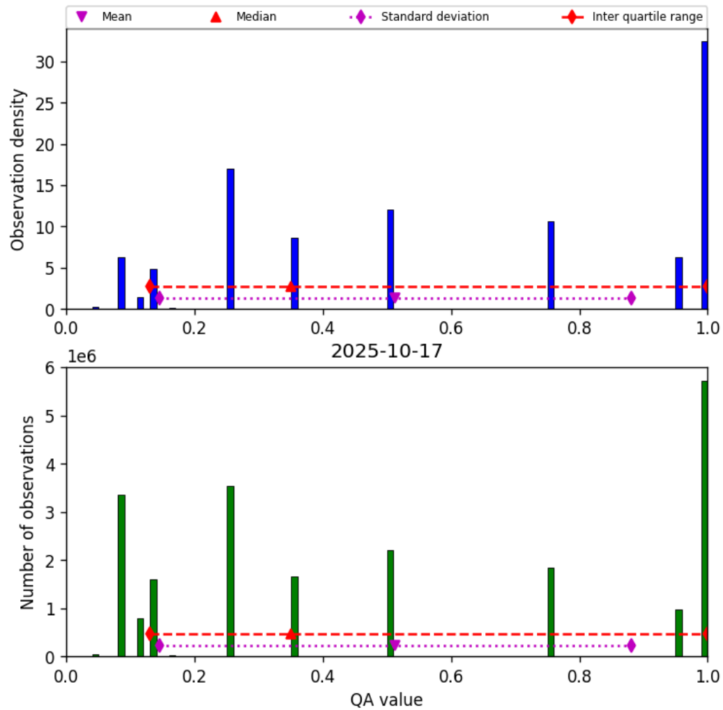
Figure 32: Histogram of “QA value” for 2025-10-17 to 2025-10-18
