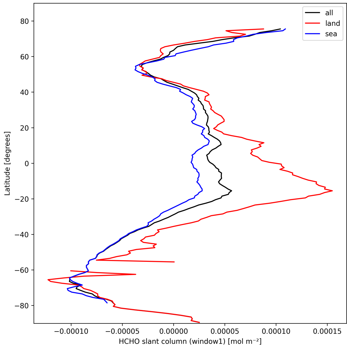
Figure 22: Zonal average of “HCHO slant column (window1)” for 2025-10-17 to 2025-10-18.
