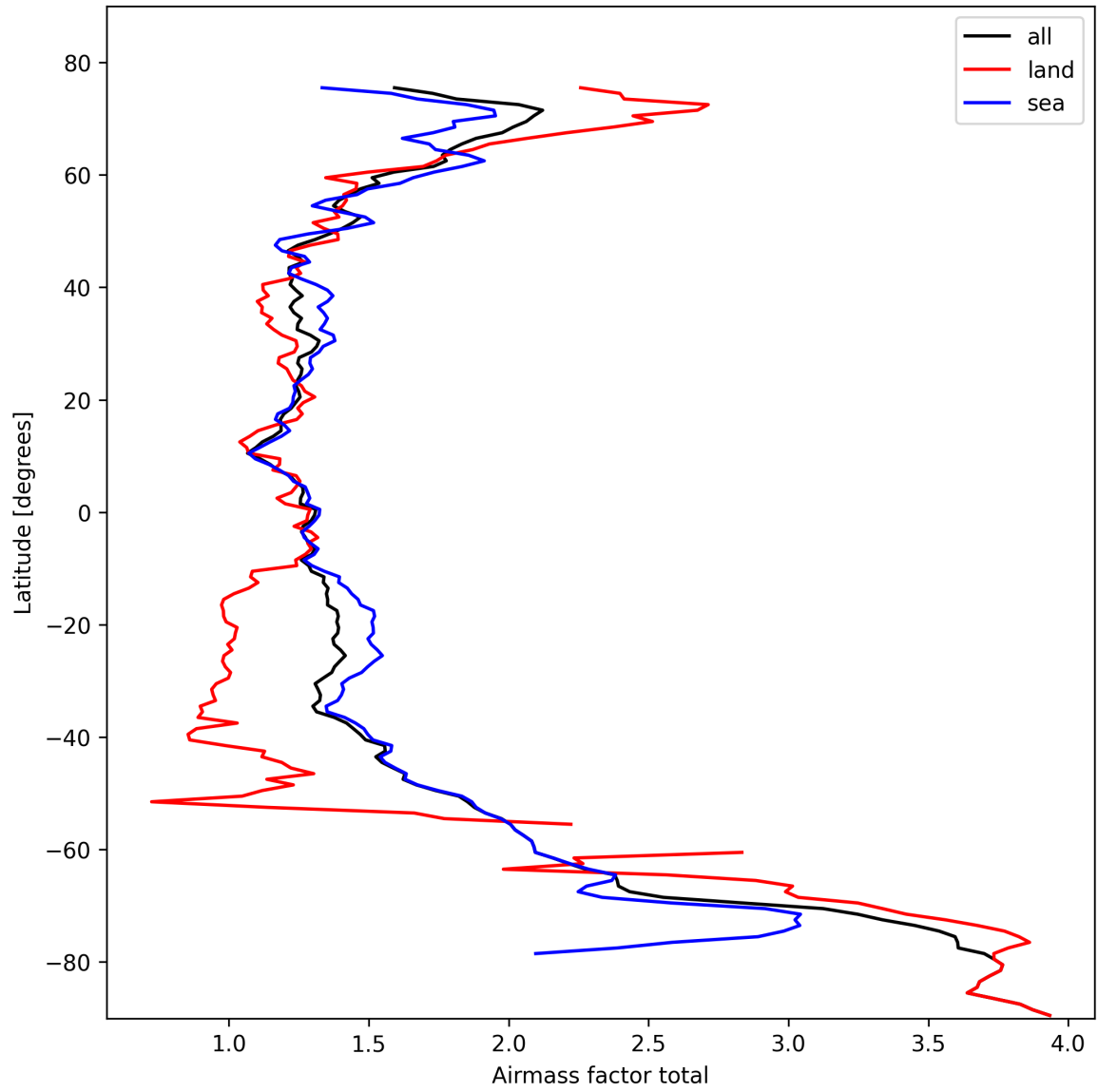
Figure 24: Zonal average of “Airmass factor total” for 2025-10-17 to 2025-10-18.
