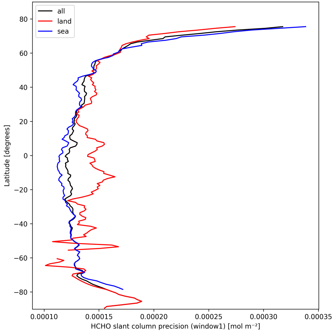
Figure 23: Zonal average of “HCHO slant column precision (window1)” for 2025-10-17 to 2025-10-18.
