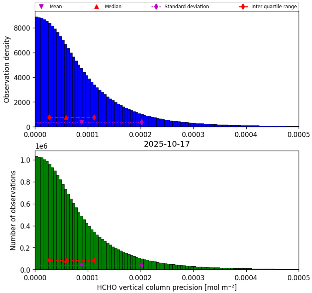
Figure 34: Histogram of “HCHO vertical column precision” for 2025-10-17 to 2025-10-18
