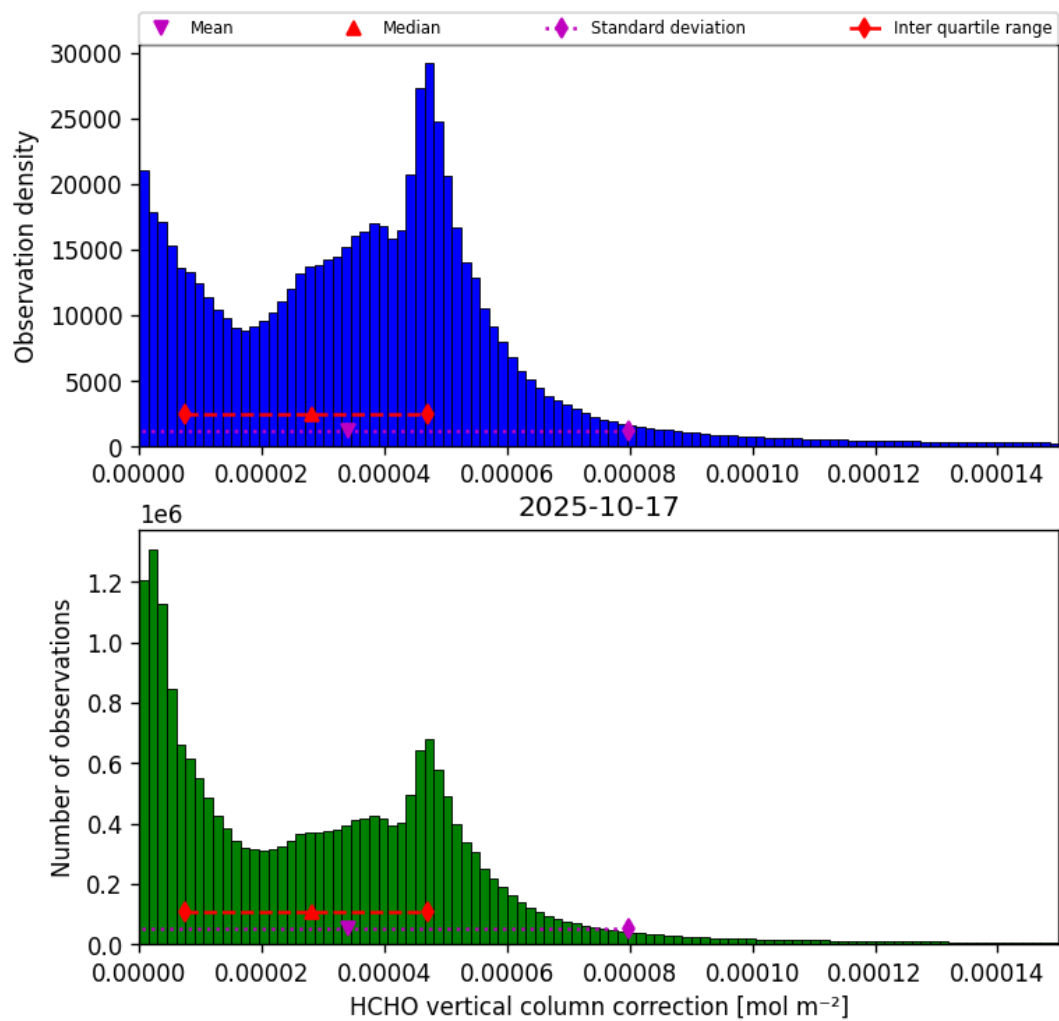
Figure 35: Histogram of “HCHO vertical column correction” for 2025-10-17 to 2025-10-18
