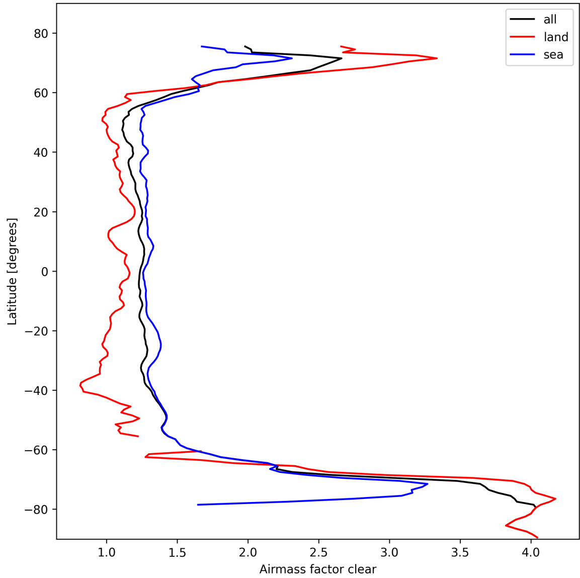
Figure 26: Zonal average of “Airmass factor clear” for 2025-10-17 to 2025-10-18.
