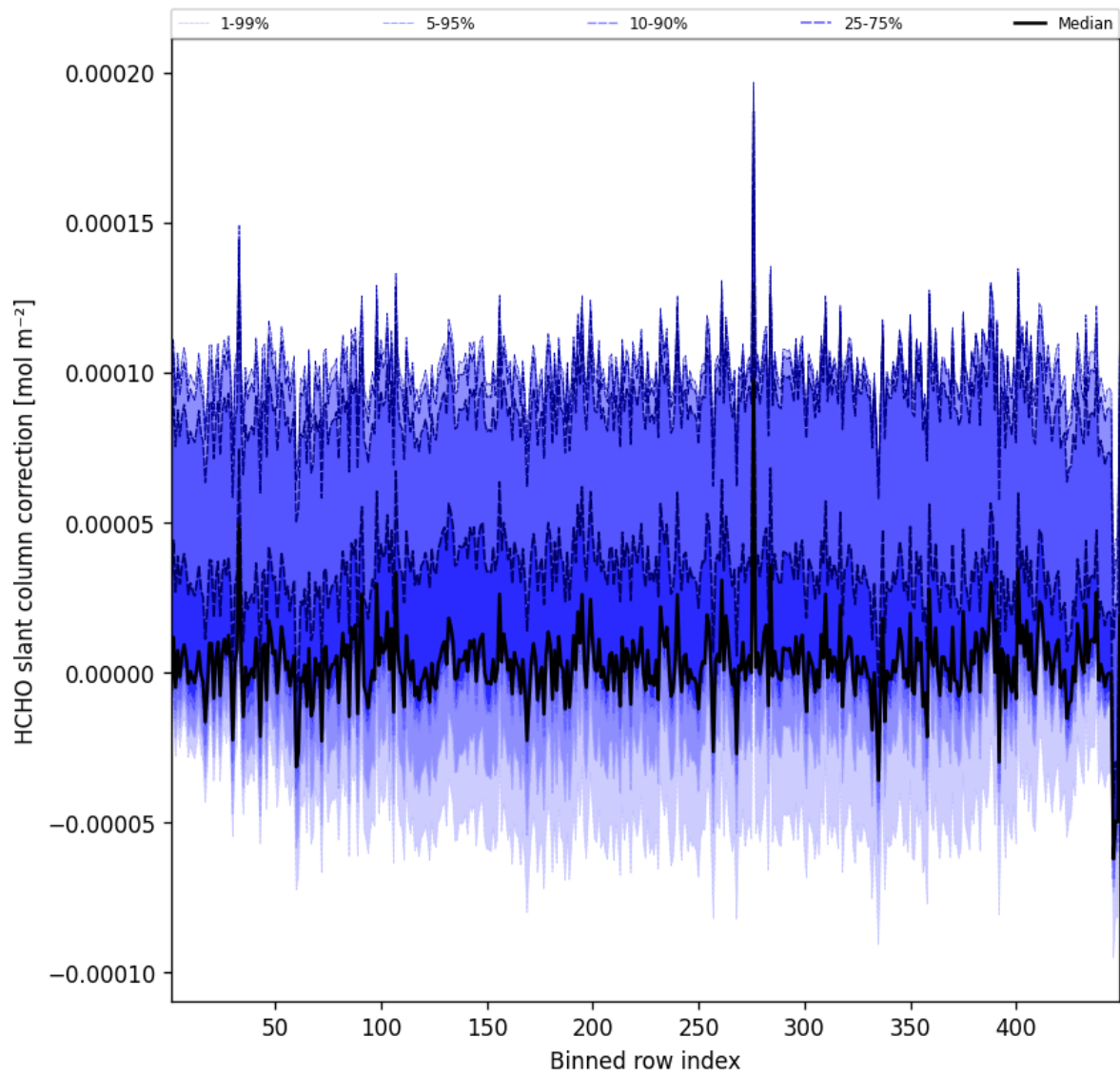
Figure 59: Along track statistics of “HCHO slant column correction” for 2025-10-17 to 2025-10-18
