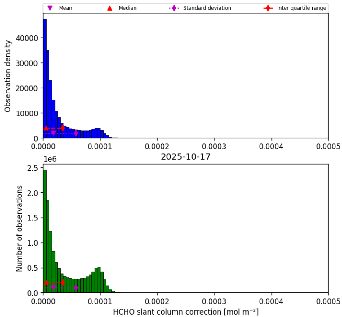
Figure 45: Histogram of “HCHO slant column correction” for 2025-10-17 to 2025-10-18
