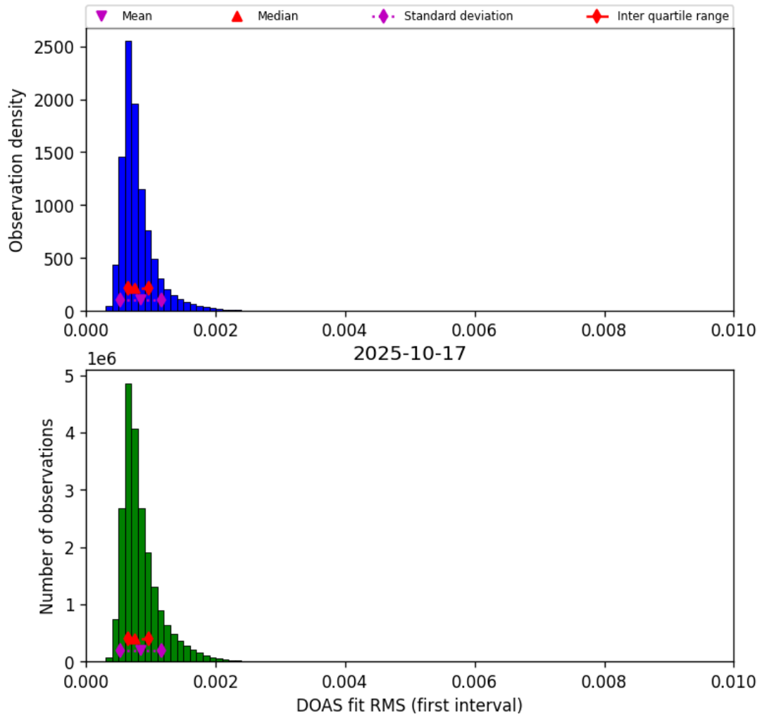
Figure 44: Histogram of “DOAS fit RMS (first interval)” for 2025-10-17 to 2025-10-18
