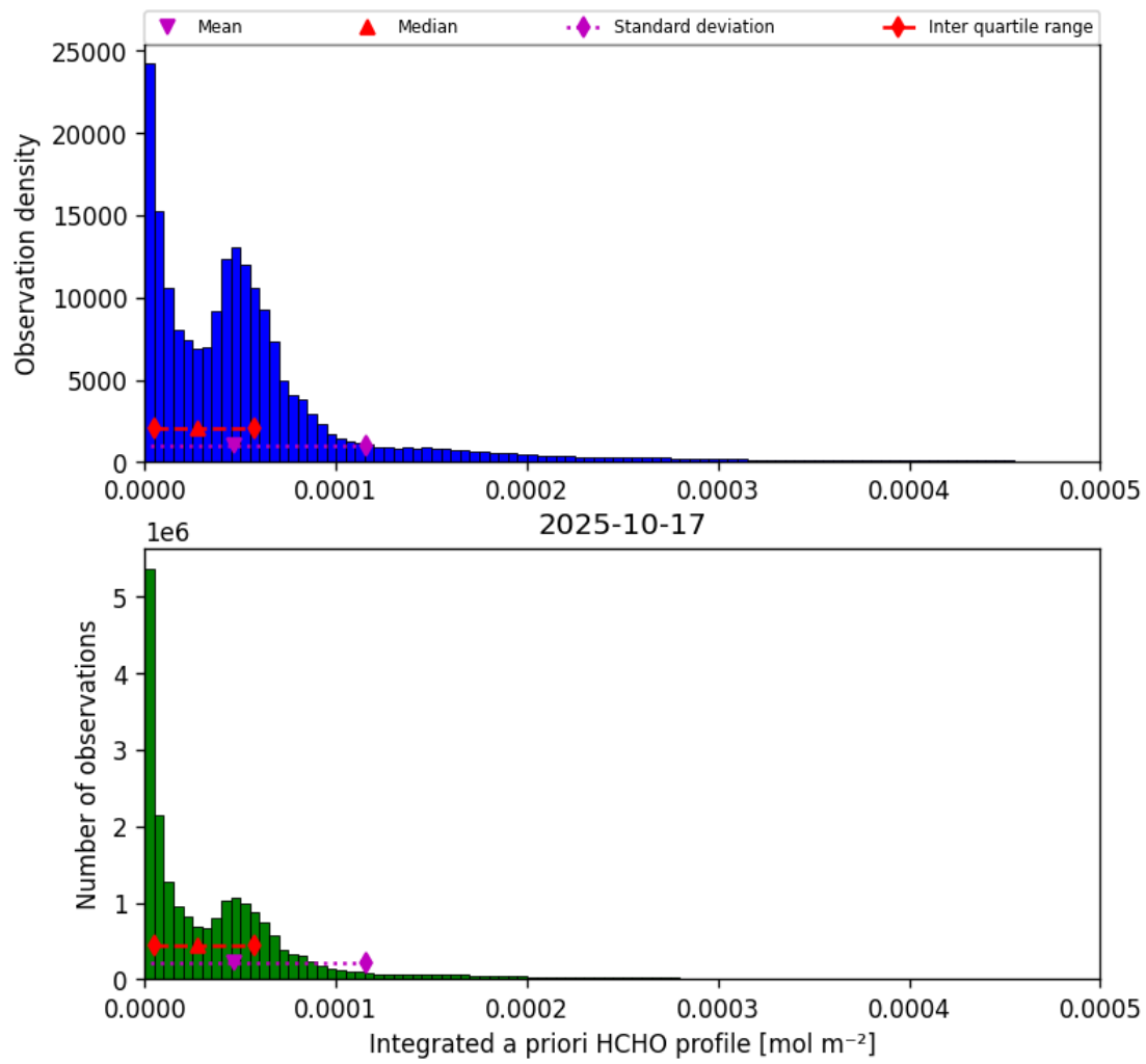
Figure 41: Histogram of “Integrated a priori HCHO profile” for 2025-10-17 to 2025-10-18
