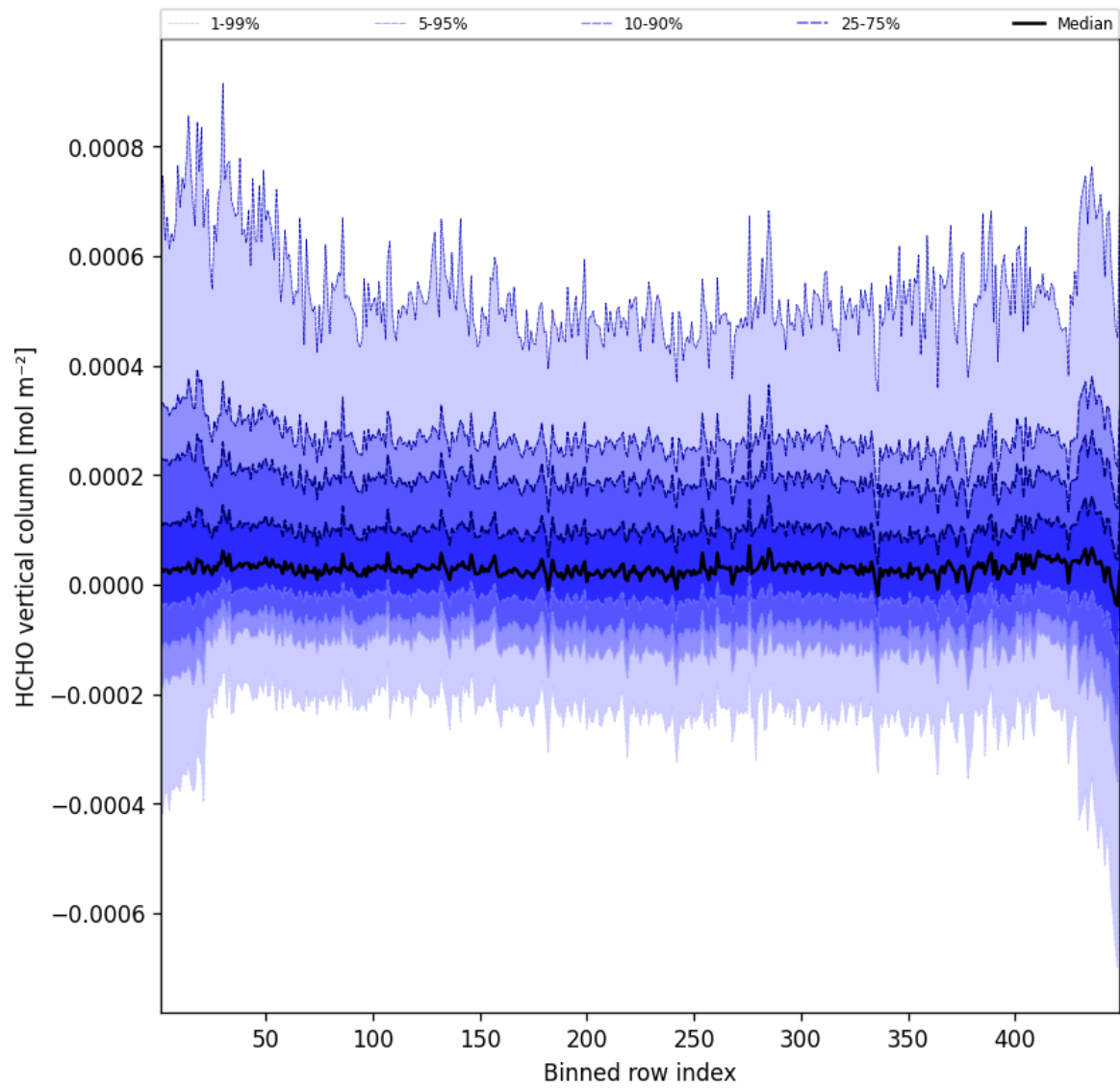
Figure 47: Along track statistics of “HCHO vertical column” for 2025-10-17 to 2025-10-18
