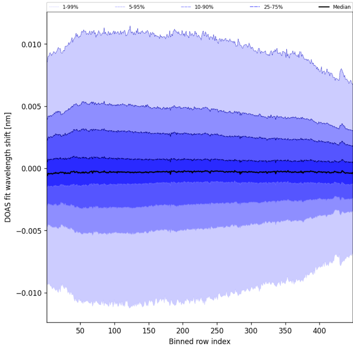
Figure 56: Along track statistics of “DOAS fit wavelength shift” for 2025-10-17 to 2025-10-18
