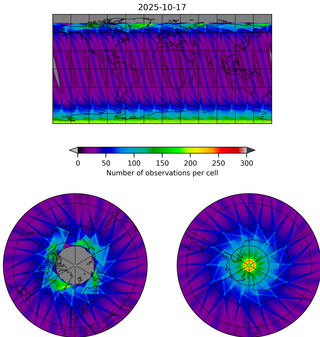
Figure 17: Map of the number of observations for 2025-10-17 to 2025-10-18
