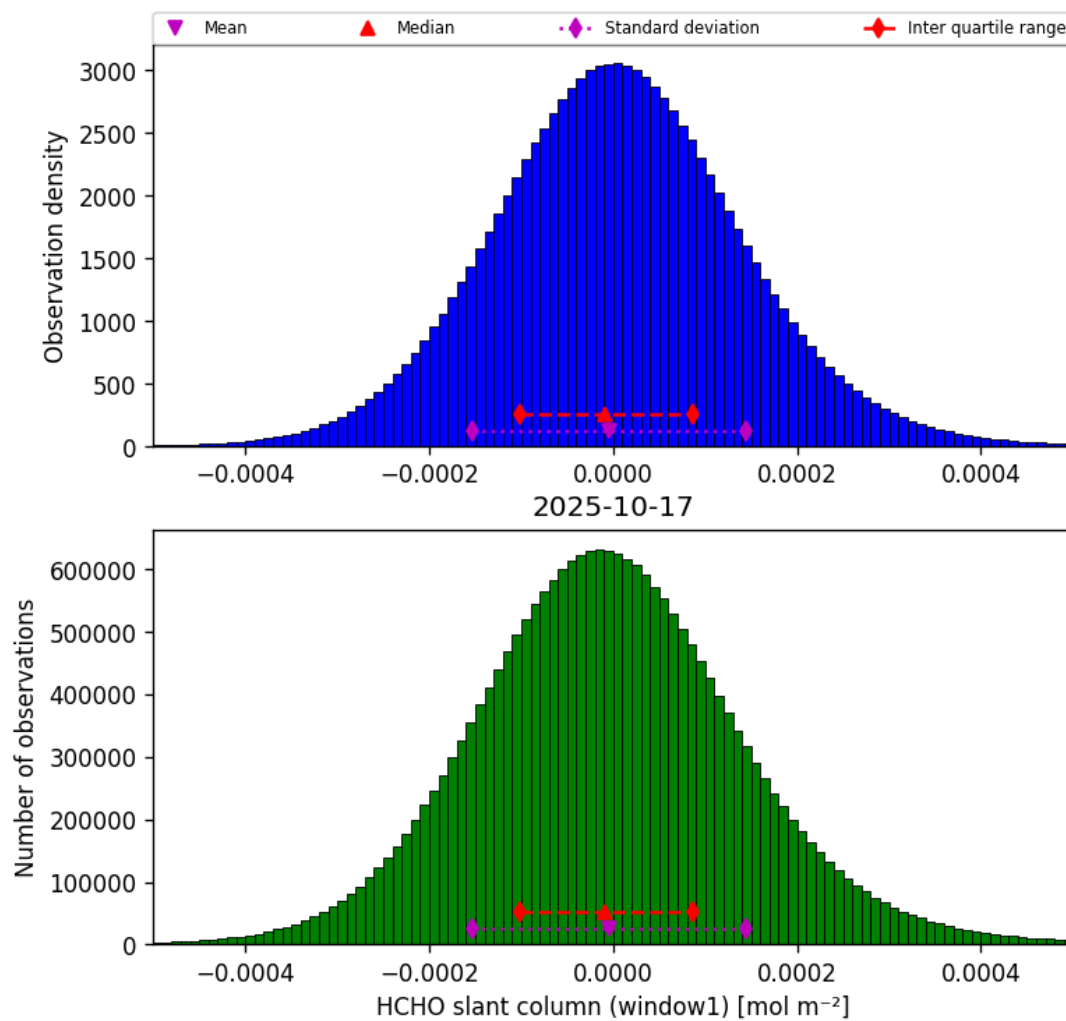
Figure 36: Histogram of “HCHO slant column (window1)” for 2025-10-17 to 2025-10-18
