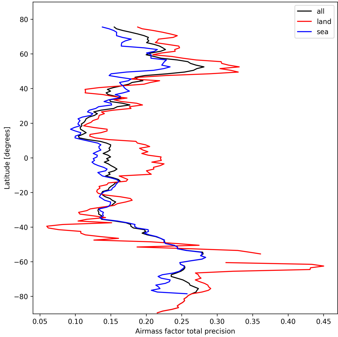
Figure 25: Zonal average of “Airmass factor total precision” for 2025-10-17 to 2025-10-18.
