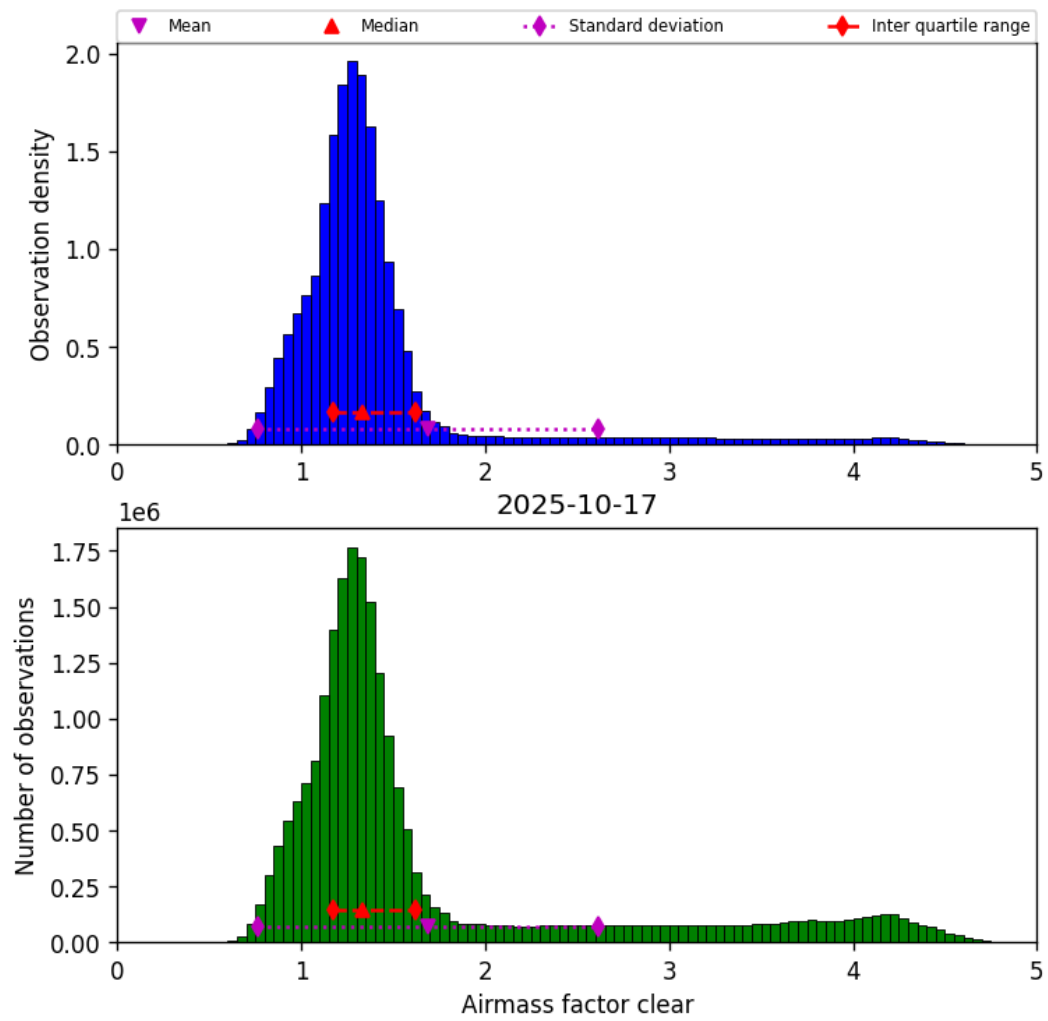
Figure 40: Histogram of “Airmass factor clear” for 2025-10-17 to 2025-10-18
