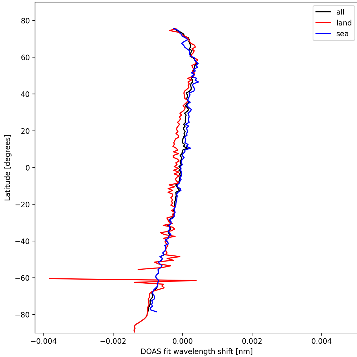
Figure 28: Zonal average of “DOAS fit wavelength shift” for 2025-10-17 to 2025-10-18.
