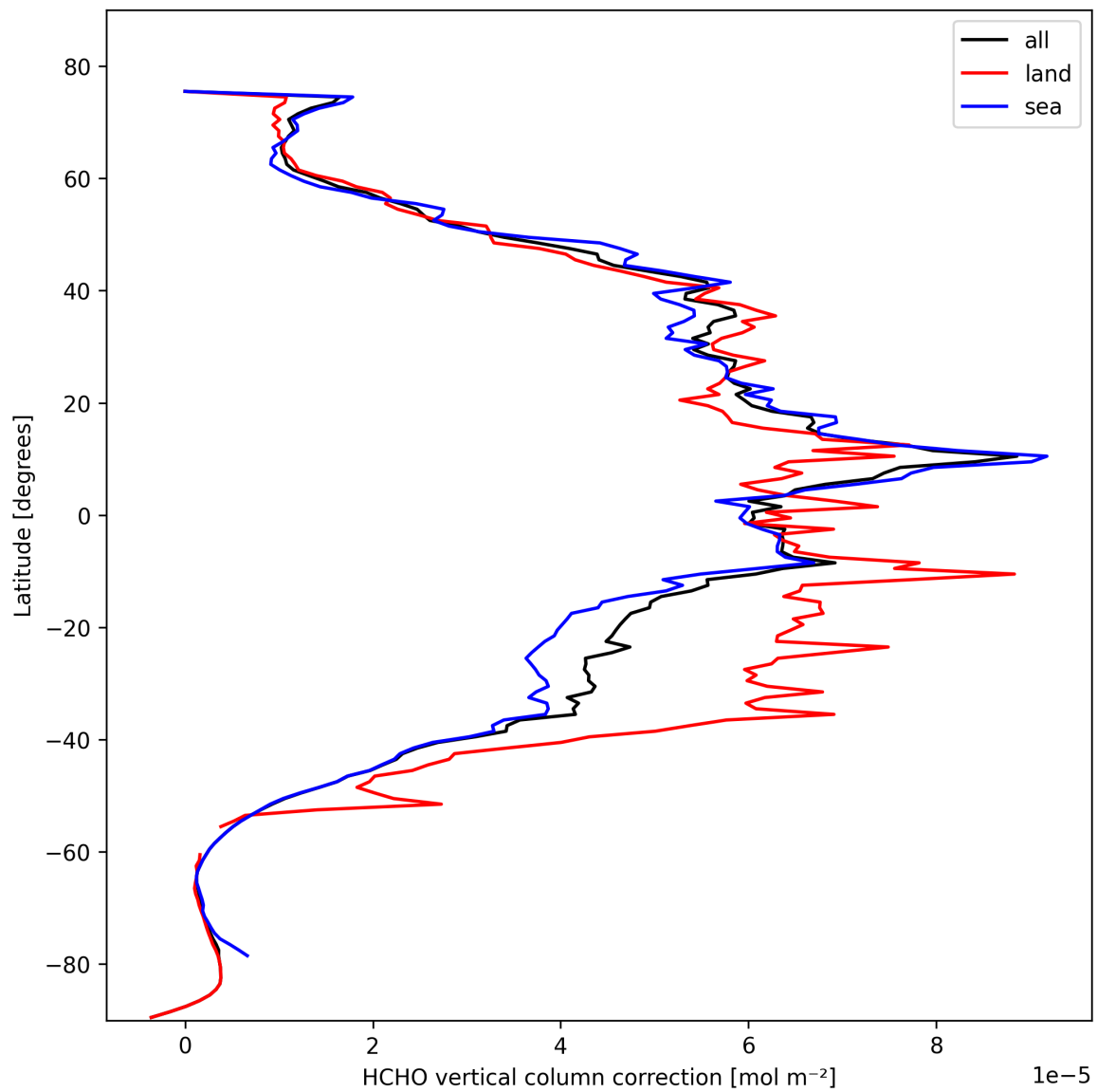
Figure 21: Zonal average of “HCHO vertical column correction” for 2025-10-17 to 2025-10-18.
