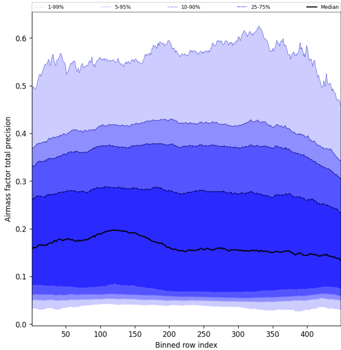
Figure 53: Along track statistics of “Airmass factor total precision” for 2025-10-17 to 2025-10-18
