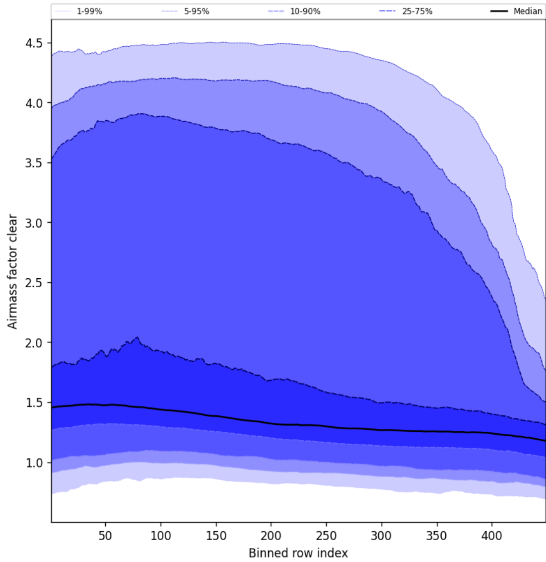
Figure 54: Along track statistics of “Airmass factor clear” for 2025-10-17 to 2025-10-18
