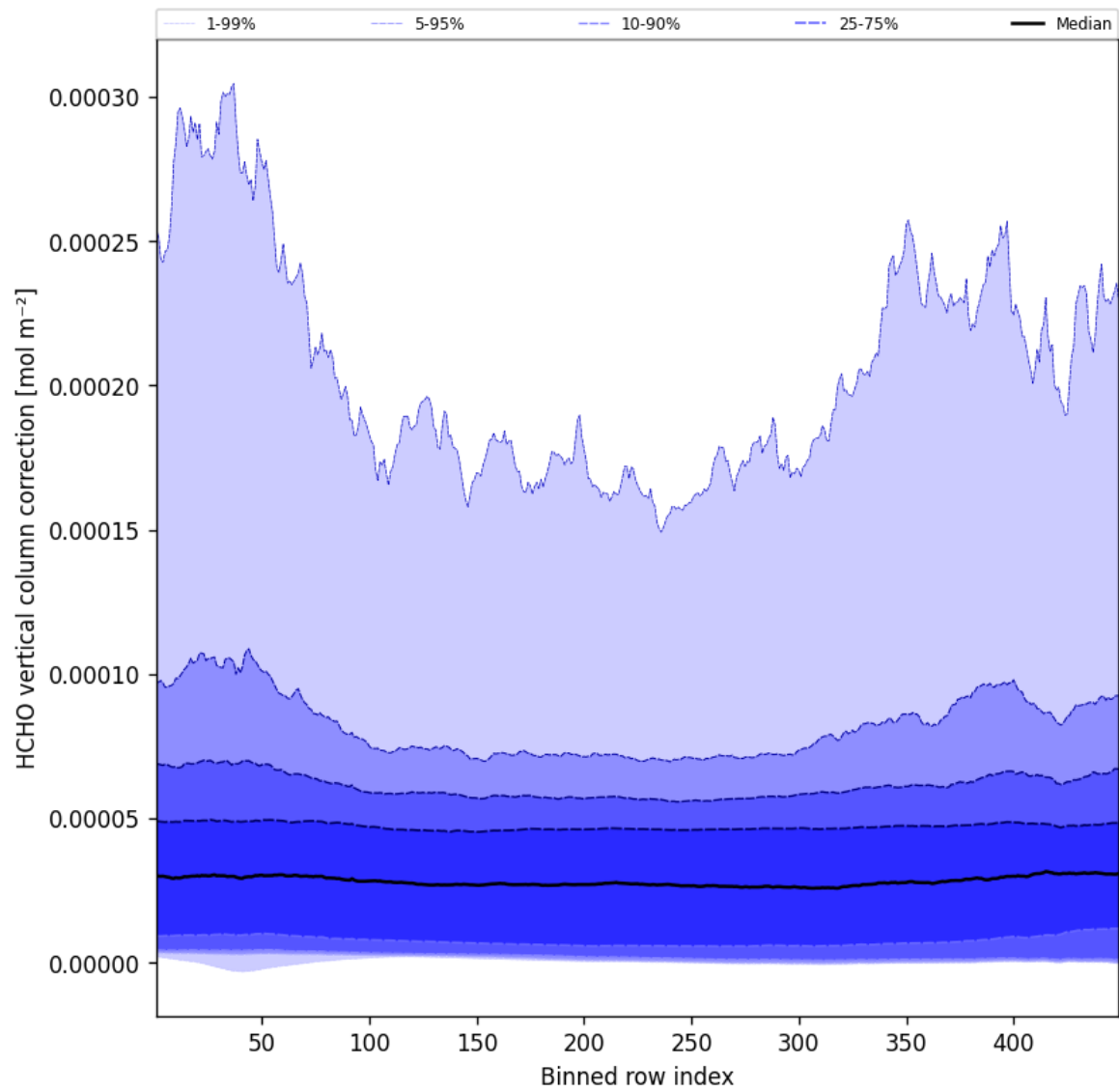
Figure 49: Along track statistics of “HCHO vertical column correction” for 2025-10-17 to 2025-10-18
