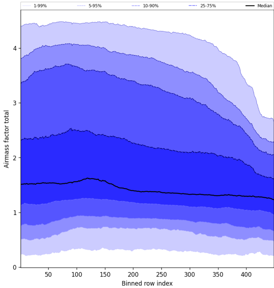
Figure 52: Along track statistics of “Airmass factor total” for 2025-10-17 to 2025-10-18
