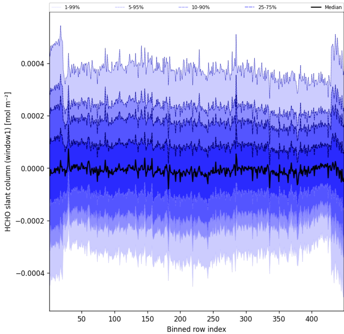
Figure 50: Along track statistics of “HCHO slant column (window1)” for 2025-10-17 to 2025-10-18
