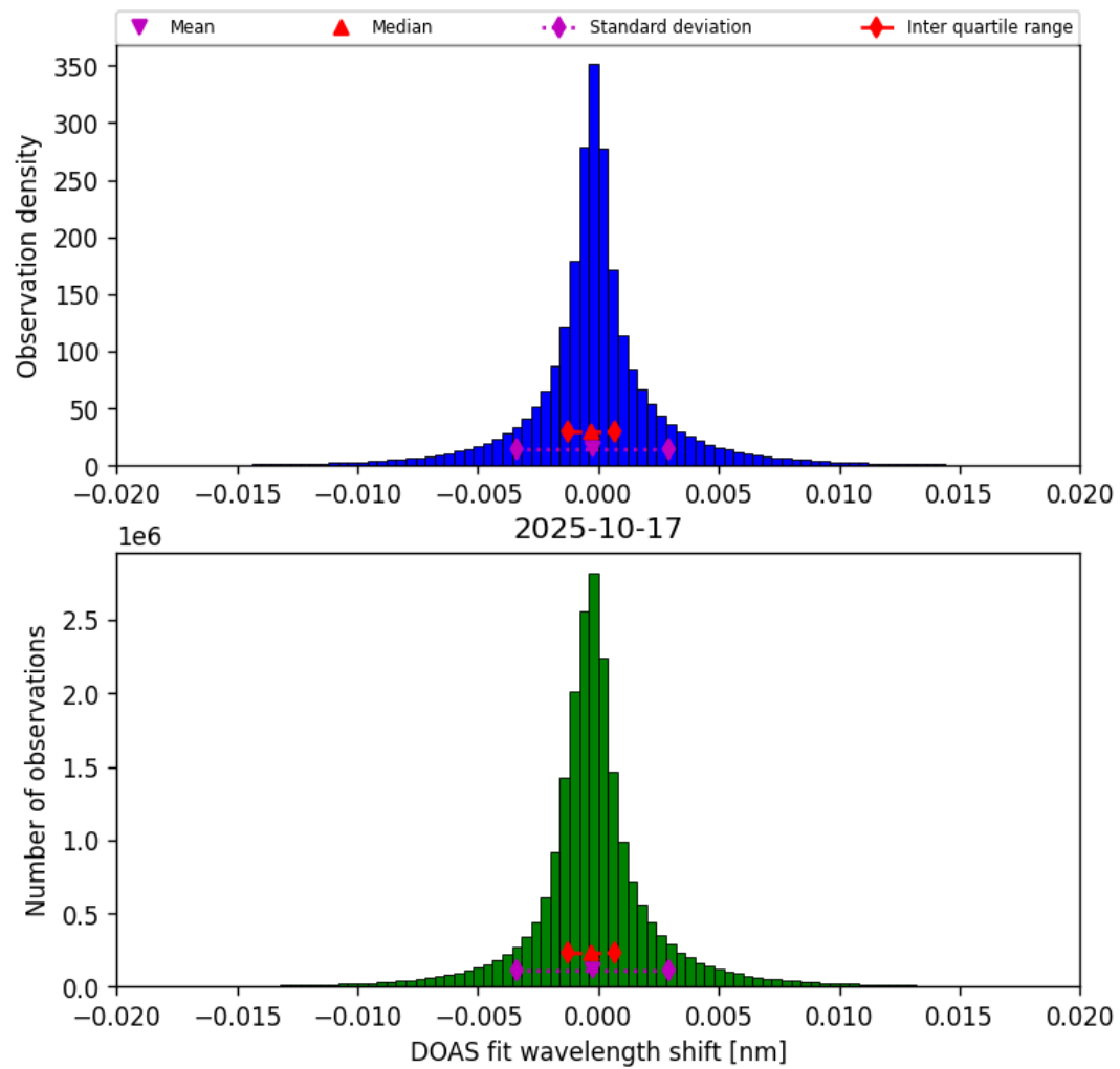
Figure 42: Histogram of “DOAS fit wavelength shift” for 2025-10-17 to 2025-10-18
