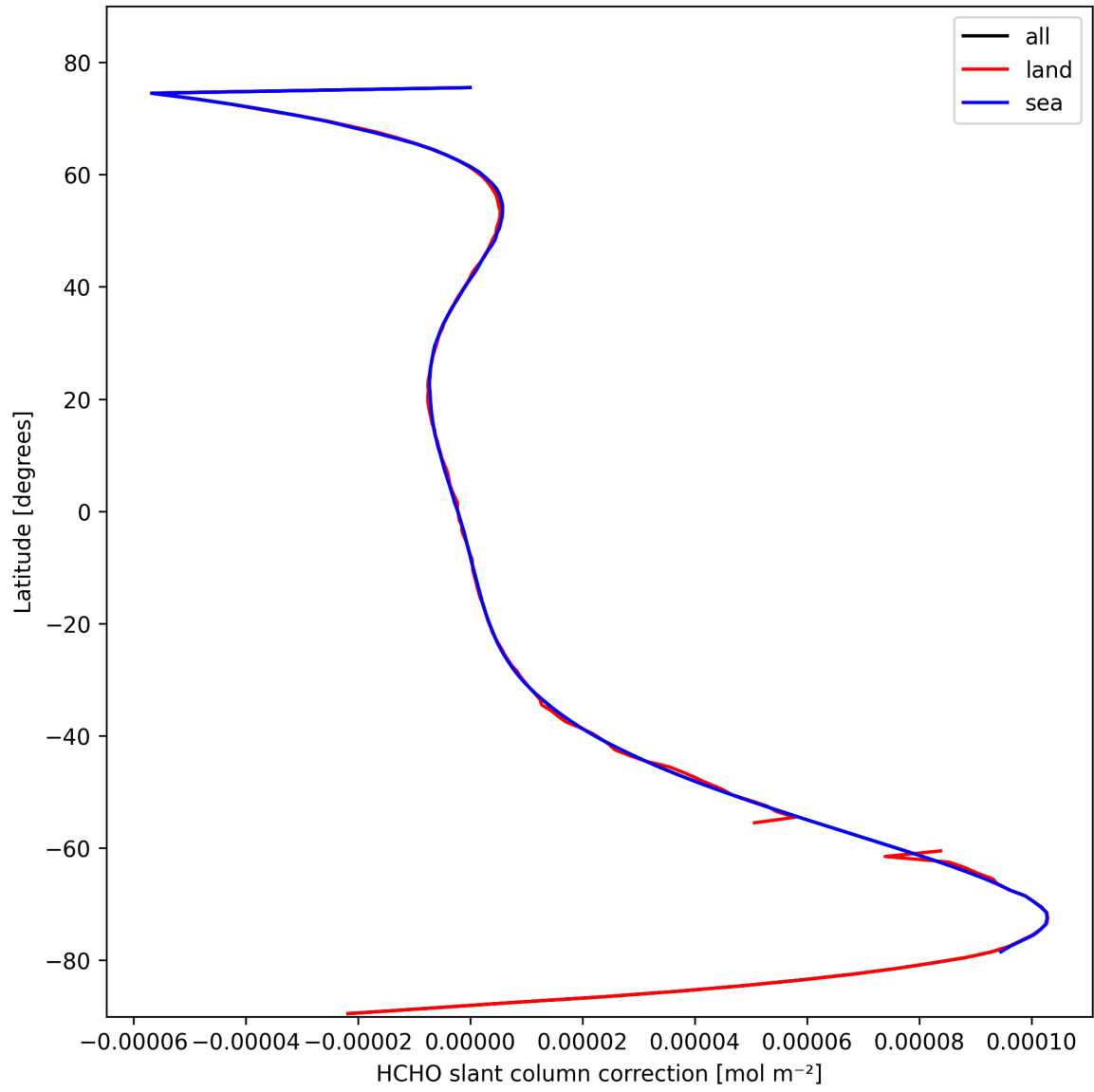
Figure 31: Zonal average of “HCHO slant column correction” for 2025-10-17 to 2025-10-18.
