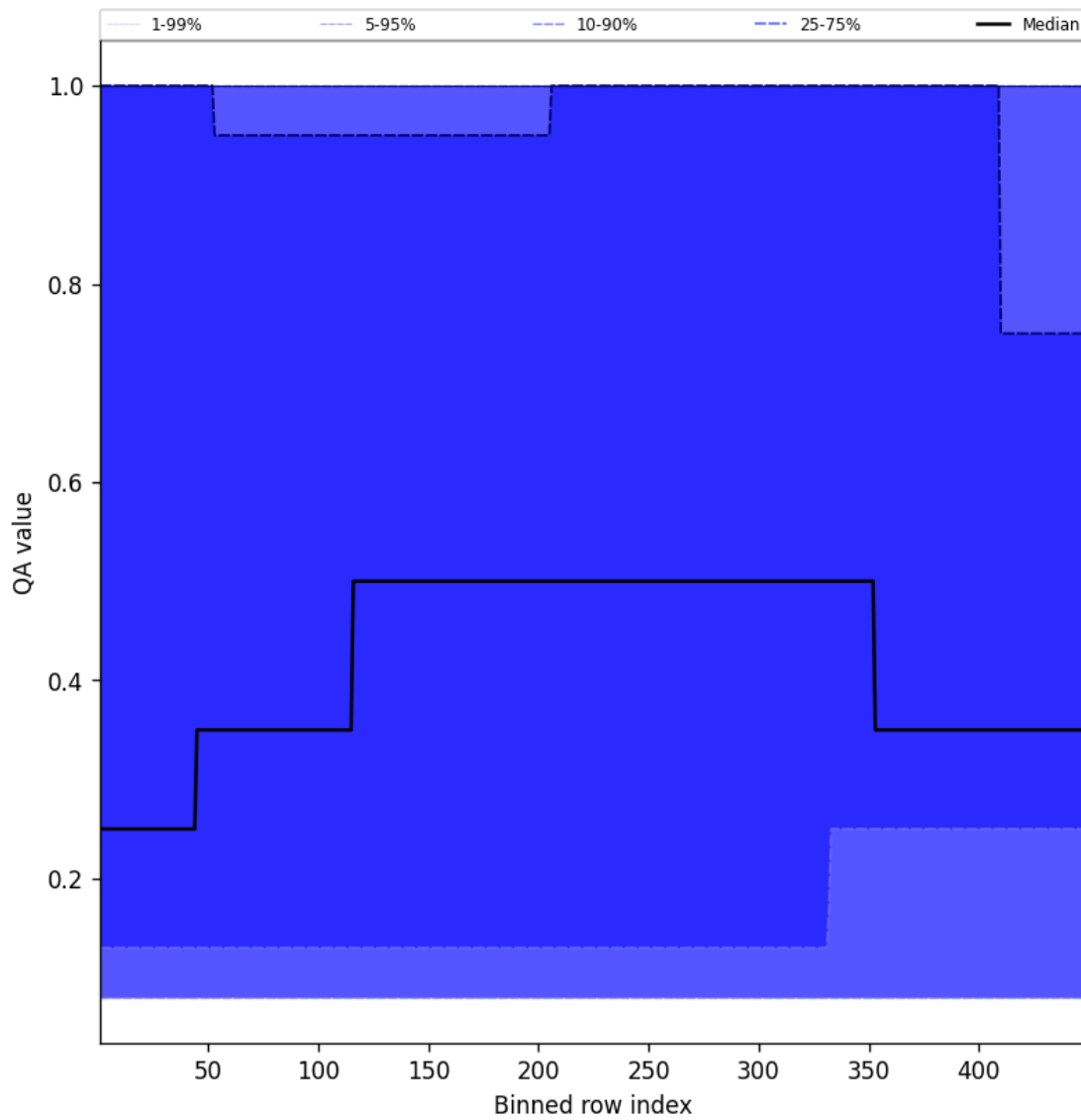
Figure 46: Along track statistics of "QA value" for 2025-10-17 to 2025-10-18
