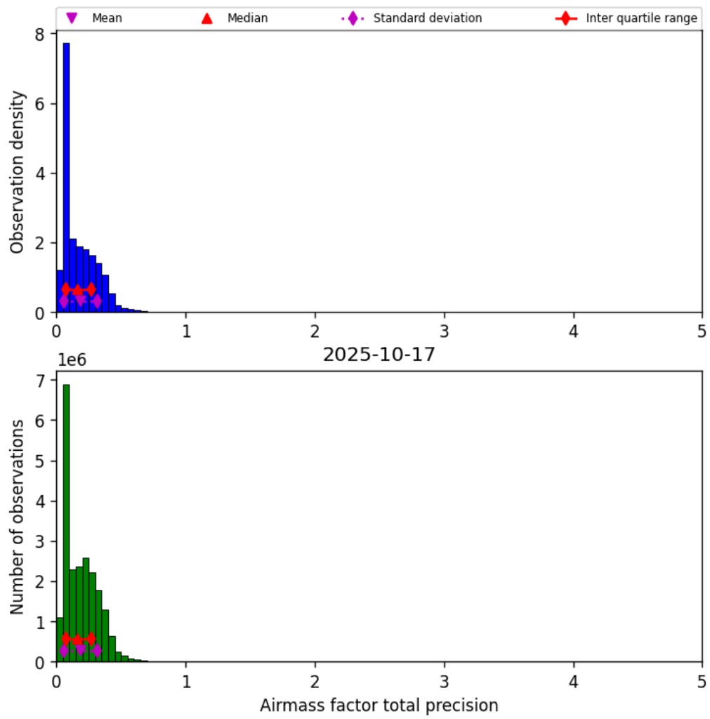
Figure 39: Histogram of “Airmass factor total precision” for 2025-10-17 to 2025-10-18
