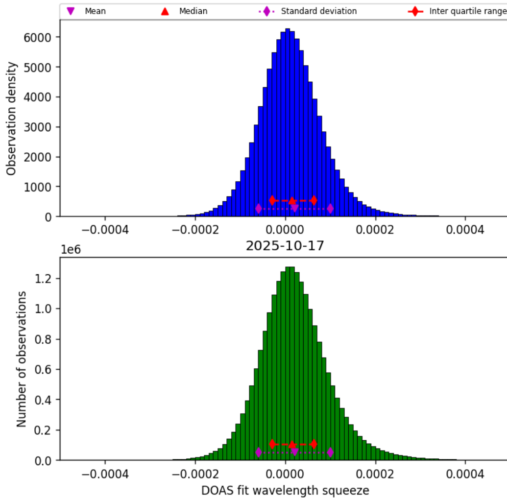
Figure 43: Histogram of "DOAS fit wavelength squeeze" for 2025-10-17 to 2025-10-18
