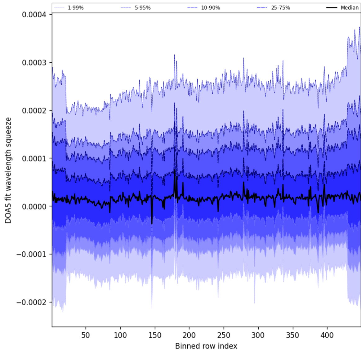
Figure 57: Along track statistics of “DOAS fit wavelength squeeze” for 2025-10-17 to 2025-10-18
