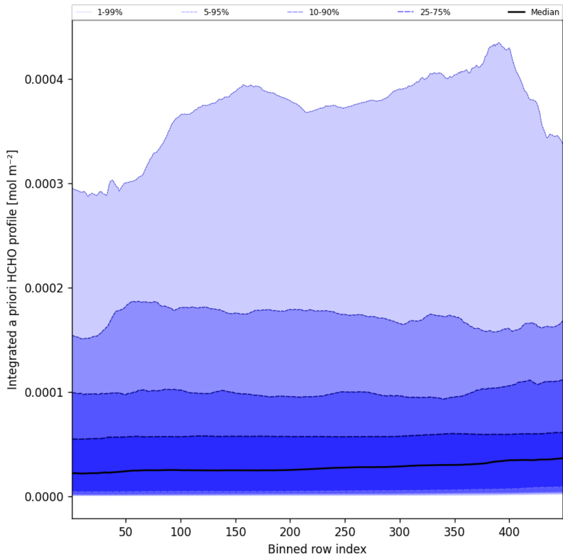
Figure 55: Along track statistics of "Integrated a priori HCHO profile" for 2025-10-17 to 2025-10-18
