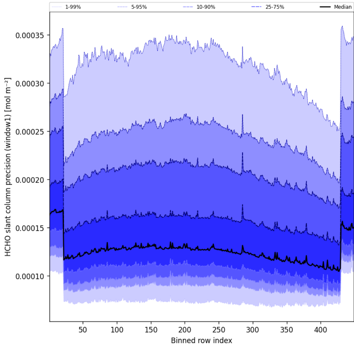
Figure 51: Along track statistics of “HCHO slant column precision (window1)” for 2025-10-17 to 2025-10-18
