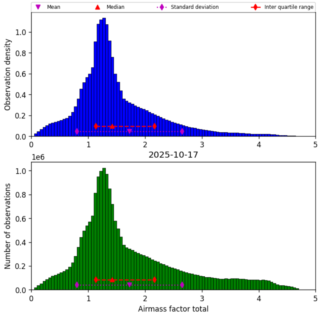
Figure 38: Histogram of “Airmass factor total” for 2025-10-17 to 2025-10-18
