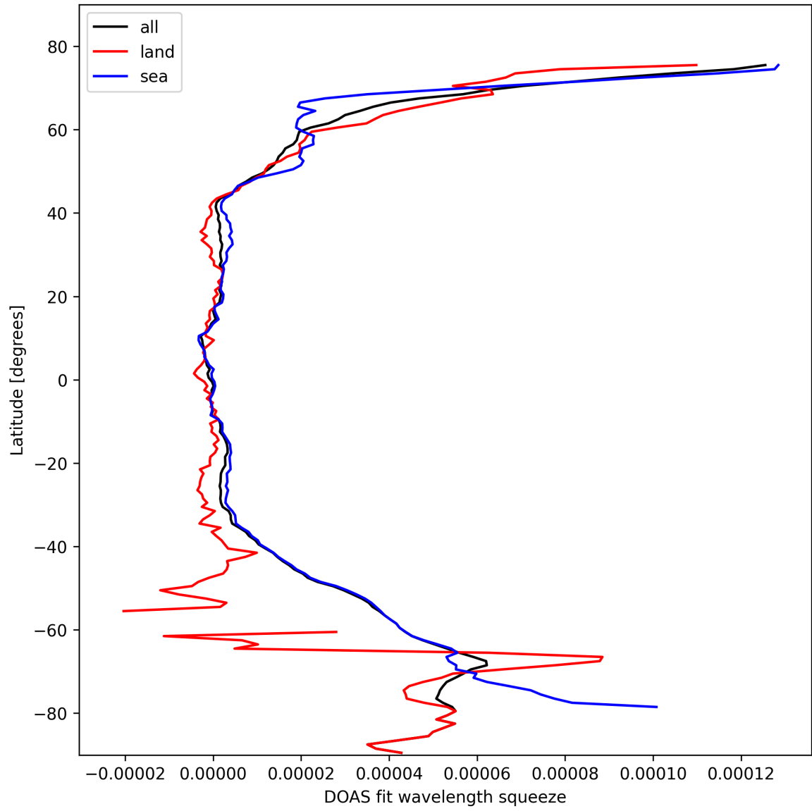
Figure 29: Zonal average of “DOAS fit wavelength squeeze” for 2025-10-17 to 2025-10-18.
