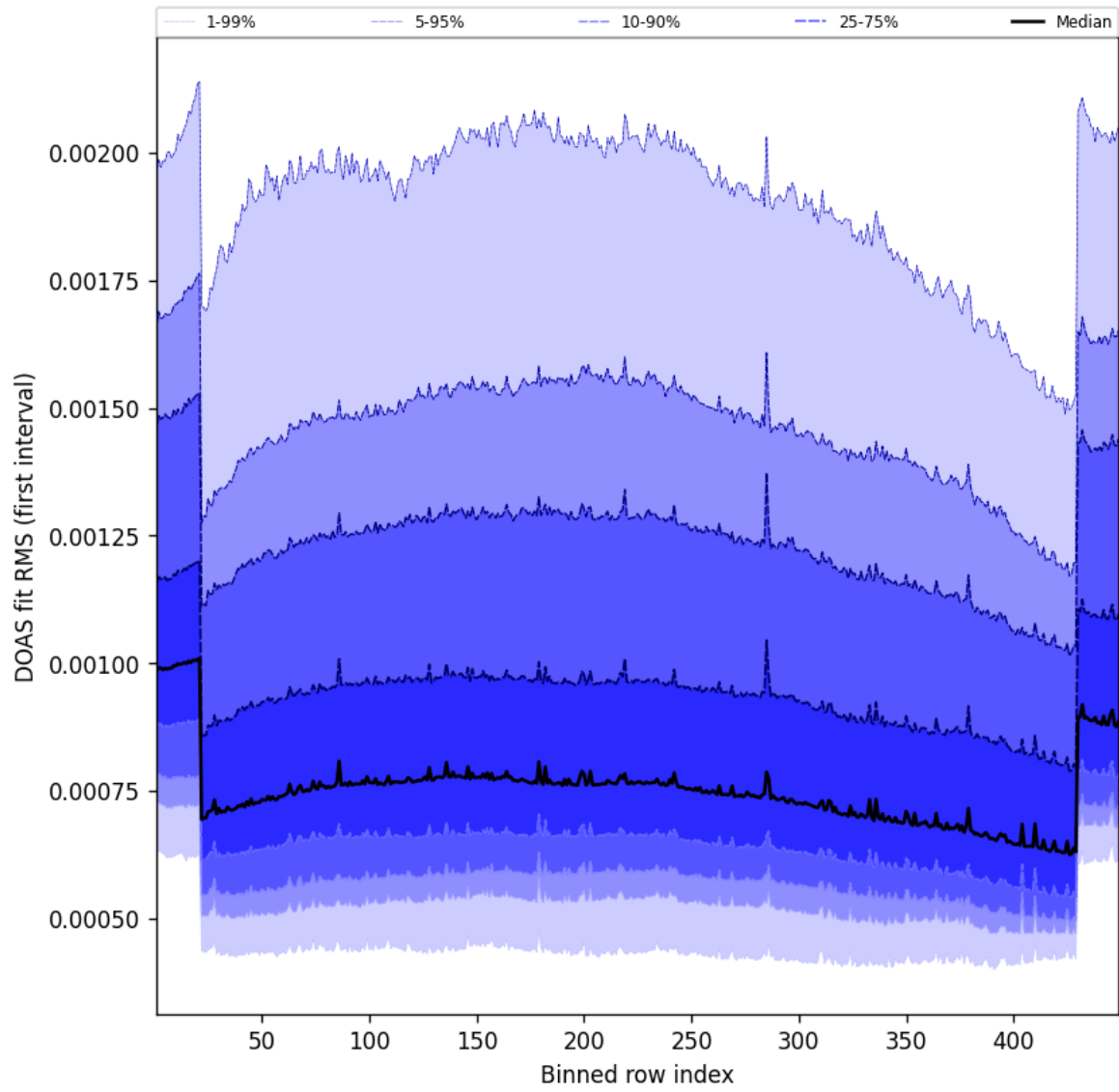
Figure 58: Along track statistics of “DOAS fit RMS (first interval)” for 2025-10-17 to 2025-10-18
