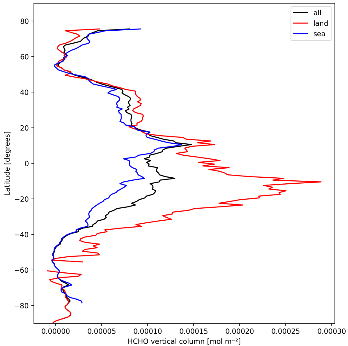
Figure 19: Zonal average of “HCHO vertical column” for 2025-10-17 to 2025-10-18.
