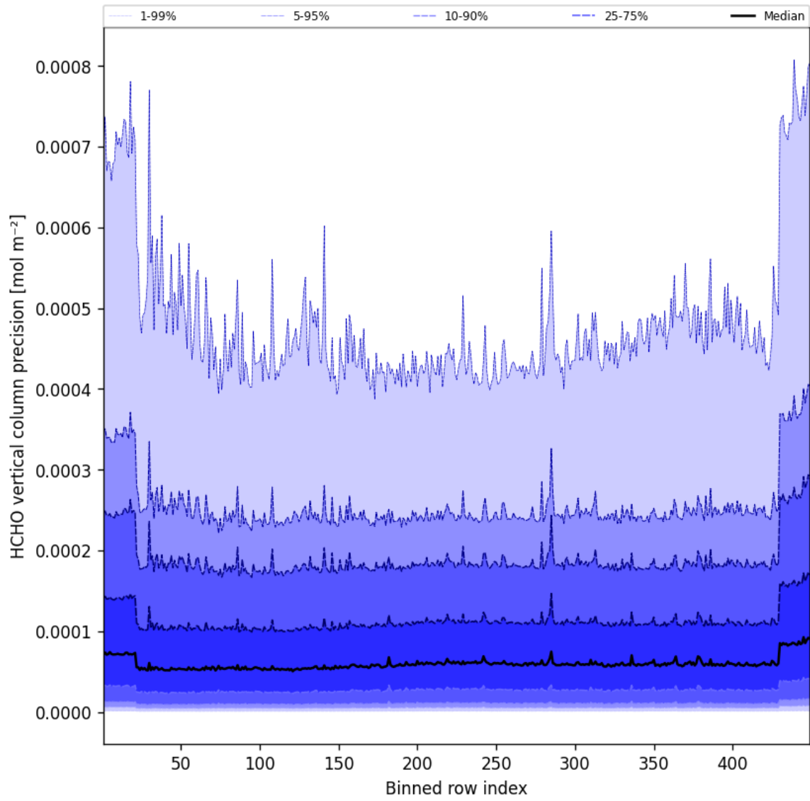
Figure 48: Along track statistics of “HCHO vertical column precision” for 2025-10-17 to 2025-10-18
