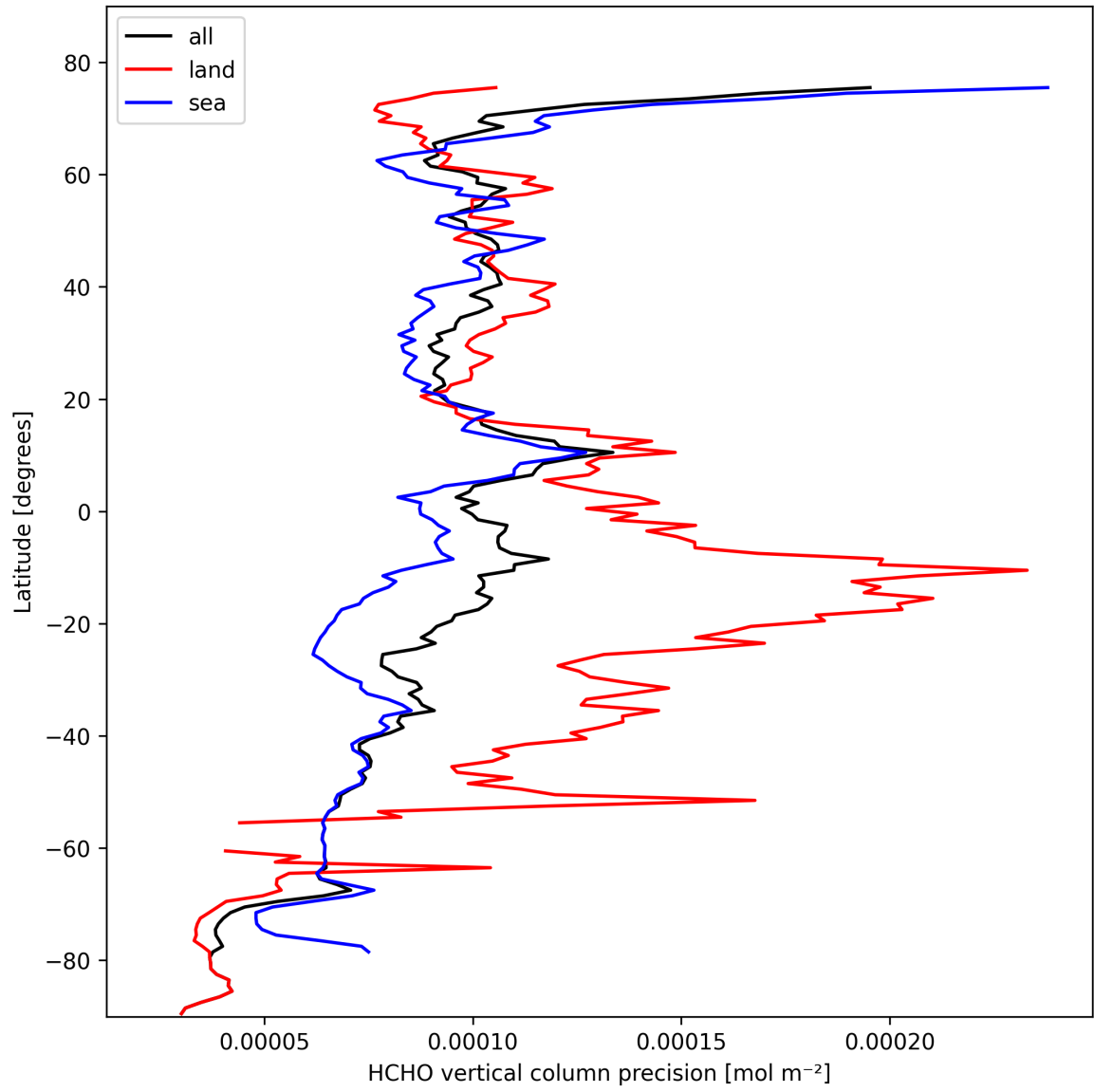
Figure 20: Zonal average of “HCHO vertical column precision” for 2025-10-17 to 2025-10-18.
