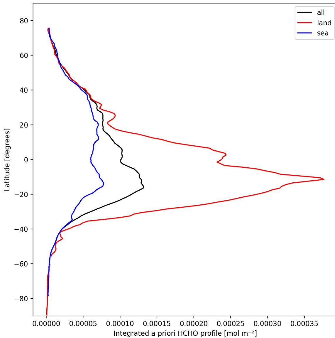
Figure 27: Zonal average of “Integrated a priori HCHO profile” for 2025-10-17 to 2025-10-18.
