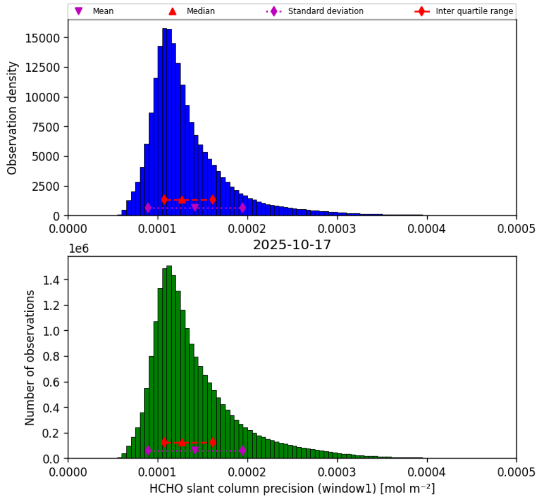
Figure 37: Histogram of “HCHO slant column precision (window1)” for 2025-10-17 to 2025-10-18
