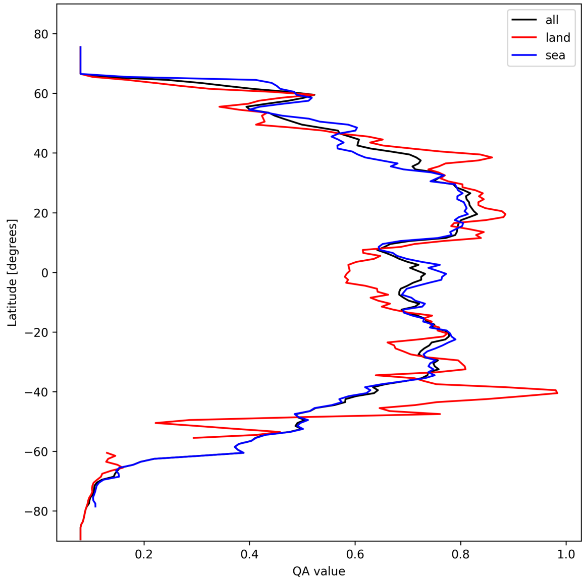
Figure 18: Zonal average of “QA value” for 2025-10-17 to 2025-10-18.
