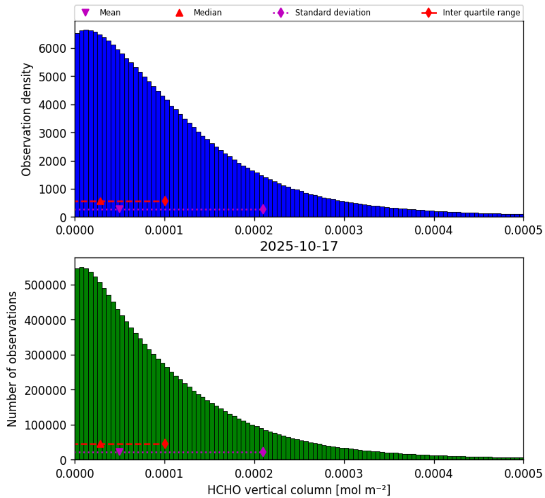
Figure 33: Histogram of “HCHO vertical column” for 2025-10-17 to 2025-10-18
