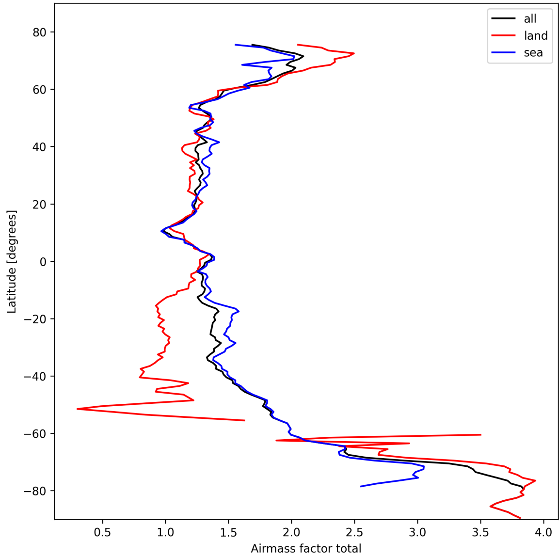
Figure 24: Zonal average of “Airmass factor total” for 2025-10-18 to 2025-10-19.
