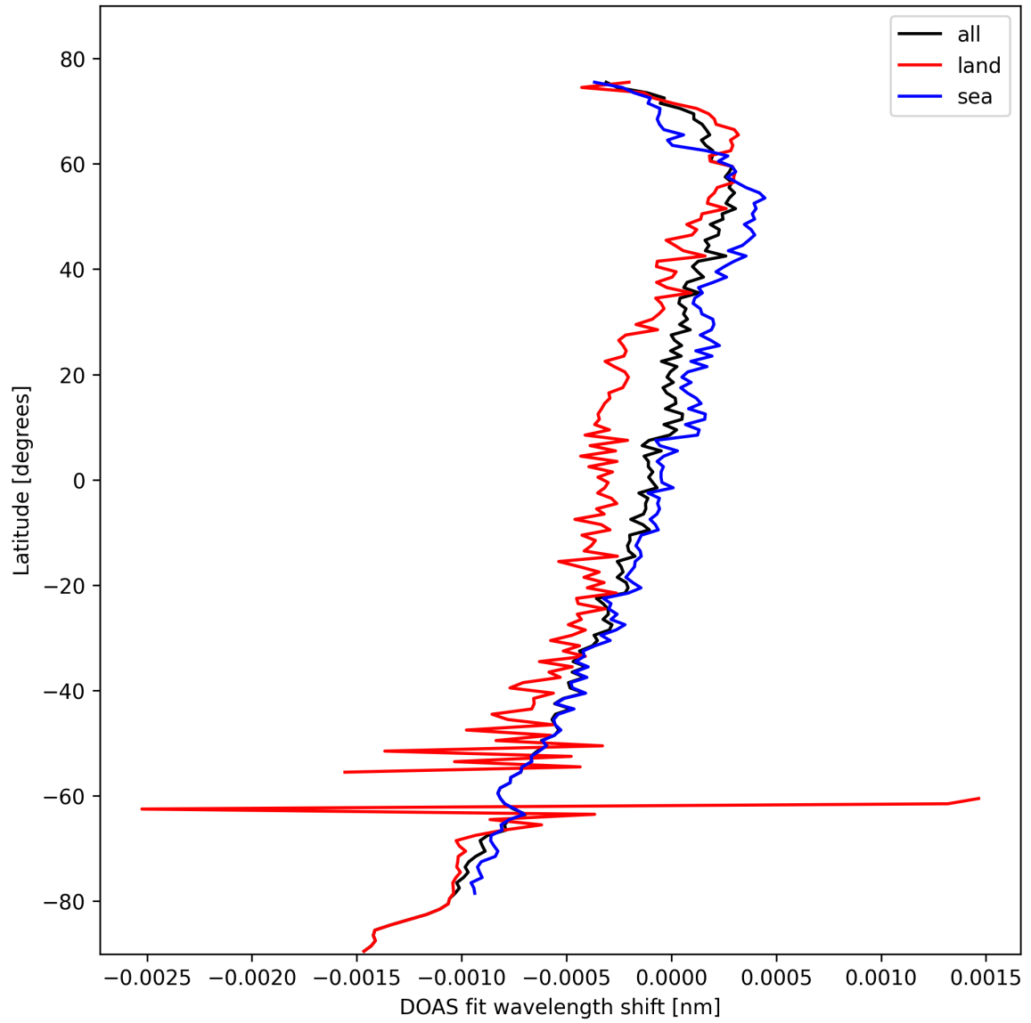
Figure 28: Zonal average of “DOAS fit wavelength shift” for 2025-10-18 to 2025-10-19.
