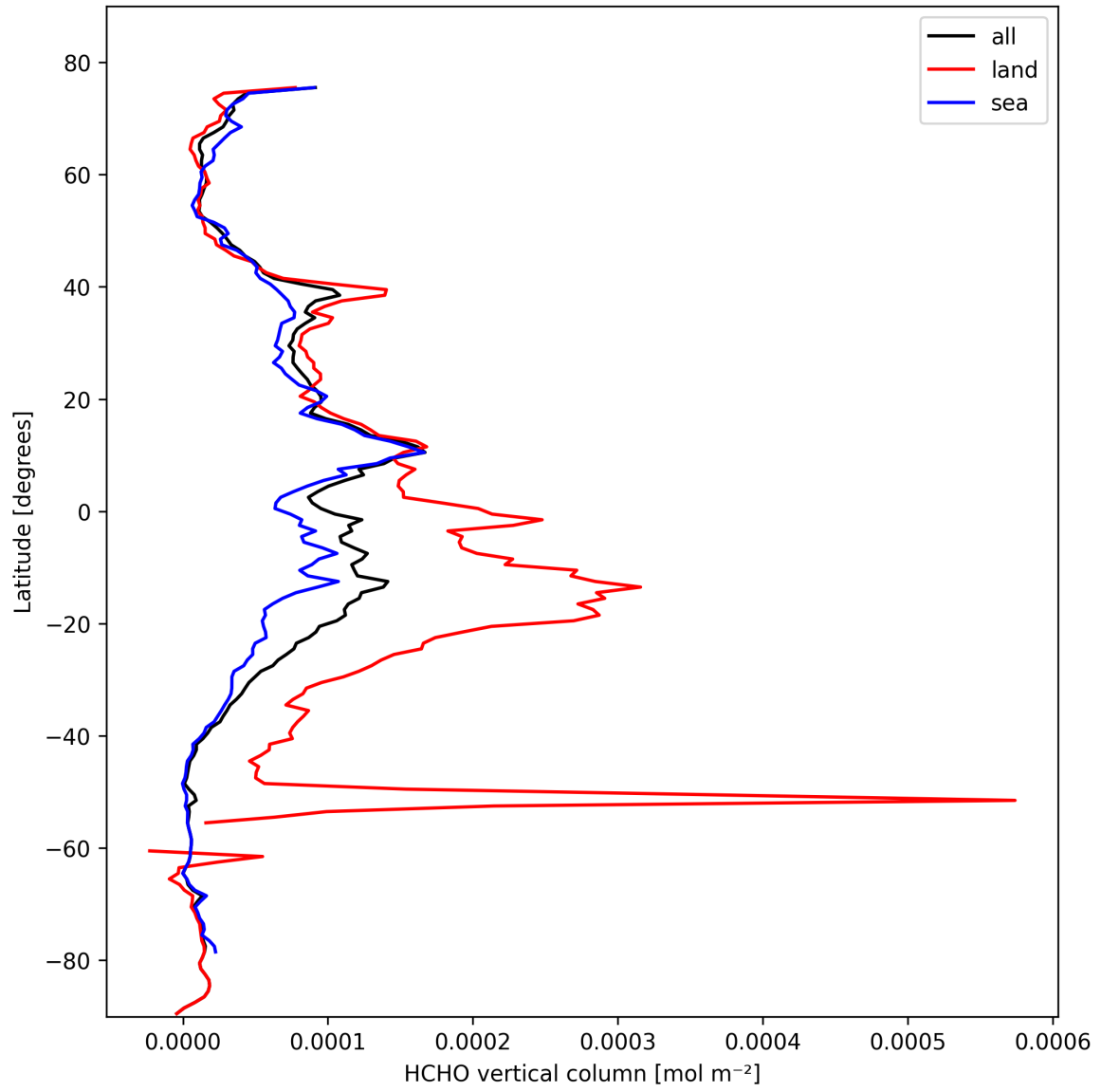
Figure 19: Zonal average of “HCHO vertical column” for 2025-10-18 to 2025-10-19.
