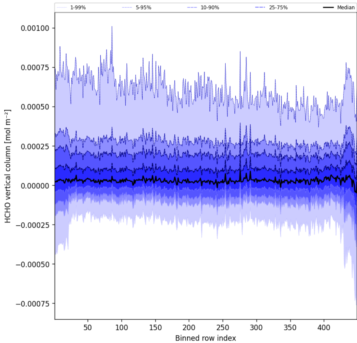
Figure 47: Along track statistics of "HCHO vertical column" for 2025-10-18 to 2025-10-19
