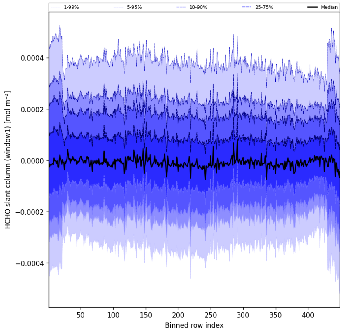
Figure 50: Along track statistics of “HCHO slant column (window1)” for 2025-10-18 to 2025-10-19
