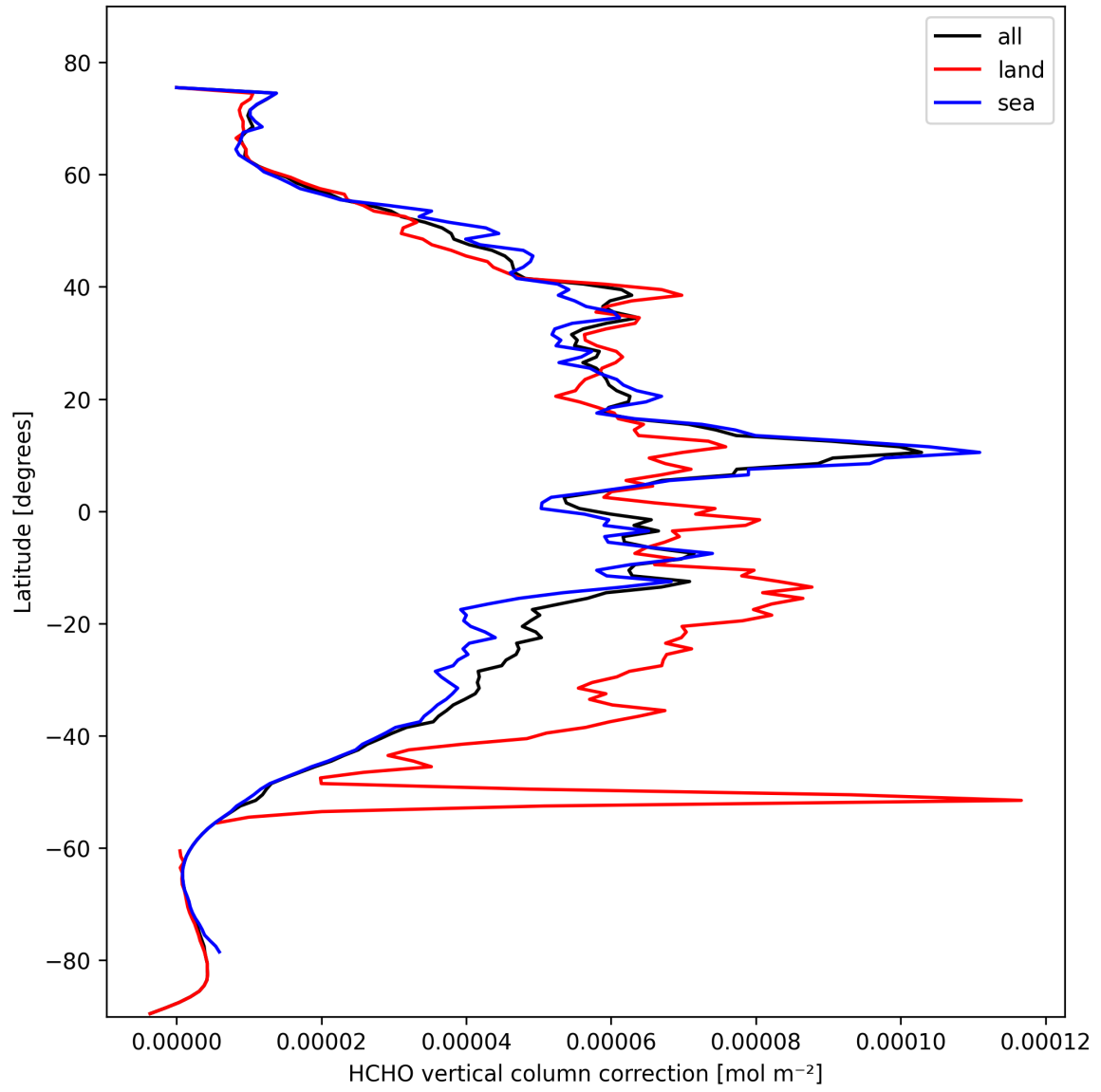
Figure 21: Zonal average of “HCHO vertical column correction” for 2025-10-18 to 2025-10-19.
