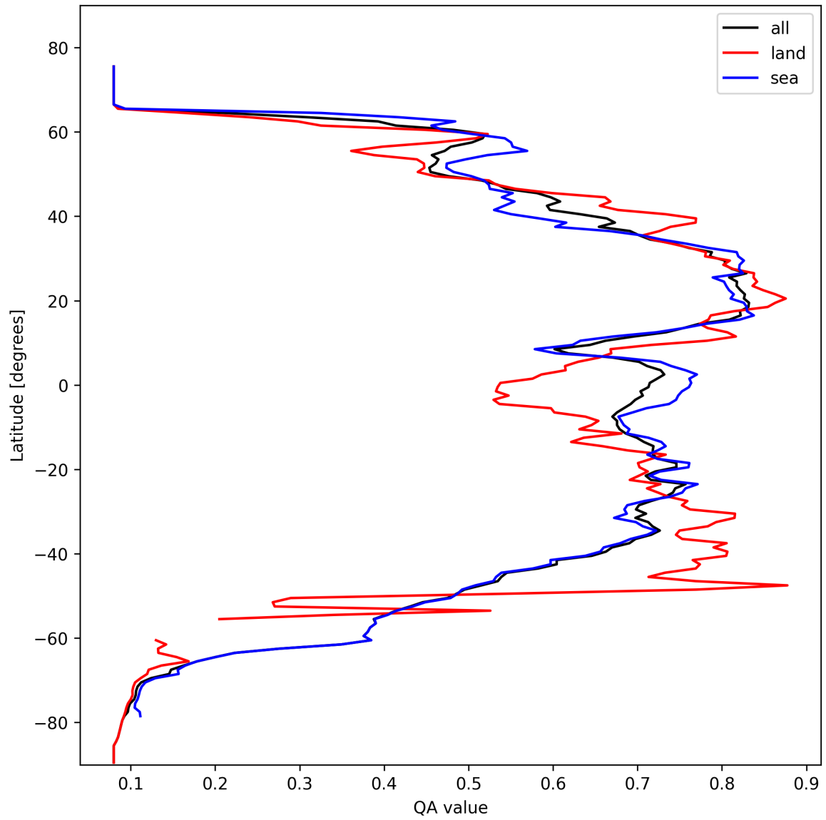
Figure 18: Zonal average of “QA value” for 2025-10-18 to 2025-10-19.
