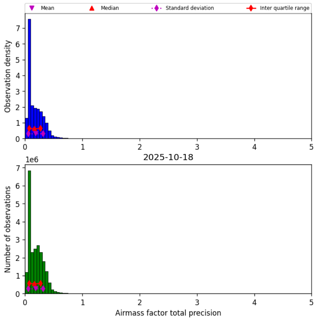
Figure 39: Histogram of “Airmass factor total precision” for 2025-10-18 to 2025-10-19
