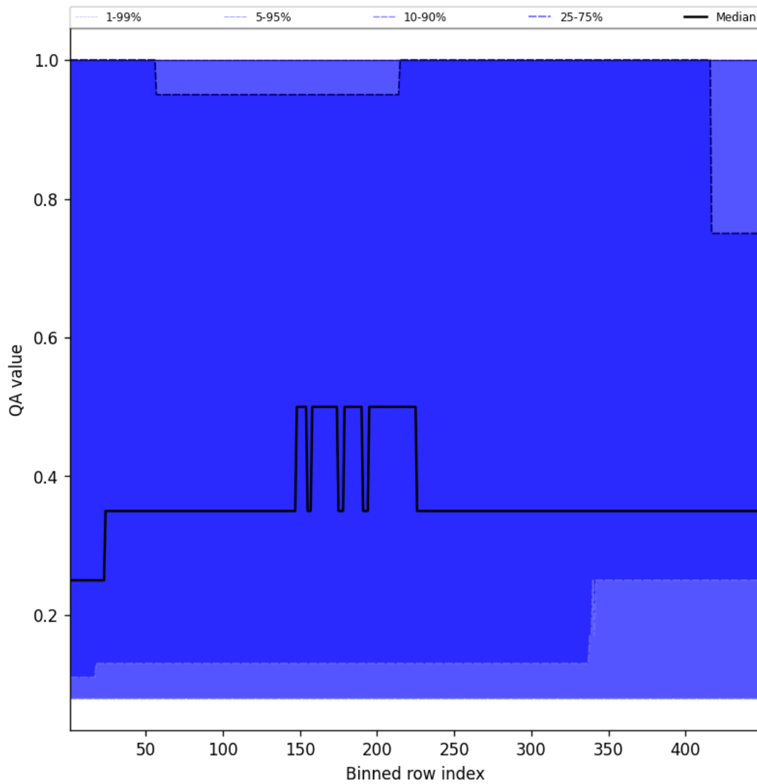
Figure 46: Along track statistics of “QA value” for 2025-10-18 to 2025-10-19
