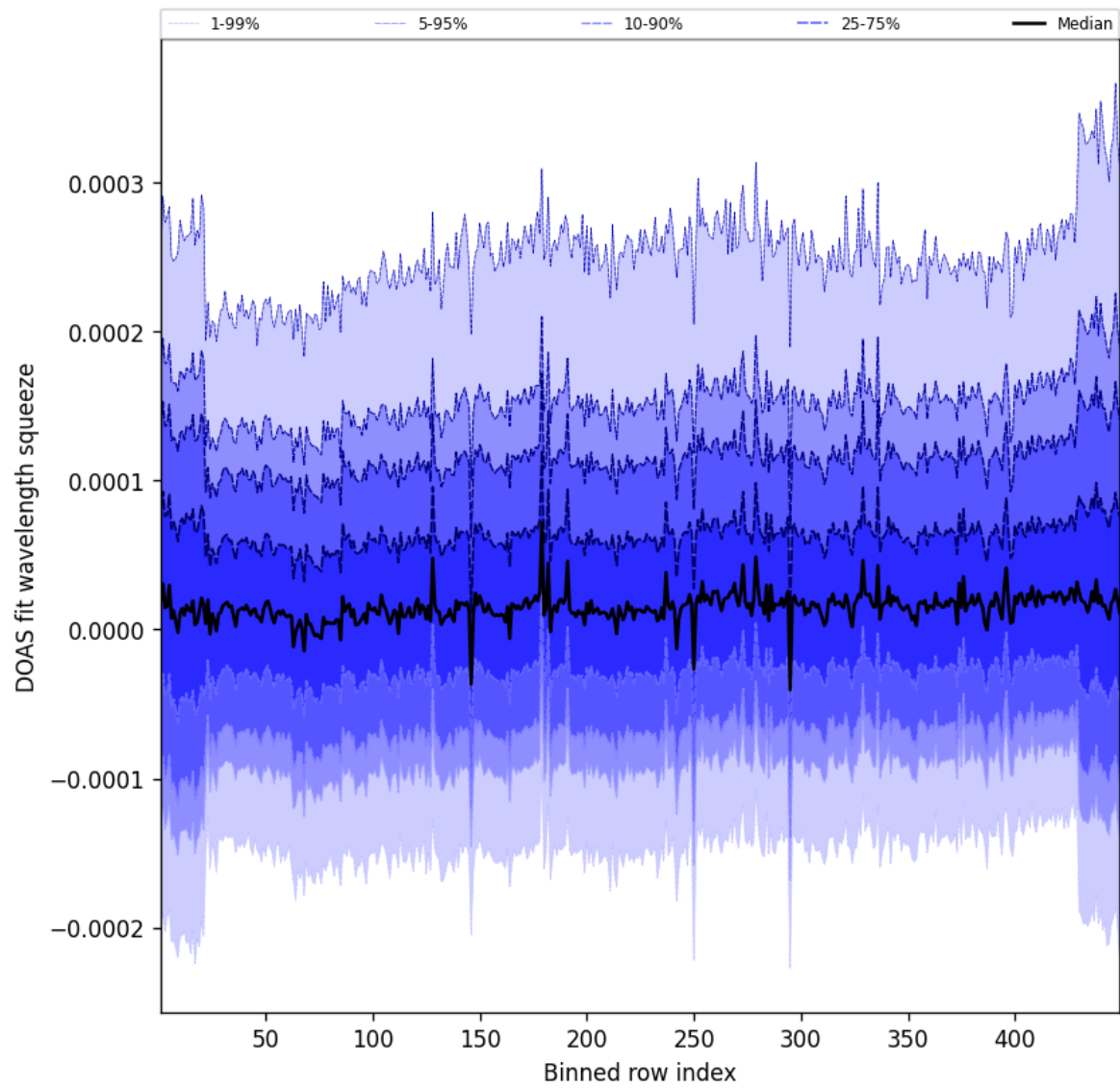
Figure 57: Along track statistics of “DOAS fit wavelength squeeze” for 2025-10-18 to 2025-10-19
