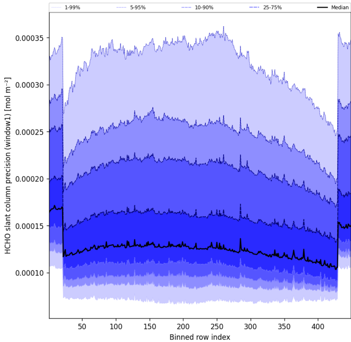
Figure 51: Along track statistics of “HCHO slant column precision (window1)” for 2025-10-18 to 2025-10-19
