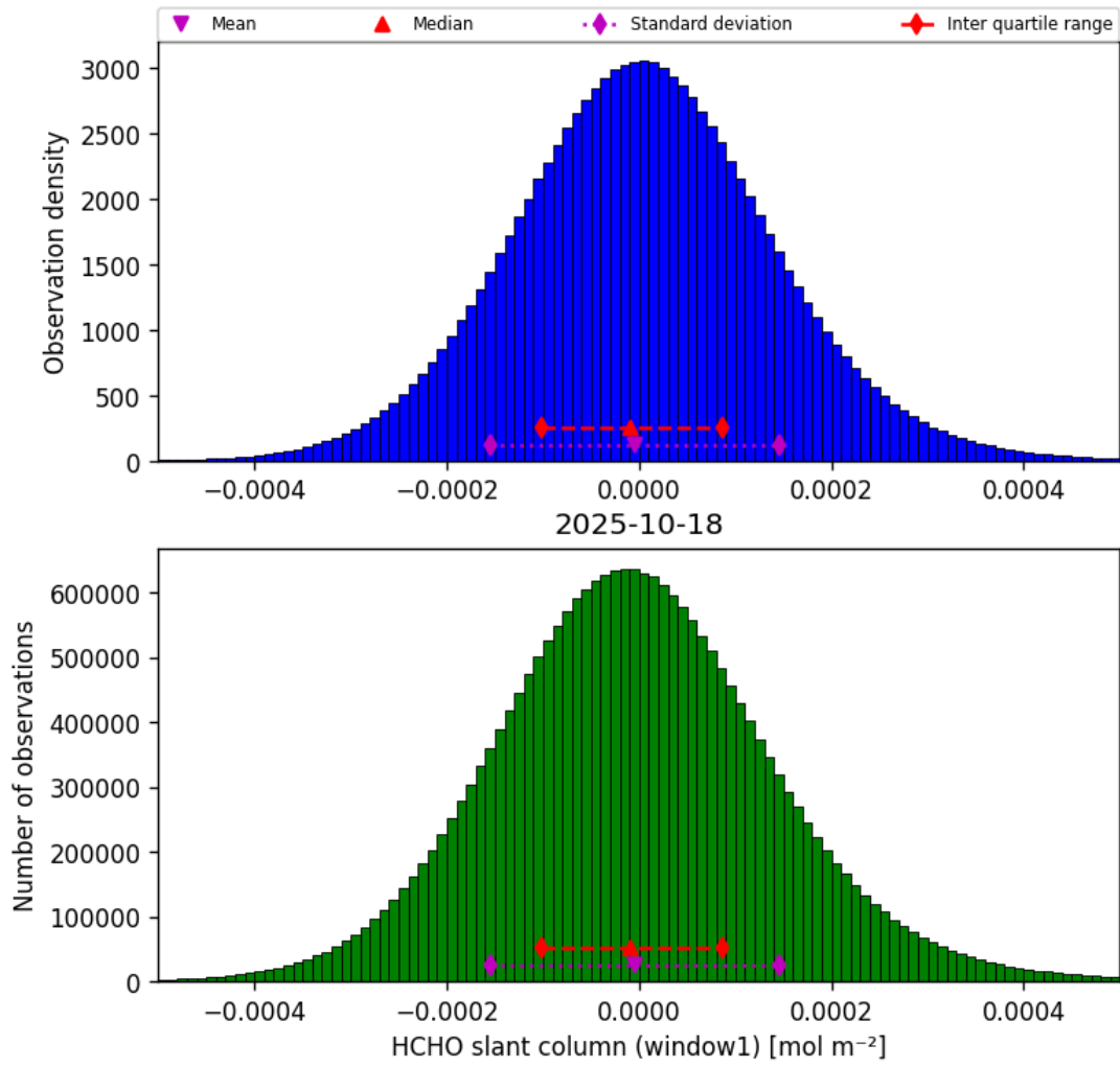
Figure 36: Histogram of “HCHO slant column (window1)” for 2025-10-18 to 2025-10-19
