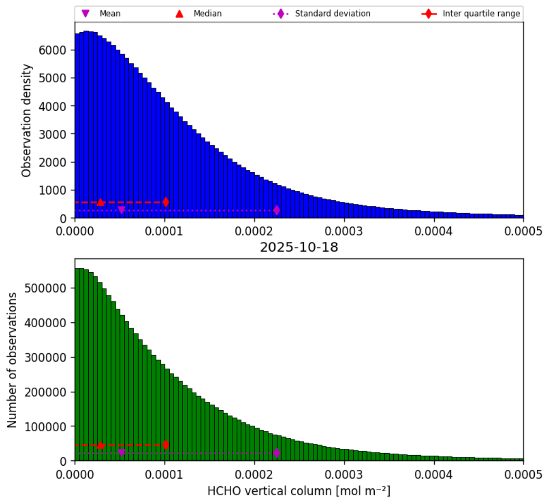
Figure 33: Histogram of “HCHO vertical column” for 2025-10-18 to 2025-10-19
