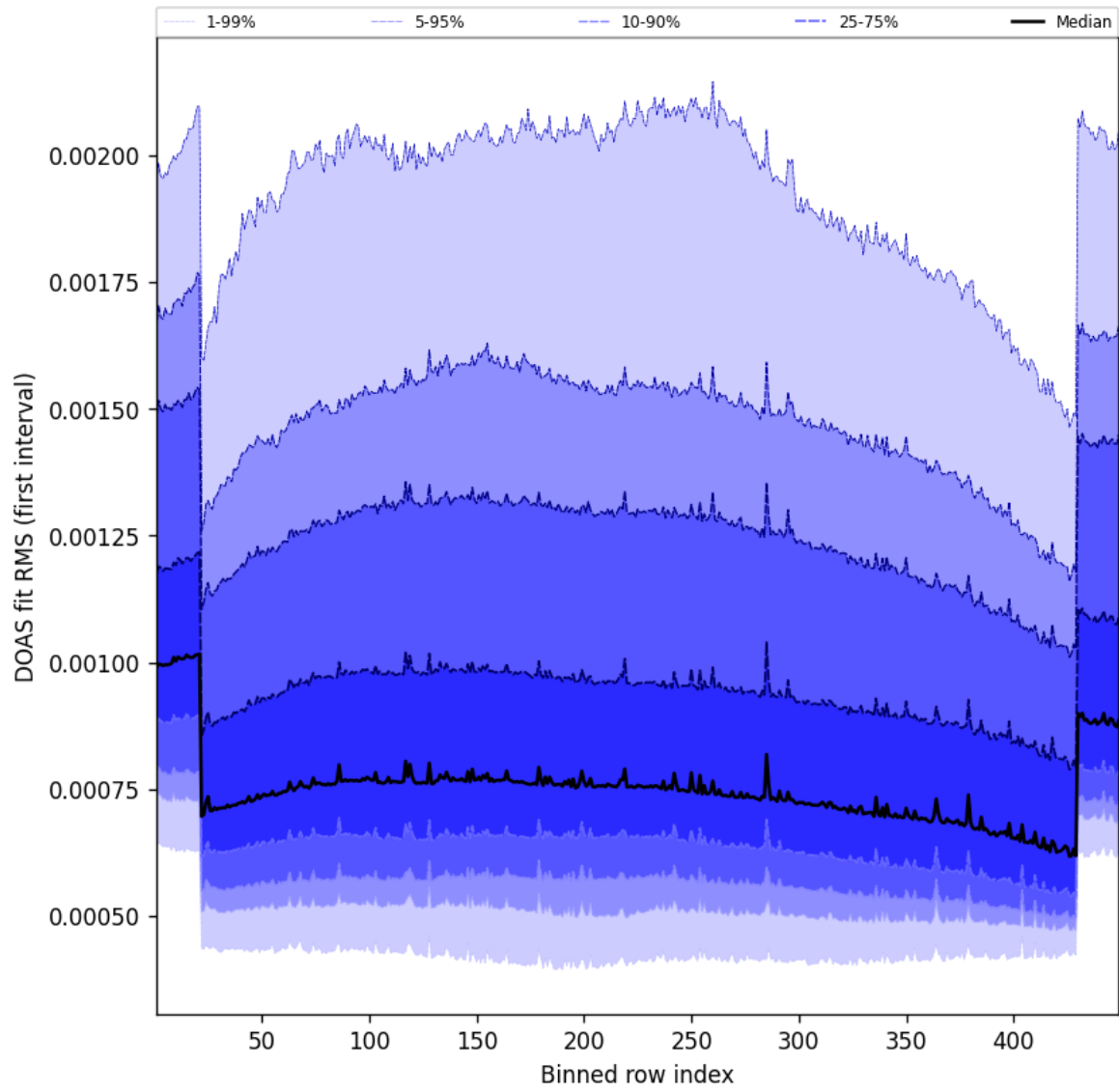
Figure 58: Along track statistics of “DOAS fit RMS (first interval)” for 2025-10-18 to 2025-10-19
