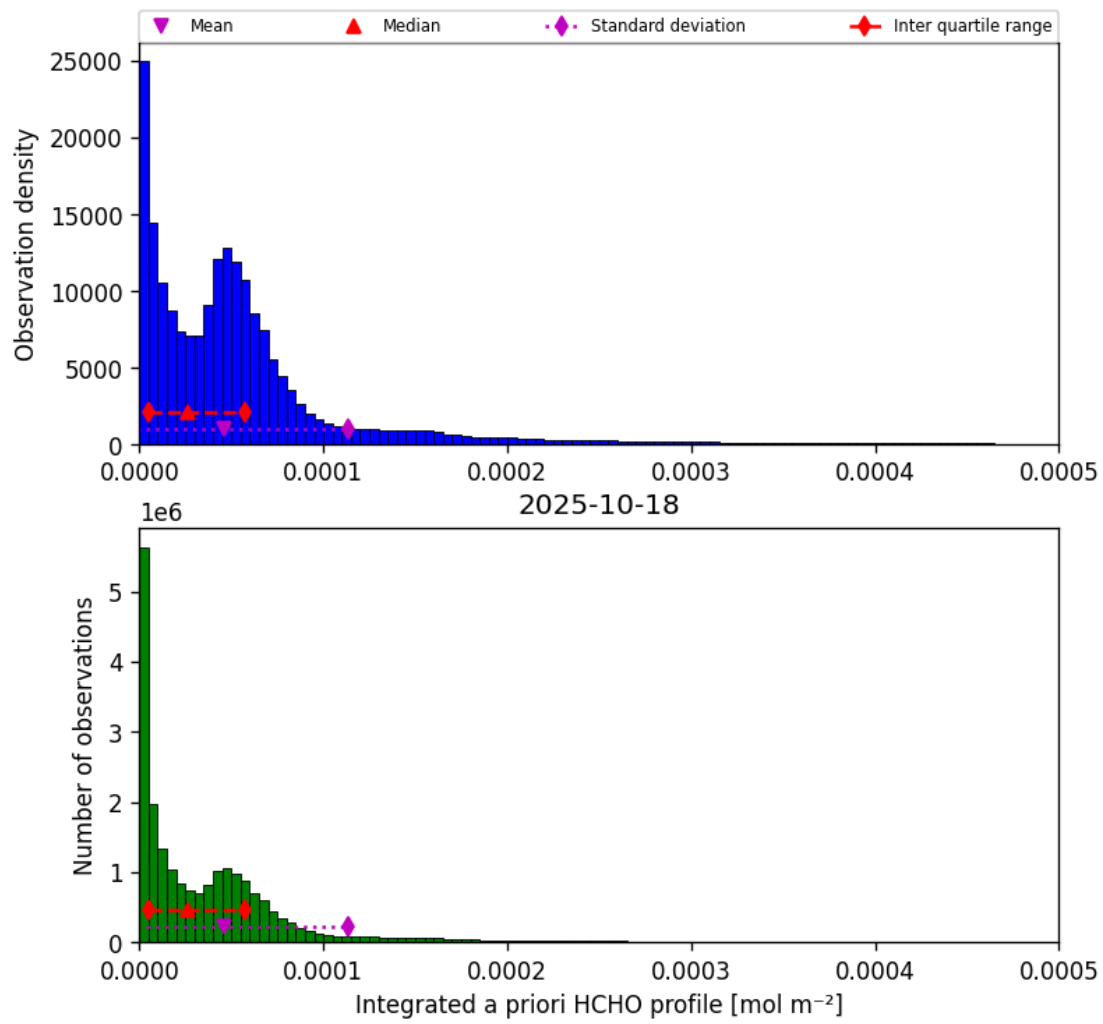
Figure 41: Histogram of “Integrated a priori HCHO profile” for 2025-10-18 to 2025-10-19
