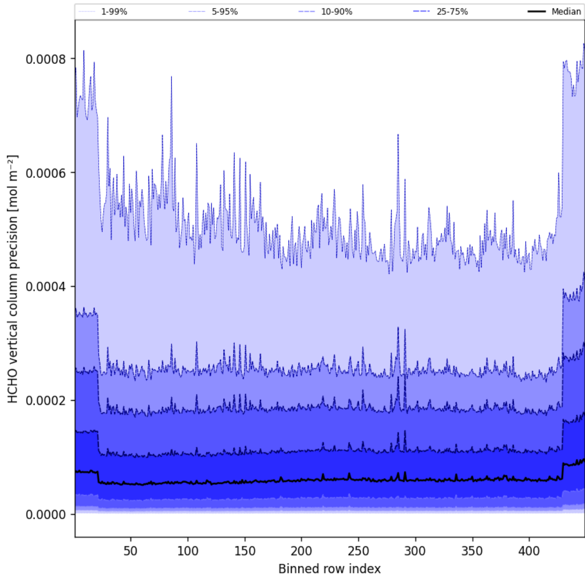
Figure 48: Along track statistics of “HCHO vertical column precision” for 2025-10-18 to 2025-10-19
