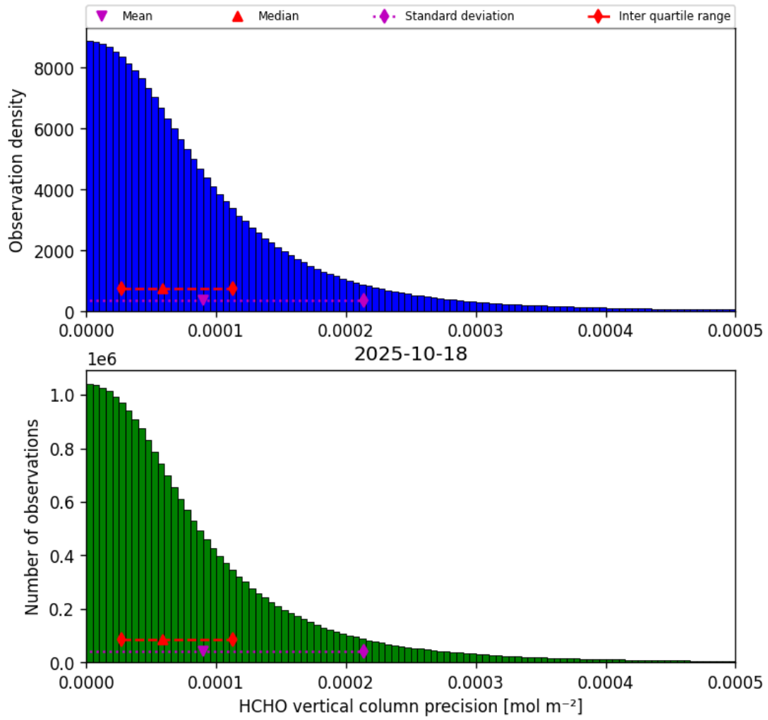
Figure 34: Histogram of “HCHO vertical column precision” for 2025-10-18 to 2025-10-19
