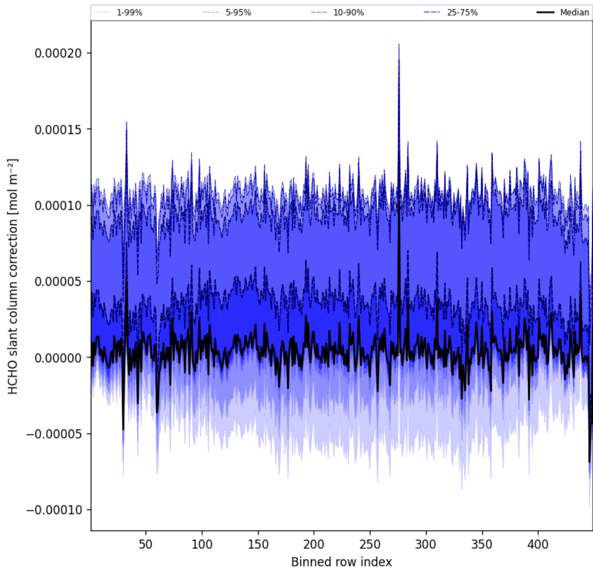
Figure 59: Along track statistics of “HCHO slant column correction” for 2025-10-18 to 2025-10-19
