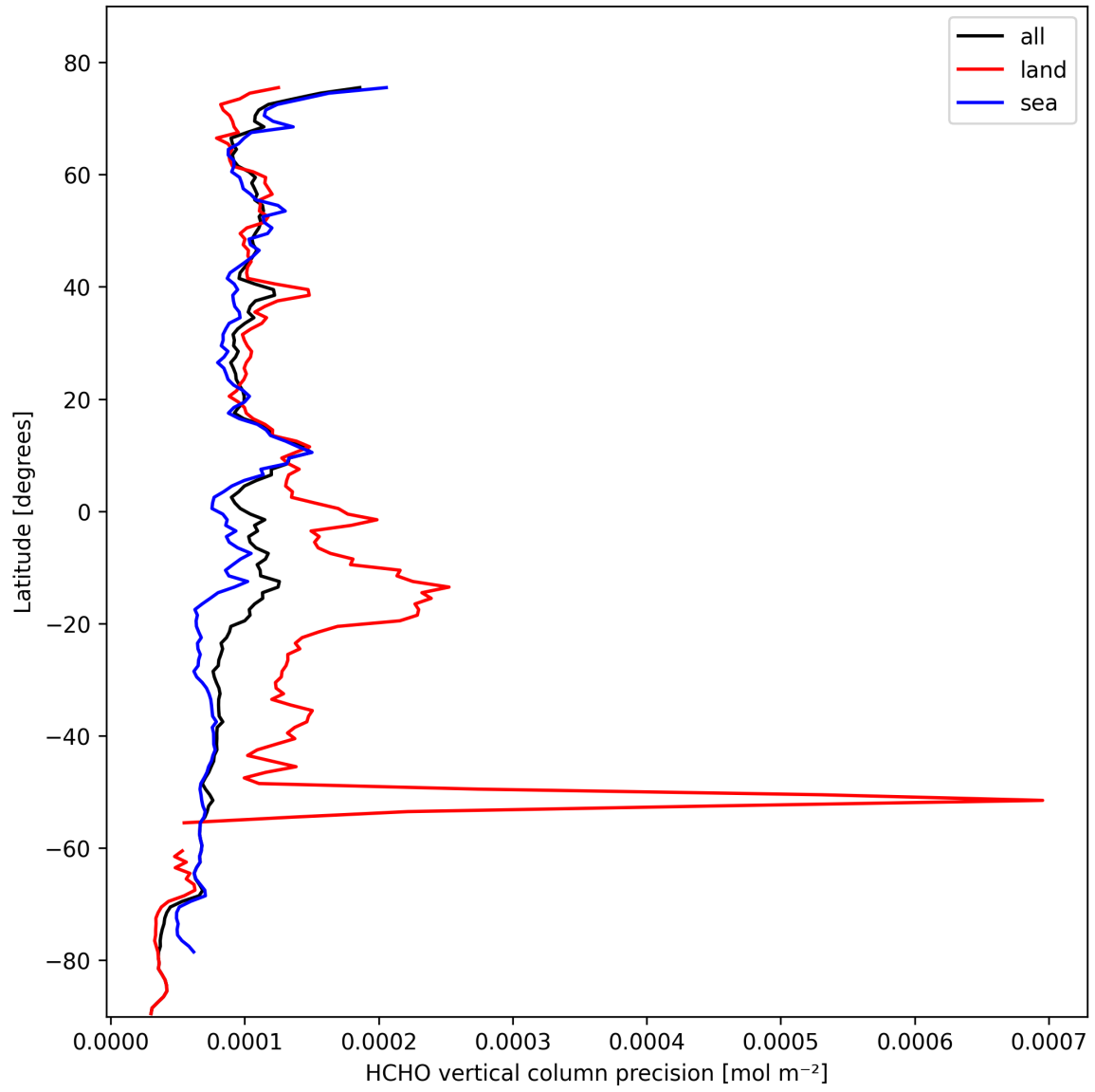
Figure 20: Zonal average of “HCHO vertical column precision” for 2025-10-18 to 2025-10-19.
