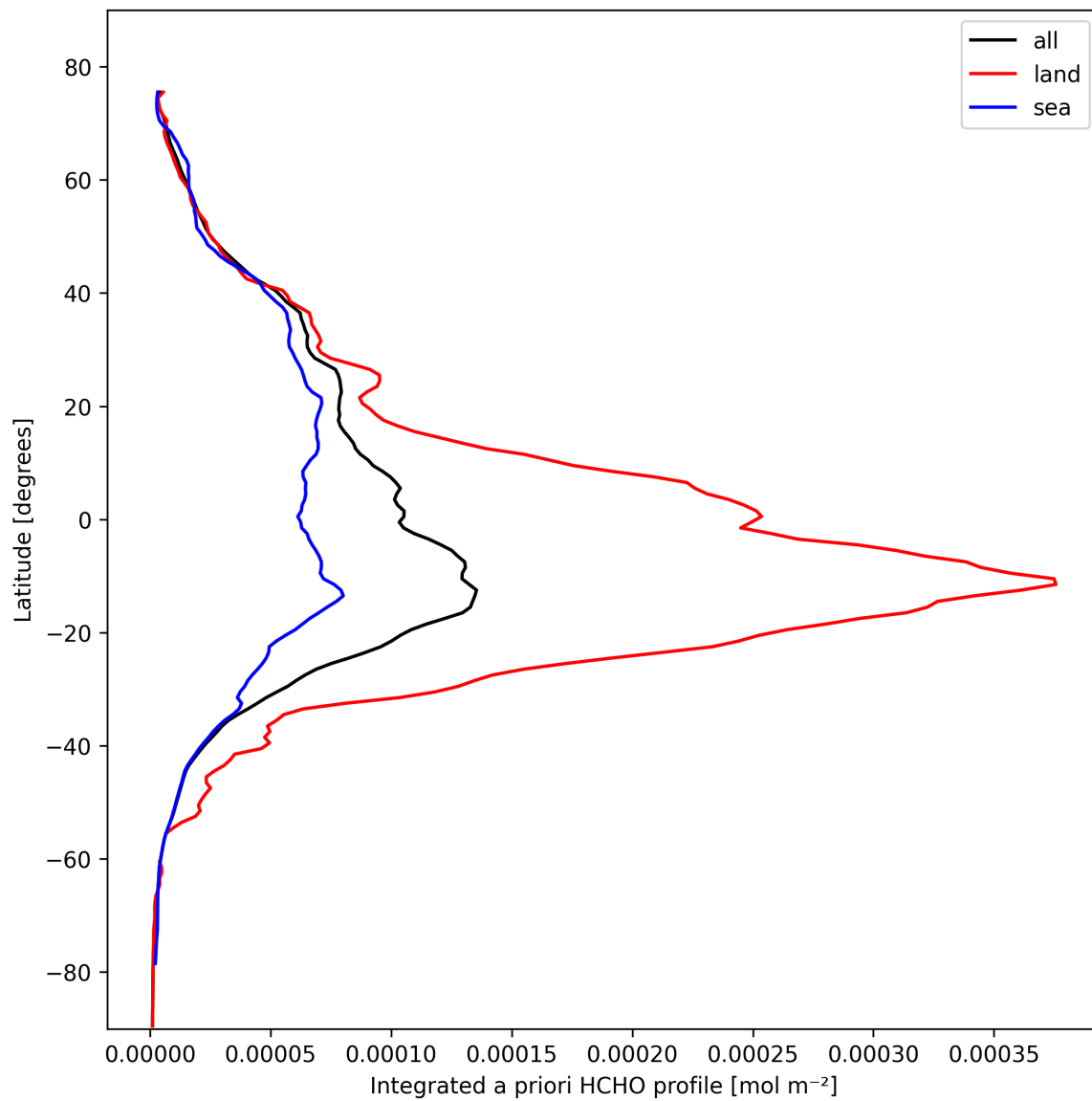
Figure 27: Zonal average of “Integrated a priori HCHO profile” for 2025-10-18 to 2025-10-19.
