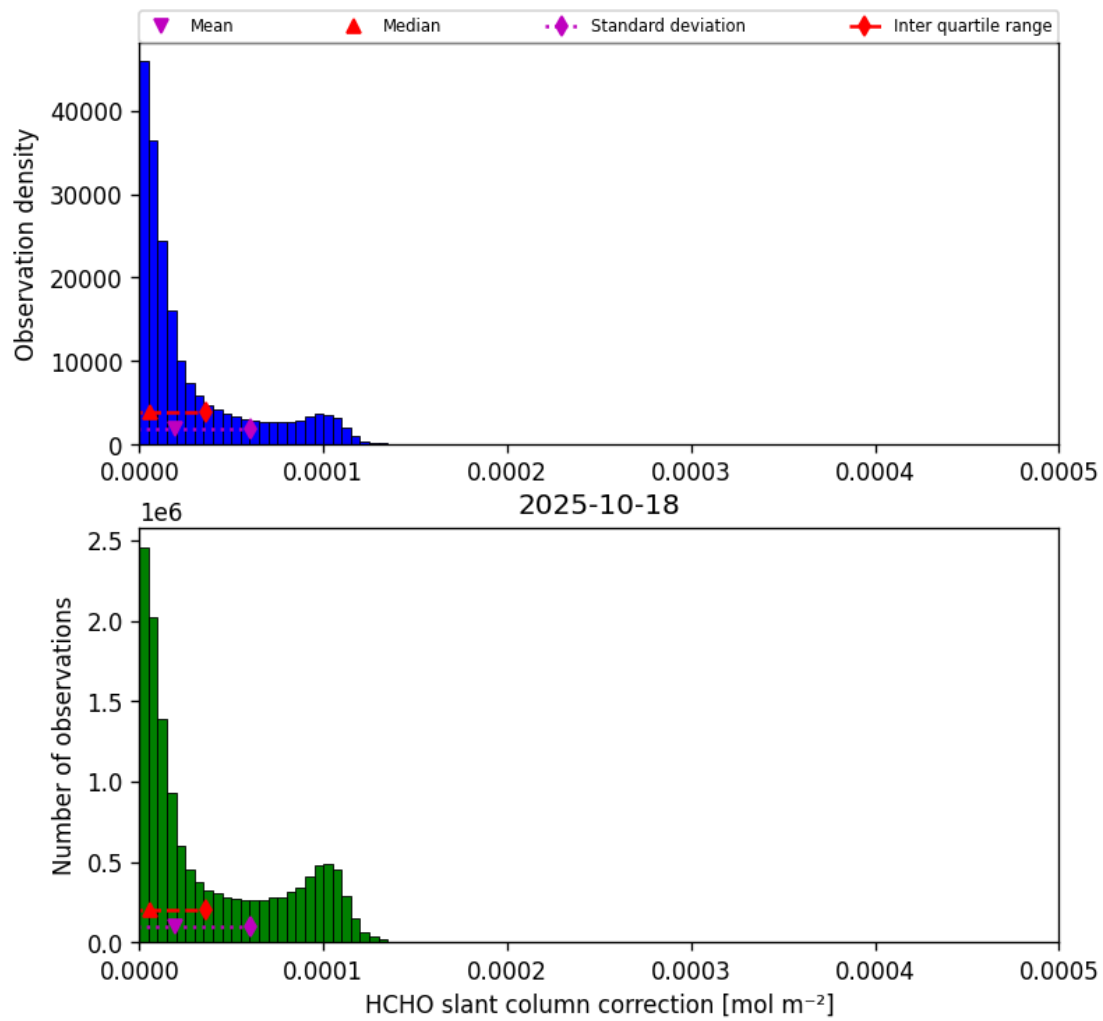
Figure 45: Histogram of “HCHO slant column correction” for 2025-10-18 to 2025-10-19
