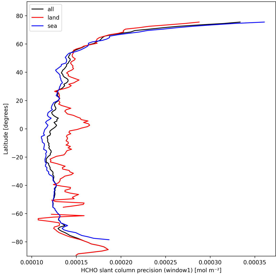
Figure 23: Zonal average of “HCHO slant column precision (window1)” for 2025-10-18 to 2025-10-19.
