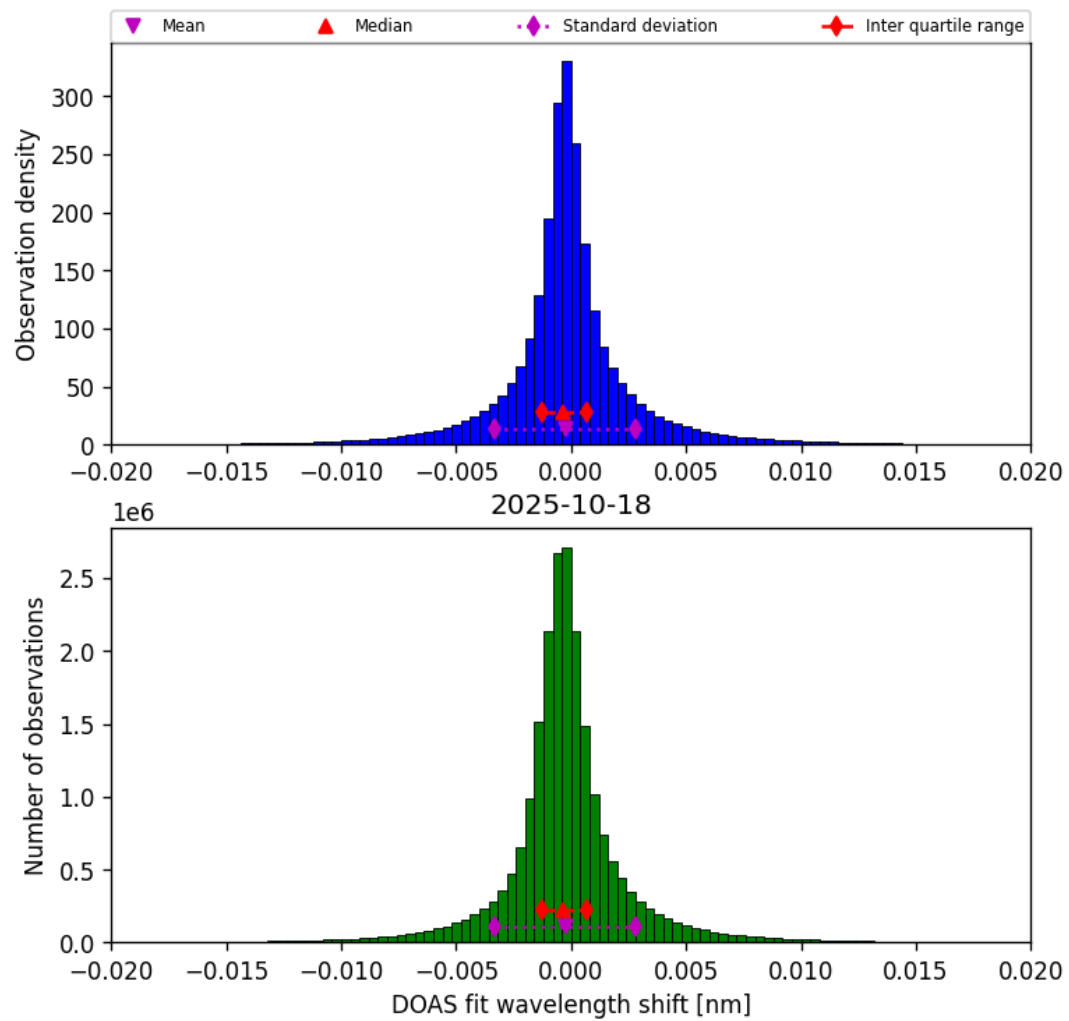
Figure 42: Histogram of “DOAS fit wavelength shift” for 2025-10-18 to 2025-10-19
