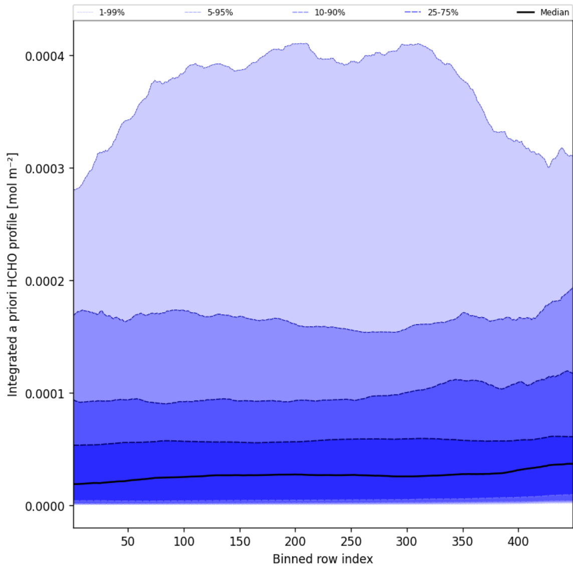
Figure 55: Along track statistics of "Integrated a priori HCHO profile" for 2025-10-18 to 2025-10-19
