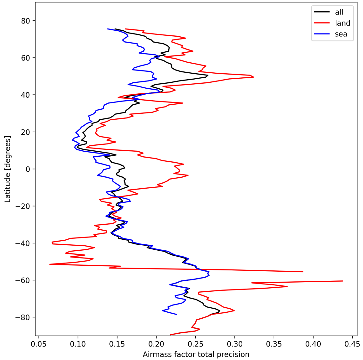
Figure 25: Zonal average of “Airmass factor total precision” for 2025-10-18 to 2025-10-19.
