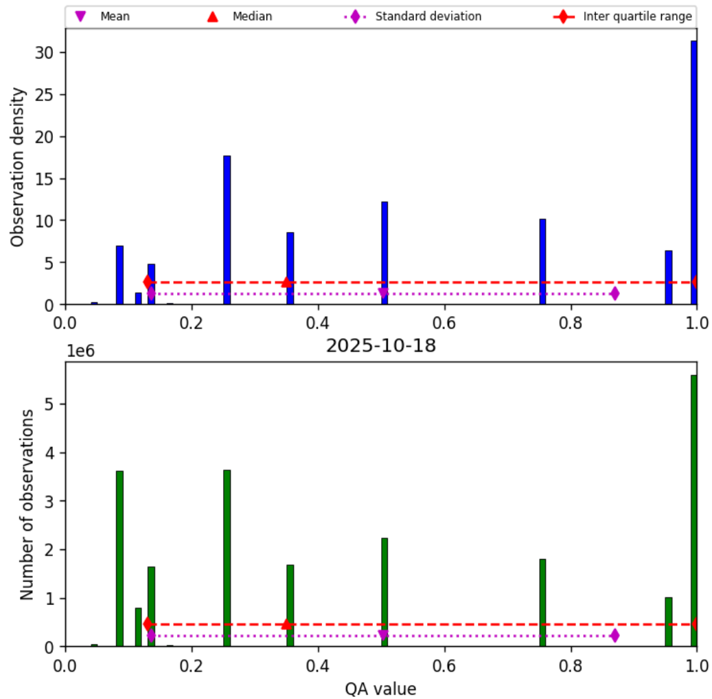
Figure 32: Histogram of “QA value” for 2025-10-18 to 2025-10-19
