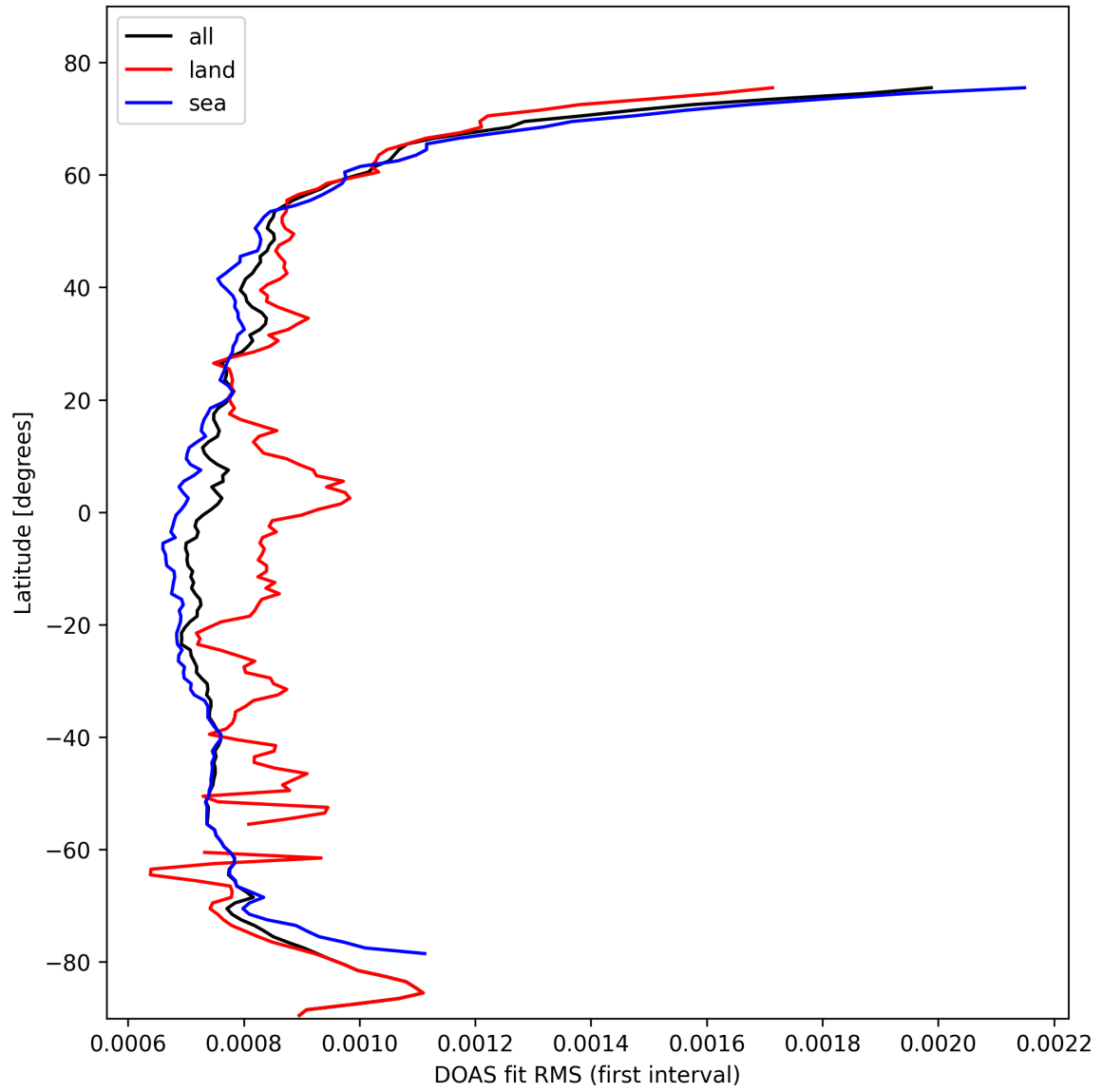
Figure 30: Zonal average of “DOAS fit RMS (first interval)” for 2025-10-18 to 2025-10-19.
