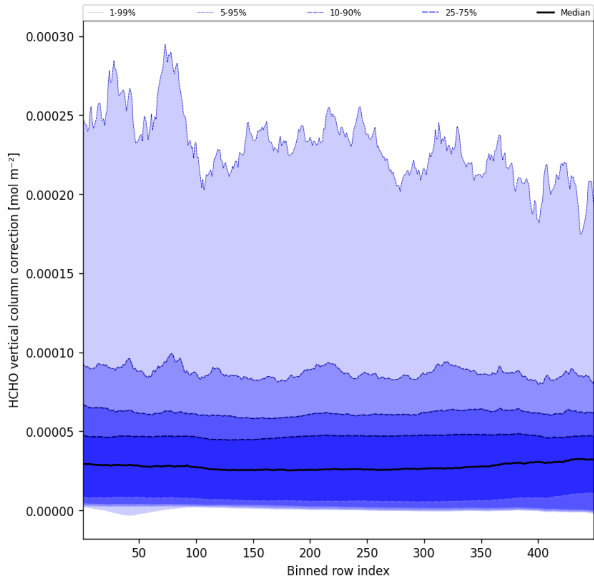
Figure 49: Along track statistics of “HCHO vertical column correction” for 2025-10-18 to 2025-10-19
