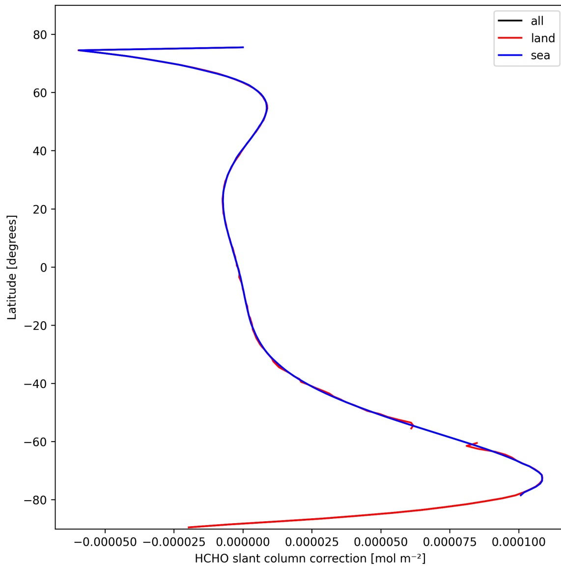
Figure 31: Zonal average of “HCHO slant column correction” for 2025-10-18 to 2025-10-19.
