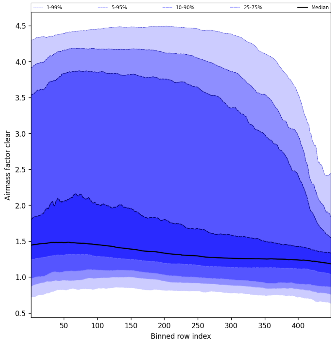
Figure 54: Along track statistics of “Air mass factor clear” for 2025-10-18 to 2025-10-19
