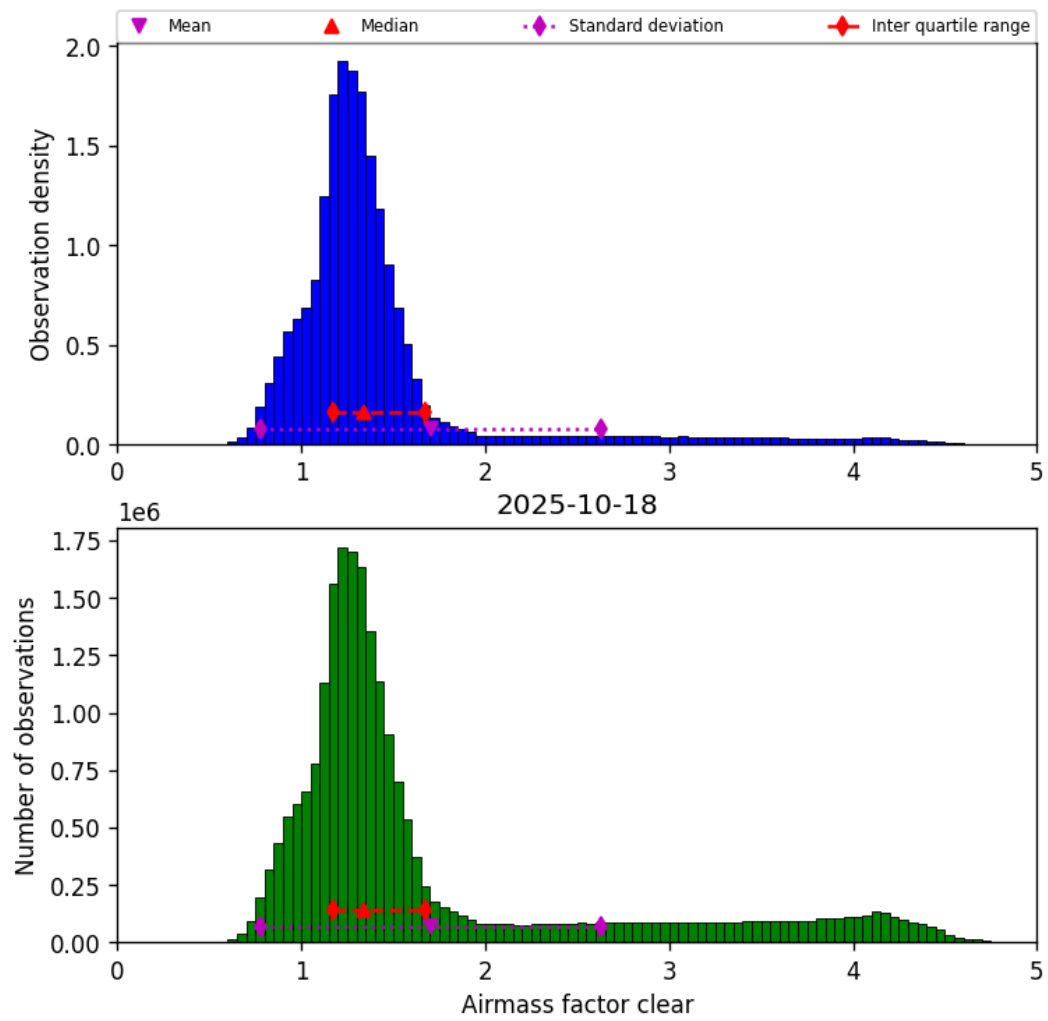
Figure 40: Histogram of “Airmass factor clear” for 2025-10-18 to 2025-10-19
