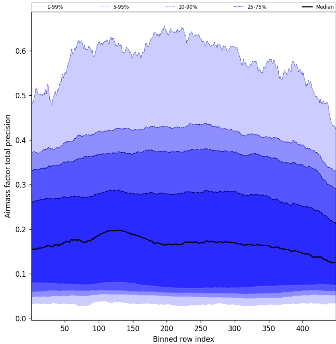
Figure 53: Along track statistics of “Airmass factor total precision” for 2025-10-18 to 2025-10-19
