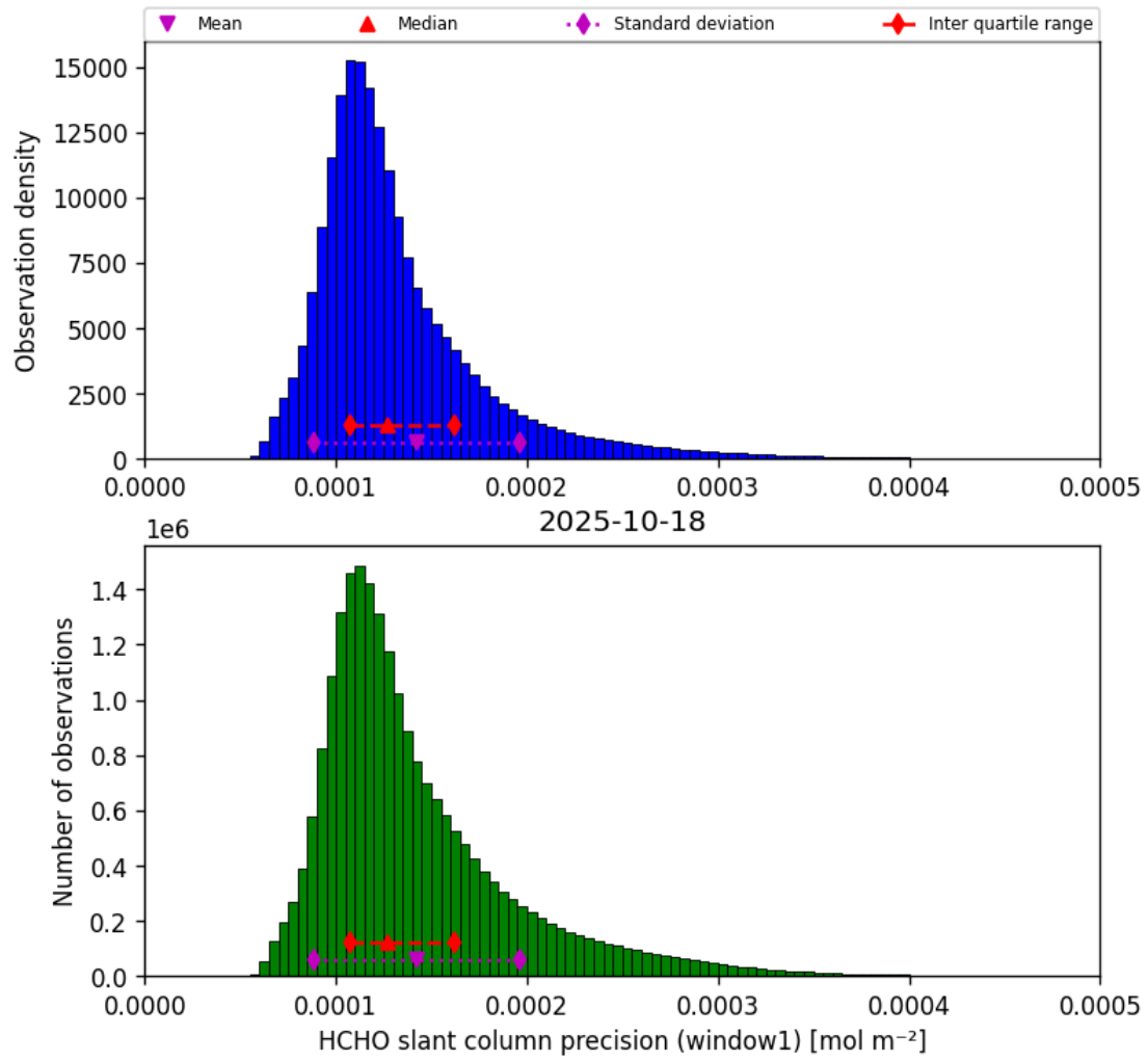
Figure 37: Histogram of “HCHO slant column precision (window1)” for 2025-10-18 to 2025-10-19
