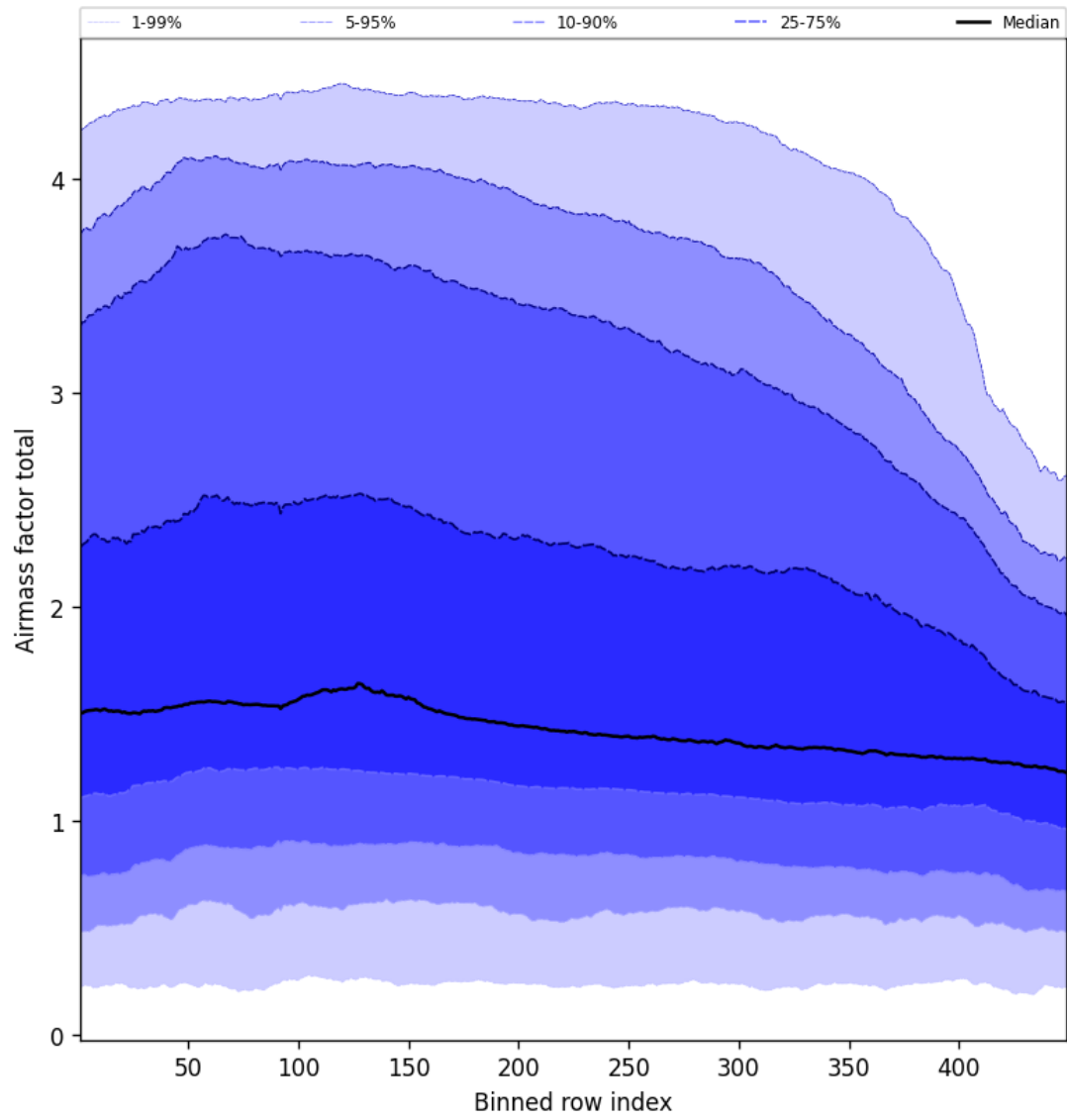
Figure 52: Along track statistics of “Airmass factor total” for 2025-10-18 to 2025-10-19
