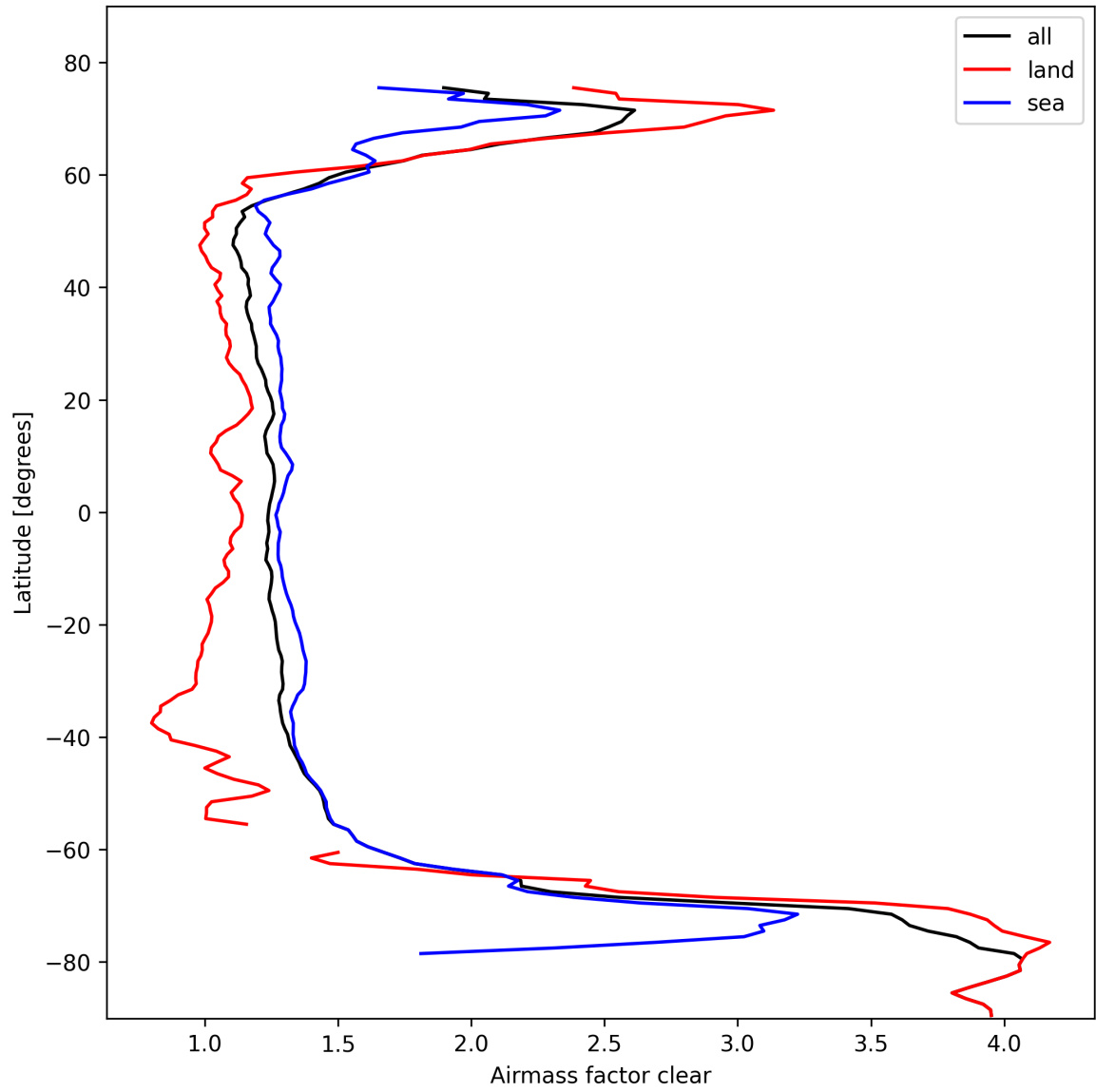
Figure 26: Zonal average of “Airmass factor clear” for 2025-10-18 to 2025-10-19.
