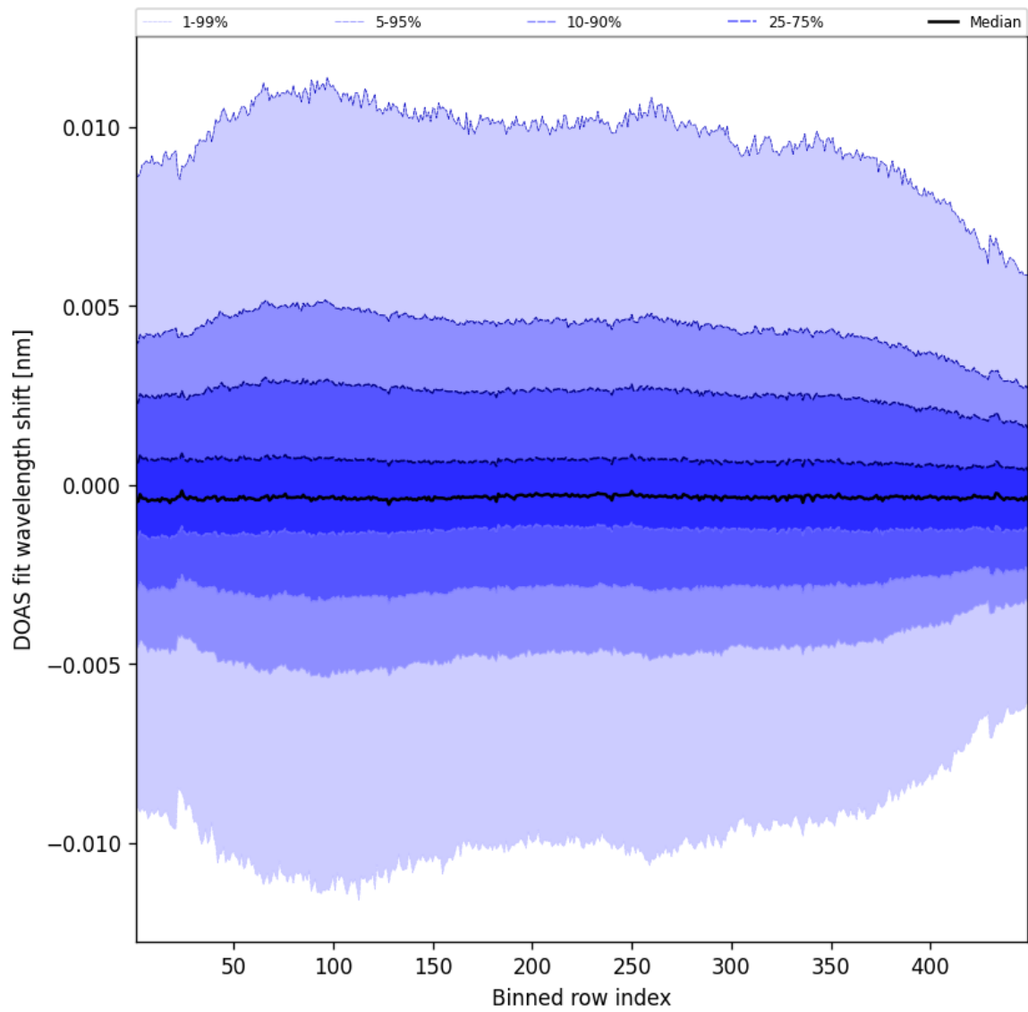
Figure 56: Along track statistics of “DOAS fit wavelength shift” for 2025-10-18 to 2025-10-19
