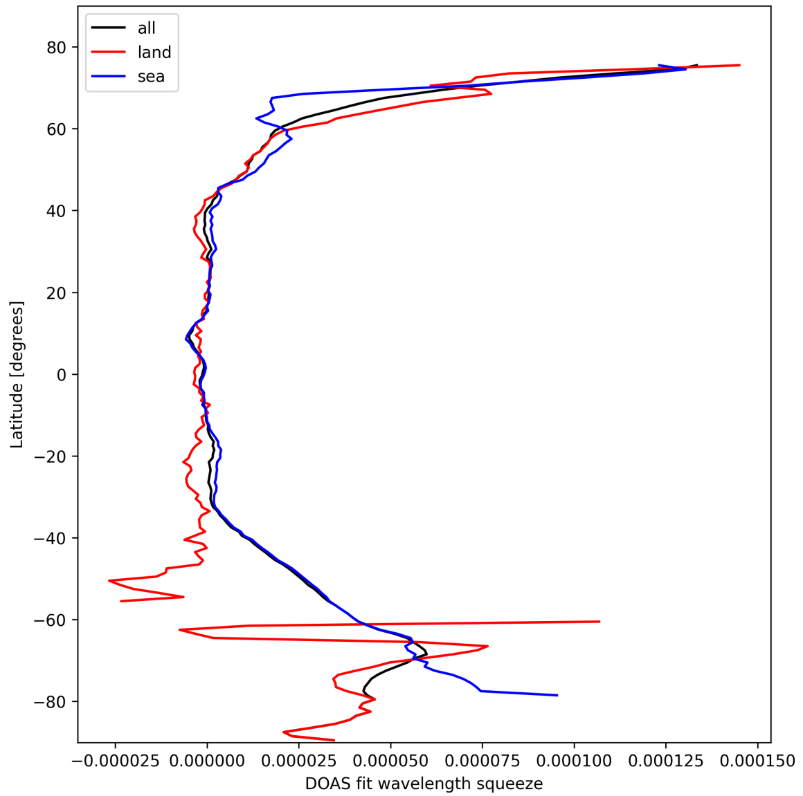
Figure 29: Zonal average of “DOAS fit wavelength squeeze” for 2025-10-18 to 2025-10-19.
