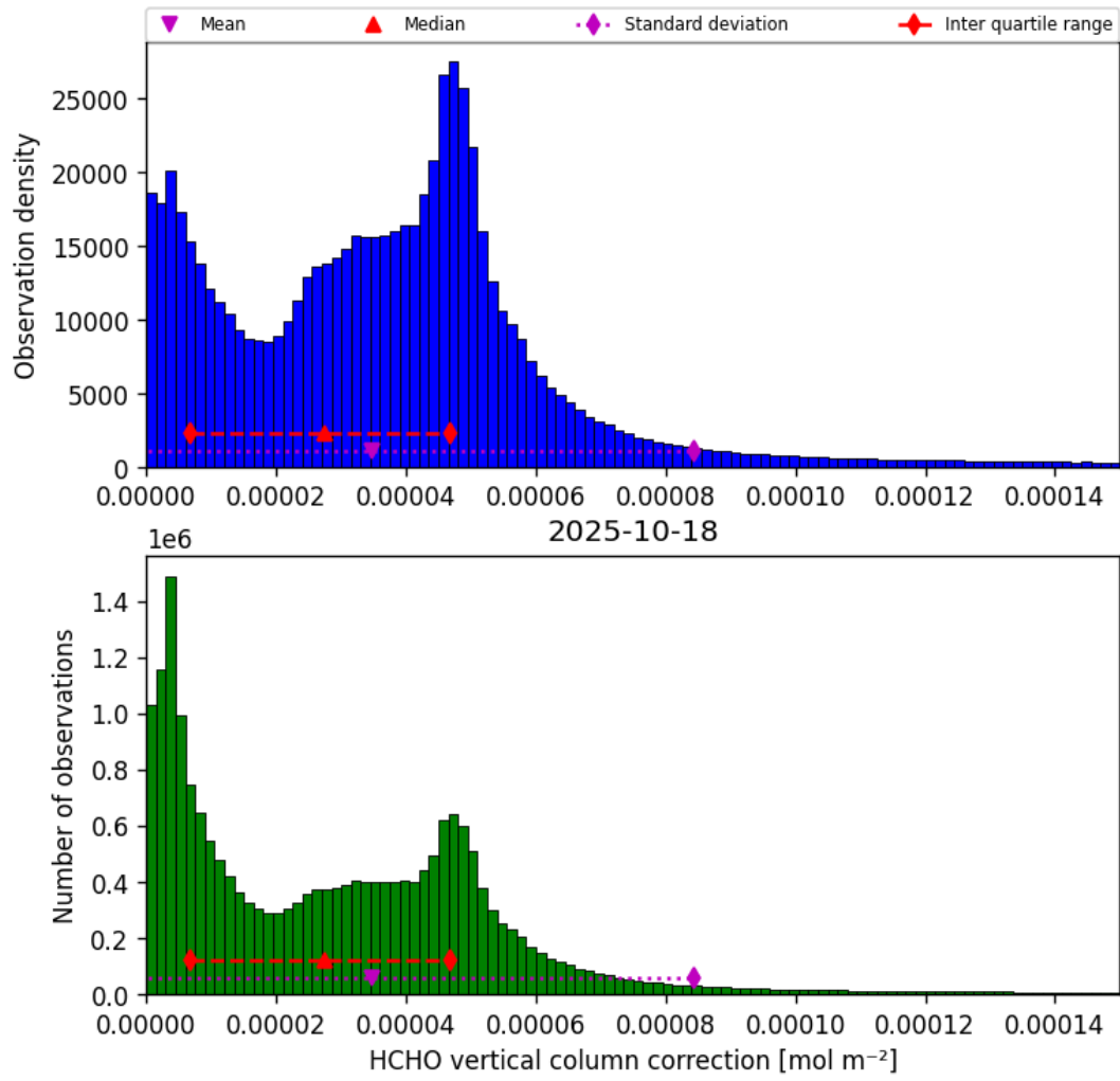
Figure 35: Histogram of “HCHO vertical column correction” for 2025-10-18 to 2025-10-19
