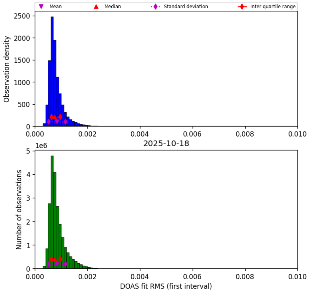
Figure 44: Histogram of “DOAS fit RMS (first interval)” for 2025-10-18 to 2025-10-19
