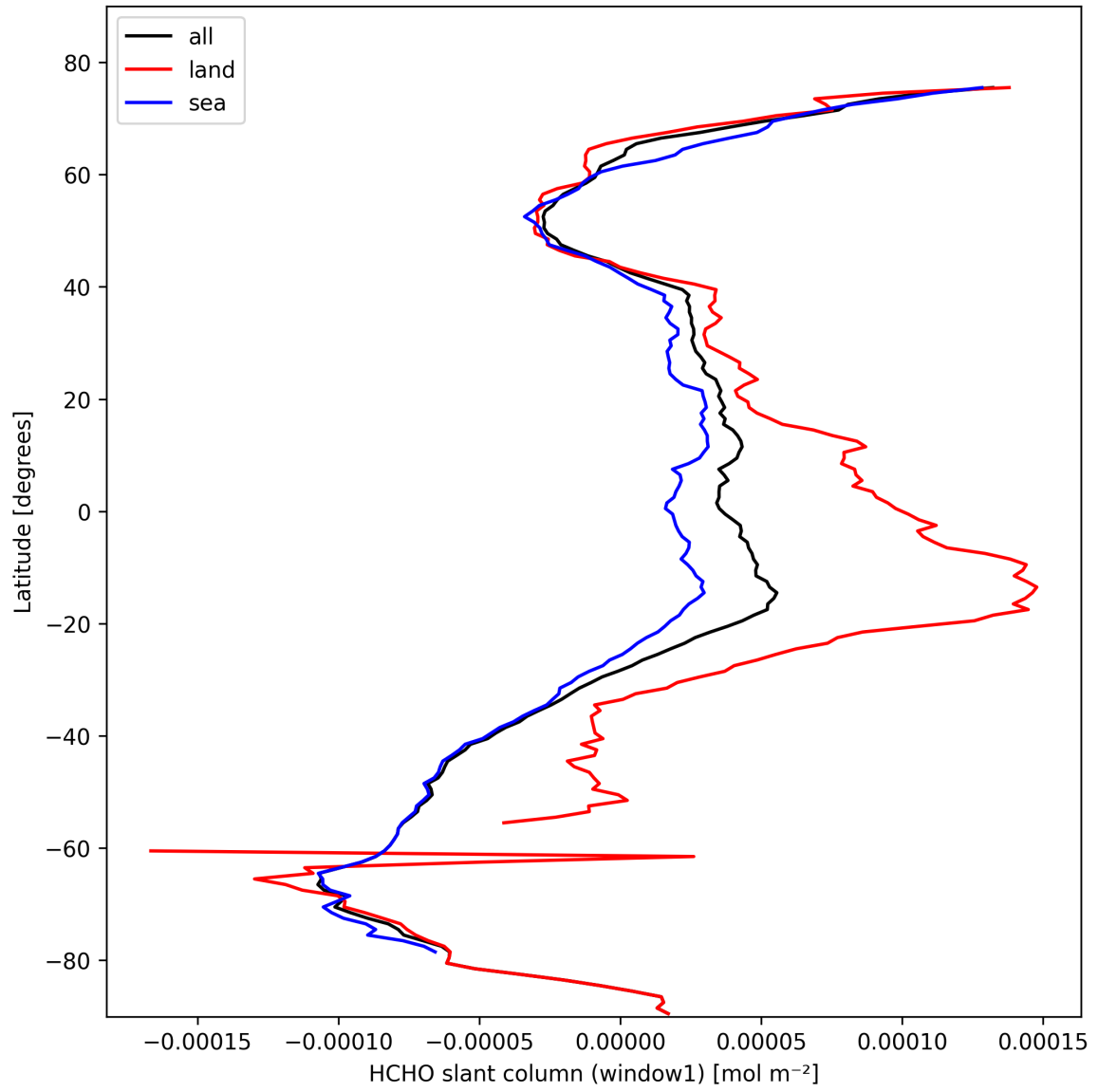
Figure 22: Zonal average of “HCHO slant column (window1)” for 2025-10-18 to 2025-10-19.
