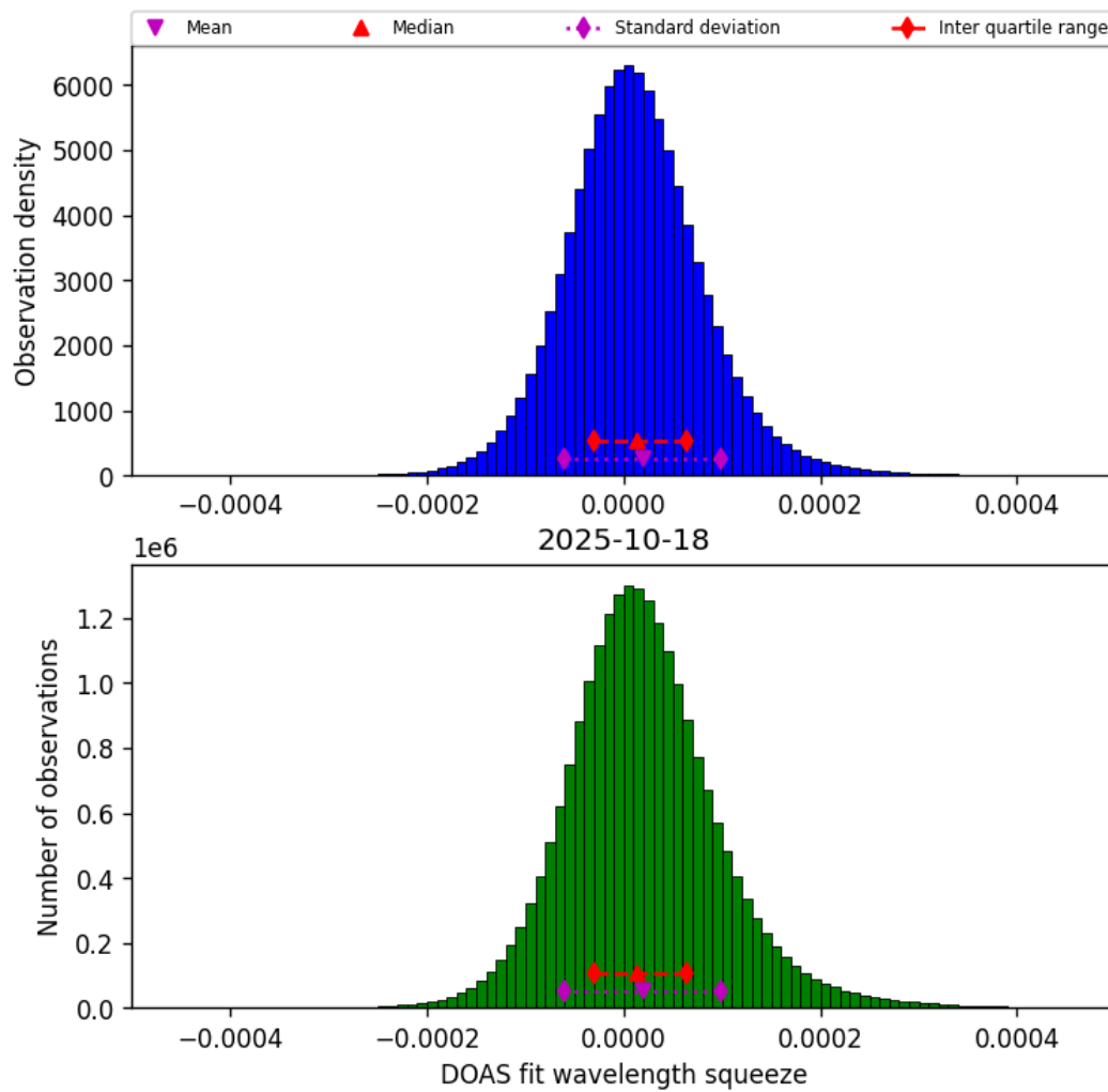
Figure 43: Histogram of "DOAS fit wavelength squeeze" for 2025-10-18 to 2025-10-19
