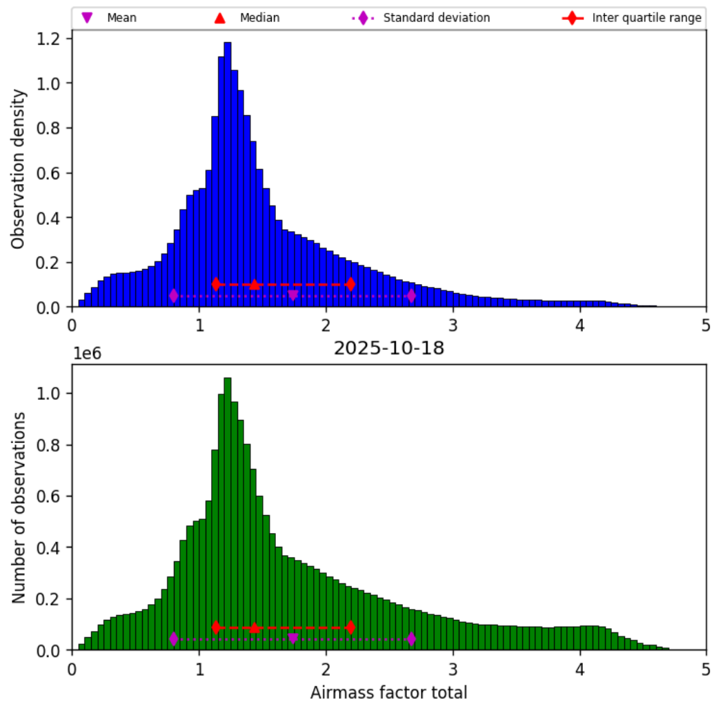
Figure 38: Histogram of “Airmass factor total” for 2025-10-18 to 2025-10-19
