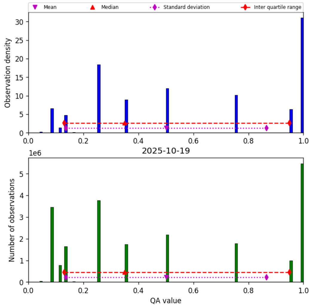
Figure 32: Histogram of “QA value” for 2025-10-19 to 2025-10-20
