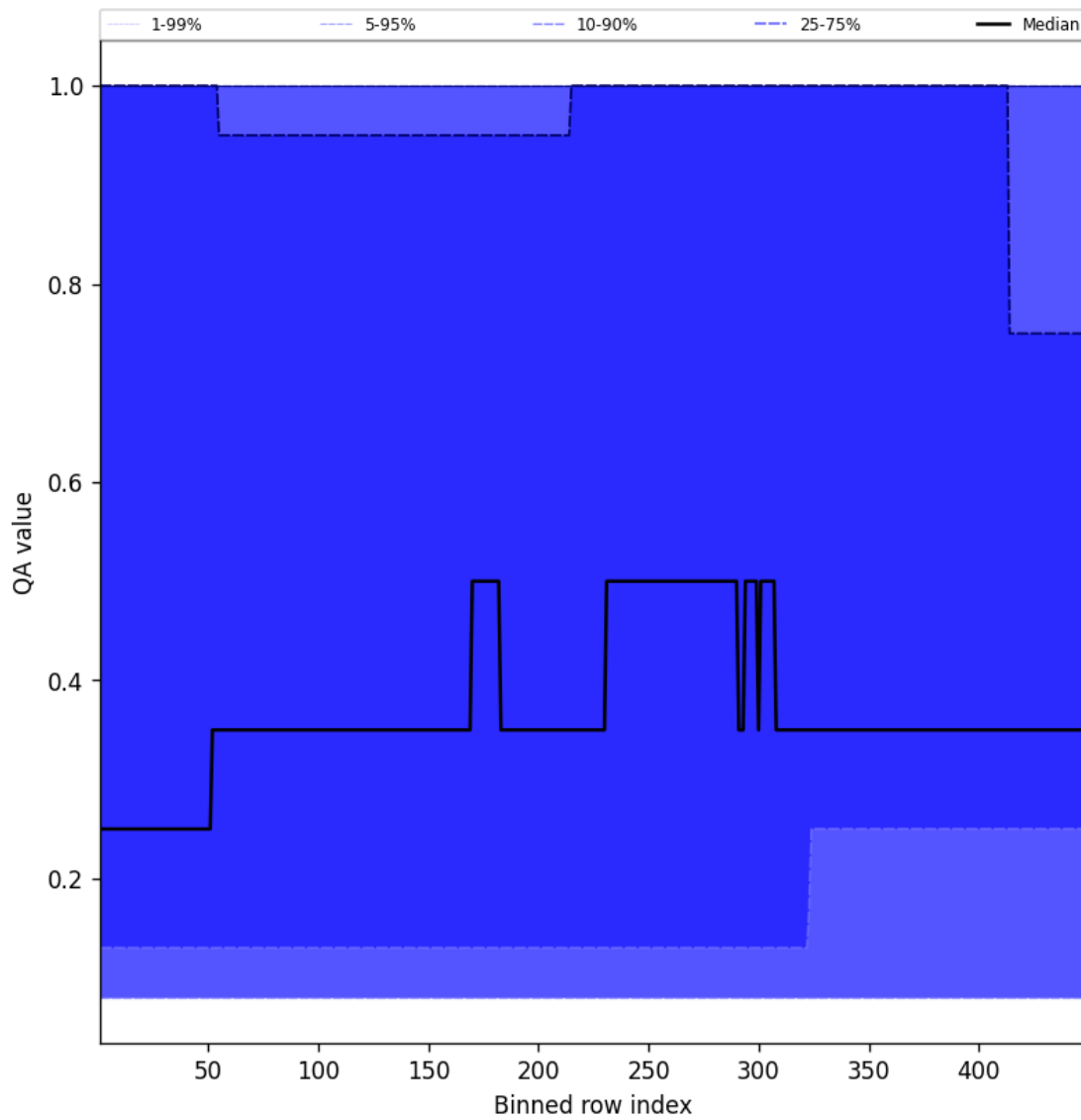
Figure 46: Along track statistics of “QA value” for 2025-10-19 to 2025-10-20
