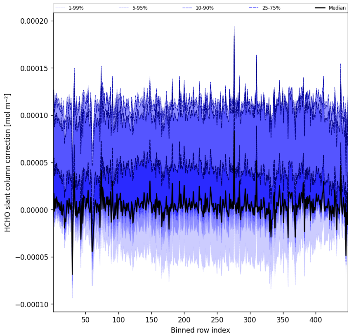
Figure 59: Along track statistics of “HCHO slant column correction” for 2025-10-19 to 2025-10-20
