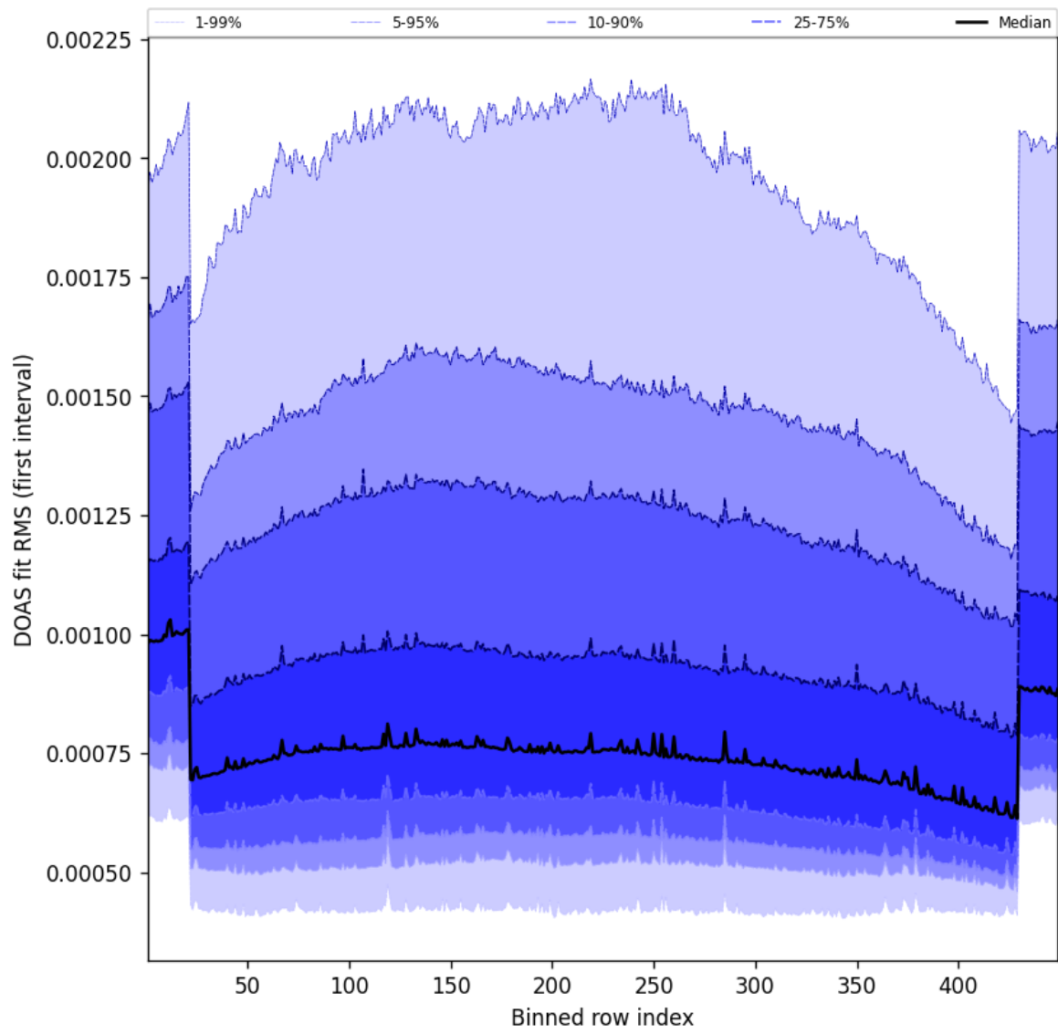
Figure 58: Along track statistics of “DOAS fit RMS (first interval)” for 2025-10-19 to 2025-10-20
