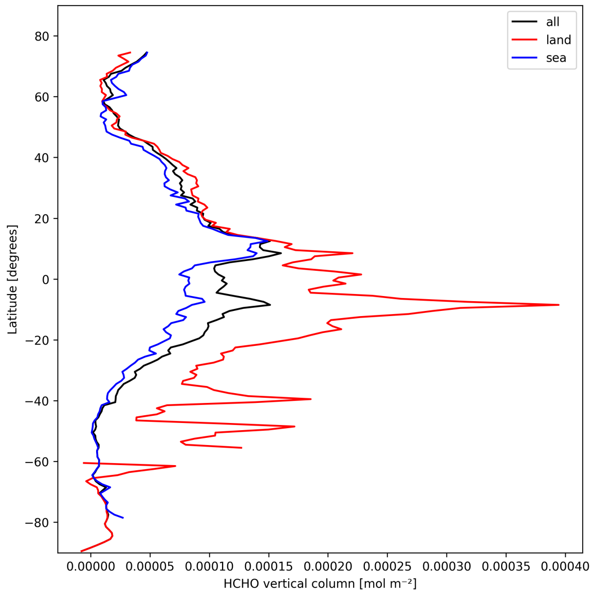
Figure 19: Zonal average of “HCHO vertical column” for 2025-10-19 to 2025-10-20.
