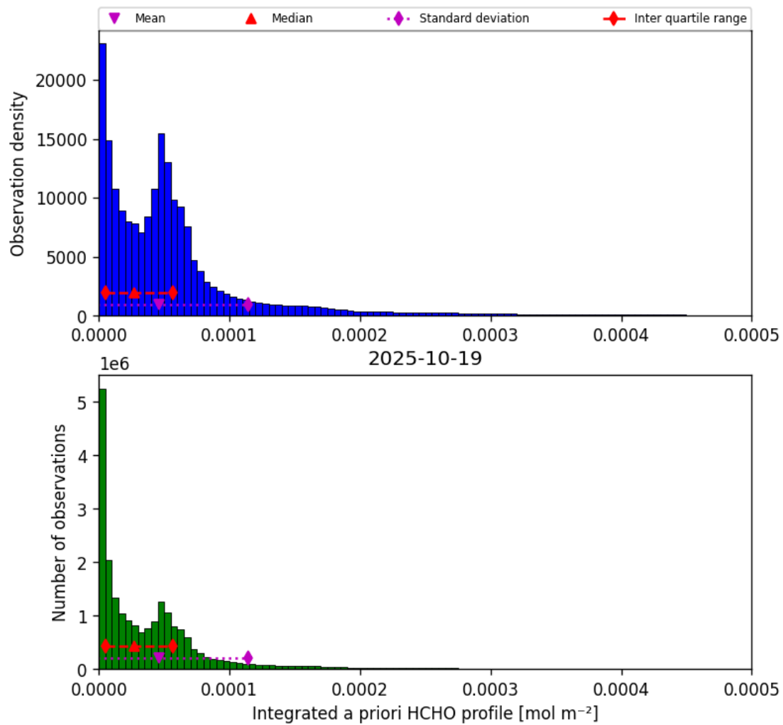
Figure 41: Histogram of “Integrated a priori HCHO profile” for 2025-10-19 to 2025-10-20
