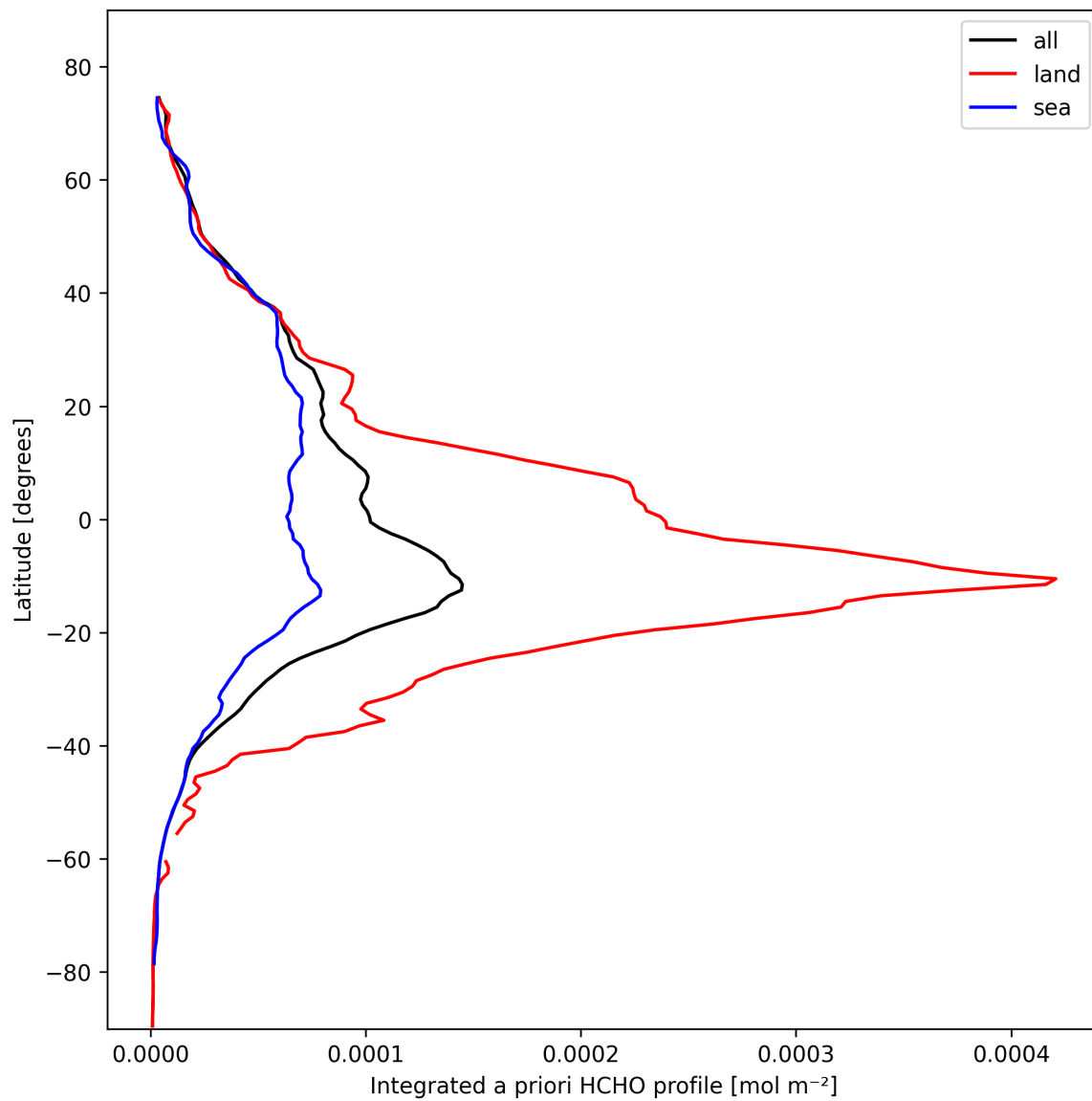
Figure 27: Zonal average of “Integrated a priori HCHO profile” for 2025-10-19 to 2025-10-20.
