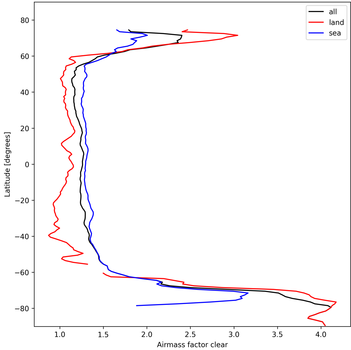
Figure 26: Zonal average of “Airmass factor clear” for 2025-10-19 to 2025-10-20.
