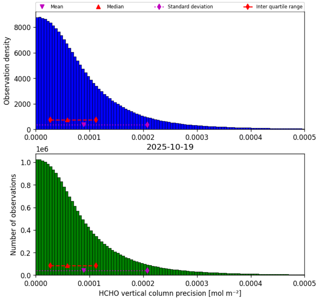
Figure 34: Histogram of “HCHO vertical column precision” for 2025-10-19 to 2025-10-20
