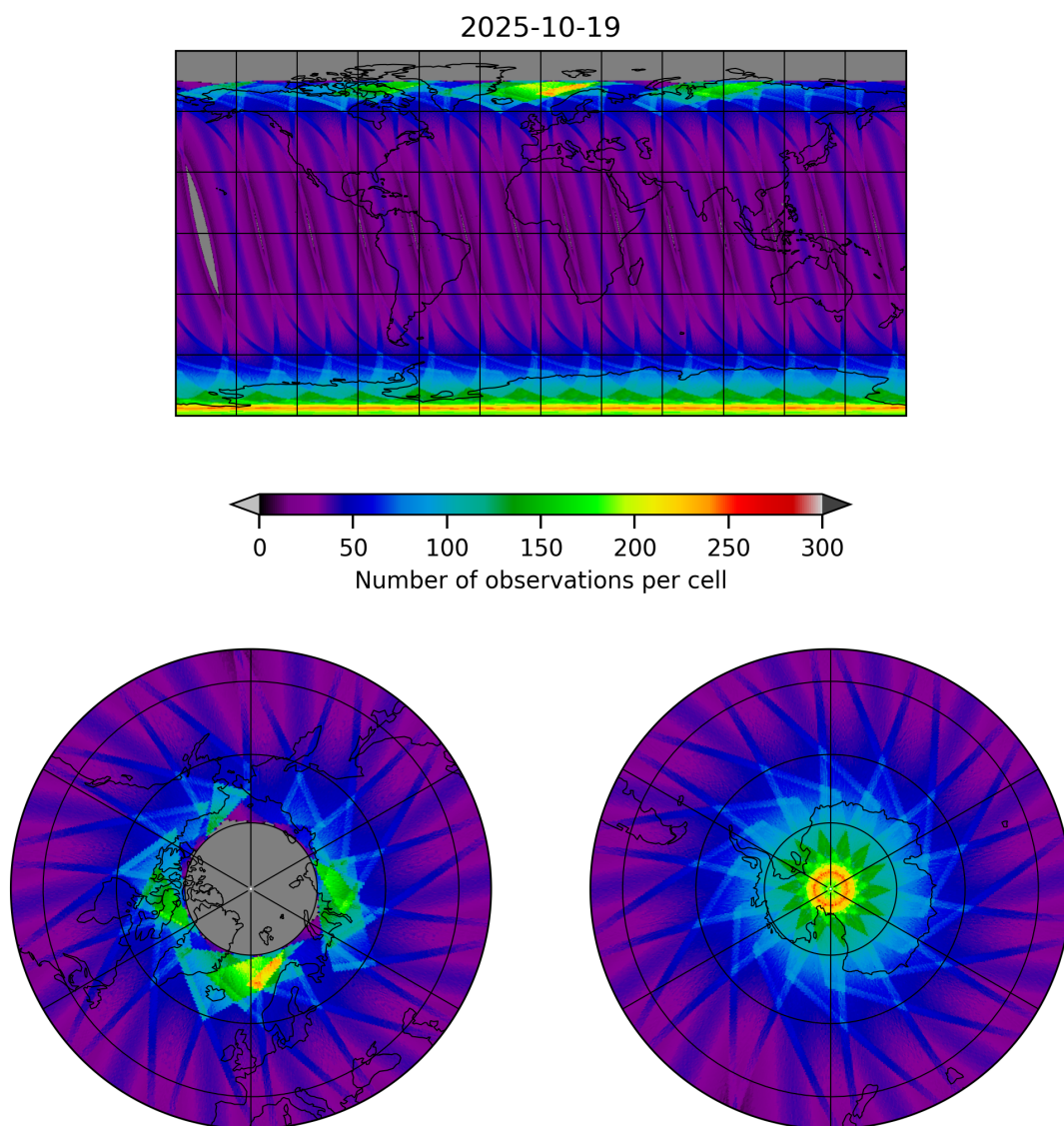
Figure 17: Map of the number of observations for 2025-10-19 to 2025-10-20
