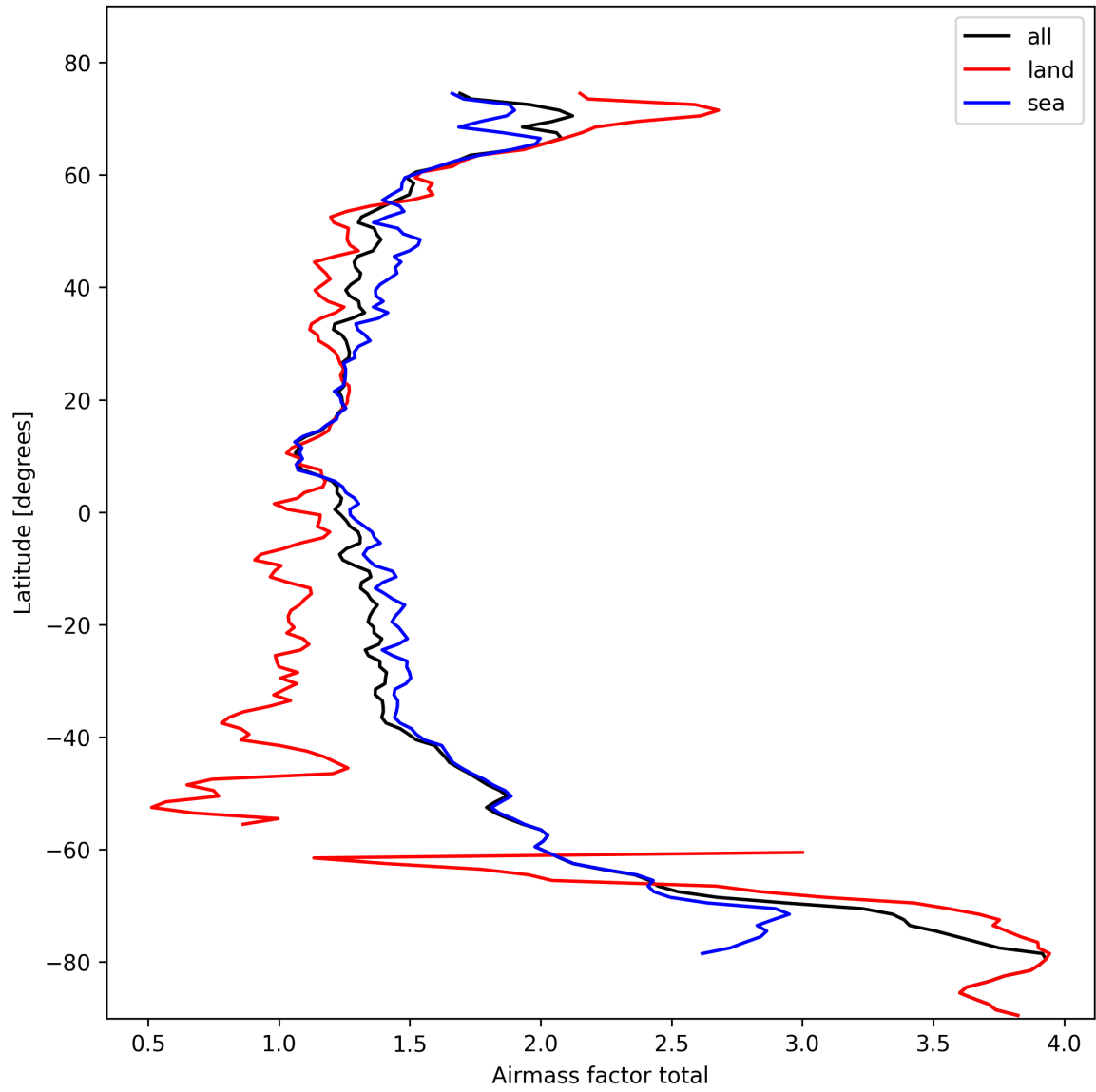
Figure 24: Zonal average of “Airmass factor total” for 2025-10-19 to 2025-10-20.
