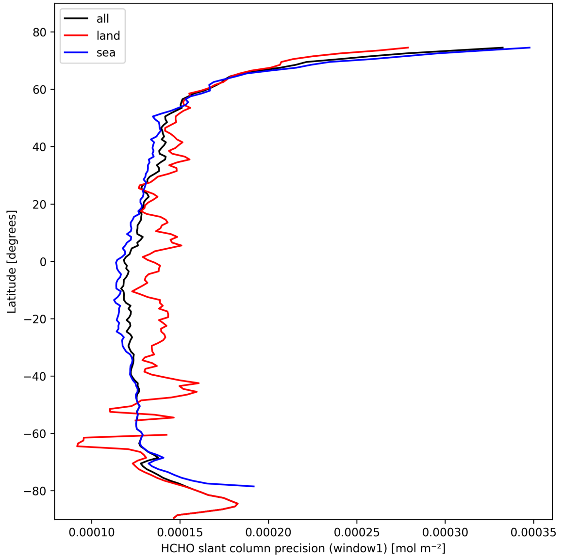
Figure 23: Zonal average of “HCHO slant column precision (window1)” for 2025-10-19 to 2025-10-20.
