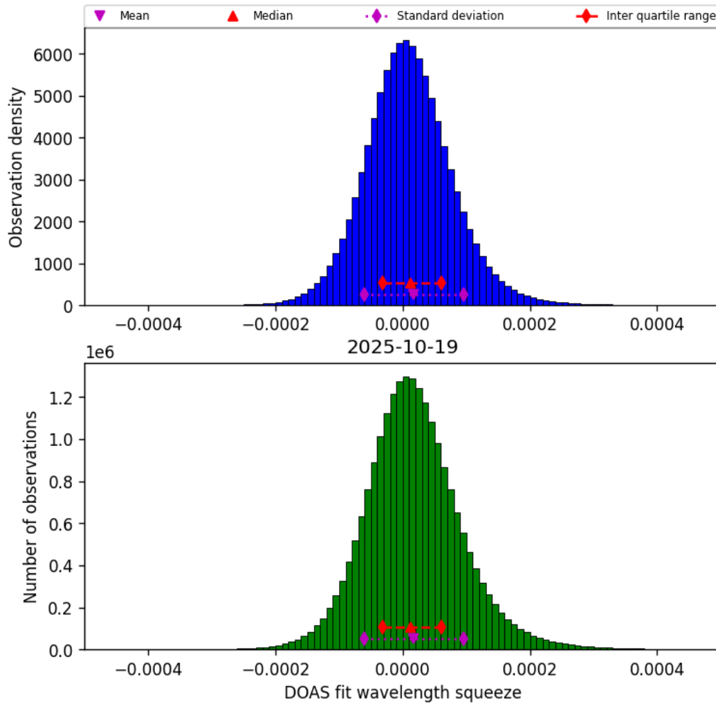
Figure 43: Histogram of “DOAS fit wavelength squeeze” for 2025-10-19 to 2025-10-20
