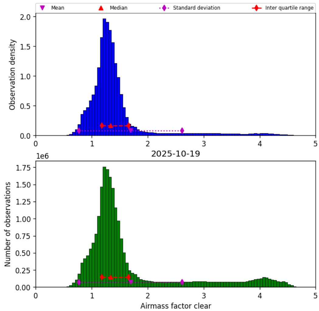
Figure 40: Histogram of “Airmass factor clear” for 2025-10-19 to 2025-10-20
