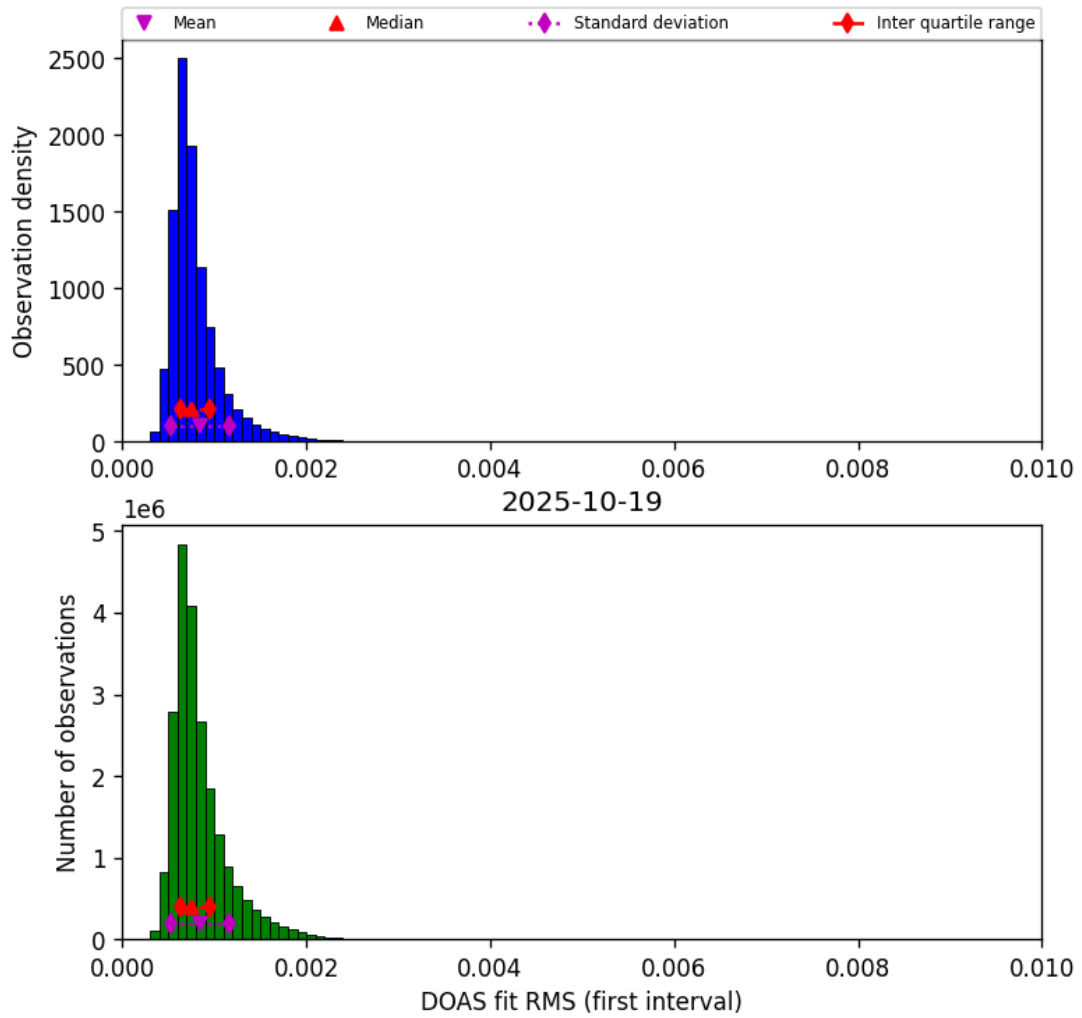
Figure 44: Histogram of “DOAS fit RMS (first interval)” for 2025-10-19 to 2025-10-20
