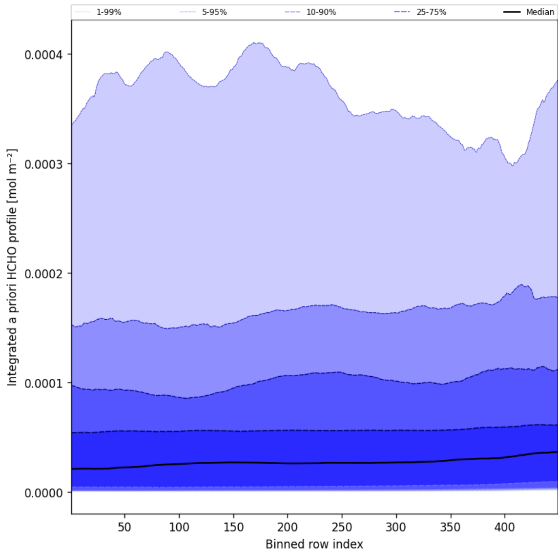
Figure 55: Along track statistics of "Integrated a priori HCHO profile" for 2025-10-19 to 2025-10-20
