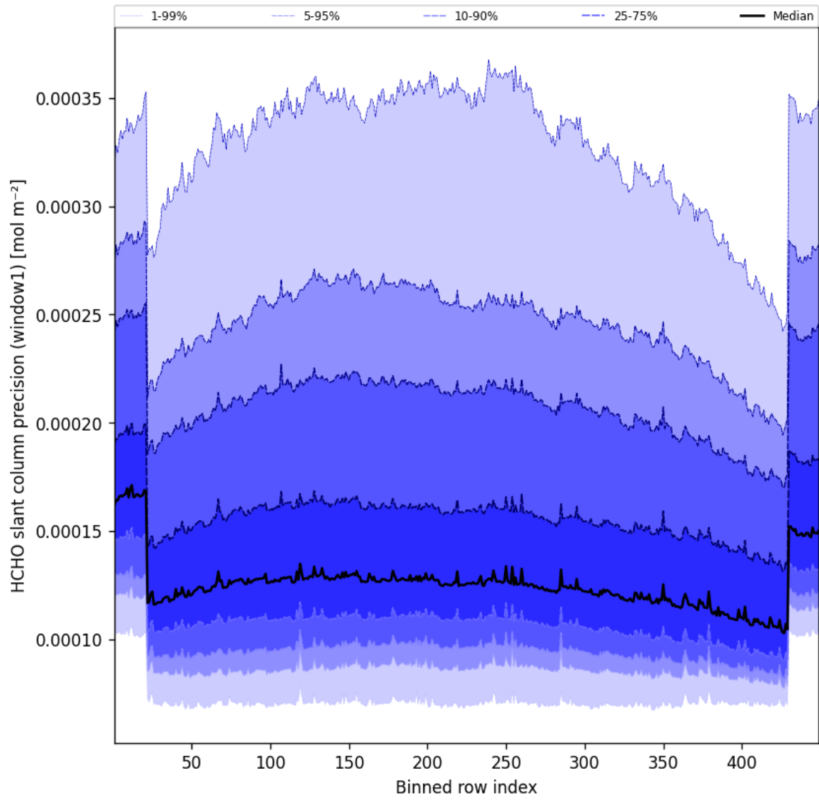
Figure 51: Along track statistics of “HCHO slant column precision (window1)” for 2025-10-19 to 2025-10-20
