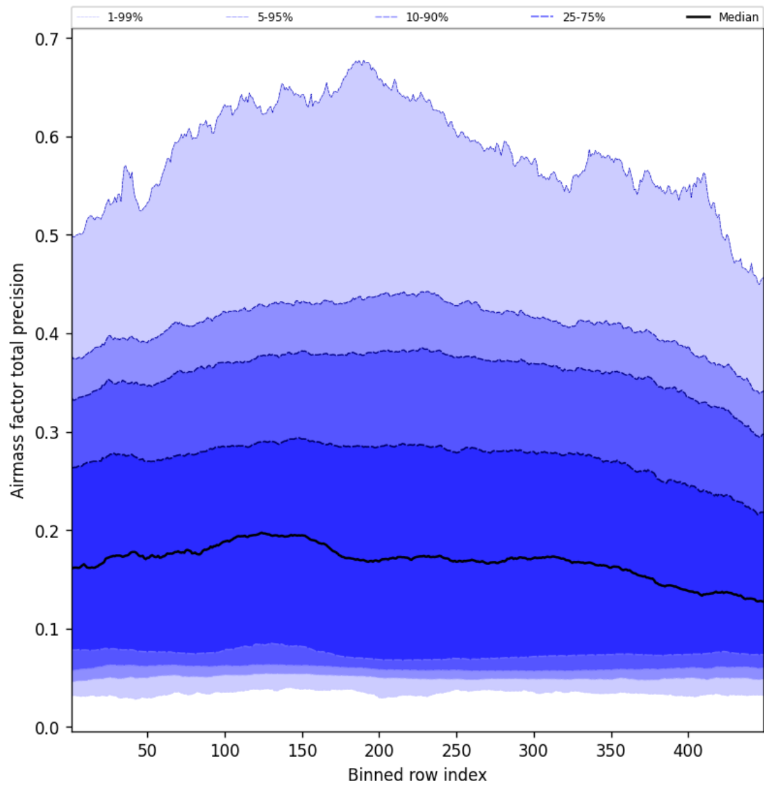
Figure 53: Along track statistics of “Airmass factor total precision” for 2025-10-19 to 2025-10-20
