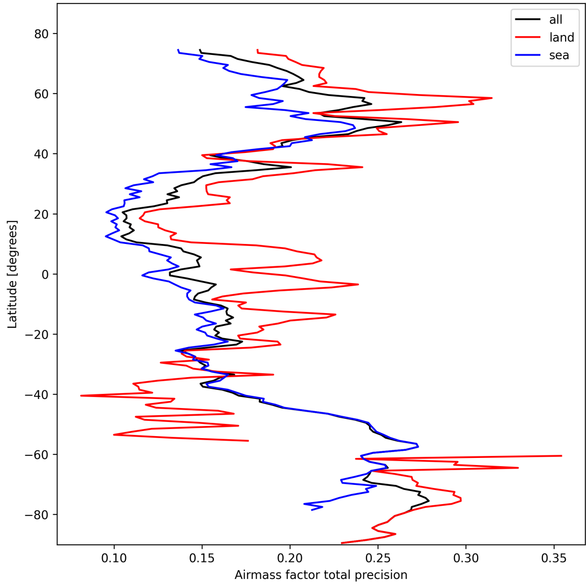
Figure 25: Zonal average of “Airmass factor total precision” for 2025-10-19 to 2025-10-20.
