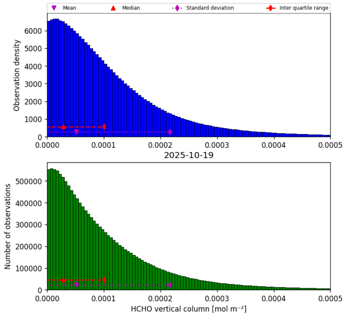
Figure 33: Histogram of “HCHO vertical column” for 2025-10-19 to 2025-10-20
