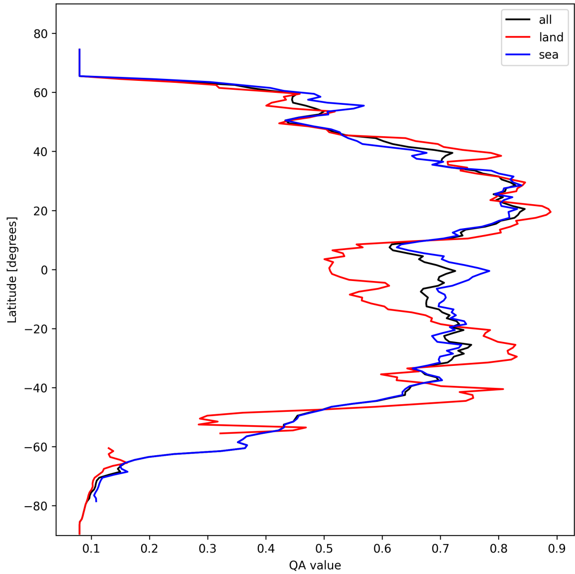
Figure 18: Zonal average of “QA value” for 2025-10-19 to 2025-10-20.
