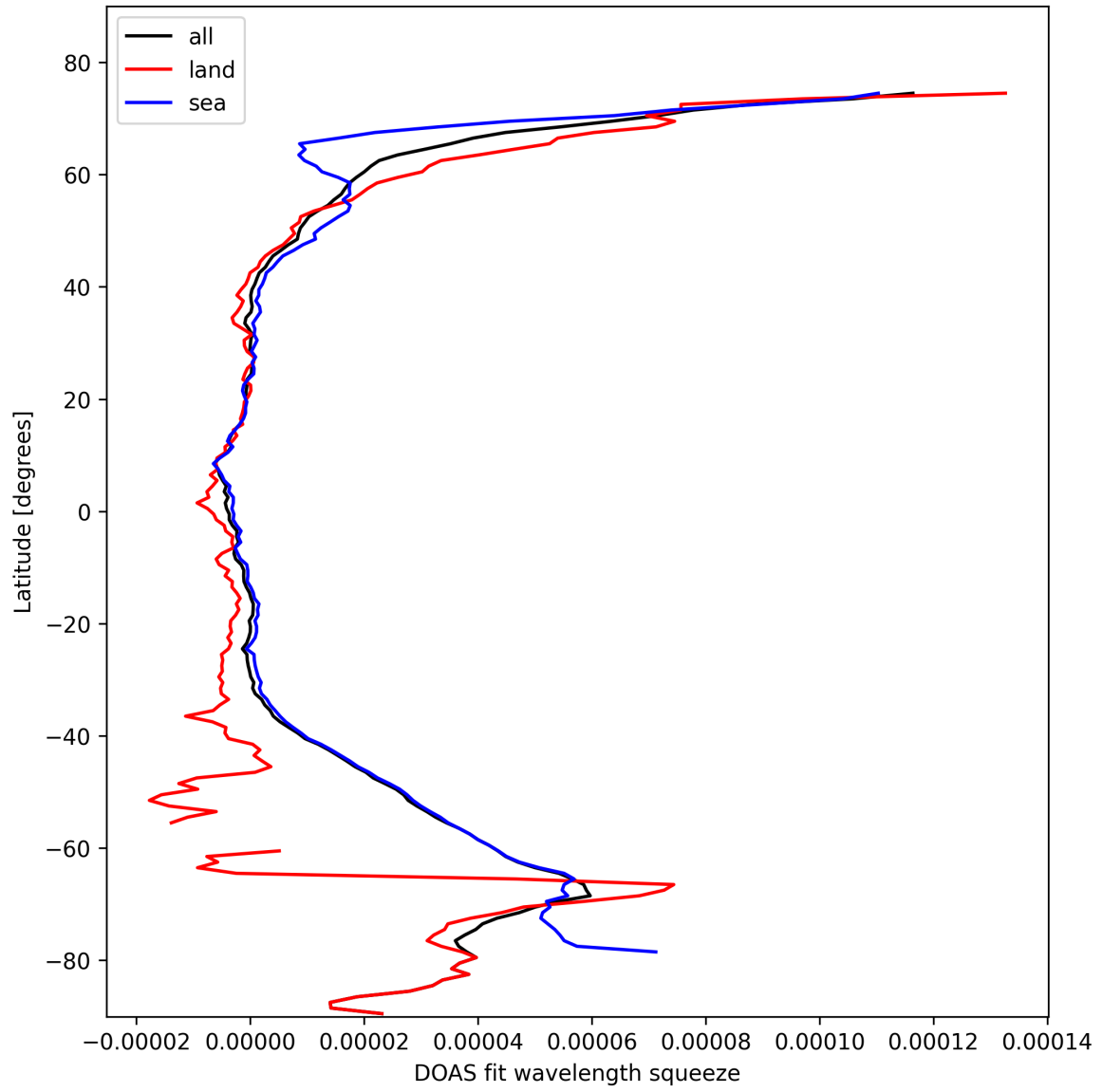
Figure 29: Zonal average of “DOAS fit wavelength squeeze” for 2025-10-19 to 2025-10-20.
