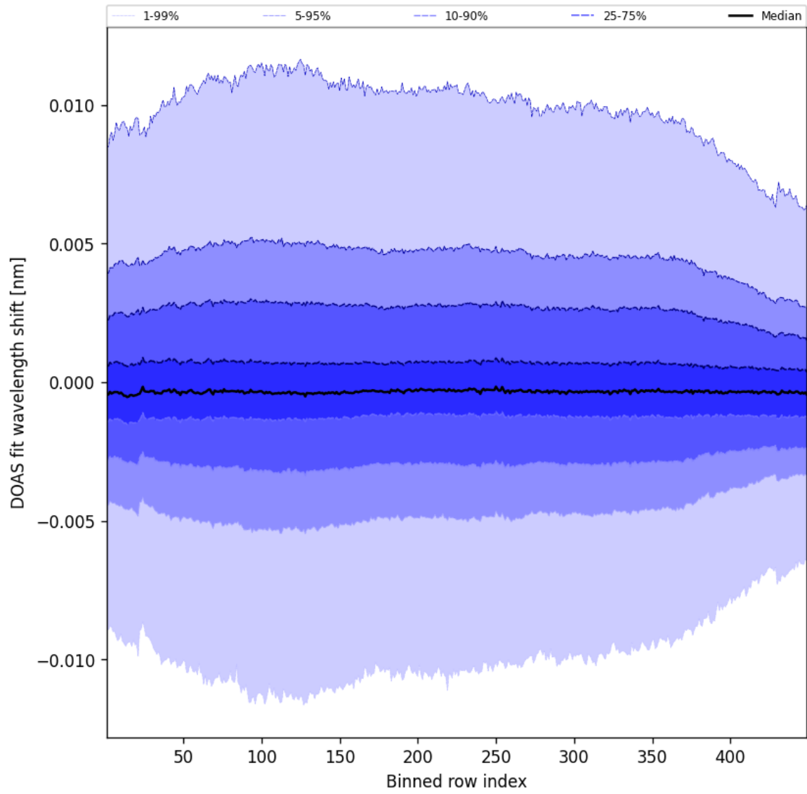
Figure 56: Along track statistics of “DOAS fit wavelength shift” for 2025-10-19 to 2025-10-20
