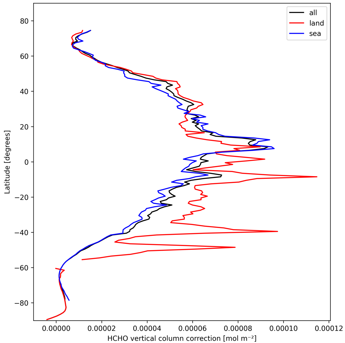
Figure 21: Zonal average of “HCHO vertical column correction” for 2025-10-19 to 2025-10-20.
