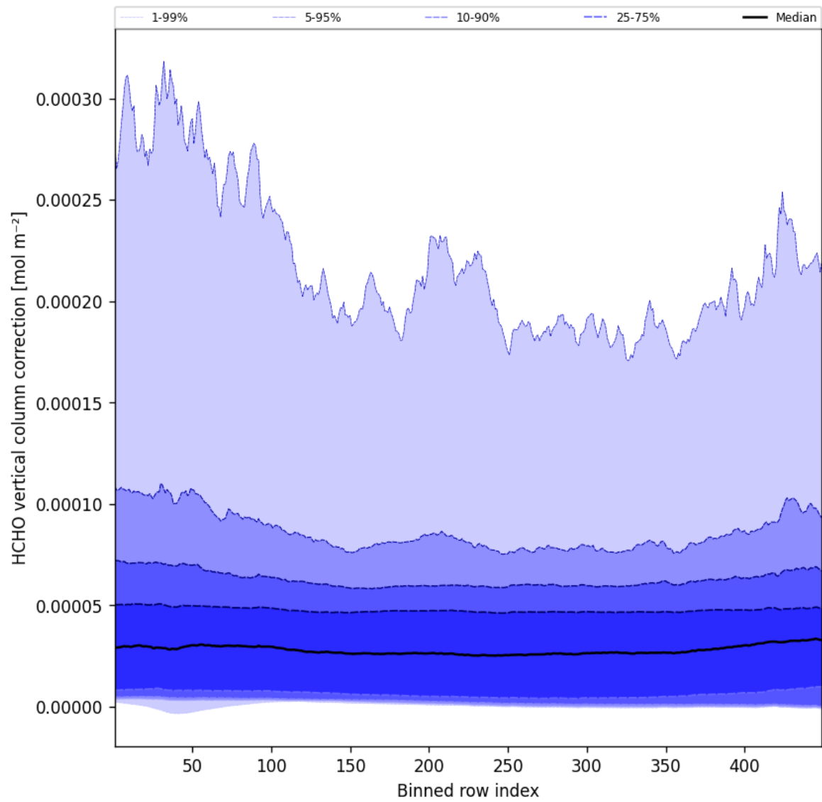
Figure 49: Along track statistics of “HCHO vertical column correction” for 2025-10-19 to 2025-10-20
