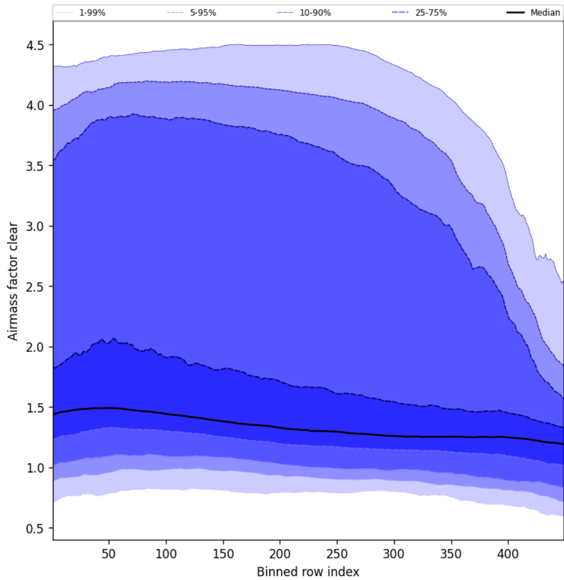
Figure 54: Along track statistics of “Airmass factor clear” for 2025-10-19 to 2025-10-20
