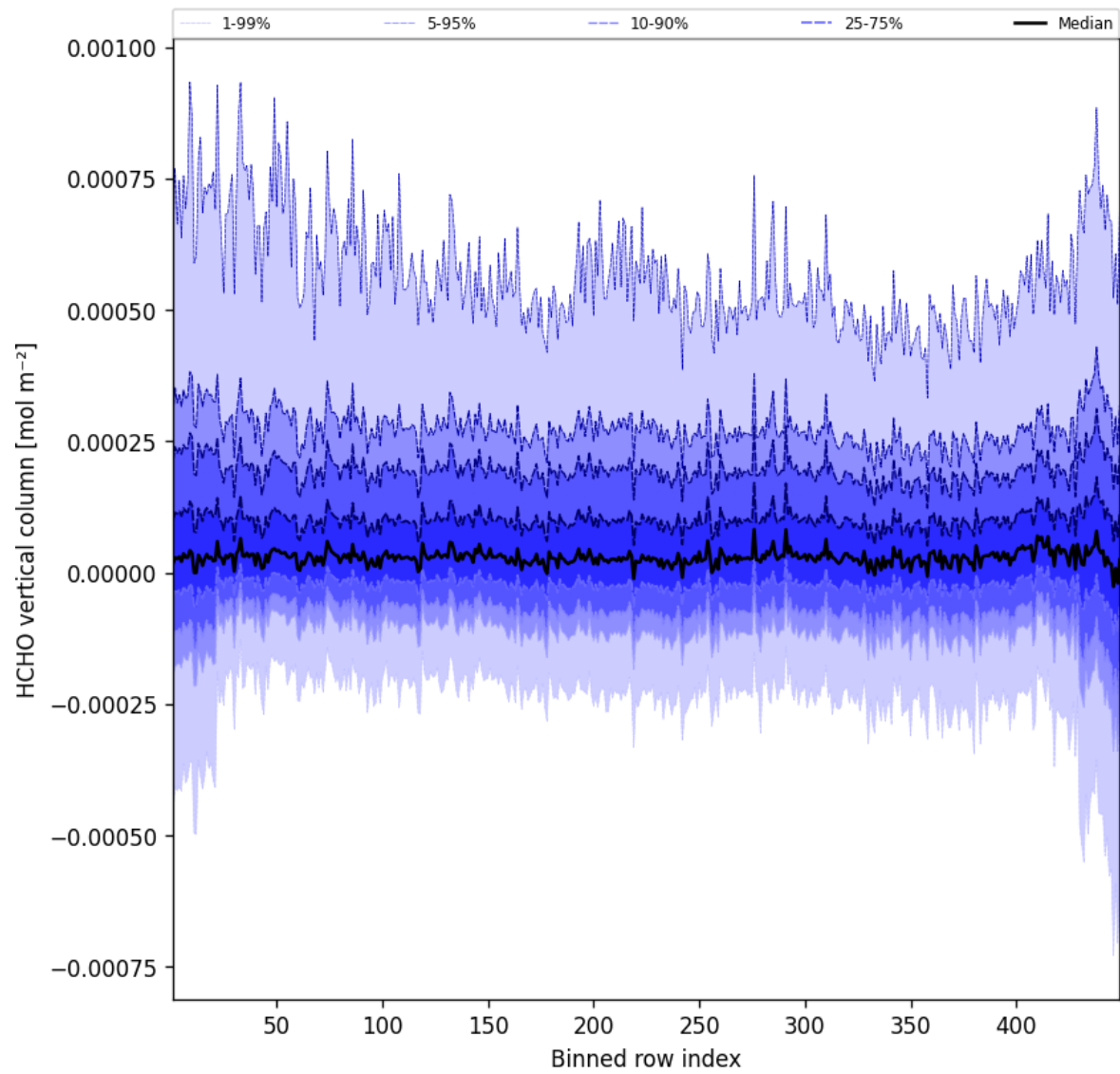
Figure 47: Along track statistics of “HCHO vertical column” for 2025-10-19 to 2025-10-20
