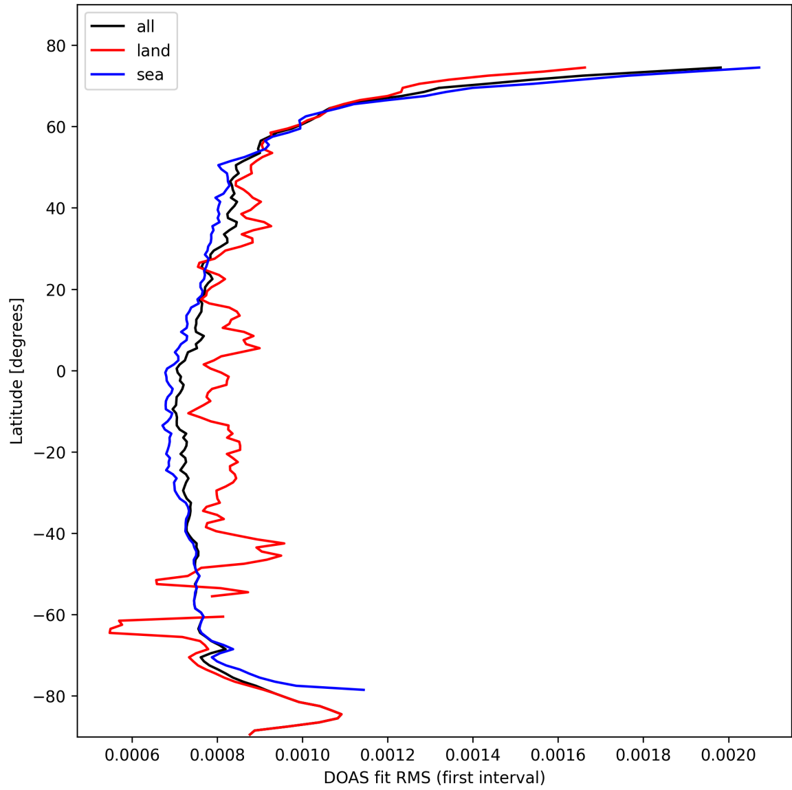
Figure 30: Zonal average of “DOAS fit RMS (first interval)” for 2025-10-19 to 2025-10-20.
