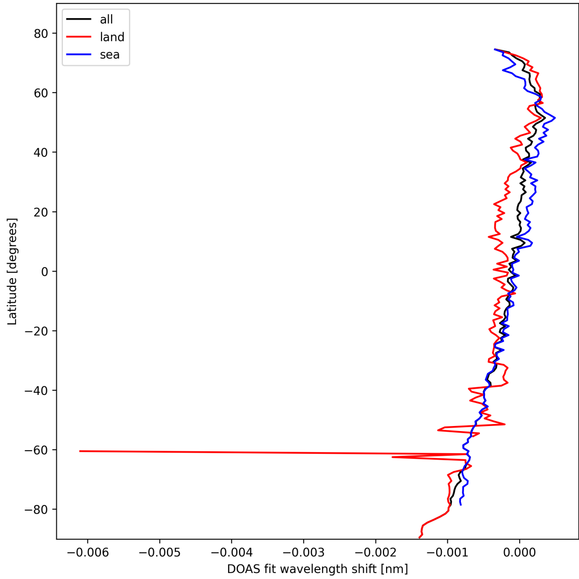
Figure 28: Zonal average of “DOAS fit wavelength shift” for 2025-10-19 to 2025-10-20.
