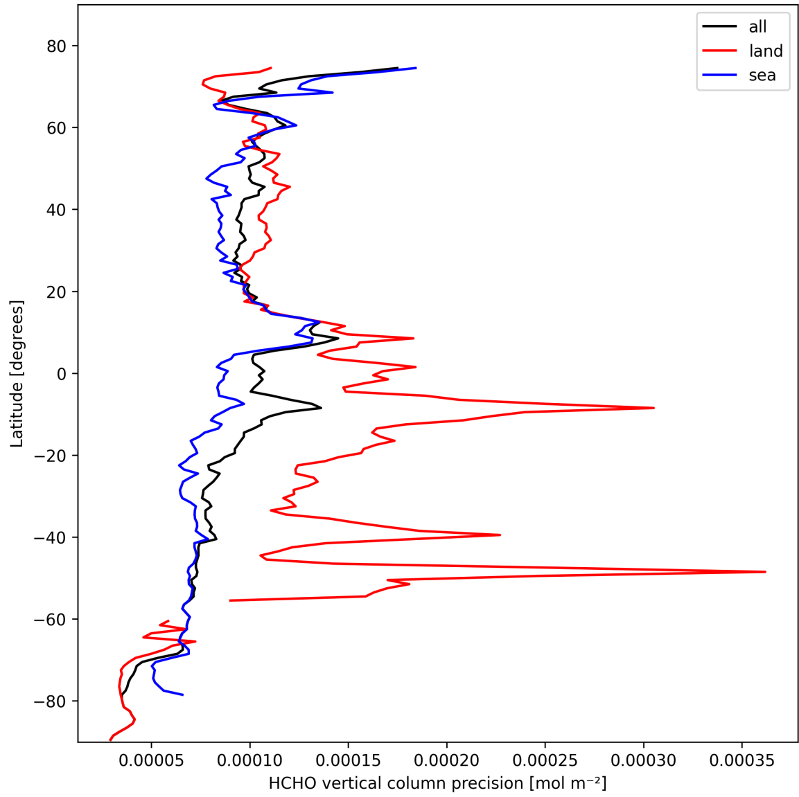
Figure 20: Zonal average of “HCHO vertical column precision” for 2025-10-19 to 2025-10-20.
