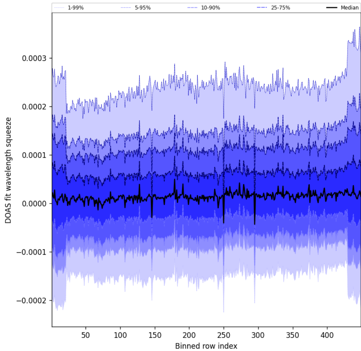
Figure 57: Along track statistics of “DOAS fit wavelength squeeze” for 2025-10-19 to 2025-10-20
