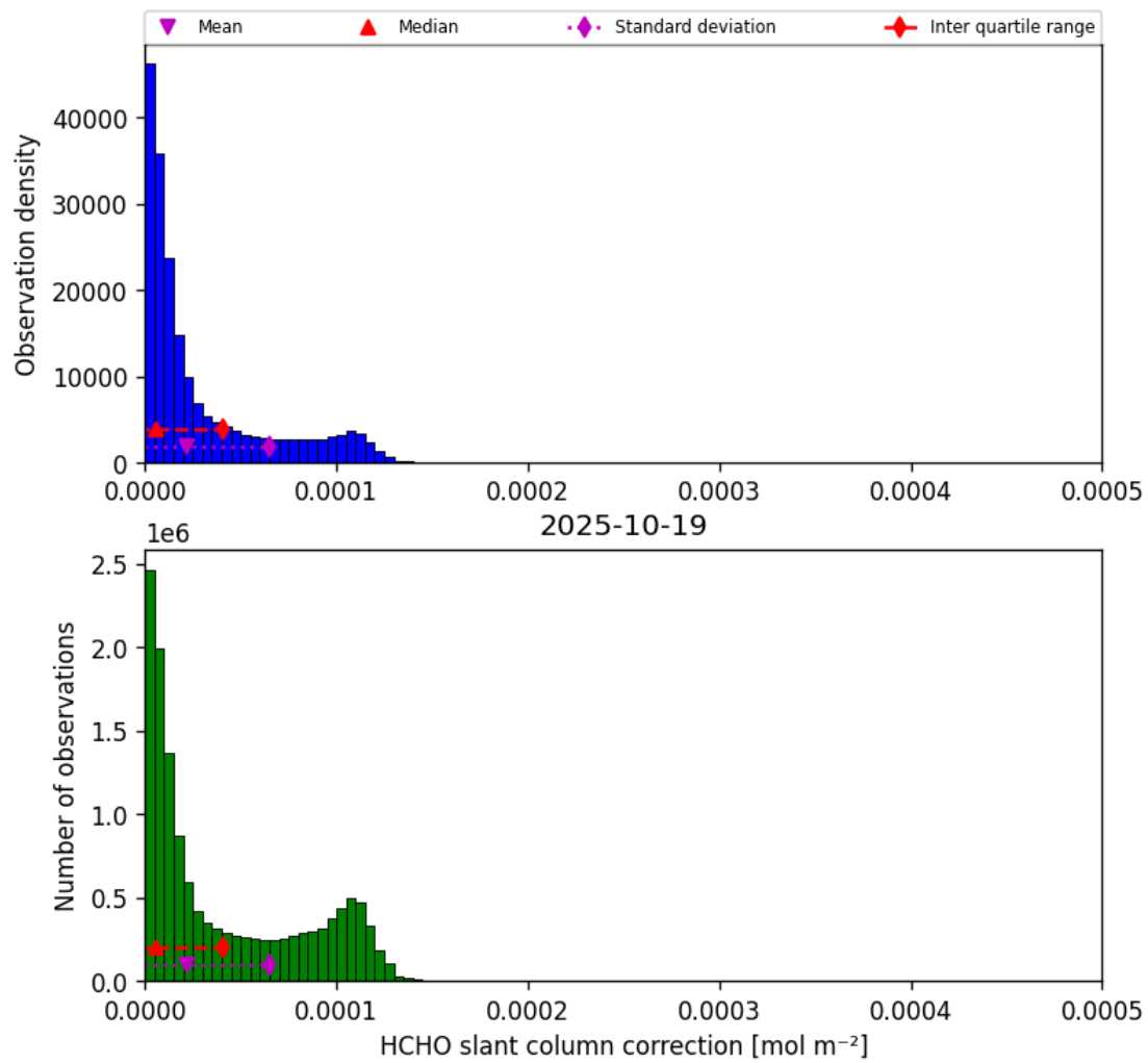
Figure 45: Histogram of “HCHO slant column correction” for 2025-10-19 to 2025-10-20
