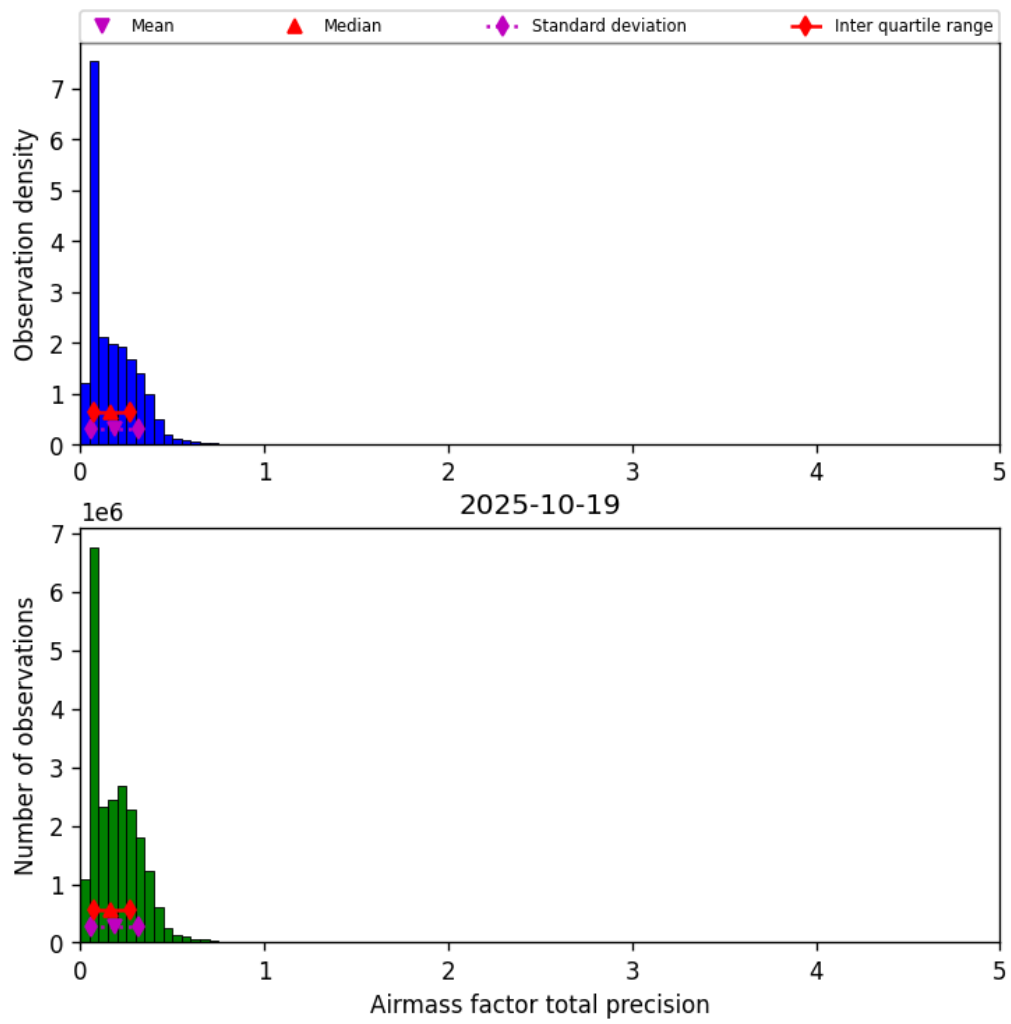
Figure 39: Histogram of “Airmass factor total precision” for 2025-10-19 to 2025-10-20
