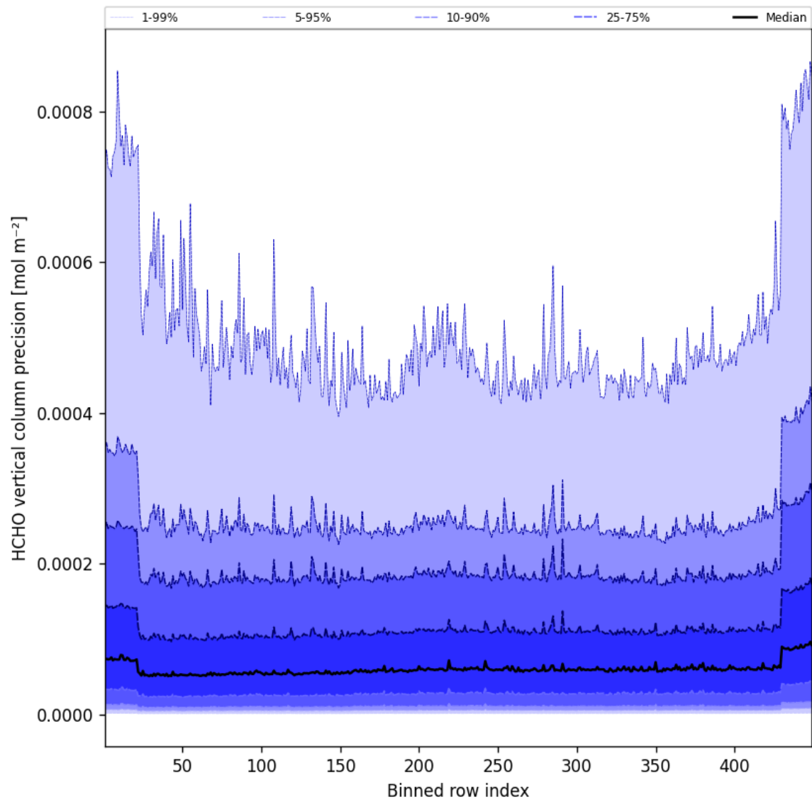
Figure 48: Along track statistics of "HCHO vertical column precision" for 2025-10-19 to 2025-10-20
