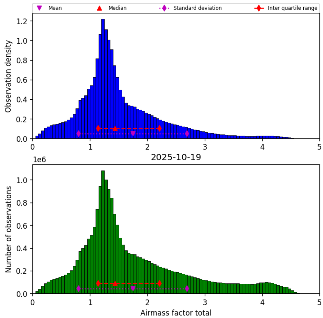
Figure 38: Histogram of “Airmass factor total” for 2025-10-19 to 2025-10-20
