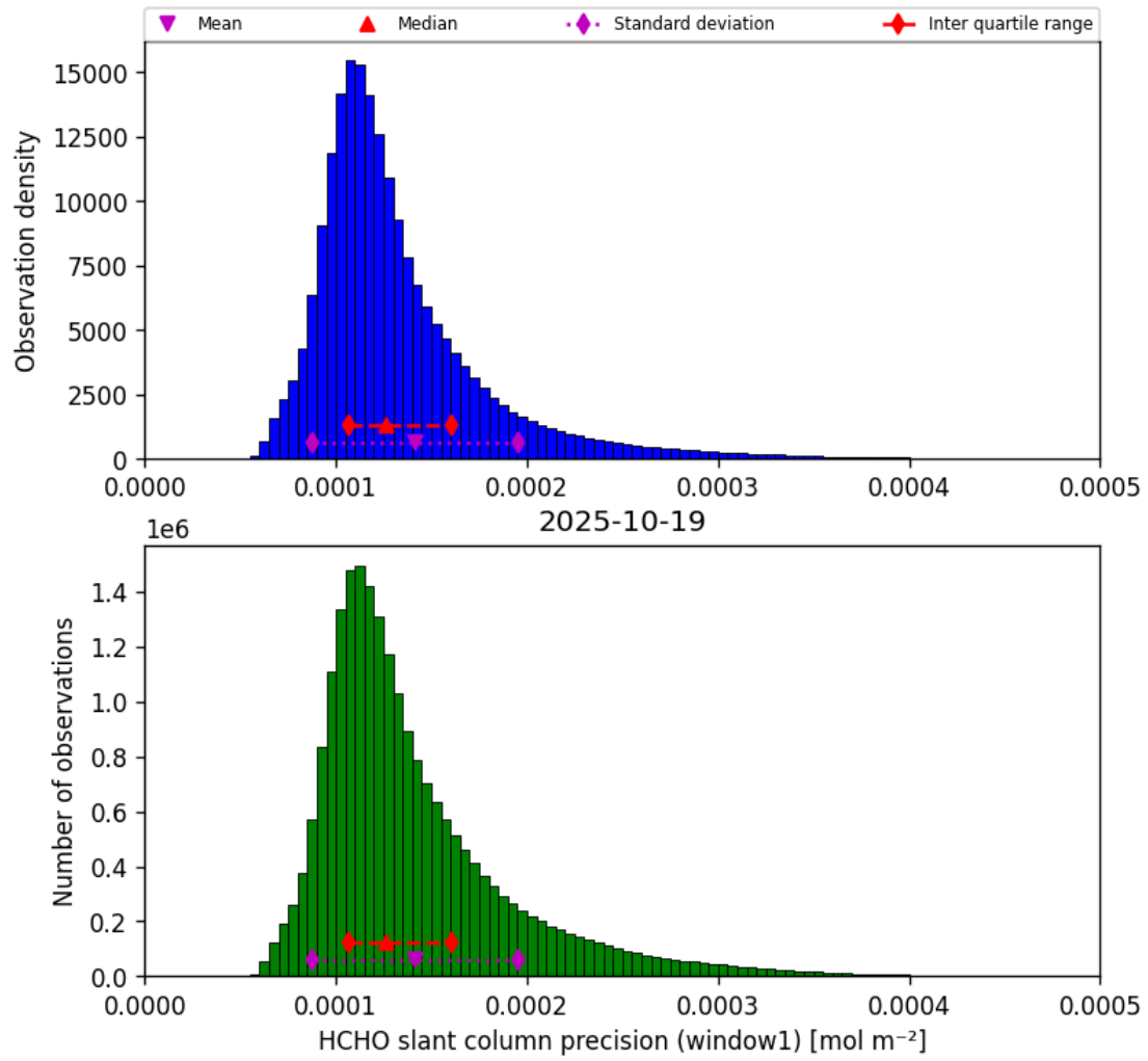
Figure 37: Histogram of “HCHO slant column precision (window1)” for 2025-10-19 to 2025-10-20
