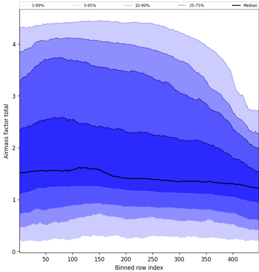
Figure 52: Along track statistics of “Airmass factor total” for 2025-10-19 to 2025-10-20
