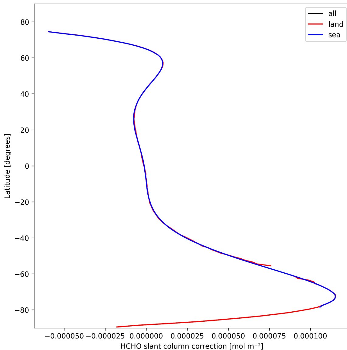
Figure 31: Zonal average of “HCHO slant column correction” for 2025-10-19 to 2025-10-20.
