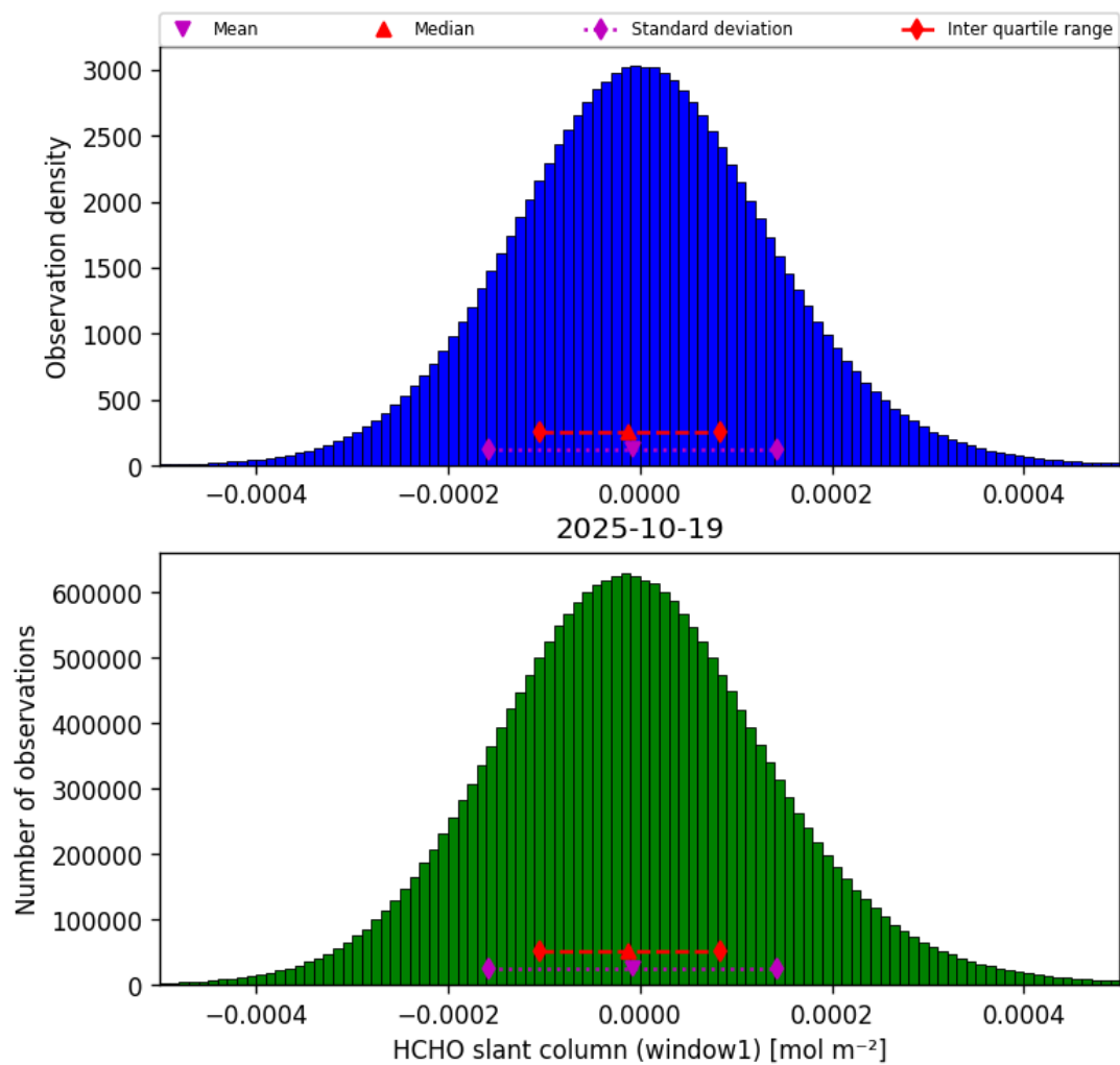
Figure 36: Histogram of “HCHO slant column (window1)” for 2025-10-19 to 2025-10-20
