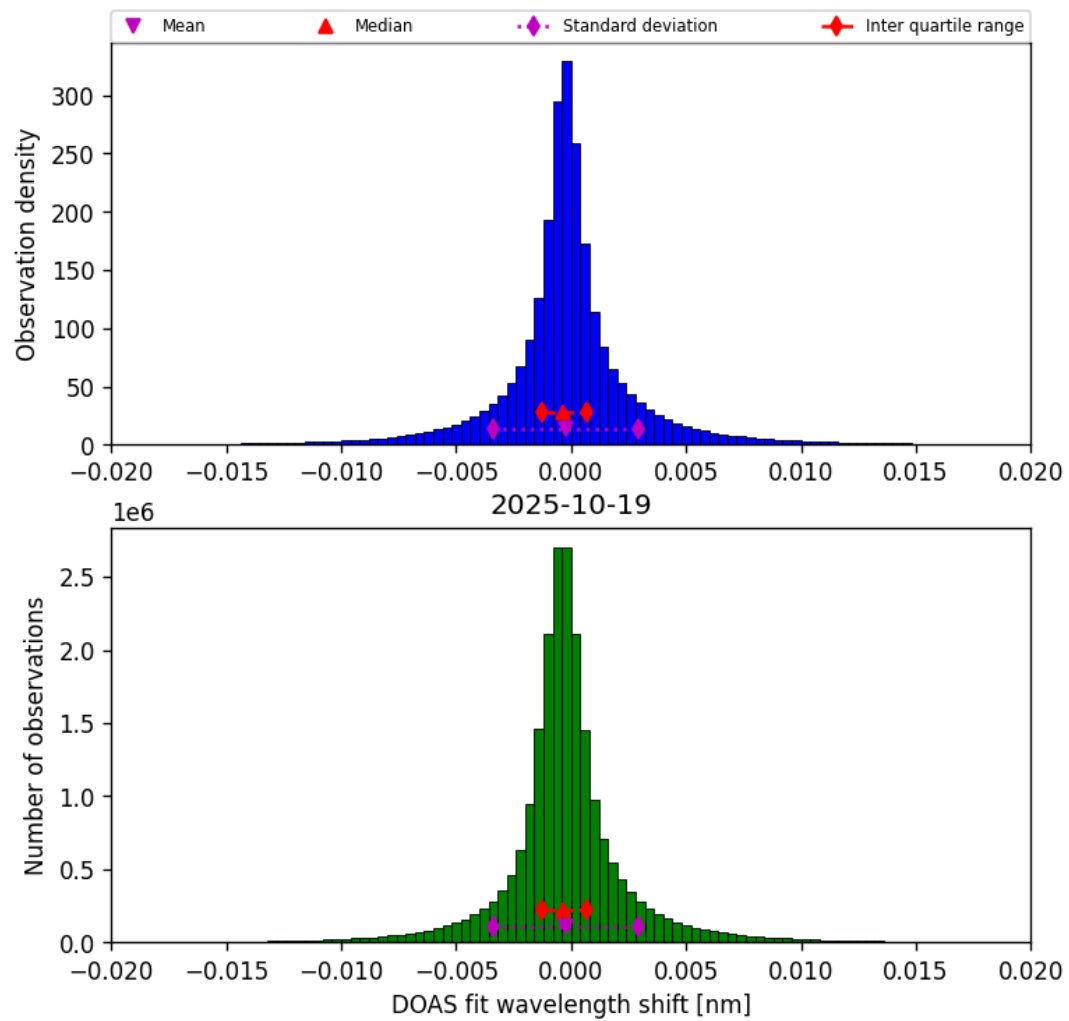
Figure 42: Histogram of “DOAS fit wavelength shift” for 2025-10-19 to 2025-10-20
