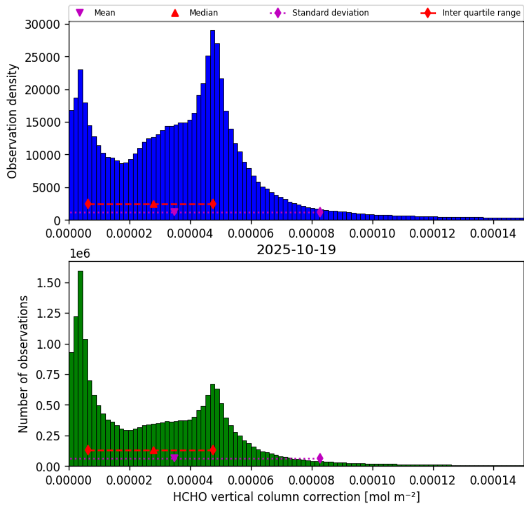
Figure 35: Histogram of “HCHO vertical column correction” for 2025-10-19 to 2025-10-20
