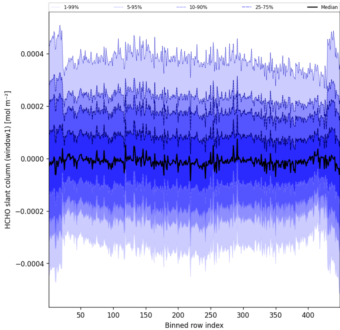
Figure 50: Along track statistics of “HCHO slant column (window1)” for 2025-10-19 to 2025-10-20
