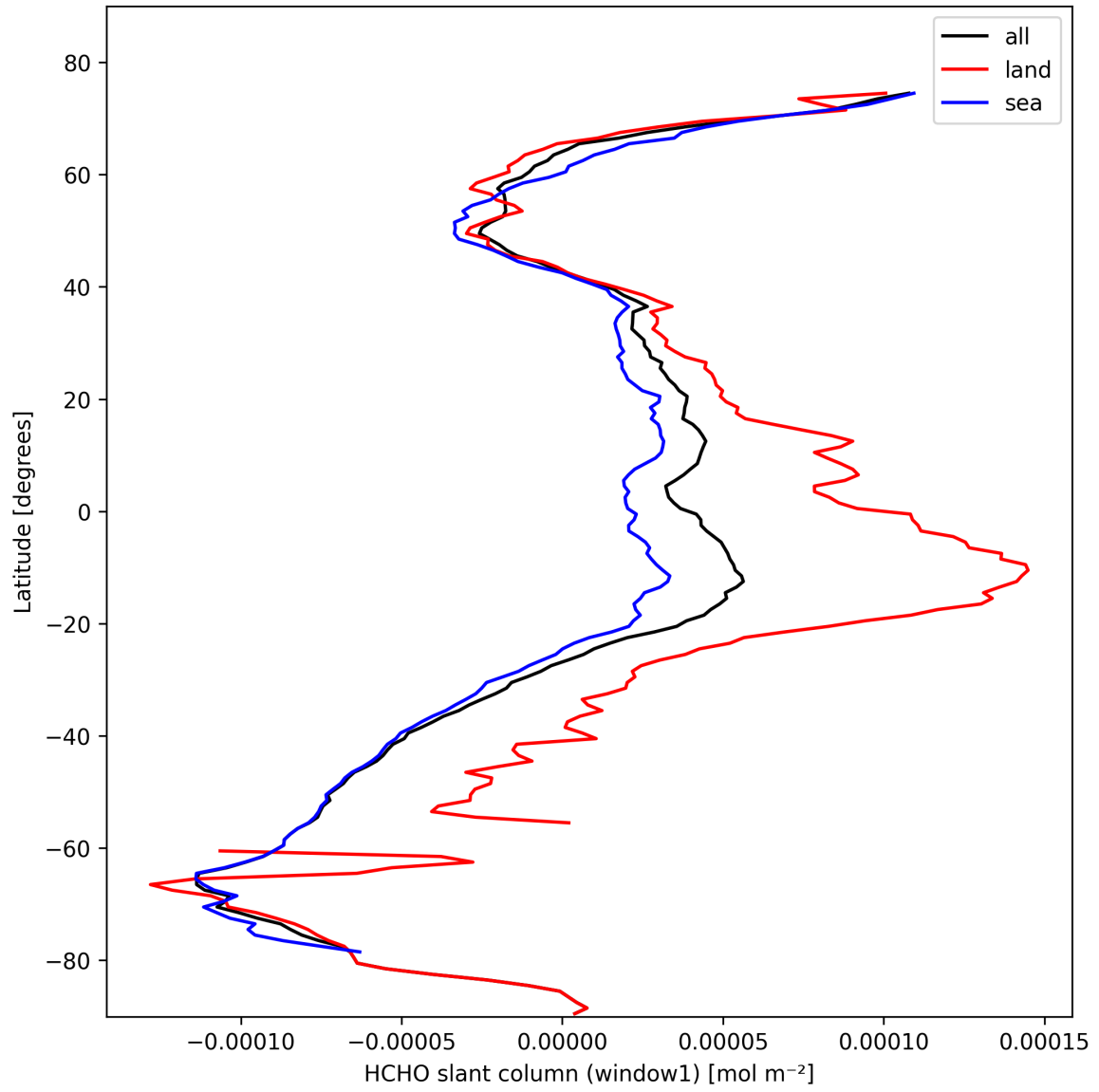
Figure 22: Zonal average of “HCHO slant column (window1)” for 2025-10-19 to 2025-10-20.
