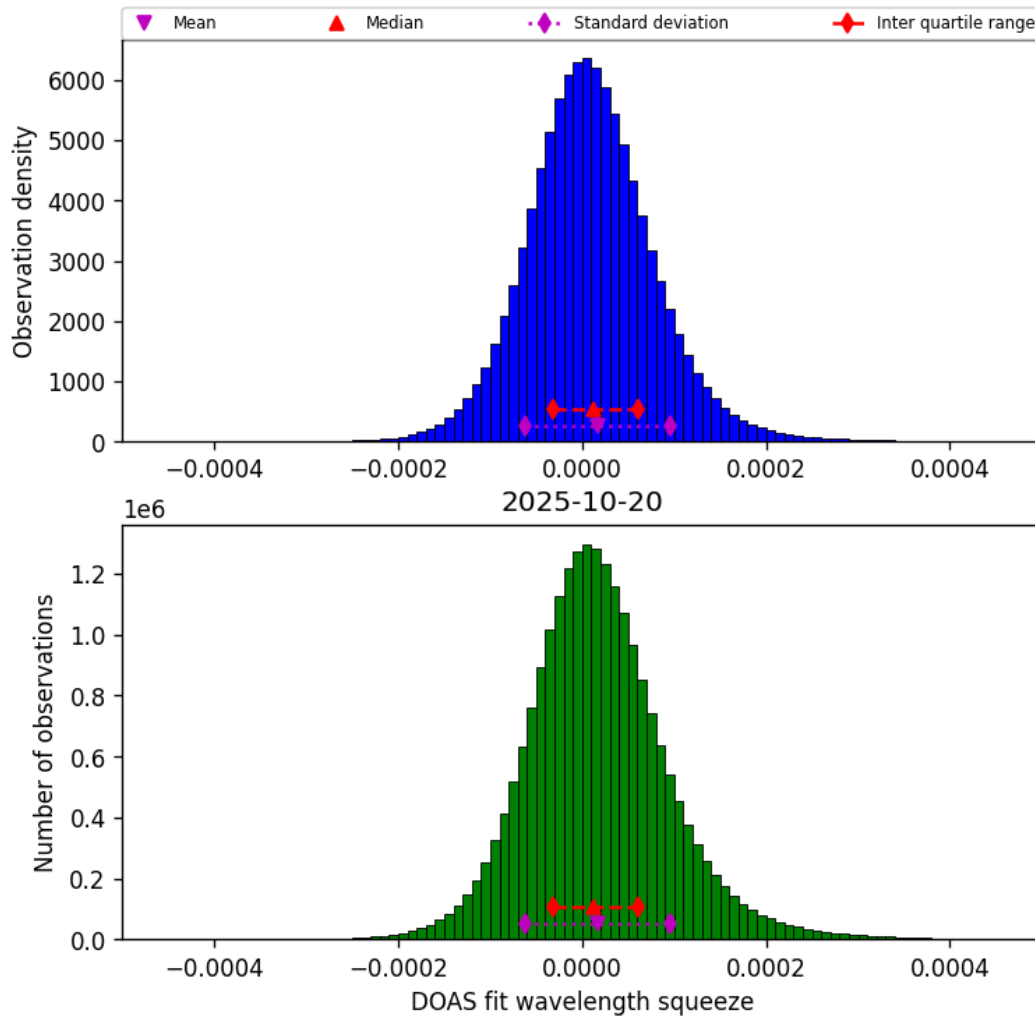
Figure 43: Histogram of “DOAS fit wavelength squeeze” for 2025-10-20 to 2025-10-20
