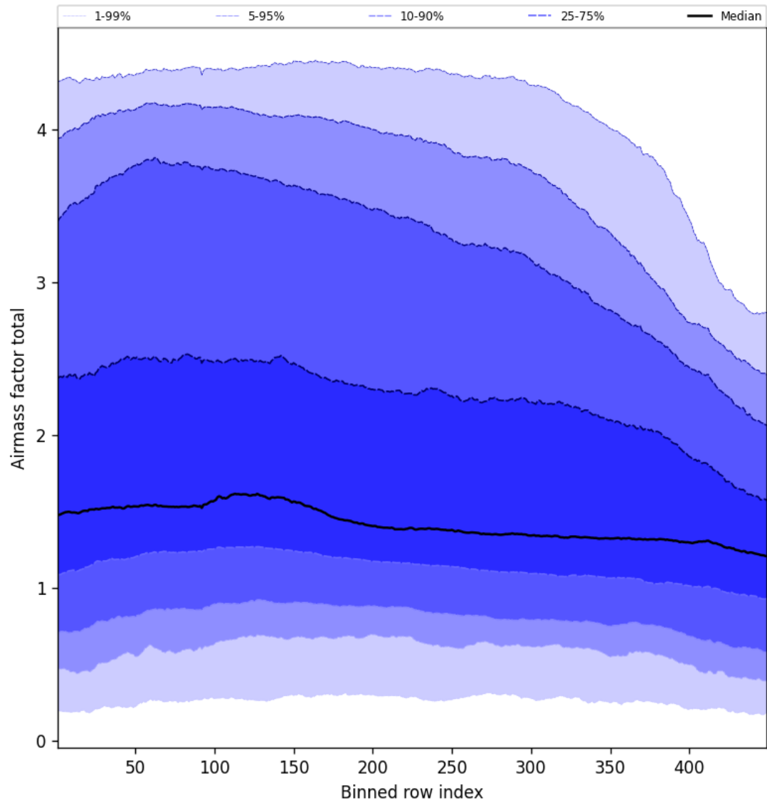
Figure 52: Along track statistics of “Airmass factor total” for 2025-10-20 to 2025-10-20
