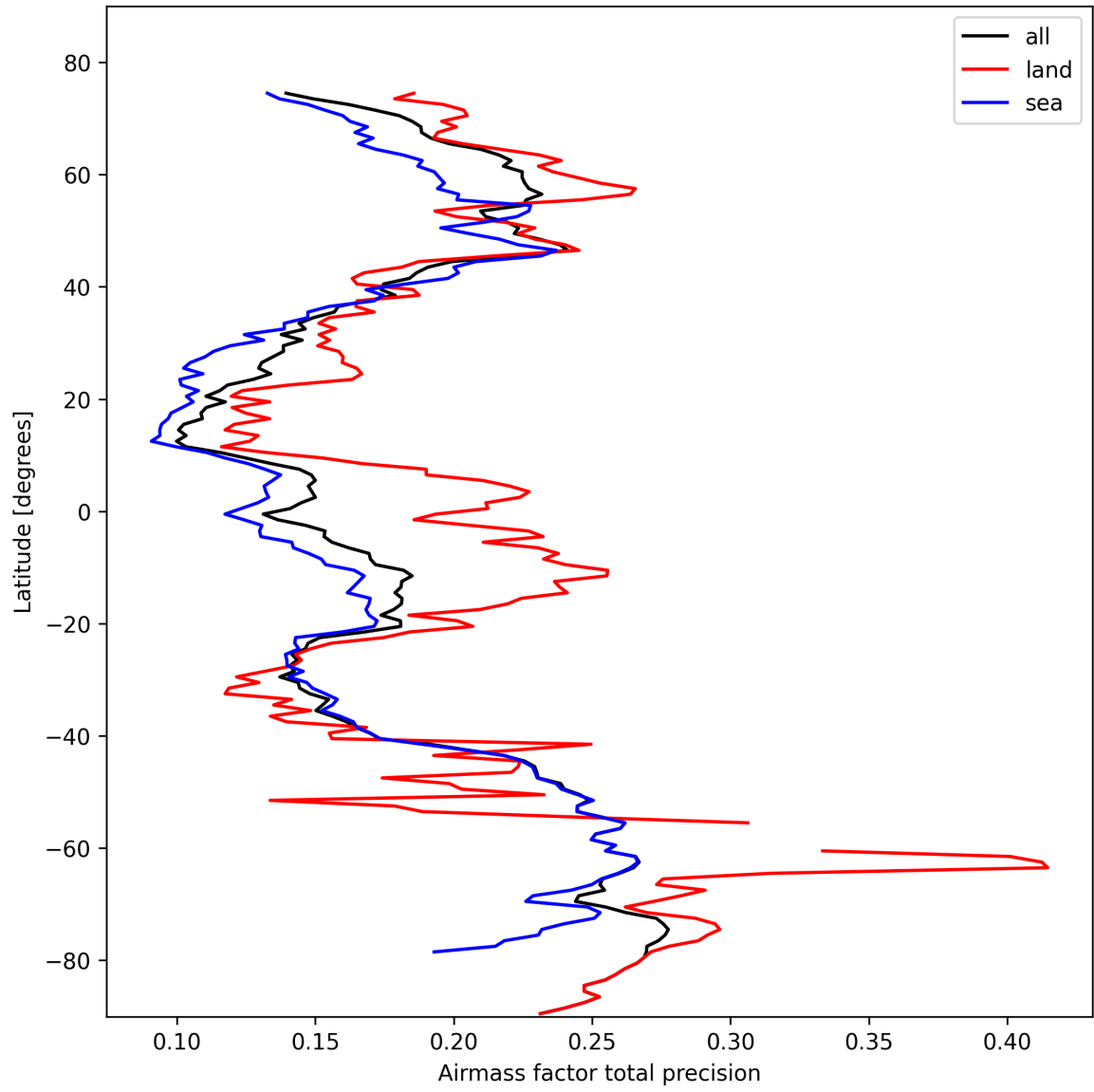
Figure 25: Zonal average of “Airmass factor total precision” for 2025-10-20 to 2025-10-20.
