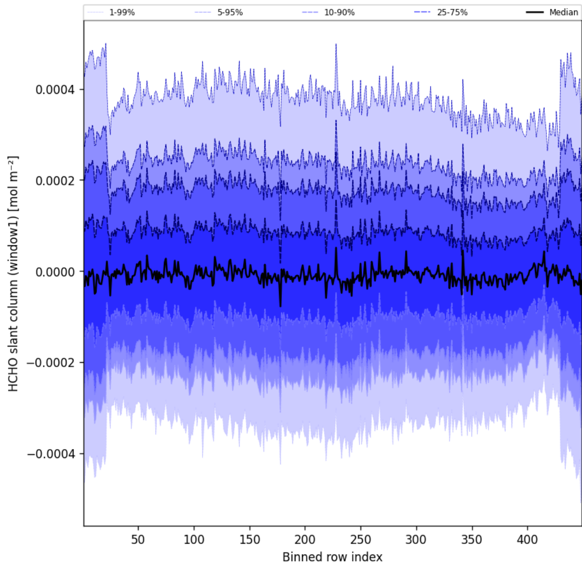
Figure 50: Along track statistics of “HCHO slant column (window1)” for 2025-10-20 to 2025-10-20
