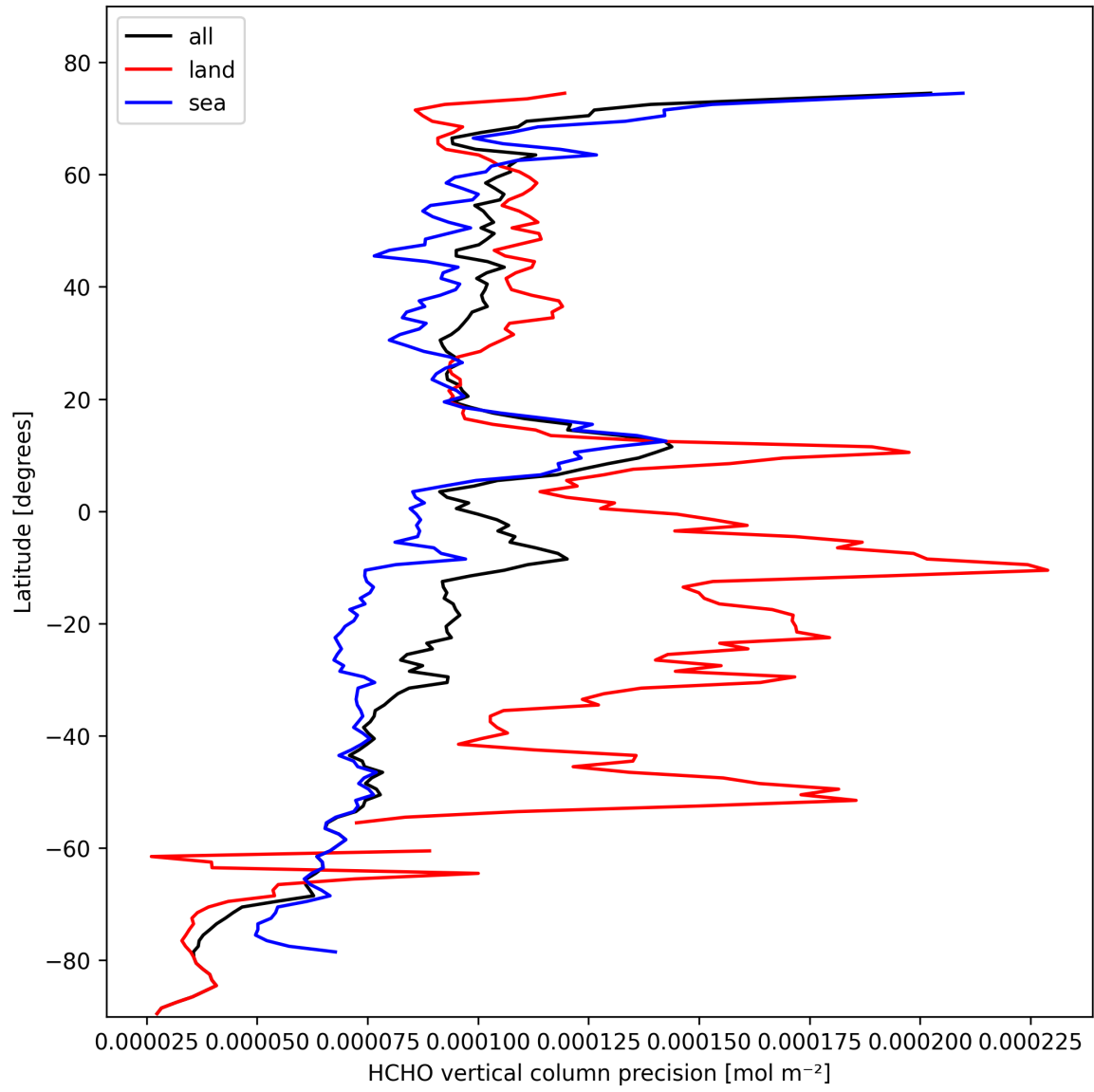
Figure 20: Zonal average of “HCHO vertical column precision” for 2025-10-20 to 2025-10-20.
