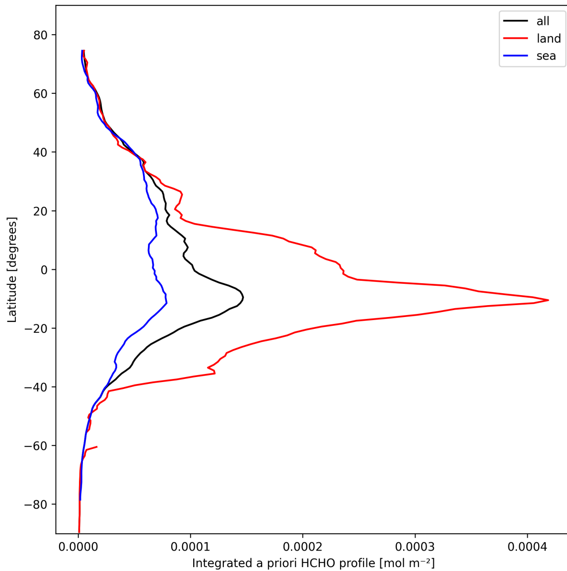
Figure 27: Zonal average of “Integrated a priori HCHO profile” for 2025-10-20 to 2025-10-20.
