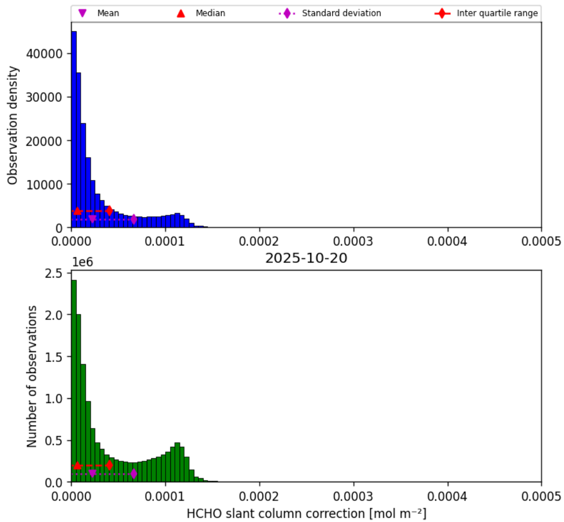
Figure 45: Histogram of “HCHO slant column correction” for 2025-10-20 to 2025-10-20
