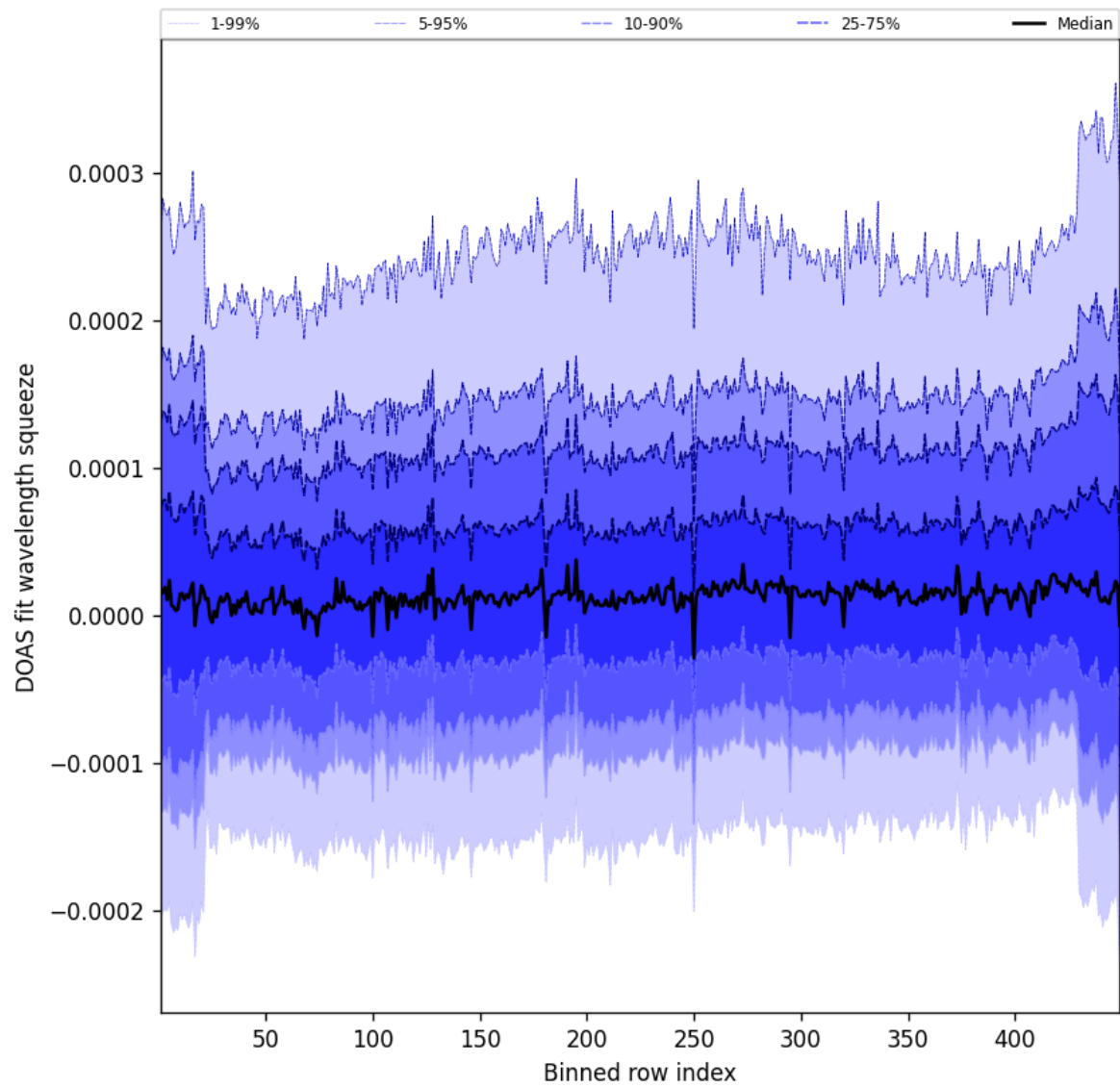
Figure 57: Along track statistics of “DOAS fit wavelength squeeze” for 2025-10-20 to 2025-10-20
