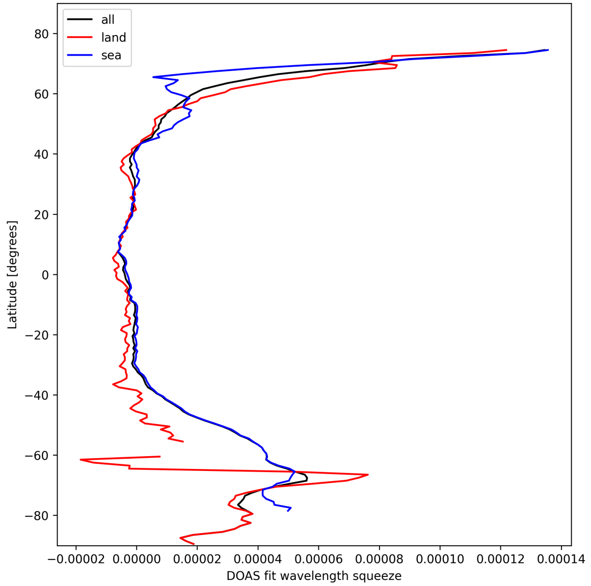
Figure 29: Zonal average of “DOAS fit wavelength squeeze” for 2025-10-20 to 2025-10-20.
