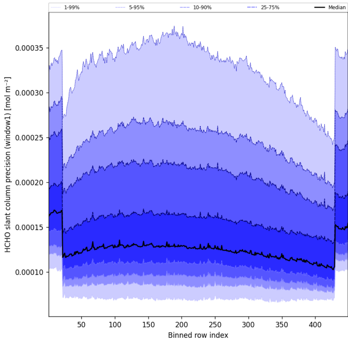
Figure 51: Along track statistics of “HCHO slant column precision (window1)” for 2025-10-20 to 2025-10-20
