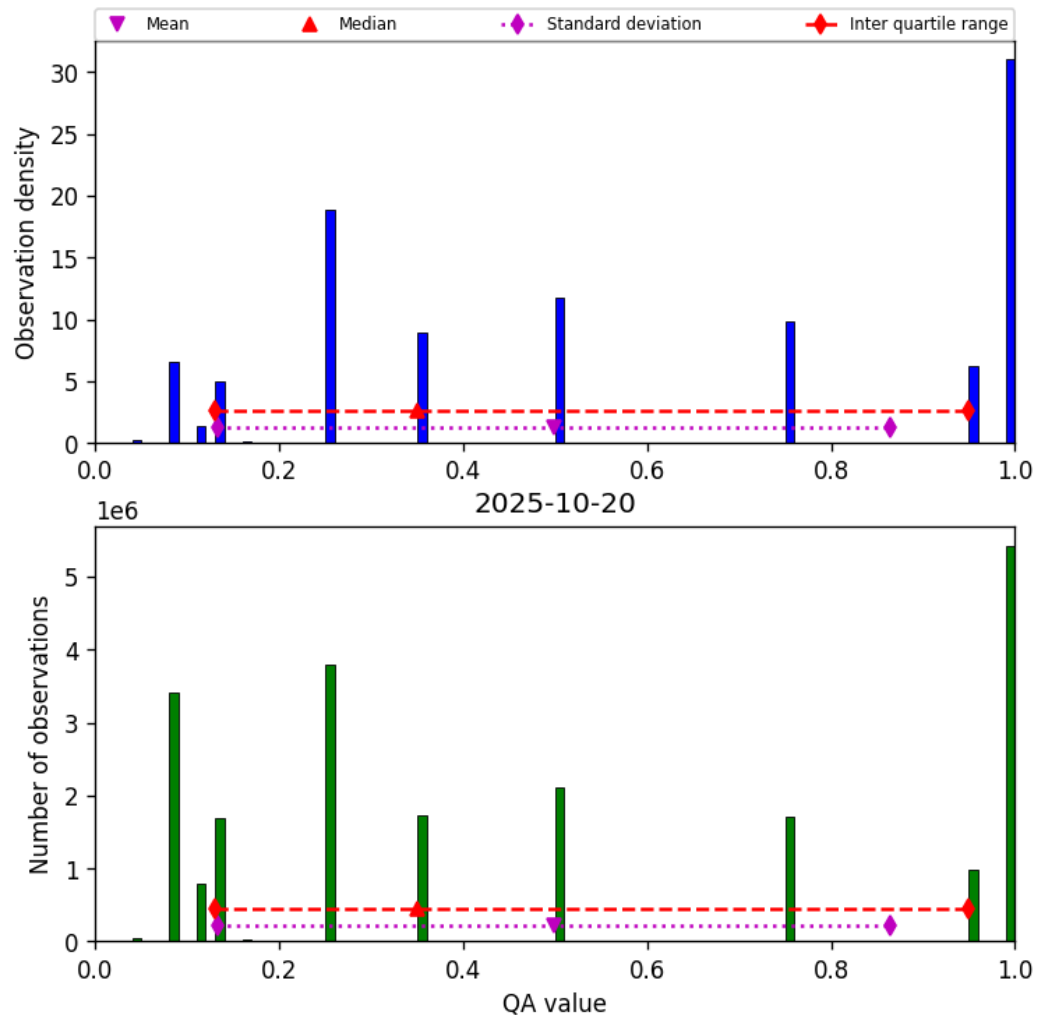
Figure 32: Histogram of “QA value” for 2025-10-20 to 2025-10-20
