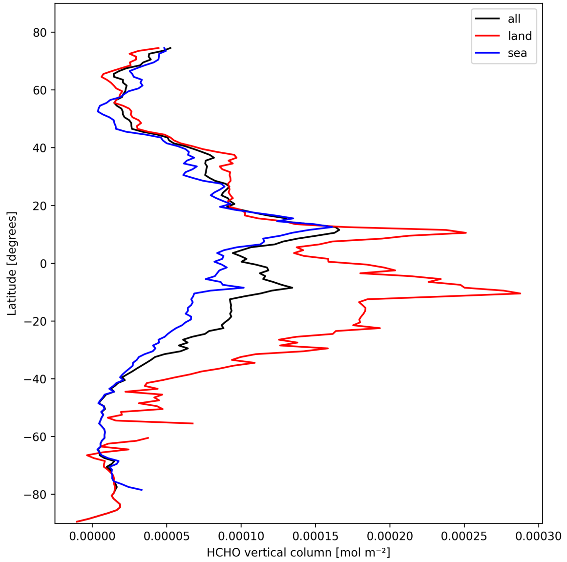
Figure 19: Zonal average of “HCHO vertical column” for 2025-10-20 to 2025-10-20.
