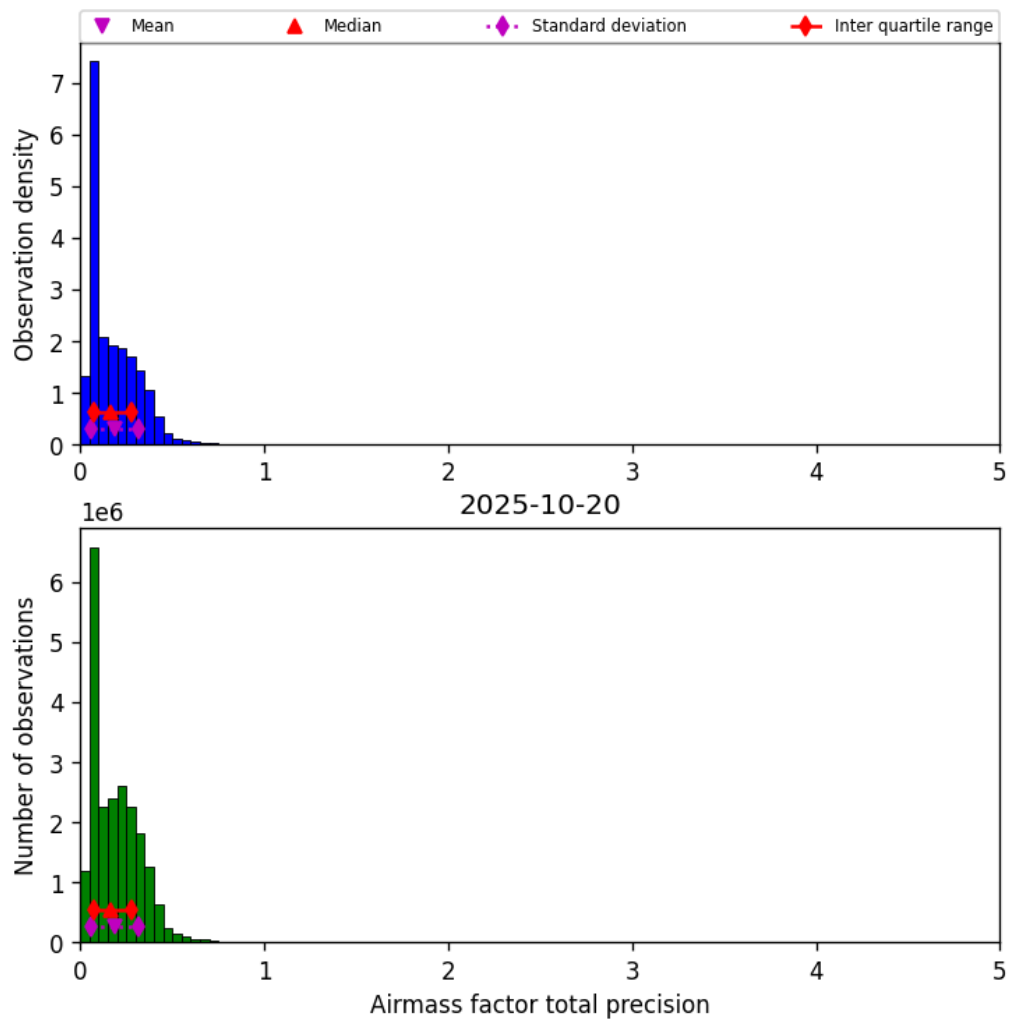
Figure 39: Histogram of “Airmass factor total precision” for 2025-10-20 to 2025-10-20
