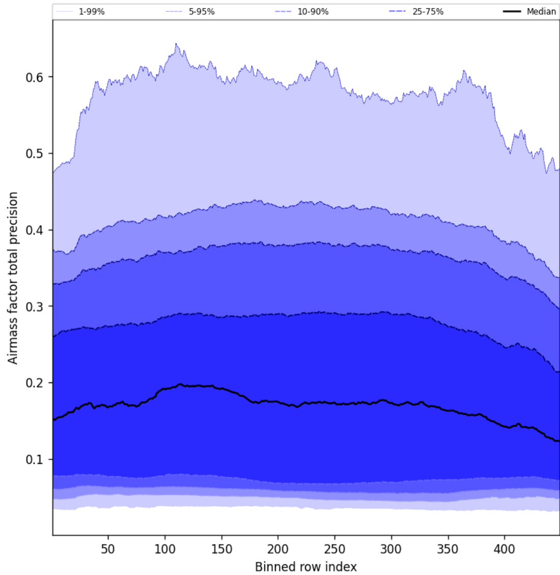
Figure 53: Along track statistics of “Airmass factor total precision” for 2025-10-20 to 2025-10-20
