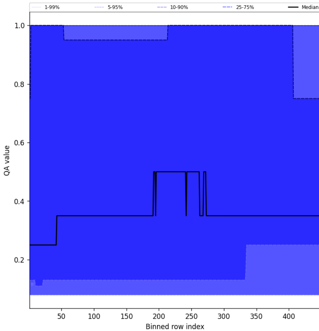
Figure 46: Along track statistics of “QA value” for 2025-10-20 to 2025-10-20
