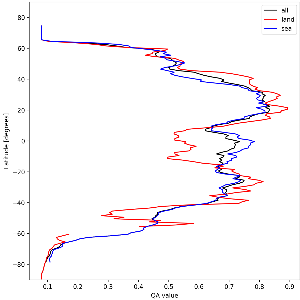
Figure 18: Zonal average of “QA value” for 2025-10-20 to 2025-10-20.
