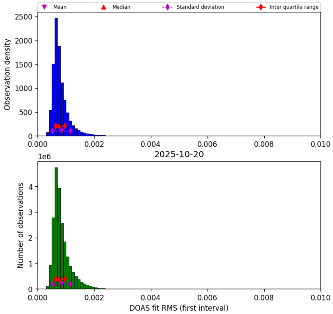
Figure 44: Histogram of “DOAS fit RMS (first interval)” for 2025-10-20 to 2025-10-20
