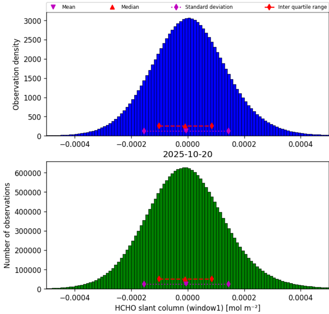
Figure 36: Histogram of "HCHO slant column (window1)" for 2025-10-20 to 2025-10-20
