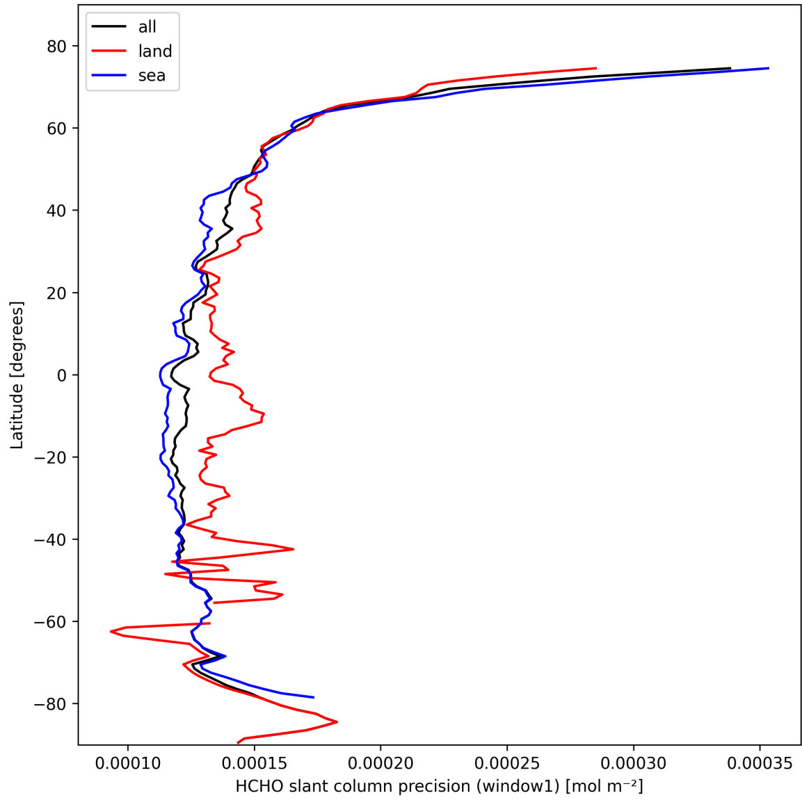
Figure 23: Zonal average of “HCHO slant column precision (window1)” for 2025-10-20 to 2025-10-20.
