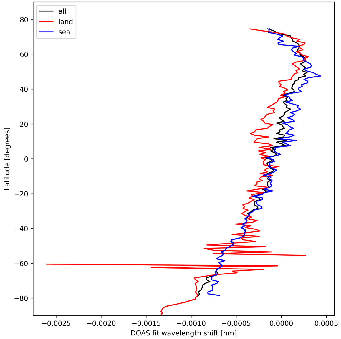
Figure 28: Zonal average of “DOAS fit wavelength shift” for 2025-10-20 to 2025-10-20.
