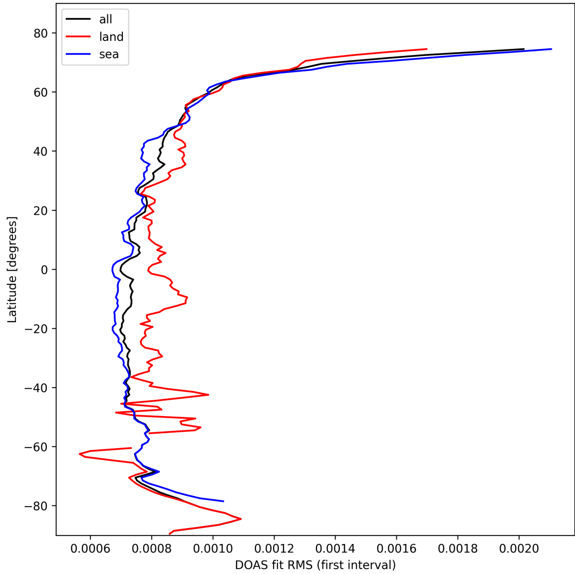
Figure 30: Zonal average of “DOAS fit RMS (first interval)” for 2025-10-20 to 2025-10-20.
