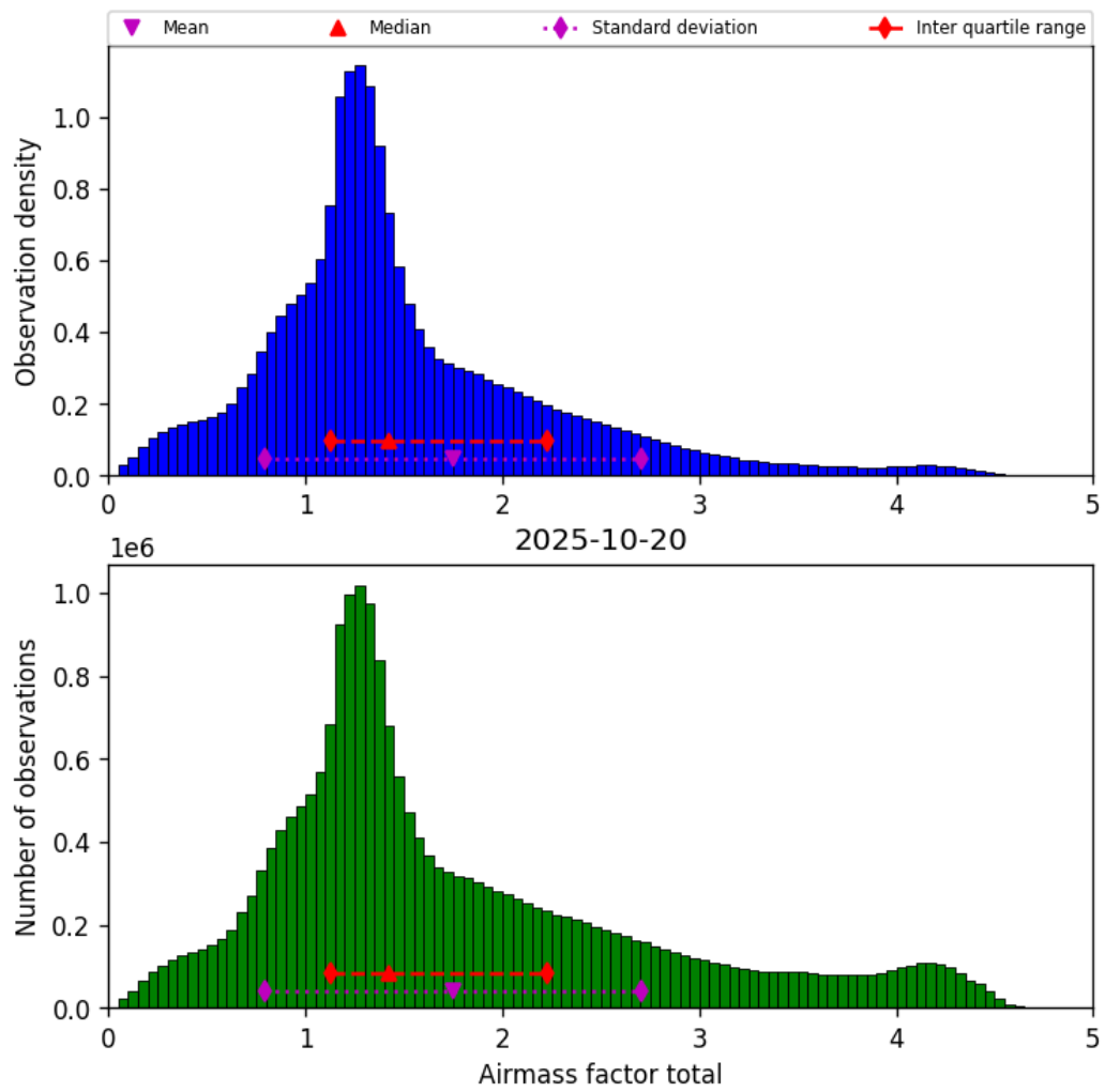
Figure 38: Histogram of “Airmass factor total” for 2025-10-20 to 2025-10-20
