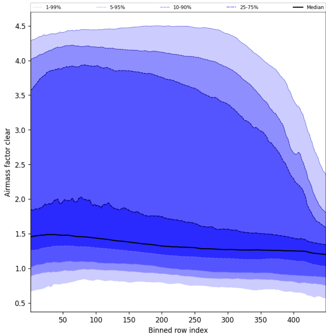
Figure 54: Along track statistics of “Airmass factor clear” for 2025-10-20 to 2025-10-20
