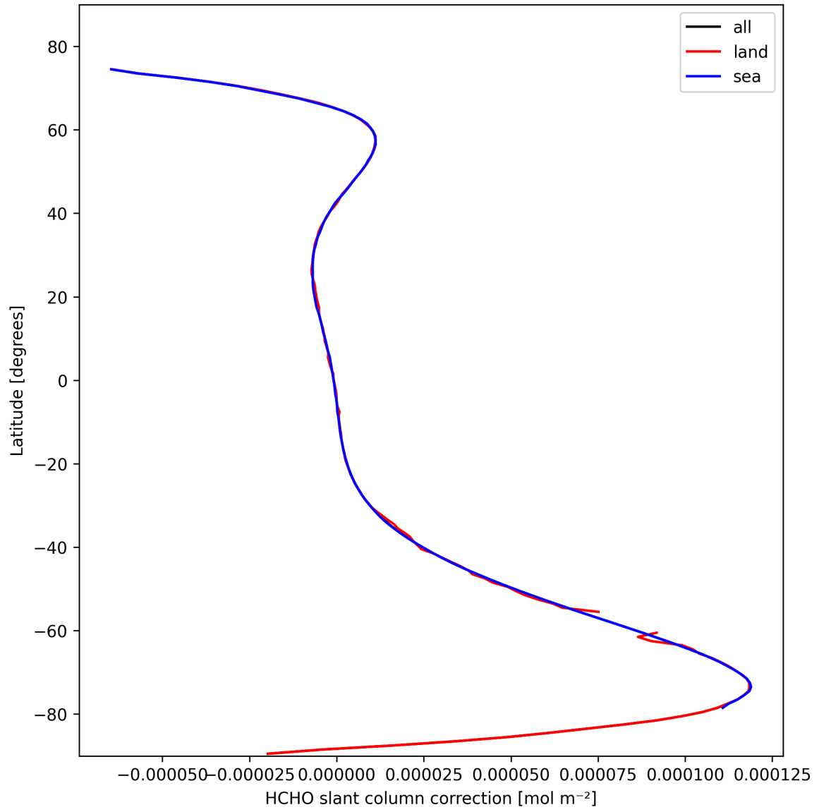
Figure 31: Zonal average of “HCHO slant column correction” for 2025-10-20 to 2025-10-20.
