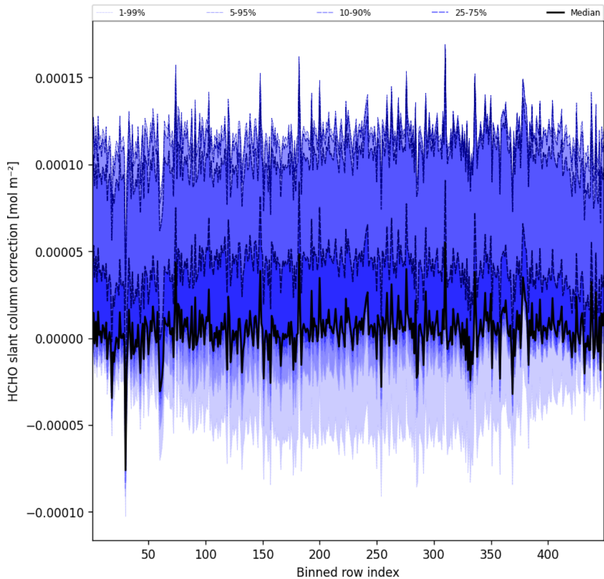
Figure 59: Along track statistics of “HCHO slant column correction” for 2025-10-20 to 2025-10-20
