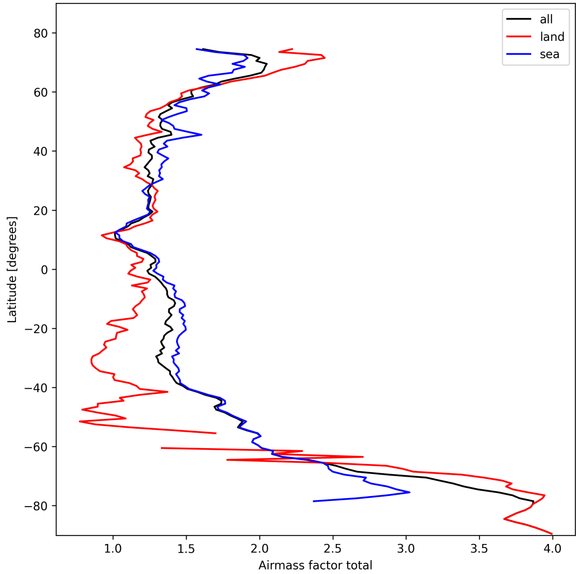
Figure 24: Zonal average of “Airmass factor total” for 2025-10-20 to 2025-10-20.
