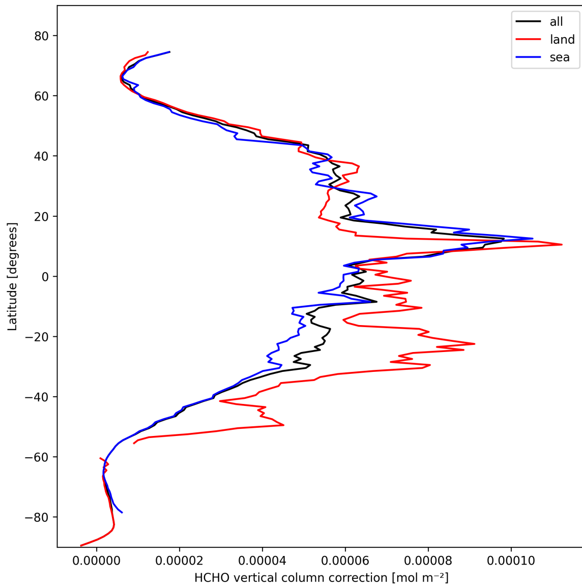
Figure 21: Zonal average of “HCHO vertical column correction” for 2025-10-20 to 2025-10-20.
