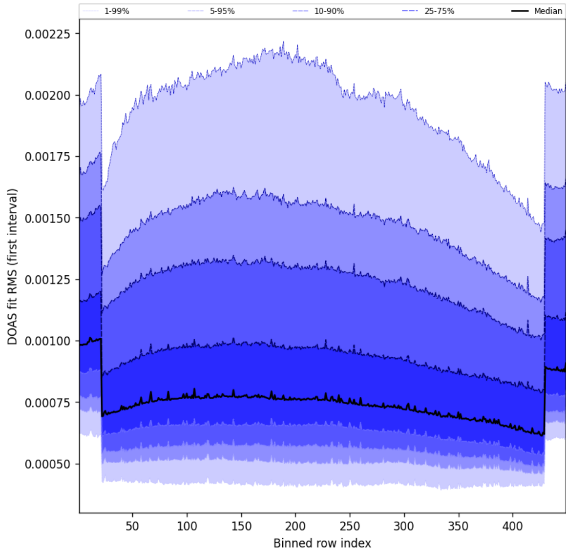
Figure 58: Along track statistics of “DOAS fit RMS (first interval)” for 2025-10-20 to 2025-10-20
