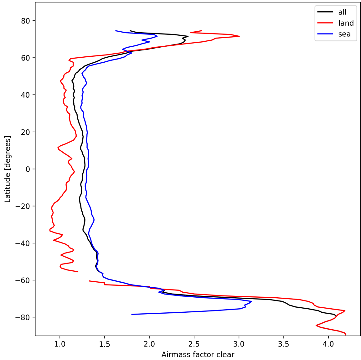
Figure 26: Zonal average of “Airmass factor clear” for 2025-10-20 to 2025-10-20.
