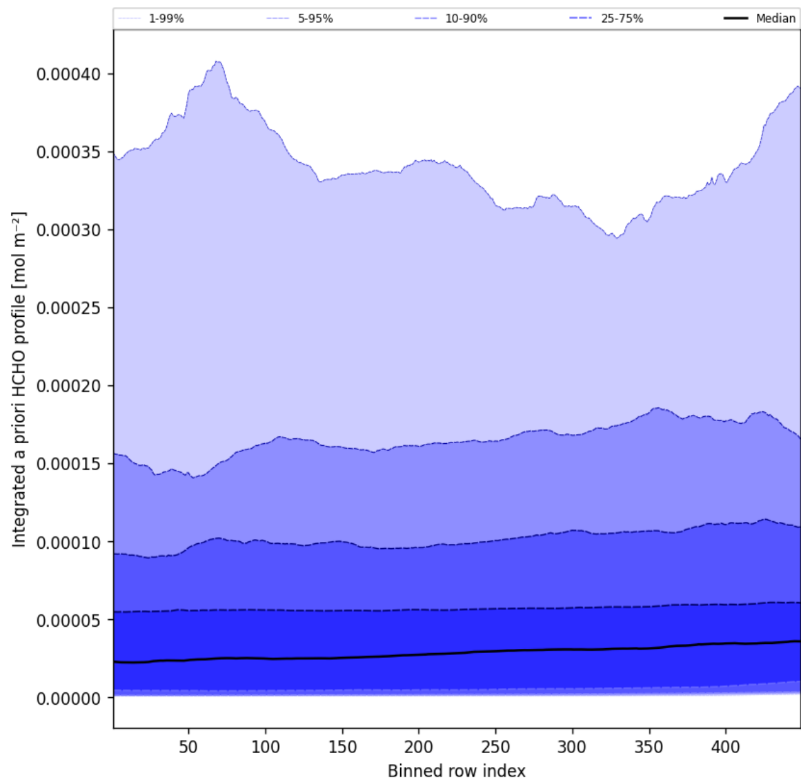
Figure 55: Along track statistics of “Integrated a priori HCHO profile” for 2025-10-20 to 2025-10-20
