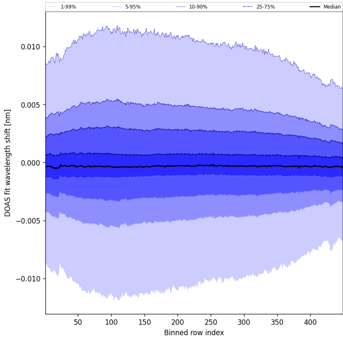
Figure 56: Along track statistics of “DOAS fit wavelength shift” for 2025-10-20 to 2025-10-20
