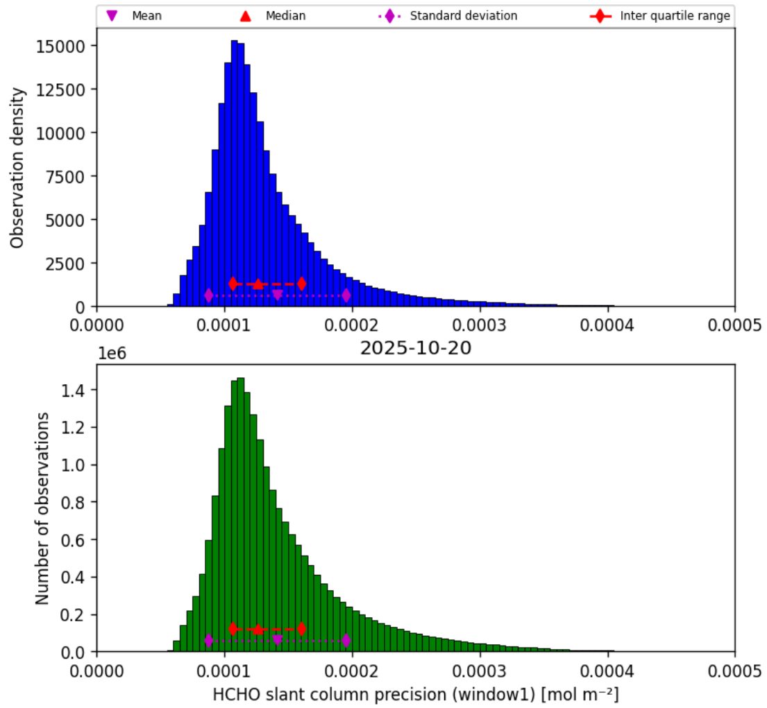
Figure 37: Histogram of “HCHO slant column precision (window1)” for 2025-10-20 to 2025-10-20
