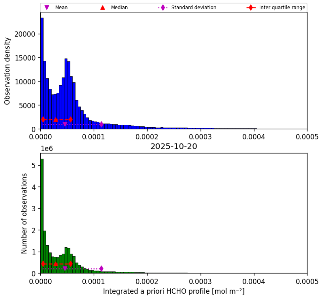
Figure 41: Histogram of “Integrated a priori HCHO profile” for 2025-10-20 to 2025-10-20
