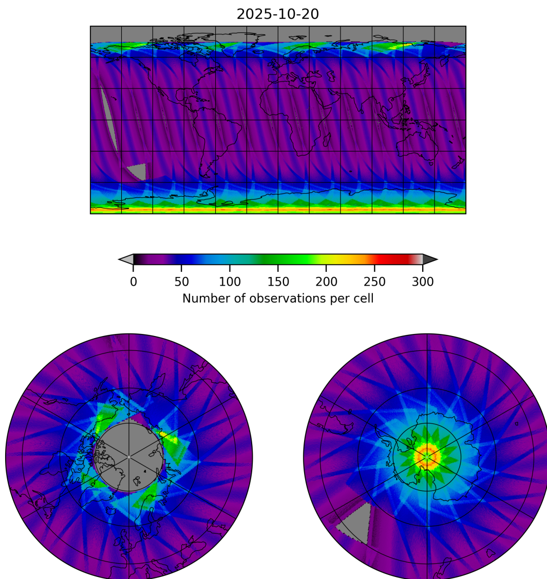
Figure 17: Map of the number of observations for 2025-10-20 to 2025-10-20
