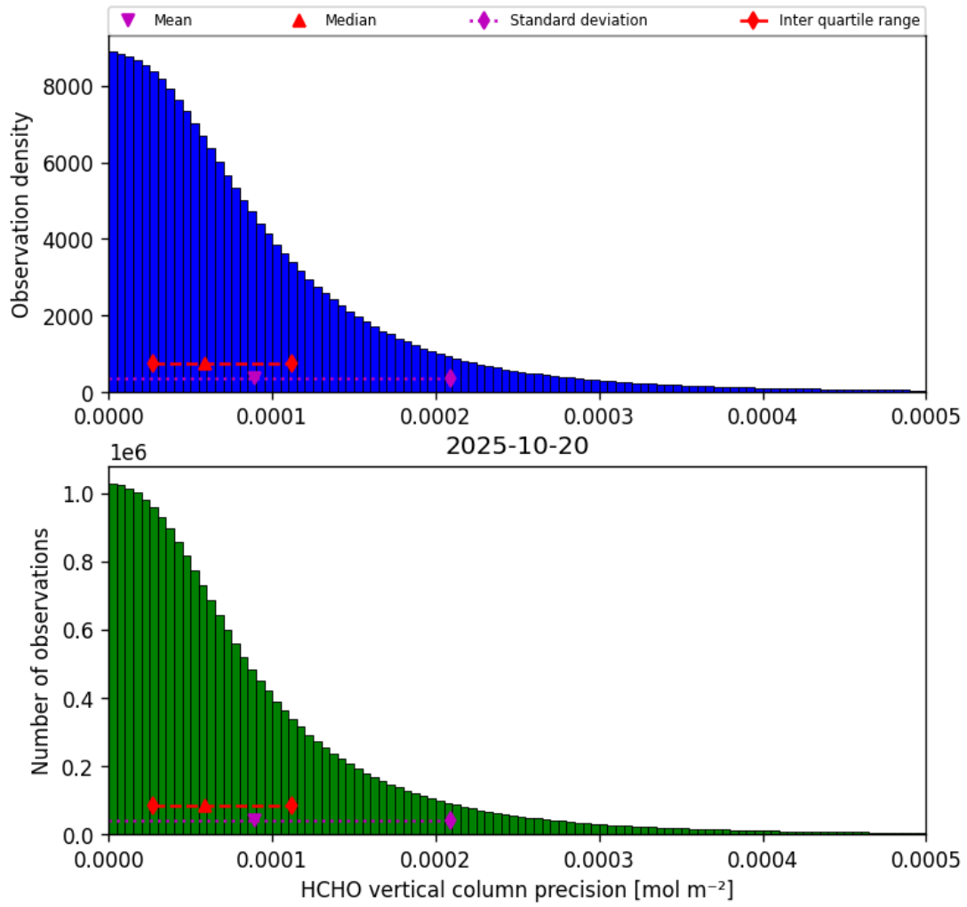
Figure 34: Histogram of “HCHO vertical column precision” for 2025-10-20 to 2025-10-20
