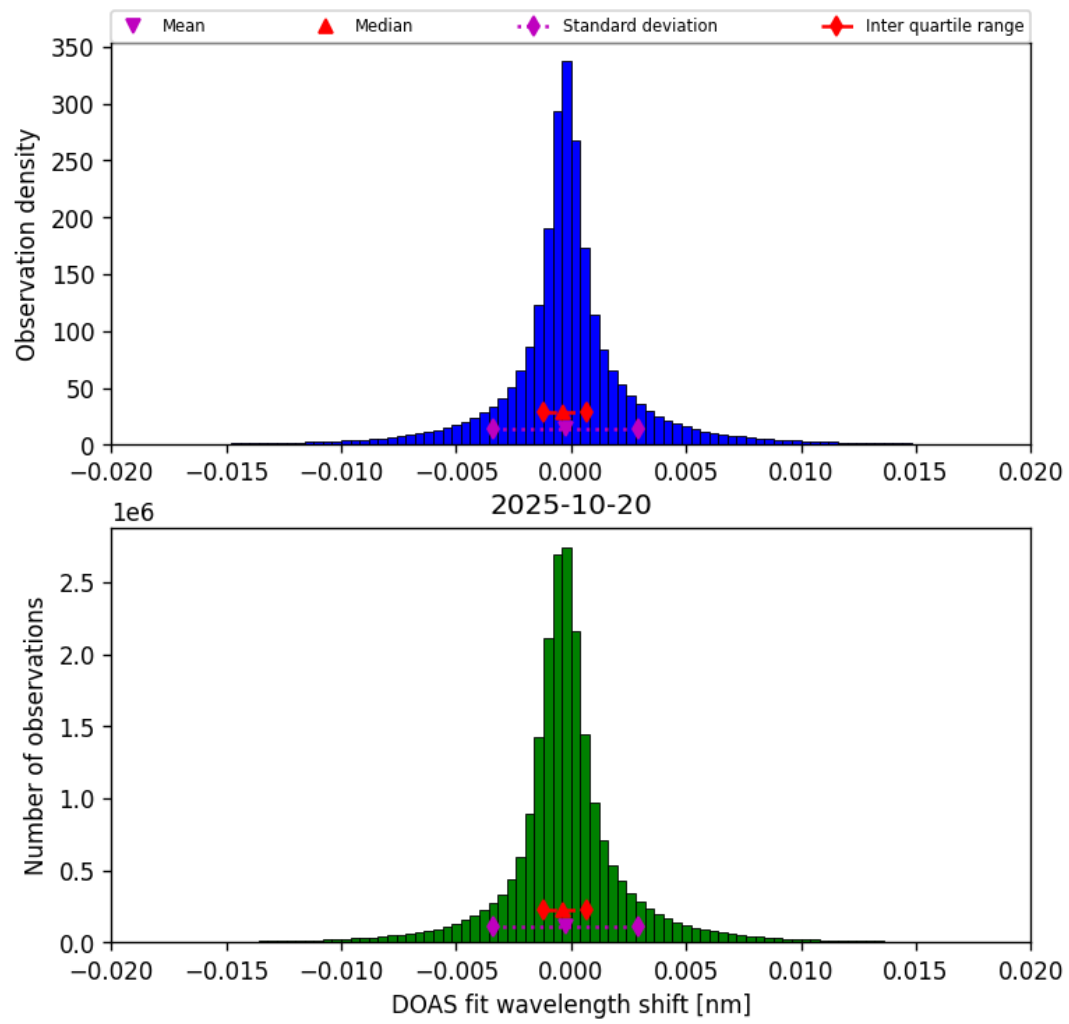
Figure 42: Histogram of “DOAS fit wavelength shift” for 2025-10-20 to 2025-10-20
