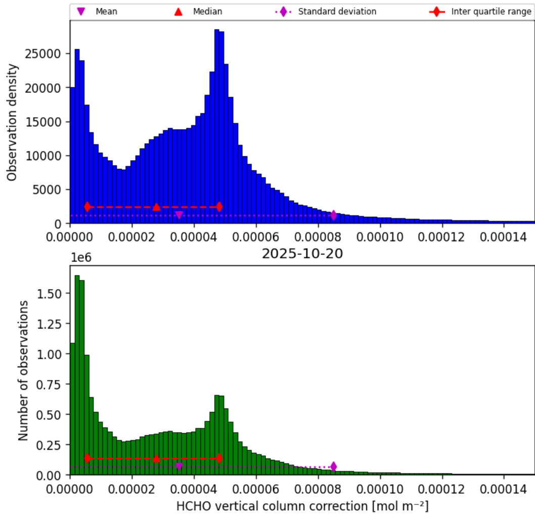
Figure 35: Histogram of “HCHO vertical column correction” for 2025-10-20 to 2025-10-20
