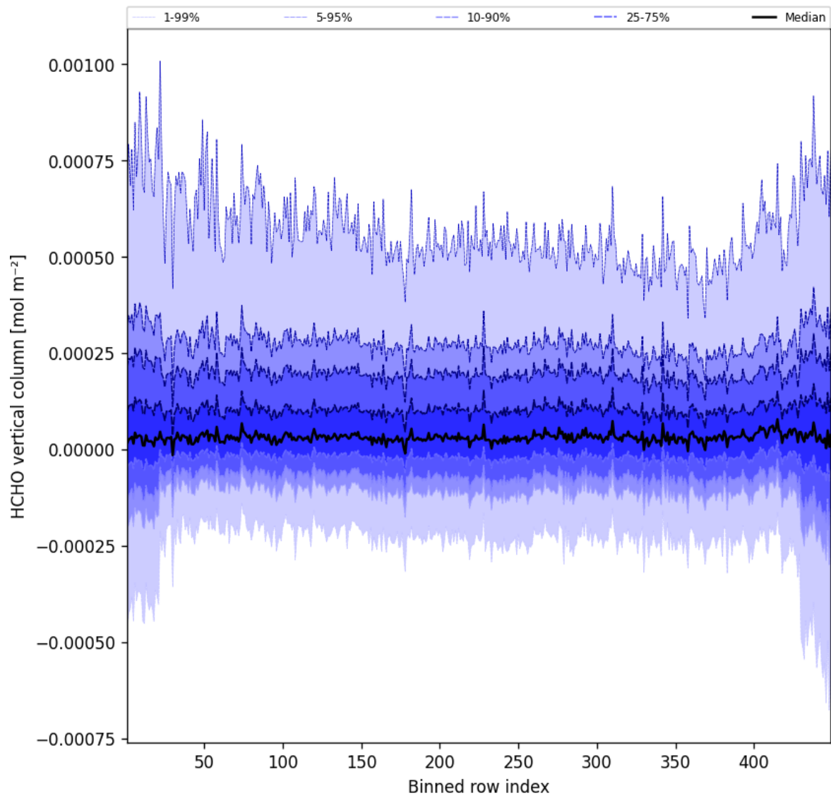
Figure 47: Along track statistics of “HCHO vertical column” for 2025-10-20 to 2025-10-20
