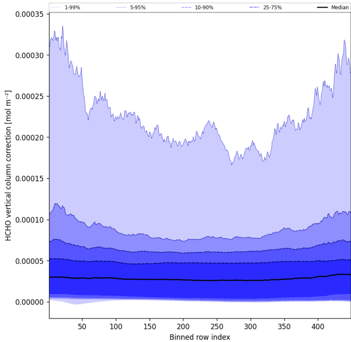
Figure 49: Along track statistics of “HCHO vertical column correction” for 2025-10-20 to 2025-10-20
