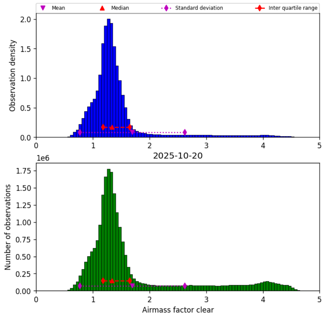
Figure 40: Histogram of “Airmass factor clear” for 2025-10-20 to 2025-10-20
