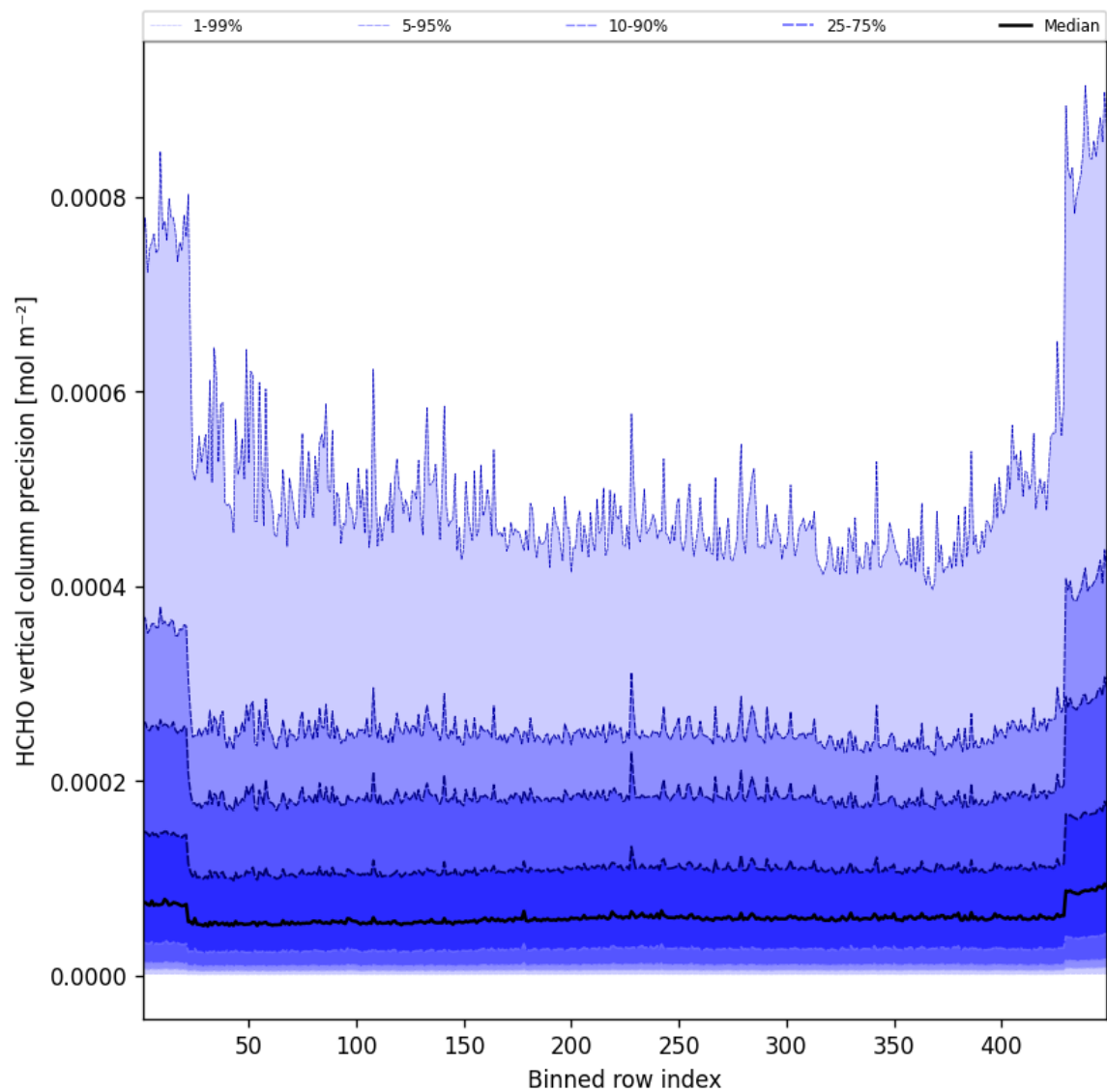
Figure 48: Along track statistics of “HCHO vertical column precision” for 2025-10-20 to 2025-10-20
