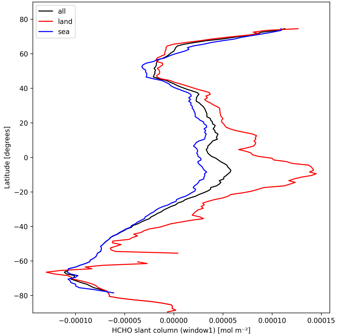
Figure 22: Zonal average of “HCHO slant column (window1)” for 2025-10-20 to 2025-10-20.
