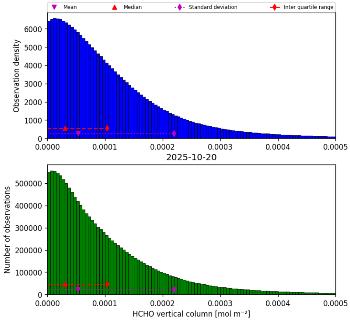
Figure 33: Histogram of “HCHO vertical column” for 2025-10-20 to 2025-10-20
