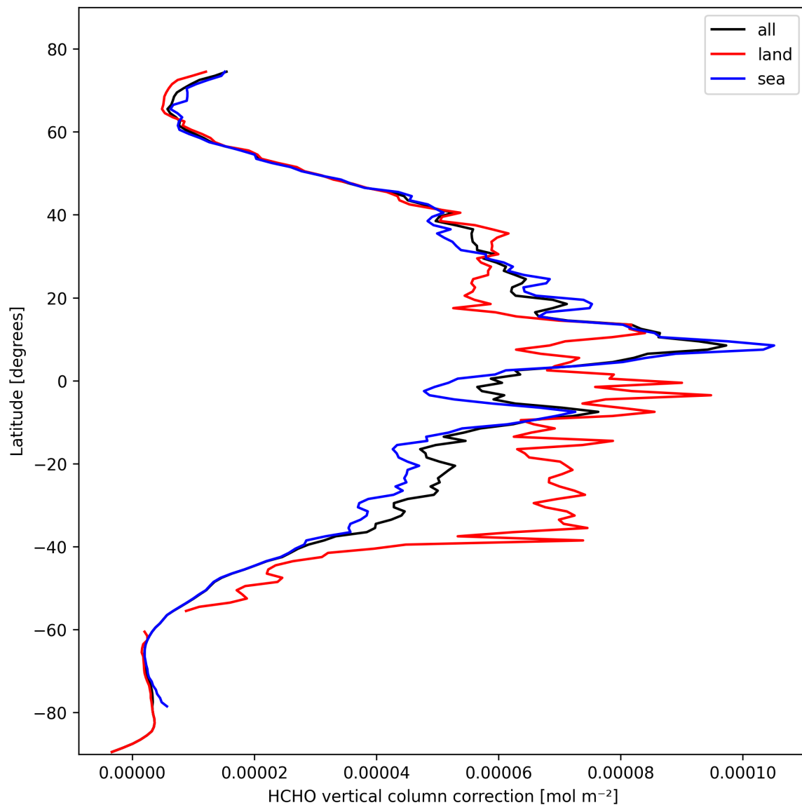
Figure 21: Zonal average of “HCHO vertical column correction” for 2025-10-21 to 2025-10-22.
