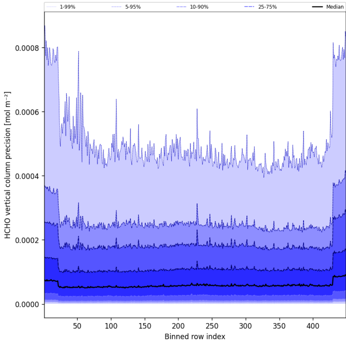
Figure 48: Along track statistics of "HCHO vertical column precision" for 2025-10-21 to 2025-10-22
