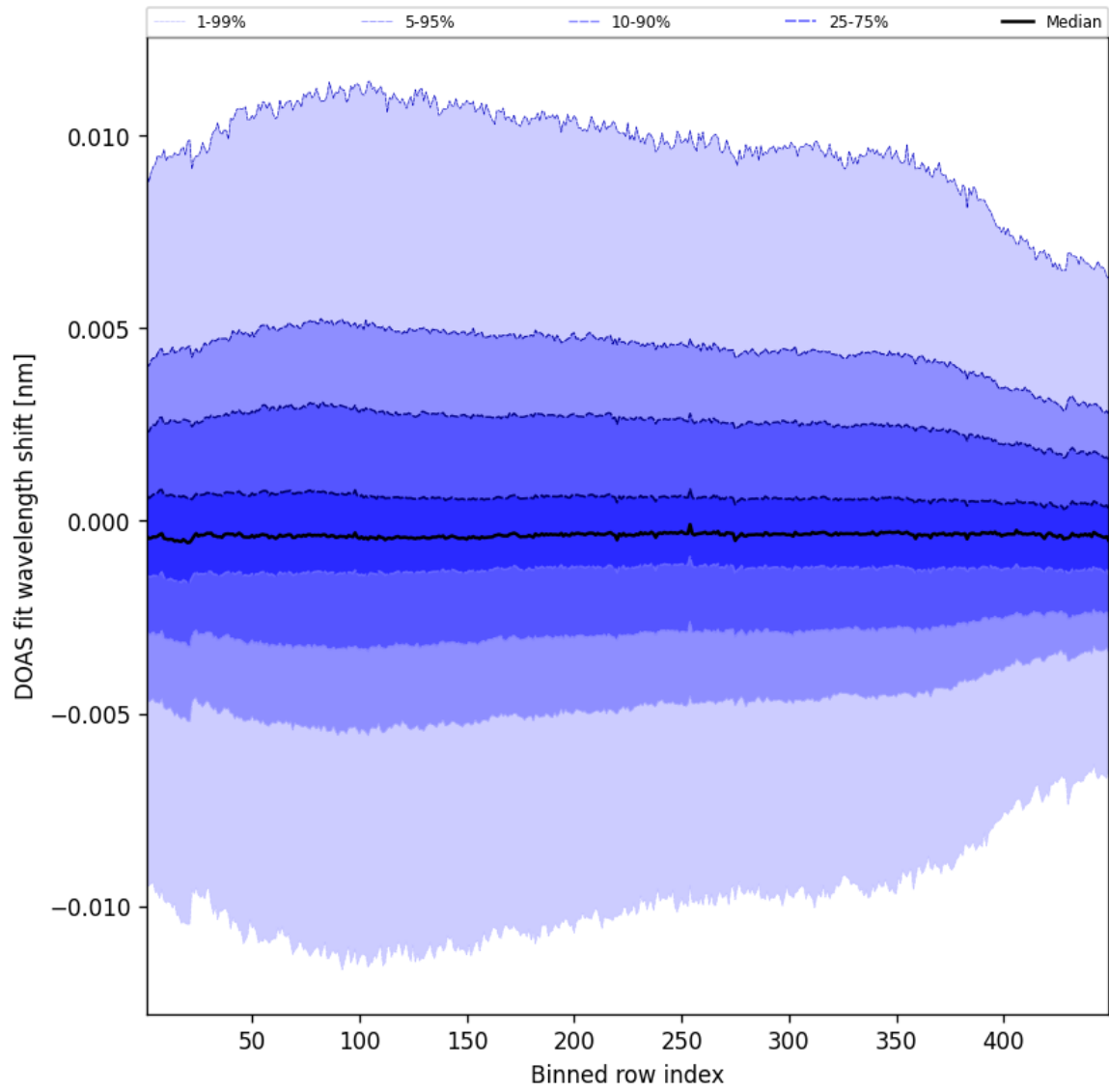
Figure 56: Along track statistics of “DOAS fit wavelength shift” for 2025-10-21 to 2025-10-22
