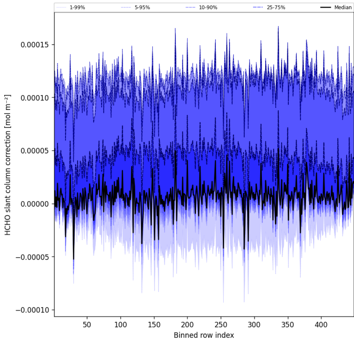
Figure 59: Along track statistics of “HCHO slant column correction” for 2025-10-21 to 2025-10-22
