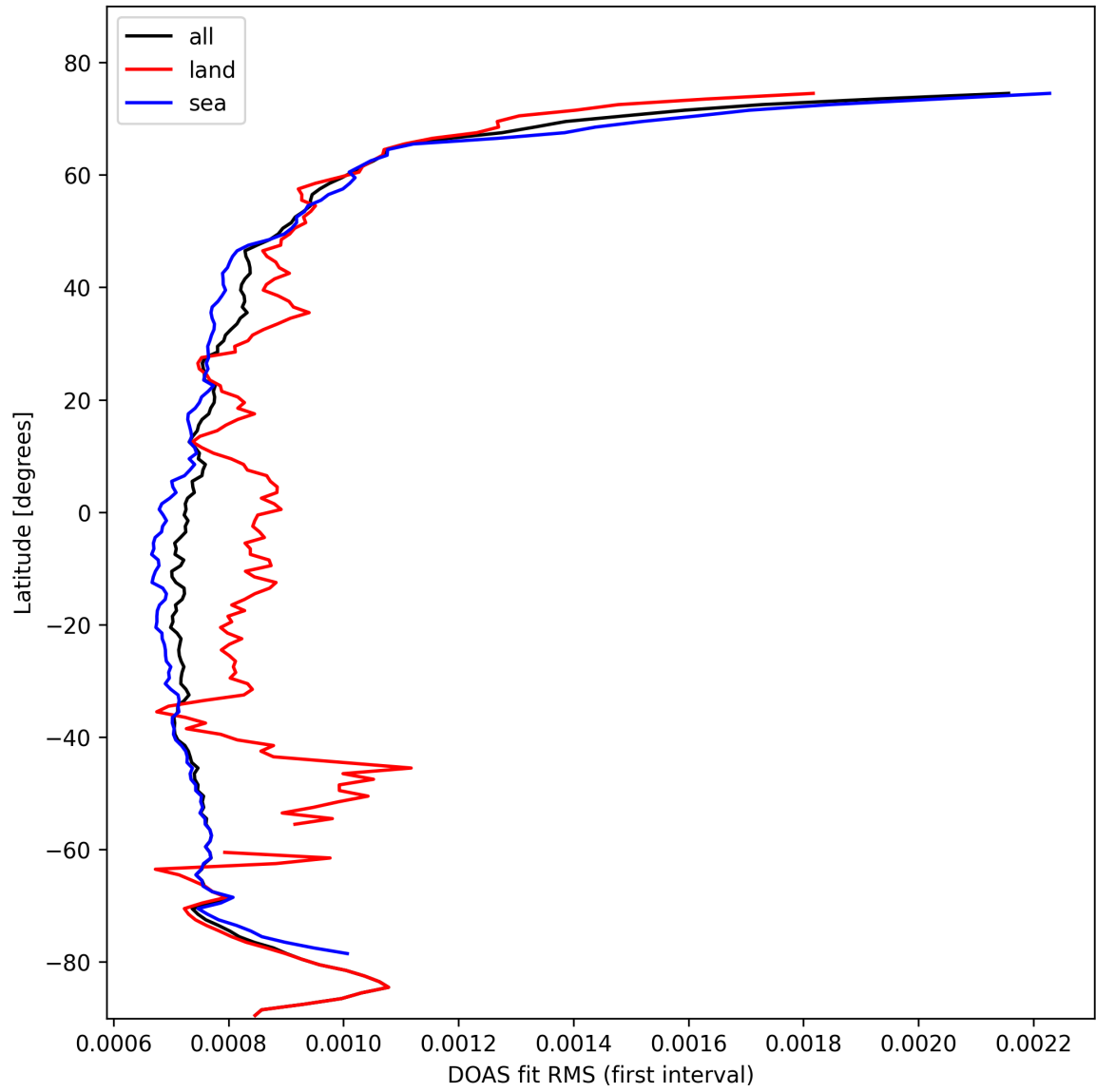
Figure 30: Zonal average of “DOAS fit RMS (first interval)” for 2025-10-21 to 2025-10-22.
