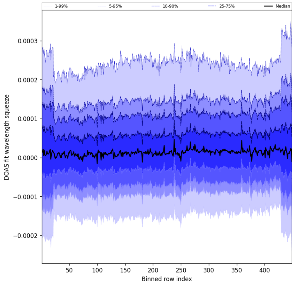
Figure 57: Along track statistics of “DOAS fit wavelength squeeze” for 2025-10-21 to 2025-10-22
