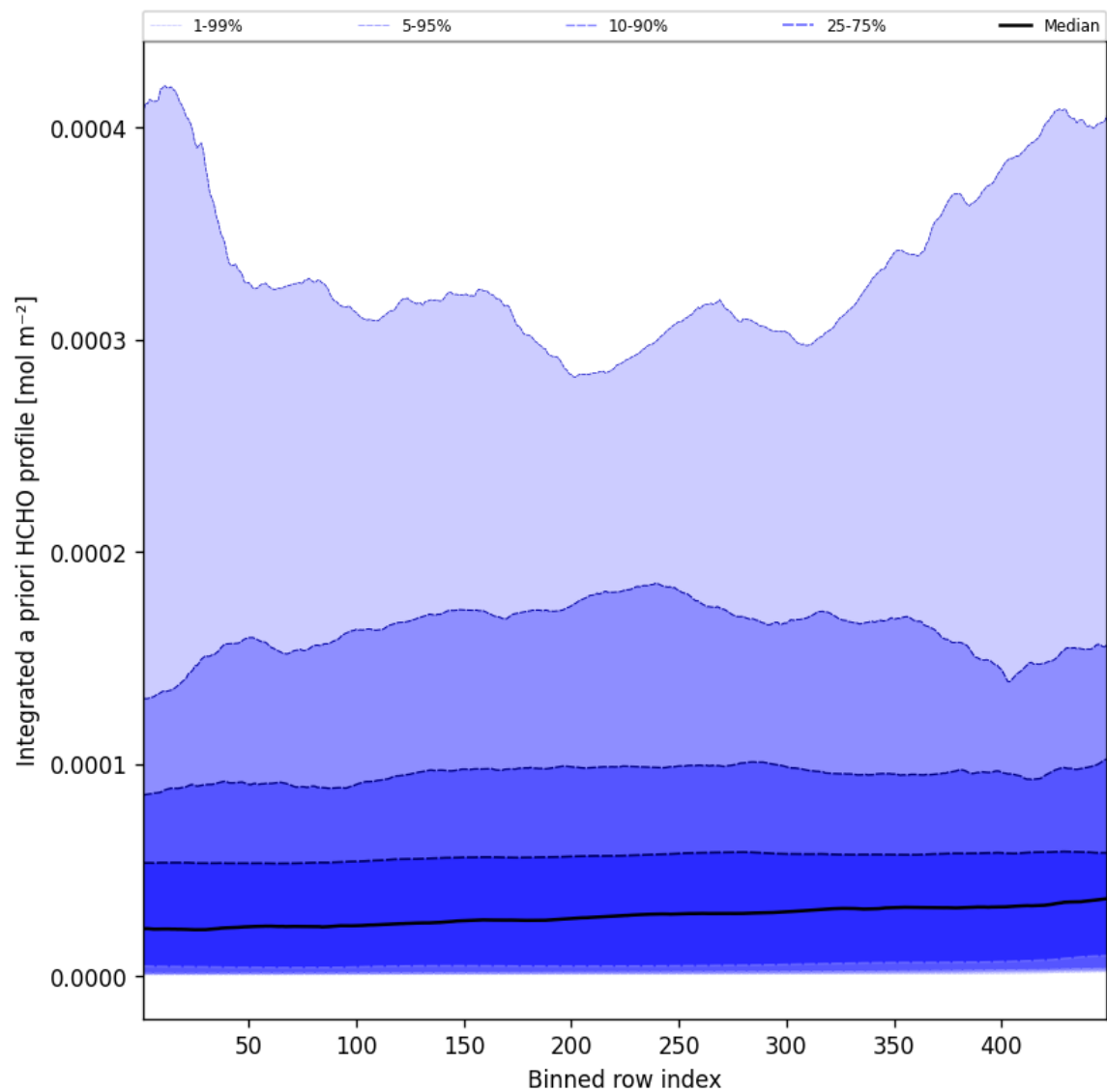
Figure 55: Along track statistics of "Integrated a priori HCHO profile" for 2025-10-21 to 2025-10-22
