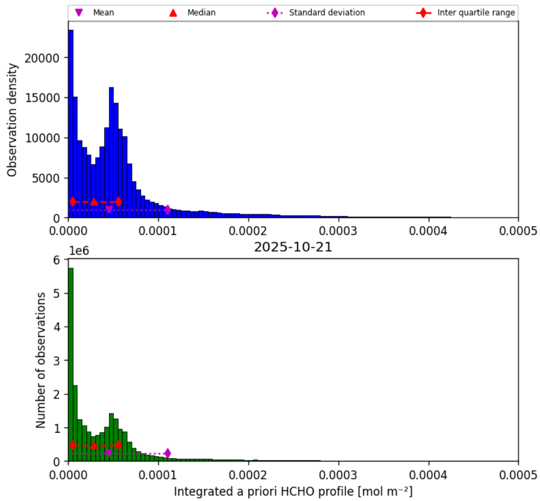
Figure 41: Histogram of “Integrated a priori HCHO profile” for 2025-10-21 to 2025-10-22
