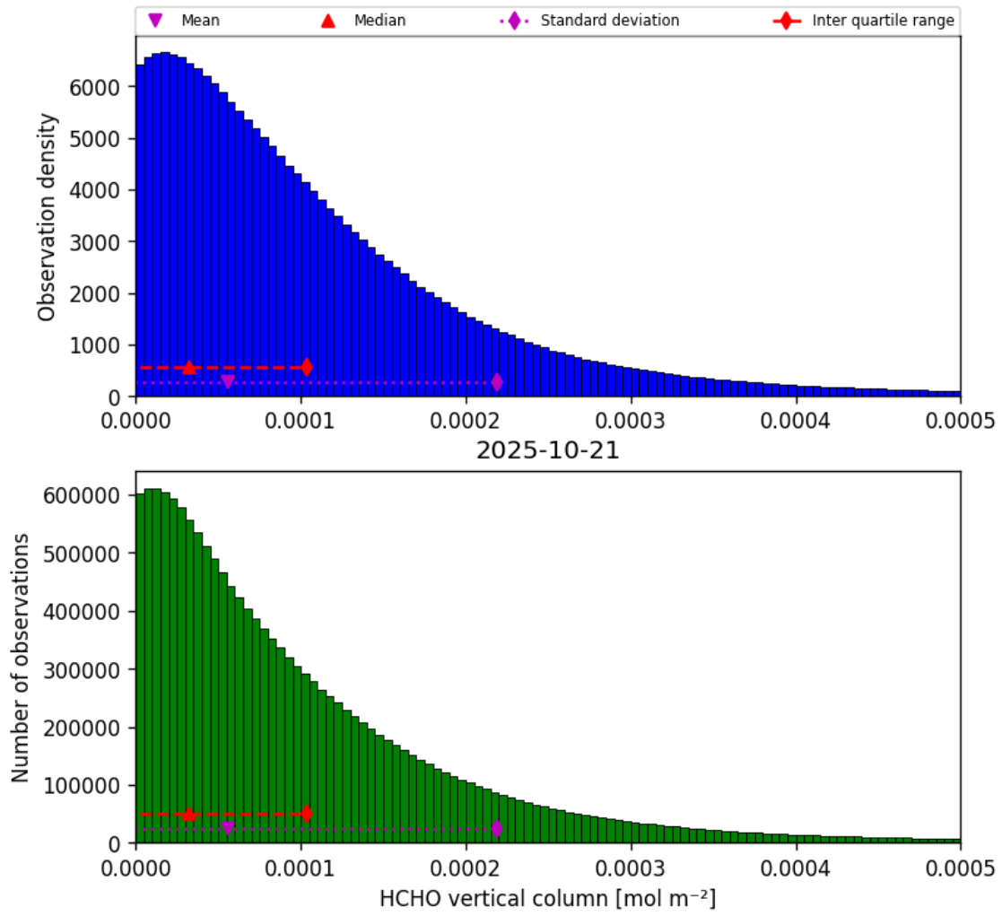
Figure 33: Histogram of “HCHO vertical column” for 2025-10-21 to 2025-10-22
