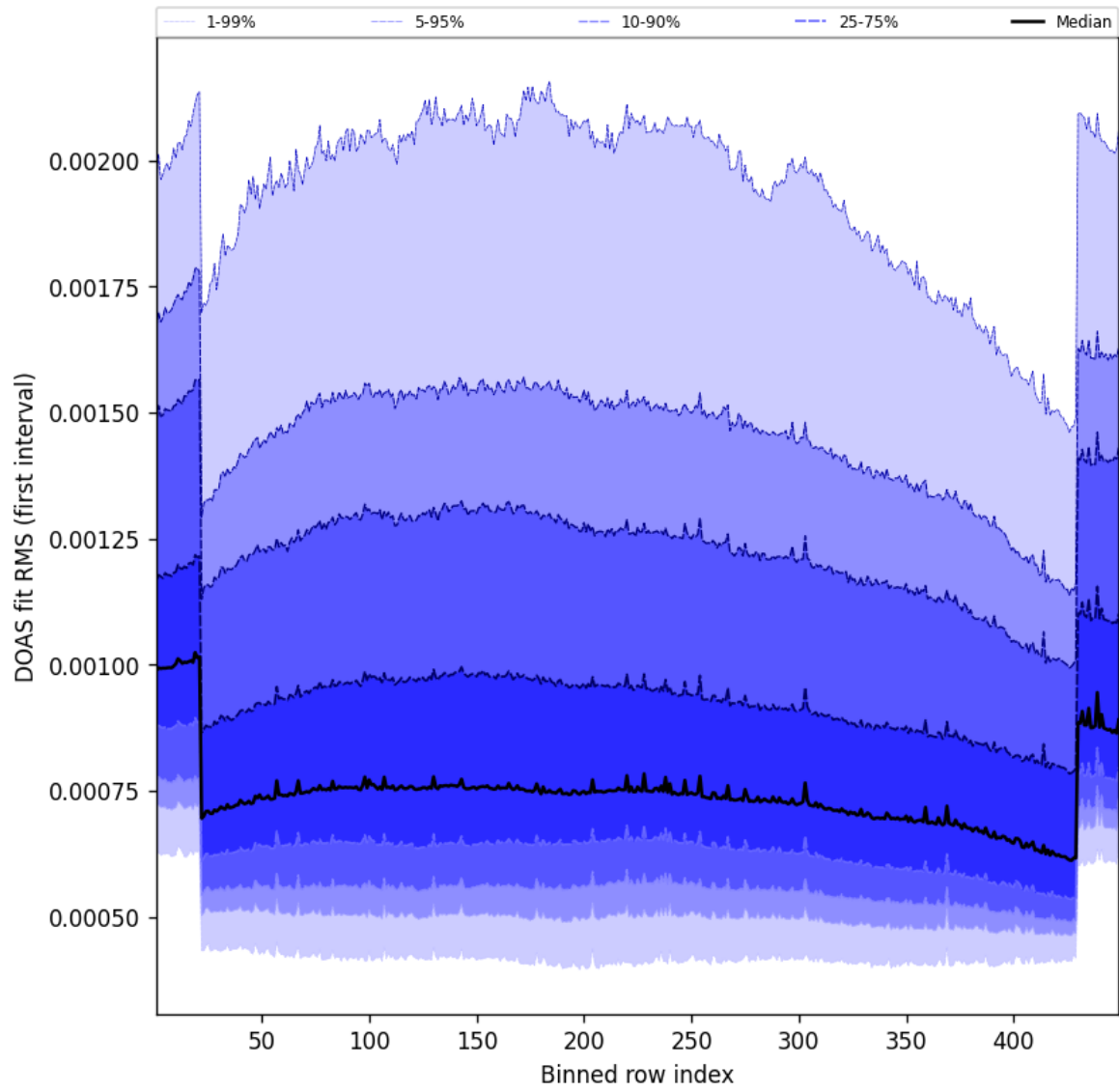
Figure 58: Along track statistics of “DOAS fit RMS (first interval)” for 2025-10-21 to 2025-10-22
