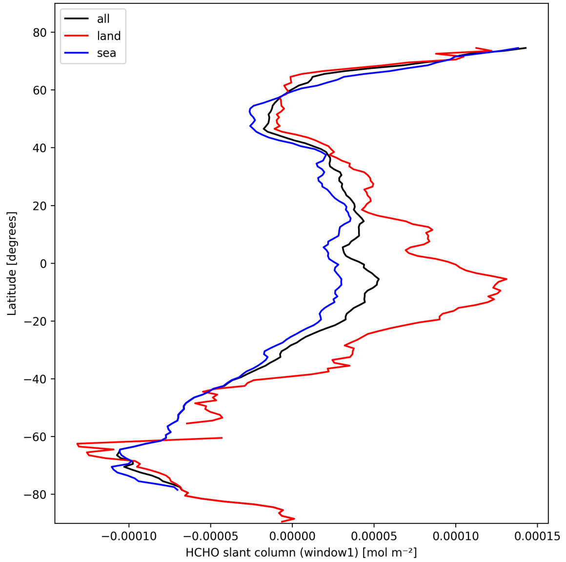
Figure 22: Zonal average of “HCHO slant column (window1)” for 2025-10-21 to 2025-10-22.
