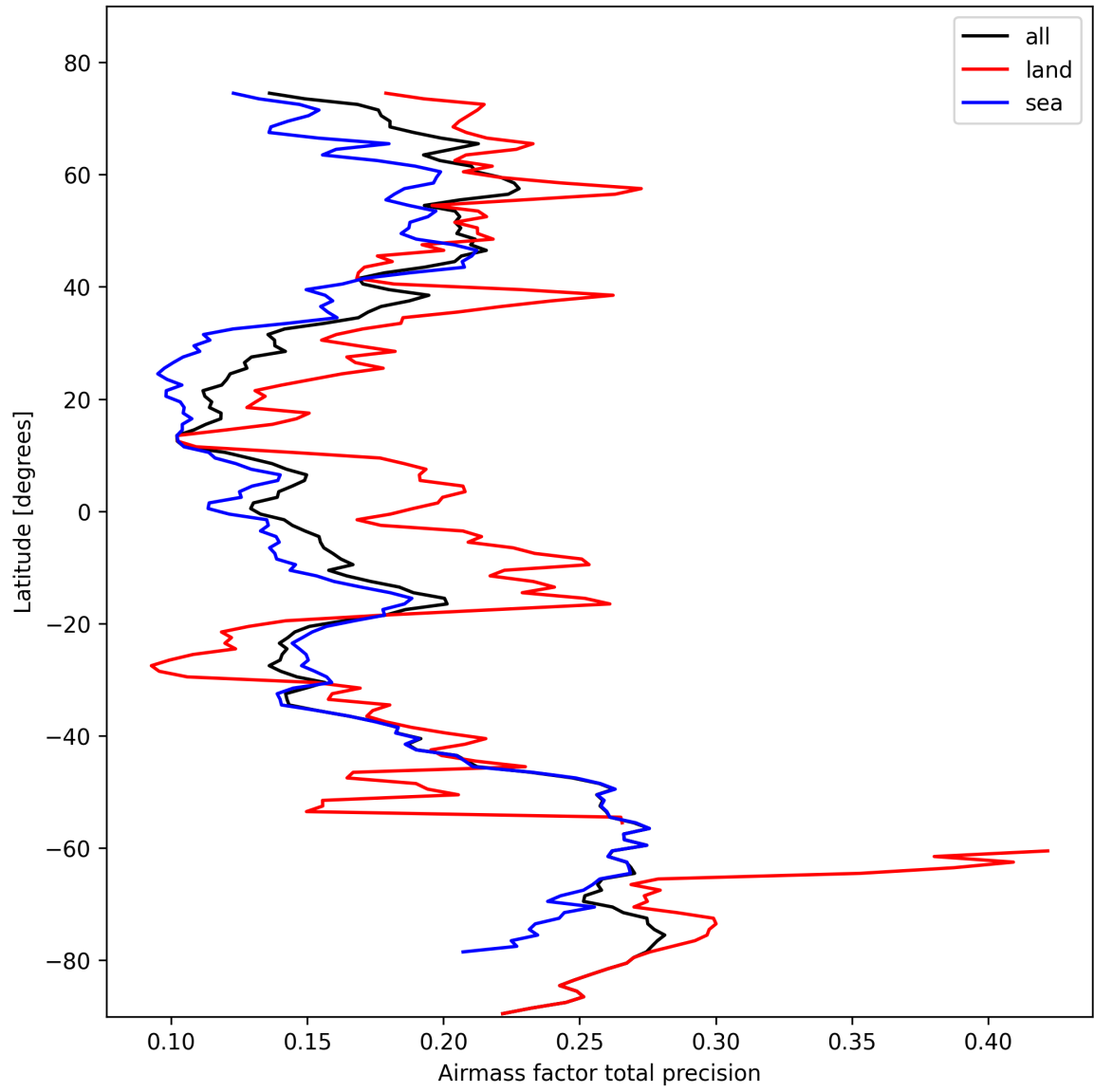
Figure 25: Zonal average of “Airmass factor total precision” for 2025-10-21 to 2025-10-22.
