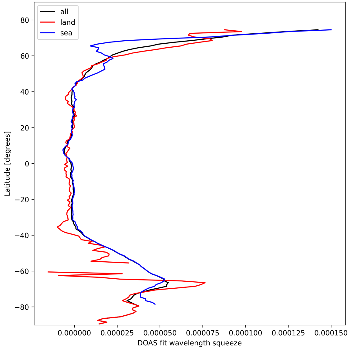
Figure 29: Zonal average of “DOAS fit wavelength squeeze” for 2025-10-21 to 2025-10-22.
