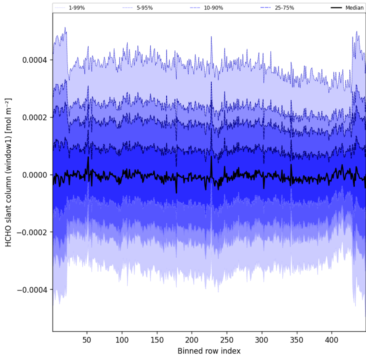
Figure 50: Along track statistics of “HCHO slant column (window1)” for 2025-10-21 to 2025-10-22
