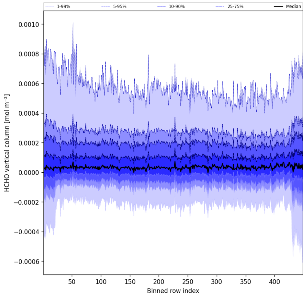
Figure 47: Along track statistics of “HCHO vertical column” for 2025-10-21 to 2025-10-22
