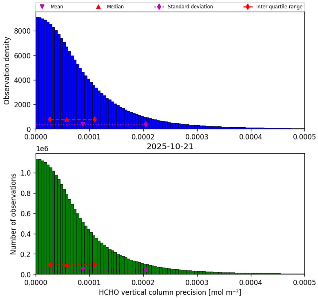
Figure 34: Histogram of “HCHO vertical column precision” for 2025-10-21 to 2025-10-22
