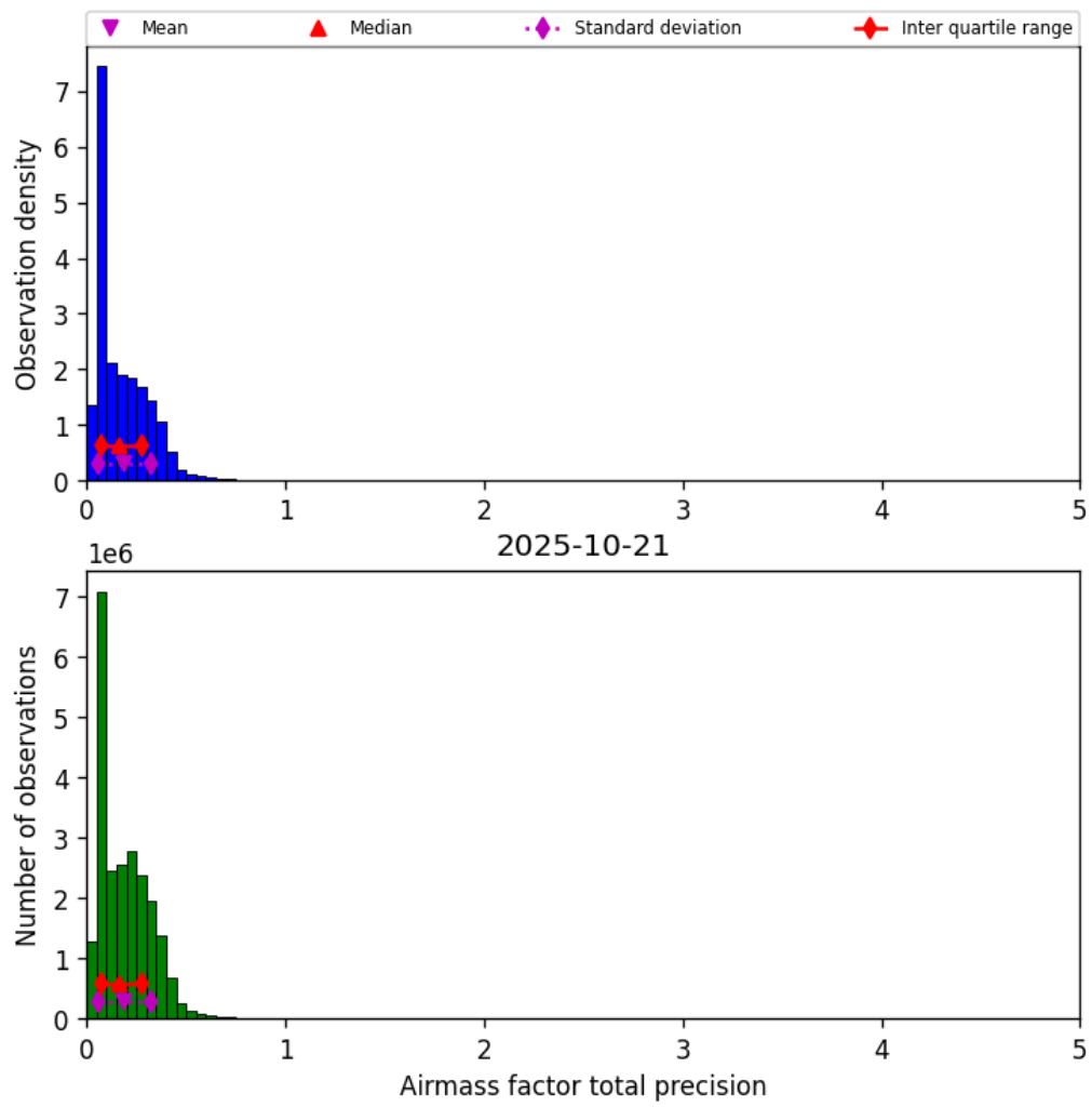
Figure 39: Histogram of “Airmass factor total precision” for 2025-10-21 to 2025-10-22
