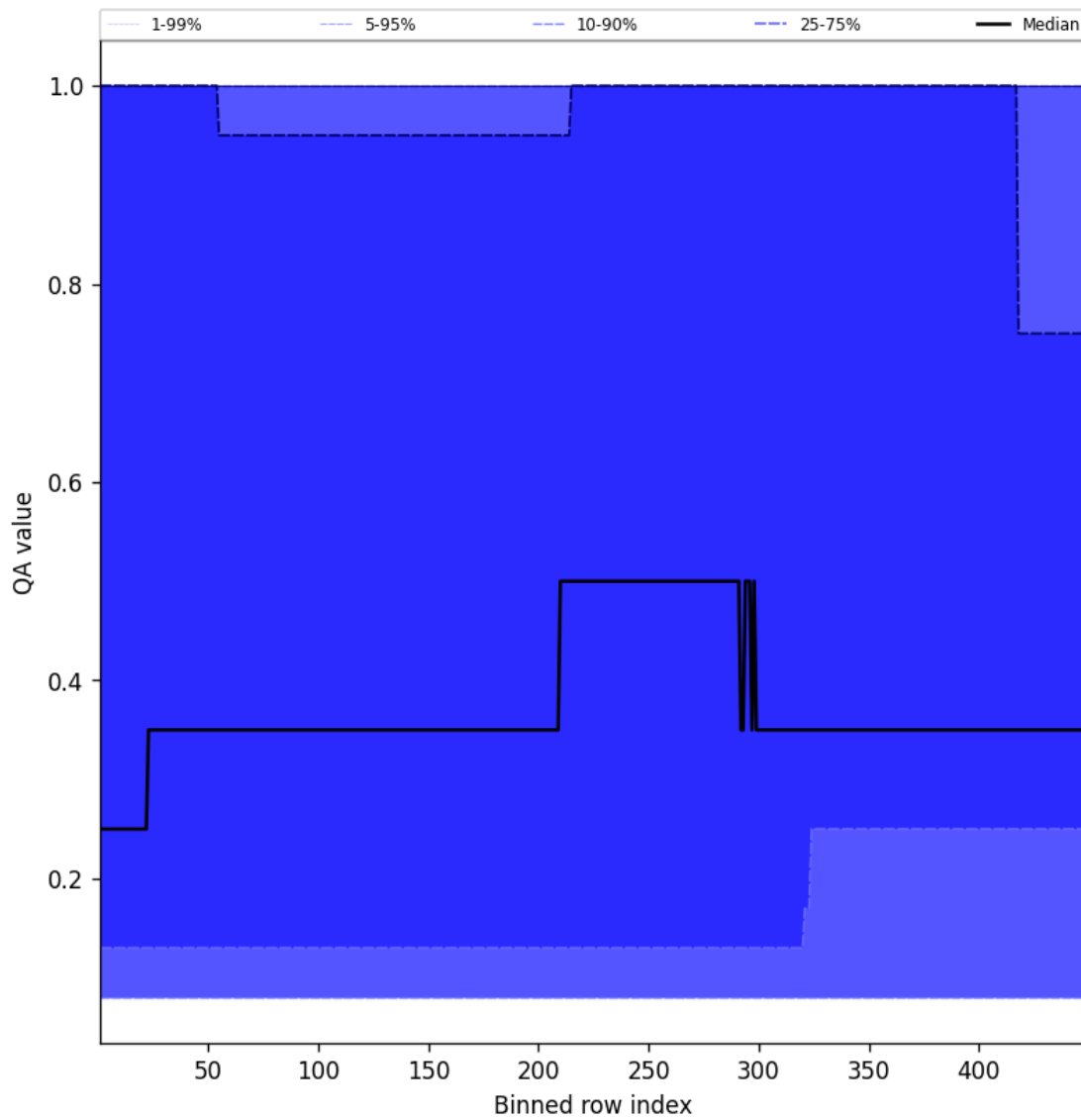
Figure 46: Along track statistics of “QA value” for 2025-10-21 to 2025-10-22
