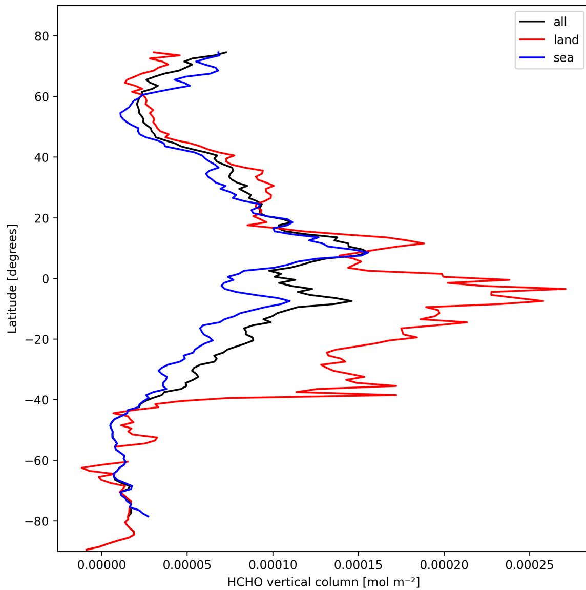
Figure 19: Zonal average of “HCHO vertical column” for 2025-10-21 to 2025-10-22.
