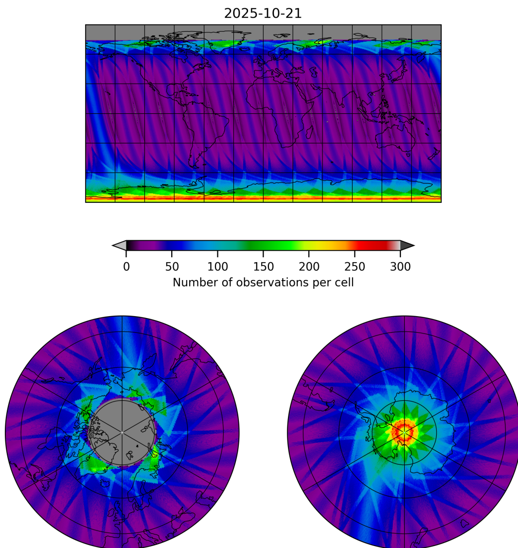
Figure 17: Map of the number of observations for 2025-10-21 to 2025-10-22
