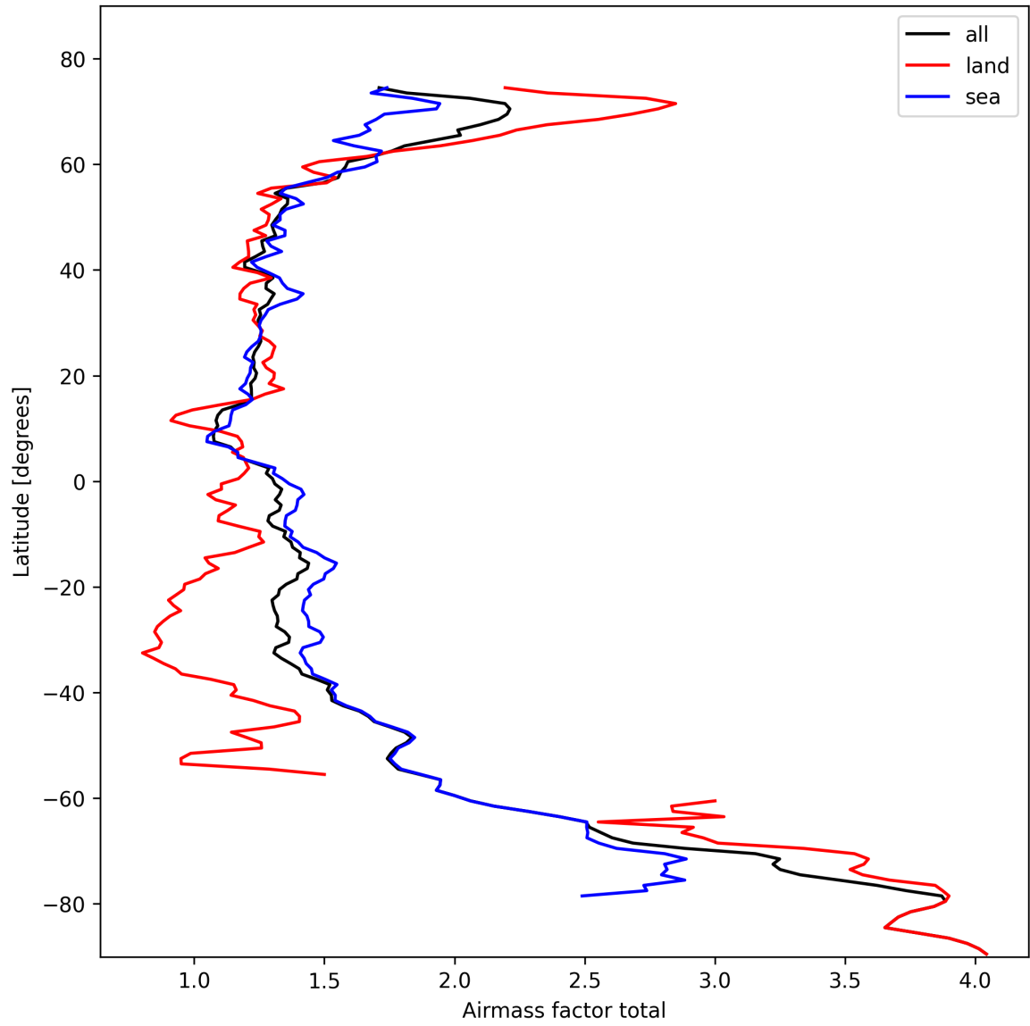
Figure 24: Zonal average of “Airmass factor total” for 2025-10-21 to 2025-10-22.
