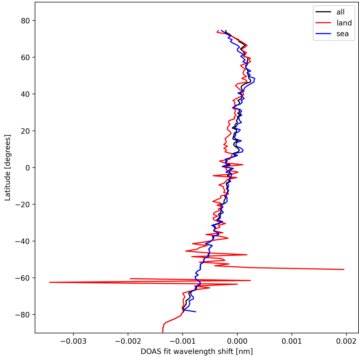
Figure 28: Zonal average of “DOAS fit wavelength shift” for 2025-10-21 to 2025-10-22.
