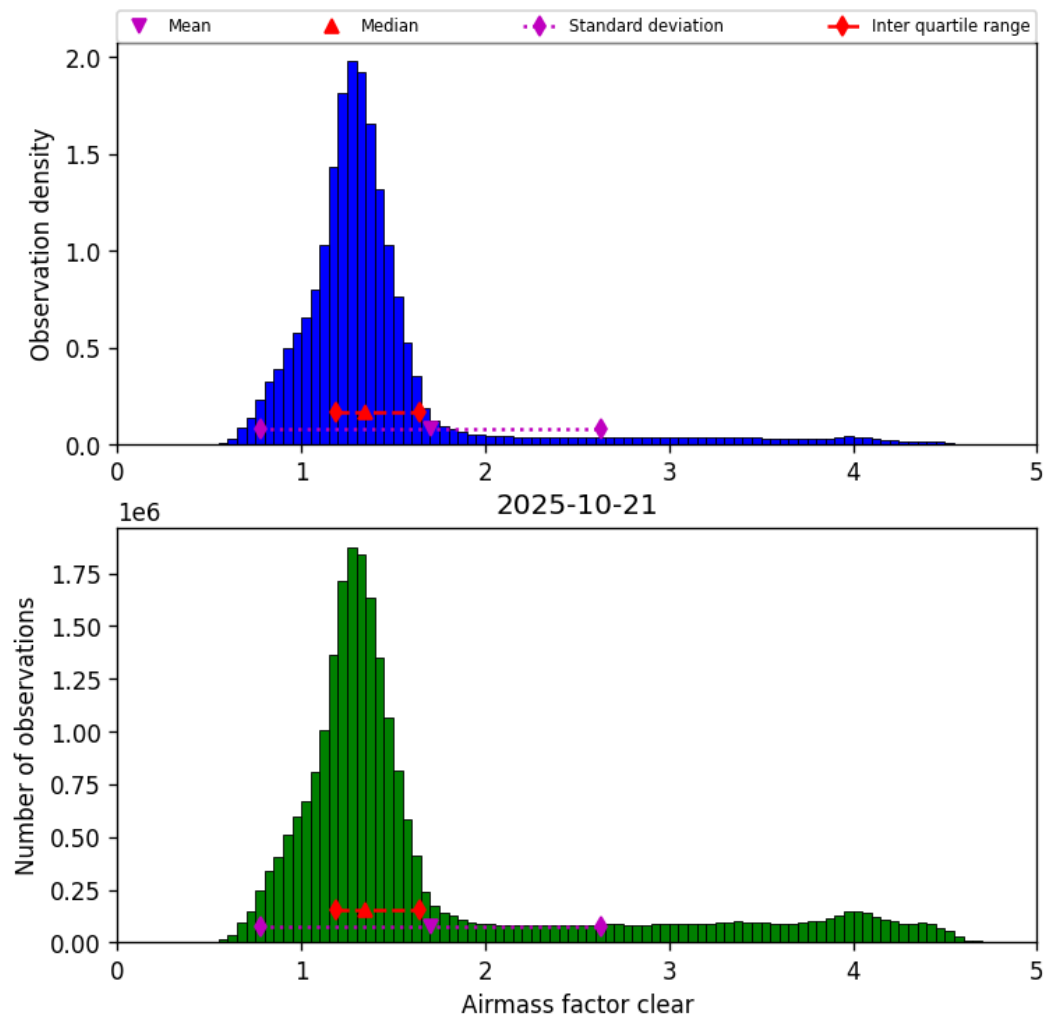
Figure 40: Histogram of “Airmass factor clear” for 2025-10-21 to 2025-10-22
