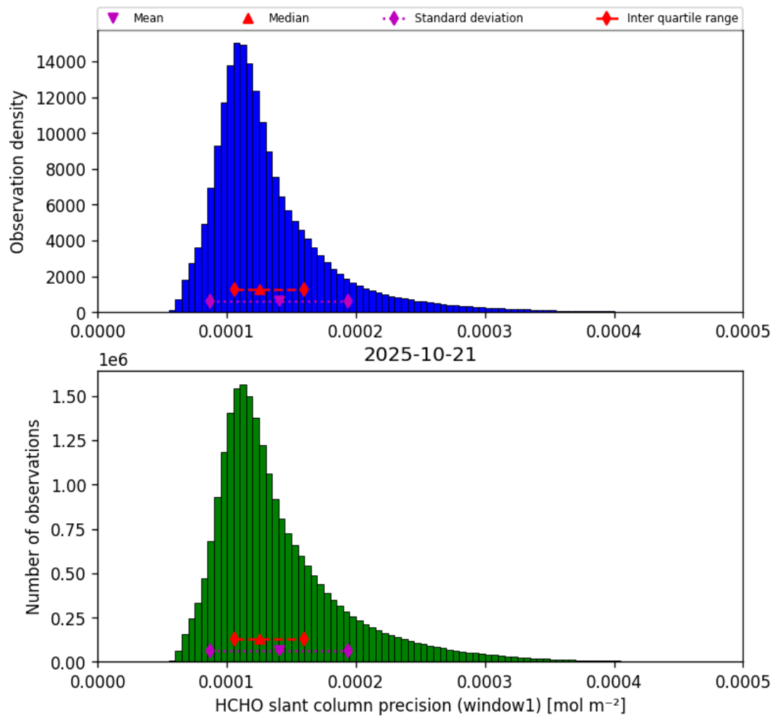
Figure 37: Histogram of “HCHO slant column precision (window1)” for 2025-10-21 to 2025-10-22
