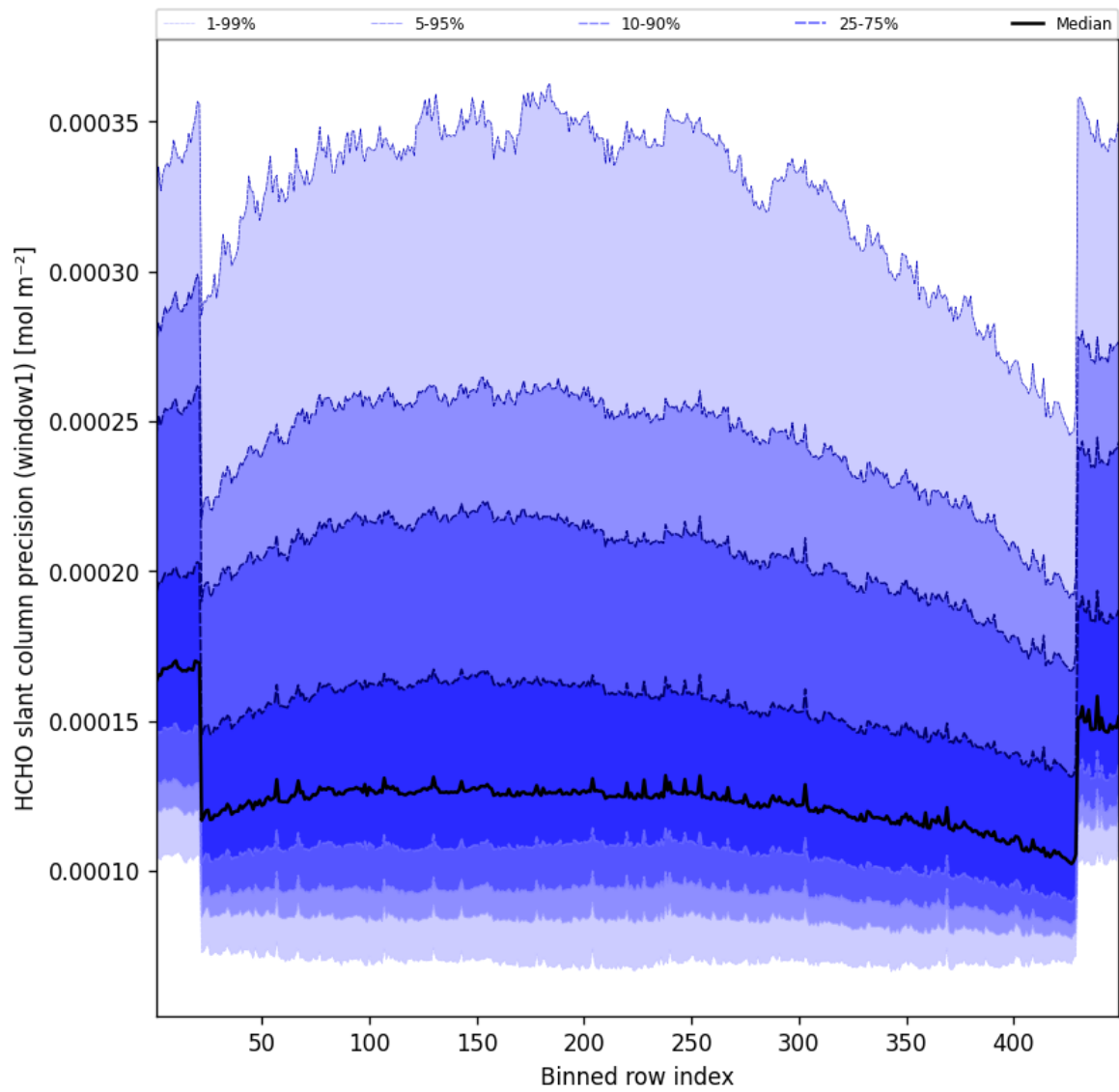
Figure 51: Along track statistics of “HCHO slant column precision (window1)” for 2025-10-21 to 2025-10-22
