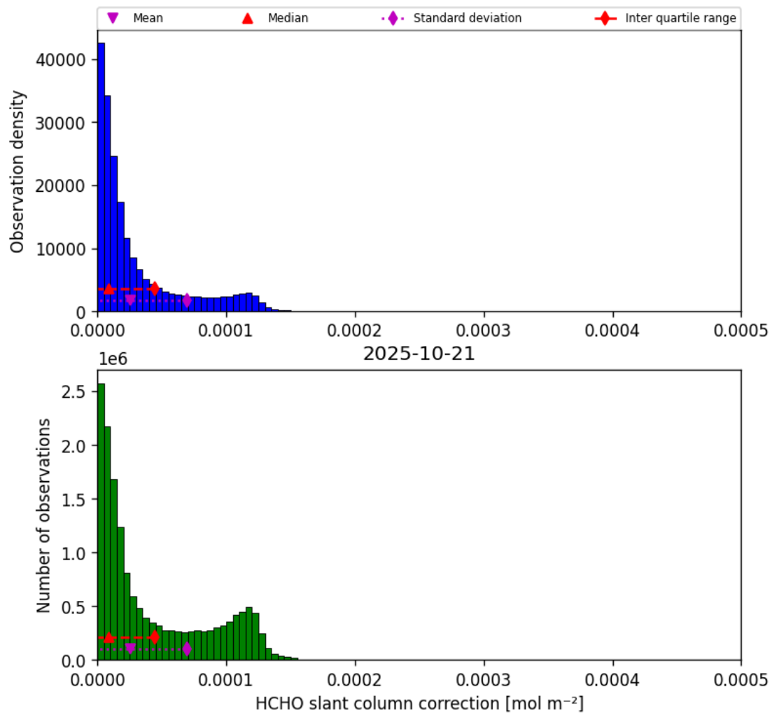
Figure 45: Histogram of “HCHO slant column correction” for 2025-10-21 to 2025-10-22
