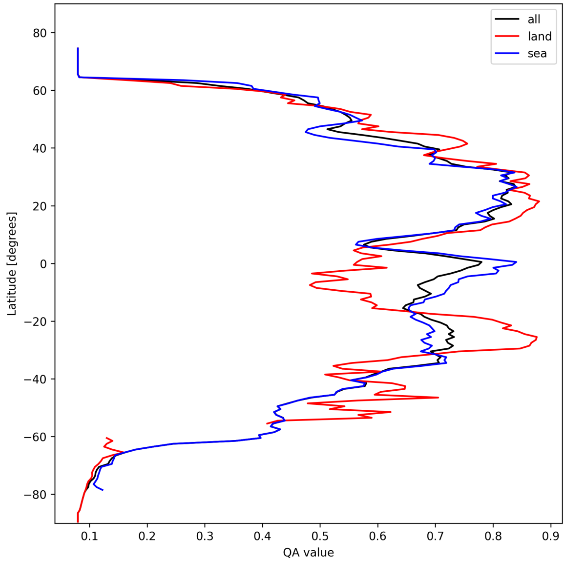
Figure 18: Zonal average of “QA value” for 2025-10-21 to 2025-10-22.
