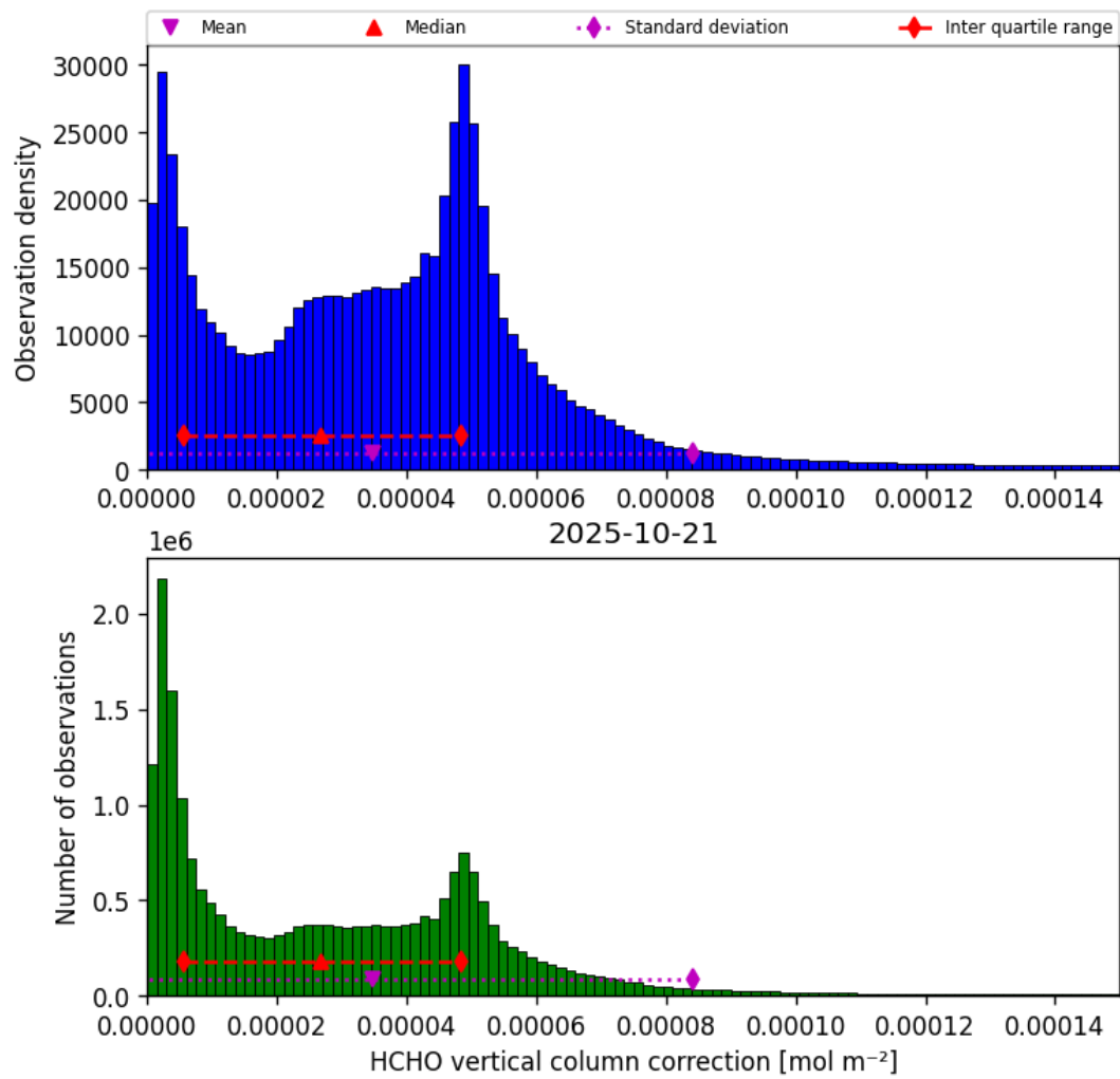
Figure 35: Histogram of “HCHO vertical column correction” for 2025-10-21 to 2025-10-22
