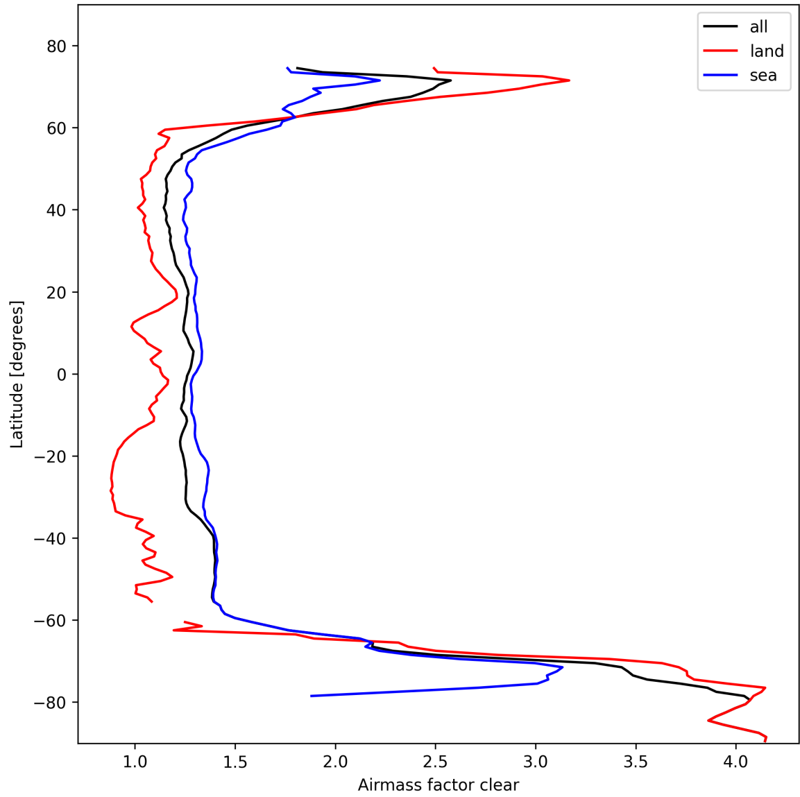
Figure 26: Zonal average of “Airmass factor clear” for 2025-10-21 to 2025-10-22.
