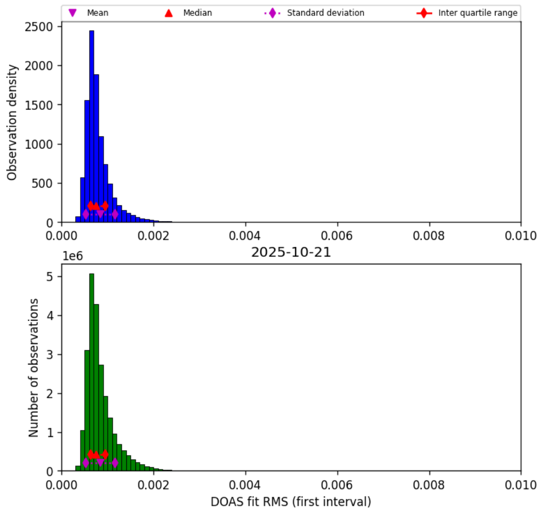
Figure 44: Histogram of “DOAS fit RMS (first interval)” for 2025-10-21 to 2025-10-22
