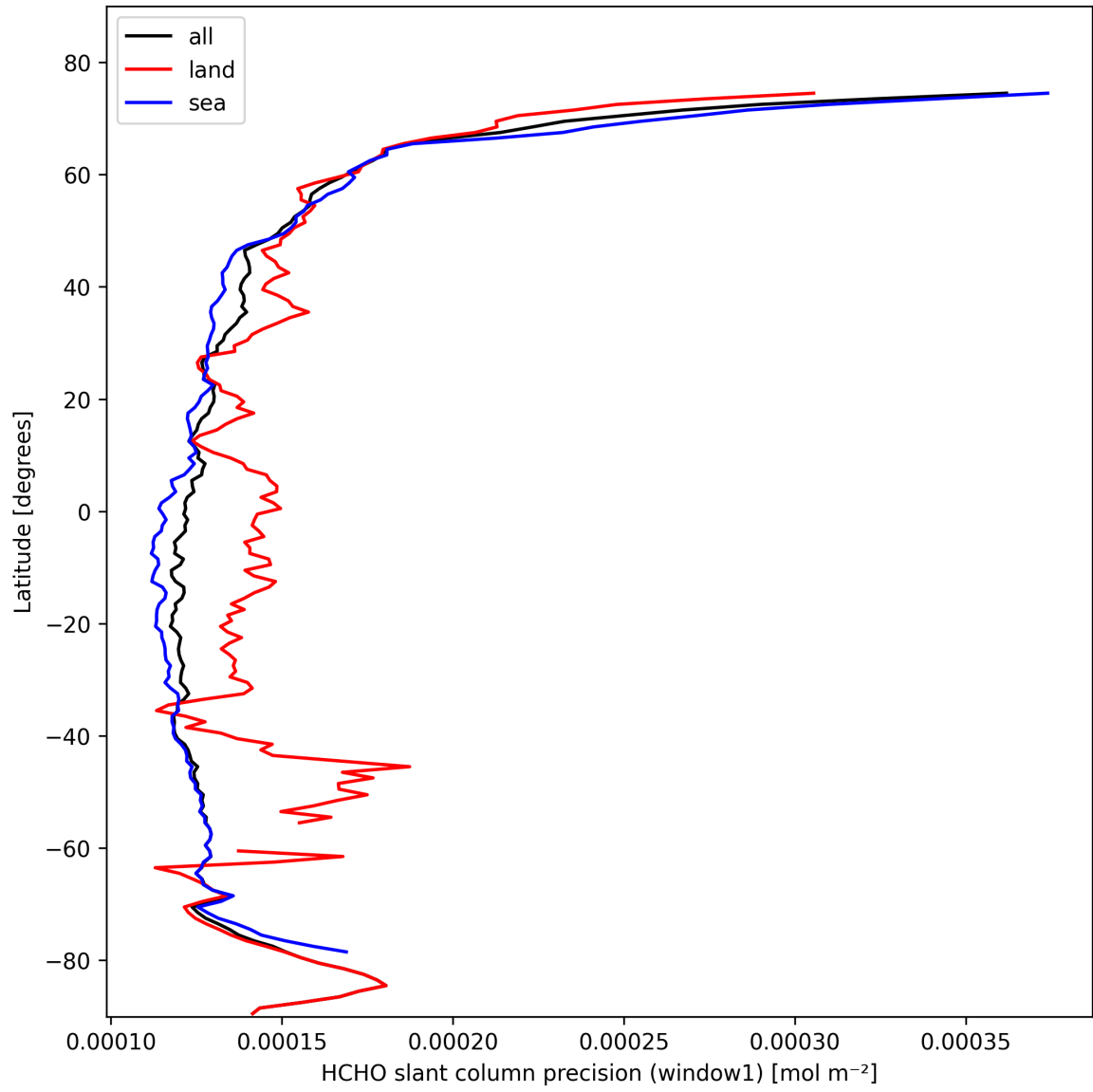
Figure 23: Zonal average of "HCHO slant column precision (window1)" for 2025-10-21 to 2025-10-22.
