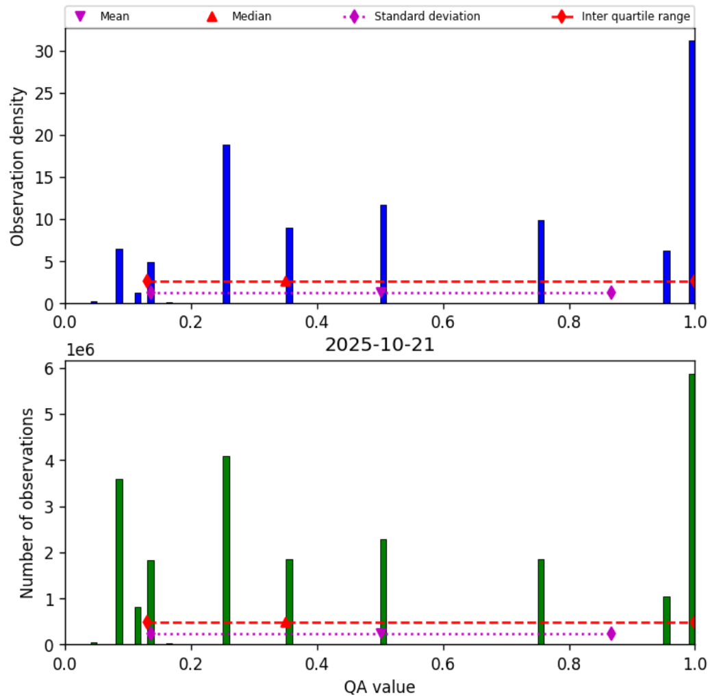
Figure 32: Histogram of “QA value” for 2025-10-21 to 2025-10-22
