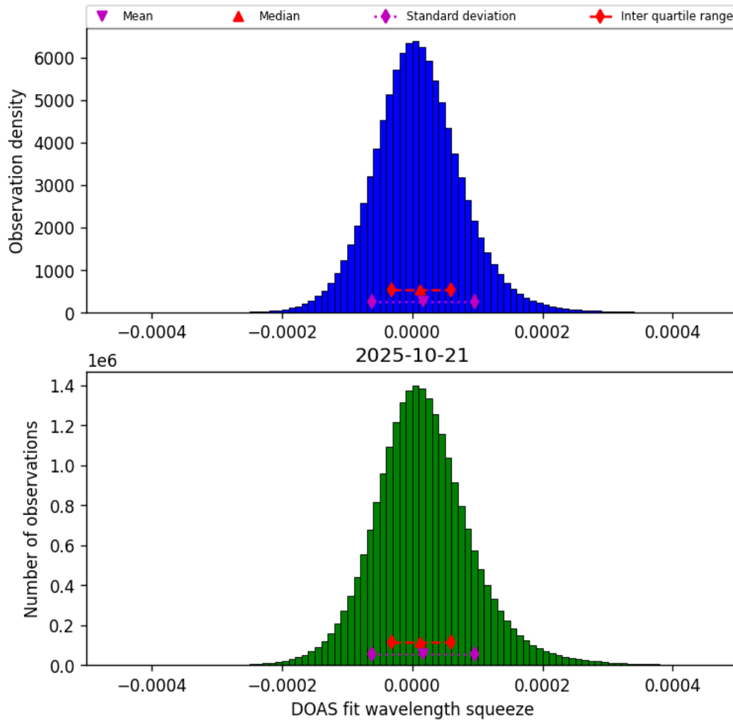
Figure 43: Histogram of “DOAS fit wavelength squeeze” for 2025-10-21 to 2025-10-22
