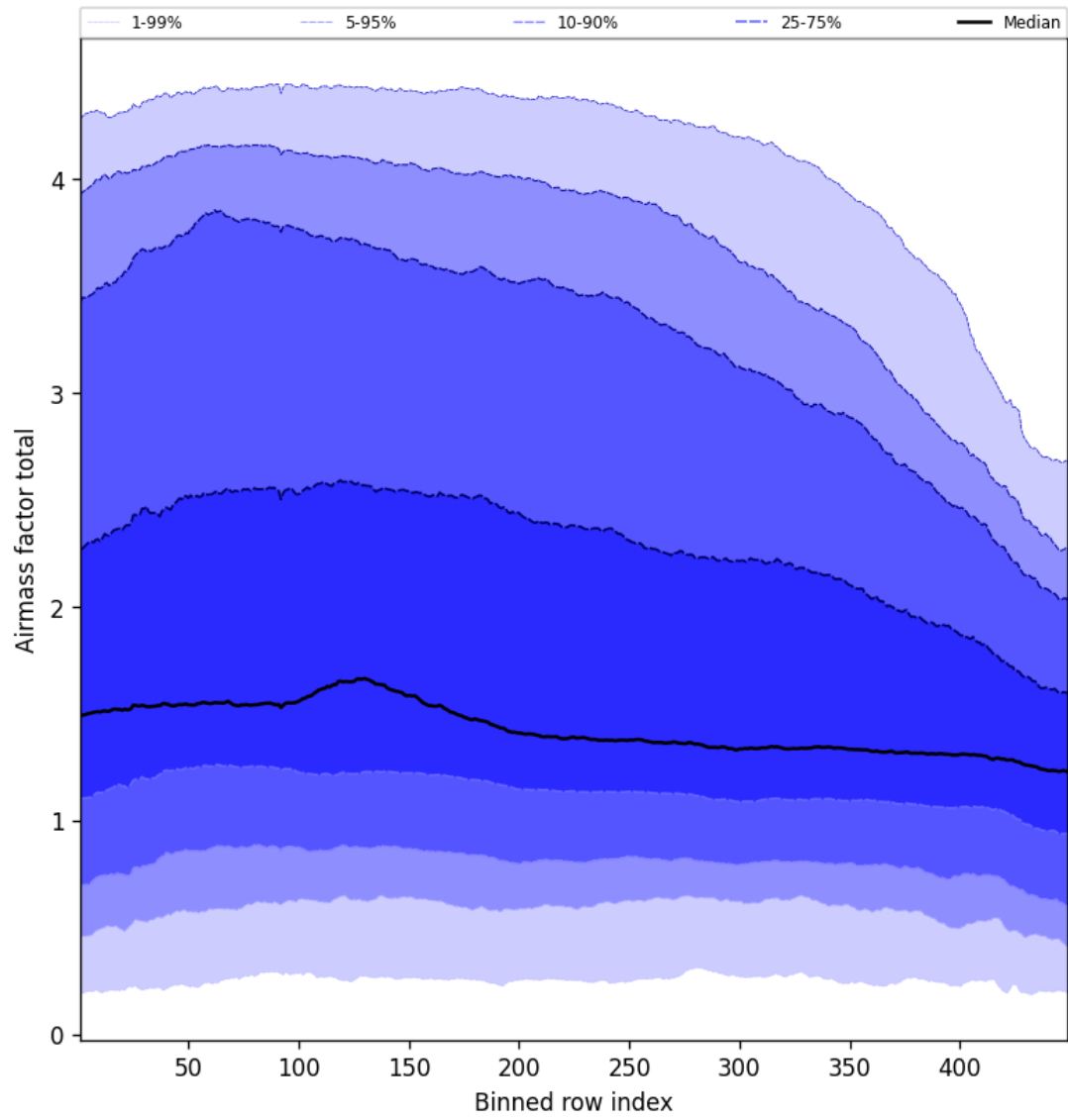
Figure 52: Along track statistics of “Airmass factor total” for 2025-10-21 to 2025-10-22
