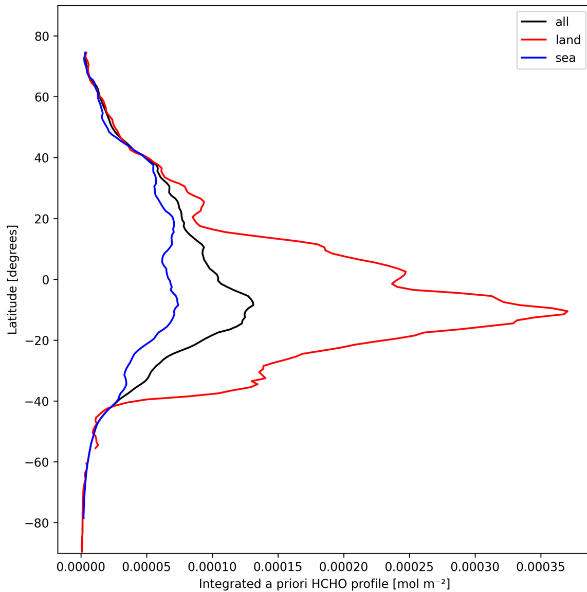
Figure 27: Zonal average of “Integrated a priori HCHO profile” for 2025-10-21 to 2025-10-22.
