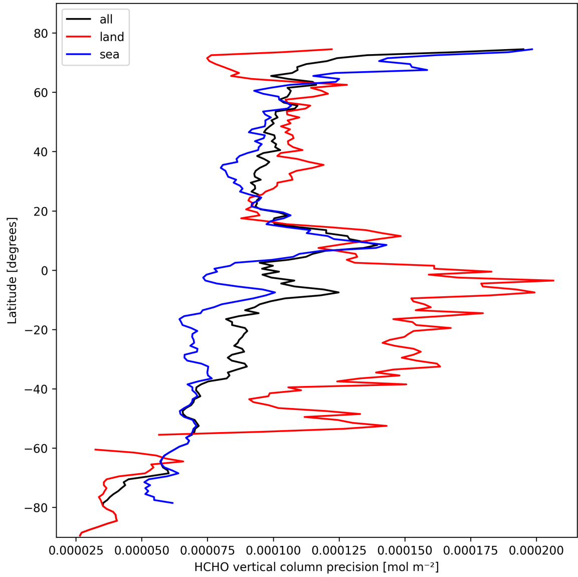
Figure 20: Zonal average of “HCHO vertical column precision” for 2025-10-21 to 2025-10-22.
