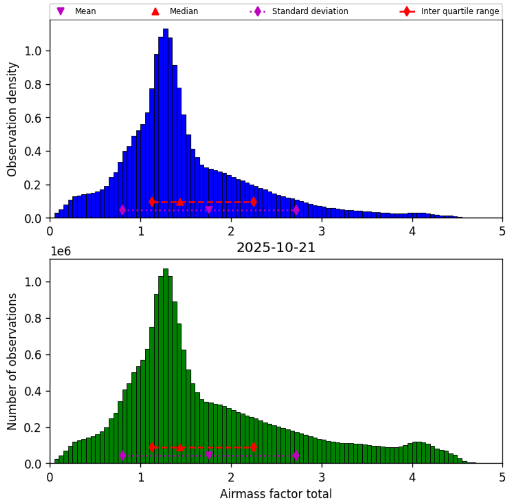
Figure 38: Histogram of “Airmass factor total” for 2025-10-21 to 2025-10-22
