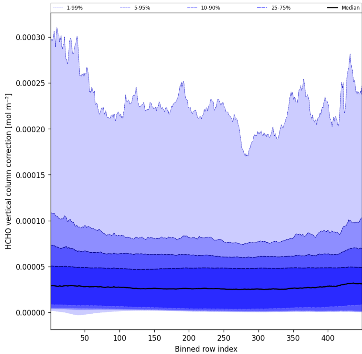
Figure 49: Along track statistics of “HCHO vertical column correction” for 2025-10-21 to 2025-10-22
