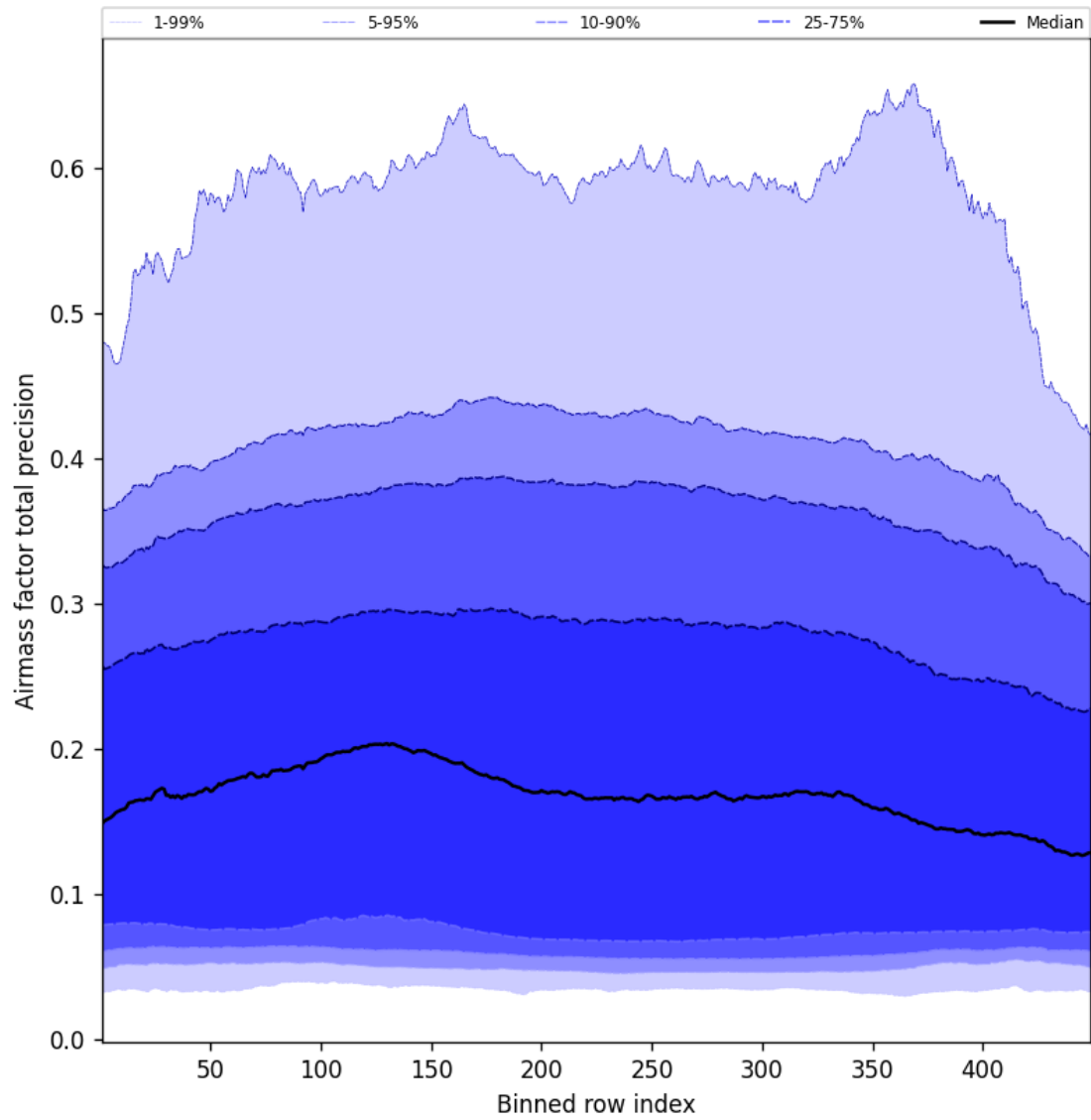
Figure 53: Along track statistics of “Airmass factor total precision” for 2025-10-21 to 2025-10-22
