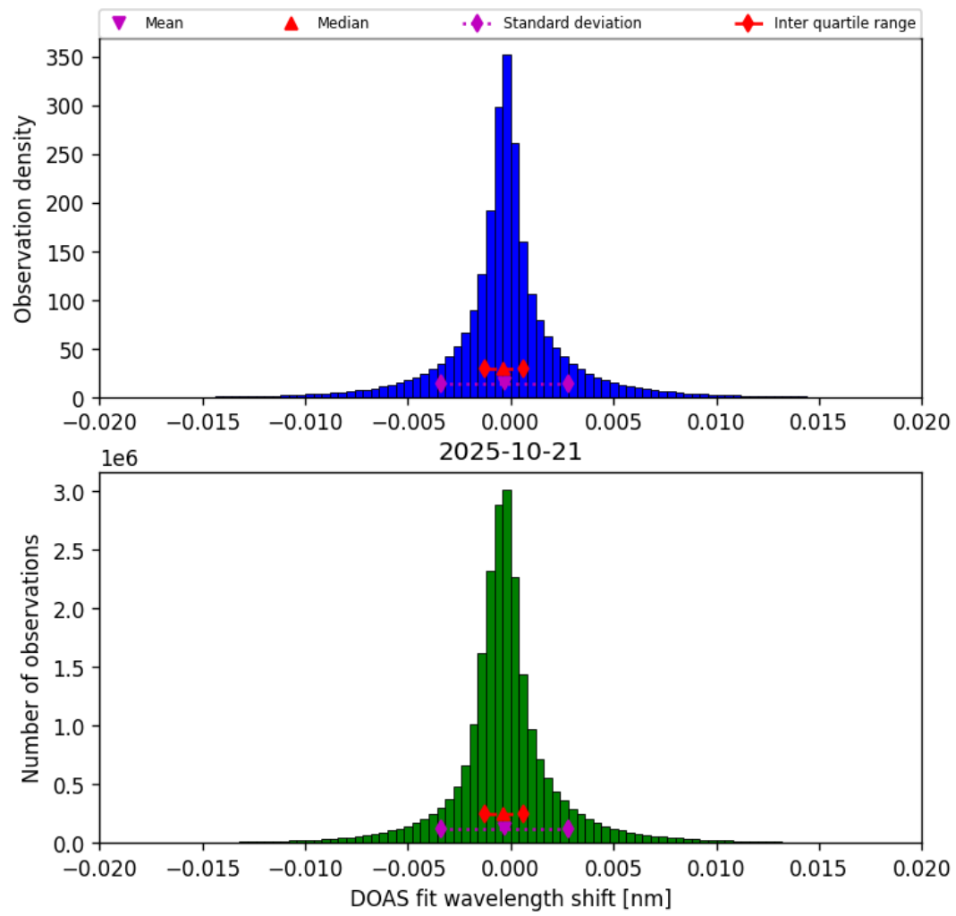
Figure 42: Histogram of “DOAS fit wavelength shift” for 2025-10-21 to 2025-10-22
