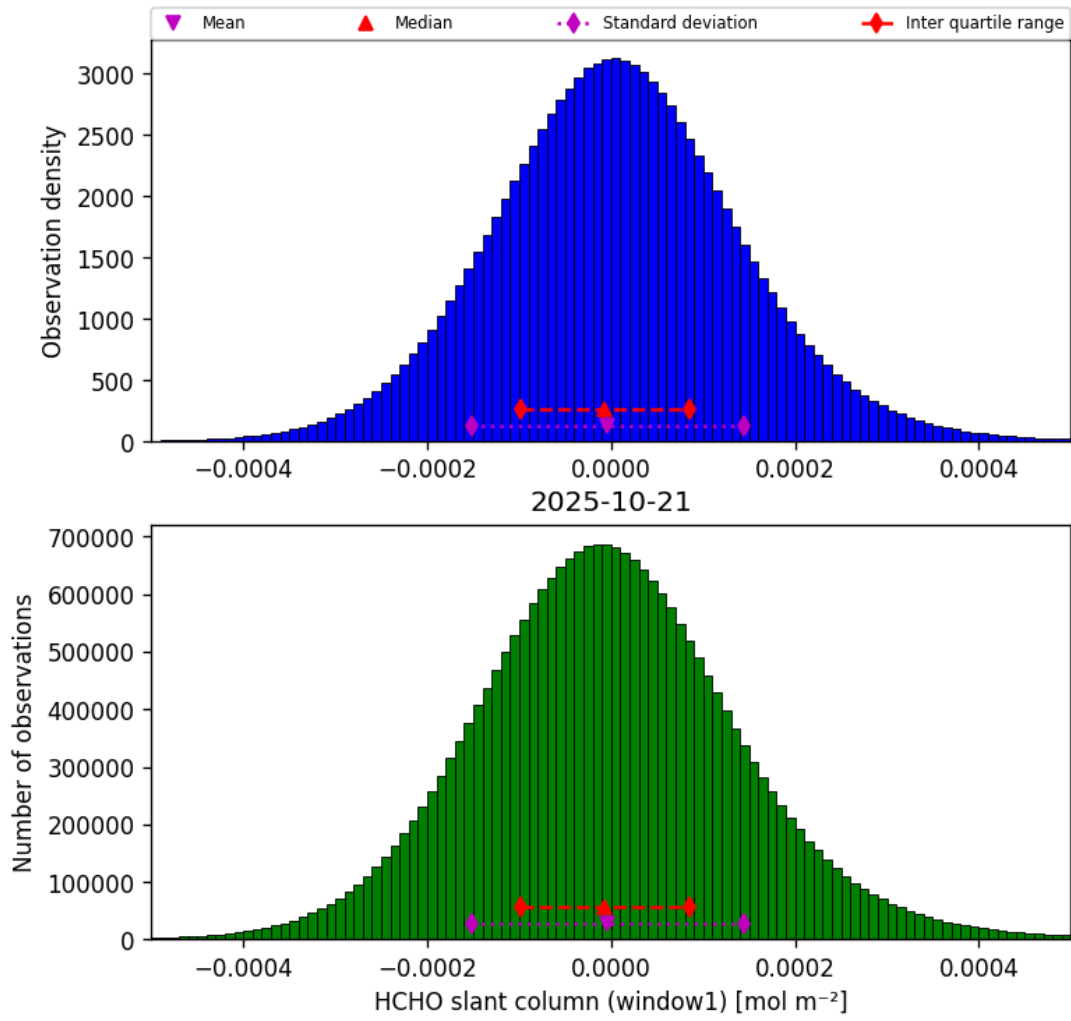
Figure 36: Histogram of “HCHO slant column (window1)” for 2025-10-21 to 2025-10-22
