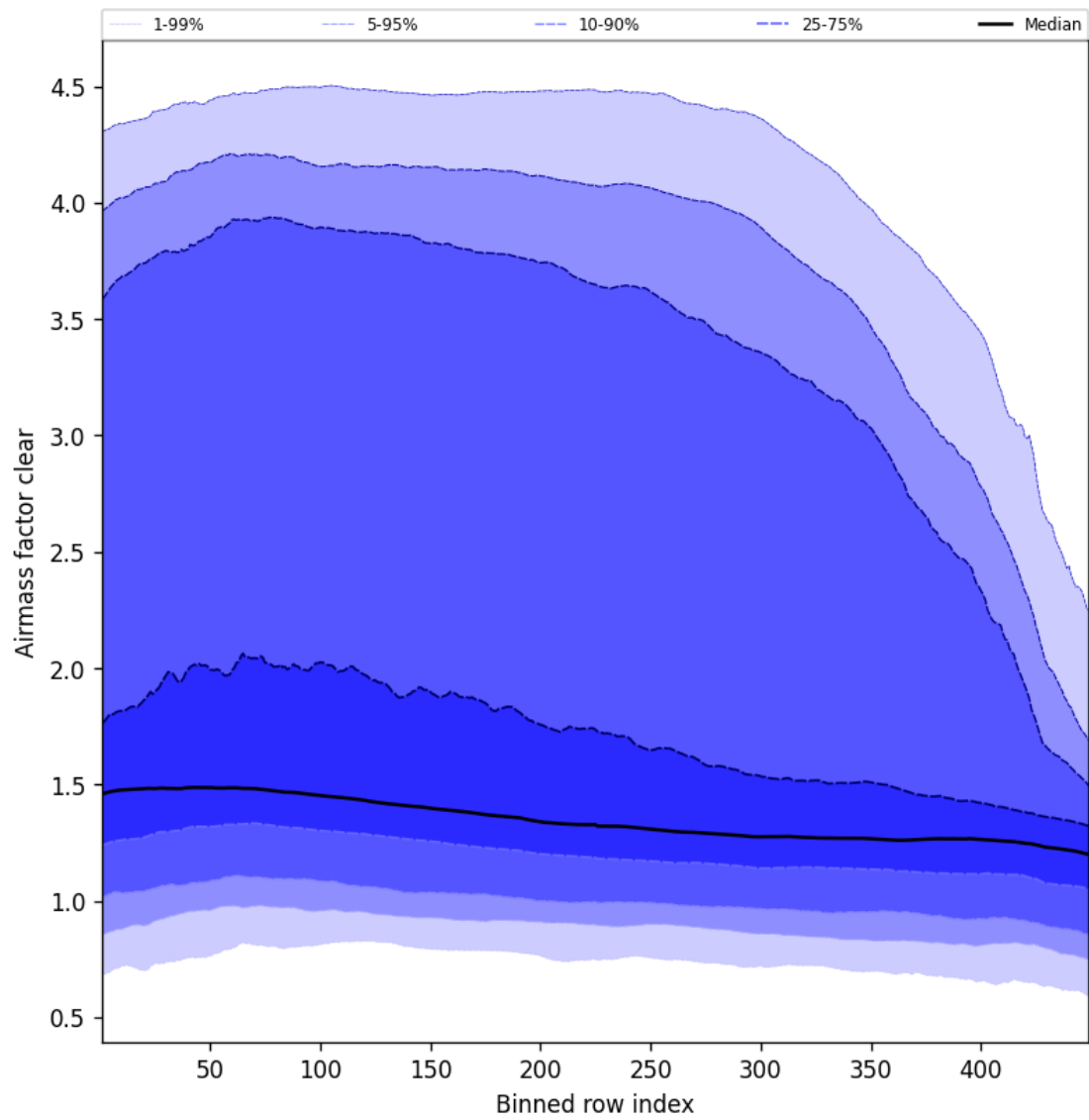
Figure 54: Along track statistics of “Airmass factor clear” for 2025-10-21 to 2025-10-22
