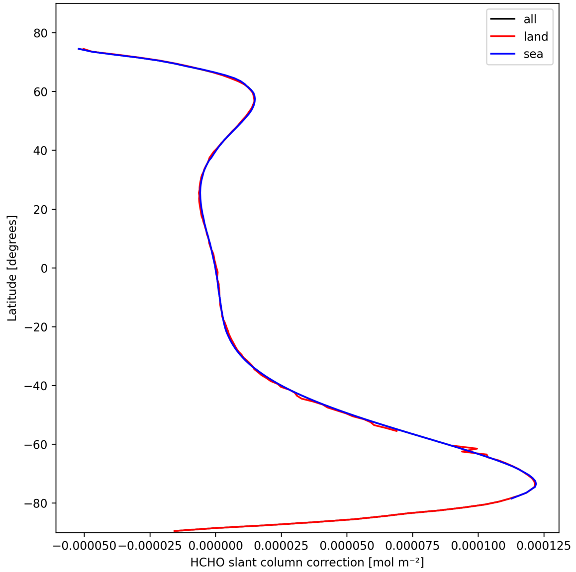
Figure 31: Zonal average of “HCHO slant column correction” for 2025-10-21 to 2025-10-22.
