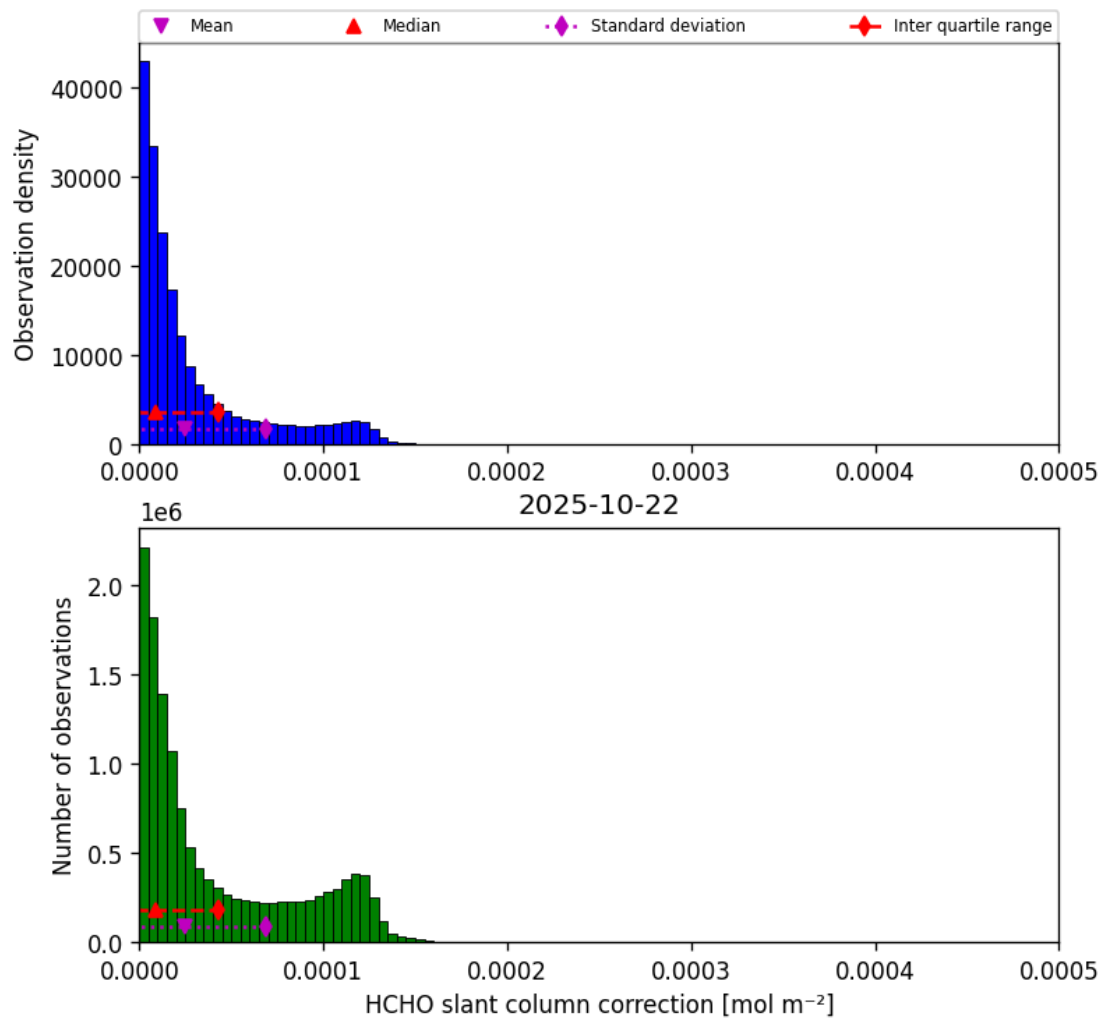
Figure 45: Histogram of “HCHO slant column correction” for 2025-10-22 to 2025-10-23
