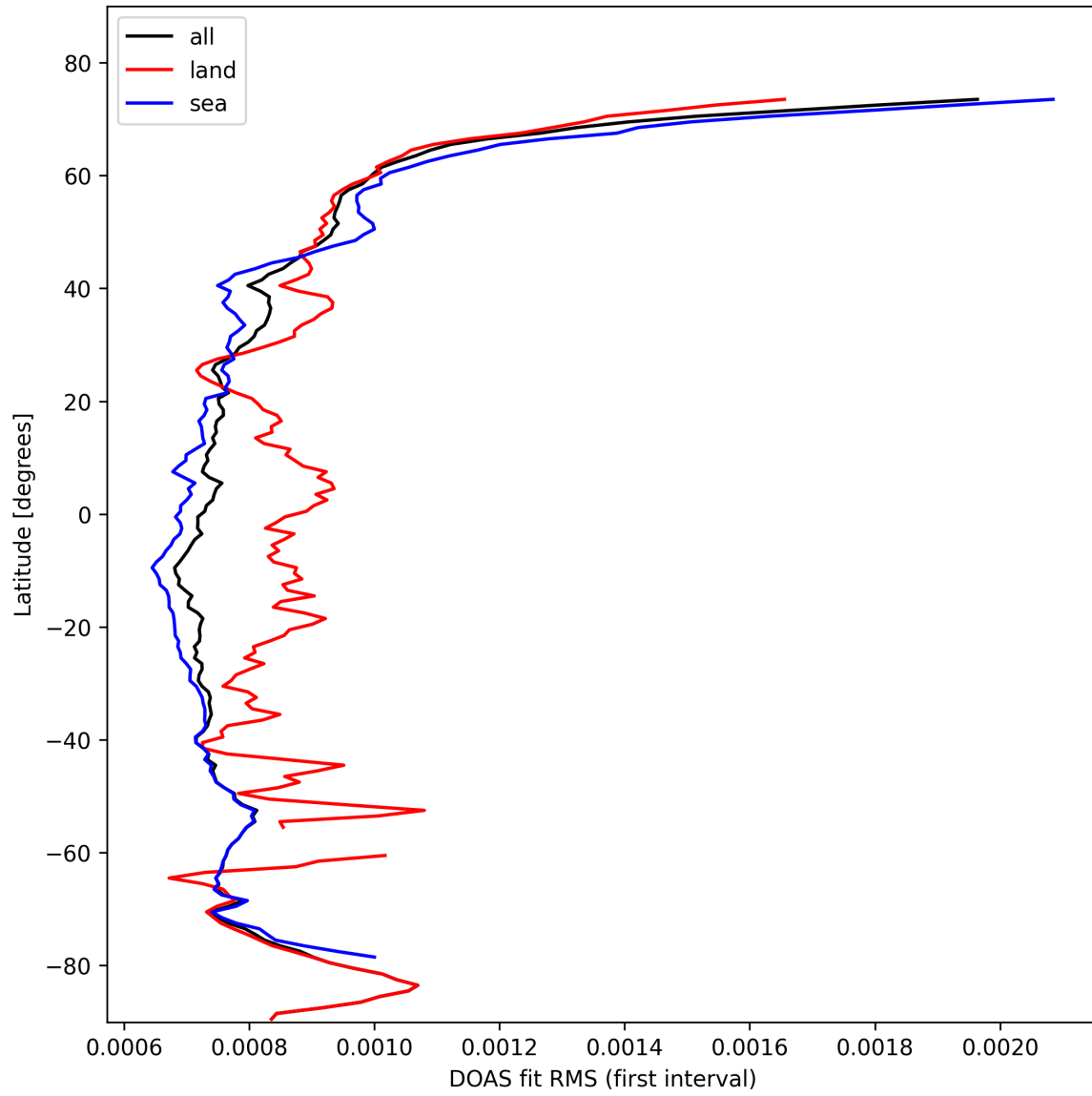
Figure 30: Zonal average of “DOAS fit RMS (first interval)” for 2025-10-22 to 2025-10-23.
