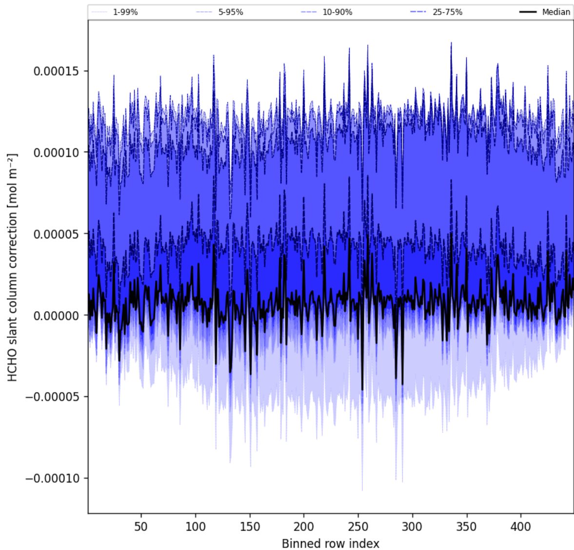
Figure 59: Along track statistics of “HCHO slant column correction” for 2025-10-22 to 2025-10-23
