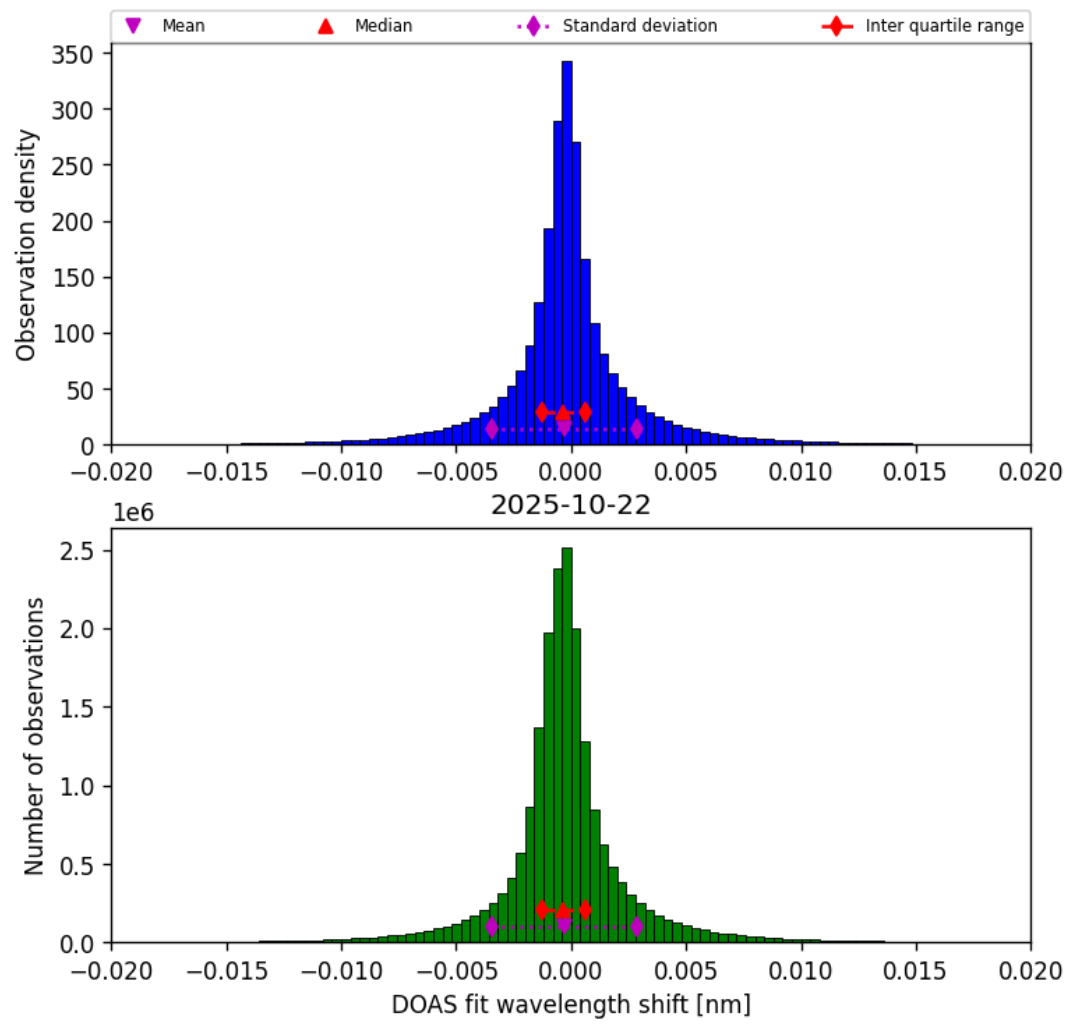
Figure 42: Histogram of “DOAS fit wavelength shift” for 2025-10-22 to 2025-10-23
