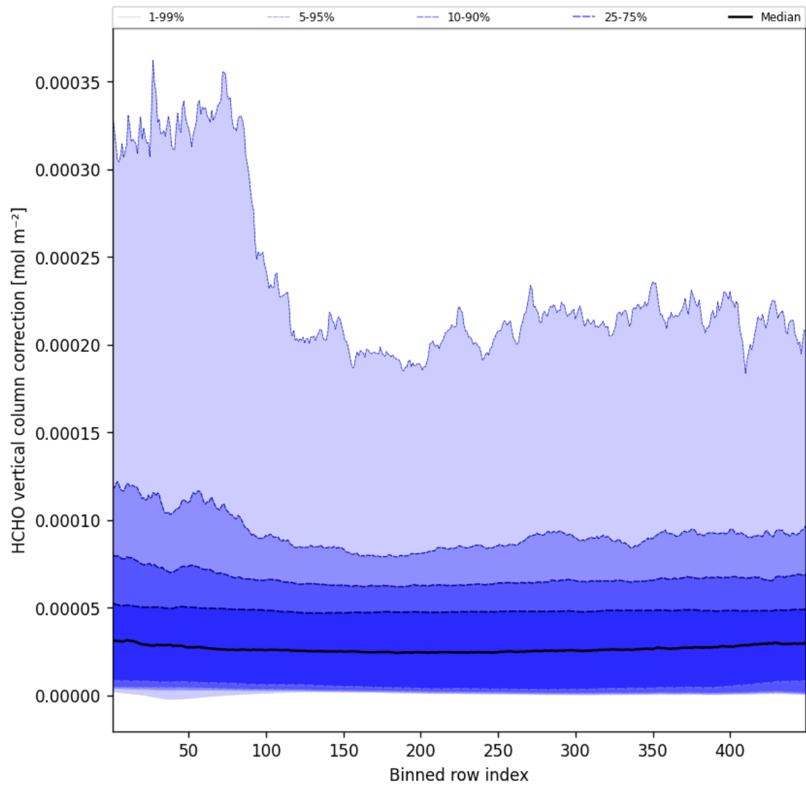
Figure 49: Along track statistics of “HCHO vertical column correction” for 2025-10-22 to 2025-10-23
