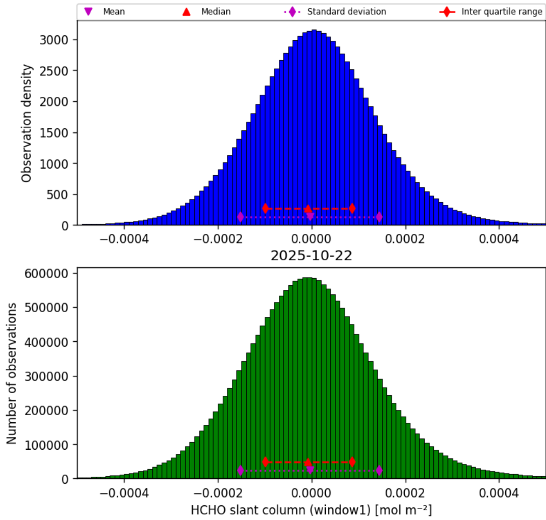
Figure 36: Histogram of “HCHO slant column (window1)” for 2025-10-22 to 2025-10-23
