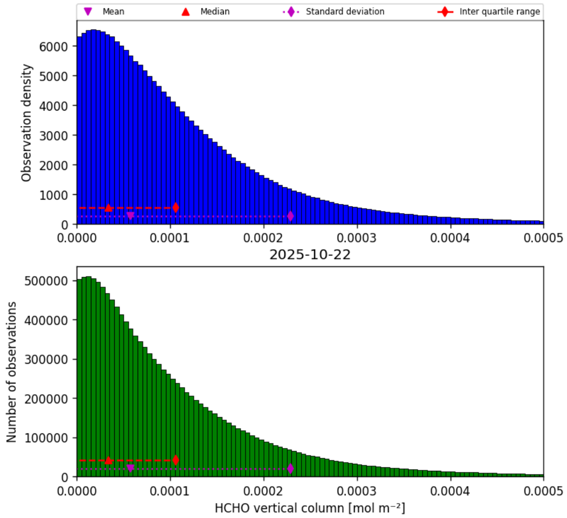
Figure 33: Histogram of “HCHO vertical column” for 2025-10-22 to 2025-10-23
