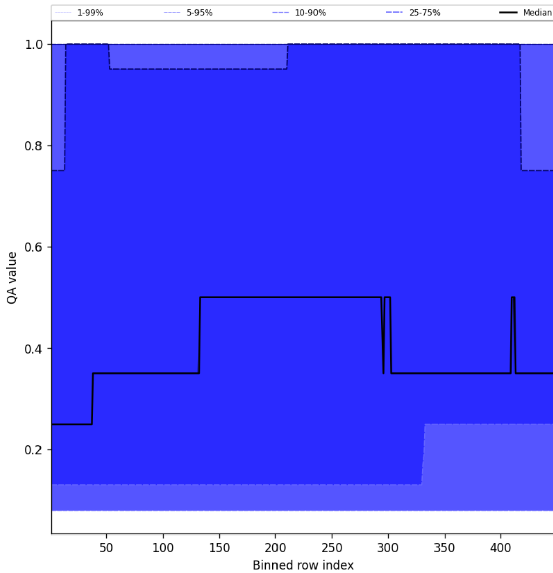
Figure 46: Along track statistics of "QA value" for 2025-10-22 to 2025-10-23
