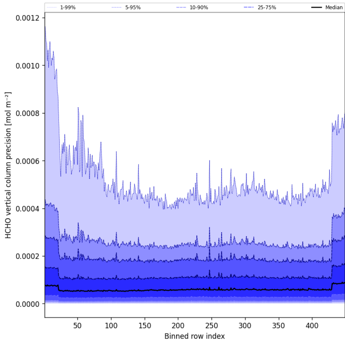
Figure 48: Along track statistics of “HCHO vertical column precision” for 2025-10-22 to 2025-10-23
