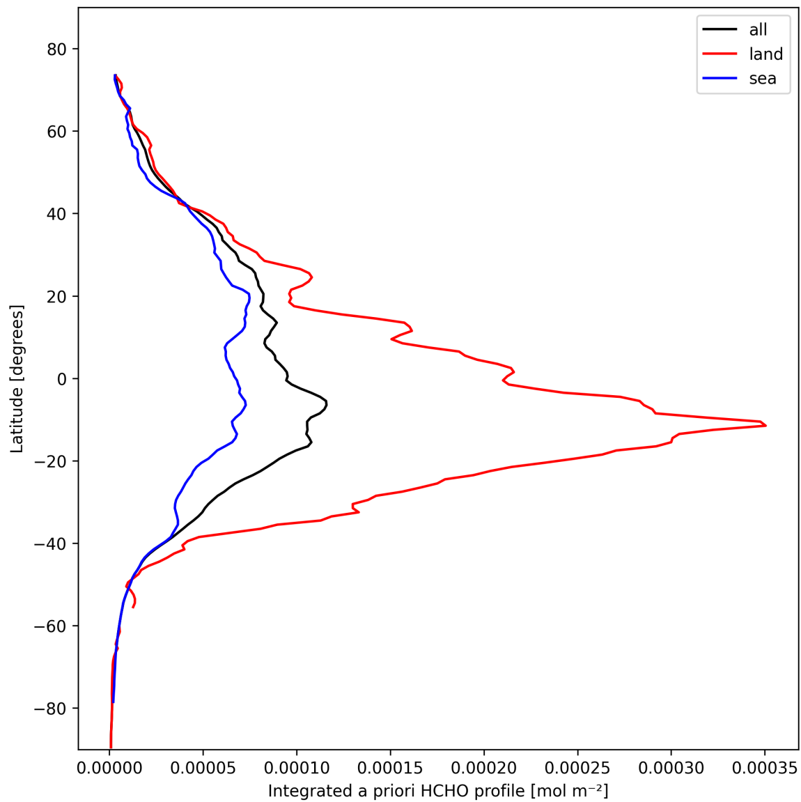
Figure 27: Zonal average of “Integrated a priori HCHO profile” for 2025-10-22 to 2025-10-23.
