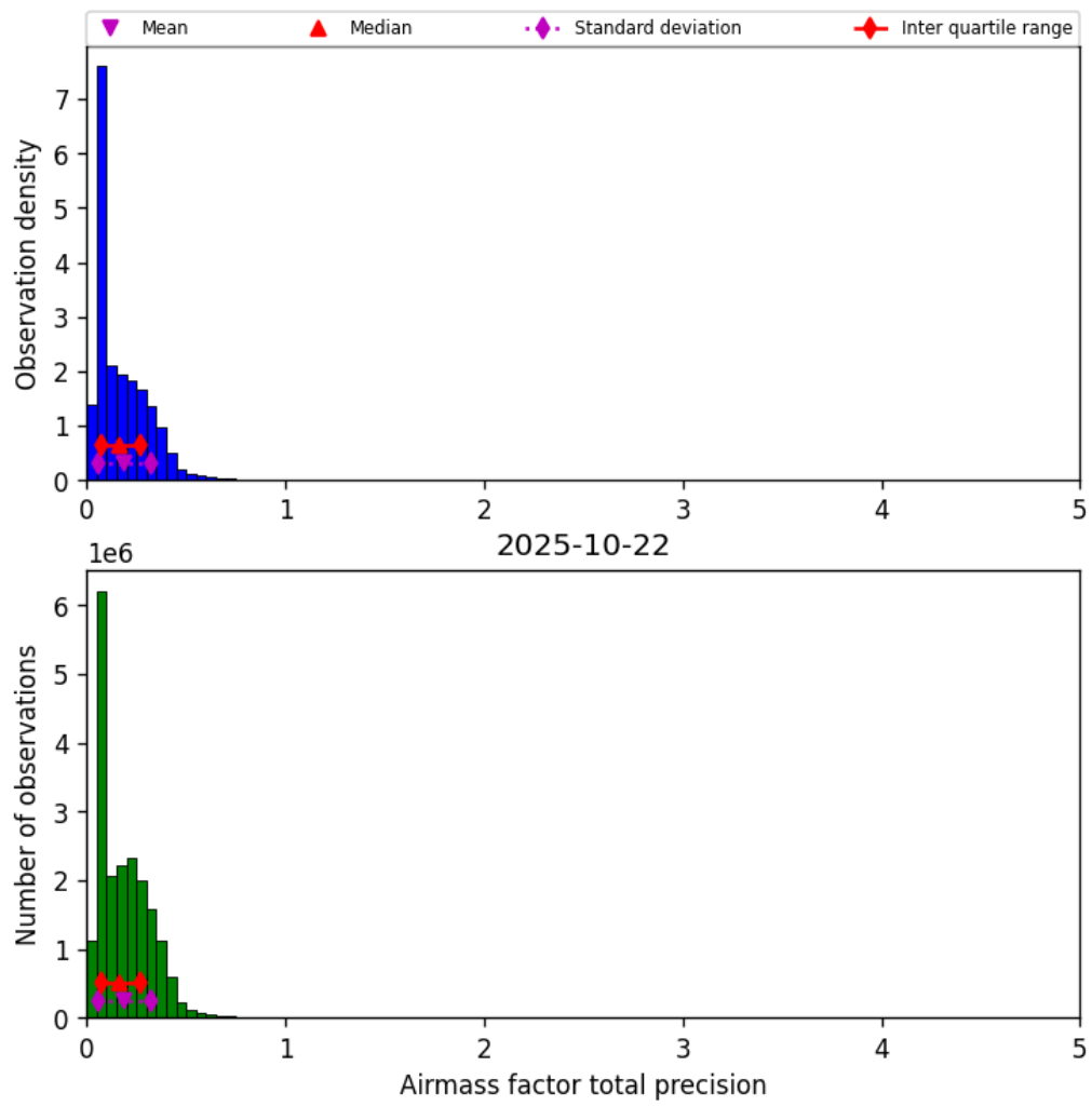
Figure 39: Histogram of “Airmass factor total precision” for 2025-10-22 to 2025-10-23
