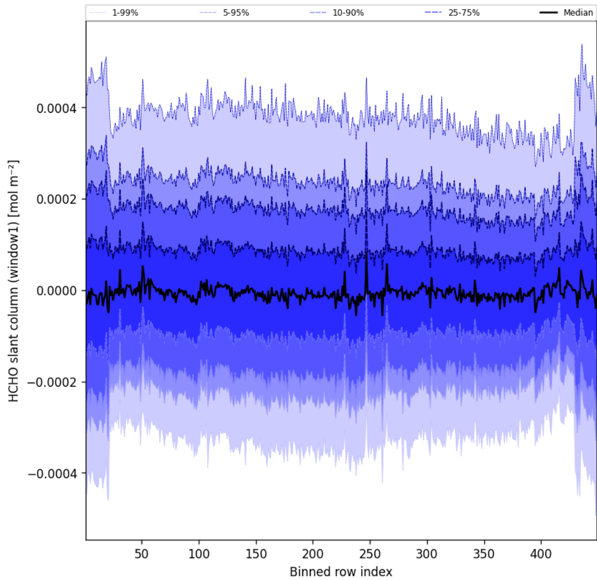
Figure 50: Along track statistics of “HCHO slant column (window1)” for 2025-10-22 to 2025-10-23
