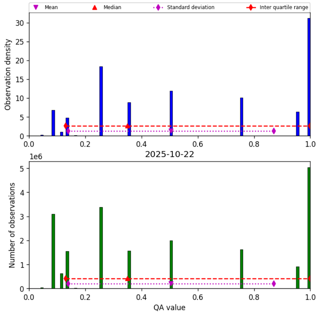
Figure 32: Histogram of “QA value” for 2025-10-22 to 2025-10-23
