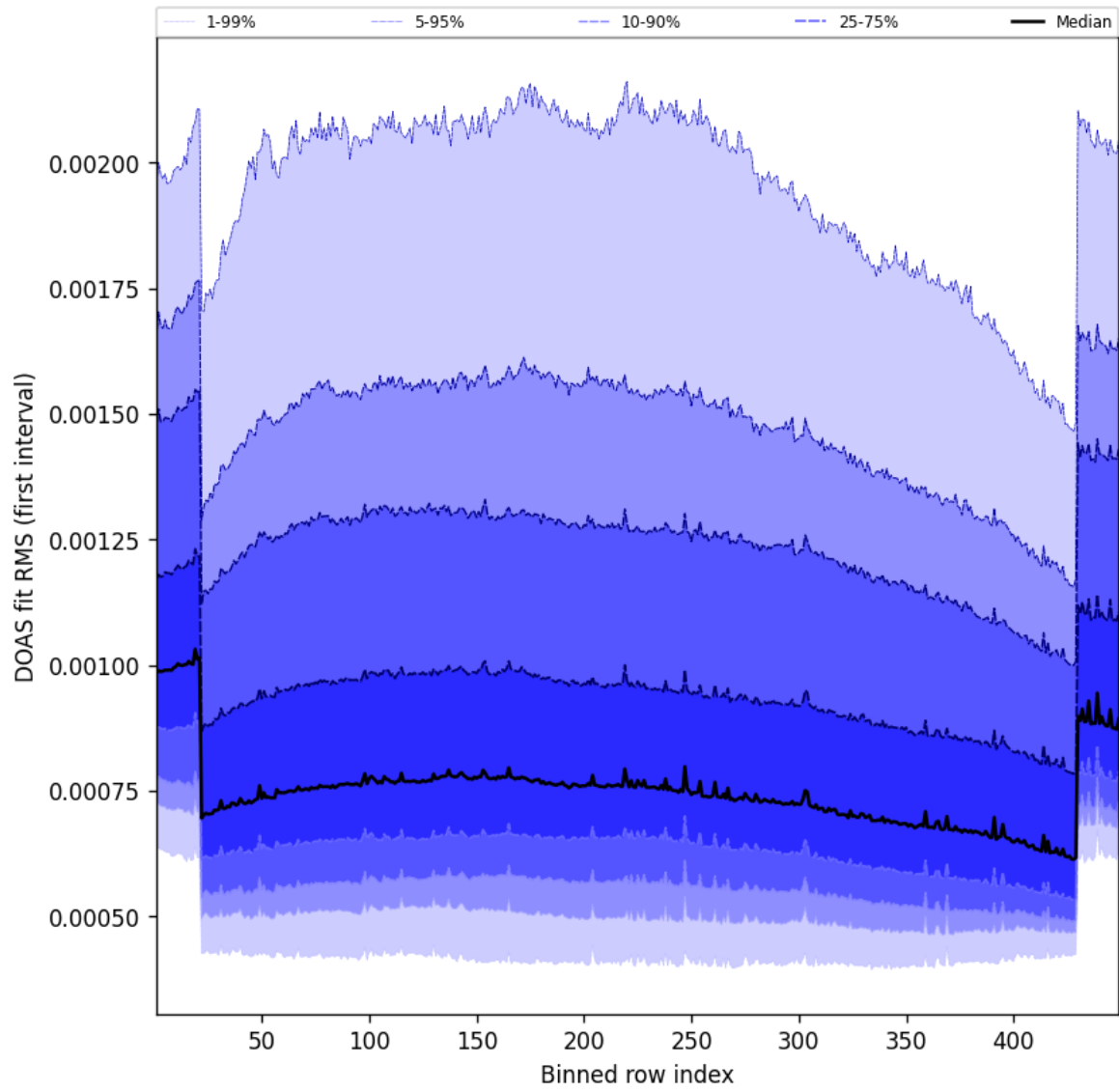
Figure 58: Along track statistics of “DOAS fit RMS (first interval)” for 2025-10-22 to 2025-10-23
