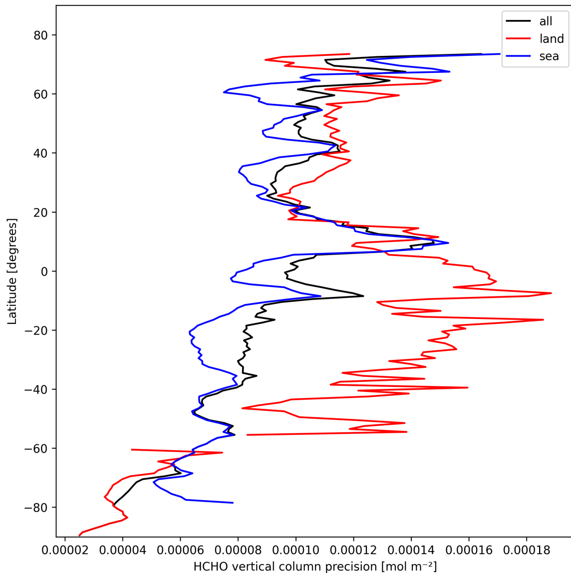
Figure 20: Zonal average of “HCHO vertical column precision” for 2025-10-22 to 2025-10-23.
