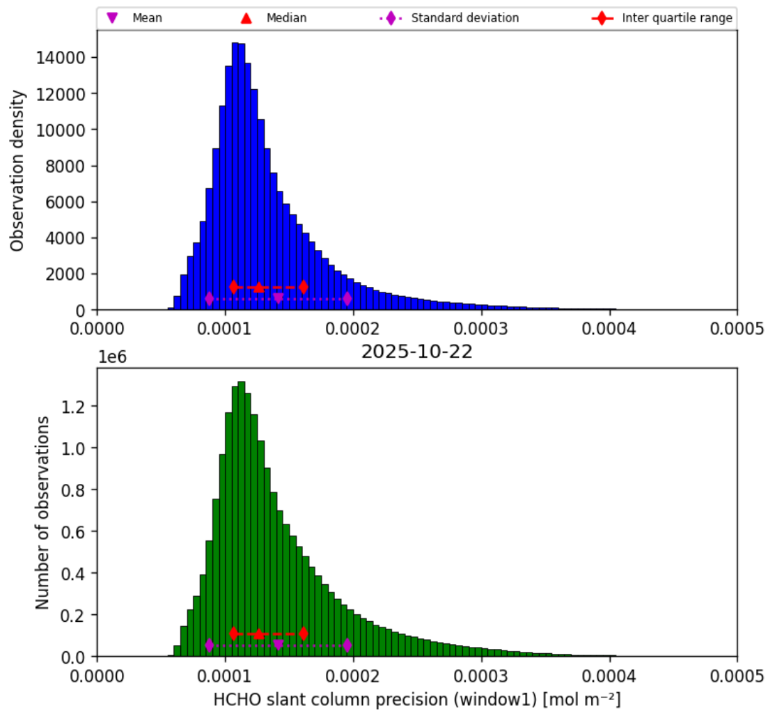
Figure 37: Histogram of “HCHO slant column precision (window1)” for 2025-10-22 to 2025-10-23
