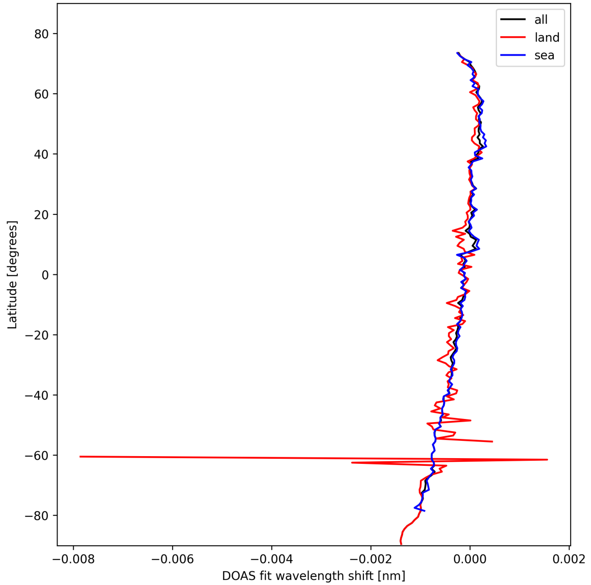
Figure 28: Zonal average of “DOAS fit wavelength shift” for 2025-10-22 to 2025-10-23.
