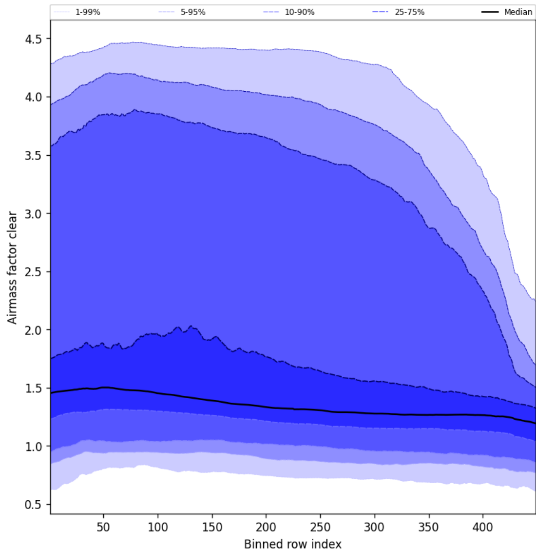
Figure 54: Along track statistics of “Airmass factor clear” for 2025-10-22 to 2025-10-23
