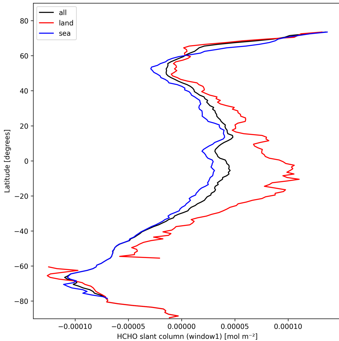
Figure 22: Zonal average of “HCHO slant column (window1)” for 2025-10-22 to 2025-10-23.
