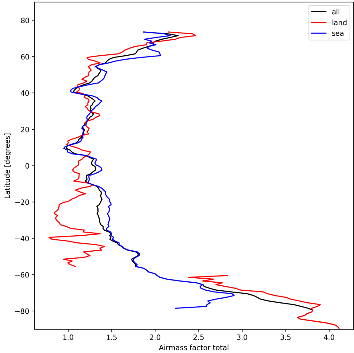
Figure 24: Zonal average of “Airmass factor total” for 2025-10-22 to 2025-10-23.
