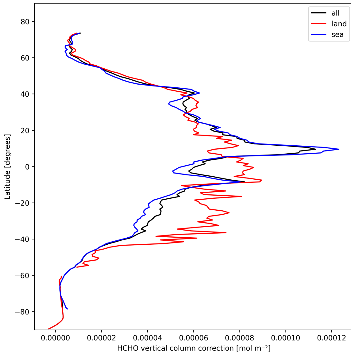
Figure 21: Zonal average of “HCHO vertical column correction” for 2025-10-22 to 2025-10-23.
