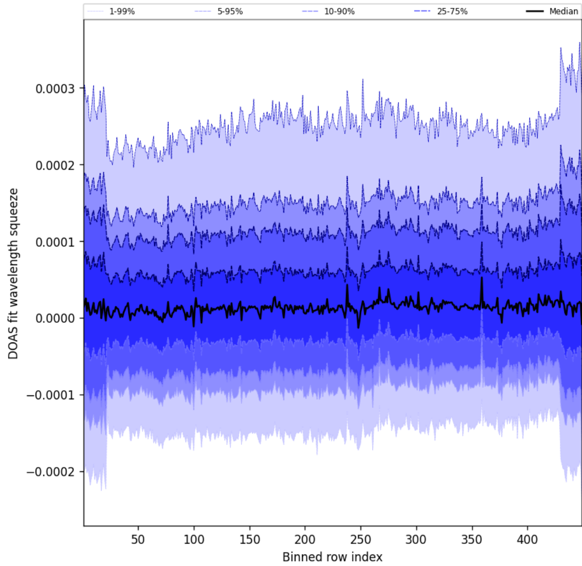
Figure 57: Along track statistics of “DOAS fit wavelength squeeze” for 2025-10-22 to 2025-10-23
