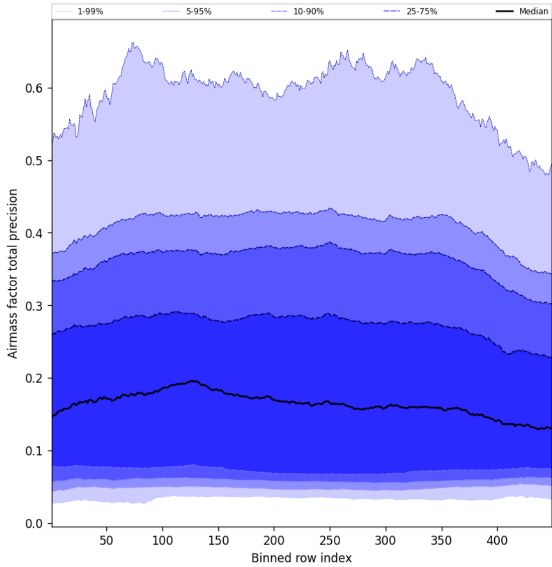
Figure 53: Along track statistics of “Airmass factor total precision” for 2025-10-22 to 2025-10-23
