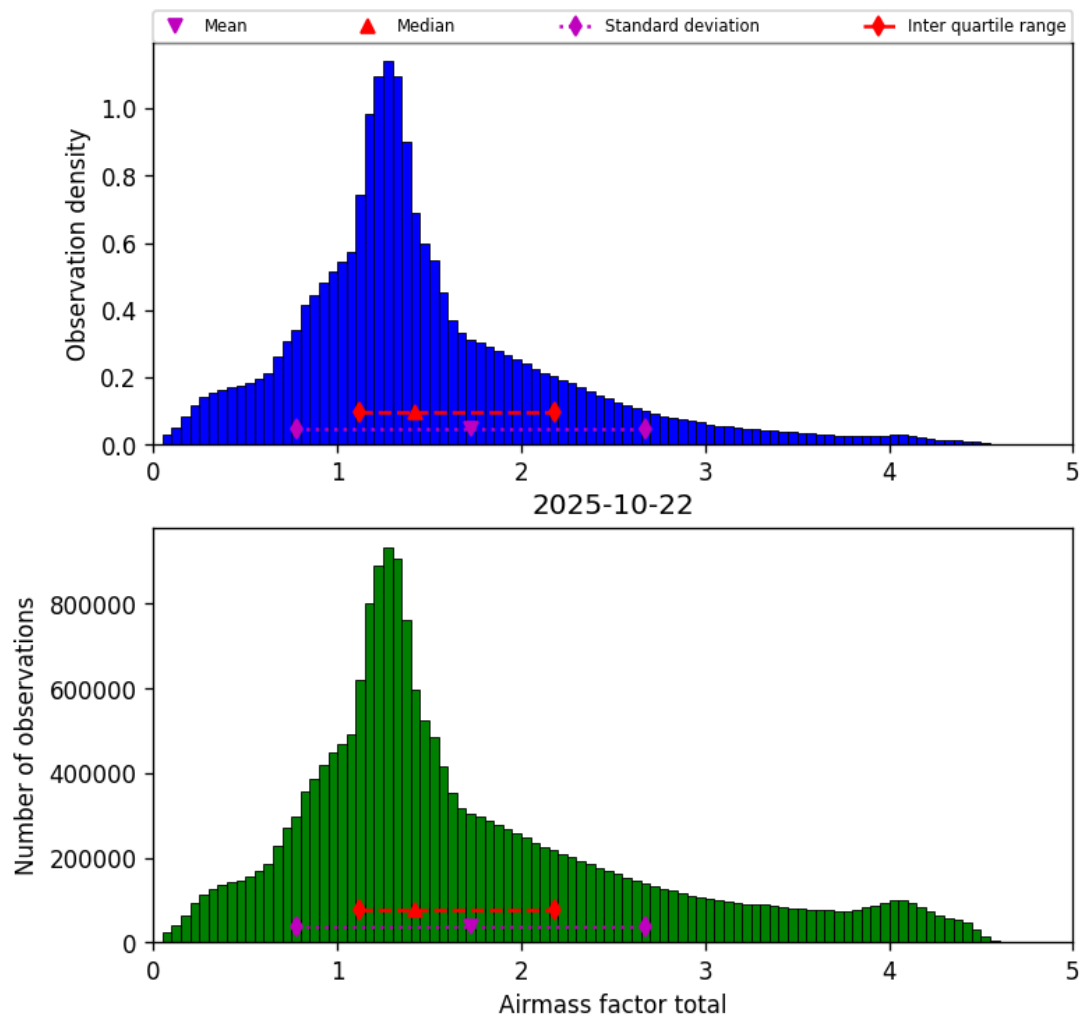
Figure 38: Histogram of “Airmass factor total” for 2025-10-22 to 2025-10-23
