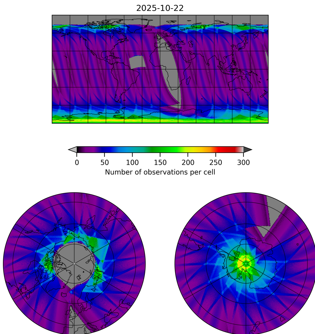
Figure 17: Map of the number of observations for 2025-10-22 to 2025-10-23
