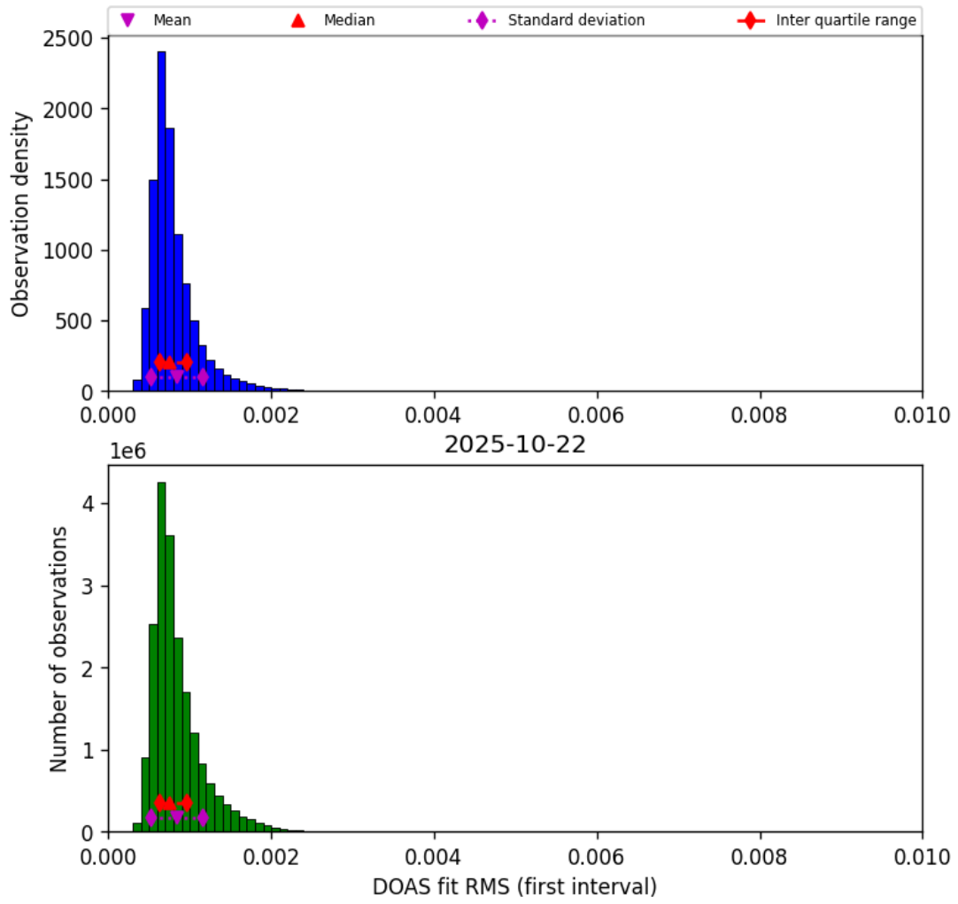
Figure 44: Histogram of “DOAS fit RMS (first interval)” for 2025-10-22 to 2025-10-23
