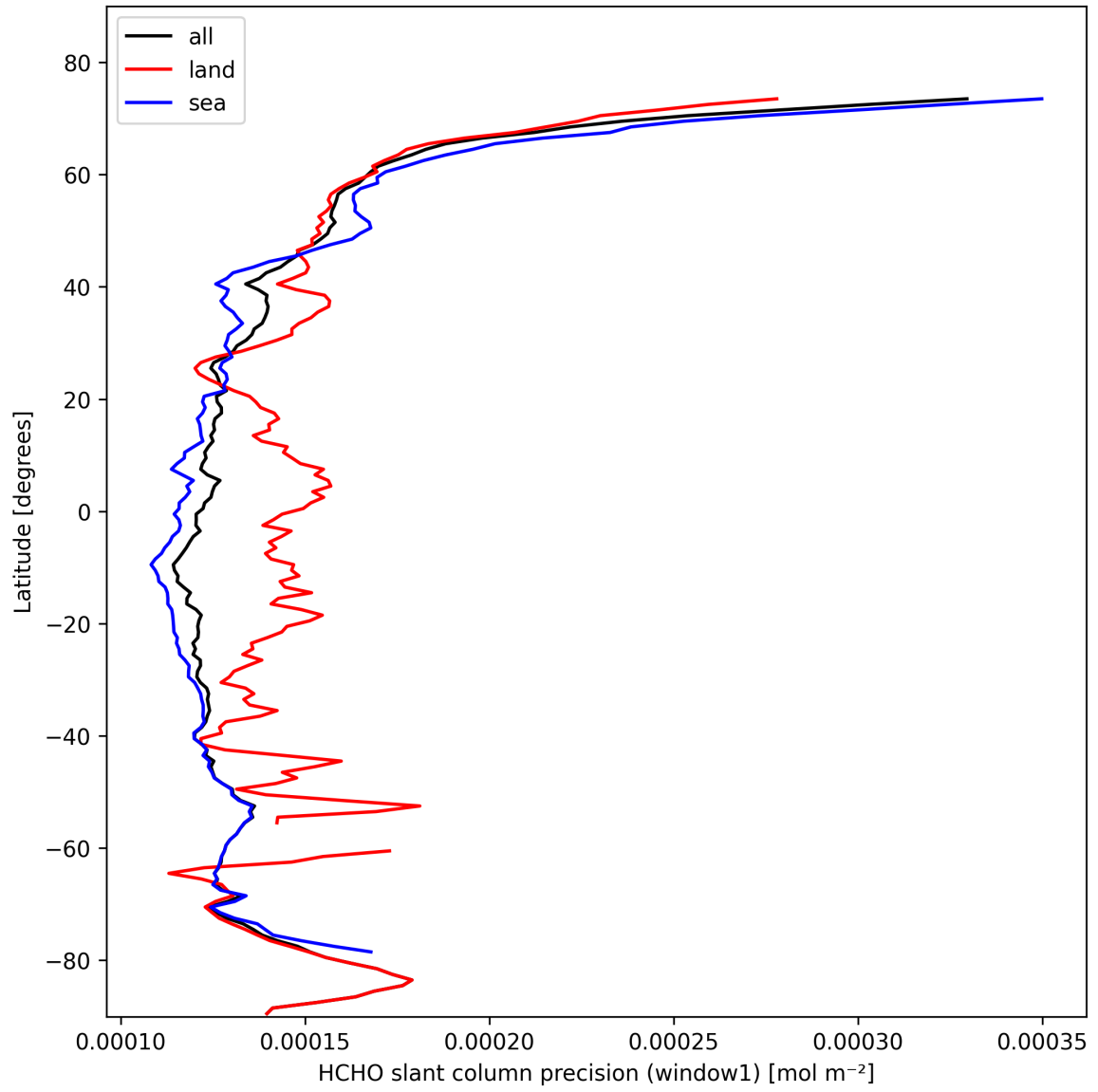
Figure 23: Zonal average of “HCHO slant column precision (window1)” for 2025-10-22 to 2025-10-23.
