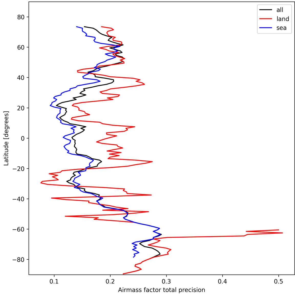
Figure 25: Zonal average of “Airmass factor total precision” for 2025-10-22 to 2025-10-23.
