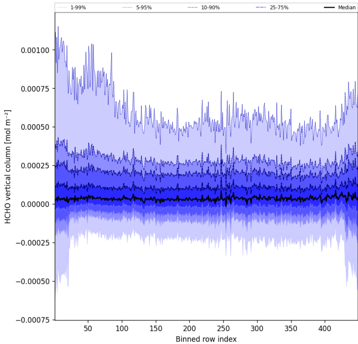
Figure 47: Along track statistics of “HCHO vertical column” for 2025-10-22 to 2025-10-23
