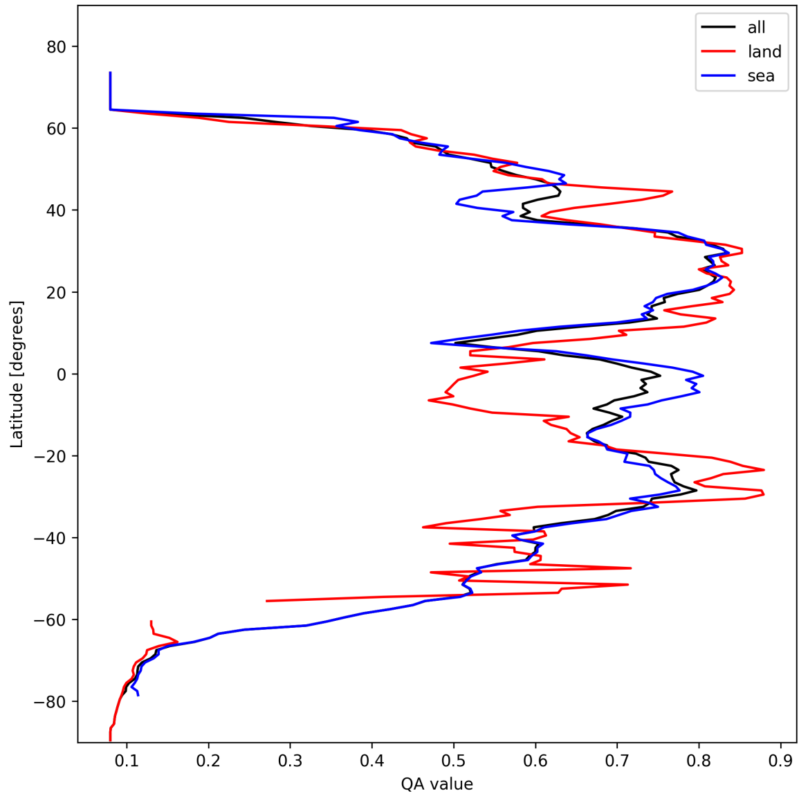
Figure 18: Zonal average of “QA value” for 2025-10-22 to 2025-10-23.
