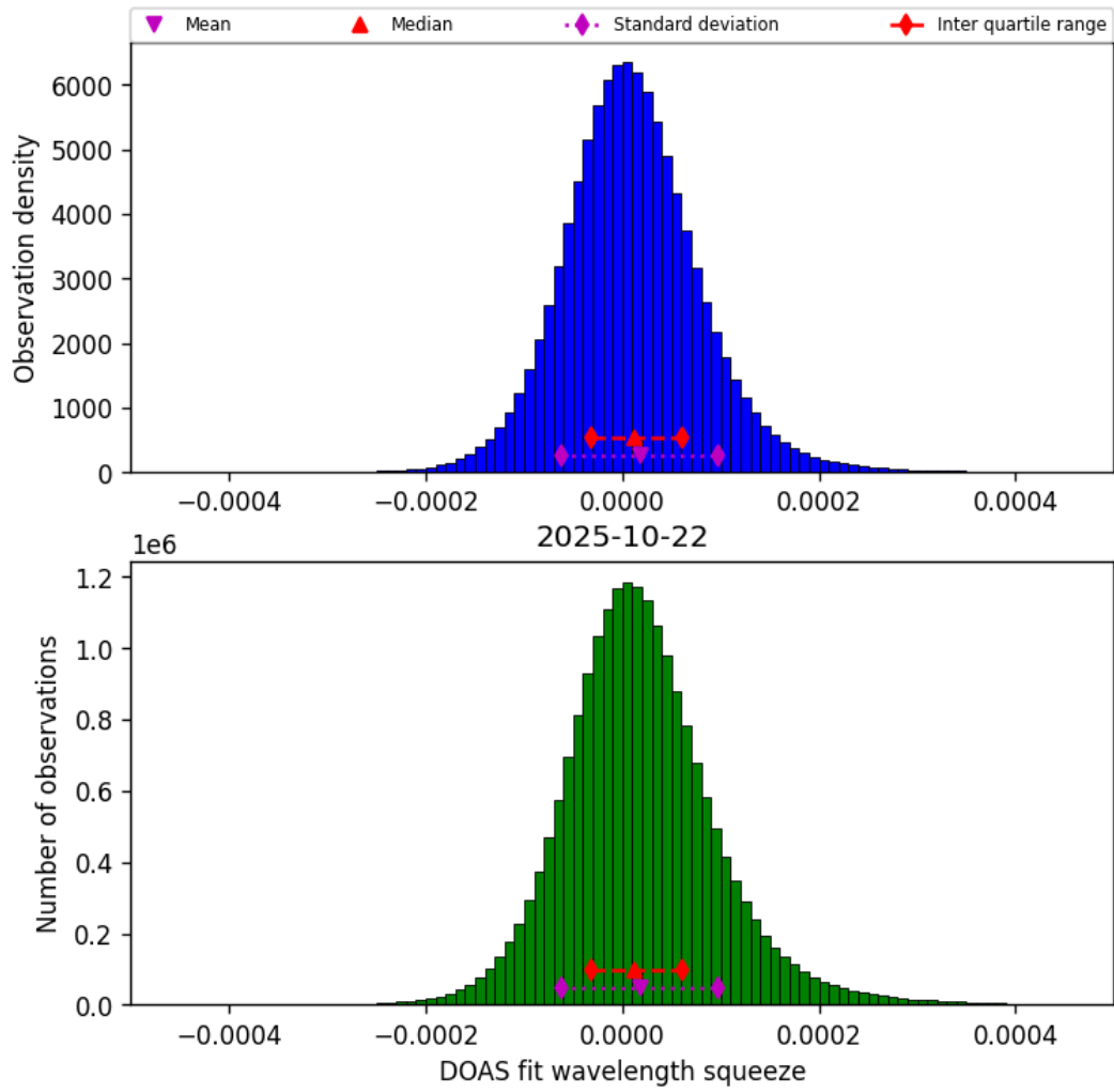
Figure 43: Histogram of “DOAS fit wavelength squeeze” for 2025-10-22 to 2025-10-23
