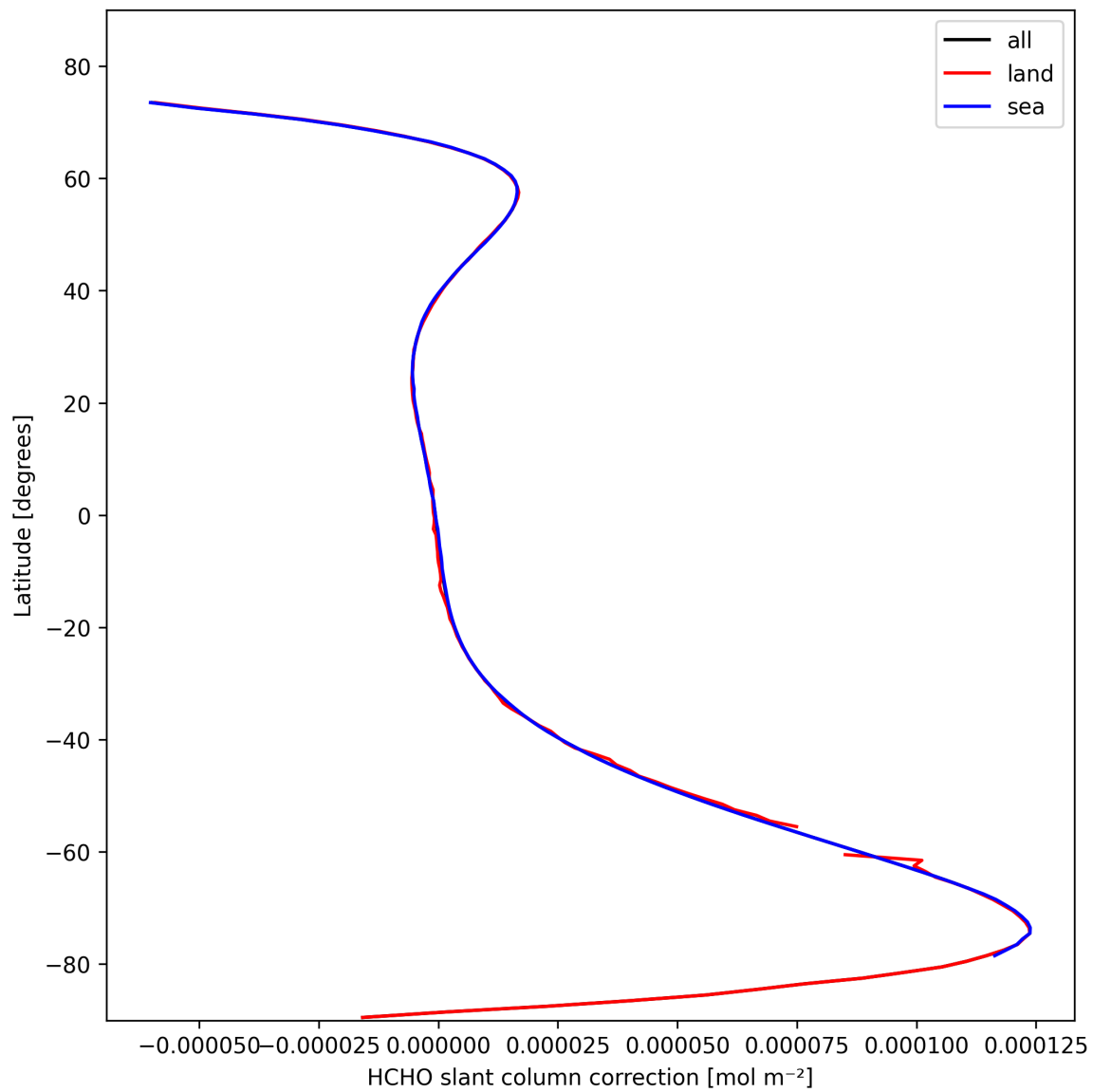
Figure 31: Zonal average of “HCHO slant column correction” for 2025-10-22 to 2025-10-23.
