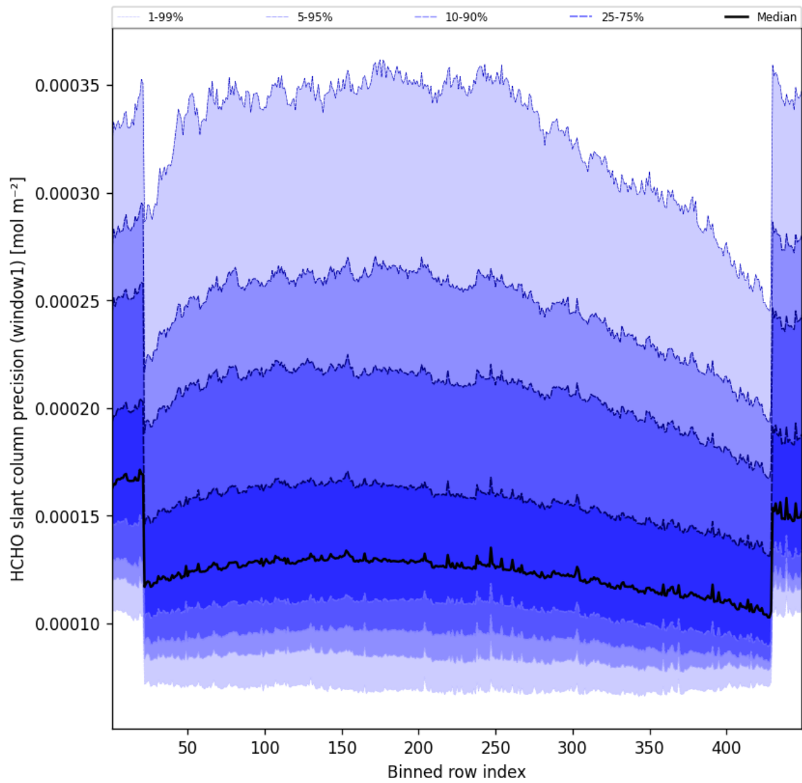
Figure 51: Along track statistics of “HCHO slant column precision (window1)” for 2025-10-22 to 2025-10-23
