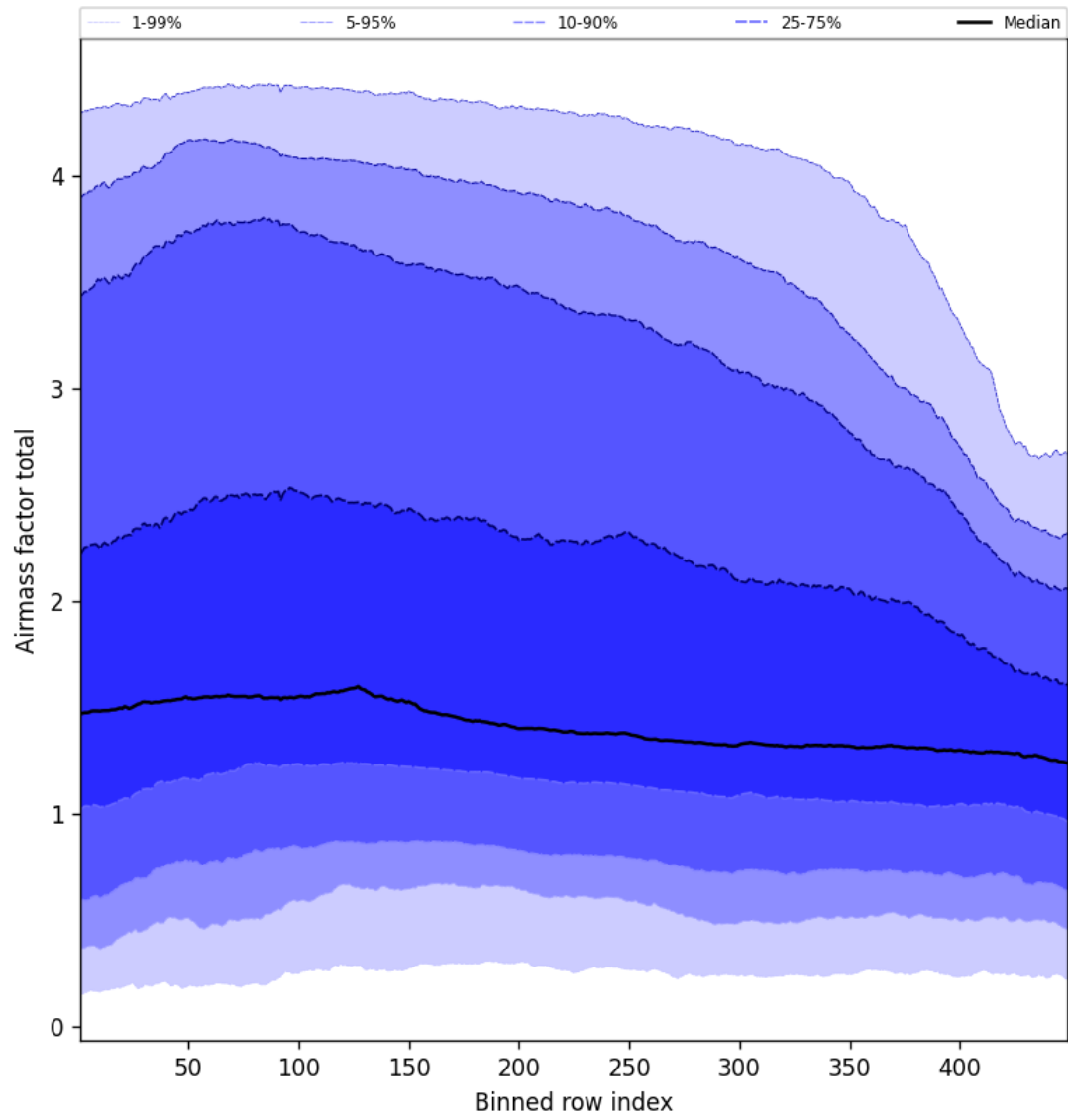
Figure 52: Along track statistics of “Airmass factor total” for 2025-10-22 to 2025-10-23
