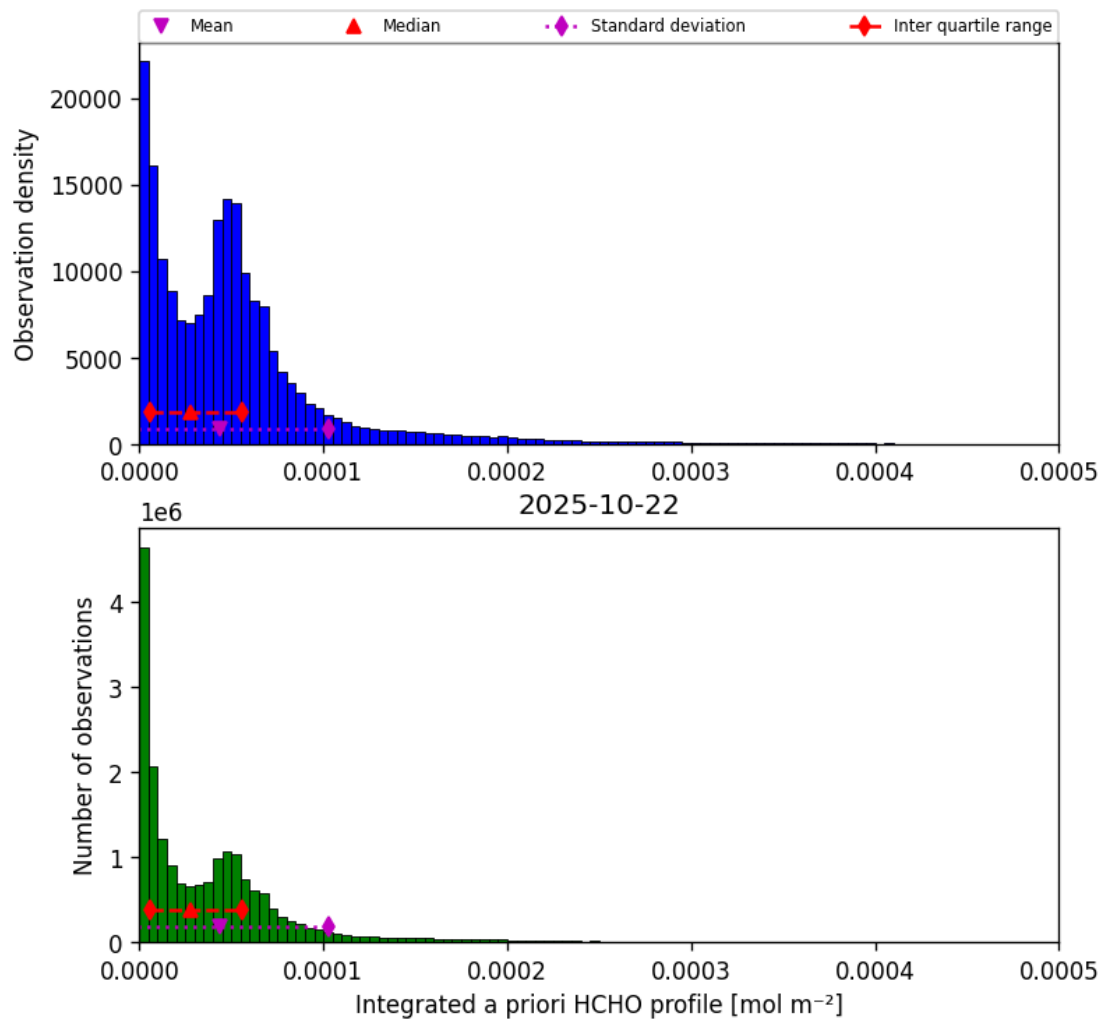
Figure 41: Histogram of “Integrated a priori HCHO profile” for 2025-10-22 to 2025-10-23
