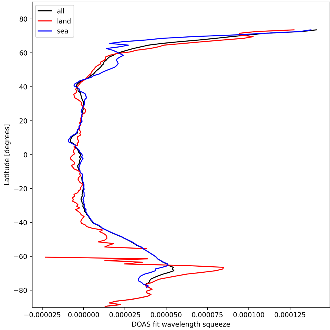
Figure 29: Zonal average of “DOAS fit wavelength squeeze” for 2025-10-22 to 2025-10-23.
