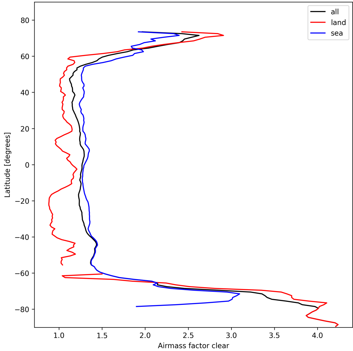
Figure 26: Zonal average of “Airmass factor clear” for 2025-10-22 to 2025-10-23.
