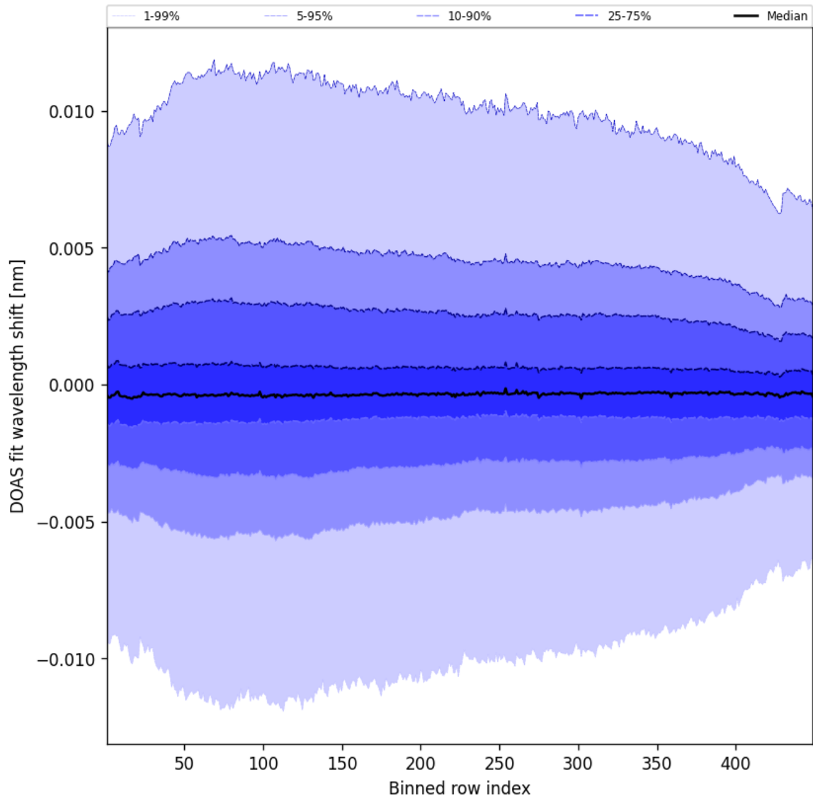
Figure 56: Along track statistics of “DOAS fit wavelength shift” for 2025-10-22 to 2025-10-23
