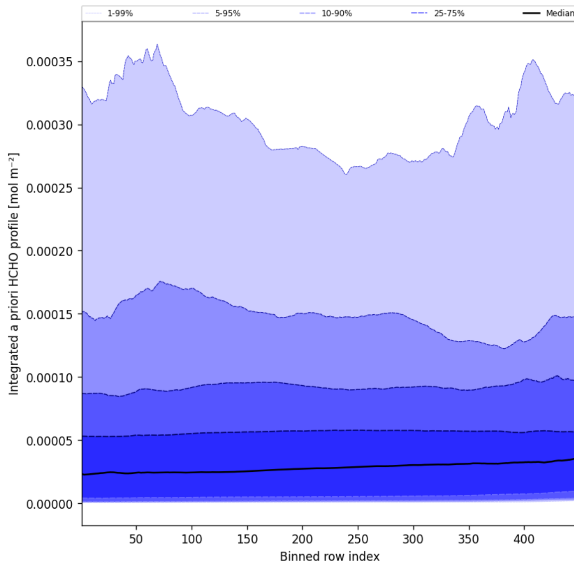
Figure 55: Along track statistics of "Integrated a priori HCHO profile" for 2025-10-22 to 2025-10-23
