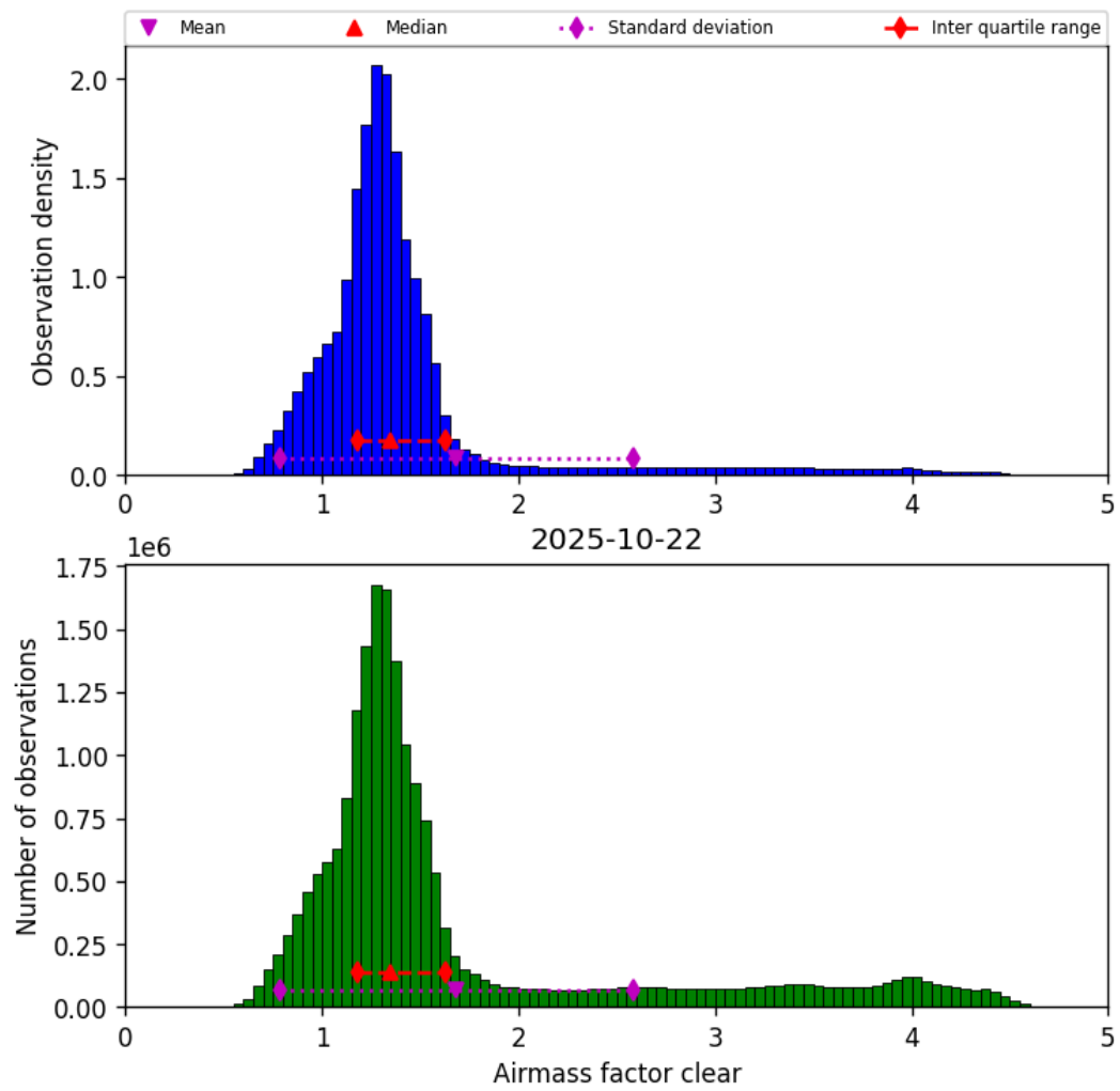
Figure 40: Histogram of “Airmass factor clear” for 2025-10-22 to 2025-10-23
