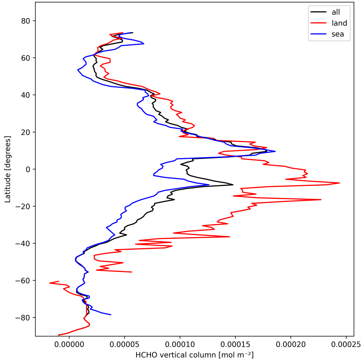
Figure 19: Zonal average of “HCHO vertical column” for 2025-10-22 to 2025-10-23.
