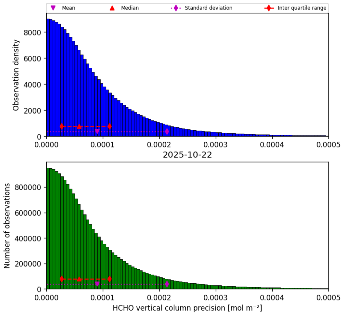
Figure 34: Histogram of “HCHO vertical column precision” for 2025-10-22 to 2025-10-23
