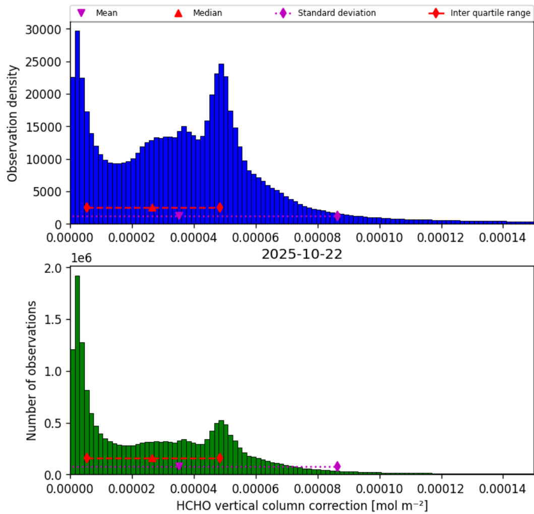
Figure 35: Histogram of “HCHO vertical column correction” for 2025-10-22 to 2025-10-23
