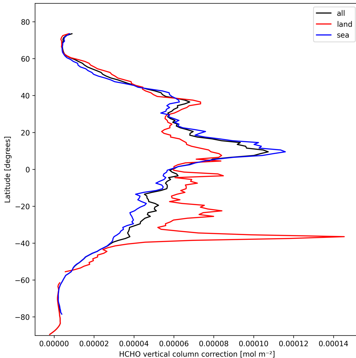
Figure 21: Zonal average of “HCHO vertical column correction” for 2025-10-23 to 2025-10-24.
