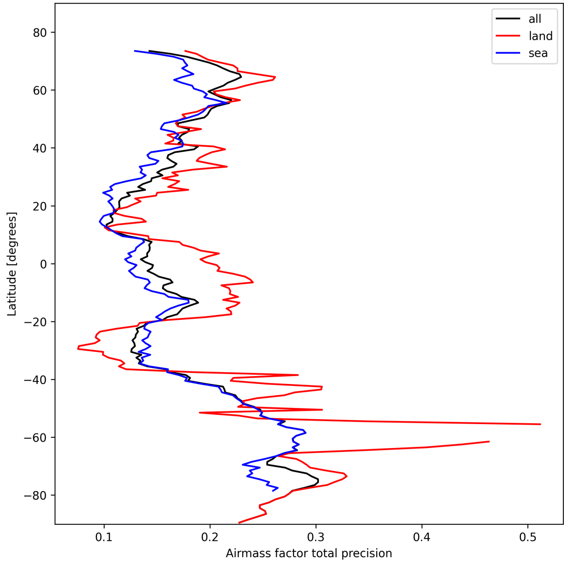
Figure 25: Zonal average of “Airmass factor total precision” for 2025-10-23 to 2025-10-24.
