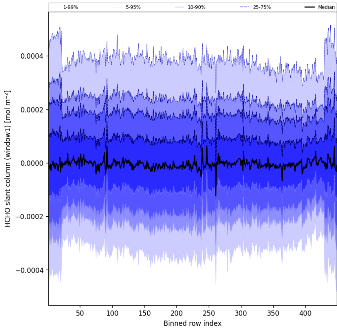
Figure 50: Along track statistics of “HCHO slant column (window1)” for 2025-10-23 to 2025-10-24
