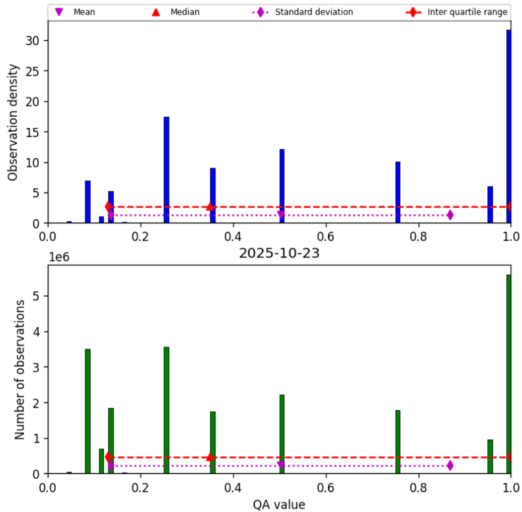
Figure 32: Histogram of “QA value” for 2025-10-23 to 2025-10-24
