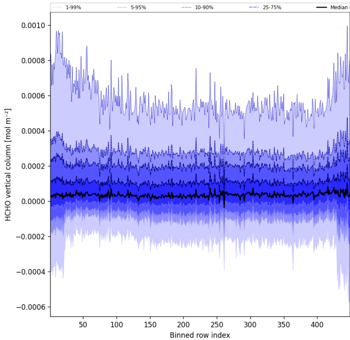
Figure 47: Along track statistics of “HCHO vertical column” for 2025-10-23 to 2025-10-24
