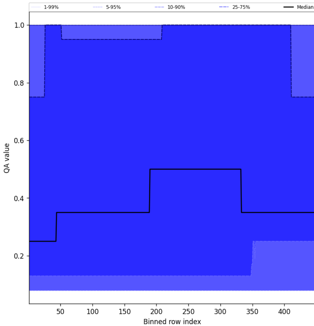
Figure 46: Along track statistics of “QA value” for 2025-10-23 to 2025-10-24
