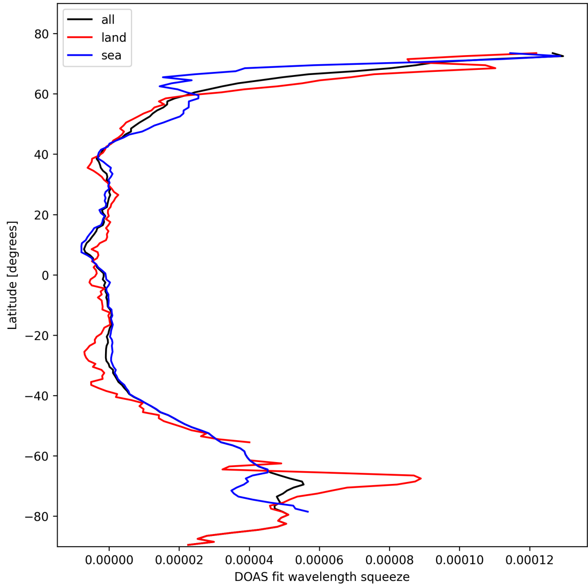
Figure 29: Zonal average of “DOAS fit wavelength squeeze” for 2025-10-23 to 2025-10-24.
