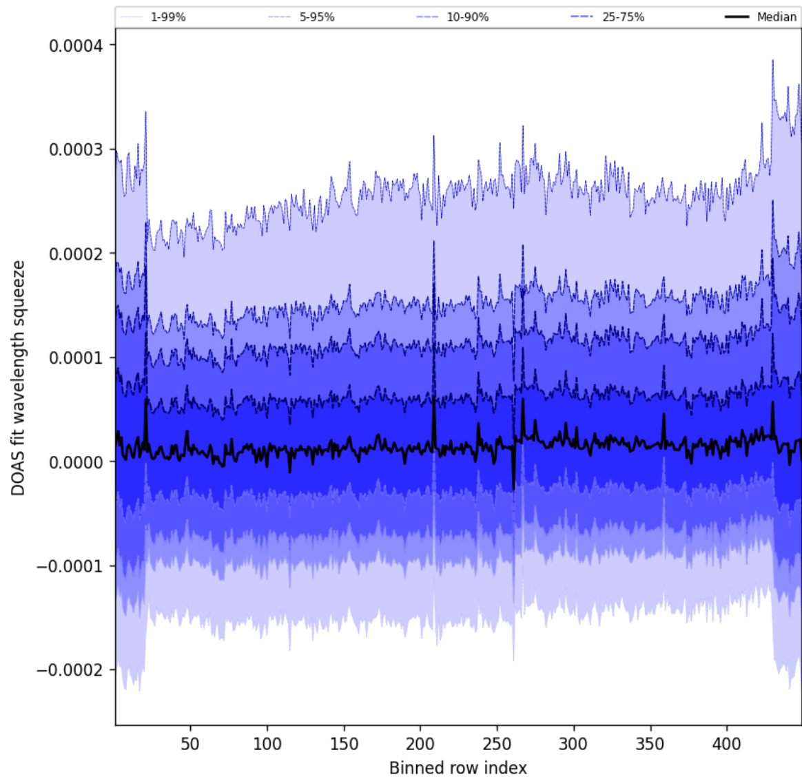
Figure 57: Along track statistics of “DOAS fit wavelength squeeze” for 2025-10-23 to 2025-10-24
