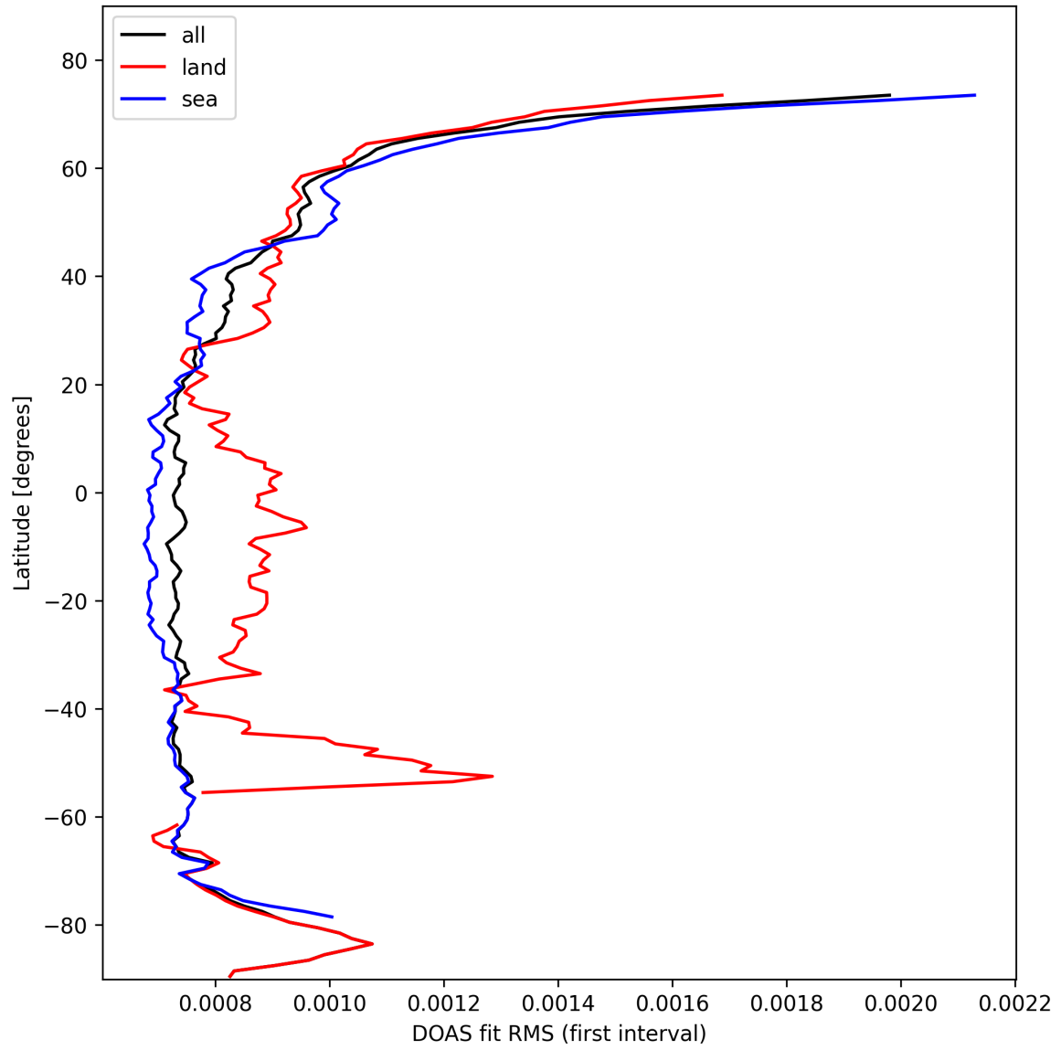
Figure 30: Zonal average of “DOAS fit RMS (first interval)” for 2025-10-23 to 2025-10-24.
