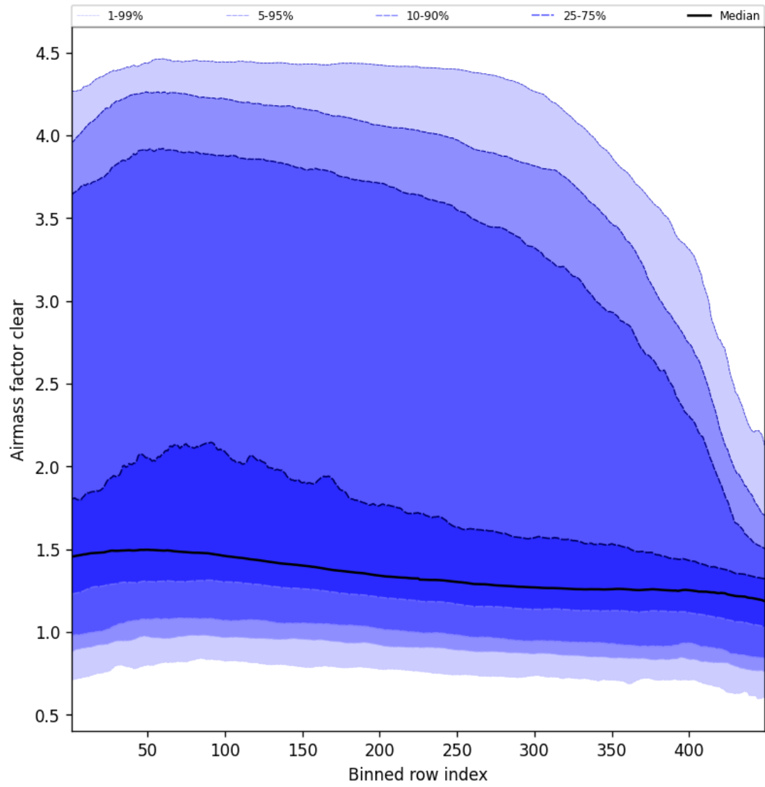
Figure 54: Along track statistics of “Airmass factor clear” for 2025-10-23 to 2025-10-24
