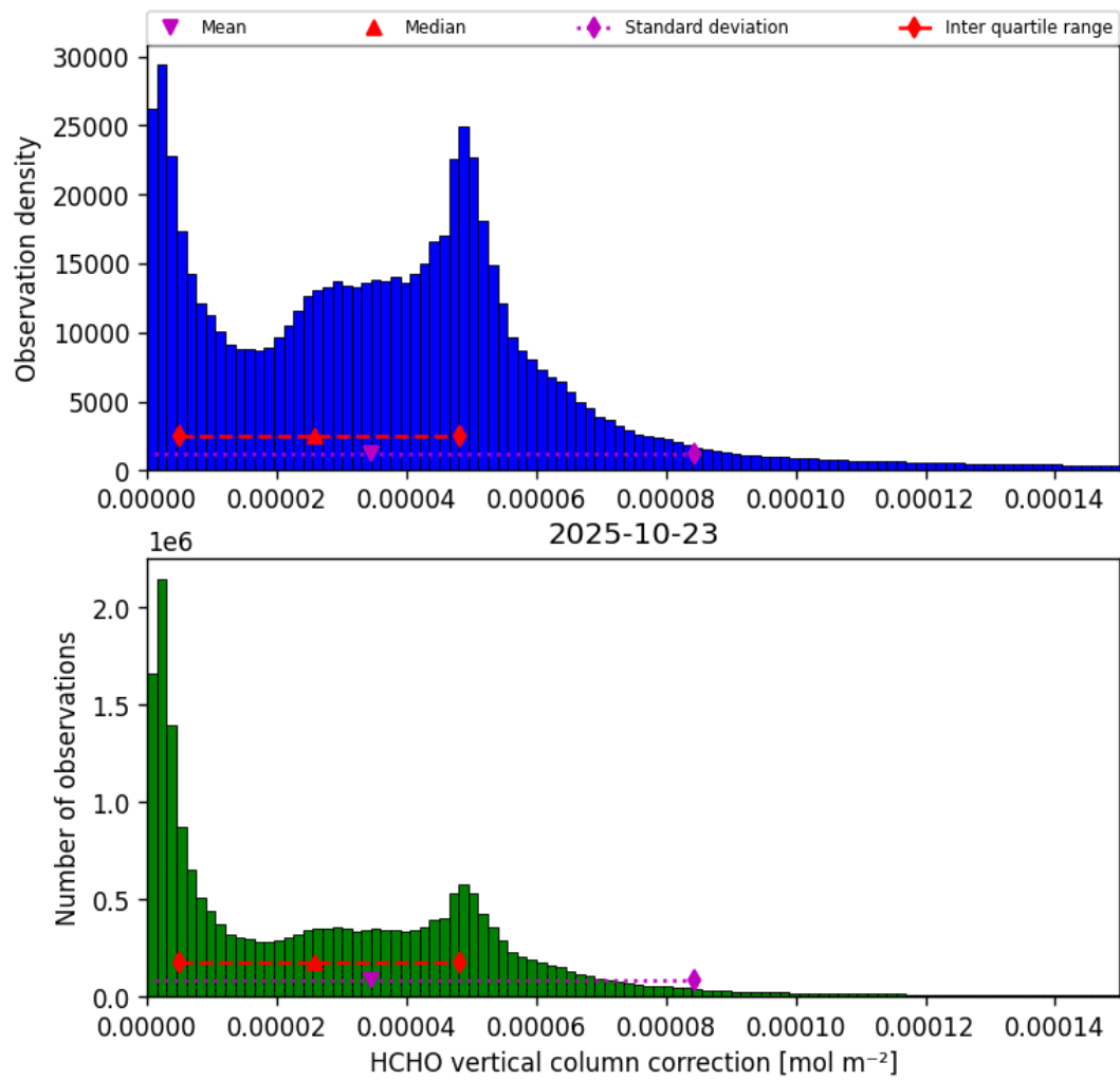
Figure 35: Histogram of “HCHO vertical column correction” for 2025-10-23 to 2025-10-24
