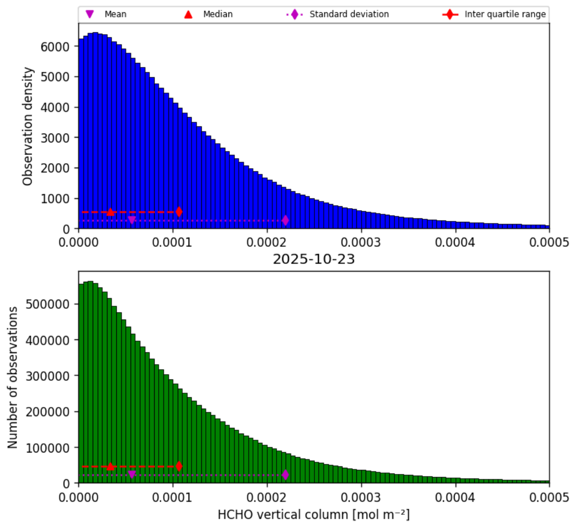
Figure 33: Histogram of “HCHO vertical column” for 2025-10-23 to 2025-10-24
