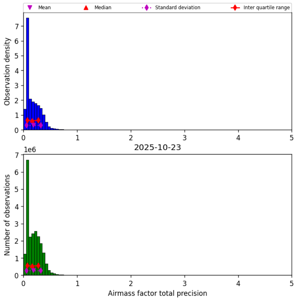
Figure 39: Histogram of “Airmass factor total precision” for 2025-10-23 to 2025-10-24
