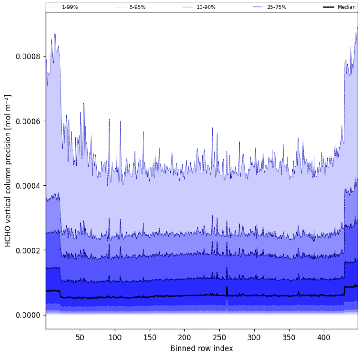
Figure 48: Along track statistics of “HCHO vertical column precision” for 2025-10-23 to 2025-10-24
