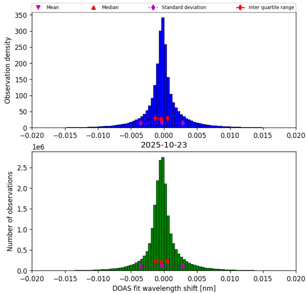
Figure 42: Histogram of “DOAS fit wavelength shift” for 2025-10-23 to 2025-10-24
