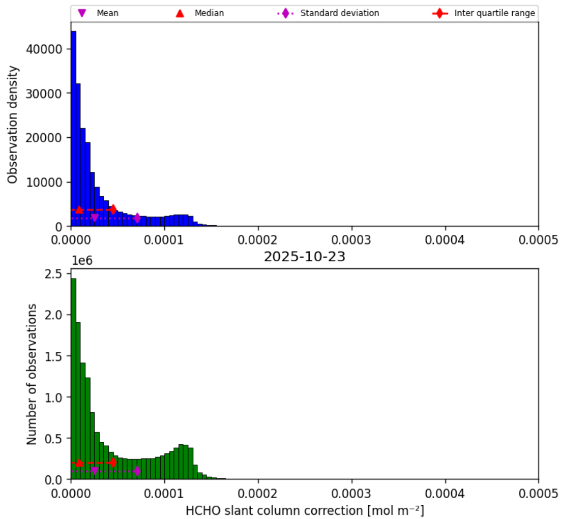
Figure 45: Histogram of “HCHO slant column correction” for 2025-10-23 to 2025-10-24
