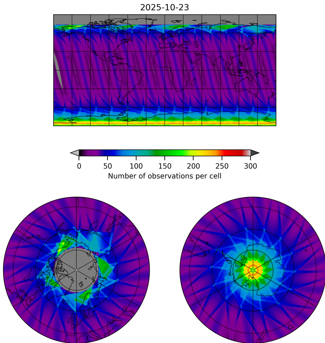
Figure 17: Map of the number of observations for 2025-10-23 to 2025-10-24
