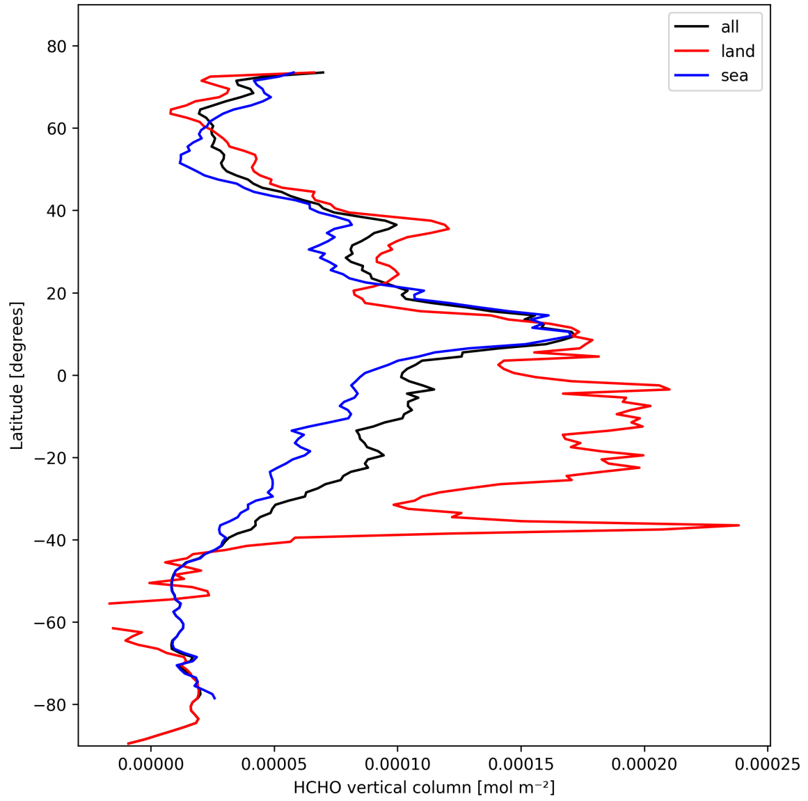
Figure 19: Zonal average of “HCHO vertical column” for 2025-10-23 to 2025-10-24.
