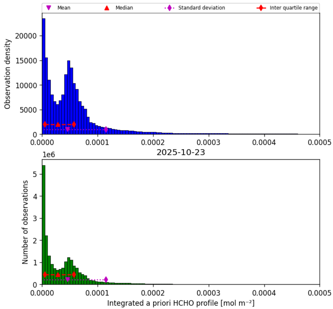
Figure 41: Histogram of “Integrated a priori HCHO profile” for 2025-10-23 to 2025-10-24
