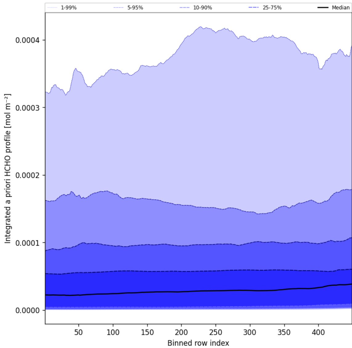
Figure 55: Along track statistics of “Integrated a priori HCHO profile” for 2025-10-23 to 2025-10-24
