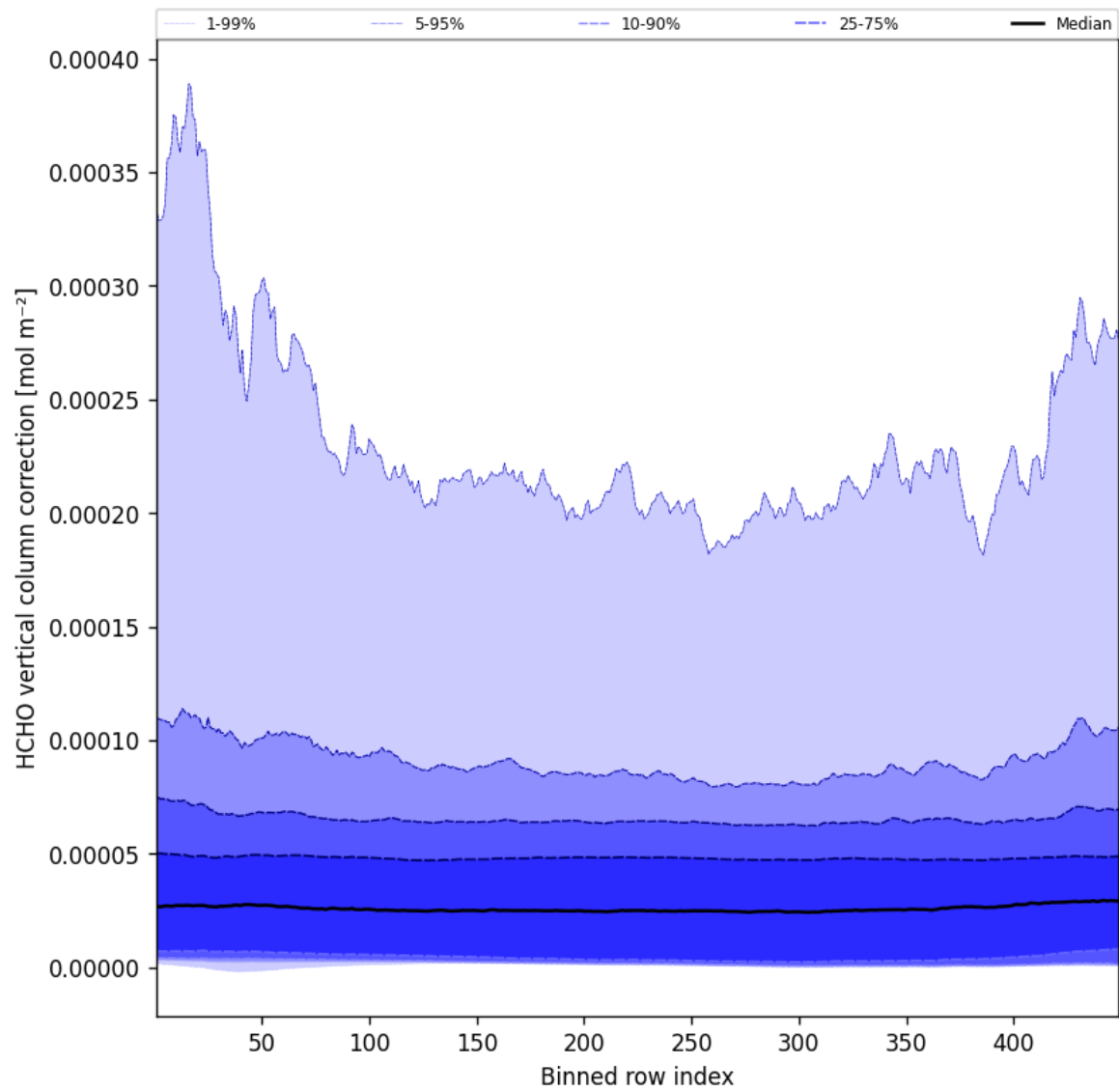
Figure 49: Along track statistics of “HCHO vertical column correction” for 2025-10-23 to 2025-10-24
