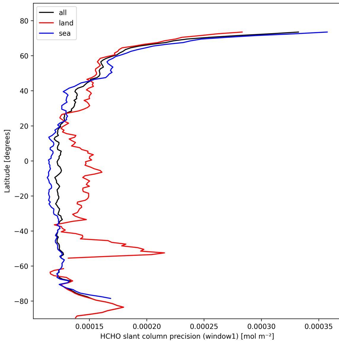
Figure 23: Zonal average of “HCHO slant column precision (window1)” for 2025-10-23 to 2025-10-24.
