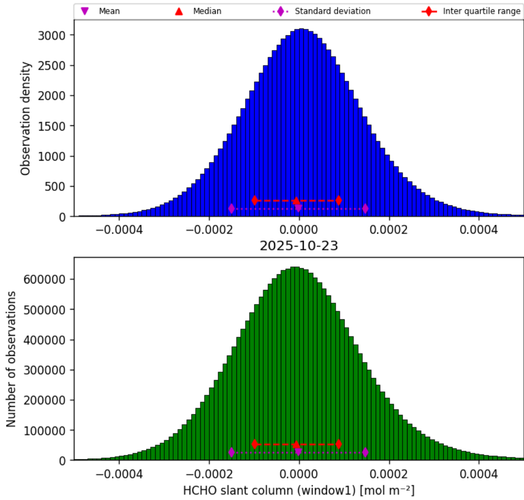
Figure 36: Histogram of “HCHO slant column (window1)” for 2025-10-23 to 2025-10-24
