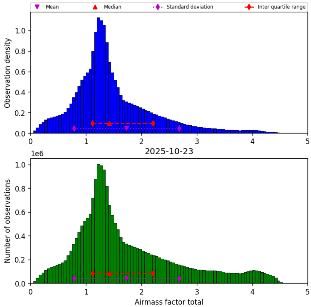
Figure 38: Histogram of “Airmass factor total” for 2025-10-23 to 2025-10-24
