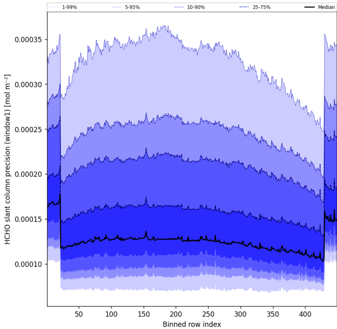
Figure 51: Along track statistics of “HCHO slant column precision (window1)” for 2025-10-23 to 2025-10-24
