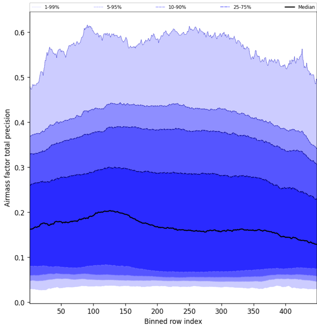
Figure 53: Along track statistics of “Airmass factor total precision” for 2025-10-23 to 2025-10-24
