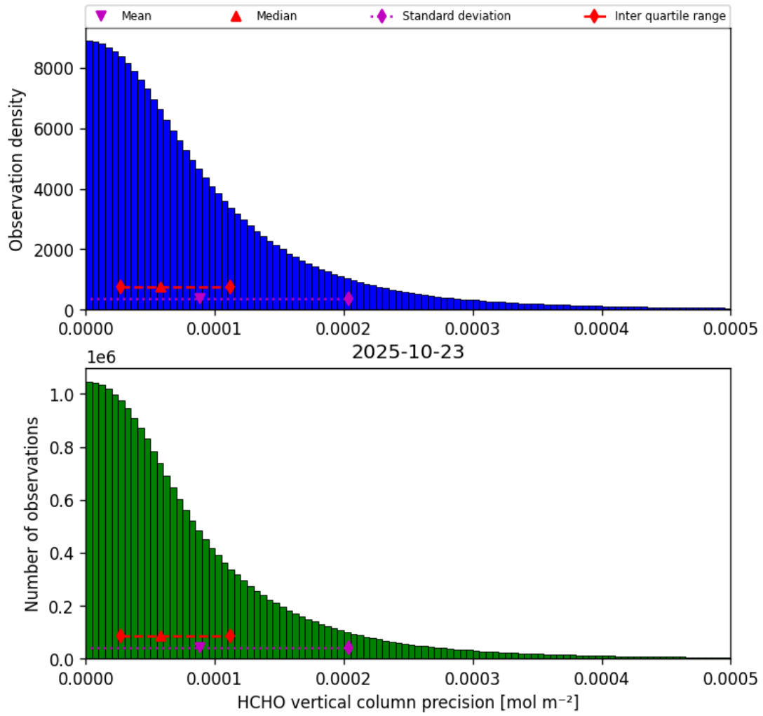
Figure 34: Histogram of “HCHO vertical column precision” for 2025-10-23 to 2025-10-24
