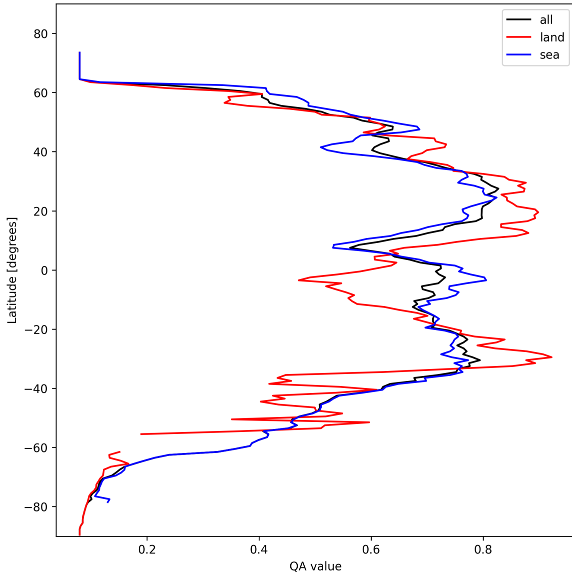
Figure 18: Zonal average of “QA value” for 2025-10-23 to 2025-10-24.
