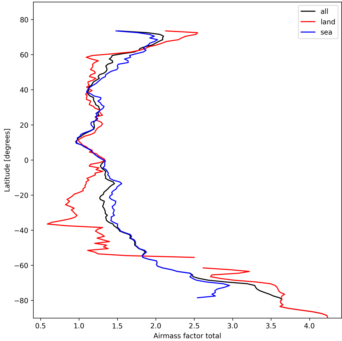
Figure 24: Zonal average of “Airmass factor total” for 2025-10-23 to 2025-10-24.
