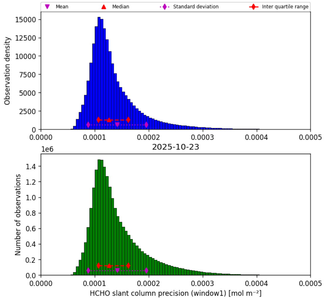
Figure 37: Histogram of “HCHO slant column precision (window1)” for 2025-10-23 to 2025-10-24
