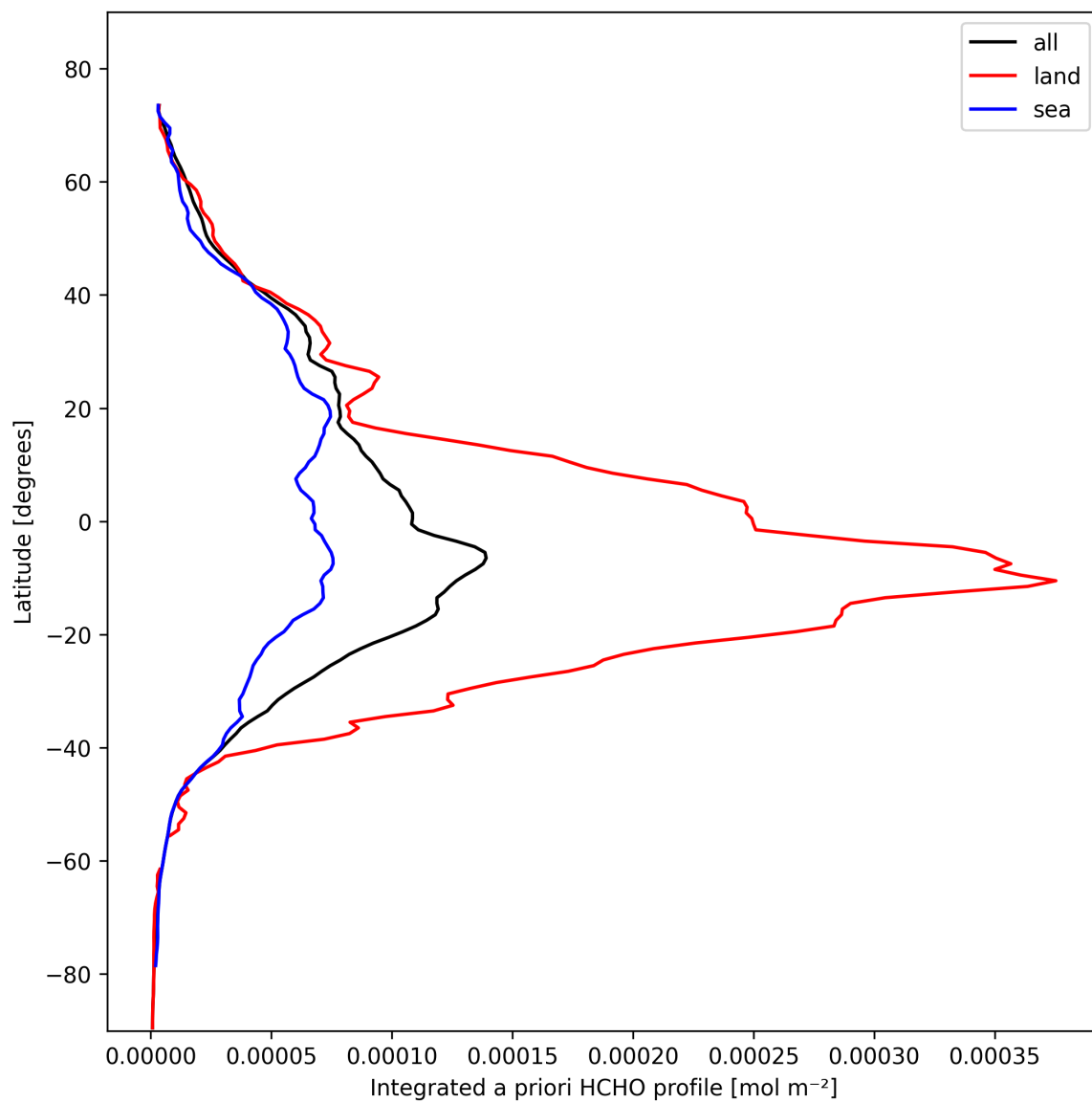
Figure 27: Zonal average of “Integrated a priori HCHO profile” for 2025-10-23 to 2025-10-24.
