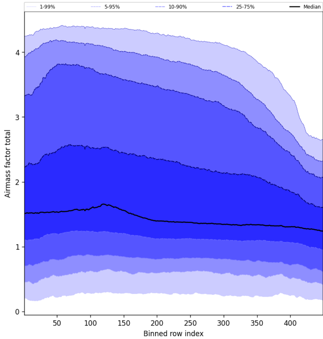
Figure 52: Along track statistics of “Airmass factor total” for 2025-10-23 to 2025-10-24
