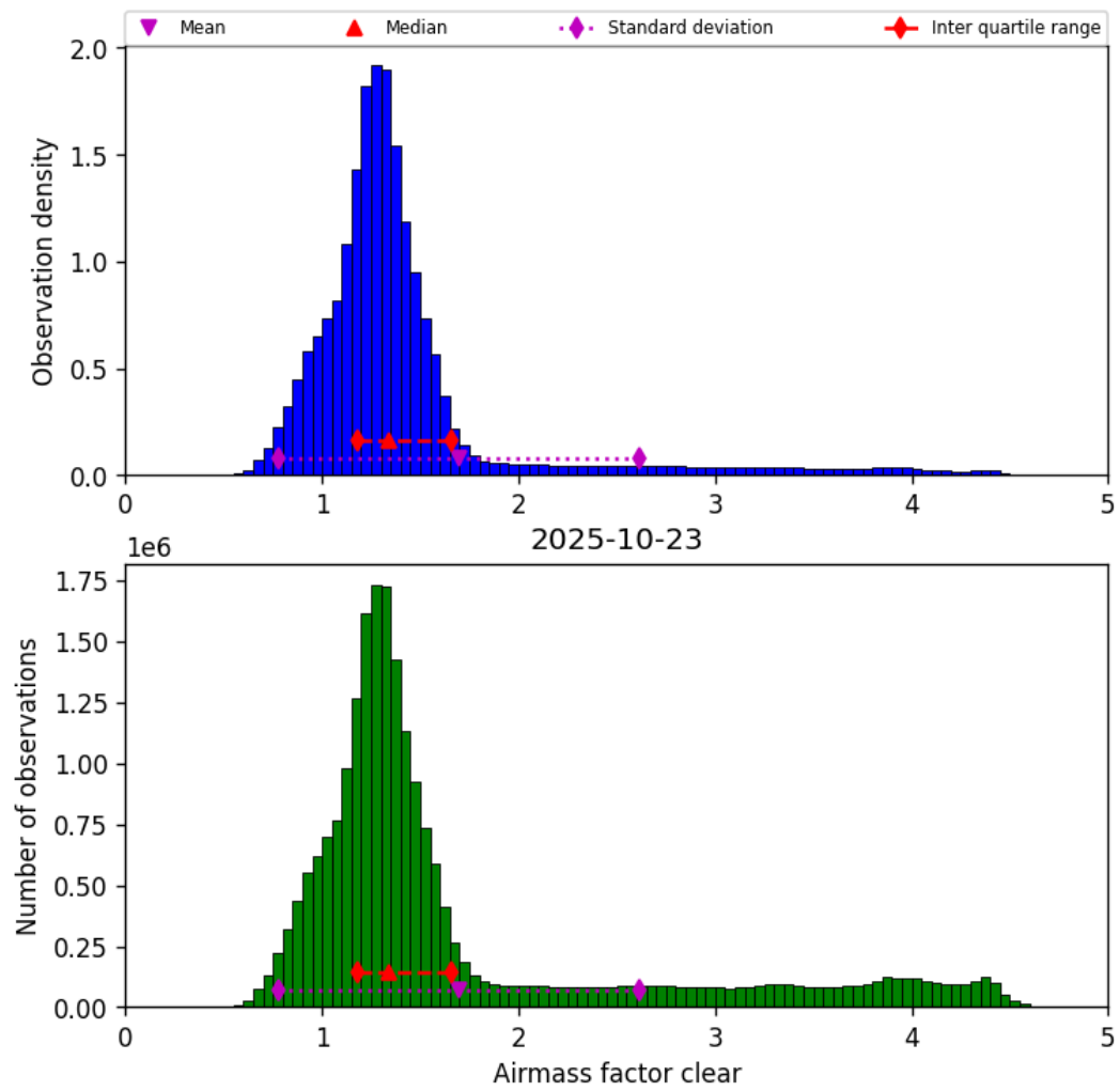
Figure 40: Histogram of “Airmass factor clear” for 2025-10-23 to 2025-10-24
