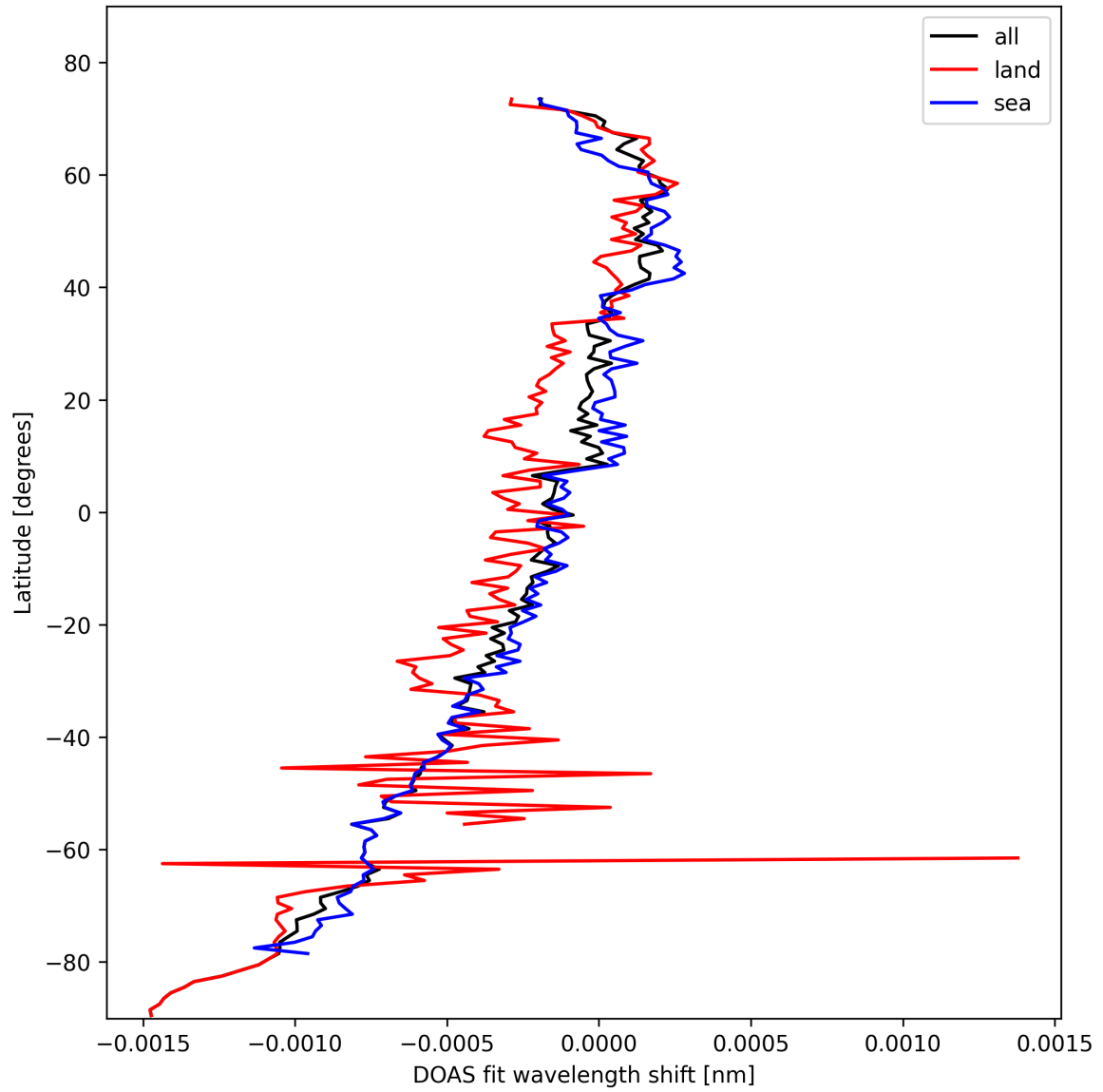
Figure 28: Zonal average of “DOAS fit wavelength shift” for 2025-10-23 to 2025-10-24.
