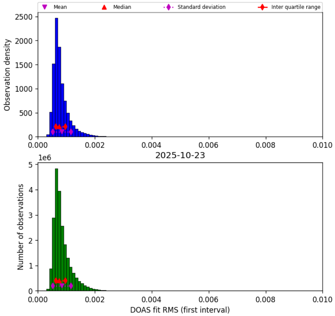
Figure 44: Histogram of “DOAS fit RMS (first interval)” for 2025-10-23 to 2025-10-24
