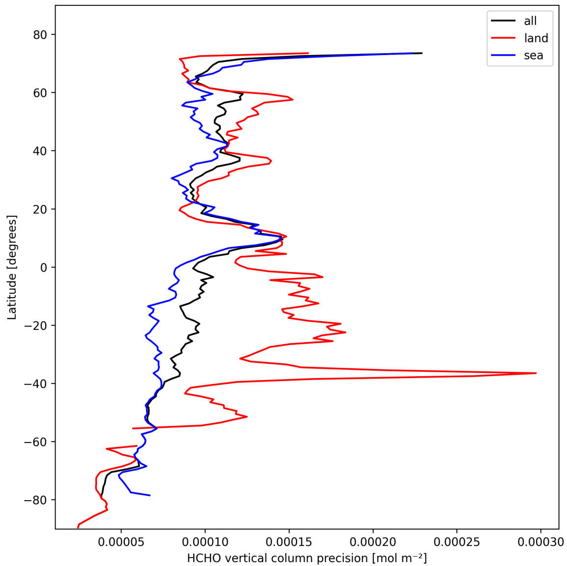
Figure 20: Zonal average of “HCHO vertical column precision” for 2025-10-23 to 2025-10-24.
