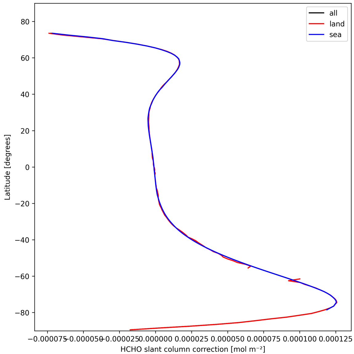
Figure 31: Zonal average of “HCHO slant column correction” for 2025-10-23 to 2025-10-24.
