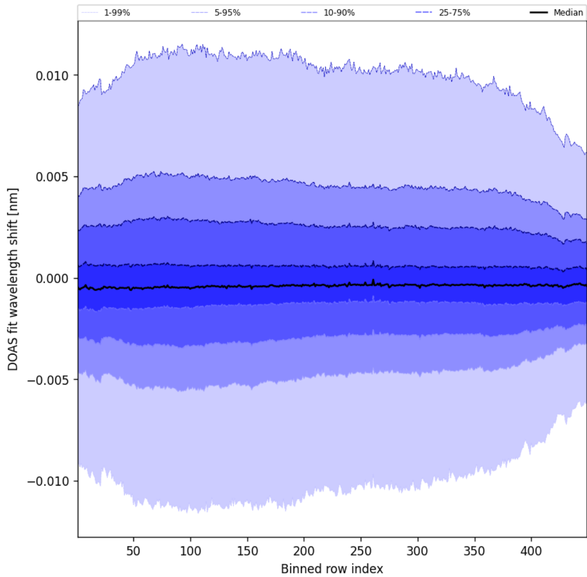
Figure 56: Along track statistics of “DOAS fit wavelength shift” for 2025-10-23 to 2025-10-24
