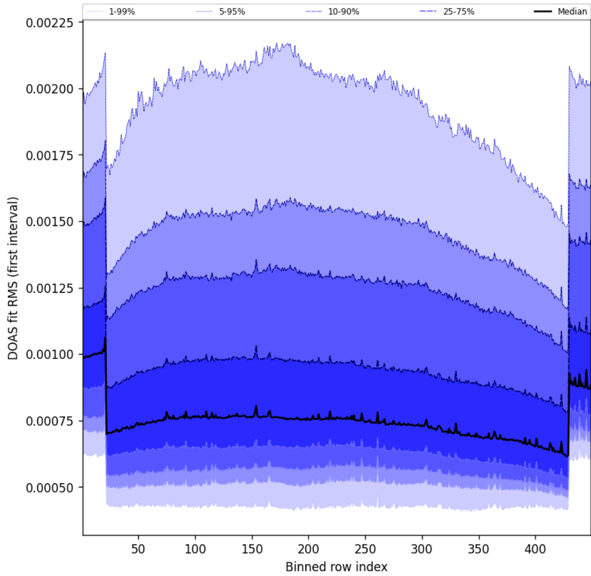
Figure 58: Along track statistics of “DOAS fit RMS (first interval)” for 2025-10-23 to 2025-10-24
