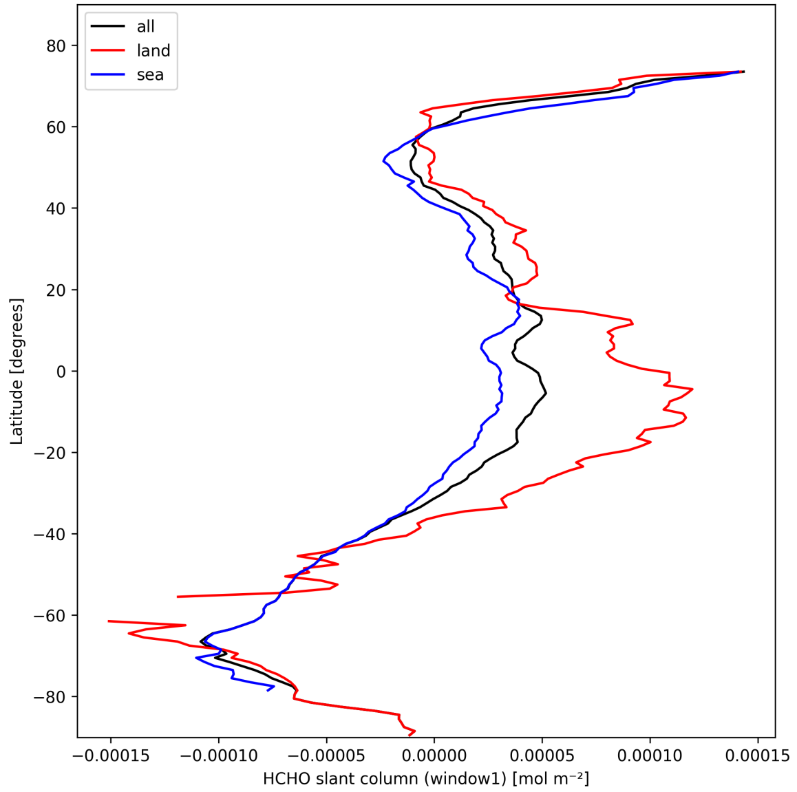
Figure 22: Zonal average of “HCHO slant column (window1)” for 2025-10-23 to 2025-10-24.
