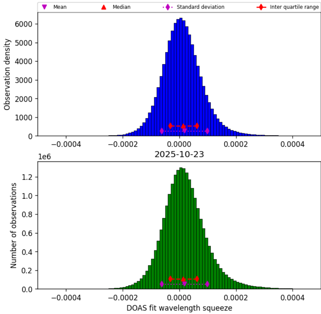
Figure 43: Histogram of "DOAS fit wavelength squeeze" for 2025-10-23 to 2025-10-24
