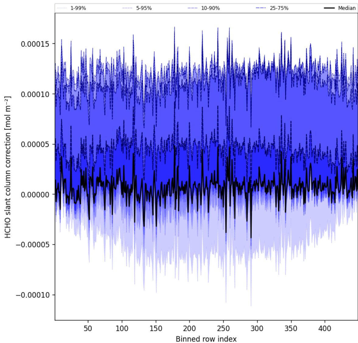
Figure 59: Along track statistics of “HCHO slant column correction” for 2025-10-23 to 2025-10-24
