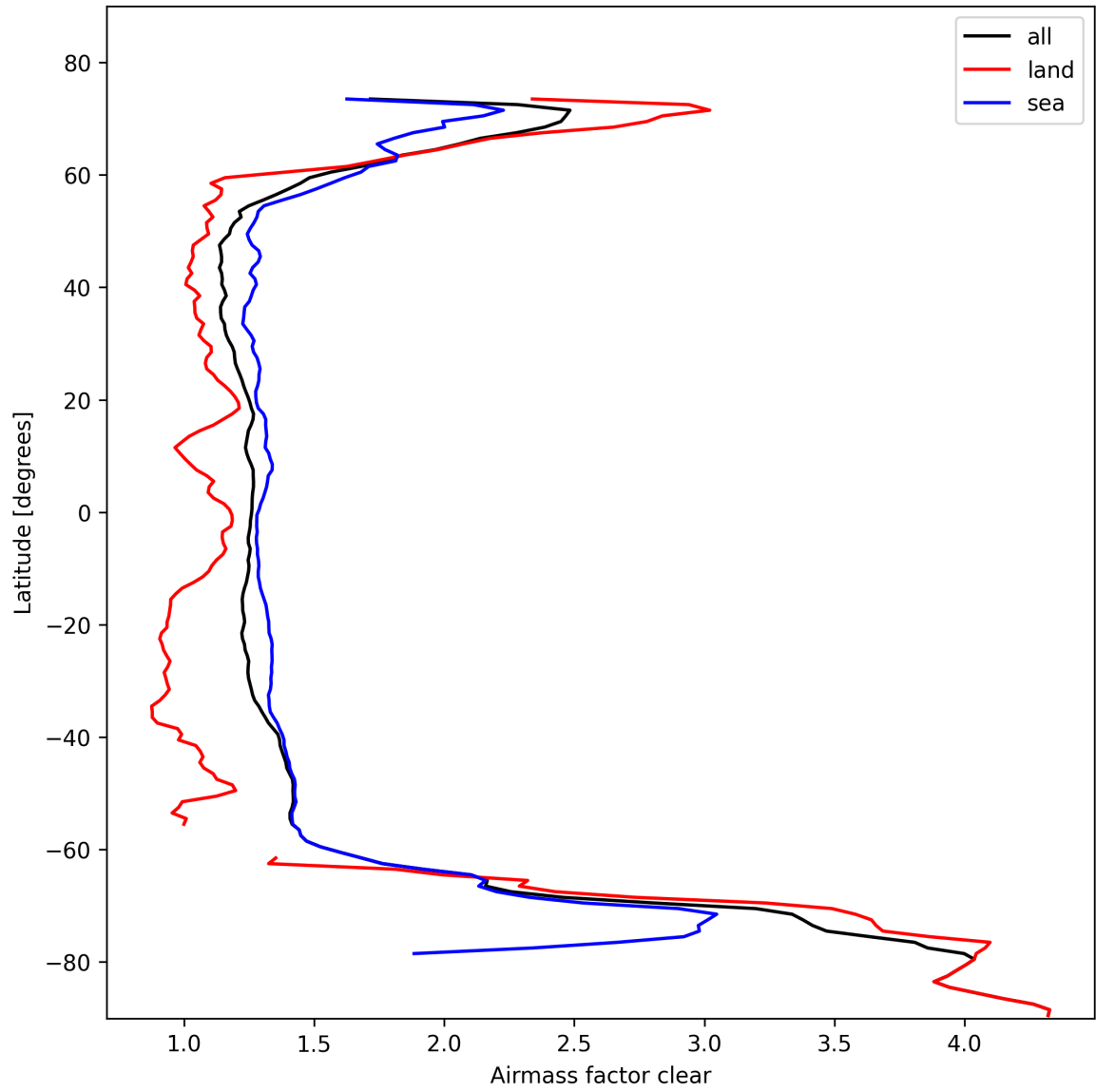
Figure 26: Zonal average of “Airmass factor clear” for 2025-10-23 to 2025-10-24.
