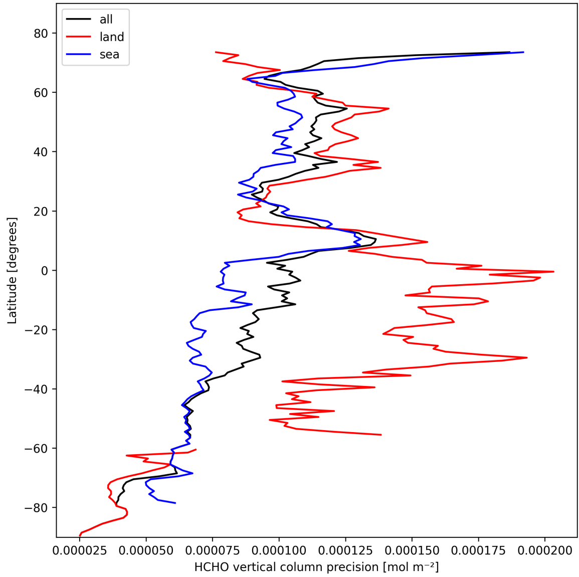
Figure 20: Zonal average of “HCHO vertical column precision” for 2025-10-24 to 2025-10-25.
