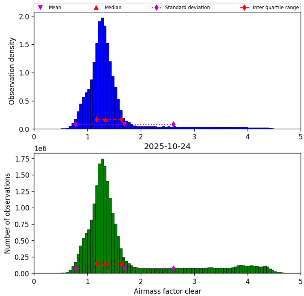
Figure 40: Histogram of “Airmass factor clear” for 2025-10-24 to 2025-10-25
