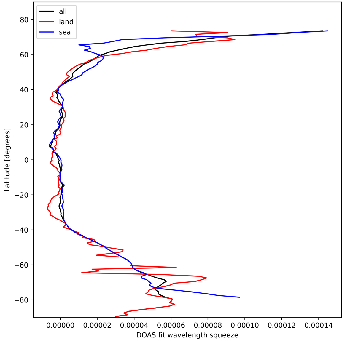
Figure 29: Zonal average of “DOAS fit wavelength squeeze” for 2025-10-24 to 2025-10-25.
