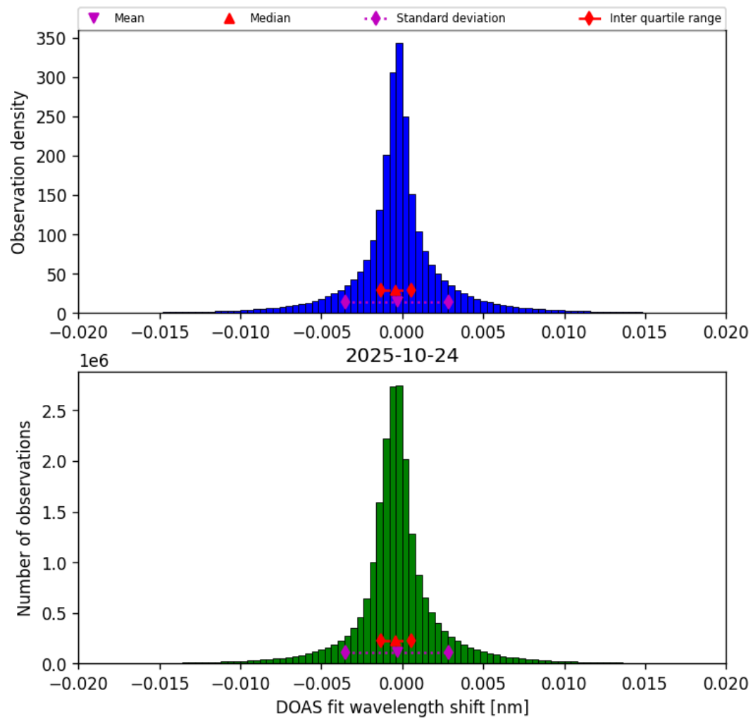
Figure 42: Histogram of “DOAS fit wavelength shift” for 2025-10-24 to 2025-10-25
