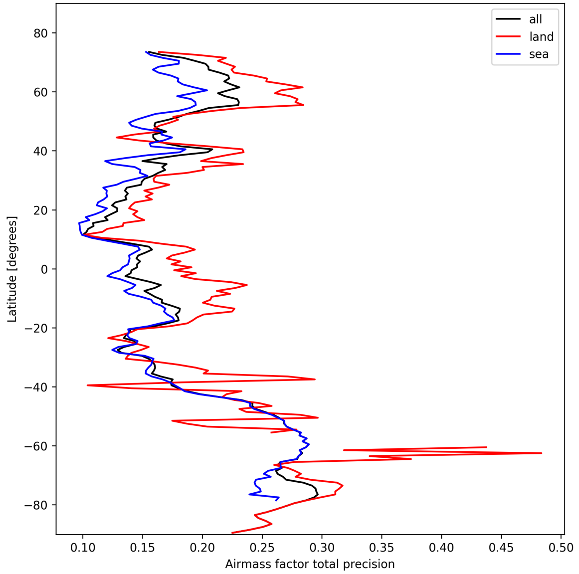
Figure 25: Zonal average of “Airmass factor total precision” for 2025-10-24 to 2025-10-25.
