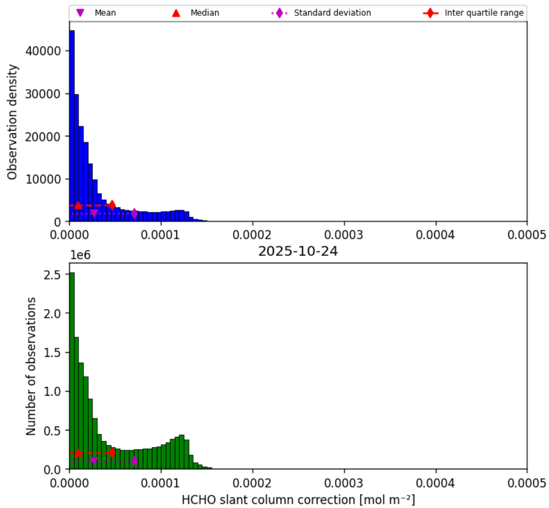
Figure 45: Histogram of “HCHO slant column correction” for 2025-10-24 to 2025-10-25
