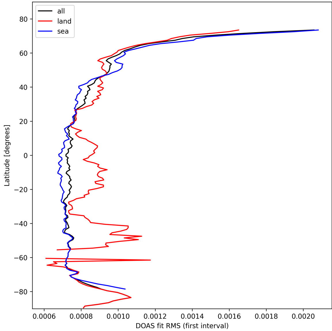
Figure 30: Zonal average of “DOAS fit RMS (first interval)” for 2025-10-24 to 2025-10-25.
