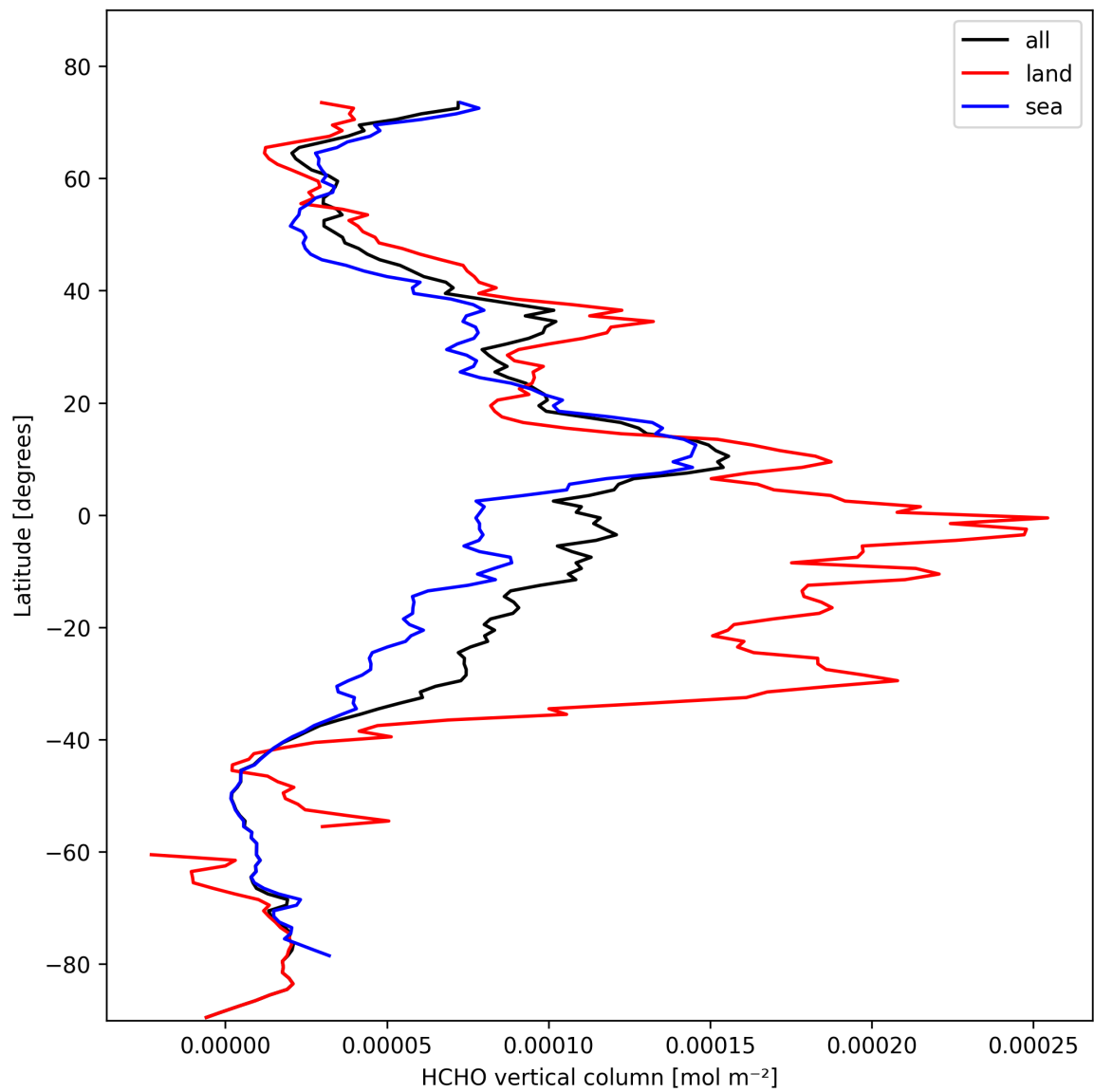
Figure 19: Zonal average of “HCHO vertical column” for 2025-10-24 to 2025-10-25.
