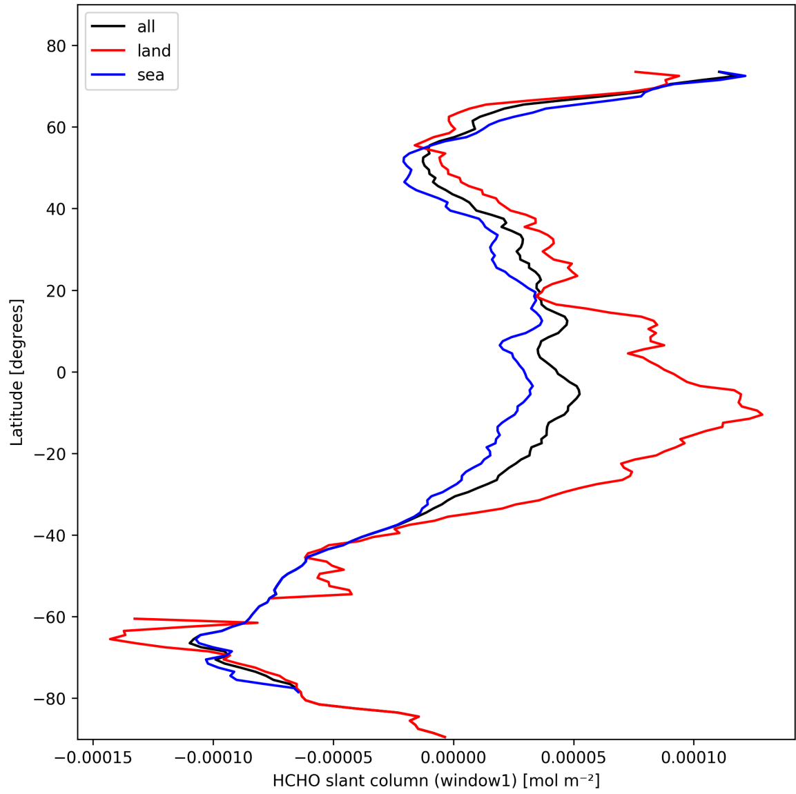
Figure 22: Zonal average of “HCHO slant column (window1)” for 2025-10-24 to 2025-10-25.
