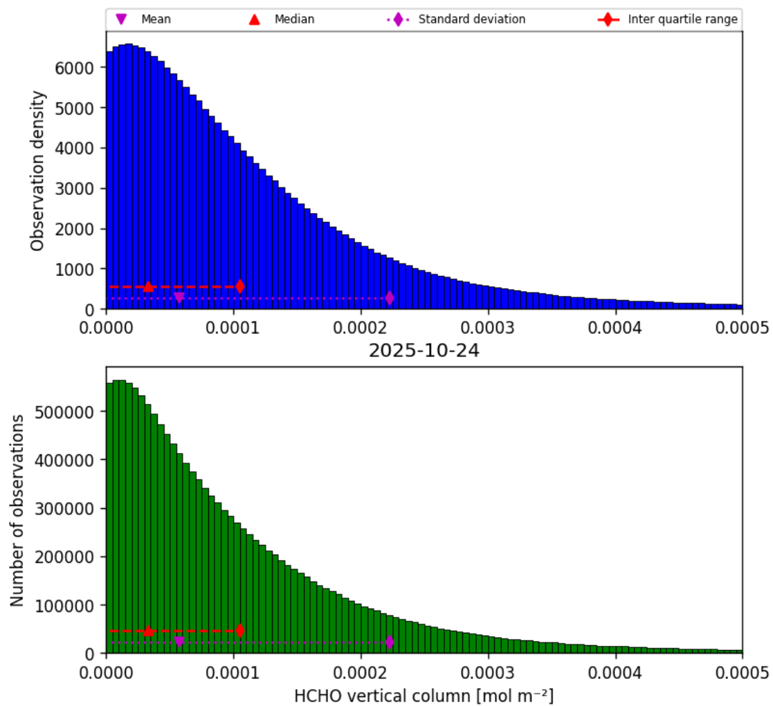
Figure 33: Histogram of “HCHO vertical column” for 2025-10-24 to 2025-10-25
