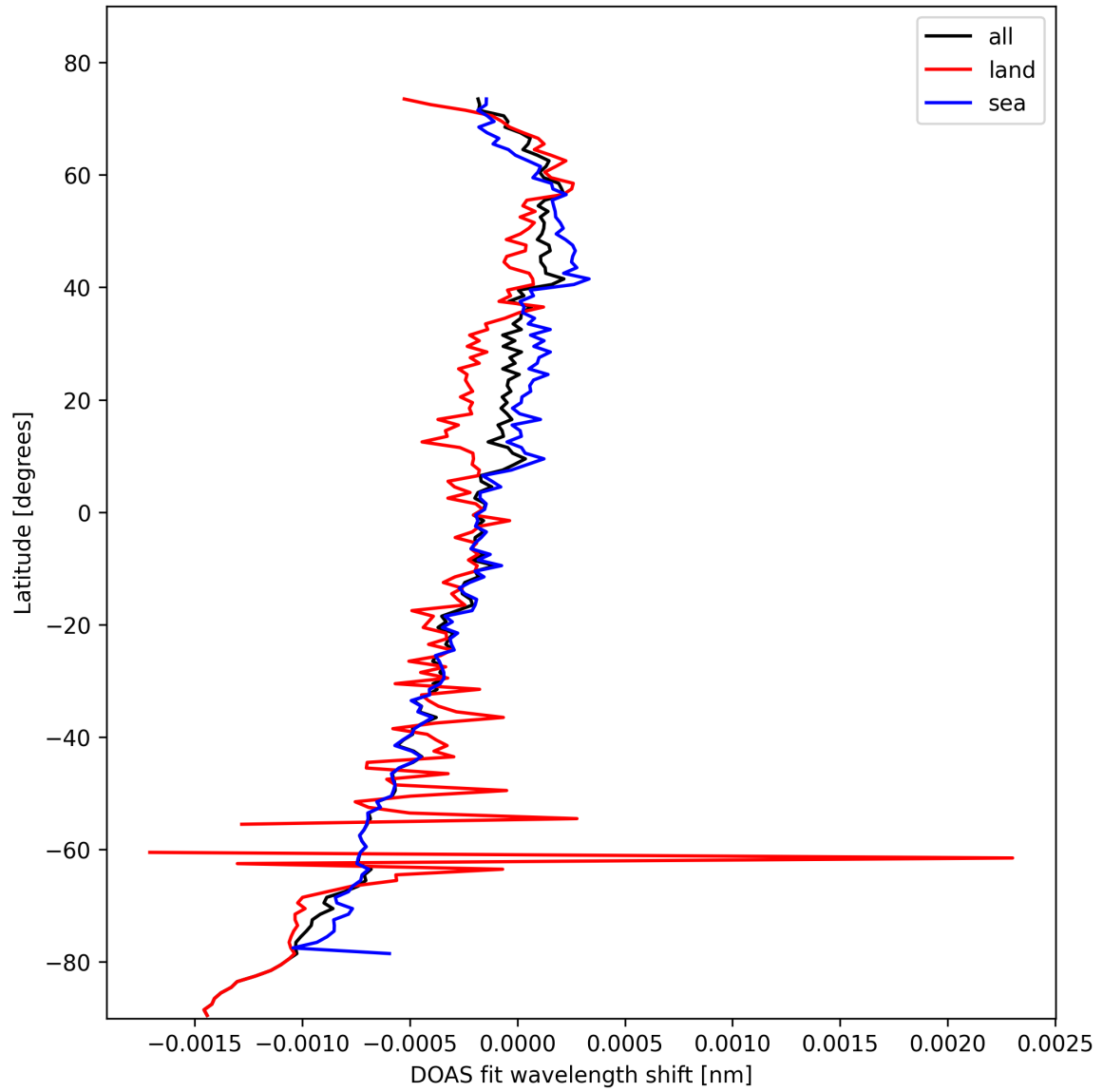
Figure 28: Zonal average of "DOAS fit wavelength shift" for 2025-10-24 to 2025-10-25.
