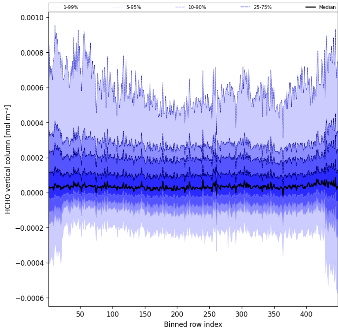
Figure 47: Along track statistics of “HCHO vertical column” for 2025-10-24 to 2025-10-25
