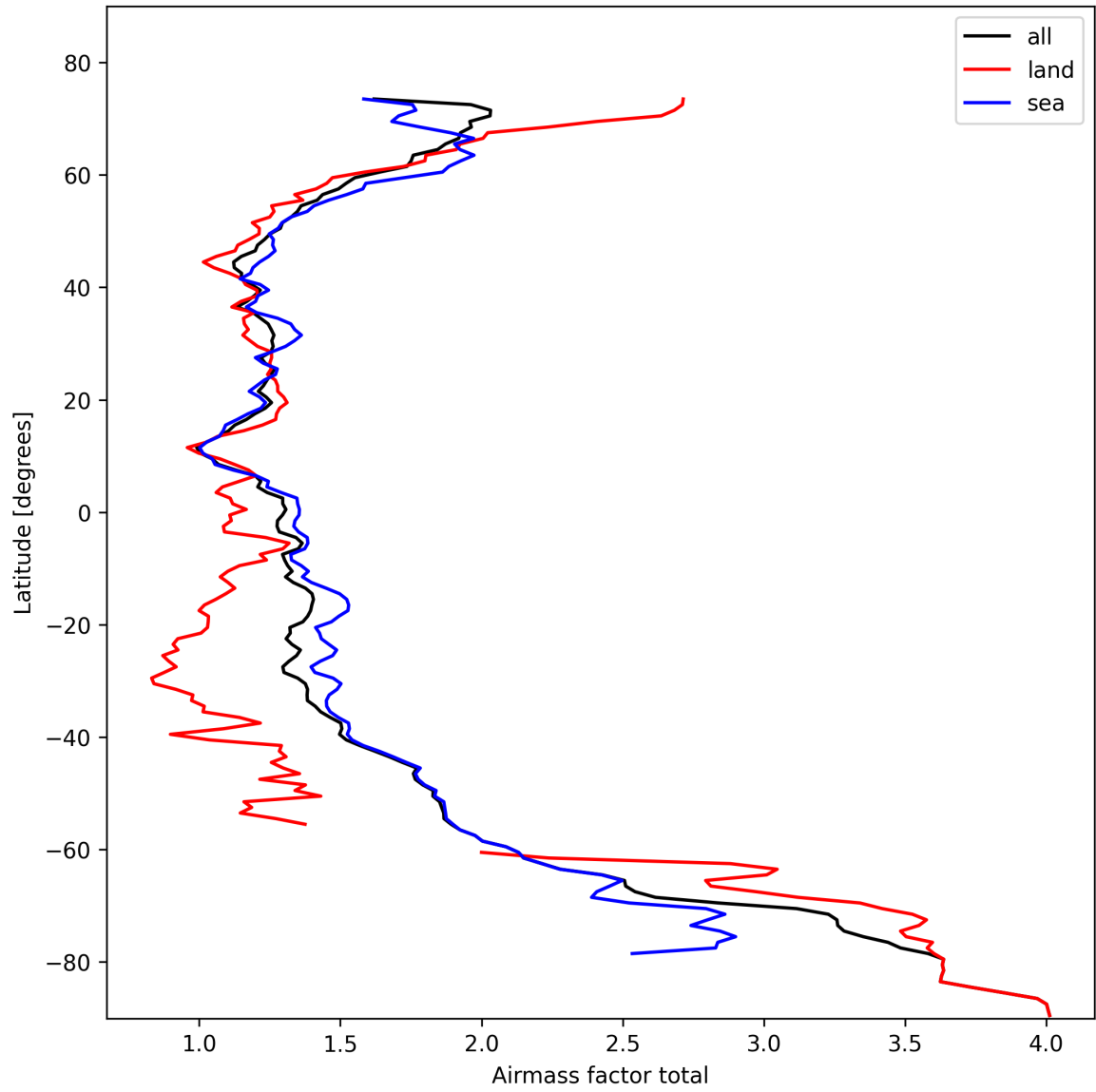
Figure 24: Zonal average of “Airmass factor total” for 2025-10-24 to 2025-10-25.
