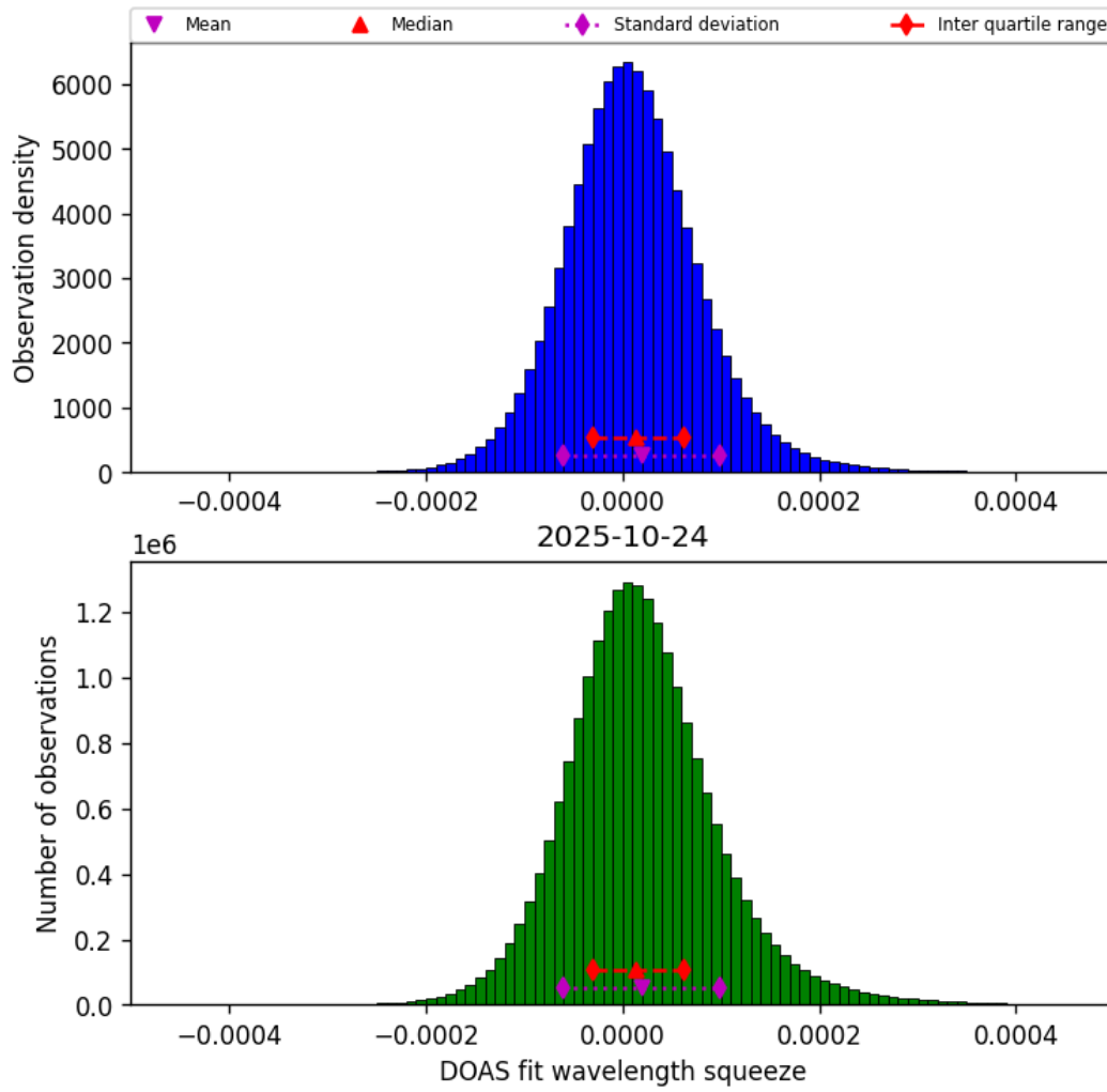
Figure 43: Histogram of “DOAS fit wavelength squeeze” for 2025-10-24 to 2025-10-25
