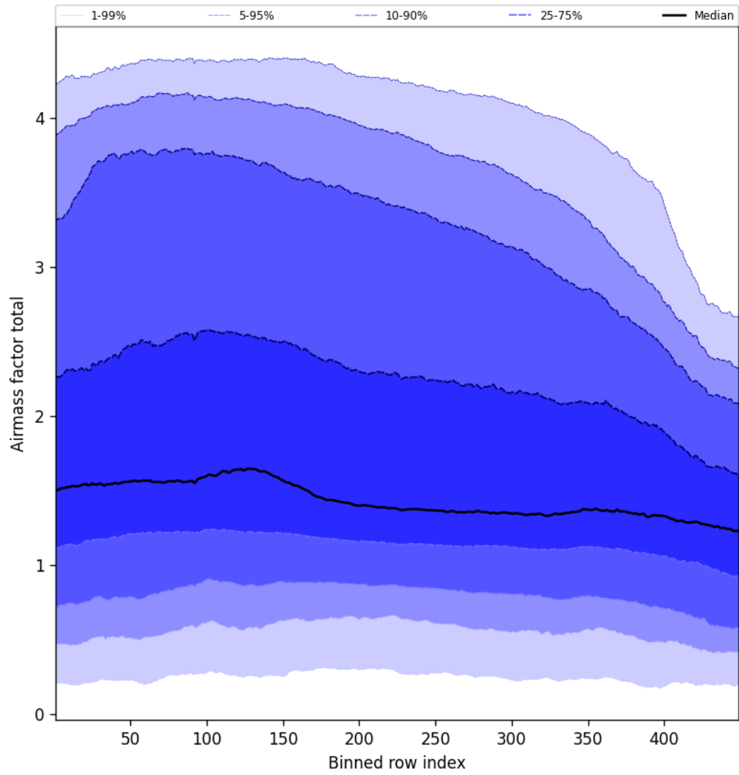
Figure 52: Along track statistics of “Airmass factor total” for 2025-10-24 to 2025-10-25
