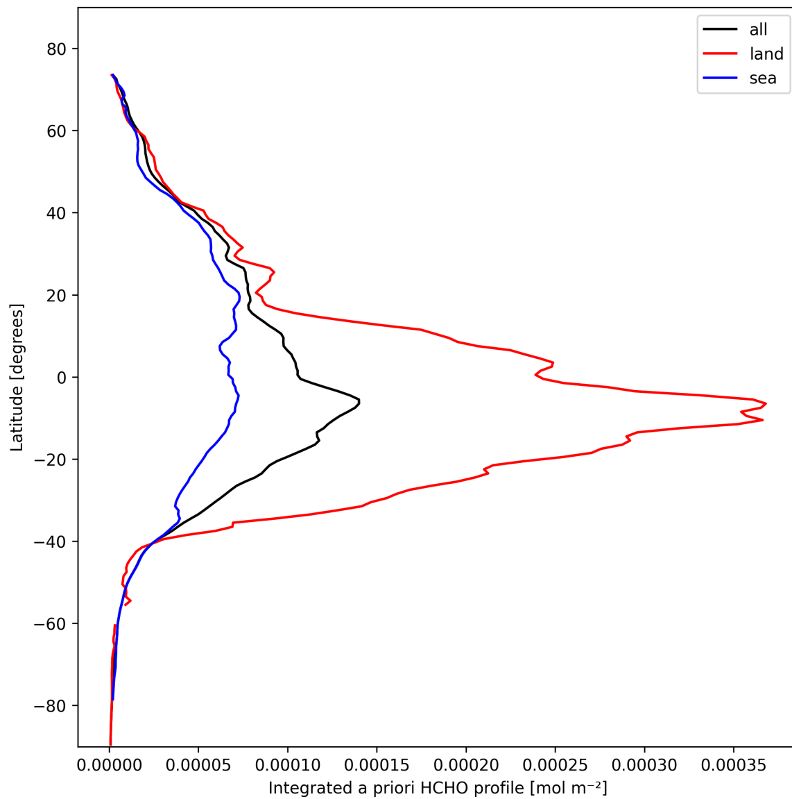
Figure 27: Zonal average of “Integrated a priori HCHO profile” for 2025-10-24 to 2025-10-25.
