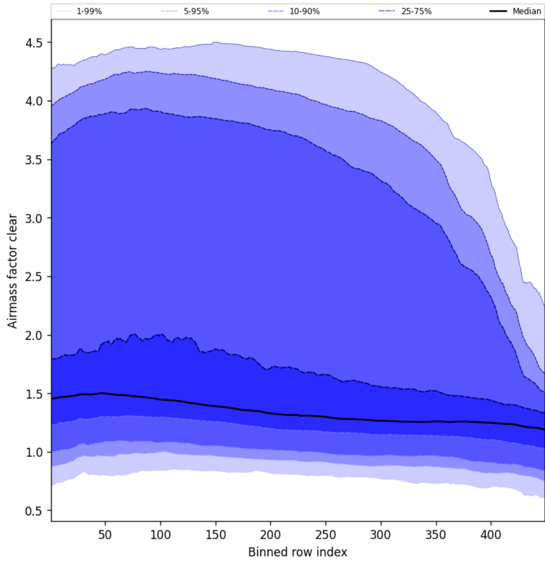
Figure 54: Along track statistics of “Airmass factor clear” for 2025-10-24 to 2025-10-25
