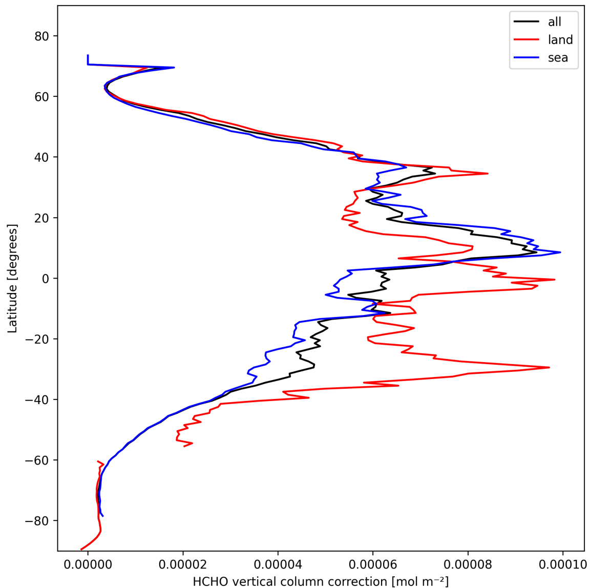
Figure 21: Zonal average of “HCHO vertical column correction” for 2025-10-24 to 2025-10-25.
