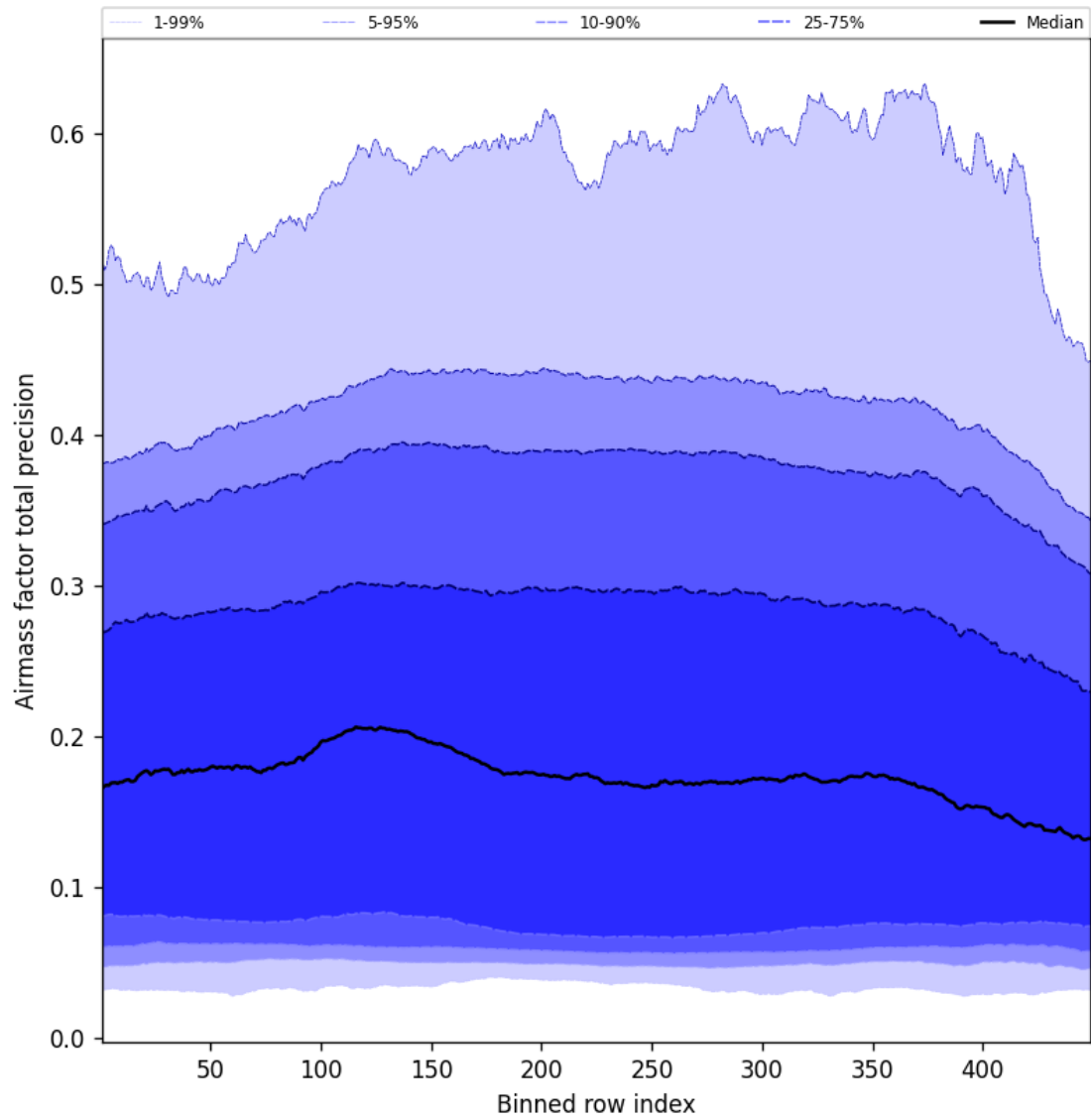
Figure 53: Along track statistics of “Airmass factor total precision” for 2025-10-24 to 2025-10-25
