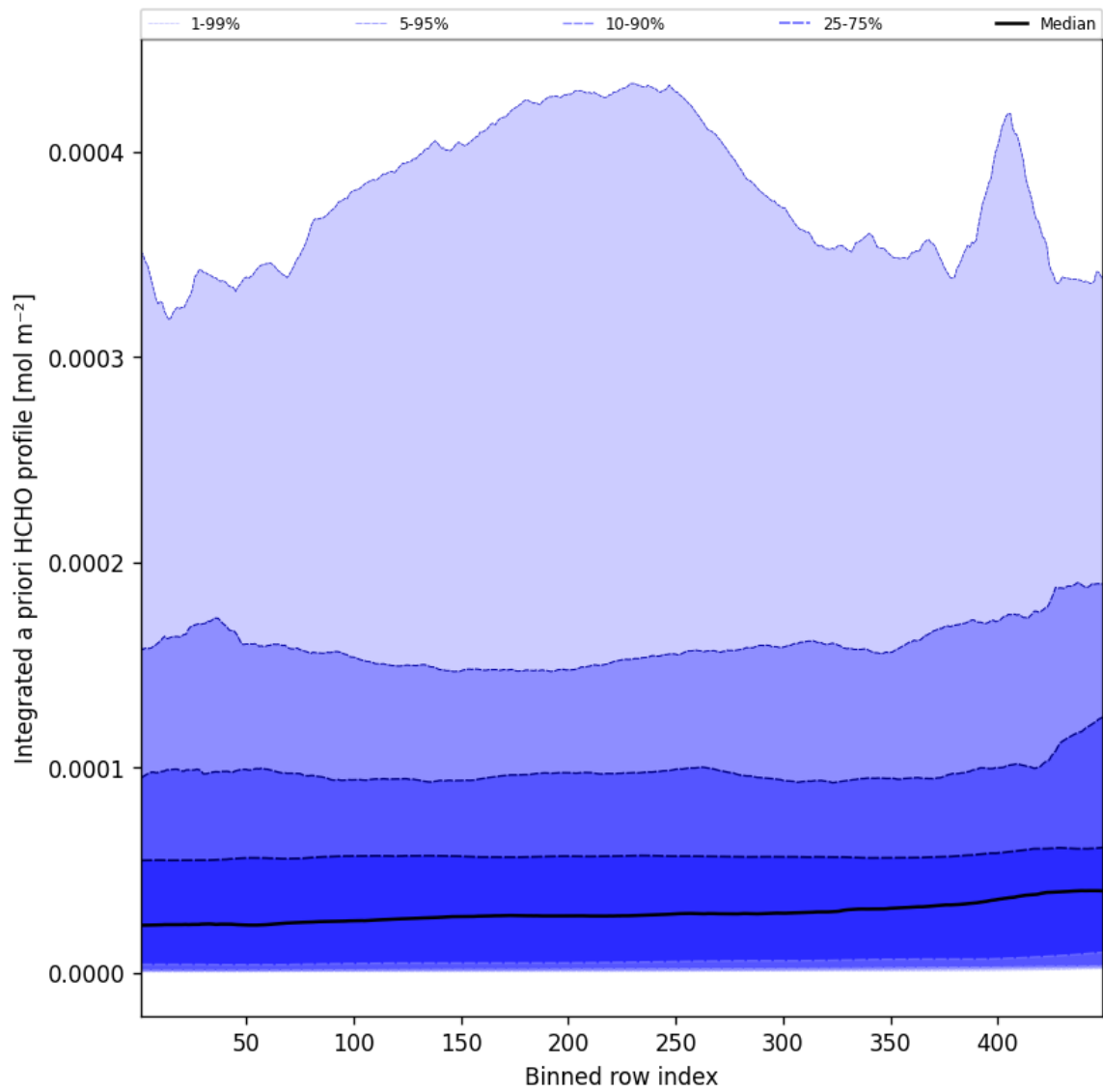
Figure 55: Along track statistics of “Integrated a priori HCHO profile” for 2025-10-24 to 2025-10-25
