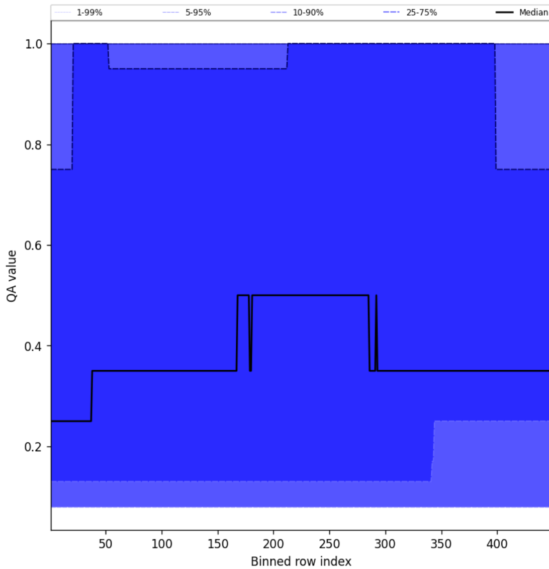
Figure 46: Along track statistics of “QA value” for 2025-10-24 to 2025-10-25
