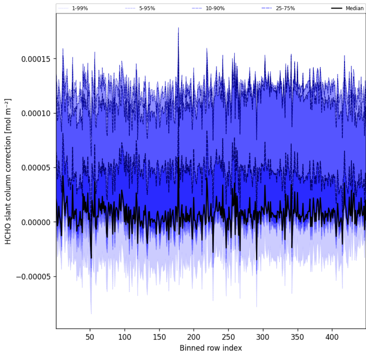
Figure 59: Along track statistics of “HCHO slant column correction” for 2025-10-24 to 2025-10-25
