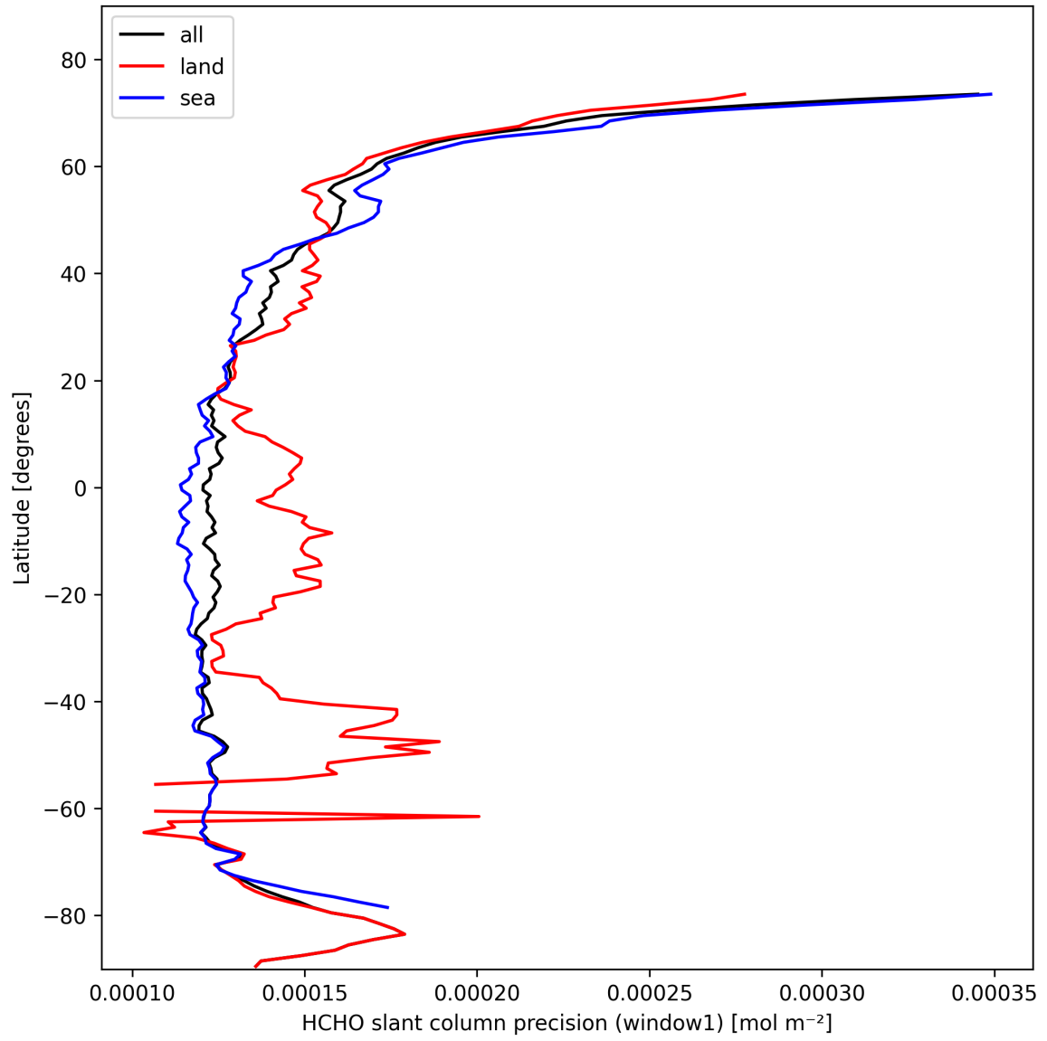
Figure 23: Zonal average of “HCHO slant column precision (window1)” for 2025-10-24 to 2025-10-25.
