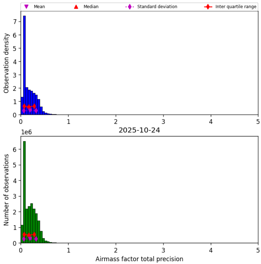
Figure 39: Histogram of “Airmass factor total precision” for 2025-10-24 to 2025-10-25
