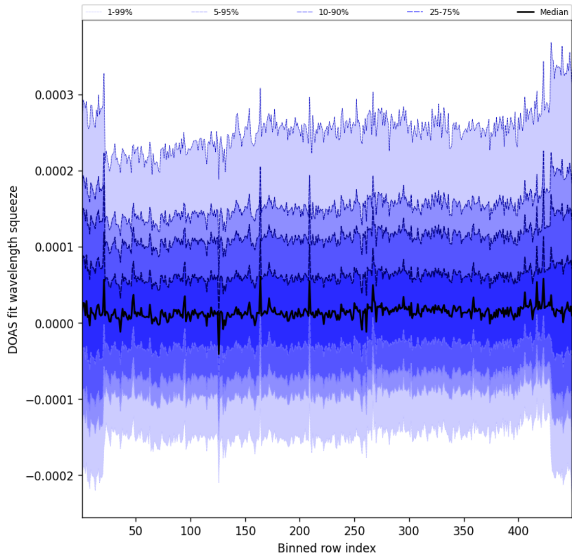
Figure 57: Along track statistics of “DOAS fit wavelength squeeze” for 2025-10-24 to 2025-10-25
