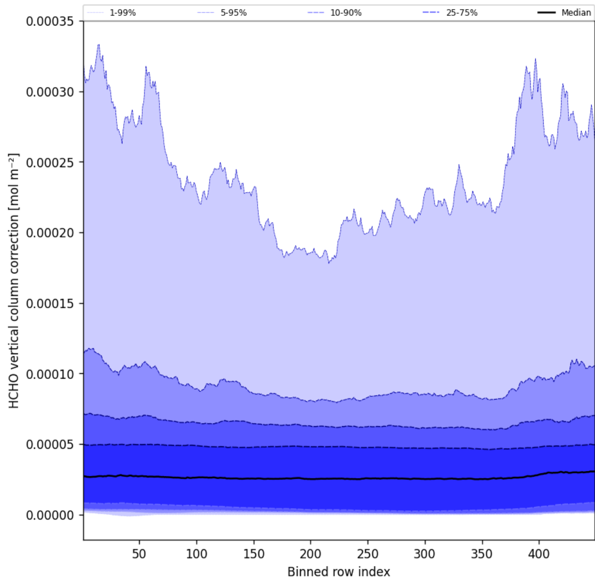
Figure 49: Along track statistics of “HCHO vertical column correction” for 2025-10-24 to 2025-10-25
