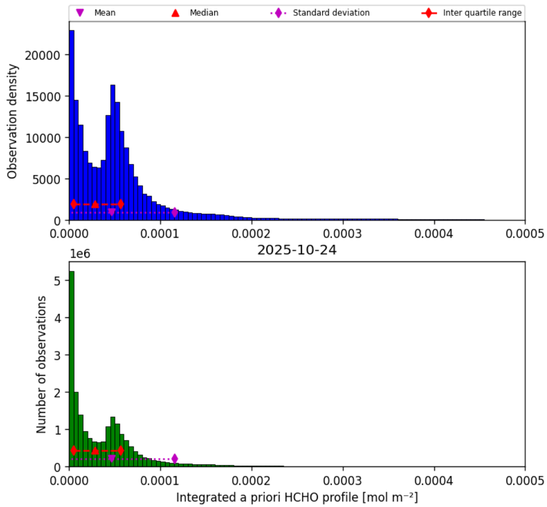
Figure 41: Histogram of “Integrated a priori HCHO profile” for 2025-10-24 to 2025-10-25
