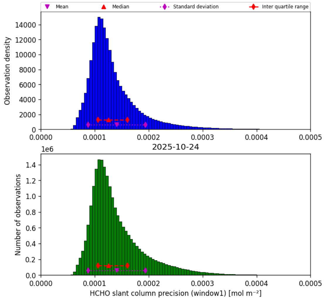
Figure 37: Histogram of “HCHO slant column precision (window1)” for 2025-10-24 to 2025-10-25
