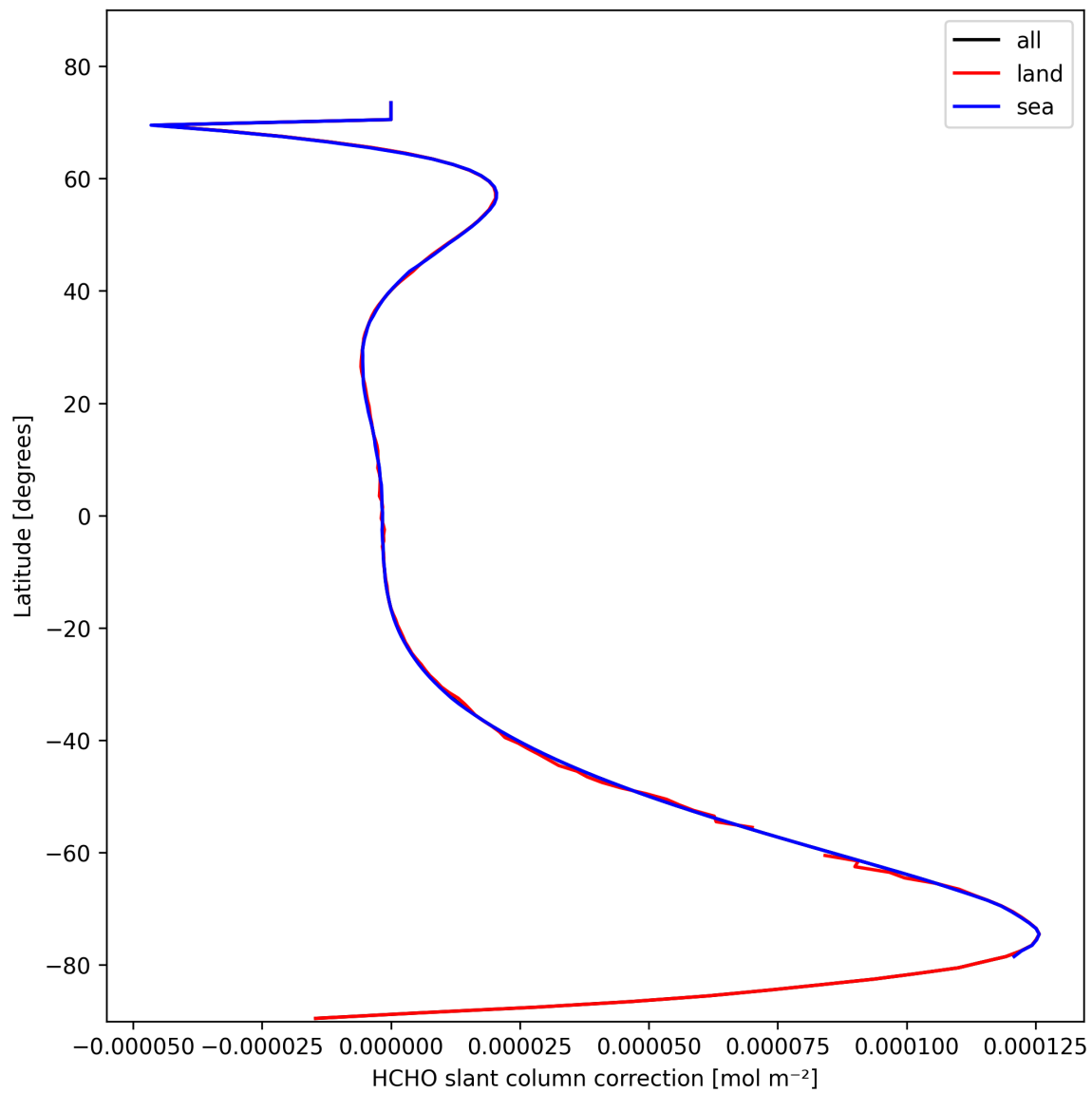
Figure 31: Zonal average of “HCHO slant column correction” for 2025-10-24 to 2025-10-25.
