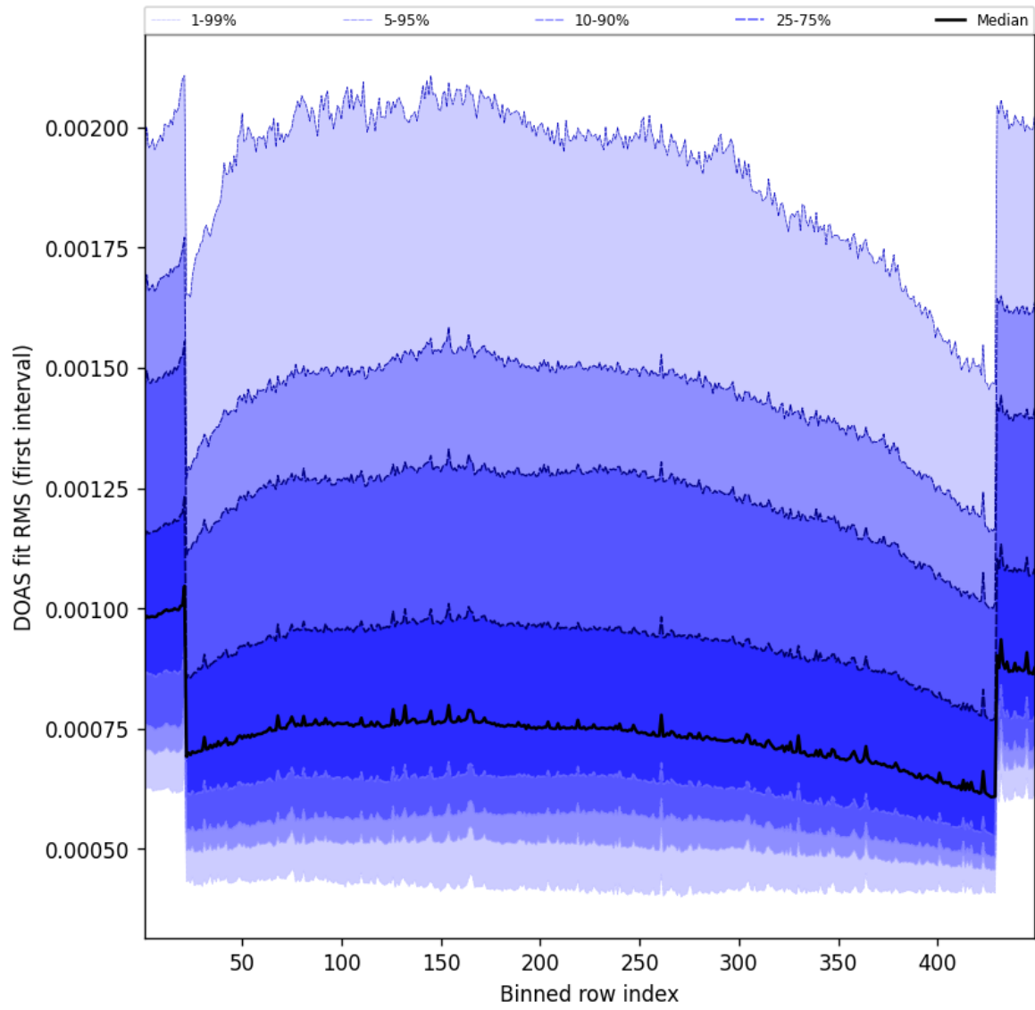
Figure 58: Along track statistics of “DOAS fit RMS (first interval)” for 2025-10-24 to 2025-10-25
