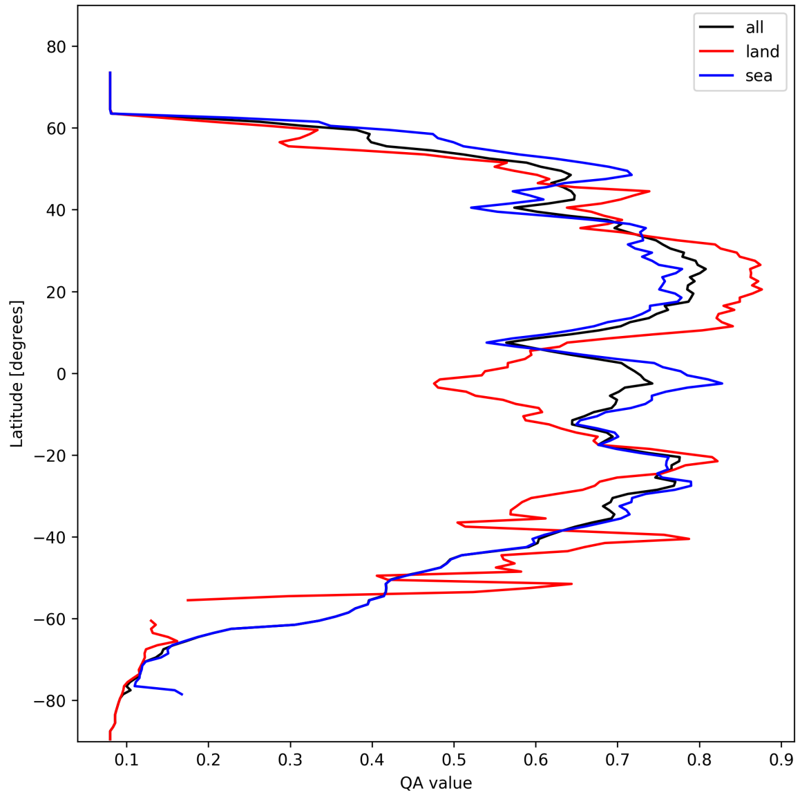
Figure 18: Zonal average of “QA value” for 2025-10-24 to 2025-10-25.
