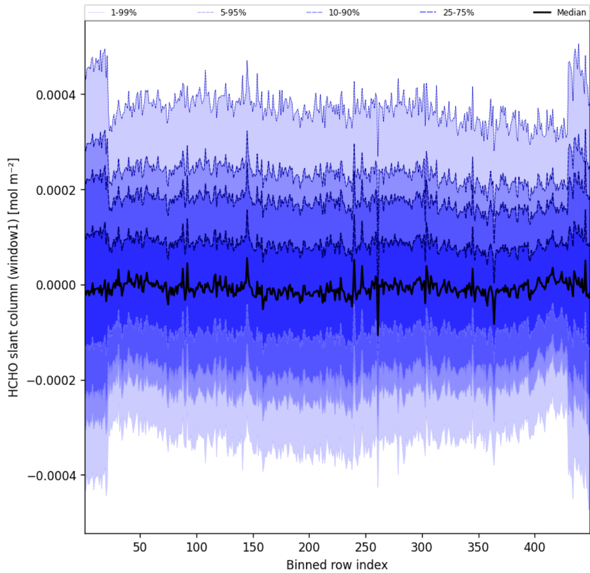
Figure 50: Along track statistics of “HCHO slant column (window1)” for 2025-10-24 to 2025-10-25
