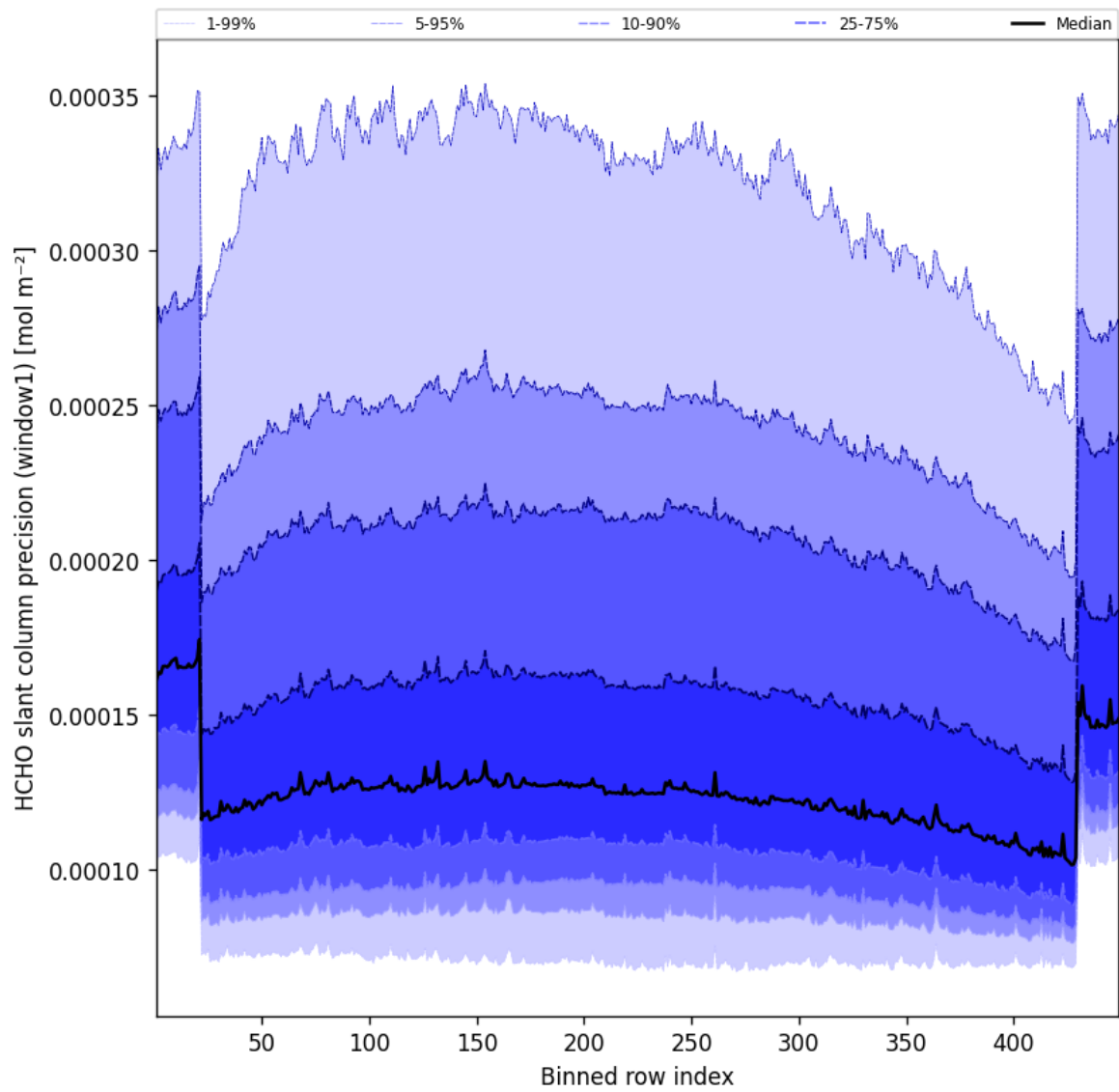
Figure 51: Along track statistics of “HCHO slant column precision (window1)” for 2025-10-24 to 2025-10-25
