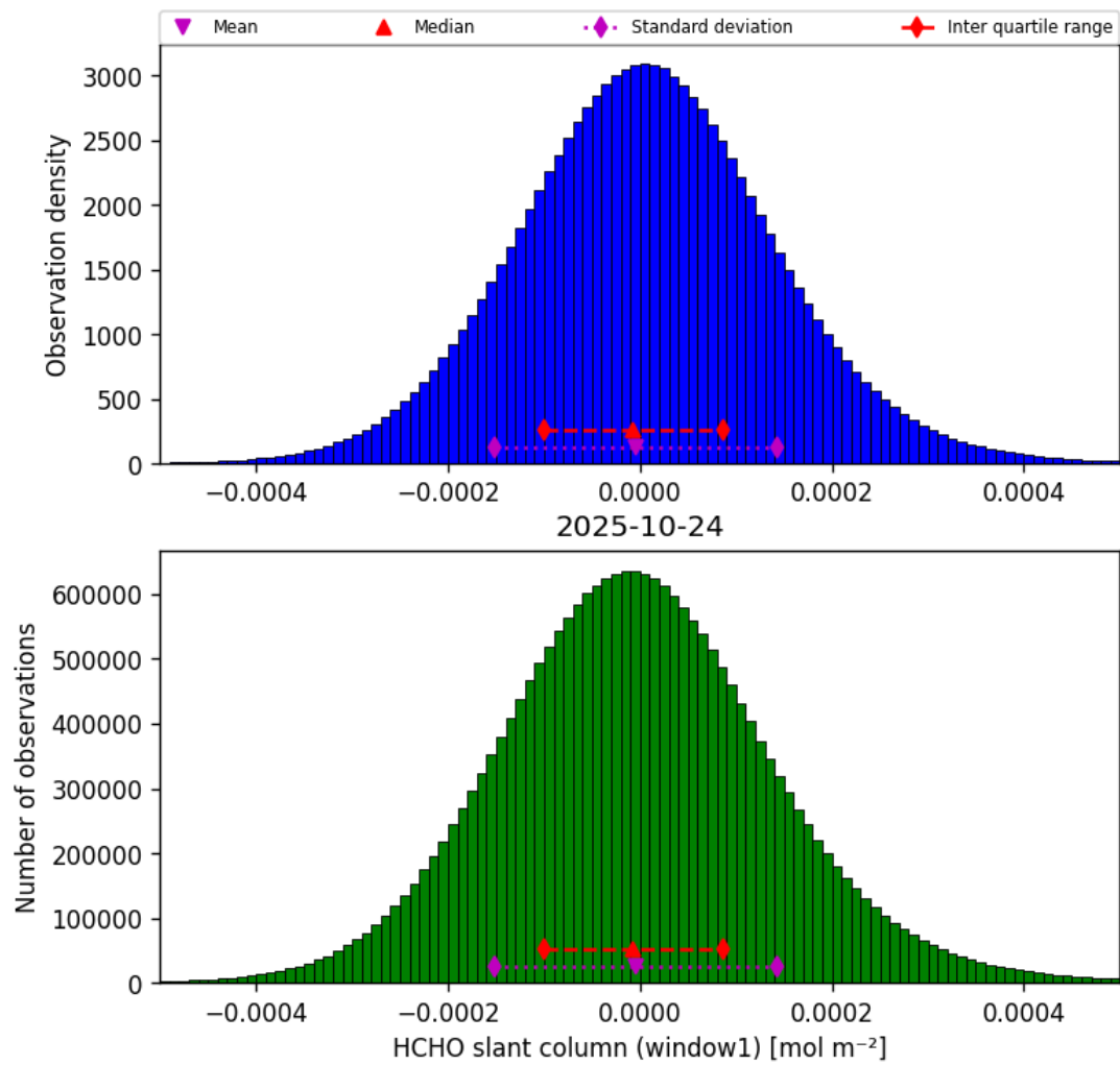
Figure 36: Histogram of “HCHO slant column (window1)” for 2025-10-24 to 2025-10-25
