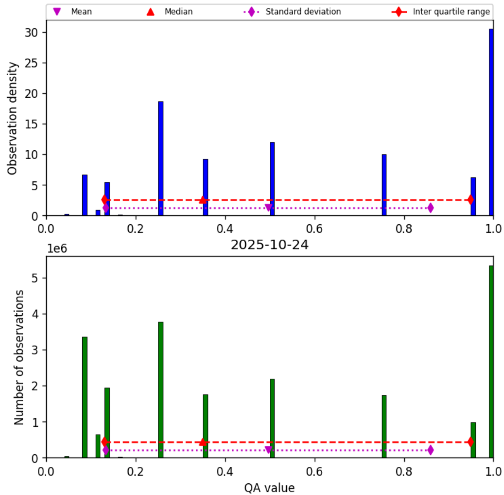
Figure 32: Histogram of “QA value” for 2025-10-24 to 2025-10-25
