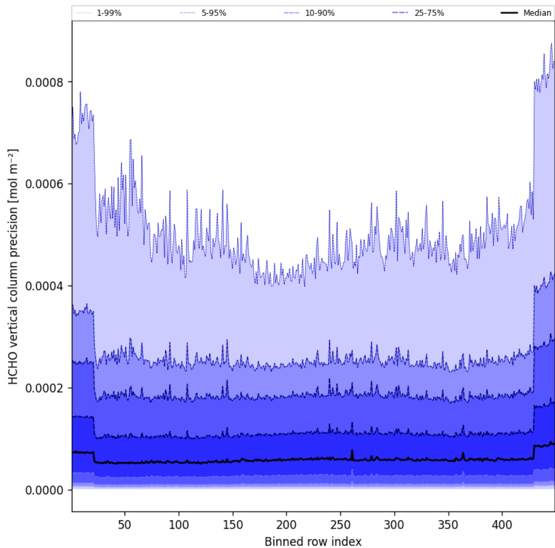
Figure 48: Along track statistics of "HCHO vertical column precision" for 2025-10-24 to 2025-10-25
