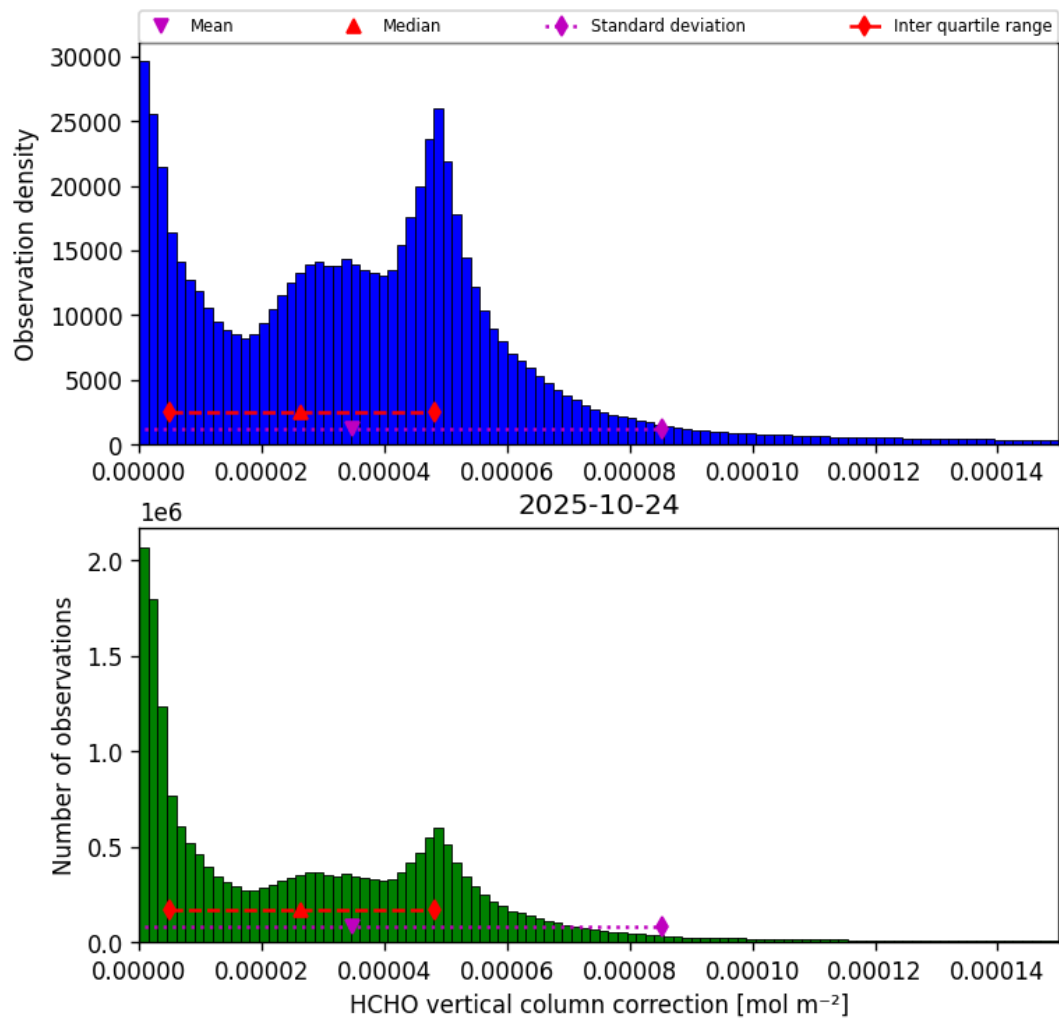
Figure 35: Histogram of “HCHO vertical column correction” for 2025-10-24 to 2025-10-25
