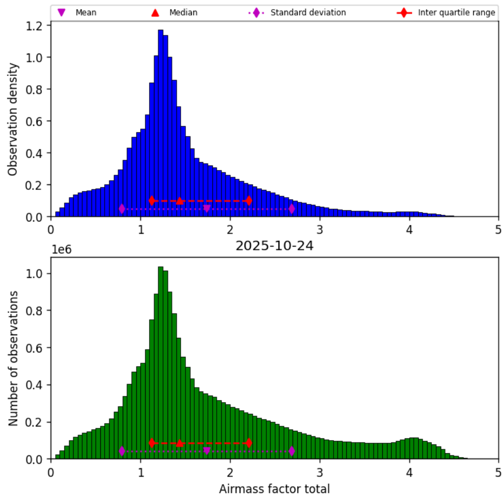
Figure 38: Histogram of “Airmass factor total” for 2025-10-24 to 2025-10-25
