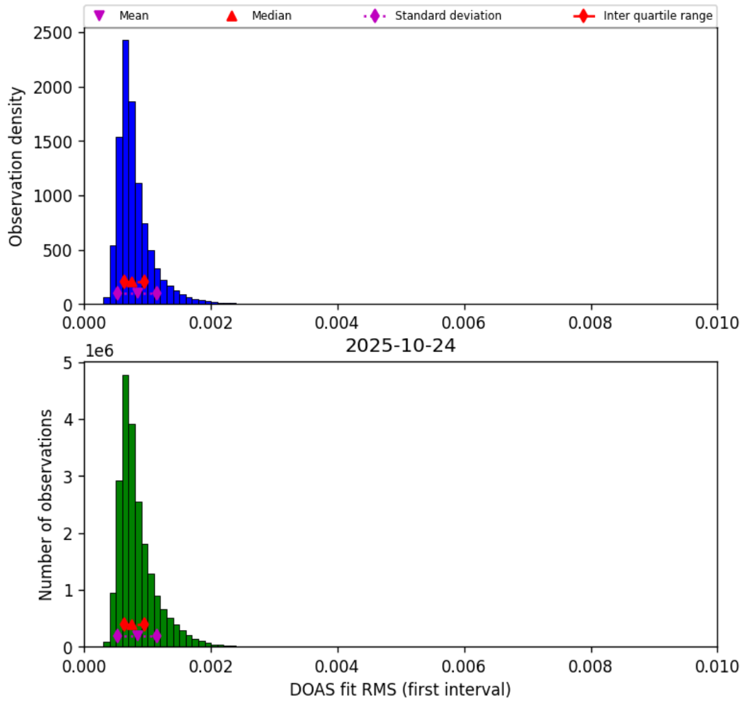
Figure 44: Histogram of “DOAS fit RMS (first interval)” for 2025-10-24 to 2025-10-25
