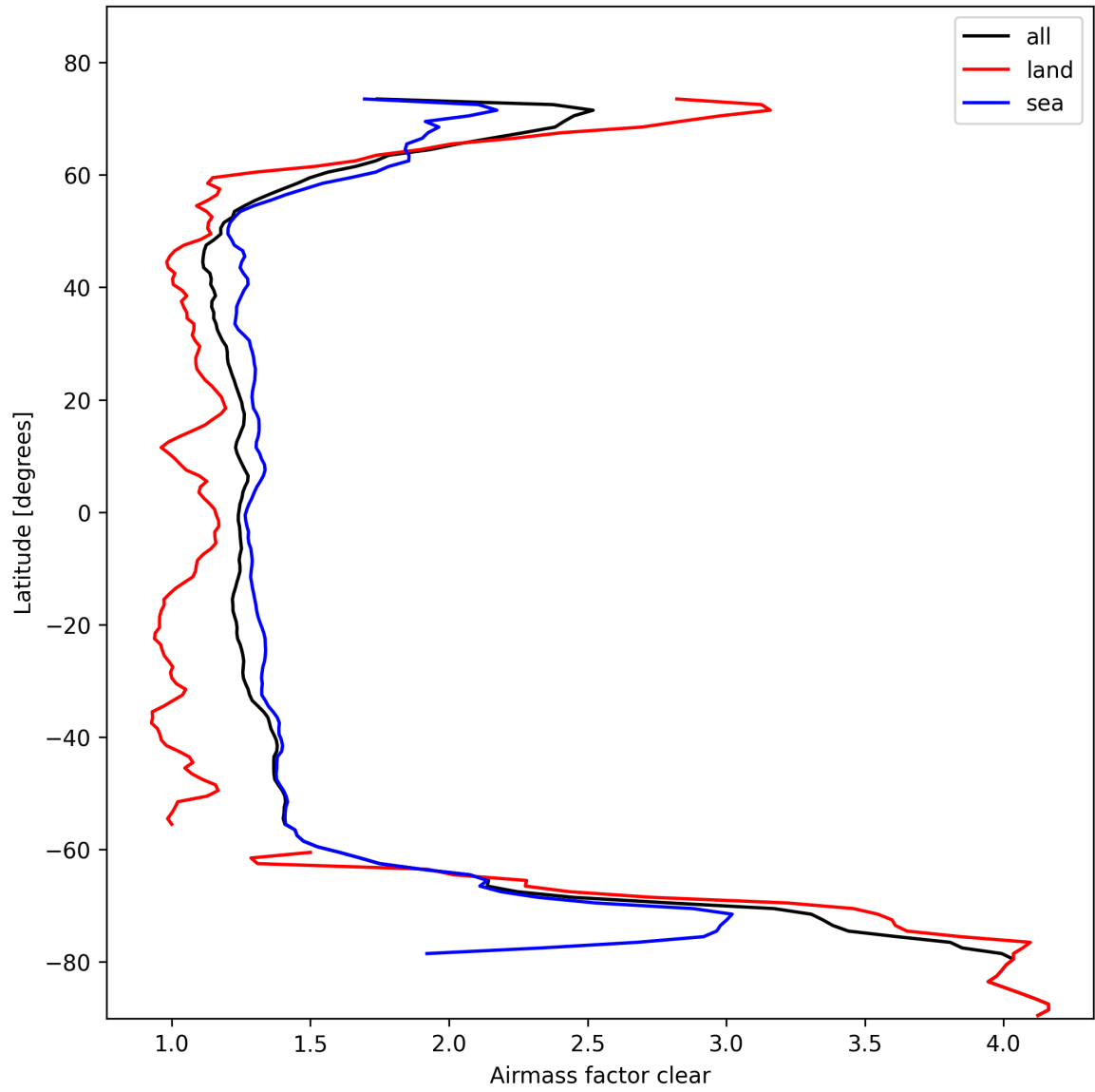
Figure 26: Zonal average of “Airmass factor clear” for 2025-10-24 to 2025-10-25.
