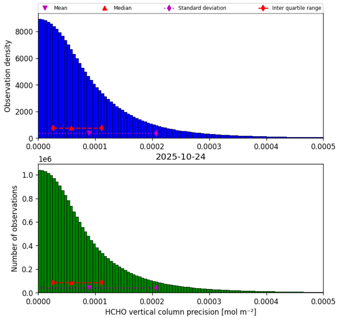
Figure 34: Histogram of “HCHO vertical column precision” for 2025-10-24 to 2025-10-25
