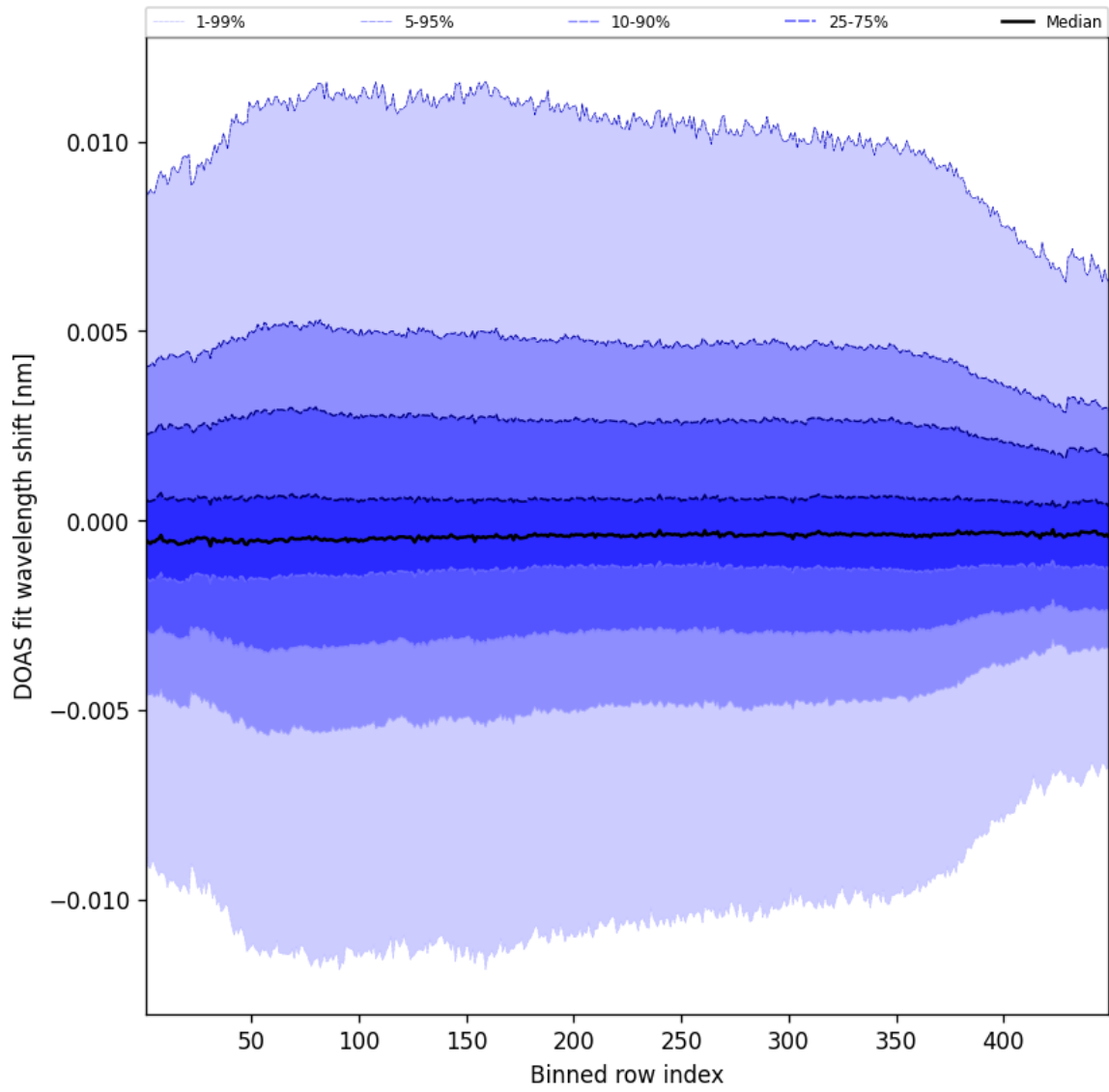
Figure 56: Along track statistics of “DOAS fit wavelength shift” for 2025-10-24 to 2025-10-25
