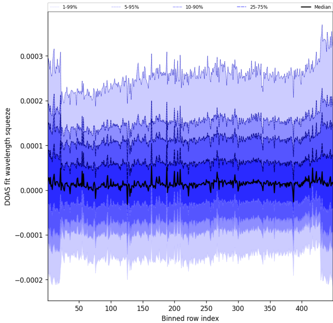
Figure 57: Along track statistics of “DOAS fit wavelength squeeze” for 2025-10-25 to 2025-10-25
