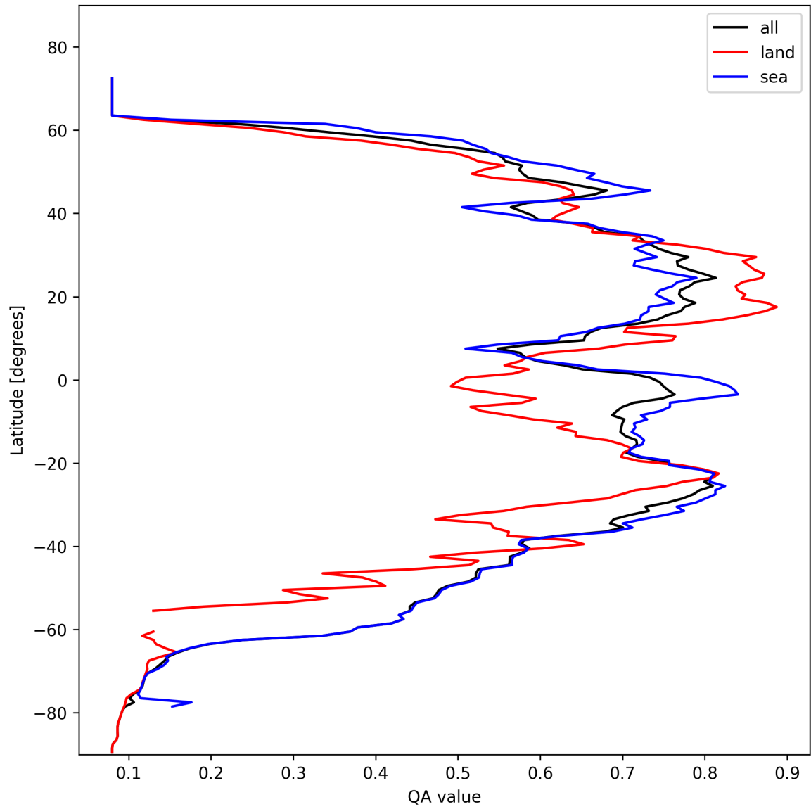
Figure 18: Zonal average of “QA value” for 2025-10-25 to 2025-10-25.
