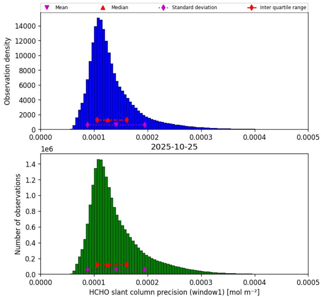
Figure 37: Histogram of “HCHO slant column precision (window1)” for 2025-10-25 to 2025-10-25
