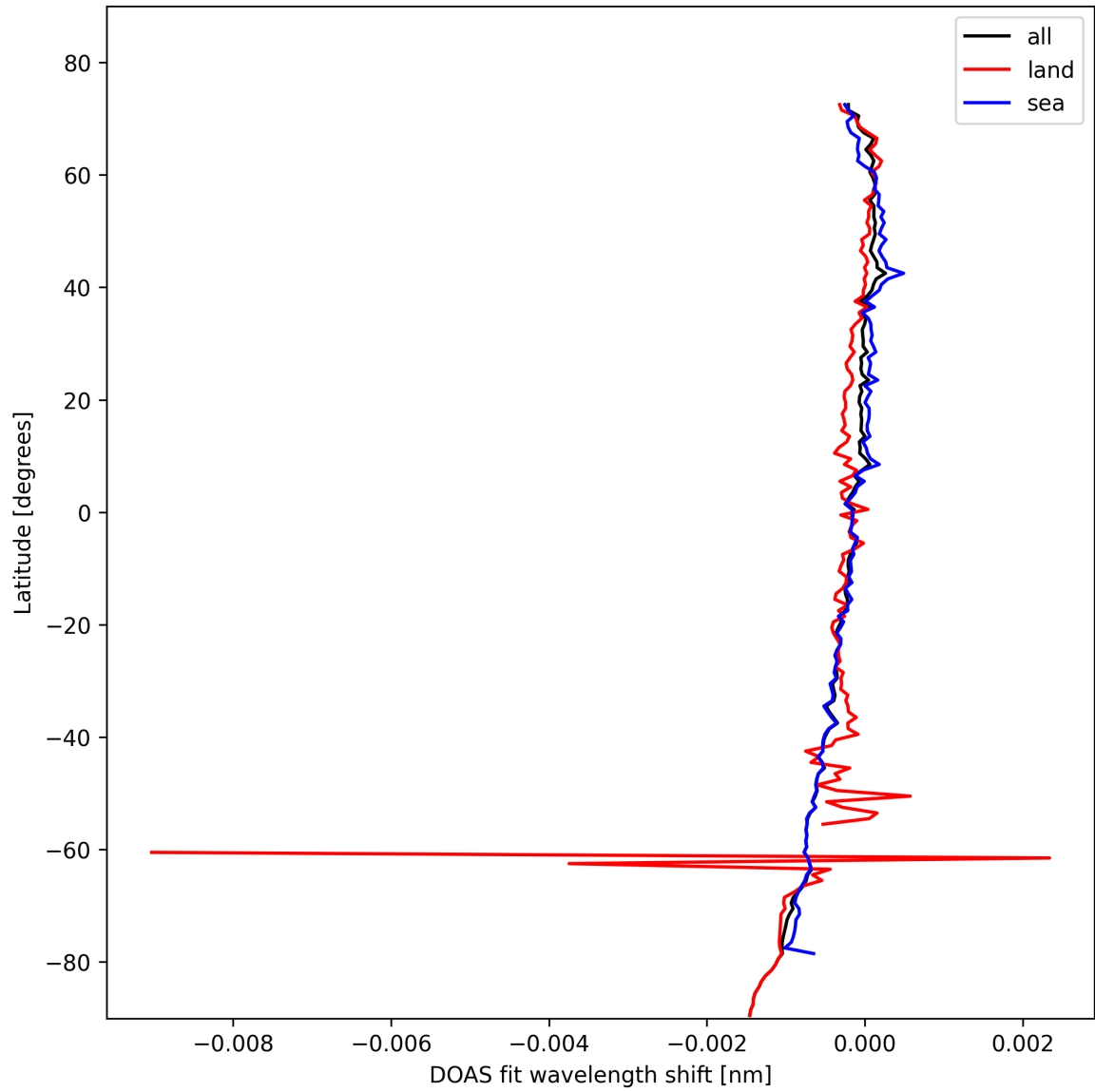
Figure 28: Zonal average of “DOAS fit wavelength shift” for 2025-10-25 to 2025-10-25.
