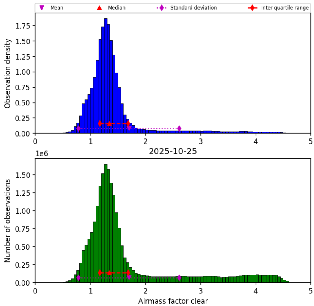
Figure 40: Histogram of “Airmass factor clear” for 2025-10-25 to 2025-10-25
