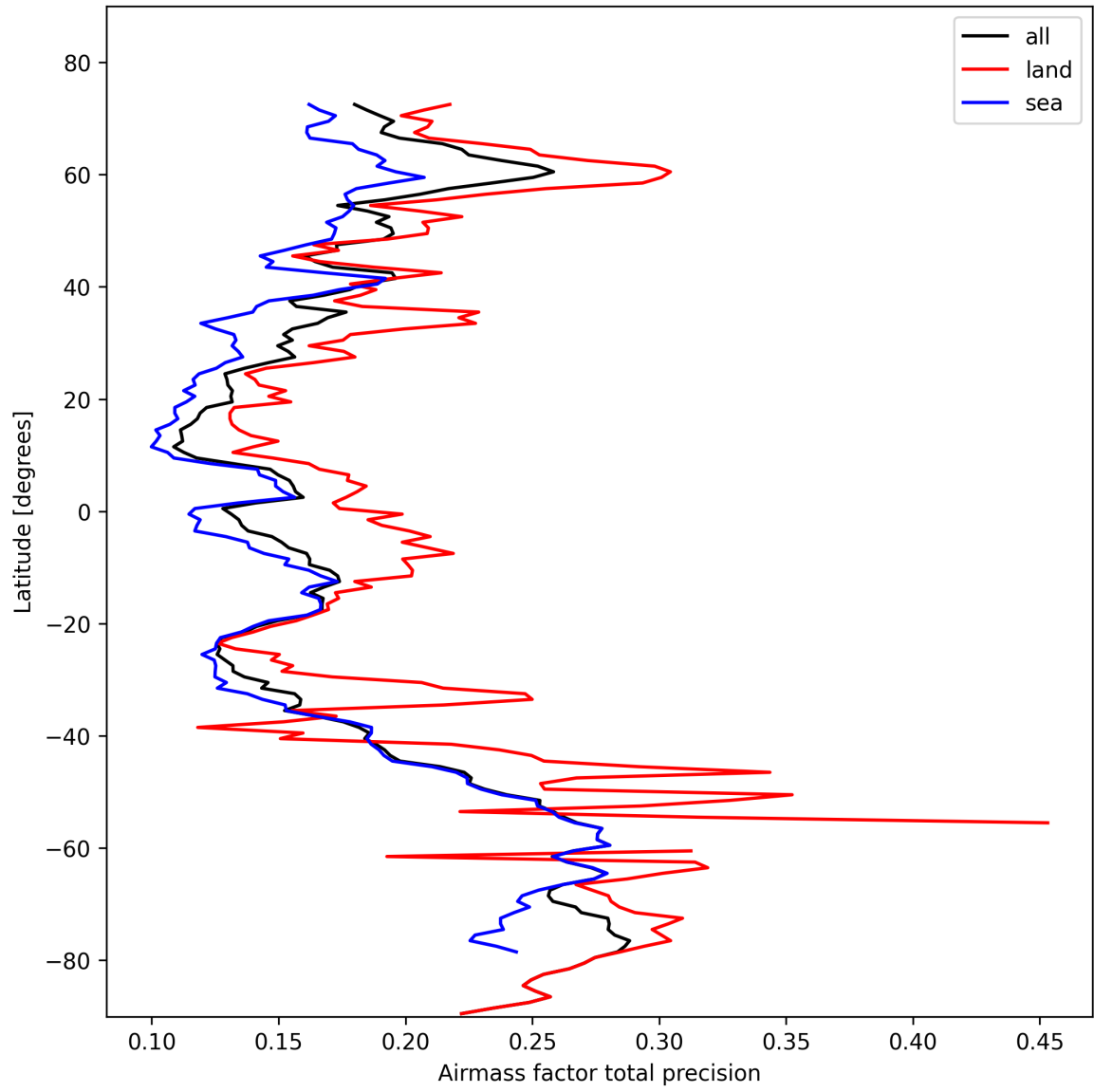
Figure 25: Zonal average of “Airmass factor total precision” for 2025-10-25 to 2025-10-25.
