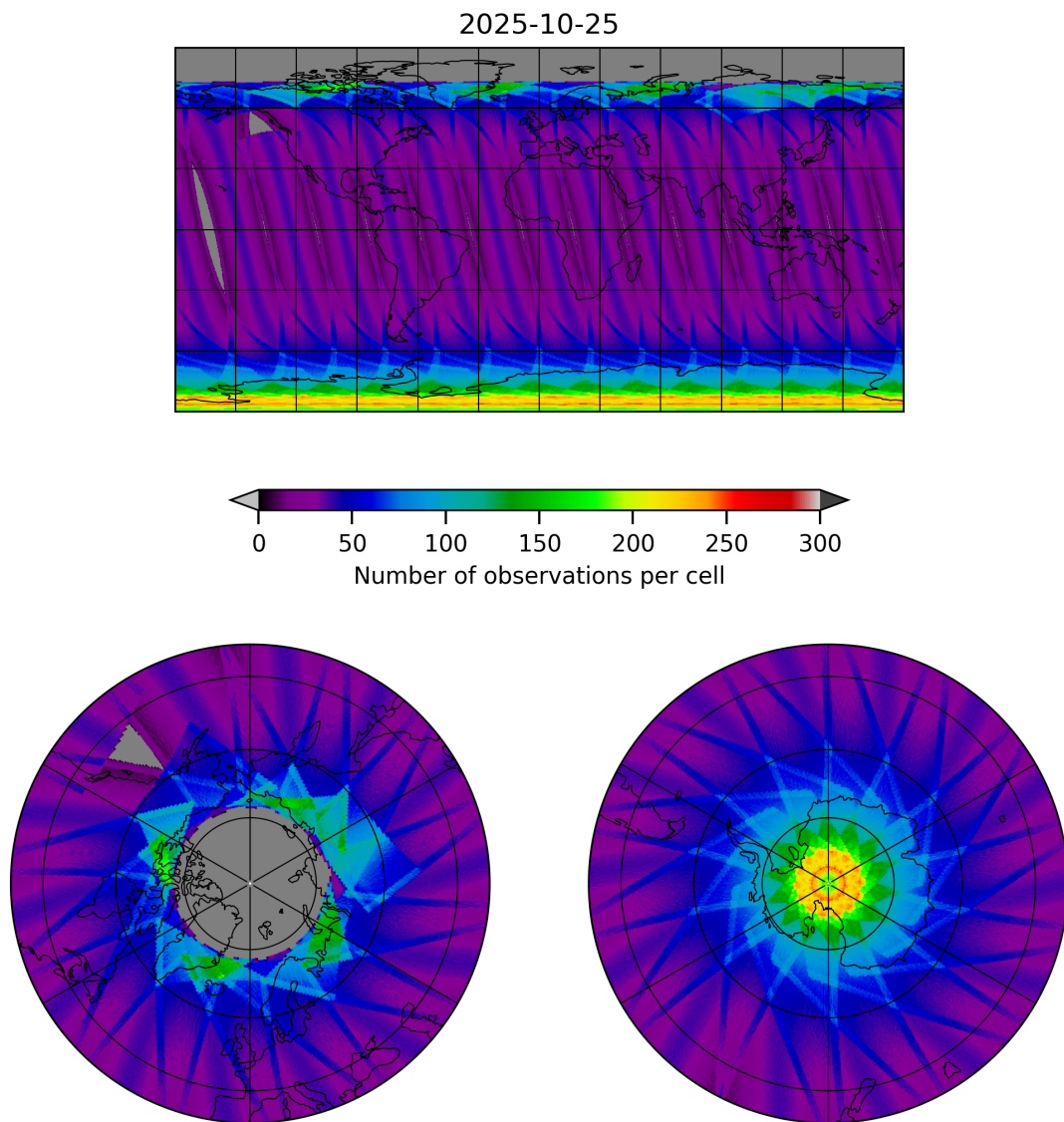
Figure 17: Map of the number of observations for 2025-10-25 to 2025-10-25
