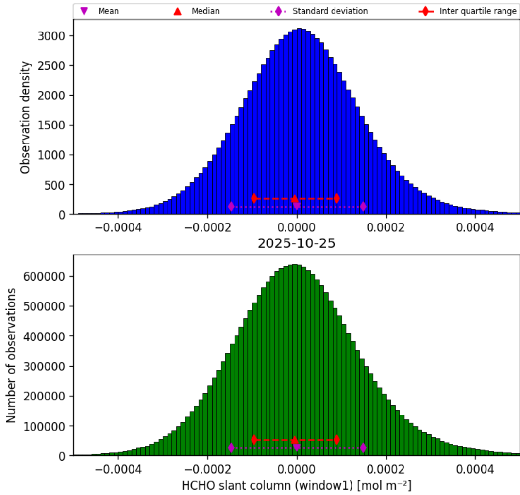
Figure 36: Histogram of “HCHO slant column (window1)” for 2025-10-25 to 2025-10-25
