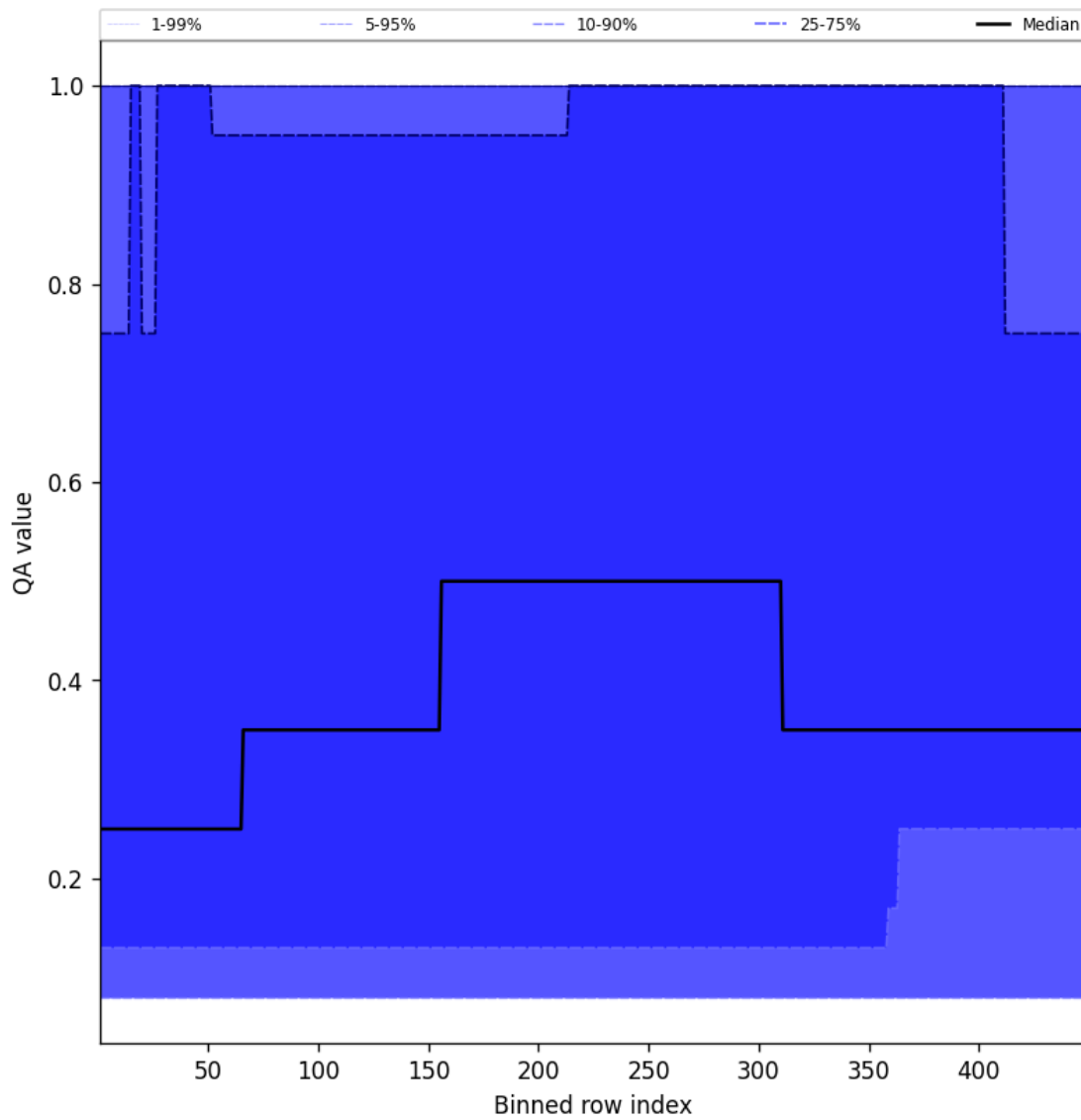
Figure 46: Along track statistics of “QA value” for 2025-10-25 to 2025-10-25
