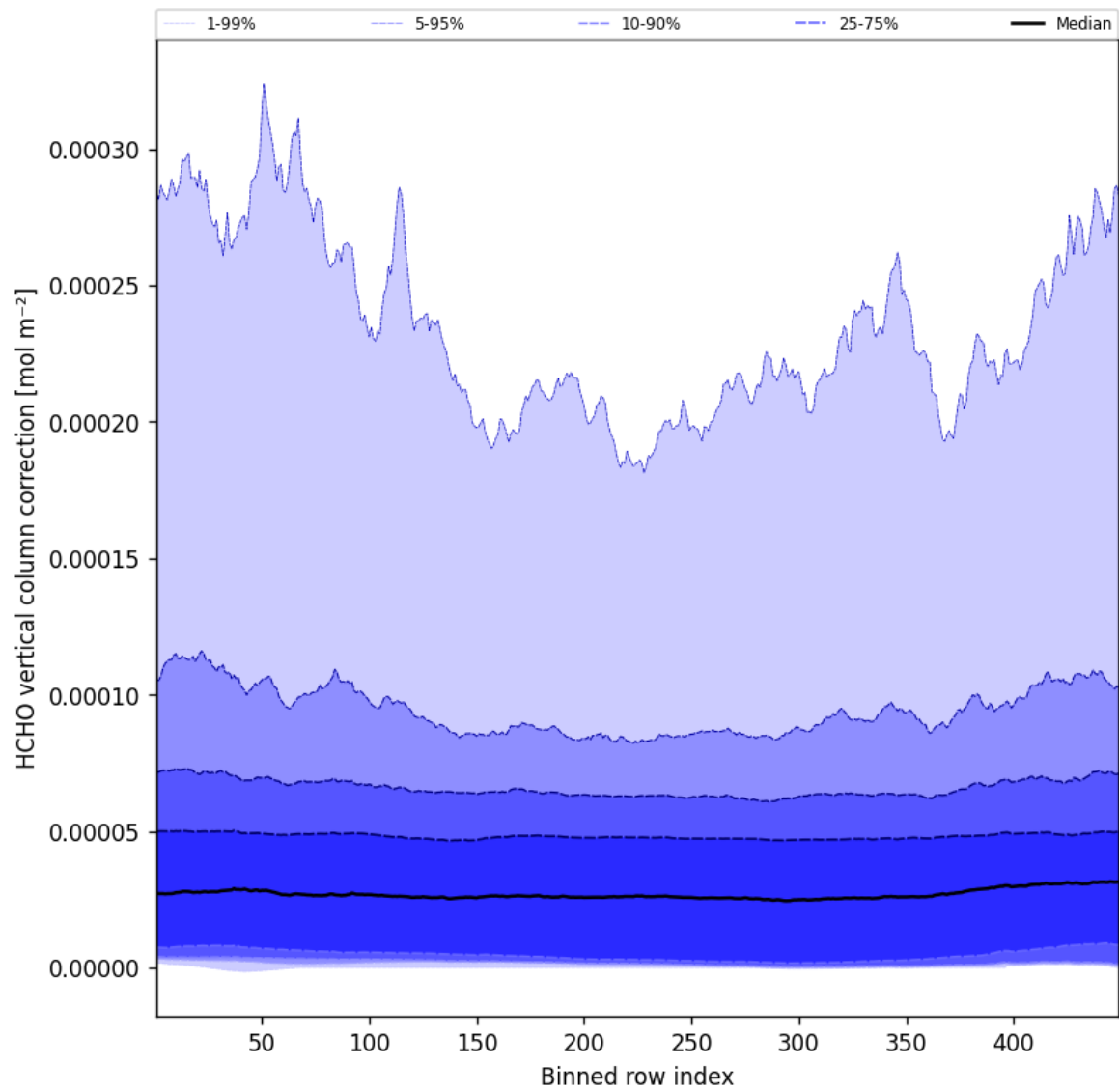
Figure 49: Along track statistics of “HCHO vertical column correction” for 2025-10-25 to 2025-10-25
