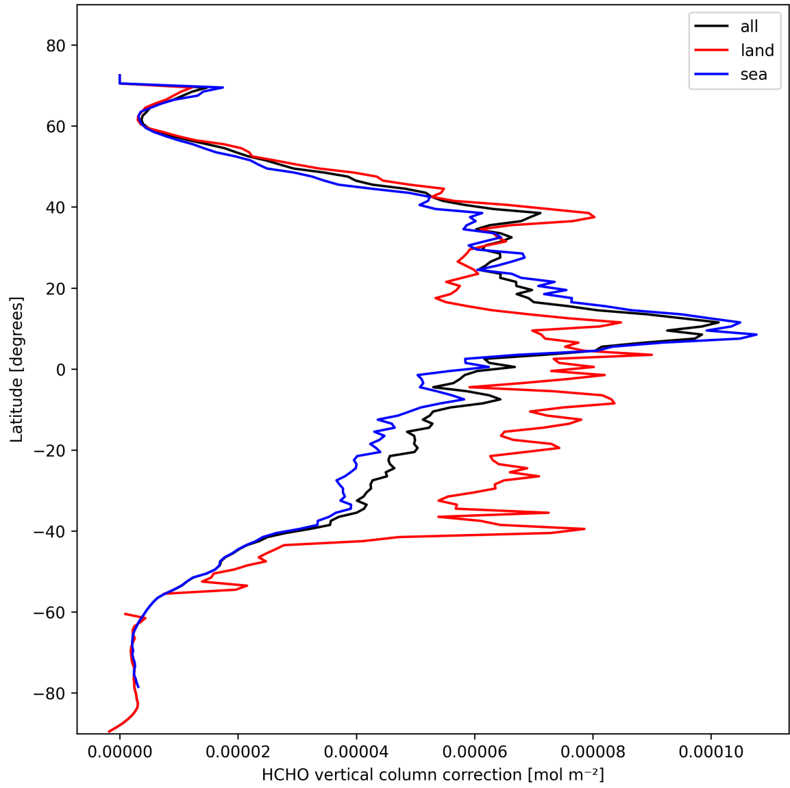
Figure 21: Zonal average of “HCHO vertical column correction” for 2025-10-25 to 2025-10-25.
