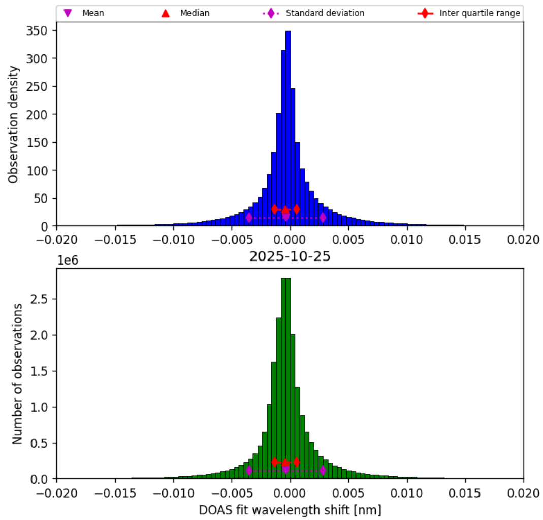
Figure 42: Histogram of “DOAS fit wavelength shift” for 2025-10-25 to 2025-10-25
