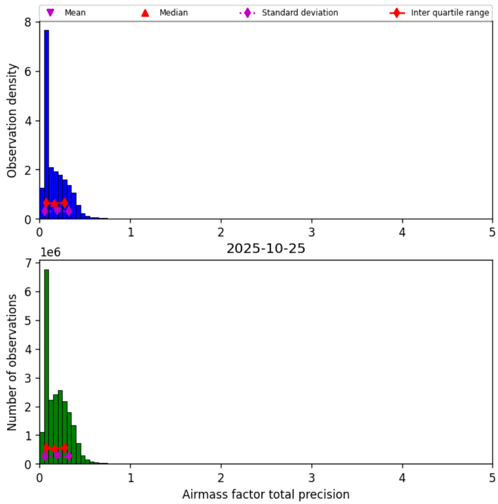
Figure 39: Histogram of “Airmass factor total precision” for 2025-10-25 to 2025-10-25
