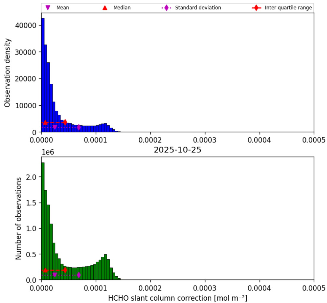
Figure 45: Histogram of “HCHO slant column correction” for 2025-10-25 to 2025-10-25
