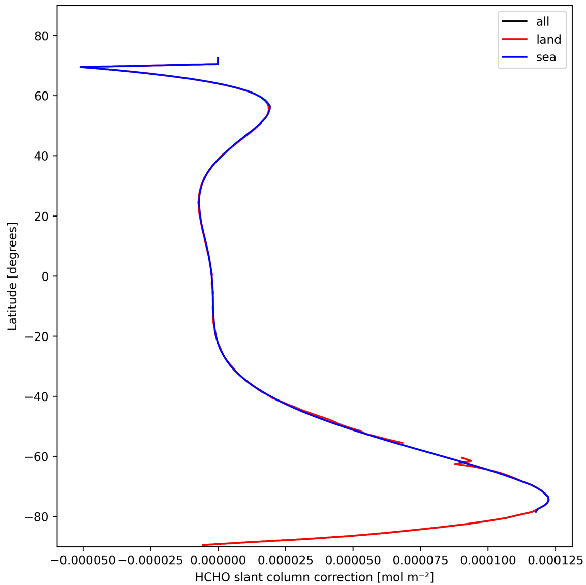
Figure 31: Zonal average of “HCHO slant column correction” for 2025-10-25 to 2025-10-25.
