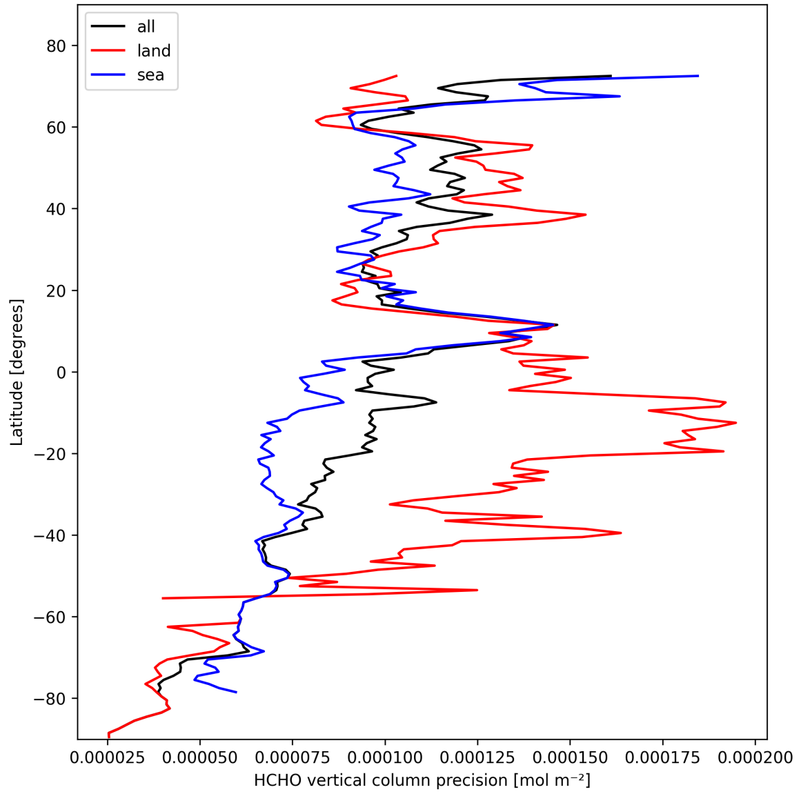
Figure 20: Zonal average of “HCHO vertical column precision” for 2025-10-25 to 2025-10-25.
