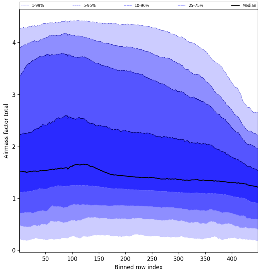
Figure 52: Along track statistics of “Airmass factor total” for 2025-10-25 to 2025-10-25
