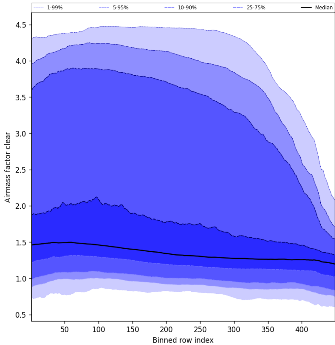
Figure 54: Along track statistics of “Airmass factor clear” for 2025-10-25 to 2025-10-25
