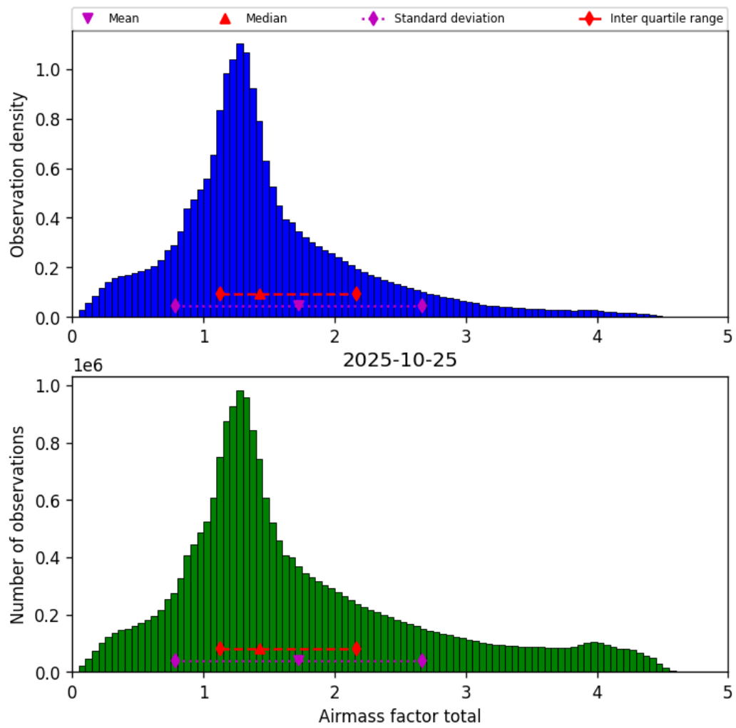
Figure 38: Histogram of “Airmass factor total” for 2025-10-25 to 2025-10-25
