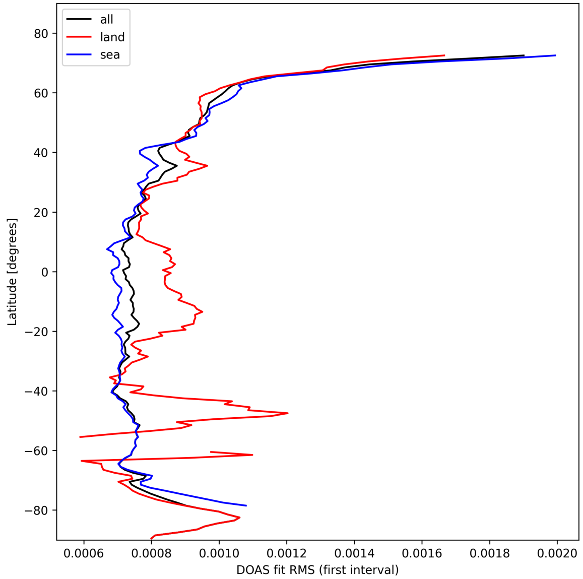
Figure 30: Zonal average of "DOAS fit RMS (first interval)" for 2025-10-25 to 2025-10-25.
