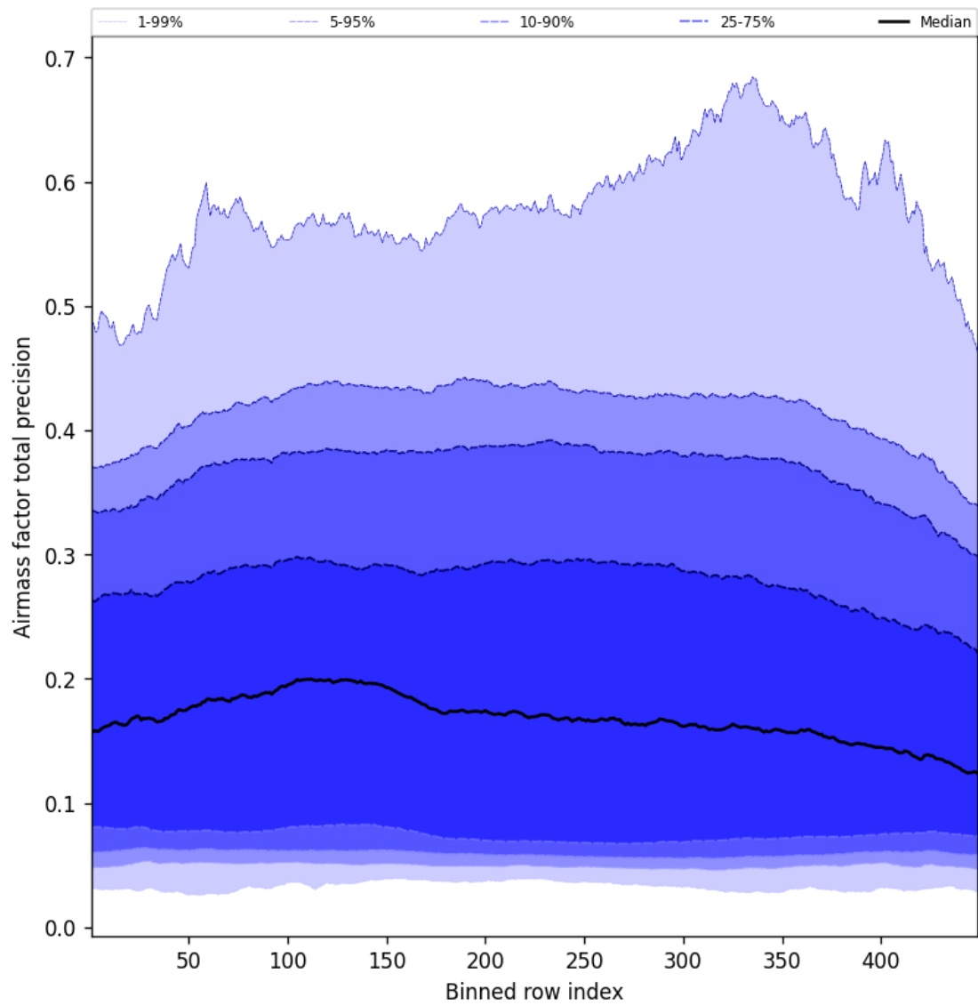
Figure 53: Along track statistics of “Airmass factor total precision” for 2025-10-25 to 2025-10-25
