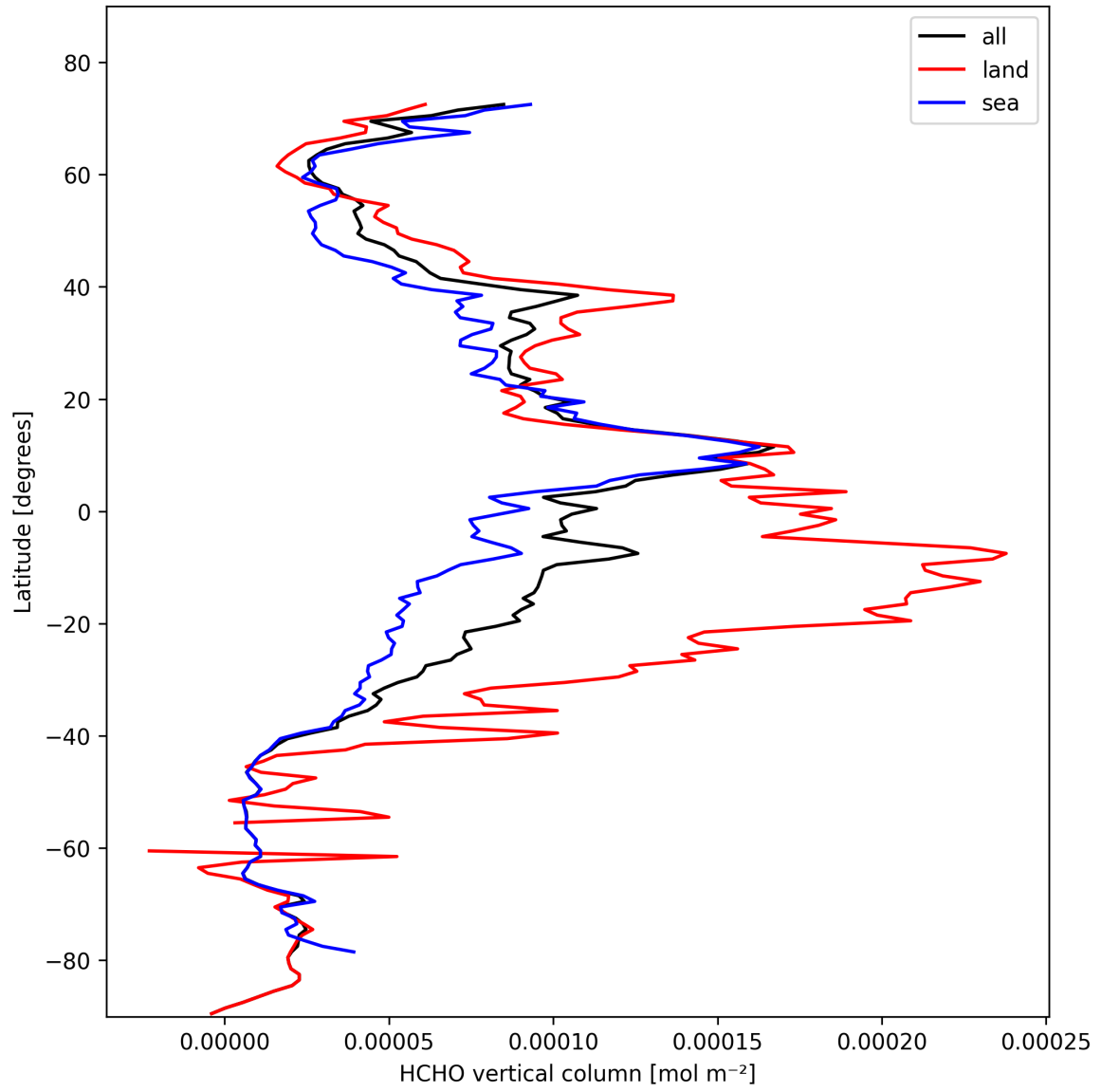
Figure 19: Zonal average of “HCHO vertical column” for 2025-10-25 to 2025-10-25.
