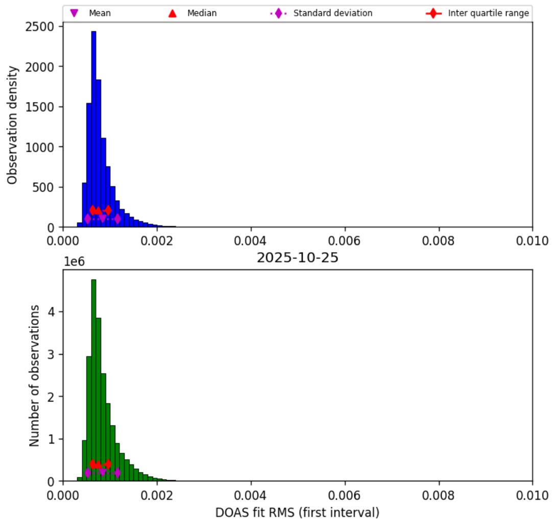
Figure 44: Histogram of “DOAS fit RMS (first interval)” for 2025-10-25 to 2025-10-25
