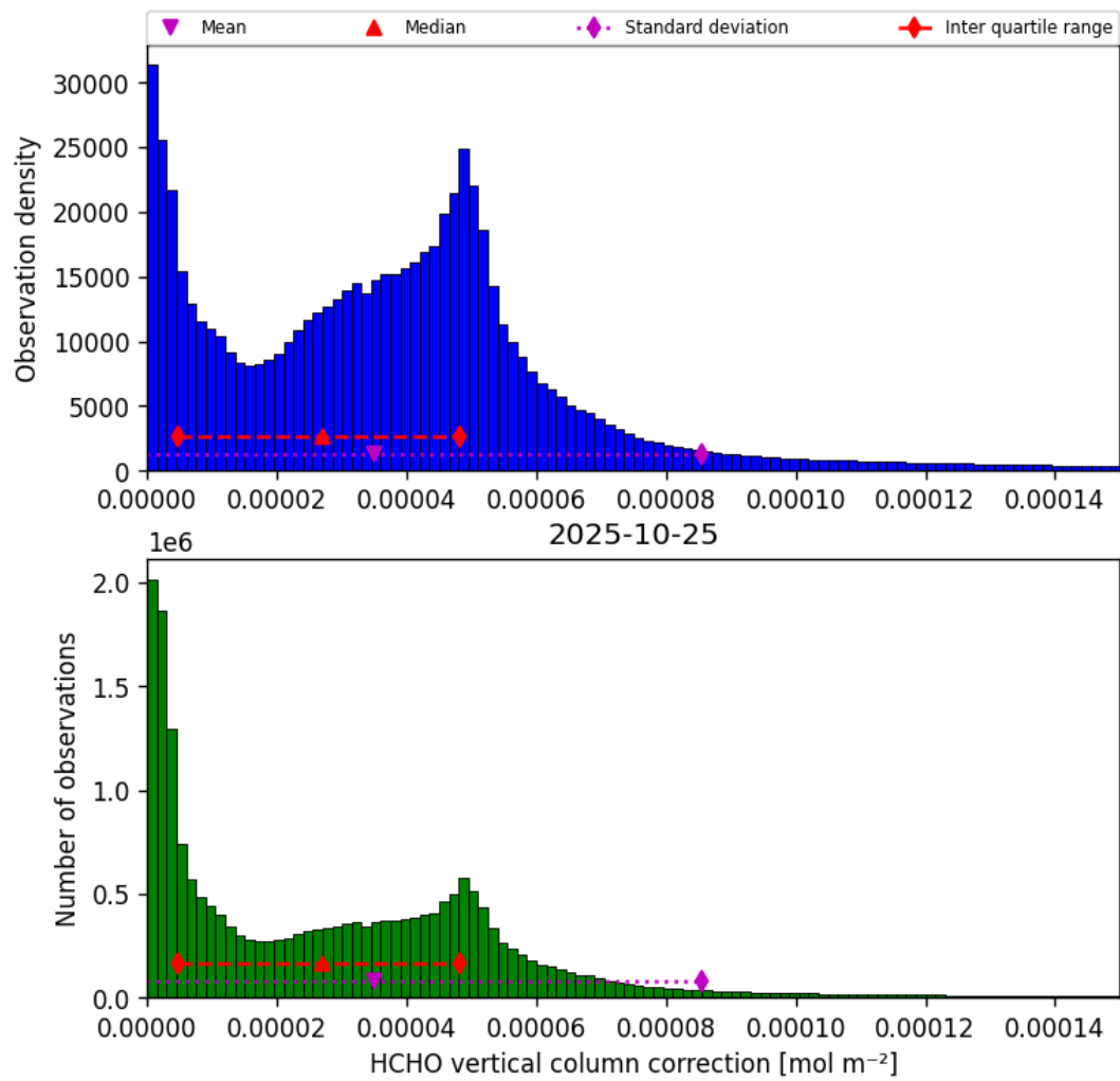
Figure 35: Histogram of “HCHO vertical column correction” for 2025-10-25 to 2025-10-25
