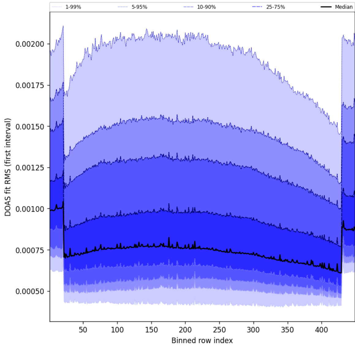
Figure 58: Along track statistics of “DOAS fit RMS (first interval)” for 2025-10-25 to 2025-10-25
