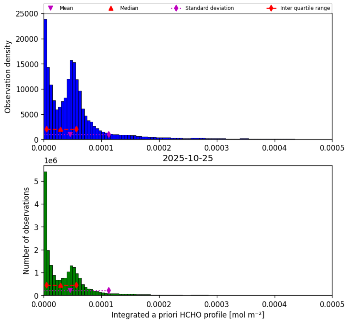
Figure 41: Histogram of “Integrated a priori HCHO profile” for 2025-10-25 to 2025-10-25
