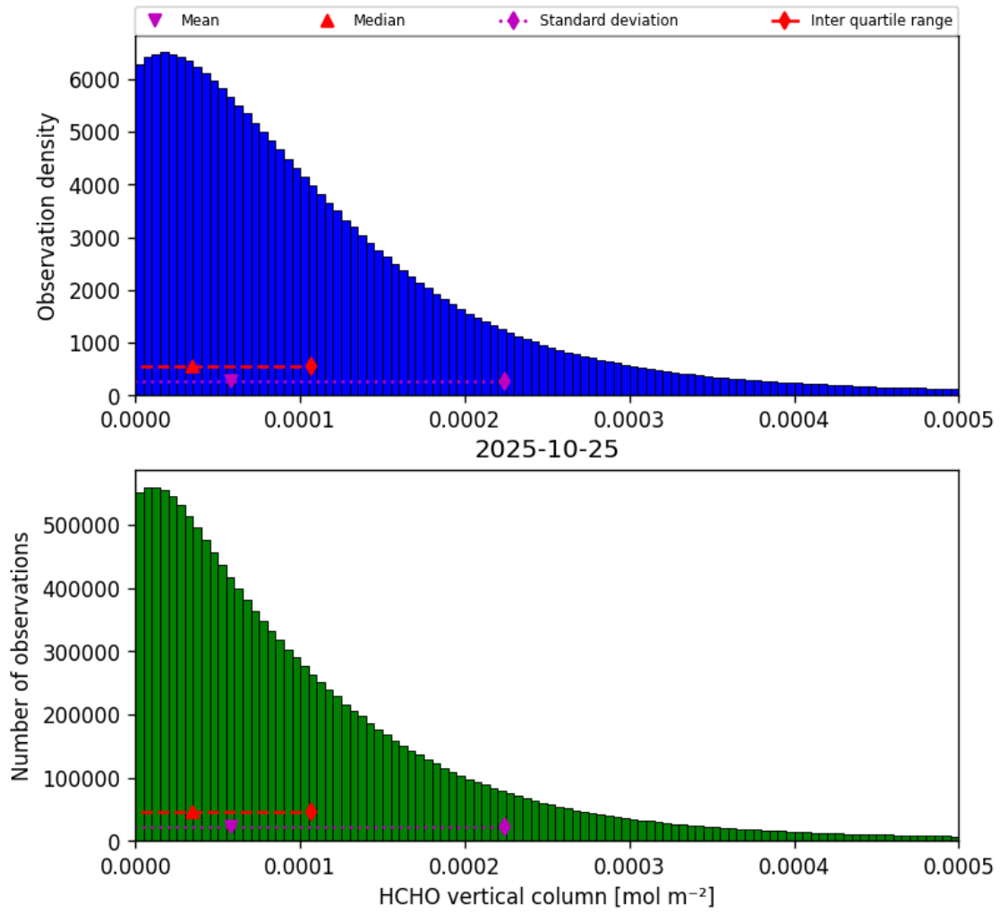
Figure 33: Histogram of “HCHO vertical column” for 2025-10-25 to 2025-10-25
