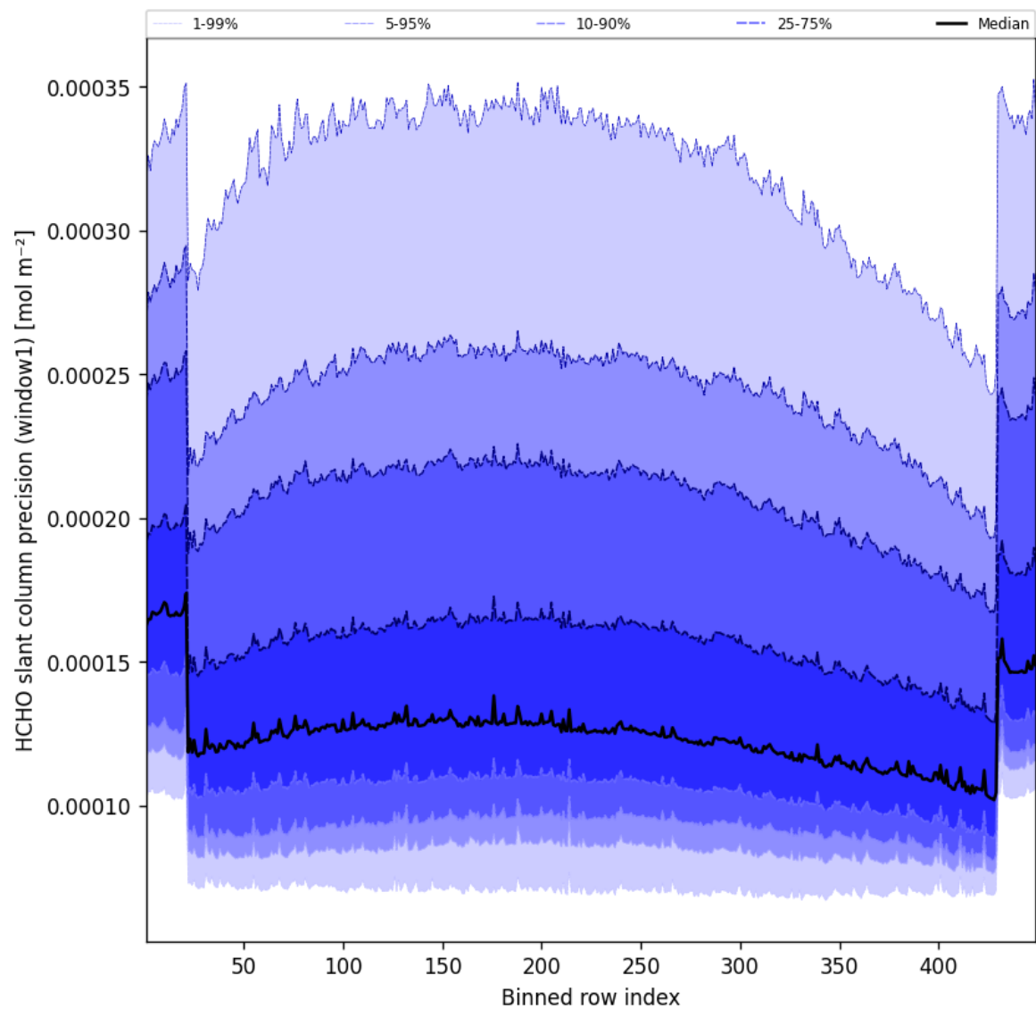
Figure 51: Along track statistics of “HCHO slant column precision (window1)” for 2025-10-25 to 2025-10-25
