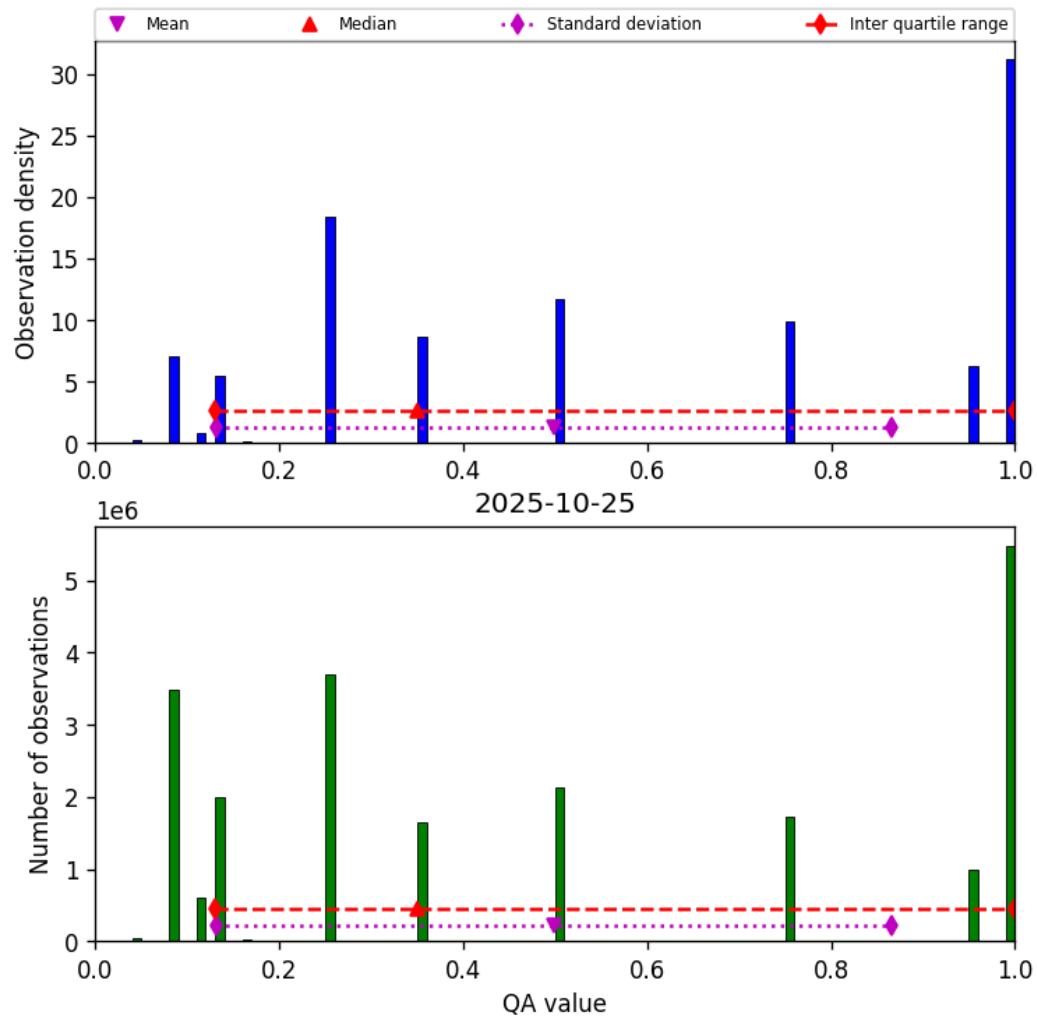
Figure 32: Histogram of “QA value” for 2025-10-25 to 2025-10-25
