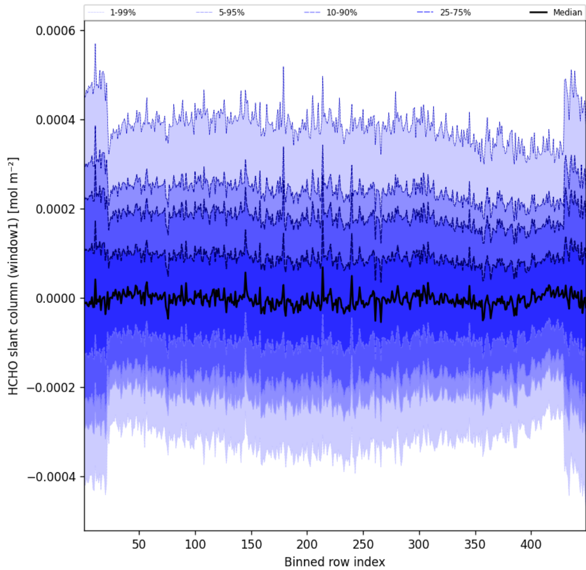
Figure 50: Along track statistics of “HCHO slant column (window1)” for 2025-10-25 to 2025-10-25
