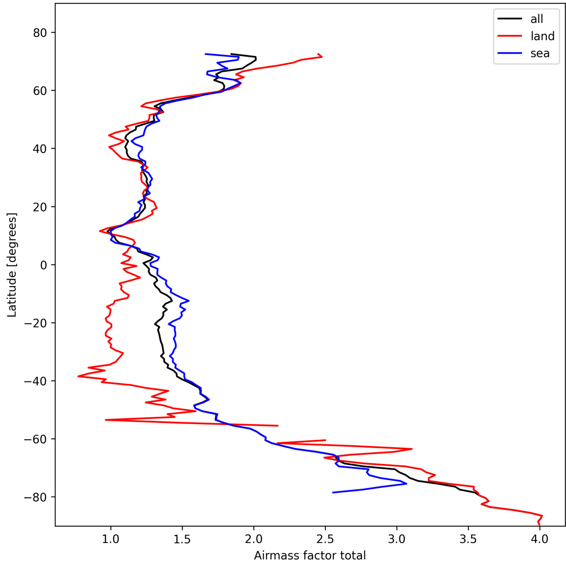
Figure 24: Zonal average of “Airmass factor total” for 2025-10-25 to 2025-10-25.
