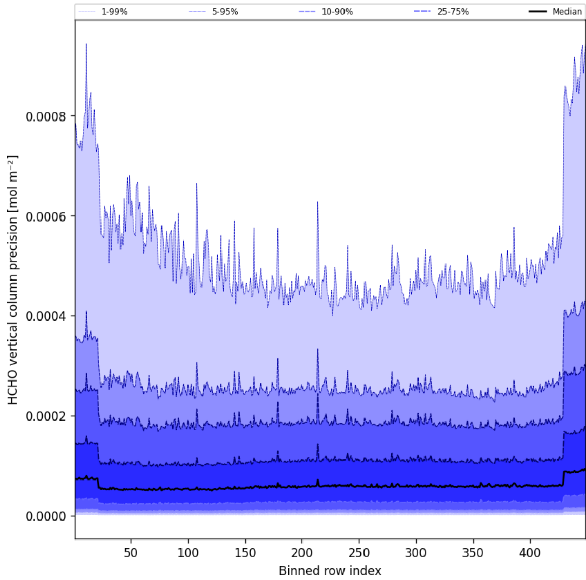
Figure 48: Along track statistics of “HCHO vertical column precision” for 2025-10-25 to 2025-10-25
