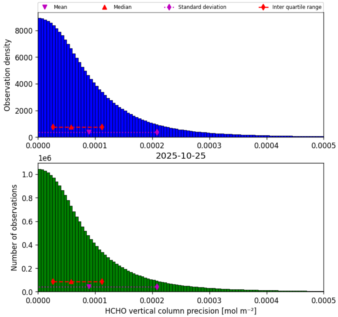
Figure 34: Histogram of “HCHO vertical column precision” for 2025-10-25 to 2025-10-25
