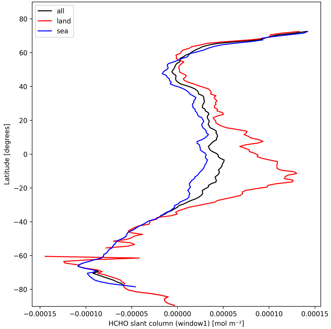
Figure 22: Zonal average of “HCHO slant column (window1)” for 2025-10-25 to 2025-10-25.
