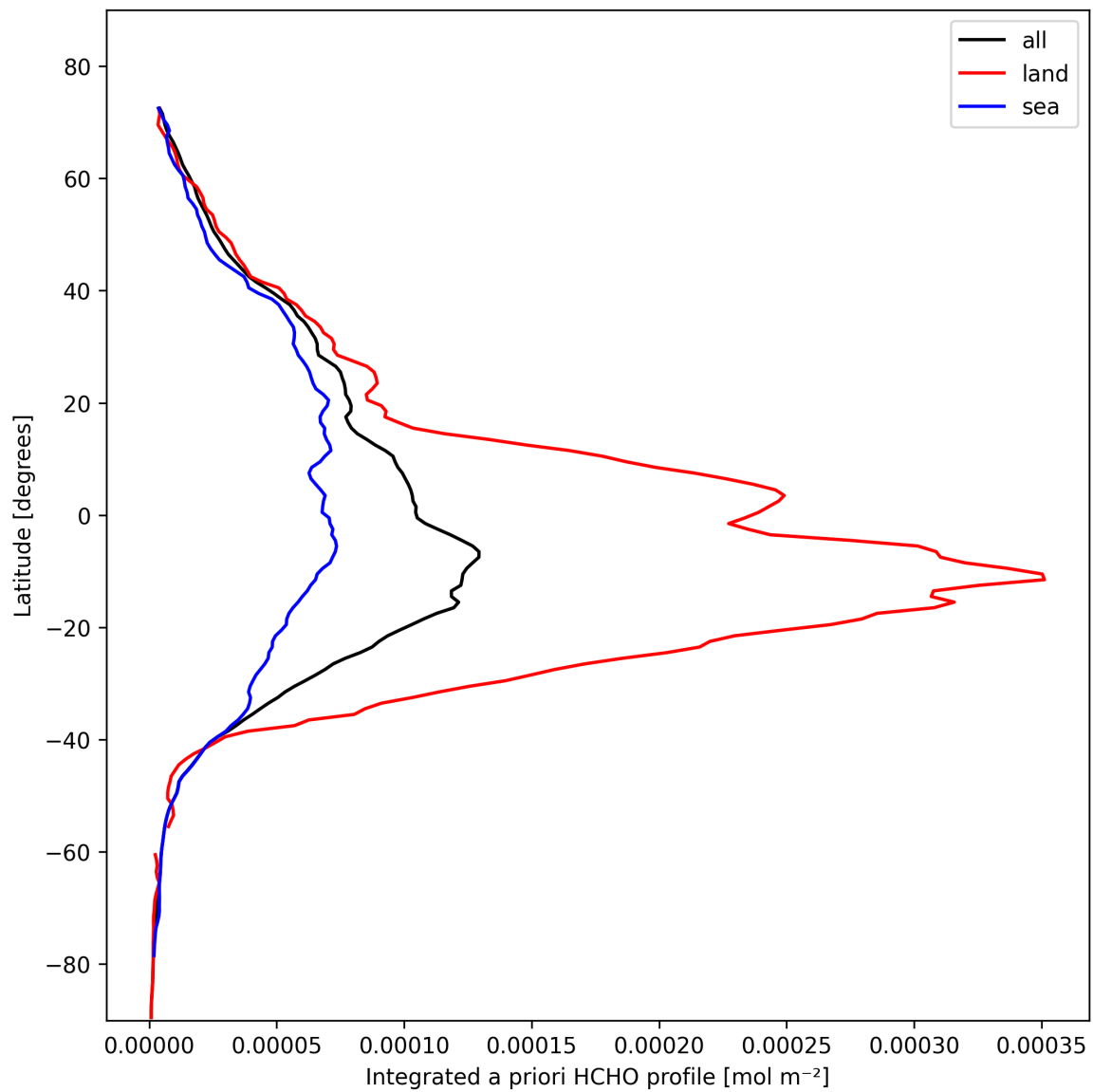
Figure 27: Zonal average of “Integrated a priori HCHO profile” for 2025-10-25 to 2025-10-25.
