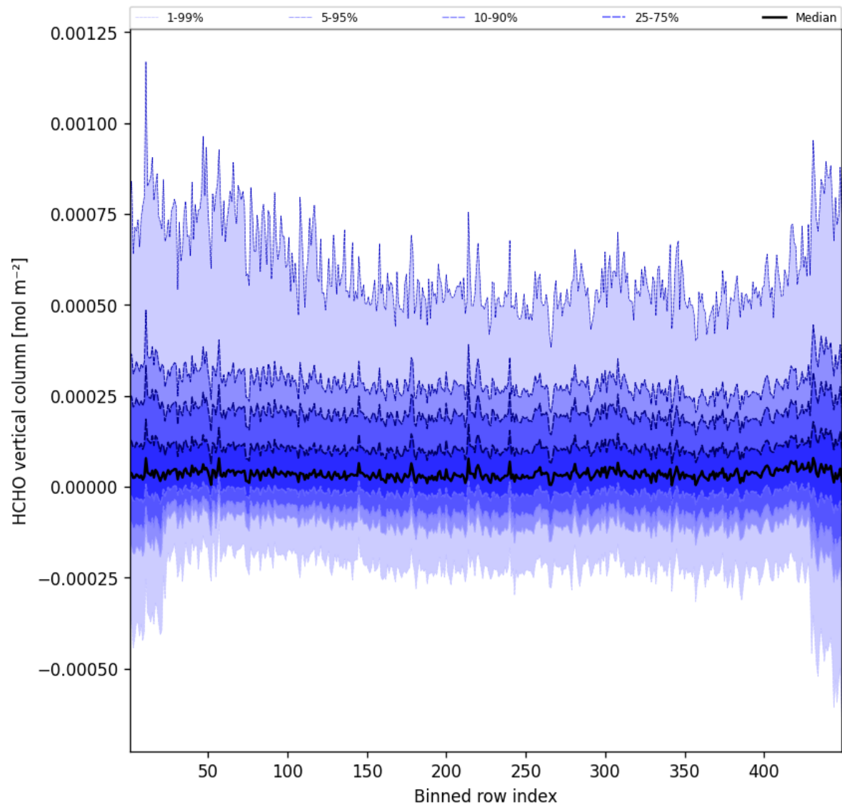
Figure 47: Along track statistics of “HCHO vertical column” for 2025-10-25 to 2025-10-25
