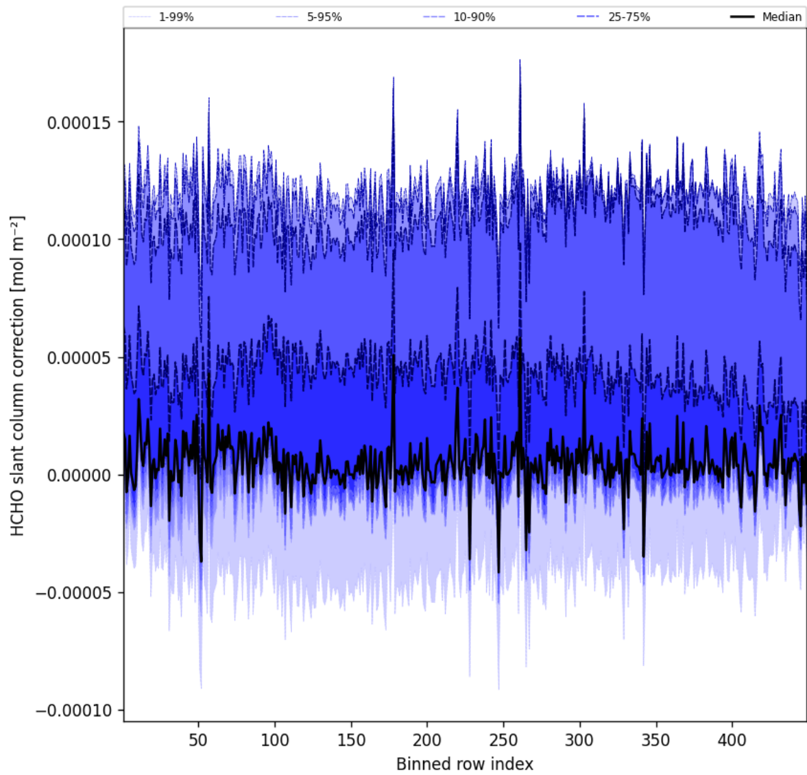
Figure 59: Along track statistics of “HCHO slant column correction” for 2025-10-25 to 2025-10-25
