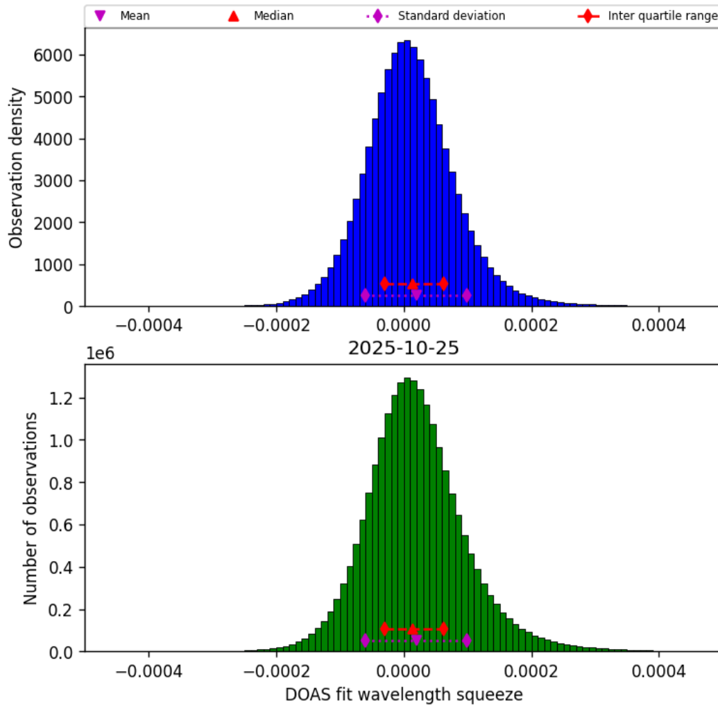
Figure 43: Histogram of “DOAS fit wavelength squeeze” for 2025-10-25 to 2025-10-25
