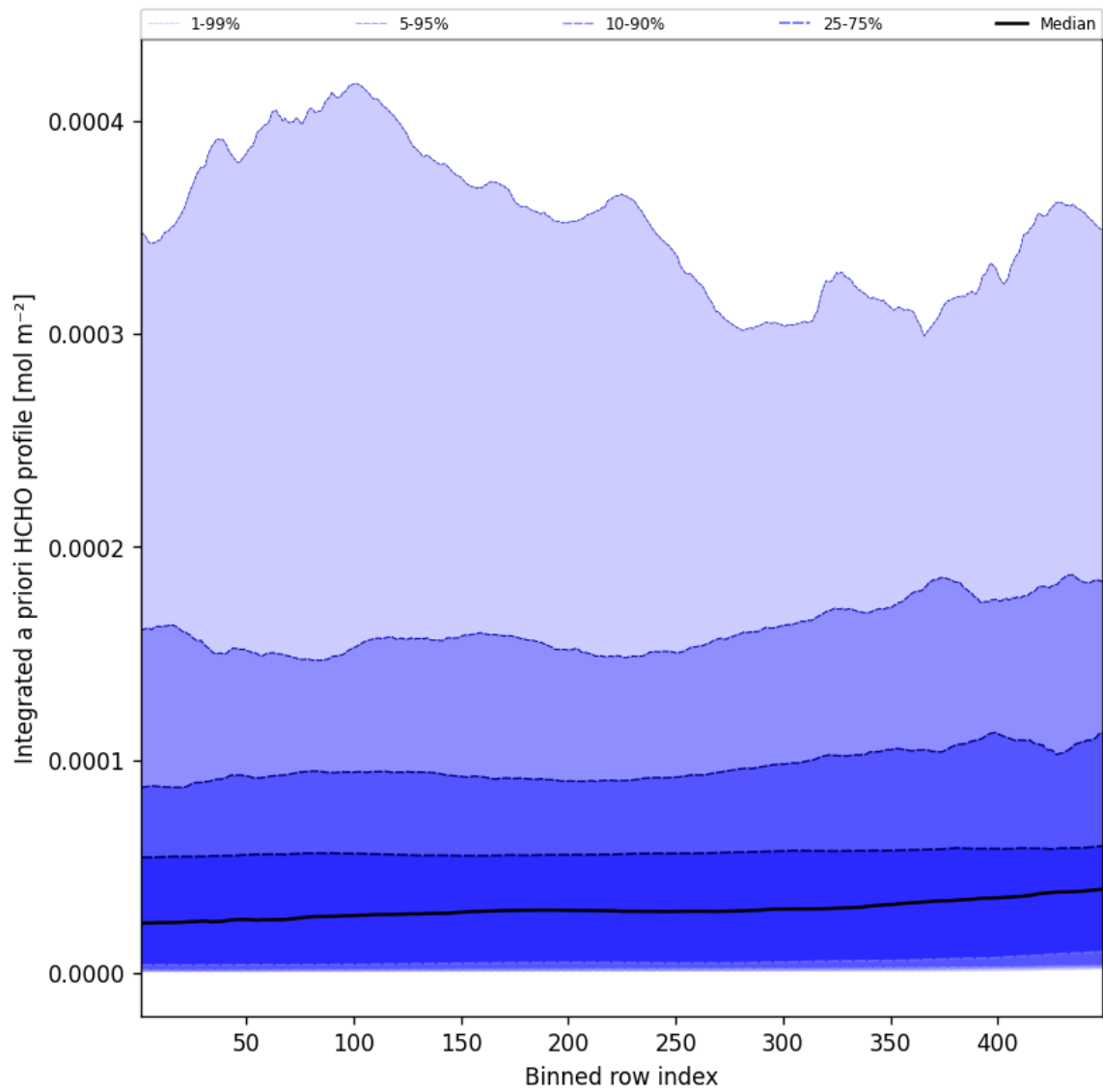
Figure 55: Along track statistics of "Integrated a priori HCHO profile" for 2025-10-25 to 2025-10-25
