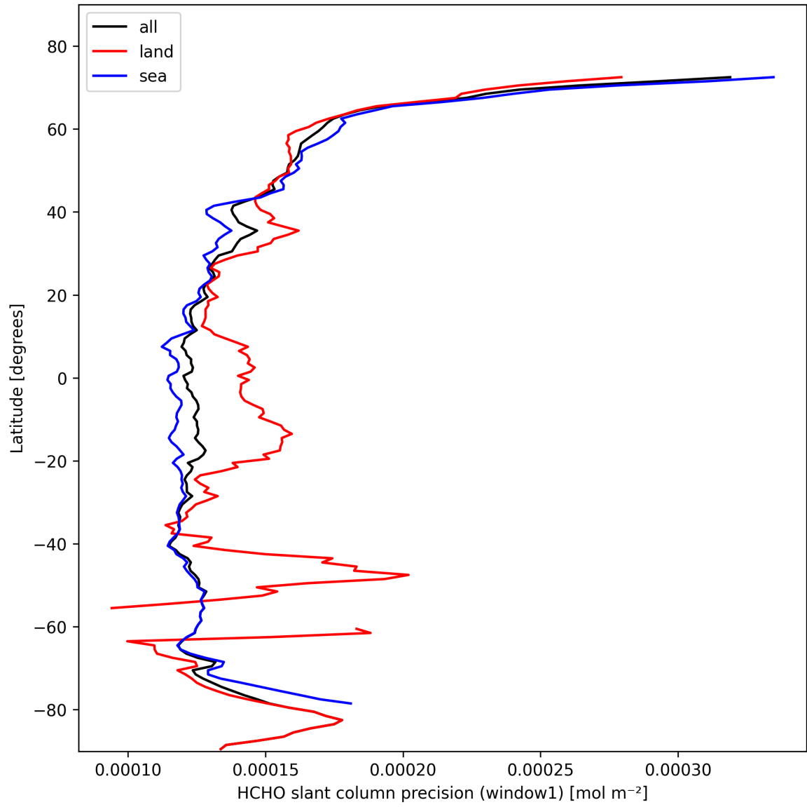
Figure 23: Zonal average of “HCHO slant column precision (window1)” for 2025-10-25 to 2025-10-25.
