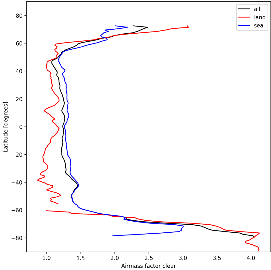
Figure 26: Zonal average of “Airmass factor clear” for 2025-10-25 to 2025-10-25.
