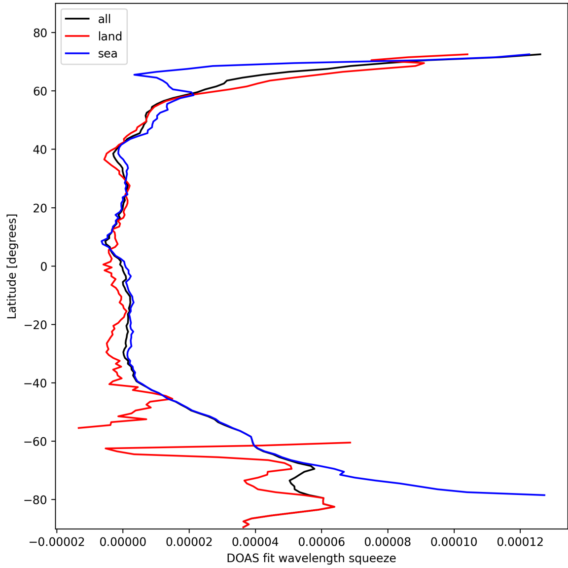
Figure 29: Zonal average of “DOAS fit wavelength squeeze” for 2025-10-25 to 2025-10-25.
