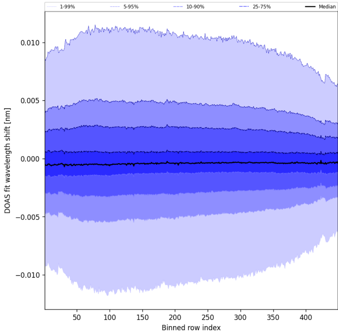
Figure 56: Along track statistics of “DOAS fit wavelength shift” for 2025-10-25 to 2025-10-25
