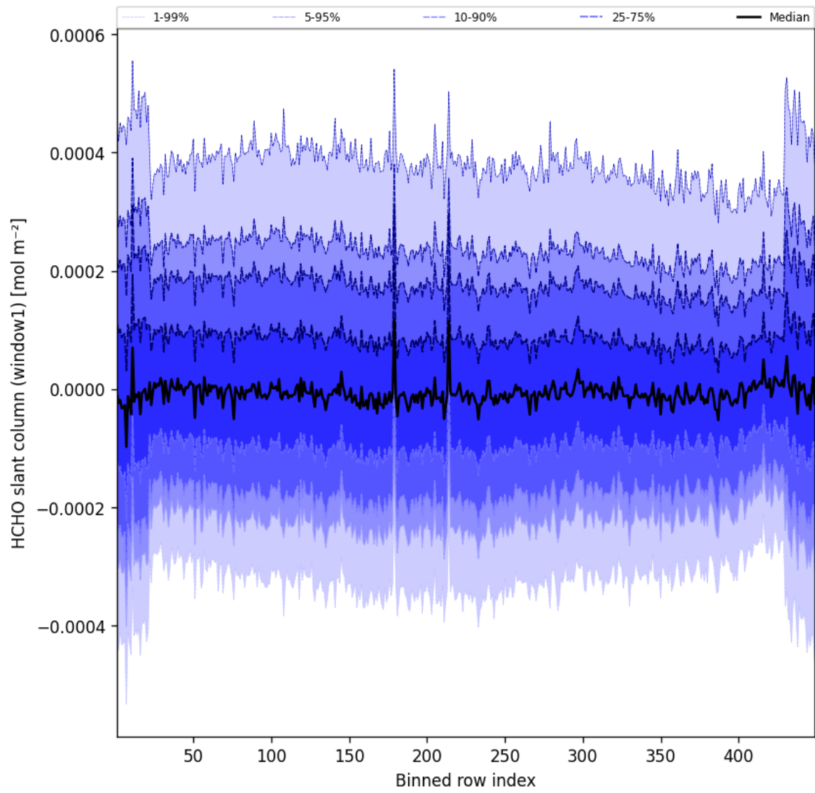
Figure 50: Along track statistics of “HCHO slant column (window1)” for 2025-10-26 to 2025-10-27
