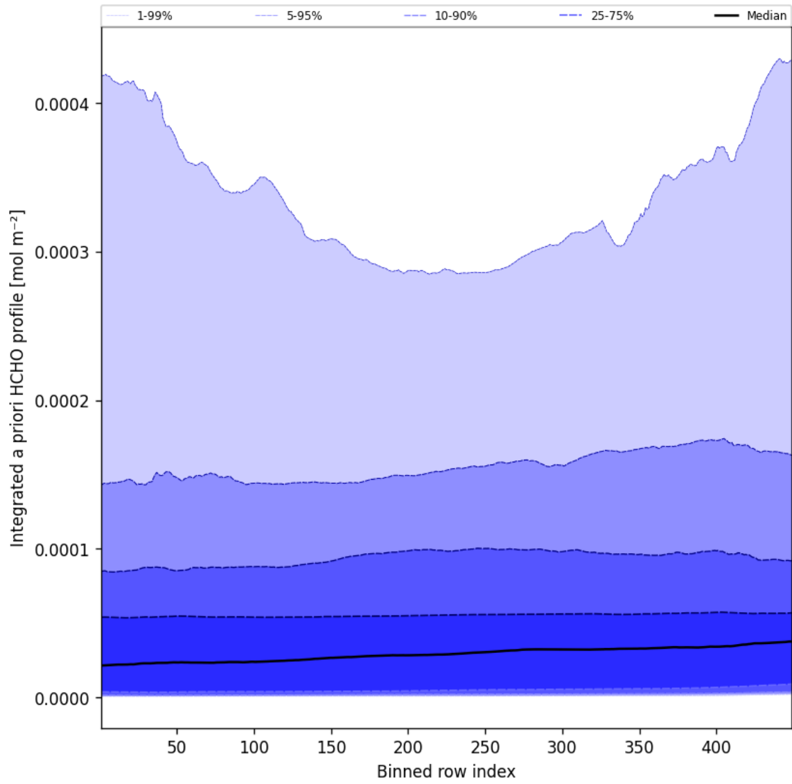
Figure 55: Along track statistics of “Integrated a priori HCHO profile” for 2025-10-26 to 2025-10-27
