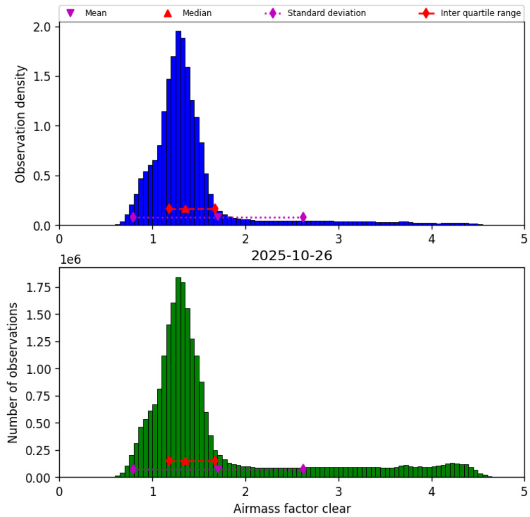
Figure 40: Histogram of “Airmass factor clear” for 2025-10-26 to 2025-10-27
