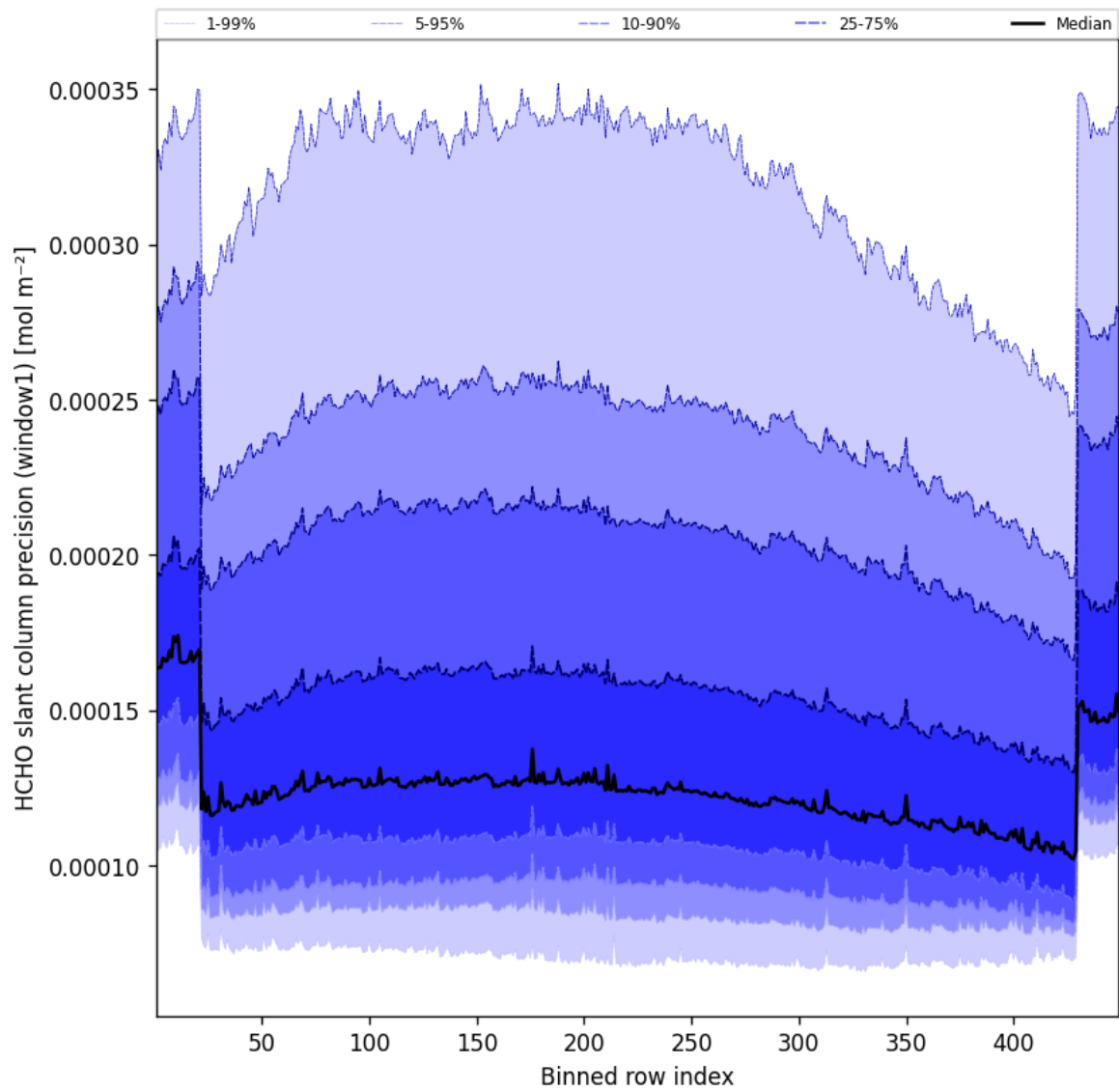
Figure 51: Along track statistics of “HCHO slant column precision (window1)” for 2025-10-26 to 2025-10-27
