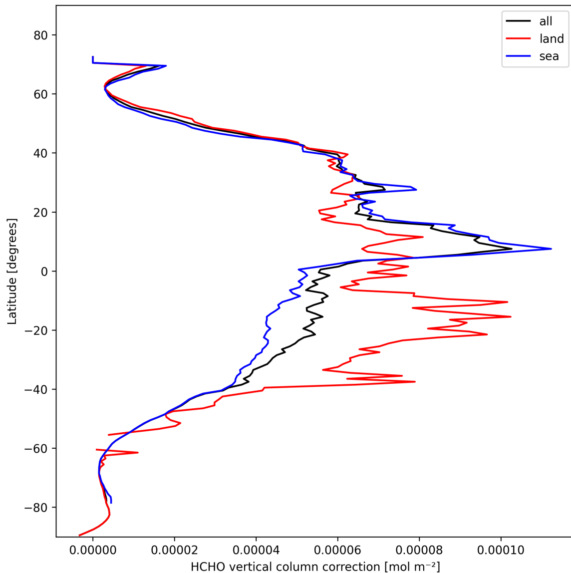
Figure 21: Zonal average of “HCHO vertical column correction” for 2025-10-26 to 2025-10-27.
