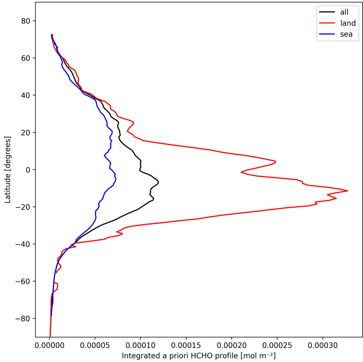
Figure 27: Zonal average of “Integrated a priori HCHO profile” for 2025-10-26 to 2025-10-27.
