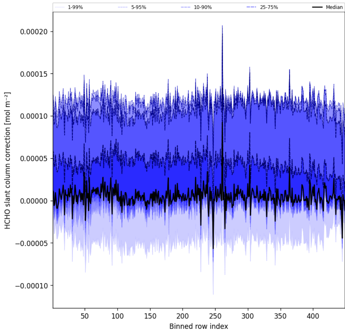
Figure 59: Along track statistics of “HCHO slant column correction” for 2025-10-26 to 2025-10-27
