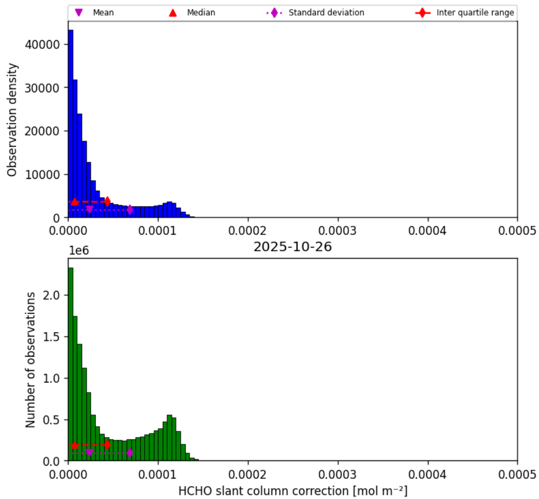
Figure 45: Histogram of “HCHO slant column correction” for 2025-10-26 to 2025-10-27
