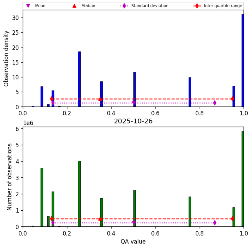
Figure 32: Histogram of “QA value” for 2025-10-26 to 2025-10-27
