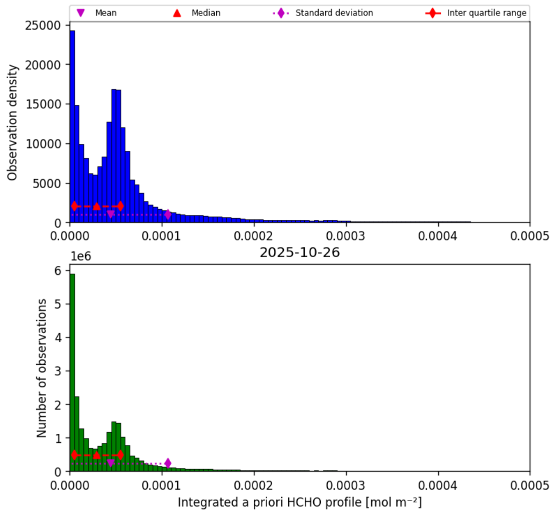
Figure 41: Histogram of “Integrated a priori HCHO profile” for 2025-10-26 to 2025-10-27
