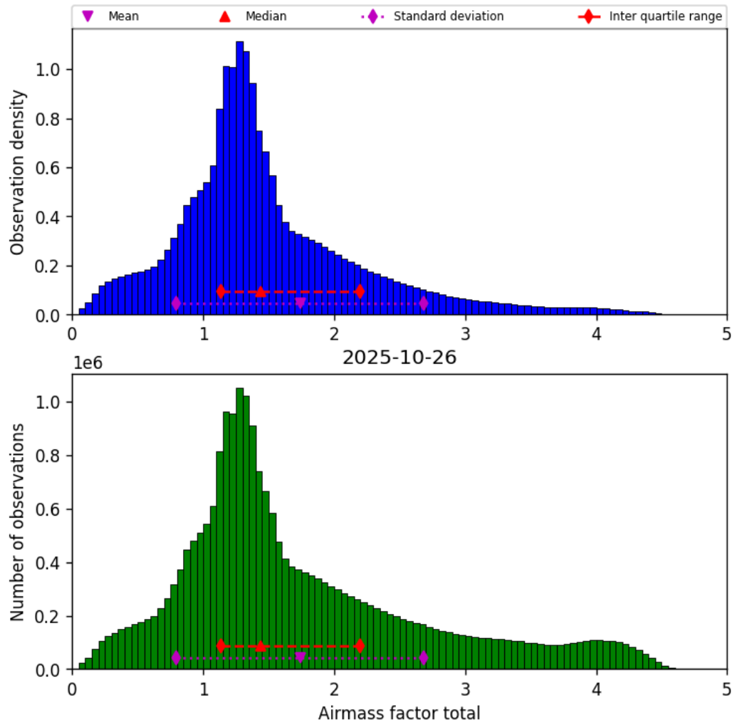
Figure 38: Histogram of “Airmass factor total” for 2025-10-26 to 2025-10-27
