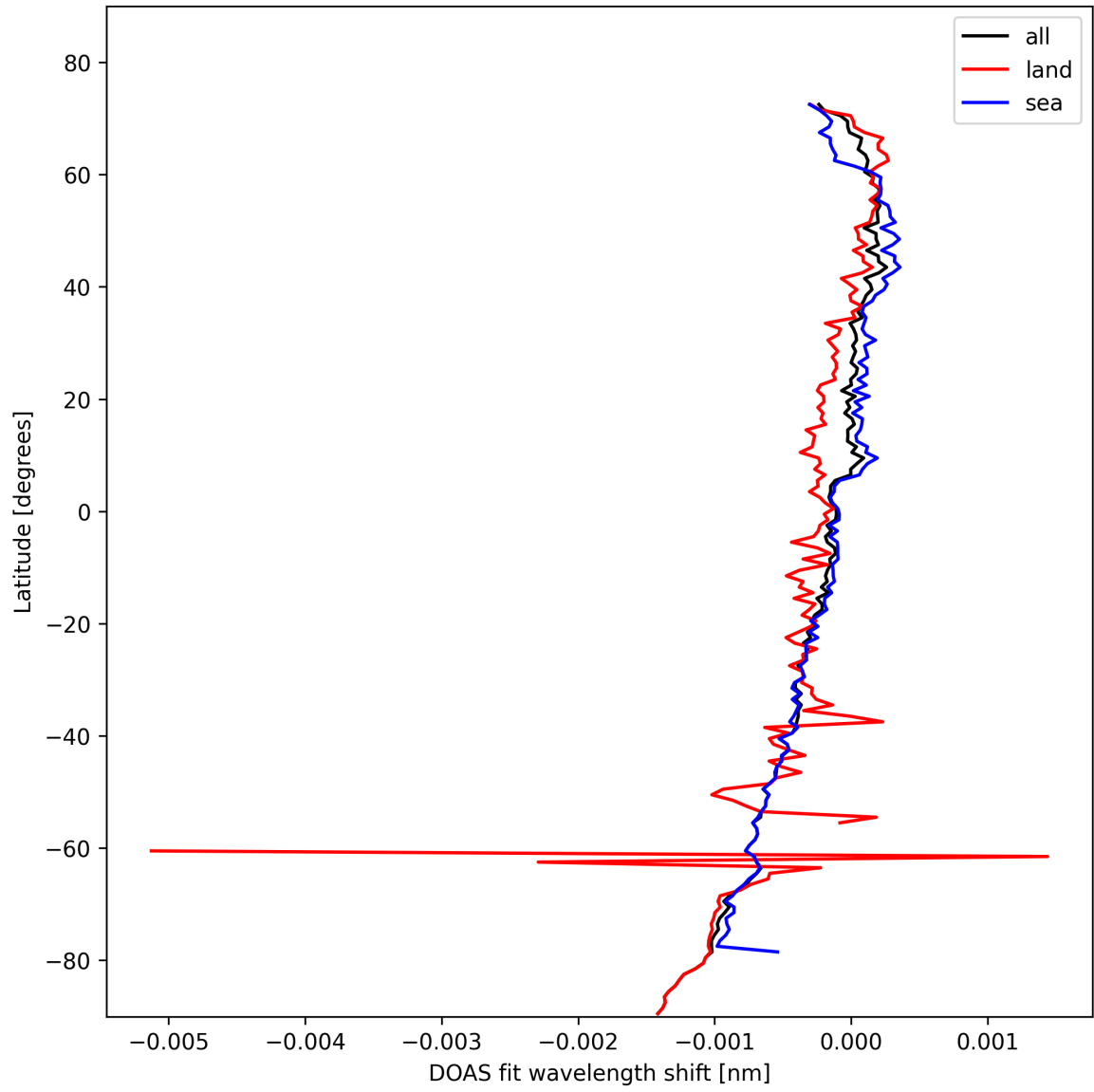
Figure 28: Zonal average of “DOAS fit wavelength shift” for 2025-10-26 to 2025-10-27.
