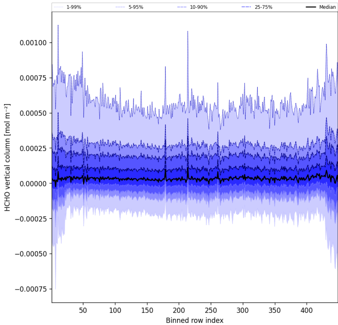
Figure 47: Along track statistics of “HCHO vertical column” for 2025-10-26 to 2025-10-27
