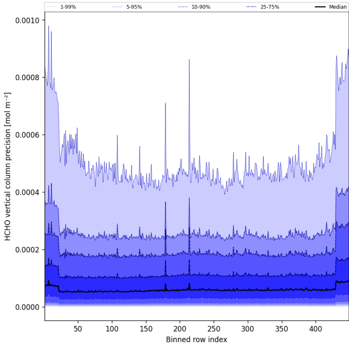
Figure 48: Along track statistics of “HCHO vertical column precision” for 2025-10-26 to 2025-10-27
