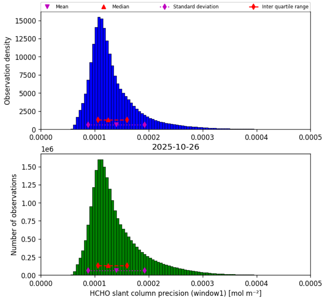
Figure 37: Histogram of “HCHO slant column precision (window1)” for 2025-10-26 to 2025-10-27
