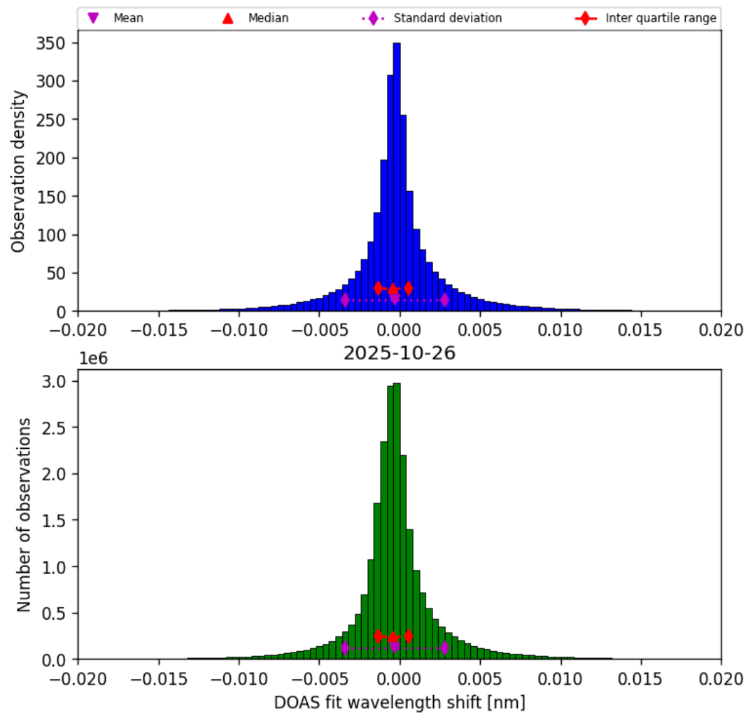
Figure 42: Histogram of “DOAS fit wavelength shift” for 2025-10-26 to 2025-10-27
