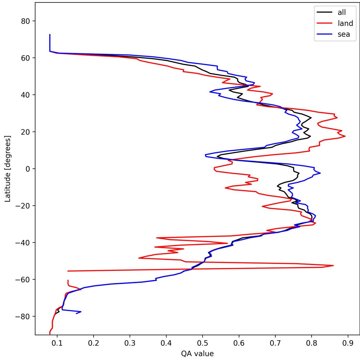
Figure 18: Zonal average of “QA value” for 2025-10-26 to 2025-10-27.
