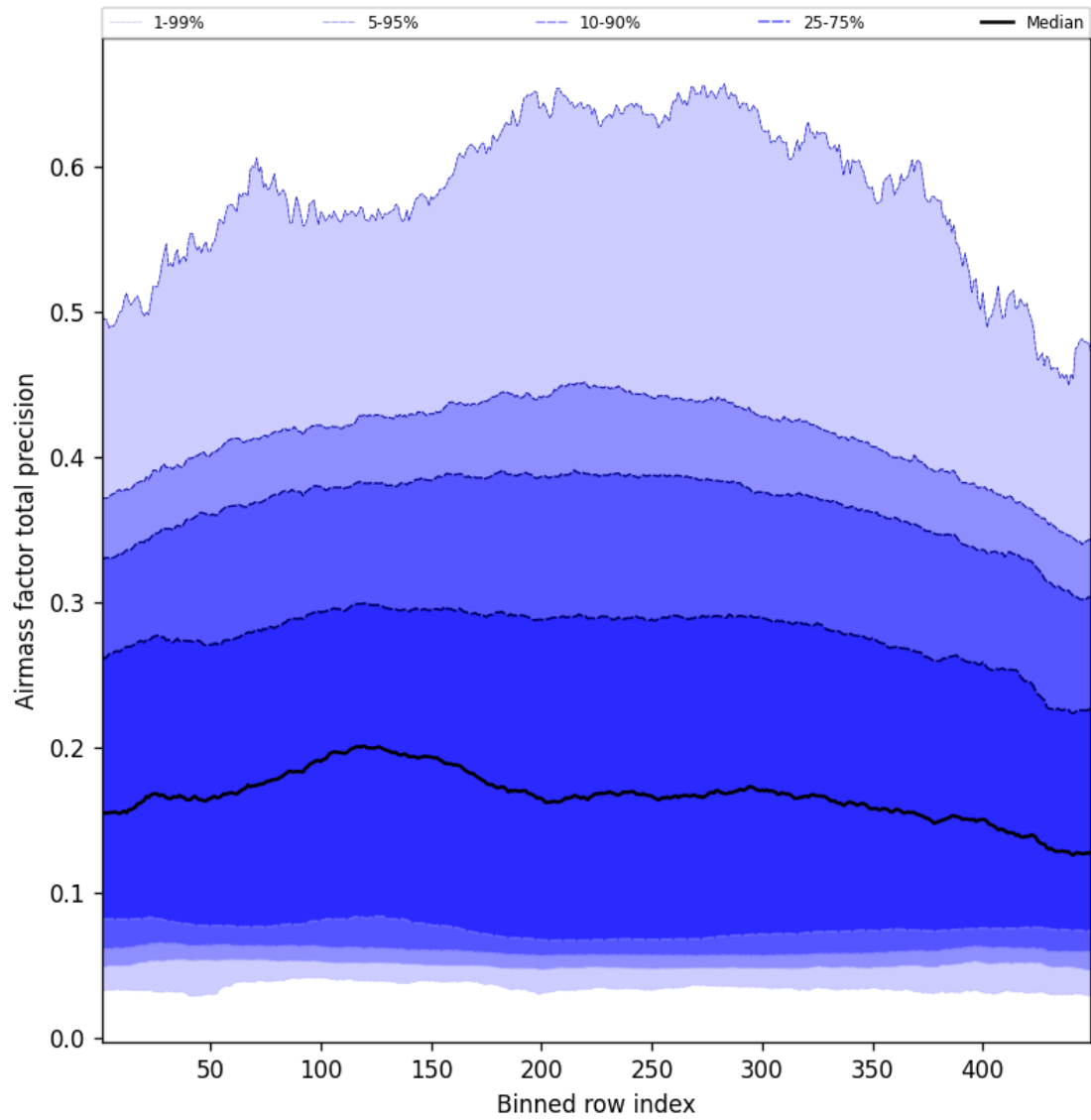
Figure 53: Along track statistics of “Airmass factor total precision” for 2025-10-26 to 2025-10-27
