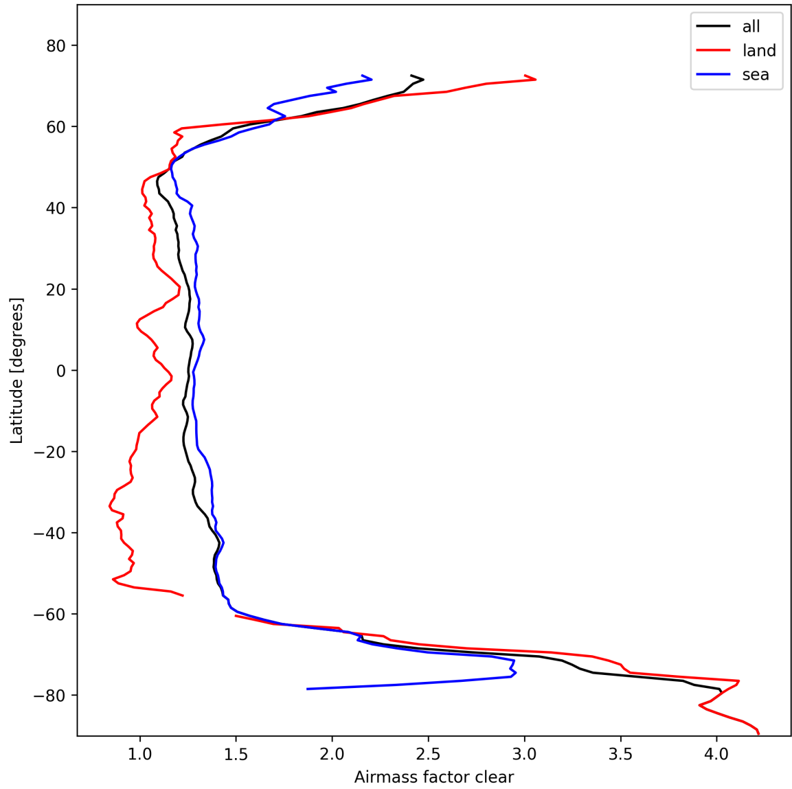
Figure 26: Zonal average of “Airmass factor clear” for 2025-10-26 to 2025-10-27.
