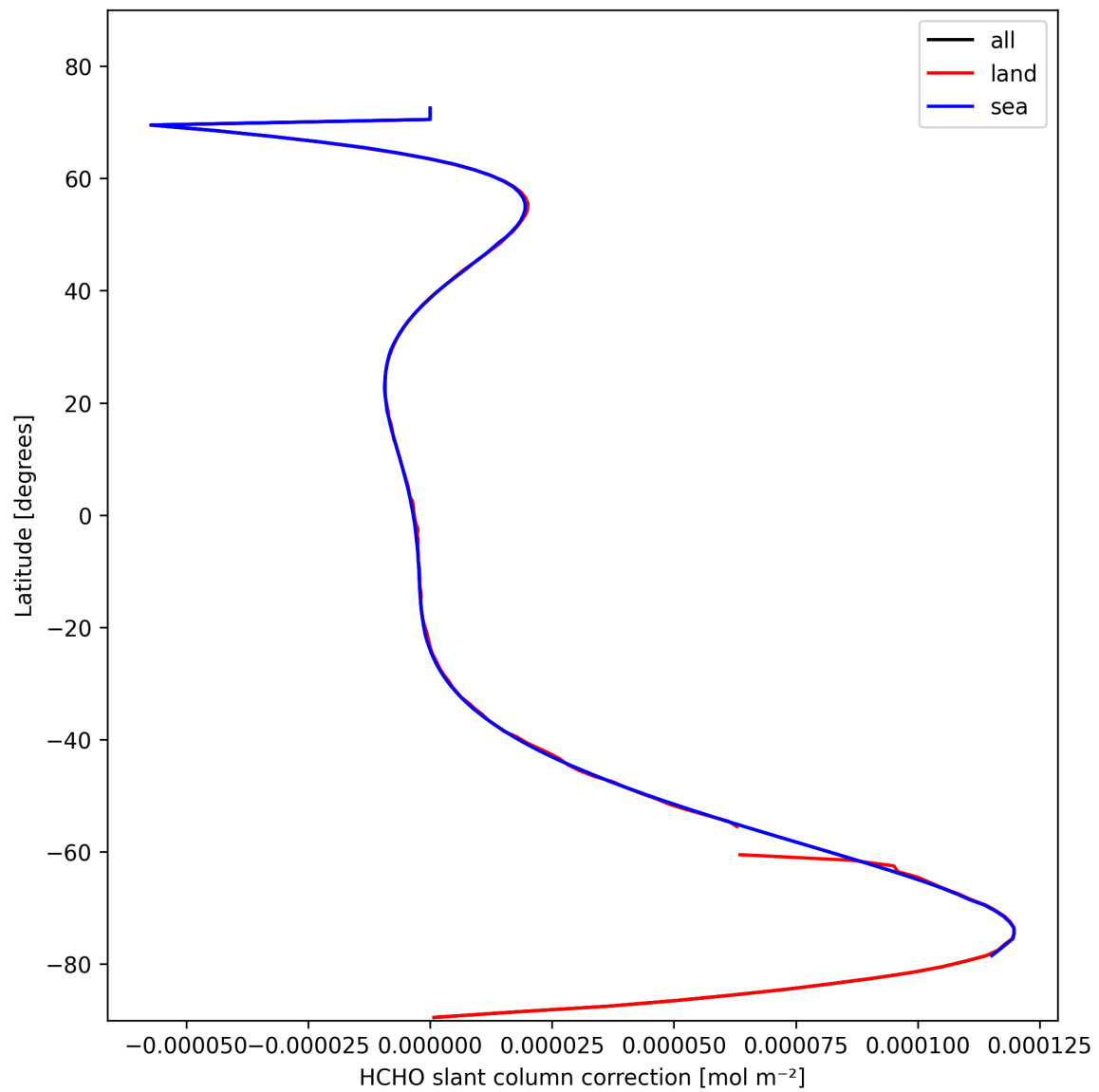
Figure 31: Zonal average of “HCHO slant column correction” for 2025-10-26 to 2025-10-27.
