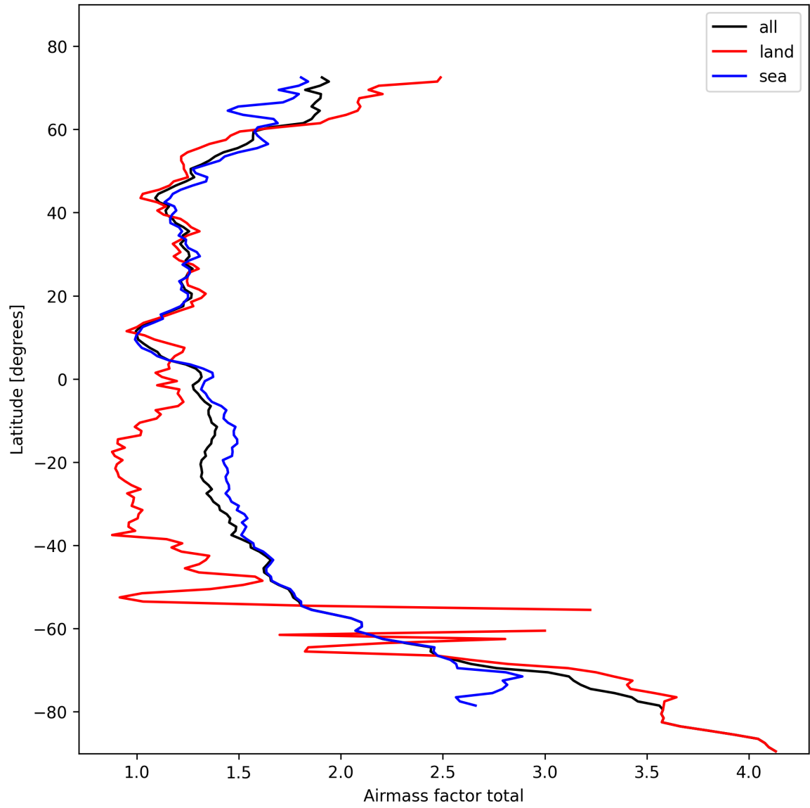
Figure 24: Zonal average of “Airmass factor total” for 2025-10-26 to 2025-10-27.
