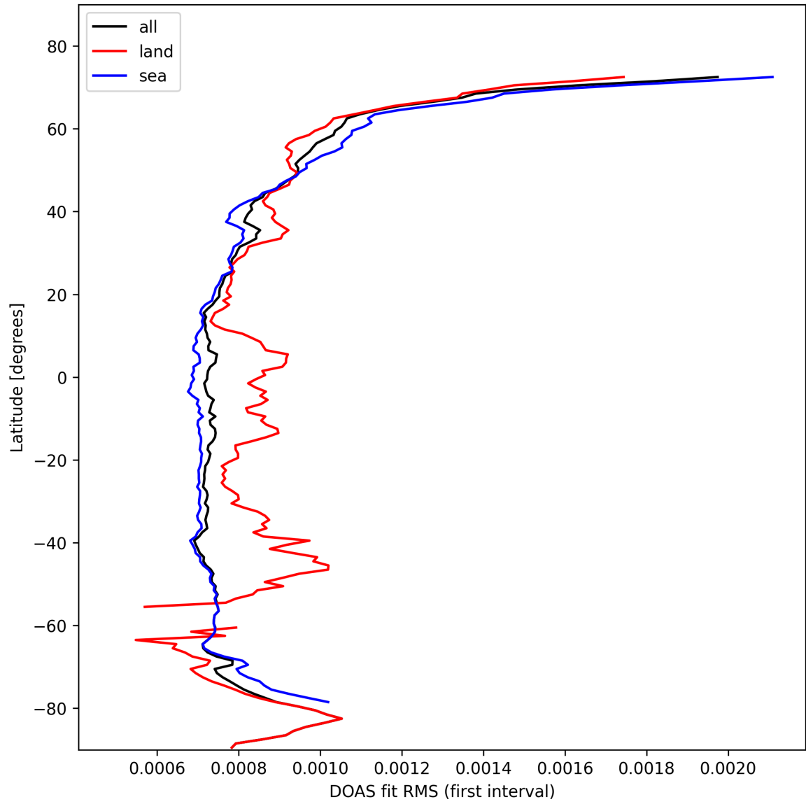
Figure 30: Zonal average of “DOAS fit RMS (first interval)” for 2025-10-26 to 2025-10-27.
