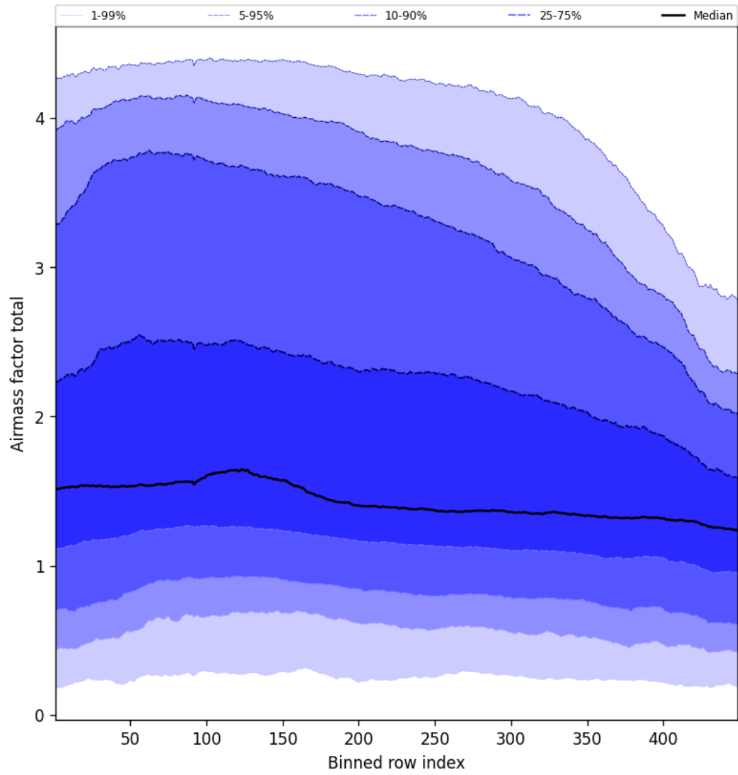
Figure 52: Along track statistics of “Airmass factor total” for 2025-10-26 to 2025-10-27
