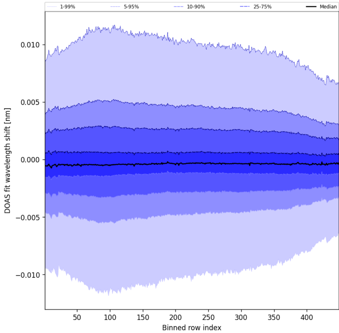
Figure 56: Along track statistics of “DOAS fit wavelength shift” for 2025-10-26 to 2025-10-27
