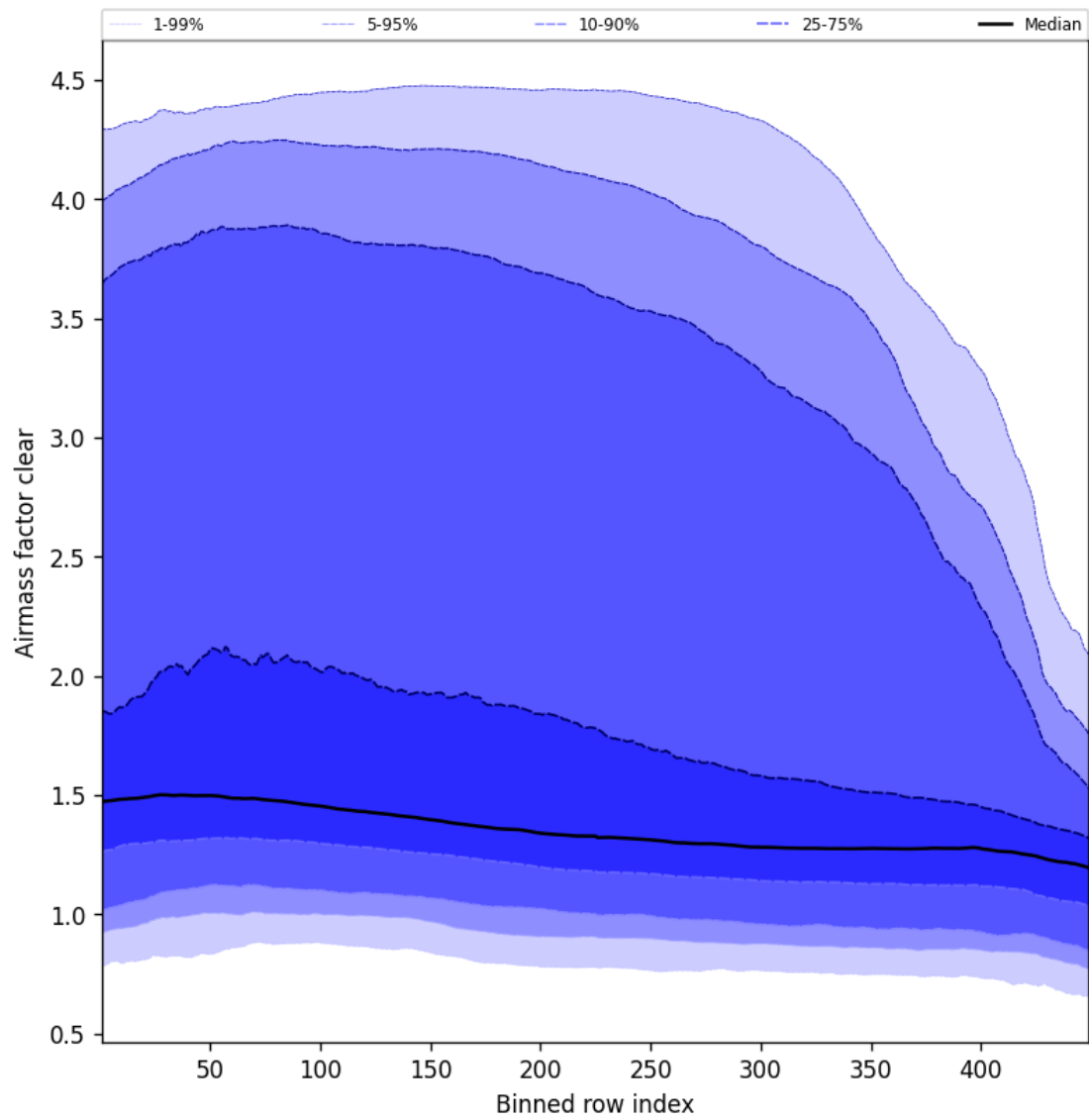
Figure 54: Along track statistics of “Airmass factor clear” for 2025-10-26 to 2025-10-27
