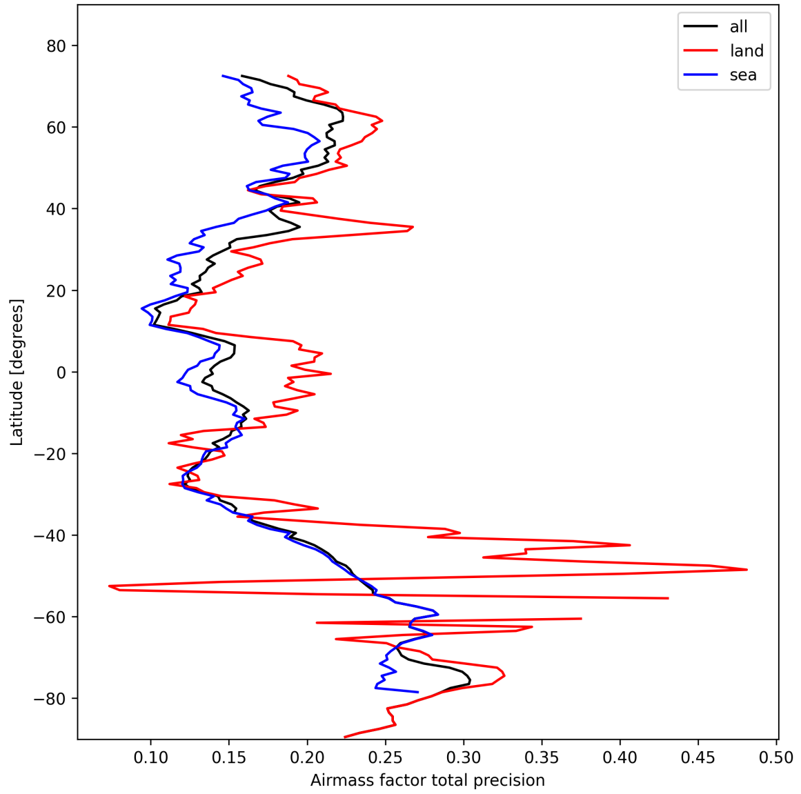
Figure 25: Zonal average of “Airmass factor total precision” for 2025-10-26 to 2025-10-27.
