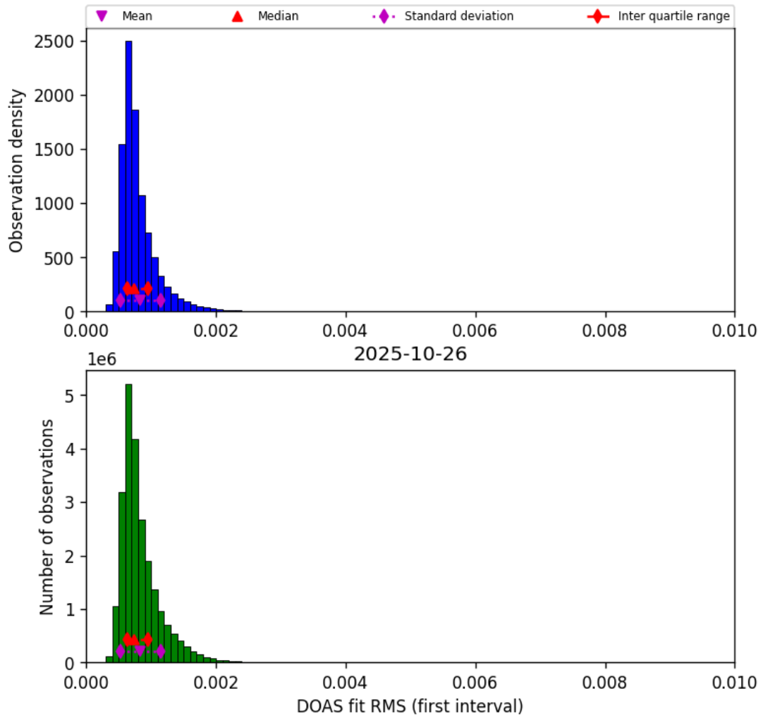
Figure 44: Histogram of “DOAS fit RMS (first interval)” for 2025-10-26 to 2025-10-27
