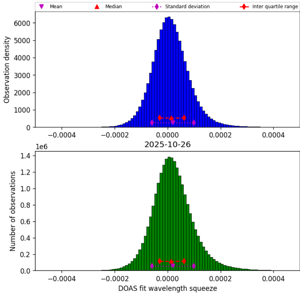
Figure 43: Histogram of “DOAS fit wavelength squeeze” for 2025-10-26 to 2025-10-27
