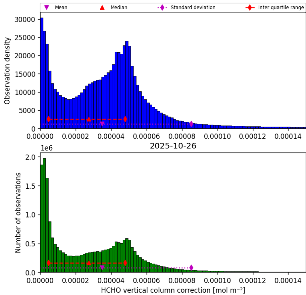
Figure 35: Histogram of “HCHO vertical column correction” for 2025-10-26 to 2025-10-27
