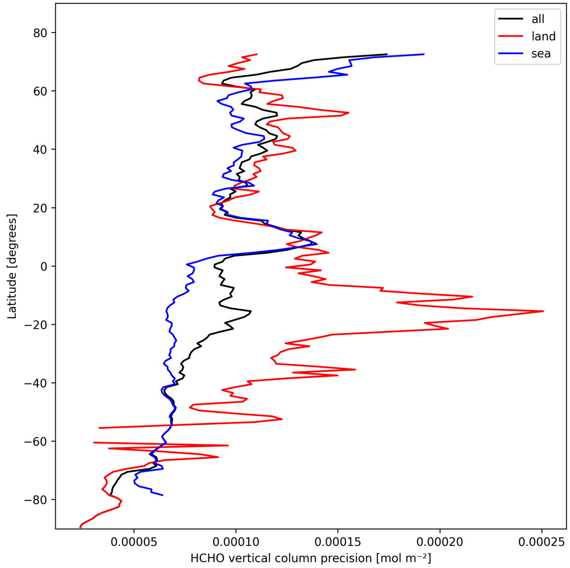
Figure 20: Zonal average of “HCHO vertical column precision” for 2025-10-26 to 2025-10-27.
