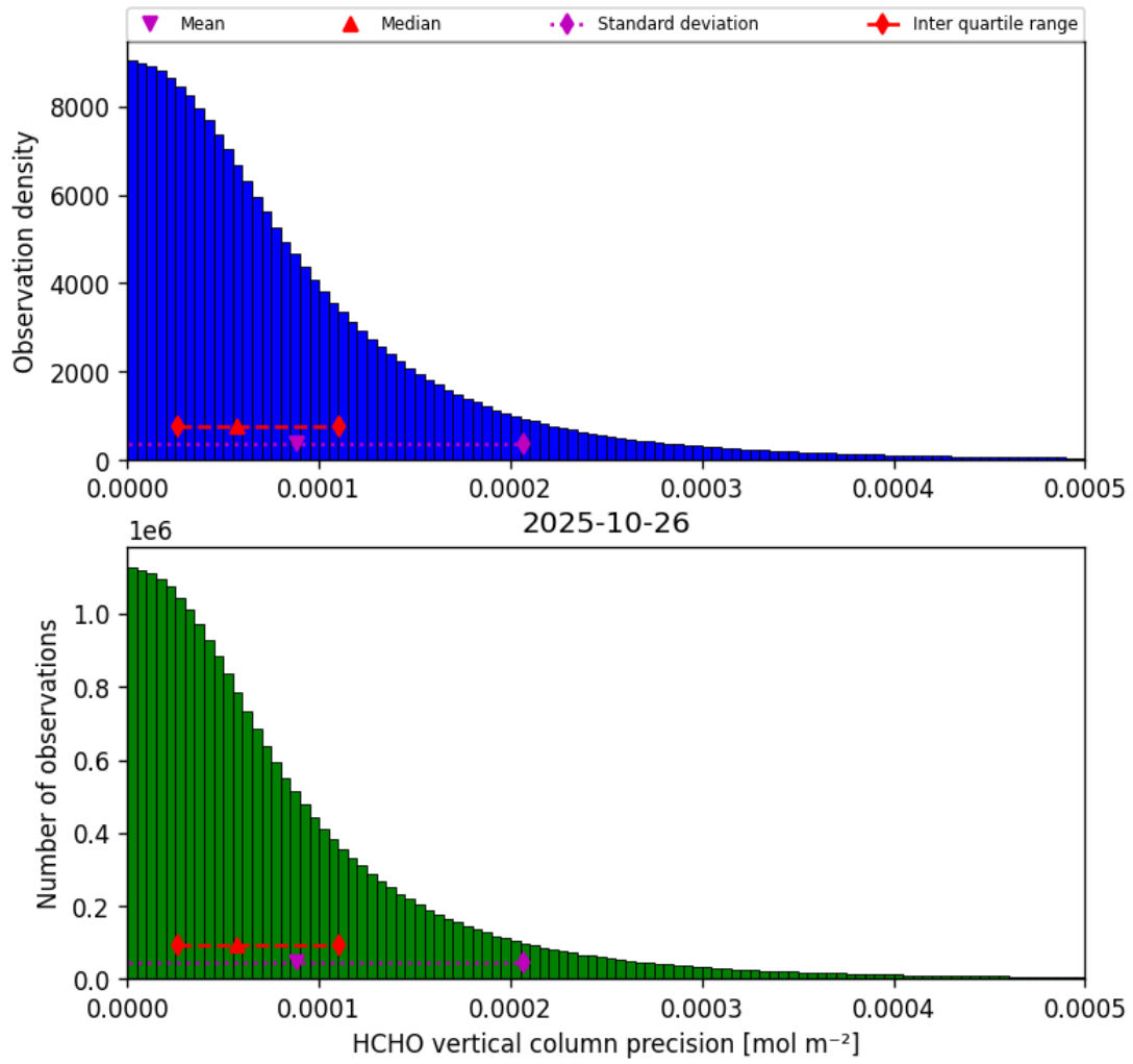
Figure 34: Histogram of “HCHO vertical column precision” for 2025-10-26 to 2025-10-27
