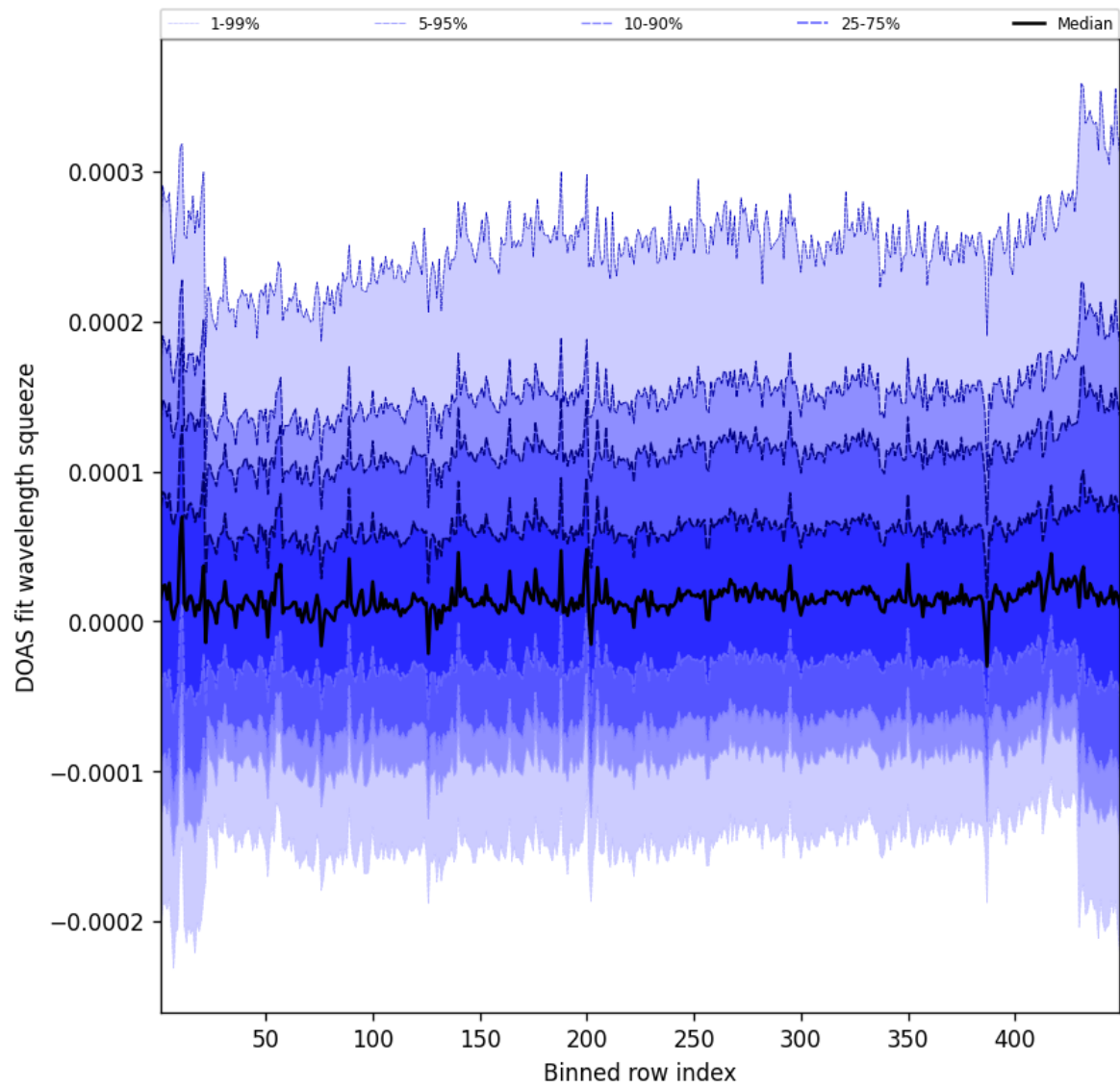
Figure 57: Along track statistics of “DOAS fit wavelength squeeze” for 2025-10-26 to 2025-10-27
