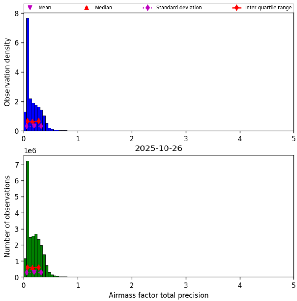
Figure 39: Histogram of “Airmass factor total precision” for 2025-10-26 to 2025-10-27
