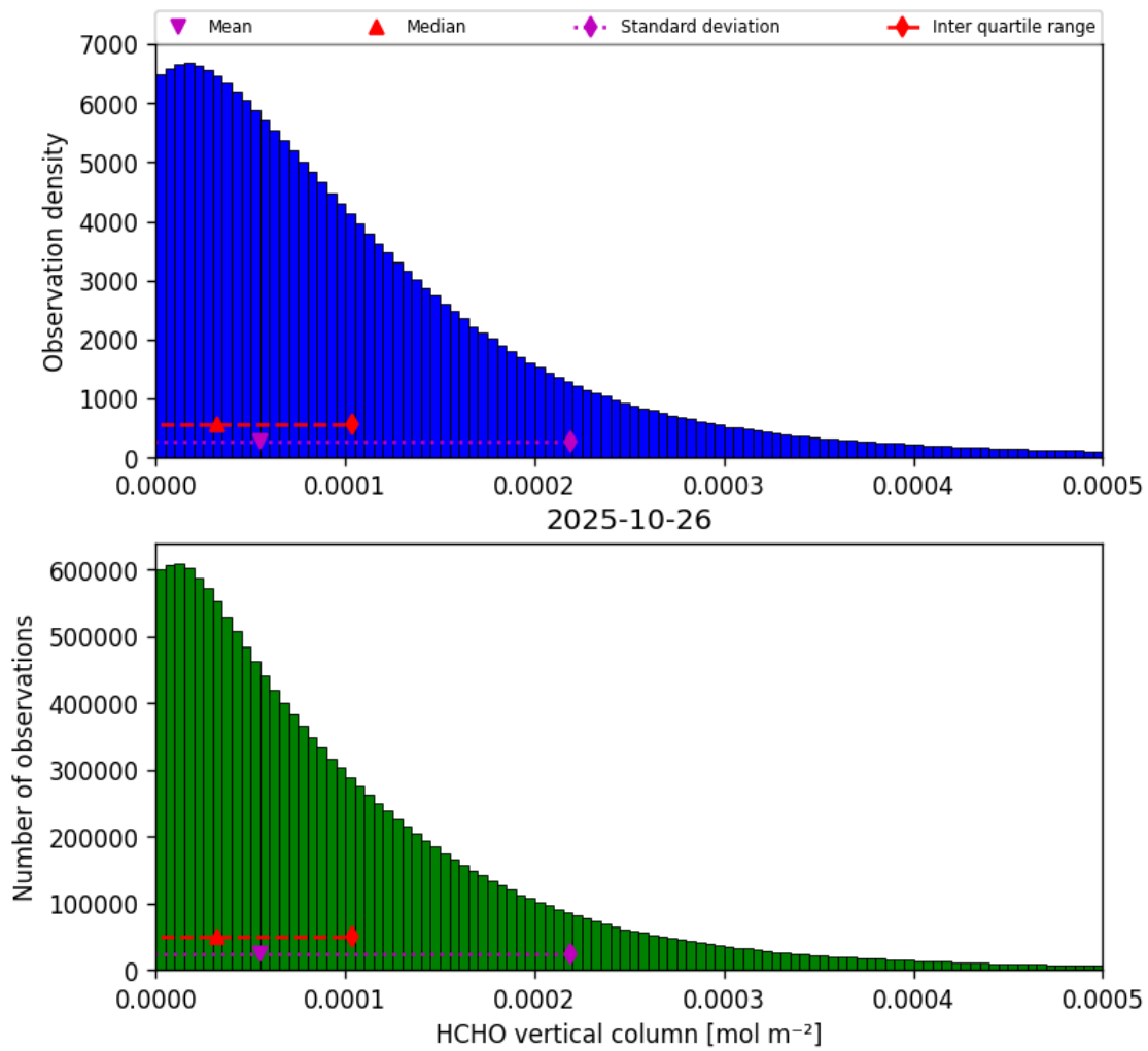
Figure 33: Histogram of “HCHO vertical column” for 2025-10-26 to 2025-10-27
