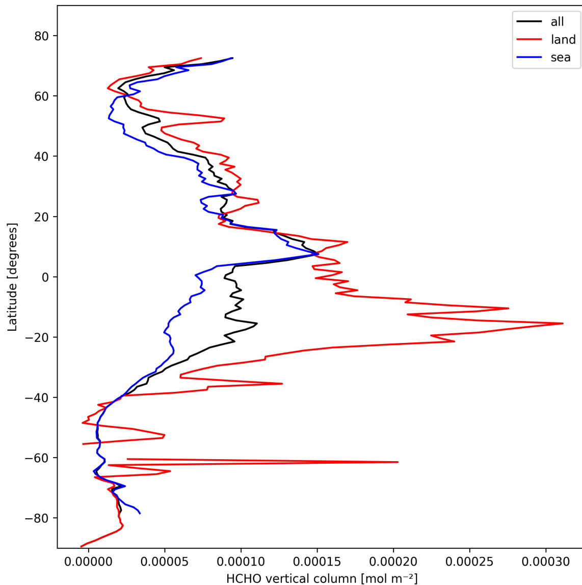
Figure 19: Zonal average of “HCHO vertical column” for 2025-10-26 to 2025-10-27.
