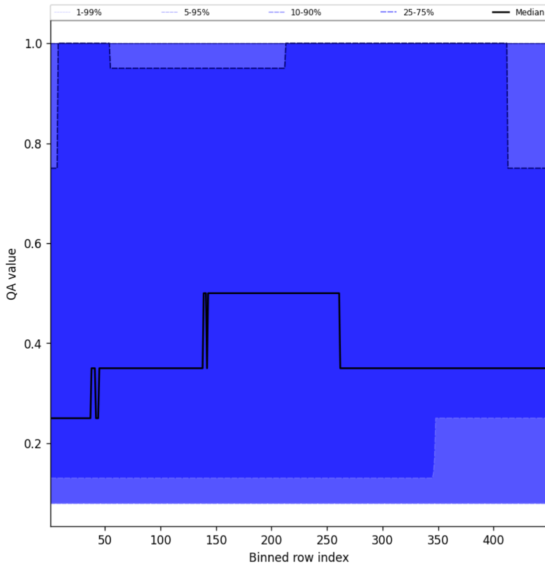
Figure 46: Along track statistics of “QA value” for 2025-10-26 to 2025-10-27
