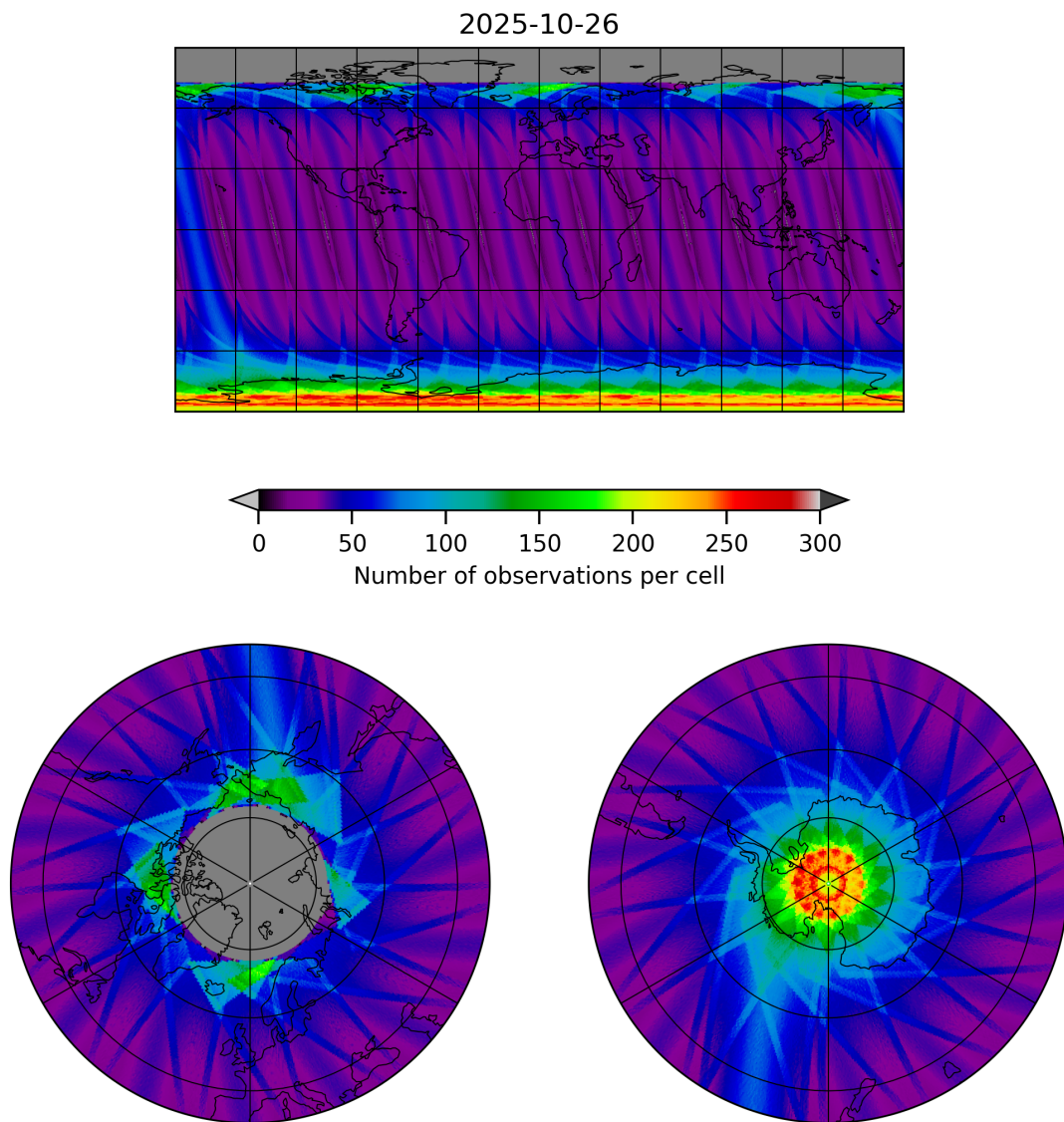
Figure 17: Map of the number of observations for 2025-10-26 to 2025-10-27
