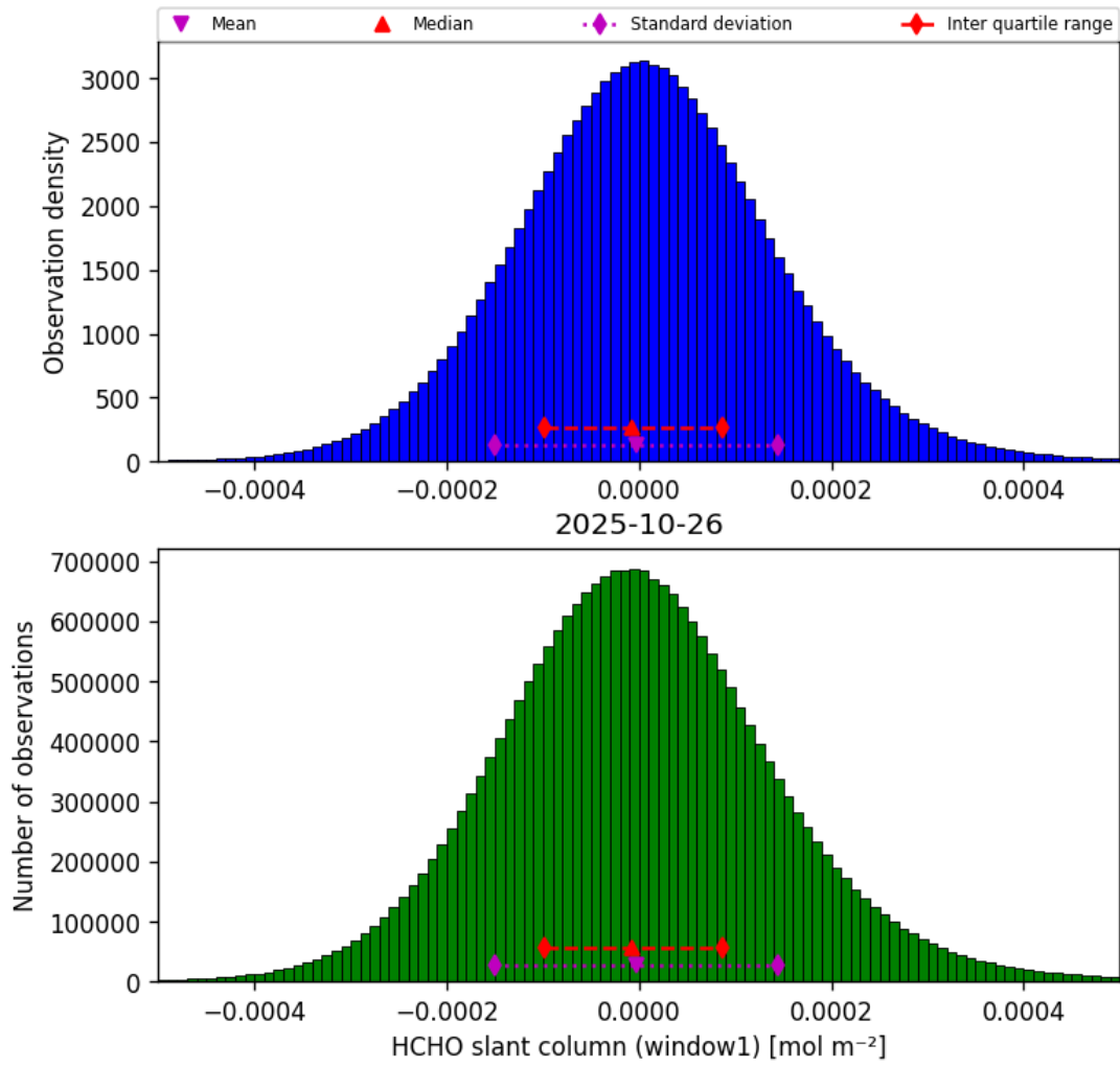
Figure 36: Histogram of “HCHO slant column (window1)” for 2025-10-26 to 2025-10-27
