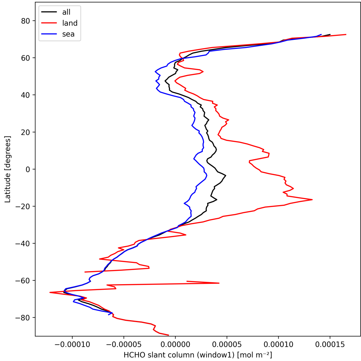
Figure 22: Zonal average of “HCHO slant column (window1)” for 2025-10-26 to 2025-10-27.
