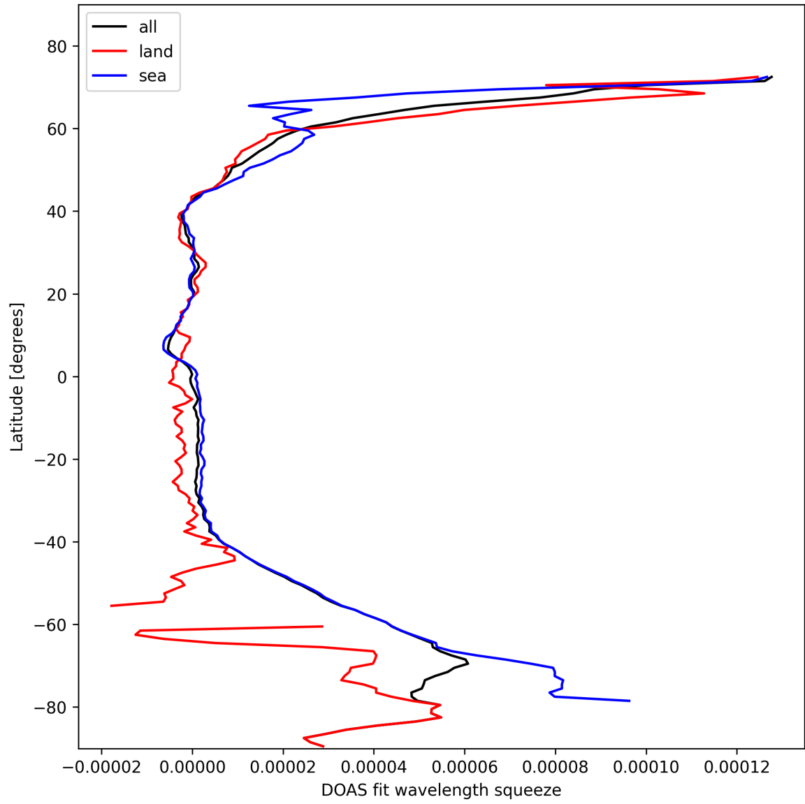
Figure 29: Zonal average of “DOAS fit wavelength squeeze” for 2025-10-26 to 2025-10-27.
