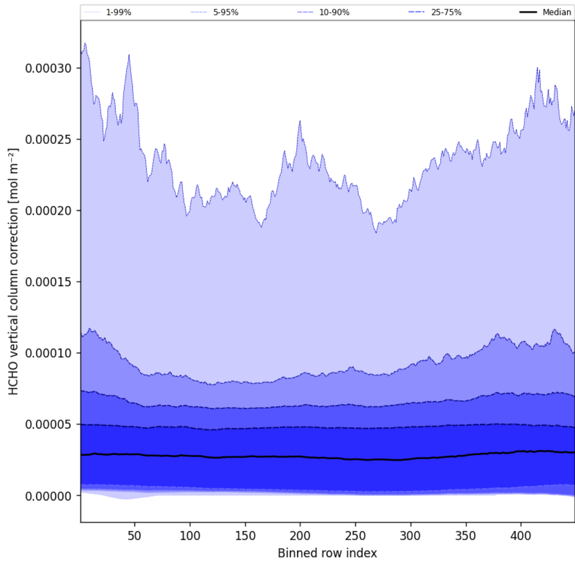
Figure 49: Along track statistics of “HCHO vertical column correction” for 2025-10-26 to 2025-10-27
