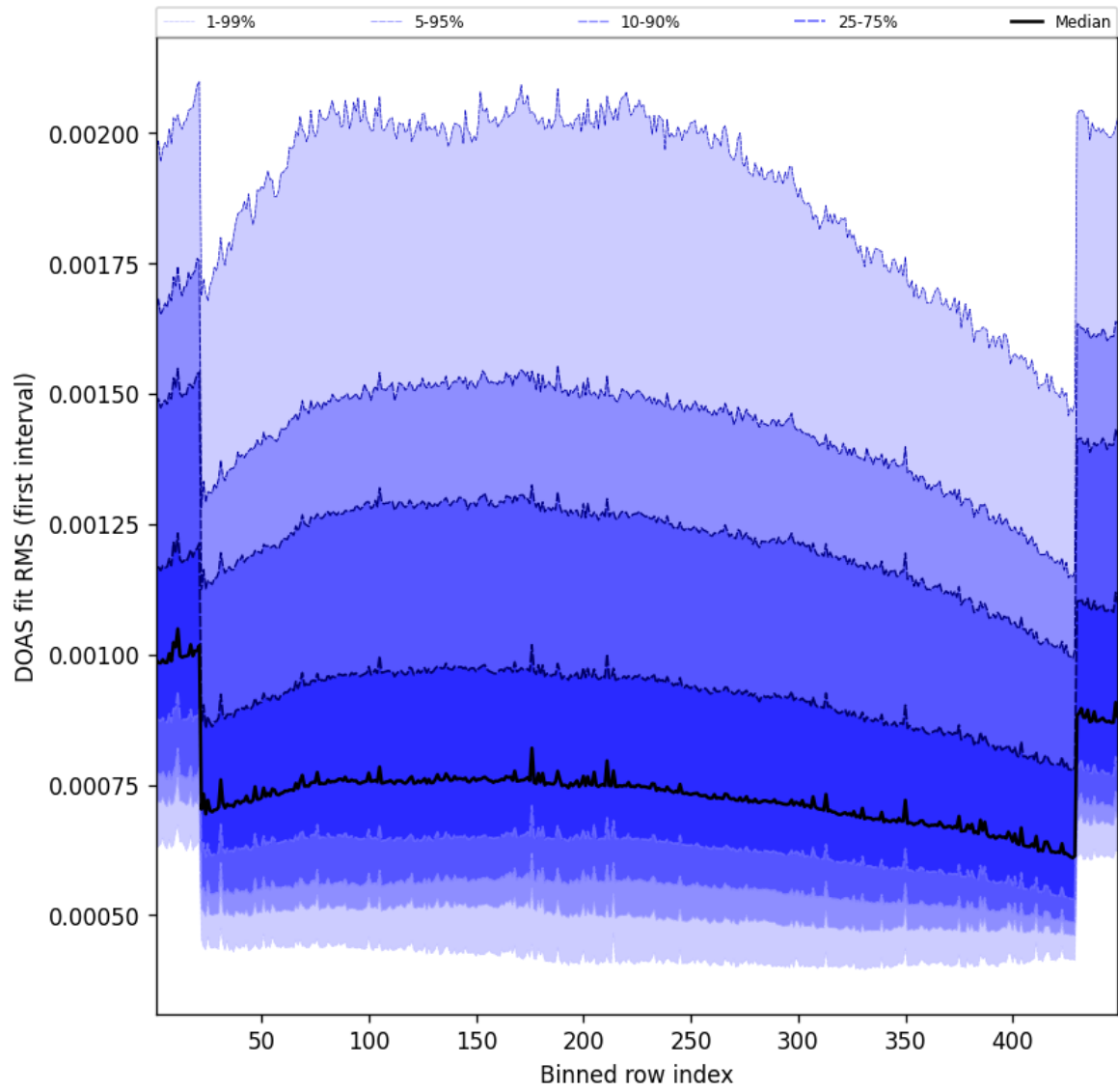
Figure 58: Along track statistics of “DOAS fit RMS (first interval)” for 2025-10-26 to 2025-10-27
