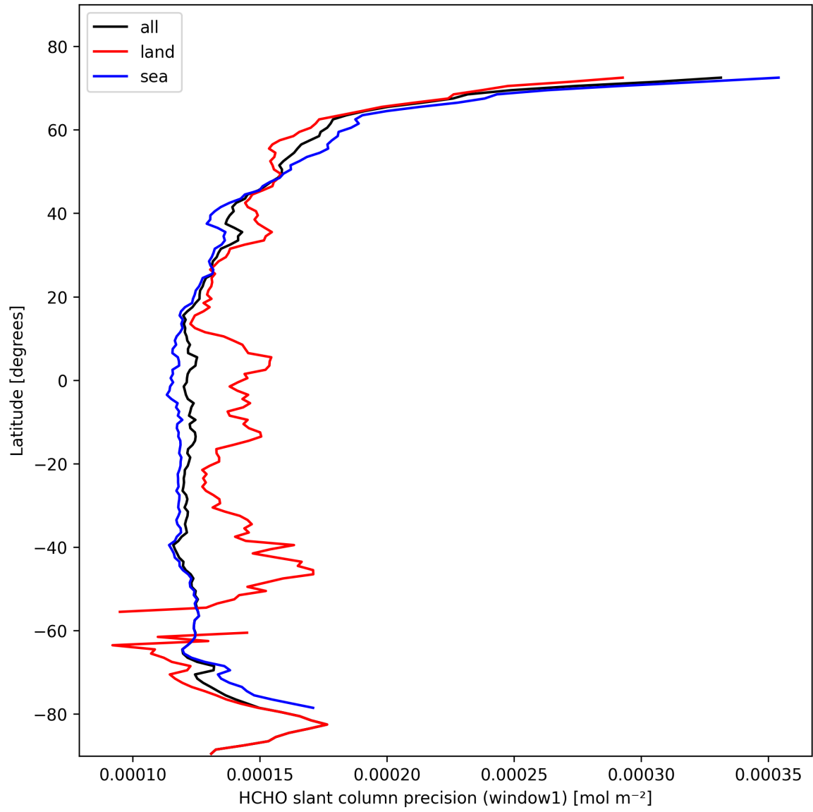
Figure 23: Zonal average of “HCHO slant column precision (window1)” for 2025-10-26 to 2025-10-27.
