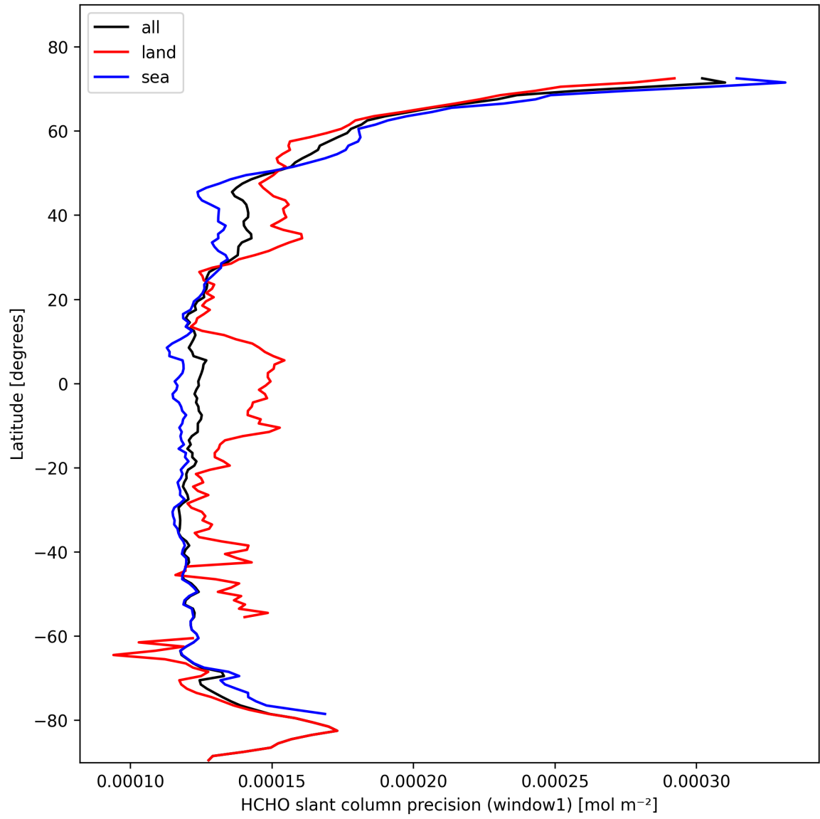
Figure 23: Zonal average of “HCHO slant column precision (window1)” for 2025-10-27 to 2025-10-28.
