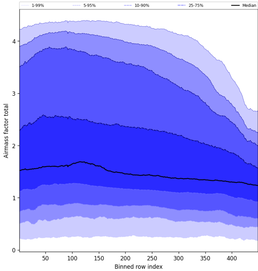
Figure 52: Along track statistics of “Airmass factor total” for 2025-10-27 to 2025-10-28
