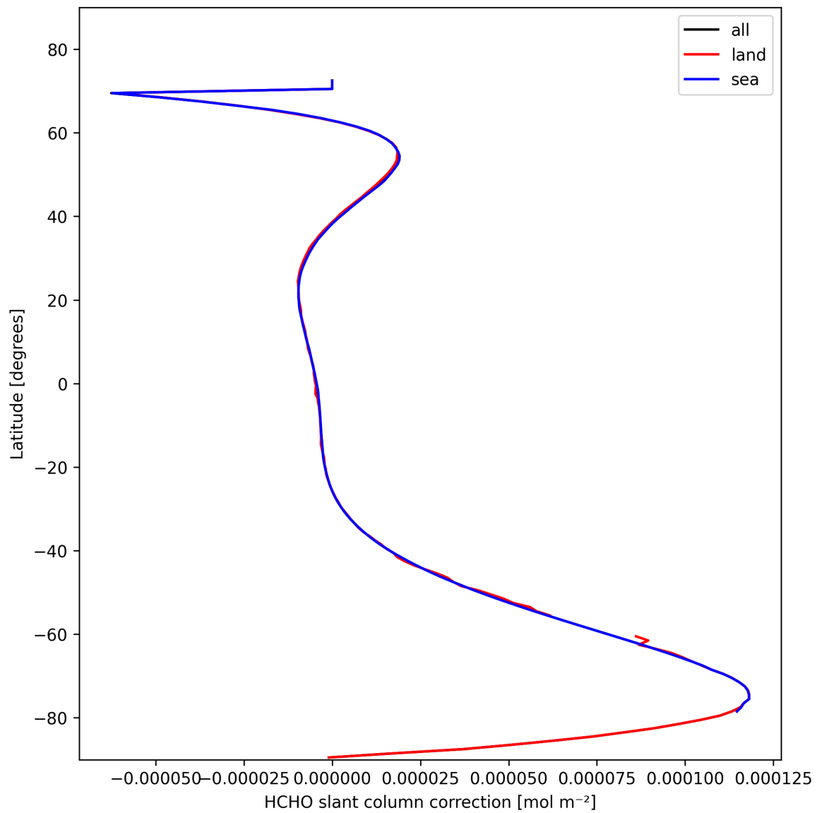
Figure 31: Zonal average of “HCHO slant column correction” for 2025-10-27 to 2025-10-28.
