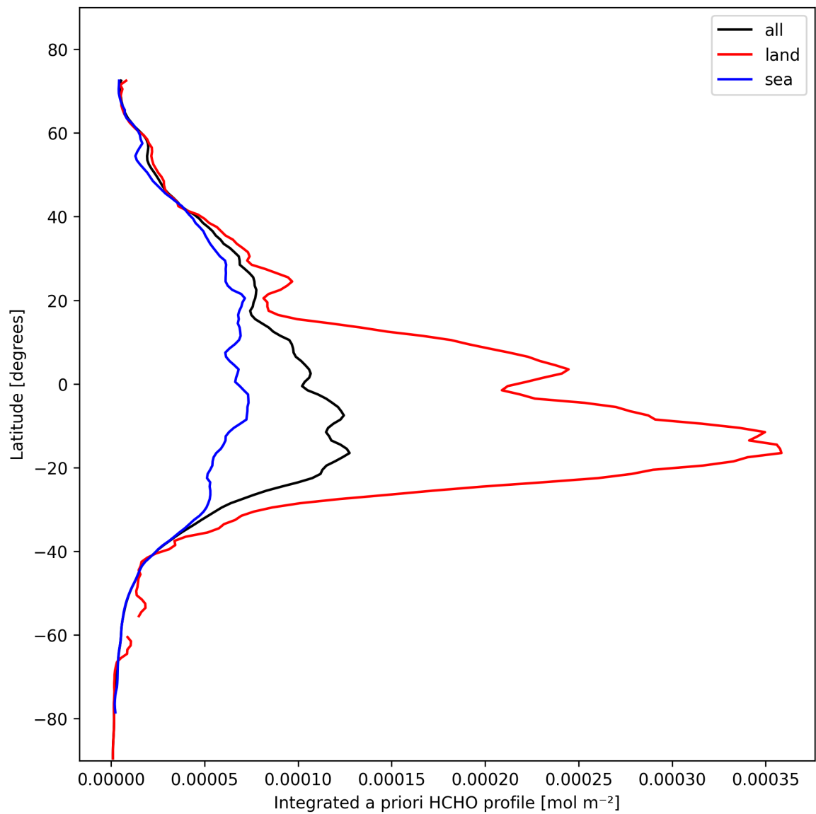
Figure 27: Zonal average of “Integrated a priori HCHO profile” for 2025-10-27 to 2025-10-28.
