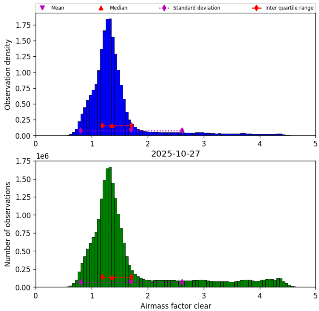
Figure 40: Histogram of “Airmass factor clear” for 2025-10-27 to 2025-10-28
