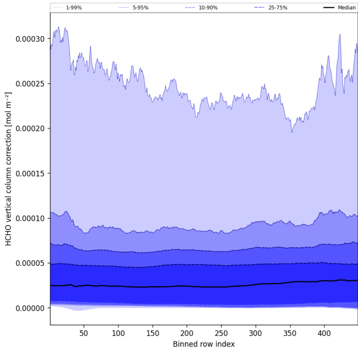
Figure 49: Along track statistics of “HCHO vertical column correction” for 2025-10-27 to 2025-10-28
