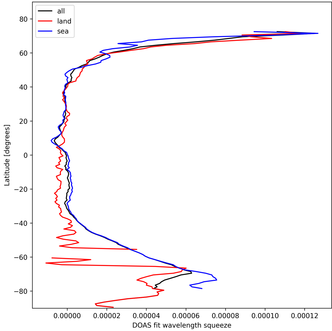
Figure 29: Zonal average of “DOAS fit wavelength squeeze” for 2025-10-27 to 2025-10-28.
