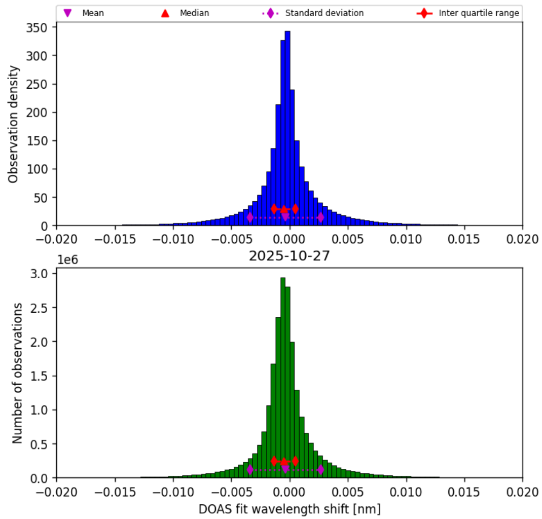
Figure 42: Histogram of “DOAS fit wavelength shift” for 2025-10-27 to 2025-10-28
