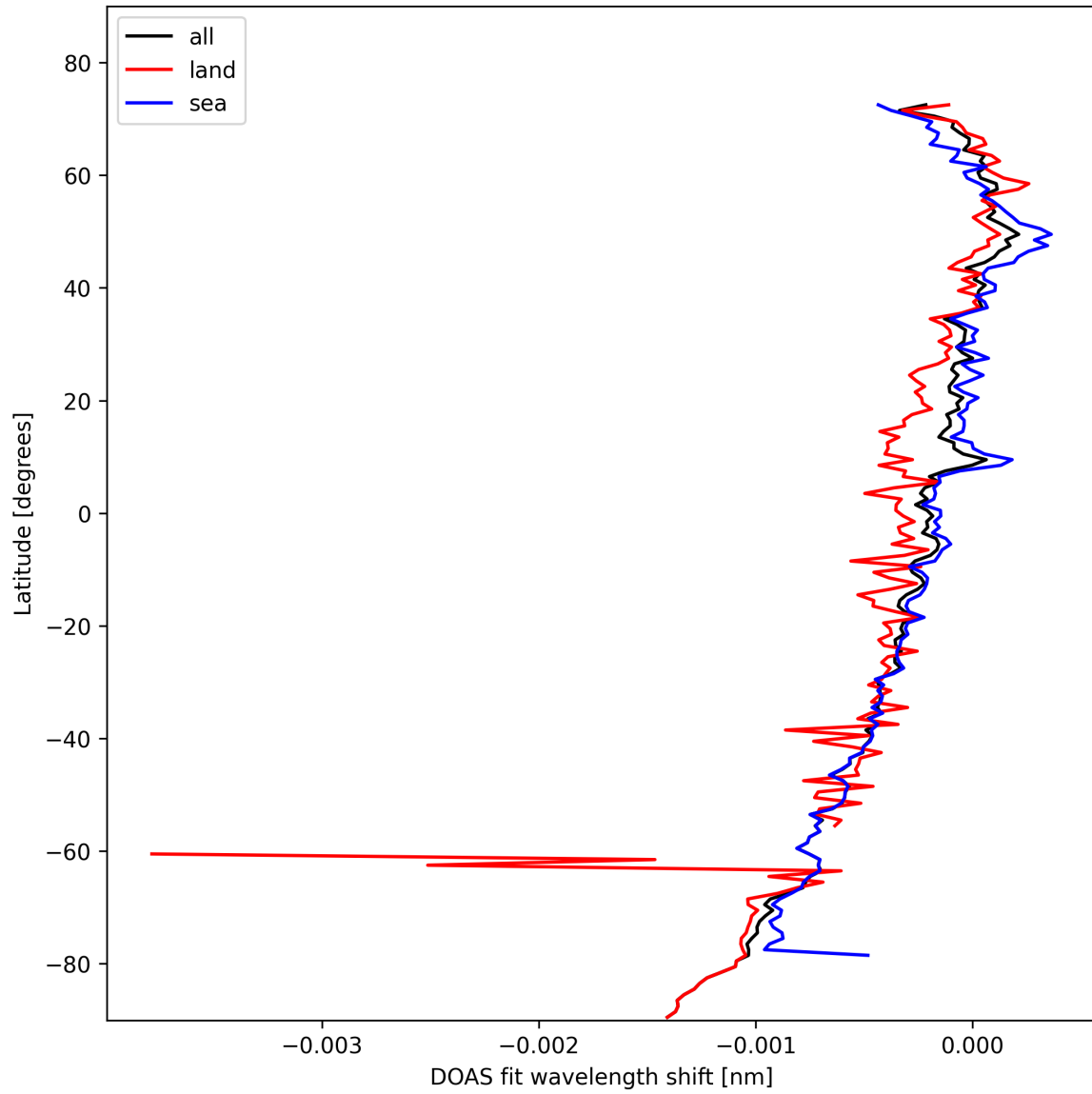
Figure 28: Zonal average of “DOAS fit wavelength shift” for 2025-10-27 to 2025-10-28.
