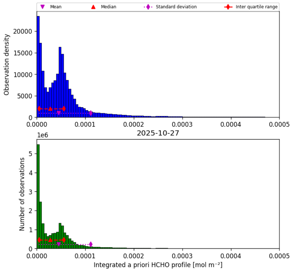
Figure 41: Histogram of “Integrated a priori HCHO profile” for 2025-10-27 to 2025-10-28
