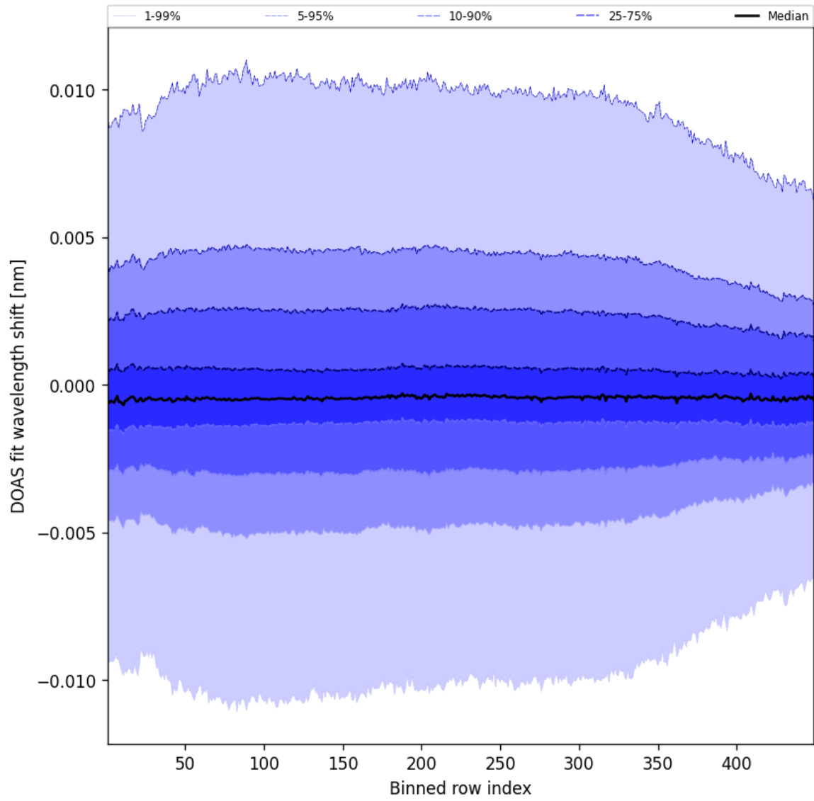
Figure 56: Along track statistics of “DOAS fit wavelength shift” for 2025-10-27 to 2025-10-28
