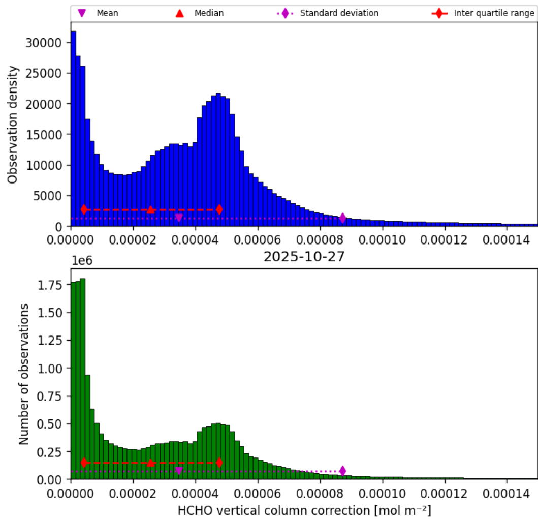
Figure 35: Histogram of “HCHO vertical column correction” for 2025-10-27 to 2025-10-28
