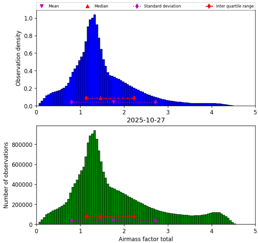
Figure 38: Histogram of “Airmass factor total” for 2025-10-27 to 2025-10-28
