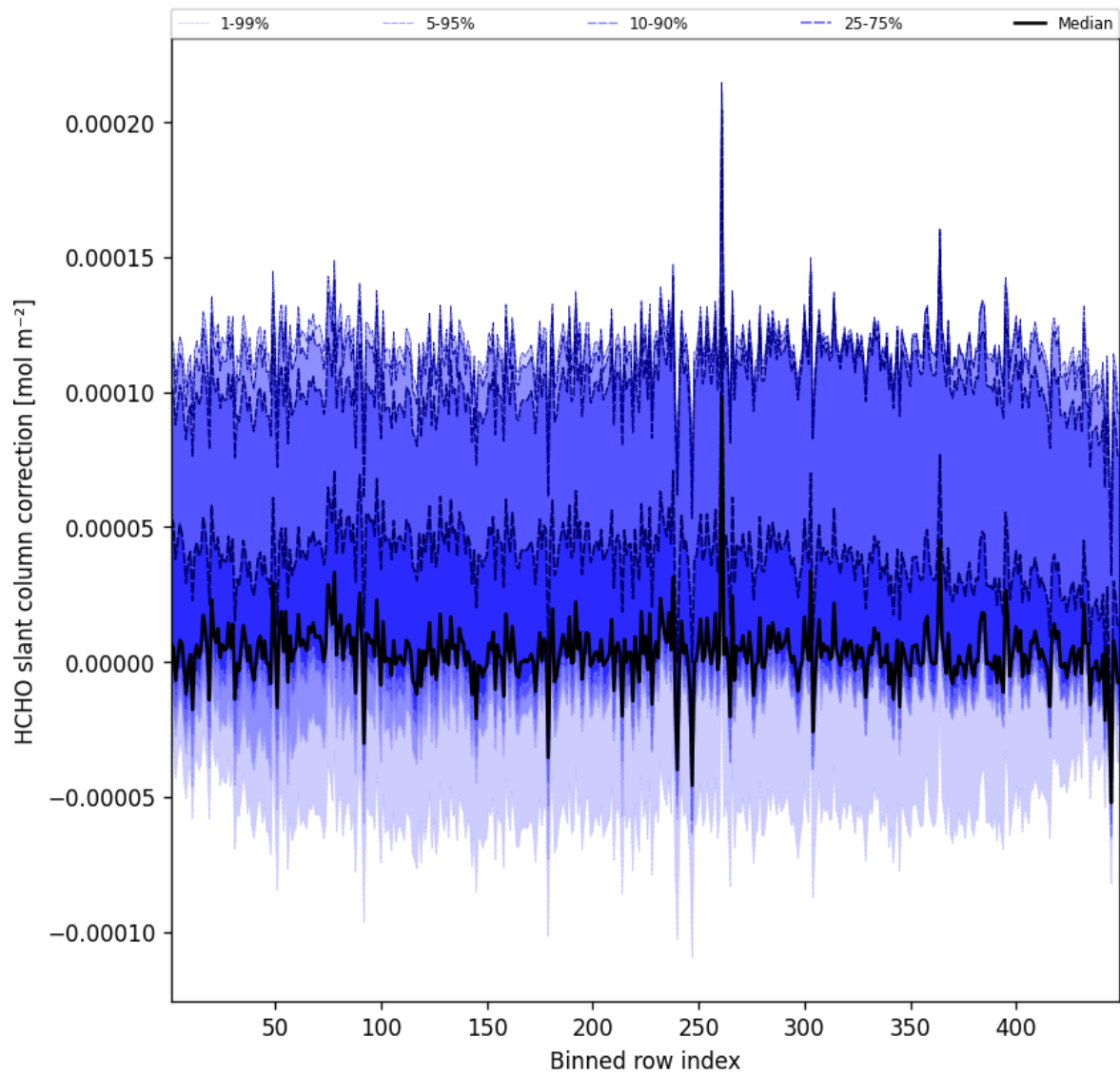
Figure 59: Along track statistics of “HCHO slant column correction” for 2025-10-27 to 2025-10-28
