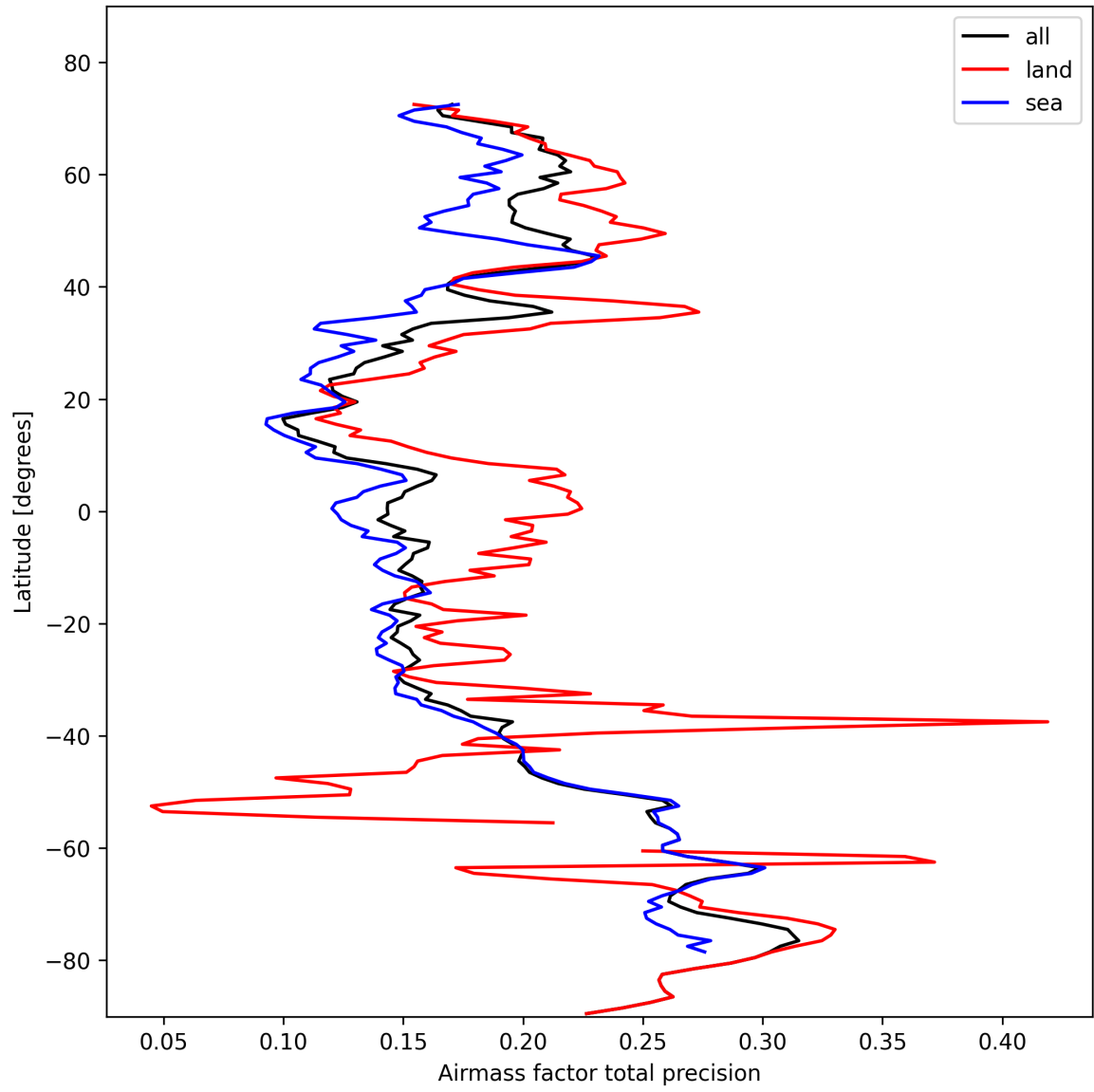
Figure 25: Zonal average of “Airmass factor total precision” for 2025-10-27 to 2025-10-28.
