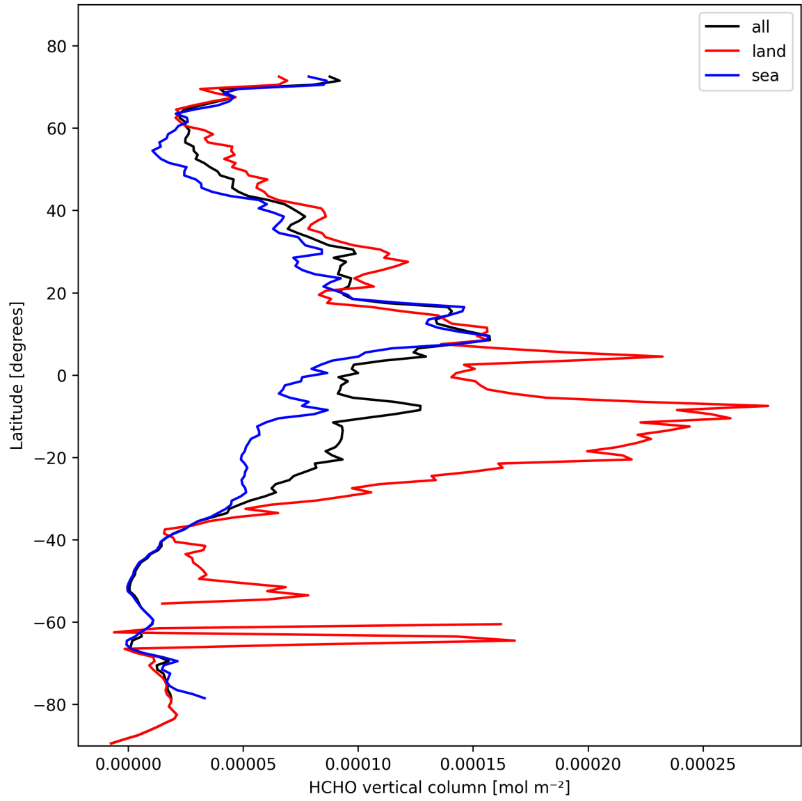
Figure 19: Zonal average of “HCHO vertical column” for 2025-10-27 to 2025-10-28.
