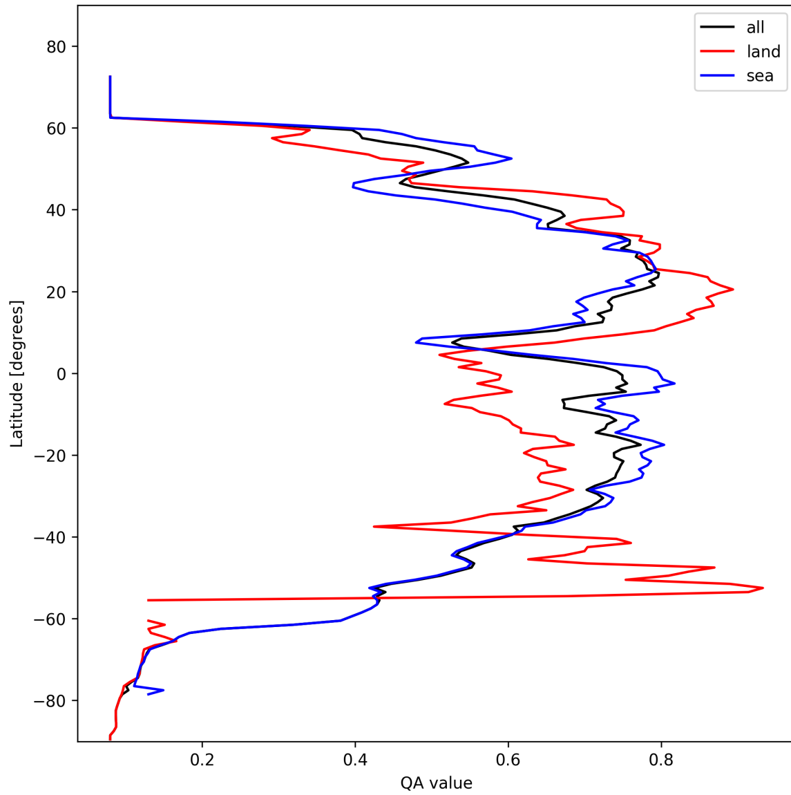
Figure 18: Zonal average of “QA value” for 2025-10-27 to 2025-10-28.
