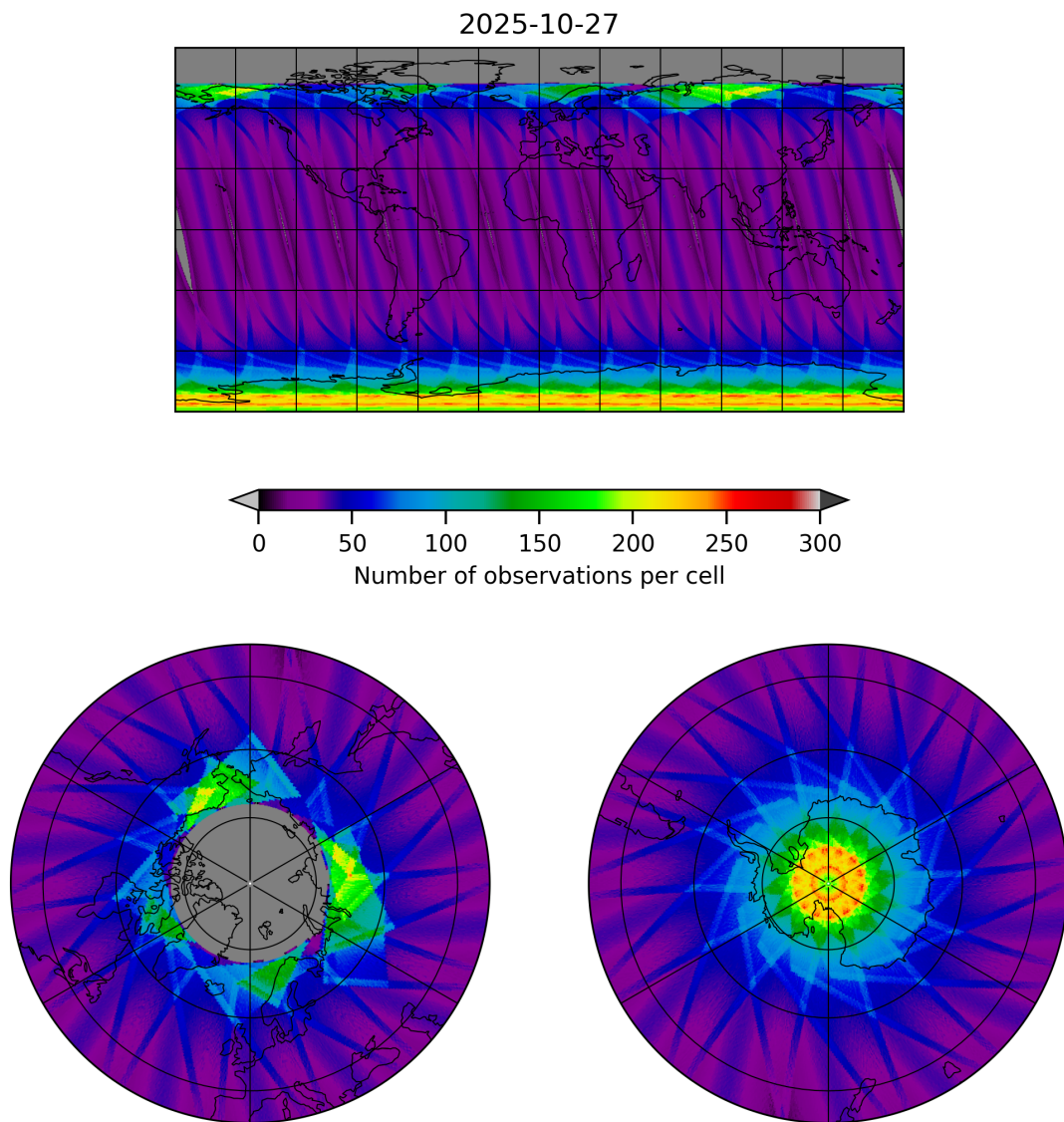
Figure 17: Map of the number of observations for 2025-10-27 to 2025-10-28
