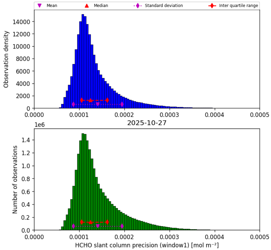
Figure 37: Histogram of “HCHO slant column precision (window1)” for 2025-10-27 to 2025-10-28
