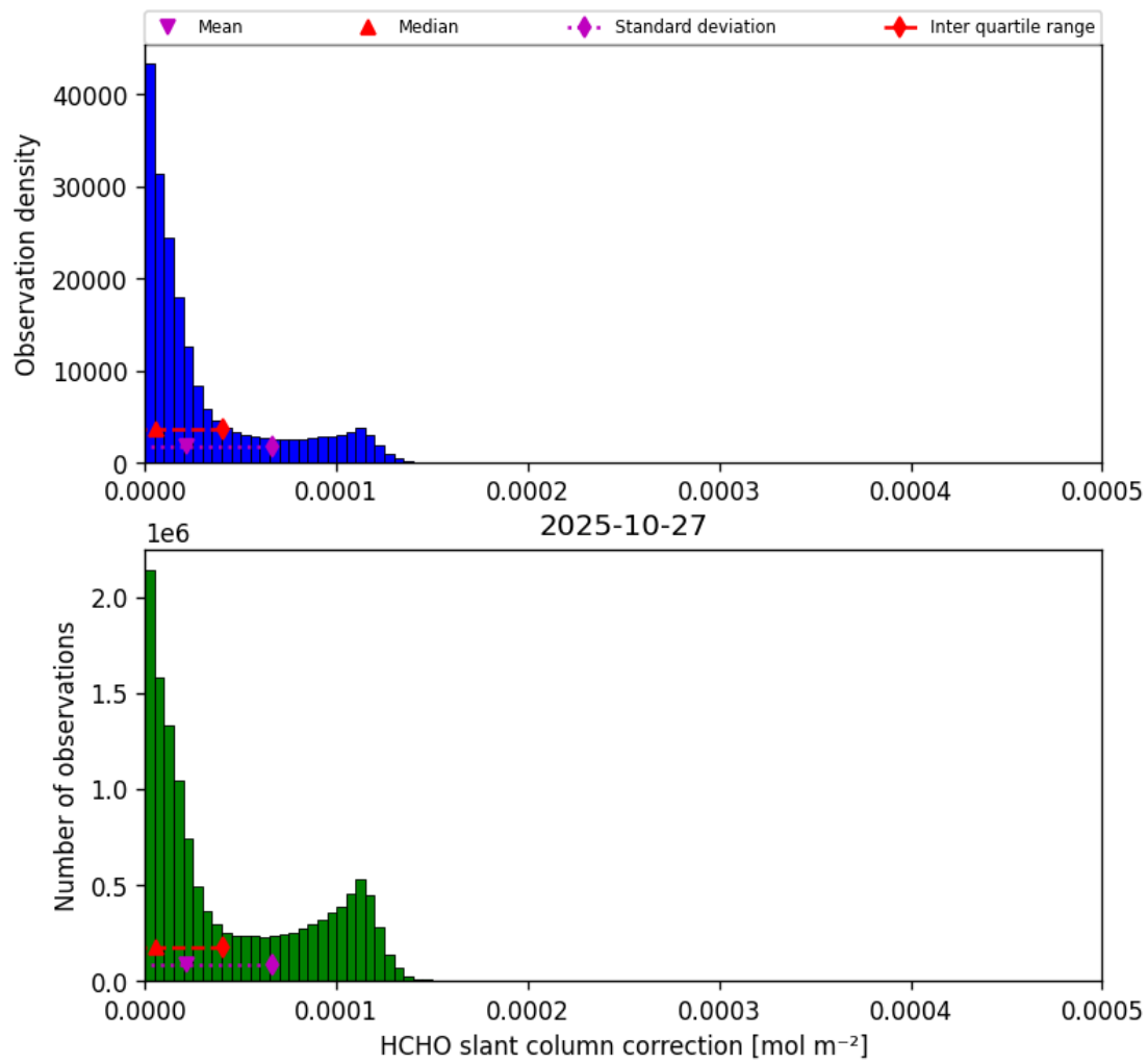
Figure 45: Histogram of “HCHO slant column correction” for 2025-10-27 to 2025-10-28
