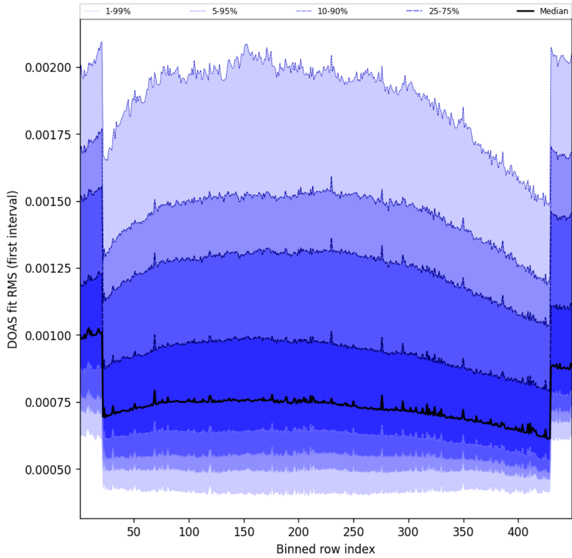
Figure 58: Along track statistics of “DOAS fit RMS (first interval)” for 2025-10-27 to 2025-10-28
