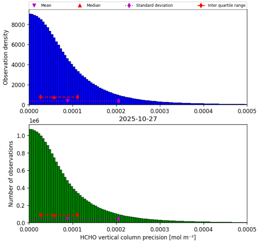
Figure 34: Histogram of “HCHO vertical column precision” for 2025-10-27 to 2025-10-28
