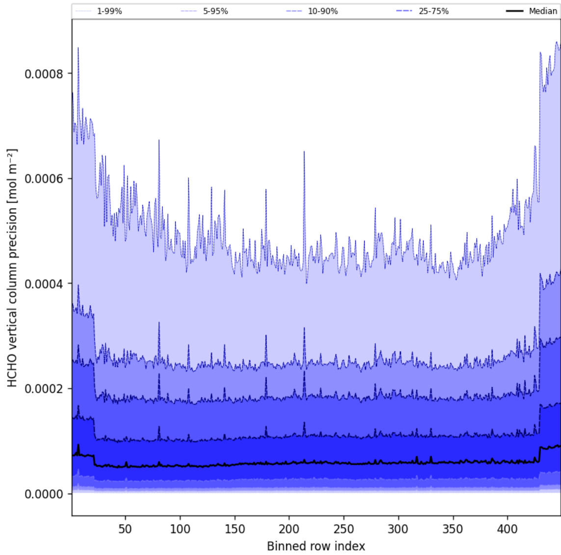
Figure 48: Along track statistics of “HCHO vertical column precision” for 2025-10-27 to 2025-10-28
