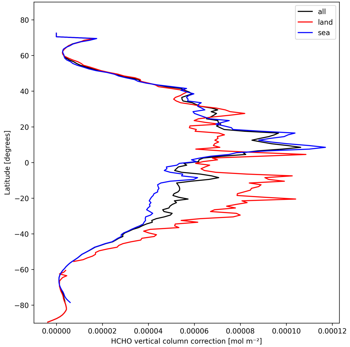
Figure 21: Zonal average of “HCHO vertical column correction” for 2025-10-27 to 2025-10-28.
