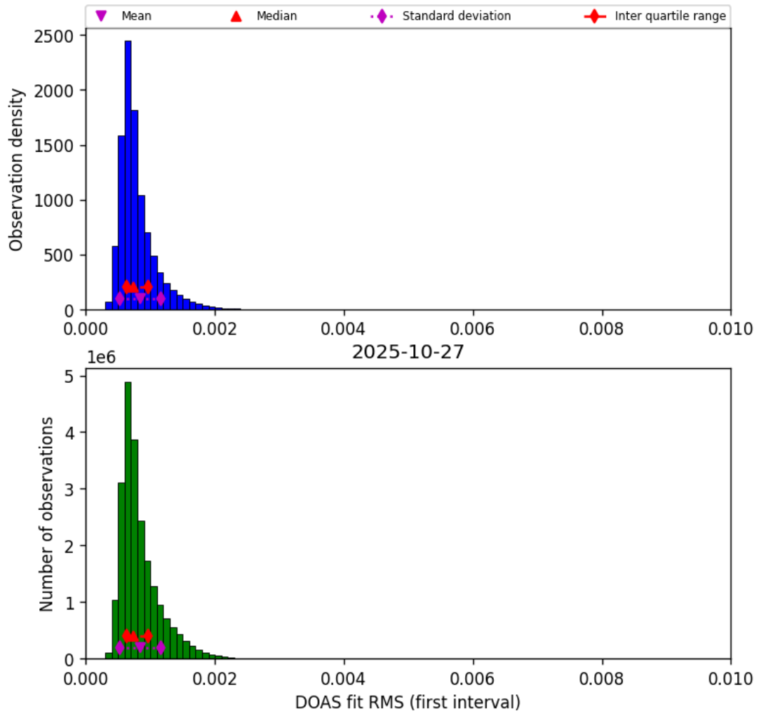
Figure 44: Histogram of “DOAS fit RMS (first interval)” for 2025-10-27 to 2025-10-28
