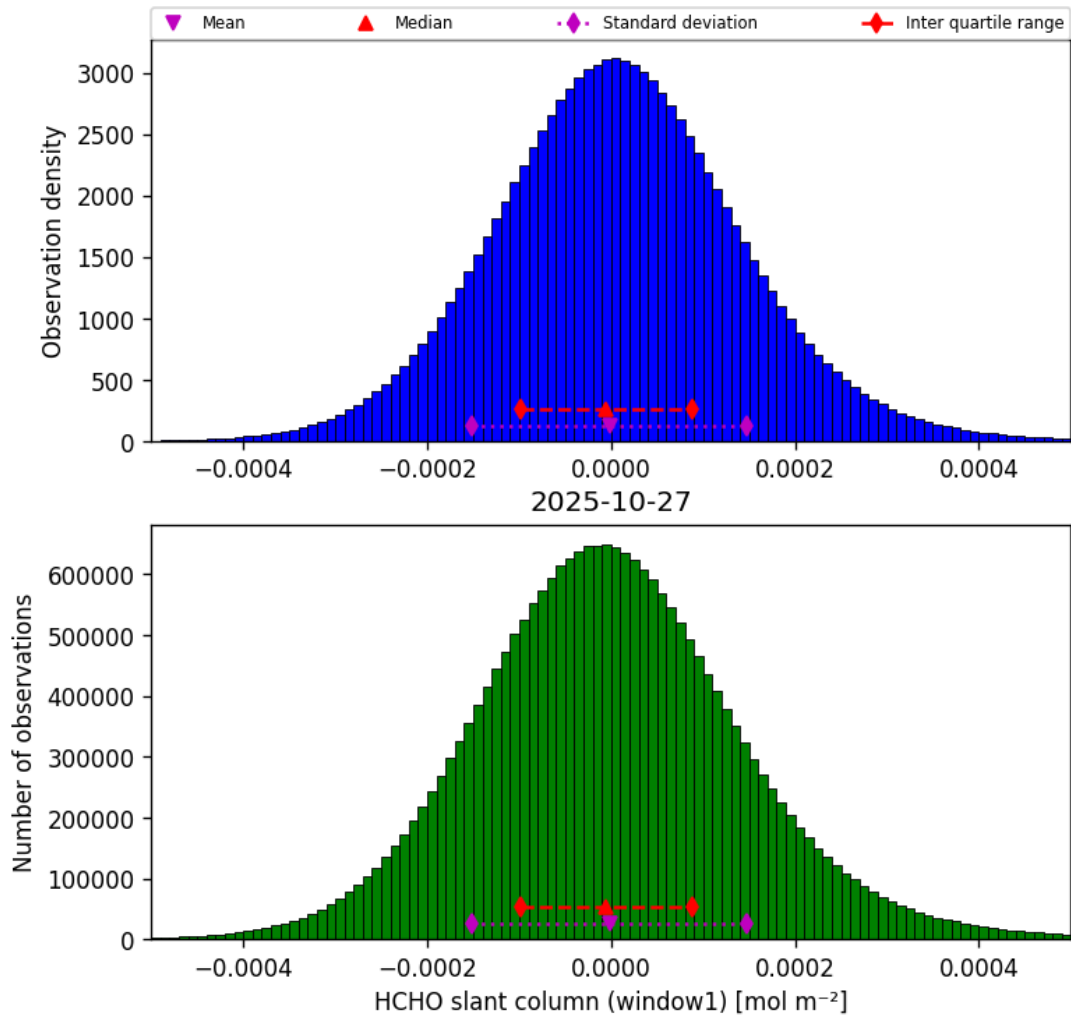
Figure 36: Histogram of “HCHO slant column (window1)” for 2025-10-27 to 2025-10-28
