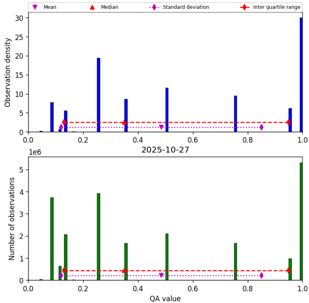
Figure 32: Histogram of “QA value” for 2025-10-27 to 2025-10-28
