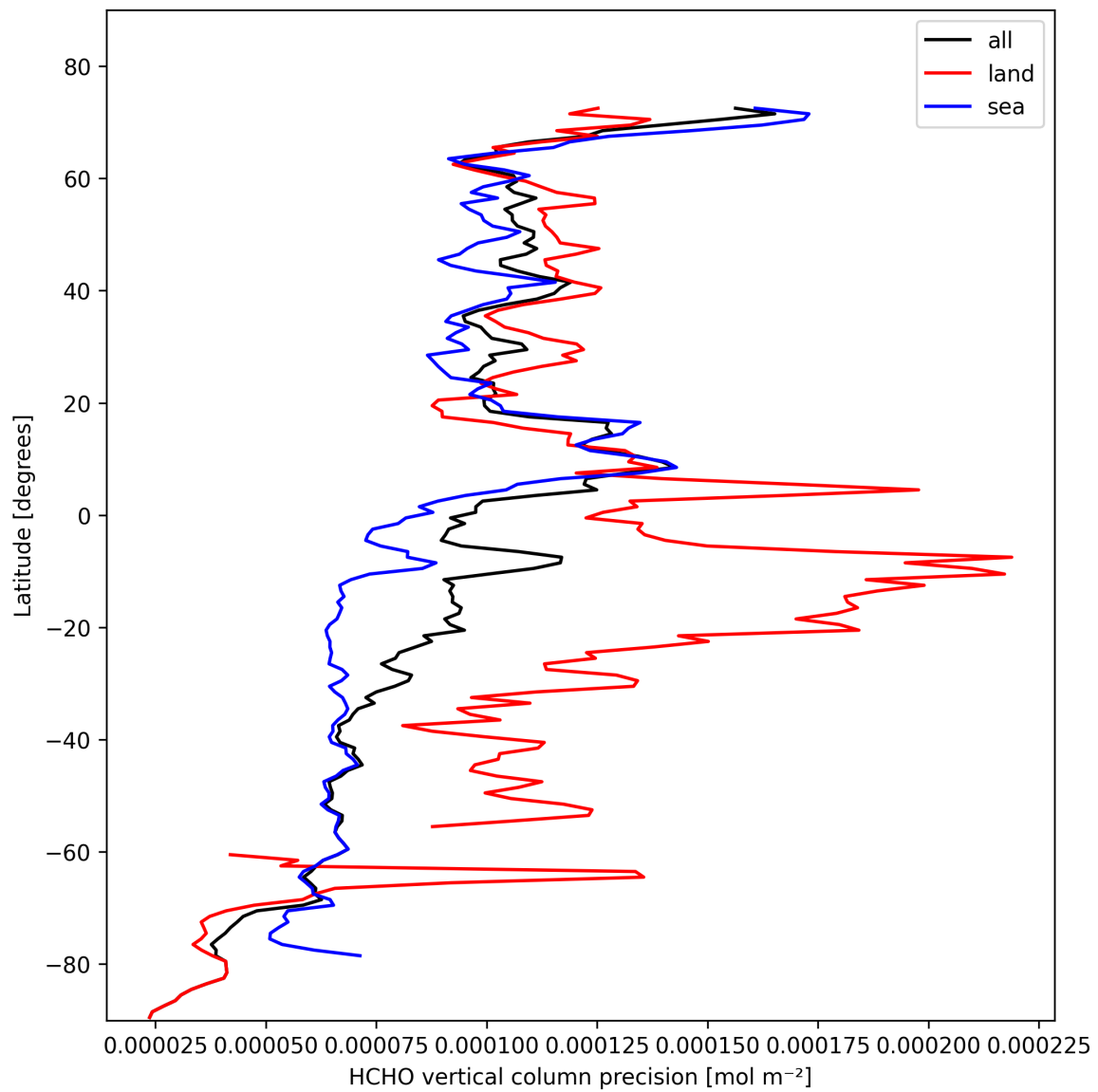
Figure 20: Zonal average of “HCHO vertical column precision” for 2025-10-27 to 2025-10-28.
