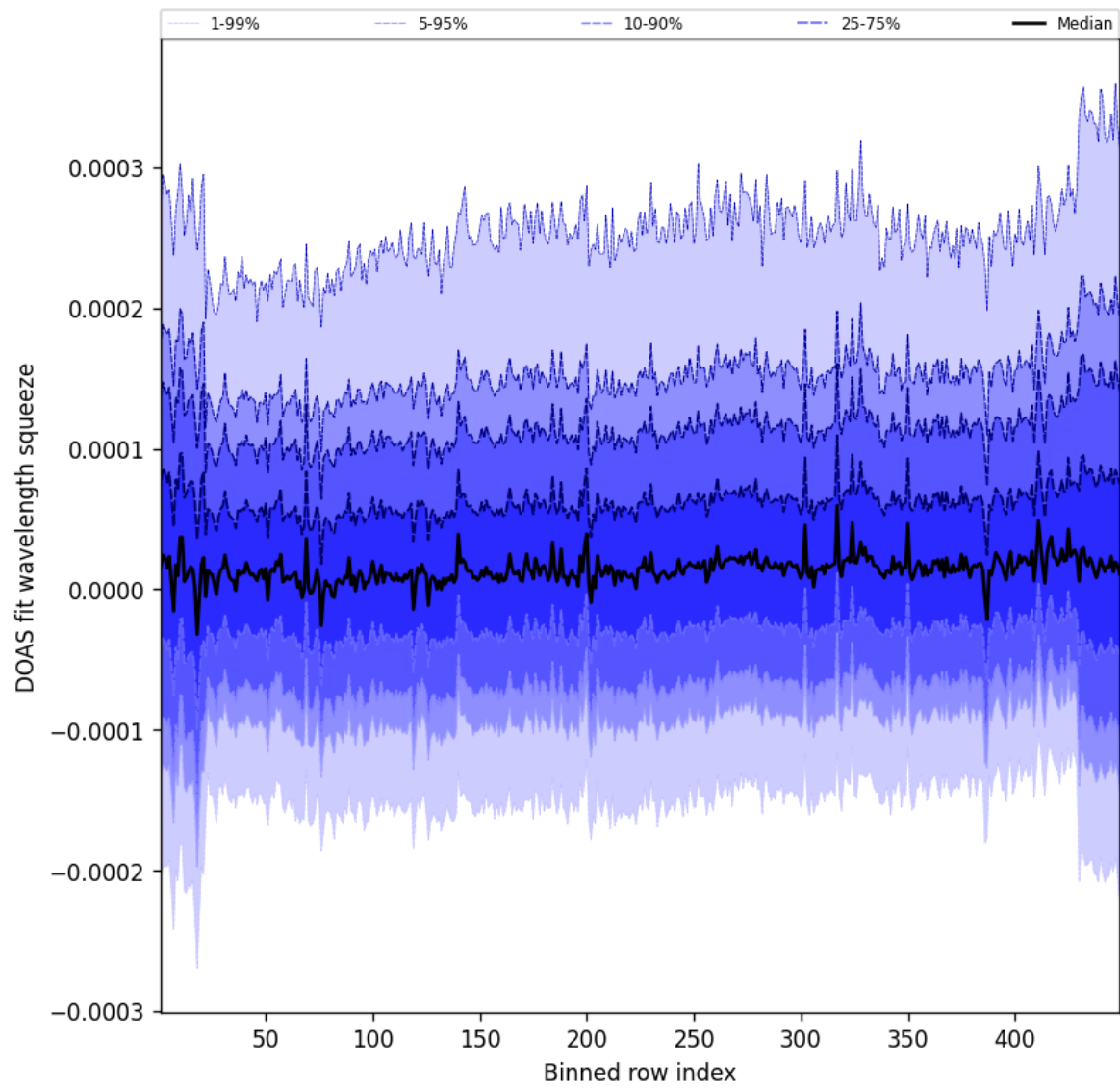
Figure 57: Along track statistics of “DOAS fit wavelength squeeze” for 2025-10-27 to 2025-10-28
