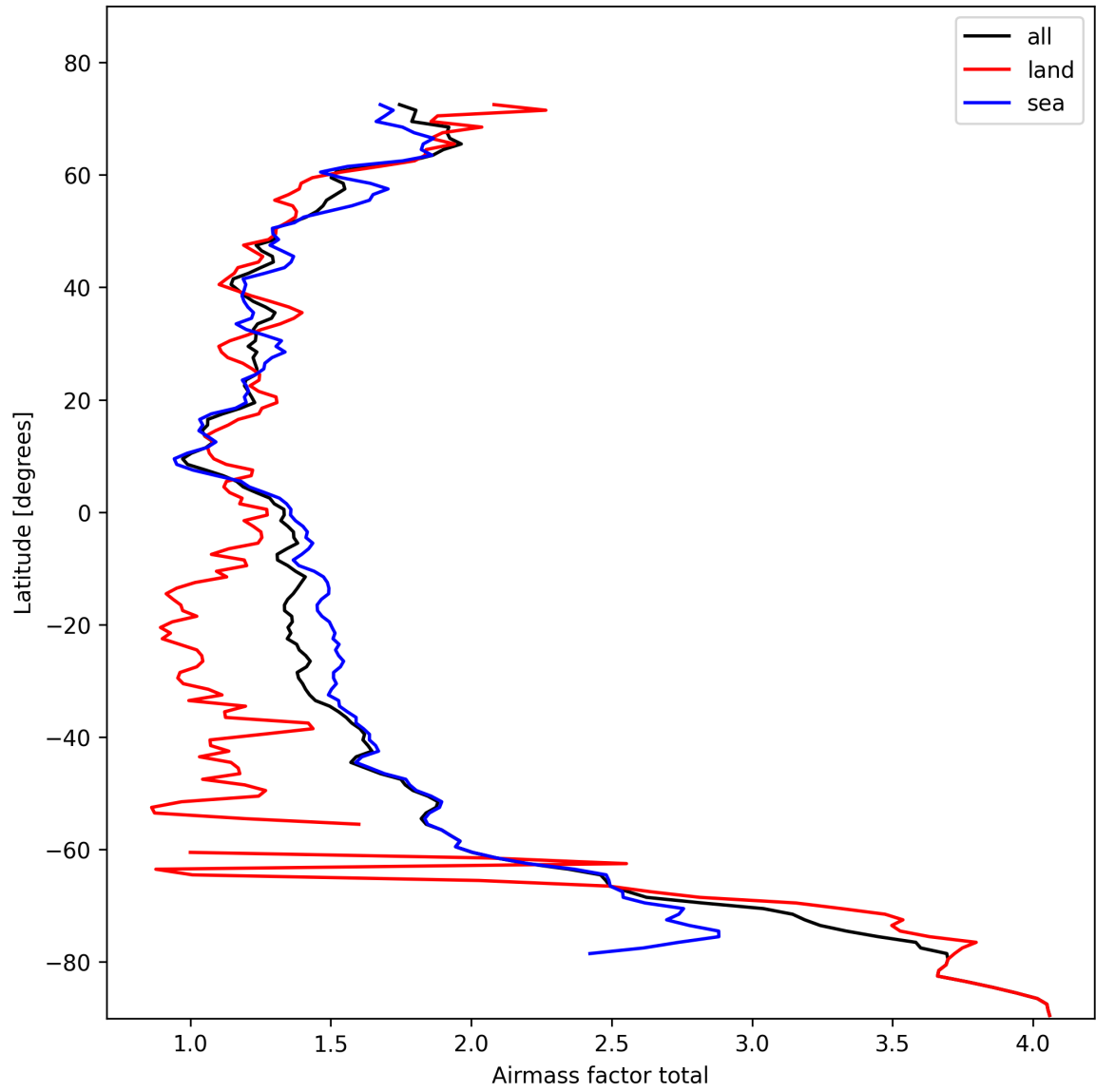
Figure 24: Zonal average of “Airmass factor total” for 2025-10-27 to 2025-10-28.
