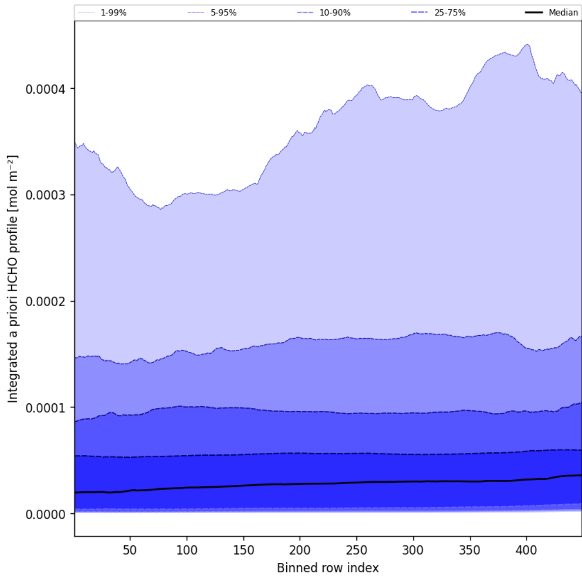
Figure 55: Along track statistics of “Integrated a priori HCHO profile” for 2025-10-27 to 2025-10-28
