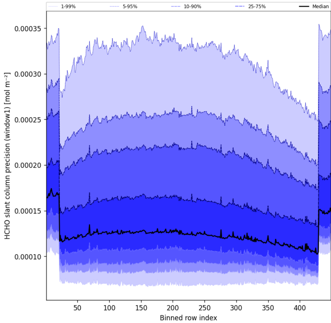
Figure 51: Along track statistics of “HCHO slant column precision (window1)” for 2025-10-27 to 2025-10-28
