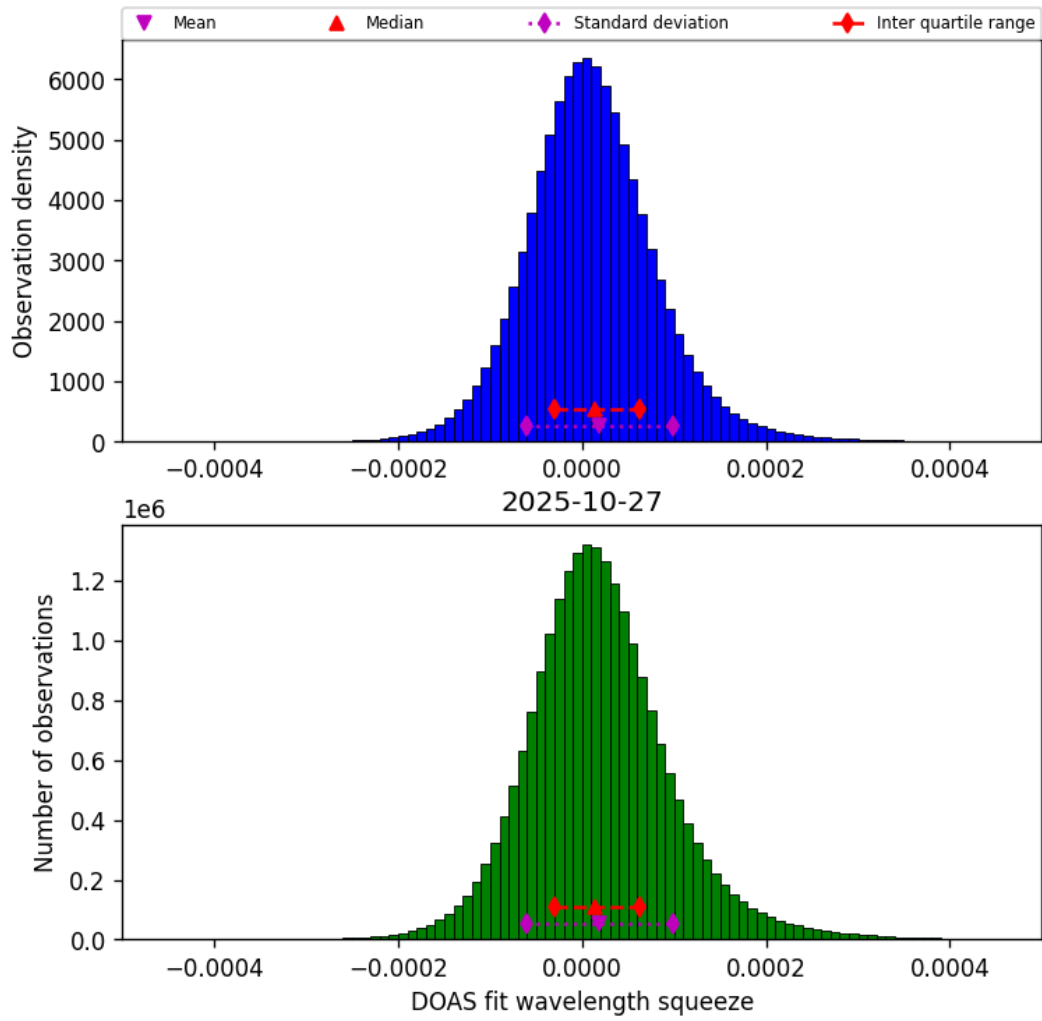
Figure 43: Histogram of “DOAS fit wavelength squeeze” for 2025-10-27 to 2025-10-28
