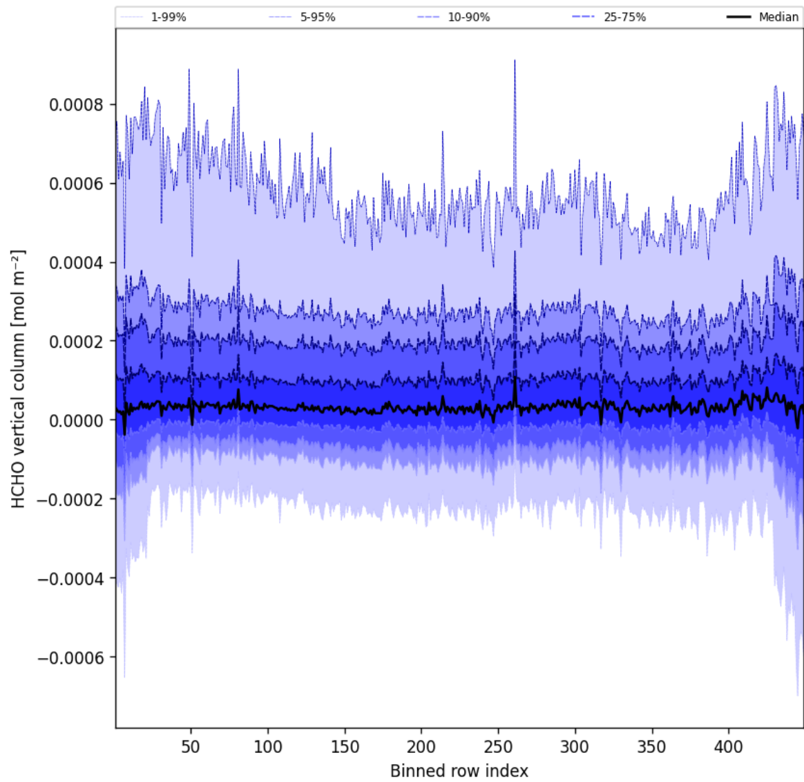
Figure 47: Along track statistics of “HCHO vertical column” for 2025-10-27 to 2025-10-28
