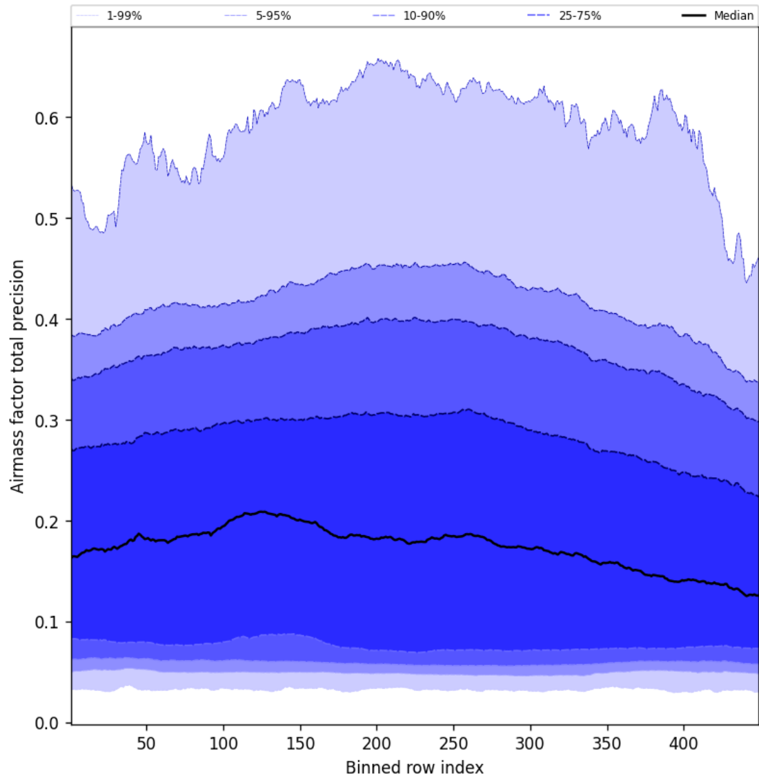
Figure 53: Along track statistics of “Airmass factor total precision” for 2025-10-27 to 2025-10-28
