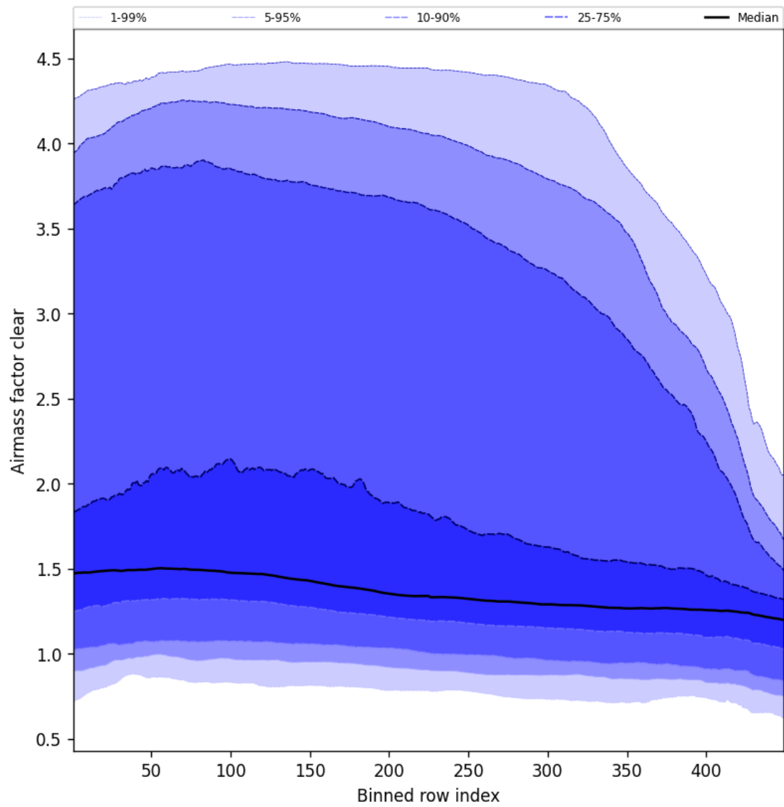
Figure 54: Along track statistics of “Airmass factor clear” for 2025-10-27 to 2025-10-28
