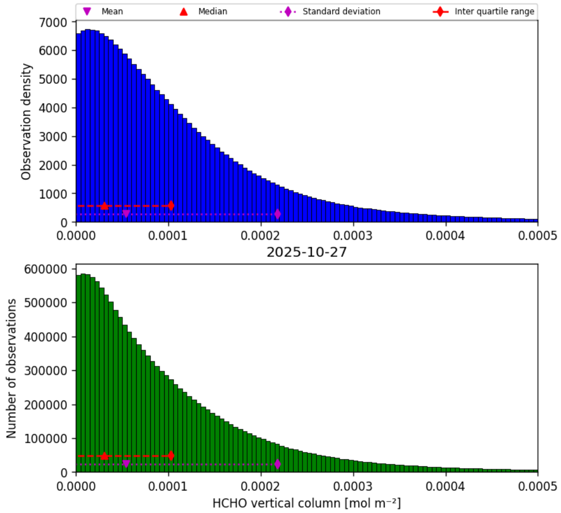
Figure 33: Histogram of “HCHO vertical column” for 2025-10-27 to 2025-10-28
