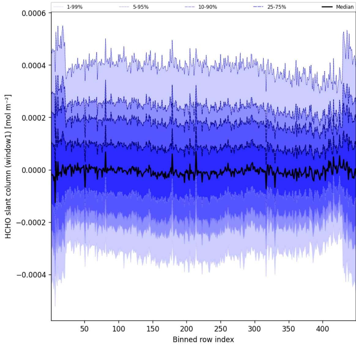
Figure 50: Along track statistics of “HCHO slant column (window1)” for 2025-10-27 to 2025-10-28
