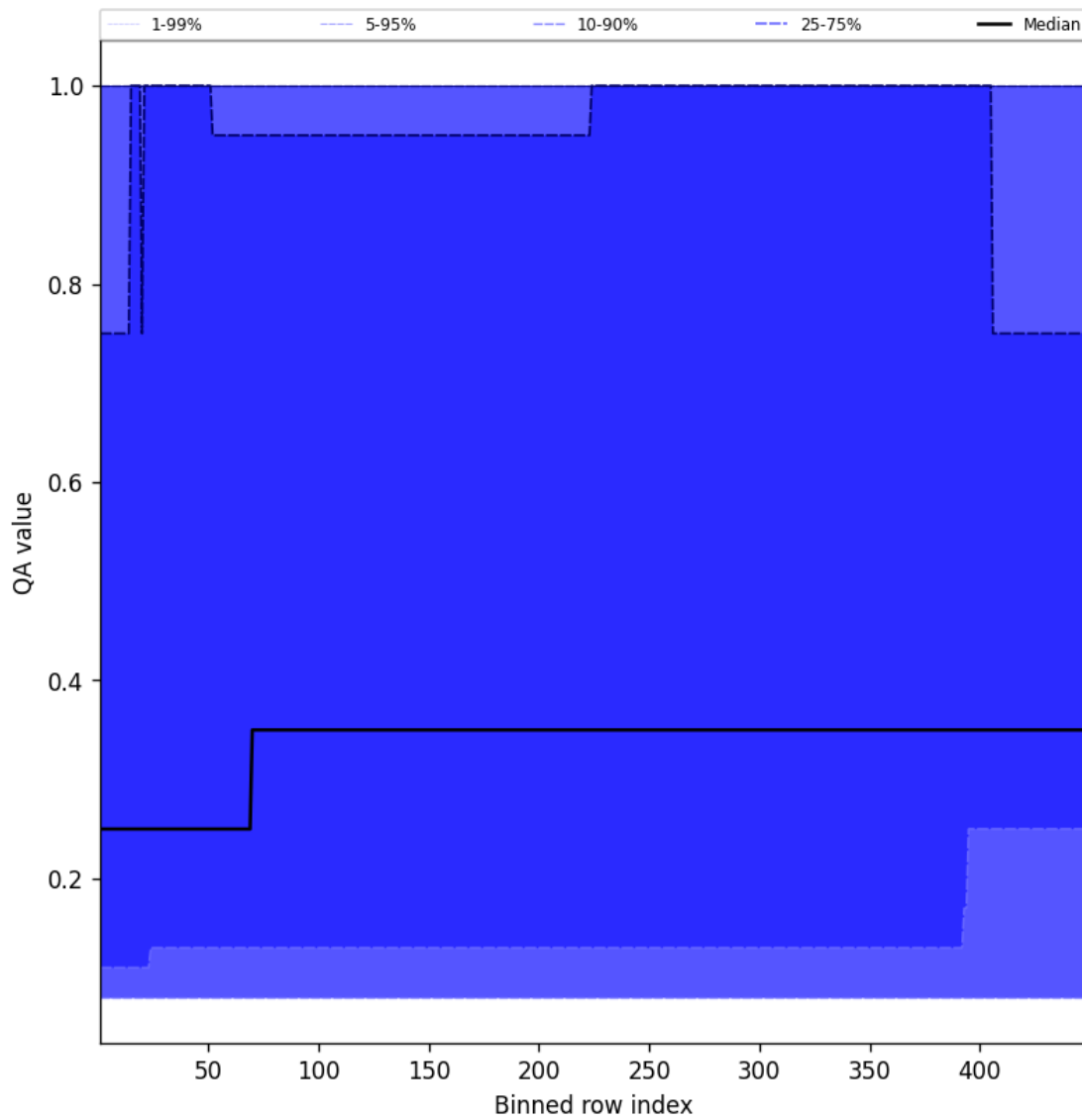
Figure 46: Along track statistics of “QA value” for 2025-10-27 to 2025-10-28
