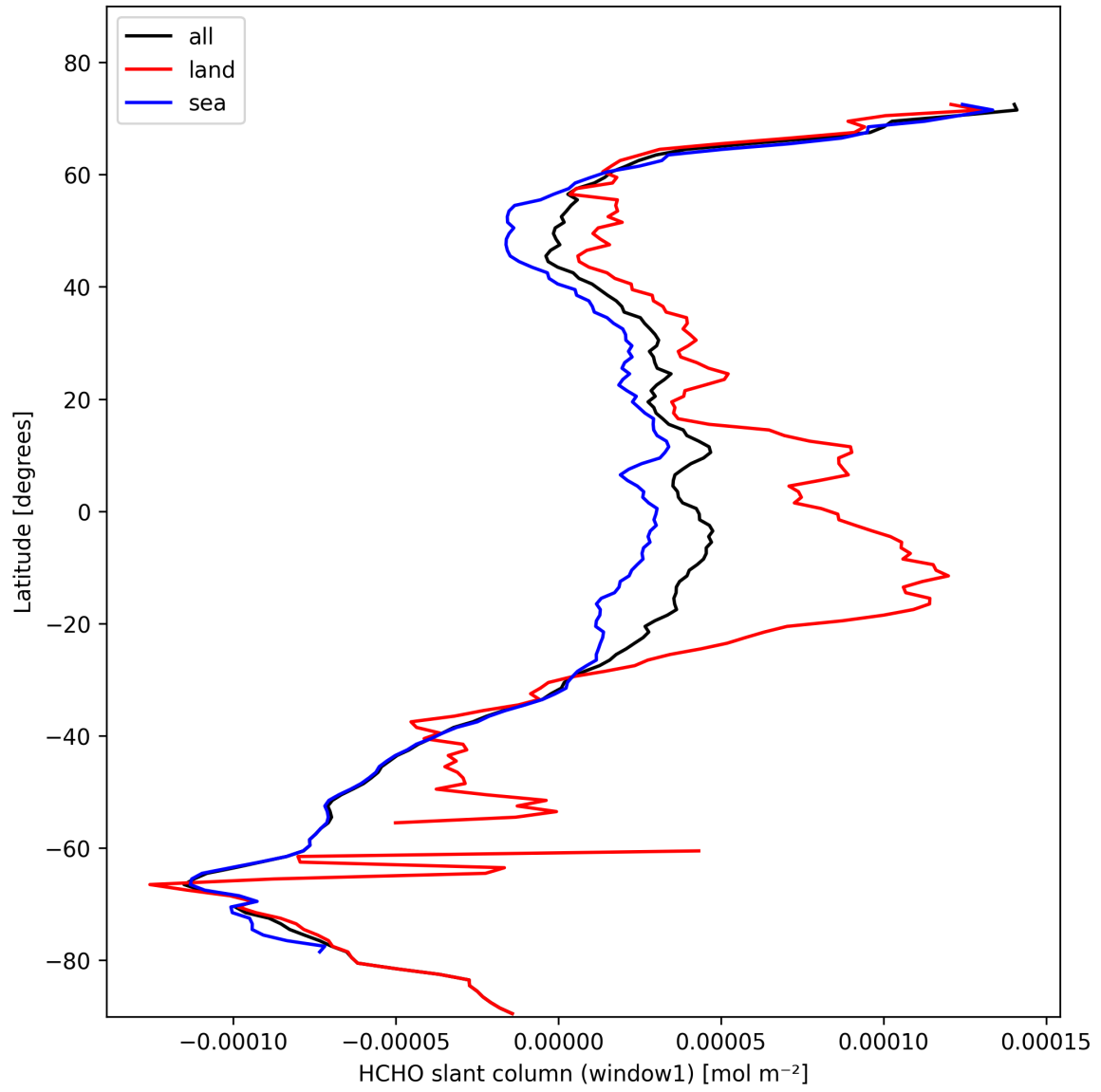
Figure 22: Zonal average of “HCHO slant column (window1)” for 2025-10-27 to 2025-10-28.
