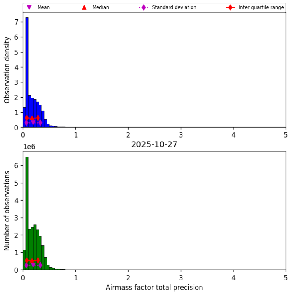
Figure 39: Histogram of “Airmass factor total precision” for 2025-10-27 to 2025-10-28
