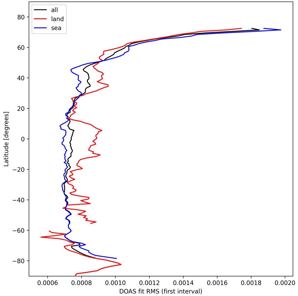
Figure 30: Zonal average of "DOAS fit RMS (first interval)" for 2025-10-27 to 2025-10-28.
