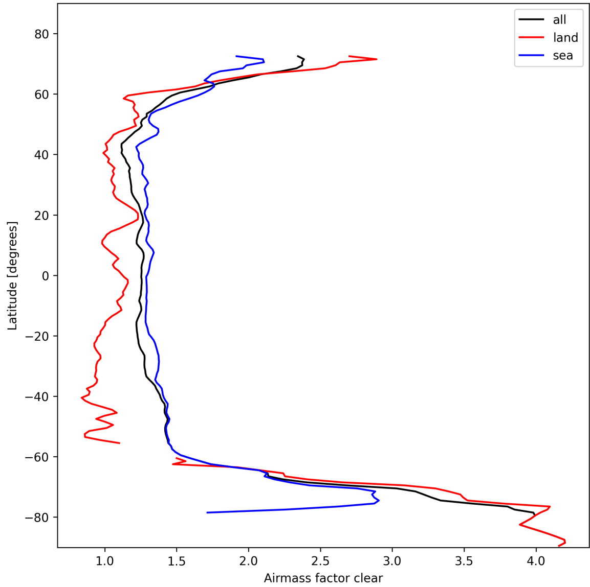
Figure 26: Zonal average of “Airmass factor clear” for 2025-10-27 to 2025-10-28.
