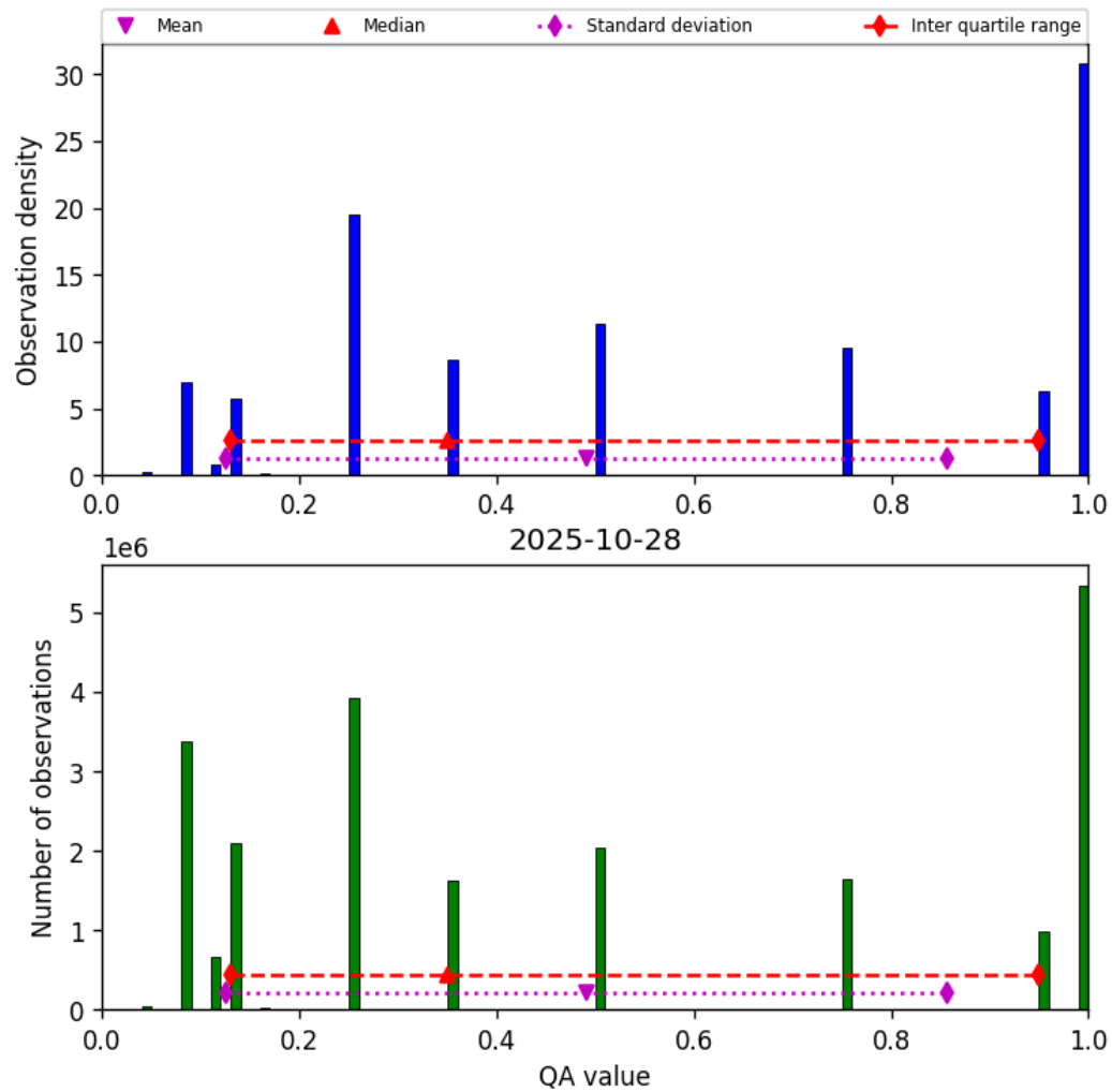
Figure 32: Histogram of “QA value” for 2025-10-28 to 2025-10-29
