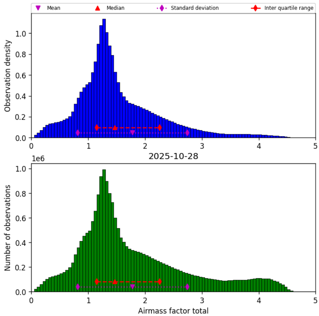
Figure 38: Histogram of “Airmass factor total” for 2025-10-28 to 2025-10-29
