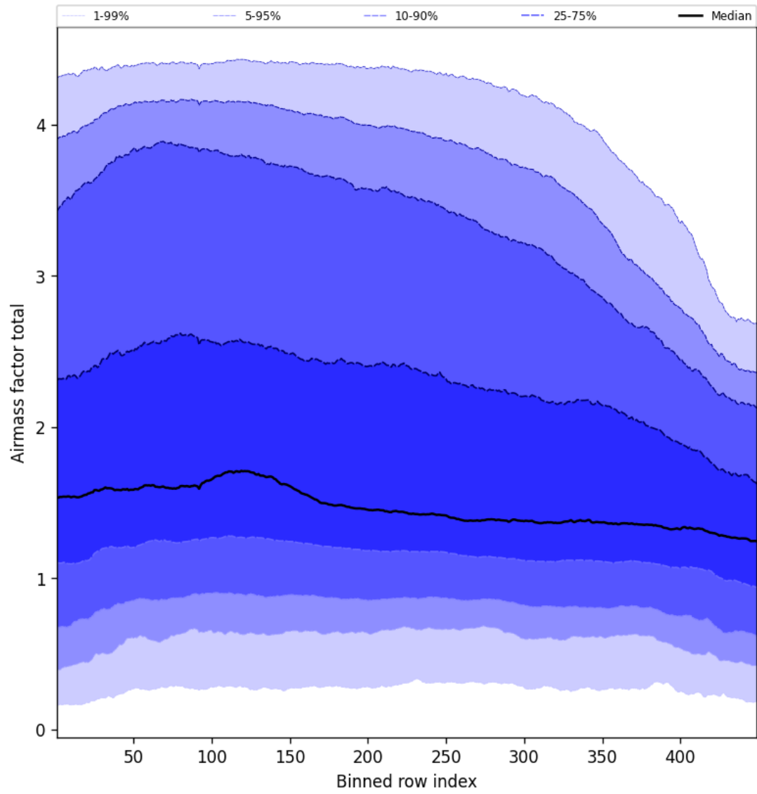
Figure 52: Along track statistics of “Airmass factor total” for 2025-10-28 to 2025-10-29
