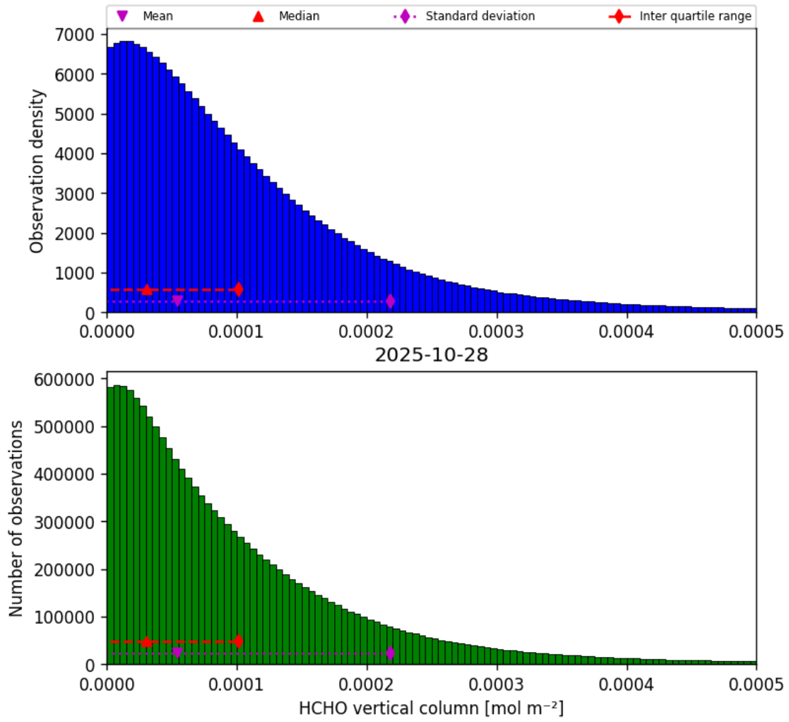
Figure 33: Histogram of “HCHO vertical column” for 2025-10-28 to 2025-10-29
