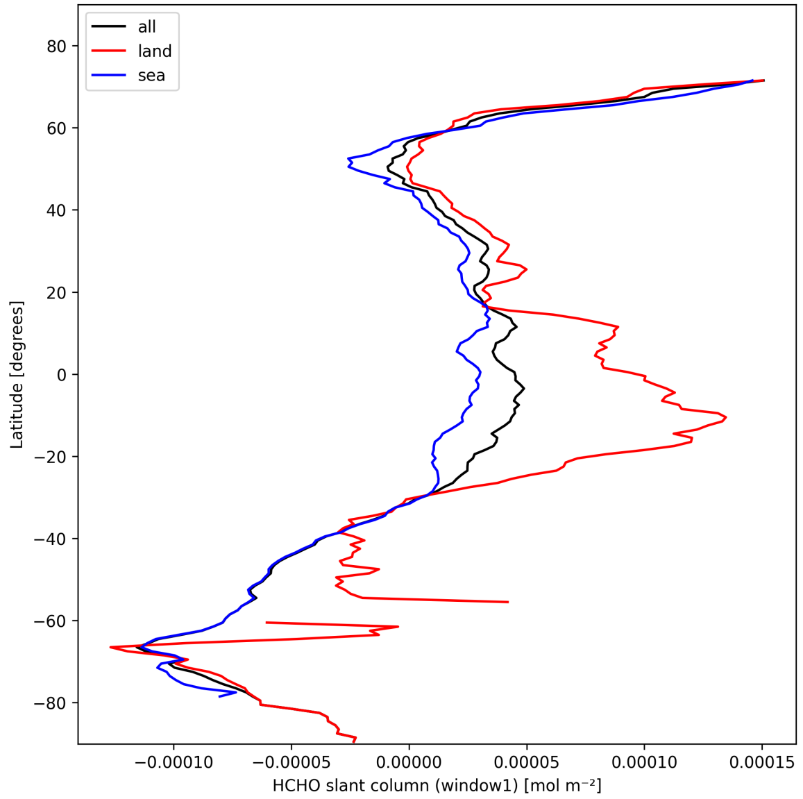
Figure 22: Zonal average of “HCHO slant column (window1)” for 2025-10-28 to 2025-10-29.
