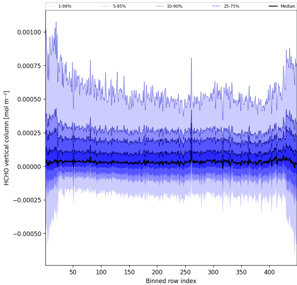
Figure 47: Along track statistics of “HCHO vertical column” for 2025-10-28 to 2025-10-29
