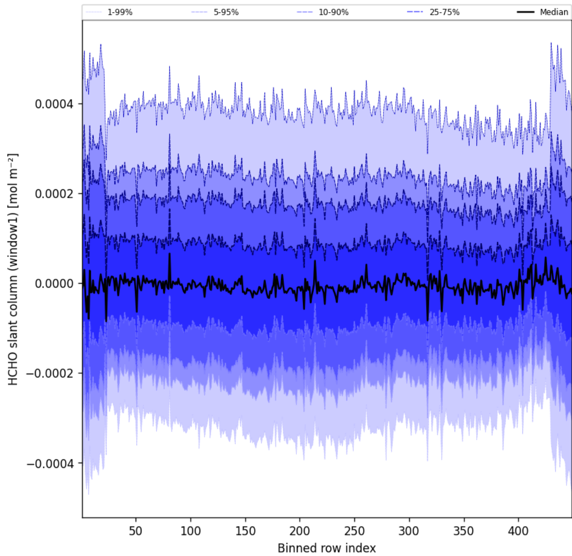
Figure 50: Along track statistics of “HCHO slant column (window1)” for 2025-10-28 to 2025-10-29
