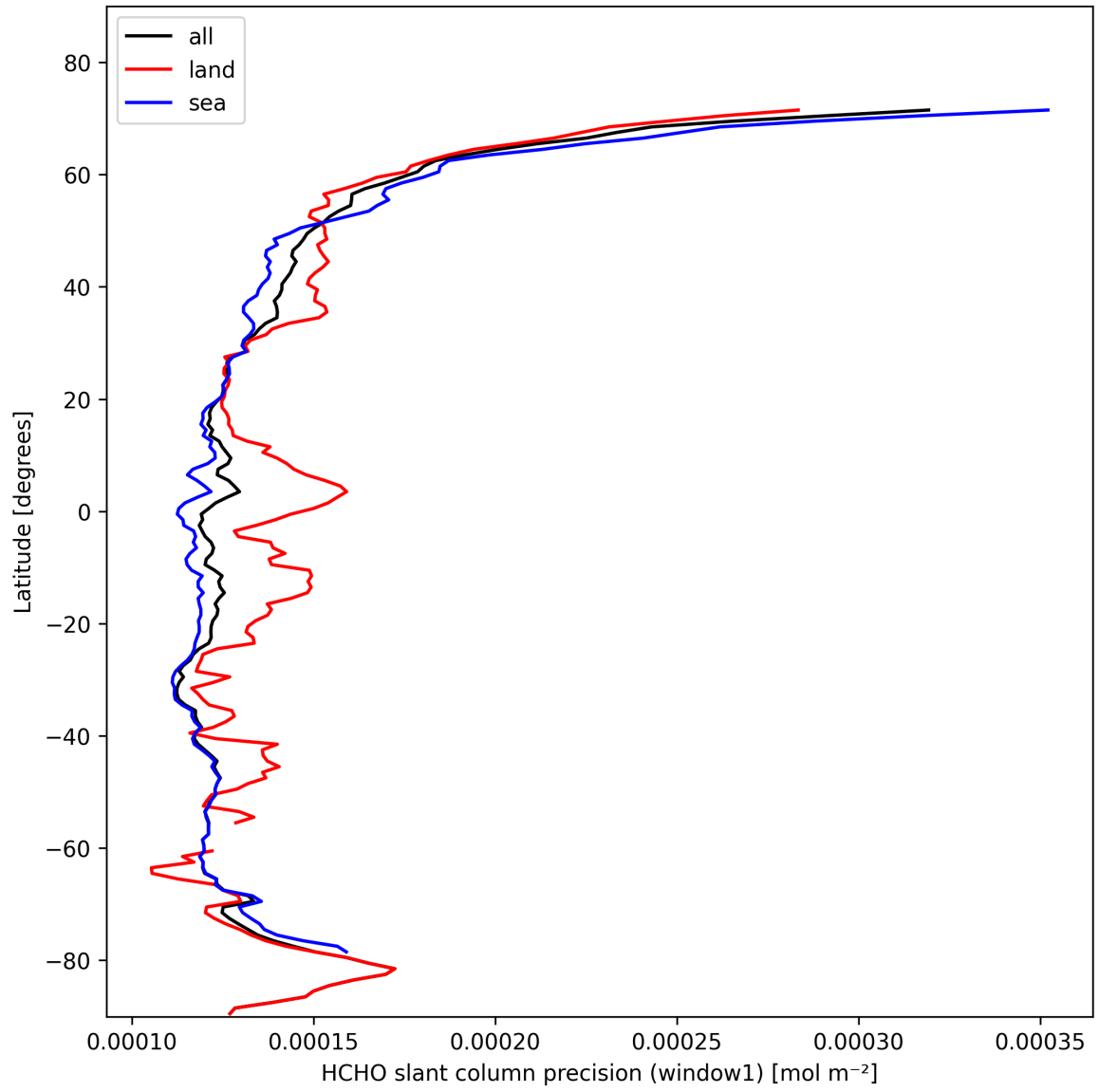
Figure 23: Zonal average of “HCHO slant column precision (window1)” for 2025-10-28 to 2025-10-29.
