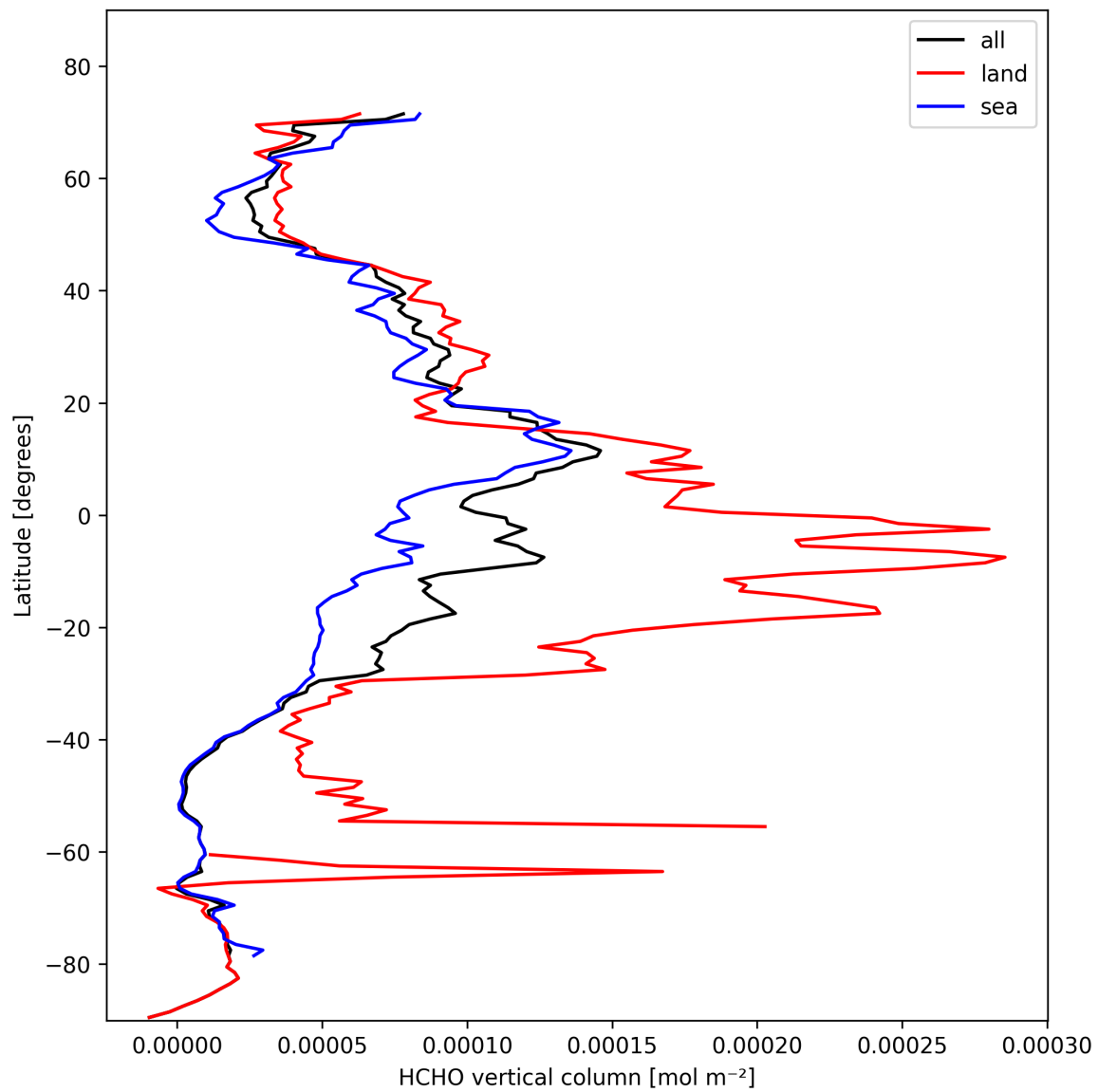
Figure 19: Zonal average of “HCHO vertical column” for 2025-10-28 to 2025-10-29.
