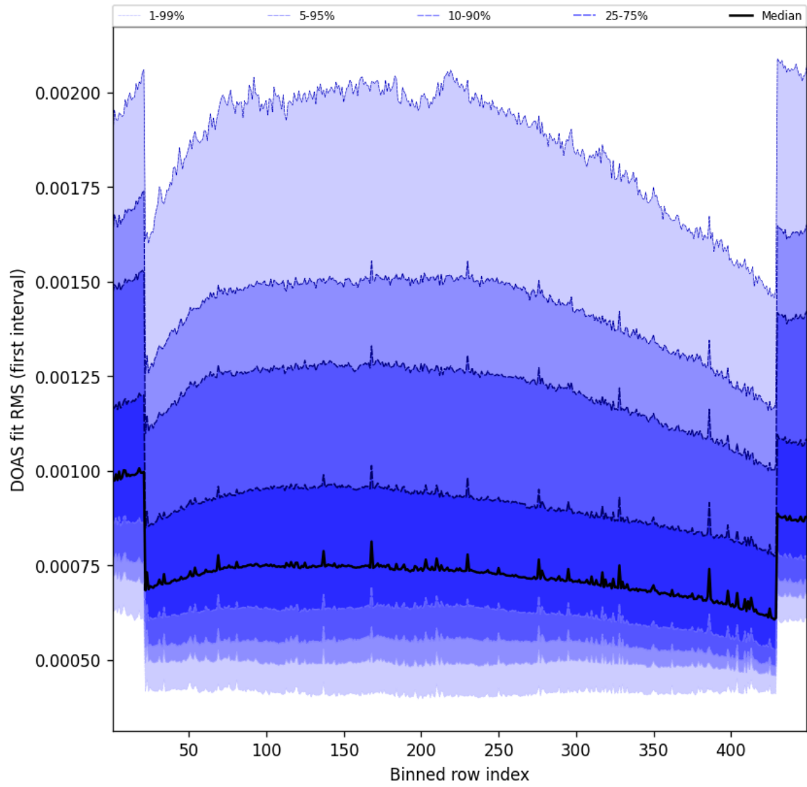
Figure 58: Along track statistics of “DOAS fit RMS (first interval)” for 2025-10-28 to 2025-10-29
