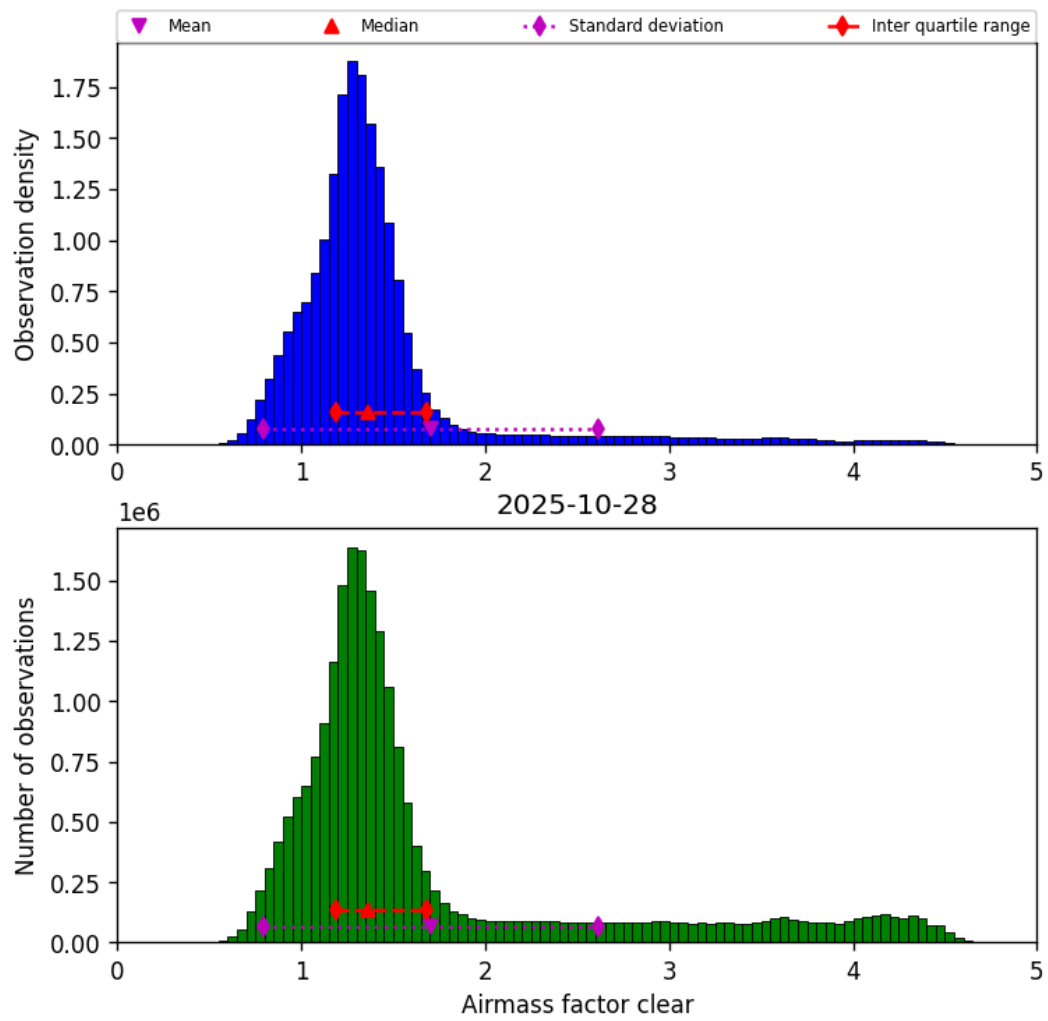
Figure 40: Histogram of “Airmass factor clear” for 2025-10-28 to 2025-10-29
