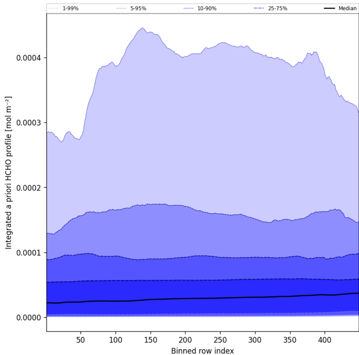
Figure 55: Along track statistics of “Integrated a priori HCHO profile” for 2025-10-28 to 2025-10-29
