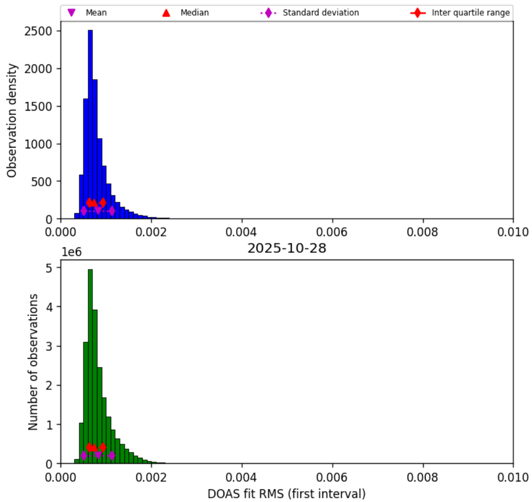
Figure 44: Histogram of “DOAS fit RMS (first interval)” for 2025-10-28 to 2025-10-29
