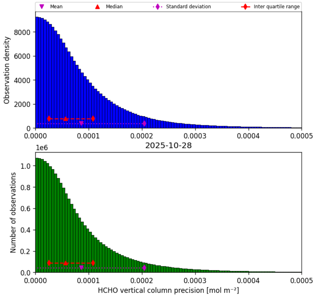
Figure 34: Histogram of “HCHO vertical column precision” for 2025-10-28 to 2025-10-29
