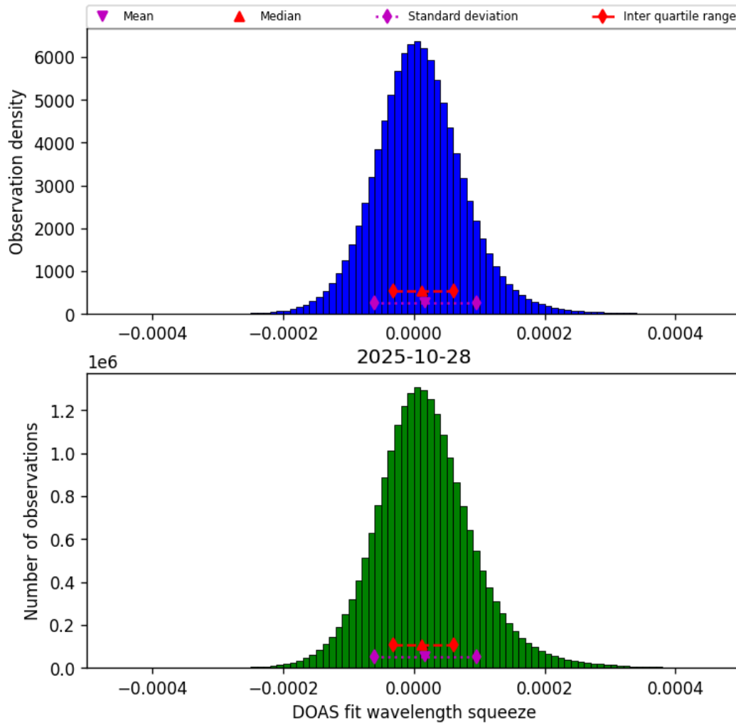
Figure 43: Histogram of “DOAS fit wavelength squeeze” for 2025-10-28 to 2025-10-29
