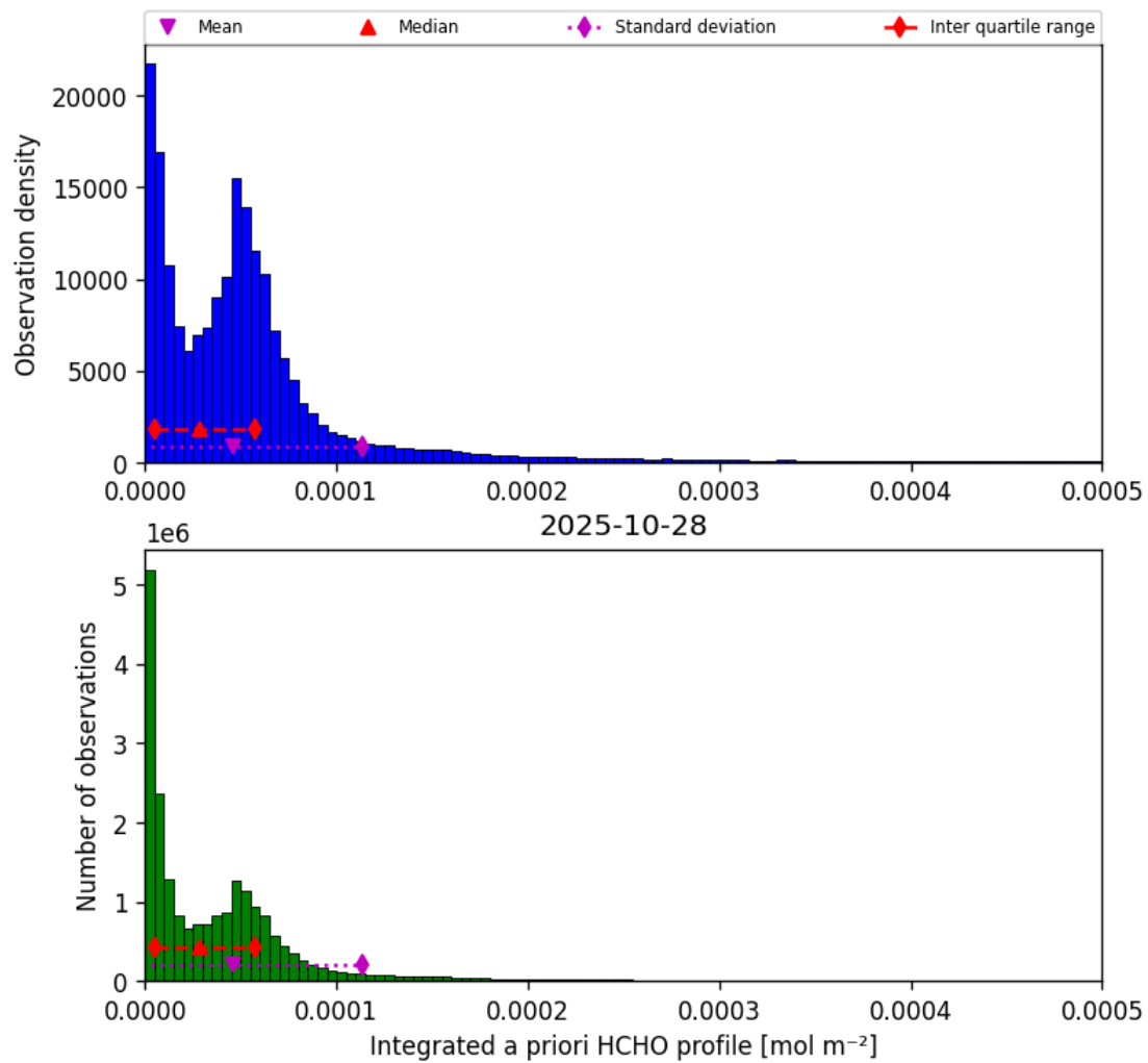
Figure 41: Histogram of “Integrated a priori HCHO profile” for 2025-10-28 to 2025-10-29
