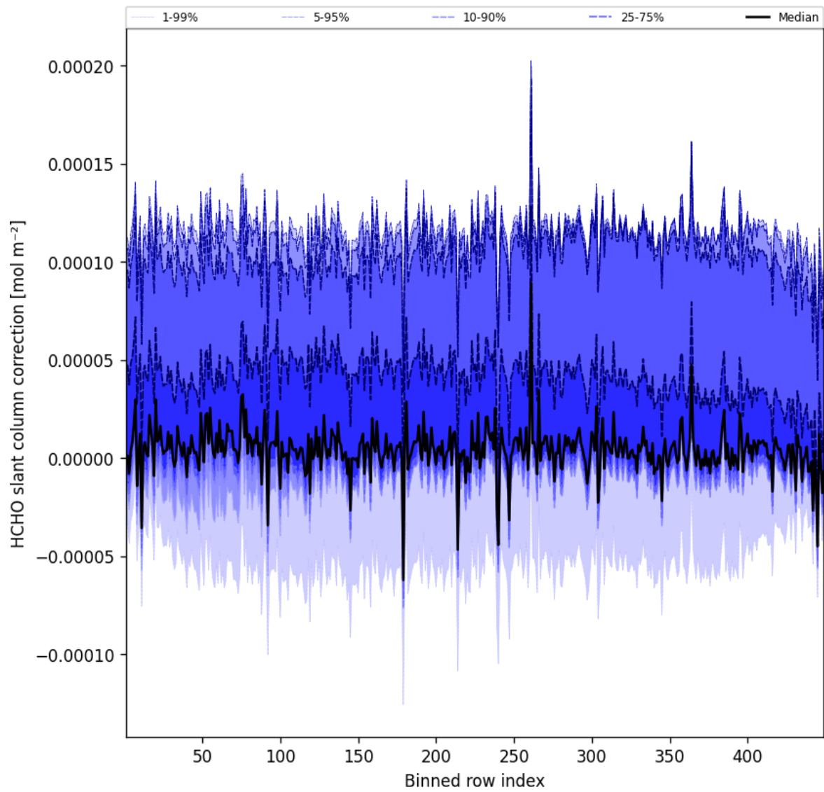
Figure 59: Along track statistics of “HCHO slant column correction” for 2025-10-28 to 2025-10-29
