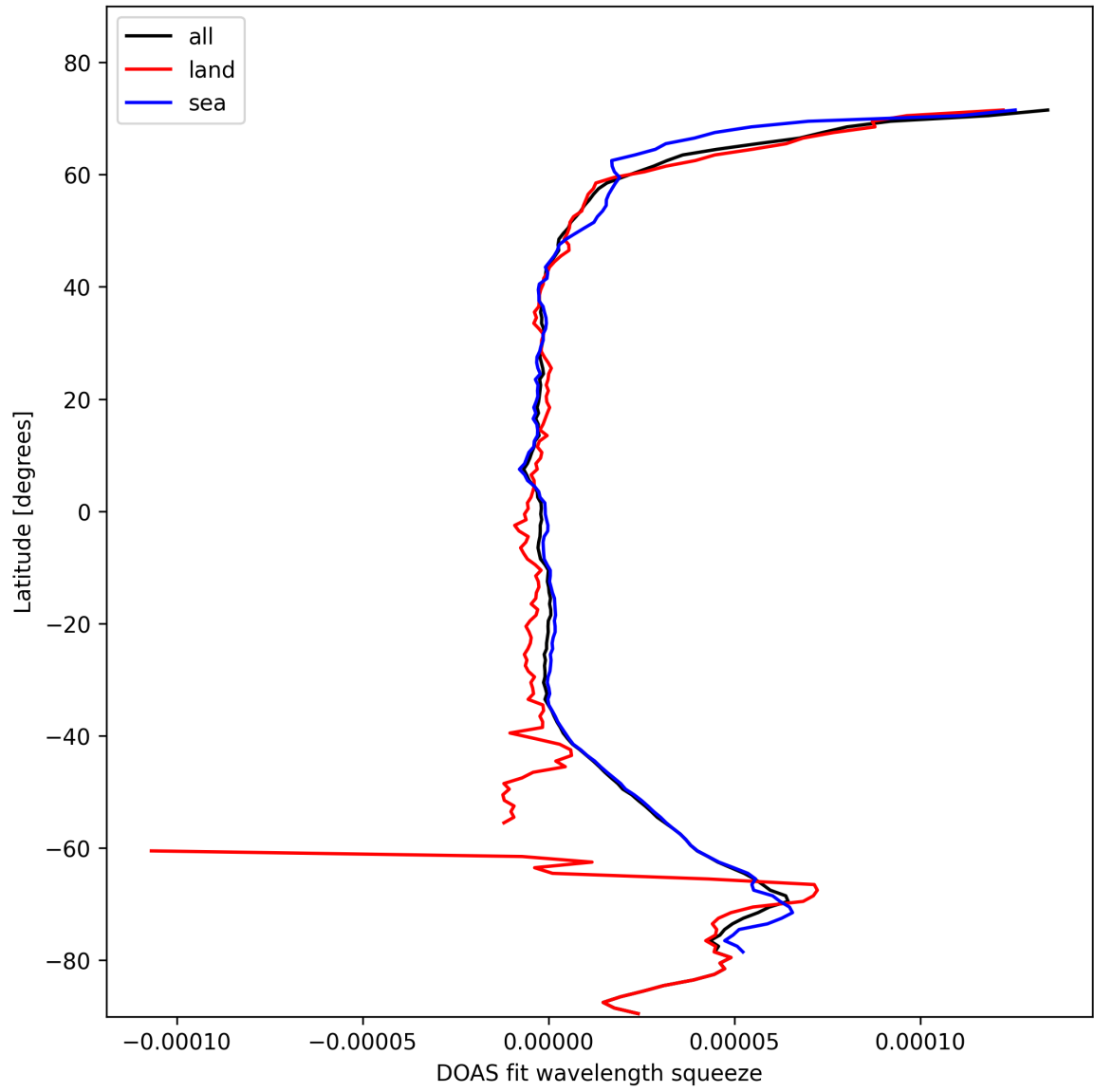
Figure 29: Zonal average of “DOAS fit wavelength squeeze” for 2025-10-28 to 2025-10-29.
