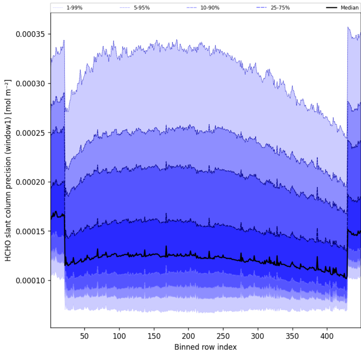
Figure 51: Along track statistics of “HCHO slant column precision (window1)” for 2025-10-28 to 2025-10-29
