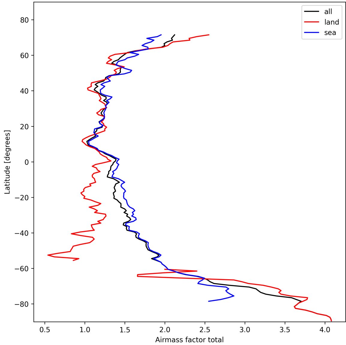
Figure 24: Zonal average of “Airmass factor total” for 2025-10-28 to 2025-10-29.
