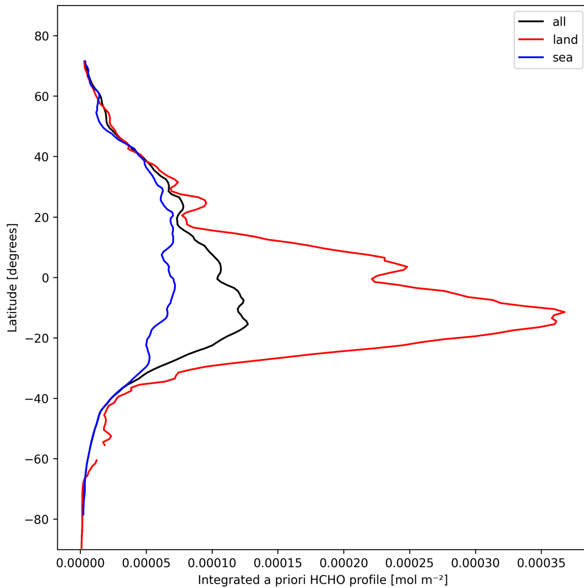
Figure 27: Zonal average of “Integrated a priori HCHO profile” for 2025-10-28 to 2025-10-29.
