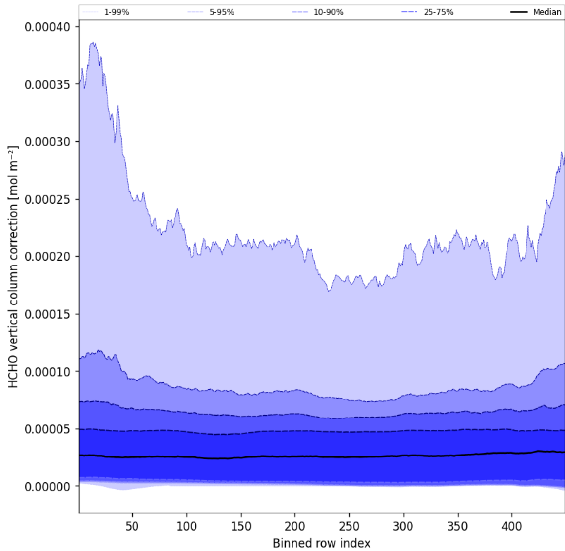
Figure 49: Along track statistics of “HCHO vertical column correction” for 2025-10-28 to 2025-10-29
