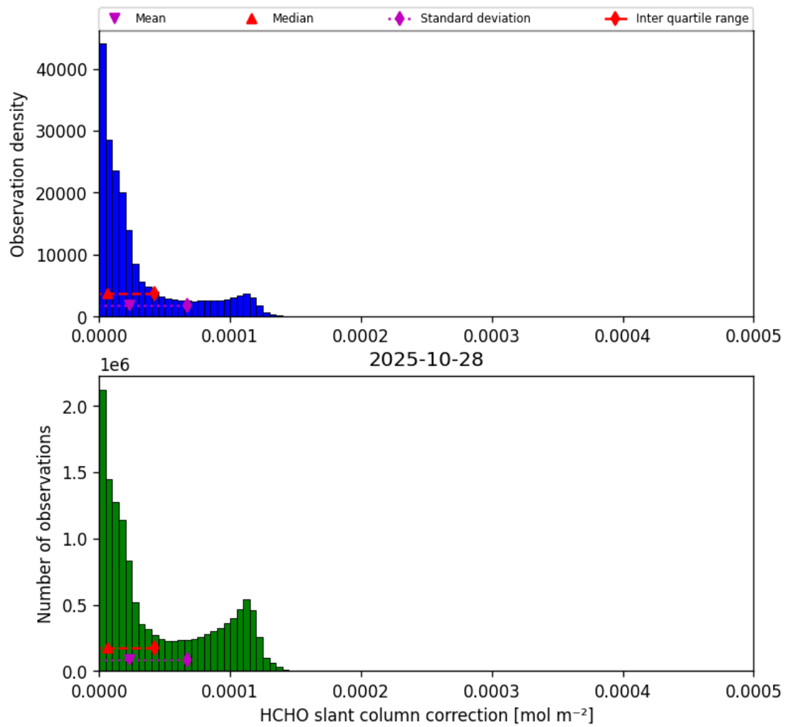
Figure 45: Histogram of “HCHO slant column correction” for 2025-10-28 to 2025-10-29
