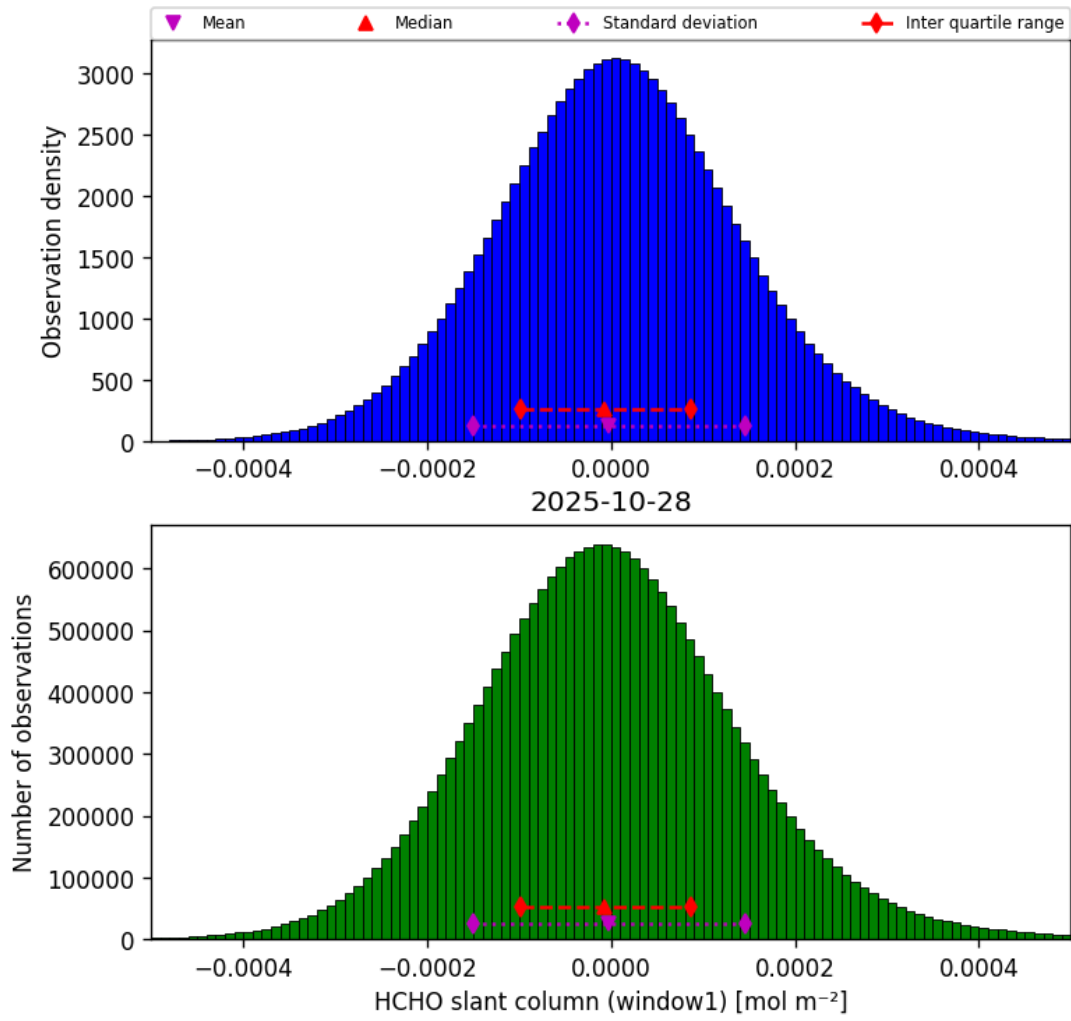
Figure 36: Histogram of “HCHO slant column (window1)” for 2025-10-28 to 2025-10-29
