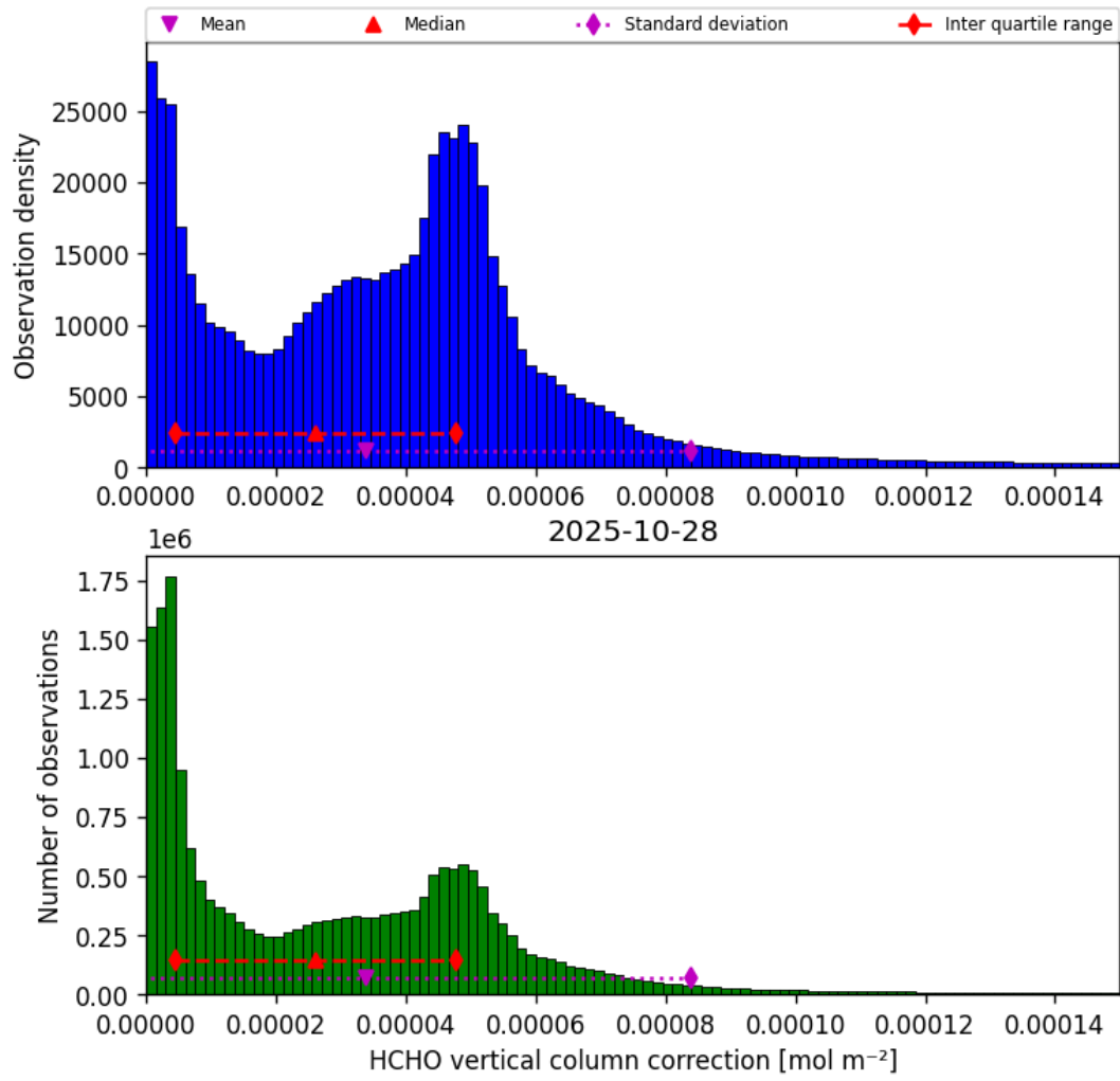
Figure 35: Histogram of “HCHO vertical column correction” for 2025-10-28 to 2025-10-29
