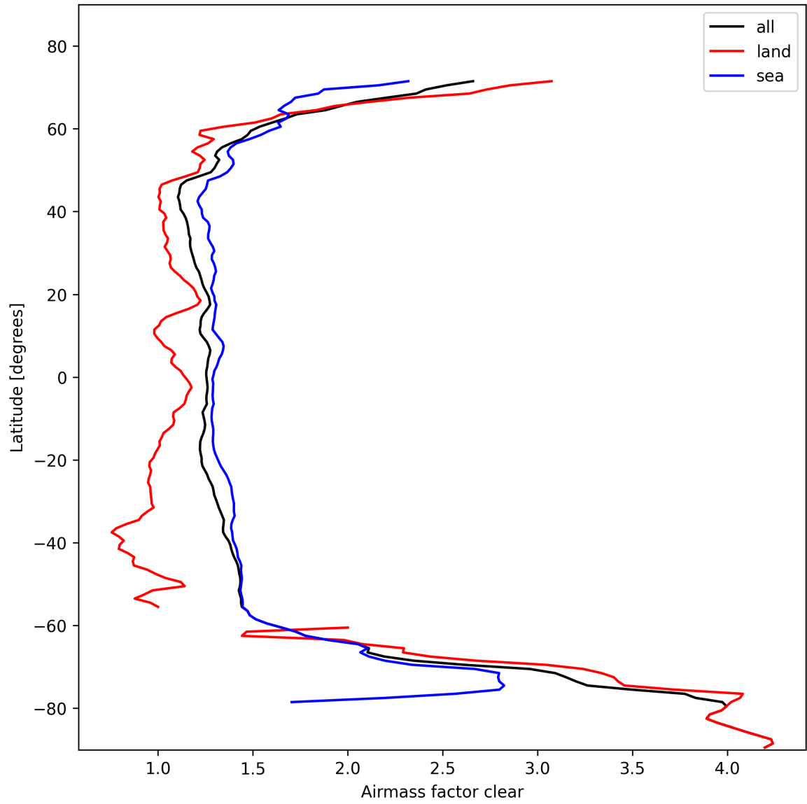
Figure 26: Zonal average of “Airmass factor clear” for 2025-10-28 to 2025-10-29.
