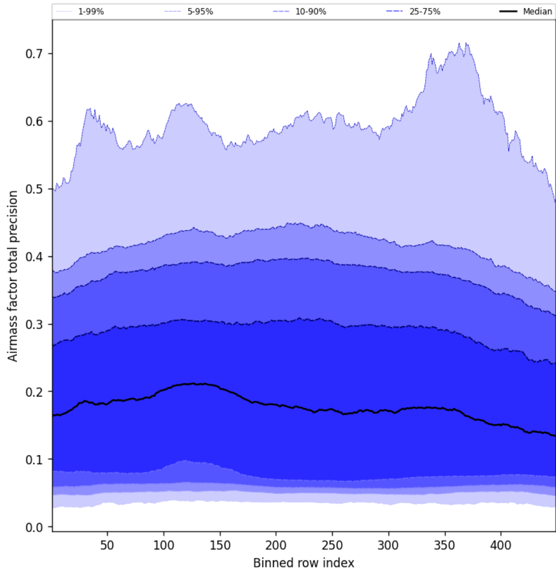
Figure 53: Along track statistics of “Airmass factor total precision” for 2025-10-28 to 2025-10-29
