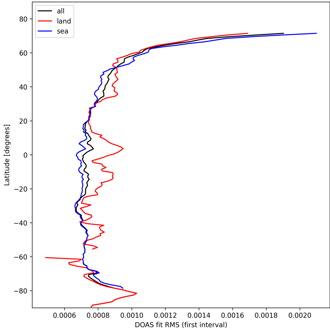
Figure 30: Zonal average of “DOAS fit RMS (first interval)” for 2025-10-28 to 2025-10-29.
