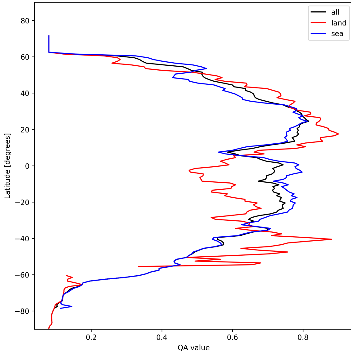
Figure 18: Zonal average of “QA value” for 2025-10-28 to 2025-10-29.
