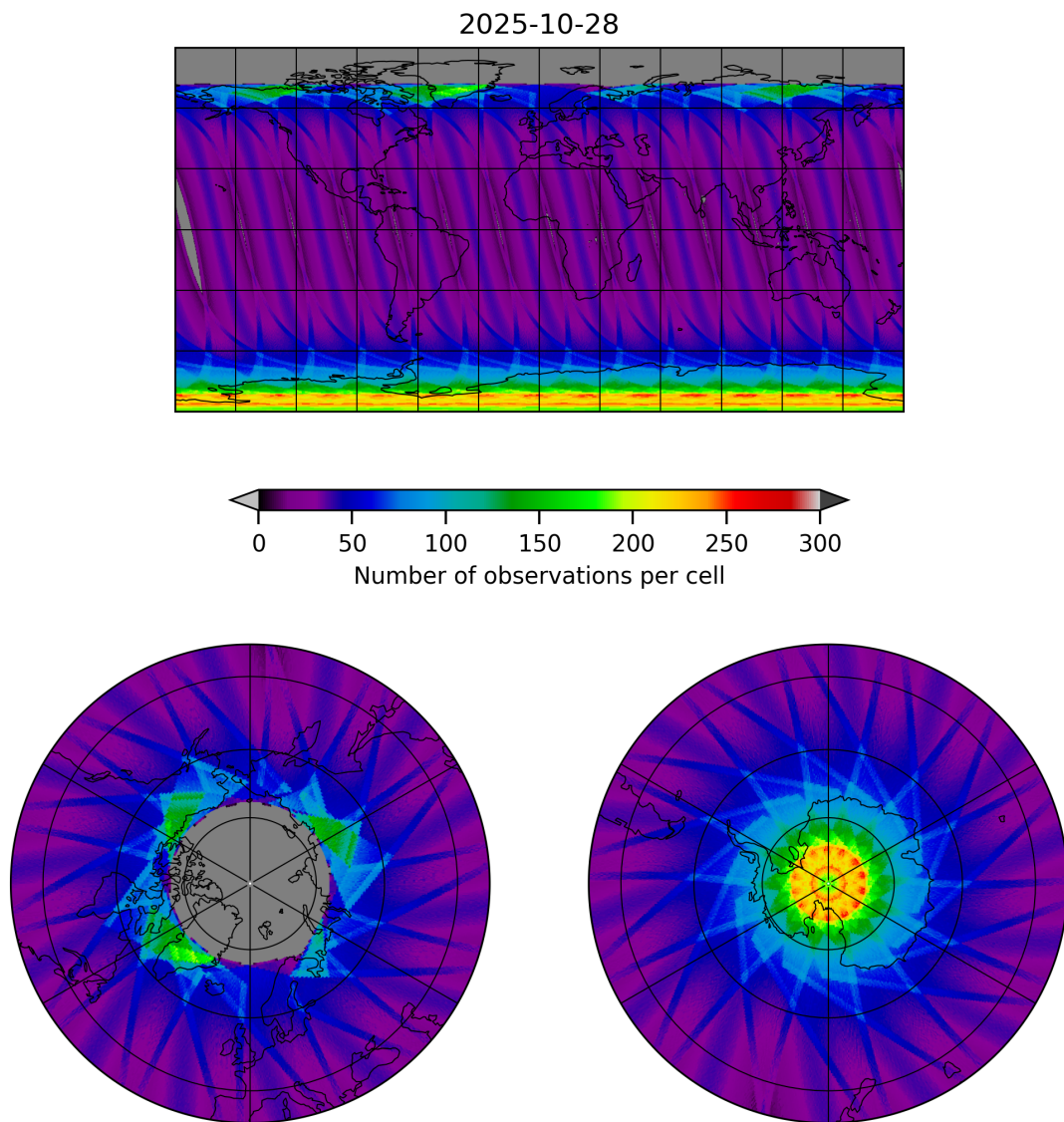
Figure 17: Map of the number of observations for 2025-10-28 to 2025-10-29
