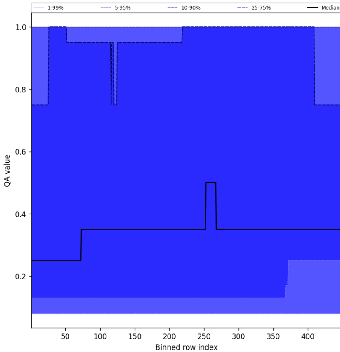
Figure 46: Along track statistics of “QA value” for 2025-10-28 to 2025-10-29
