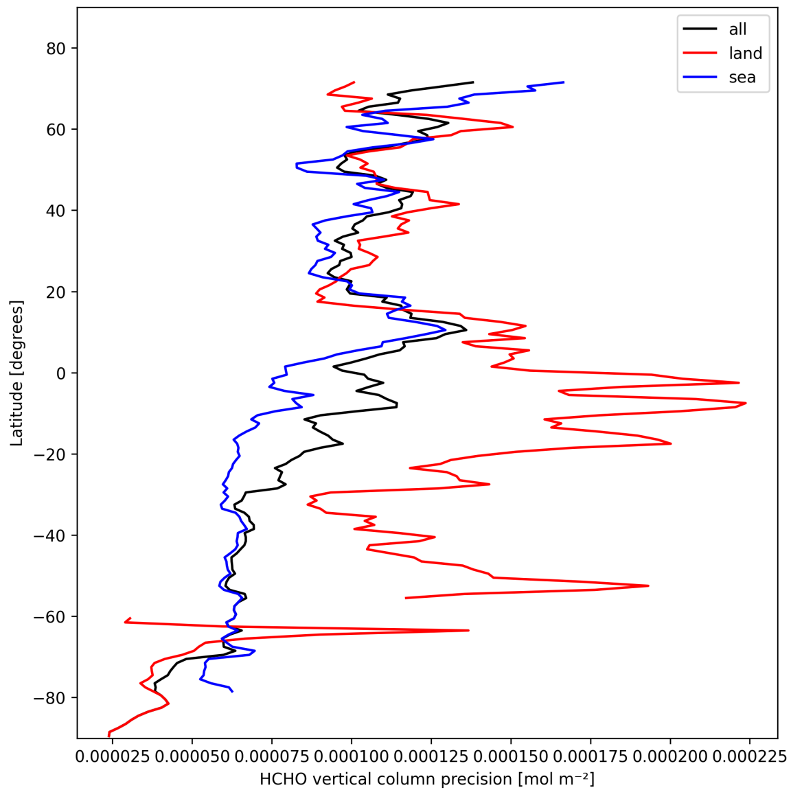
Figure 20: Zonal average of “HCHO vertical column precision” for 2025-10-28 to 2025-10-29.
