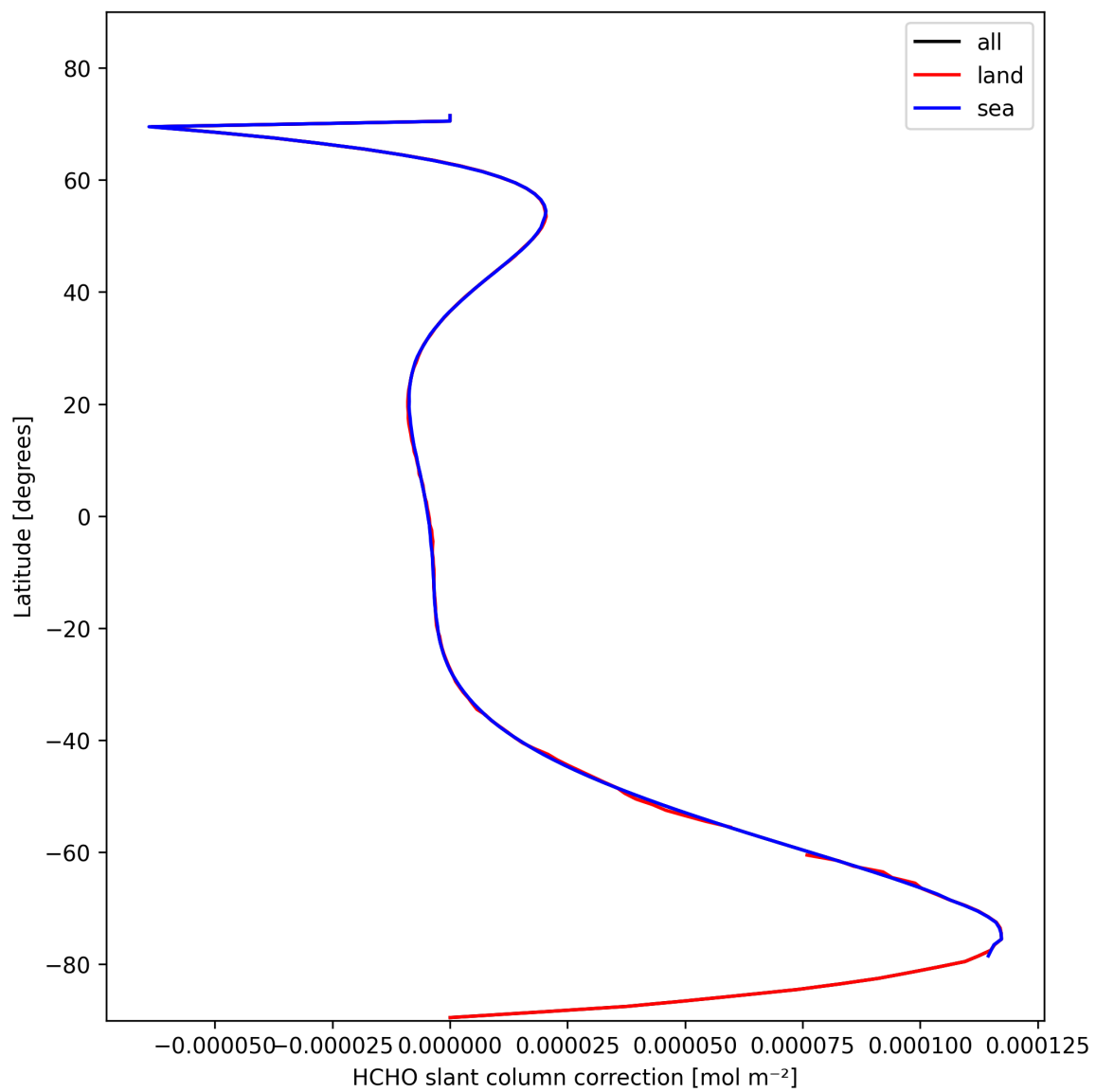
Figure 31: Zonal average of “HCHO slant column correction” for 2025-10-28 to 2025-10-29.
