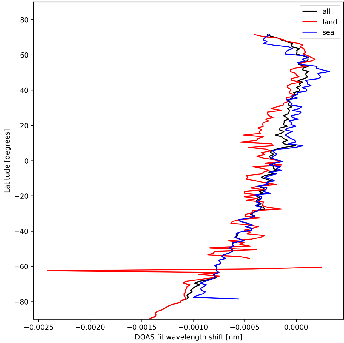
Figure 28: Zonal average of “DOAS fit wavelength shift” for 2025-10-28 to 2025-10-29.
