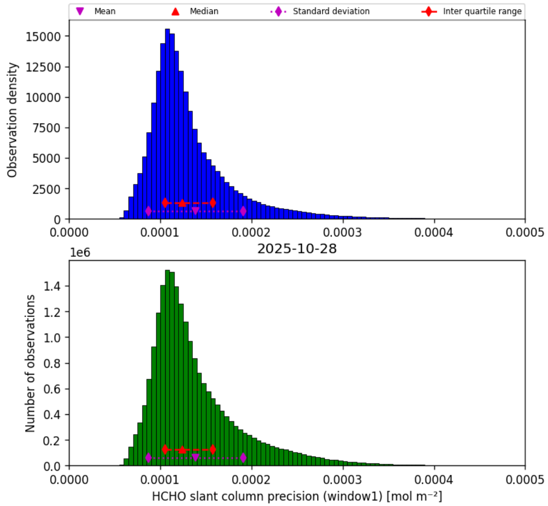
Figure 37: Histogram of “HCHO slant column precision (window1)” for 2025-10-28 to 2025-10-29
