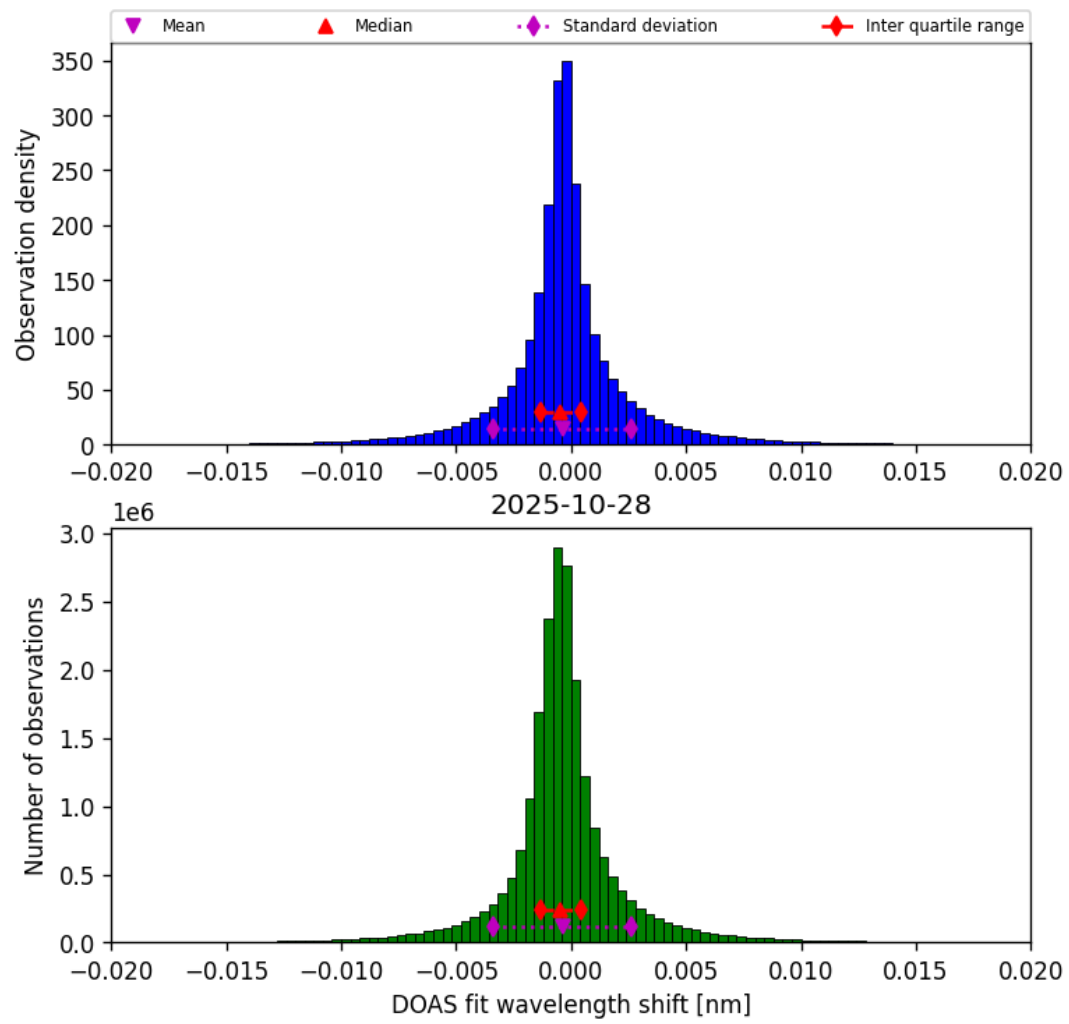
Figure 42: Histogram of “DOAS fit wavelength shift” for 2025-10-28 to 2025-10-29
