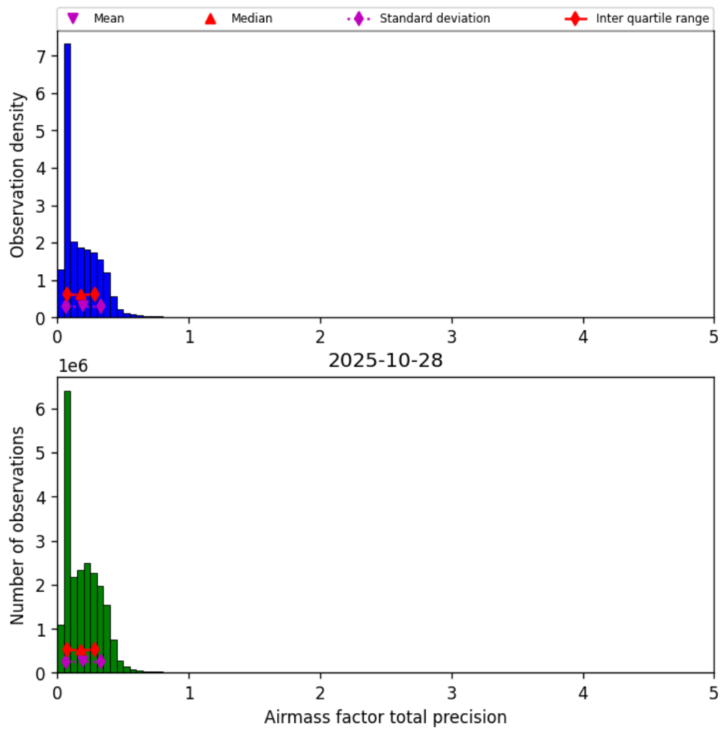
Figure 39: Histogram of “Airmass factor total precision” for 2025-10-28 to 2025-10-29
