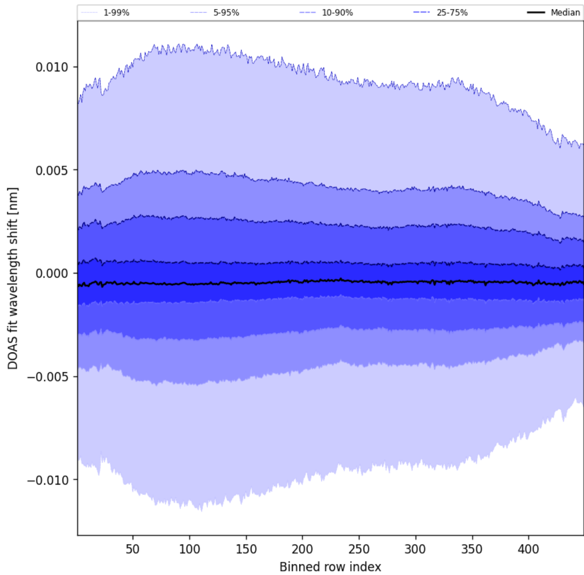
Figure 56: Along track statistics of “DOAS fit wavelength shift” for 2025-10-28 to 2025-10-29
