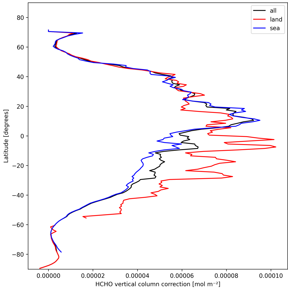
Figure 21: Zonal average of “HCHO vertical column correction” for 2025-10-28 to 2025-10-29.
