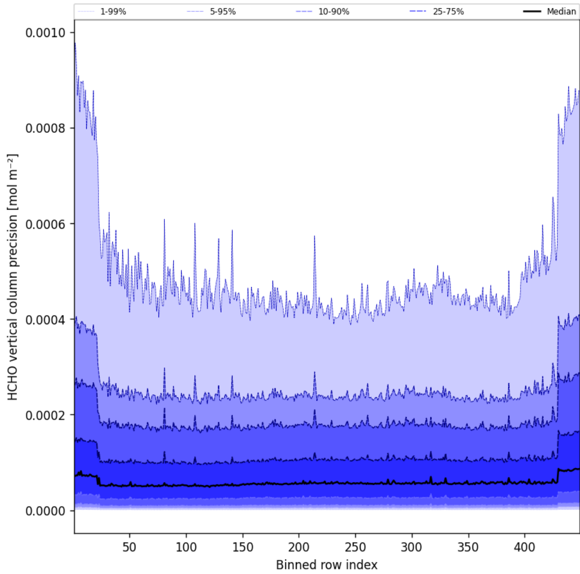
Figure 48: Along track statistics of “HCHO vertical column precision” for 2025-10-28 to 2025-10-29
