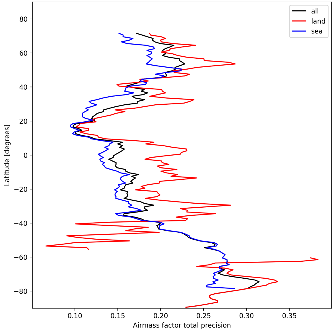
Figure 25: Zonal average of “Airmass factor total precision” for 2025-10-28 to 2025-10-29.
