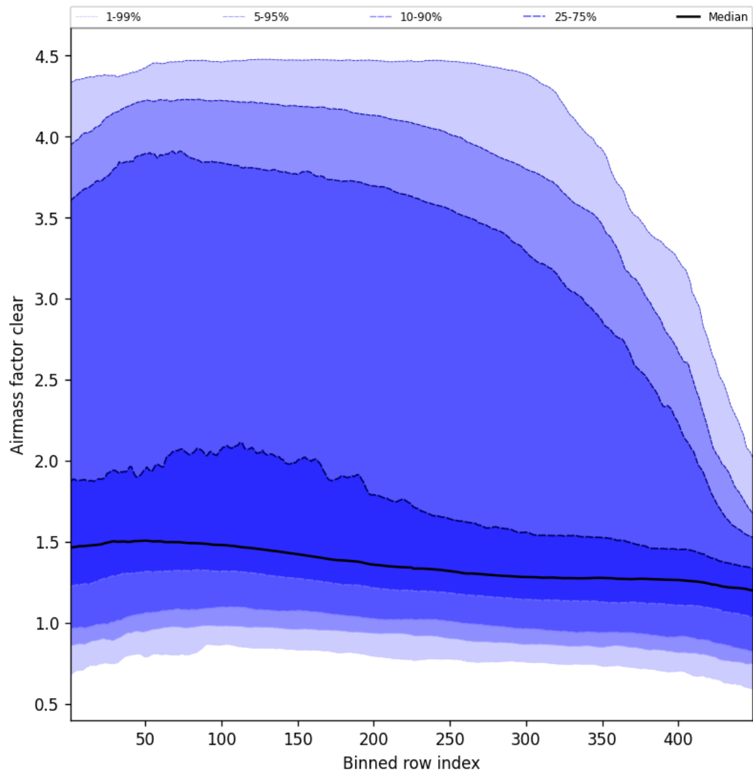
Figure 54: Along track statistics of “Airmass factor clear” for 2025-10-28 to 2025-10-29
