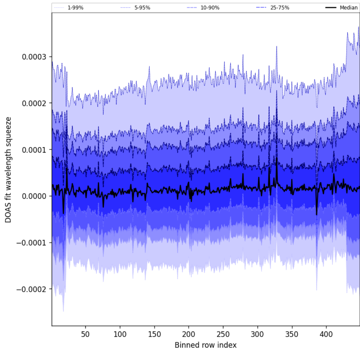
Figure 57: Along track statistics of “DOAS fit wavelength squeeze” for 2025-10-28 to 2025-10-29
