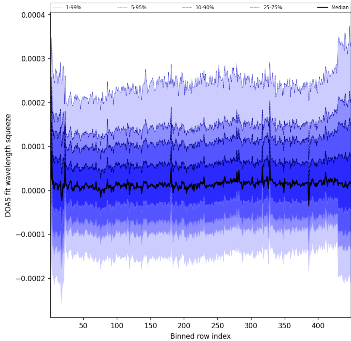
Figure 57: Along track statistics of “DOAS fit wavelength squeeze” for 2025-10-29 to 2025-10-30
