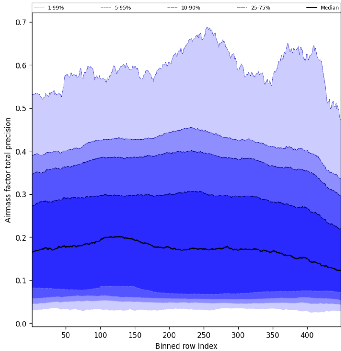
Figure 53: Along track statistics of “Airmass factor total precision” for 2025-10-29 to 2025-10-30
