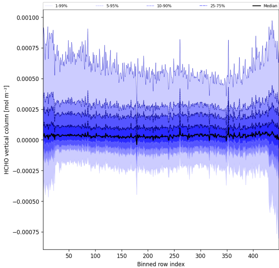
Figure 47: Along track statistics of “HCHO vertical column” for 2025-10-29 to 2025-10-30
