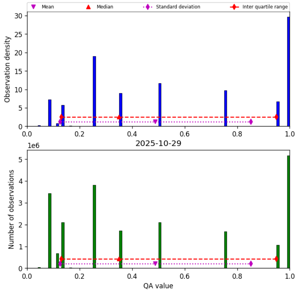
Figure 32: Histogram of “QA value” for 2025-10-29 to 2025-10-30
