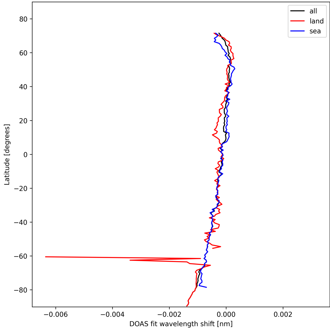
Figure 28: Zonal average of "DOAS fit wavelength shift" for 2025-10-29 to 2025-10-30.
