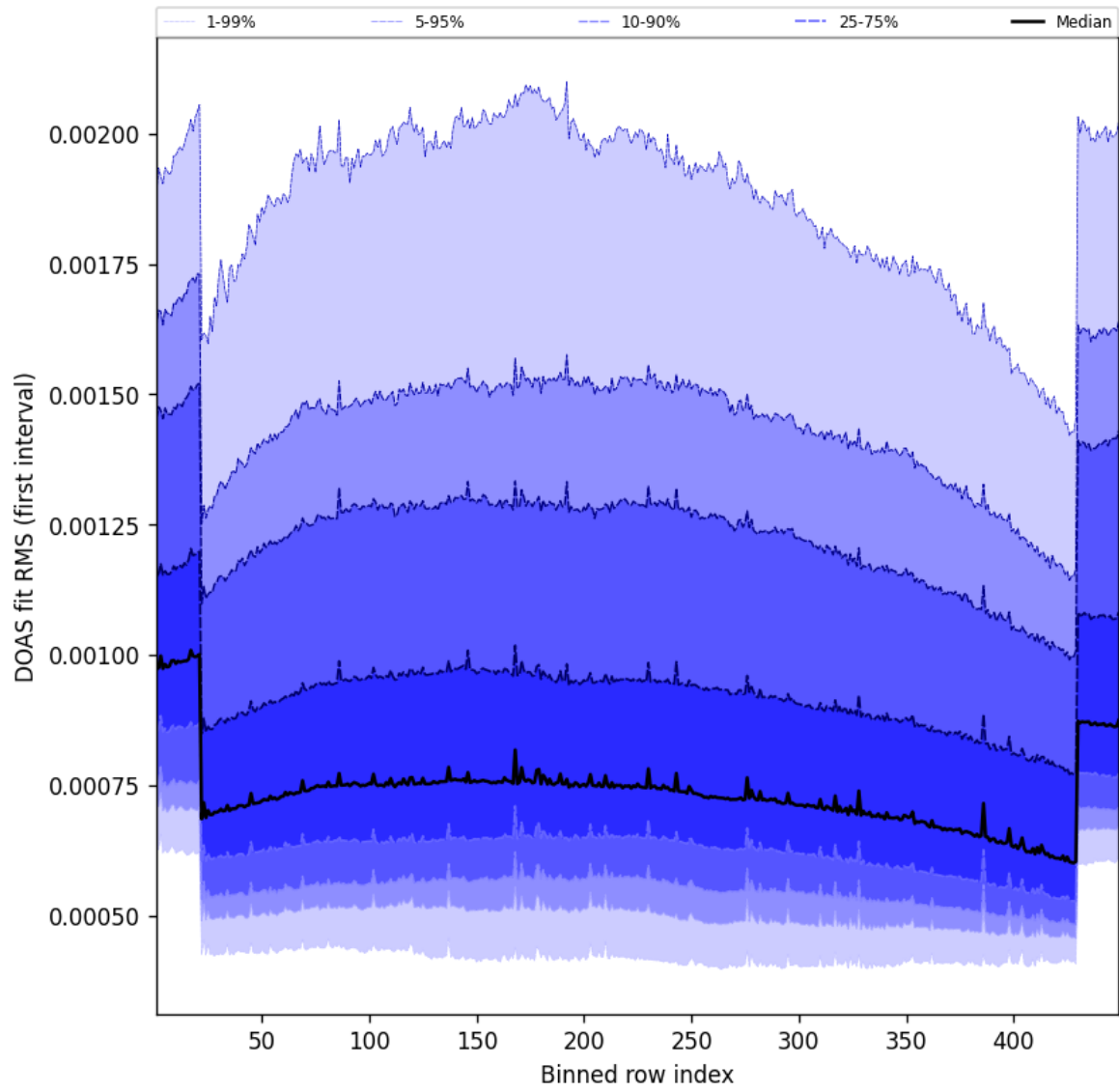
Figure 58: Along track statistics of “DOAS fit RMS (first interval)” for 2025-10-29 to 2025-10-30
