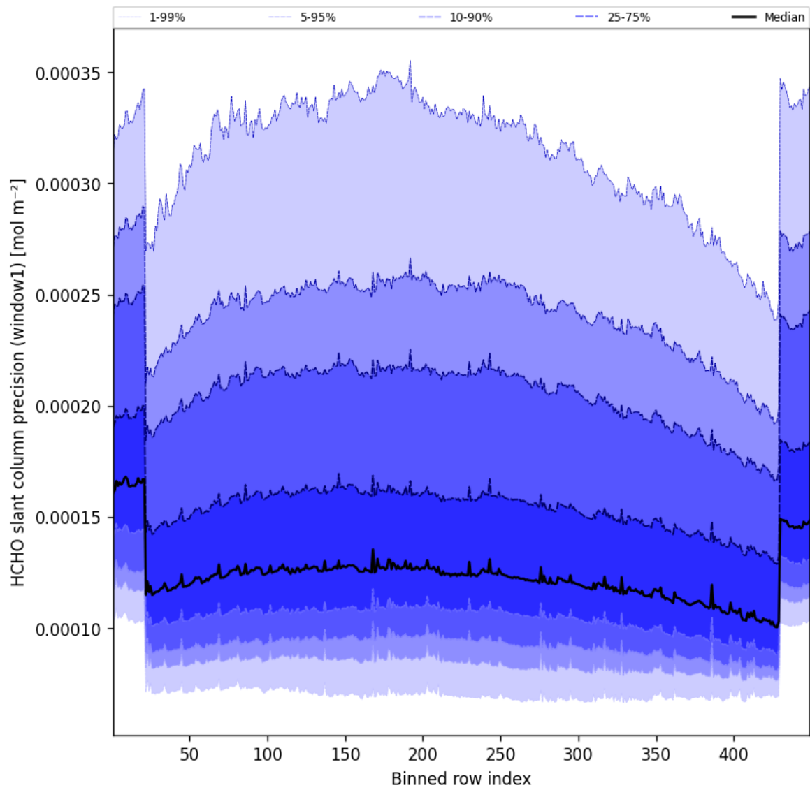
Figure 51: Along track statistics of “HCHO slant column precision (window1)” for 2025-10-29 to 2025-10-30
