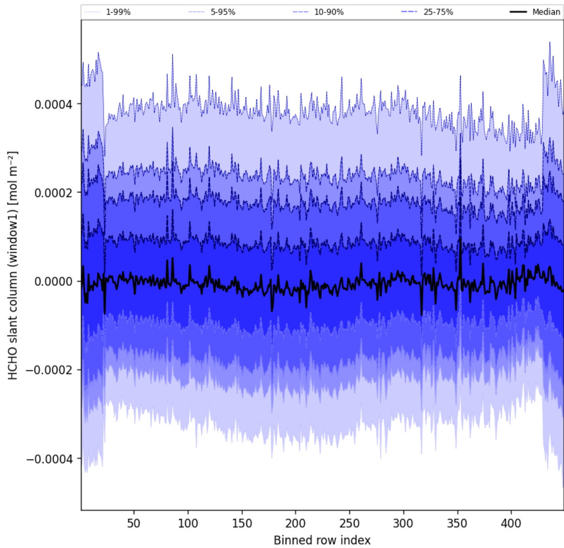
Figure 50: Along track statistics of “HCHO slant column (window1)” for 2025-10-29 to 2025-10-30
