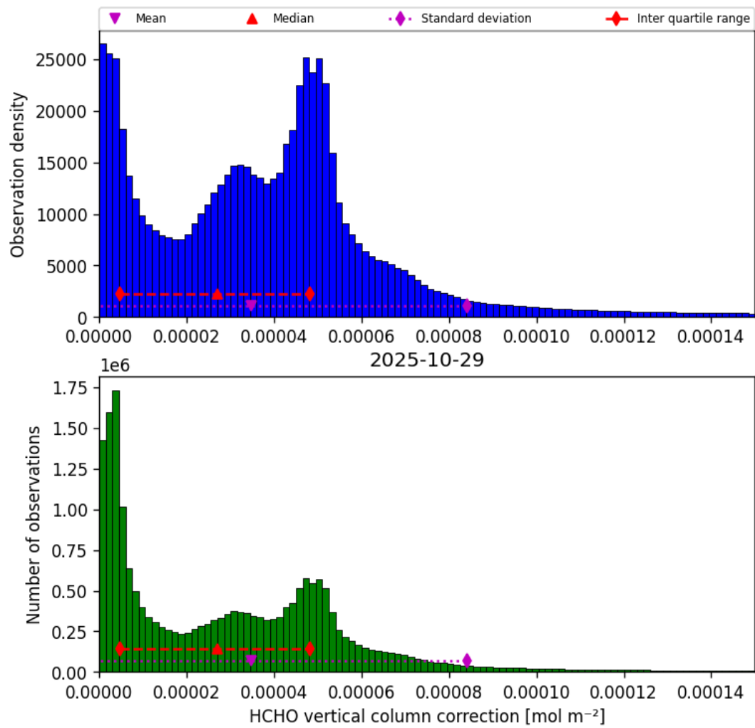
Figure 35: Histogram of “HCHO vertical column correction” for 2025-10-29 to 2025-10-30
