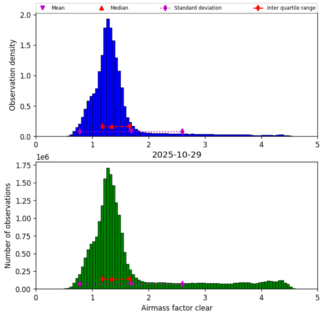
Figure 40: Histogram of “Airmass factor clear” for 2025-10-29 to 2025-10-30
