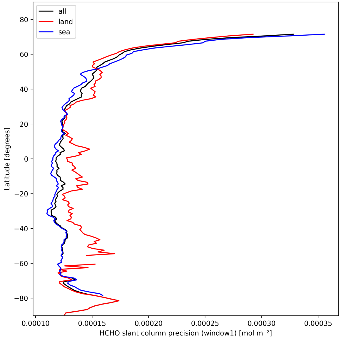
Figure 23: Zonal average of "HCHO slant column precision (window1)" for 2025-10-29 to 2025-10-30.
