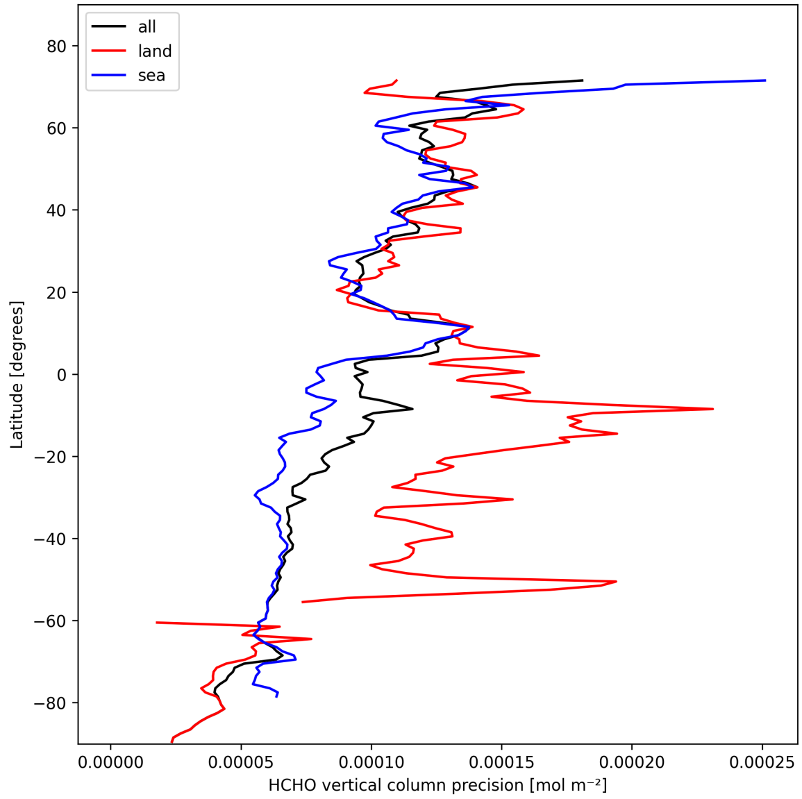
Figure 20: Zonal average of “HCHO vertical column precision” for 2025-10-29 to 2025-10-30.
