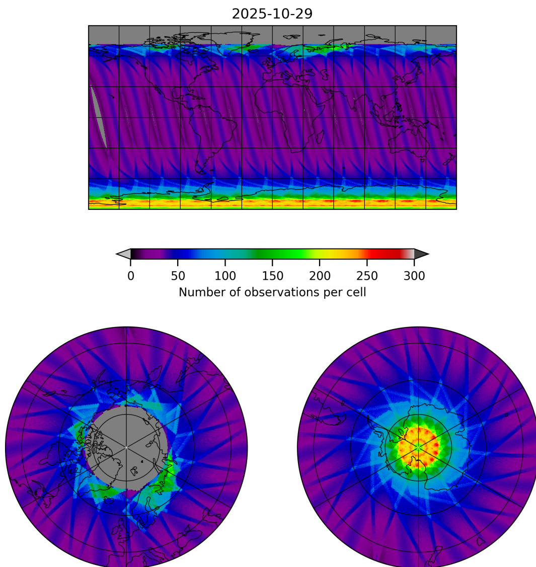
Figure 17: Map of the number of observations for 2025-10-29 to 2025-10-30
