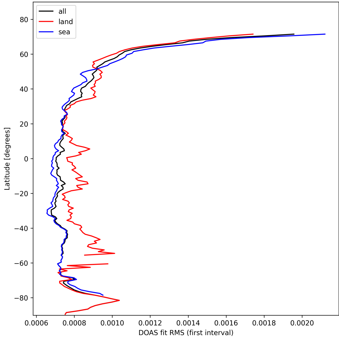
Figure 30: Zonal average of “DOAS fit RMS (first interval)” for 2025-10-29 to 2025-10-30.
