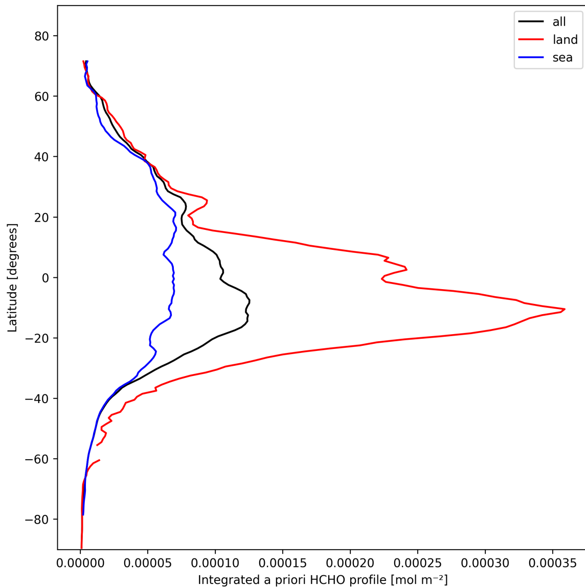
Figure 27: Zonal average of “Integrated a priori HCHO profile” for 2025-10-29 to 2025-10-30.
