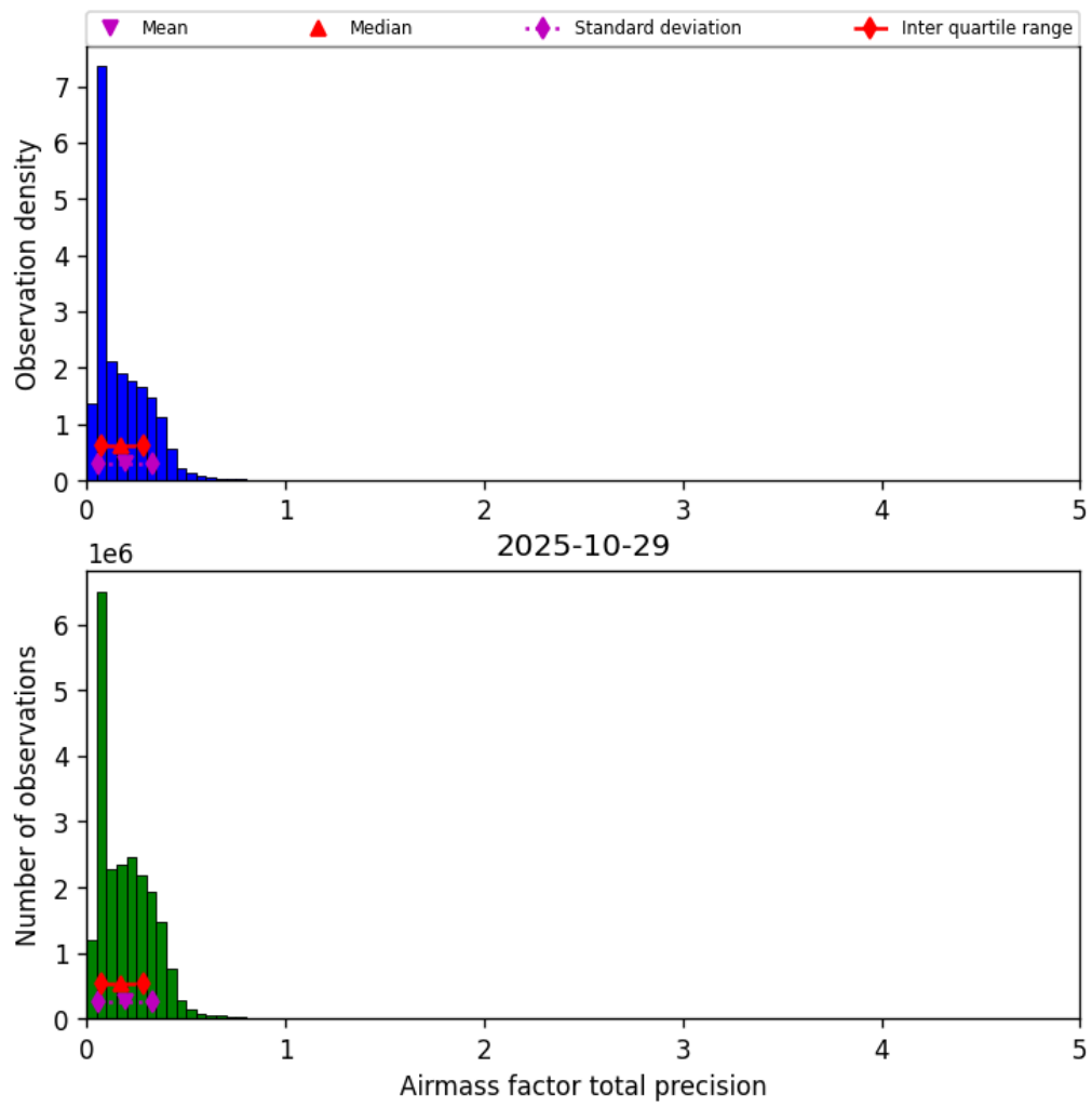
Figure 39: Histogram of “Airmass factor total precision” for 2025-10-29 to 2025-10-30
