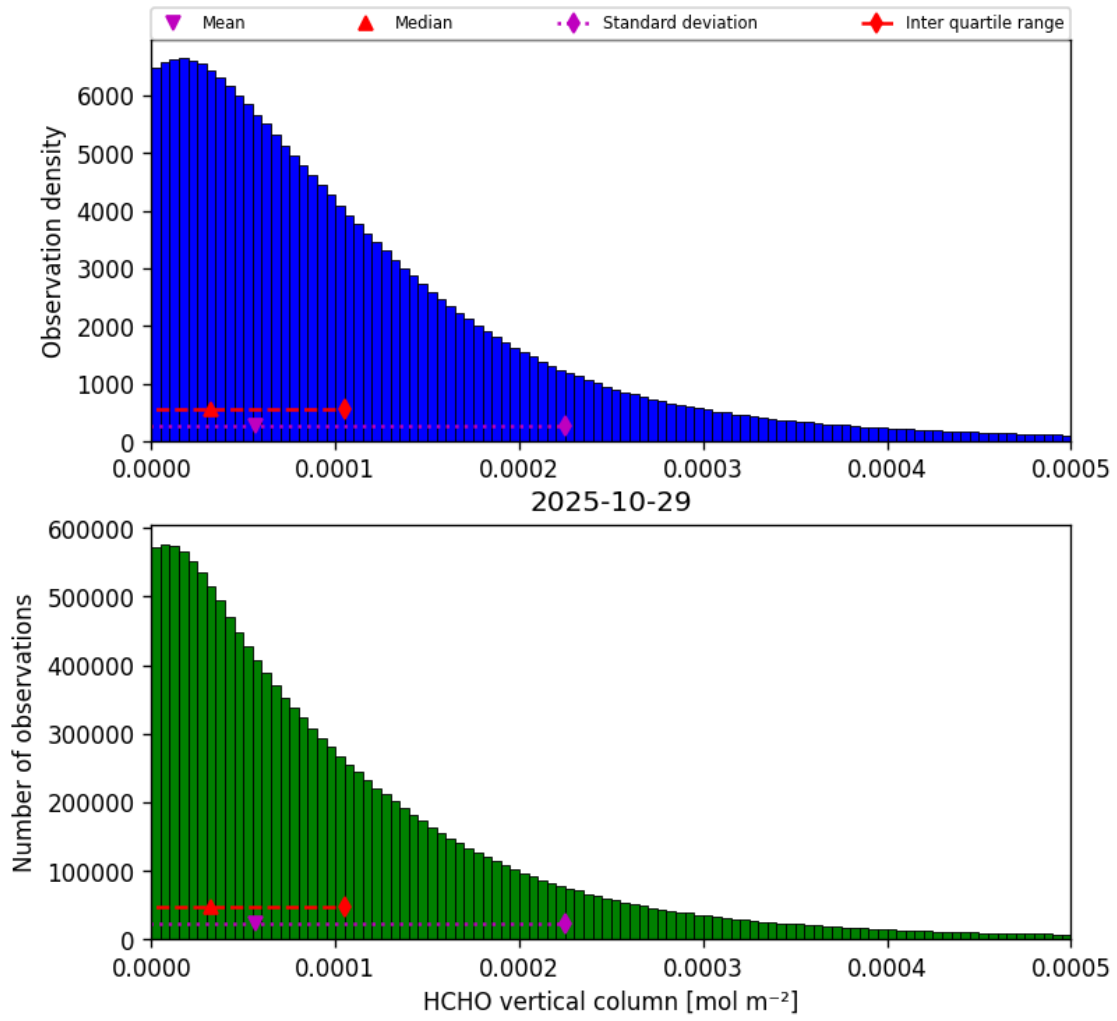
Figure 33: Histogram of “HCHO vertical column” for 2025-10-29 to 2025-10-30
