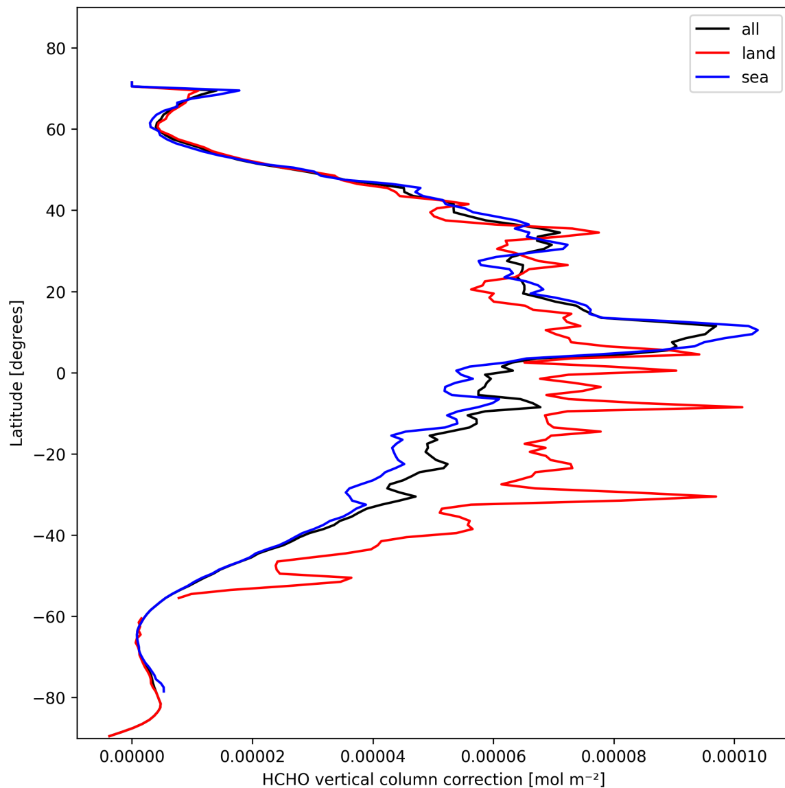
Figure 21: Zonal average of “HCHO vertical column correction” for 2025-10-29 to 2025-10-30.
