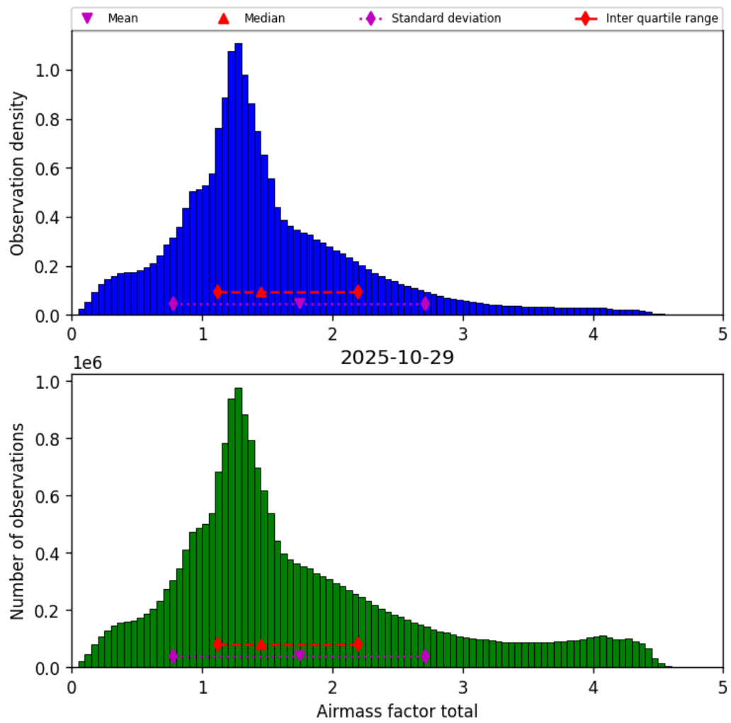
Figure 38: Histogram of “Airmass factor total” for 2025-10-29 to 2025-10-30
