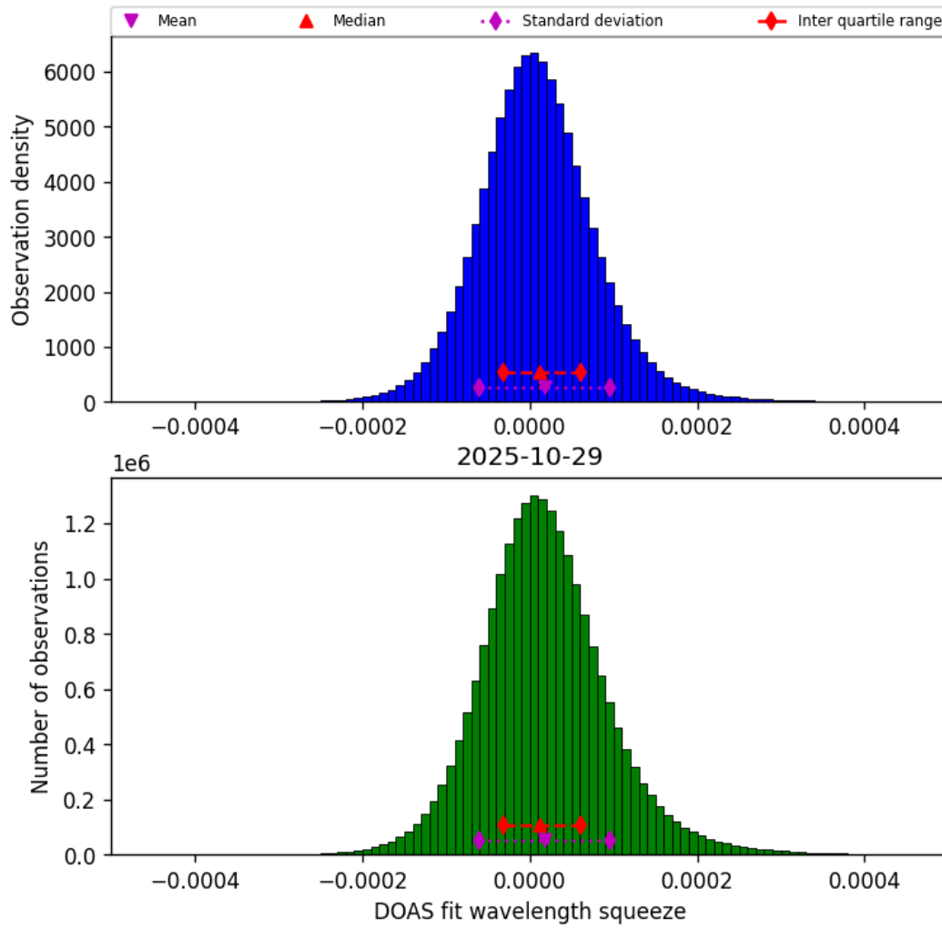
Figure 43: Histogram of “DOAS fit wavelength squeeze” for 2025-10-29 to 2025-10-30
