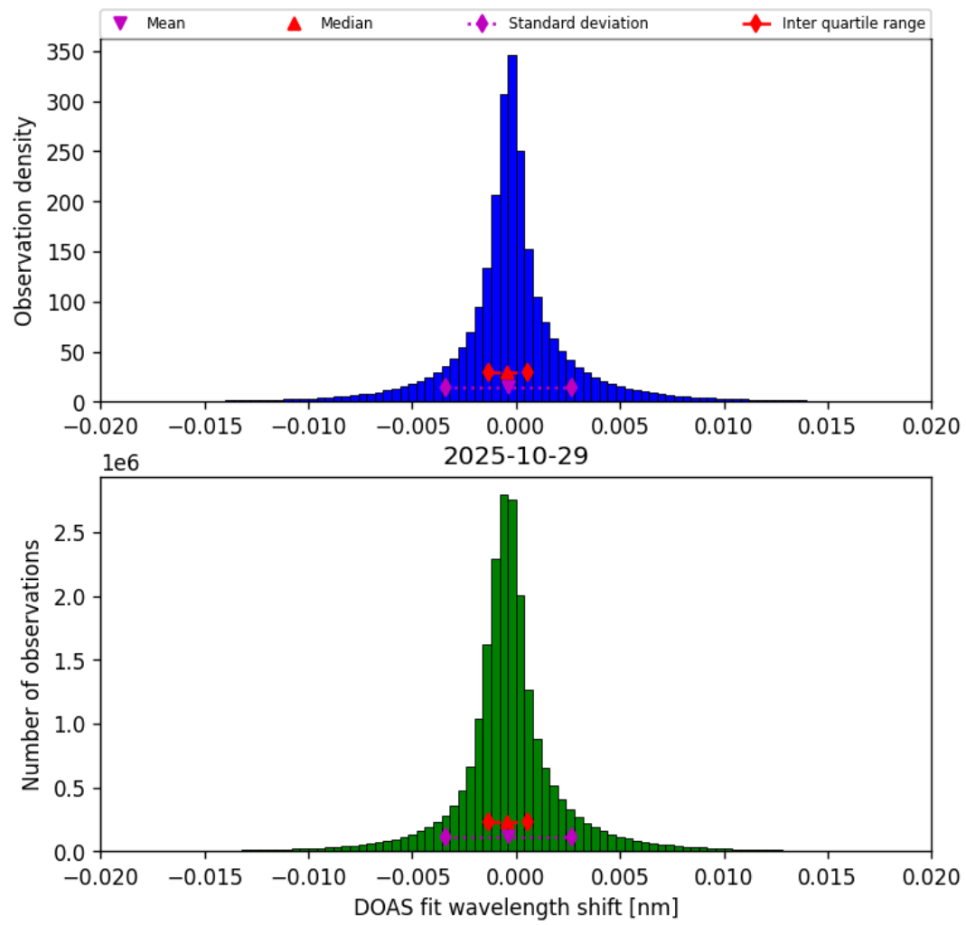
Figure 42: Histogram of “DOAS fit wavelength shift” for 2025-10-29 to 2025-10-30
