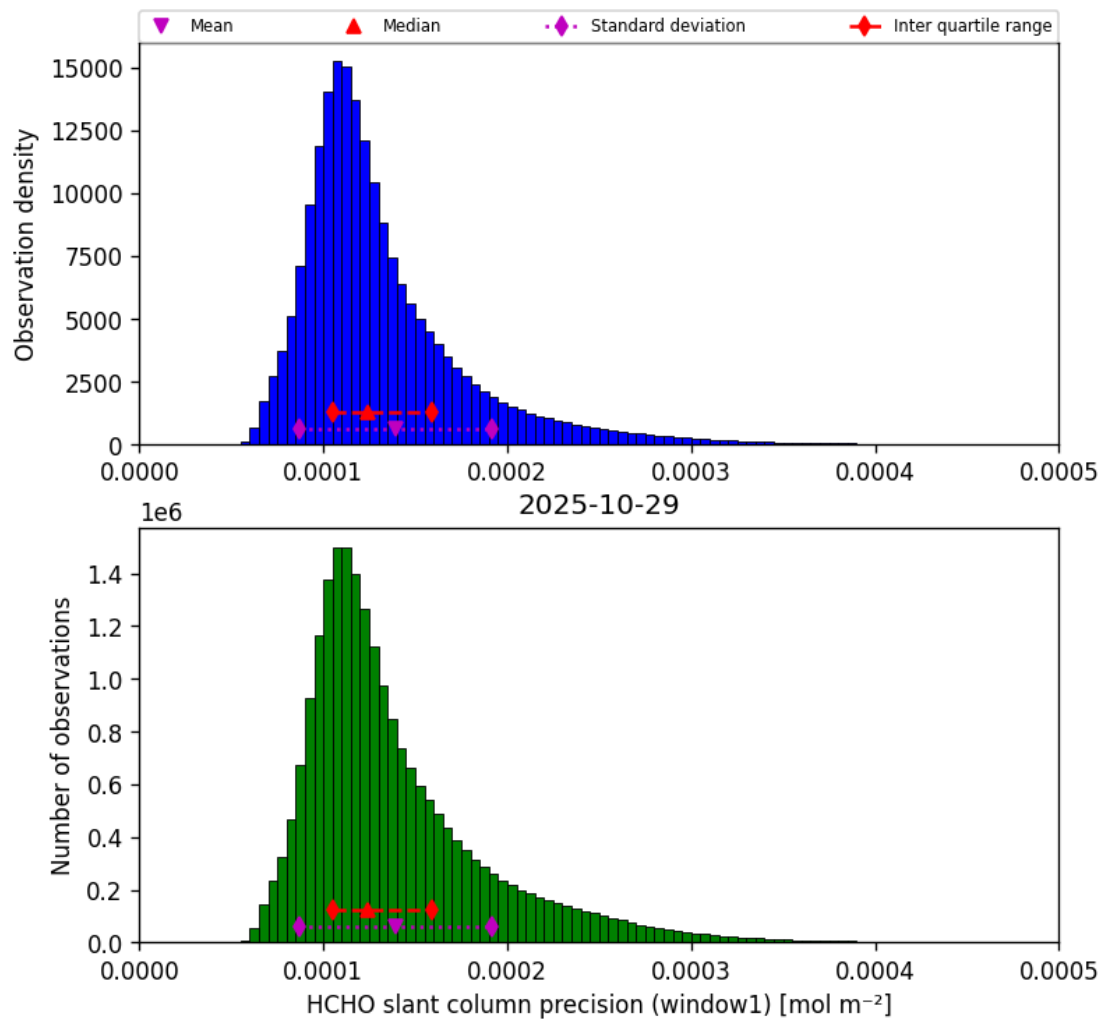
Figure 37: Histogram of “HCHO slant column precision (window1)” for 2025-10-29 to 2025-10-30
