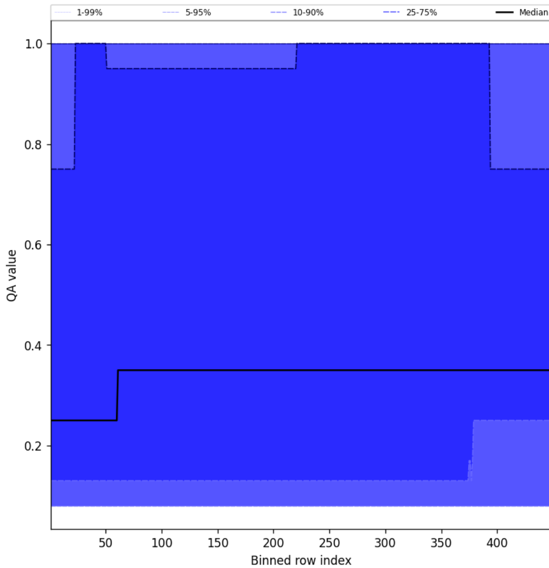
Figure 46: Along track statistics of “QA value” for 2025-10-29 to 2025-10-30
