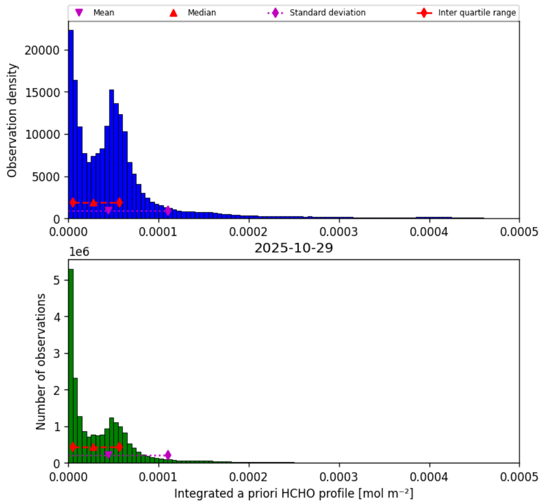
Figure 41: Histogram of “Integrated a priori HCHO profile” for 2025-10-29 to 2025-10-30
