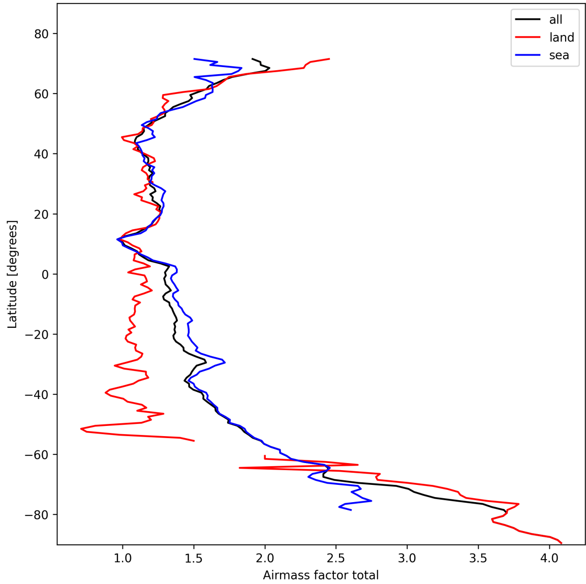
Figure 24: Zonal average of “Airmass factor total” for 2025-10-29 to 2025-10-30.
