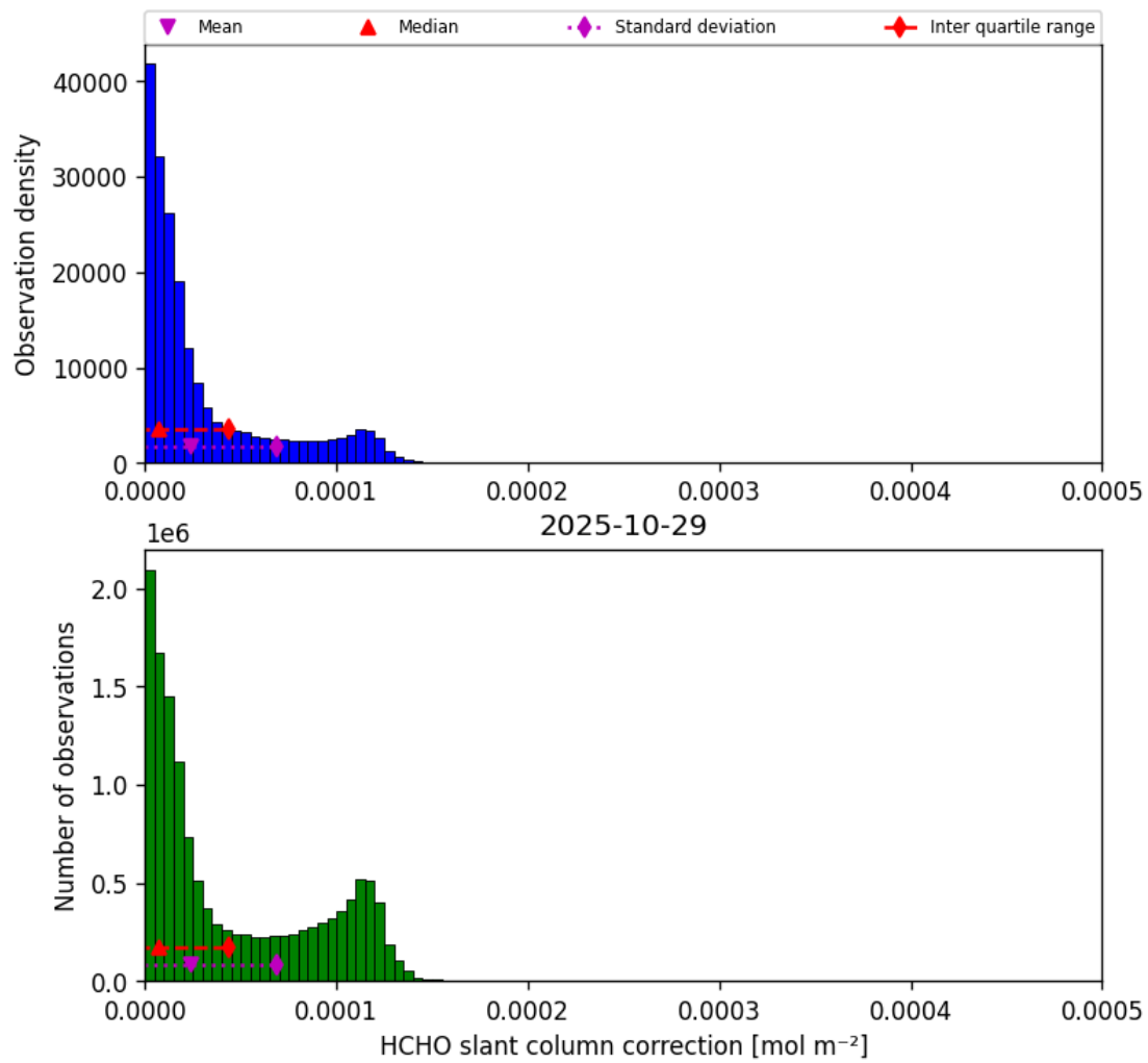
Figure 45: Histogram of “HCHO slant column correction” for 2025-10-29 to 2025-10-30
