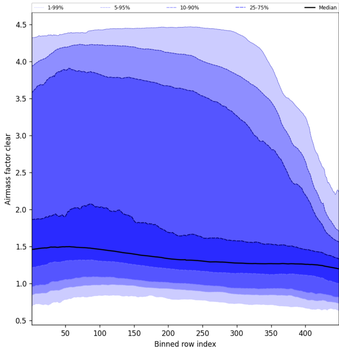
Figure 54: Along track statistics of “Airmass factor clear” for 2025-10-29 to 2025-10-30
