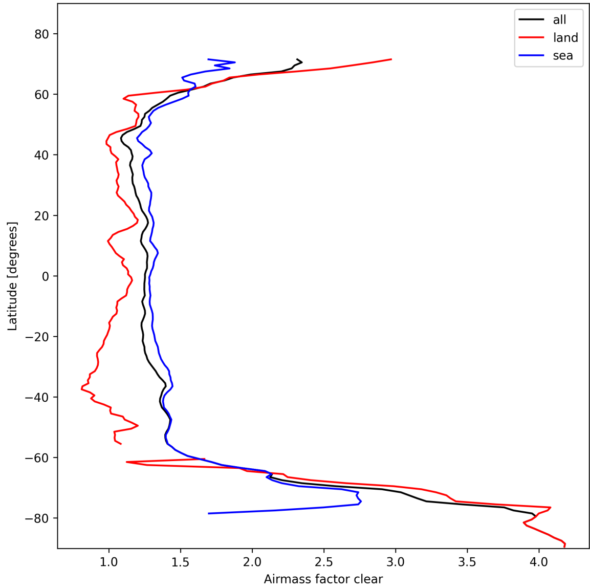
Figure 26: Zonal average of “Airmass factor clear” for 2025-10-29 to 2025-10-30.
