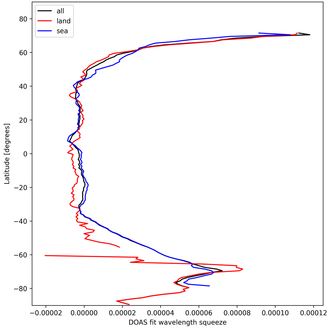
Figure 29: Zonal average of “DOAS fit wavelength squeeze” for 2025-10-29 to 2025-10-30.
