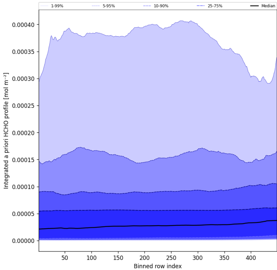
Figure 55: Along track statistics of “Integrated a priori HCHO profile” for 2025-10-29 to 2025-10-30
