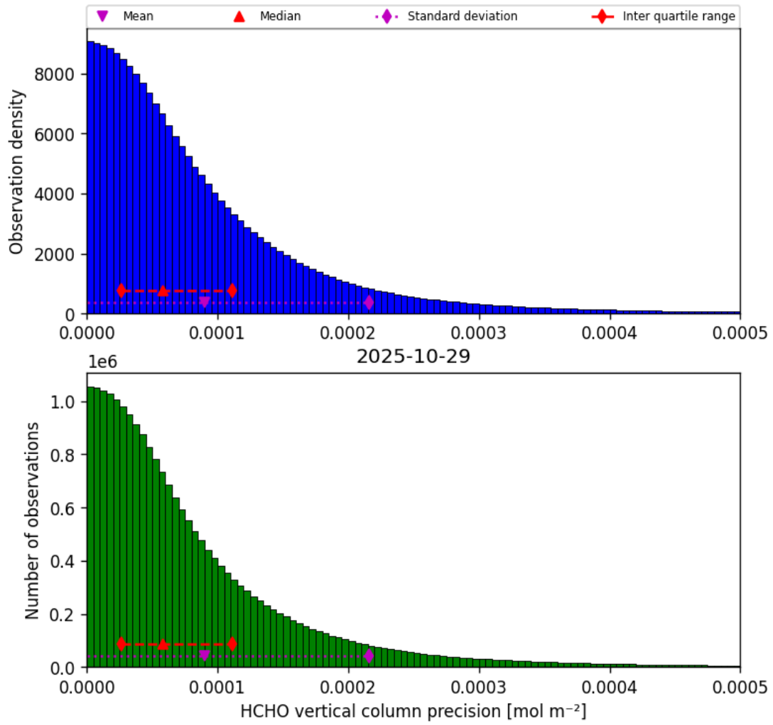
Figure 34: Histogram of “HCHO vertical column precision” for 2025-10-29 to 2025-10-30
