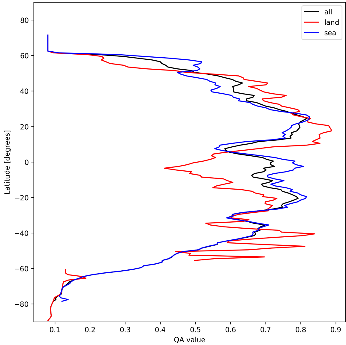
Figure 18: Zonal average of “QA value” for 2025-10-29 to 2025-10-30.
