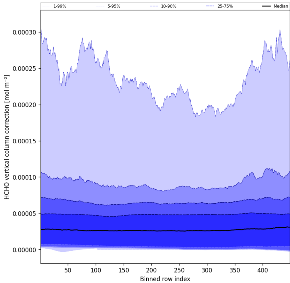
Figure 49: Along track statistics of “HCHO vertical column correction” for 2025-10-29 to 2025-10-30
