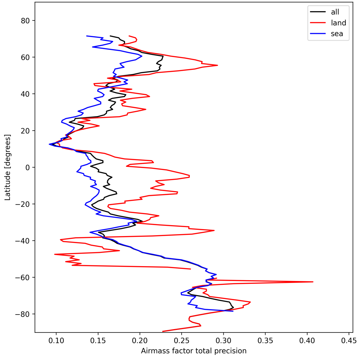
Figure 25: Zonal average of “Airmass factor total precision” for 2025-10-29 to 2025-10-30.
