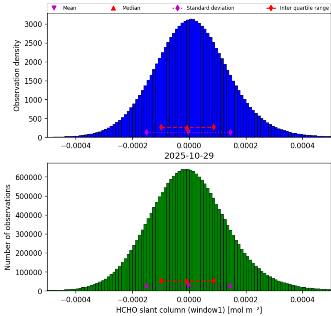
Figure 36: Histogram of “HCHO slant column (window1)” for 2025-10-29 to 2025-10-30
