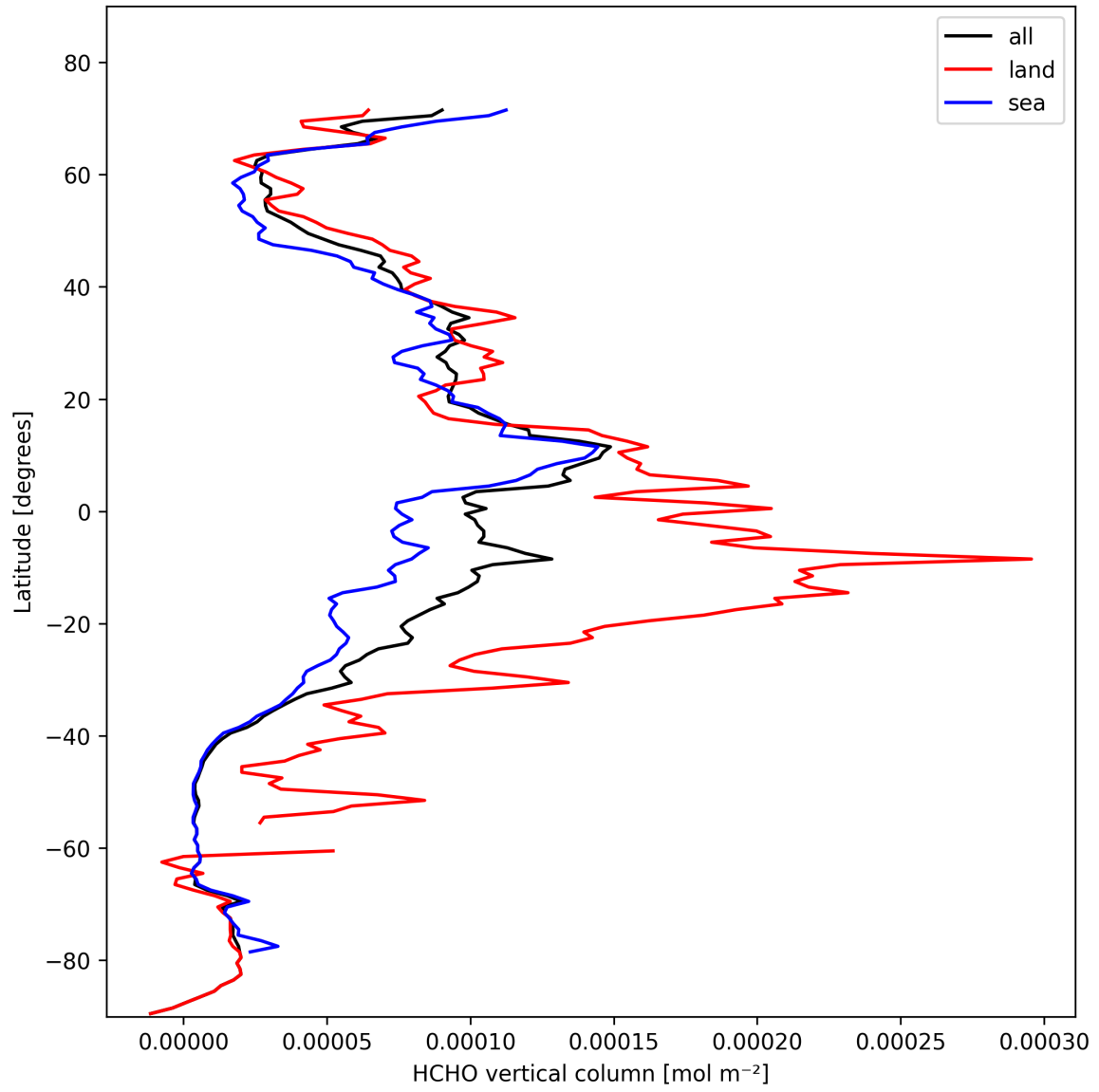
Figure 19: Zonal average of “HCHO vertical column” for 2025-10-29 to 2025-10-30.
