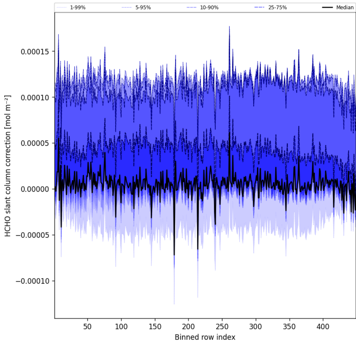
Figure 59: Along track statistics of “HCHO slant column correction” for 2025-10-29 to 2025-10-30
