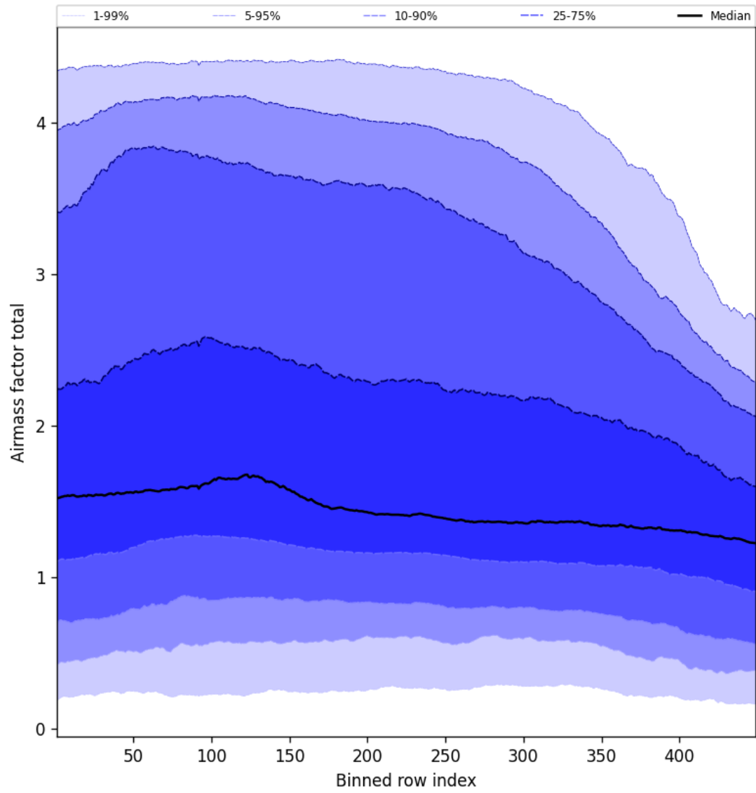
Figure 52: Along track statistics of “Airmass factor total” for 2025-10-29 to 2025-10-30
