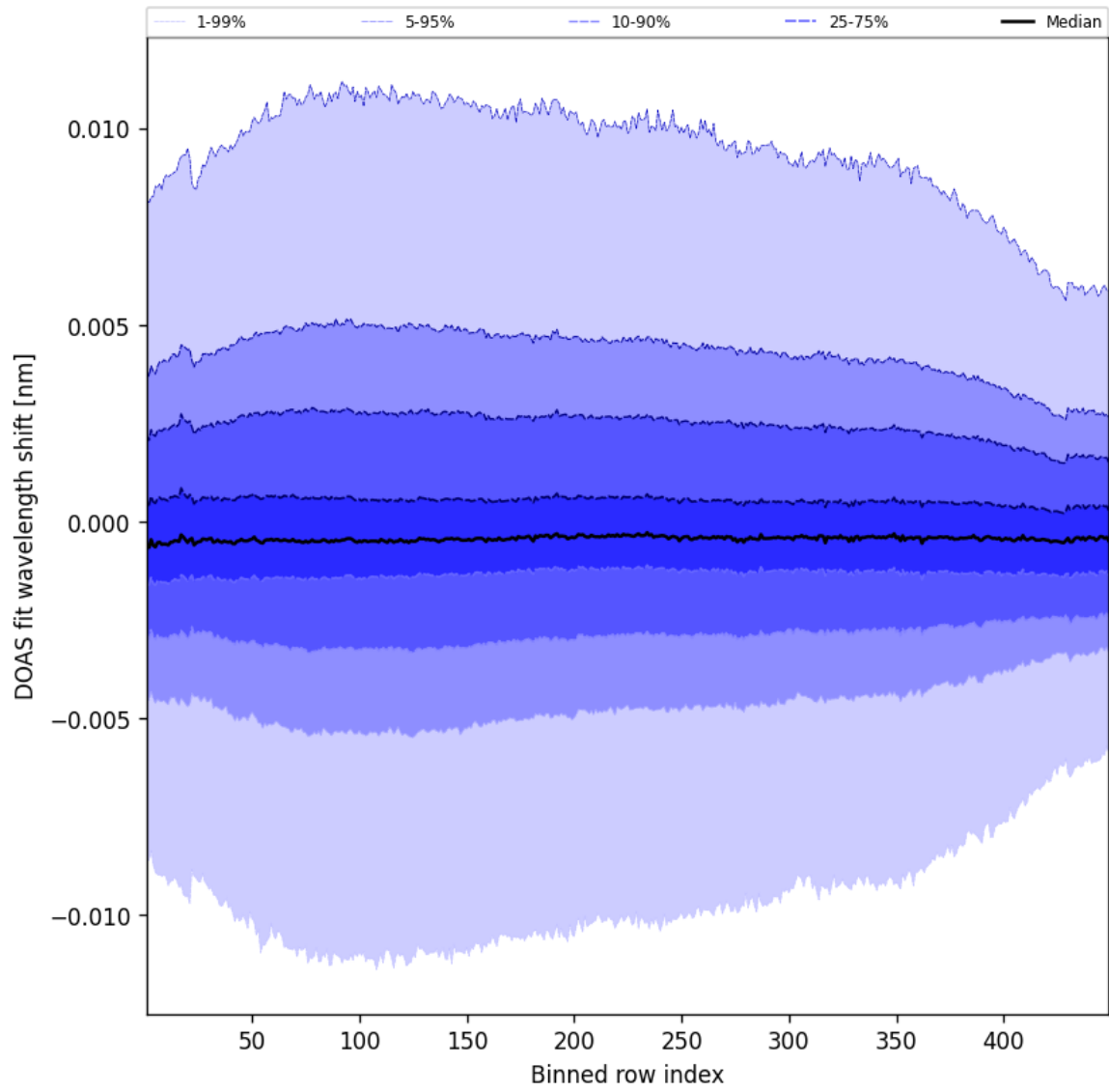
Figure 56: Along track statistics of “DOAS fit wavelength shift” for 2025-10-29 to 2025-10-30
