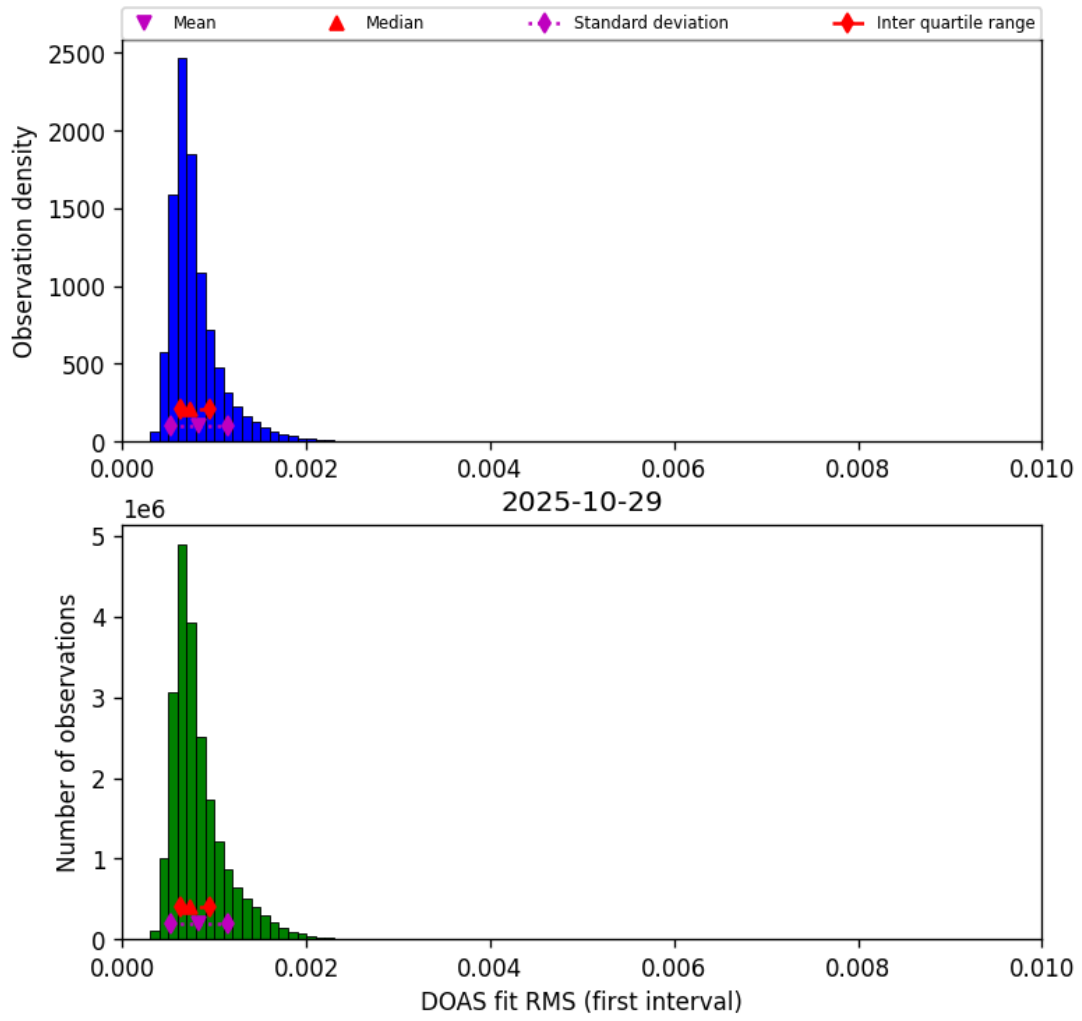
Figure 44: Histogram of “DOAS fit RMS (first interval)” for 2025-10-29 to 2025-10-30
