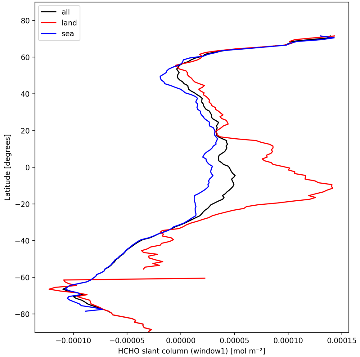
Figure 22: Zonal average of “HCHO slant column (window1)” for 2025-10-29 to 2025-10-30.
