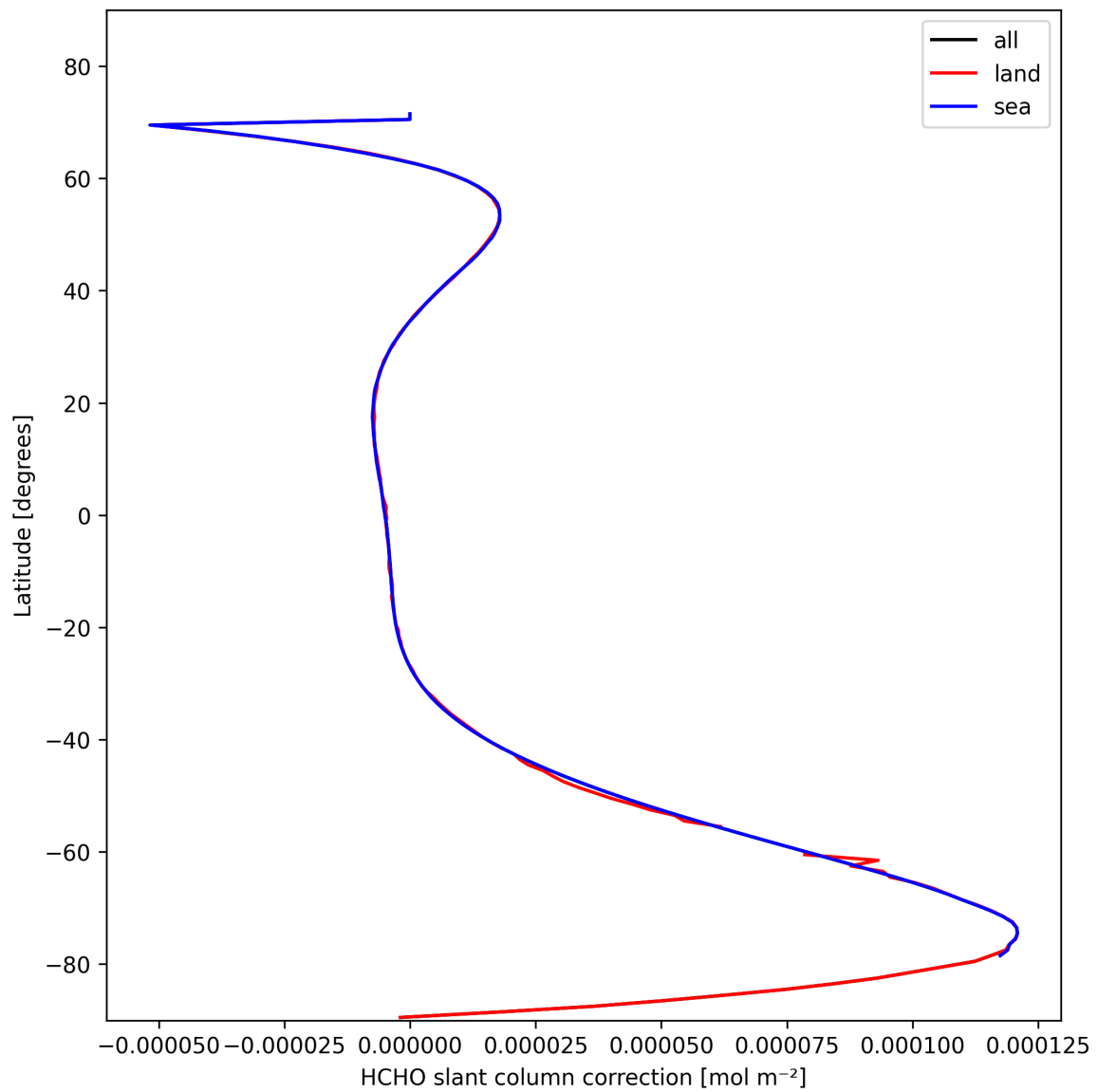
Figure 31: Zonal average of “HCHO slant column correction” for 2025-10-29 to 2025-10-30.
