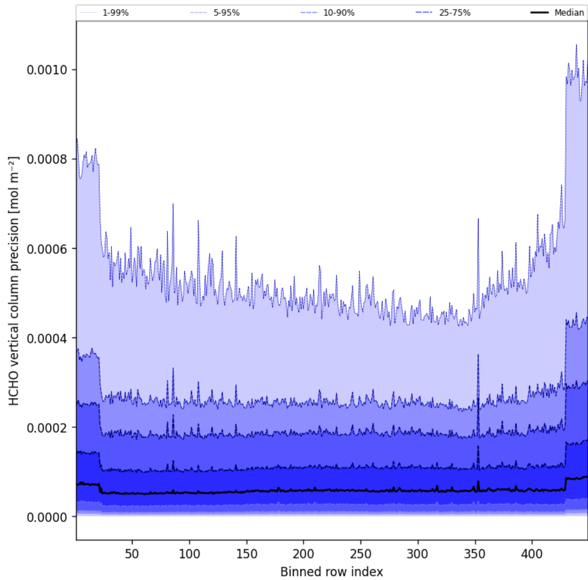
Figure 48: Along track statistics of “HCHO vertical column precision” for 2025-10-29 to 2025-10-30
