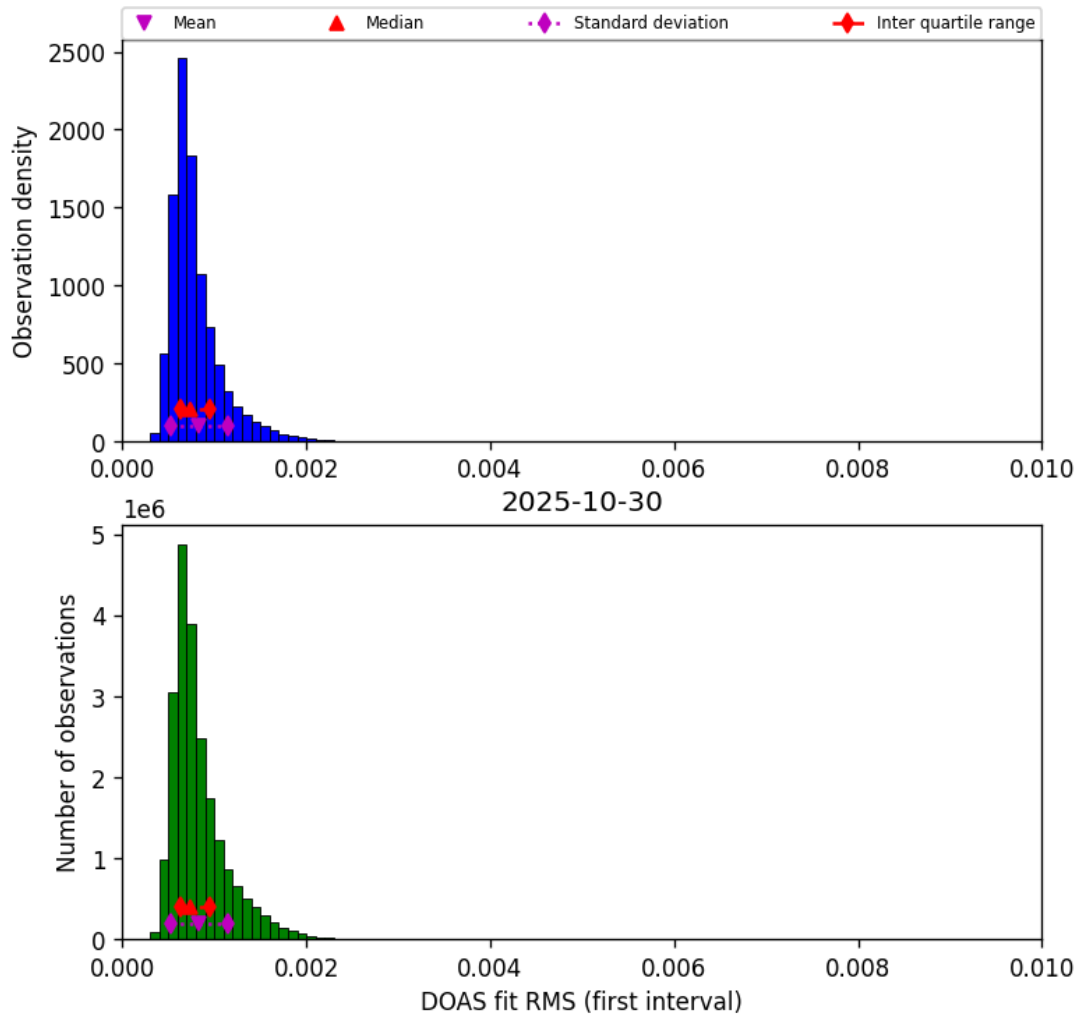
Figure 44: Histogram of “DOAS fit RMS (first interval)” for 2025-10-30 to 2025-10-30
