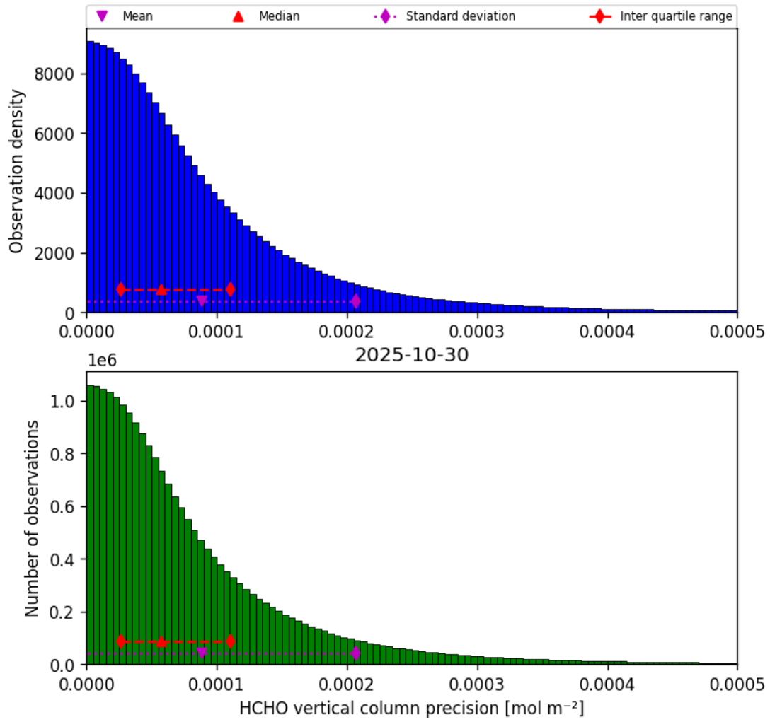
Figure 34: Histogram of “HCHO vertical column precision” for 2025-10-30 to 2025-10-30
