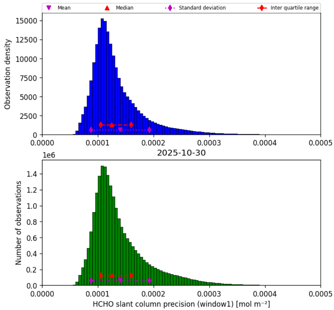
Figure 37: Histogram of “HCHO slant column precision (window1)” for 2025-10-30 to 2025-10-30
