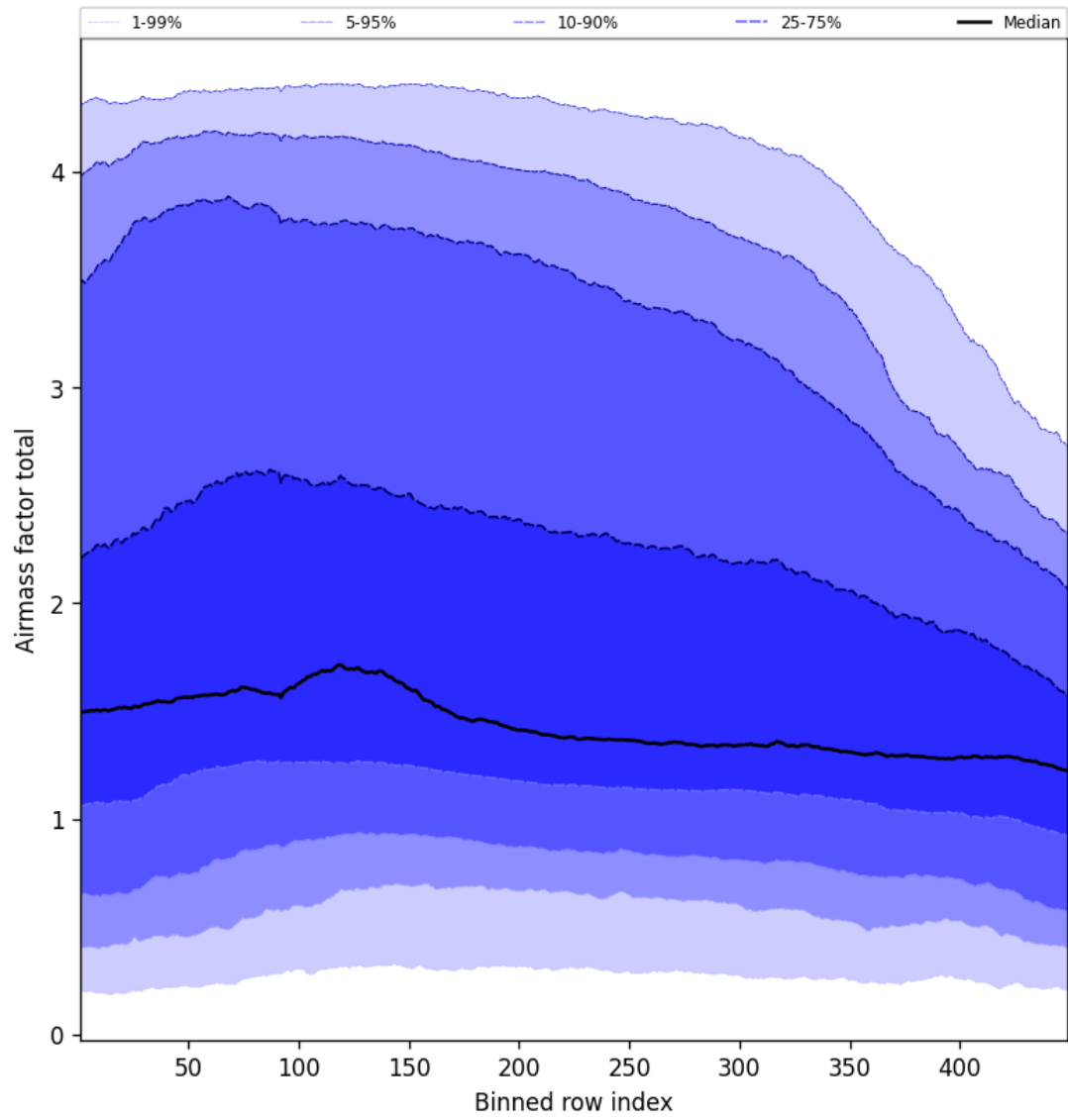
Figure 52: Along track statistics of “Airmass factor total” for 2025-10-30 to 2025-10-30
