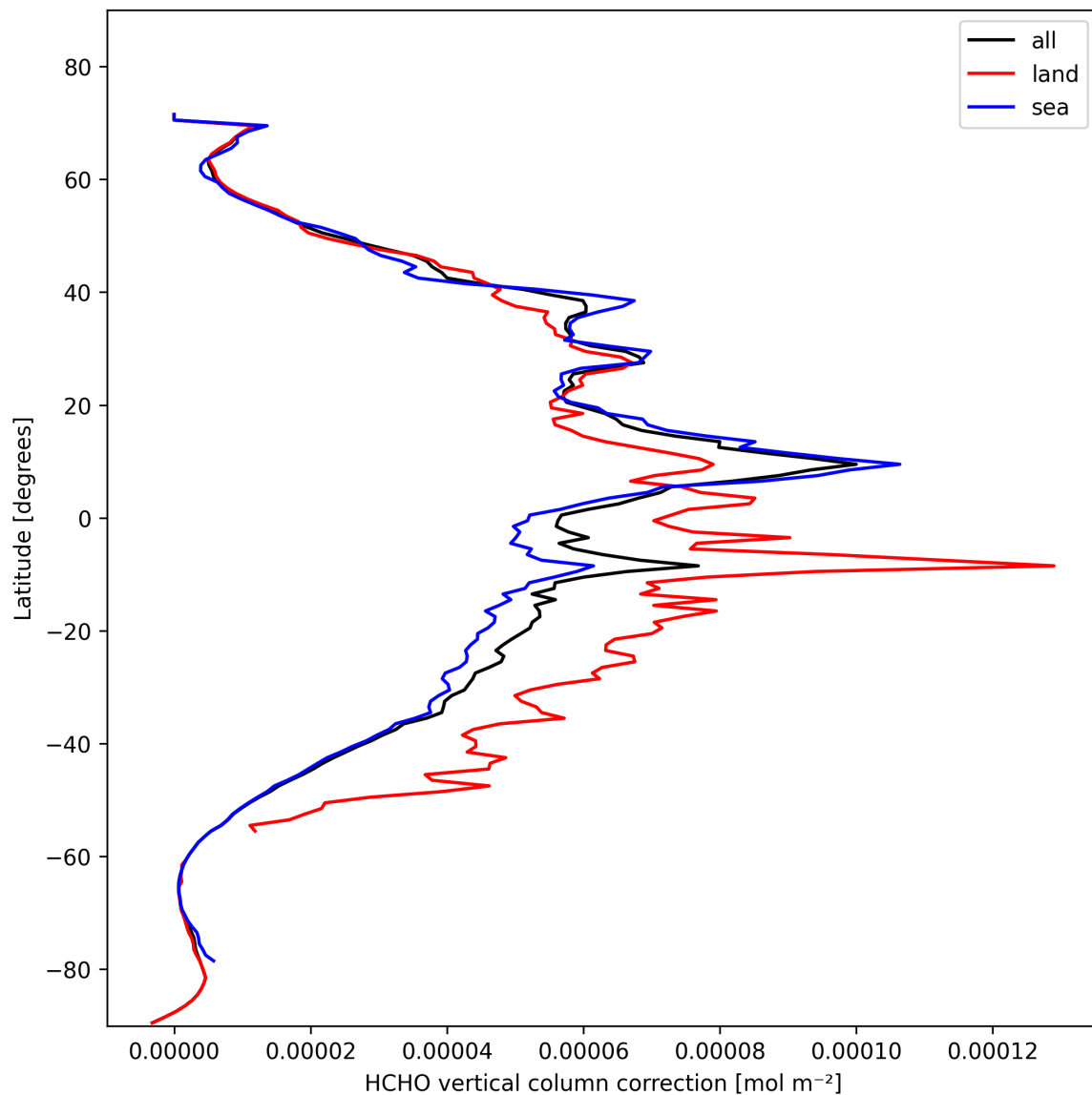
Figure 21: Zonal average of “HCHO vertical column correction” for 2025-10-30 to 2025-10-30.
