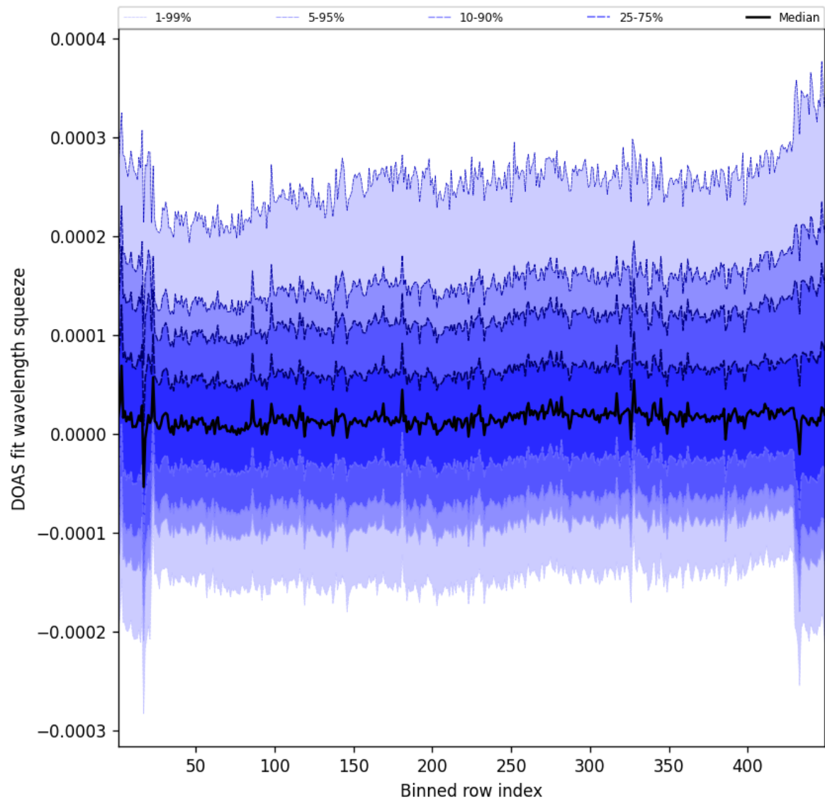
Figure 57: Along track statistics of “DOAS fit wavelength squeeze” for 2025-10-30 to 2025-10-30
