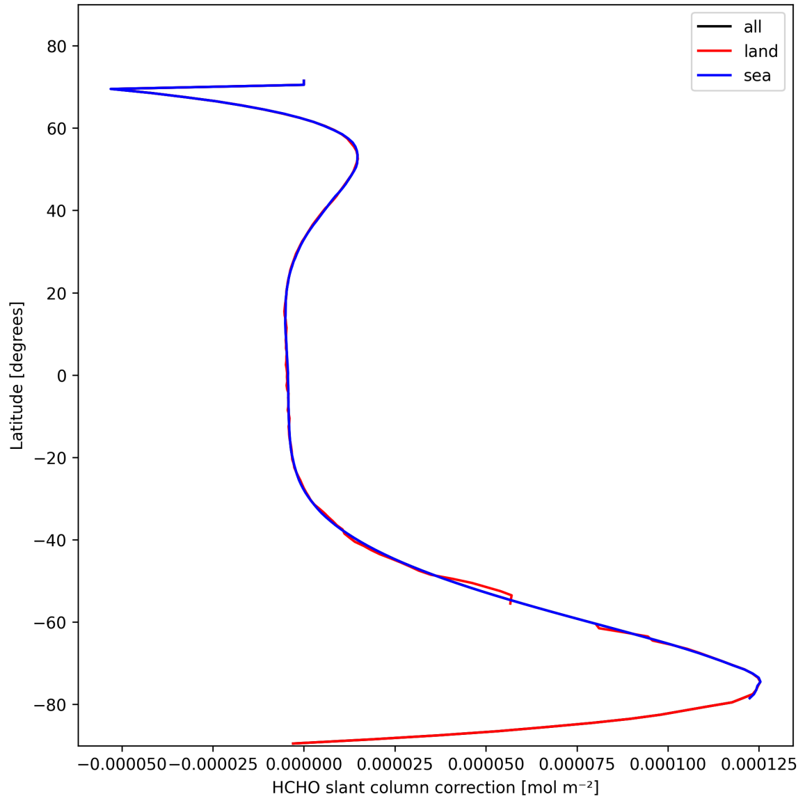
Figure 31: Zonal average of “HCHO slant column correction” for 2025-10-30 to 2025-10-30.
