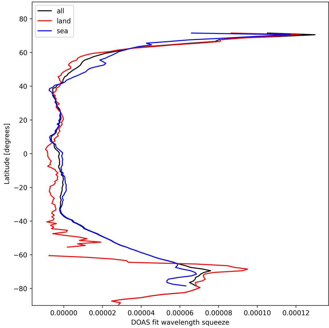
Figure 29: Zonal average of “DOAS fit wavelength squeeze” for 2025-10-30 to 2025-10-30.
