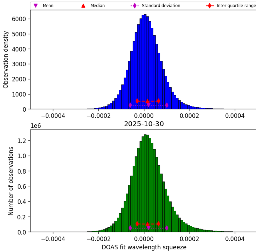
Figure 43: Histogram of “DOAS fit wavelength squeeze” for 2025-10-30 to 2025-10-30
