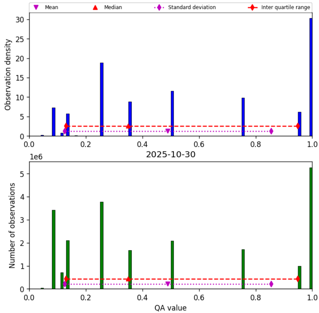
Figure 32: Histogram of “QA value” for 2025-10-30 to 2025-10-30
