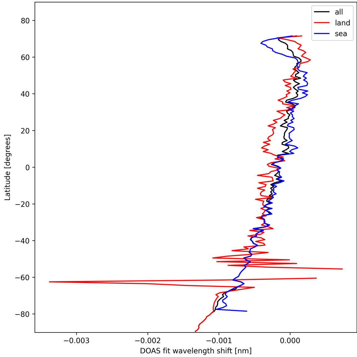
Figure 28: Zonal average of “DOAS fit wavelength shift” for 2025-10-30 to 2025-10-30.
