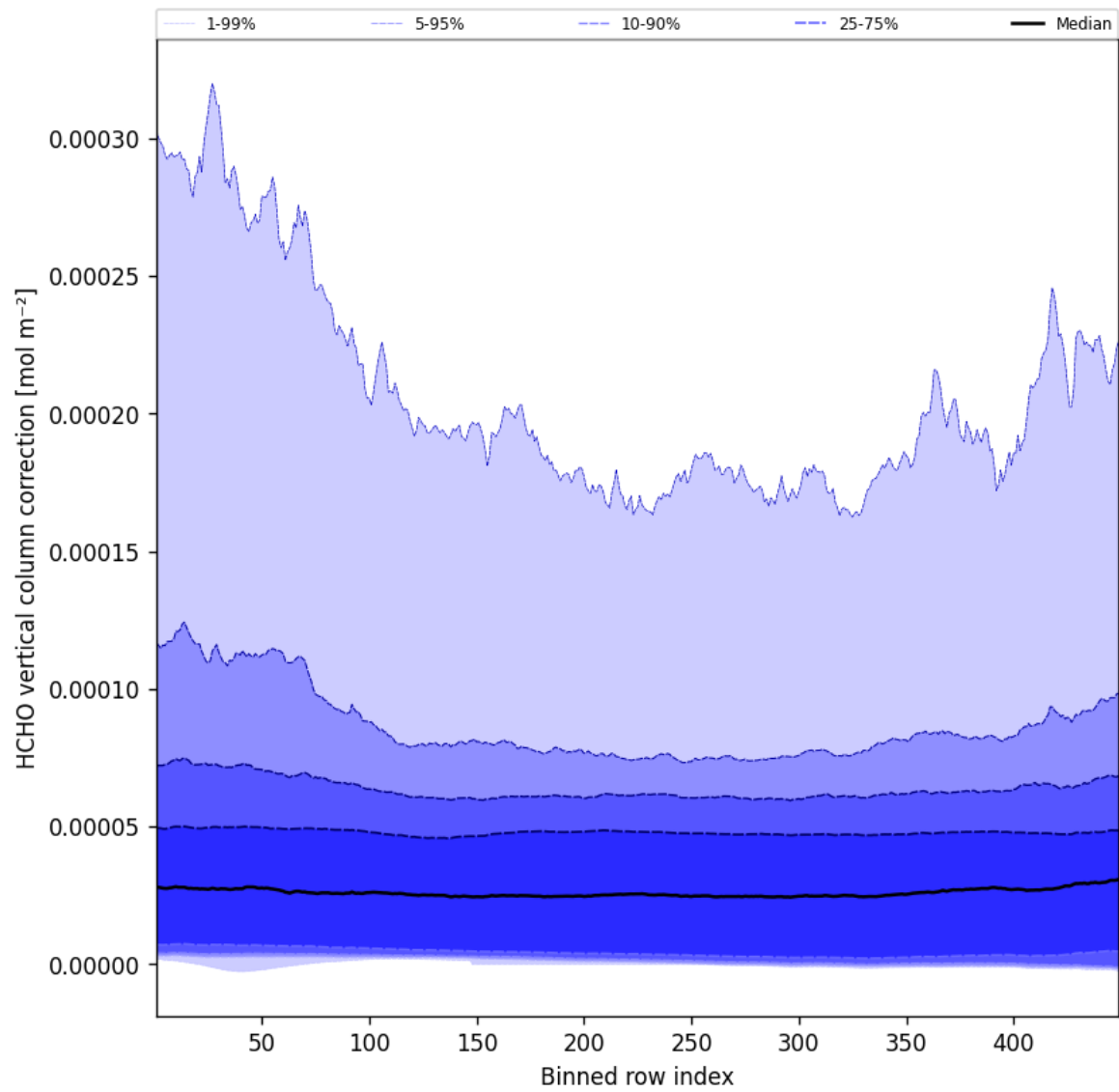
Figure 49: Along track statistics of “HCHO vertical column correction” for 2025-10-30 to 2025-10-30
