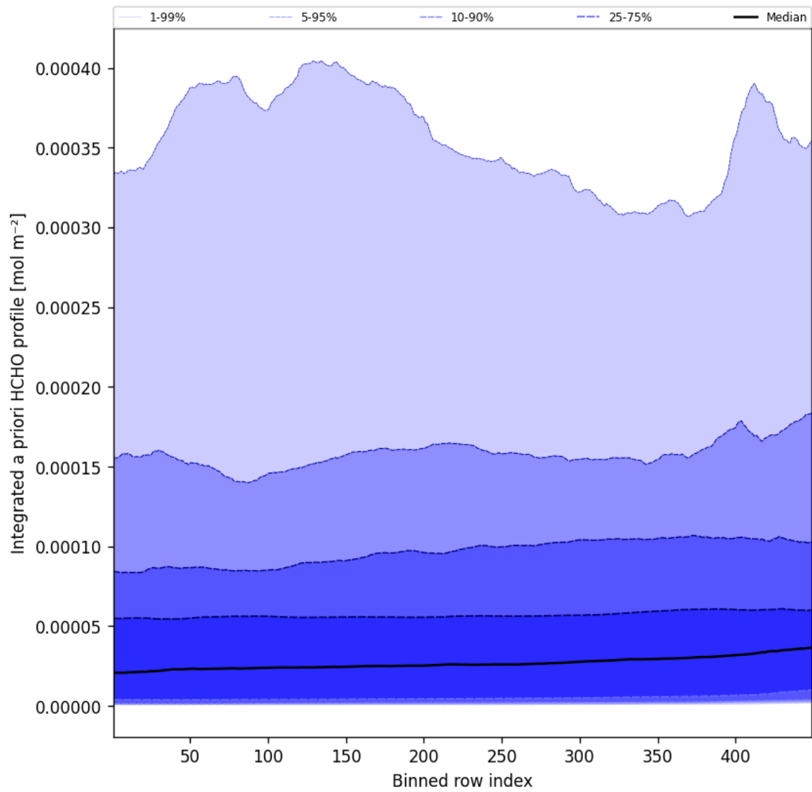
Figure 55: Along track statistics of “Integrated a priori HCHO profile” for 2025-10-30 to 2025-10-30
