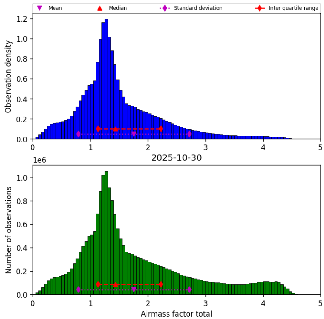
Figure 38: Histogram of “Airmass factor total” for 2025-10-30 to 2025-10-30
