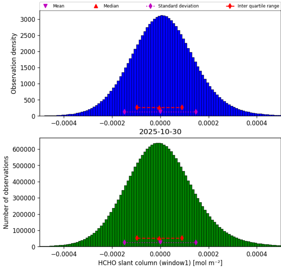
Figure 36: Histogram of "HCHO slant column (window1)" for 2025-10-30 to 2025-10-30
