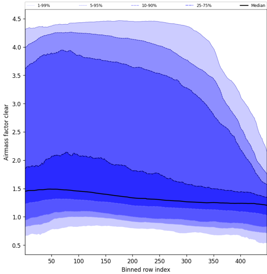
Figure 54: Along track statistics of “Airmass factor clear” for 2025-10-30 to 2025-10-30
