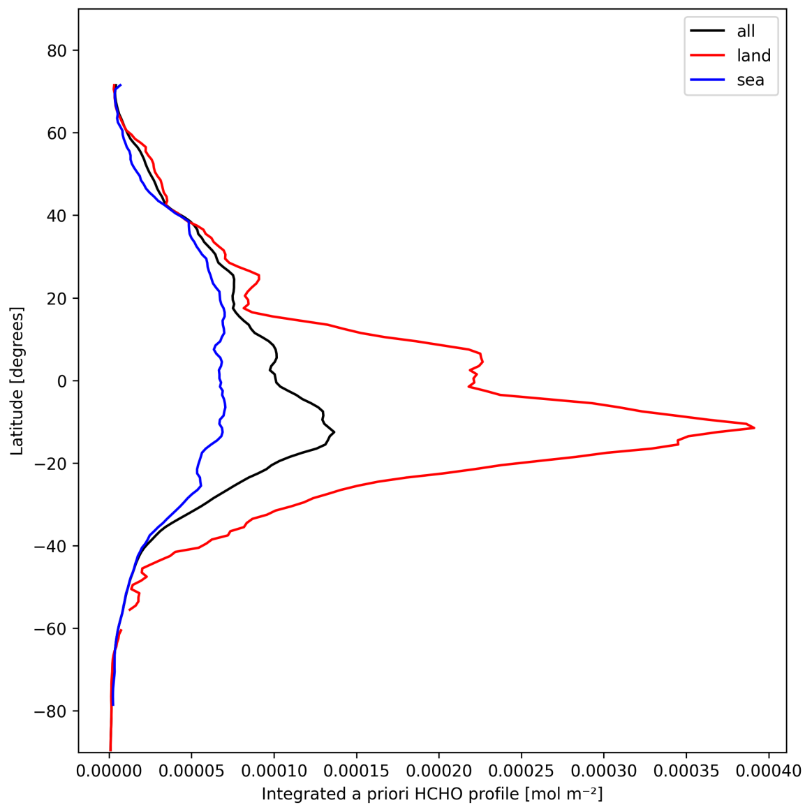
Figure 27: Zonal average of “Integrated a priori HCHO profile” for 2025-10-30 to 2025-10-30.
