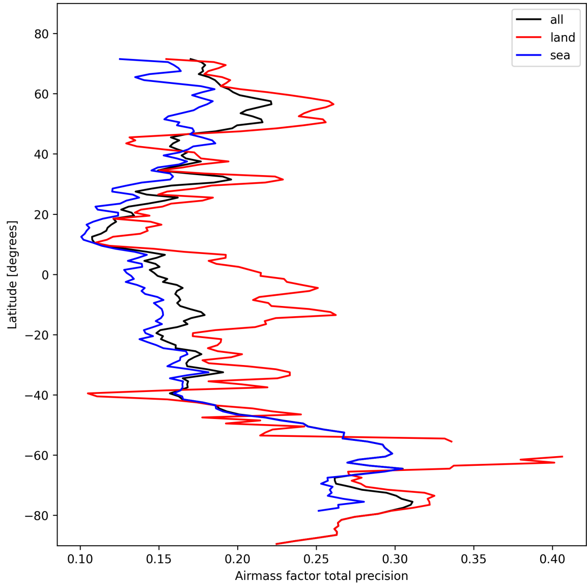
Figure 25: Zonal average of “Airmass factor total precision” for 2025-10-30 to 2025-10-30.
