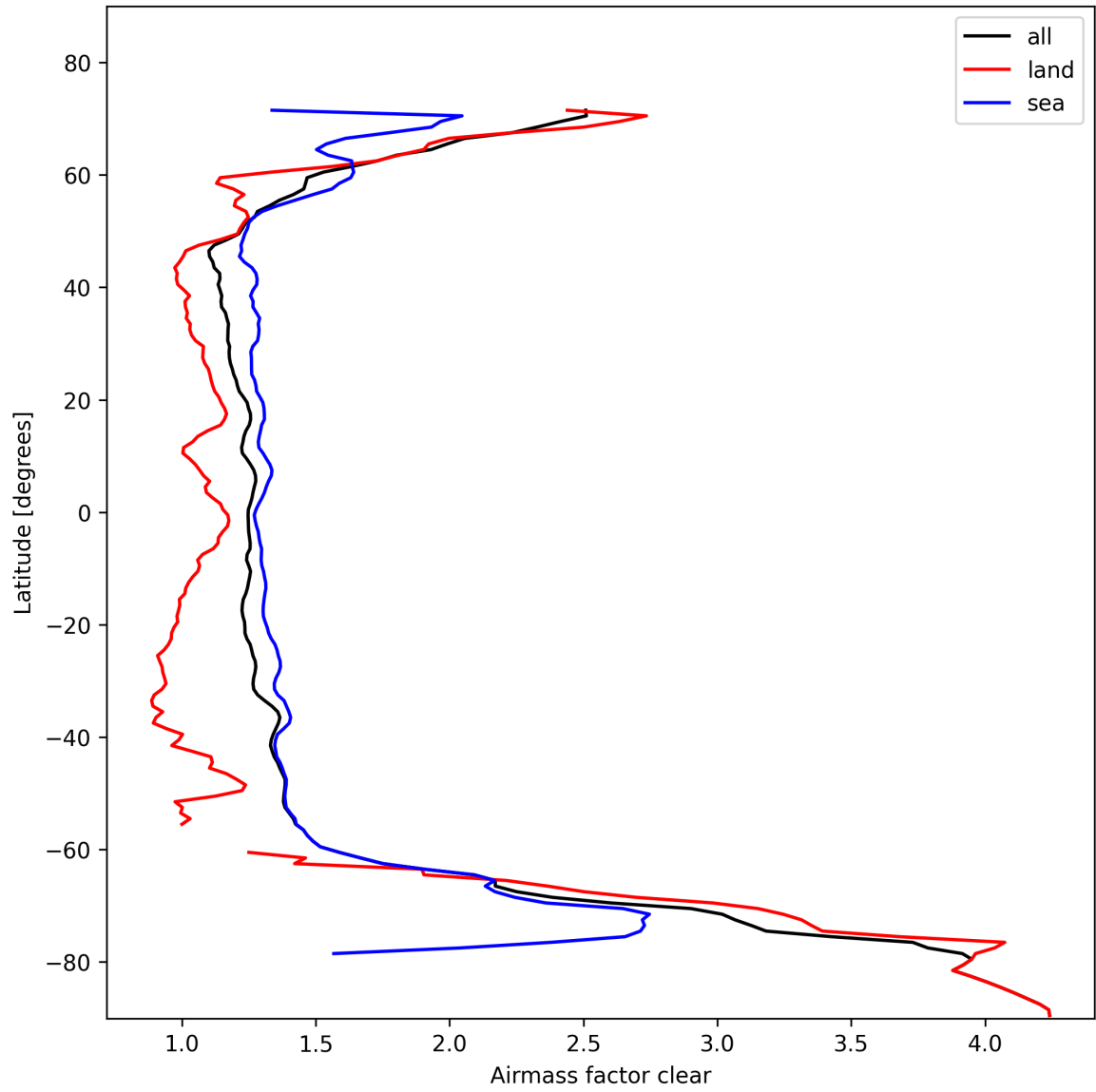
Figure 26: Zonal average of “Airmass factor clear” for 2025-10-30 to 2025-10-30.
