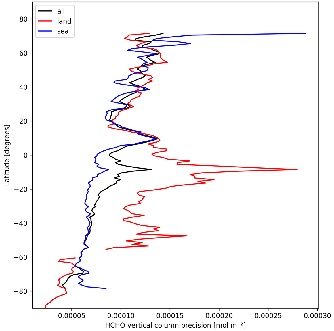
Figure 20: Zonal average of “HCHO vertical column precision” for 2025-10-30 to 2025-10-30.
