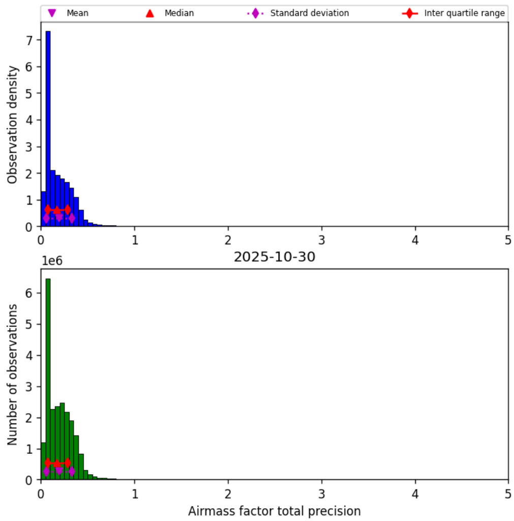
Figure 39: Histogram of “Airmass factor total precision” for 2025-10-30 to 2025-10-30
