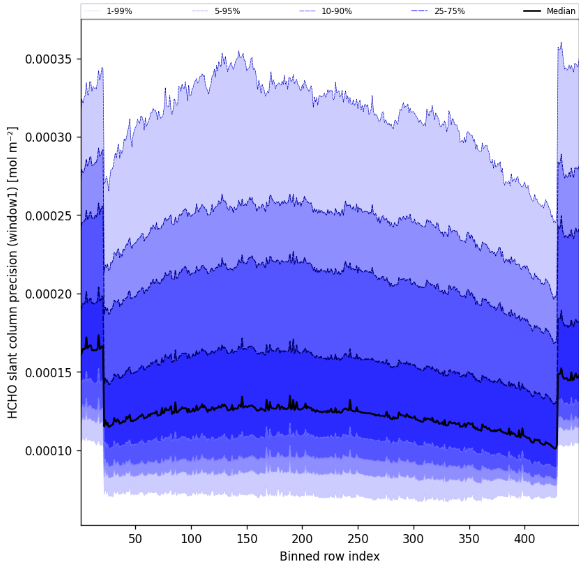
Figure 51: Along track statistics of “HCHO slant column precision (window1)” for 2025-10-30 to 2025-10-30
