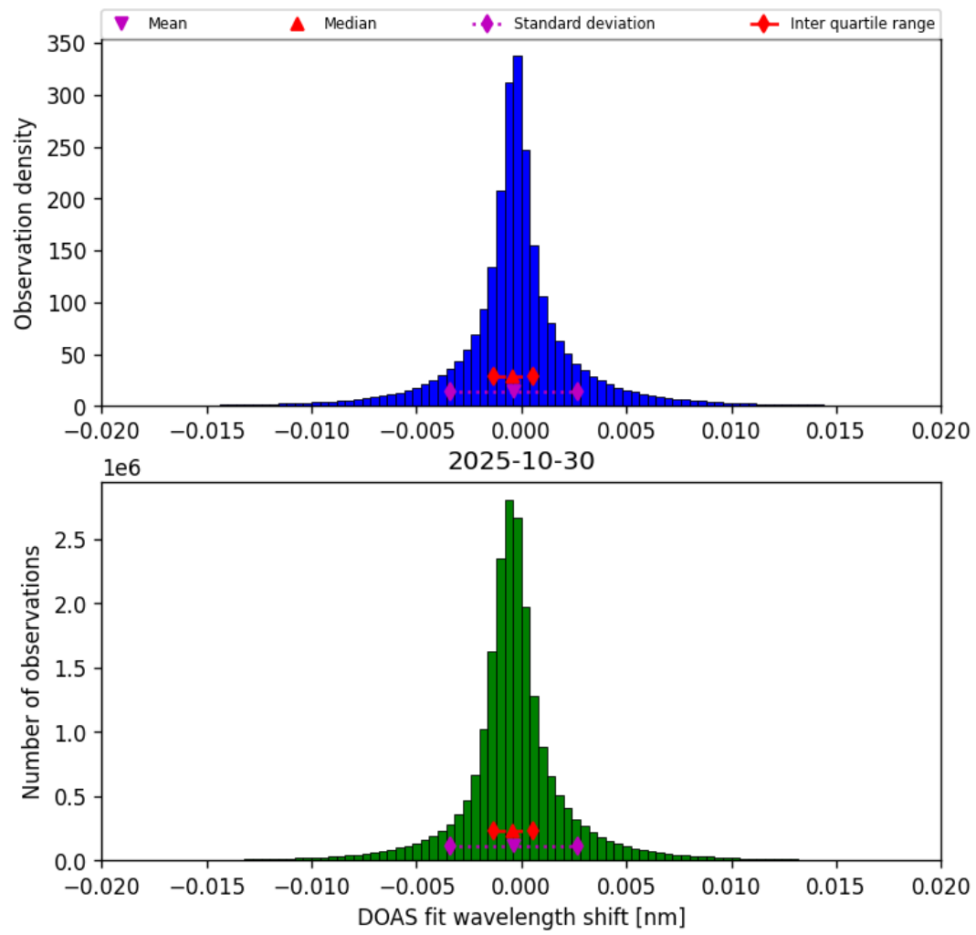
Figure 42: Histogram of “DOAS fit wavelength shift” for 2025-10-30 to 2025-10-30
