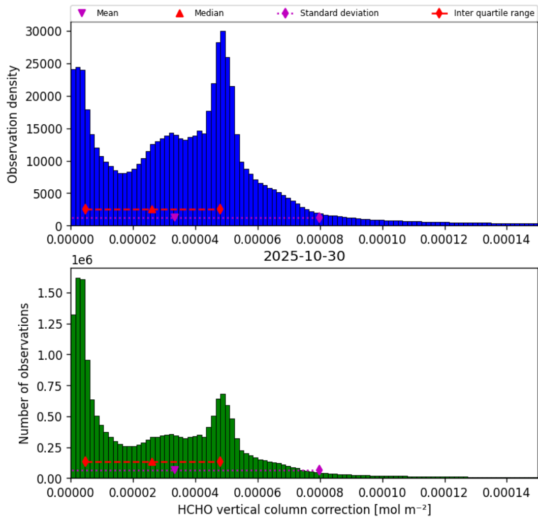
Figure 35: Histogram of "HCHO vertical column correction" for 2025-10-30 to 2025-10-30
