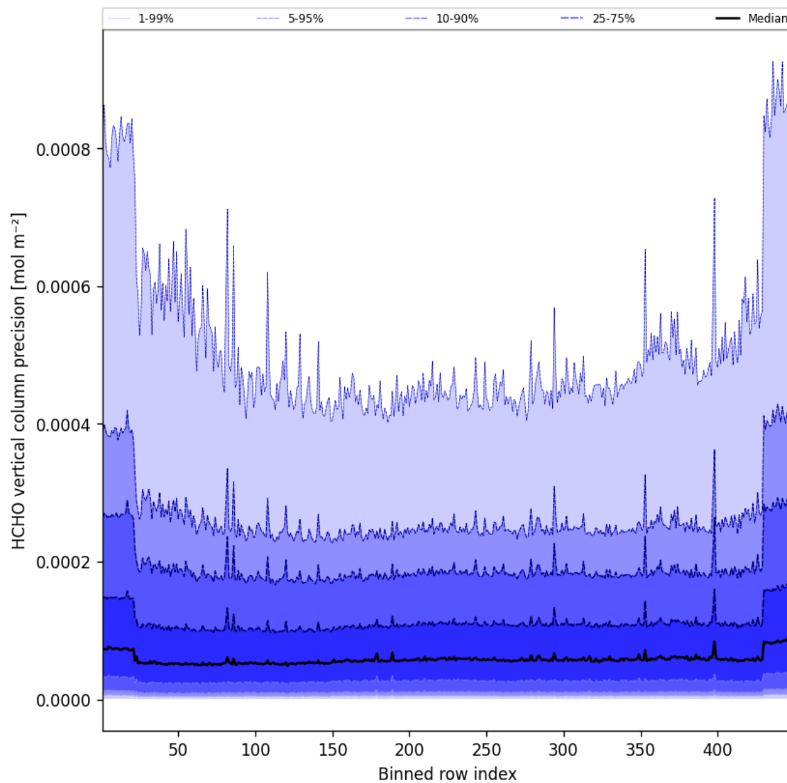
Figure 48: Along track statistics of “HCHO vertical column precision” for 2025-10-30 to 2025-10-30
