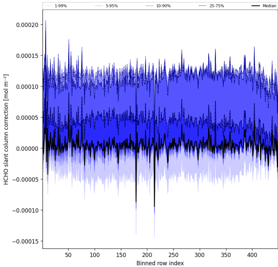
Figure 59: Along track statistics of “HCHO slant column correction” for 2025-10-30 to 2025-10-30
