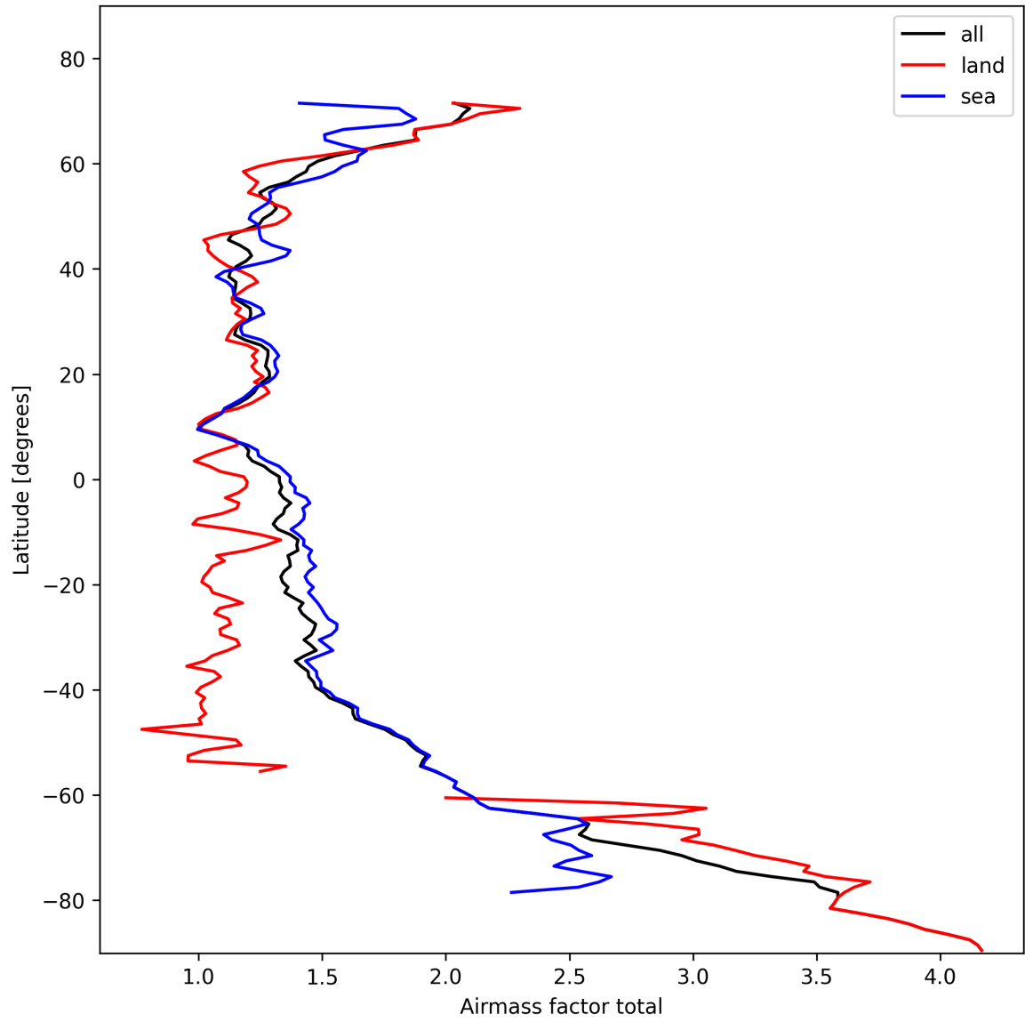
Figure 24: Zonal average of “Airmass factor total” for 2025-10-30 to 2025-10-30.
