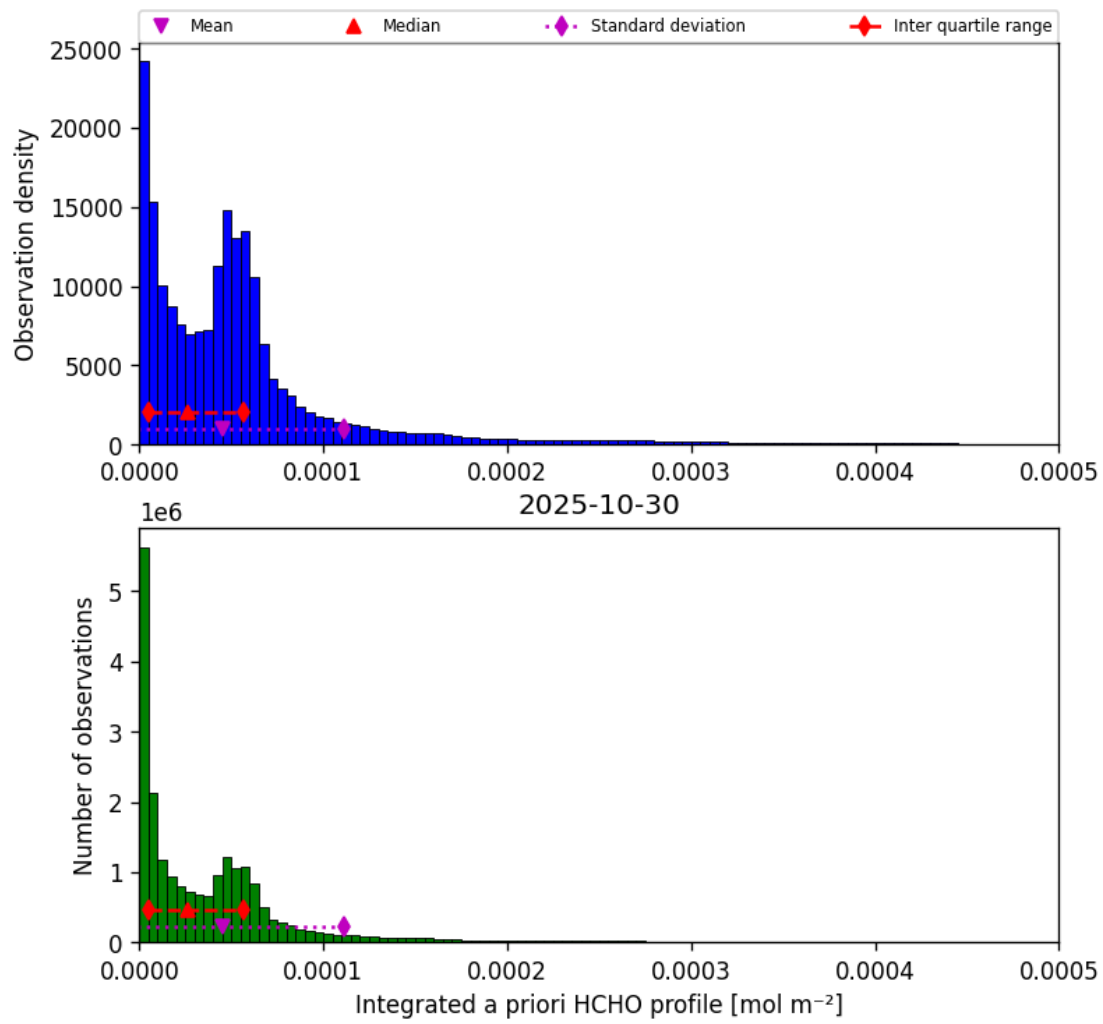
Figure 41: Histogram of “Integrated a priori HCHO profile” for 2025-10-30 to 2025-10-30
