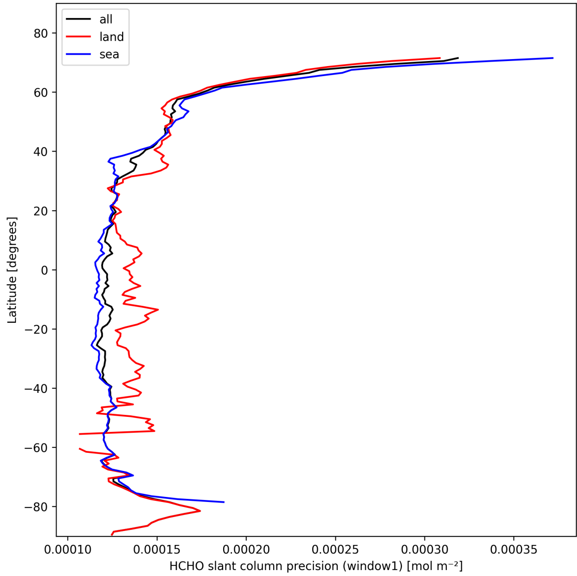
Figure 23: Zonal average of "HCHO slant column precision (window1)" for 2025-10-30 to 2025-10-30.
