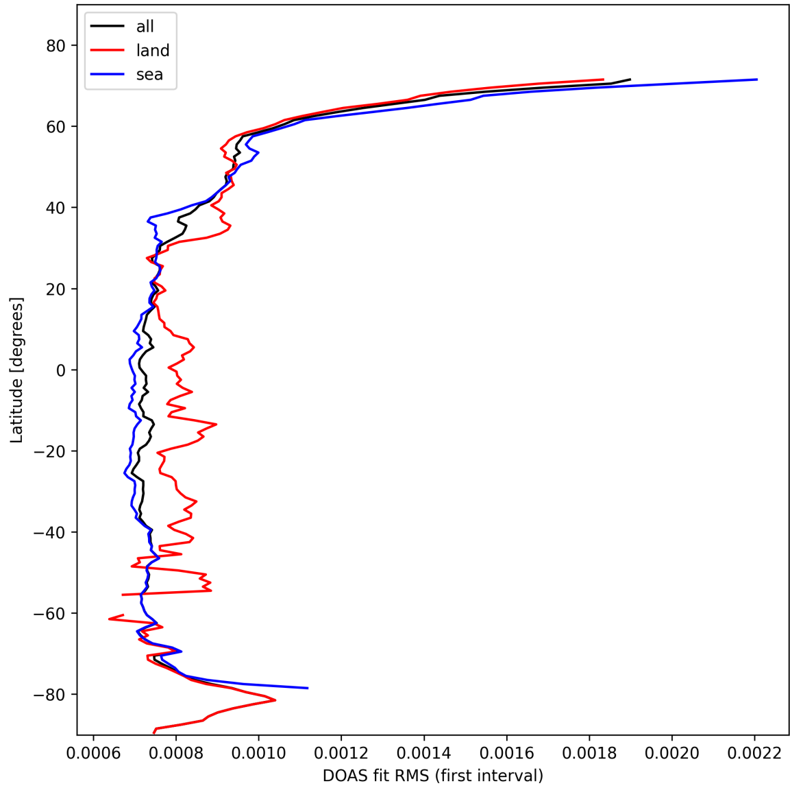
Figure 30: Zonal average of “DOAS fit RMS (first interval)” for 2025-10-30 to 2025-10-30.
