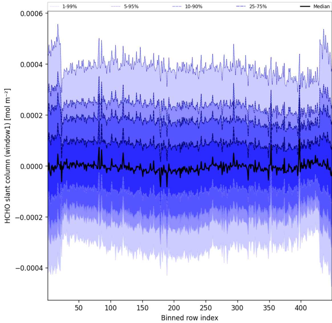
Figure 50: Along track statistics of “HCHO slant column (window1)” for 2025-10-30 to 2025-10-30
