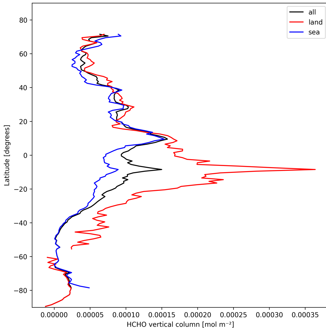
Figure 19: Zonal average of “HCHO vertical column” for 2025-10-30 to 2025-10-30.
