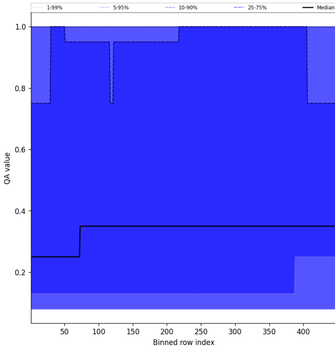
Figure 46: Along track statistics of “QA value” for 2025-10-30 to 2025-10-30
