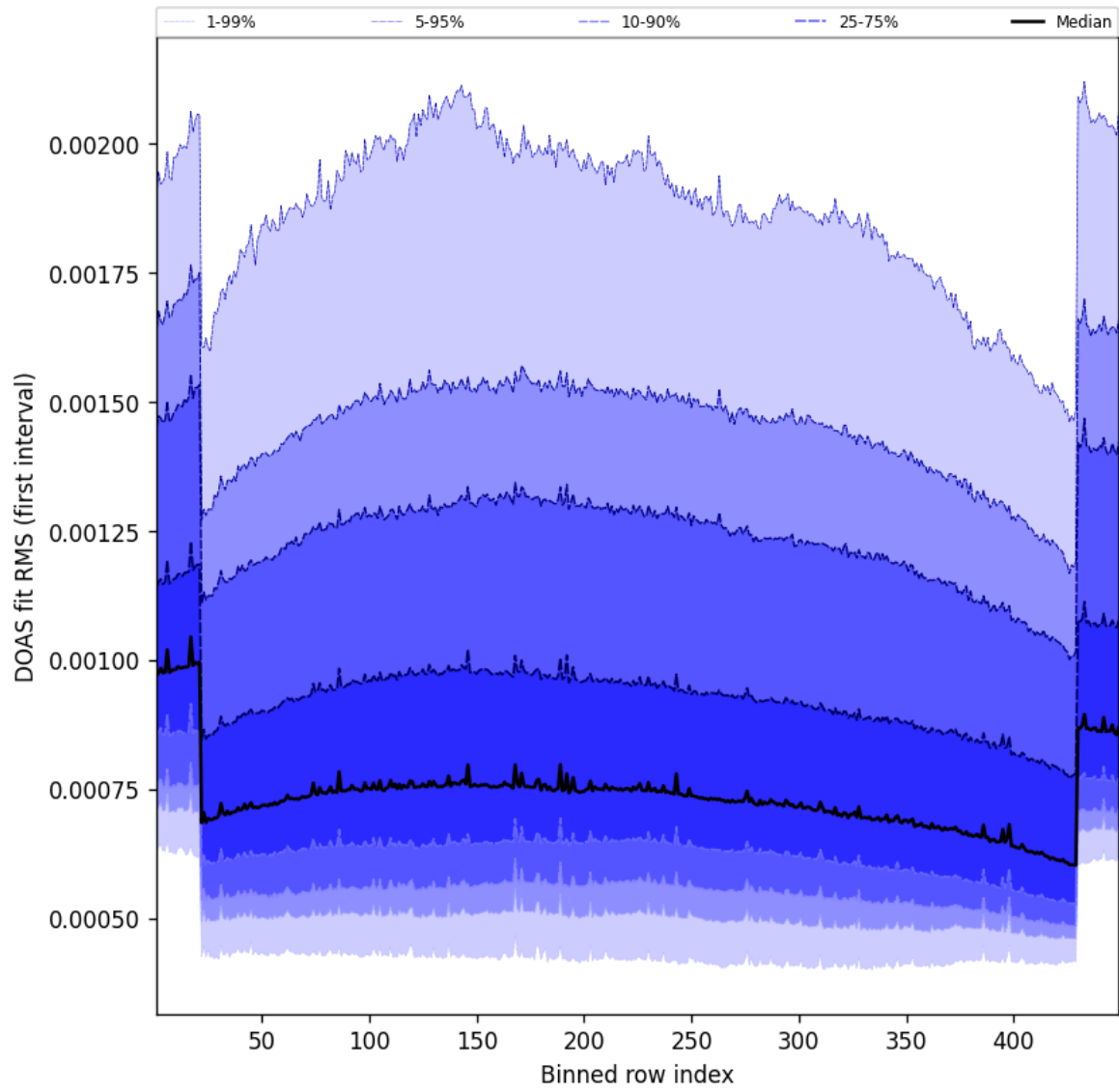
Figure 58: Along track statistics of “DOAS fit RMS (first interval)” for 2025-10-30 to 2025-10-30
