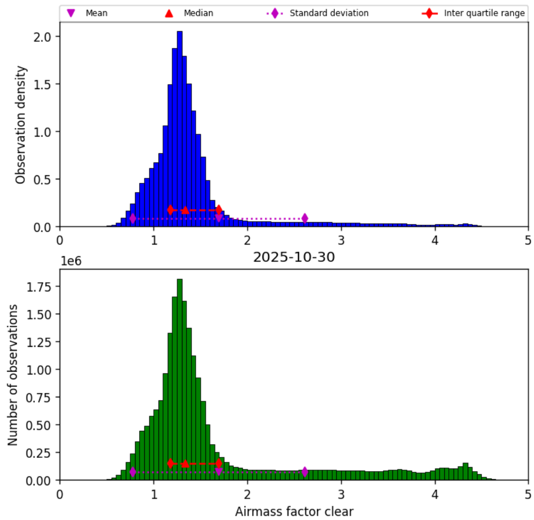
Figure 40: Histogram of “Airmass factor clear” for 2025-10-30 to 2025-10-30
