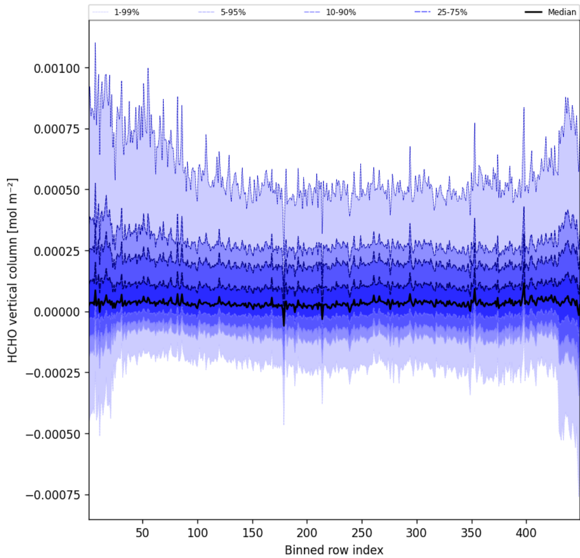
Figure 47: Along track statistics of “HCHO vertical column” for 2025-10-30 to 2025-10-30
