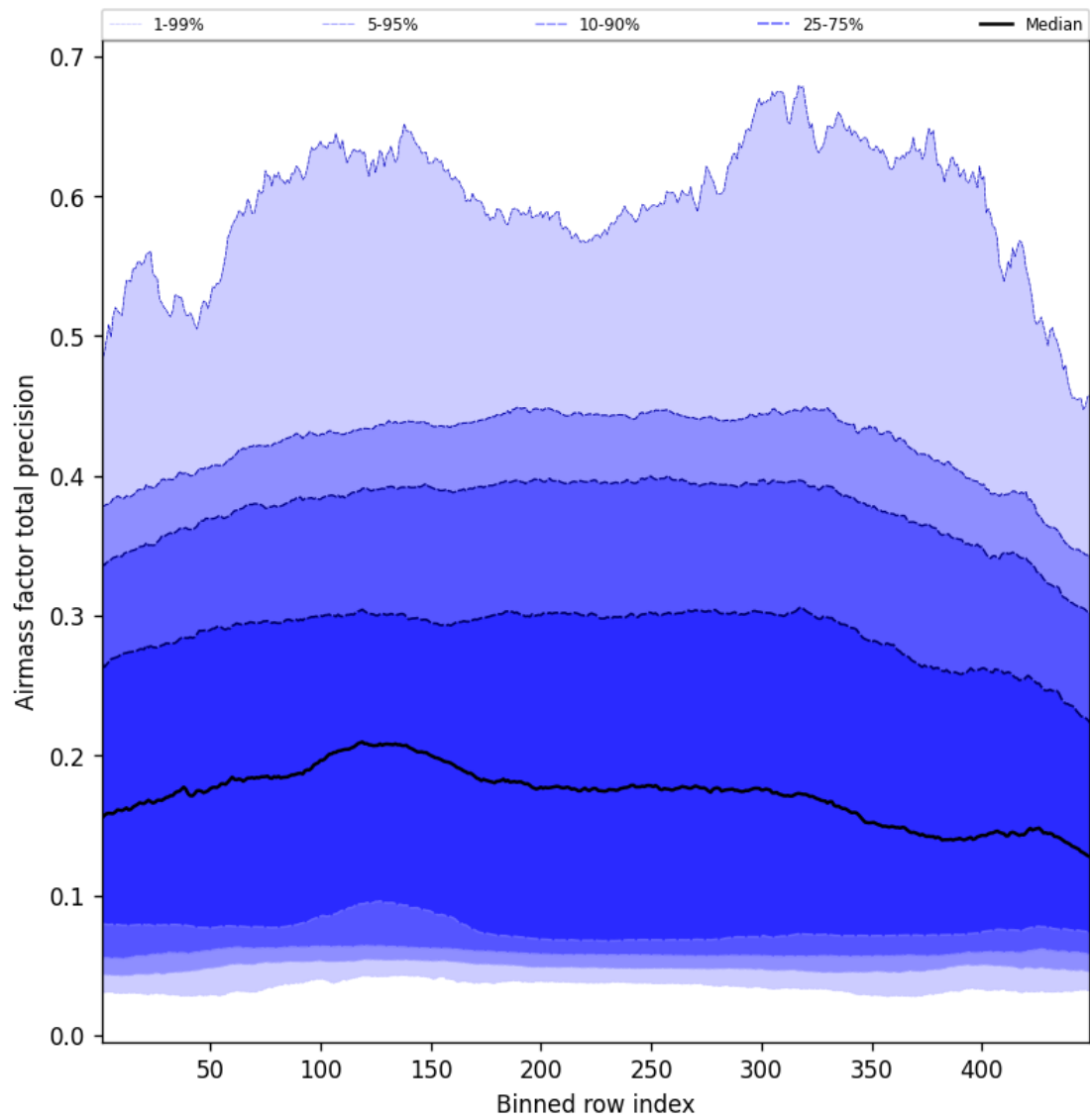
Figure 53: Along track statistics of “Airmass factor total precision” for 2025-10-30 to 2025-10-30
