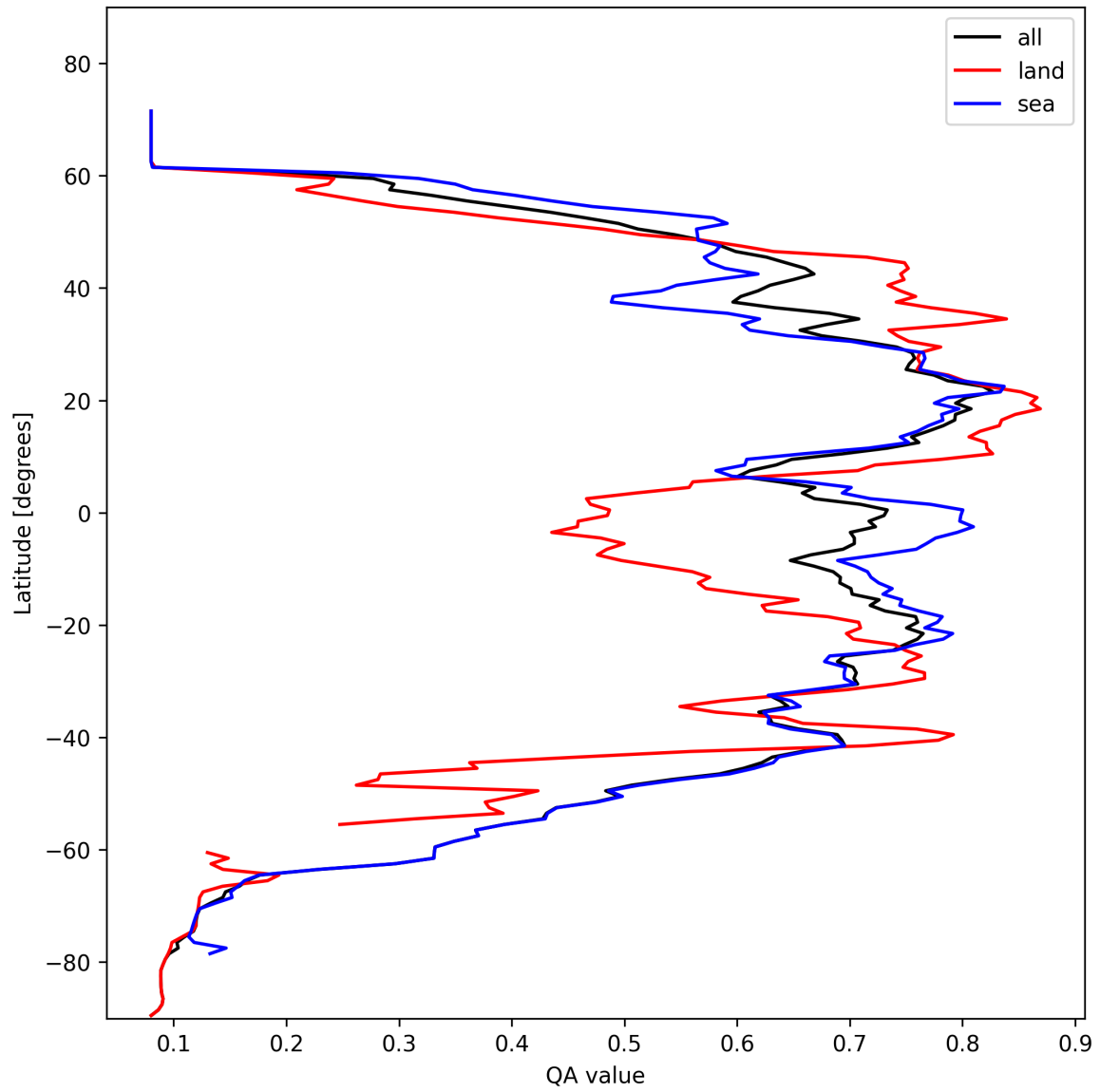
Figure 18: Zonal average of “QA value” for 2025-10-30 to 2025-10-30.
