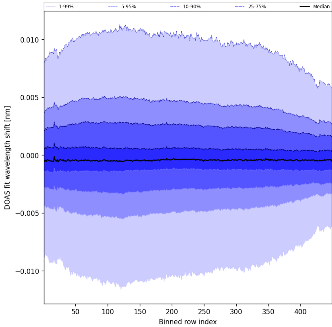
Figure 56: Along track statistics of “DOAS fit wavelength shift” for 2025-10-30 to 2025-10-30
