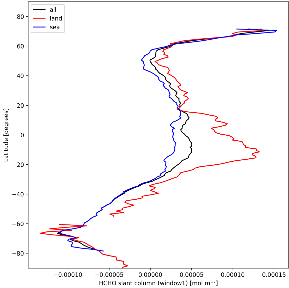
Figure 22: Zonal average of “HCHO slant column (window1)” for 2025-10-30 to 2025-10-30.
