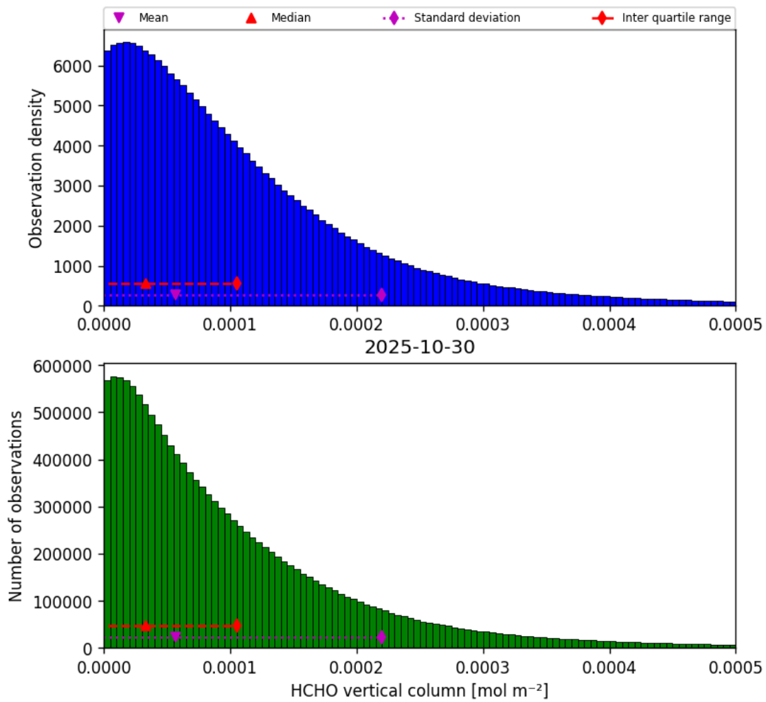
Figure 33: Histogram of “HCHO vertical column” for 2025-10-30 to 2025-10-30
