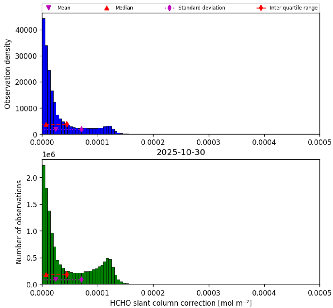
Figure 45: Histogram of “HCHO slant column correction” for 2025-10-30 to 2025-10-30
