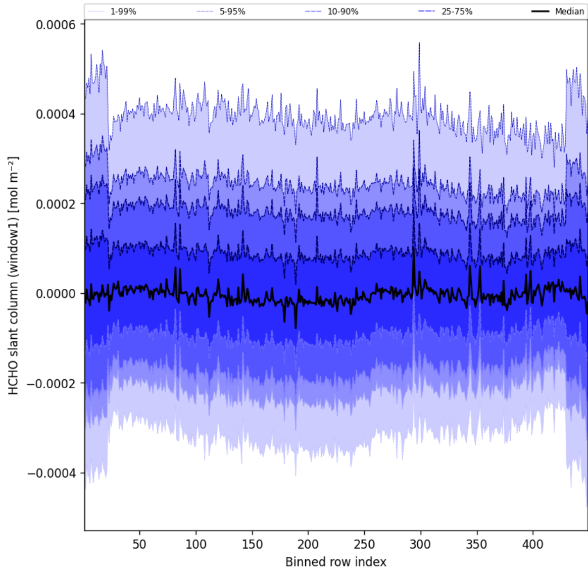
Figure 50: Along track statistics of “HCHO slant column (window1)” for 2025-10-31 to 2025-10-31
