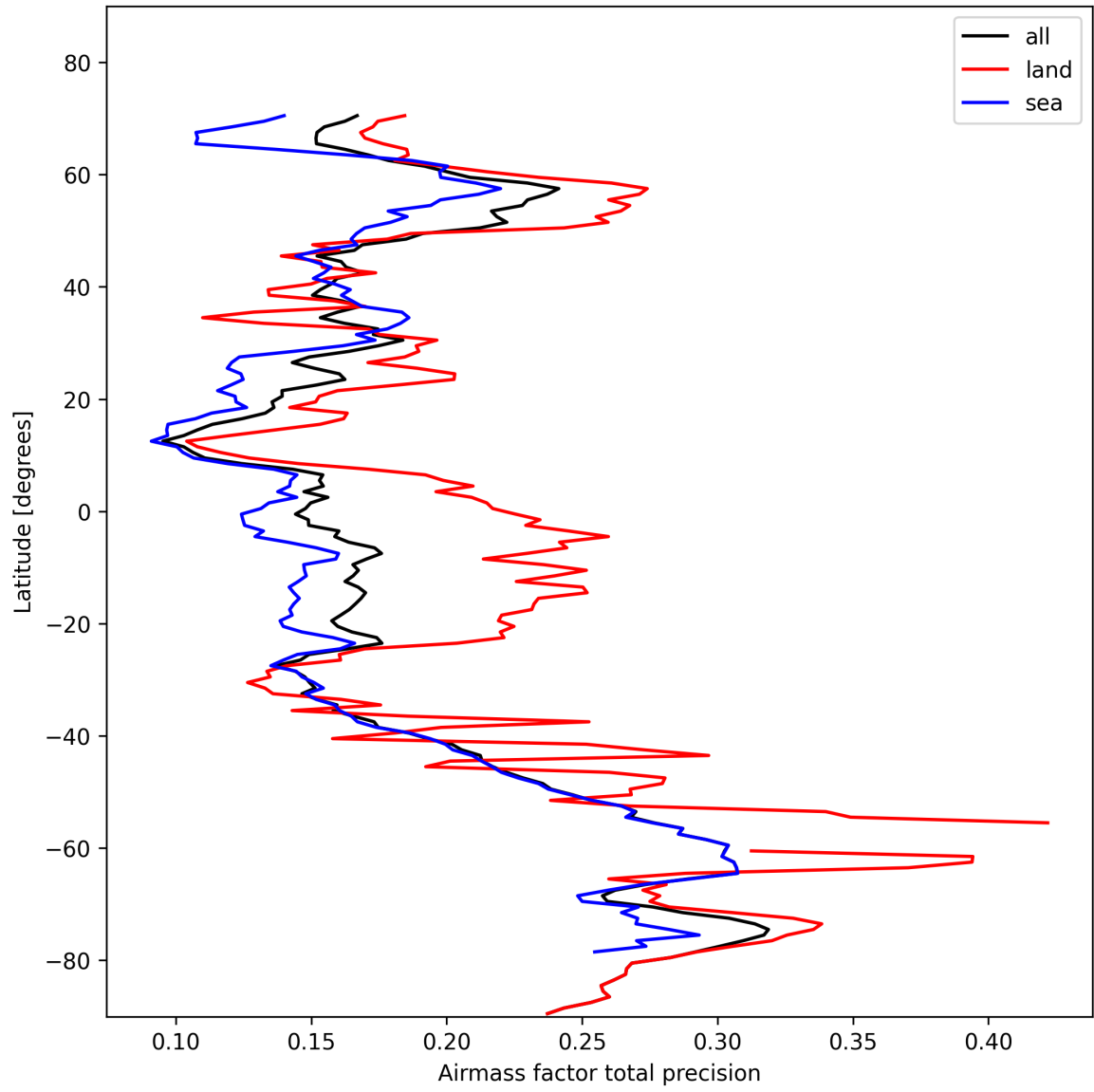
Figure 25: Zonal average of “Airmass factor total precision” for 2025-10-31 to 2025-10-31.
