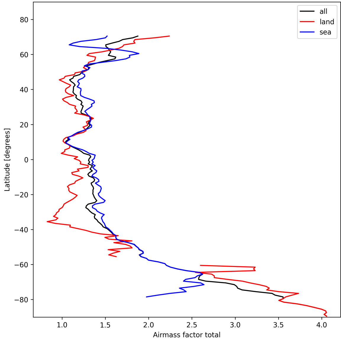
Figure 24: Zonal average of “Airmass factor total” for 2025-10-31 to 2025-10-31.
