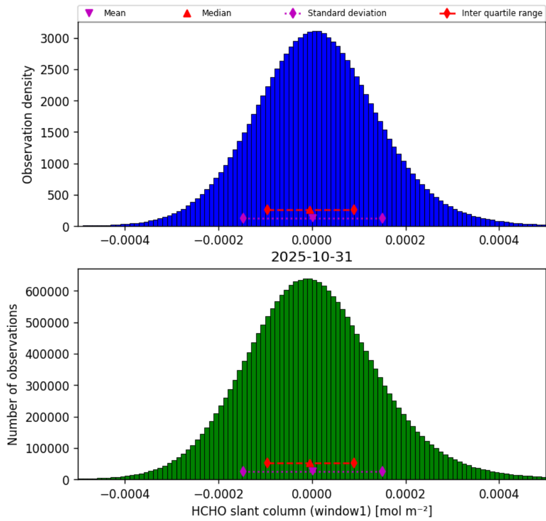
Figure 36: Histogram of “HCHO slant column (window1)” for 2025-10-31 to 2025-10-31
