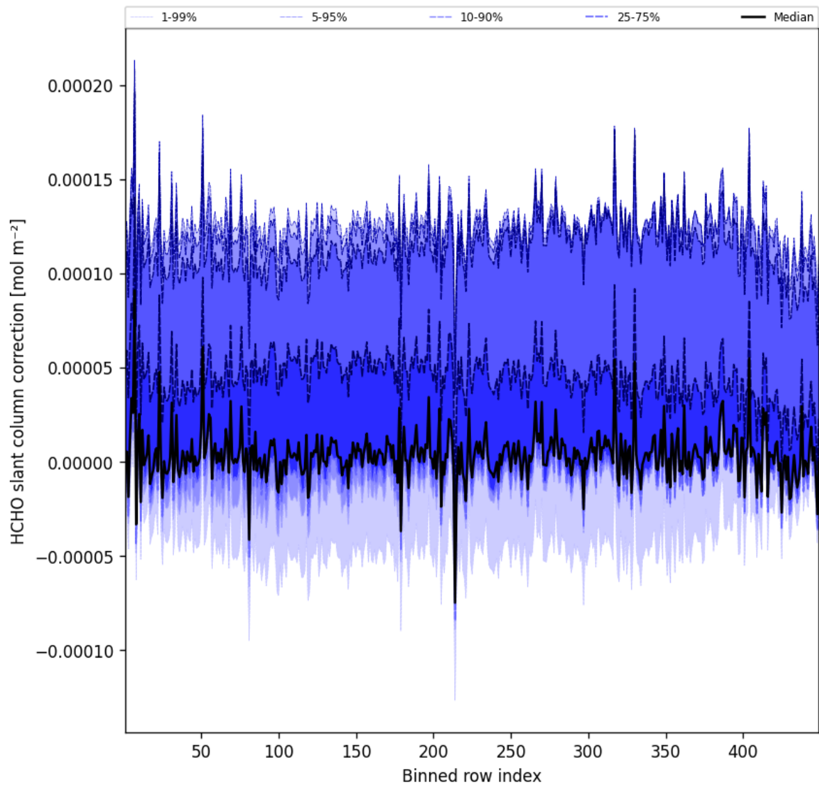
Figure 59: Along track statistics of “HCHO slant column correction” for 2025-10-31 to 2025-10-31
