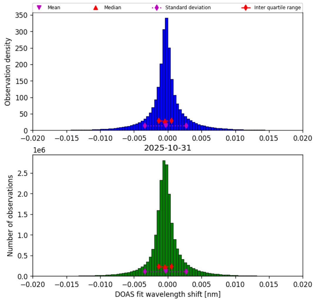
Figure 42: Histogram of “DOAS fit wavelength shift” for 2025-10-31 to 2025-10-31
