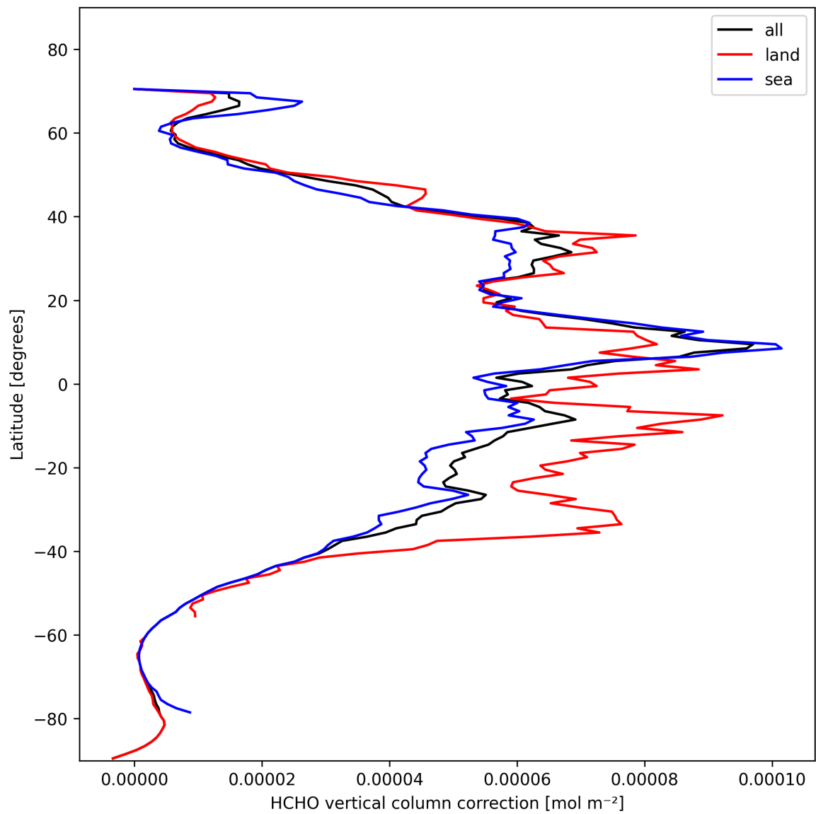
Figure 21: Zonal average of “HCHO vertical column correction” for 2025-10-31 to 2025-10-31.
