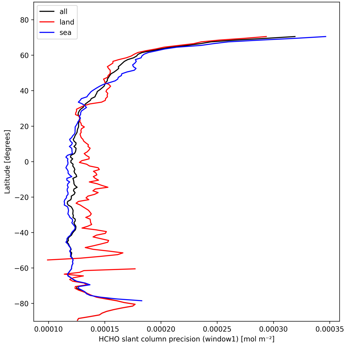
Figure 23: Zonal average of “HCHO slant column precision (window1)” for 2025-10-31 to 2025-10-31.
