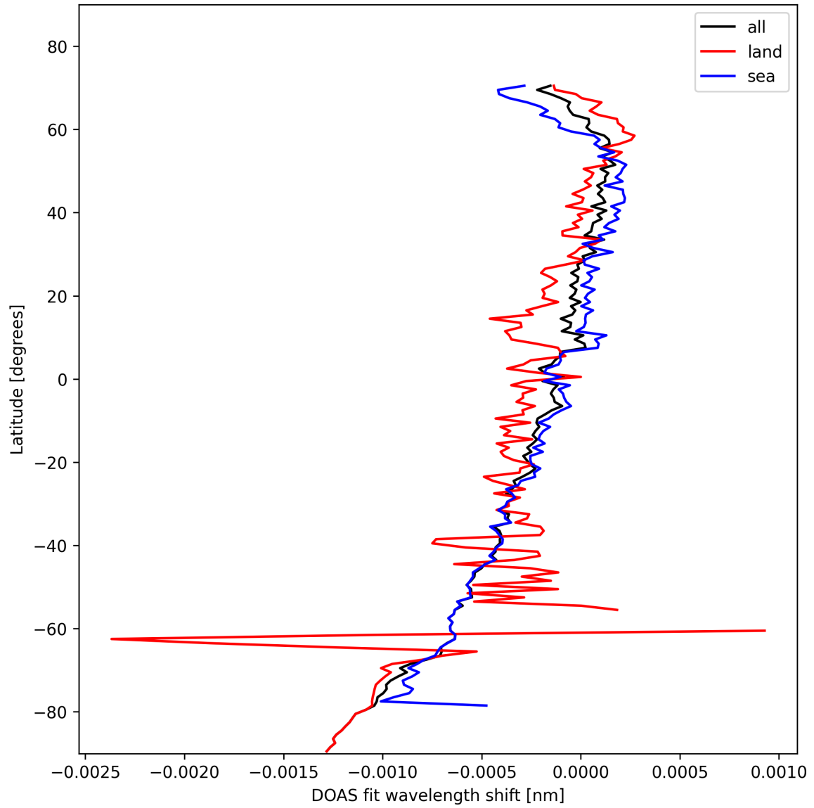
Figure 28: Zonal average of “DOAS fit wavelength shift” for 2025-10-31 to 2025-10-31.
