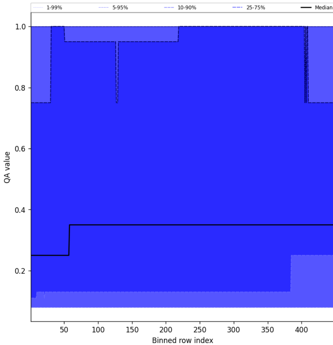
Figure 46: Along track statistics of “QA value” for 2025-10-31 to 2025-10-31
