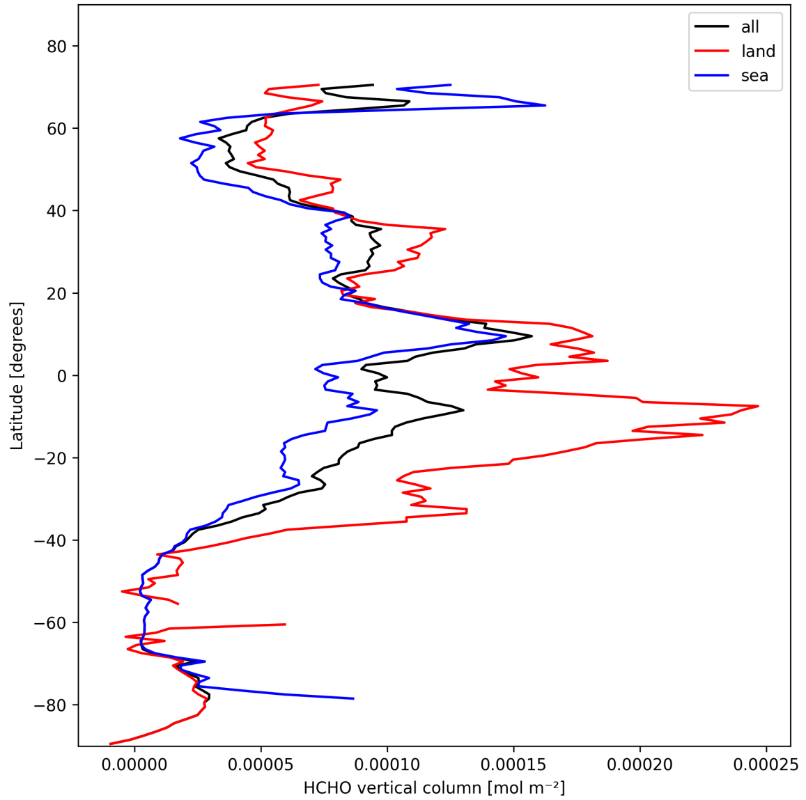
Figure 19: Zonal average of “HCHO vertical column” for 2025-10-31 to 2025-10-31.
