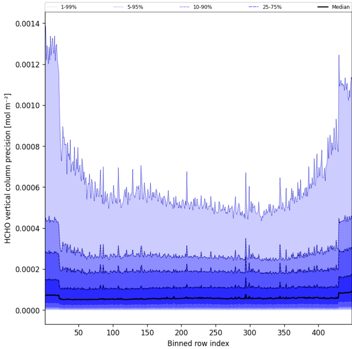
Figure 48: Along track statistics of “HCHO vertical column precision” for 2025-10-31 to 2025-10-31
