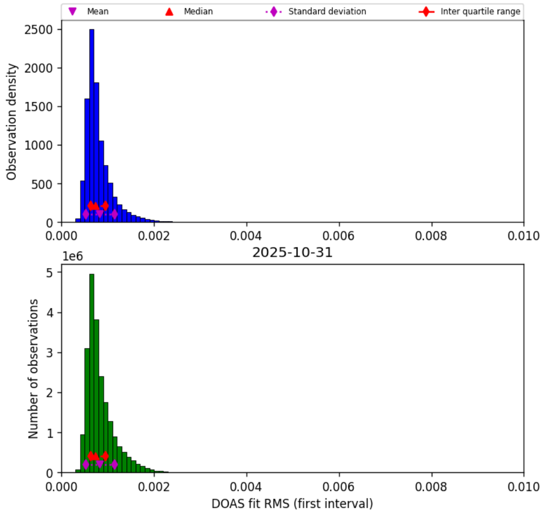
Figure 44: Histogram of “DOAS fit RMS (first interval)” for 2025-10-31 to 2025-10-31
