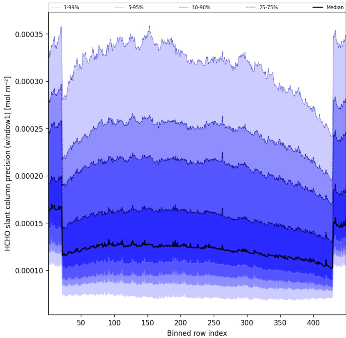
Figure 51: Along track statistics of “HCHO slant column precision (window1)” for 2025-10-31 to 2025-10-31
