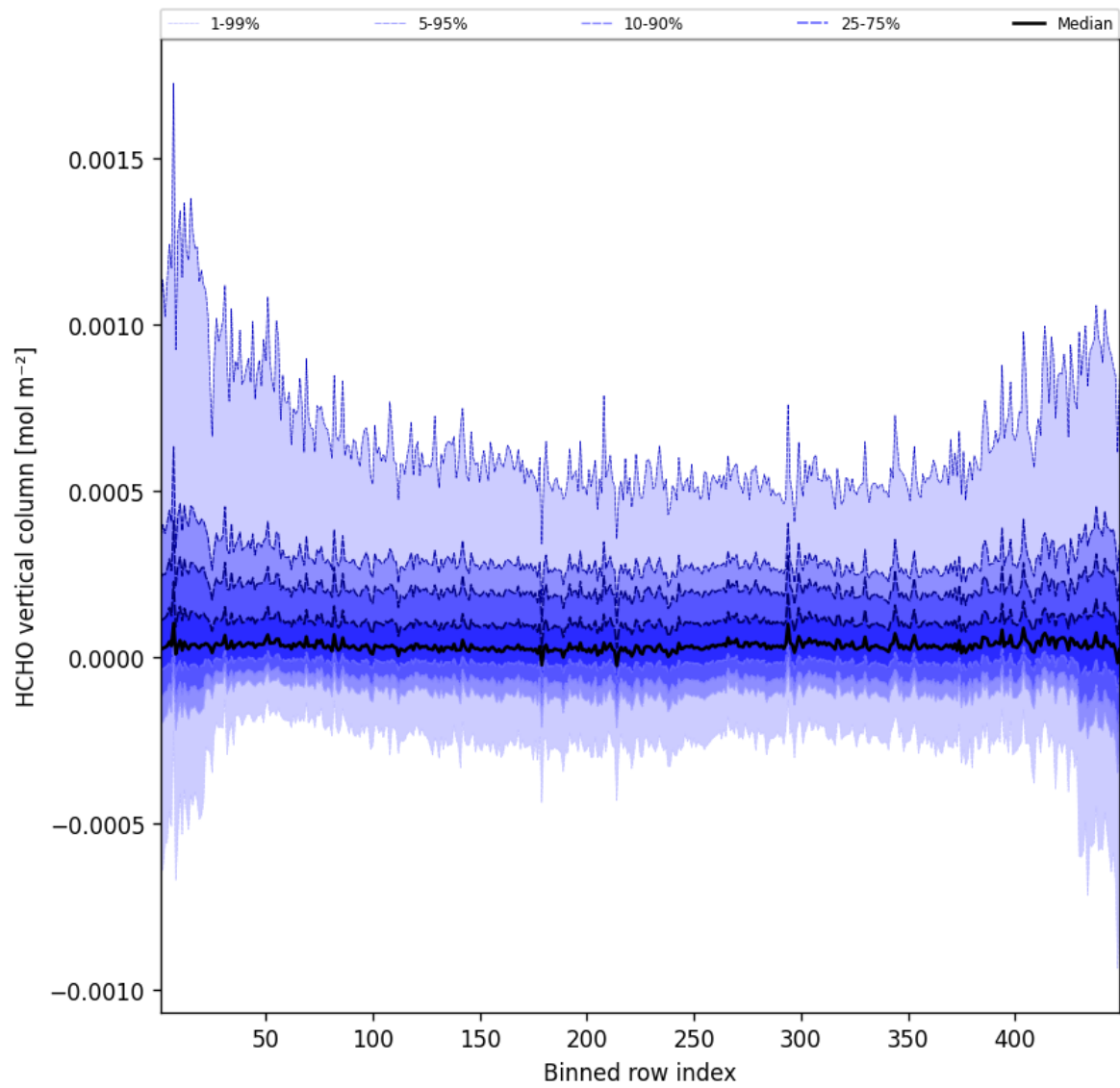
Figure 47: Along track statistics of “HCHO vertical column” for 2025-10-31 to 2025-10-31
