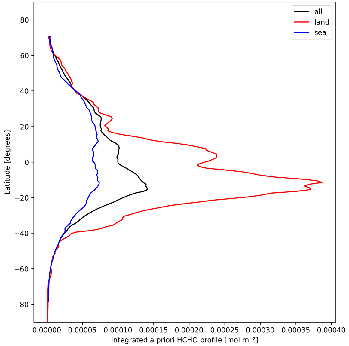
Figure 27: Zonal average of “Integrated a priori HCHO profile” for 2025-10-31 to 2025-10-31.
