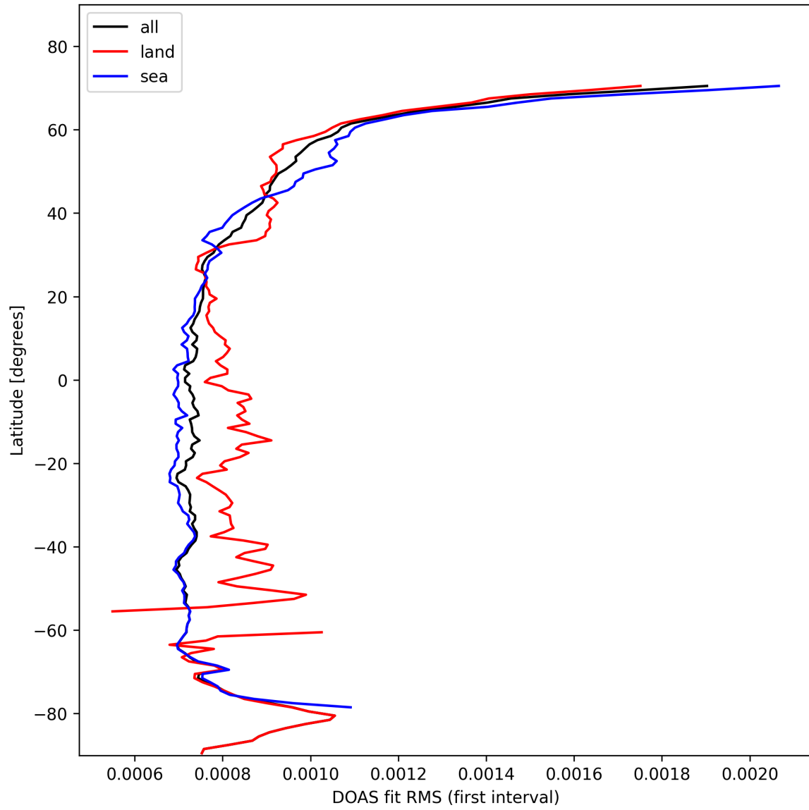
Figure 30: Zonal average of “DOAS fit RMS (first interval)” for 2025-10-31 to 2025-10-31.
