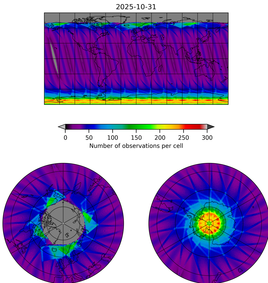
Figure 17: Map of the number of observations for 2025-10-31 to 2025-10-31
