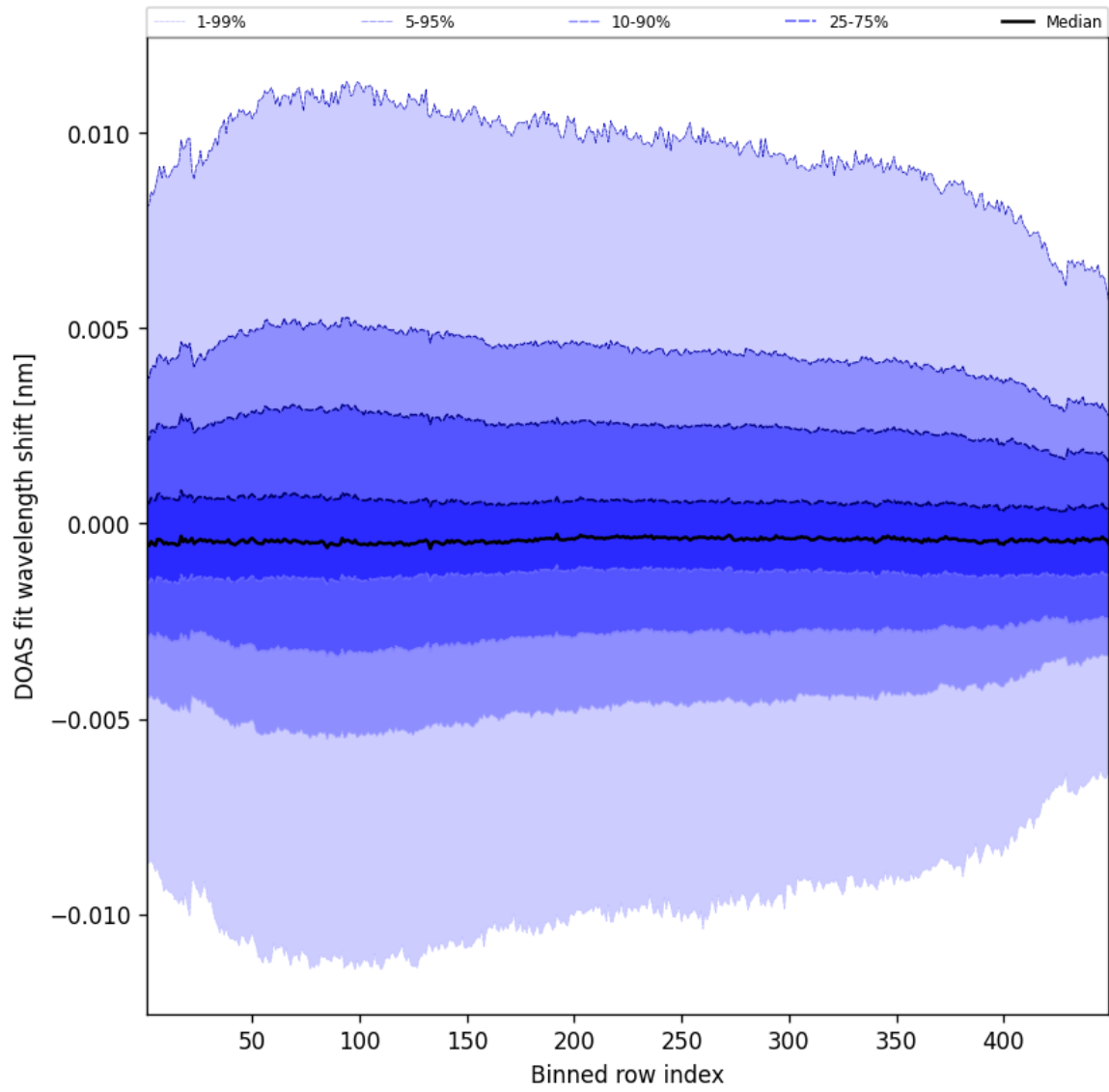
Figure 56: Along track statistics of “DOAS fit wavelength shift” for 2025-10-31 to 2025-10-31
