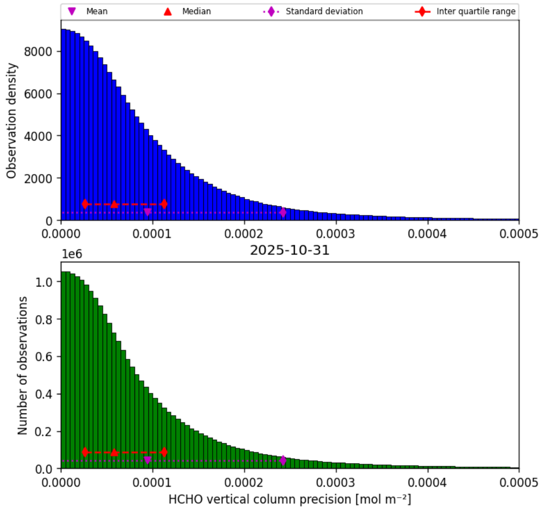
Figure 34: Histogram of “HCHO vertical column precision” for 2025-10-31 to 2025-10-31
