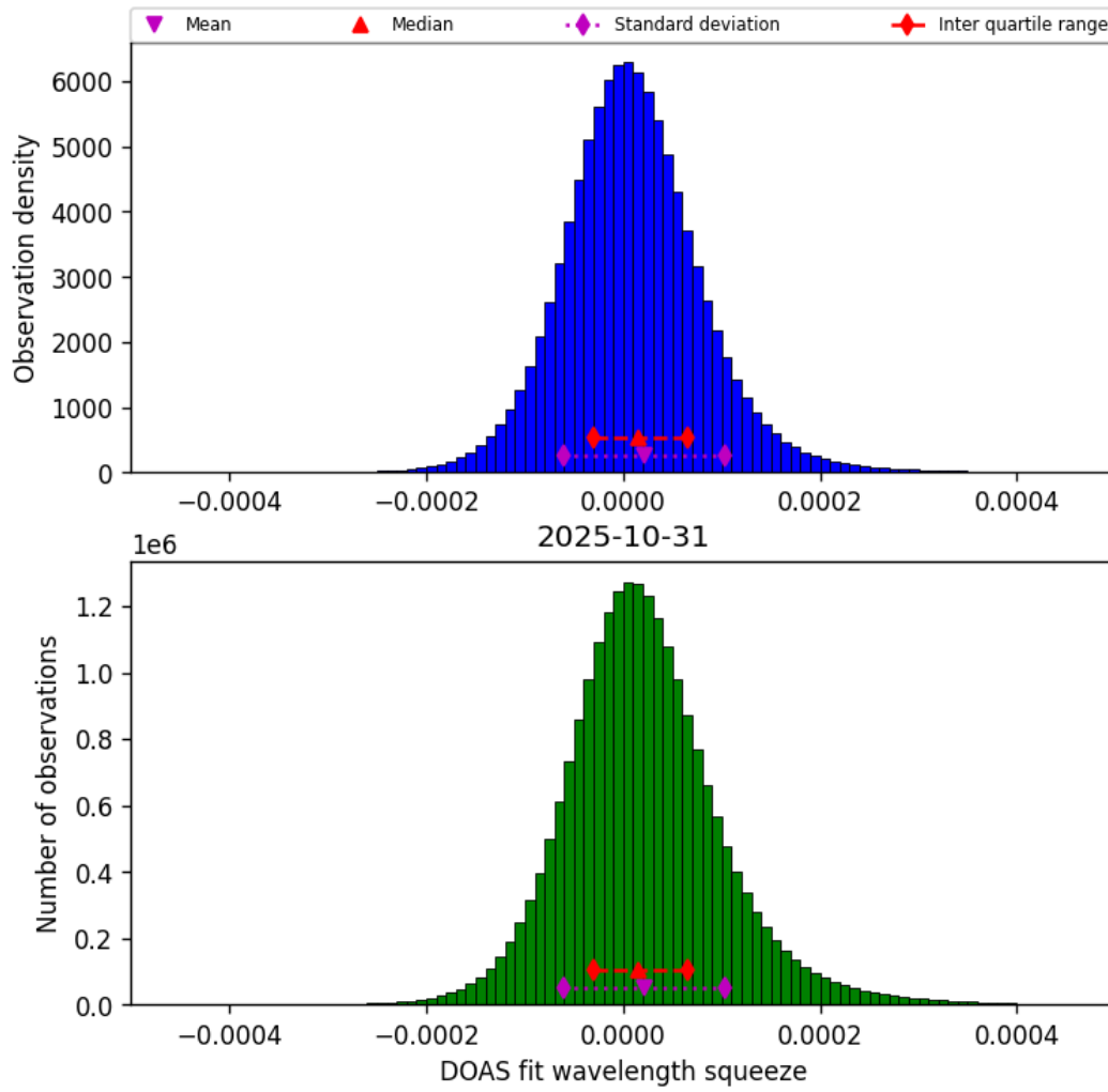
Figure 43: Histogram of “DOAS fit wavelength squeeze” for 2025-10-31 to 2025-10-31
