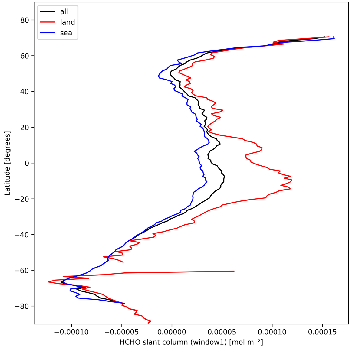
Figure 22: Zonal average of “HCHO slant column (window1)” for 2025-10-31 to 2025-10-31.
