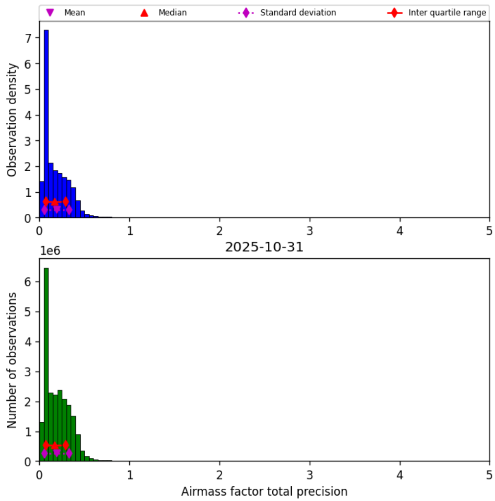
Figure 39: Histogram of “Airmass factor total precision” for 2025-10-31 to 2025-10-31
