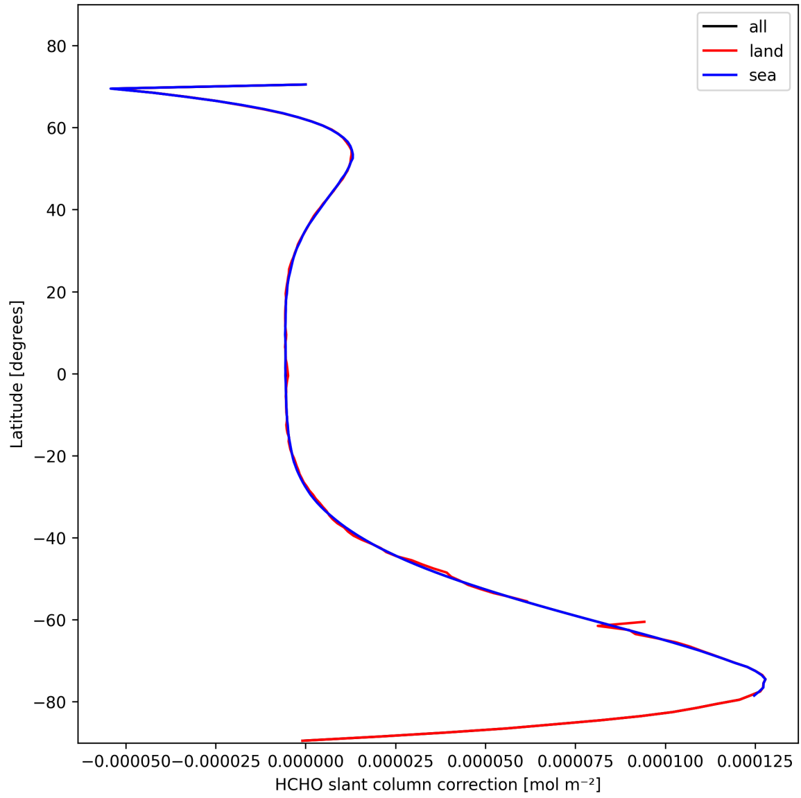
Figure 31: Zonal average of “HCHO slant column correction” for 2025-10-31 to 2025-10-31.
