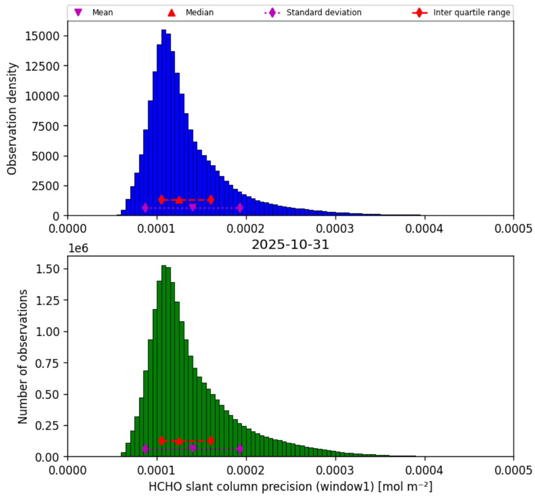
Figure 37: Histogram of “HCHO slant column precision (window1)” for 2025-10-31 to 2025-10-31
