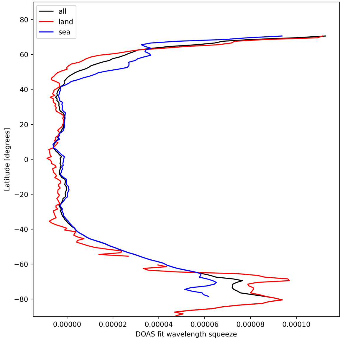
Figure 29: Zonal average of “DOAS fit wavelength squeeze” for 2025-10-31 to 2025-10-31.
