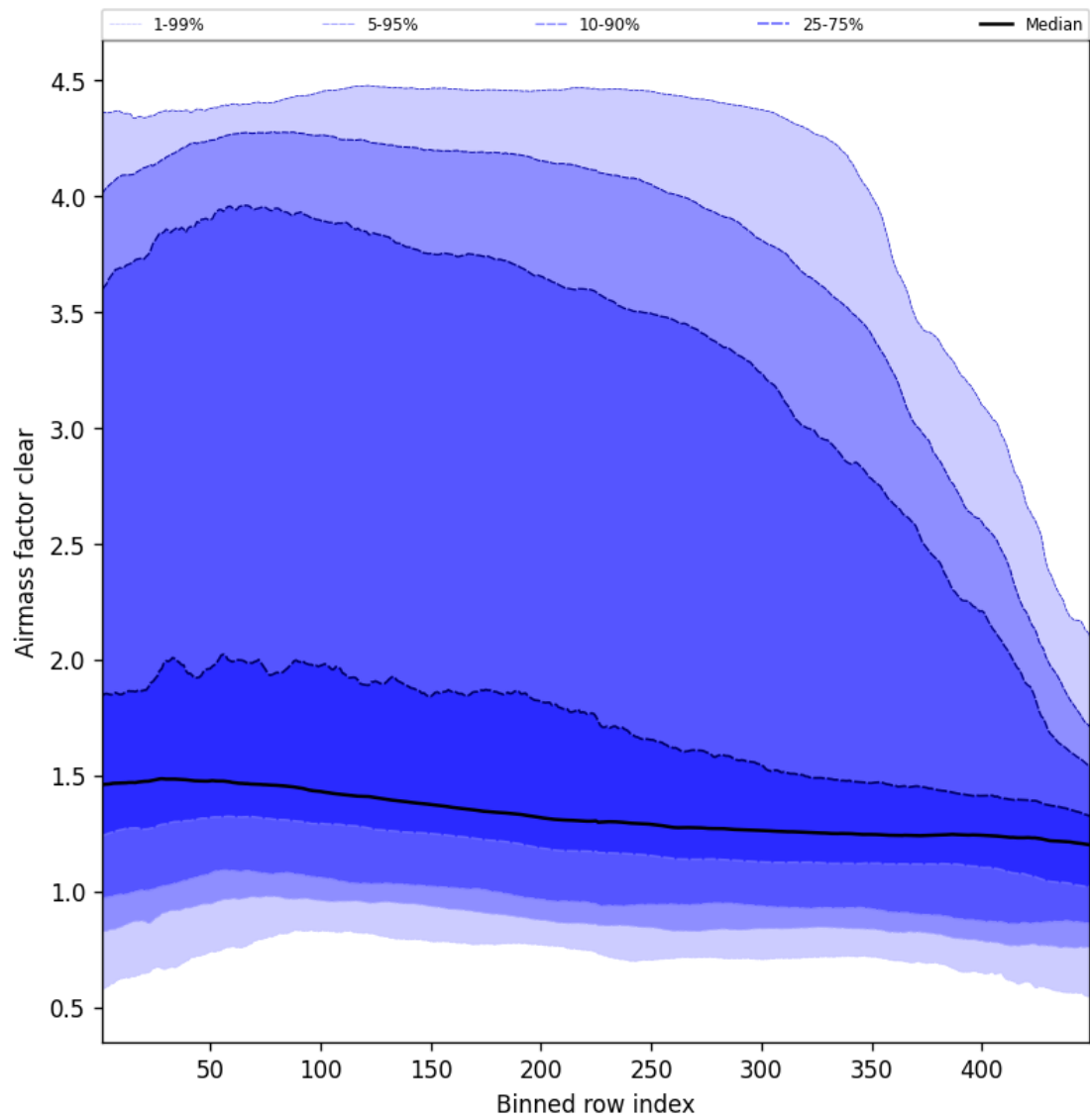
Figure 54: Along track statistics of “Air mass factor clear” for 2025-10-31 to 2025-10-31
