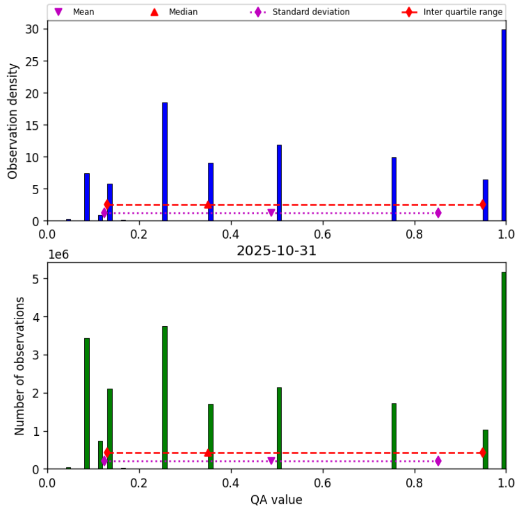
Figure 32: Histogram of “QA value” for 2025-10-31 to 2025-10-31
