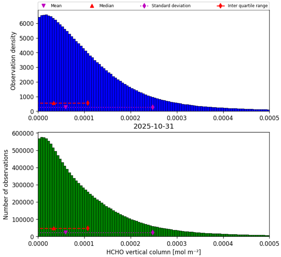
Figure 33: Histogram of “HCHO vertical column” for 2025-10-31 to 2025-10-31
