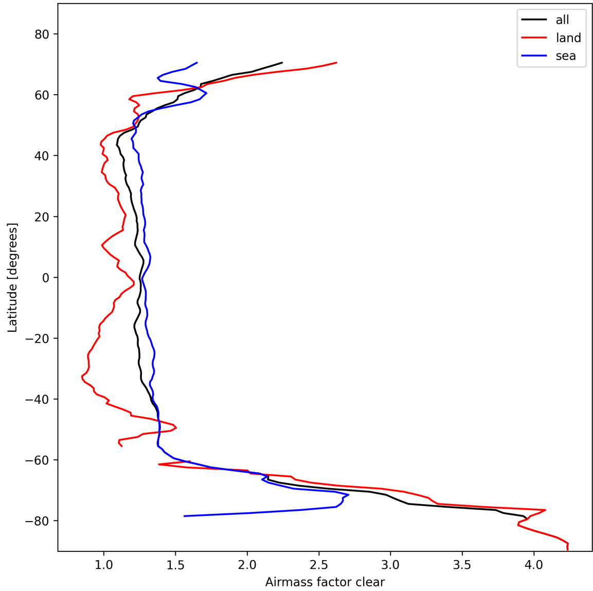
Figure 26: Zonal average of “Airmass factor clear” for 2025-10-31 to 2025-10-31.
