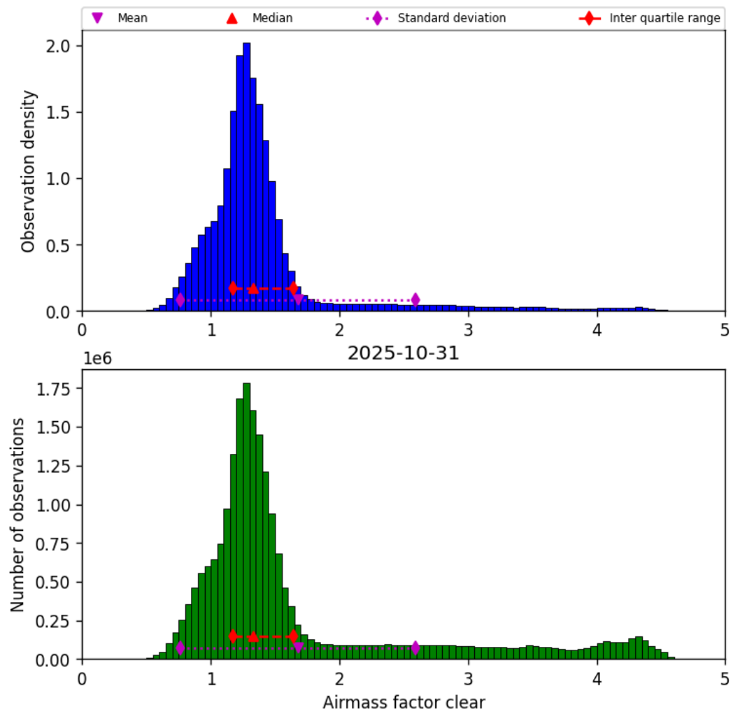
Figure 40: Histogram of “Airmass factor clear” for 2025-10-31 to 2025-10-31
