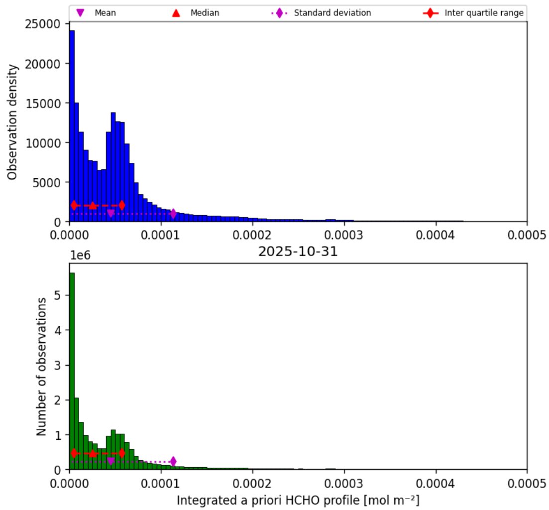
Figure 41: Histogram of “Integrated a priori HCHO profile” for 2025-10-31 to 2025-10-31
