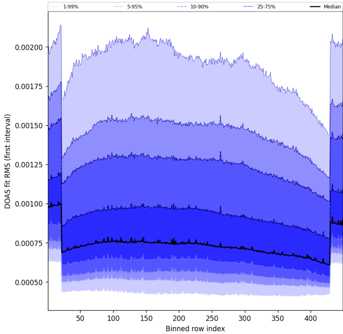
Figure 58: Along track statistics of “DOAS fit RMS (first interval)” for 2025-10-31 to 2025-10-31
