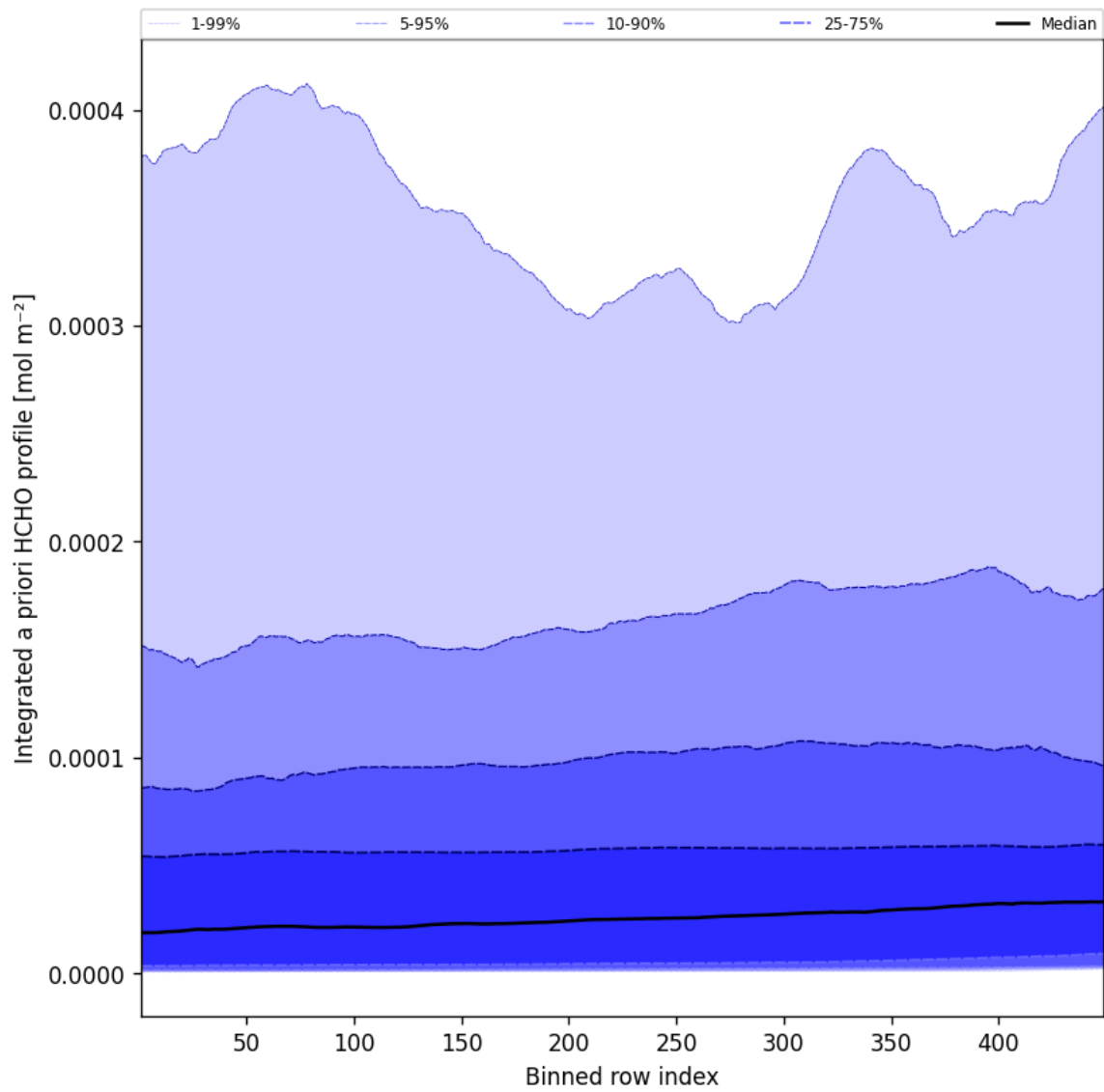
Figure 55: Along track statistics of "Integrated a priori HCHO profile" for 2025-10-31 to 2025-10-31
