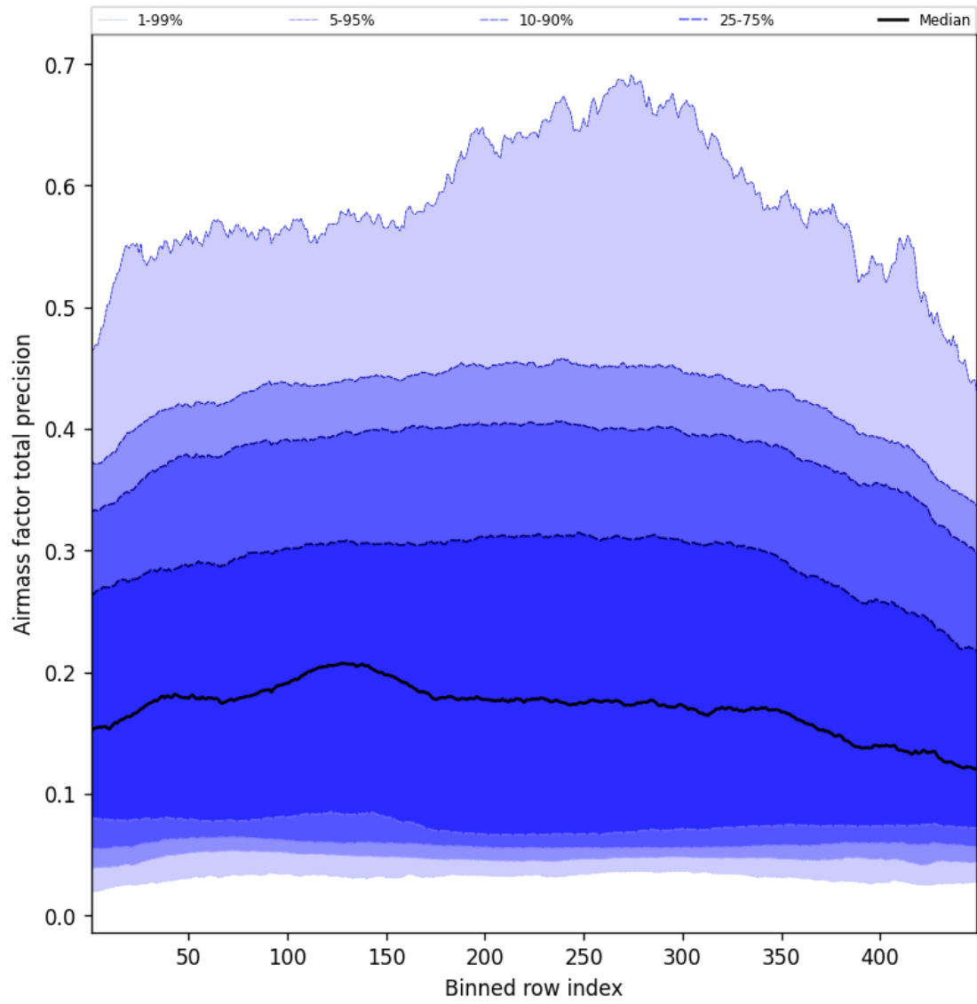
Figure 53: Along track statistics of “Airmass factor total precision” for 2025-10-31 to 2025-10-31
