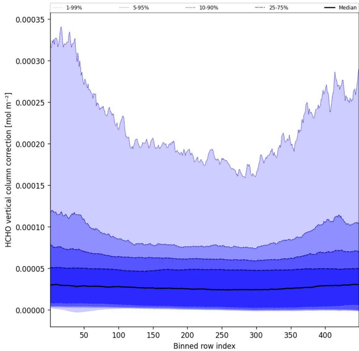
Figure 49: Along track statistics of “HCHO vertical column correction” for 2025-10-31 to 2025-10-31
