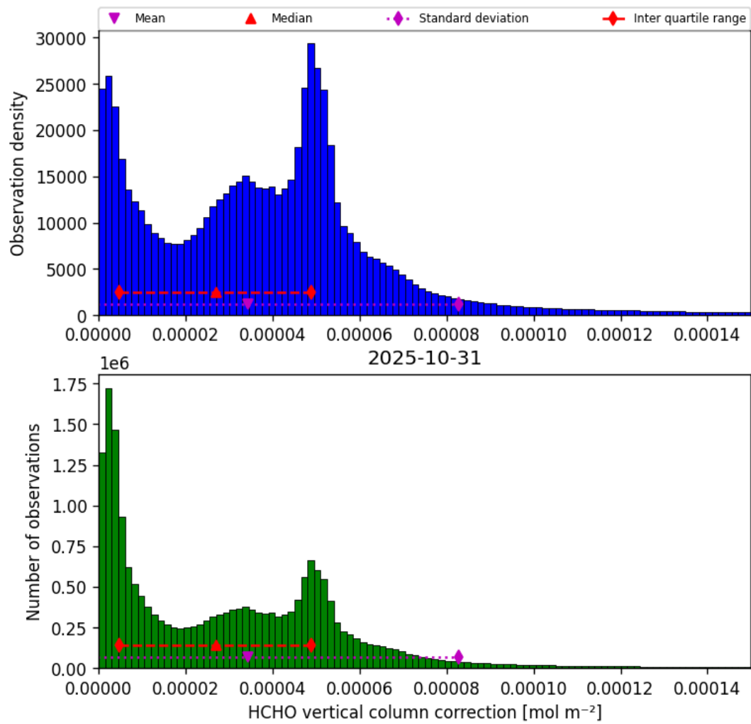
Figure 35: Histogram of “HCHO vertical column correction” for 2025-10-31 to 2025-10-31
