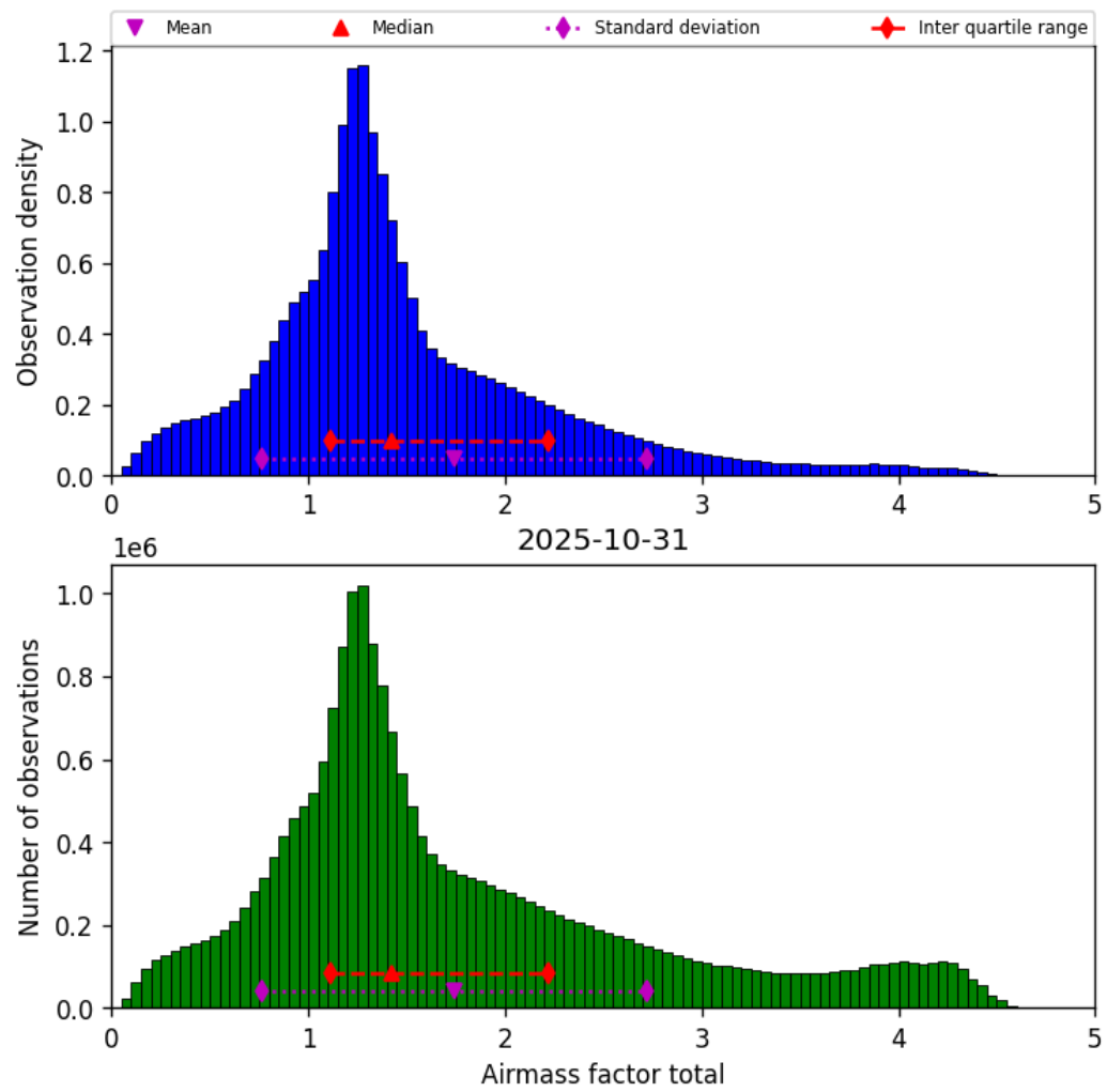
Figure 38: Histogram of “Airmass factor total” for 2025-10-31 to 2025-10-31
