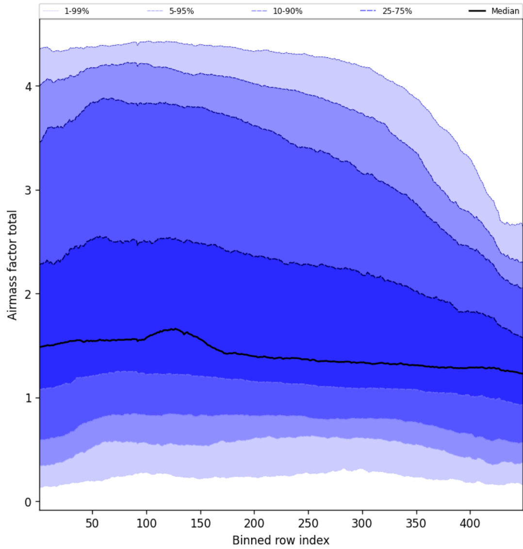
Figure 52: Along track statistics of “Airmass factor total” for 2025-10-31 to 2025-10-31
