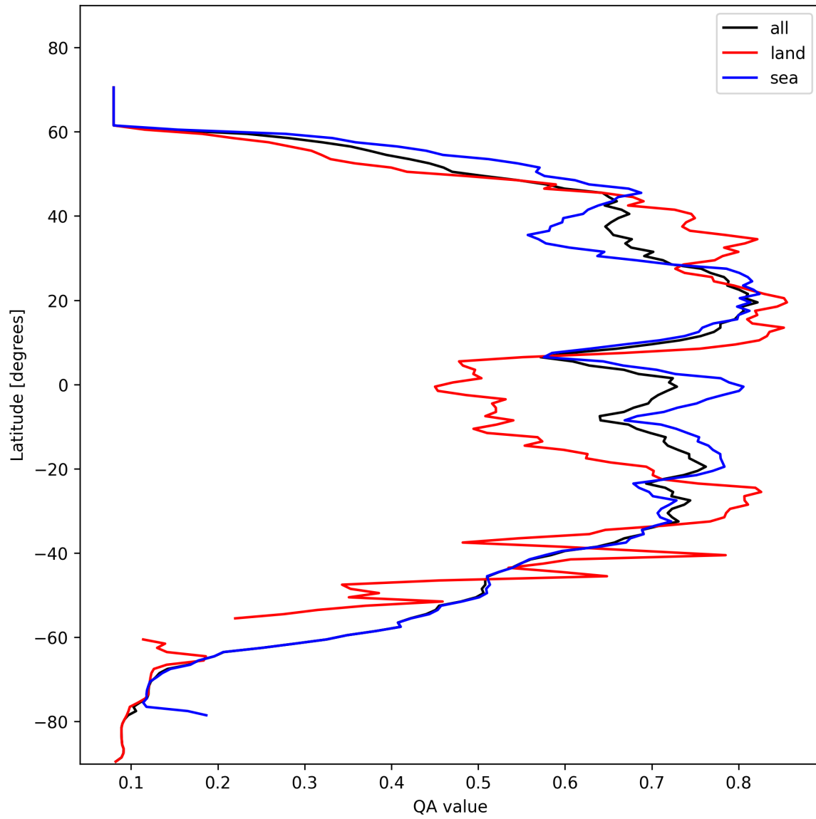
Figure 18: Zonal average of “QA value” for 2025-10-31 to 2025-10-31.
