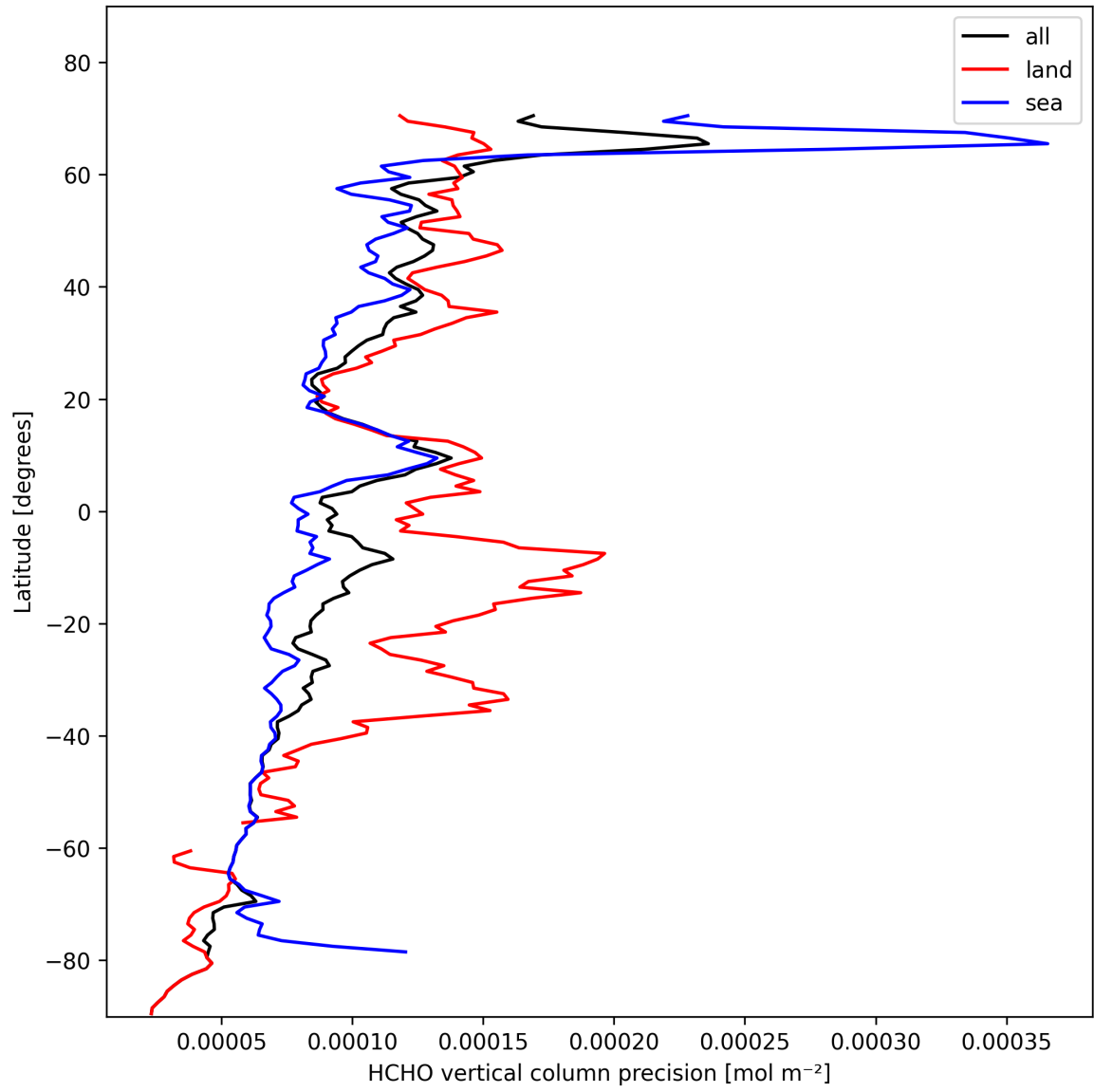
Figure 20: Zonal average of “HCHO vertical column precision” for 2025-10-31 to 2025-10-31.
