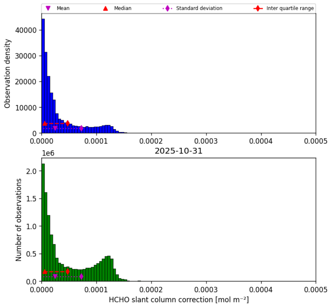
Figure 45: Histogram of “HCHO slant column correction” for 2025-10-31 to 2025-10-31
