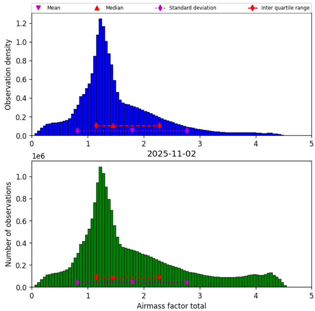
Figure 38: Histogram of “Airmass factor total” for 2025-11-02 to 2025-11-03
