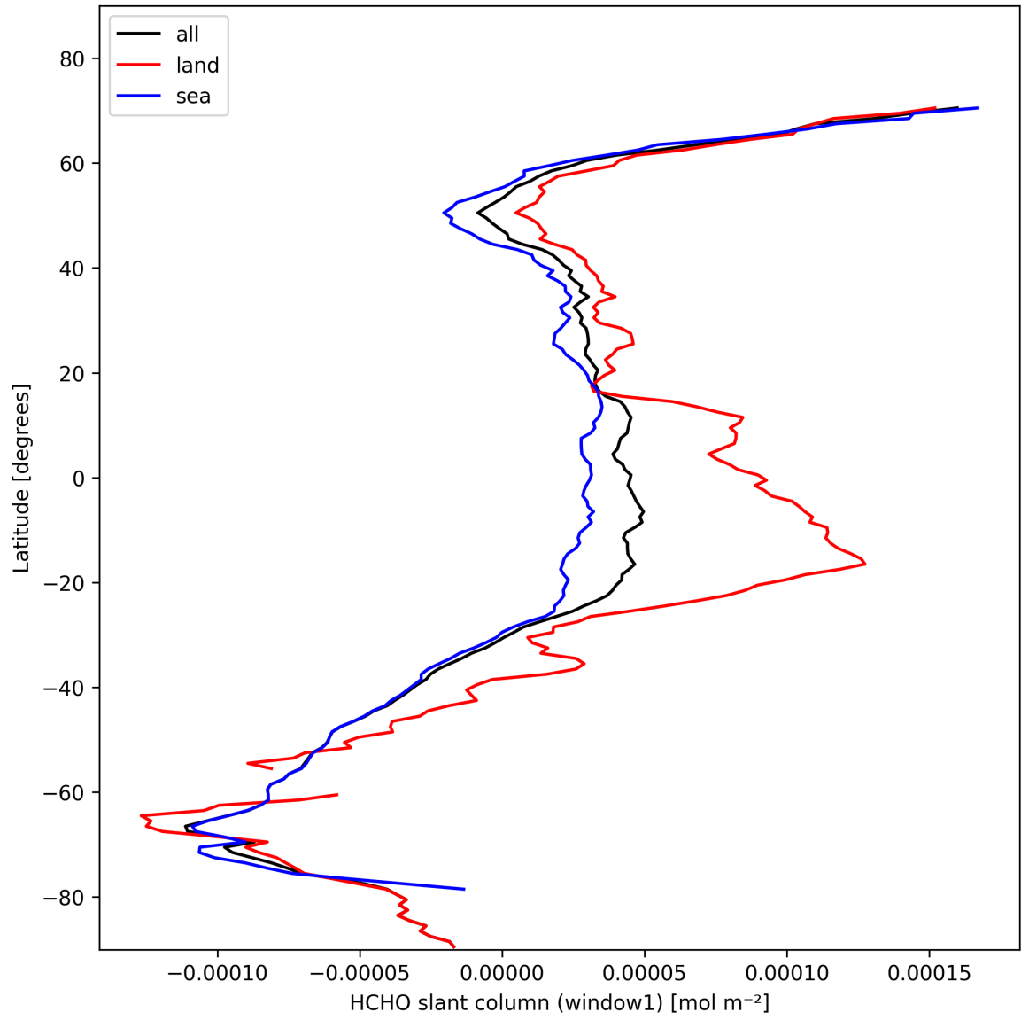
Figure 22: Zonal average of “HCHO slant column (window1)” for 2025-11-02 to 2025-11-03.
