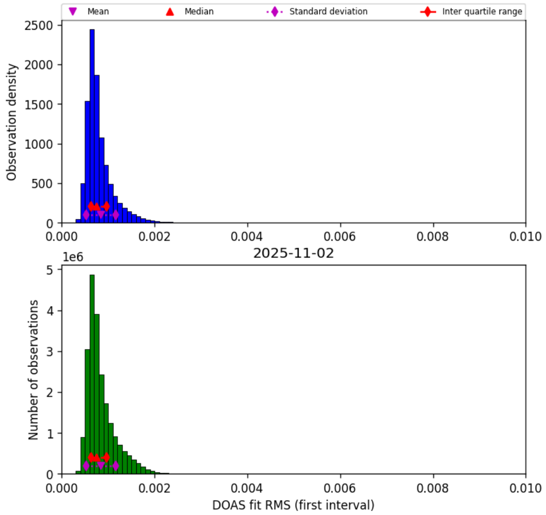
Figure 44: Histogram of “DOAS fit RMS (first interval)” for 2025-11-02 to 2025-11-03
