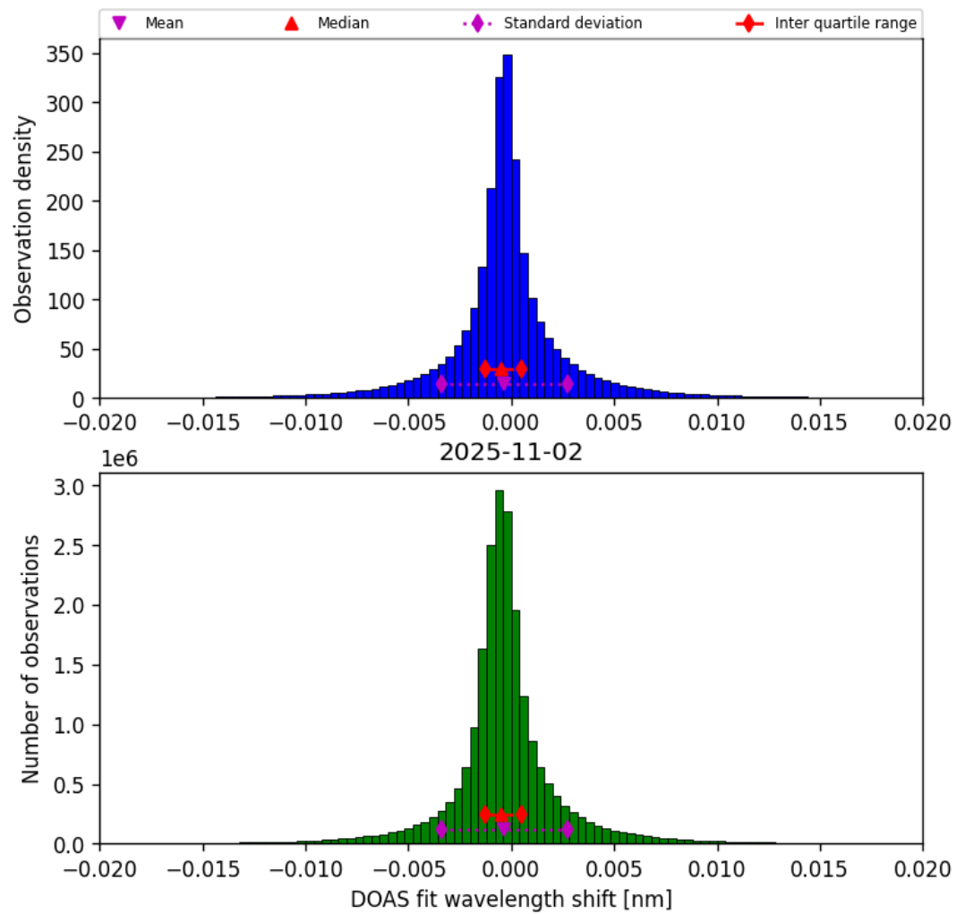
Figure 42: Histogram of “DOAS fit wavelength shift” for 2025-11-02 to 2025-11-03
