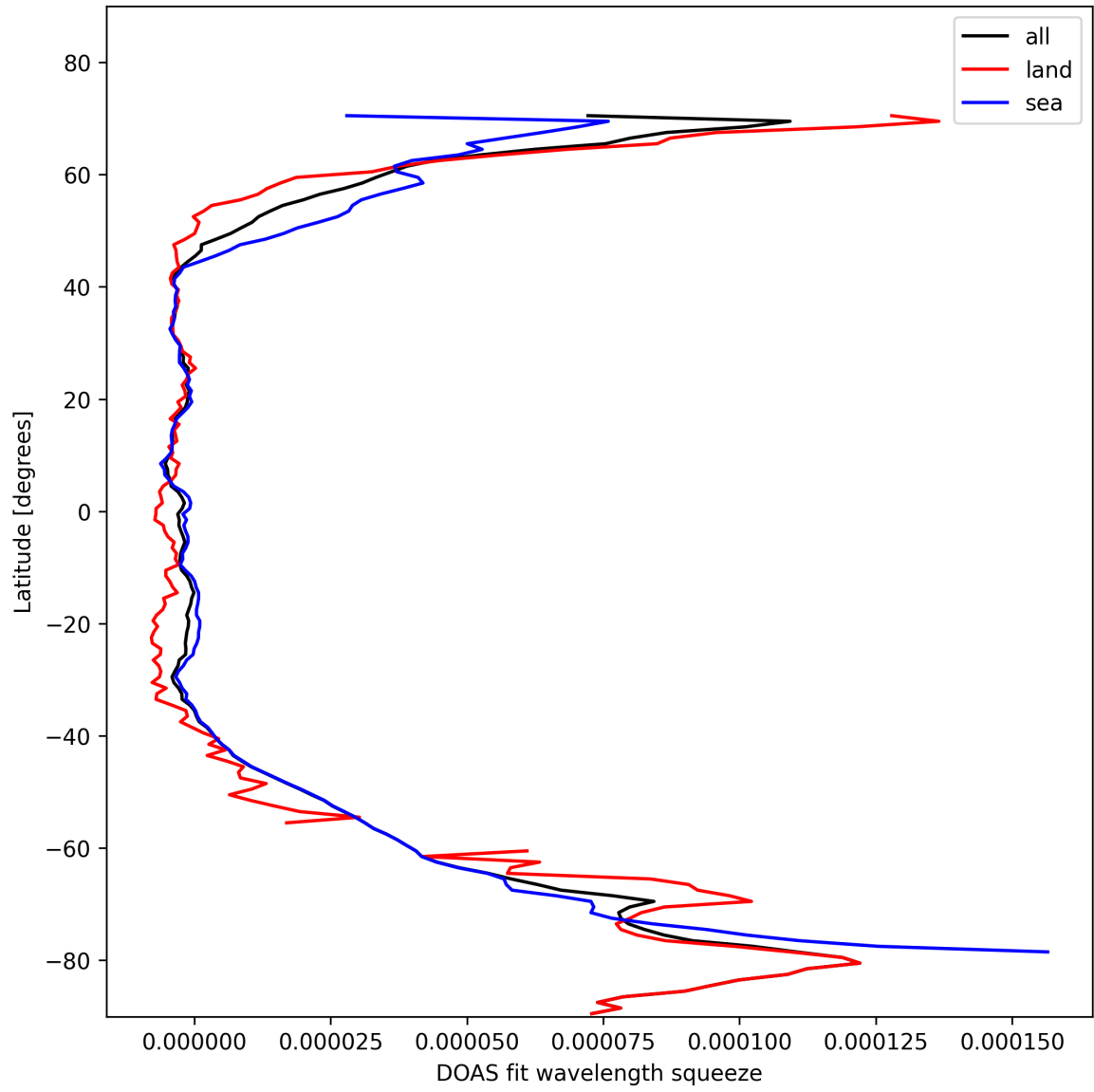
Figure 29: Zonal average of “DOAS fit wavelength squeeze” for 2025-11-02 to 2025-11-03.
