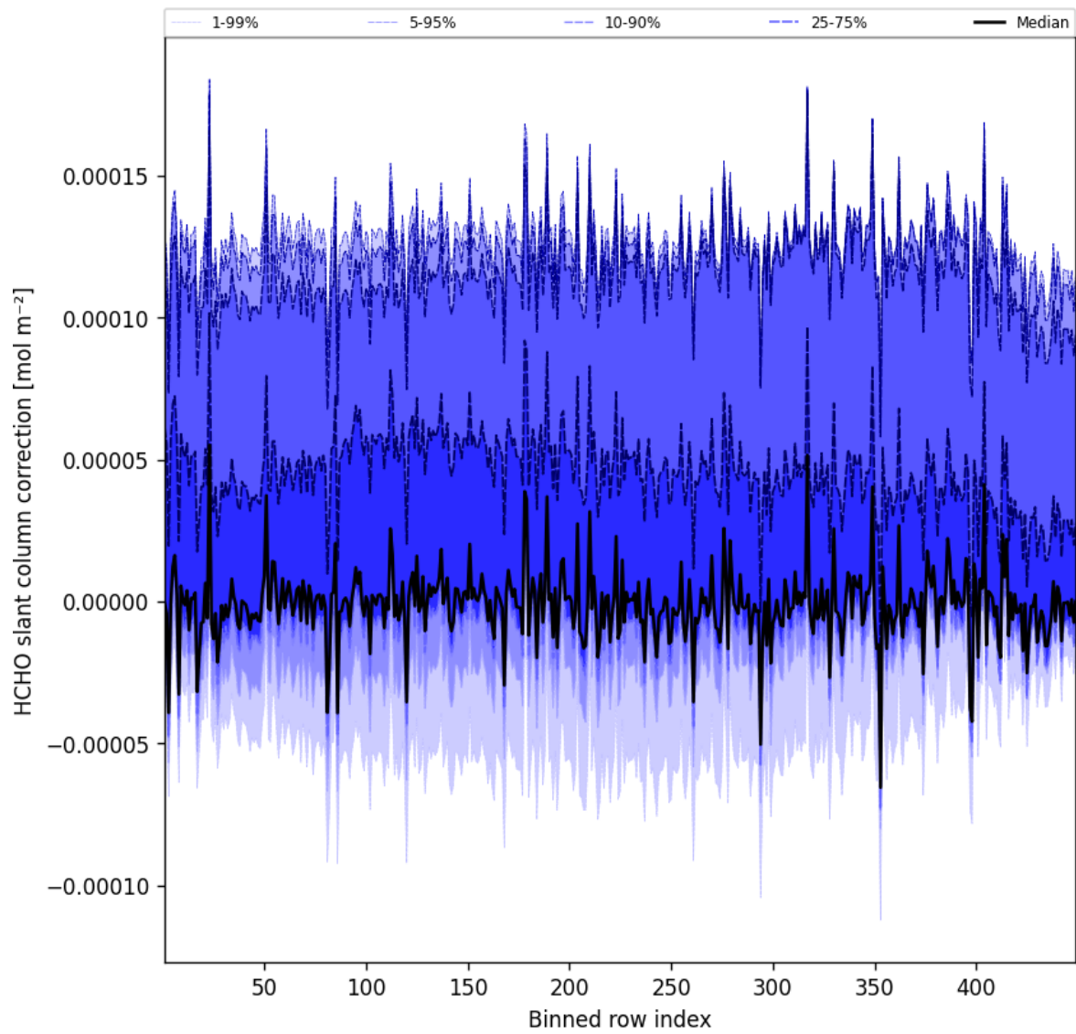
Figure 59: Along track statistics of “HCHO slant column correction” for 2025-11-02 to 2025-11-03
