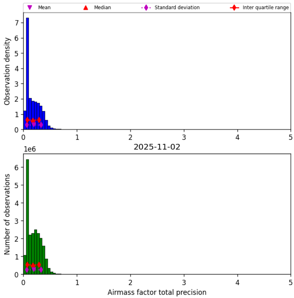
Figure 39: Histogram of “Airmass factor total precision” for 2025-11-02 to 2025-11-03
