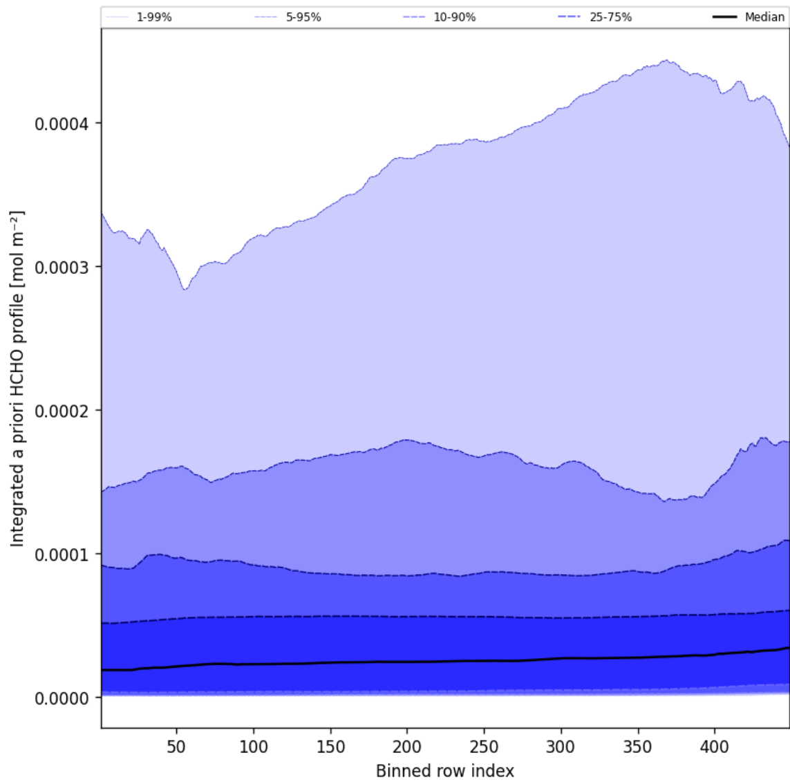
Figure 55: Along track statistics of “Integrated a priori HCHO profile” for 2025-11-02 to 2025-11-03
