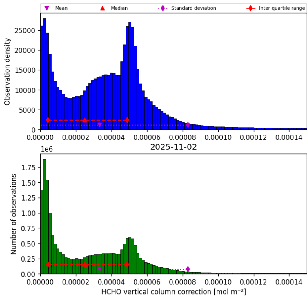
Figure 35: Histogram of “HCHO vertical column correction” for 2025-11-02 to 2025-11-03
