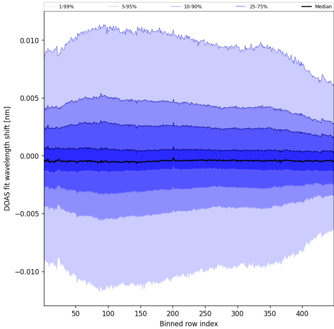
Figure 56: Along track statistics of “DOAS fit wavelength shift” for 2025-11-02 to 2025-11-03
