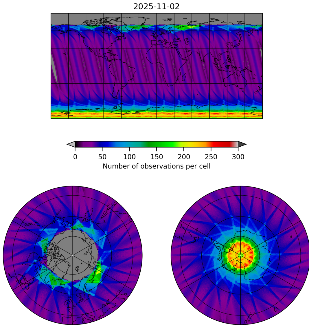
Figure 17: Map of the number of observations for 2025-11-02 to 2025-11-03
