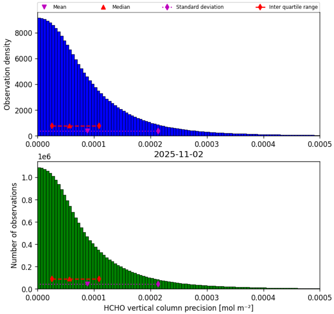
Figure 34: Histogram of “HCHO vertical column precision” for 2025-11-02 to 2025-11-03
