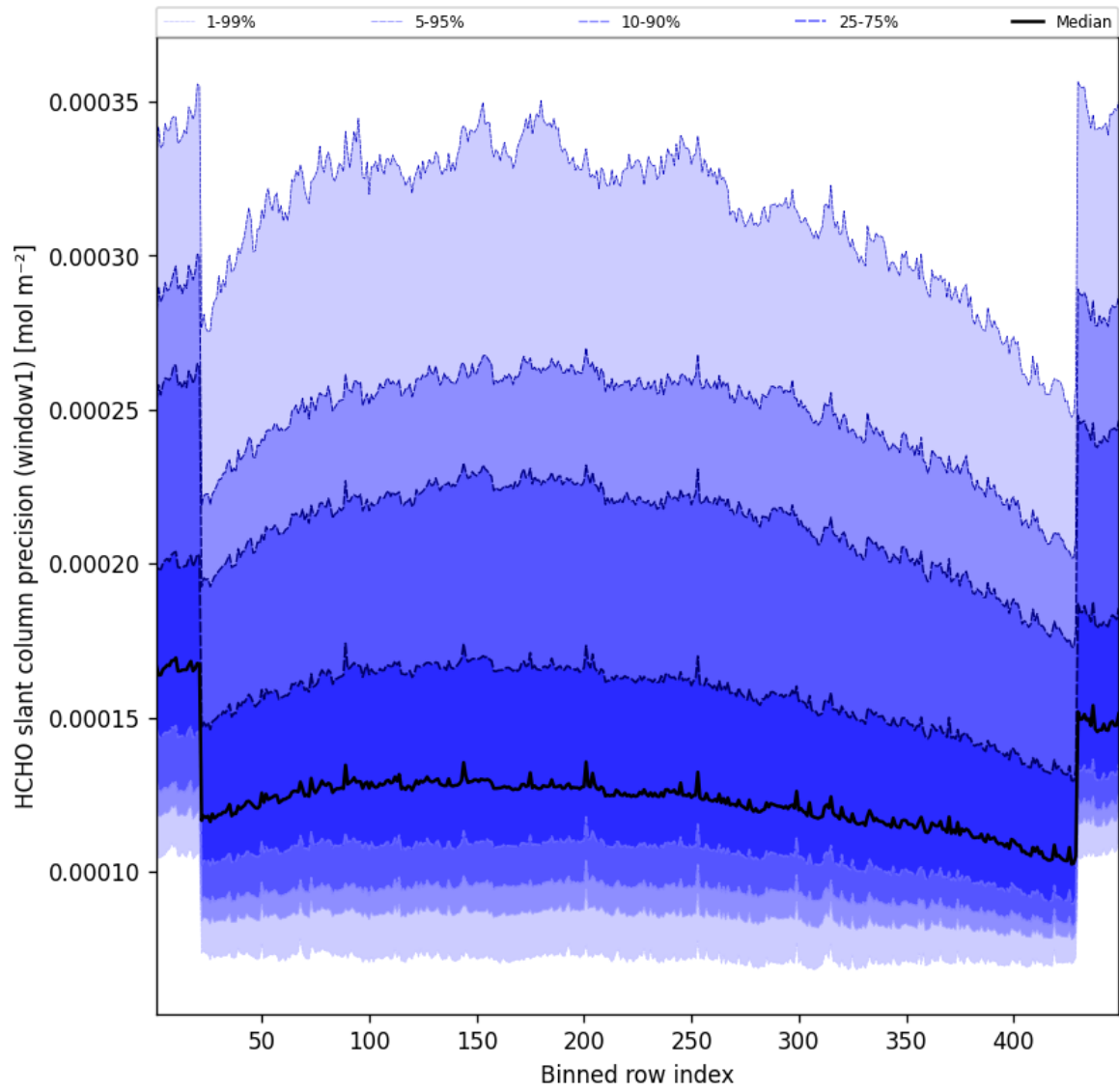
Figure 51: Along track statistics of “HCHO slant column precision (window1)” for 2025-11-02 to 2025-11-03
