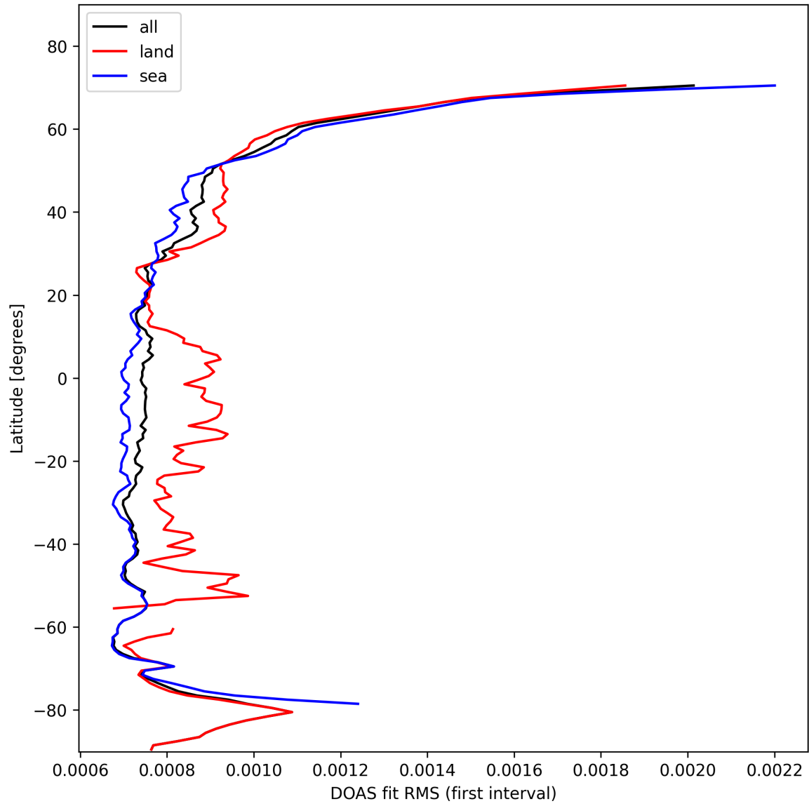
Figure 30: Zonal average of “DOAS fit RMS (first interval)” for 2025-11-02 to 2025-11-03.
