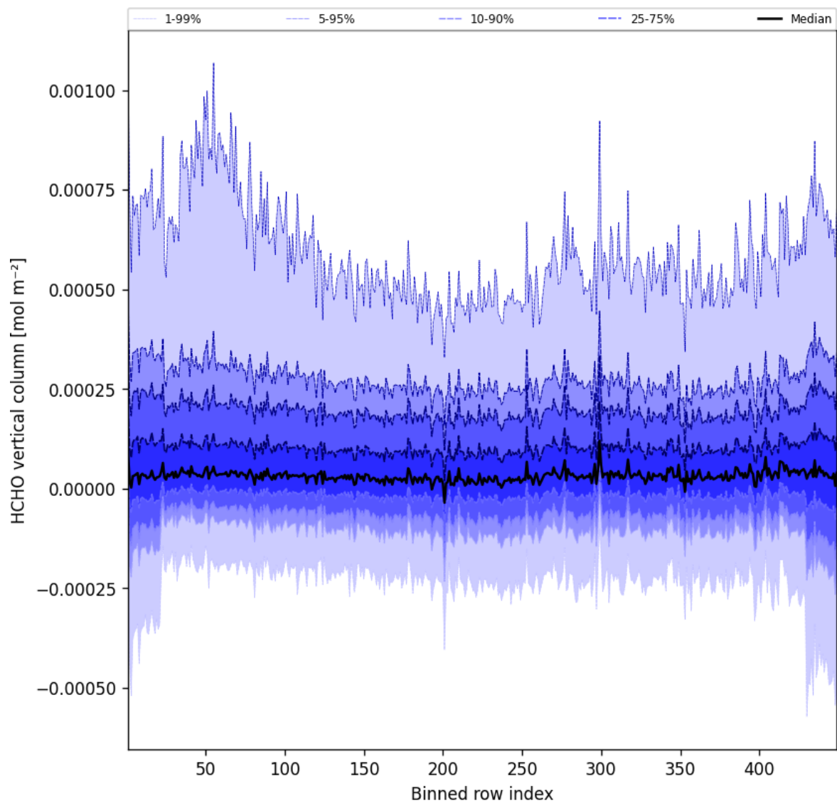
Figure 47: Along track statistics of “HCHO vertical column” for 2025-11-02 to 2025-11-03
