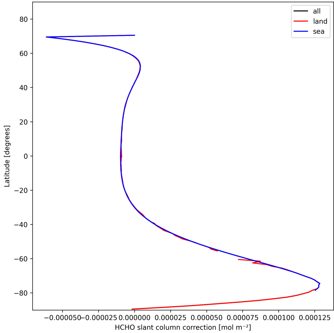
Figure 31: Zonal average of "HCHO slant column correction" for 2025-11-02 to 2025-11-03.
