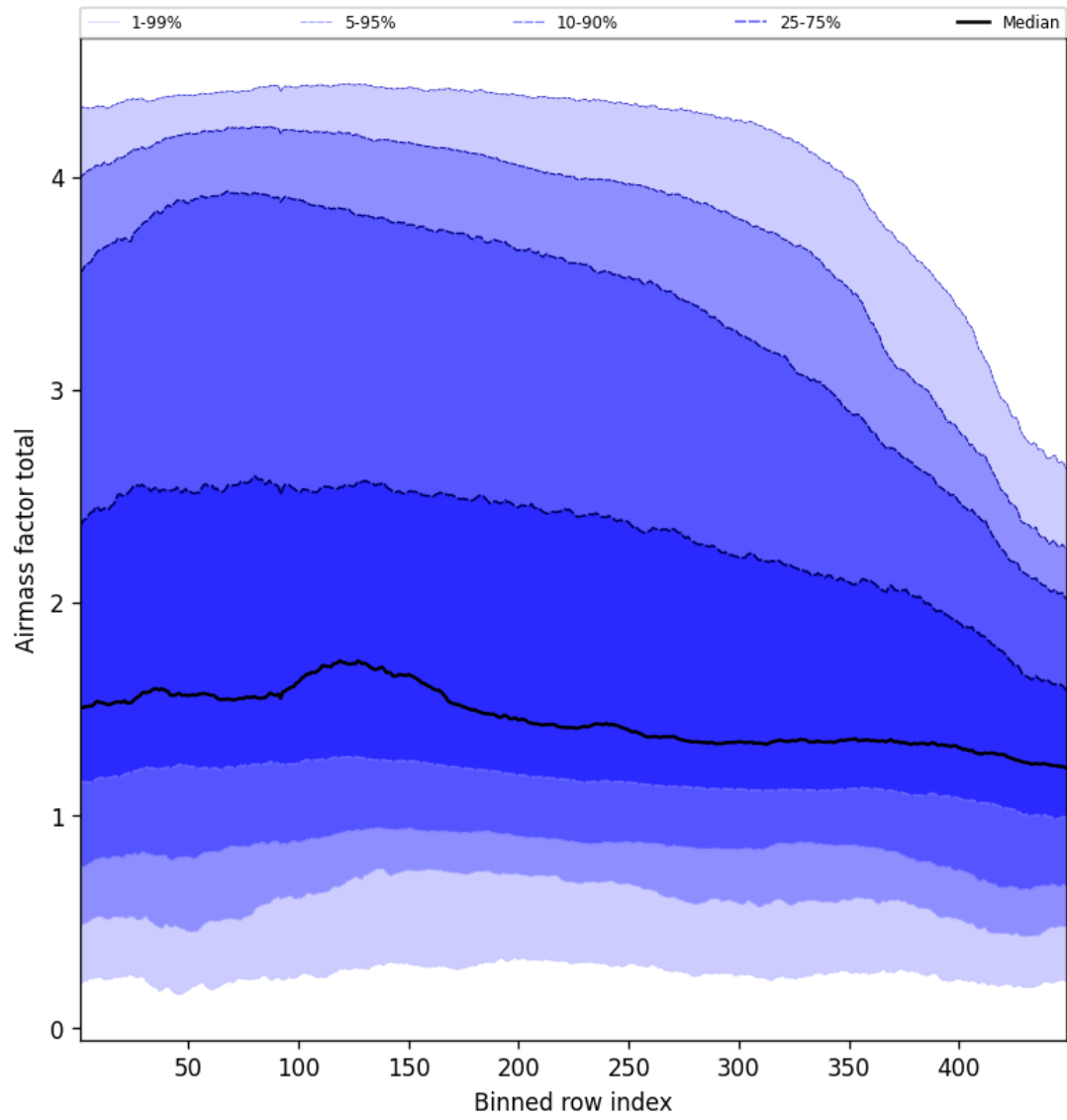
Figure 52: Along track statistics of “Airmass factor total” for 2025-11-02 to 2025-11-03
