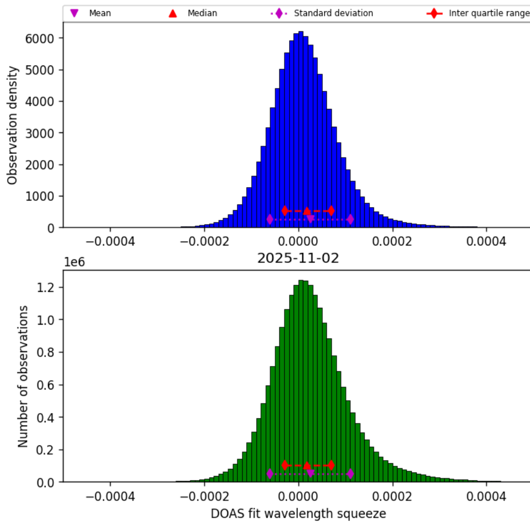
Figure 43: Histogram of “DOAS fit wavelength squeeze” for 2025-11-02 to 2025-11-03
