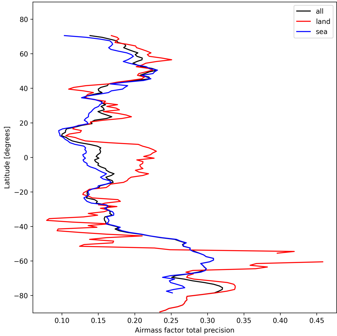
Figure 25: Zonal average of “Airmass factor total precision” for 2025-11-02 to 2025-11-03.
