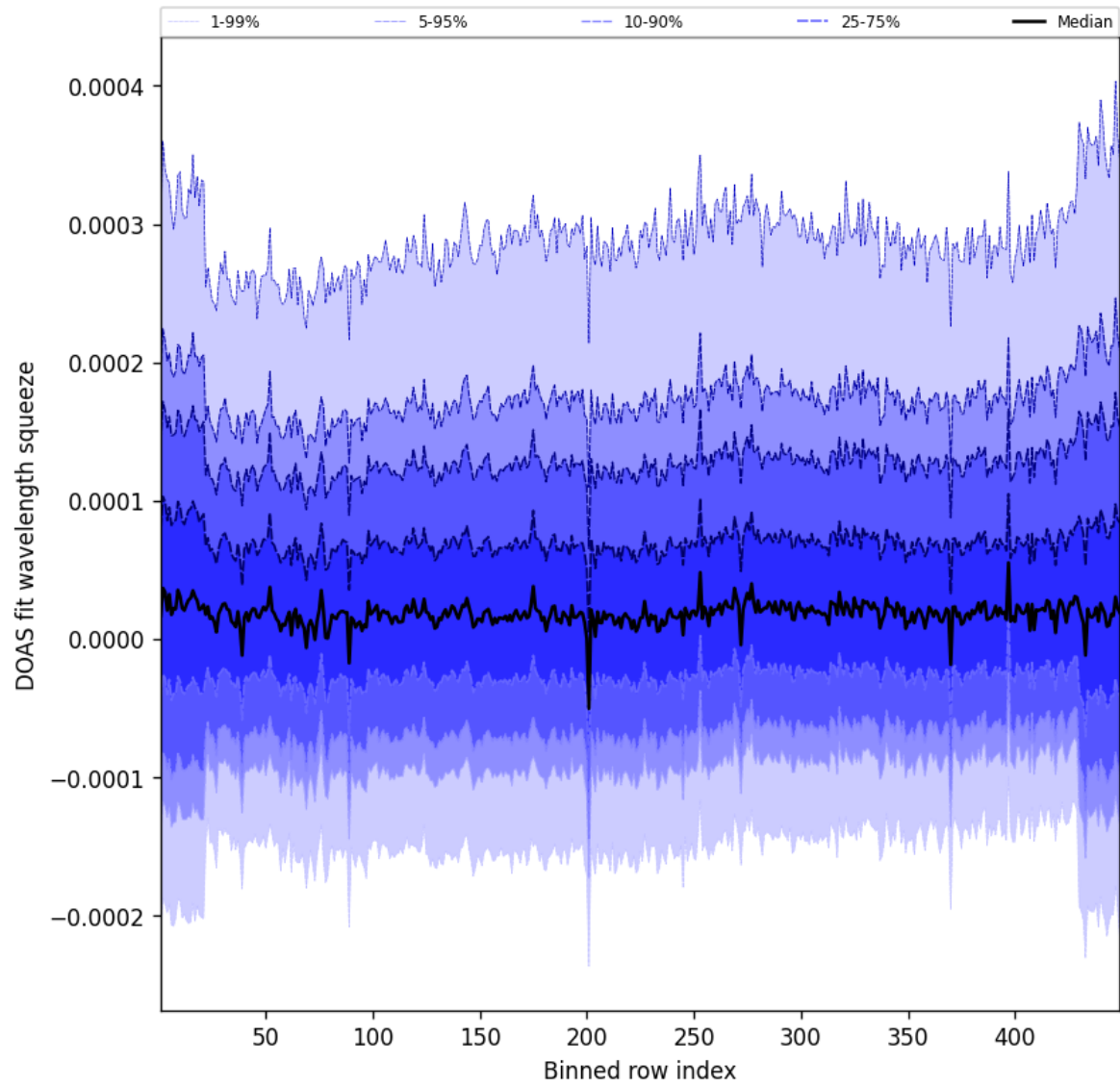
Figure 57: Along track statistics of “DOAS fit wavelength squeeze” for 2025-11-02 to 2025-11-03
