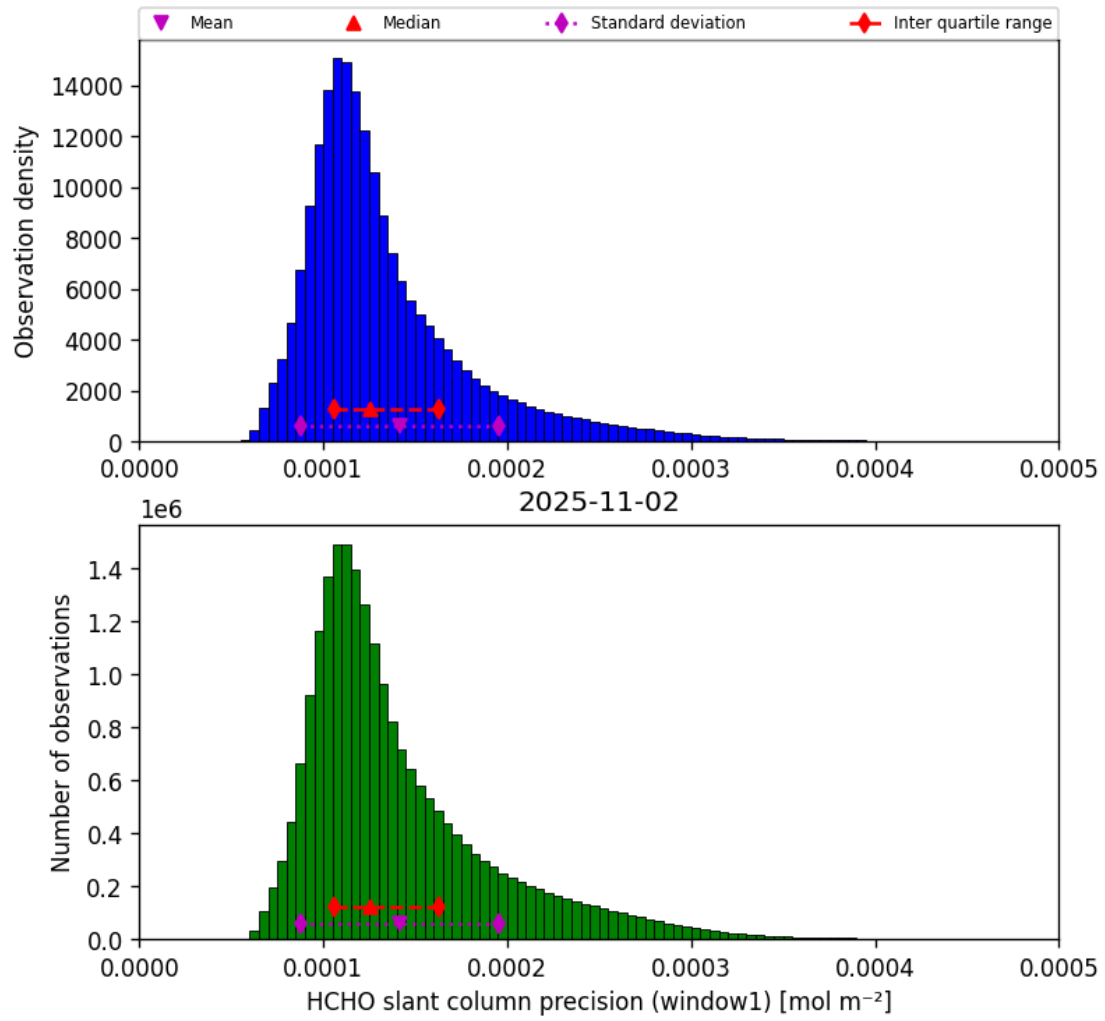
Figure 37: Histogram of “HCHO slant column precision (window1)” for 2025-11-02 to 2025-11-03
