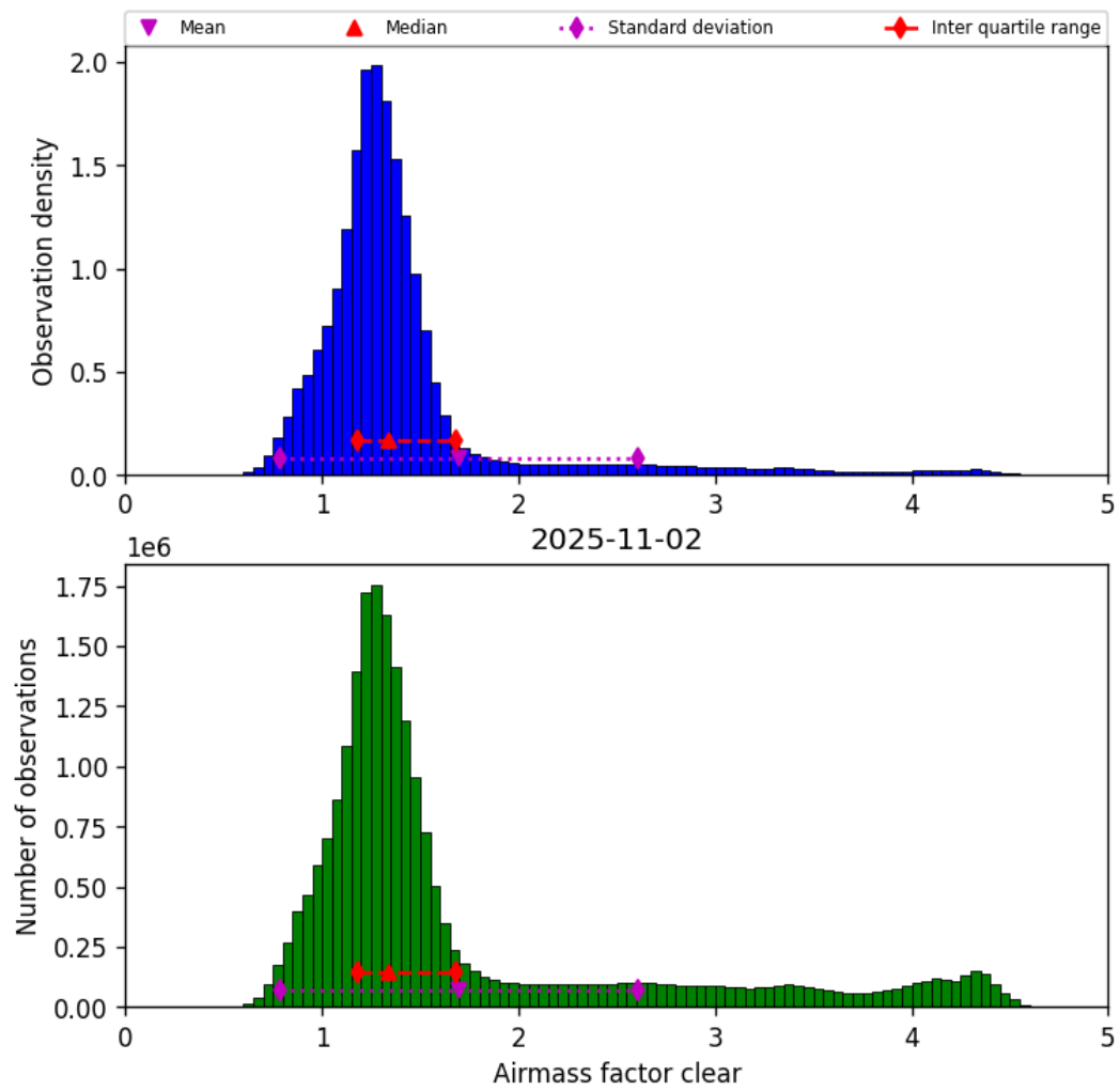
Figure 40: Histogram of “Airmass factor clear” for 2025-11-02 to 2025-11-03
