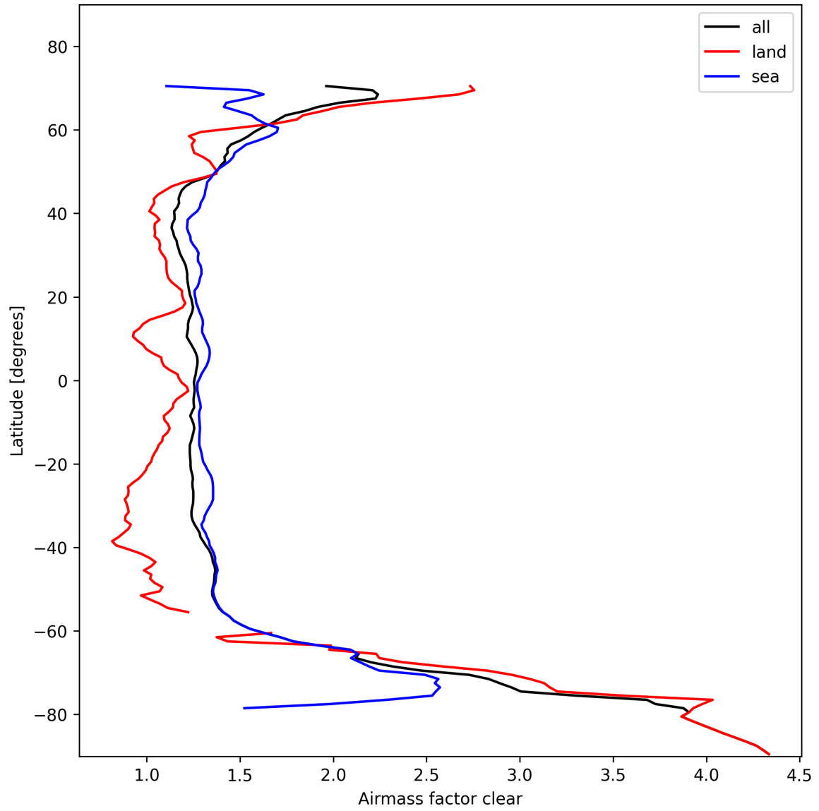
Figure 26: Zonal average of “Airmass factor clear” for 2025-11-02 to 2025-11-03.
