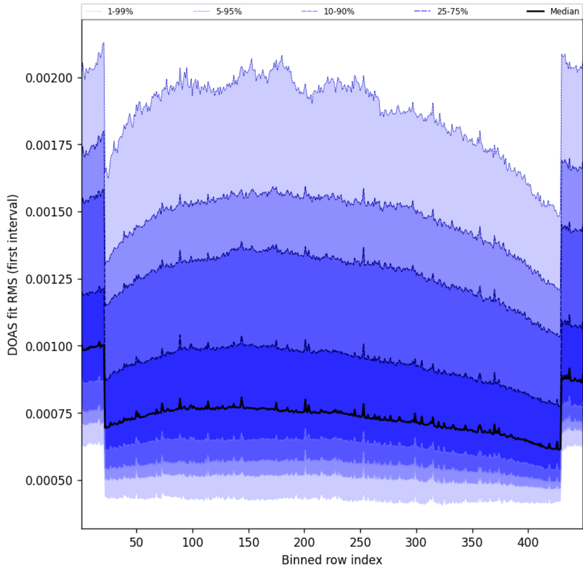
Figure 58: Along track statistics of “DOAS fit RMS (first interval)” for 2025-11-02 to 2025-11-03
