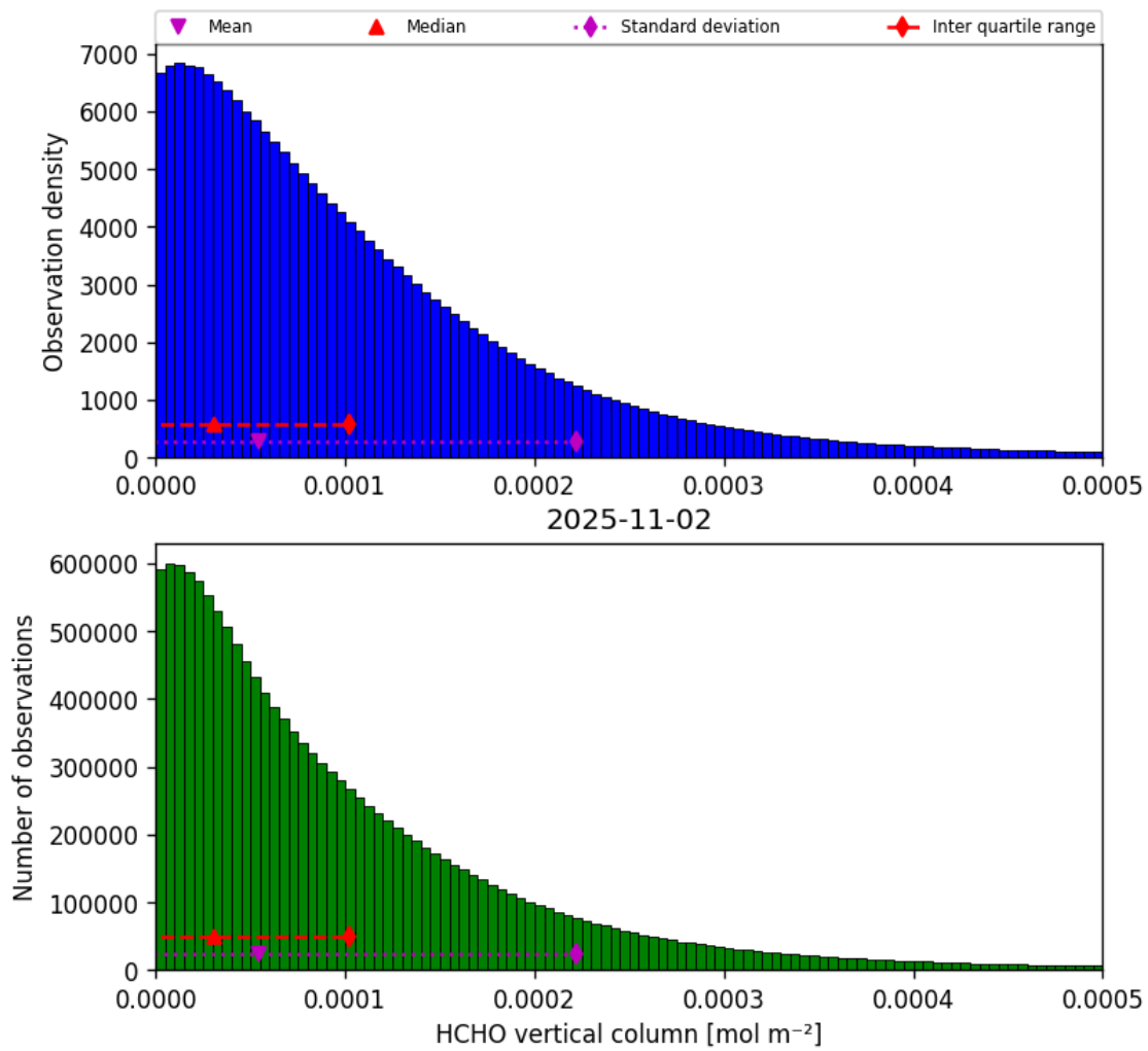
Figure 33: Histogram of “HCHO vertical column” for 2025-11-02 to 2025-11-03
