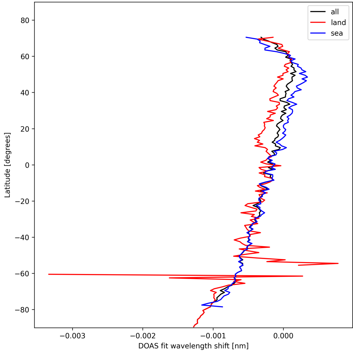
Figure 28: Zonal average of “DOAS fit wavelength shift” for 2025-11-02 to 2025-11-03.
