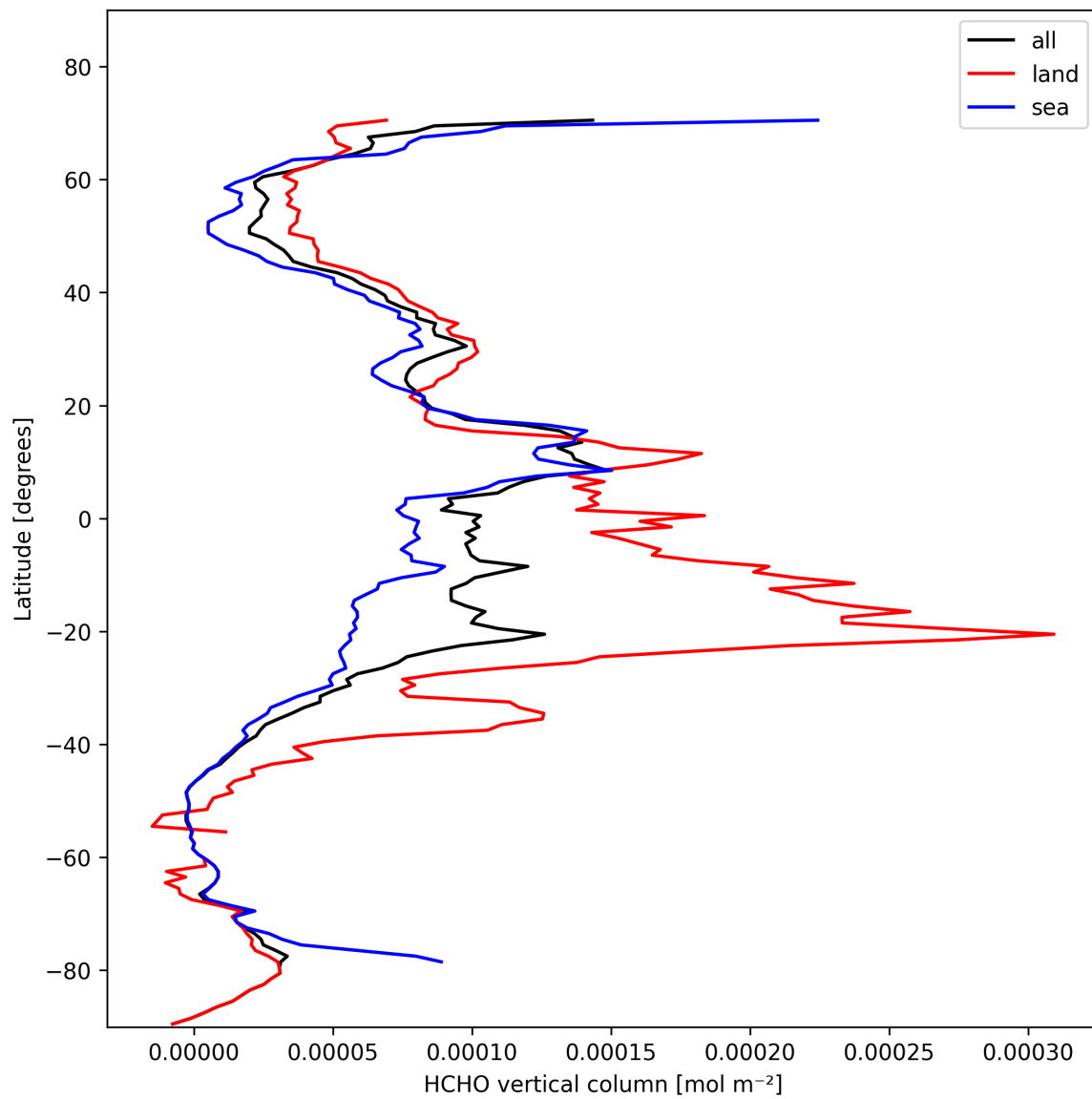
Figure 19: Zonal average of “HCHO vertical column” for 2025-11-02 to 2025-11-03.
