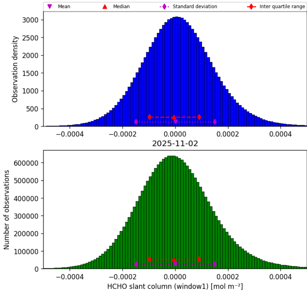
Figure 36: Histogram of “HCHO slant column (window1)” for 2025-11-02 to 2025-11-03
