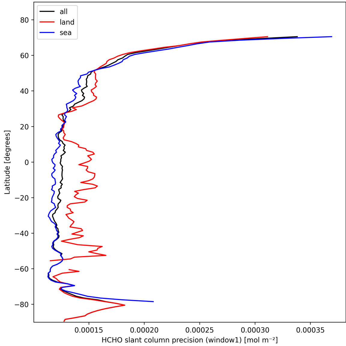
Figure 23: Zonal average of “HCHO slant column precision (window1)” for 2025-11-02 to 2025-11-03.
