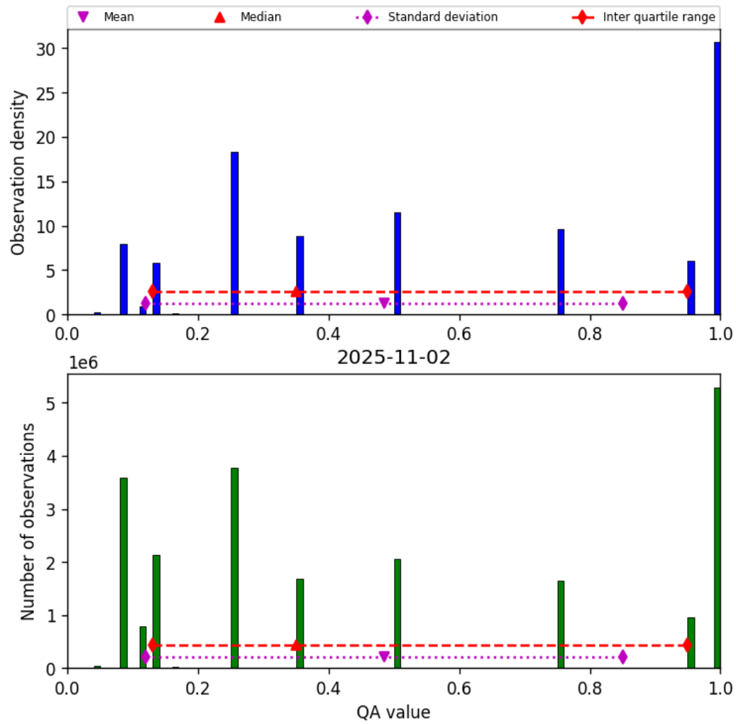
Figure 32: Histogram of “QA value” for 2025-11-02 to 2025-11-03
