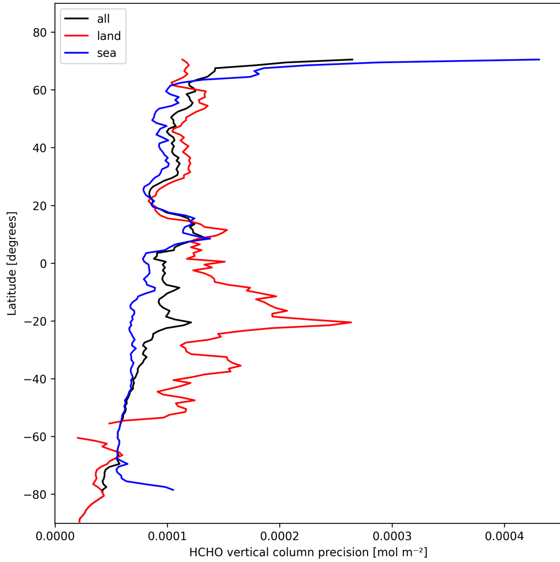
Figure 20: Zonal average of “HCHO vertical column precision” for 2025-11-02 to 2025-11-03.
