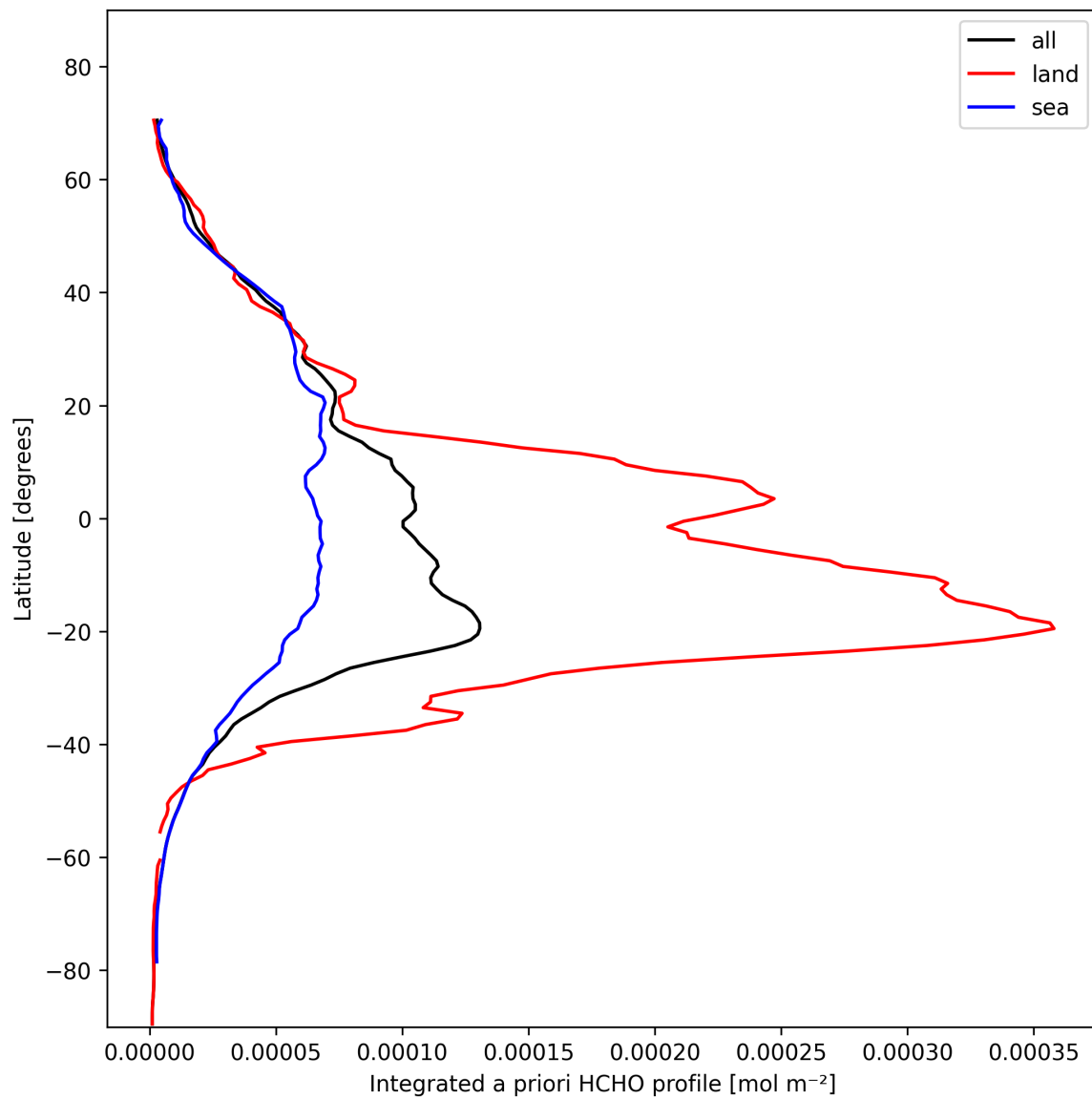
Figure 27: Zonal average of “Integrated a priori HCHO profile” for 2025-11-02 to 2025-11-03.
