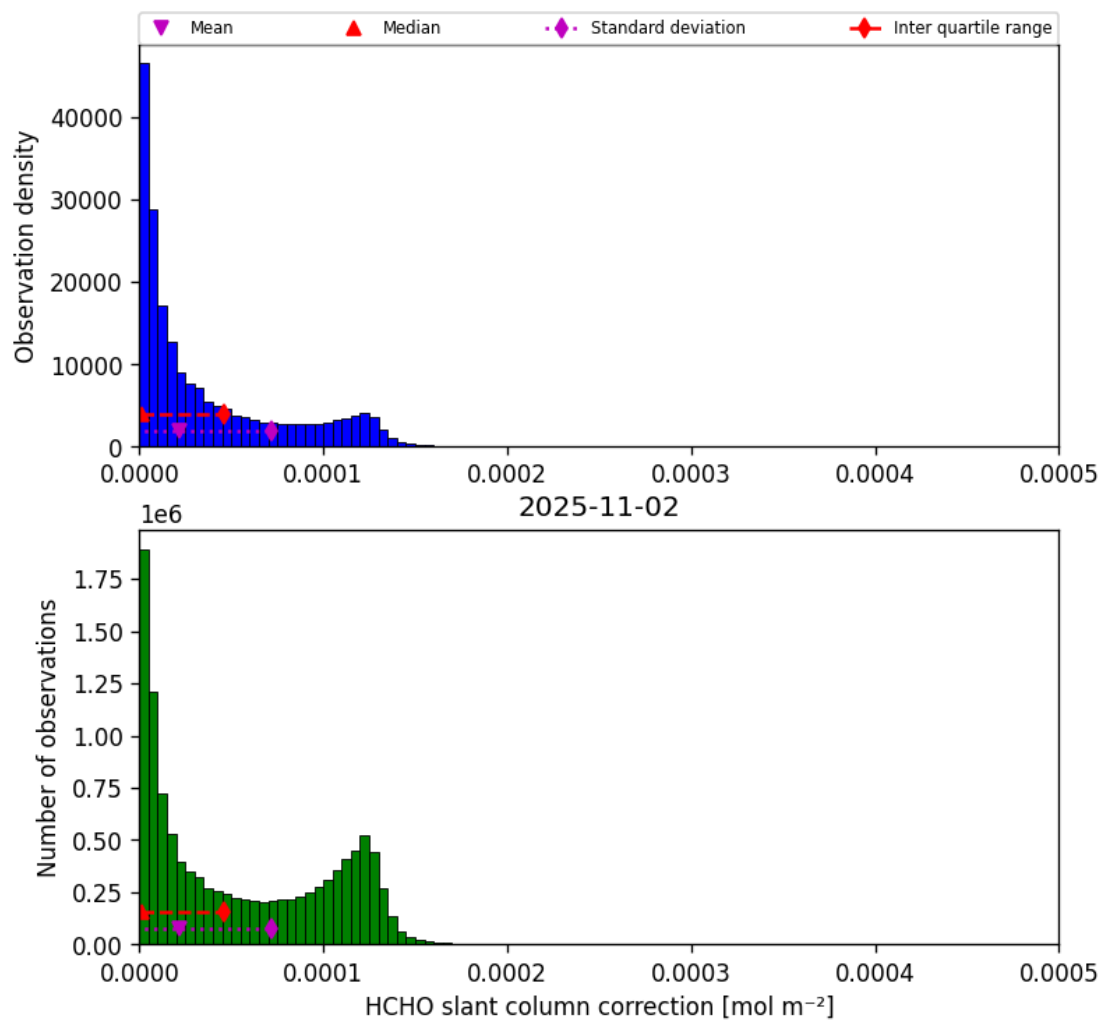
Figure 45: Histogram of “HCHO slant column correction” for 2025-11-02 to 2025-11-03
