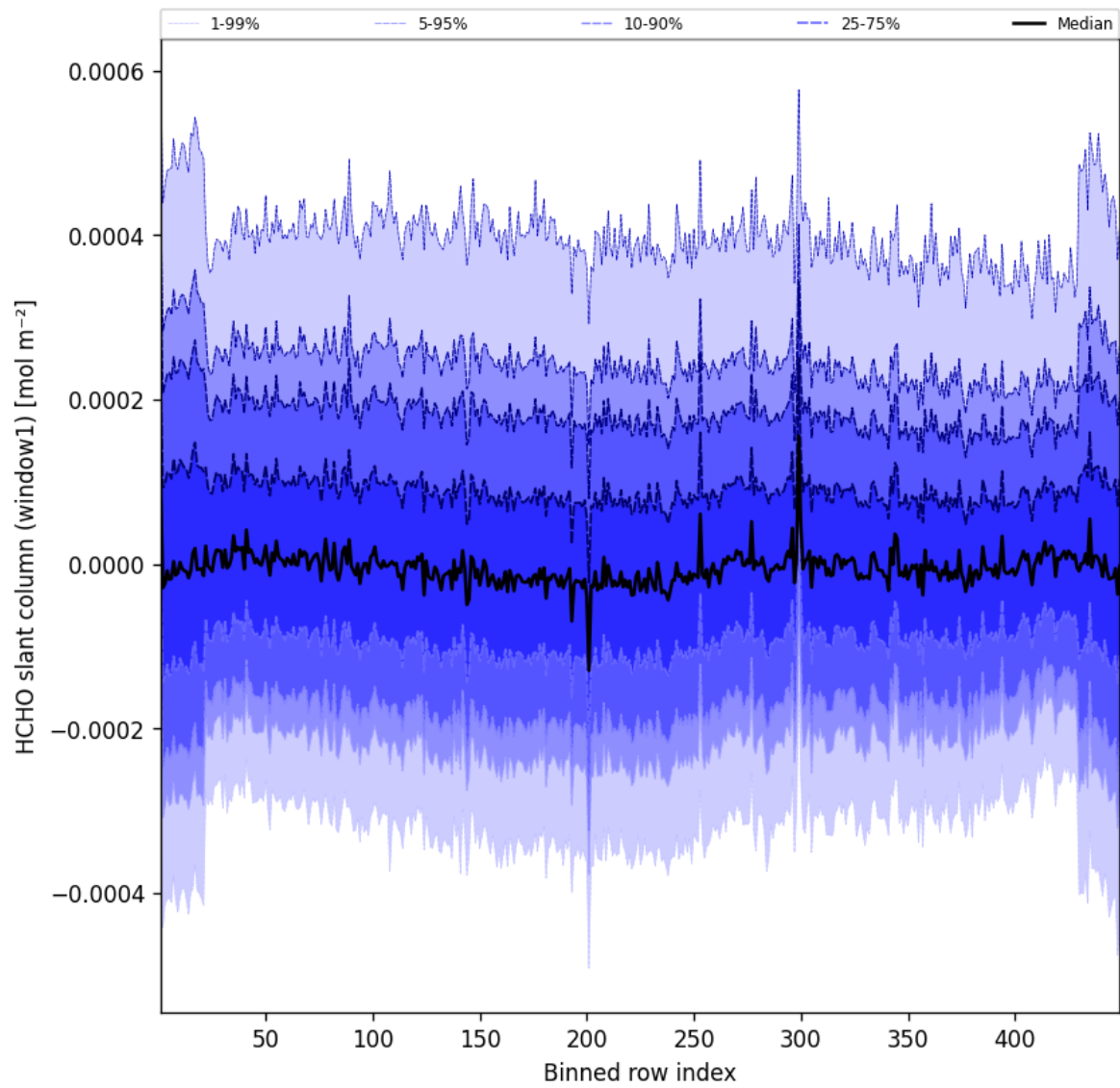
Figure 50: Along track statistics of "HCHO slant column (window1)" for 2025-11-02 to 2025-11-03
