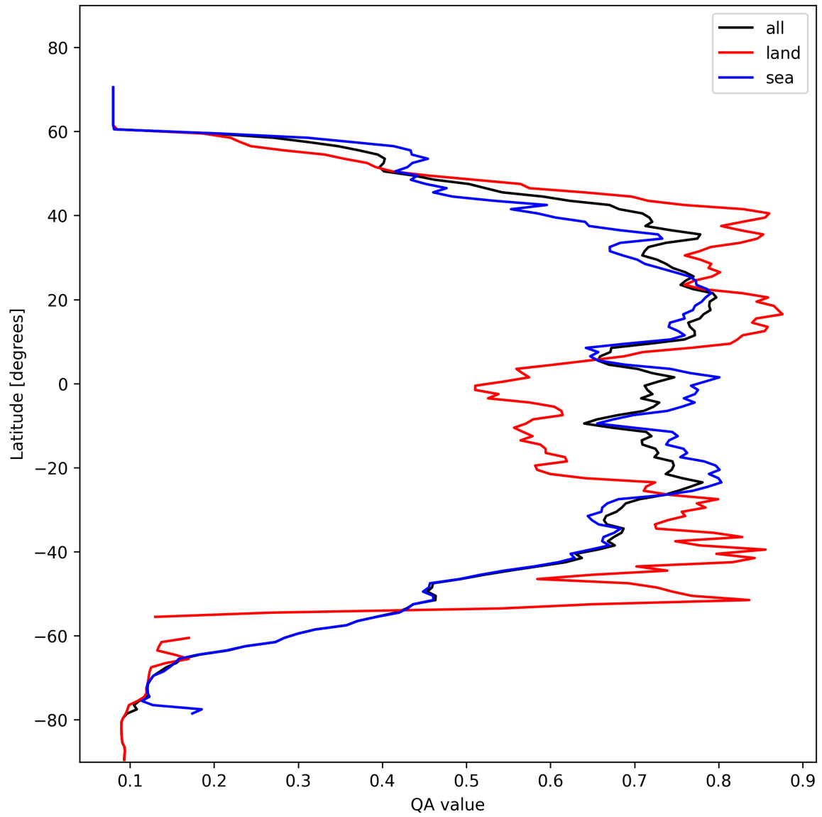
Figure 18: Zonal average of “QA value” for 2025-11-02 to 2025-11-03.
