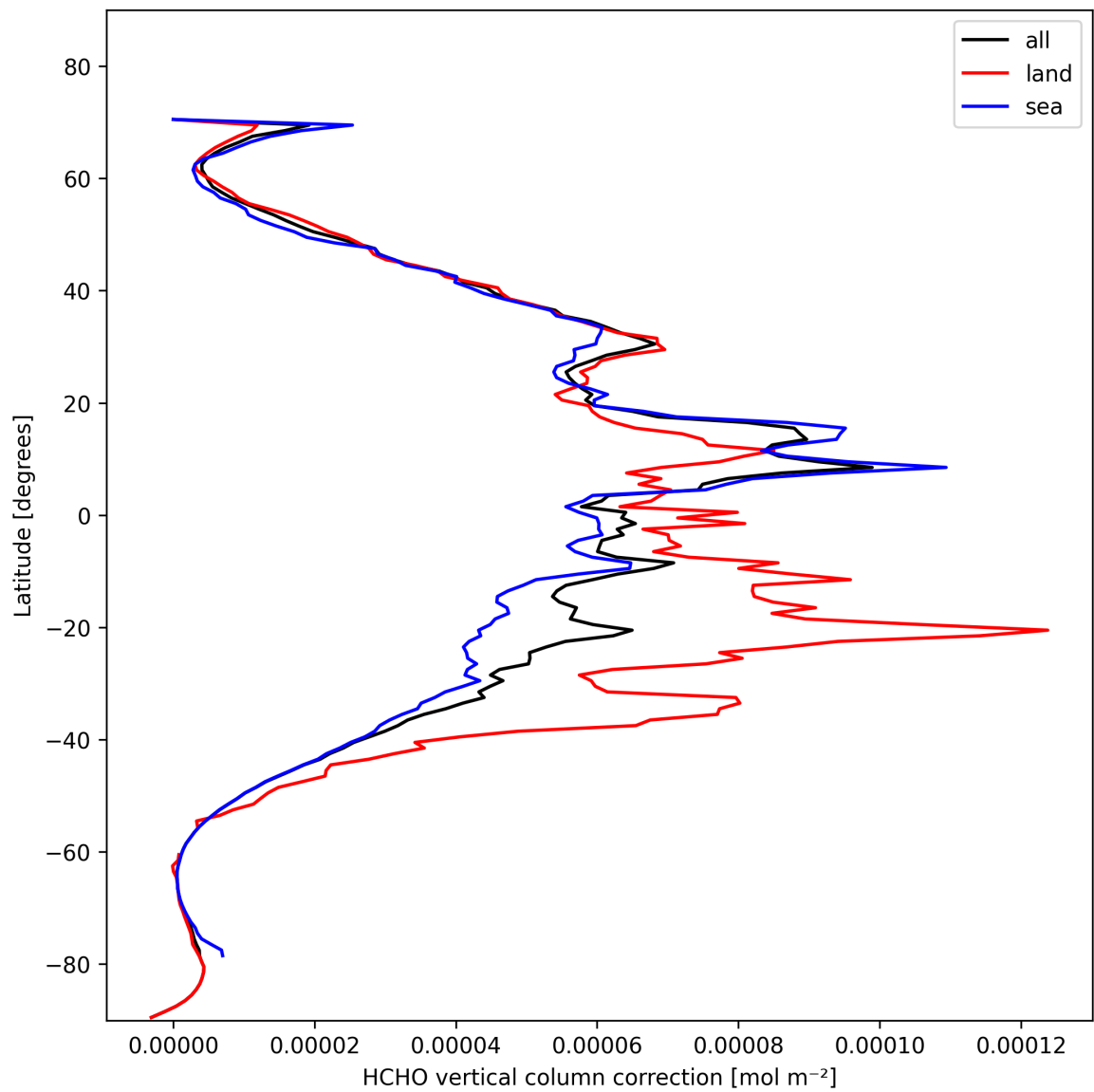
Figure 21: Zonal average of “HCHO vertical column correction” for 2025-11-02 to 2025-11-03.
