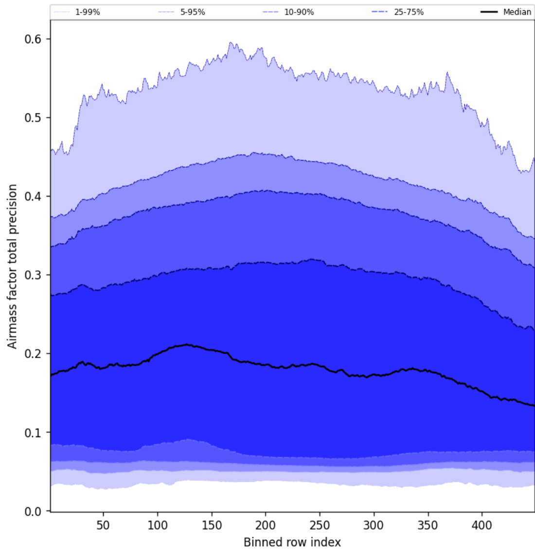
Figure 53: Along track statistics of “Airmass factor total precision” for 2025-11-02 to 2025-11-03
