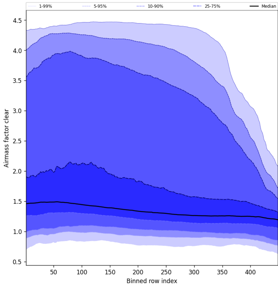
Figure 54: Along track statistics of “Airmass factor clear” for 2025-11-02 to 2025-11-03
