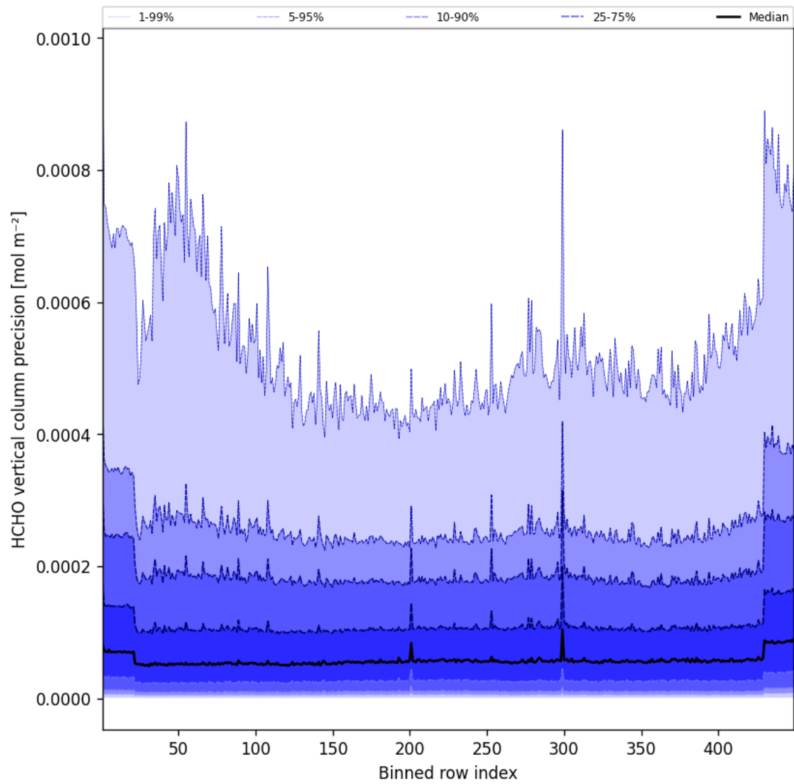
Figure 48: Along track statistics of “HCHO vertical column precision” for 2025-11-02 to 2025-11-03
