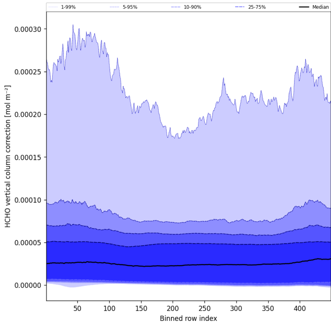
Figure 49: Along track statistics of “HCHO vertical column correction” for 2025-11-02 to 2025-11-03
