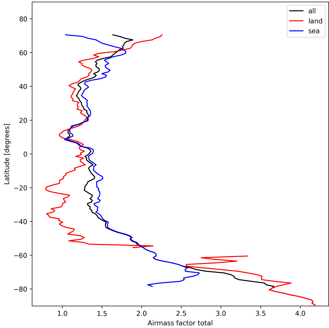
Figure 24: Zonal average of “Airmass factor total” for 2025-11-02 to 2025-11-03.
