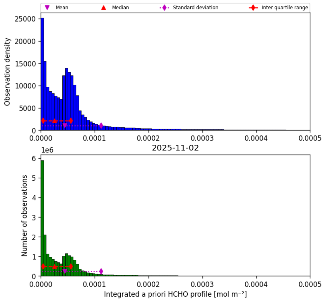
Figure 41: Histogram of “Integrated a priori HCHO profile” for 2025-11-02 to 2025-11-03
