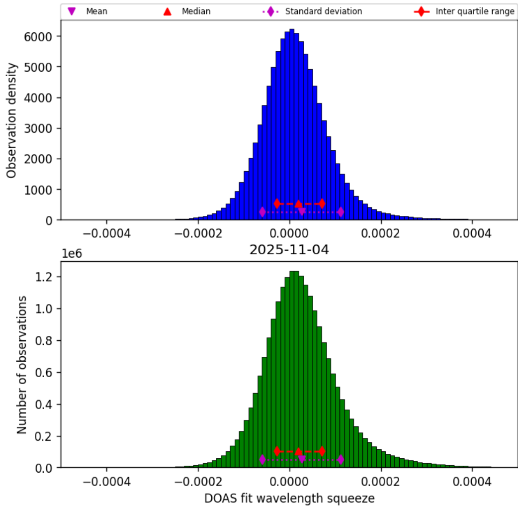
Figure 43: Histogram of “DOAS fit wavelength squeeze” for 2025-11-04 to 2025-11-05
