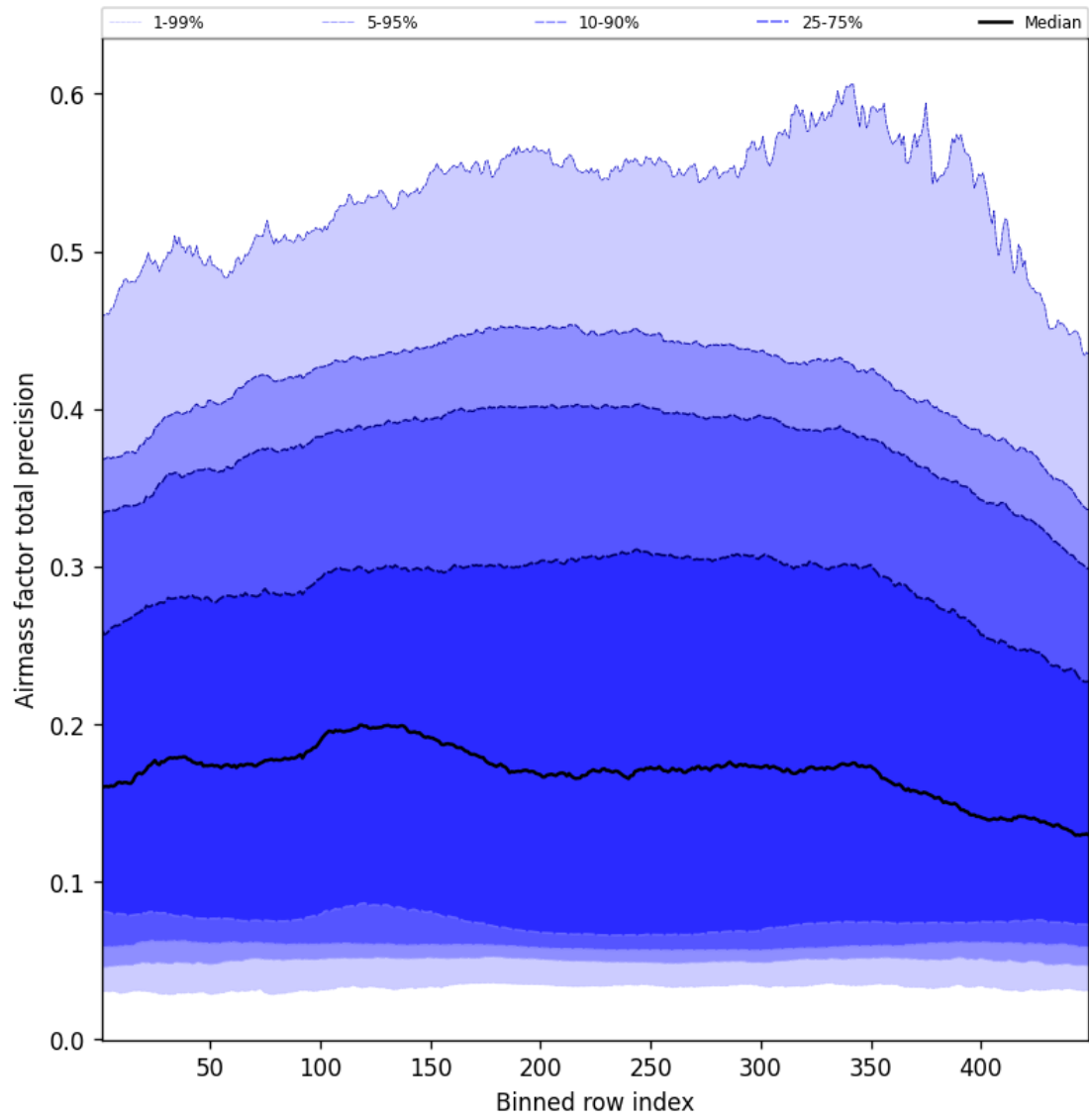
Figure 53: Along track statistics of “Airmass factor total precision” for 2025-11-04 to 2025-11-05
