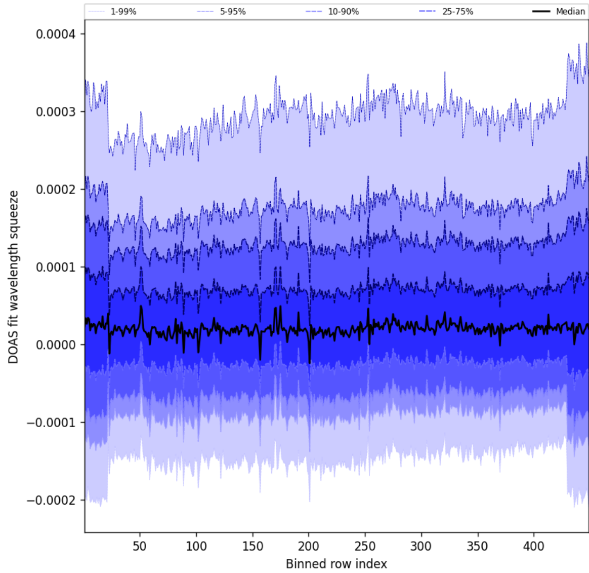
Figure 57: Along track statistics of “DOAS fit wavelength squeeze” for 2025-11-04 to 2025-11-05
