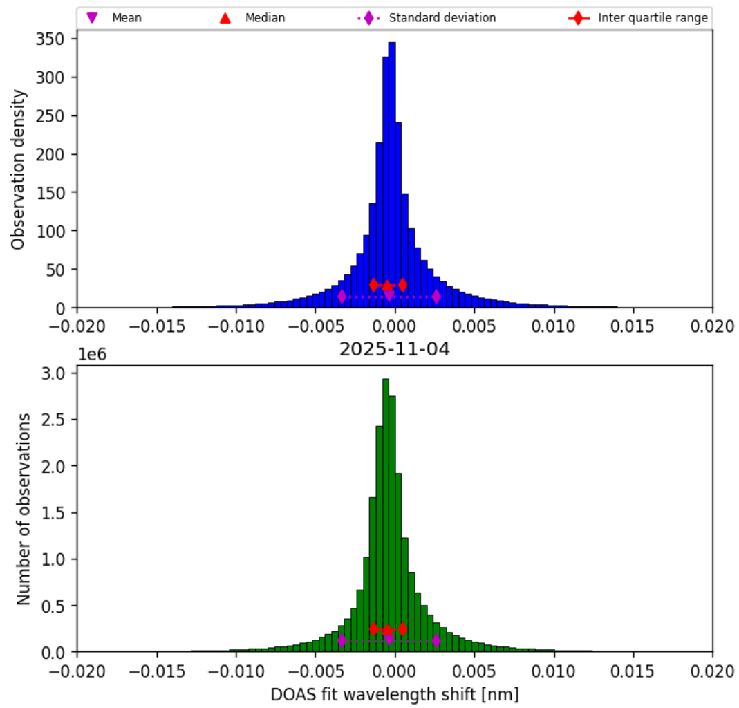
Figure 42: Histogram of “DOAS fit wavelength shift” for 2025-11-04 to 2025-11-05
