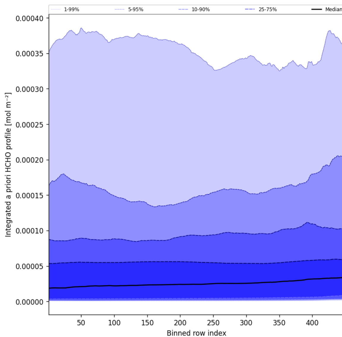
Figure 55: Along track statistics of “Integrated a priori HCHO profile” for 2025-11-04 to 2025-11-05
