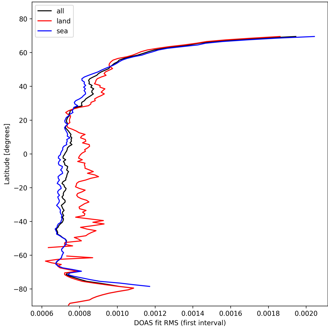
Figure 30: Zonal average of “DOAS fit RMS (first interval)” for 2025-11-04 to 2025-11-05.
