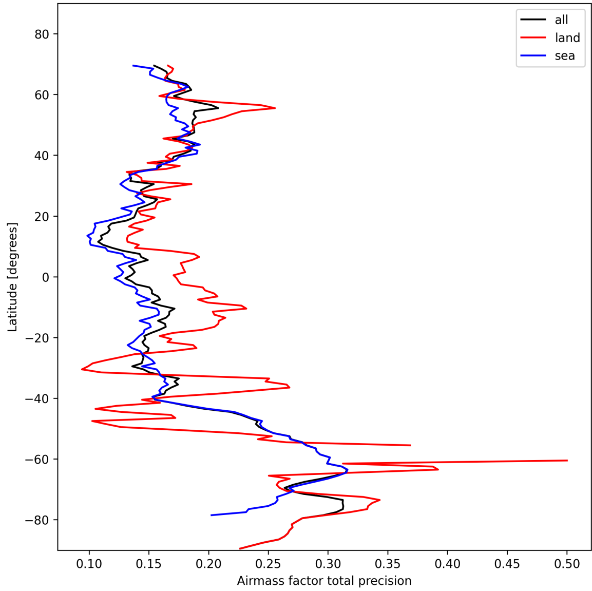
Figure 25: Zonal average of “Airmass factor total precision” for 2025-11-04 to 2025-11-05.
