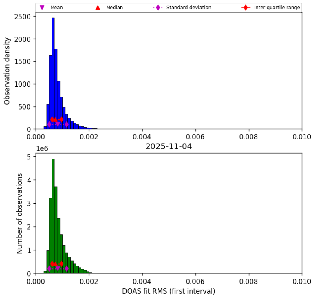
Figure 44: Histogram of “DOAS fit RMS (first interval)” for 2025-11-04 to 2025-11-05
