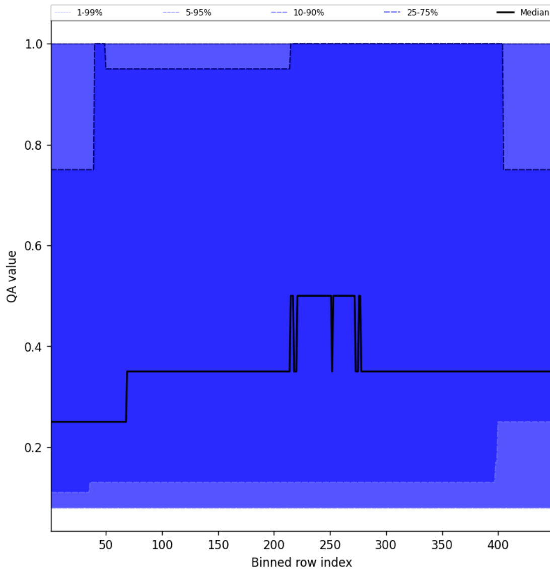
Figure 46: Along track statistics of “QA value” for 2025-11-04 to 2025-11-05
