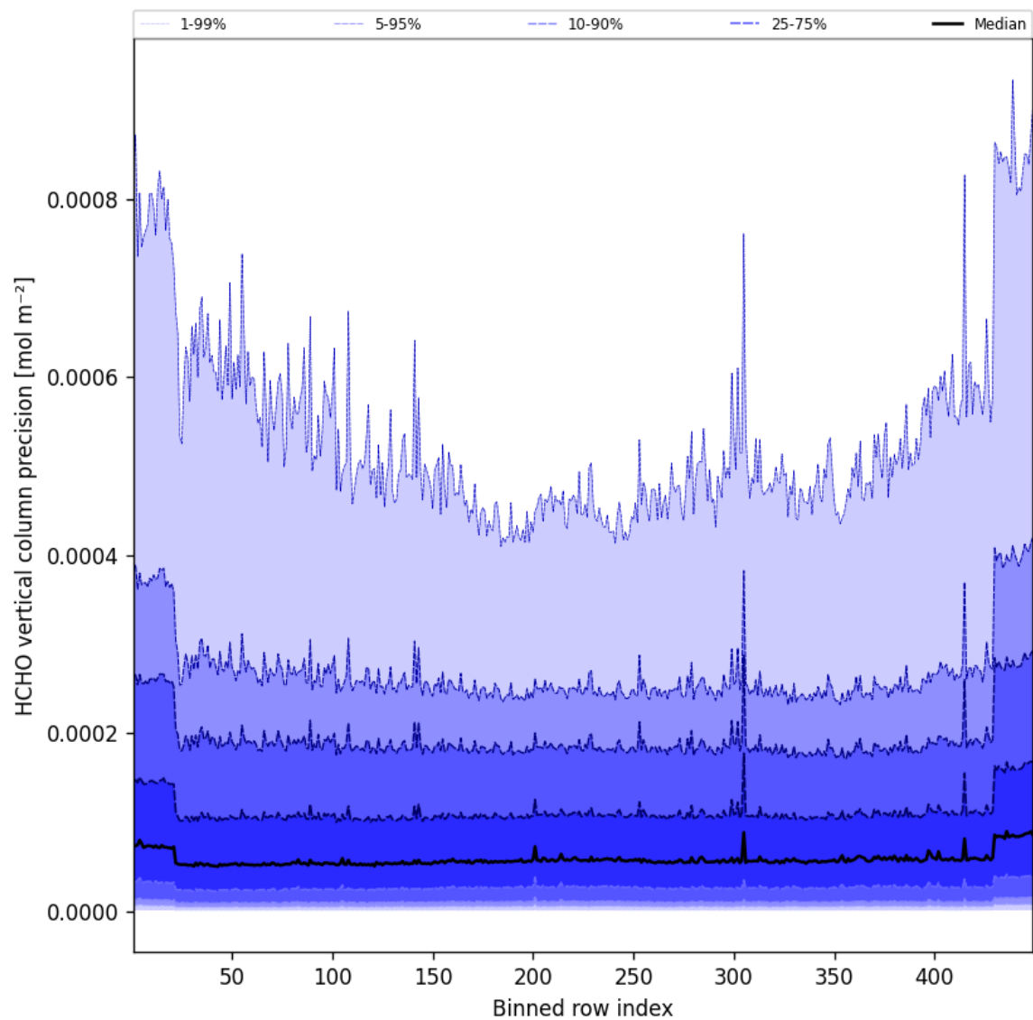
Figure 48: Along track statistics of “HCHO vertical column precision” for 2025-11-04 to 2025-11-05
