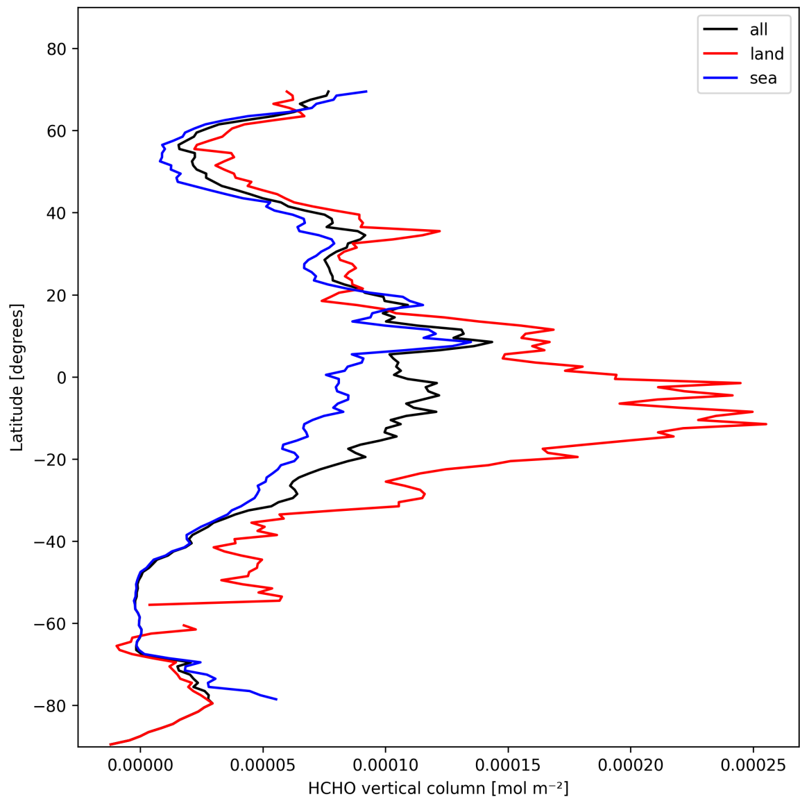
Figure 19: Zonal average of “HCHO vertical column” for 2025-11-04 to 2025-11-05.
