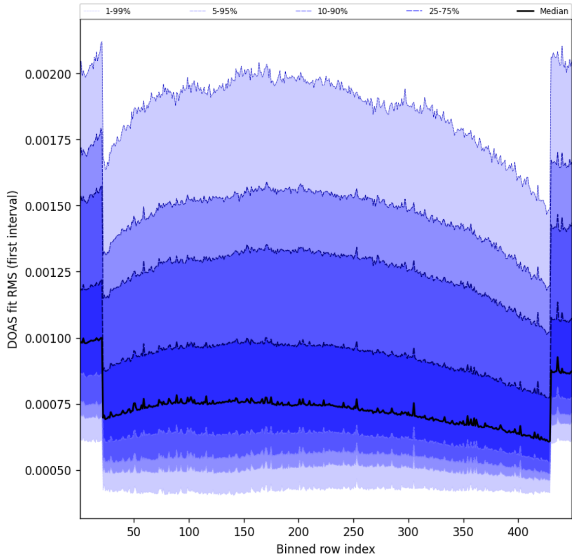
Figure 58: Along track statistics of “DOAS fit RMS (first interval)” for 2025-11-04 to 2025-11-05
