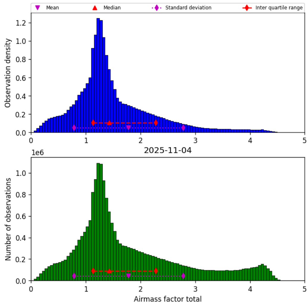
Figure 38: Histogram of “Airmass factor total” for 2025-11-04 to 2025-11-05
