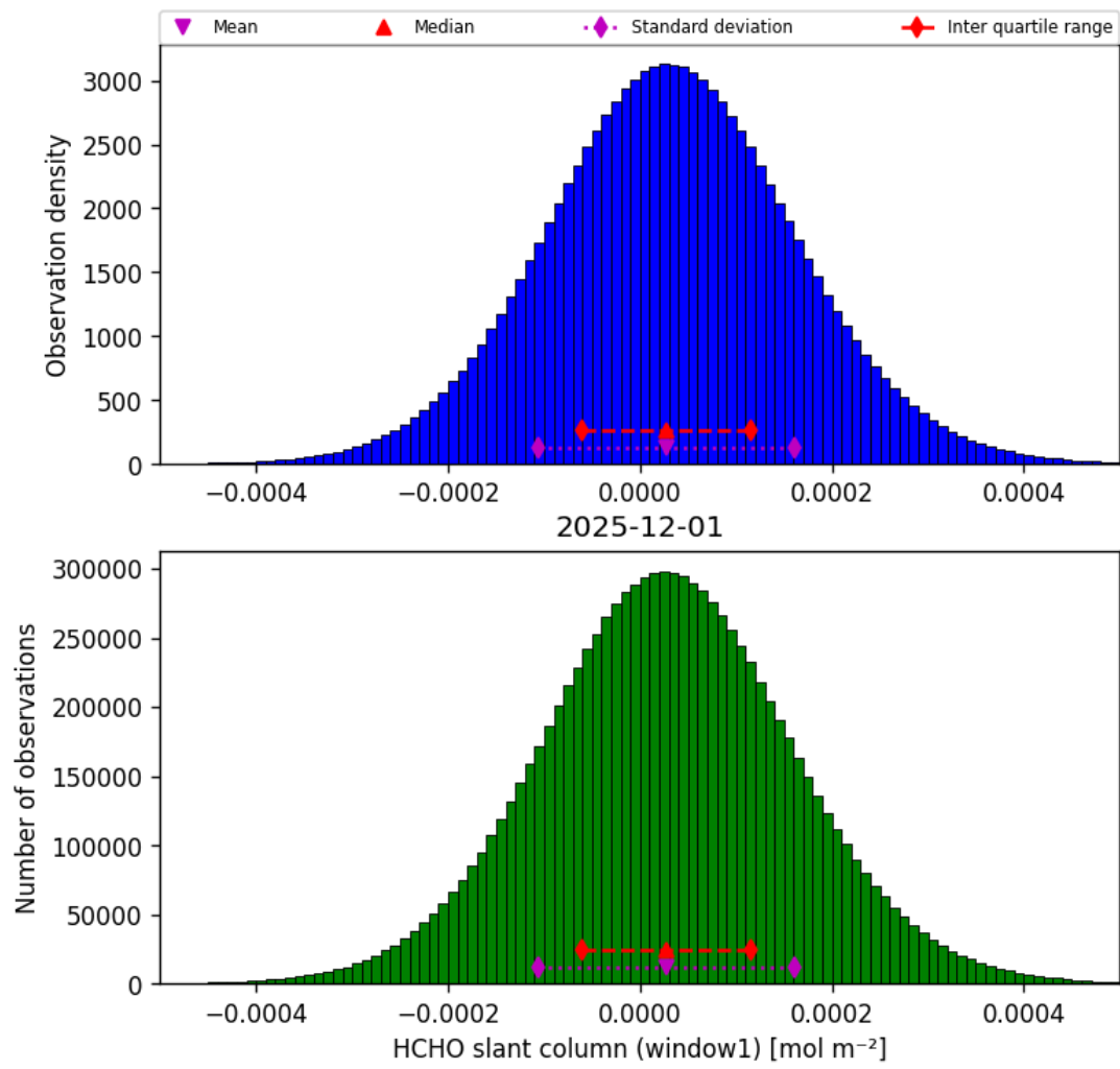
Figure 38: Histogram of “HCHO slant column (window1)” for 2025-12-01 to 2025-12-01
