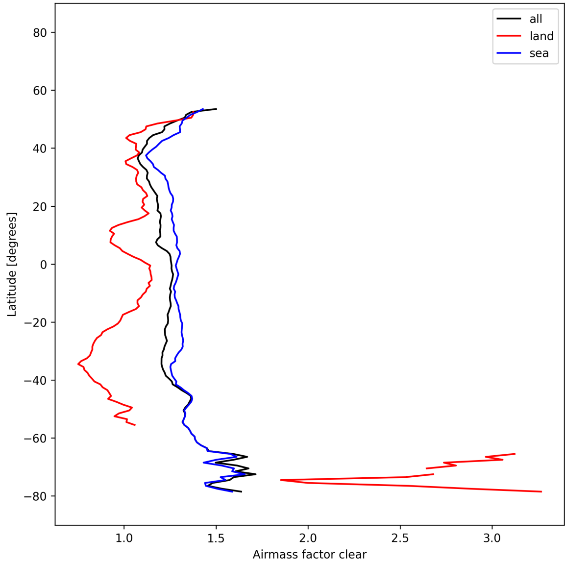
Figure 27: Zonal average of “Airmass factor clear” for 2025-12-01 to 2025-12-01.
