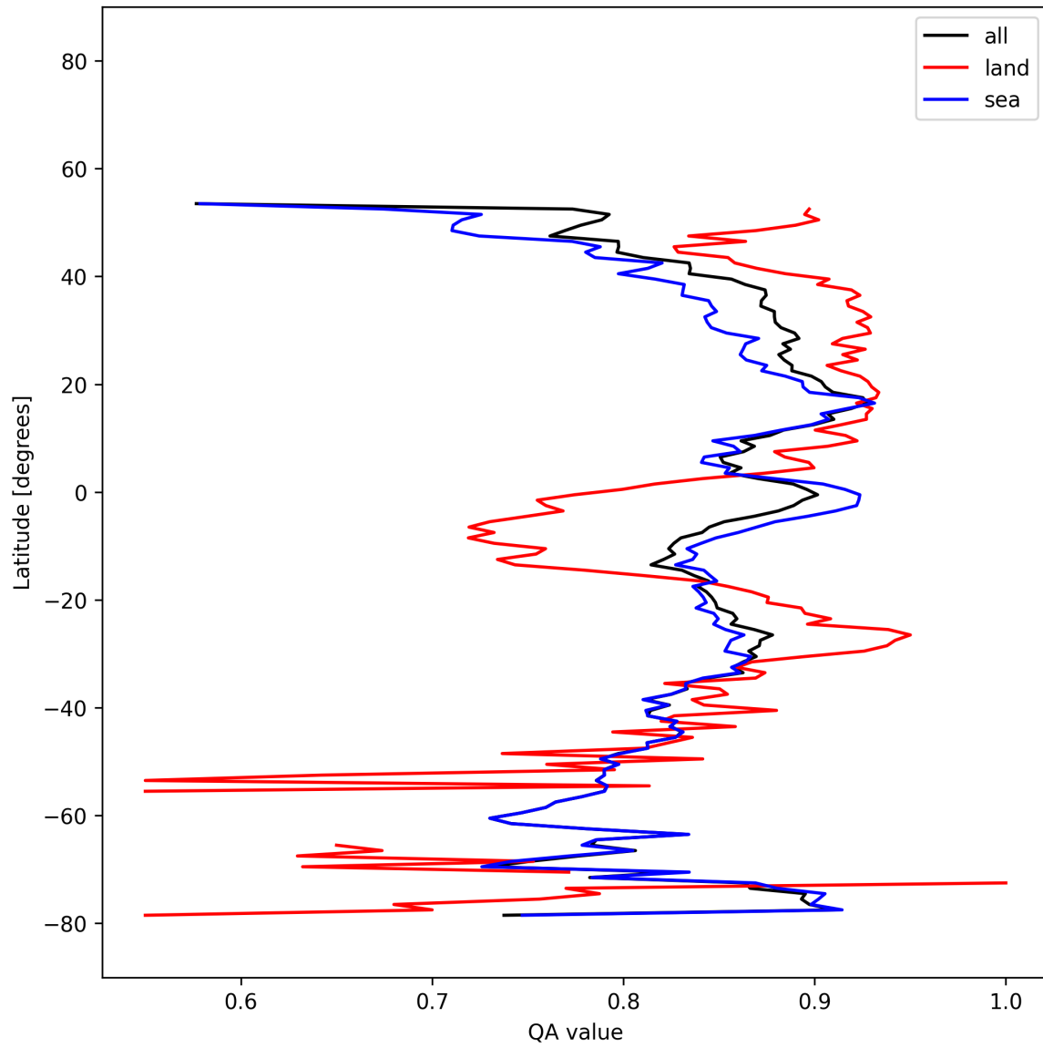
Figure 19: Zonal average of “QA value” for 2025-12-01 to 2025-12-01.
