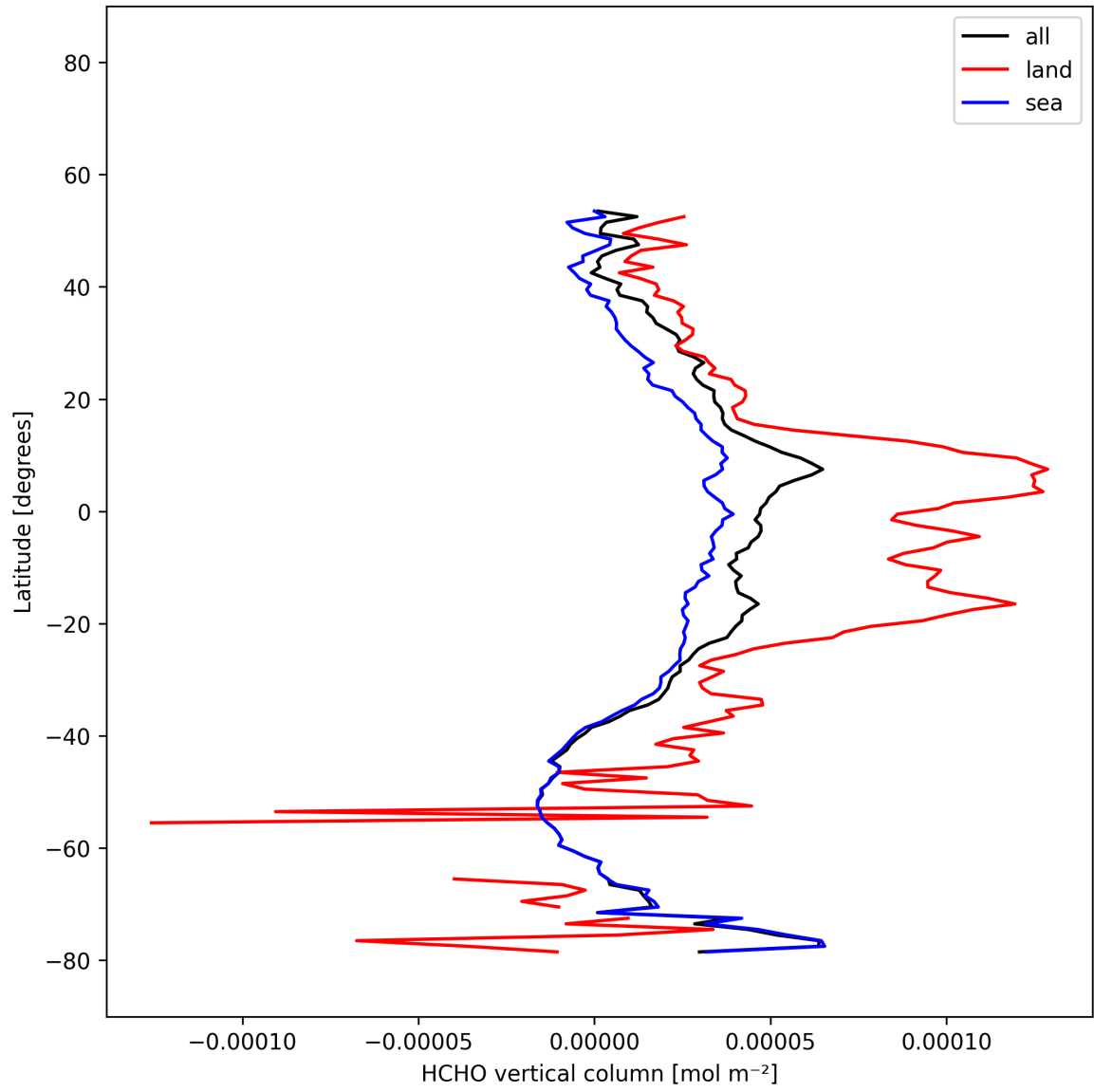
Figure 20: Zonal average of “HCHO vertical column” for 2025-12-01 to 2025-12-01.
