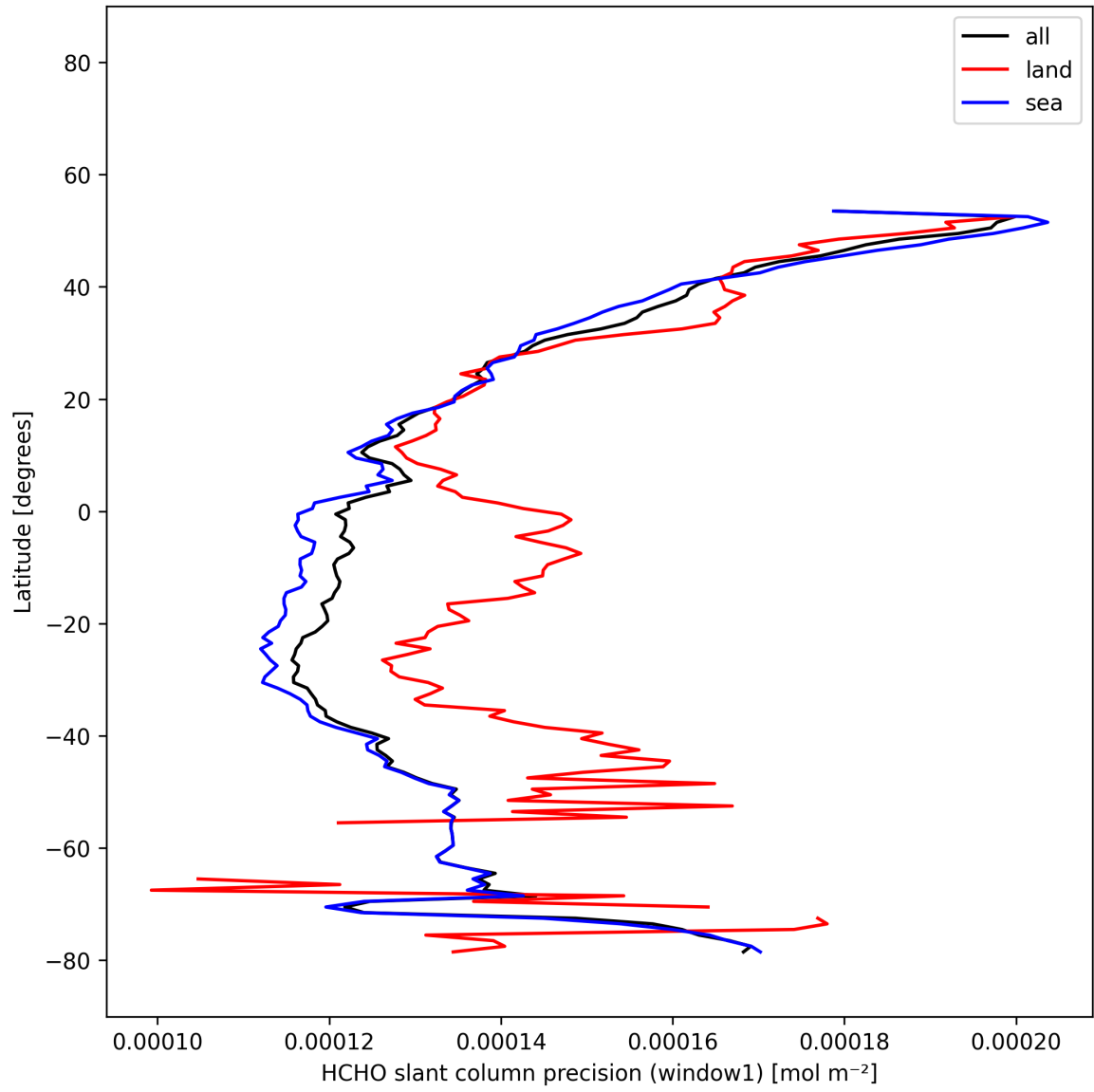
Figure 24: Zonal average of “HCHO slant column precision (window1)” for 2025-12-01 to 2025-12-01.
