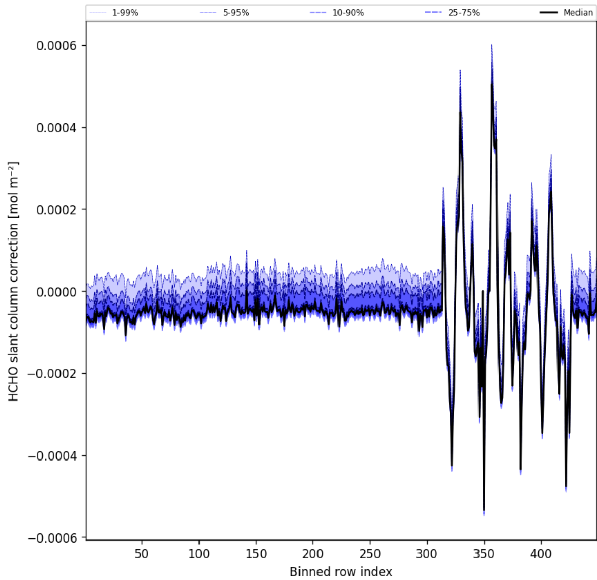
Figure 62: Along track statistics of “HCHO slant column correction” for 2025-12-01 to 2025-12-01
