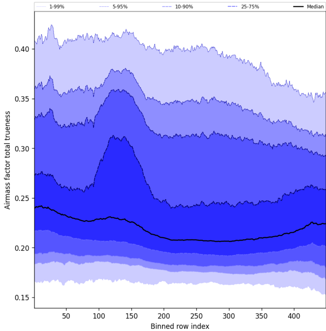
Figure 56: Along track statistics of “Airmass factor total trueness” for 2025-12-01 to 2025-12-01
