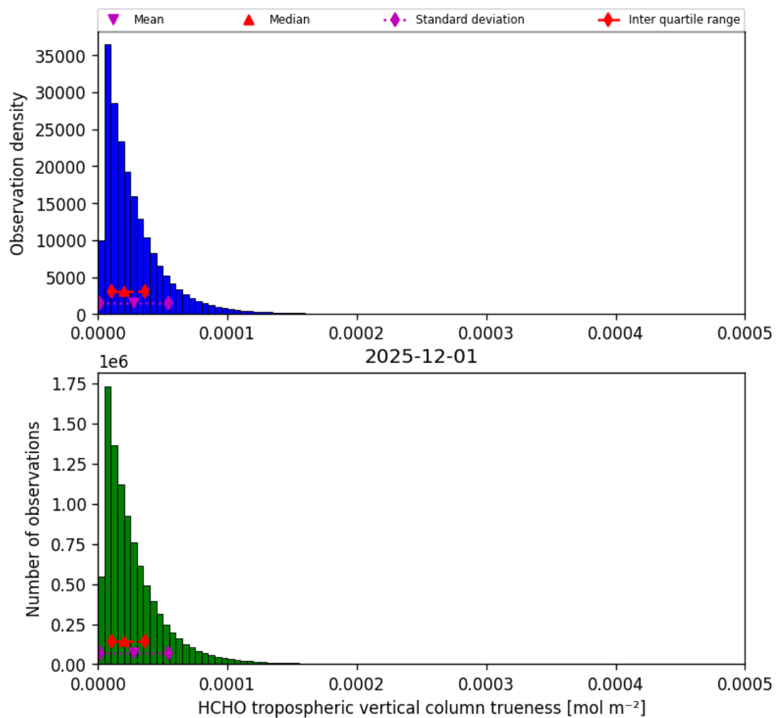
Figure 48: Histogram of “HCHO tropospheric vertical column trueness” for 2025-12-01 to 2025-12-01
