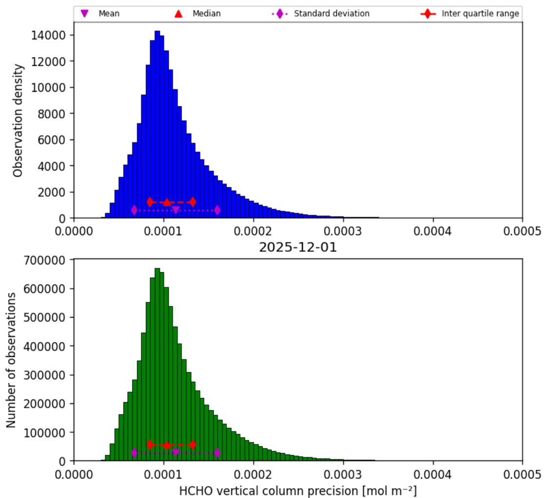
Figure 36: Histogram of “HCHO vertical column precision” for 2025-12-01 to 2025-12-01
