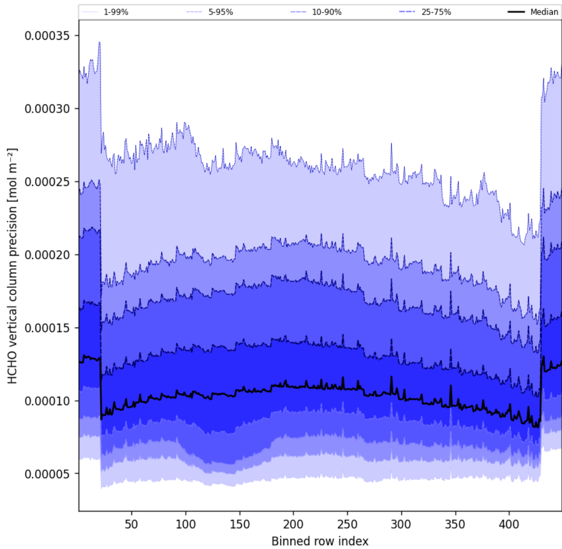
Figure 51: Along track statistics of “HCHO vertical column precision” for 2025-12-01 to 2025-12-01
