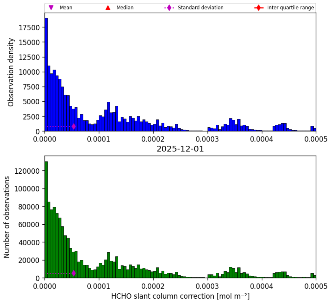
Figure 47: Histogram of “HCHO slant column correction” for 2025-12-01 to 2025-12-01
