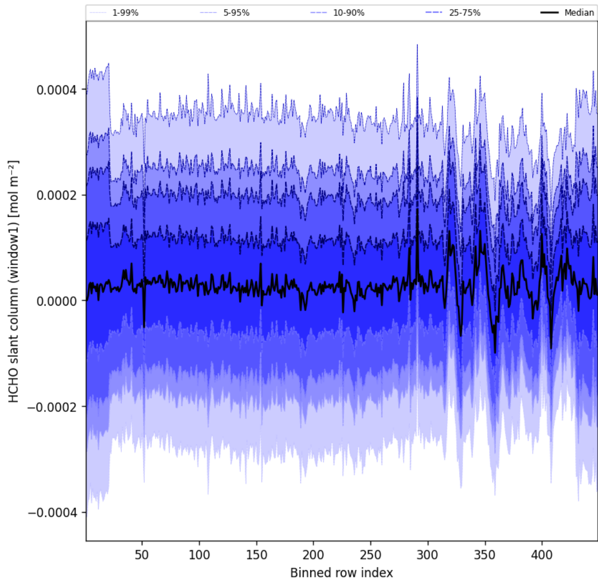
Figure 53: Along track statistics of “HCHO slant column (window1)” for 2025-12-01 to 2025-12-01
