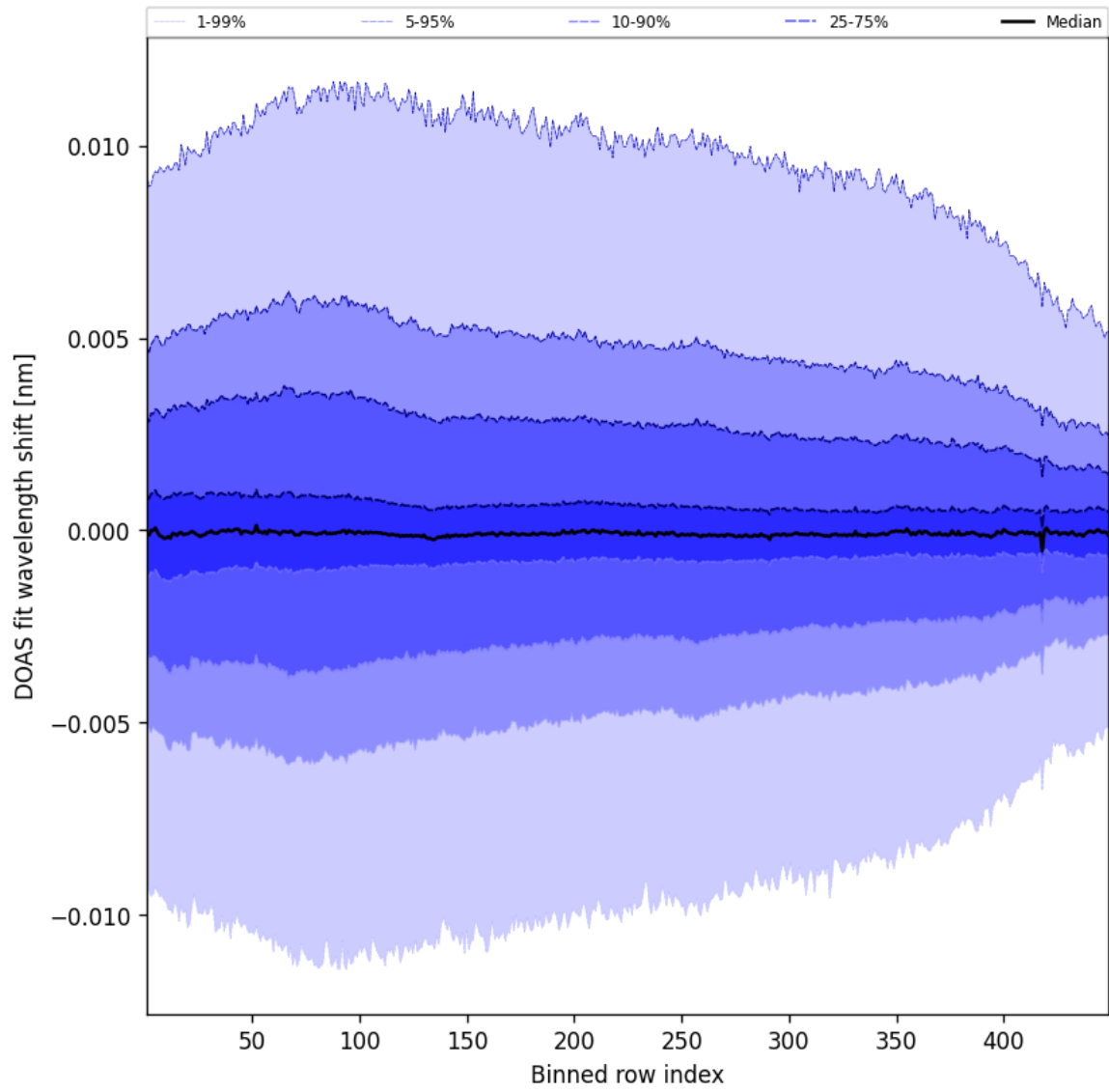
Figure 59: Along track statistics of “DOAS fit wavelength shift” for 2025-12-01 to 2025-12-01
