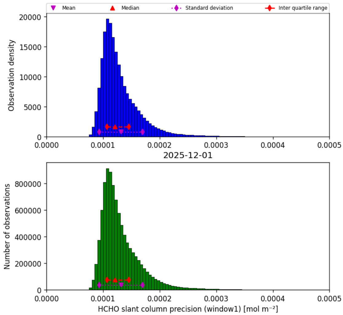
Figure 39: Histogram of “HCHO slant column precision (window1)” for 2025-12-01 to 2025-12-01
