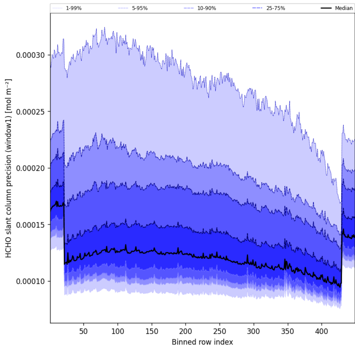
Figure 54: Along track statistics of “HCHO slant column precision (window1)” for 2025-12-01 to 2025-12-01
