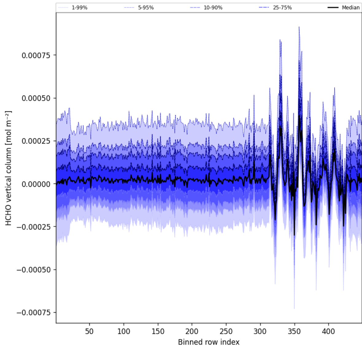
Figure 50: Along track statistics of “HCHO vertical column” for 2025-12-01 to 2025-12-01
