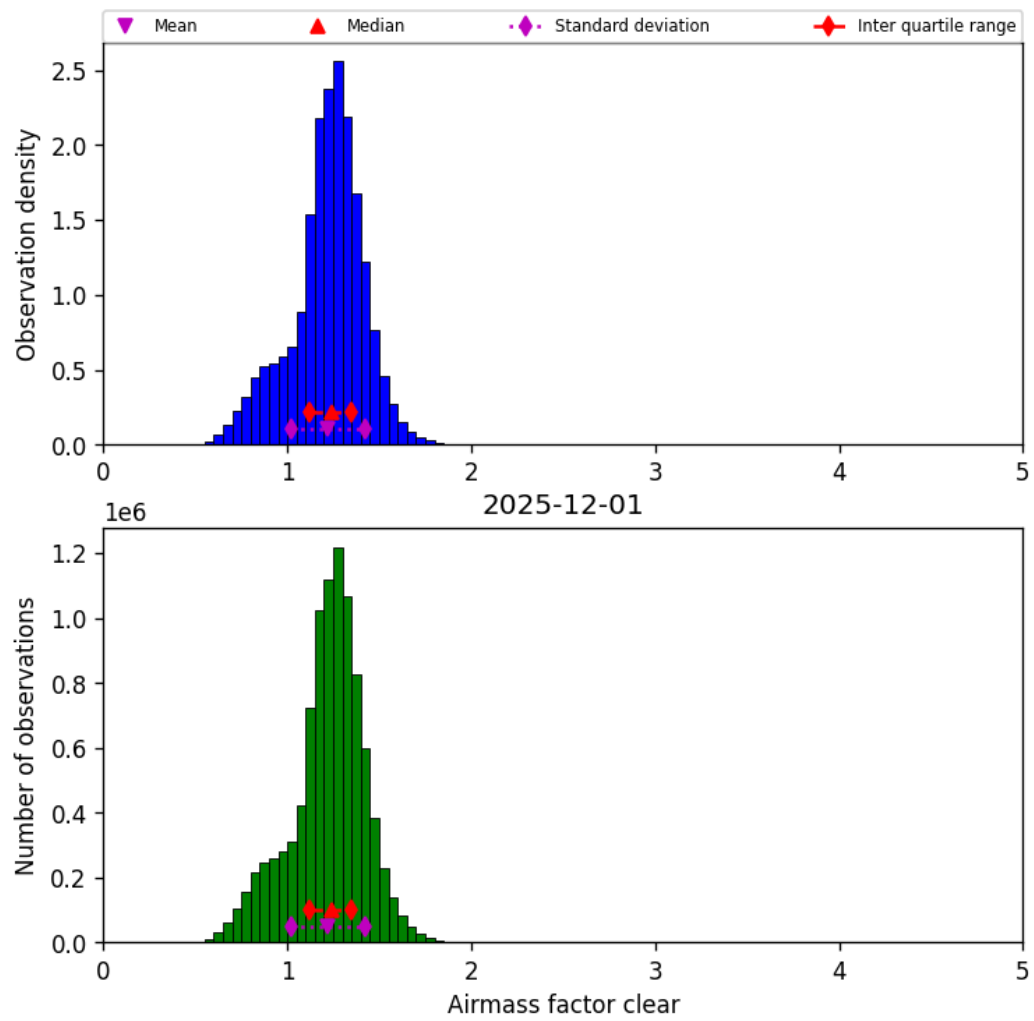
Figure 42: Histogram of “Airmass factor clear” for 2025-12-01 to 2025-12-01
