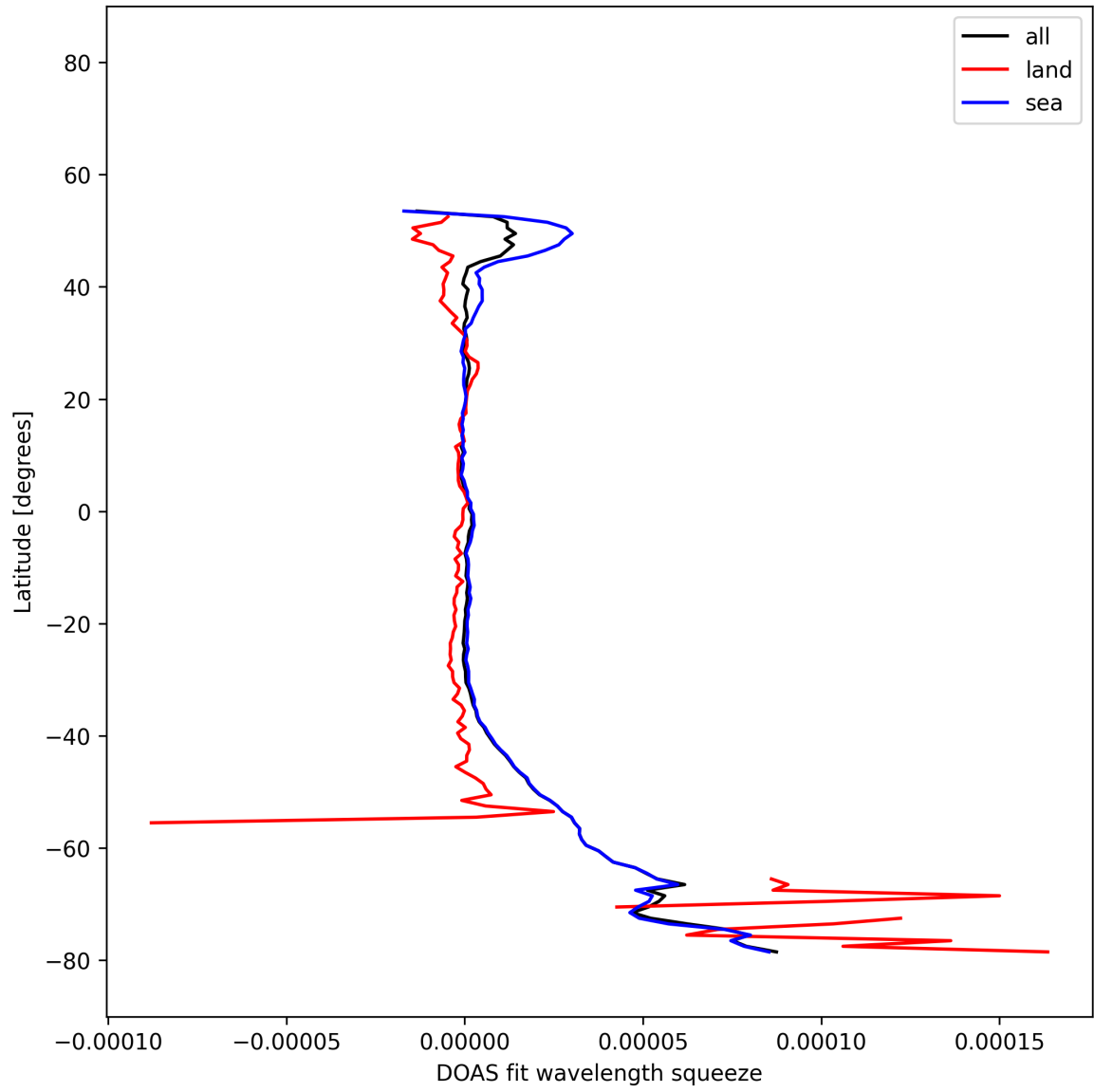
Figure 30: Zonal average of "DOAS fit wavelength squeeze" for 2025-12-01 to 2025-12-01.
