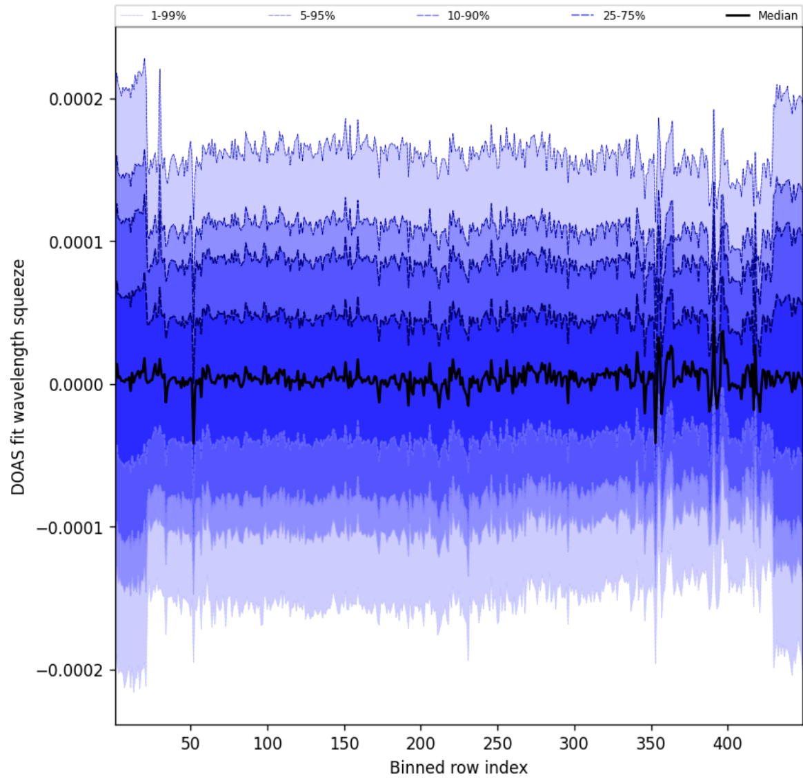
Figure 60: Along track statistics of “DOAS fit wavelength squeeze” for 2025-12-01 to 2025-12-01
