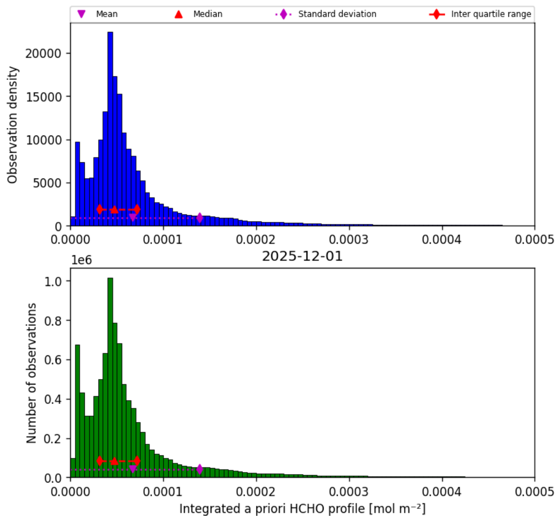
Figure 43: Histogram of “Integrated a priori HCHO profile” for 2025-12-01 to 2025-12-01
