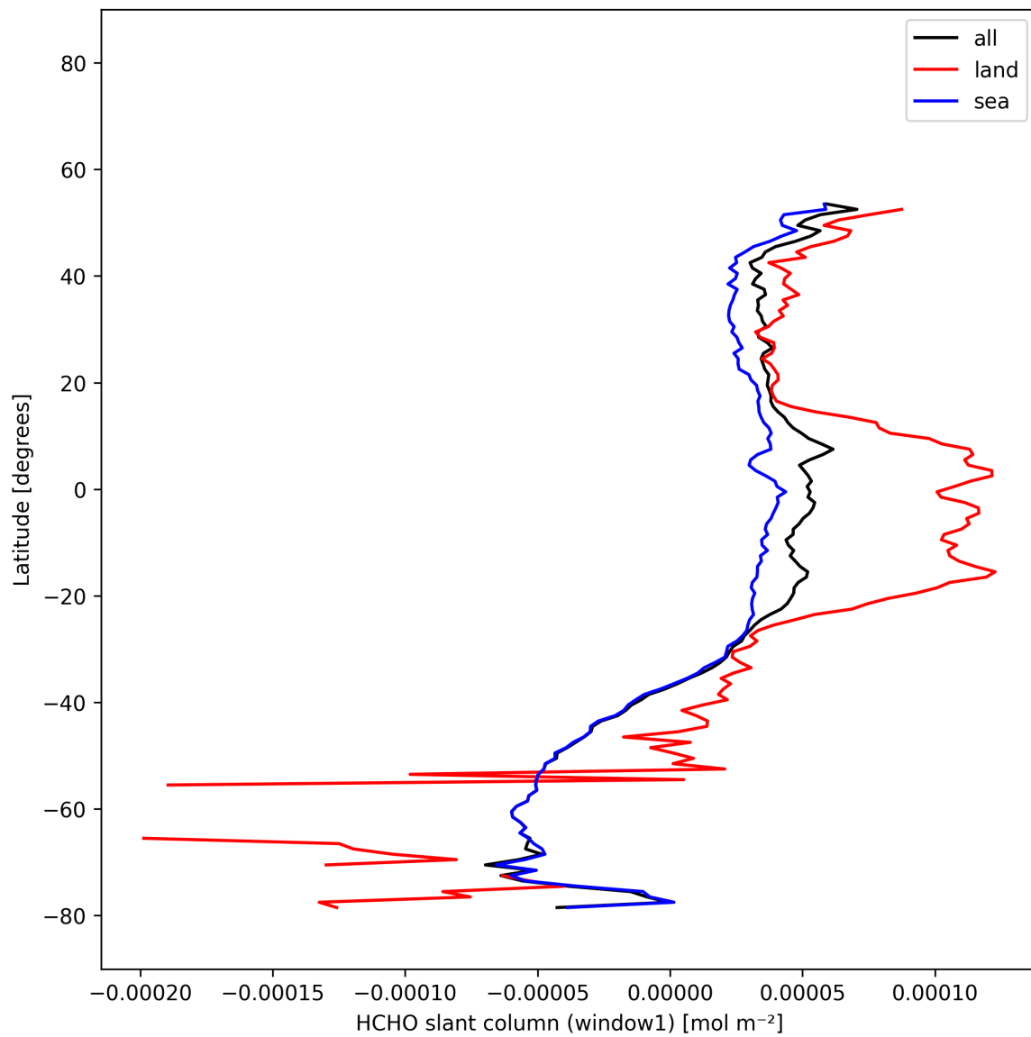
Figure 23: Zonal average of “HCHO slant column (window1)” for 2025-12-01 to 2025-12-01.
