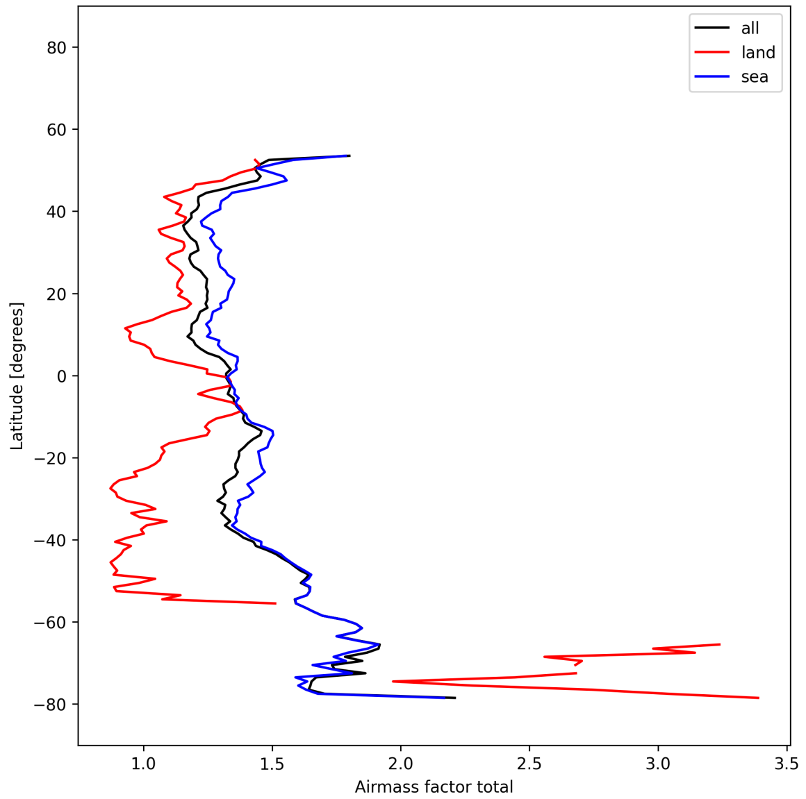
Figure 25: Zonal average of “Airmass factor total” for 2025-12-01 to 2025-12-01.
