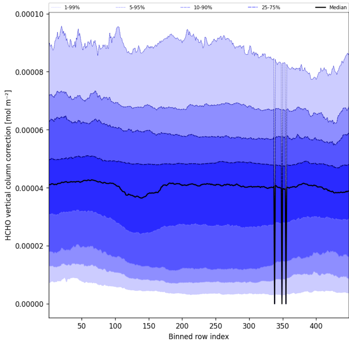
Figure 52: Along track statistics of "HCHO vertical column correction" for 2025-12-01 to 2025-12-01
