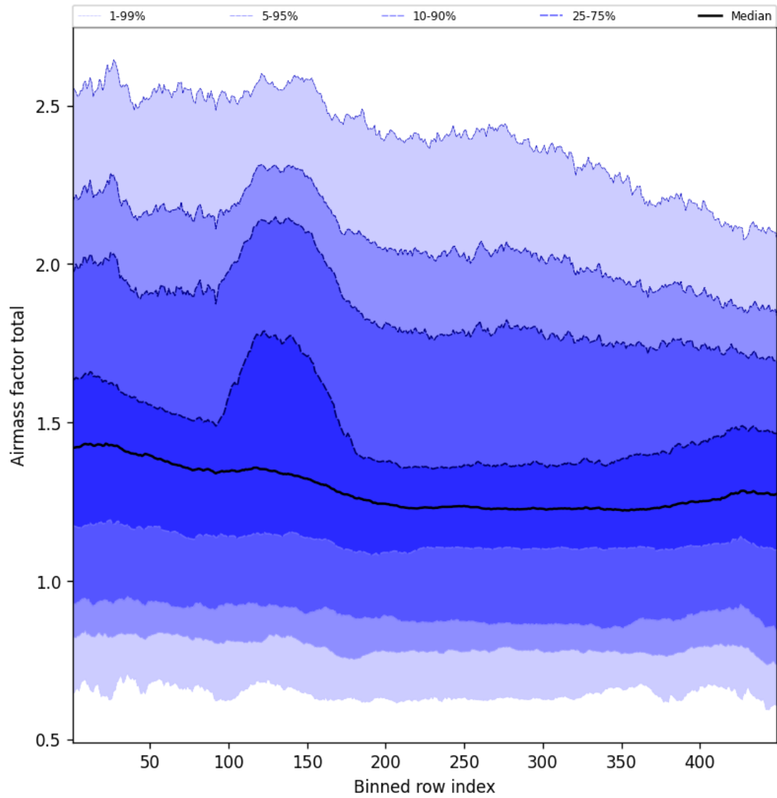
Figure 55: Along track statistics of “Airmass factor total” for 2025-12-01 to 2025-12-01
