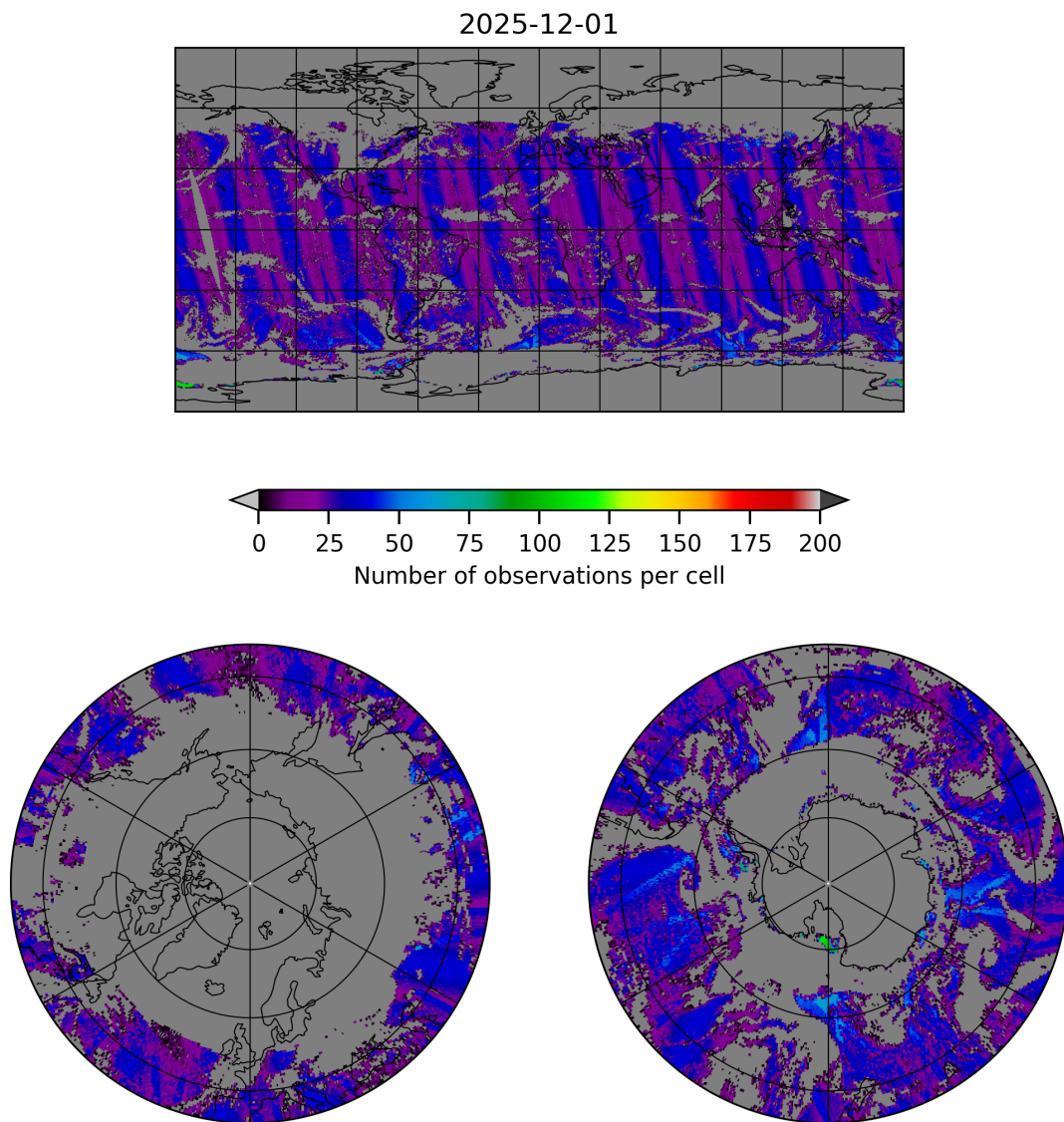
Figure 18: Map of the number of observations for 2025-12-01 to 2025-12-01
