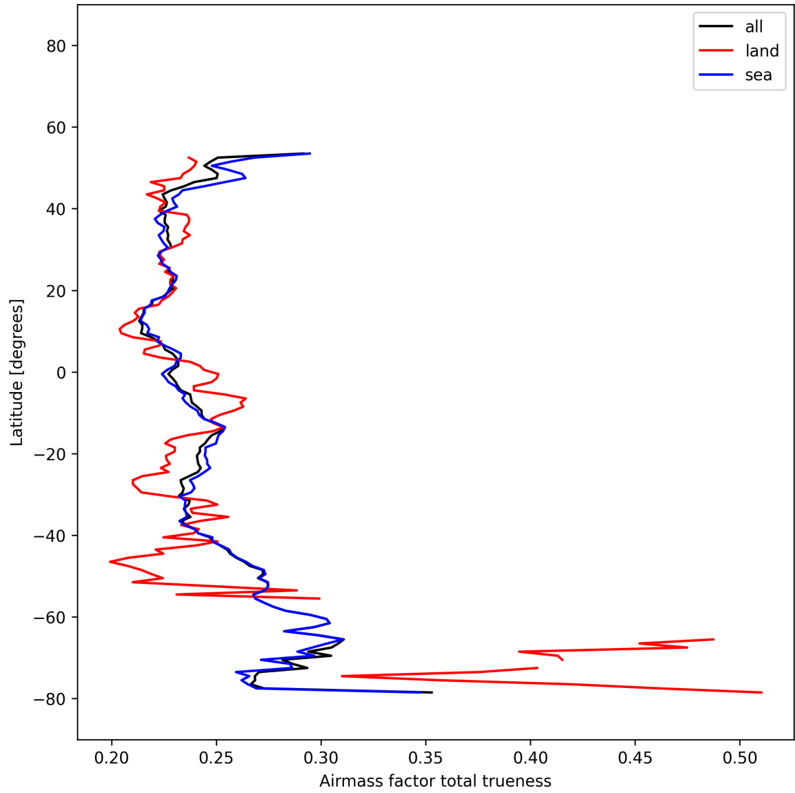
Figure 26: Zonal average of “Airmass factor total trueness” for 2025-12-01 to 2025-12-01.
