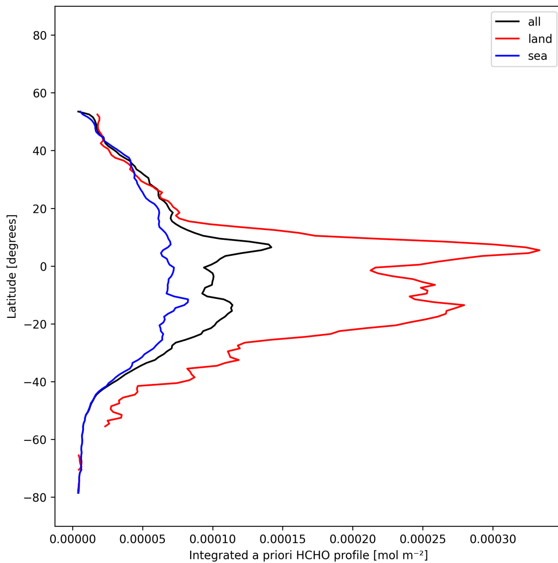
Figure 28: Zonal average of “Integrated a priori HCHO profile” for 2025-12-01 to 2025-12-01.
