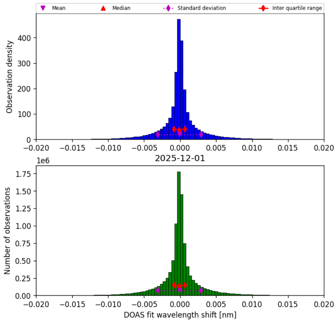
Figure 44: Histogram of “DOAS fit wavelength shift” for 2025-12-01 to 2025-12-01
