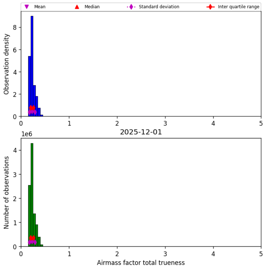
Figure 41: Histogram of “Airmass factor total trueness” for 2025-12-01 to 2025-12-01
