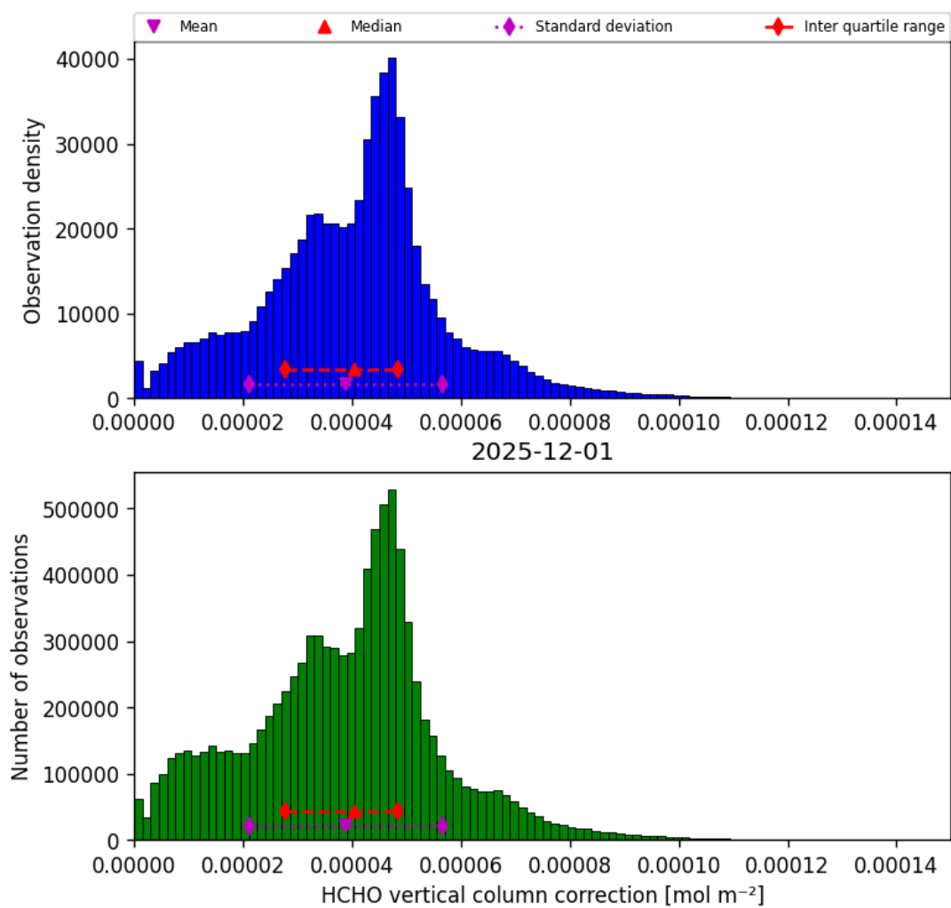
Figure 37: Histogram of “HCHO vertical column correction” for 2025-12-01 to 2025-12-01
