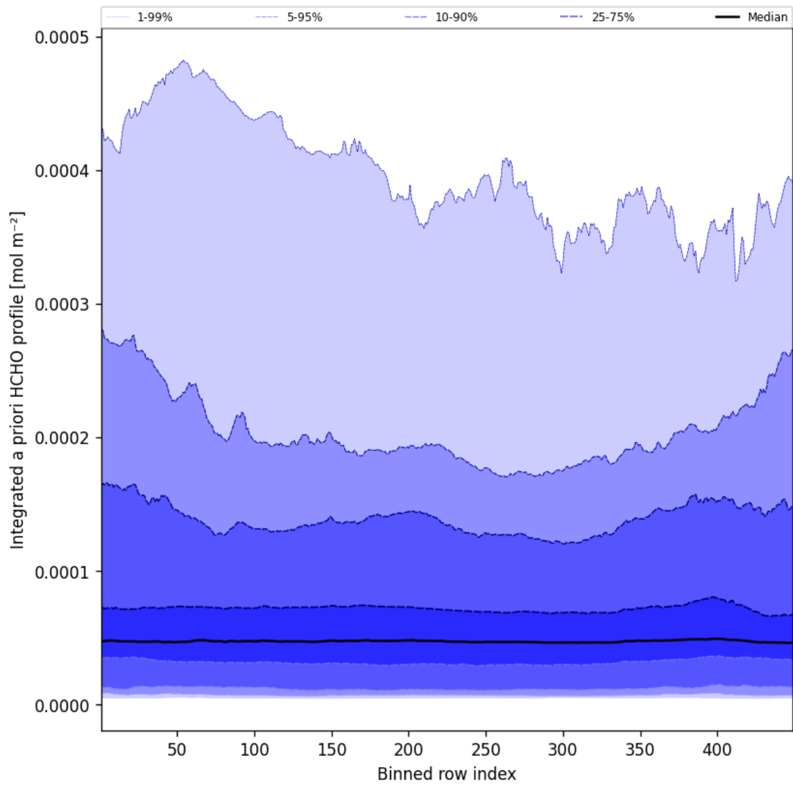
Figure 58: Along track statistics of “Integrated a priori HCHO profile” for 2025-12-01 to 2025-12-01
