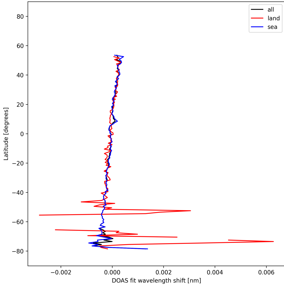
Figure 29: Zonal average of “DOAS fit wavelength shift” for 2025-12-01 to 2025-12-01.
