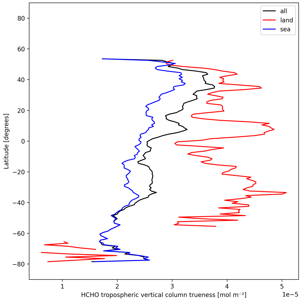
Figure 33: Zonal average of “HCHO tropospheric vertical column trueness” for 2025-12-01 to 2025-12-01.
