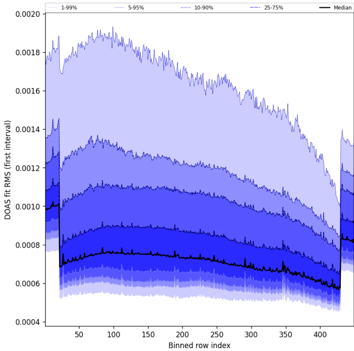
Figure 61: Along track statistics of “DOAS fit RMS (first interval)” for 2025-12-01 to 2025-12-01
