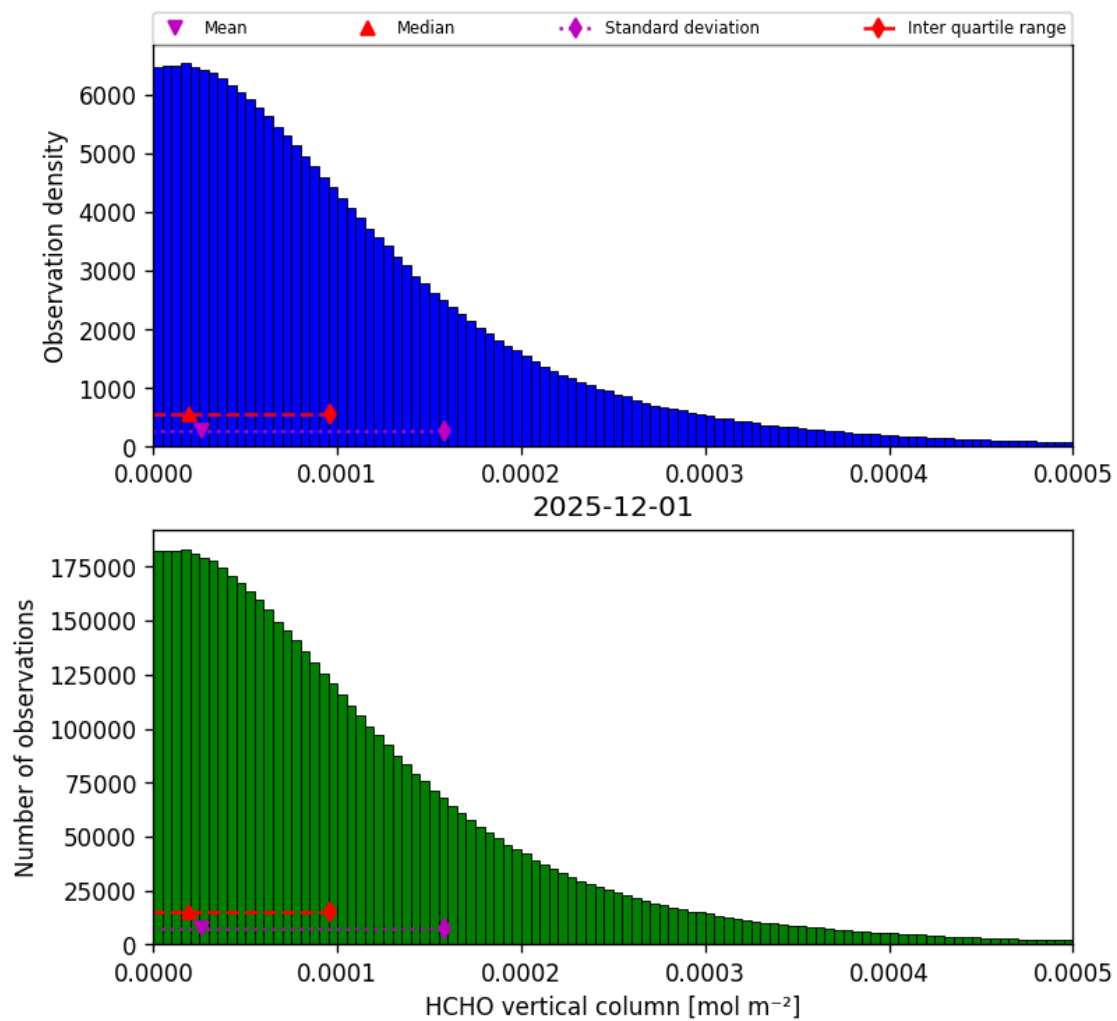
Figure 35: Histogram of “HCHO vertical column” for 2025-12-01 to 2025-12-01
