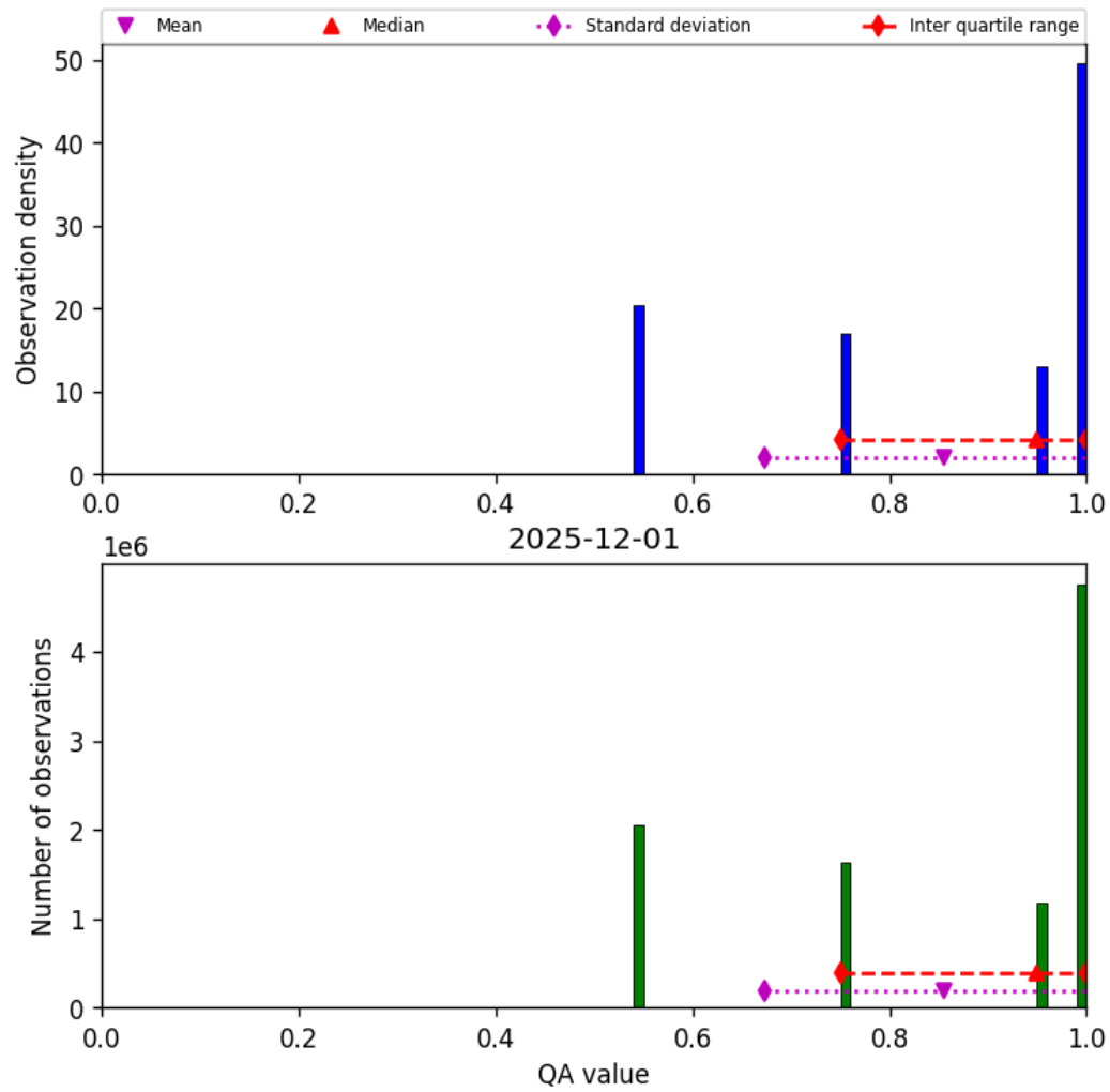
Figure 34: Histogram of “QA value” for 2025-12-01 to 2025-12-01
