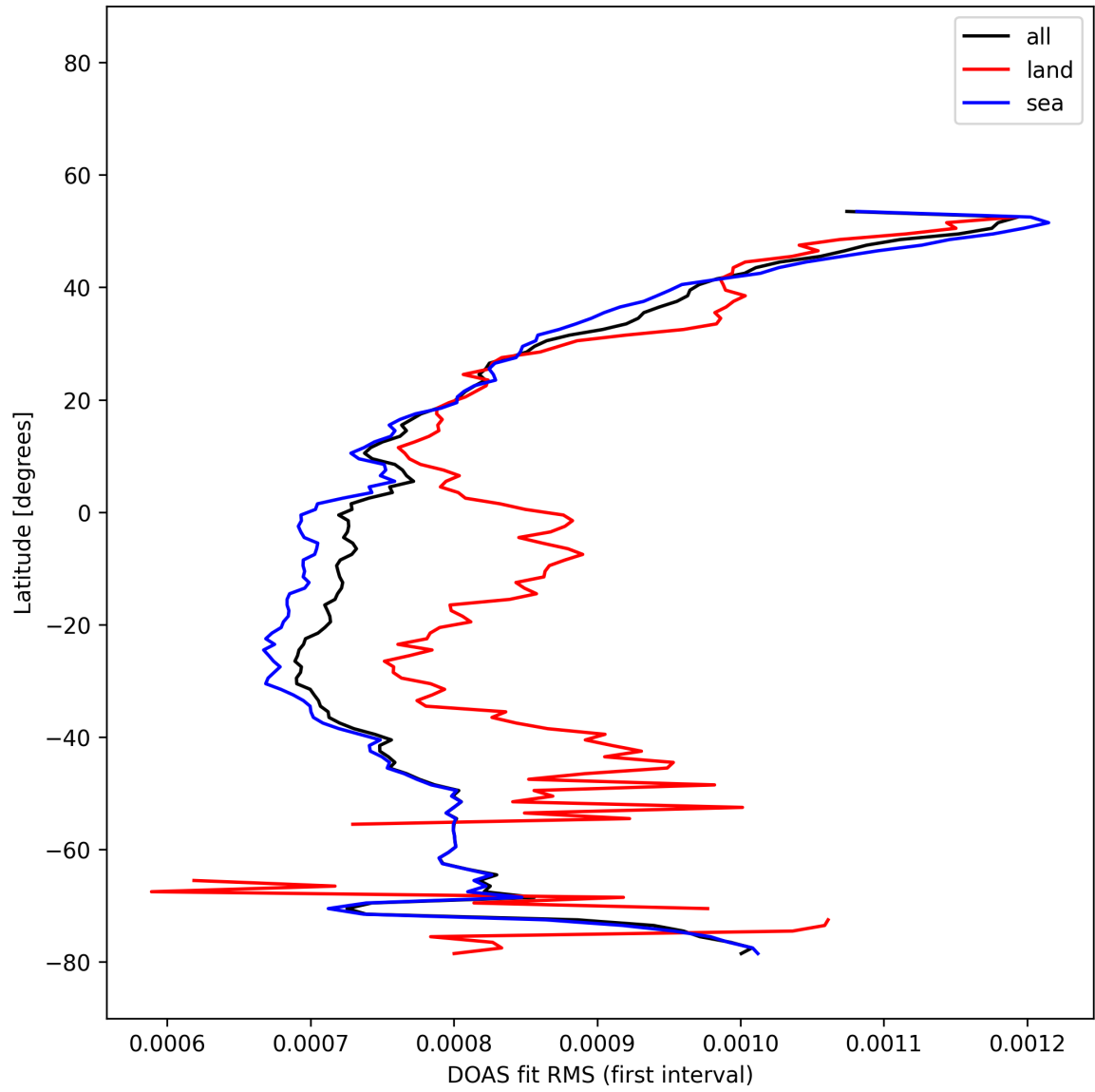
Figure 31: Zonal average of “DOAS fit RMS (first interval)” for 2025-12-01 to 2025-12-01.
