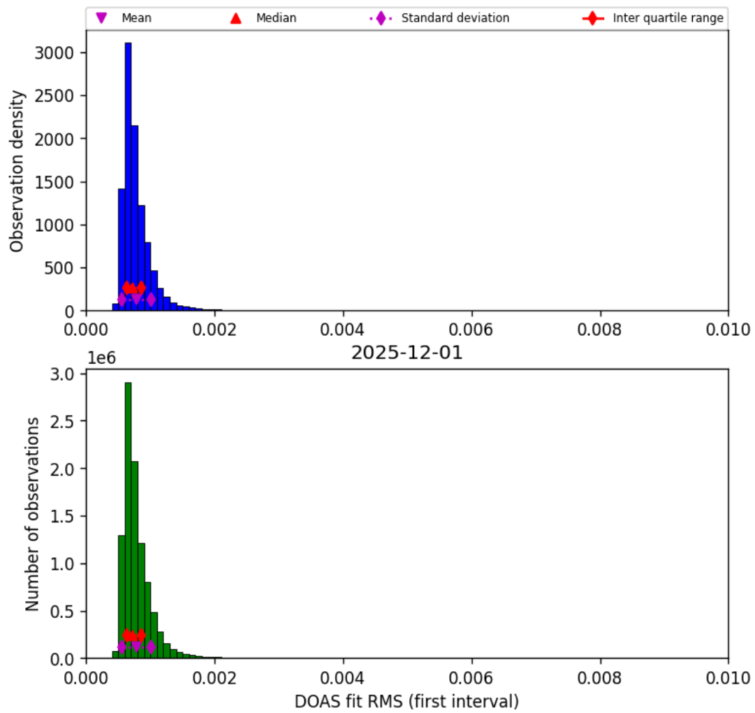
Figure 46: Histogram of “DOAS fit RMS (first interval)” for 2025-12-01 to 2025-12-01
