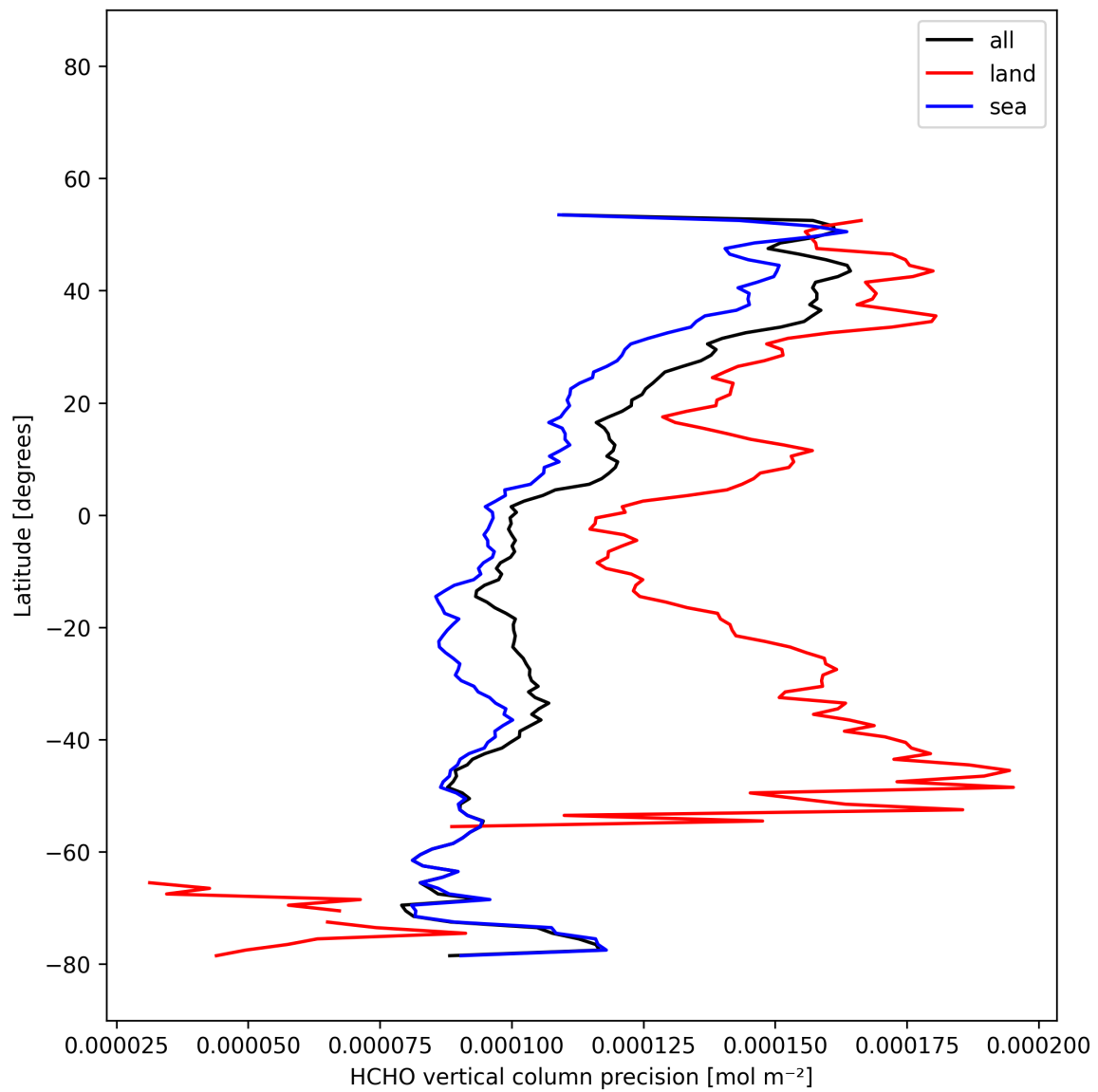
Figure 21: Zonal average of “HCHO vertical column precision” for 2025-12-01 to 2025-12-01.
