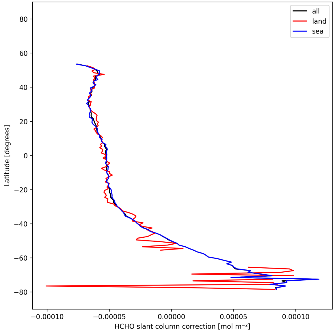
Figure 32: Zonal average of “HCHO slant column correction” for 2025-12-01 to 2025-12-01.
