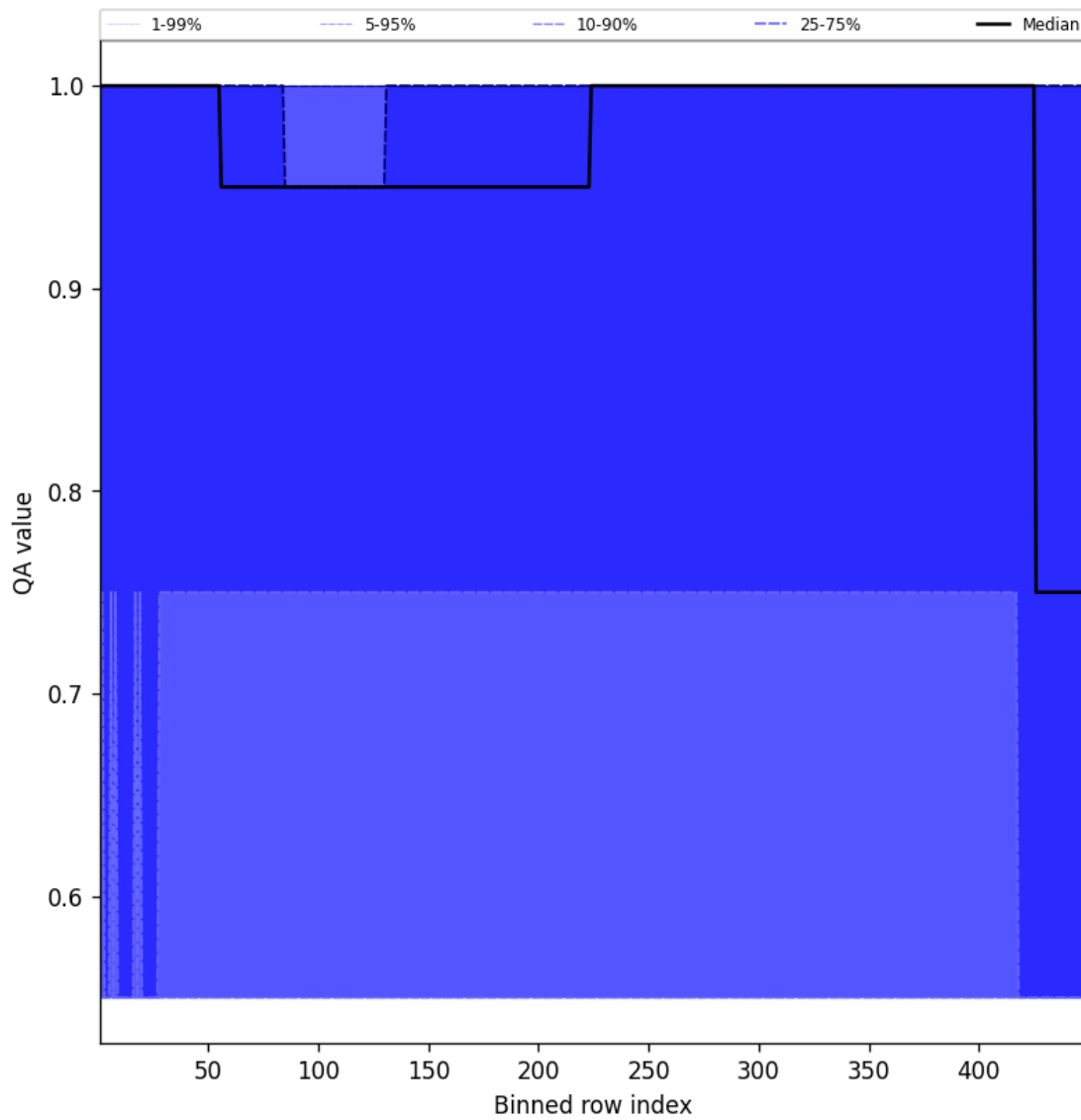
Figure 49: Along track statistics of “QA value” for 2025-12-01 to 2025-12-01
