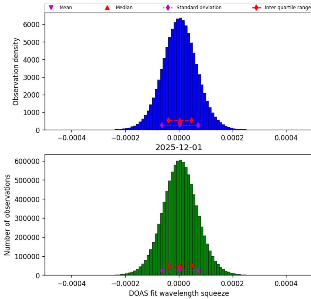
Figure 45: Histogram of “DOAS fit wavelength squeeze” for 2025-12-01 to 2025-12-01
