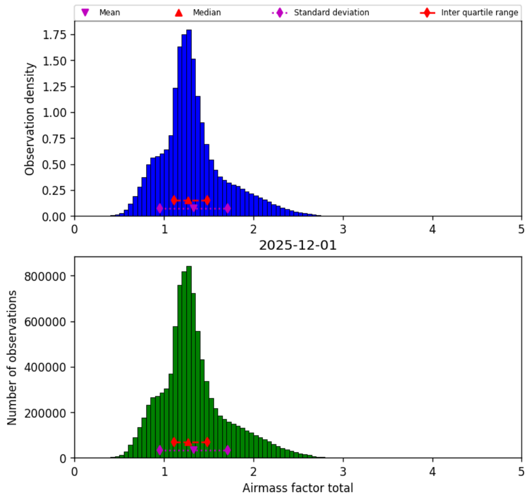
Figure 40: Histogram of “Airmass factor total” for 2025-12-01 to 2025-12-01
