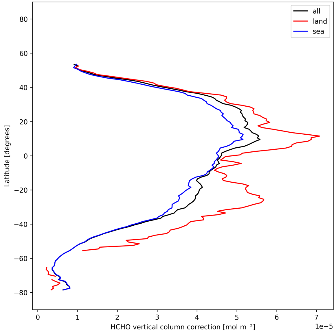
Figure 22: Zonal average of “HCHO vertical column correction” for 2025-12-01 to 2025-12-01.
