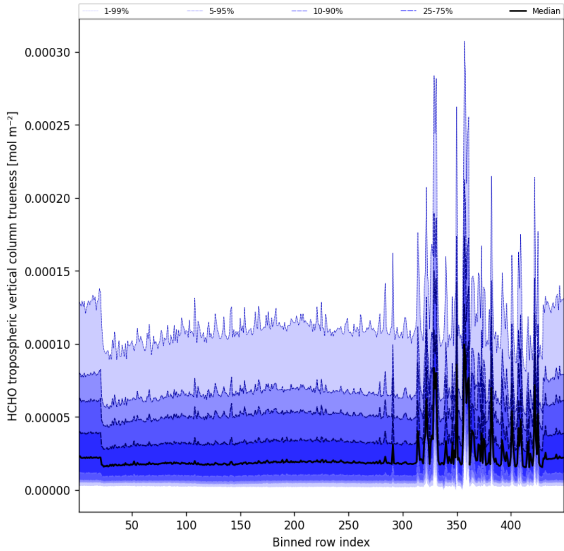
Figure 63: Along track statistics of “HCHO tropospheric vertical column trueness” for 2025-12-01 to 2025-12-01
