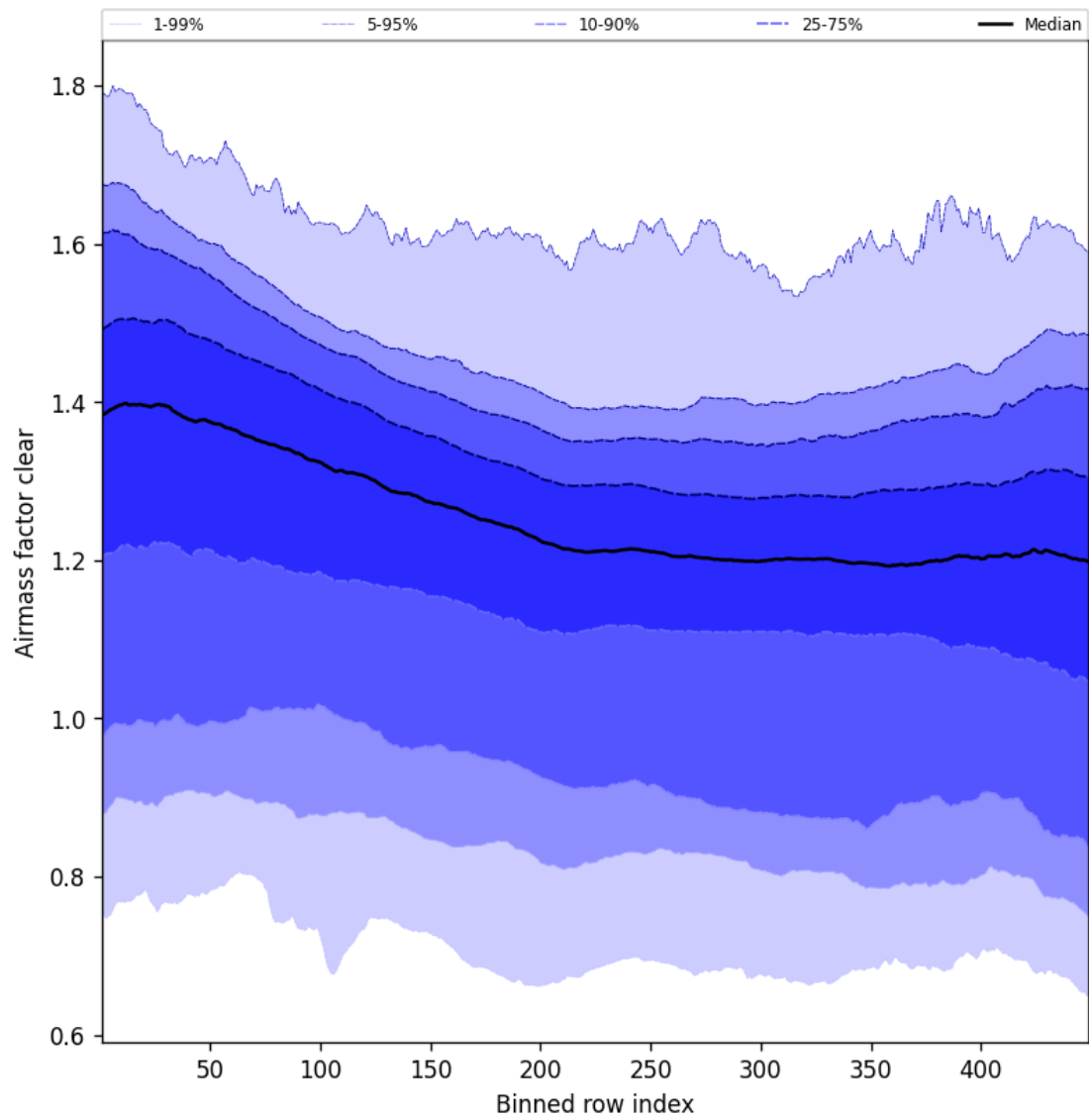
Figure 57: Along track statistics of “Airmass factor clear” for 2025-12-01 to 2025-12-01
