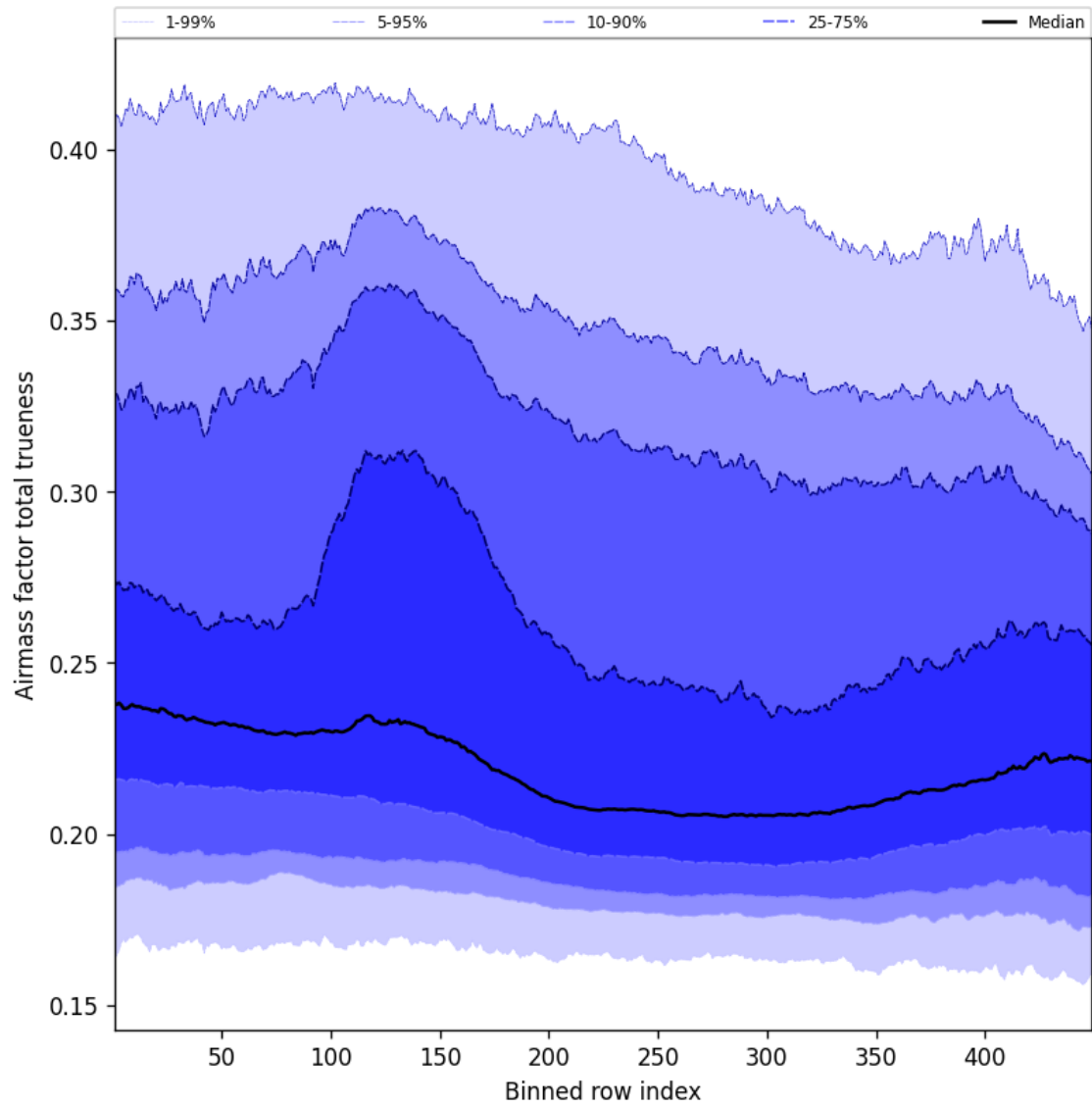
Figure 56: Along track statistics of “Airmass factor total trueness” for 2025-12-02 to 2025-12-02
