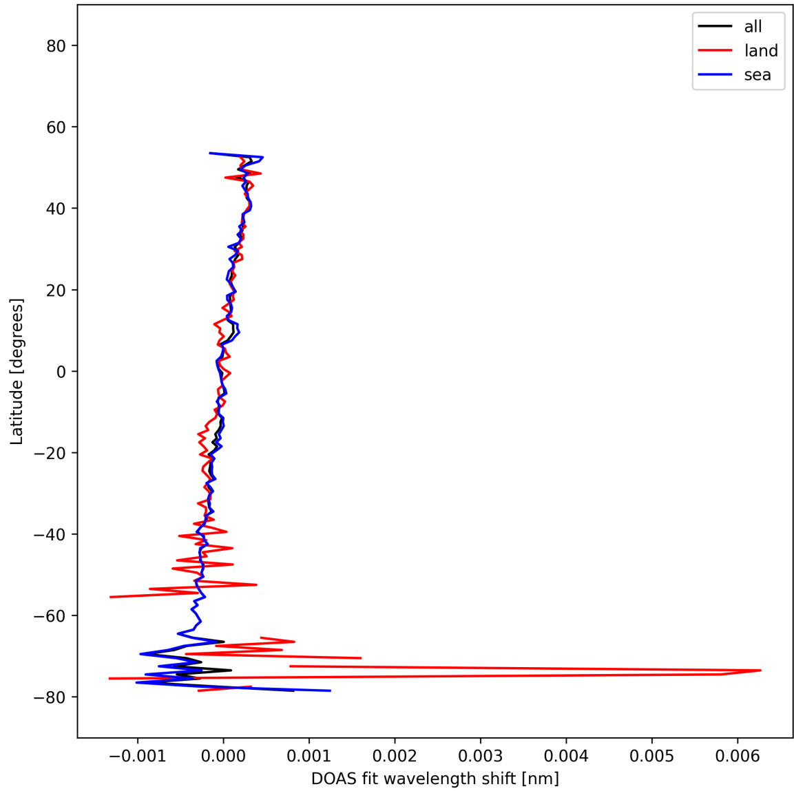
Figure 29: Zonal average of "DOAS fit wavelength shift" for 2025-12-02 to 2025-12-02.
