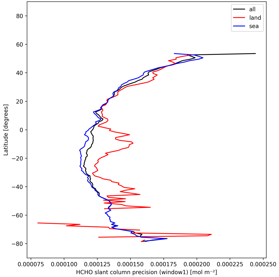
Figure 24: Zonal average of “HCHO slant column precision (window1)” for 2025-12-02 to 2025-12-02.
