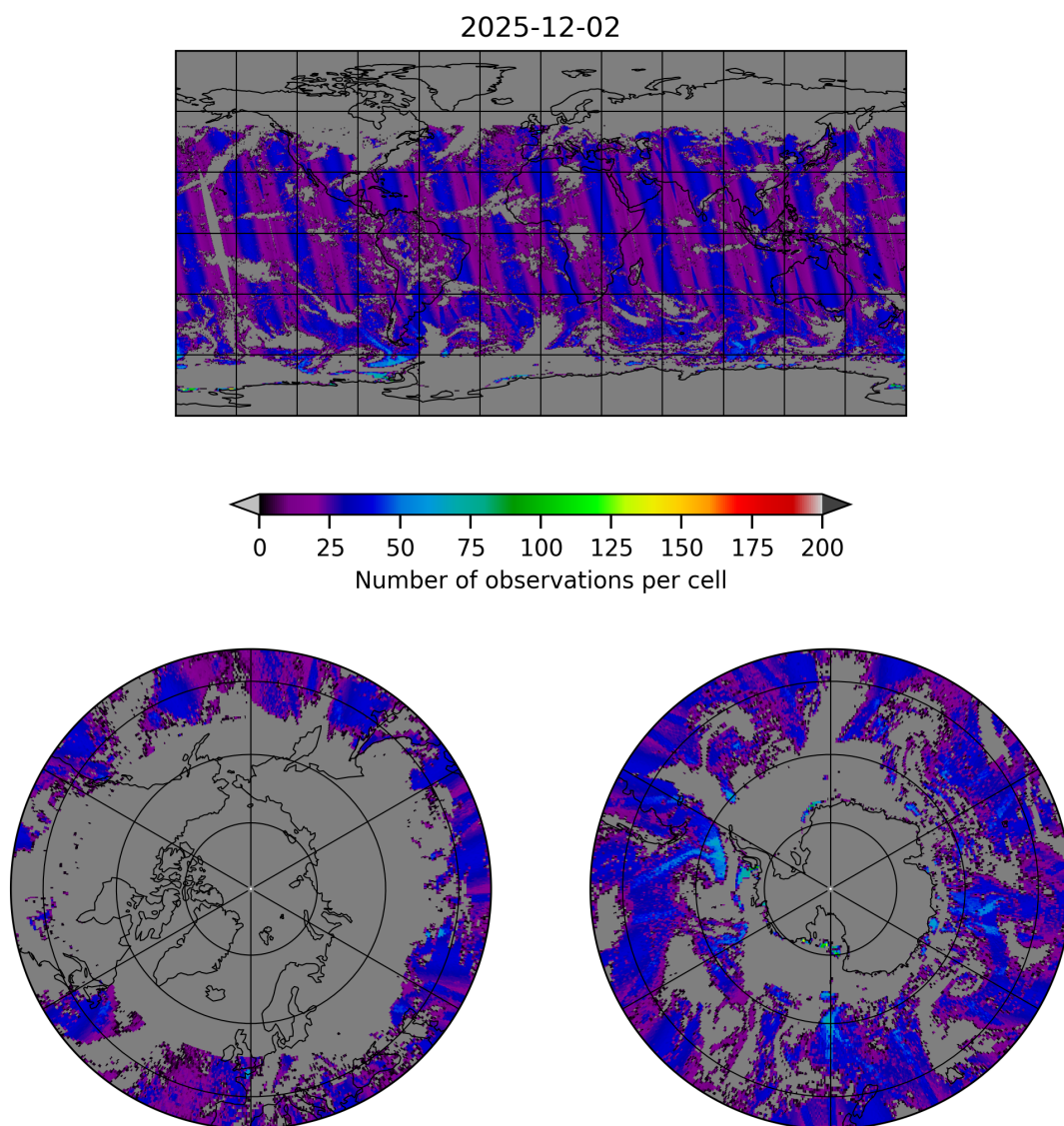
Figure 18: Map of the number of observations for 2025-12-02 to 2025-12-02
