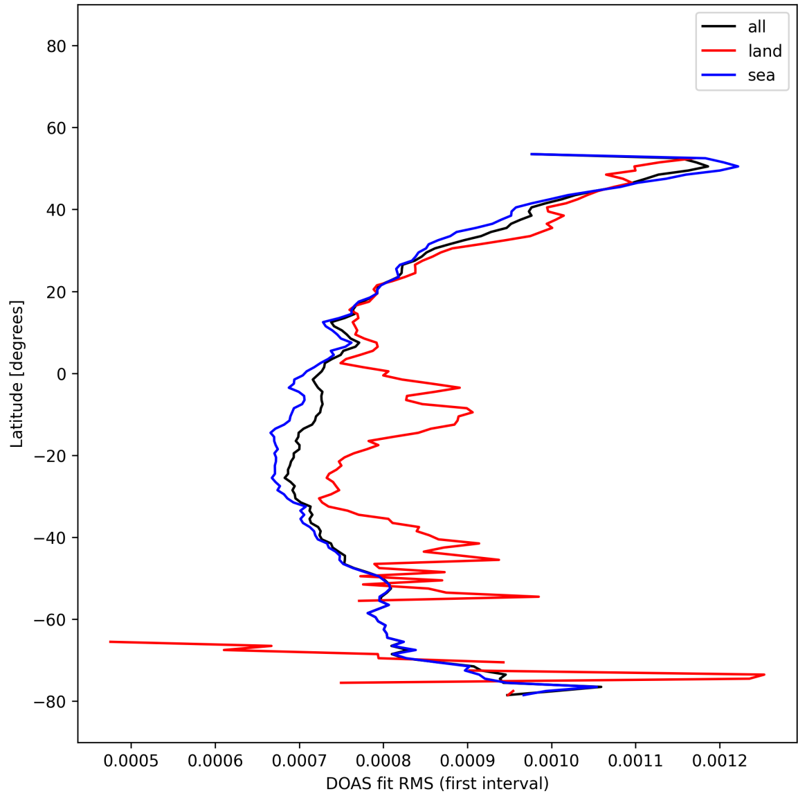
Figure 31: Zonal average of “DOAS fit RMS (first interval)” for 2025-12-02 to 2025-12-02.
