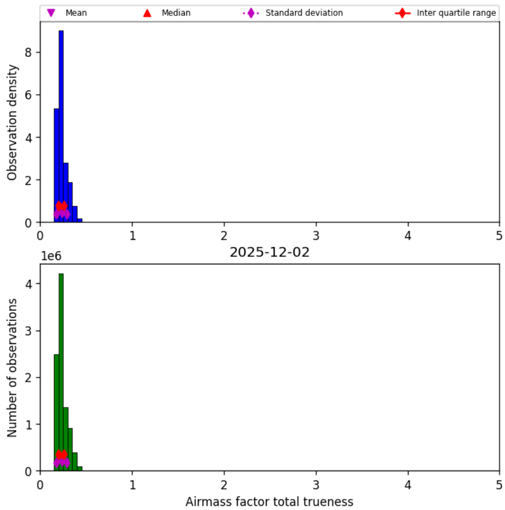
Figure 41: Histogram of “Airmass factor total trueness” for 2025-12-02 to 2025-12-02
