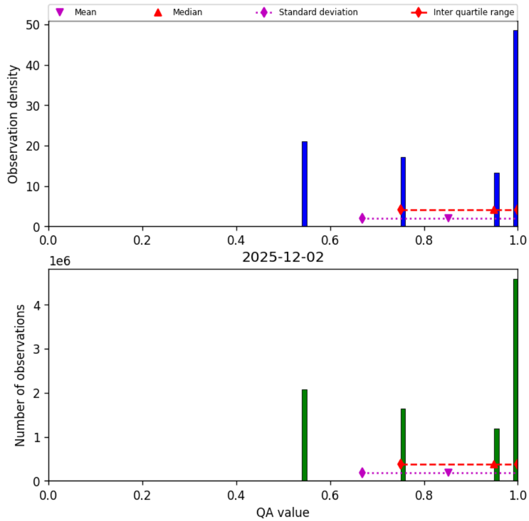
Figure 34: Histogram of “QA value” for 2025-12-02 to 2025-12-02
