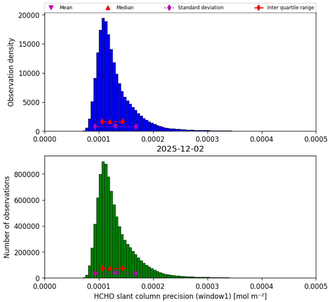
Figure 39: Histogram of "HCHO slant column precision (window1)" for 2025-12-02 to 2025-12-02
