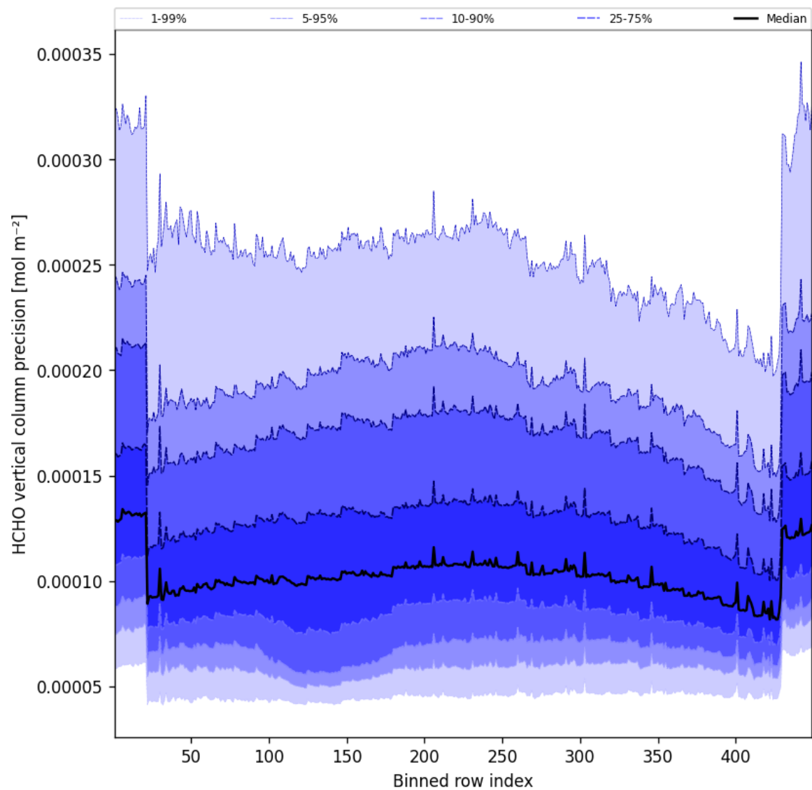
Figure 51: Along track statistics of “HCHO vertical column precision” for 2025-12-02 to 2025-12-02
