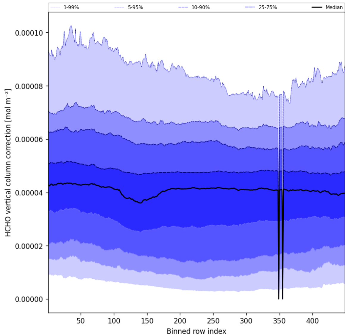
Figure 52: Along track statistics of “HCHO vertical column correction” for 2025-12-02 to 2025-12-02
