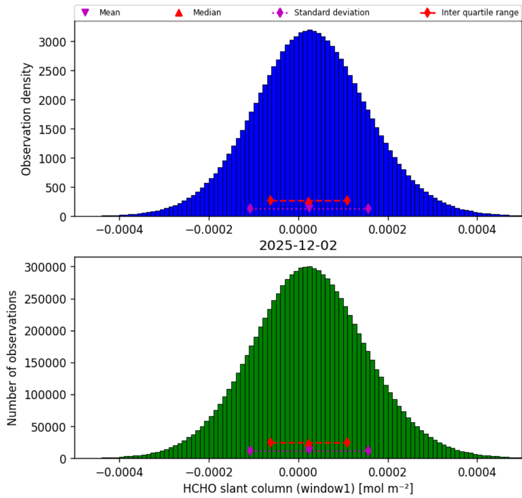
Figure 38: Histogram of "HCHO slant column (window1)" for 2025-12-02 to 2025-12-02
