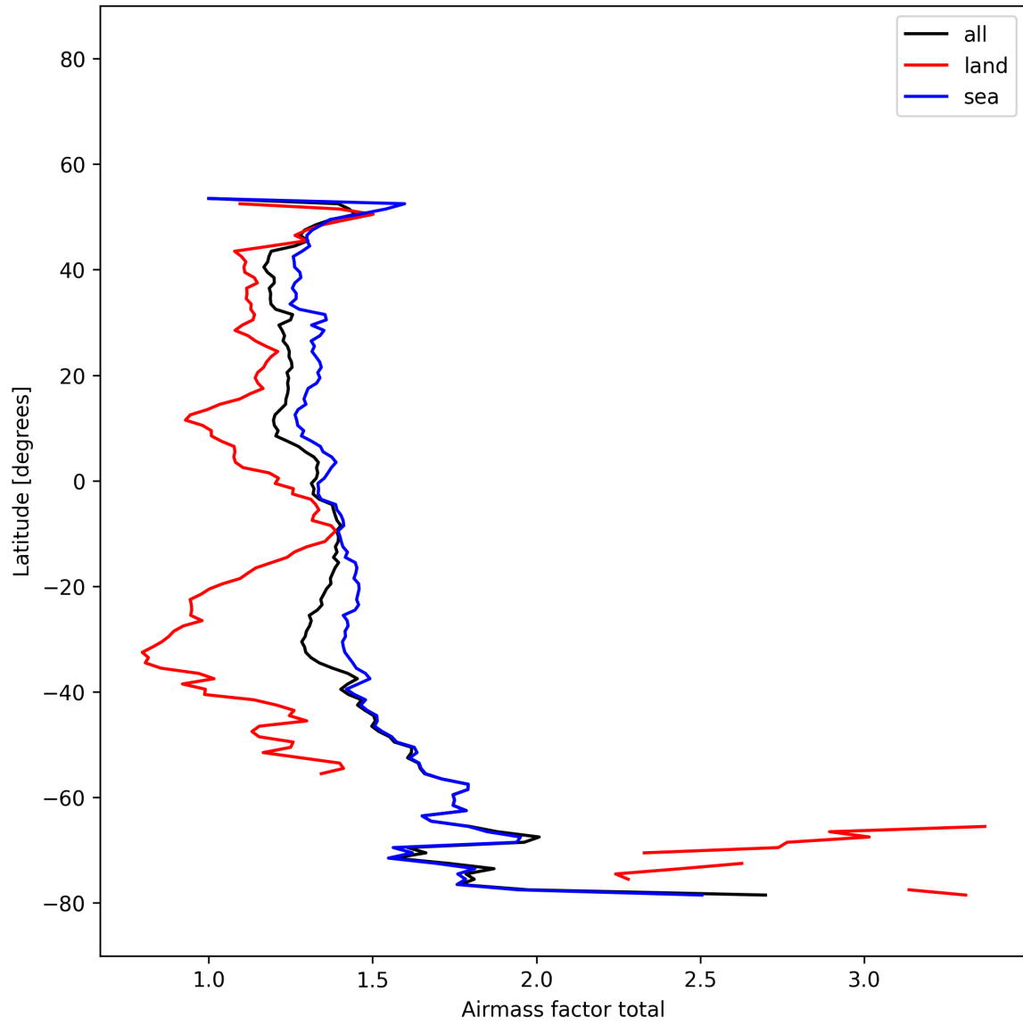
Figure 25: Zonal average of “Airmass factor total” for 2025-12-02 to 2025-12-02.
