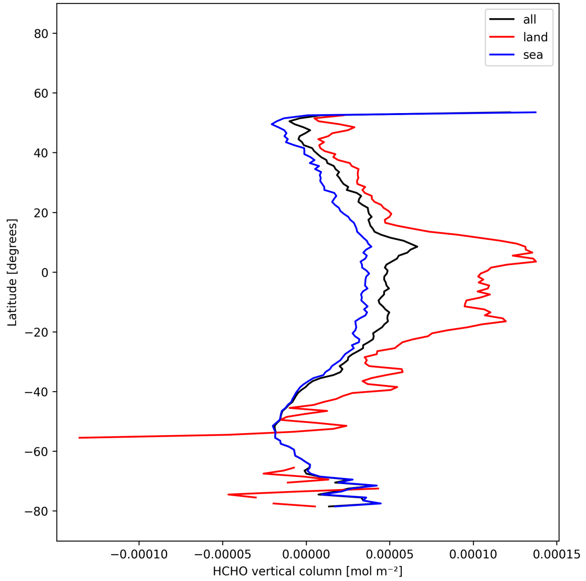
Figure 20: Zonal average of “HCHO vertical column” for 2025-12-02 to 2025-12-02.
