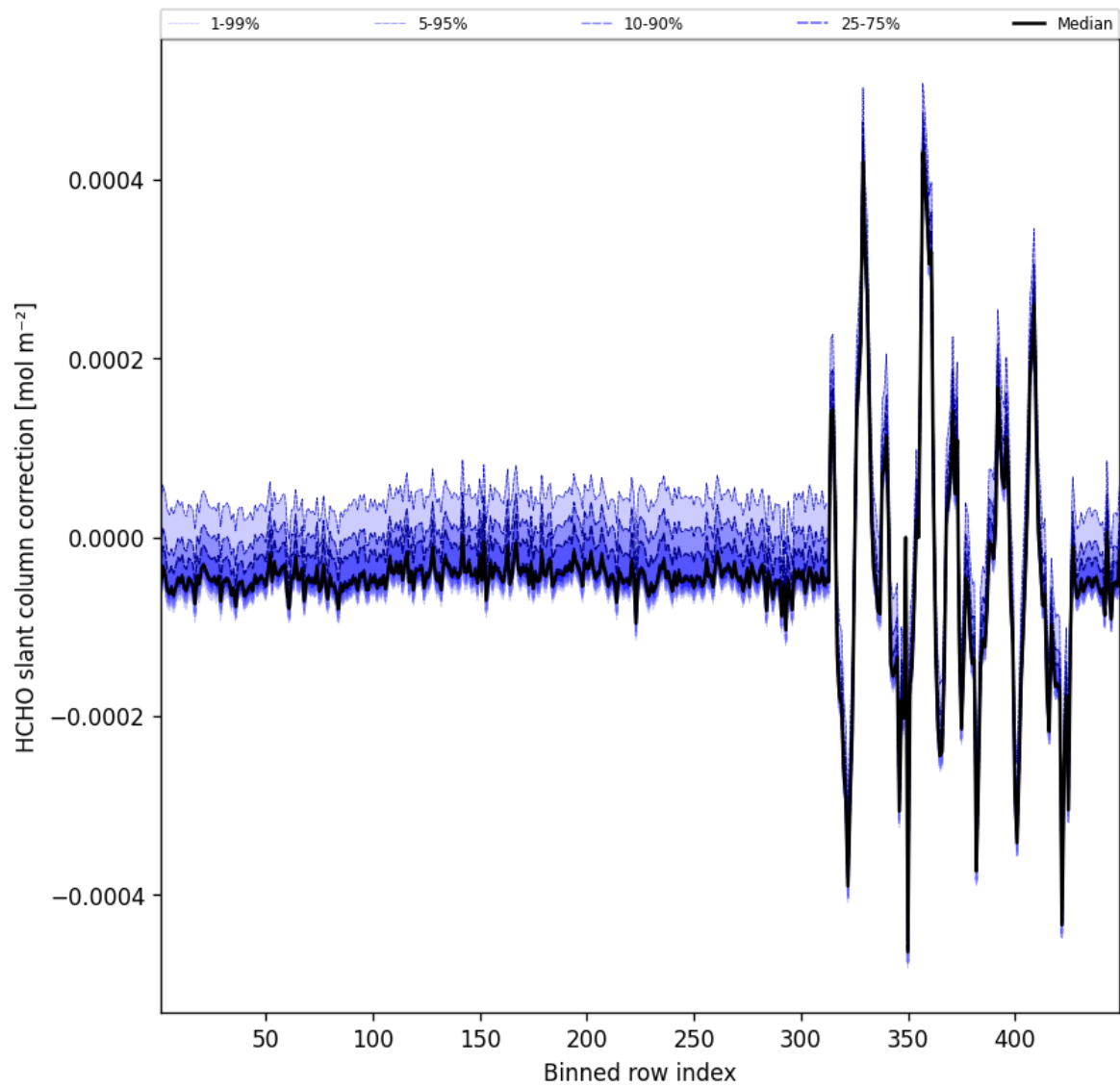
Figure 62: Along track statistics of “HCHO slant column correction” for 2025-12-02 to 2025-12-02
