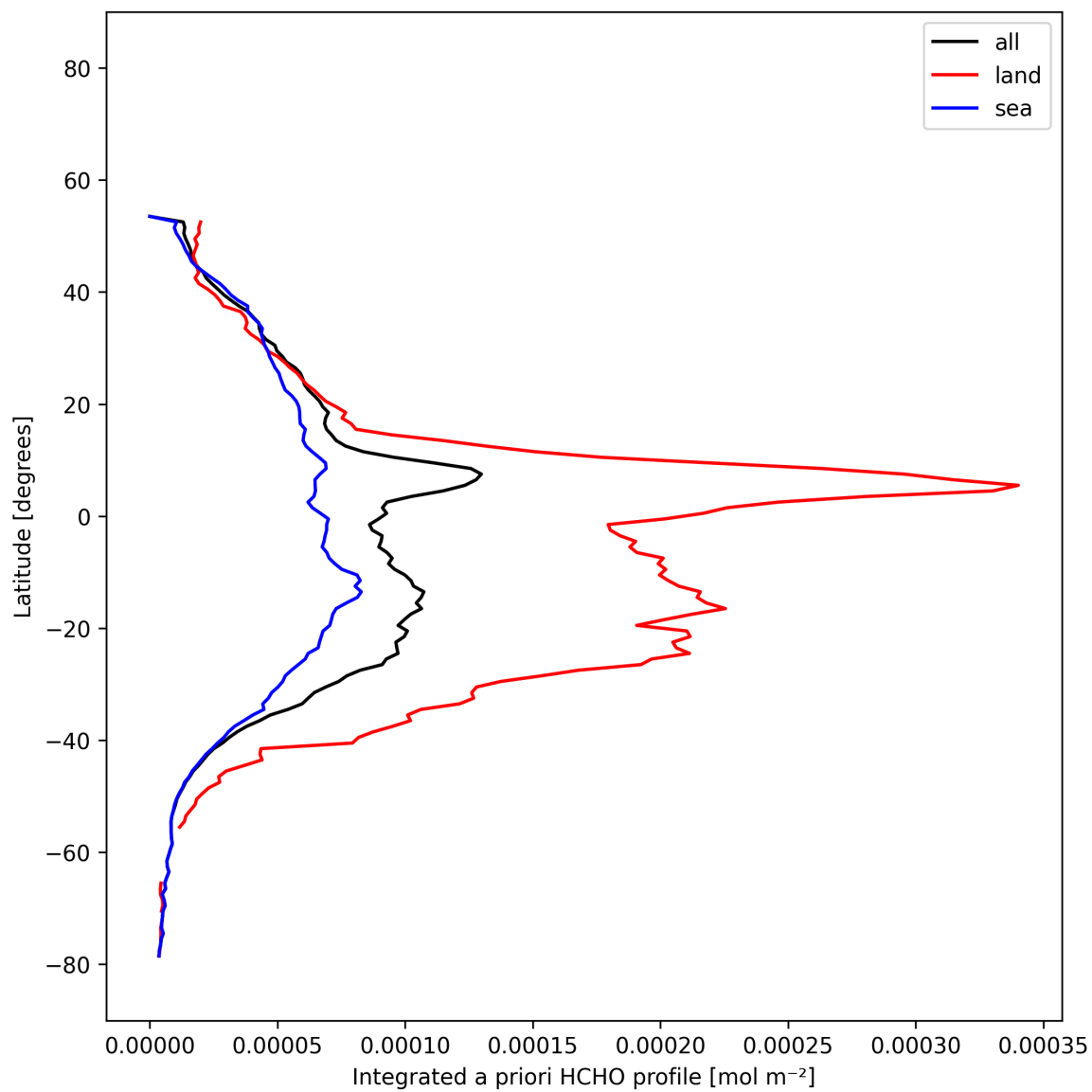
Figure 28: Zonal average of “Integrated a priori HCHO profile” for 2025-12-02 to 2025-12-02.
