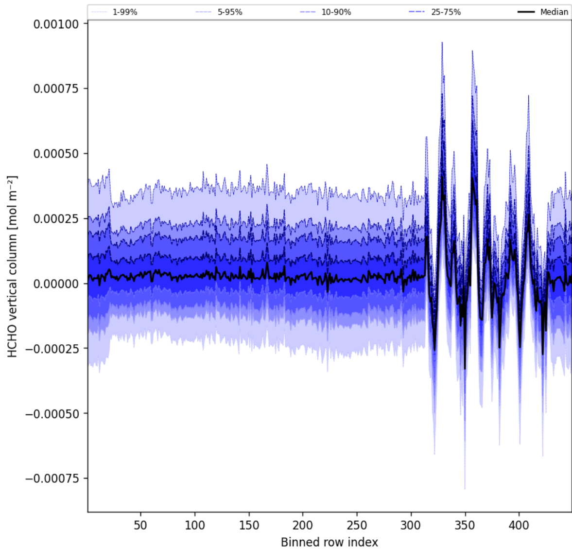
Figure 50: Along track statistics of “HCHO vertical column” for 2025-12-02 to 2025-12-02
