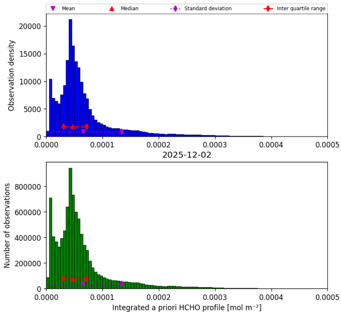
Figure 43: Histogram of “Integrated a priori HCHO profile” for 2025-12-02 to 2025-12-02
