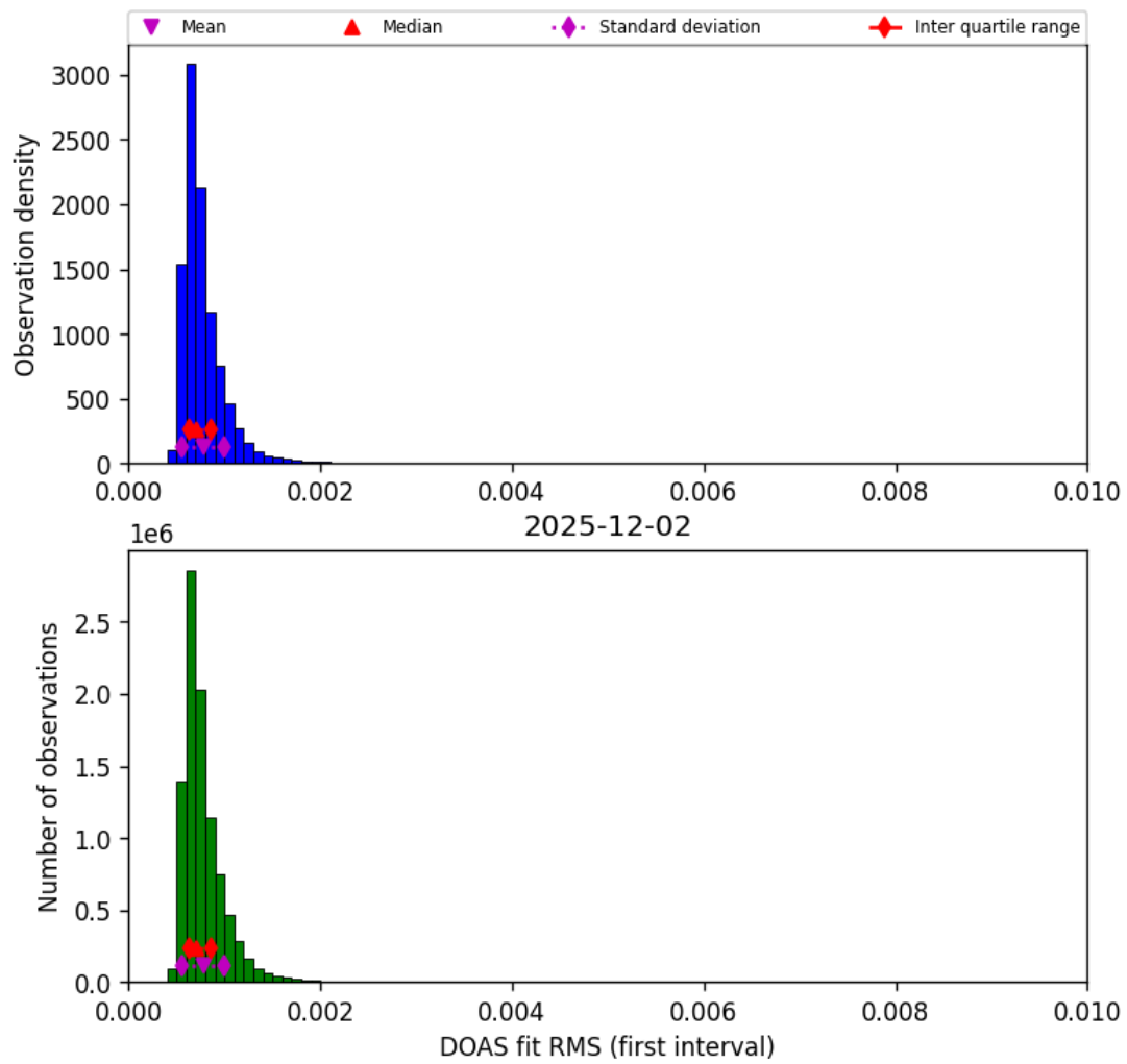
Figure 46: Histogram of “DOAS fit RMS (first interval)” for 2025-12-02 to 2025-12-02
