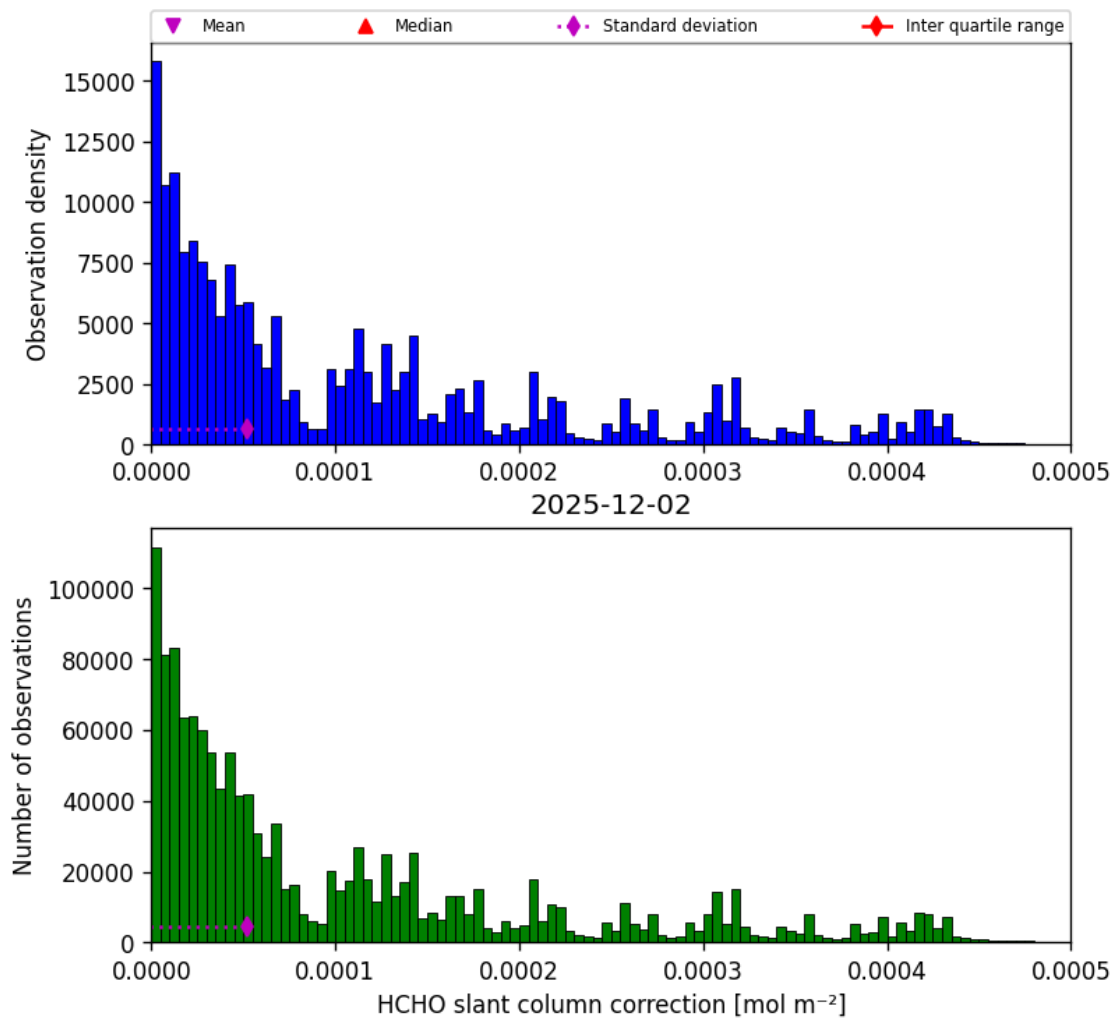
Figure 47: Histogram of “HCHO slant column correction” for 2025-12-02 to 2025-12-02
