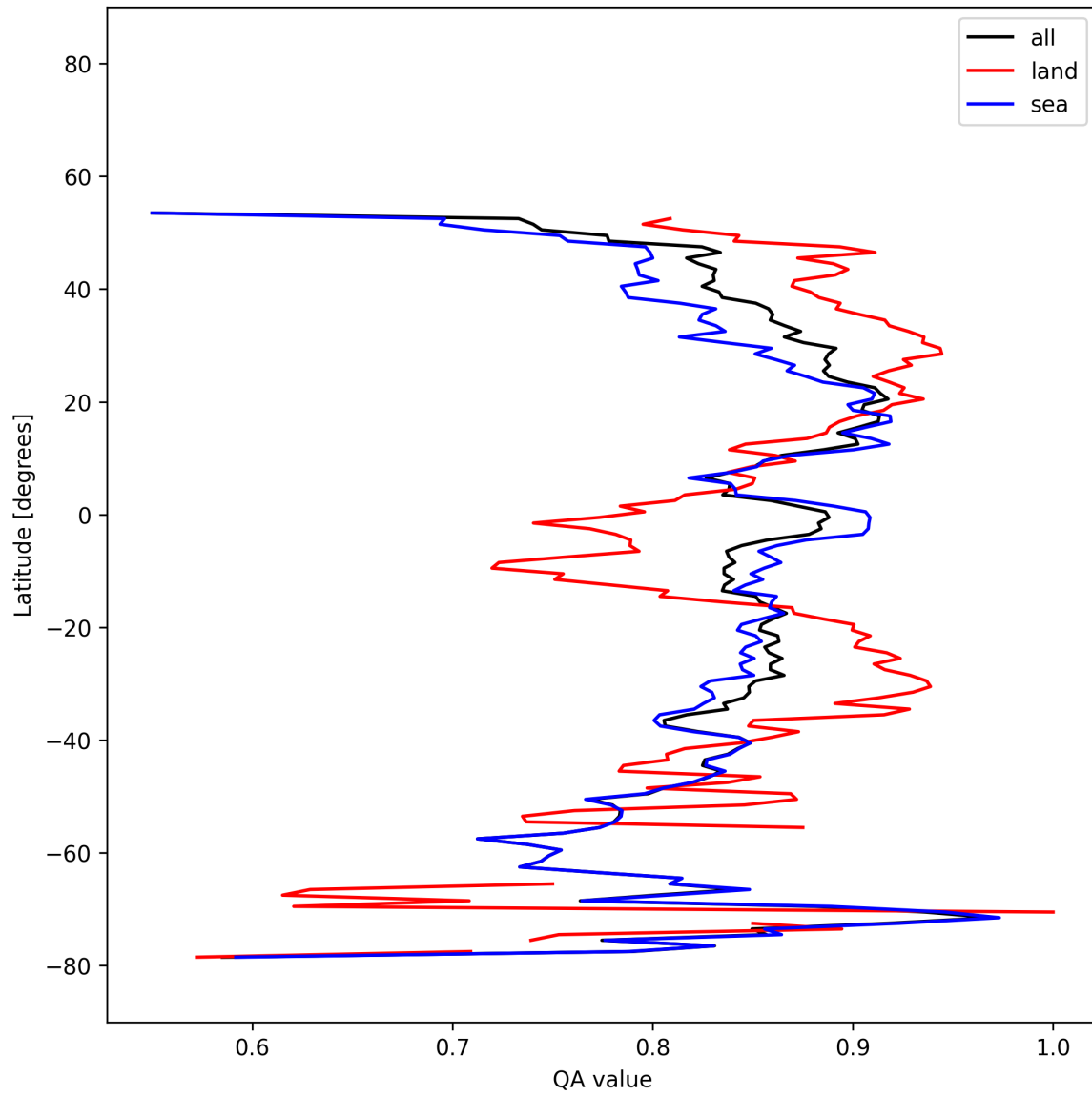
Figure 19: Zonal average of “QA value” for 2025-12-02 to 2025-12-02.
