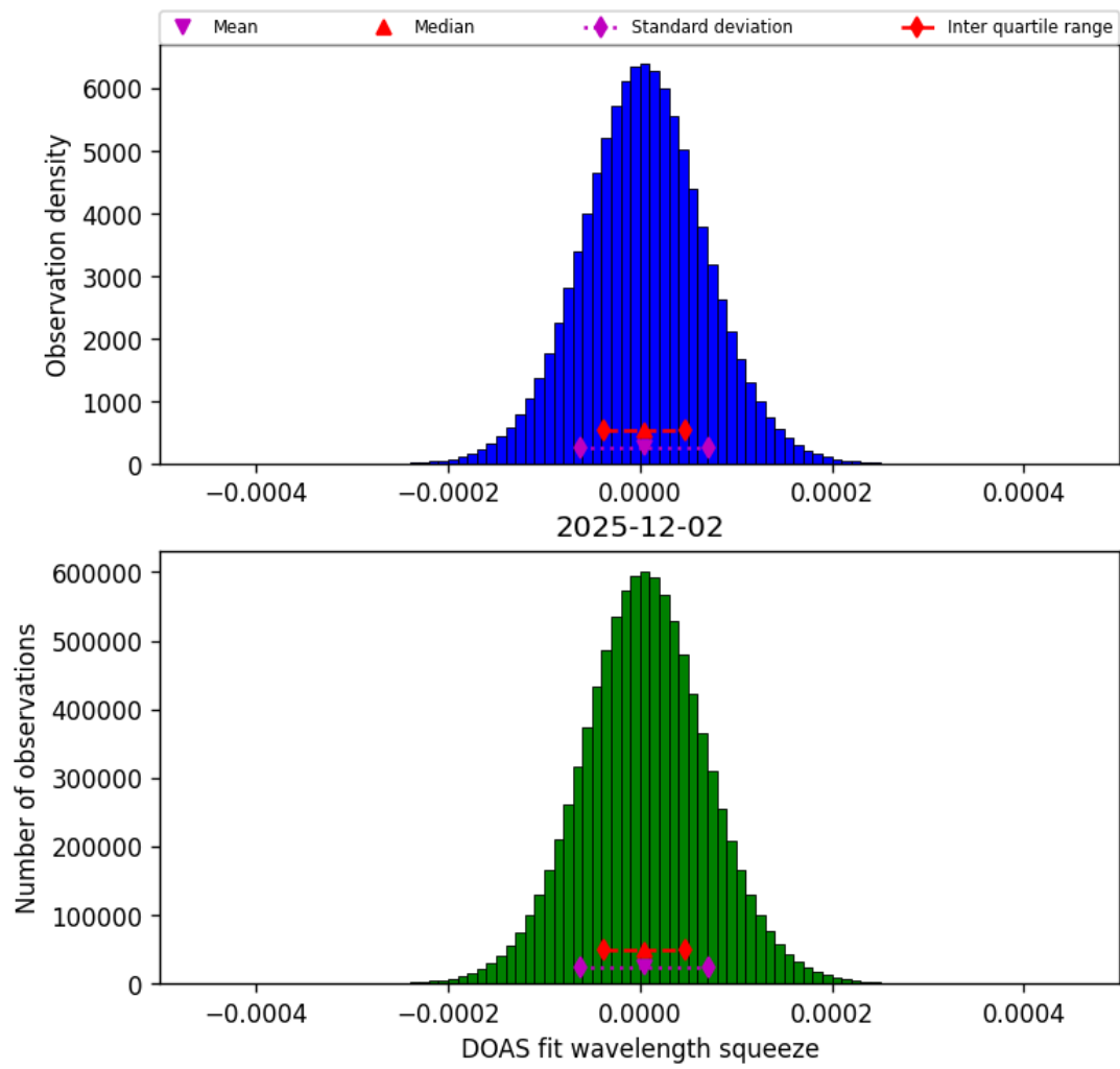
Figure 45: Histogram of “DOAS fit wavelength squeeze” for 2025-12-02 to 2025-12-02
