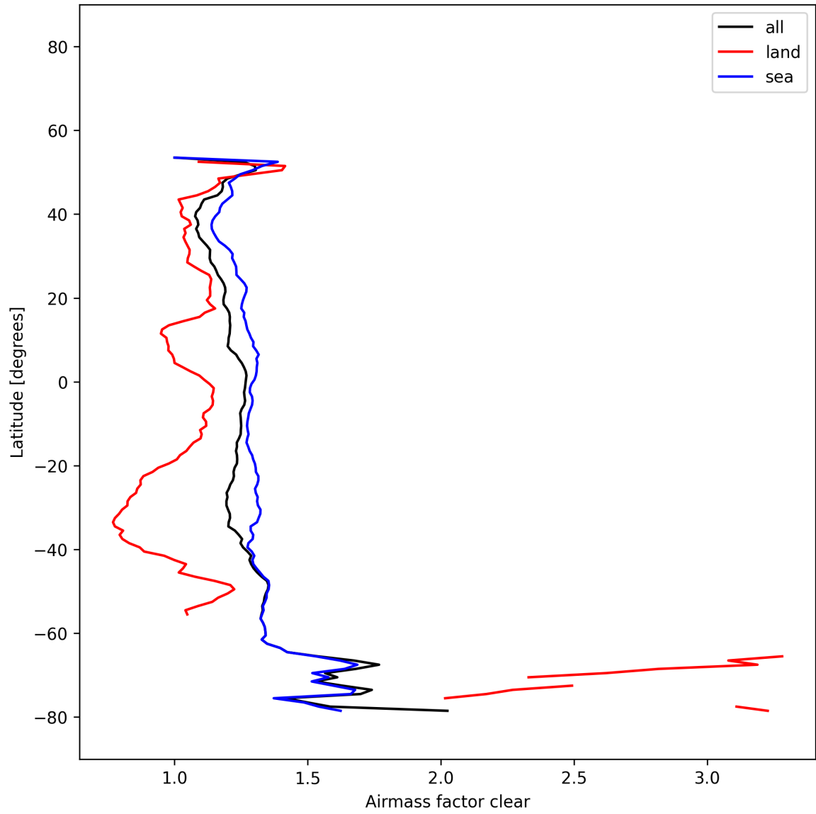
Figure 27: Zonal average of “Airmass factor clear” for 2025-12-02 to 2025-12-02.
