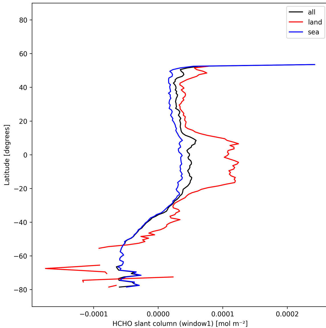
Figure 23: Zonal average of “HCHO slant column (window1)” for 2025-12-02 to 2025-12-02.
