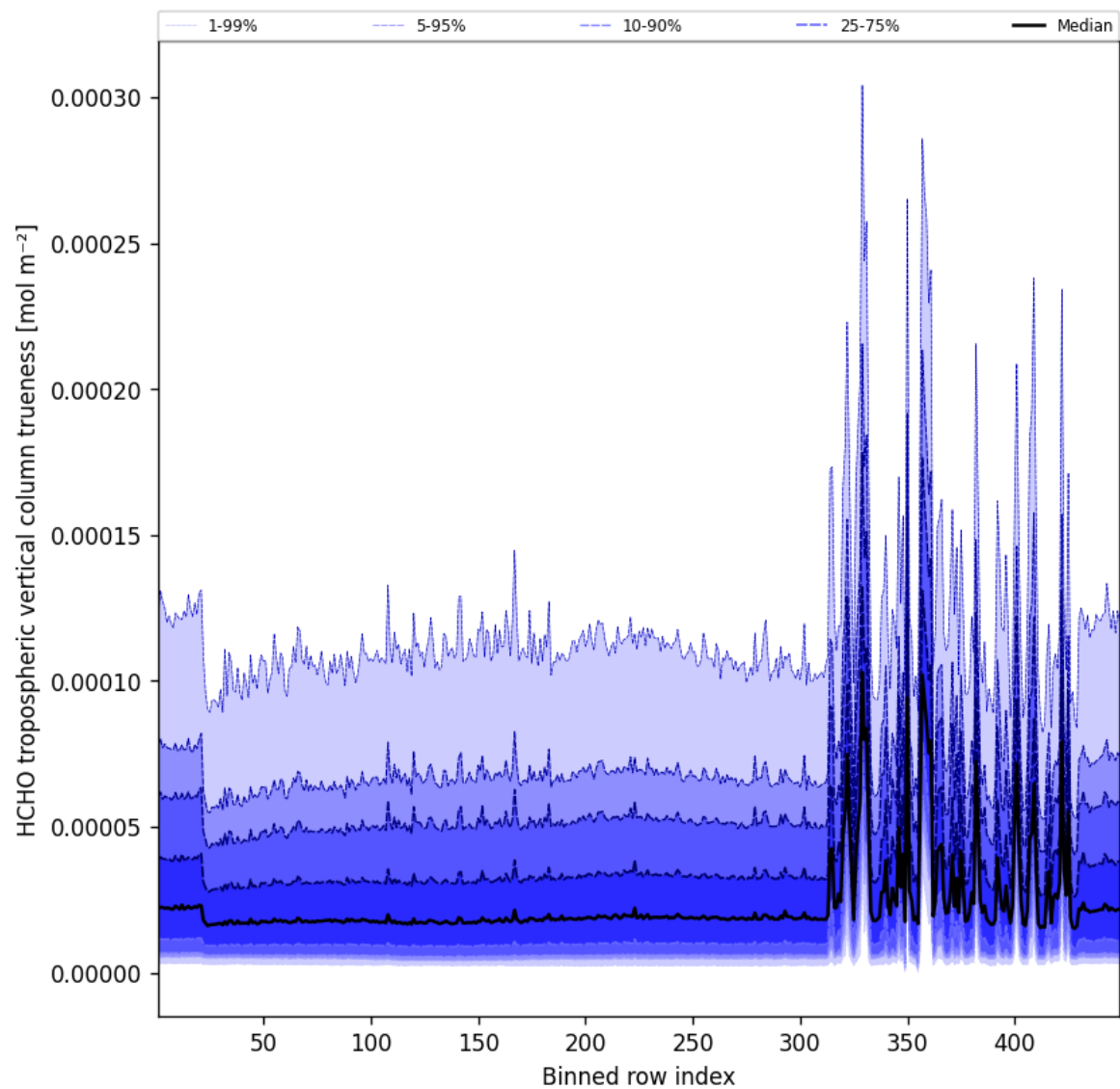
Figure 63: Along track statistics of “HCHO tropospheric vertical column trueness” for 2025-12-02 to 2025-12-02
