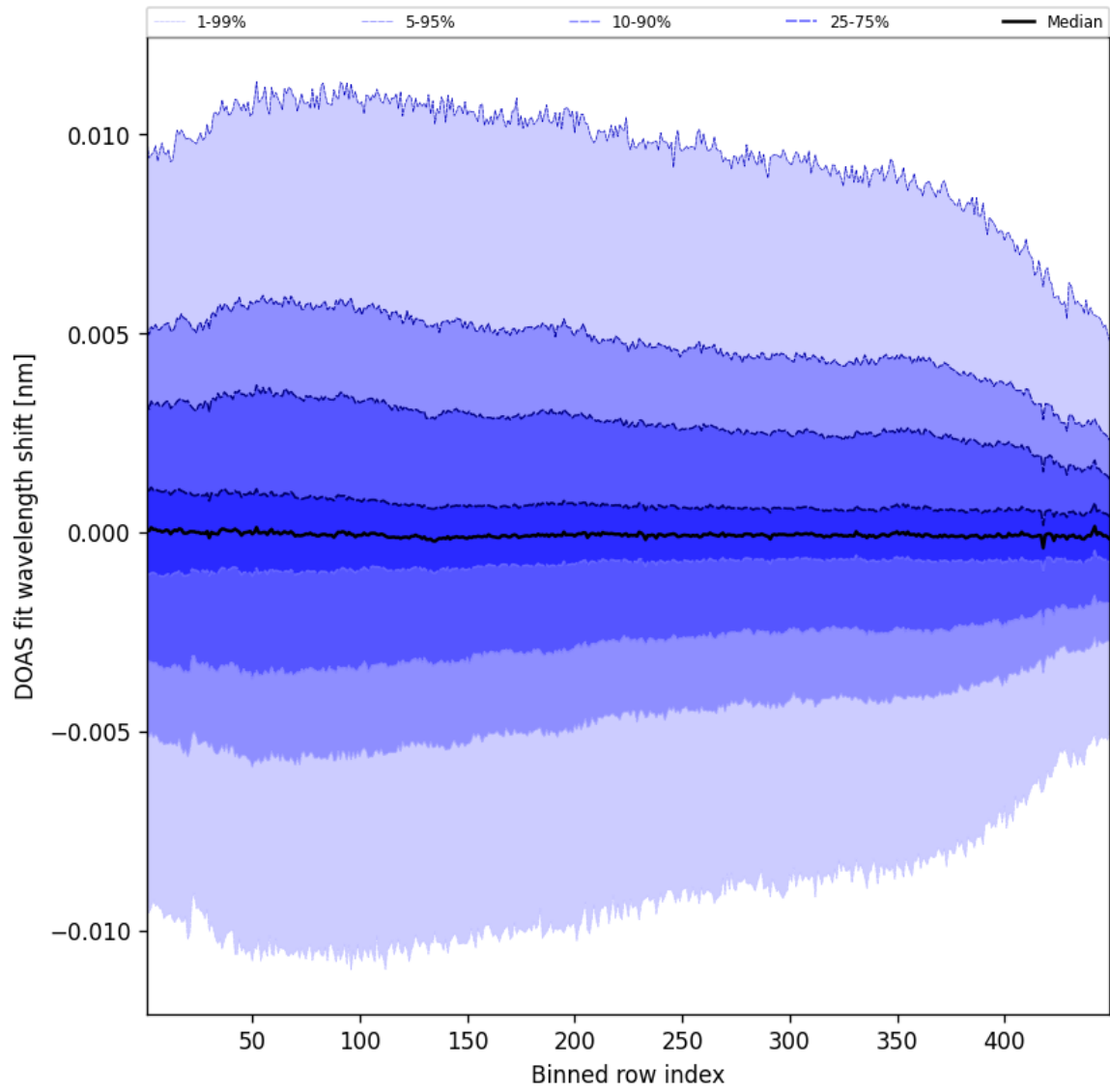
Figure 59: Along track statistics of “DOAS fit wavelength shift” for 2025-12-02 to 2025-12-02
