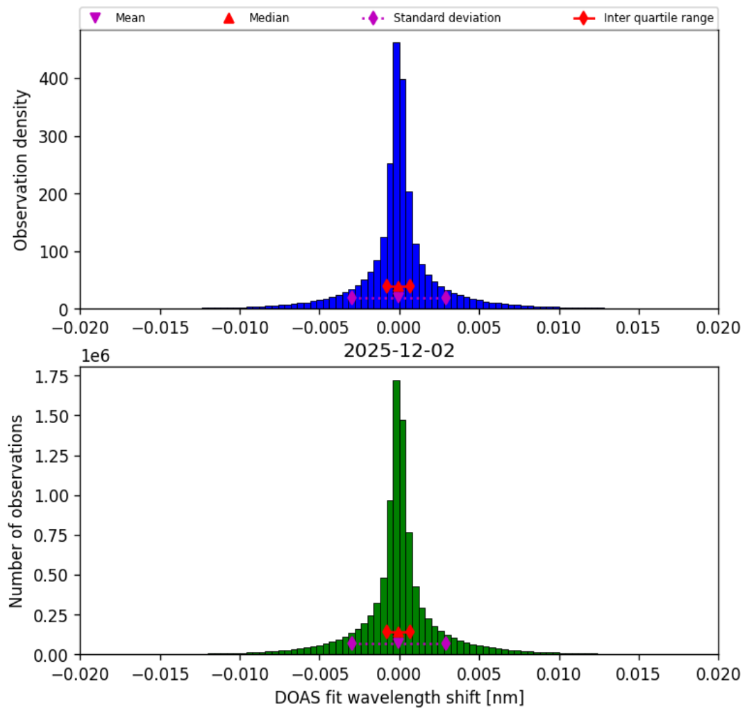
Figure 44: Histogram of “DOAS fit wavelength shift” for 2025-12-02 to 2025-12-02
