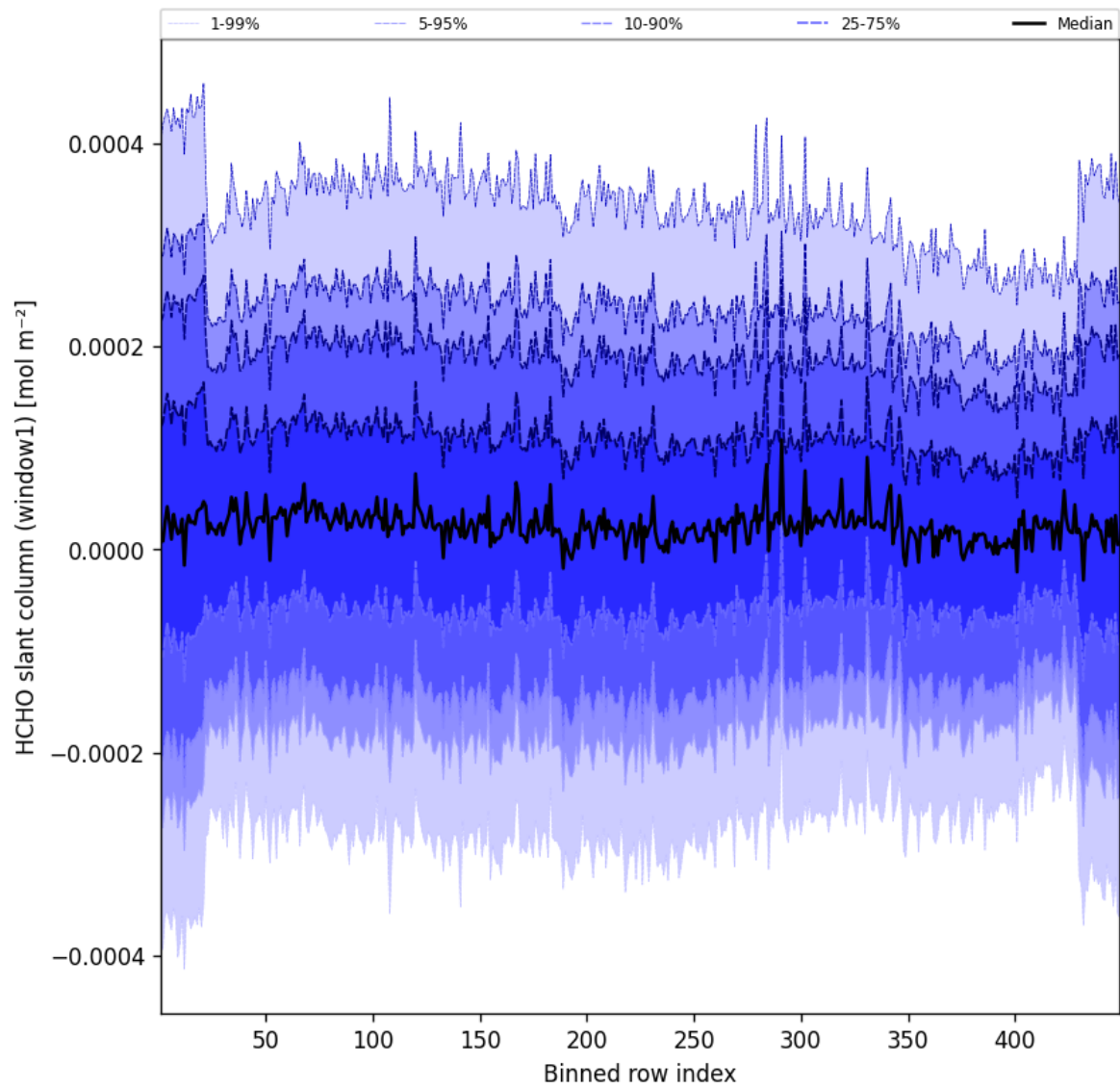
Figure 53: Along track statistics of “HCHO slant column (window1)” for 2025-12-02 to 2025-12-02
