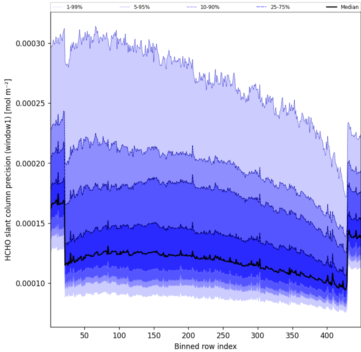
Figure 54: Along track statistics of “HCHO slant column precision (window1)” for 2025-12-02 to 2025-12-02
