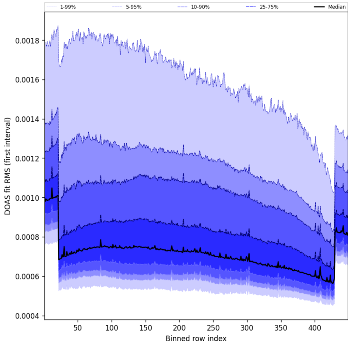
Figure 61: Along track statistics of “DOAS fit RMS (first interval)” for 2025-12-02 to 2025-12-02
