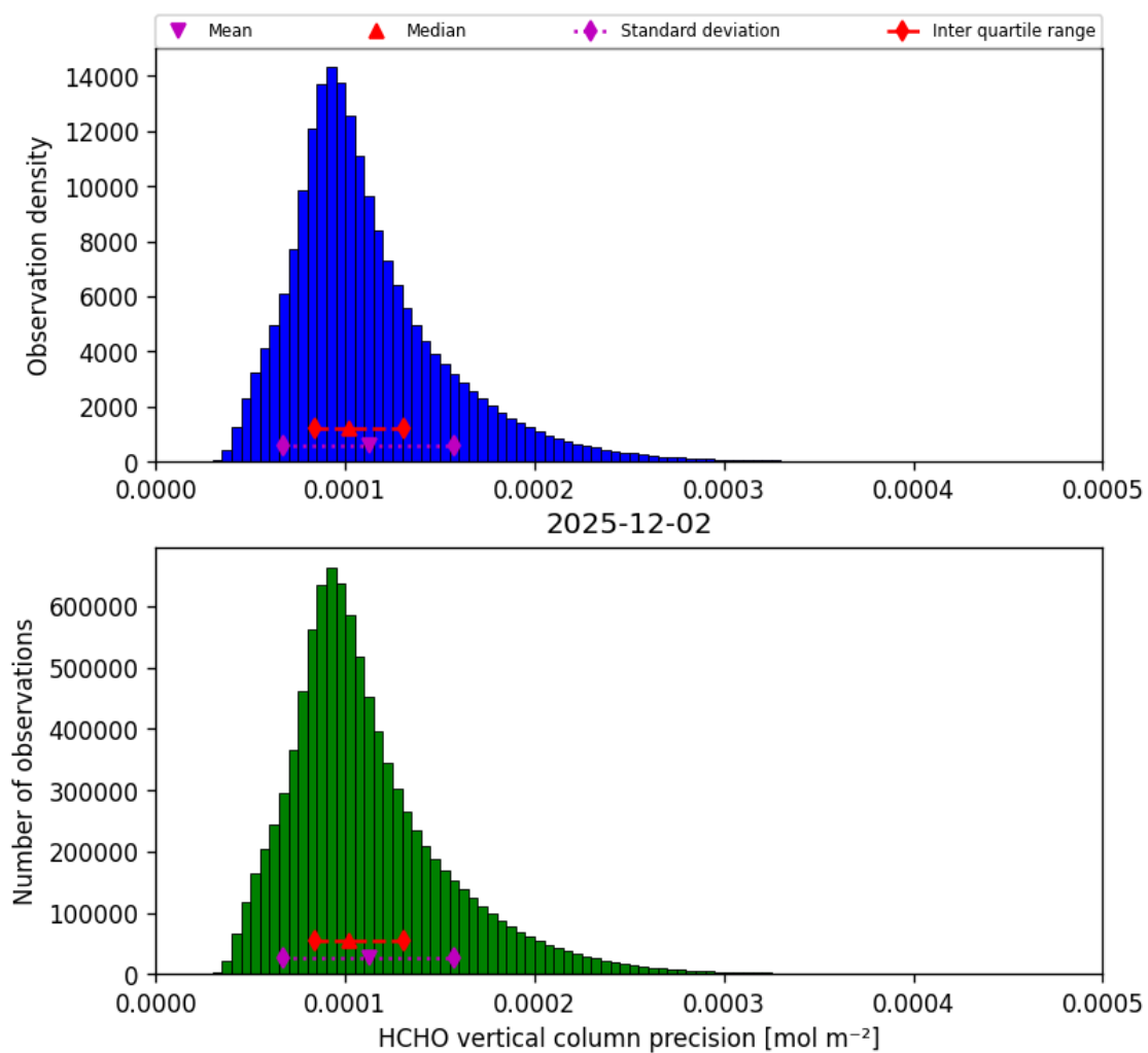
Figure 36: Histogram of “HCHO vertical column precision” for 2025-12-02 to 2025-12-02
