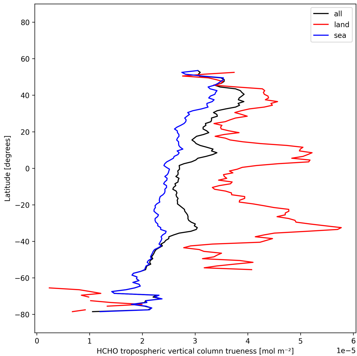
Figure 33: Zonal average of “HCHO tropospheric vertical column trueness” for 2025-12-02 to 2025-12-02.
