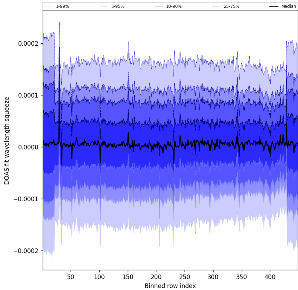
Figure 60: Along track statistics of “DOAS fit wavelength squeeze” for 2025-12-02 to 2025-12-02
