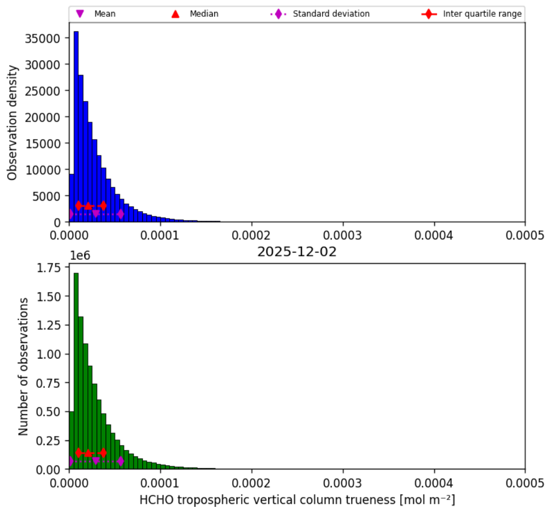
Figure 48: Histogram of “HCHO tropospheric vertical column trueness” for 2025-12-02 to 2025-12-02
