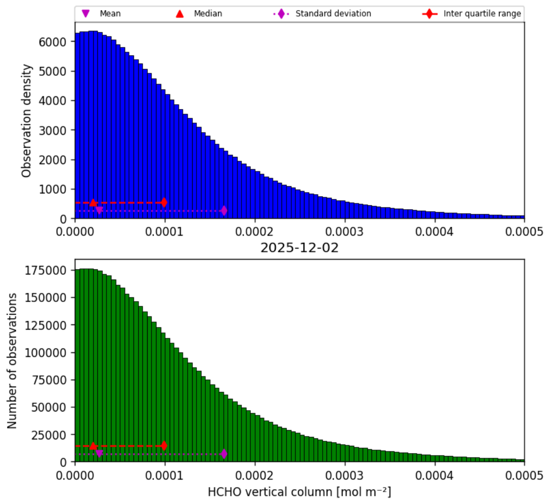
Figure 35: Histogram of “HCHO vertical column” for 2025-12-02 to 2025-12-02
