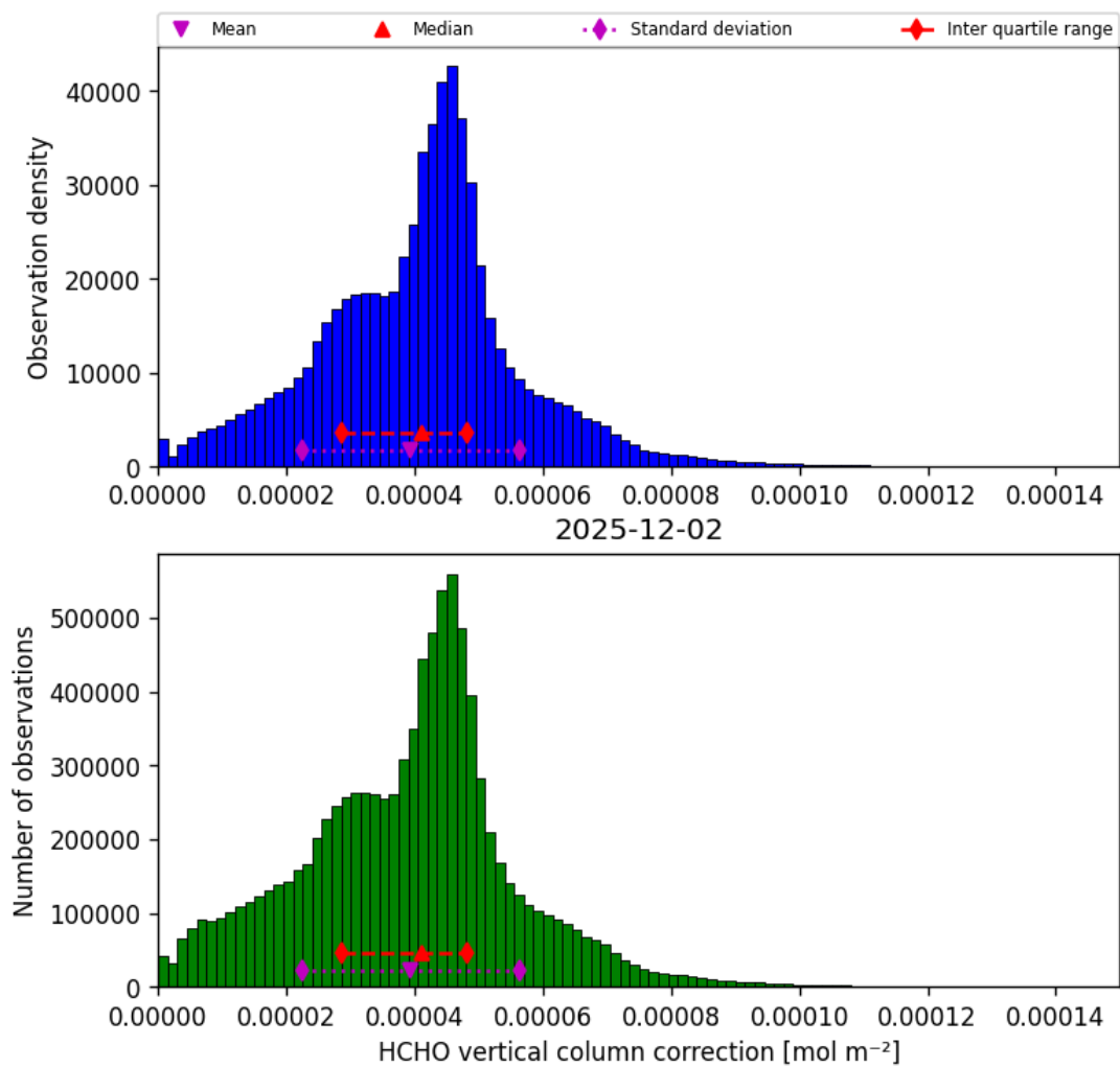
Figure 37: Histogram of “HCHO vertical column correction” for 2025-12-02 to 2025-12-02
