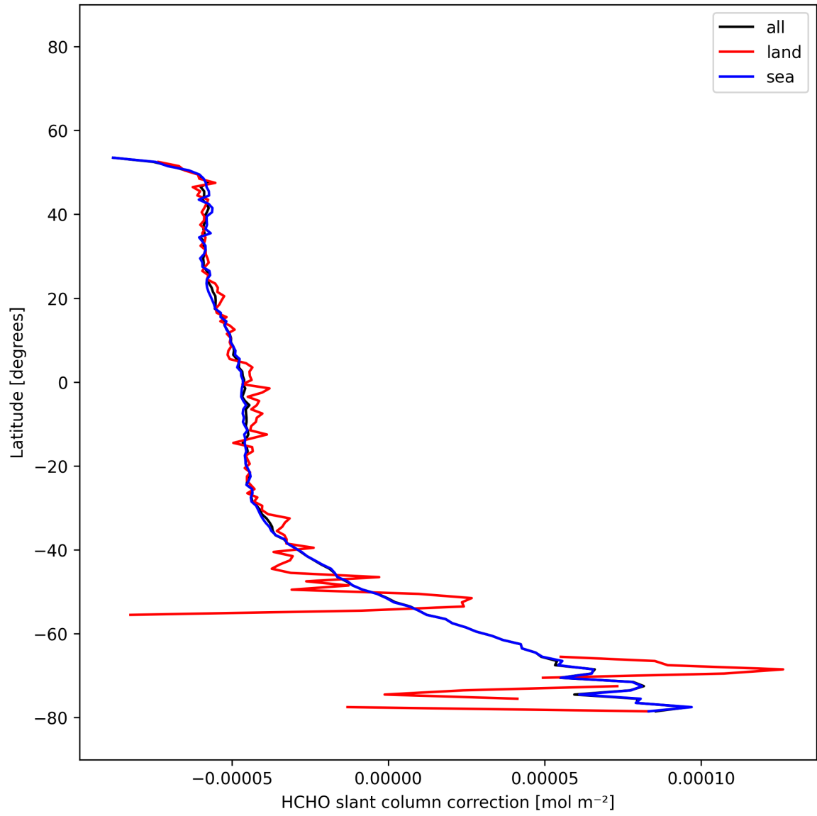
Figure 32: Zonal average of “HCHO slant column correction” for 2025-12-02 to 2025-12-02.
