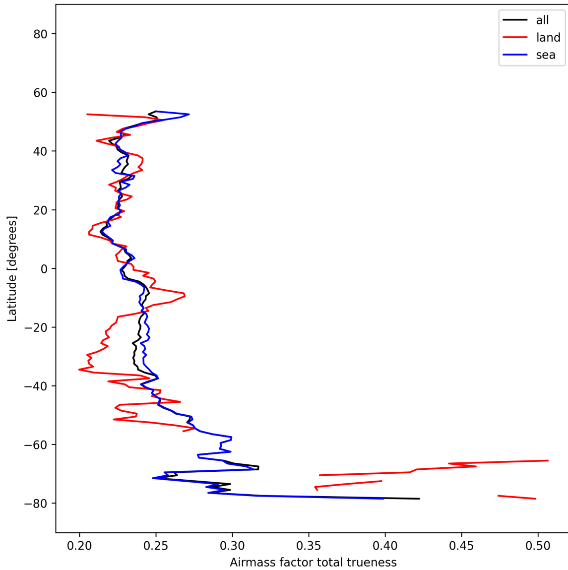
Figure 26: Zonal average of “Airmass factor total trueness” for 2025-12-02 to 2025-12-02.
