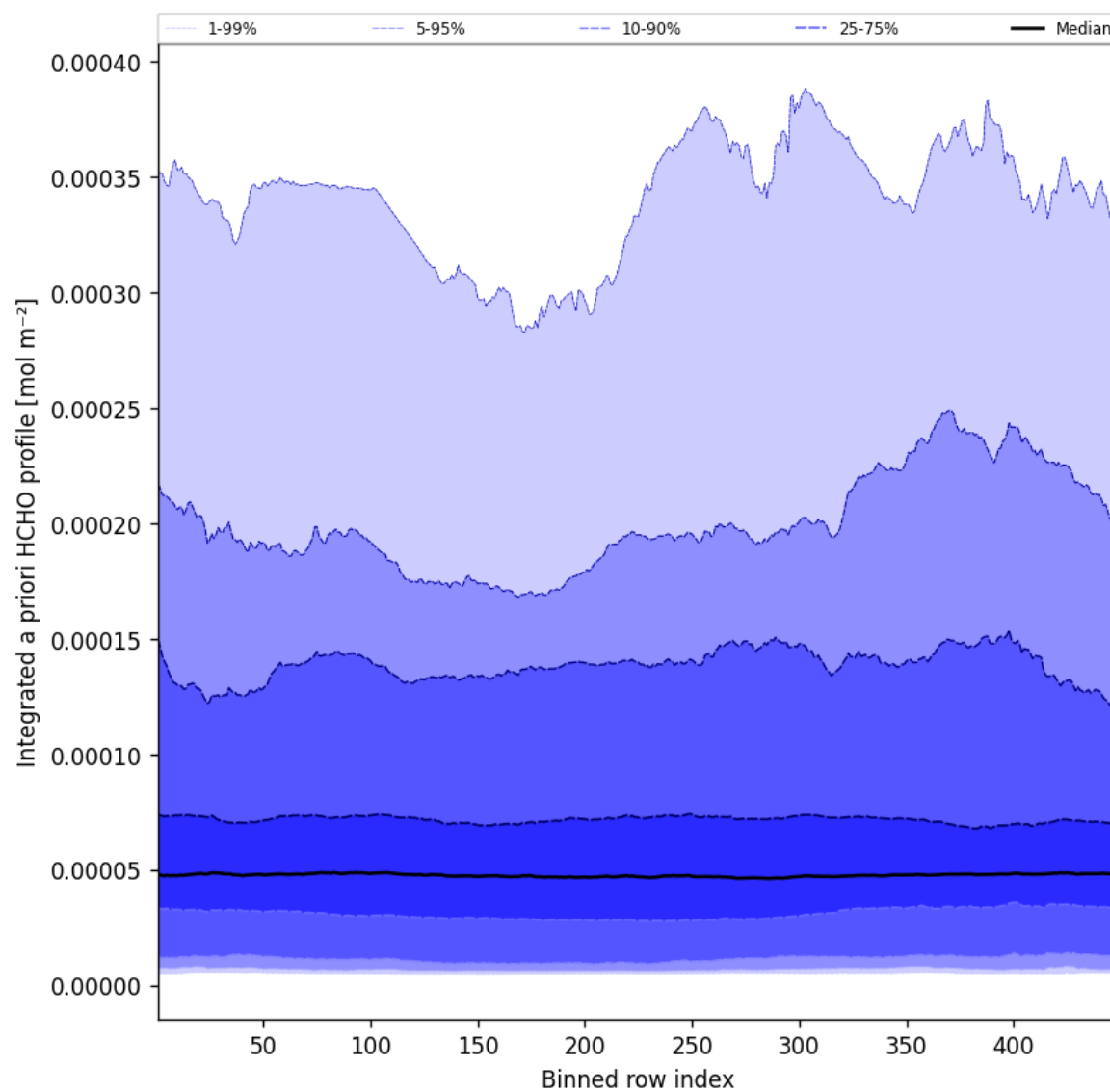
Figure 58: Along track statistics of “Integrated a priori HCHO profile” for 2025-12-02 to 2025-12-02
