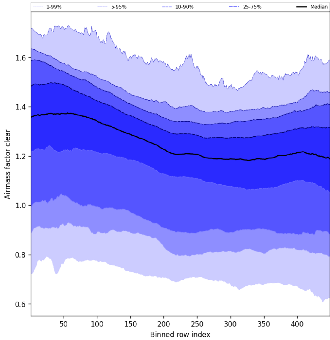
Figure 57: Along track statistics of “Airmass factor clear” for 2025-12-02 to 2025-12-02
