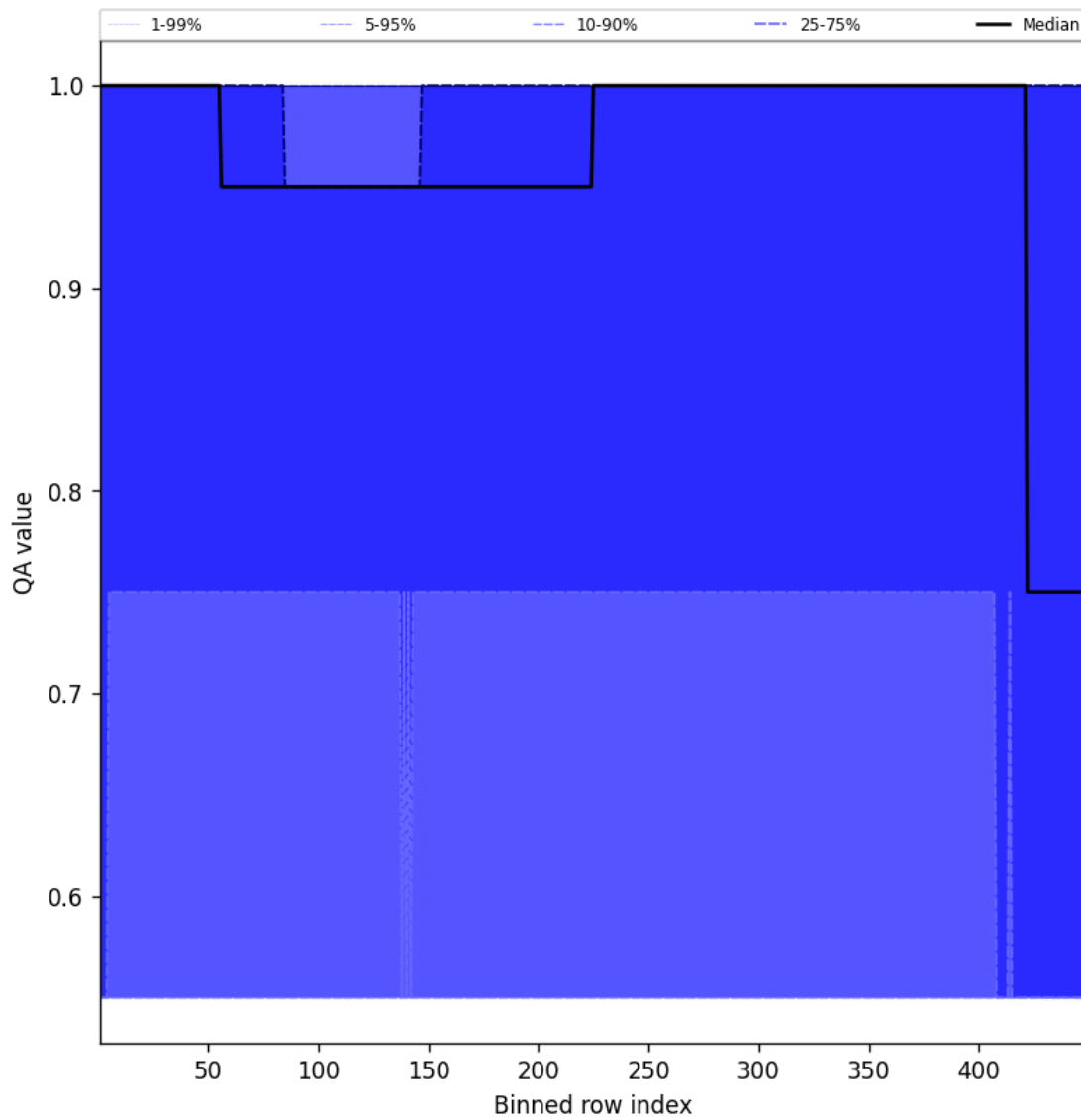
Figure 49: Along track statistics of “QA value” for 2025-12-02 to 2025-12-02
