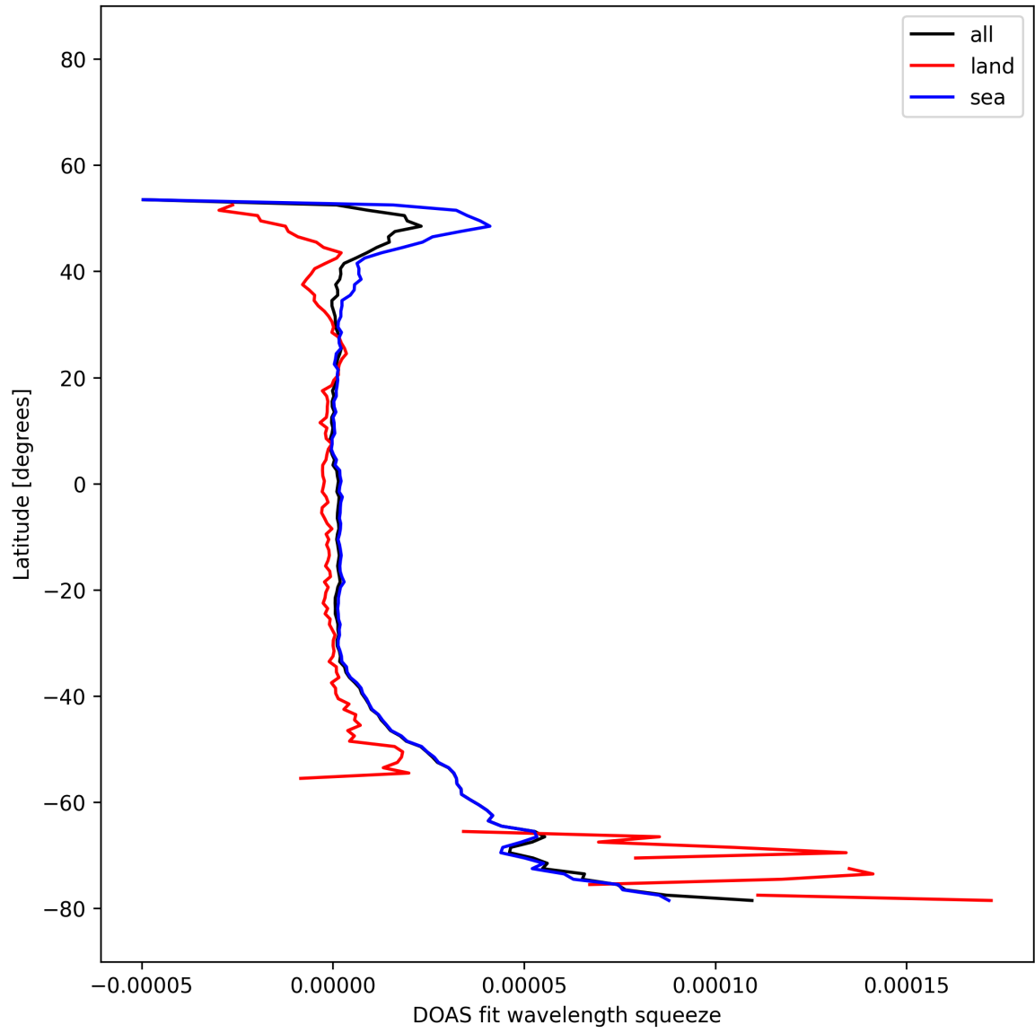
Figure 30: Zonal average of “DOAS fit wavelength squeeze” for 2025-12-02 to 2025-12-02.
