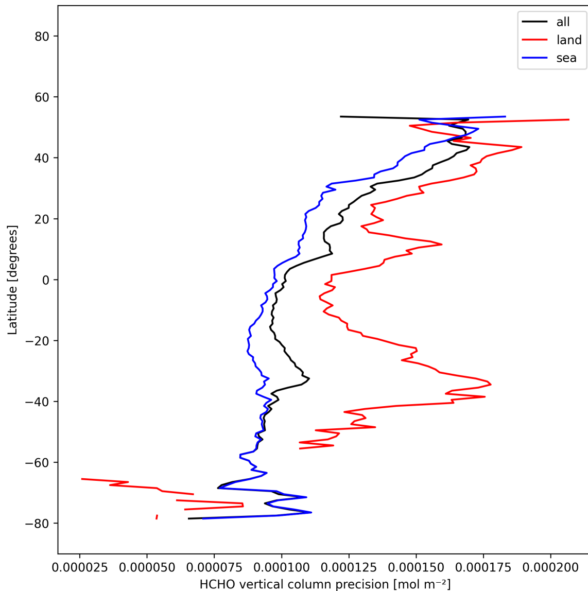
Figure 21: Zonal average of “HCHO vertical column precision” for 2025-12-02 to 2025-12-02.
