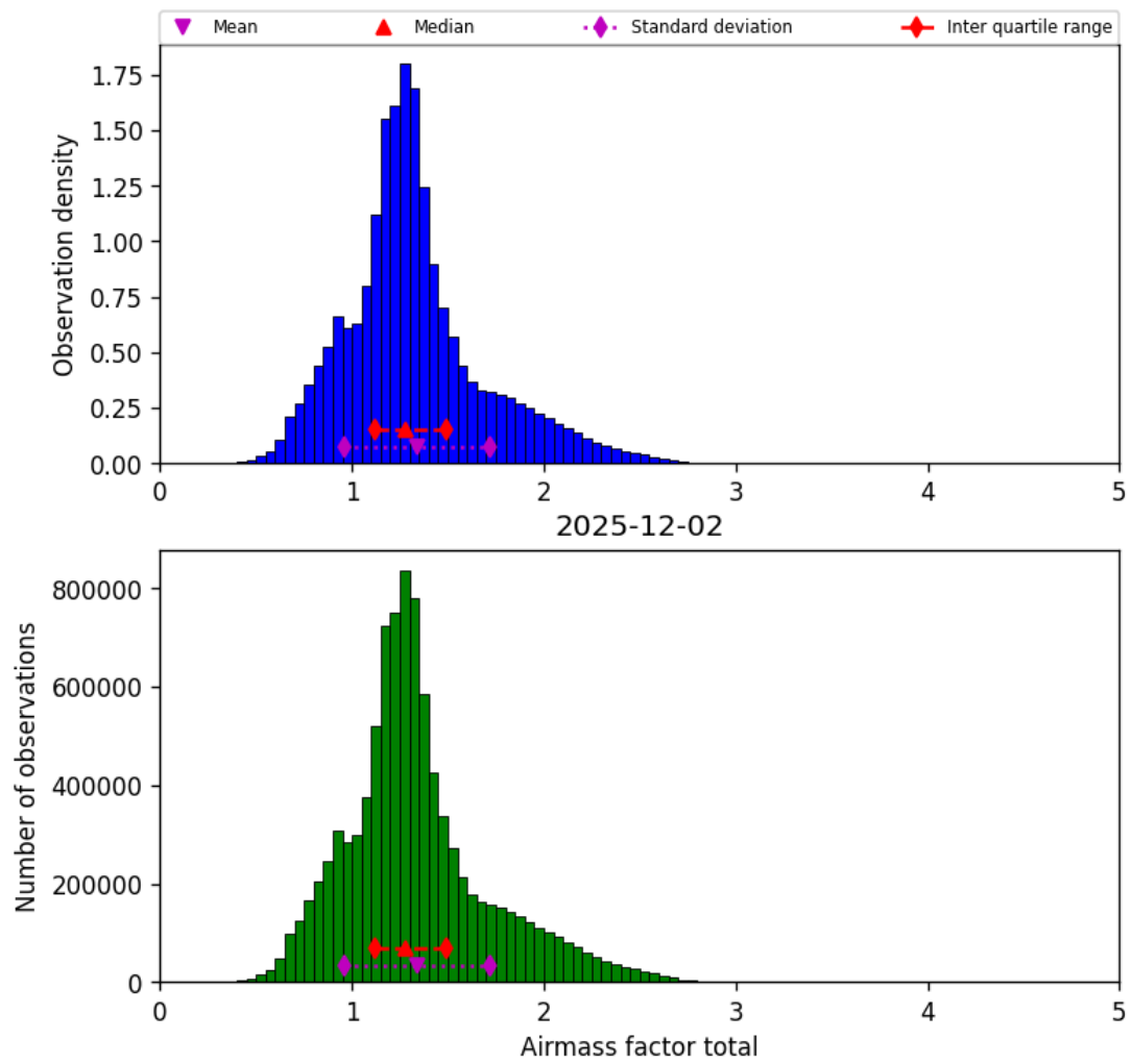
Figure 40: Histogram of “Airmass factor total” for 2025-12-02 to 2025-12-02
