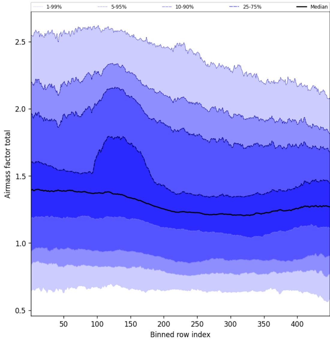
Figure 55: Along track statistics of “Airmass factor total” for 2025-12-02 to 2025-12-02
