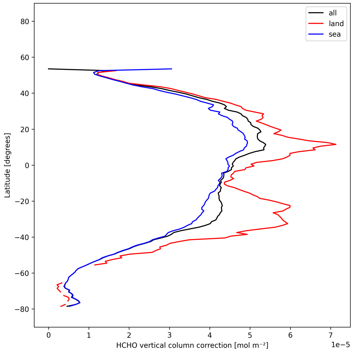
Figure 22: Zonal average of “HCHO vertical column correction” for 2025-12-02 to 2025-12-02.
