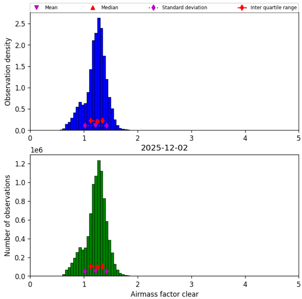
Figure 42: Histogram of “Airmass factor clear” for 2025-12-02 to 2025-12-02
