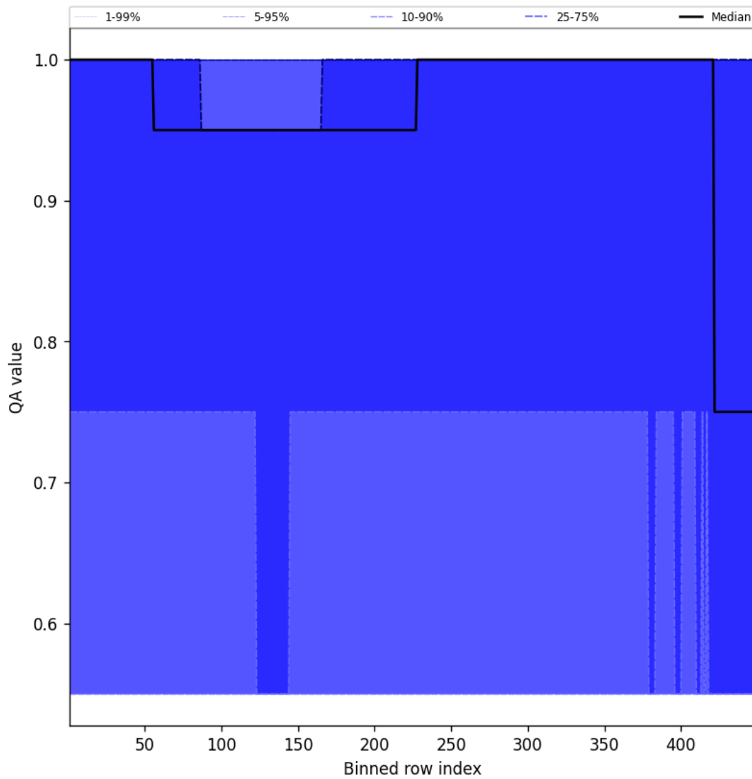
Figure 49: Along track statistics of “QA value” for 2025-12-03 to 2025-12-04
