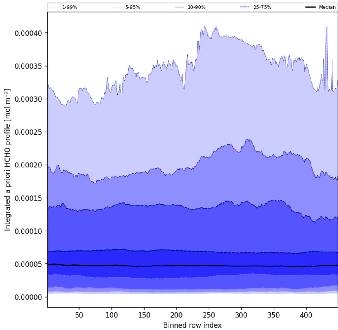
Figure 58: Along track statistics of “Integrated a priori HCHO profile” for 2025-12-03 to 2025-12-04
