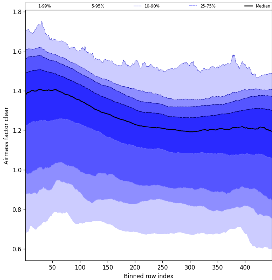
Figure 57: Along track statistics of “Airmass factor clear” for 2025-12-03 to 2025-12-04
