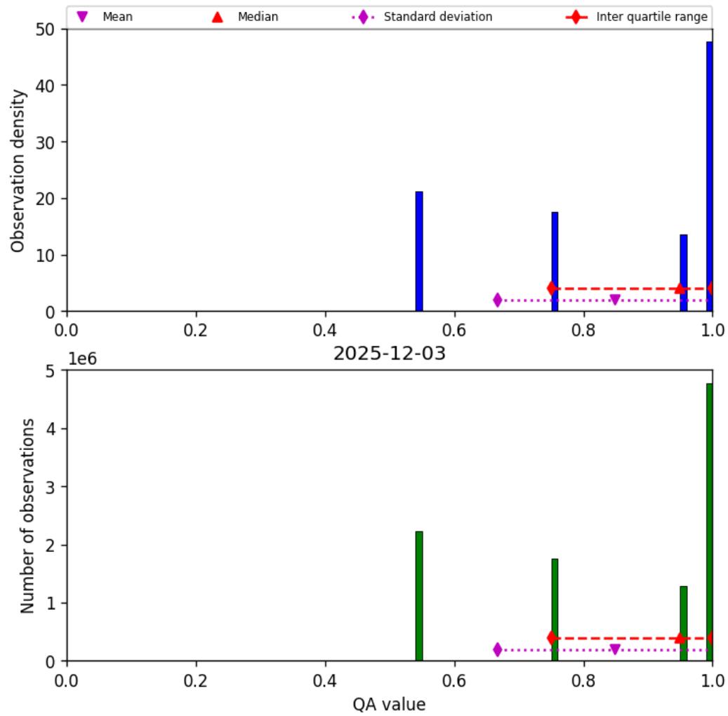
Figure 34: Histogram of “QA value” for 2025-12-03 to 2025-12-04
