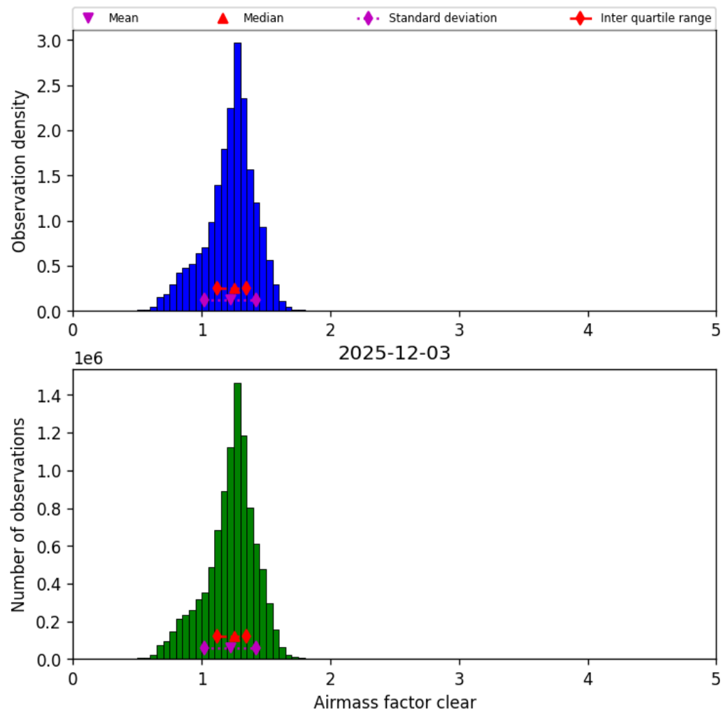
Figure 42: Histogram of “Airmass factor clear” for 2025-12-03 to 2025-12-04
