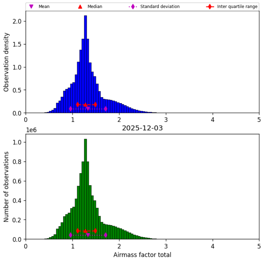
Figure 40: Histogram of “Airmass factor total” for 2025-12-03 to 2025-12-04
