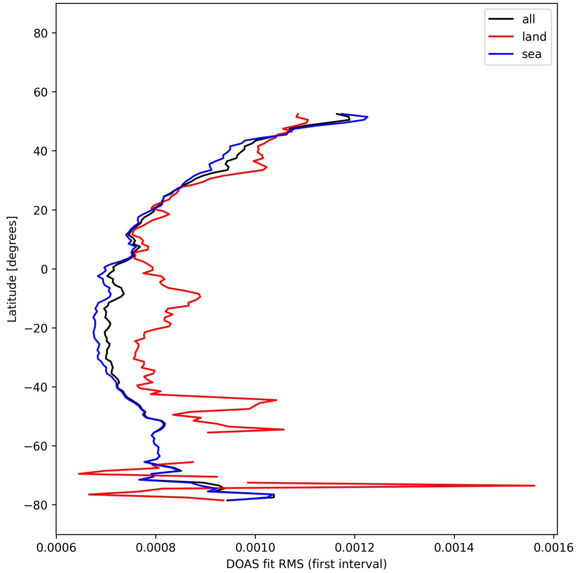
Figure 31: Zonal average of “DOAS fit RMS (first interval)” for 2025-12-03 to 2025-12-04.
