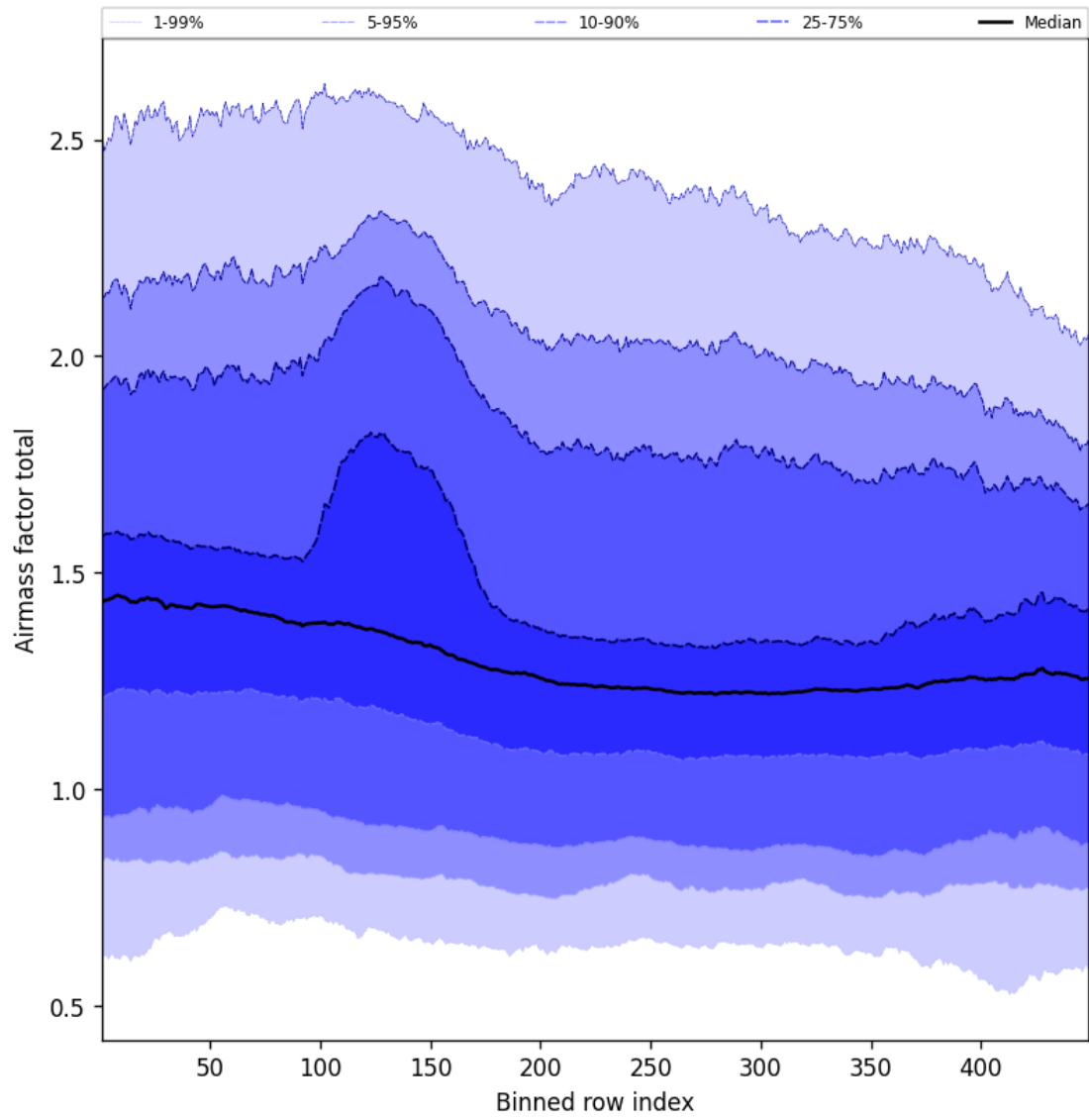
Figure 55: Along track statistics of “Airmass factor total” for 2025-12-03 to 2025-12-04
