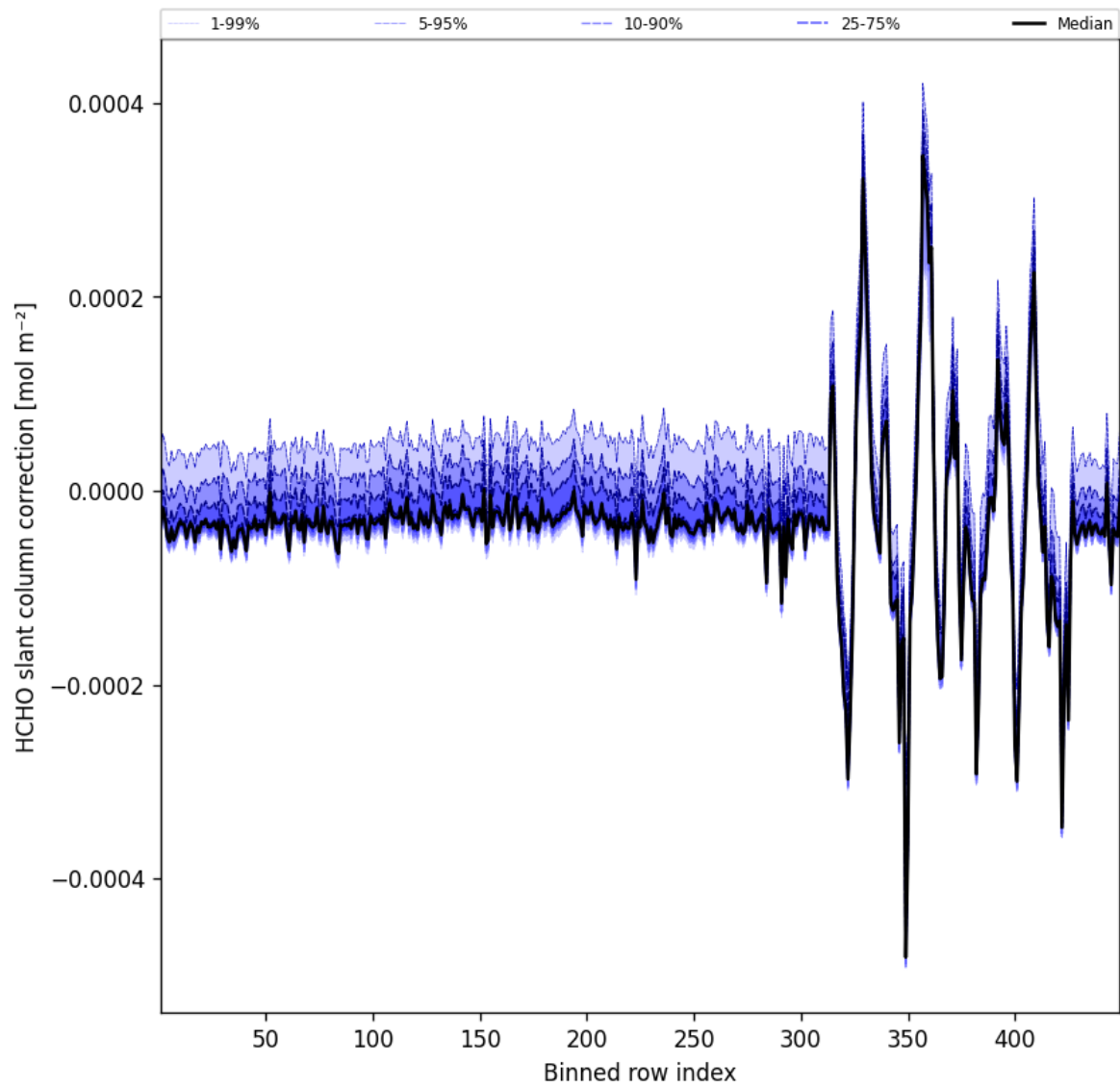
Figure 62: Along track statistics of “HCHO slant column correction” for 2025-12-03 to 2025-12-04
