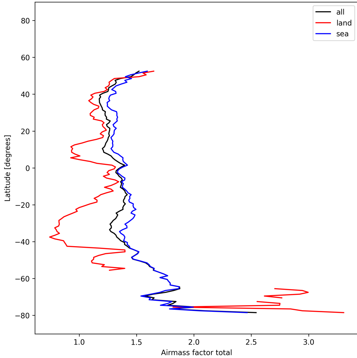
Figure 25: Zonal average of “Airmass factor total” for 2025-12-03 to 2025-12-04.
