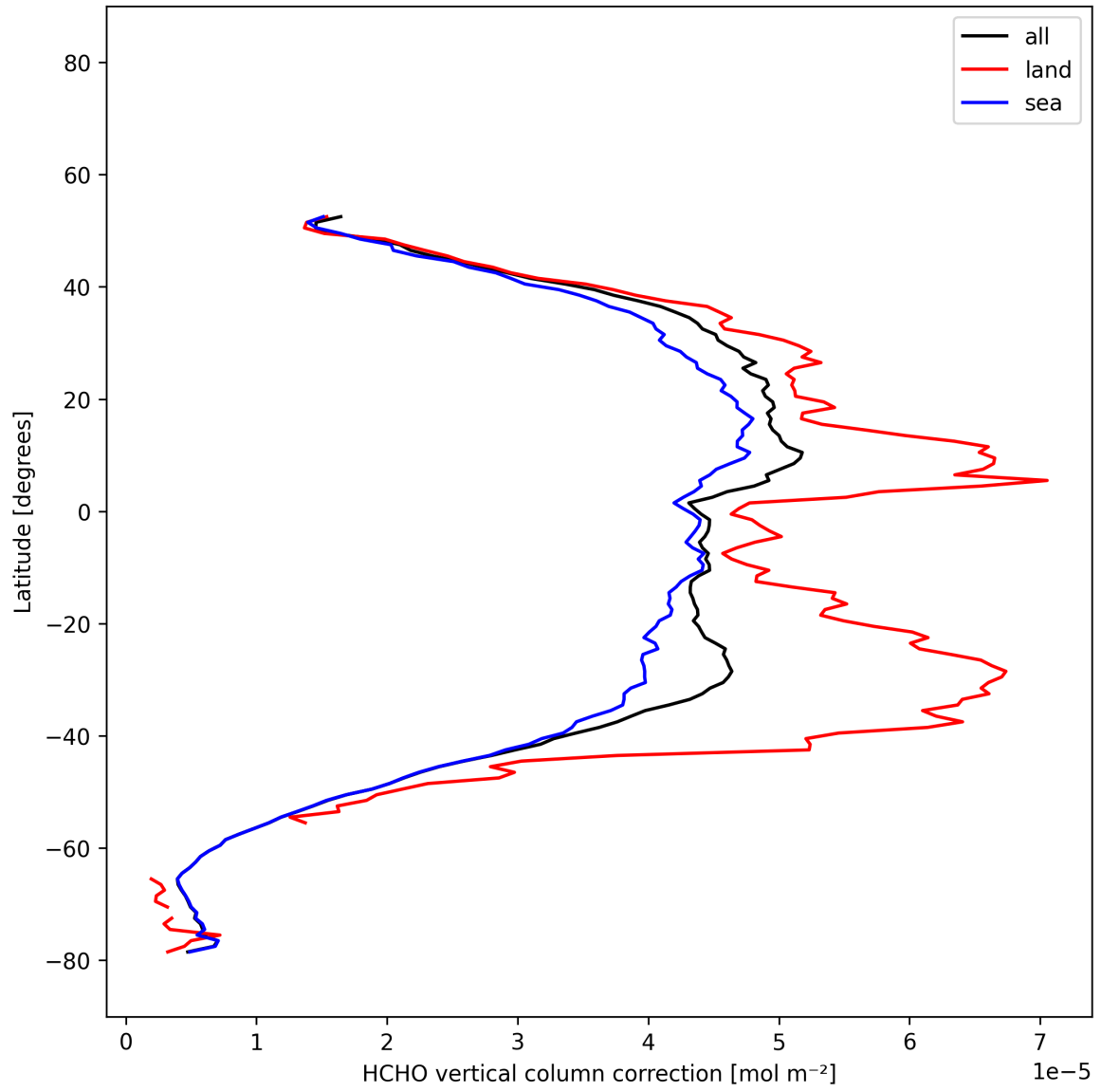
Figure 22: Zonal average of “HCHO vertical column correction” for 2025-12-03 to 2025-12-04.
