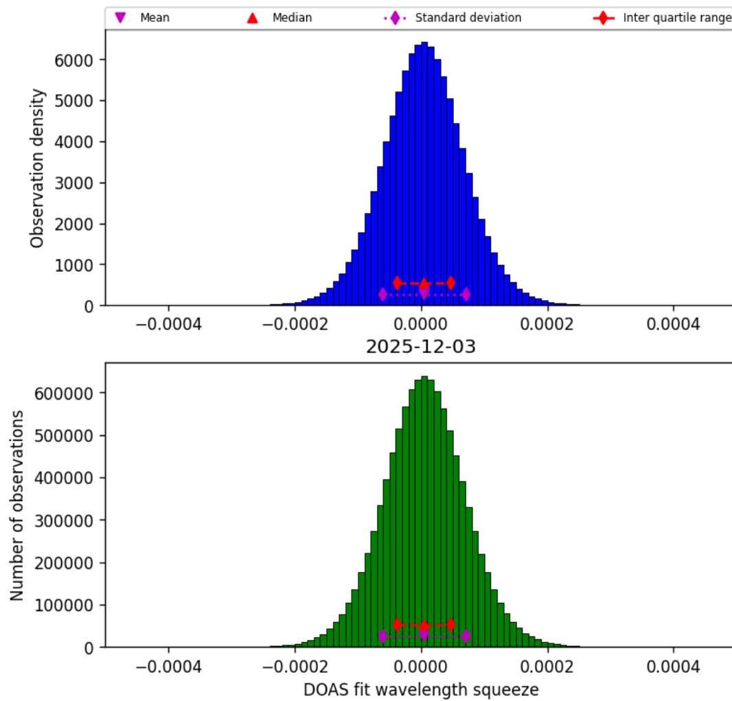
Figure 45: Histogram of “DOAS fit wavelength squeeze” for 2025-12-03 to 2025-12-04
