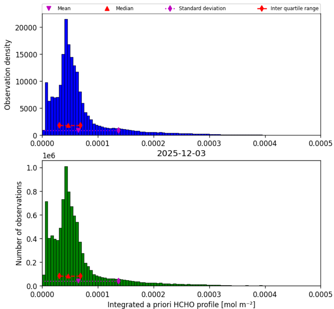
Figure 43: Histogram of “Integrated a priori HCHO profile” for 2025-12-03 to 2025-12-04
