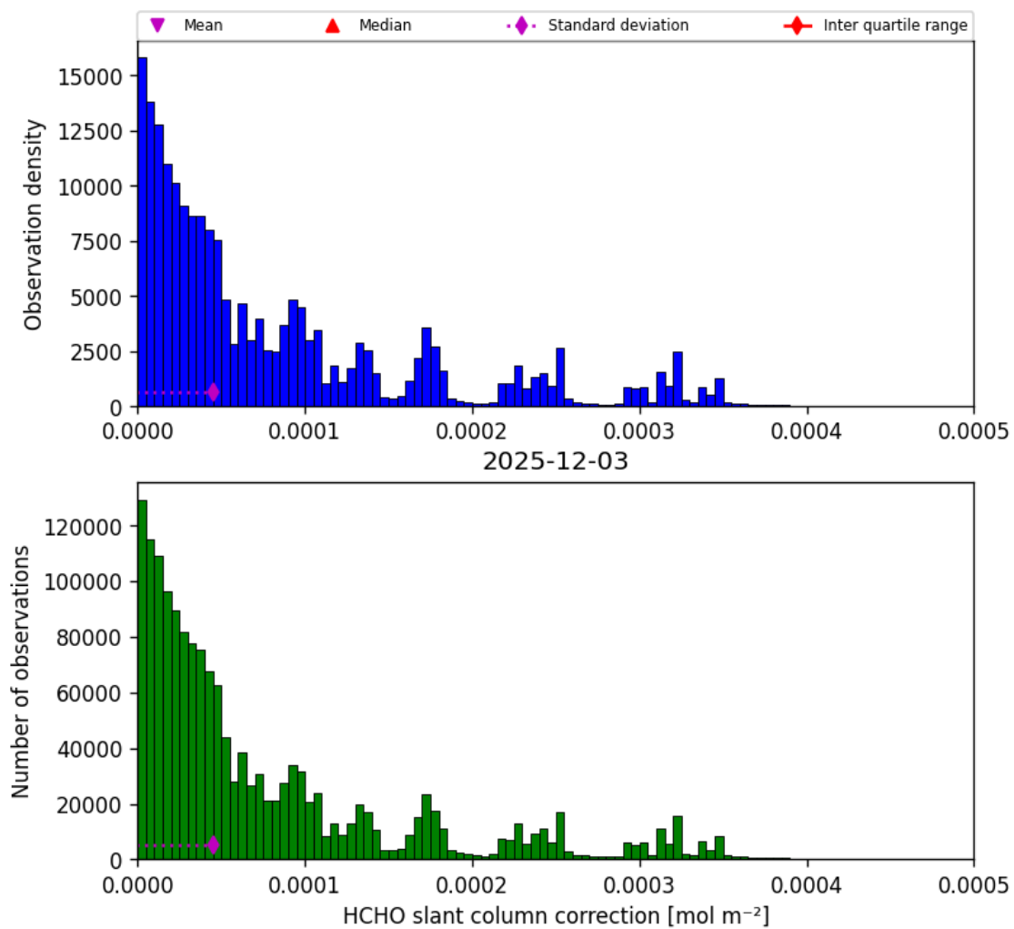
Figure 47: Histogram of “HCHO slant column correction” for 2025-12-03 to 2025-12-04
