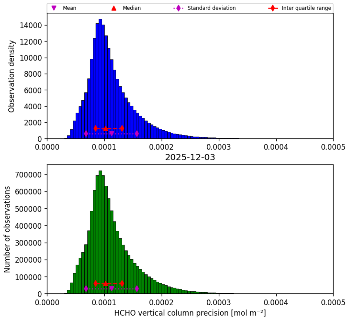
Figure 36: Histogram of “HCHO vertical column precision” for 2025-12-03 to 2025-12-04
