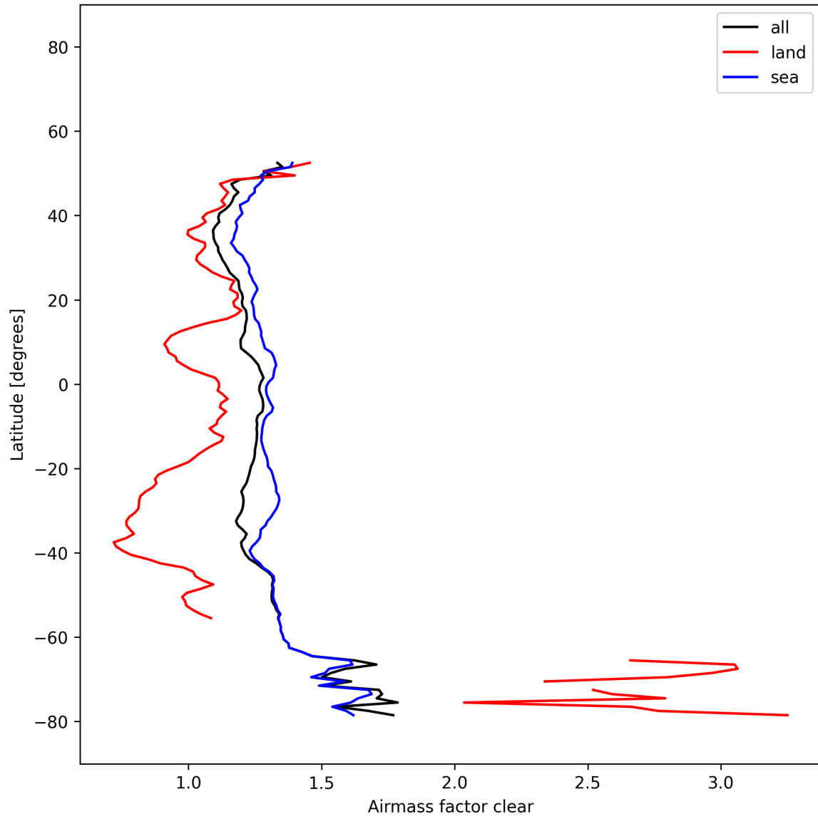
Figure 27: Zonal average of “Airmass factor clear” for 2025-12-03 to 2025-12-04.
