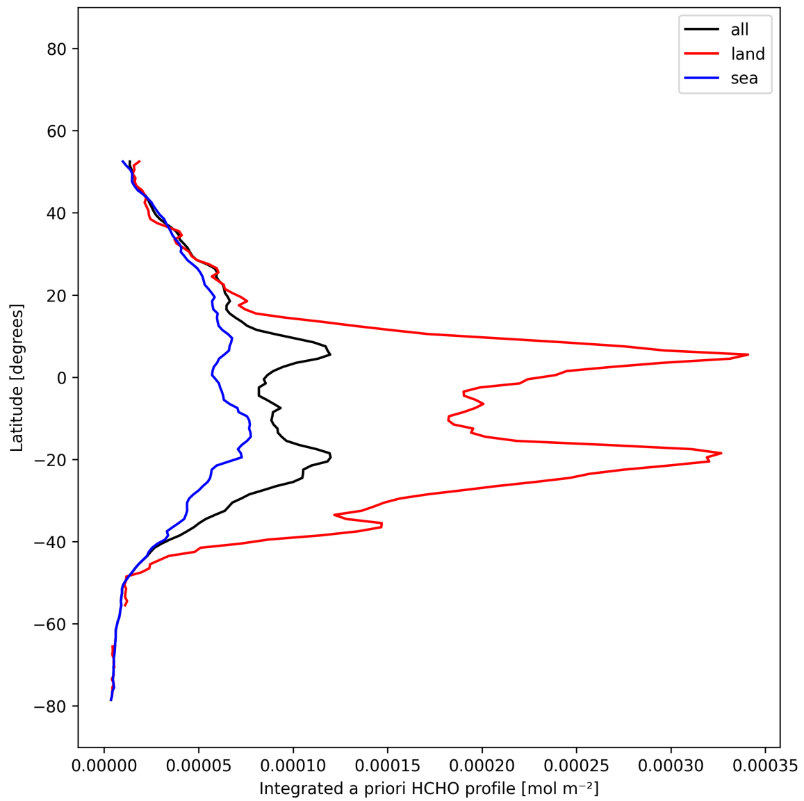
Figure 28: Zonal average of “Integrated a priori HCHO profile” for 2025-12-03 to 2025-12-04.
