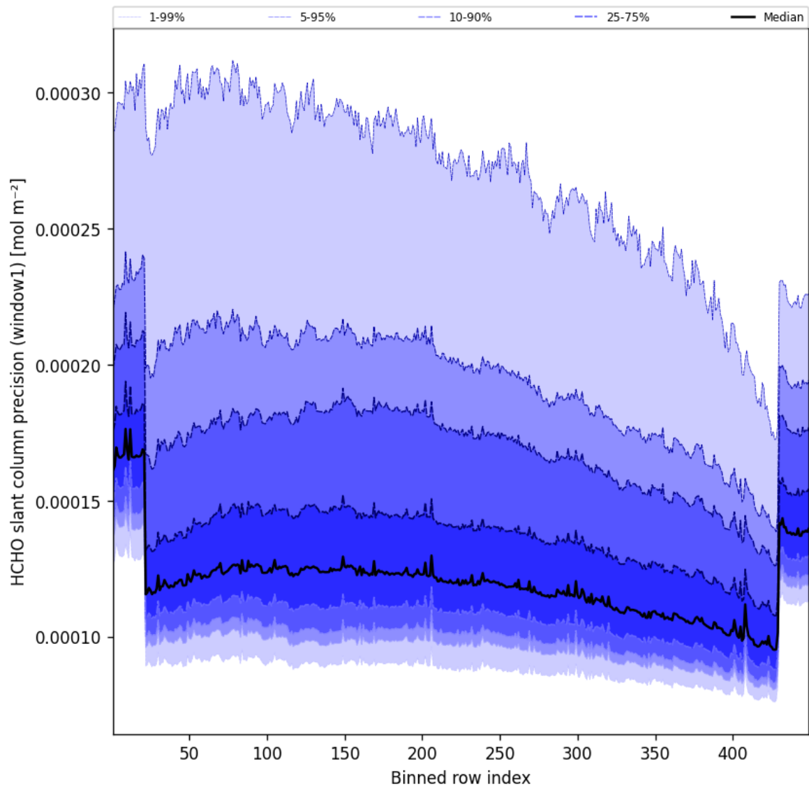
Figure 54: Along track statistics of “HCHO slant column precision (window1)” for 2025-12-03 to 2025-12-04
