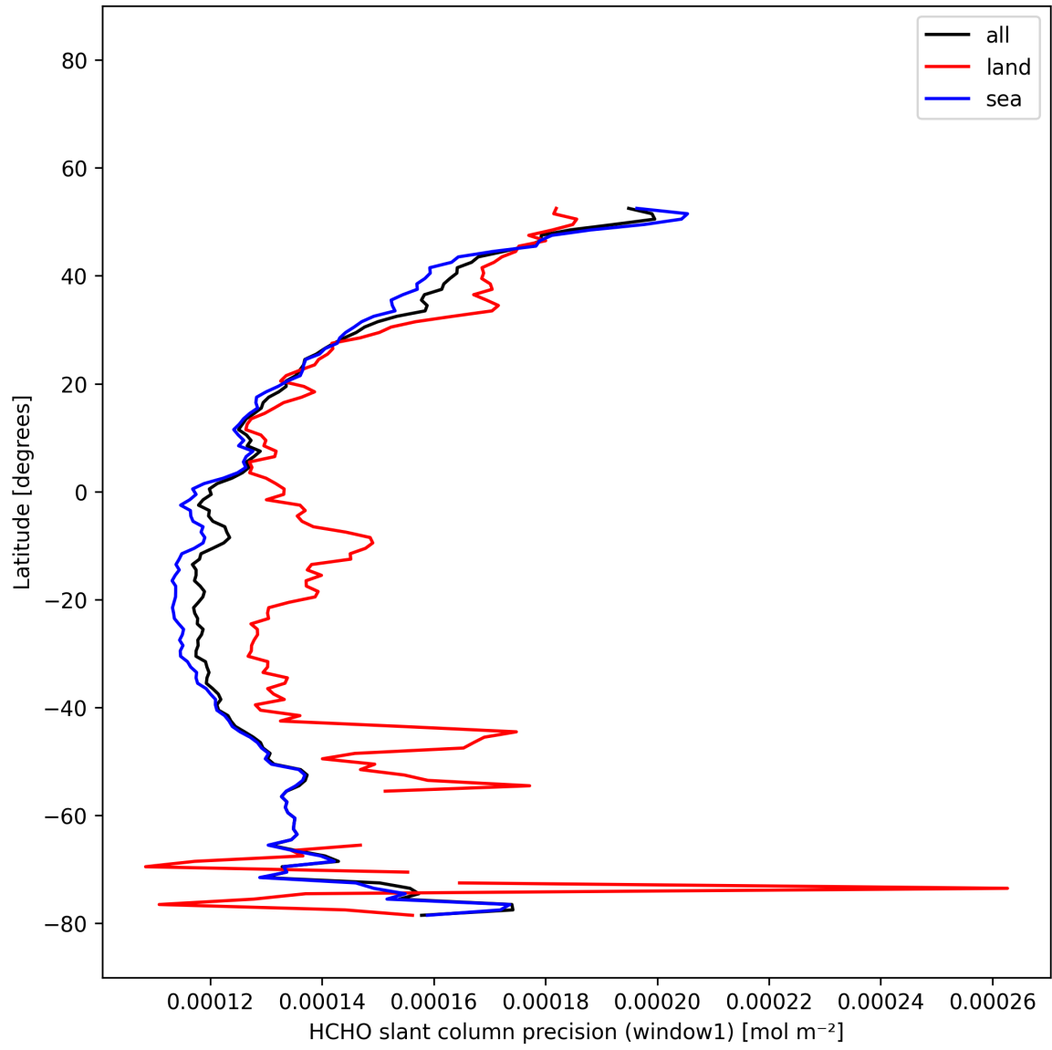
Figure 24: Zonal average of “HCHO slant column precision (window1)” for 2025-12-03 to 2025-12-04.
