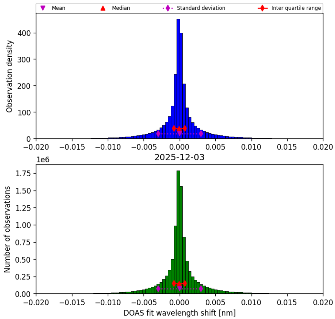
Figure 44: Histogram of “DOAS fit wavelength shift” for 2025-12-03 to 2025-12-04
