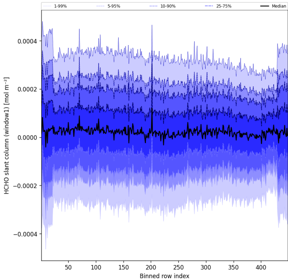
Figure 53: Along track statistics of “HCHO slant column (window1)” for 2025-12-03 to 2025-12-04
