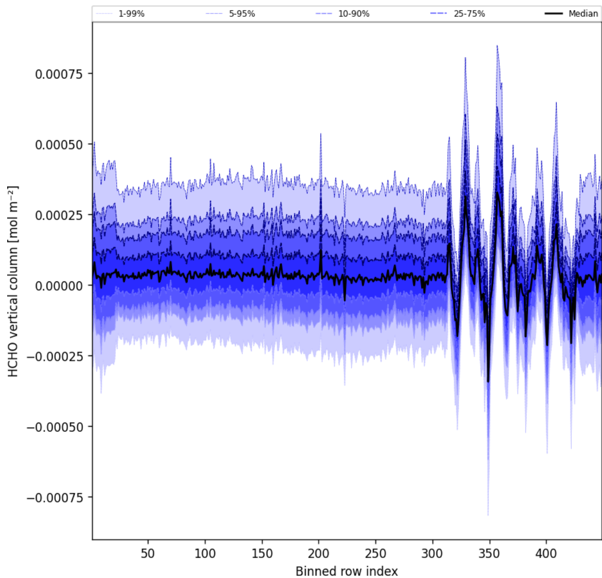
Figure 50: Along track statistics of “HCHO vertical column” for 2025-12-03 to 2025-12-04
