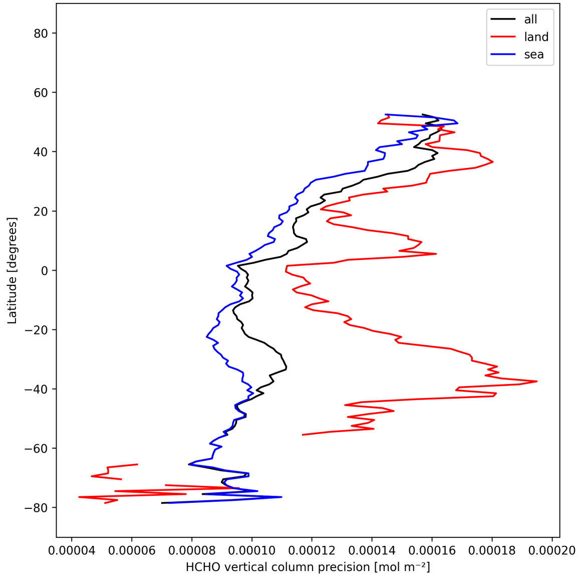
Figure 21: Zonal average of “HCHO vertical column precision” for 2025-12-03 to 2025-12-04.
