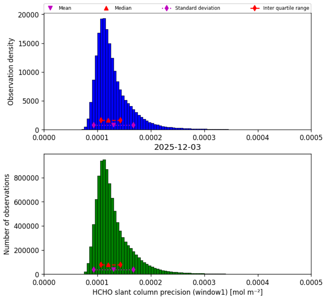
Figure 39: Histogram of “HCHO slant column precision (window1)” for 2025-12-03 to 2025-12-04
