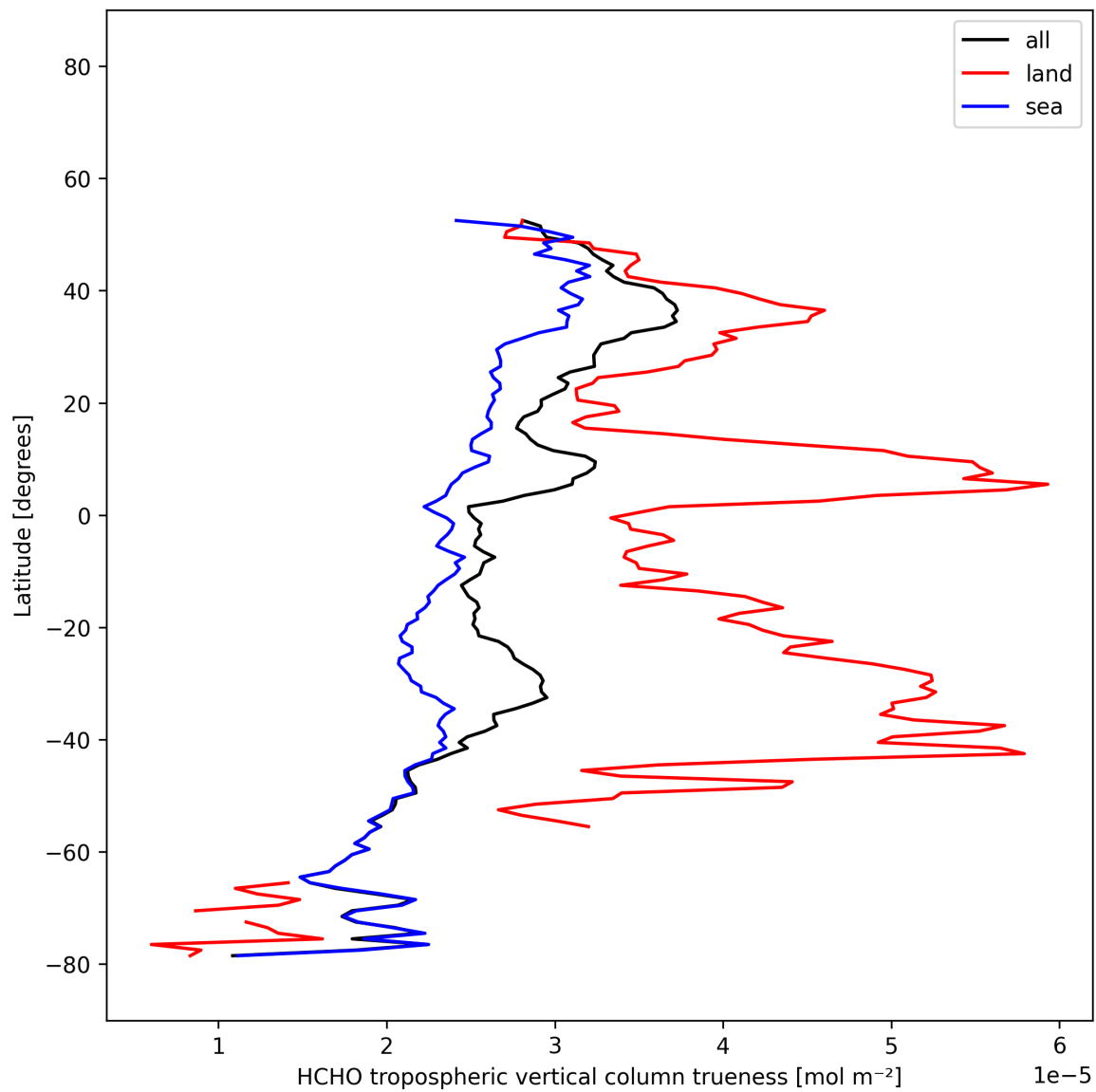
Figure 33: Zonal average of “HCHO tropospheric vertical column trueness” for 2025-12-03 to 2025-12-04.
