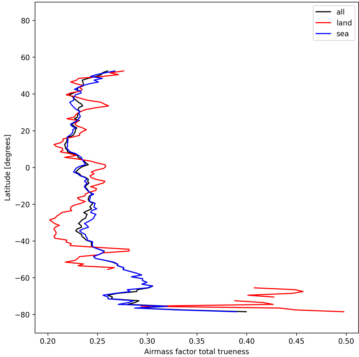
Figure 26: Zonal average of “Airmass factor total trueness” for 2025-12-03 to 2025-12-04.
