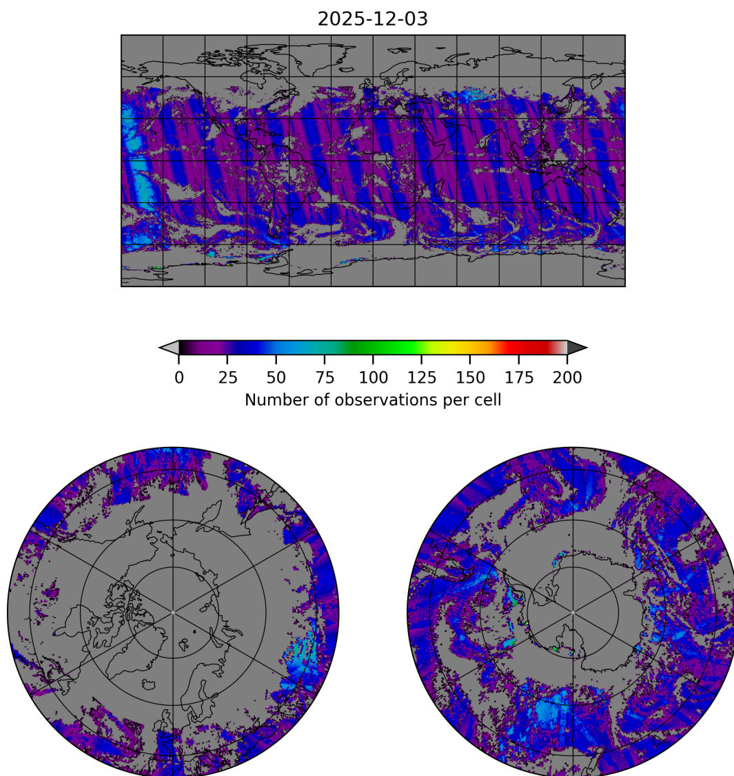
Figure 18: Map of the number of observations for 2025-12-03 to 2025-12-04
