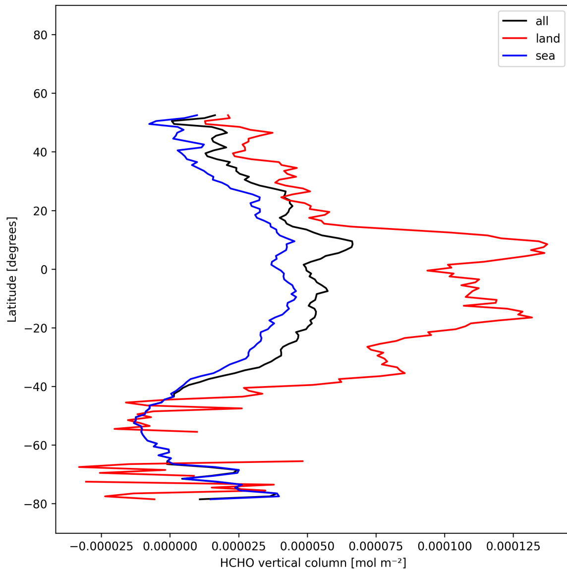
Figure 20: Zonal average of “HCHO vertical column” for 2025-12-03 to 2025-12-04.
