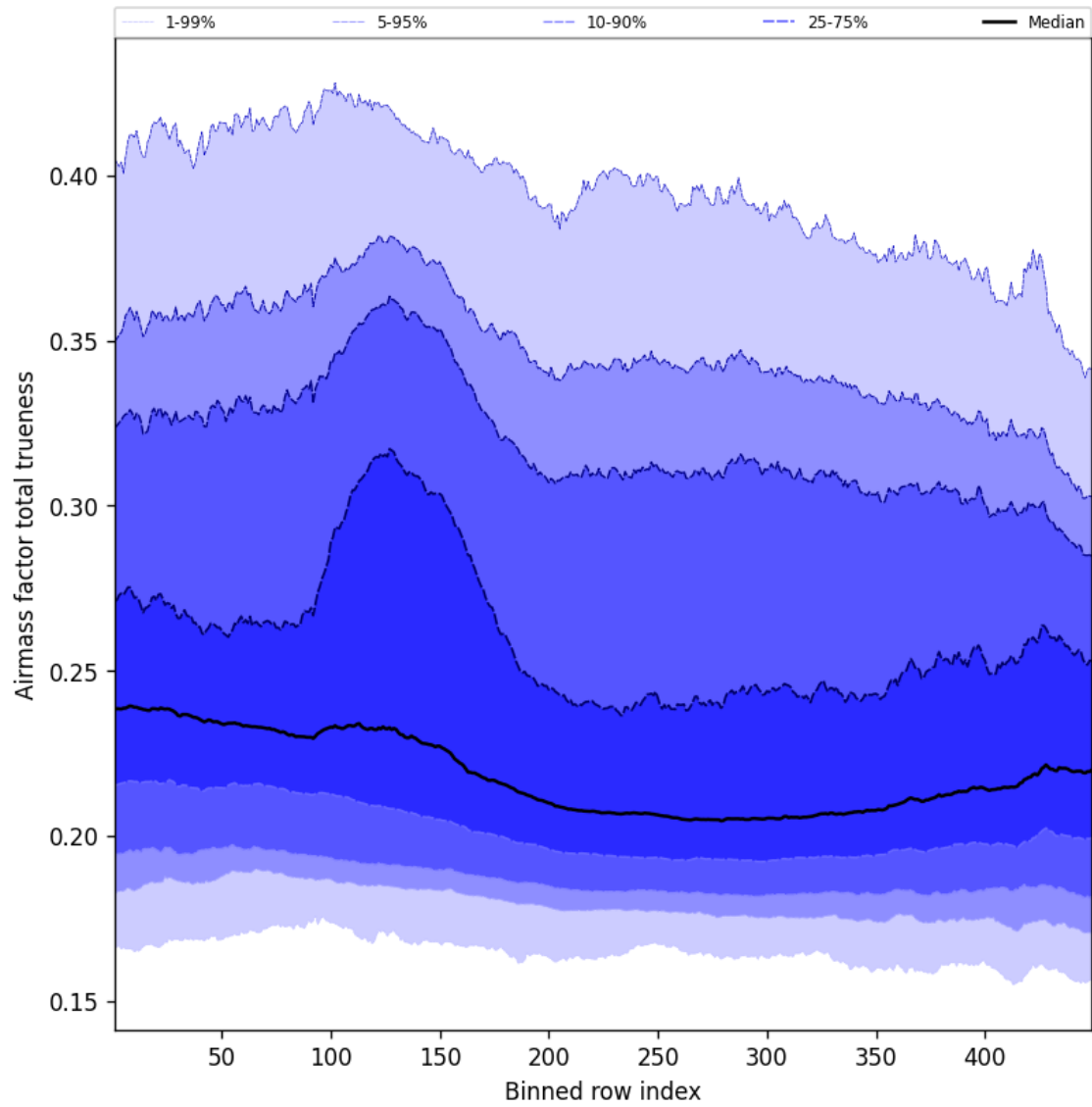
Figure 56: Along track statistics of “Airmass factor total truiness” for 2025-12-03 to 2025-12-04
