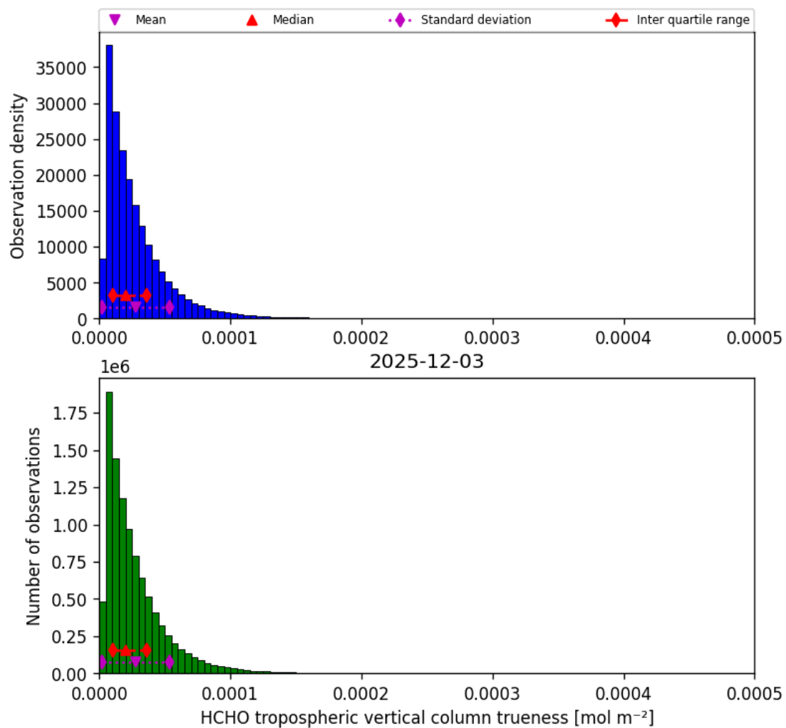
Figure 48: Histogram of “HCHO tropospheric vertical column trueness” for 2025-12-03 to 2025-12-04
