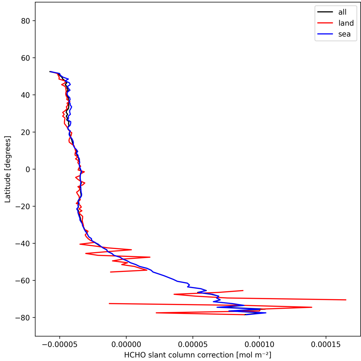
Figure 32: Zonal average of “HCHO slant column correction” for 2025-12-03 to 2025-12-04.
