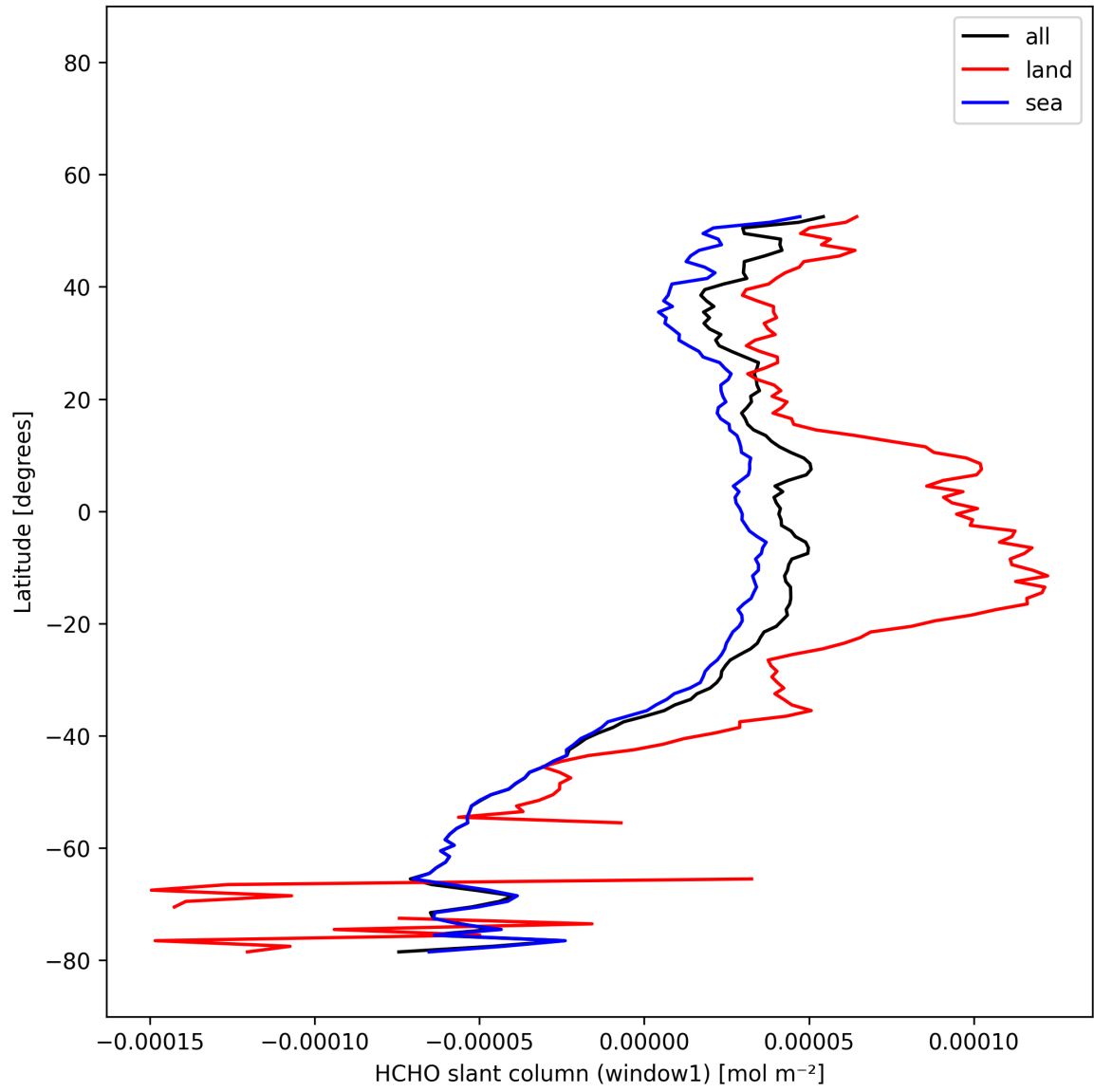
Figure 23: Zonal average of “HCHO slant column (window1)” for 2025-12-03 to 2025-12-04.
