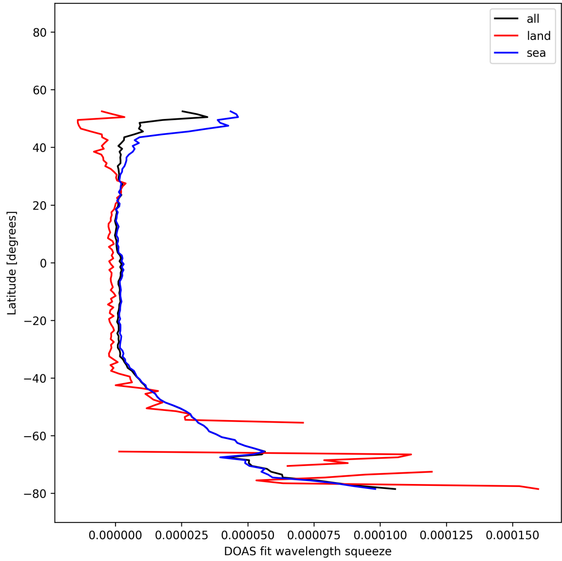
Figure 30: Zonal average of “DOAS fit wavelength squeeze” for 2025-12-03 to 2025-12-04.
