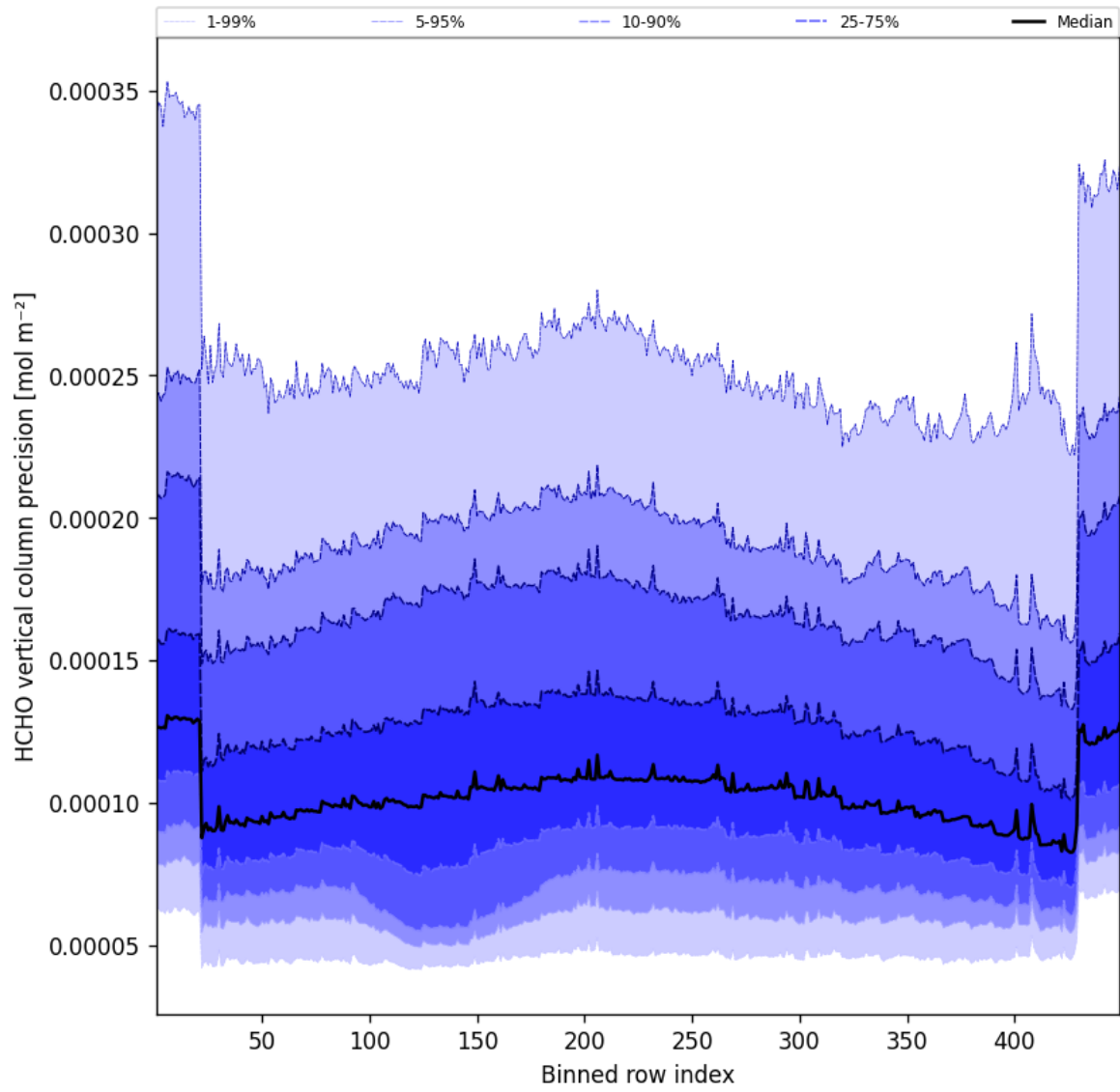
Figure 51: Along track statistics of “HCHO vertical column precision” for 2025-12-03 to 2025-12-04
