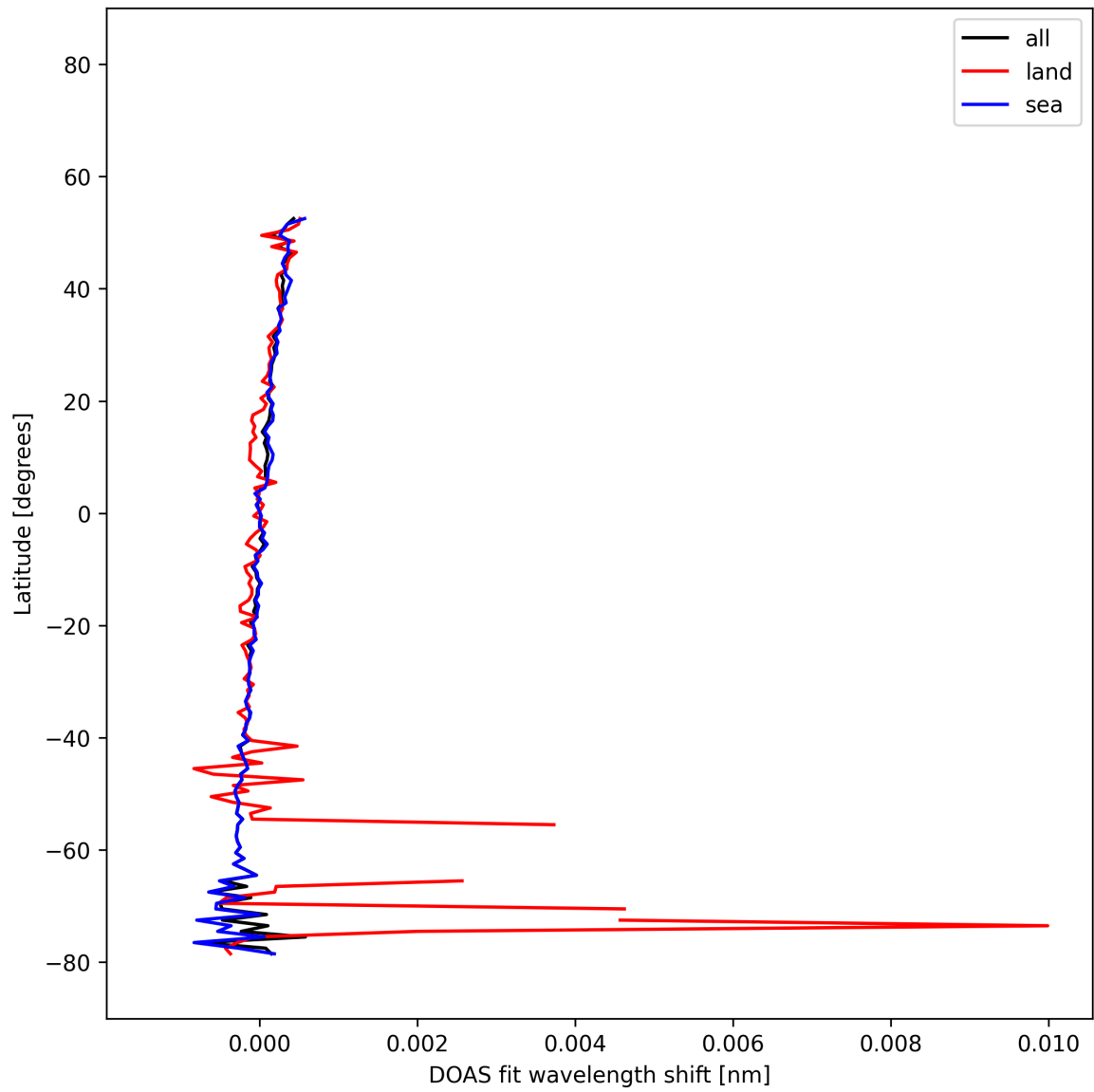
Figure 29: Zonal average of “DOAS fit wavelength shift” for 2025-12-03 to 2025-12-04.
