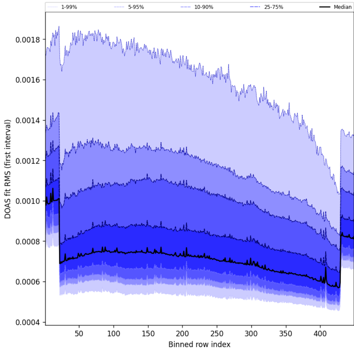
Figure 61: Along track statistics of “DOAS fit RMS (first interval)” for 2025-12-03 to 2025-12-04
