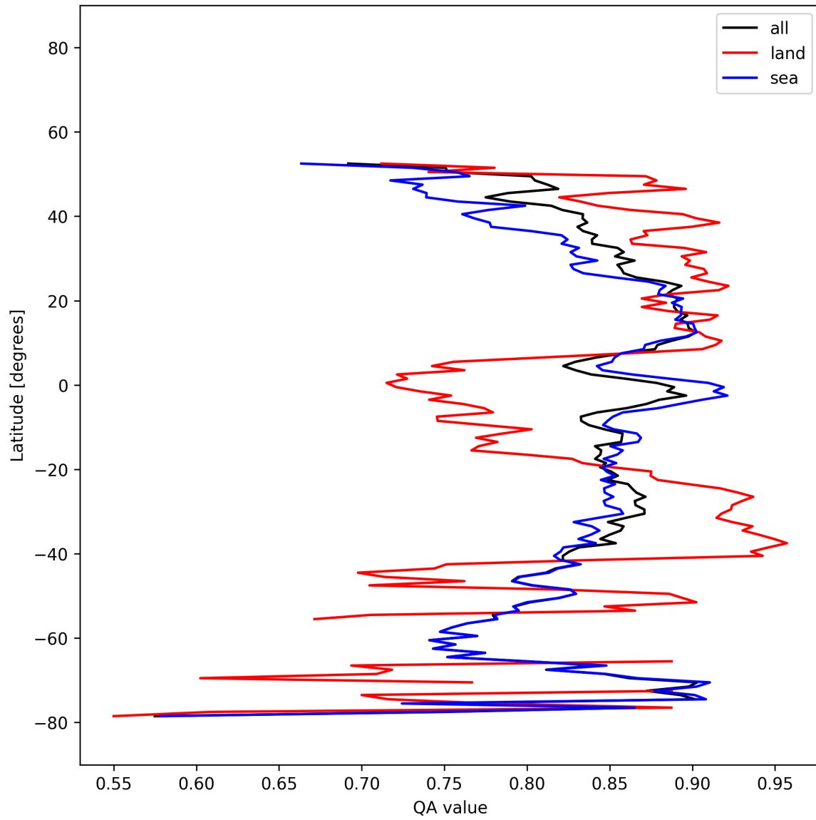
Figure 19: Zonal average of “QA value” for 2025-12-03 to 2025-12-04.
