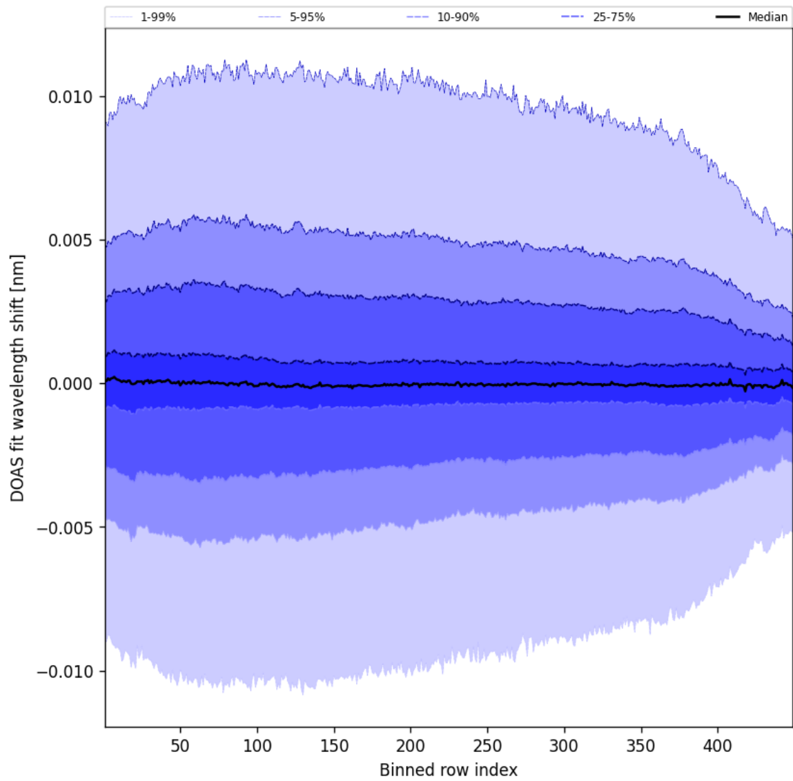
Figure 59: Along track statistics of “DOAS fit wavelength shift” for 2025-12-03 to 2025-12-04
