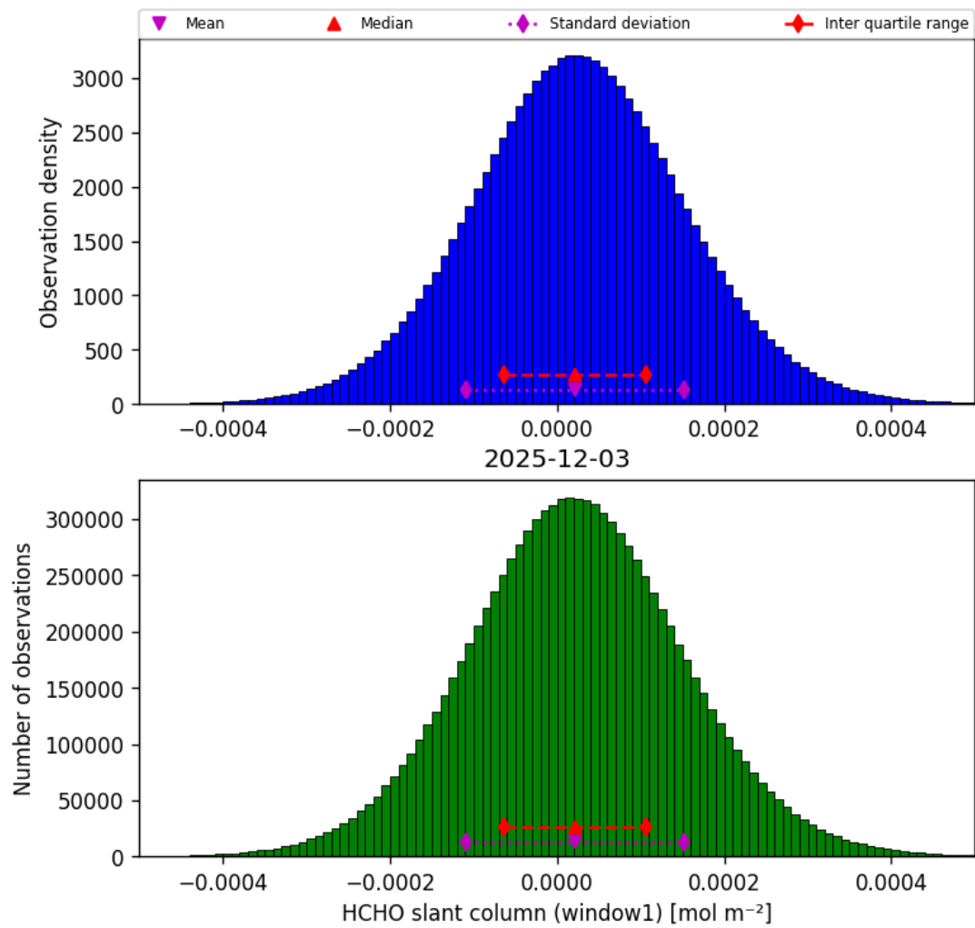
Figure 38: Histogram of “HCHO slant column (window1)” for 2025-12-03 to 2025-12-04
