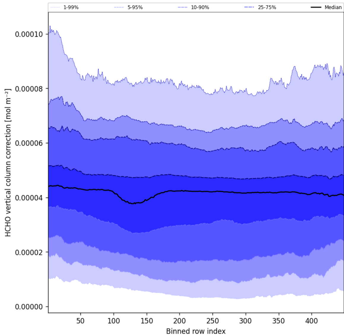
Figure 52: Along track statistics of “HCHO vertical column correction” for 2025-12-03 to 2025-12-04
