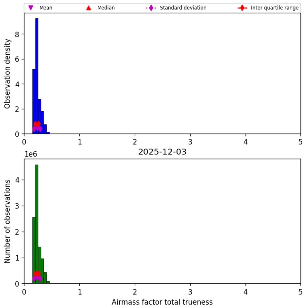
Figure 41: Histogram of “Airmass factor total trueness” for 2025-12-03 to 2025-12-04
