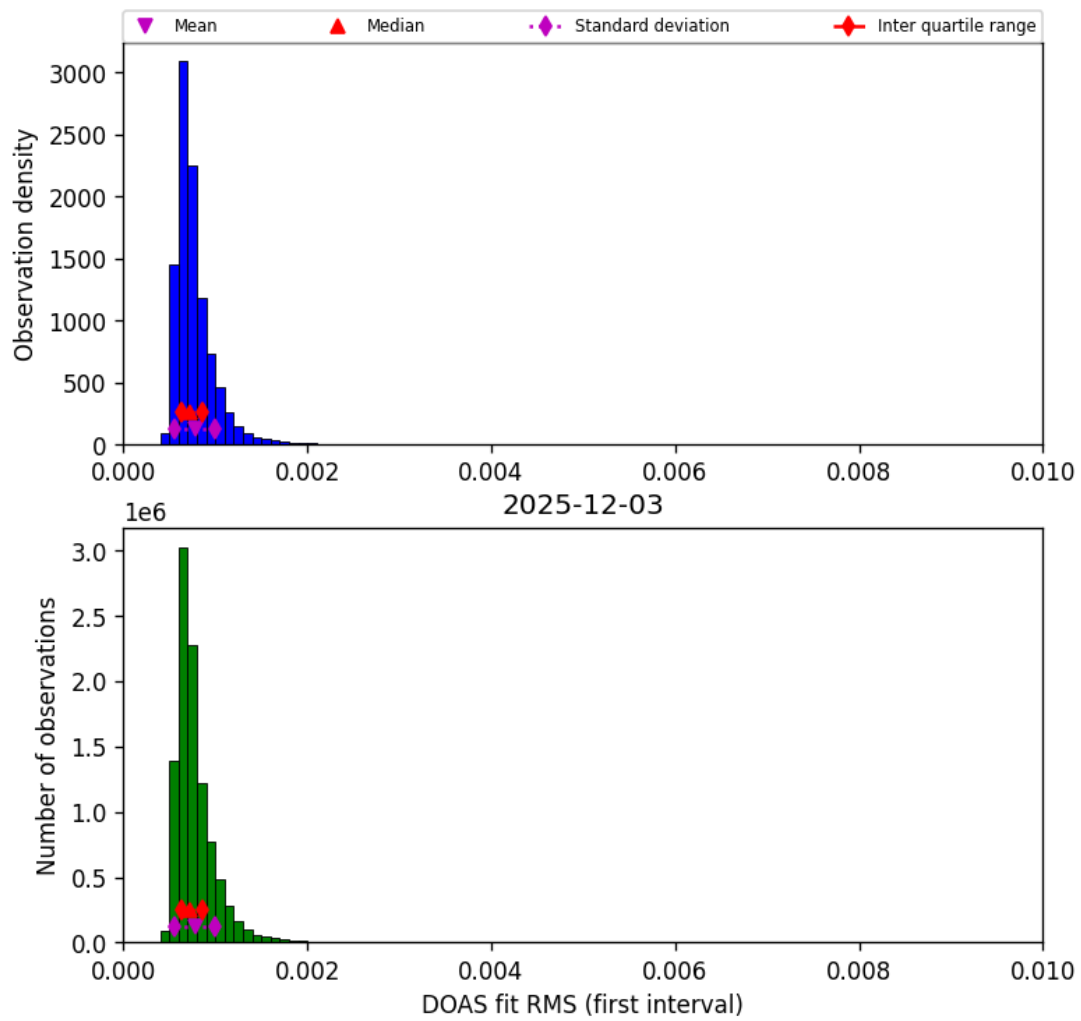
Figure 46: Histogram of “DOAS fit RMS (first interval)” for 2025-12-03 to 2025-12-04
