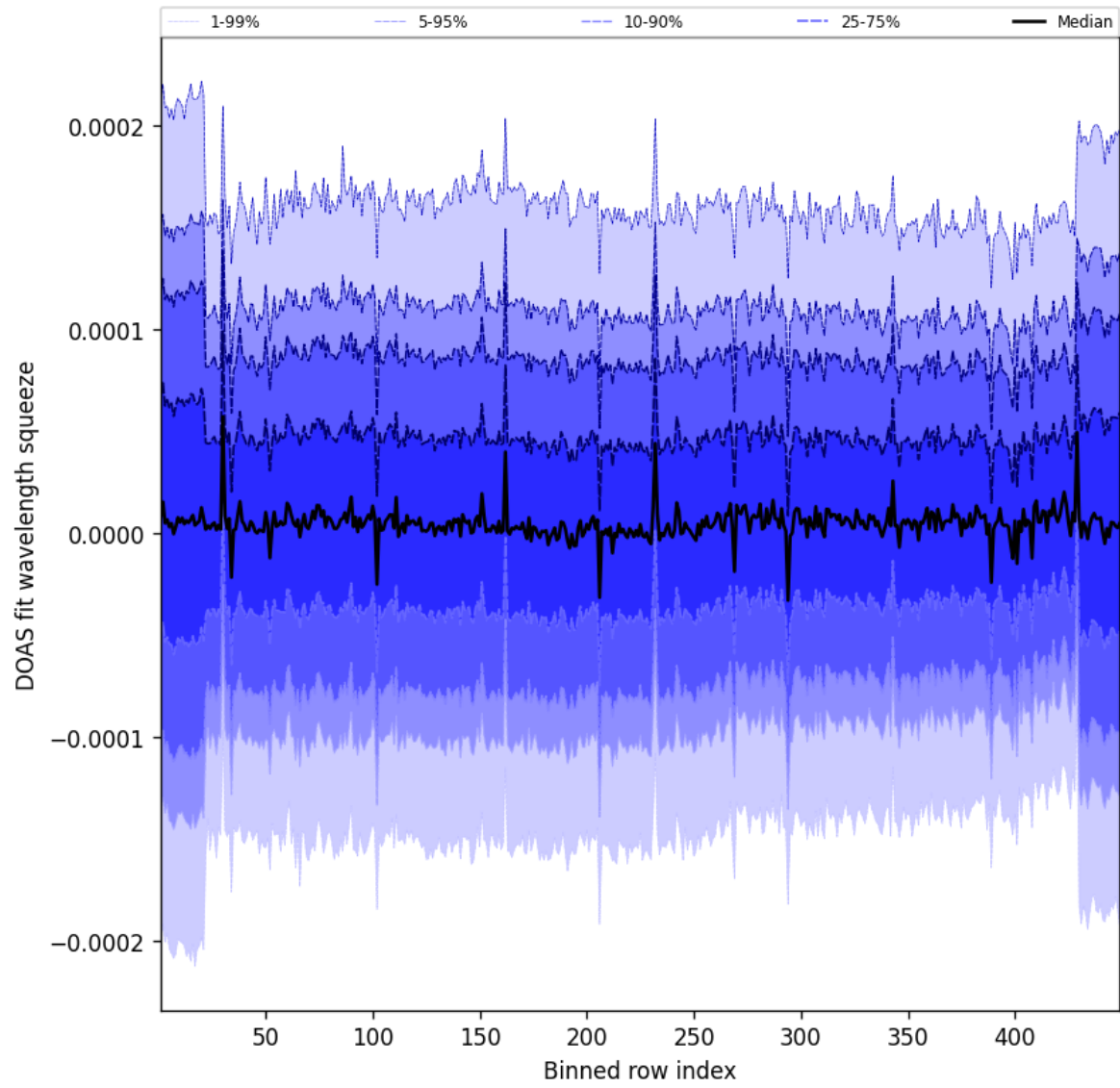
Figure 60: Along track statistics of “DOAS fit wavelength squeeze” for 2025-12-03 to 2025-12-04
