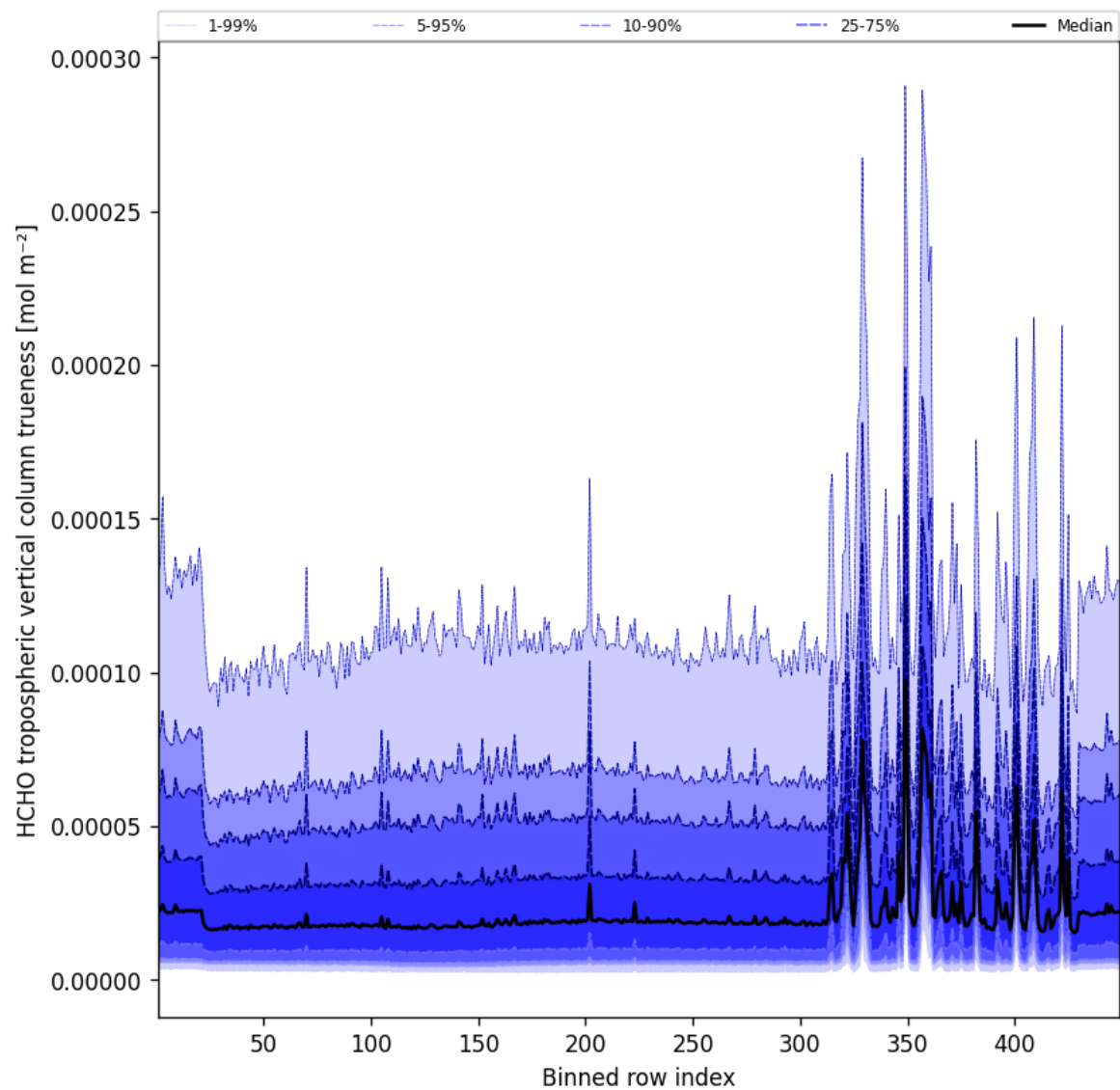
Figure 63: Along track statistics of “HCHO tropospheric vertical column trueness” for 2025-12-03 to 2025-12-04
