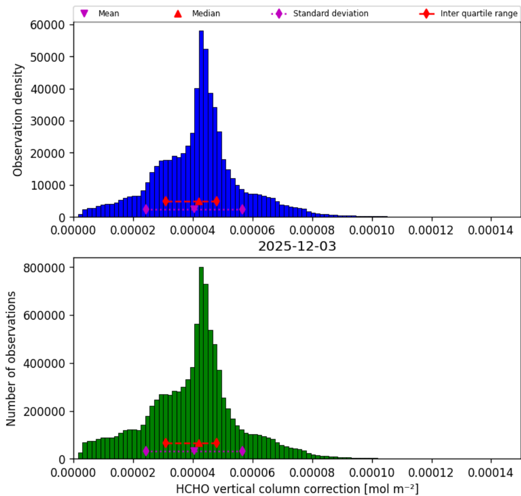
Figure 37: Histogram of “HCHO vertical column correction” for 2025-12-03 to 2025-12-04
