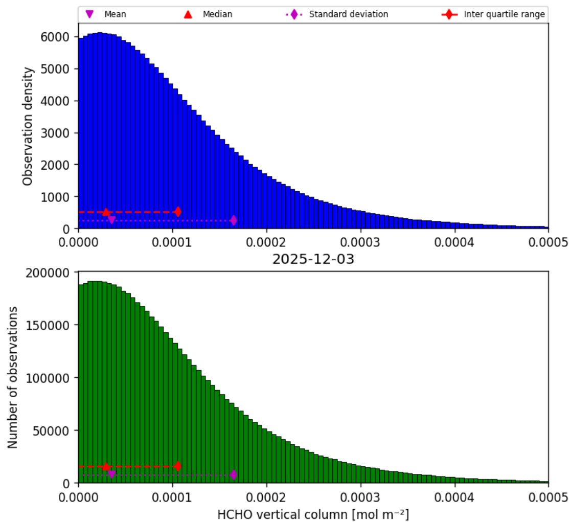
Figure 35: Histogram of “HCHO vertical column” for 2025-12-03 to 2025-12-04
