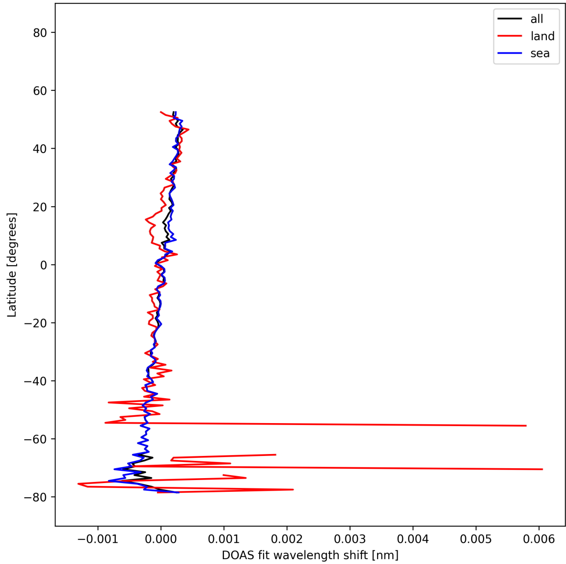
Figure 29: Zonal average of “DOAS fit wavelength shift” for 2025-12-04 to 2025-12-05.
