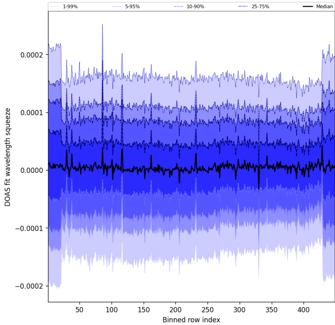
Figure 60: Along track statistics of “DOAS fit wavelength squeeze” for 2025-12-04 to 2025-12-05
