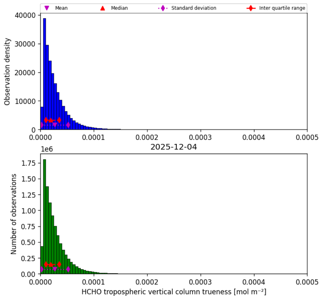
Figure 48: Histogram of “HCHO tropospheric vertical column trueness” for 2025-12-04 to 2025-12-05
