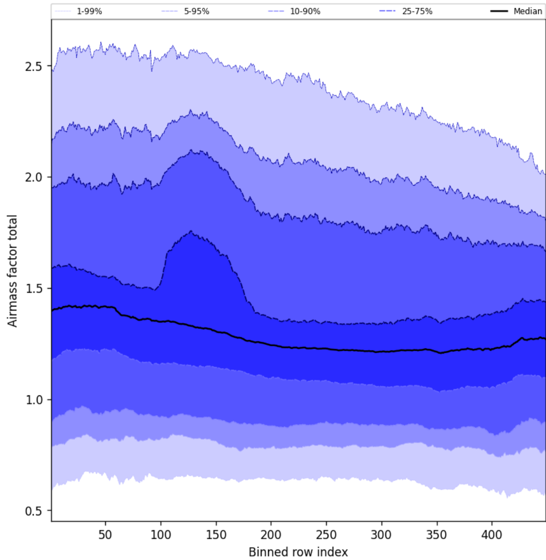
Figure 55: Along track statistics of “Airmass factor total” for 2025-12-04 to 2025-12-05
