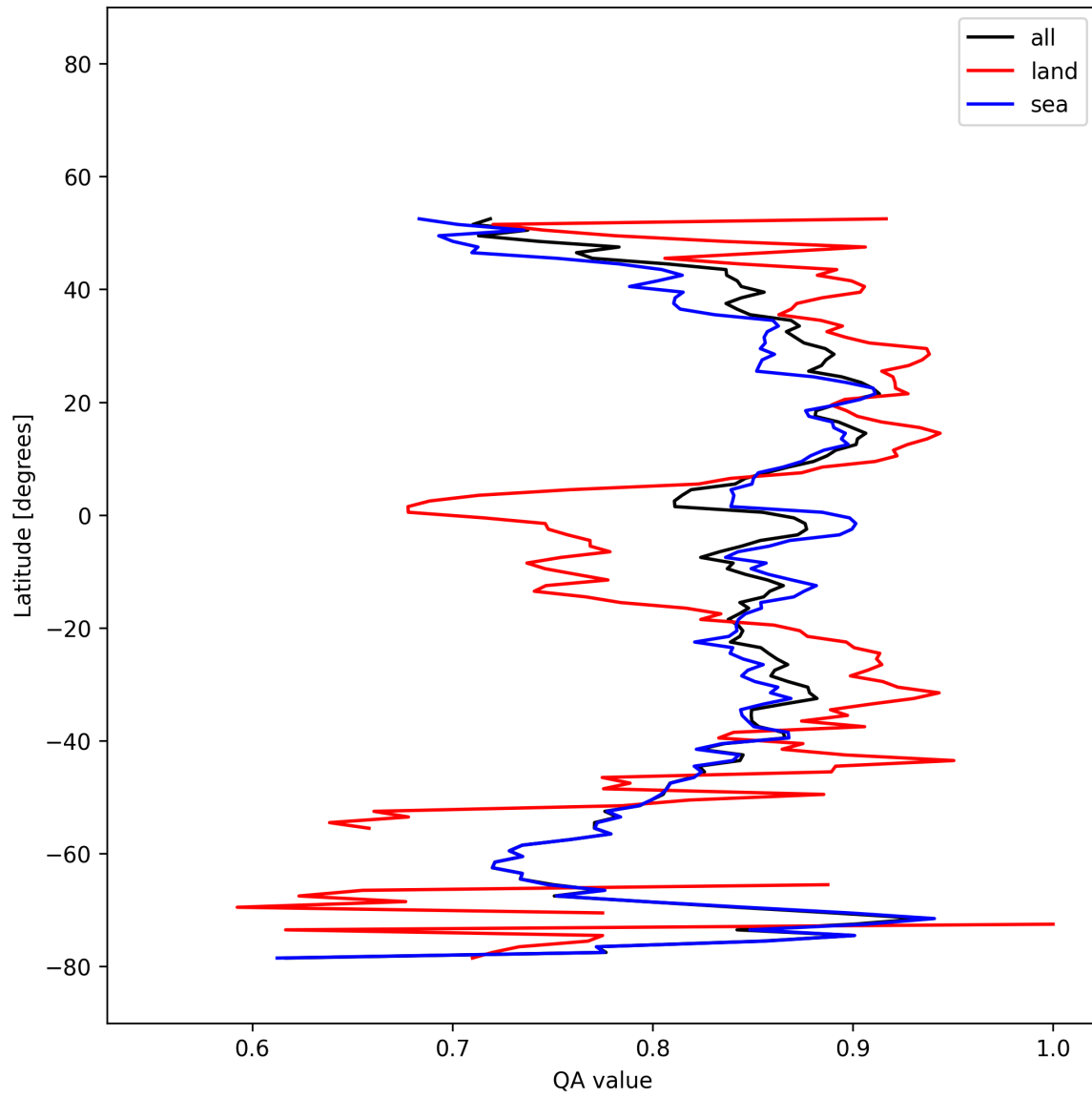
Figure 19: Zonal average of “QA value” for 2025-12-04 to 2025-12-05.
