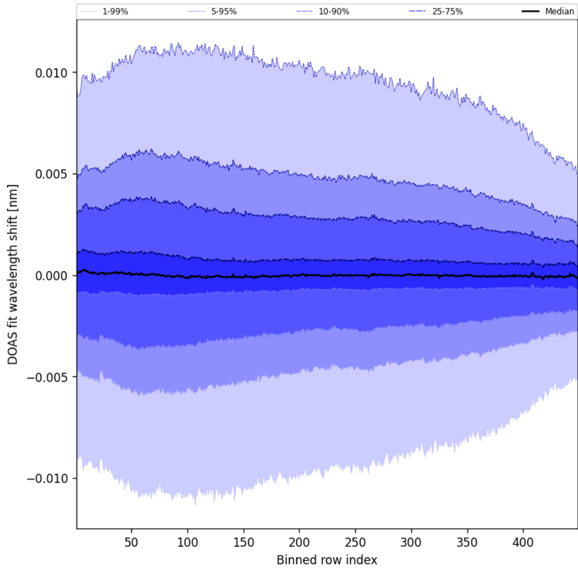
Figure 59: Along track statistics of “DOAS fit wavelength shift” for 2025-12-04 to 2025-12-05
