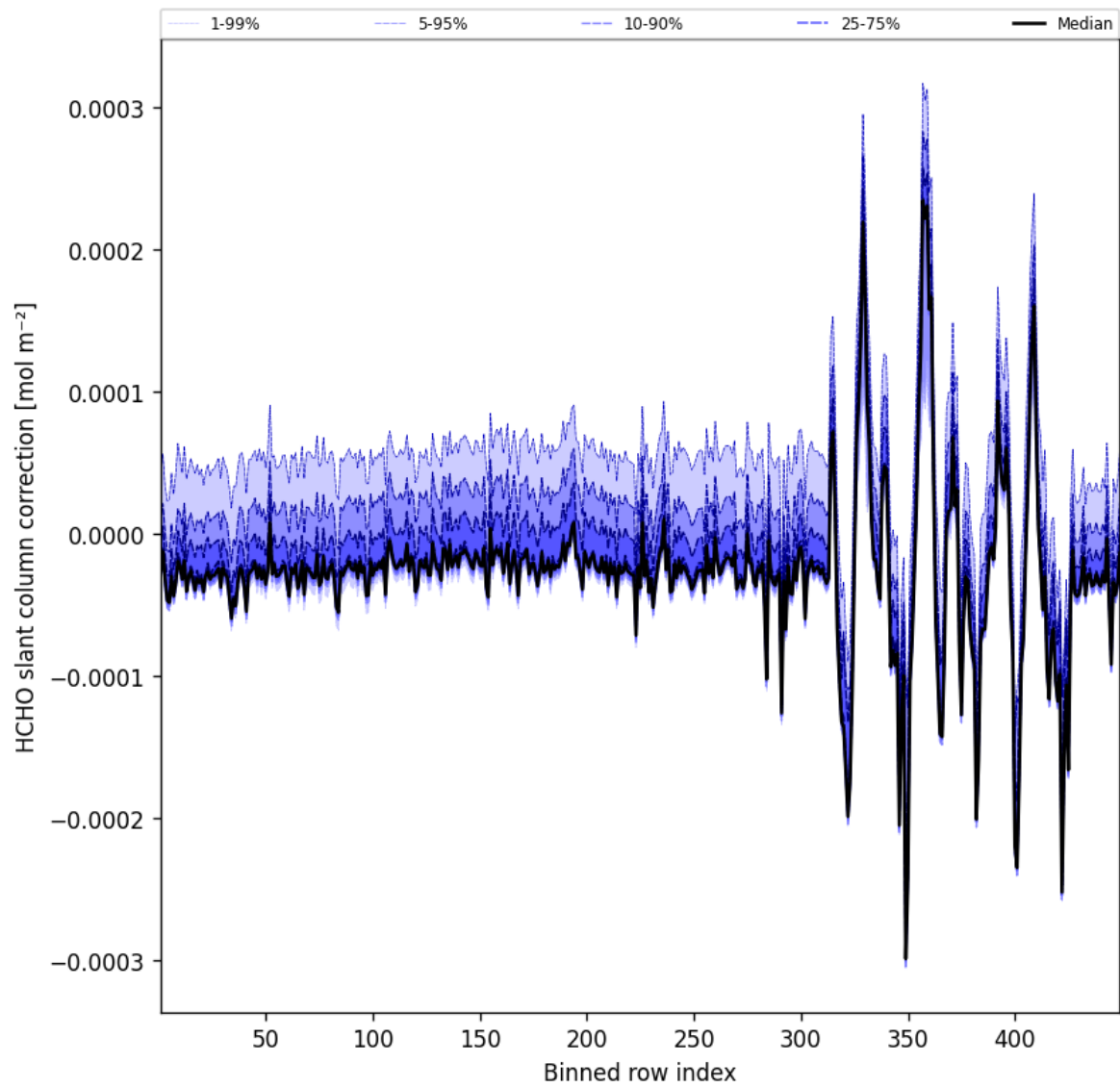
Figure 62: Along track statistics of “HCHO slant column correction” for 2025-12-04 to 2025-12-05
