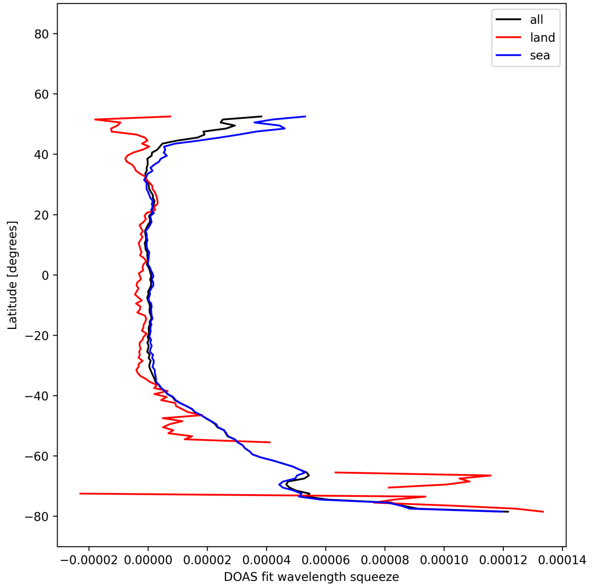
Figure 30: Zonal average of “DOAS fit wavelength squeeze” for 2025-12-04 to 2025-12-05.
