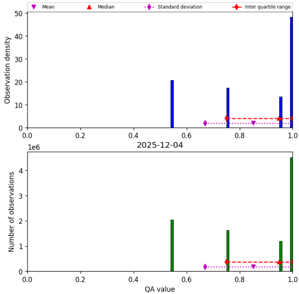
Figure 34: Histogram of “QA value” for 2025-12-04 to 2025-12-05
