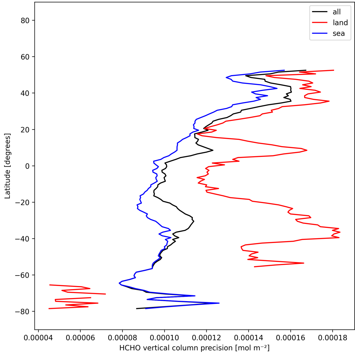
Figure 21: Zonal average of “HCHO vertical column precision” for 2025-12-04 to 2025-12-05.
