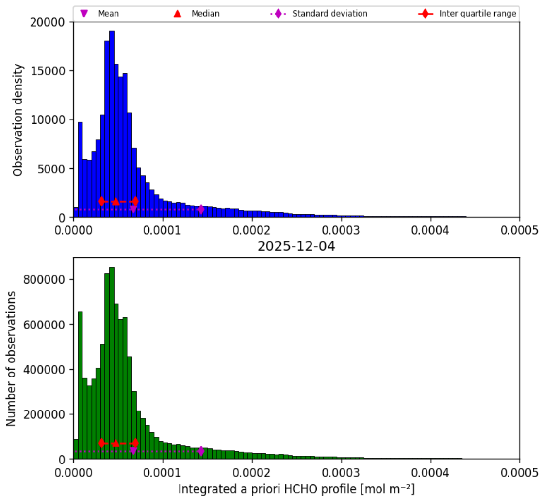
Figure 43: Histogram of “Integrated a priori HCHO profile” for 2025-12-04 to 2025-12-05
