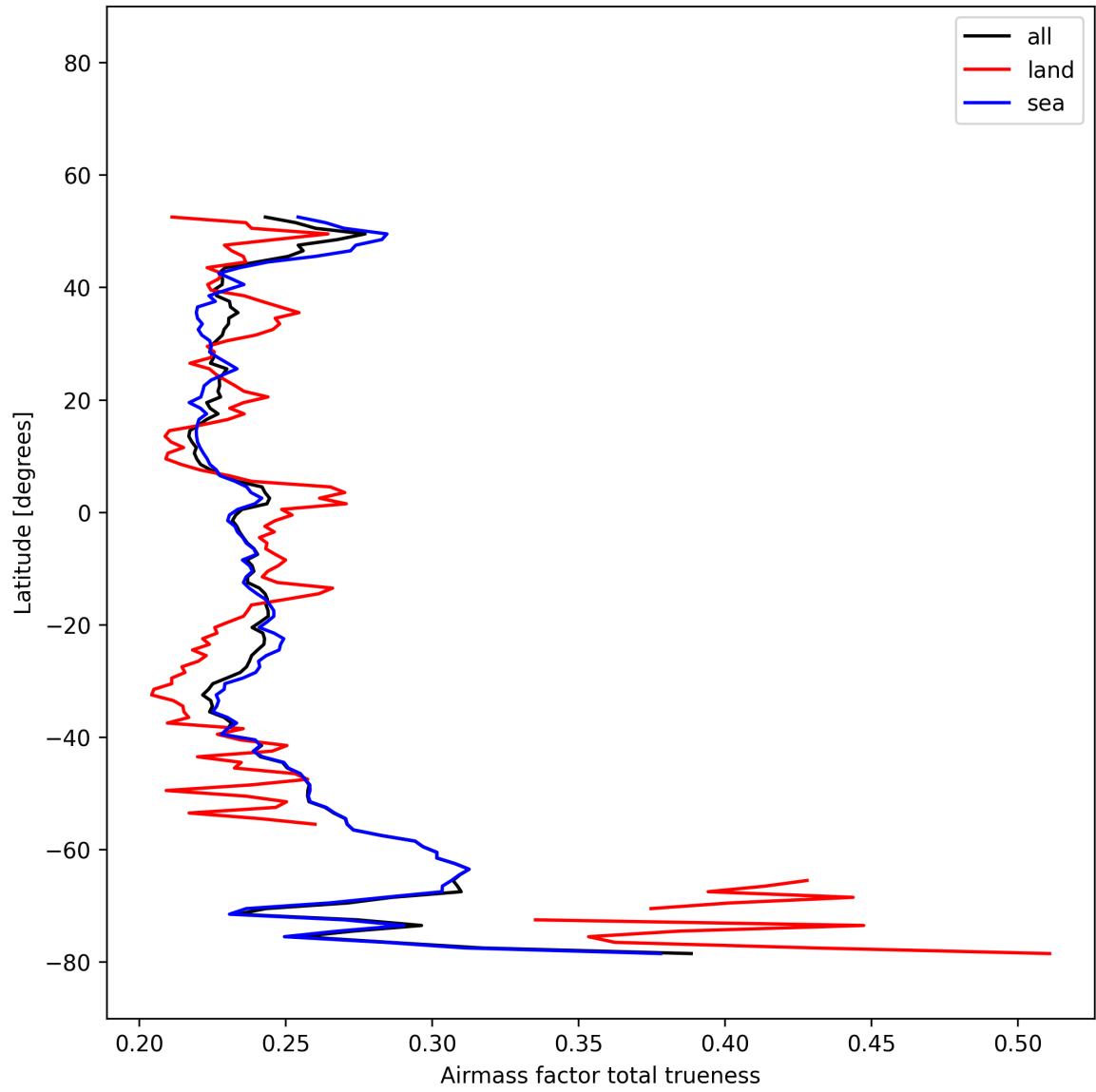
Figure 26: Zonal average of “Airmass factor total trueness” for 2025-12-04 to 2025-12-05.
