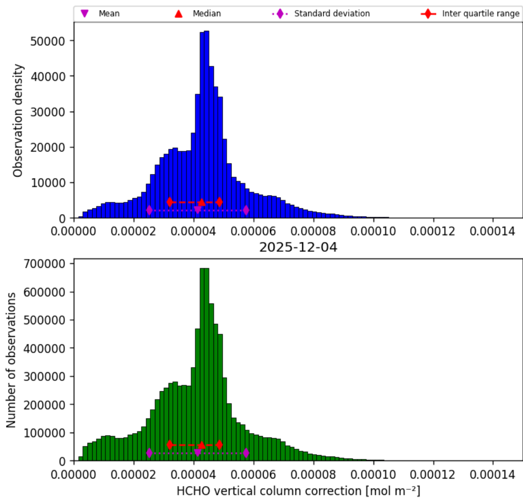
Figure 37: Histogram of “HCHO vertical column correction” for 2025-12-04 to 2025-12-05
