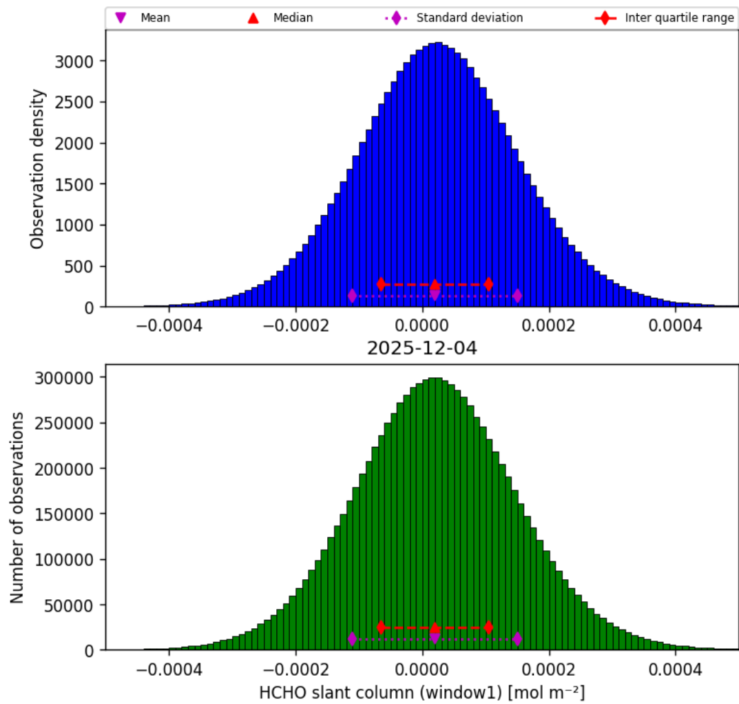
Figure 38: Histogram of “HCHO slant column (window1)” for 2025-12-04 to 2025-12-05
