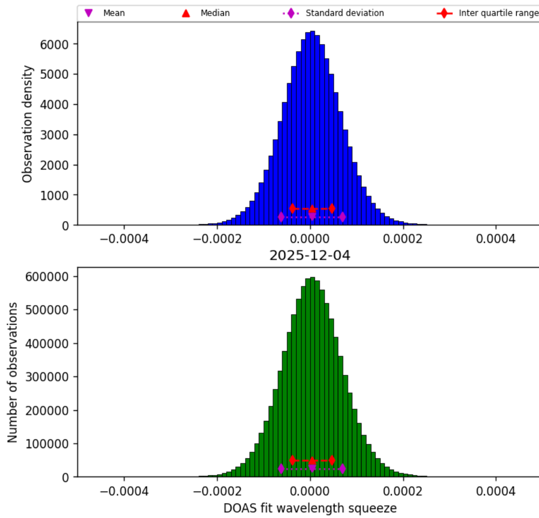
Figure 45: Histogram of “DOAS fit wavelength squeeze” for 2025-12-04 to 2025-12-05
