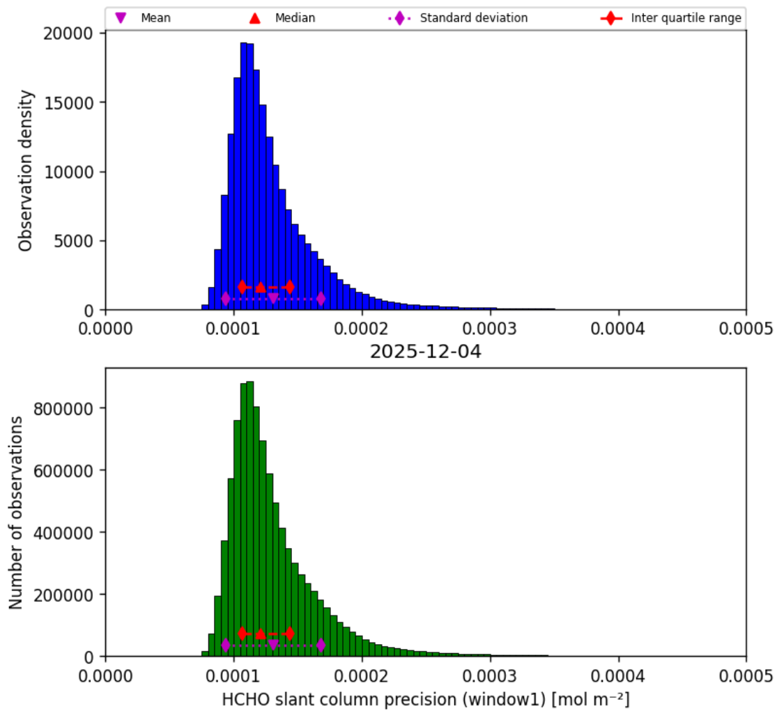
Figure 39: Histogram of “HCHO slant column precision (window1)” for 2025-12-04 to 2025-12-05
