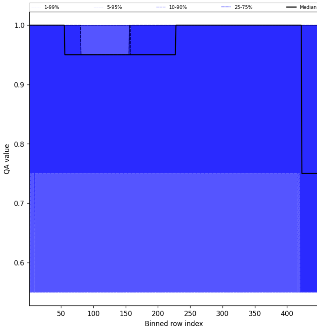
Figure 49: Along track statistics of “QA value” for 2025-12-04 to 2025-12-05
