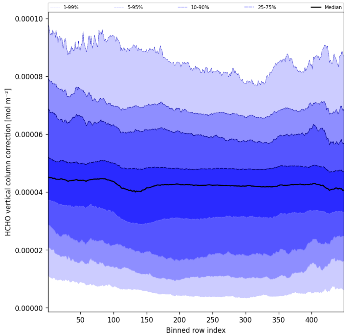
Figure 52: Along track statistics of “HCHO vertical column correction” for 2025-12-04 to 2025-12-05
