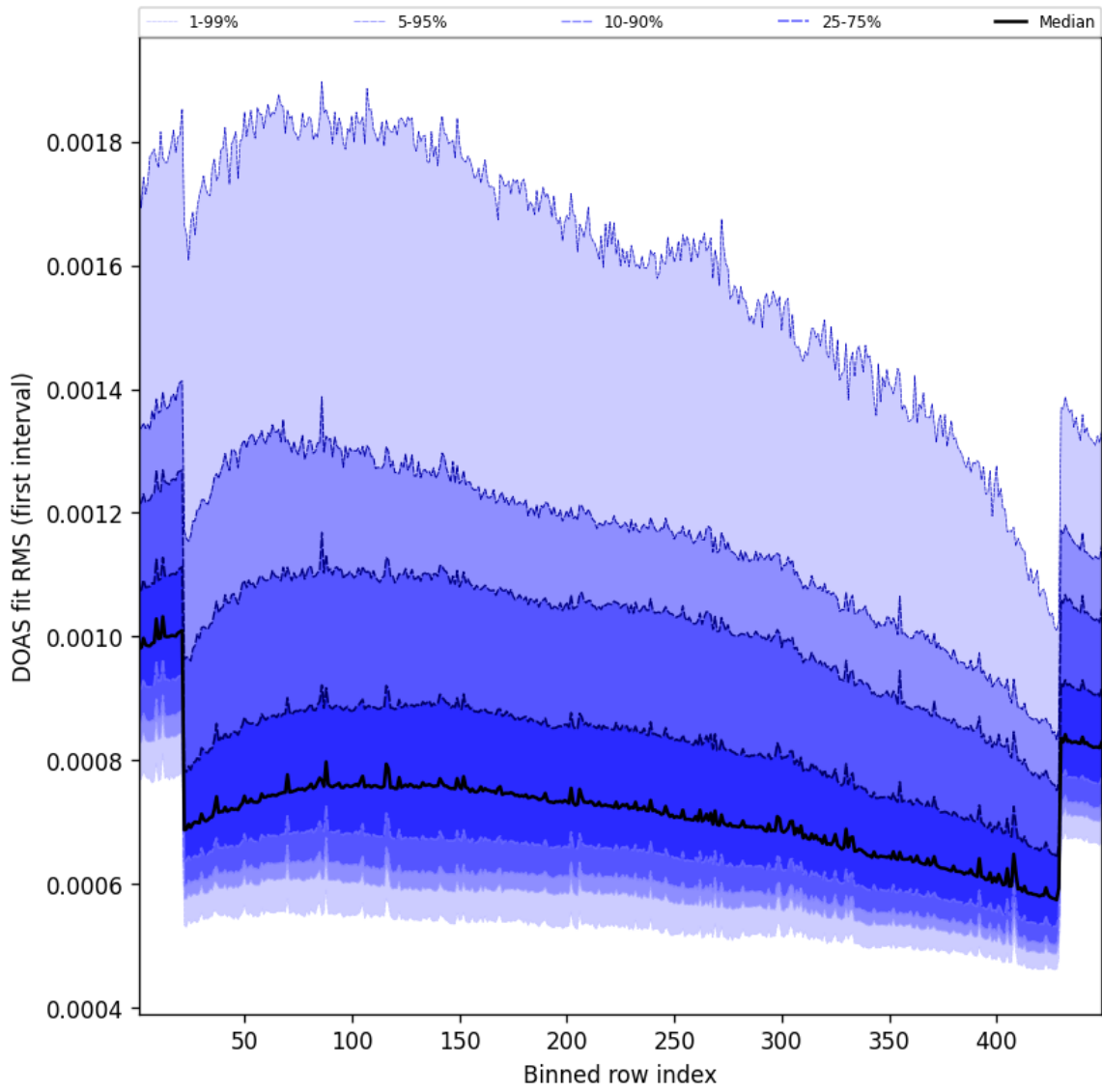
Figure 61: Along track statistics of “DOAS fit RMS (first interval)” for 2025-12-04 to 2025-12-05
