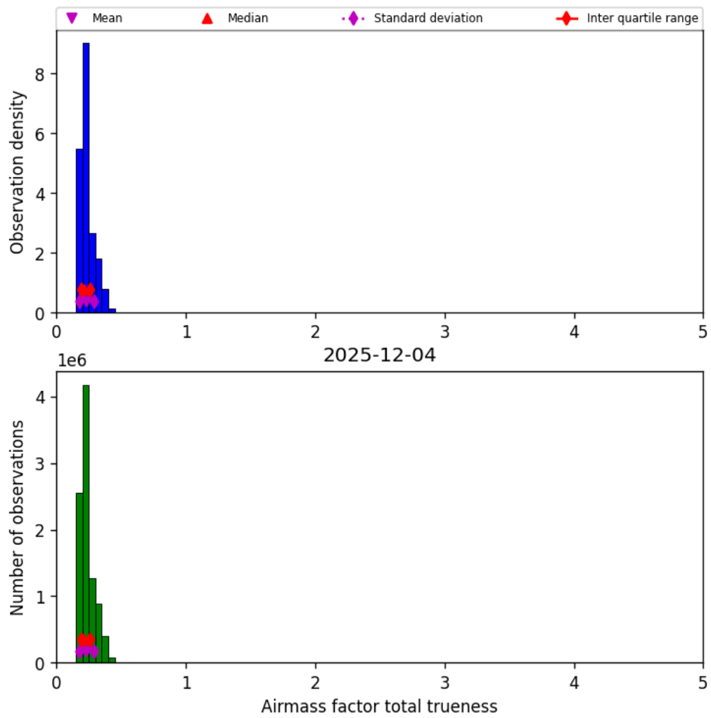
Figure 41: Histogram of “Airmass factor total trueness” for 2025-12-04 to 2025-12-05
