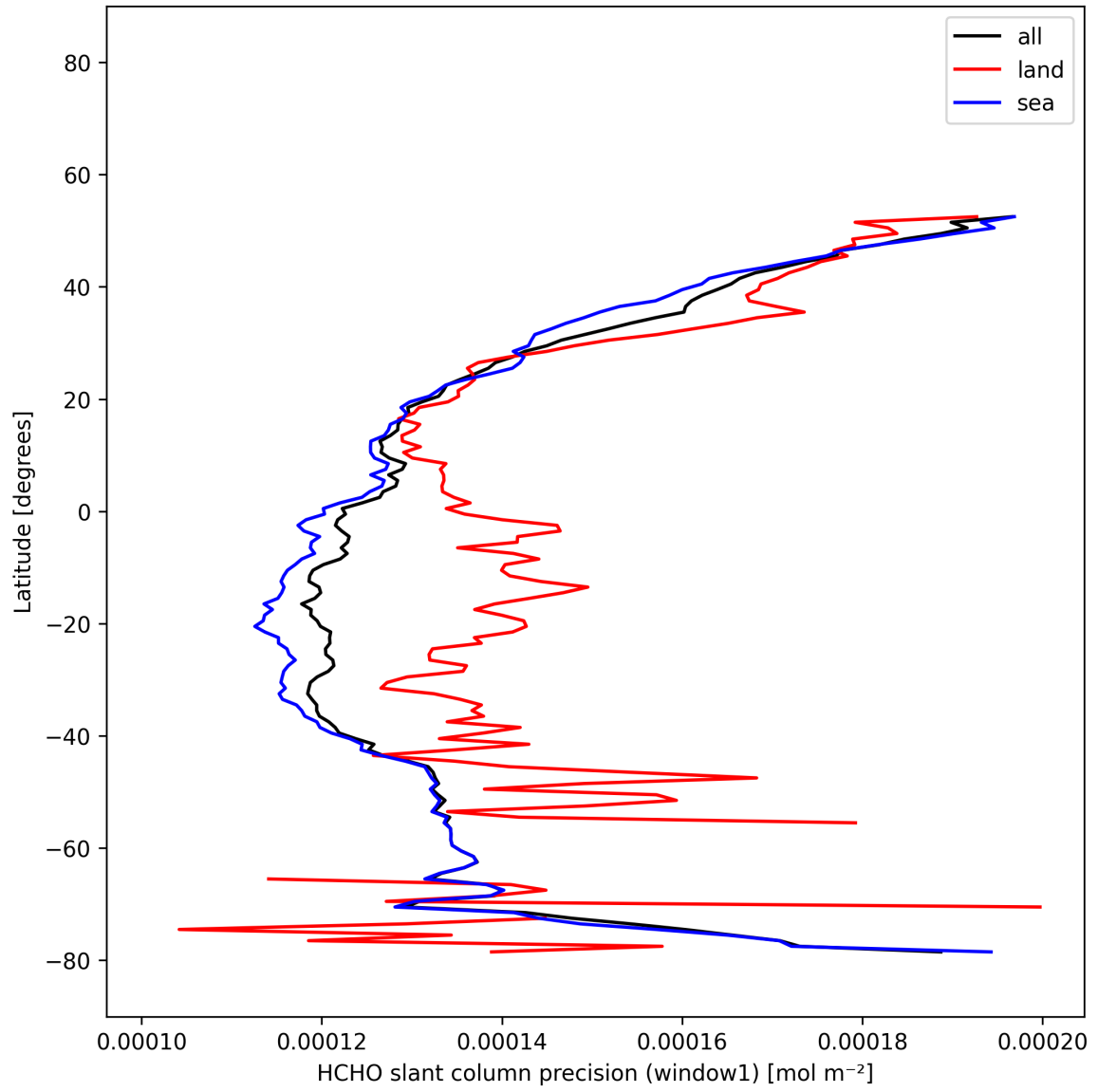
Figure 24: Zonal average of “HCHO slant column precision (window1)” for 2025-12-04 to 2025-12-05.
