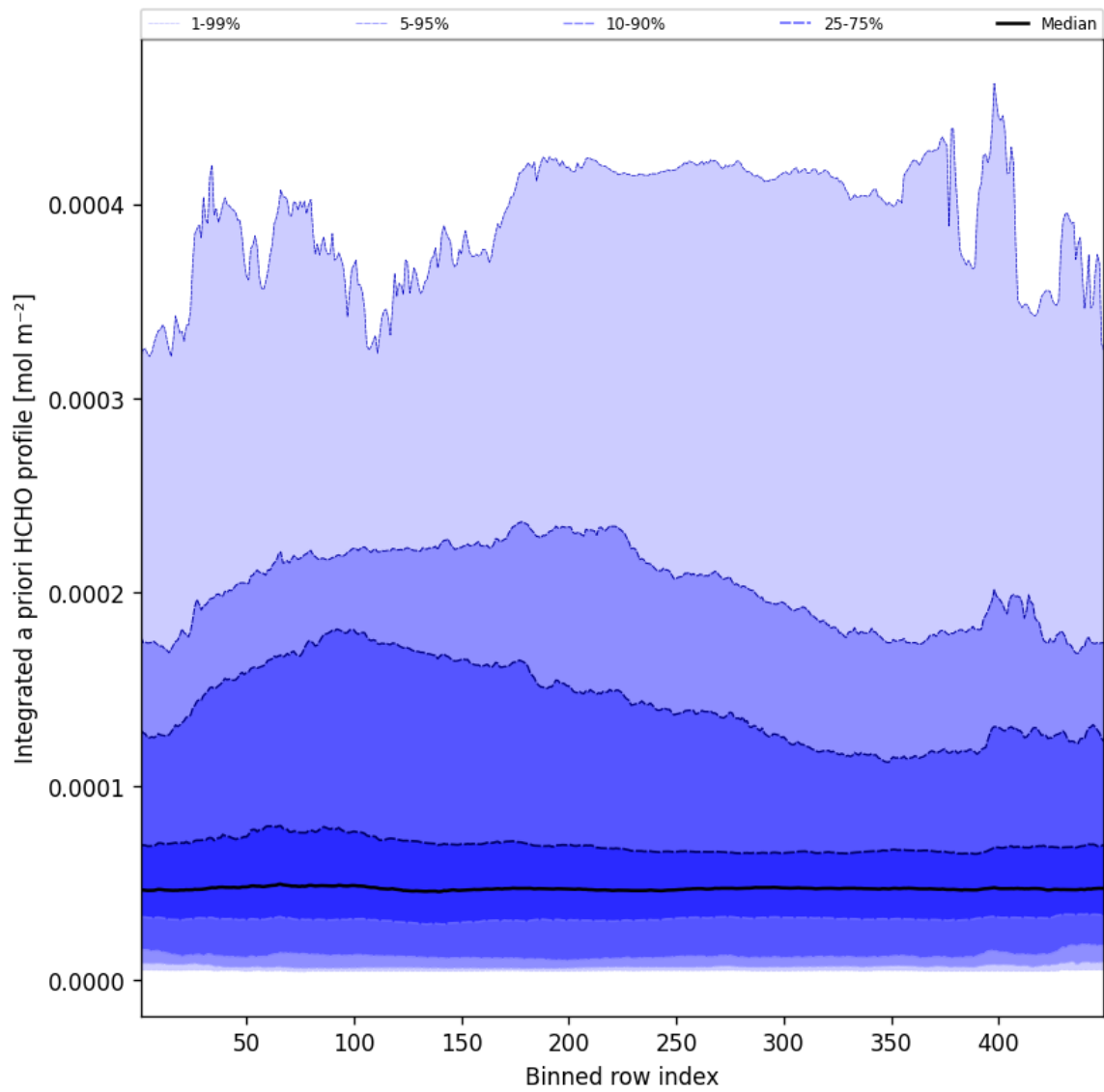
Figure 58: Along track statistics of “Integrated a priori HCHO profile” for 2025-12-04 to 2025-12-05
