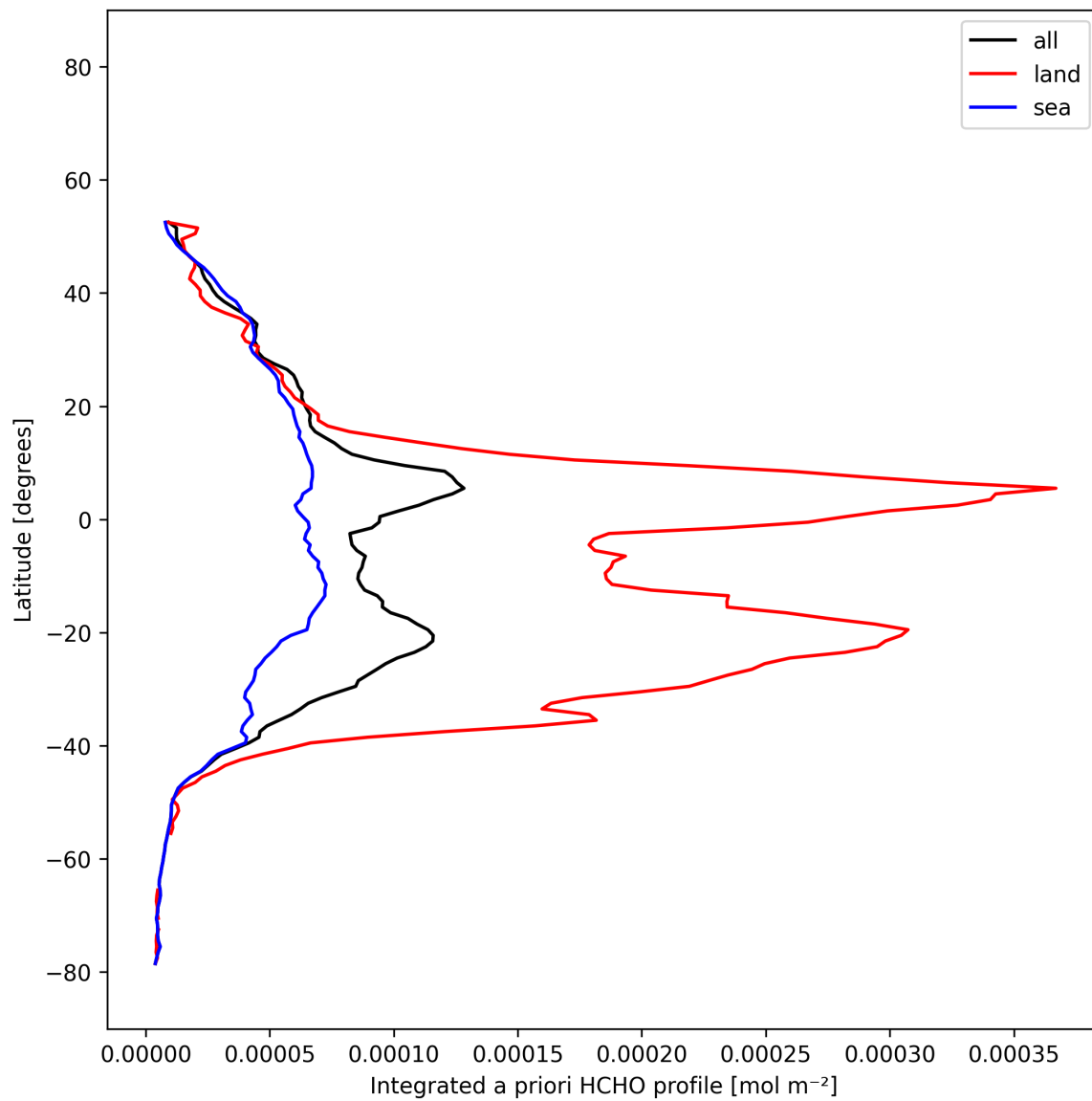
Figure 28: Zonal average of “Integrated a priori HCHO profile” for 2025-12-04 to 2025-12-05.
