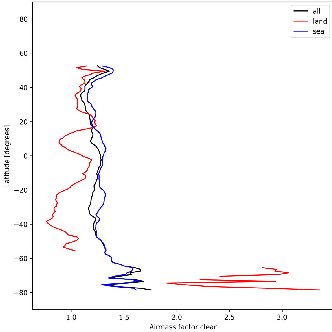
Figure 27: Zonal average of “Airmass factor clear” for 2025-12-04 to 2025-12-05.
