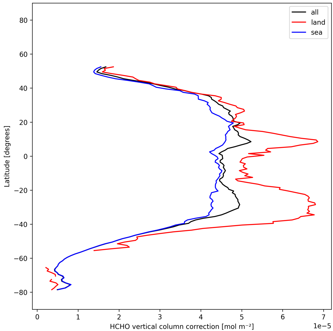
Figure 22: Zonal average of “HCHO vertical column correction” for 2025-12-04 to 2025-12-05.
