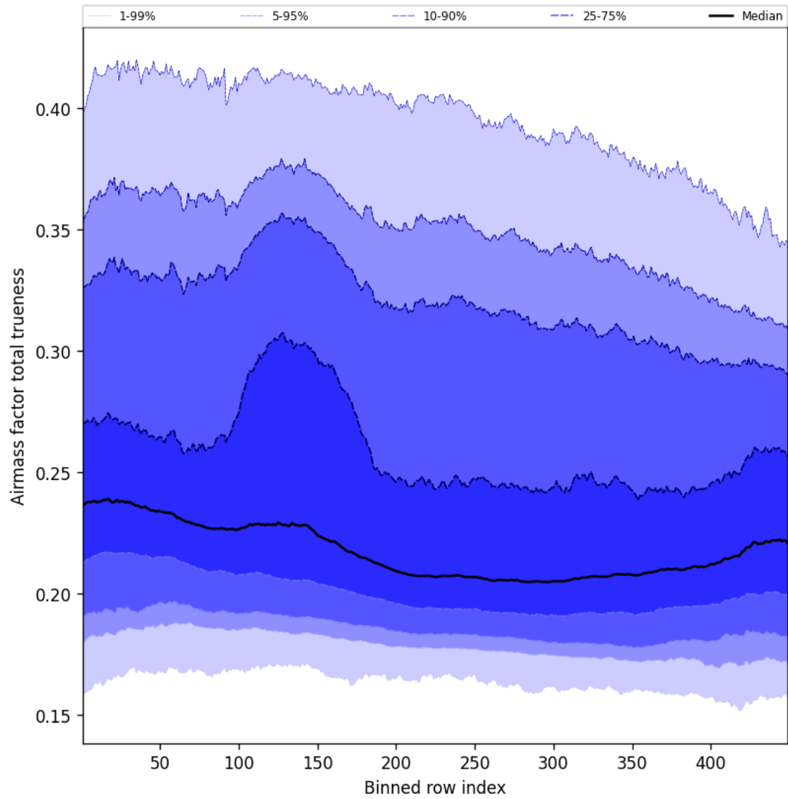
Figure 56: Along track statistics of “Airmass factor total truiness” for 2025-12-04 to 2025-12-05
