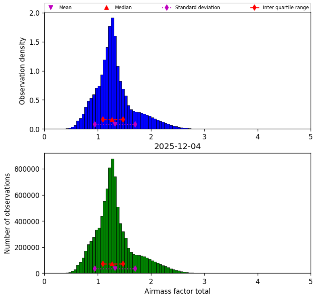
Figure 40: Histogram of “Airmass factor total” for 2025-12-04 to 2025-12-05
