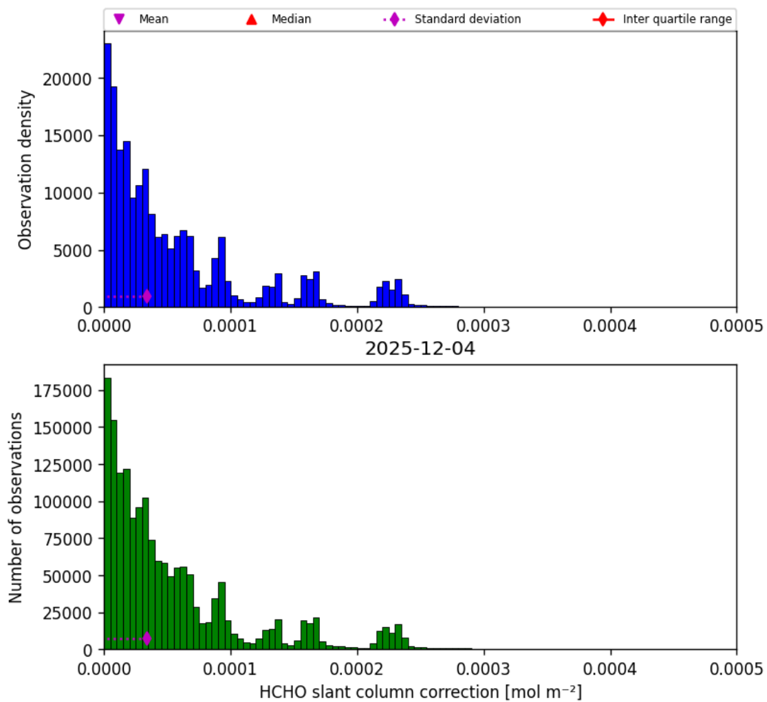
Figure 47: Histogram of “HCHO slant column correction” for 2025-12-04 to 2025-12-05
