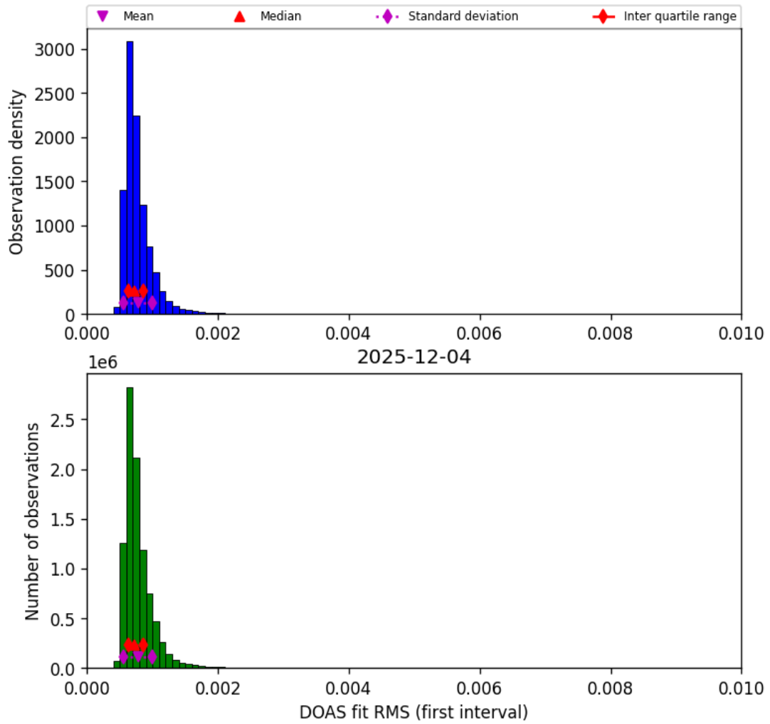
Figure 46: Histogram of “DOAS fit RMS (first interval)” for 2025-12-04 to 2025-12-05
