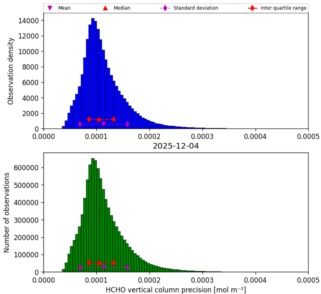
Figure 36: Histogram of “HCHO vertical column precision” for 2025-12-04 to 2025-12-05
