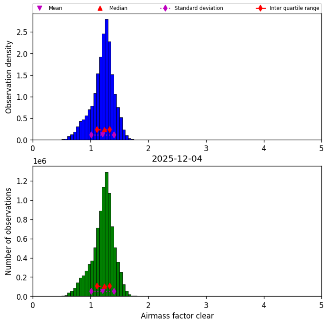
Figure 42: Histogram of “Airmass factor clear” for 2025-12-04 to 2025-12-05
