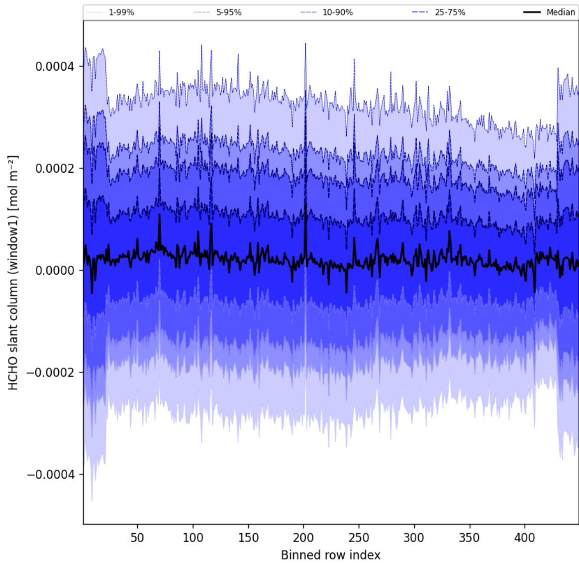
Figure 53: Along track statistics of “HCHO slant column (window1)” for 2025-12-04 to 2025-12-05
