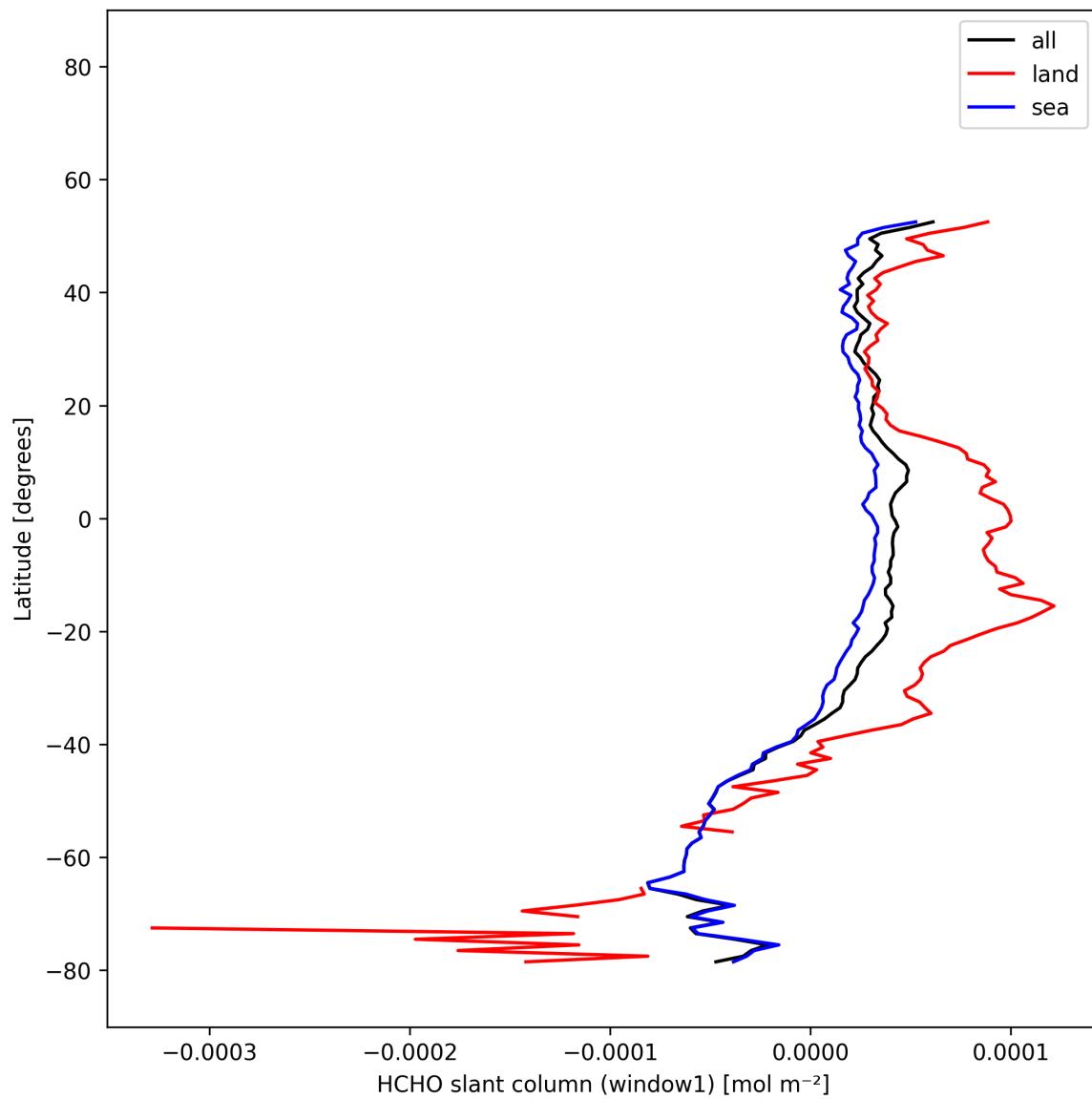
Figure 23: Zonal average of “HCHO slant column (window1)” for 2025-12-04 to 2025-12-05.
