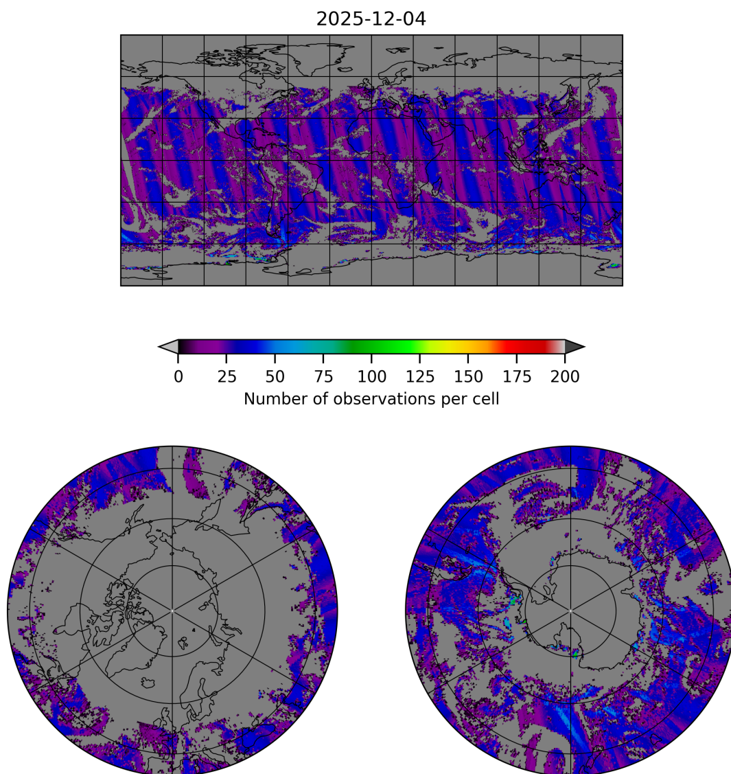
Figure 18: Map of the number of observations for 2025-12-04 to 2025-12-05
