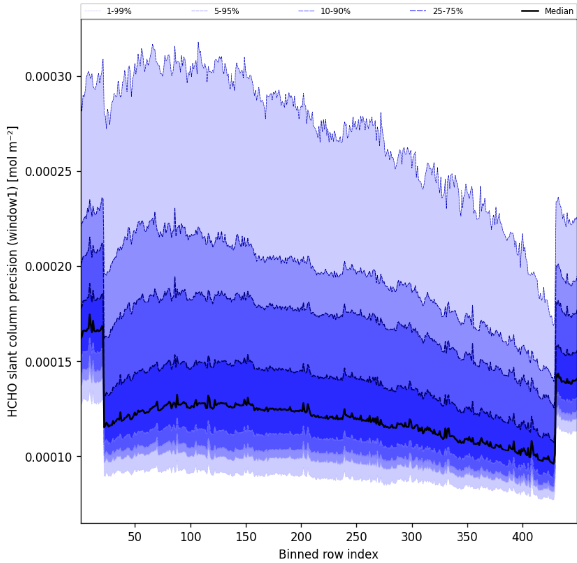
Figure 54: Along track statistics of “HCHO slant column precision (window1)” for 2025-12-04 to 2025-12-05
