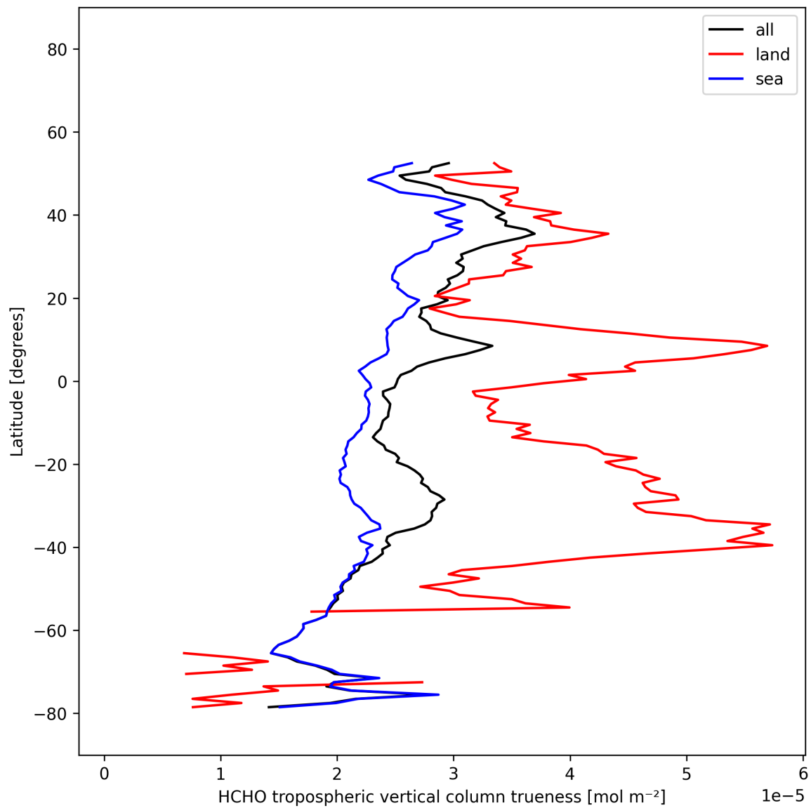
Figure 33: Zonal average of “HCHO tropospheric vertical column trueness” for 2025-12-04 to 2025-12-05.
