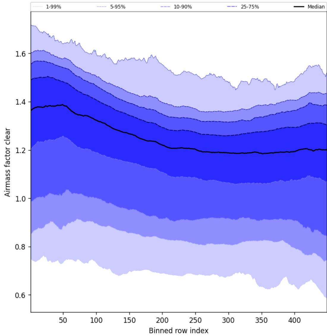
Figure 57: Along track statistics of “Airmass factor clear” for 2025-12-04 to 2025-12-05
