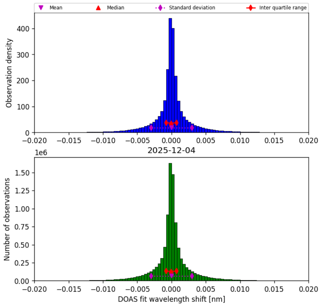
Figure 44: Histogram of “DOAS fit wavelength shift” for 2025-12-04 to 2025-12-05
