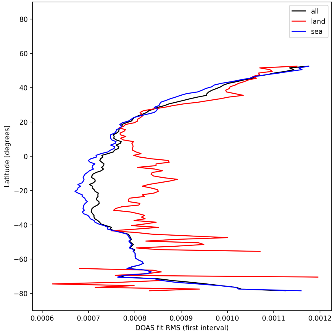
Figure 31: Zonal average of “DOAS fit RMS (first interval)” for 2025-12-04 to 2025-12-05.
