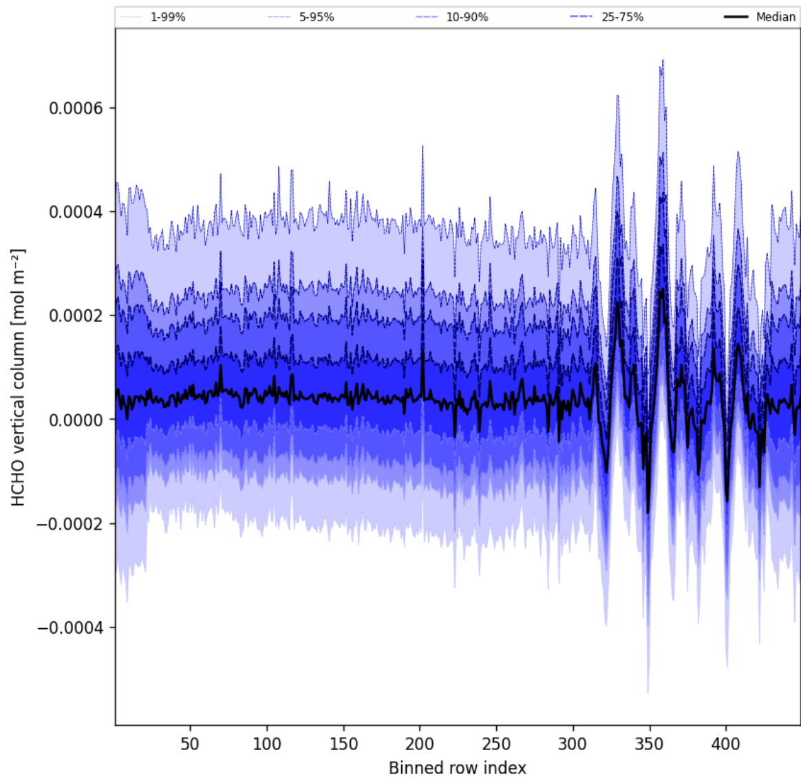
Figure 50: Along track statistics of “HCHO vertical column” for 2025-12-04 to 2025-12-05
