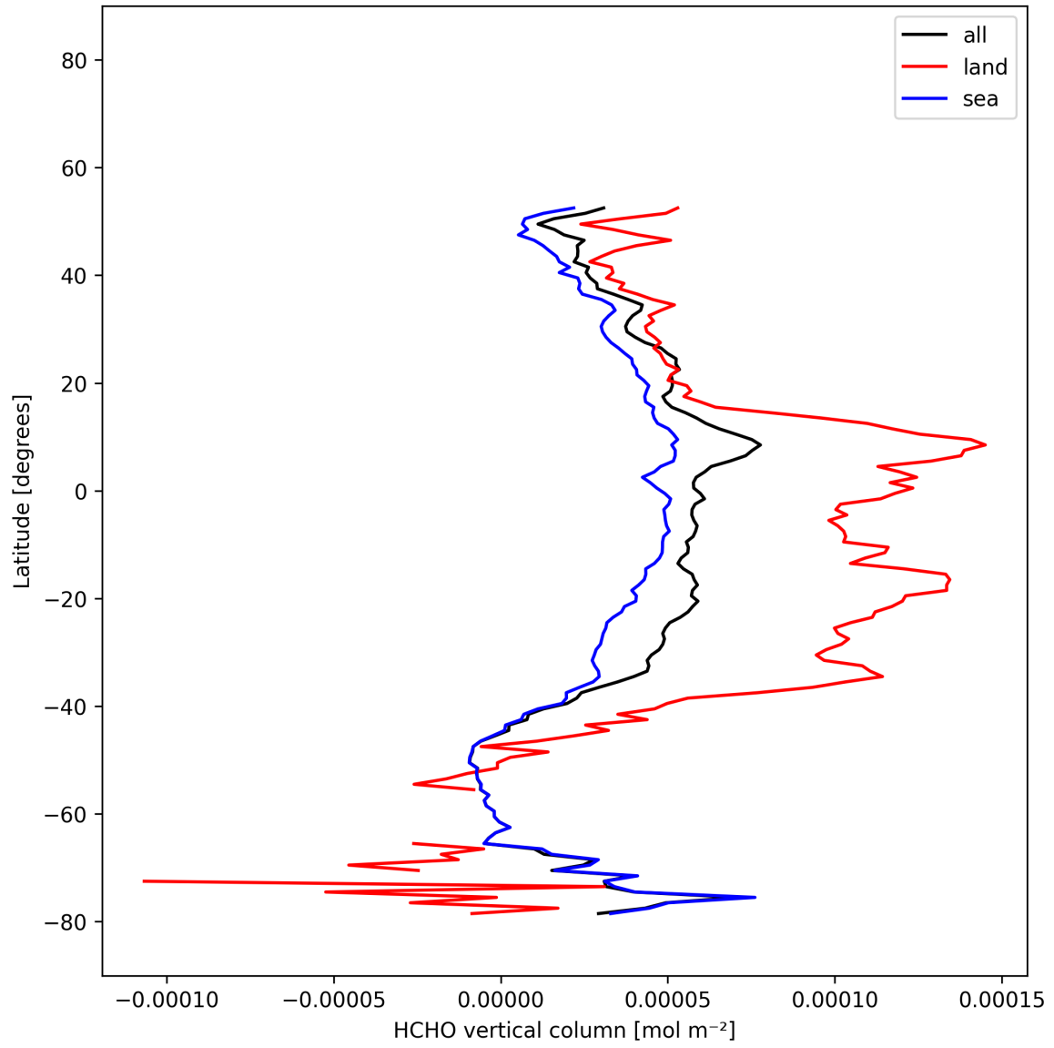
Figure 20: Zonal average of “HCHO vertical column” for 2025-12-04 to 2025-12-05.
