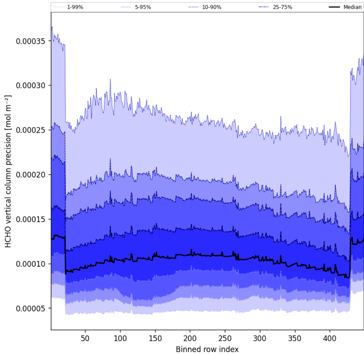
Figure 51: Along track statistics of "HCHO vertical column precision" for 2025-12-04 to 2025-12-05
