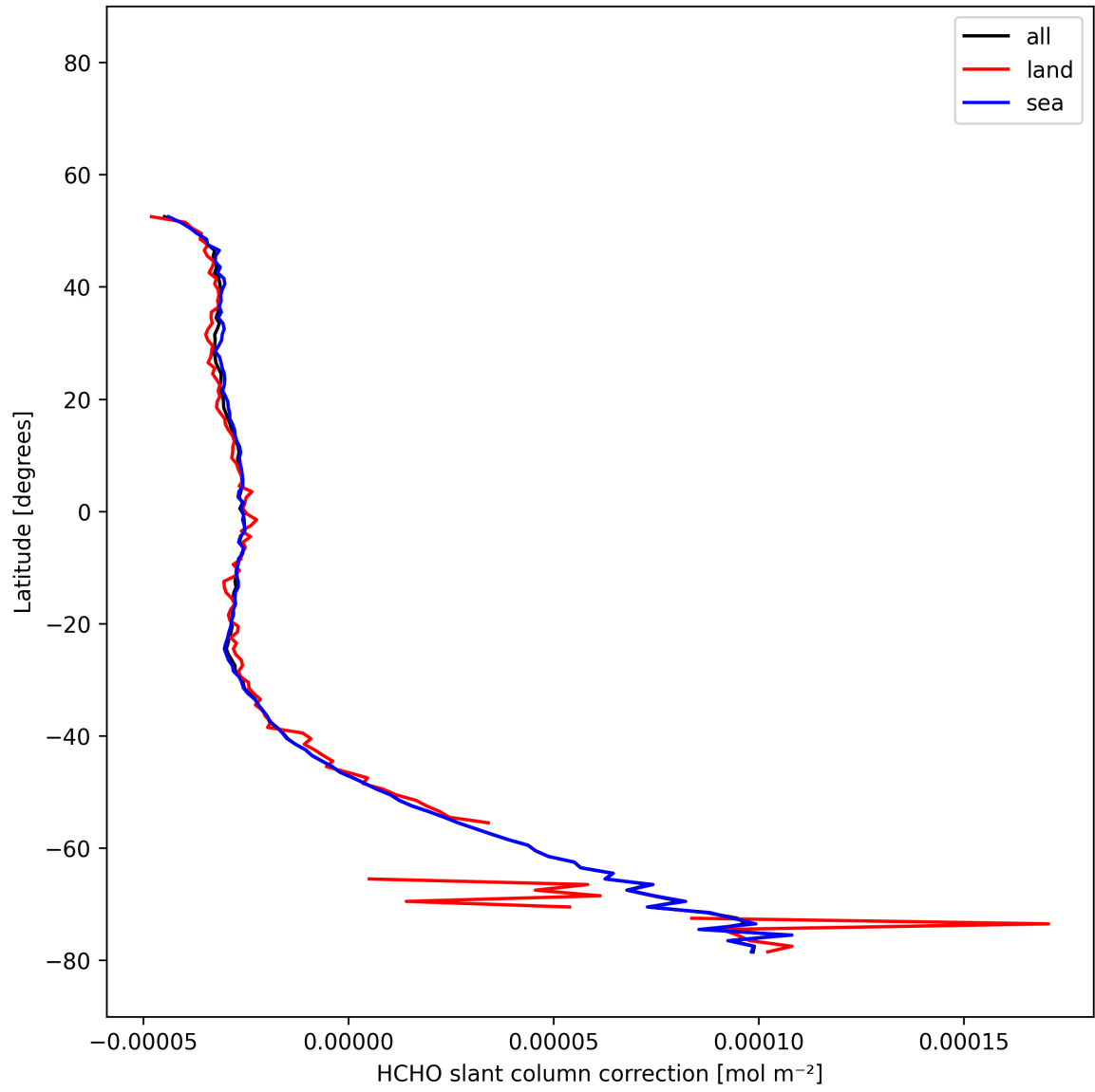
Figure 32: Zonal average of “HCHO slant column correction” for 2025-12-04 to 2025-12-05.
