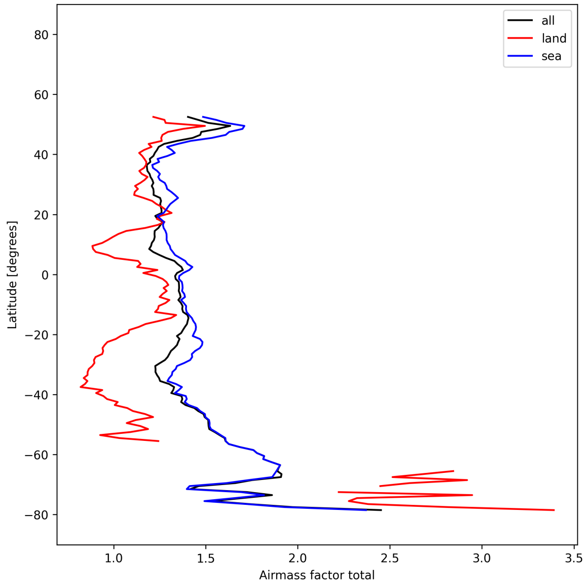
Figure 25: Zonal average of “Airmass factor total” for 2025-12-04 to 2025-12-05.
