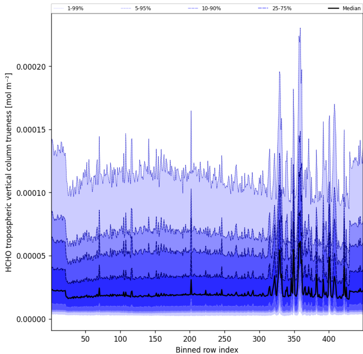
Figure 63: Along track statistics of “HCHO tropospheric vertical column trueness” for 2025-12-04 to 2025-12-05
