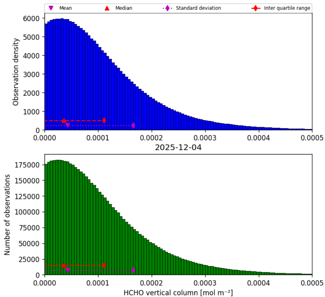
Figure 35: Histogram of “HCHO vertical column” for 2025-12-04 to 2025-12-05
