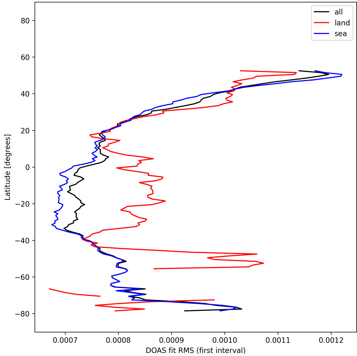
Figure 31: Zonal average of “DOAS fit RMS (first interval)” for 2025-12-05 to 2025-12-06.
