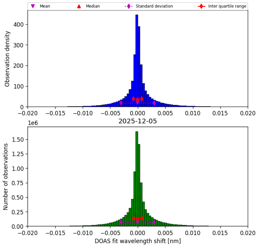
Figure 44: Histogram of “DOAS fit wavelength shift” for 2025-12-05 to 2025-12-06
