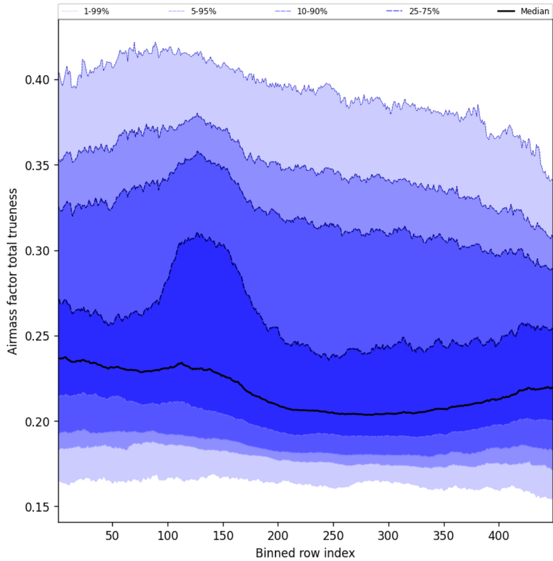
Figure 56: Along track statistics of “Airmass factor total trueness” for 2025-12-05 to 2025-12-06
