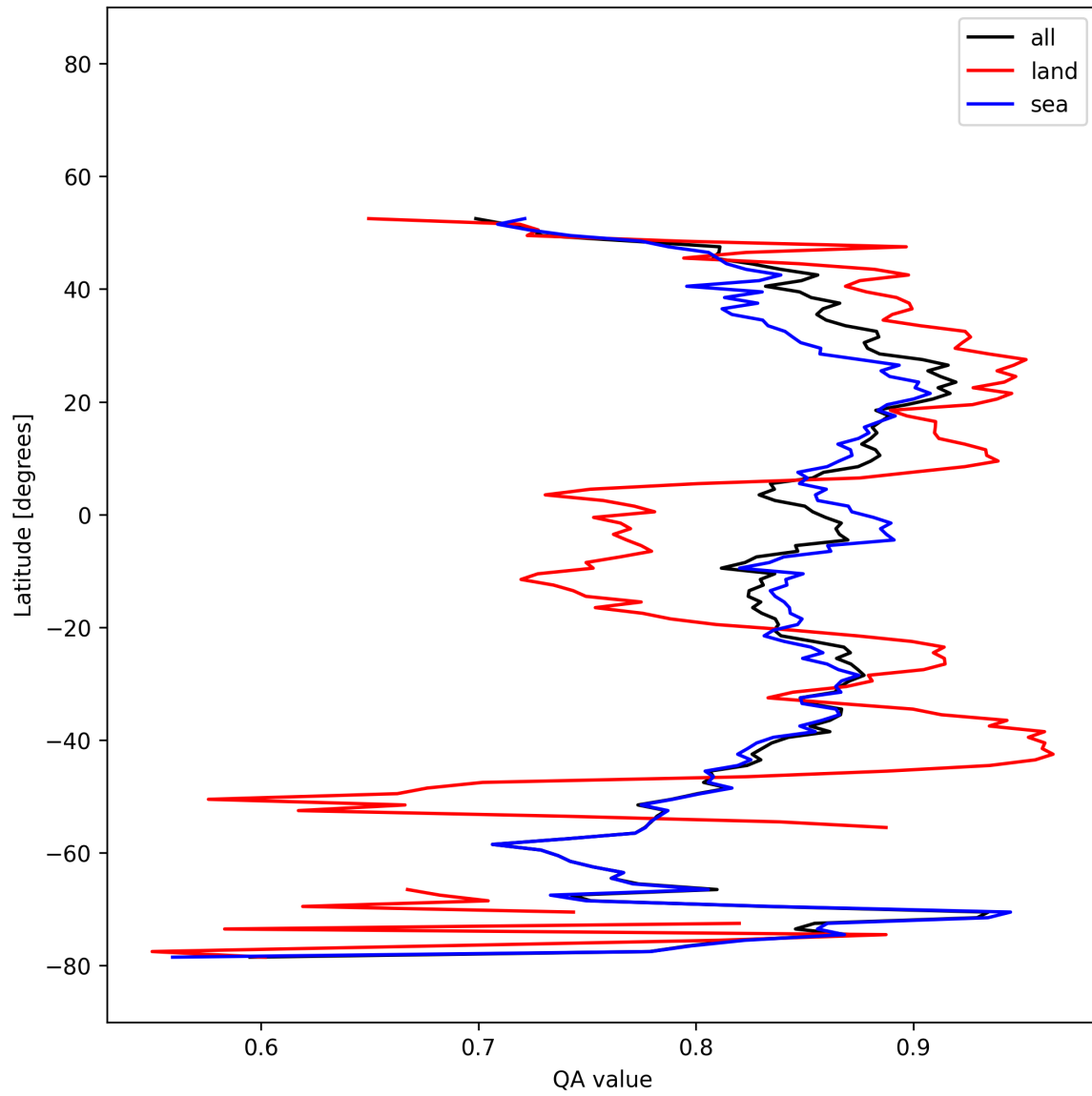
Figure 19: Zonal average of “QA value” for 2025-12-05 to 2025-12-06.
