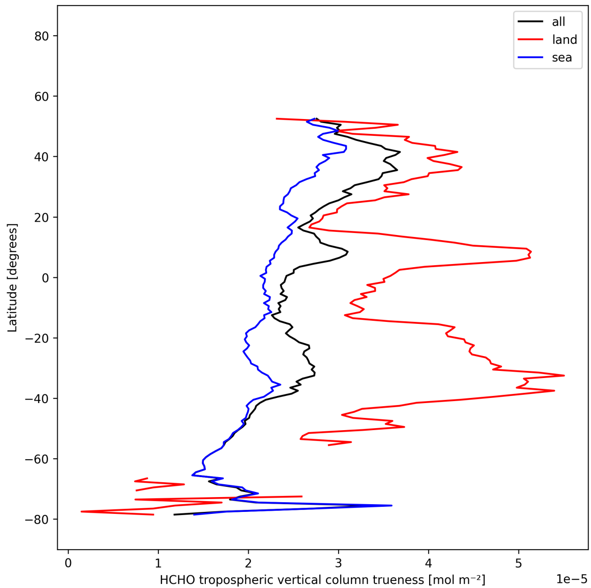
Figure 33: Zonal average of “HCHO tropospheric vertical column trueness” for 2025-12-05 to 2025-12-06.
