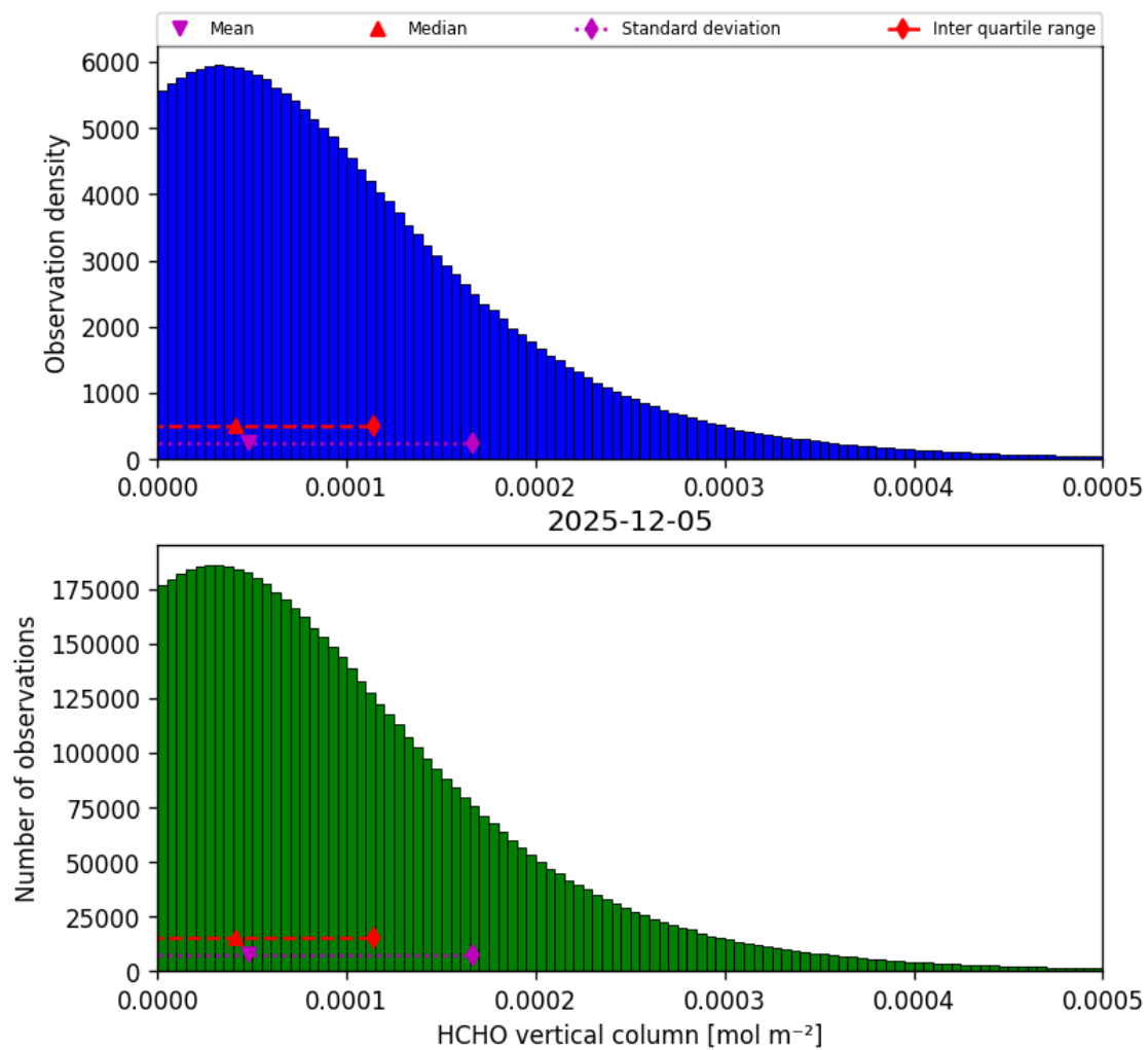
Figure 35: Histogram of “HCHO vertical column” for 2025-12-05 to 2025-12-06
