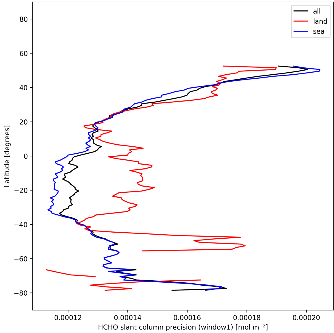
Figure 24: Zonal average of “HCHO slant column precision (window1)” for 2025-12-05 to 2025-12-06.
