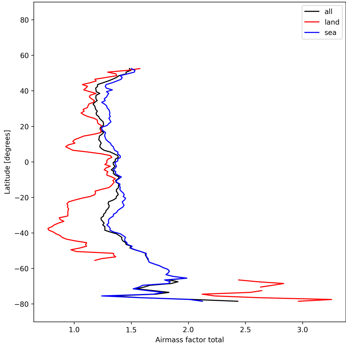
Figure 25: Zonal average of “Airmass factor total” for 2025-12-05 to 2025-12-06.
