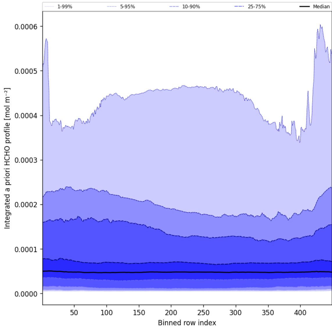
Figure 58: Along track statistics of "Integrated a priori HCHO profile" for 2025-12-05 to 2025-12-06
