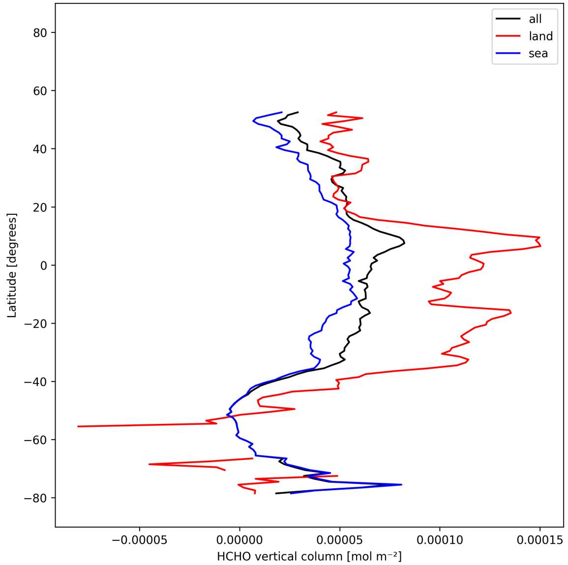
Figure 20: Zonal average of “HCHO vertical column” for 2025-12-05 to 2025-12-06.
