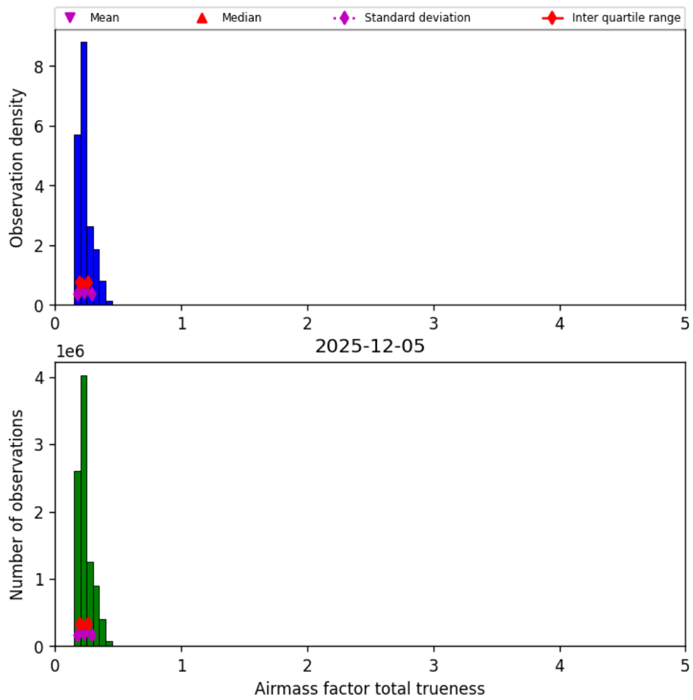
Figure 41: Histogram of “Airmass factor total trueness” for 2025-12-05 to 2025-12-06
