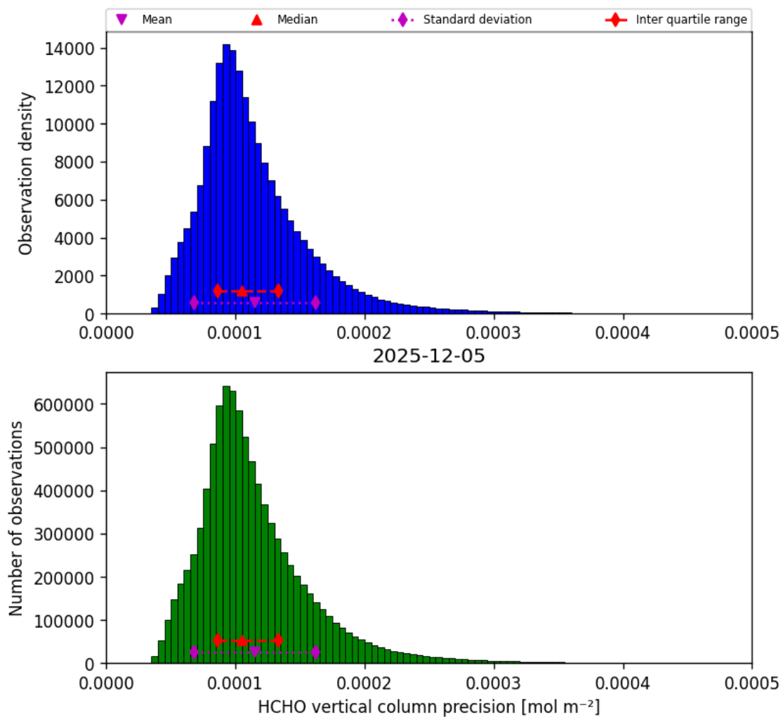
Figure 36: Histogram of “HCHO vertical column precision” for 2025-12-05 to 2025-12-06
