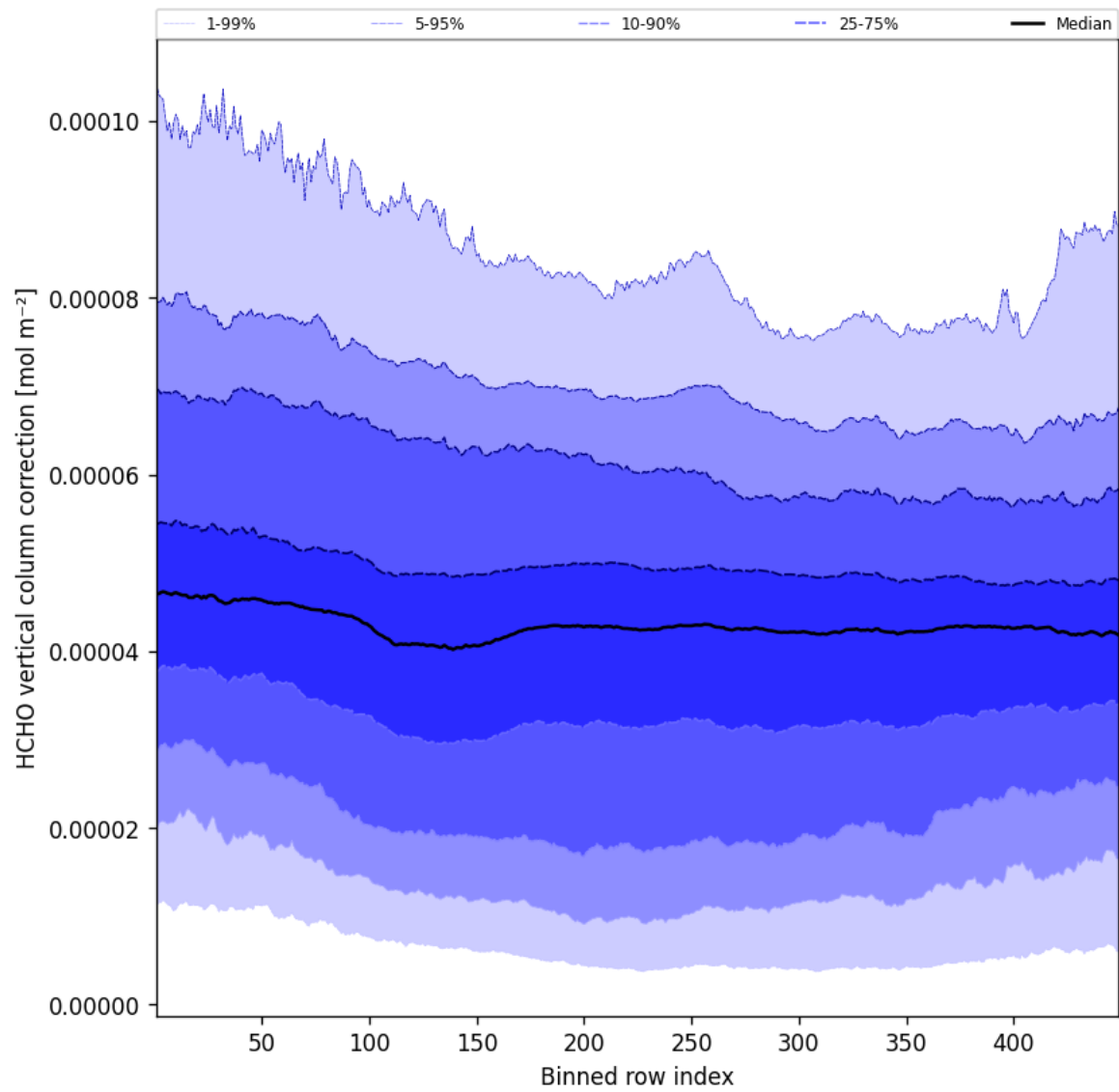
Figure 52: Along track statistics of "HCHO vertical column correction" for 2025-12-05 to 2025-12-06
