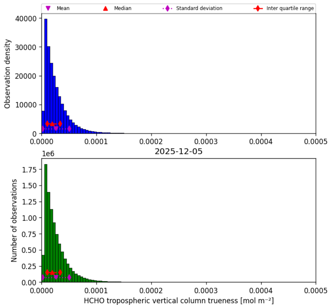
Figure 48: Histogram of “HCHO tropospheric vertical column trueness” for 2025-12-05 to 2025-12-06
