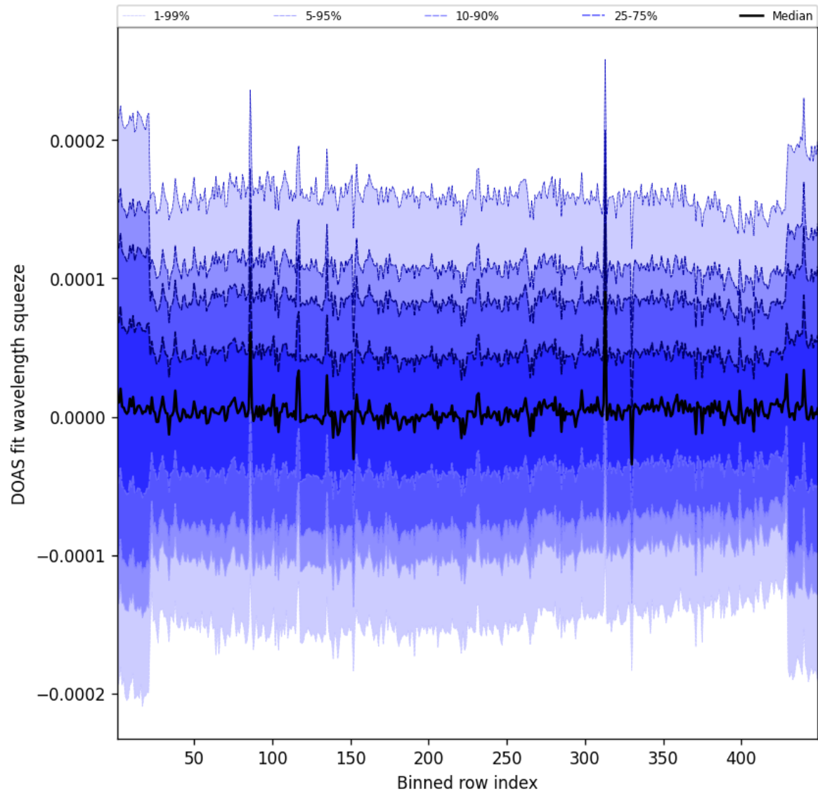
Figure 60: Along track statistics of “DOAS fit wavelength squeeze” for 2025-12-05 to 2025-12-06
