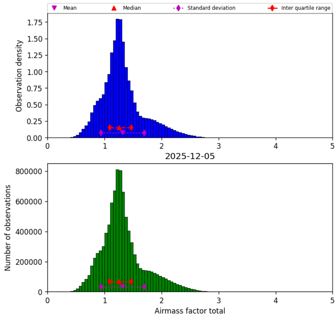
Figure 40: Histogram of “Airmass factor total” for 2025-12-05 to 2025-12-06
