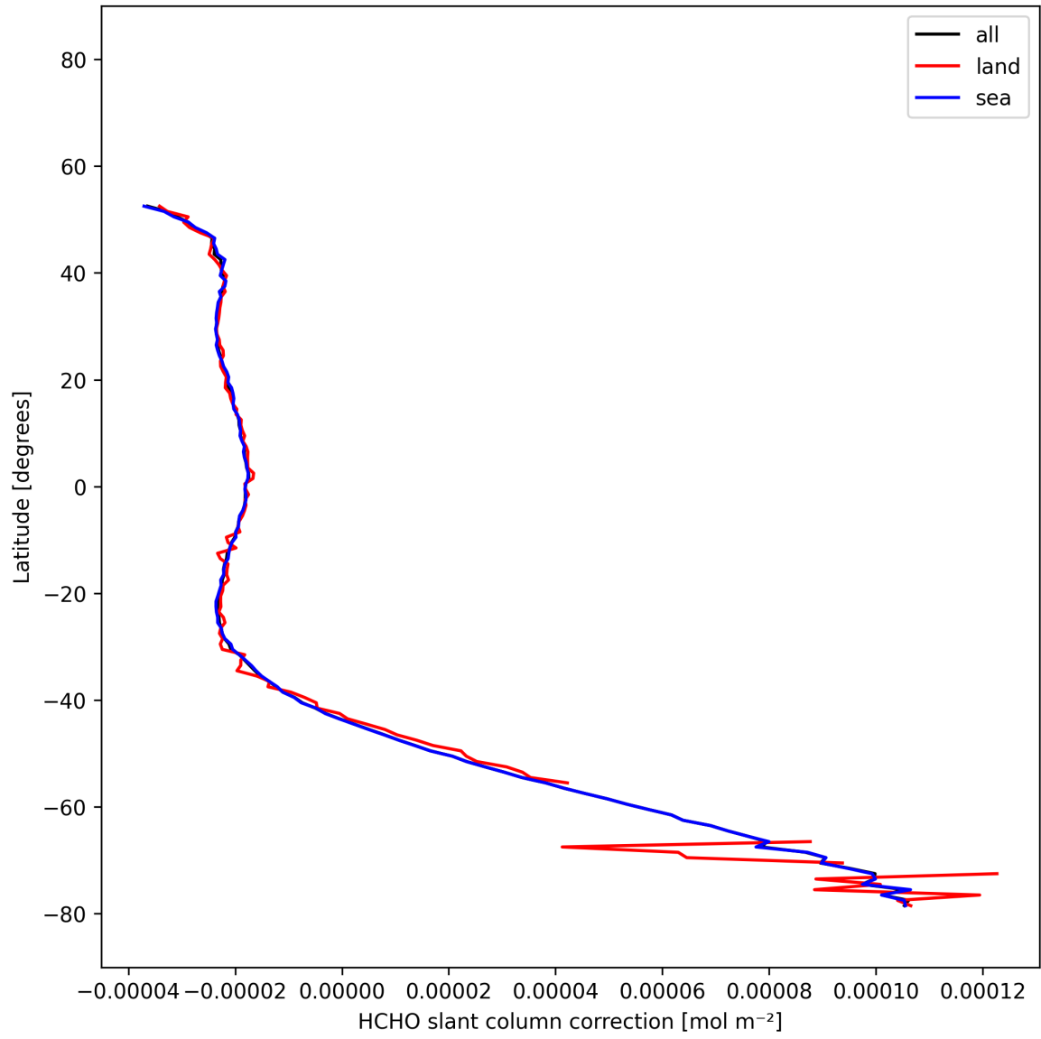
Figure 32: Zonal average of “HCHO slant column correction” for 2025-12-05 to 2025-12-06.
