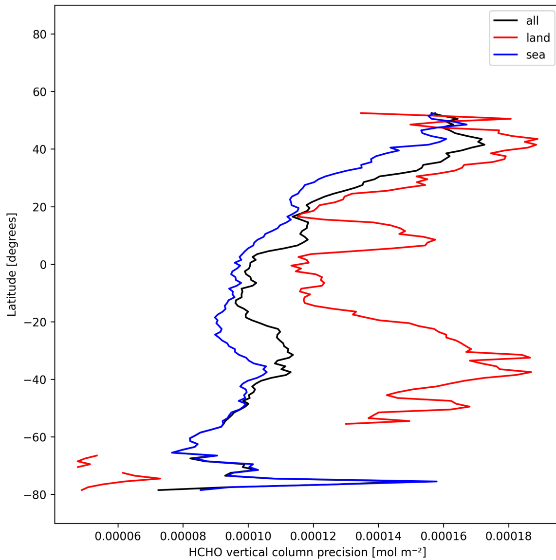
Figure 21: Zonal average of “HCHO vertical column precision” for 2025-12-05 to 2025-12-06.
