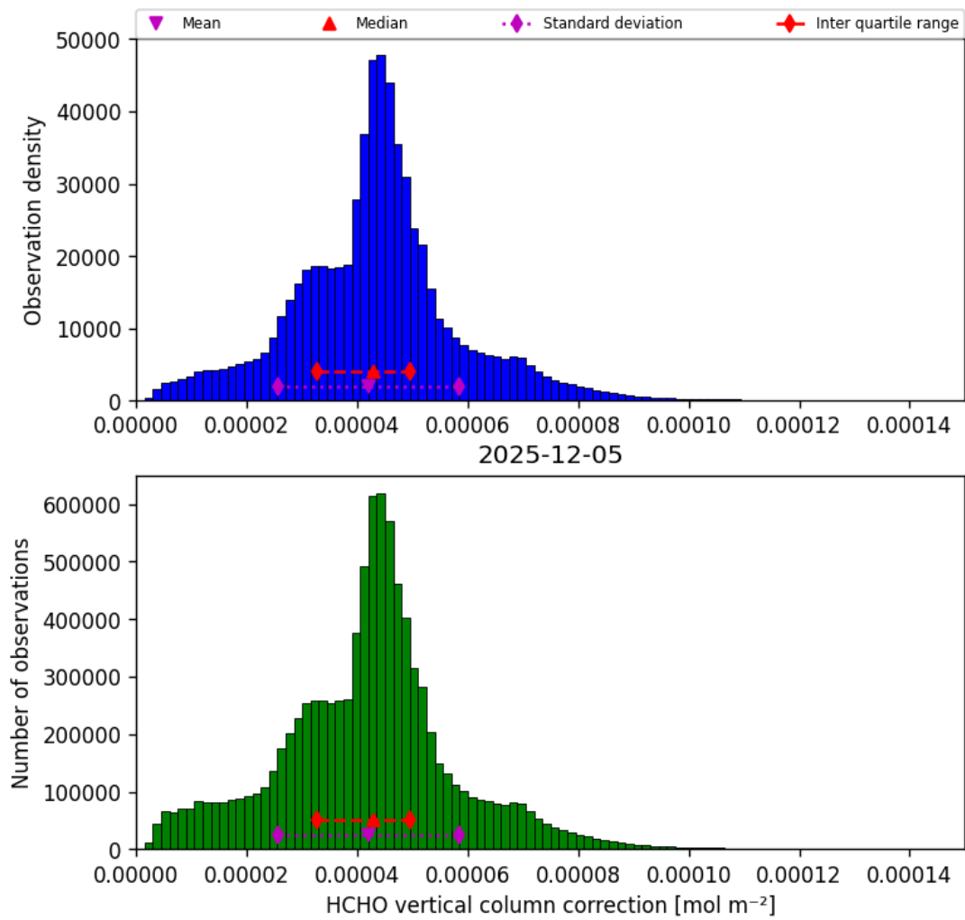
Figure 37: Histogram of “HCHO vertical column correction” for 2025-12-05 to 2025-12-06
