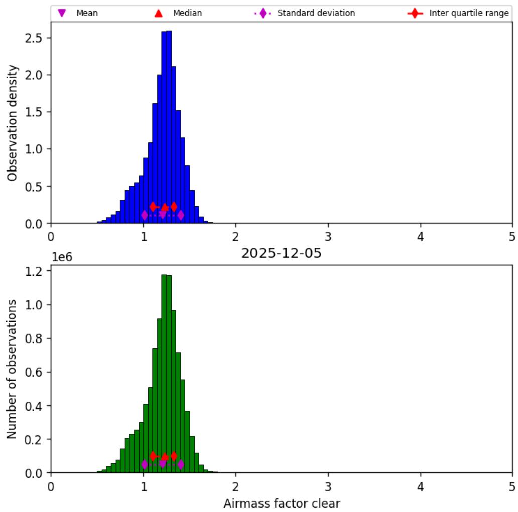
Figure 42: Histogram of “Airmass factor clear” for 2025-12-05 to 2025-12-06
