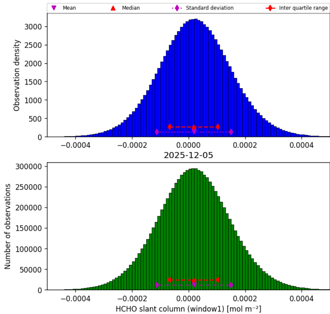
Figure 38: Histogram of “HCHO slant column (window1)” for 2025-12-05 to 2025-12-06
