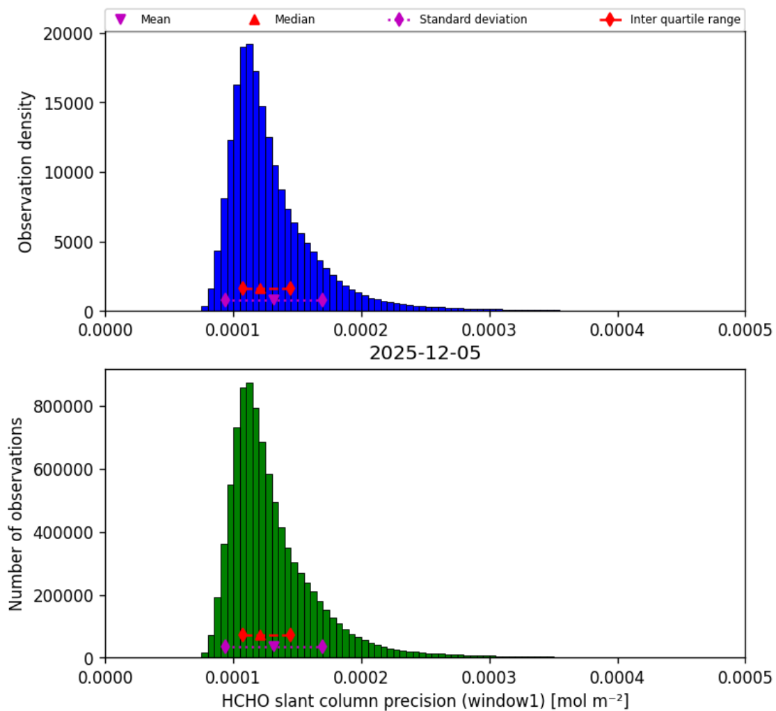
Figure 39: Histogram of "HCHO slant column precision (window1)" for 2025-12-05 to 2025-12-06
