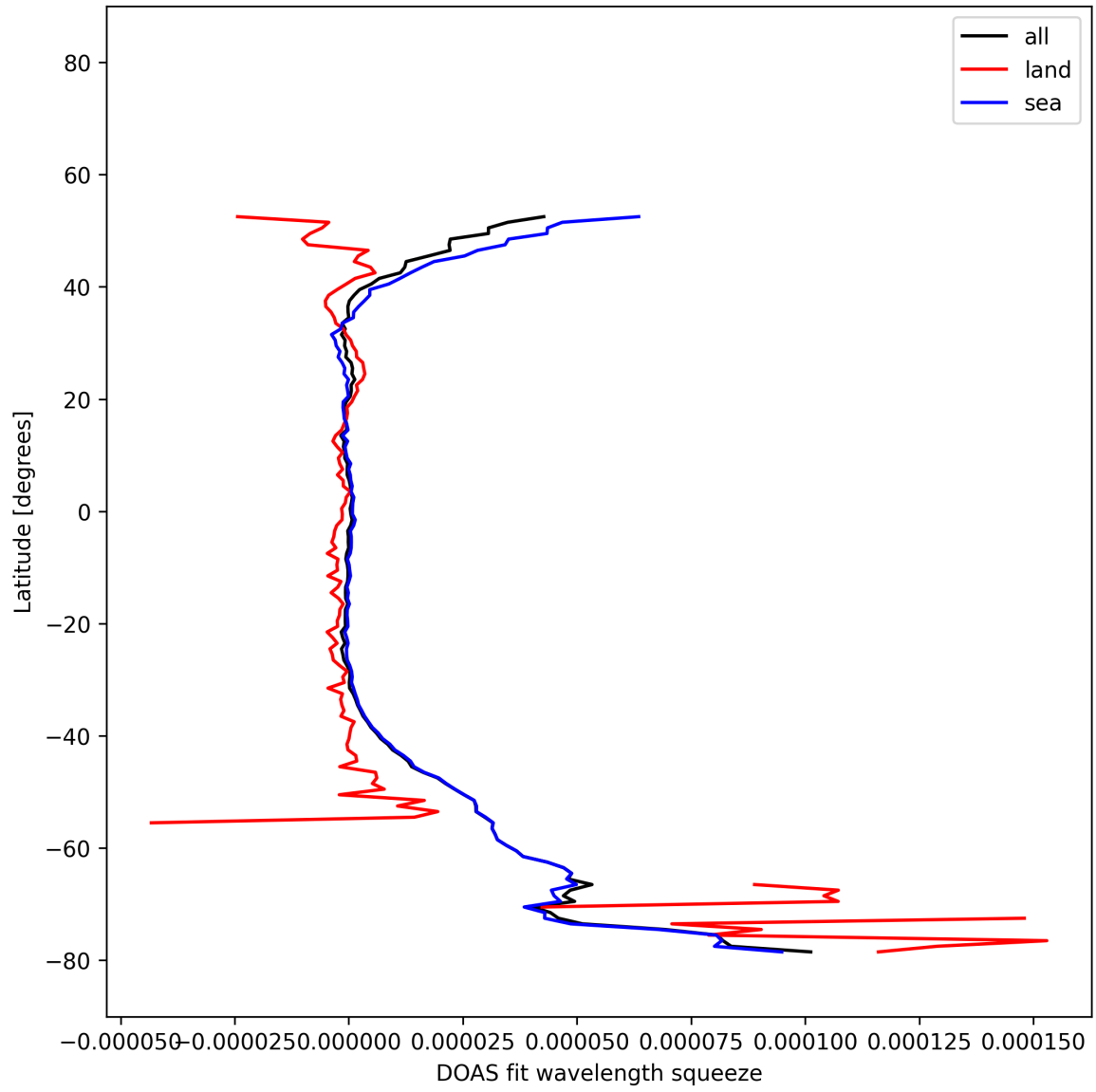
Figure 30: Zonal average of “DOAS fit wavelength squeeze” for 2025-12-05 to 2025-12-06.
