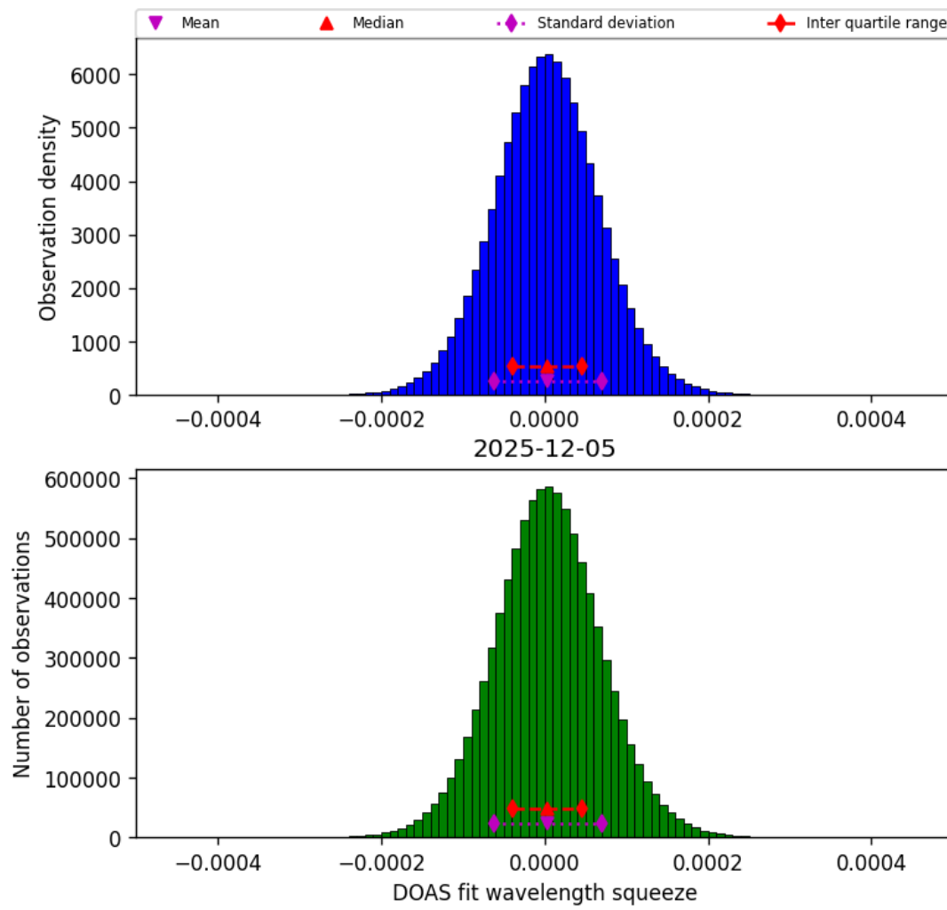
Figure 45: Histogram of “DOAS fit wavelength squeeze” for 2025-12-05 to 2025-12-06
