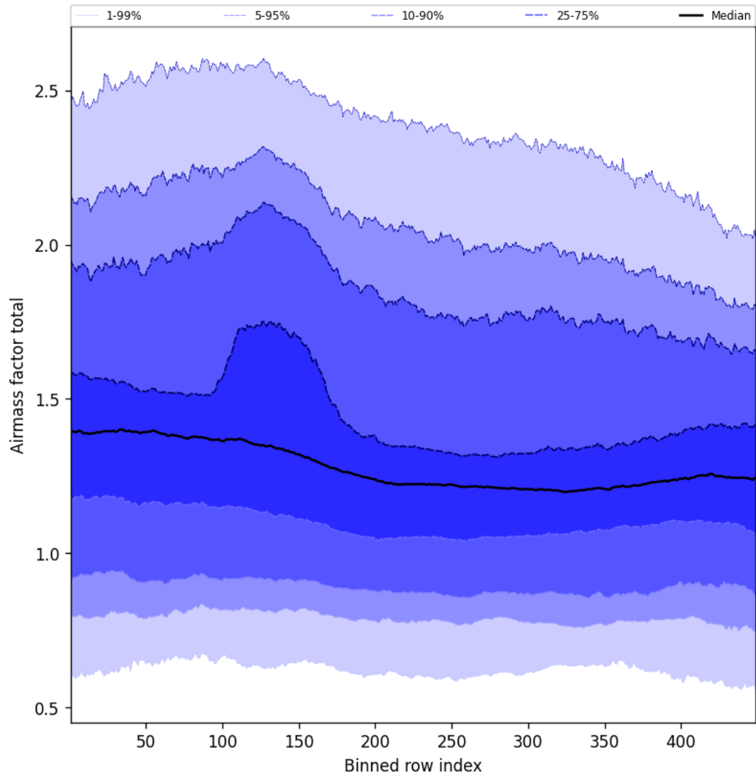
Figure 55: Along track statistics of “Airmass factor total” for 2025-12-05 to 2025-12-06
