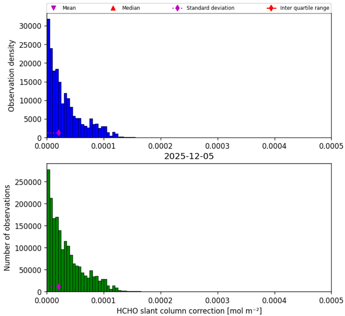
Figure 47: Histogram of “HCHO slant column correction” for 2025-12-05 to 2025-12-06
