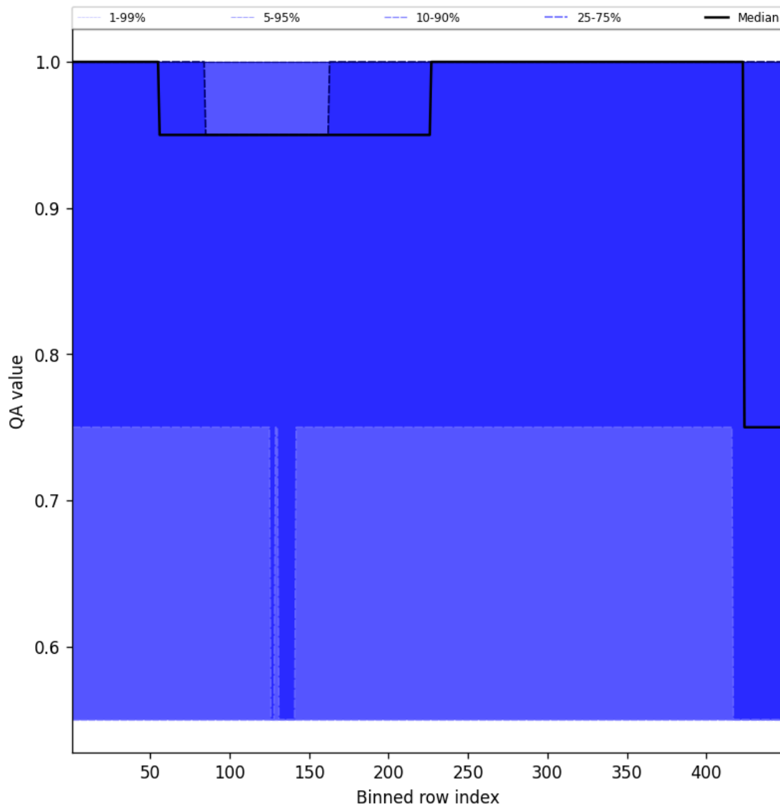
Figure 49: Along track statistics of “QA value” for 2025-12-05 to 2025-12-06
