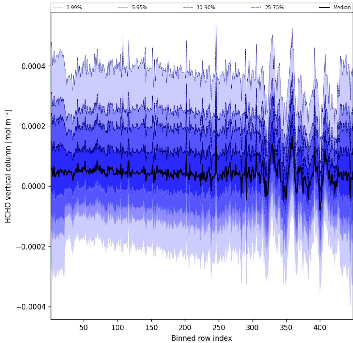
Figure 50: Along track statistics of “HCHO vertical column” for 2025-12-05 to 2025-12-06
