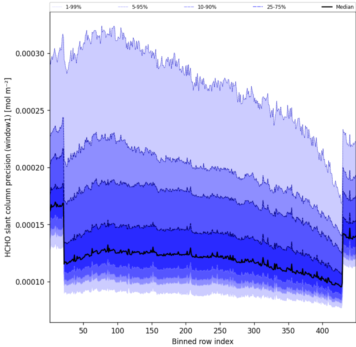
Figure 54: Along track statistics of “HCHO slant column precision (window1)” for 2025-12-05 to 2025-12-06
