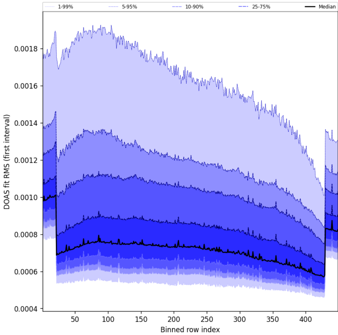
Figure 61: Along track statistics of “DOAS fit RMS (first interval)” for 2025-12-05 to 2025-12-06
