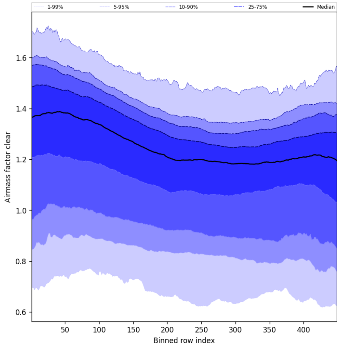
Figure 57: Along track statistics of “Airmass factor clear” for 2025-12-05 to 2025-12-06
