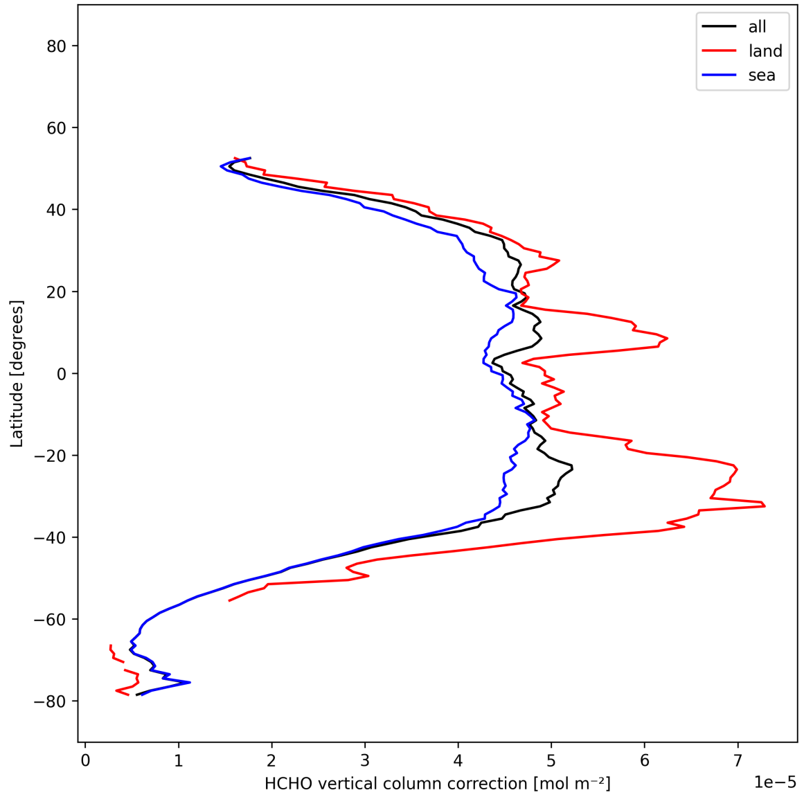
Figure 22: Zonal average of "HCHO vertical column correction" for 2025-12-05 to 2025-12-06.
