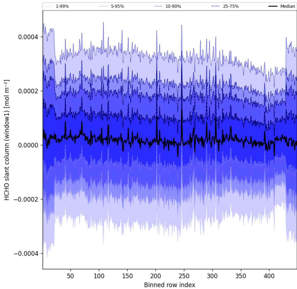
Figure 53: Along track statistics of “HCHO slant column (window1)” for 2025-12-05 to 2025-12-06
