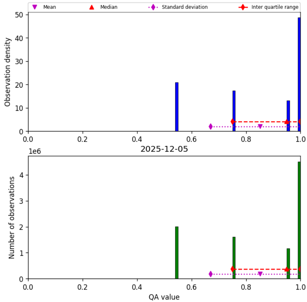
Figure 34: Histogram of “QA value” for 2025-12-05 to 2025-12-06
