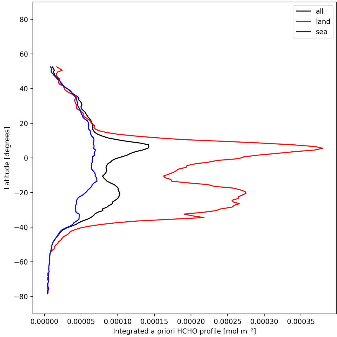
Figure 28: Zonal average of “Integrated a priori HCHO profile” for 2025-12-05 to 2025-12-06.
