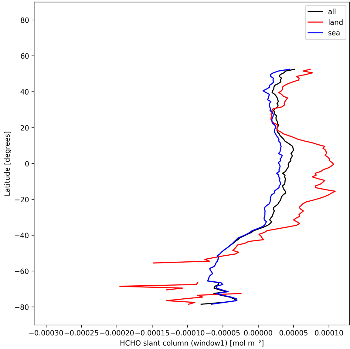
Figure 23: Zonal average of “HCHO slant column (window1)” for 2025-12-05 to 2025-12-06.
