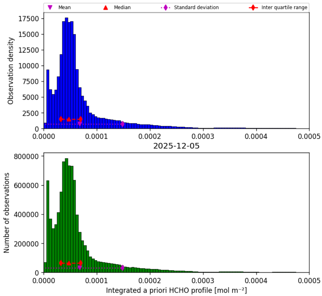
Figure 43: Histogram of “Integrated a priori HCHO profile” for 2025-12-05 to 2025-12-06
