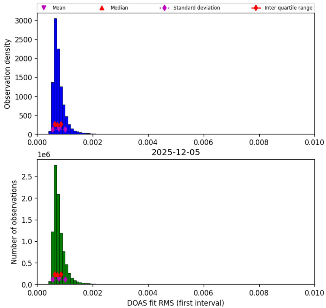
Figure 46: Histogram of “DOAS fit RMS (first interval)” for 2025-12-05 to 2025-12-06
