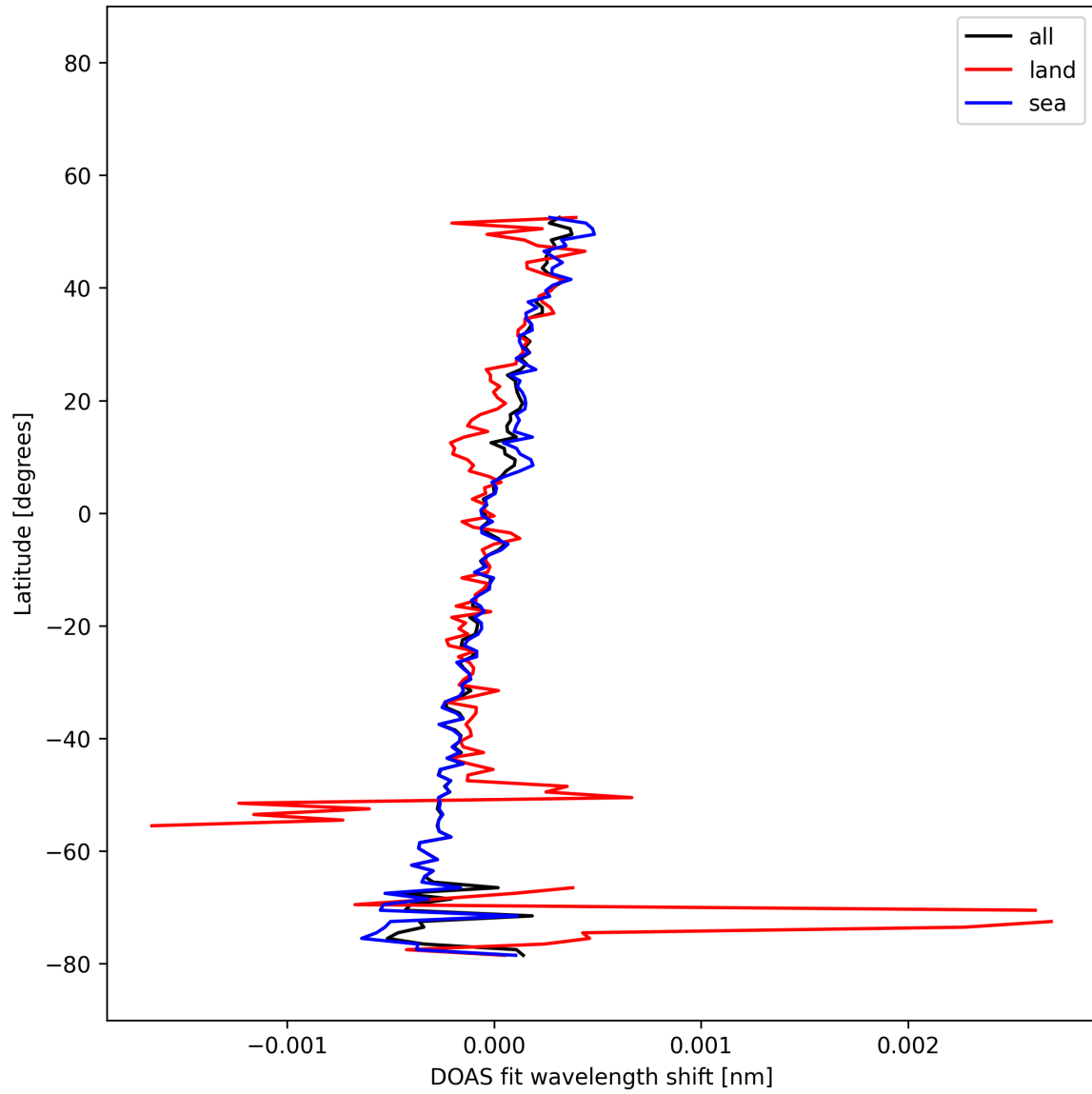
Figure 29: Zonal average of “DOAS fit wavelength shift” for 2025-12-05 to 2025-12-06.
