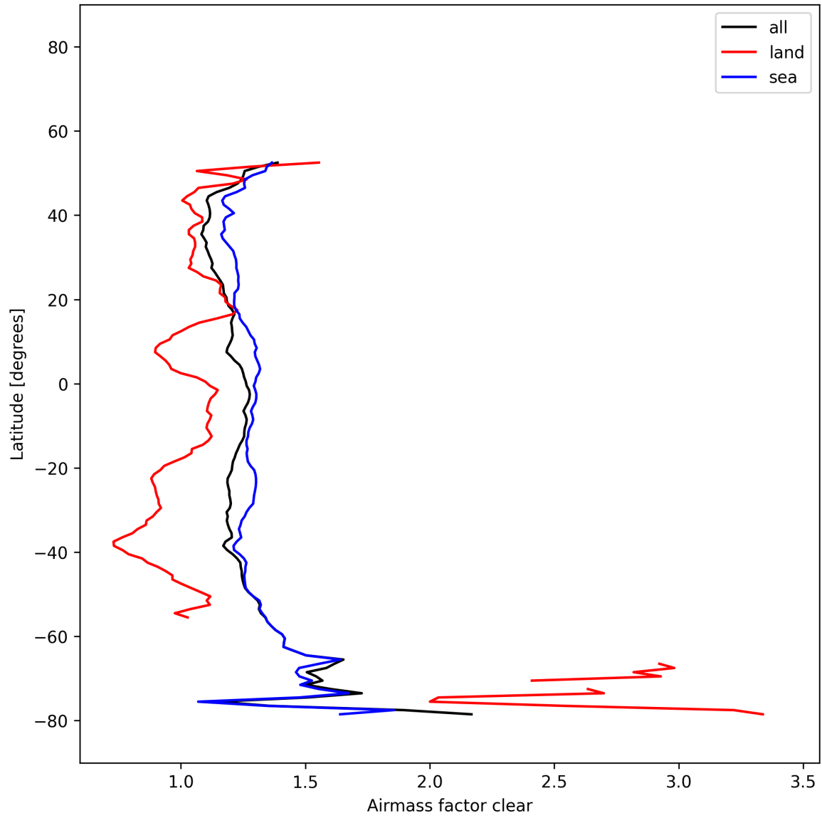
Figure 27: Zonal average of “Airmass factor clear” for 2025-12-05 to 2025-12-06.
