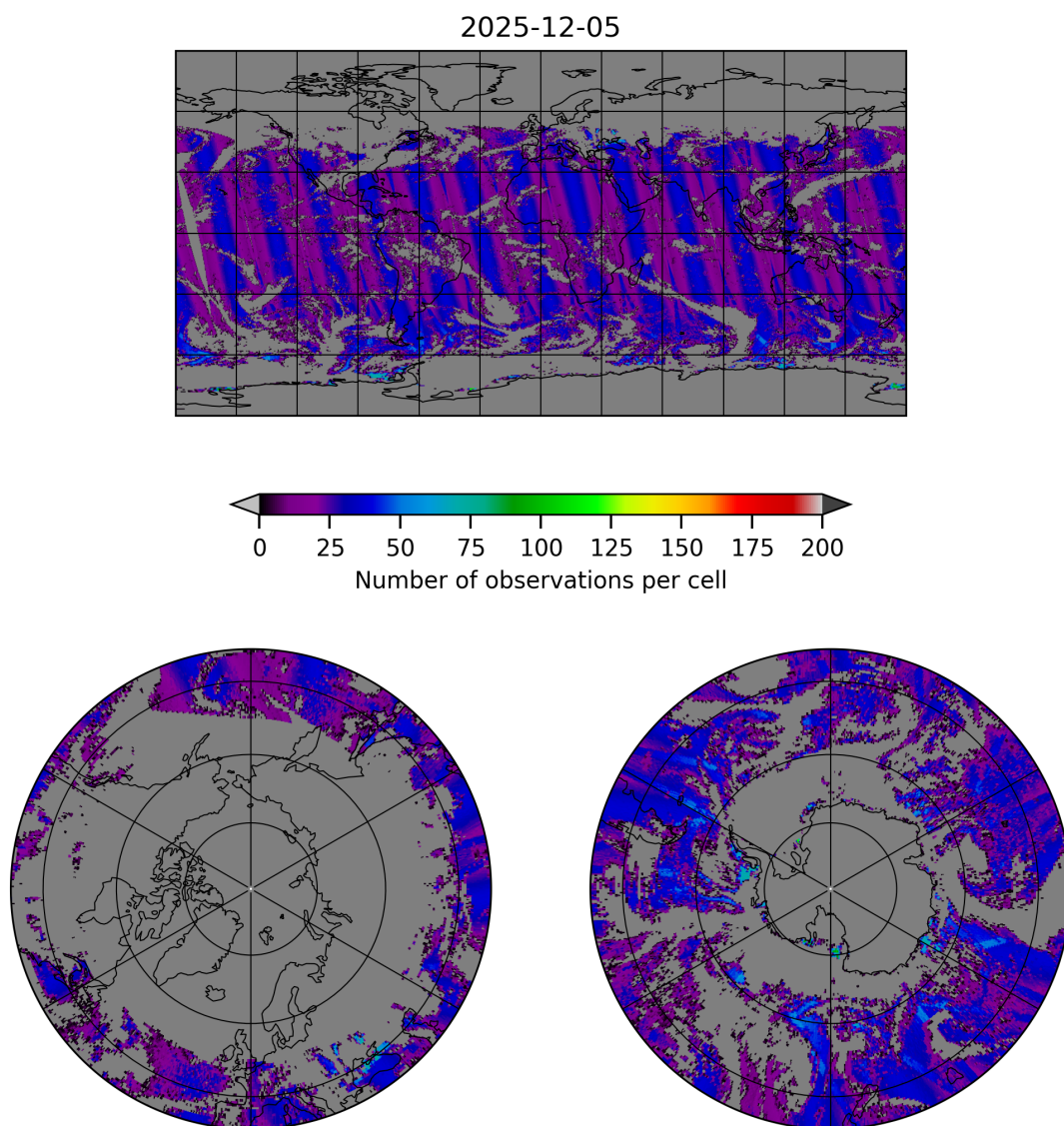
Figure 18: Map of the number of observations for 2025-12-05 to 2025-12-06
