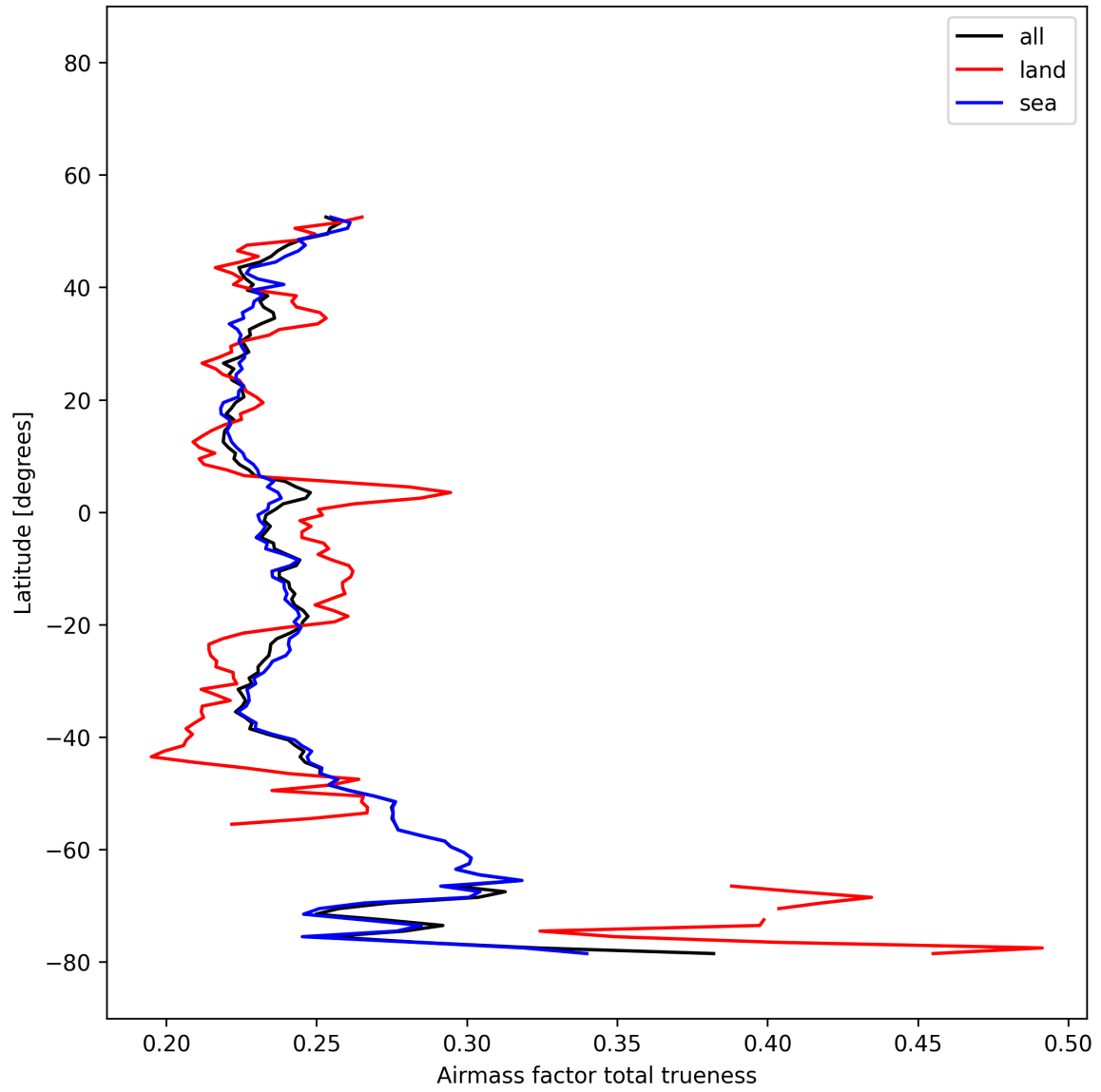
Figure 26: Zonal average of “Airmass factor total trueness” for 2025-12-05 to 2025-12-06.
