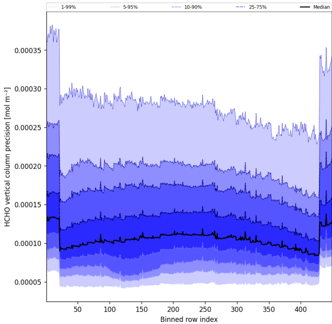
Figure 51: Along track statistics of “HCHO vertical column precision” for 2025-12-05 to 2025-12-06
