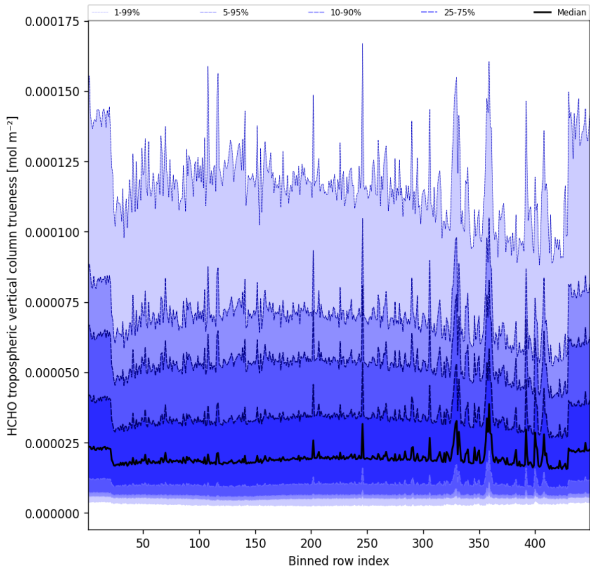
Figure 63: Along track statistics of “HCHO tropospheric vertical column trueness” for 2025-12-05 to 2025-12-06
