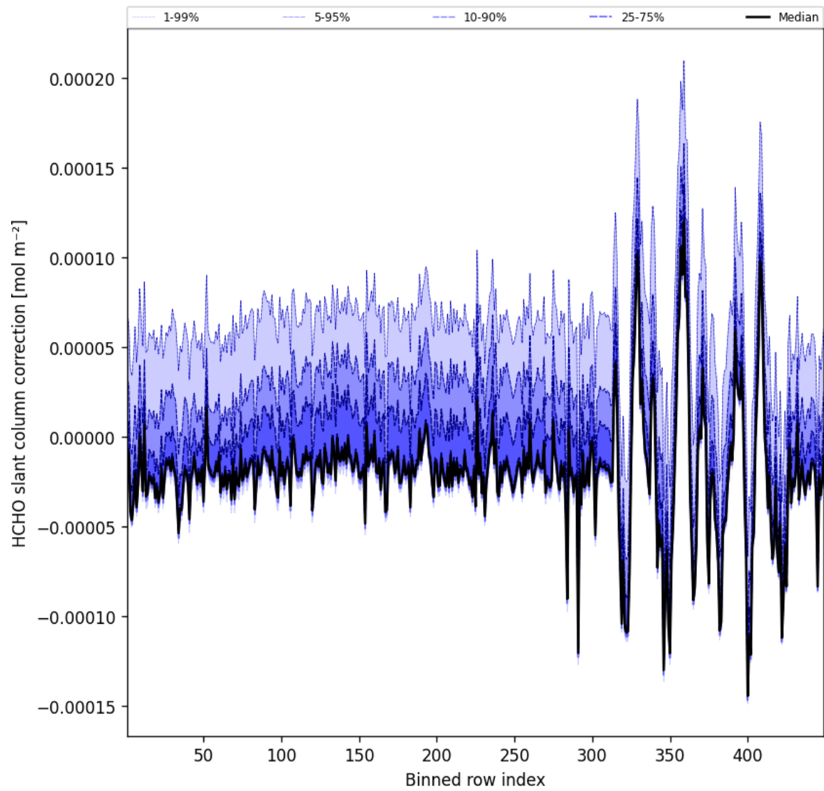
Figure 62: Along track statistics of “HCHO slant column correction” for 2025-12-05 to 2025-12-06
