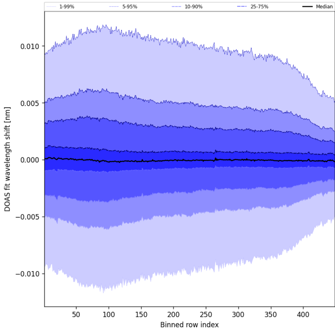
Figure 59: Along track statistics of “DOAS fit wavelength shift” for 2025-12-05 to 2025-12-06
