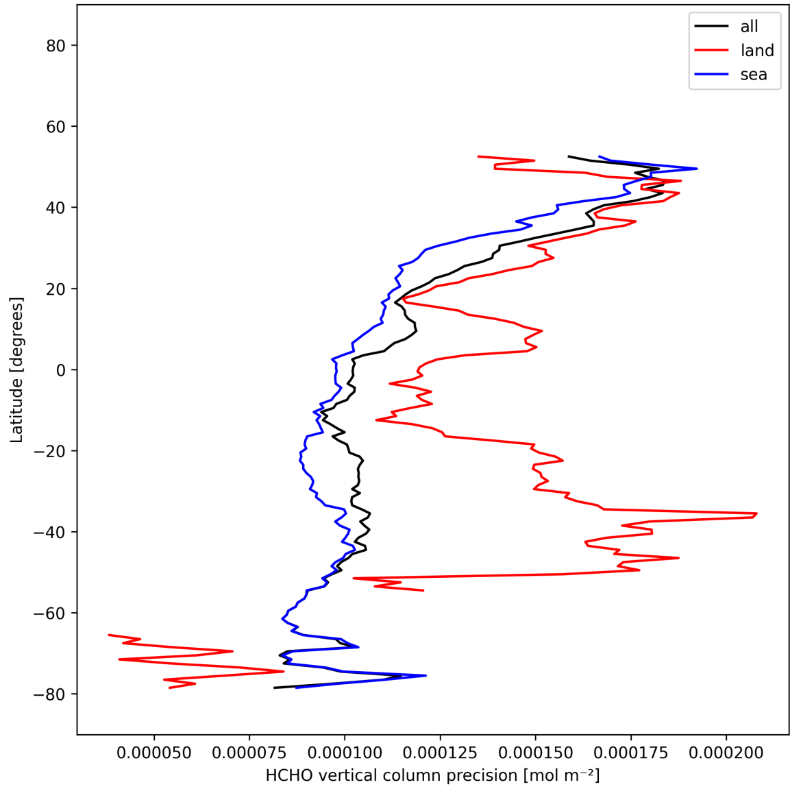
Figure 21: Zonal average of “HCHO vertical column precision” for 2025-12-06 to 2025-12-07.
