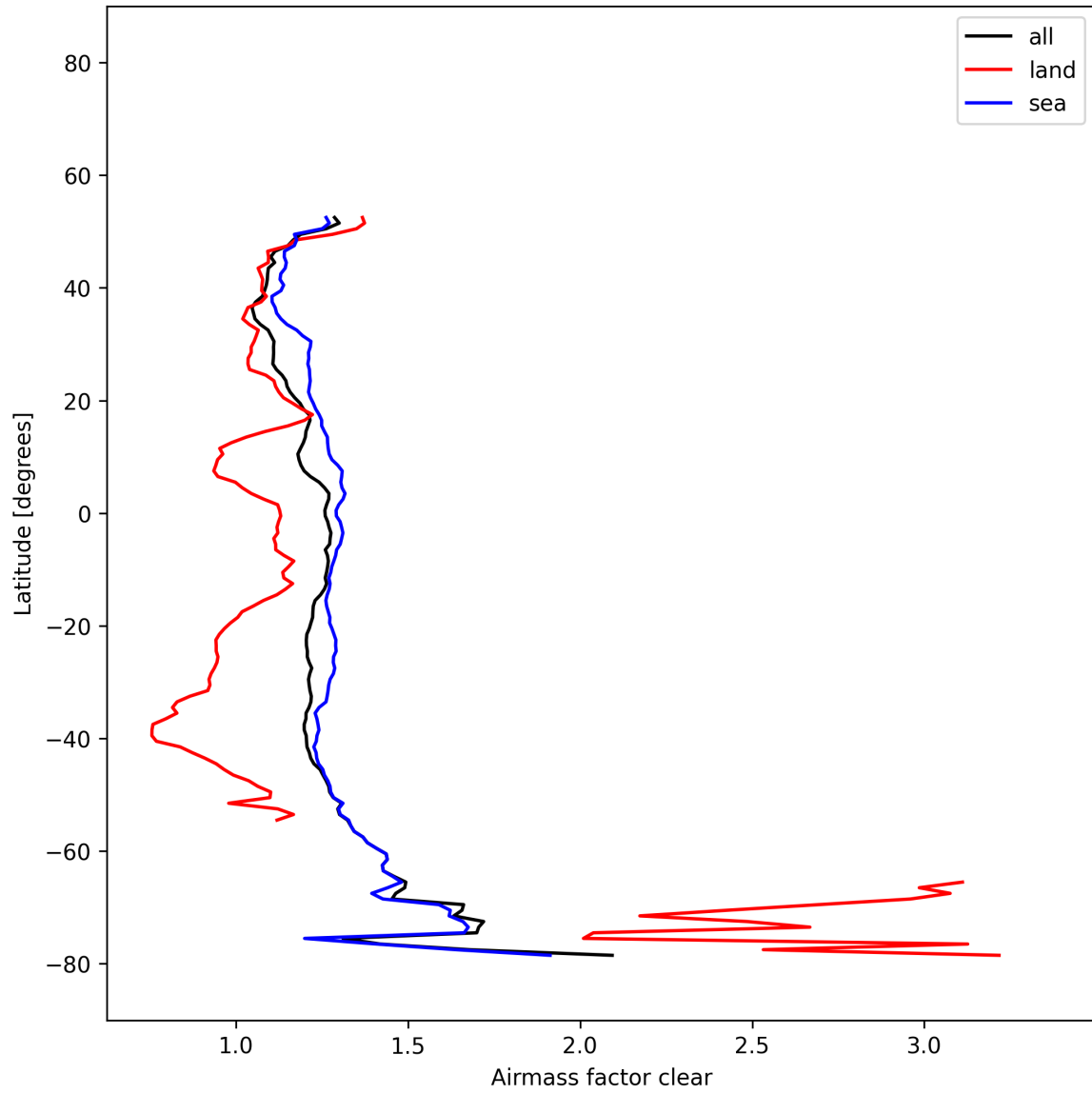
Figure 27: Zonal average of “Airmass factor clear” for 2025-12-06 to 2025-12-07.
