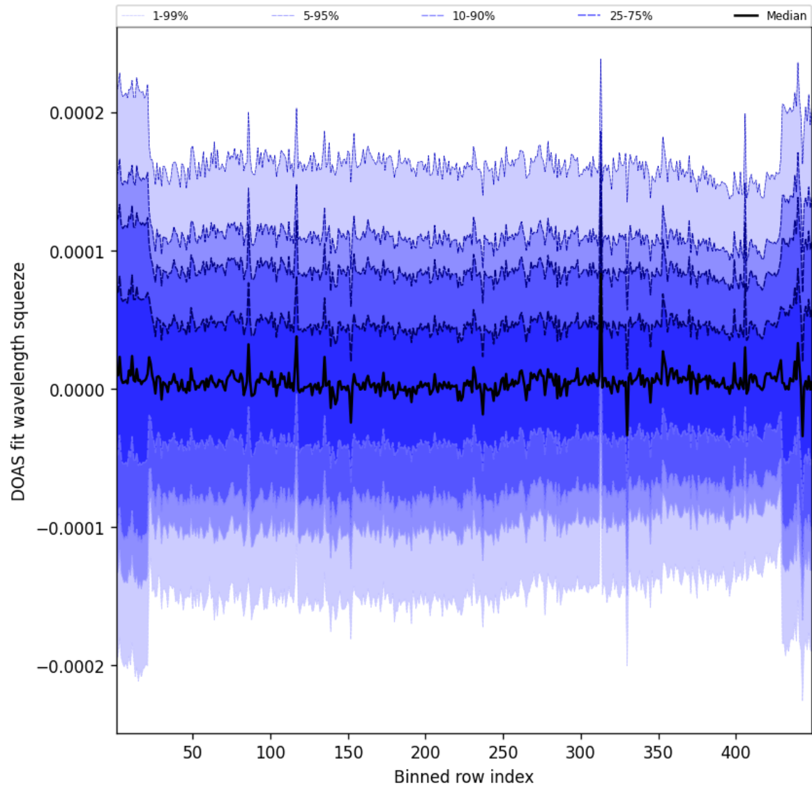
Figure 60: Along track statistics of “DOAS fit wavelength squeeze” for 2025-12-06 to 2025-12-07
