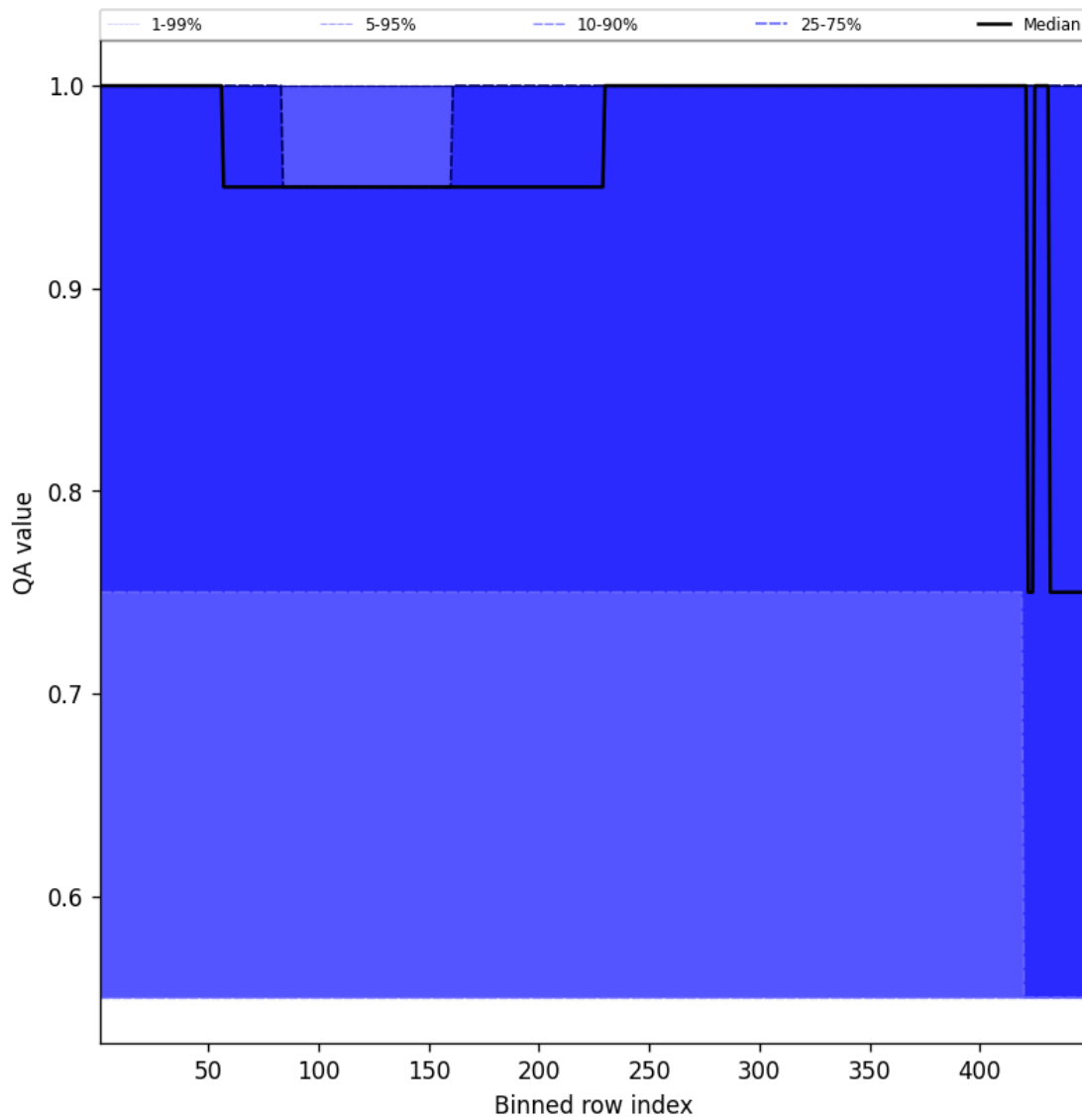
Figure 49: Along track statistics of “QA value” for 2025-12-06 to 2025-12-07
