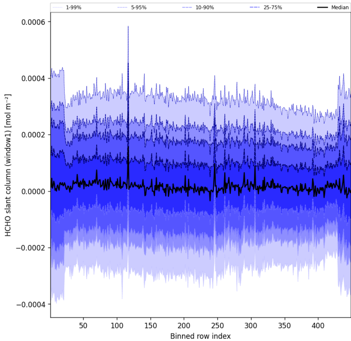
Figure 53: Along track statistics of “HCHO slant column (window1)” for 2025-12-06 to 2025-12-07
