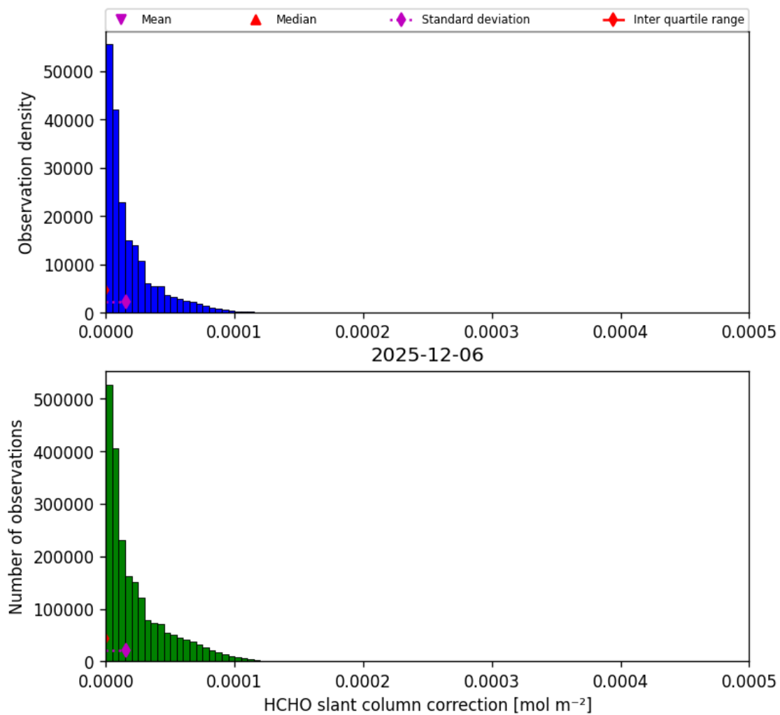
Figure 47: Histogram of “HCHO slant column correction” for 2025-12-06 to 2025-12-07
