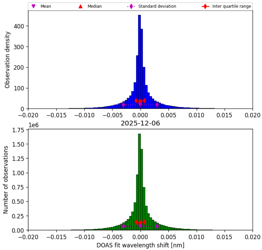
Figure 44: Histogram of “DOAS fit wavelength shift” for 2025-12-06 to 2025-12-07
