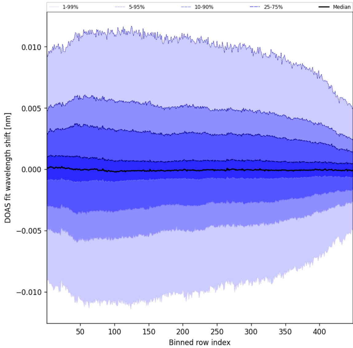
Figure 59: Along track statistics of “DOAS fit wavelength shift” for 2025-12-06 to 2025-12-07
