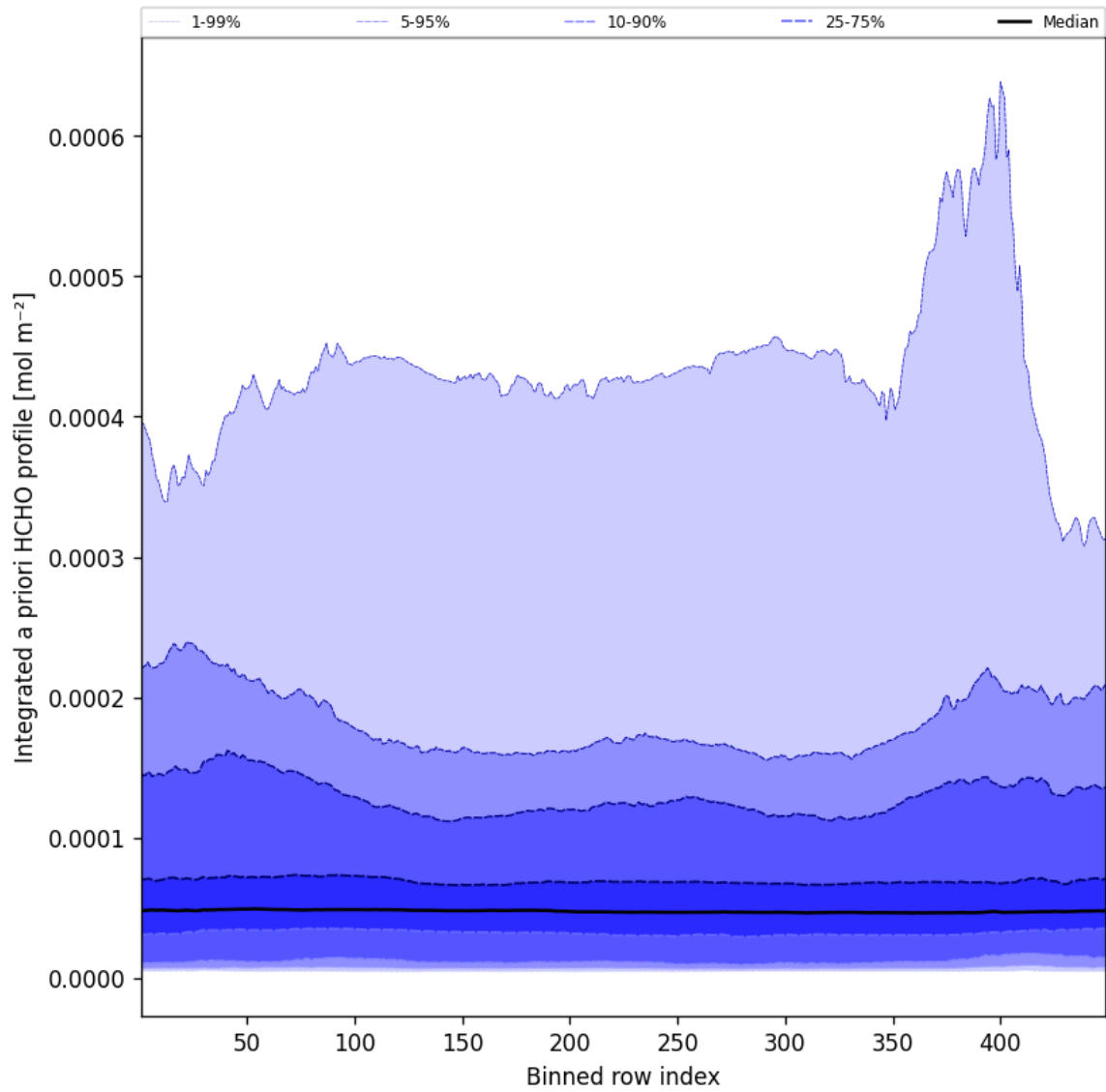
Figure 58: Along track statistics of “Integrated a priori HCHO profile” for 2025-12-06 to 2025-12-07
