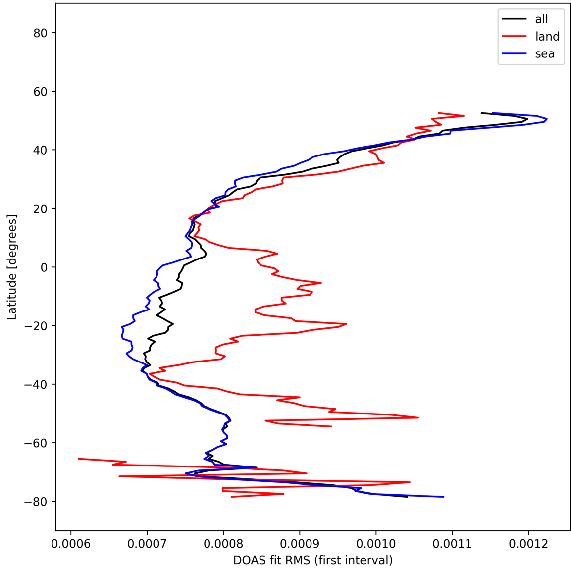
Figure 31: Zonal average of “DOAS fit RMS (first interval)” for 2025-12-06 to 2025-12-07.
