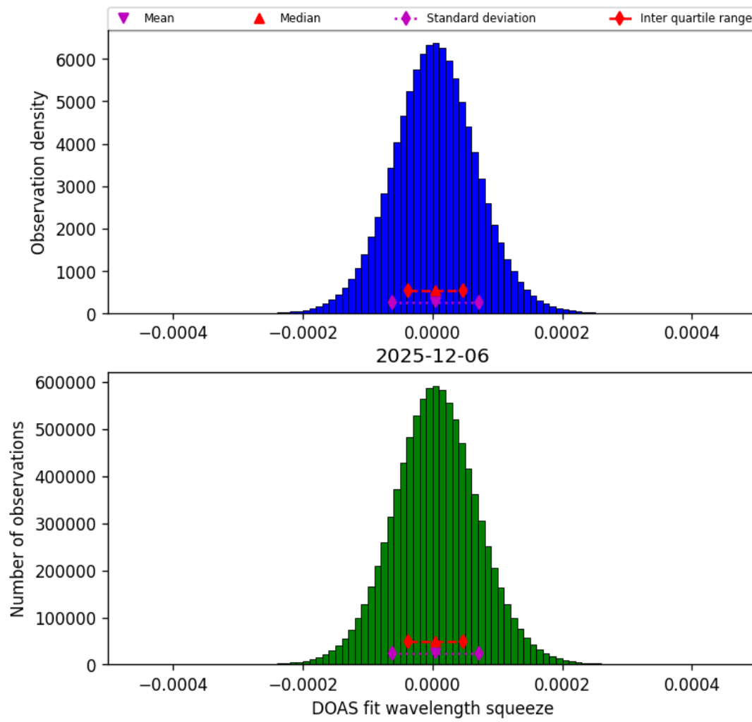
Figure 45: Histogram of “DOAS fit wavelength squeeze” for 2025-12-06 to 2025-12-07
