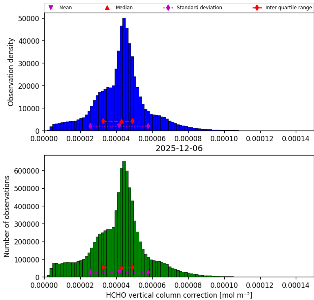
Figure 37: Histogram of “HCHO vertical column correction” for 2025-12-06 to 2025-12-07
