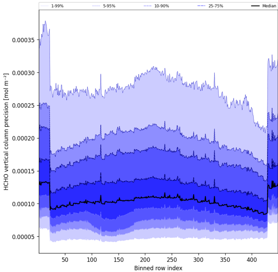
Figure 51: Along track statistics of “HCHO vertical column precision” for 2025-12-06 to 2025-12-07
