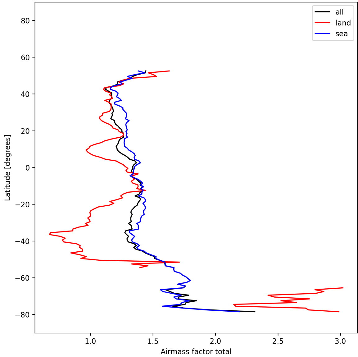
Figure 25: Zonal average of “Airmass factor total” for 2025-12-06 to 2025-12-07.
