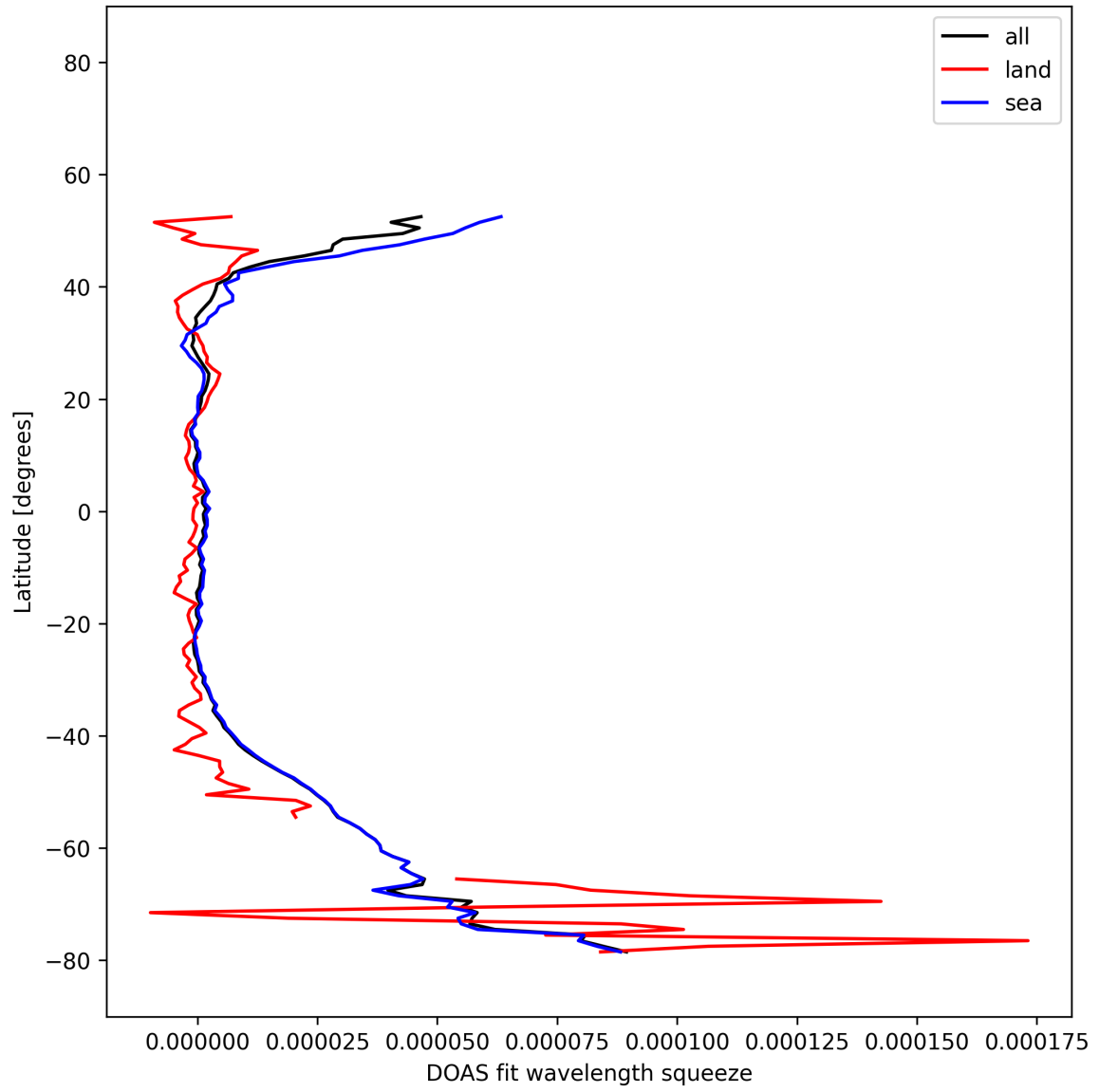
Figure 30: Zonal average of “DOAS fit wavelength squeeze” for 2025-12-06 to 2025-12-07.
