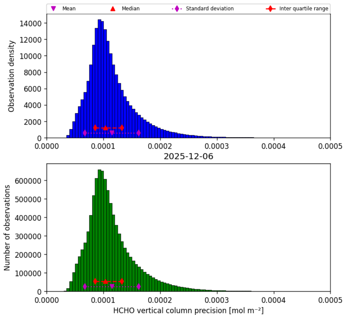
Figure 36: Histogram of “HCHO vertical column precision” for 2025-12-06 to 2025-12-07
