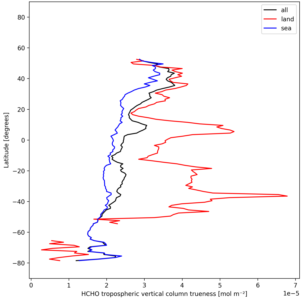
Figure 33: Zonal average of “HCHO tropospheric vertical column trueness” for 2025-12-06 to 2025-12-07.
