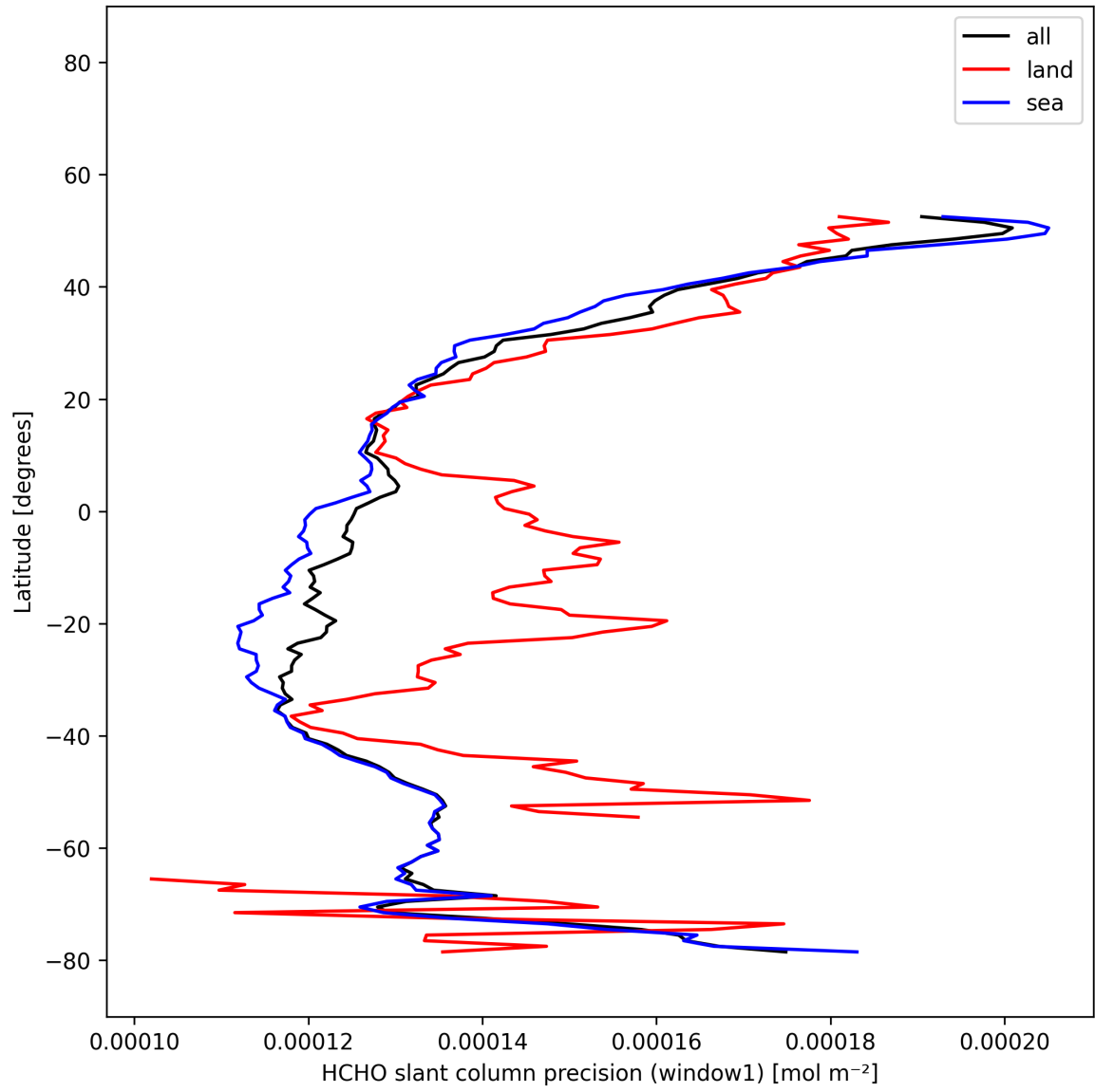
Figure 24: Zonal average of “HCHO slant column precision (window1)” for 2025-12-06 to 2025-12-07.
