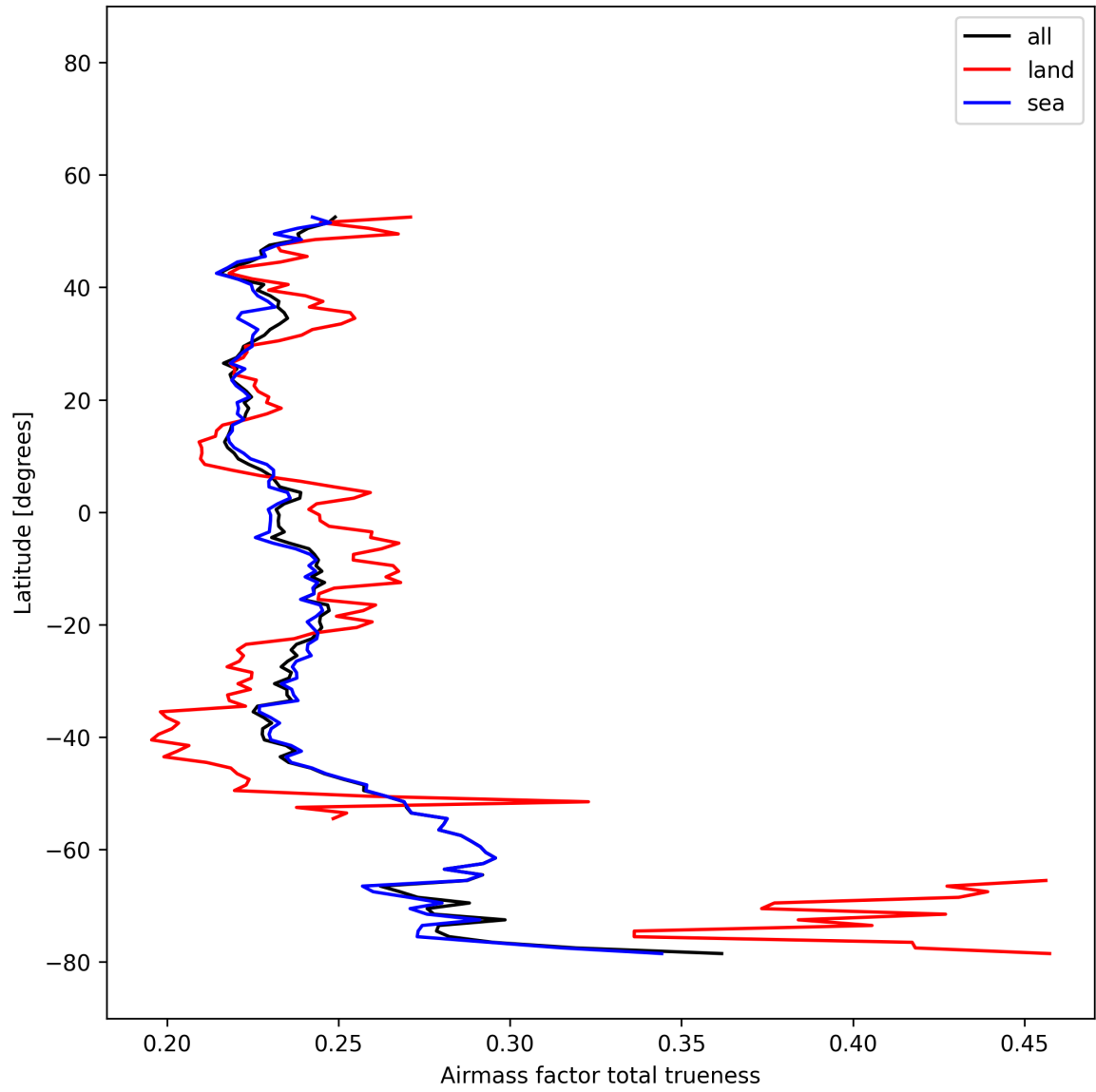
Figure 26: Zonal average of “Airmass factor total trueness” for 2025-12-06 to 2025-12-07.
