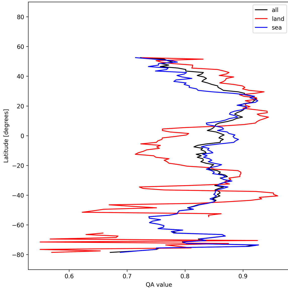
Figure 19: Zonal average of “QA value” for 2025-12-06 to 2025-12-07.
