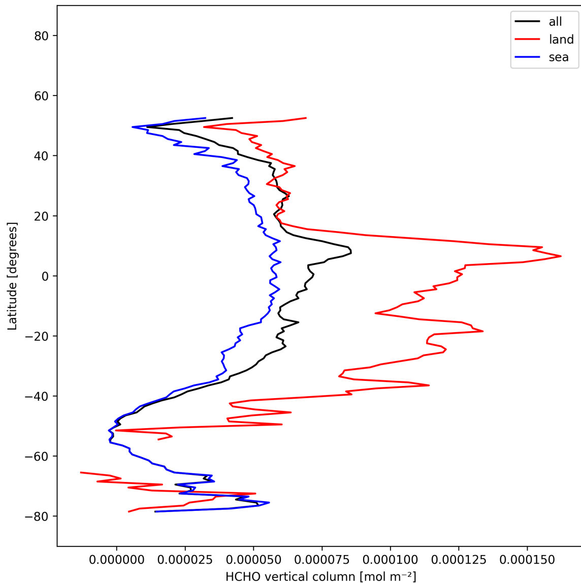
Figure 20: Zonal average of “HCHO vertical column” for 2025-12-06 to 2025-12-07.
