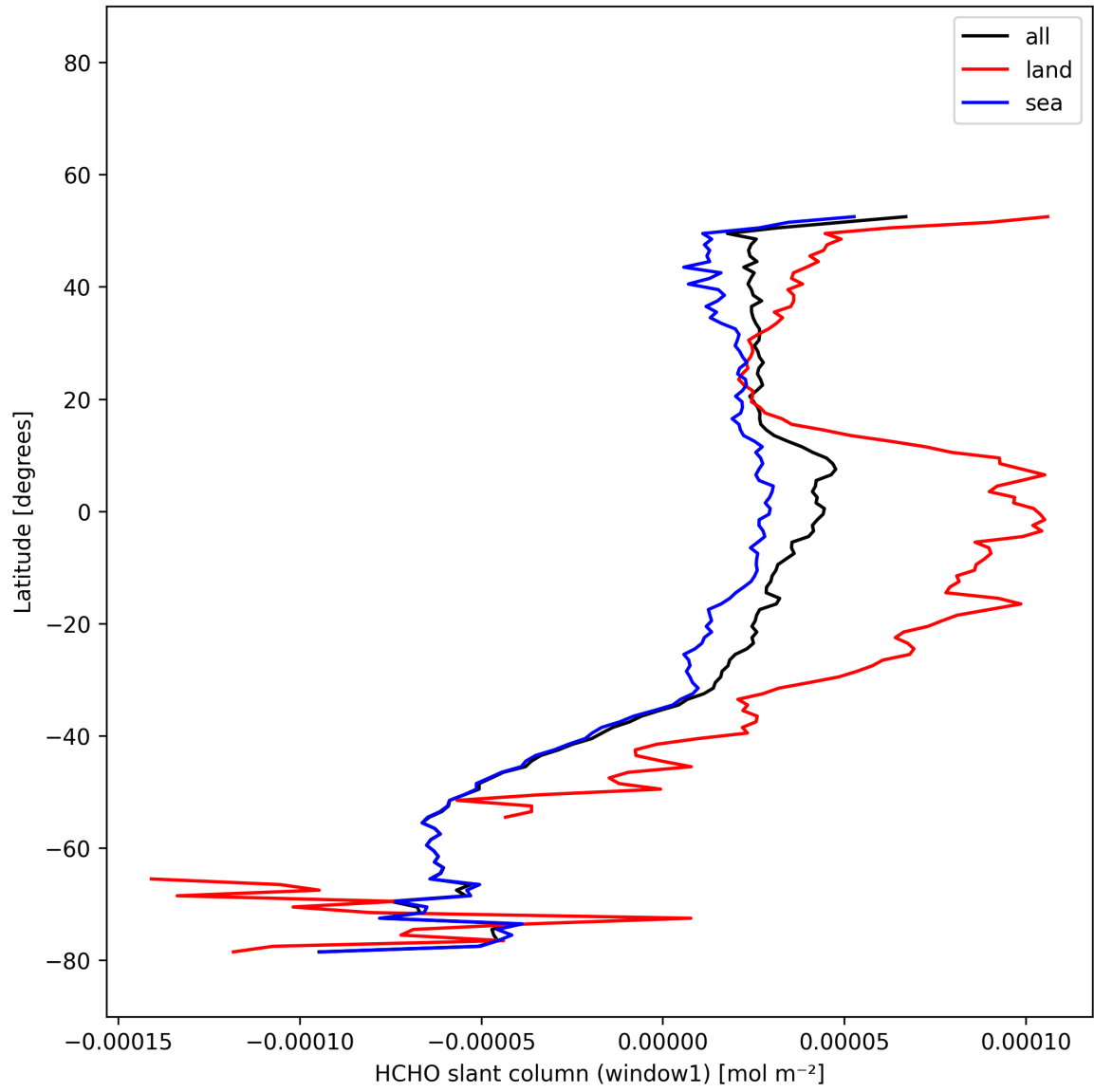
Figure 23: Zonal average of “HCHO slant column (window1)” for 2025-12-06 to 2025-12-07.
