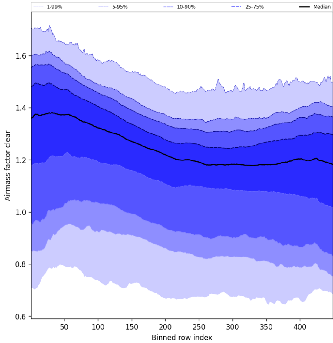
Figure 57: Along track statistics of “Airmass factor clear” for 2025-12-06 to 2025-12-07
