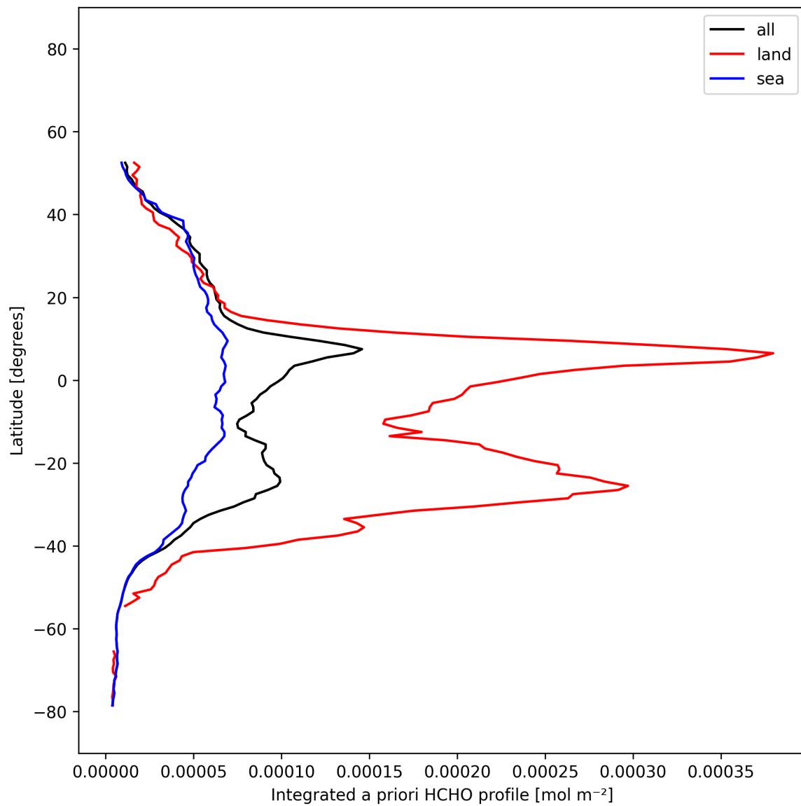
Figure 28: Zonal average of “Integrated a priori HCHO profile” for 2025-12-06 to 2025-12-07.
