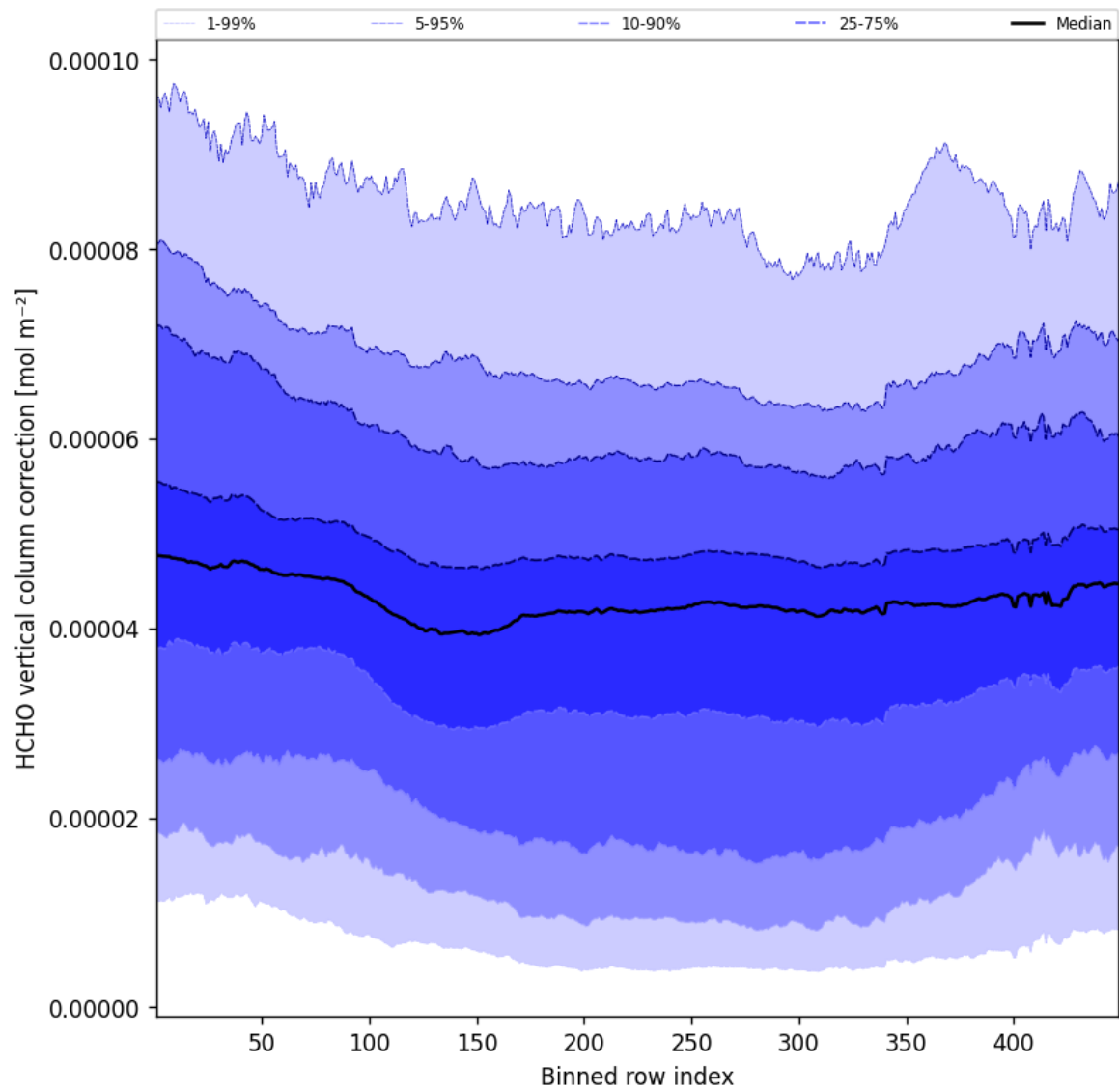
Figure 52: Along track statistics of “HCHO vertical column correction” for 2025-12-06 to 2025-12-07
