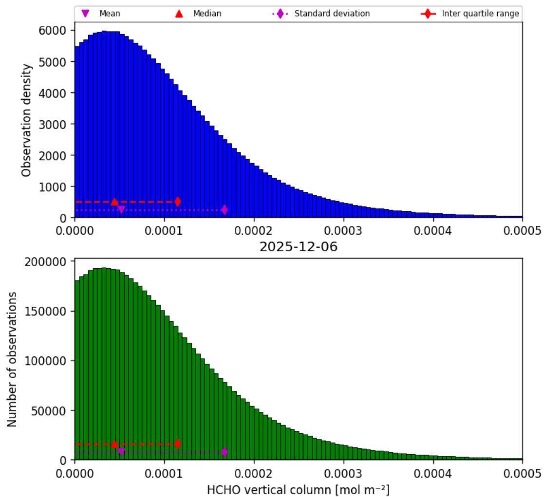
Figure 35: Histogram of “HCHO vertical column” for 2025-12-06 to 2025-12-07
