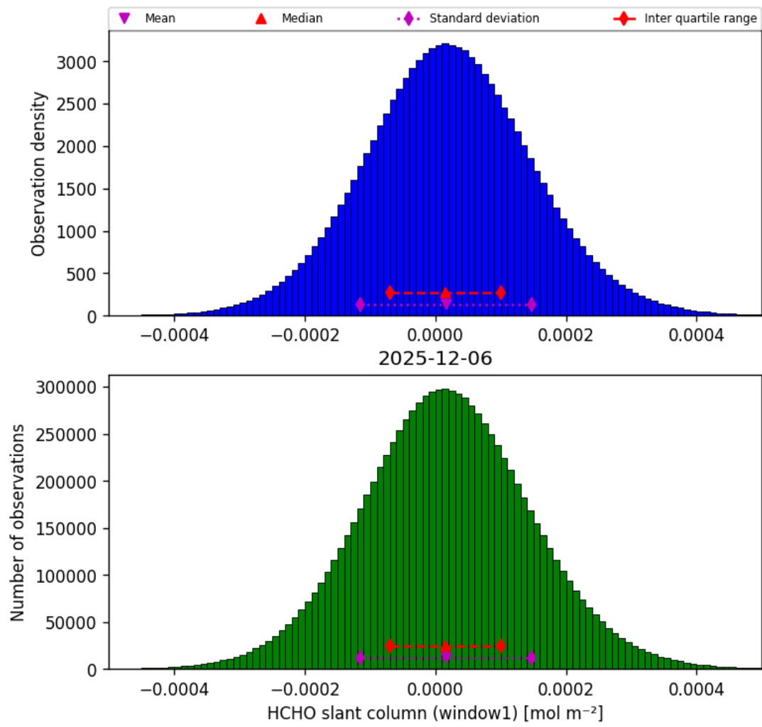
Figure 38: Histogram of “HCHO slant column (window1)” for 2025-12-06 to 2025-12-07
