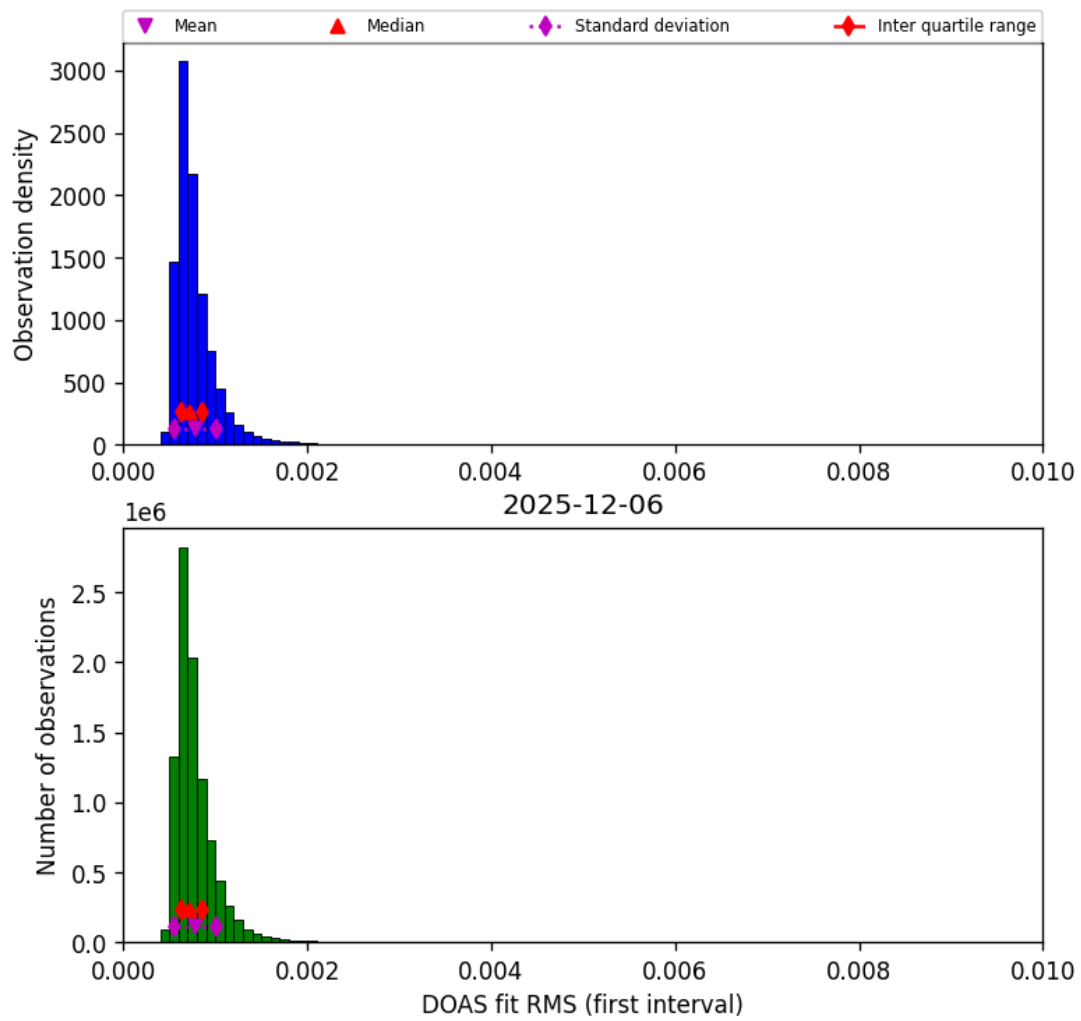
Figure 46: Histogram of “DOAS fit RMS (first interval)” for 2025-12-06 to 2025-12-07
