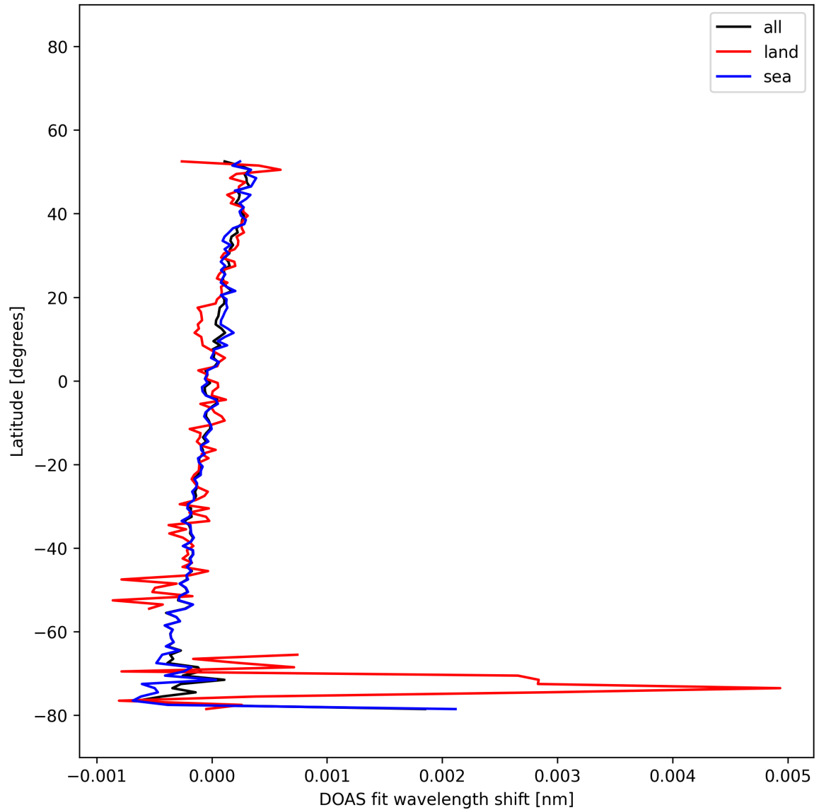
Figure 29: Zonal average of "DOAS fit wavelength shift" for 2025-12-06 to 2025-12-07.
