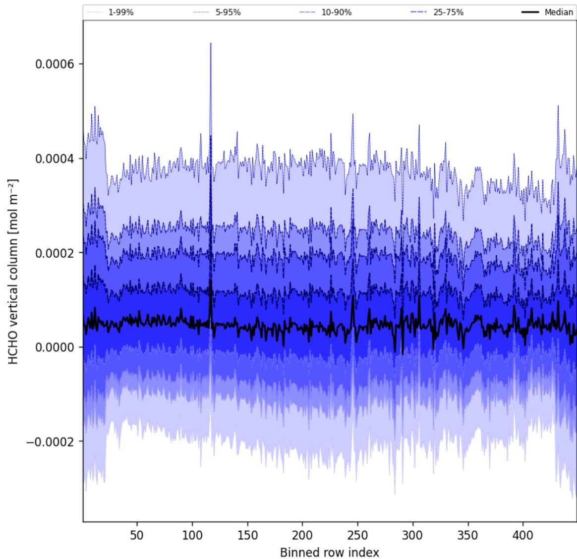
Figure 50: Along track statistics of “HCHO vertical column” for 2025-12-06 to 2025-12-07
