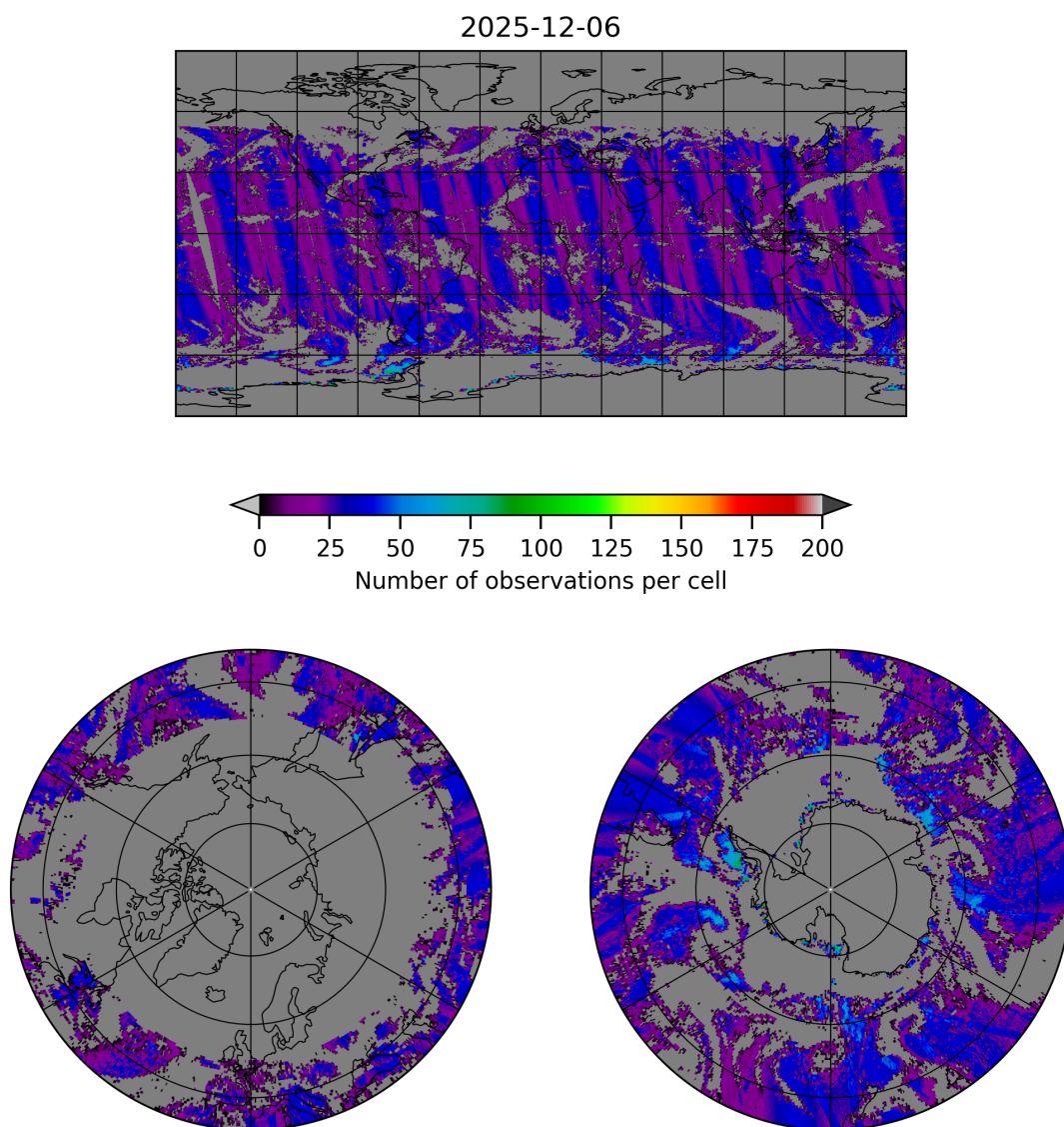
Figure 18: Map of the number of observations for 2025-12-06 to 2025-12-07
