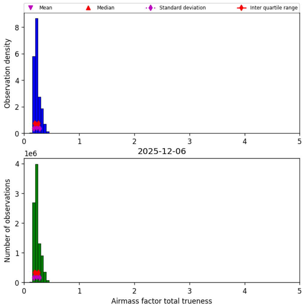
Figure 41: Histogram of “Airmass factor total trueness” for 2025-12-06 to 2025-12-07
