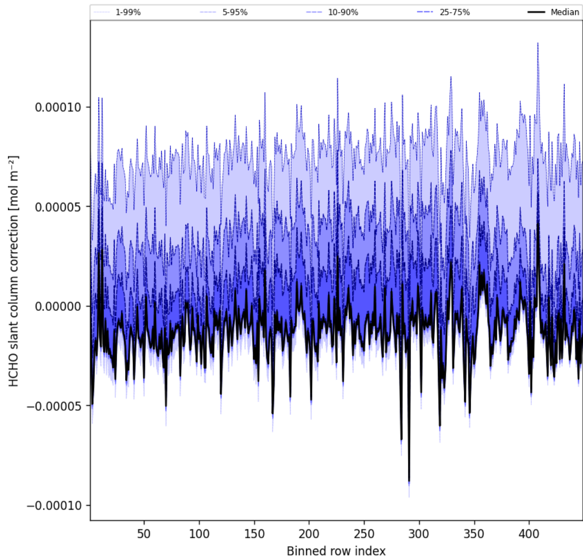
Figure 62: Along track statistics of “HCHO slant column correction” for 2025-12-06 to 2025-12-07
