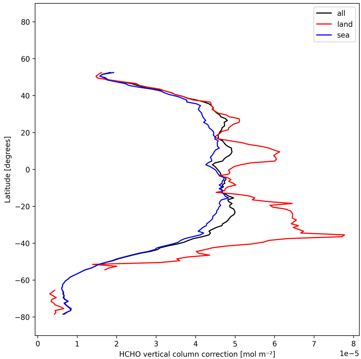
Figure 22: Zonal average of “HCHO vertical column correction” for 2025-12-06 to 2025-12-07.
