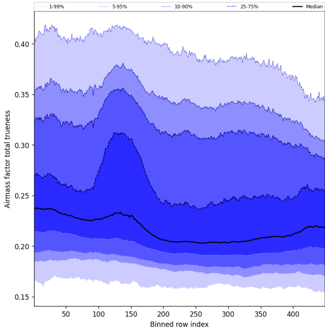
Figure 56: Along track statistics of “Airmass factor total trueness” for 2025-12-06 to 2025-12-07
