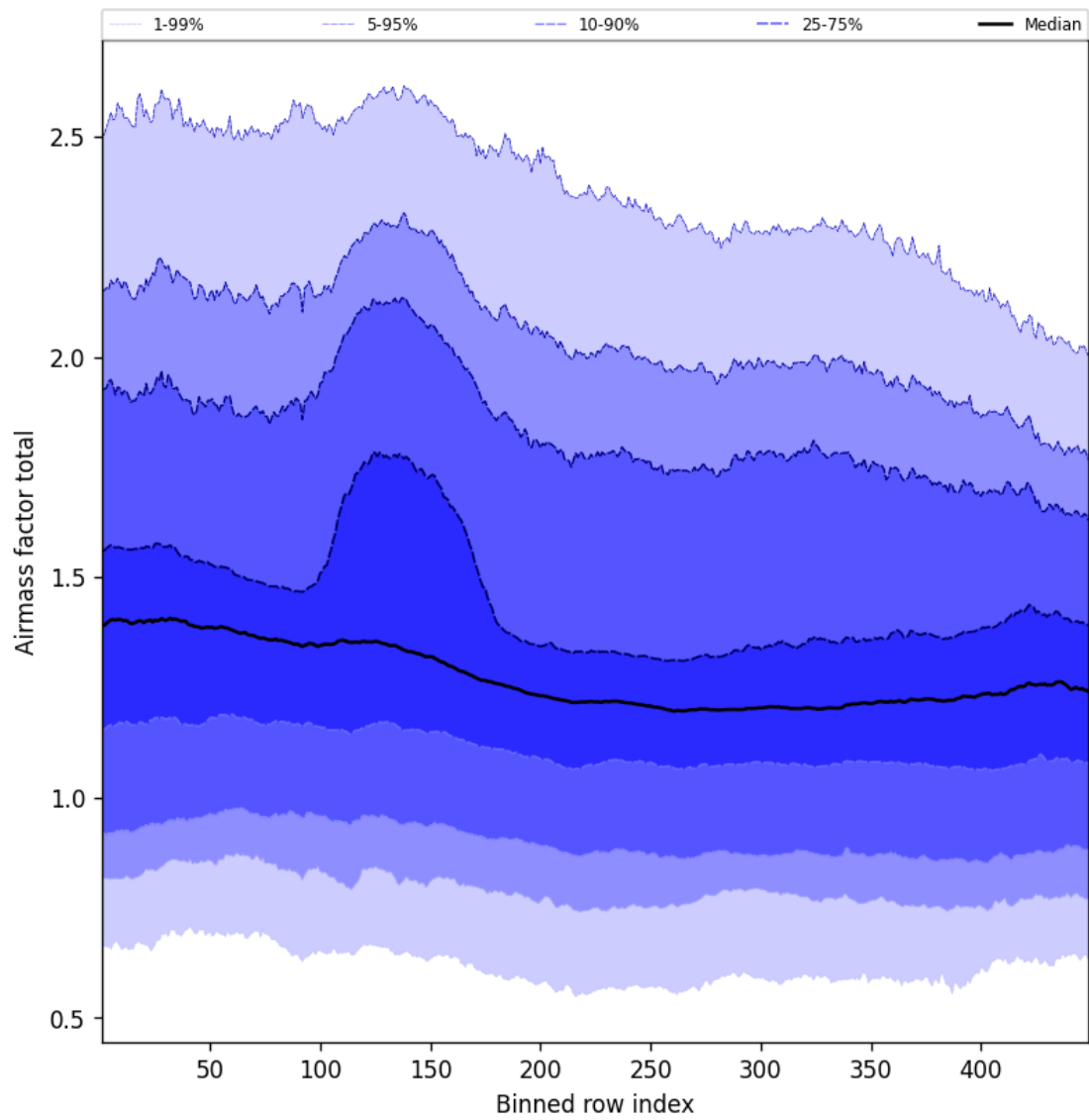
Figure 55: Along track statistics of “Airmass factor total” for 2025-12-06 to 2025-12-07
