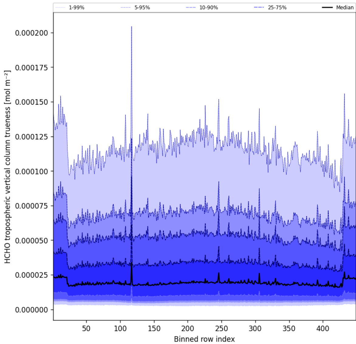
Figure 63: Along track statistics of “HCHO tropospheric vertical column trueness” for 2025-12-06 to 2025-12-07
