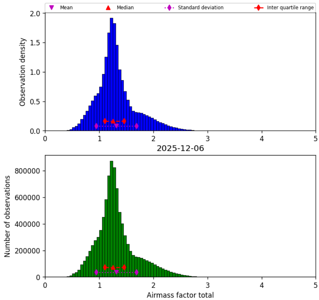
Figure 40: Histogram of “Airmass factor total” for 2025-12-06 to 2025-12-07
