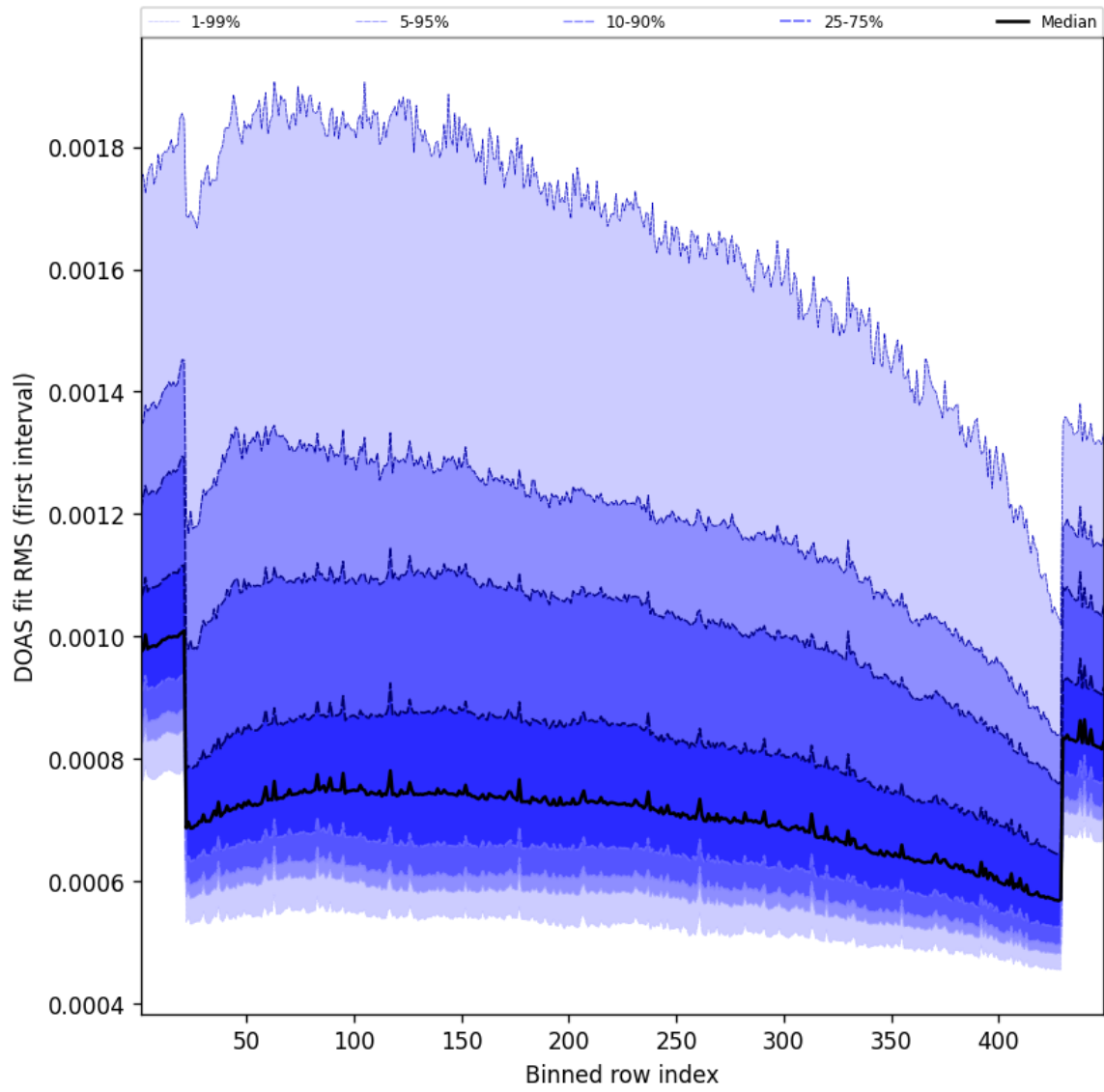
Figure 61: Along track statistics of “DOAS fit RMS (first interval)” for 2025-12-06 to 2025-12-07
