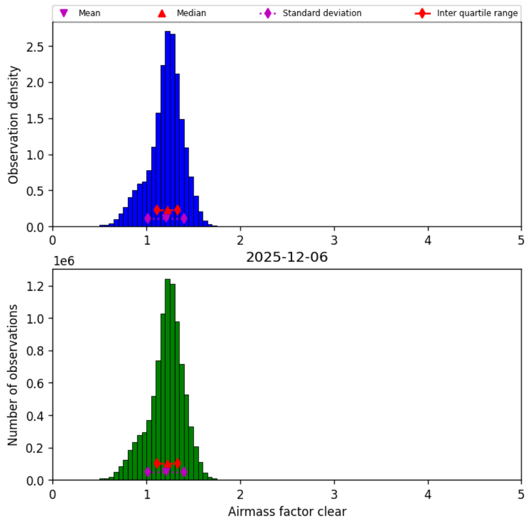
Figure 42: Histogram of “Airmass factor clear” for 2025-12-06 to 2025-12-07
