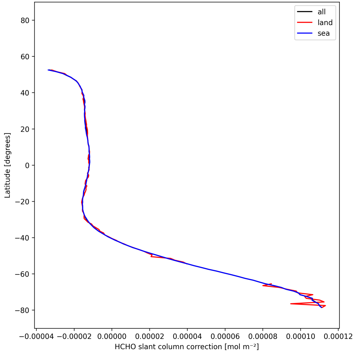
Figure 32: Zonal average of “HCHO slant column correction” for 2025-12-06 to 2025-12-07.
