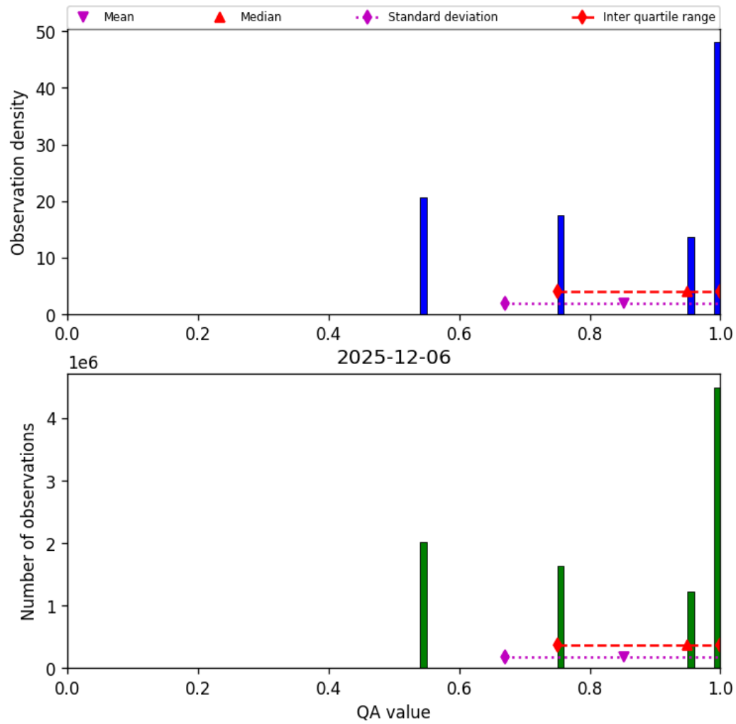
Figure 34: Histogram of “QA value” for 2025-12-06 to 2025-12-07
