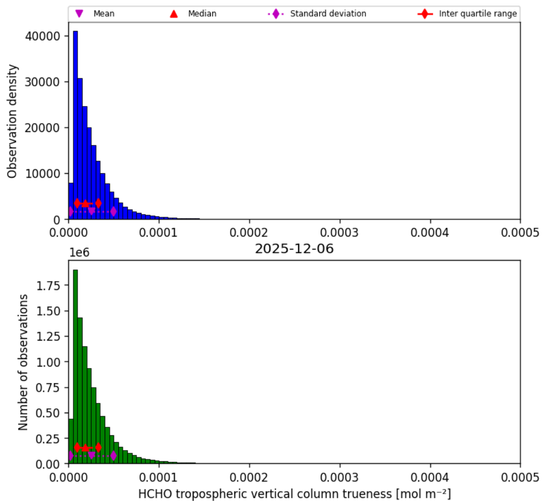
Figure 48: Histogram of “HCHO tropospheric vertical column trueness” for 2025-12-06 to 2025-12-07
