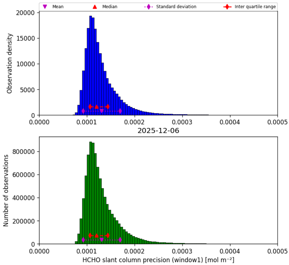
Figure 39: Histogram of “HCHO slant column precision (window1)” for 2025-12-06 to 2025-12-07
