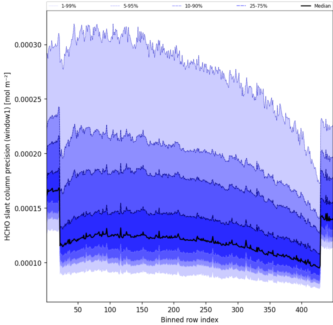
Figure 54: Along track statistics of “HCHO slant column precision (window1)” for 2025-12-06 to 2025-12-07
