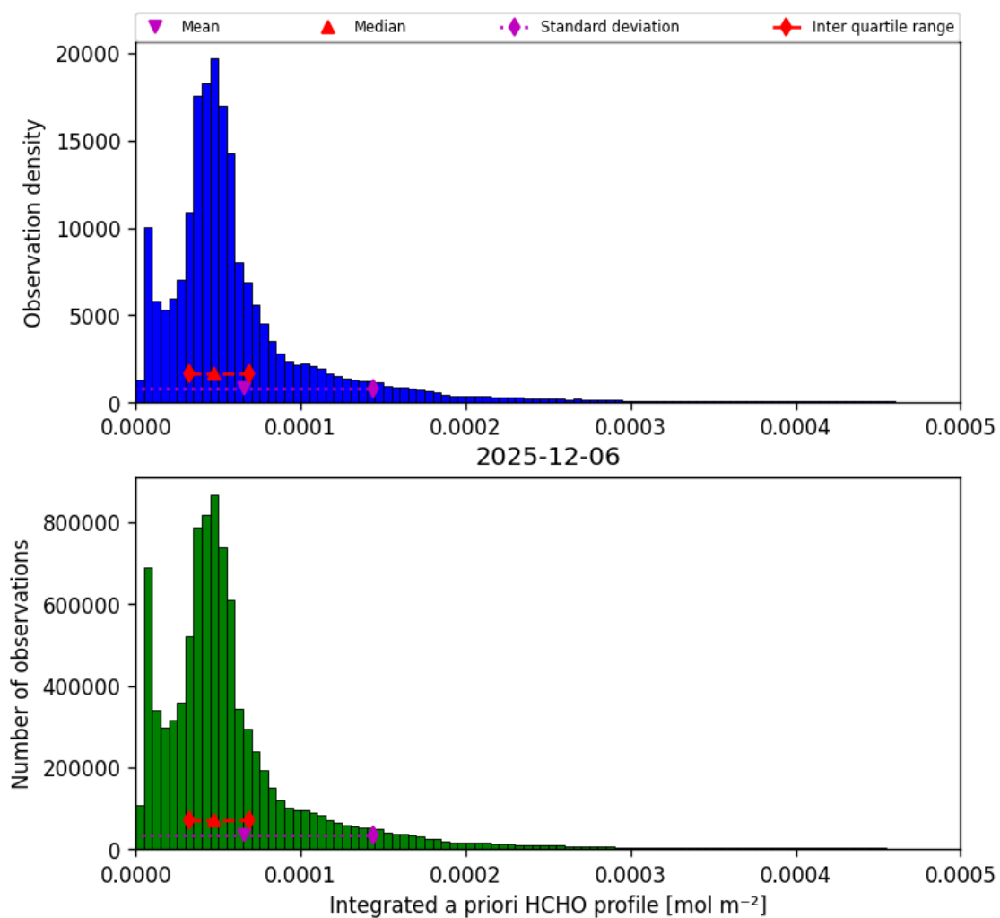
Figure 43: Histogram of “Integrated a priori HCHO profile” for 2025-12-06 to 2025-12-07
