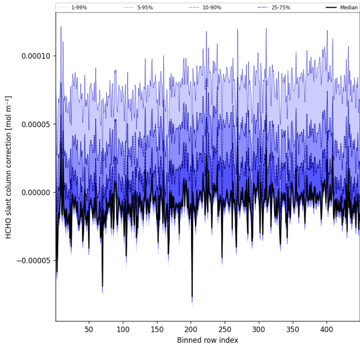
Figure 62: Along track statistics of “HCHO slant column correction” for 2025-12-07 to 2025-12-07
