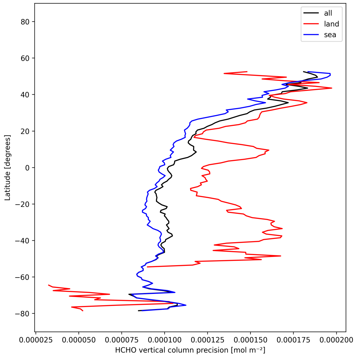
Figure 21: Zonal average of “HCHO vertical column precision” for 2025-12-07 to 2025-12-07.
