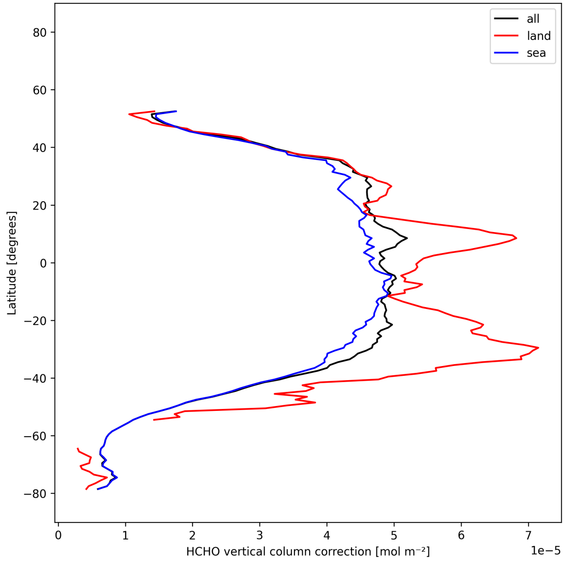
Figure 22: Zonal average of “HCHO vertical column correction” for 2025-12-07 to 2025-12-07.
