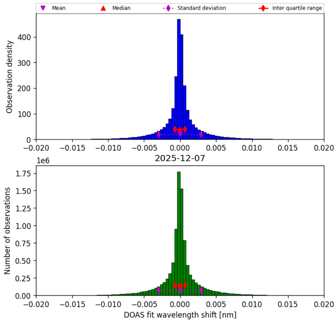
Figure 44: Histogram of “DOAS fit wavelength shift” for 2025-12-07 to 2025-12-07
