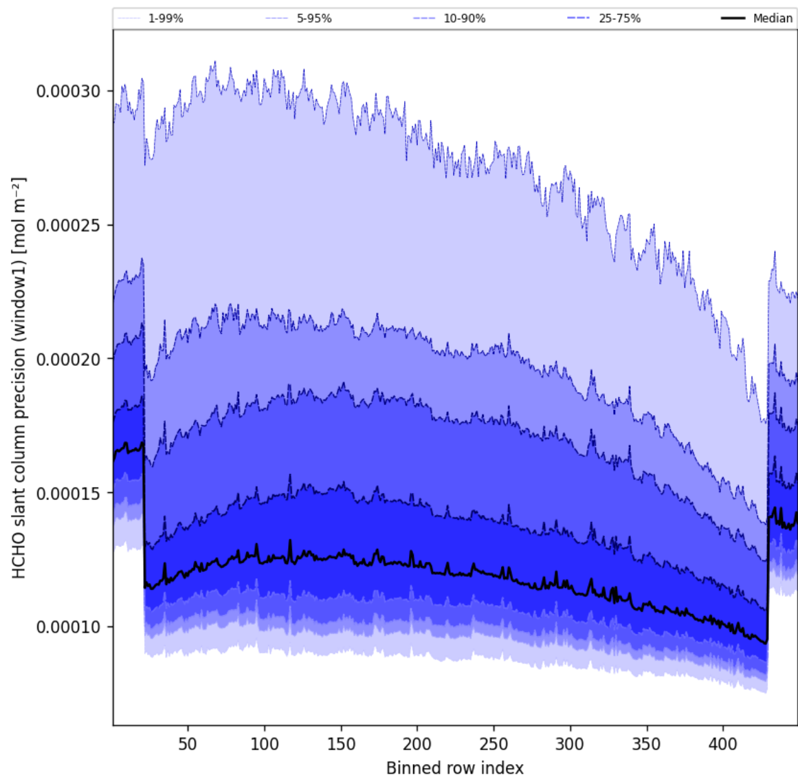
Figure 54: Along track statistics of “HCHO slant column precision (window1)” for 2025-12-07 to 2025-12-07
