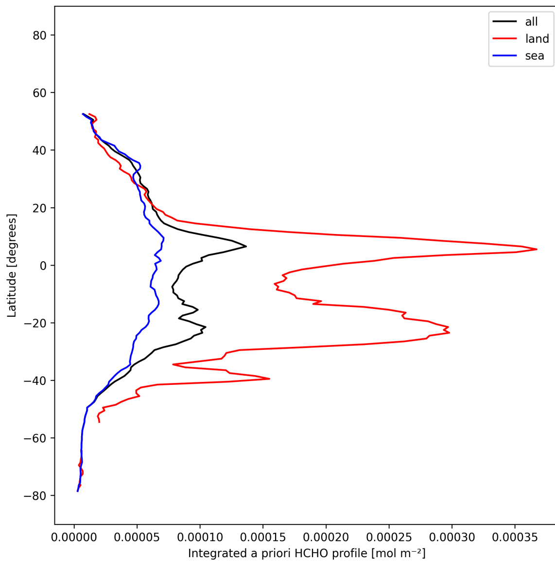
Figure 28: Zonal average of “Integrated a priori HCHO profile” for 2025-12-07 to 2025-12-07.
