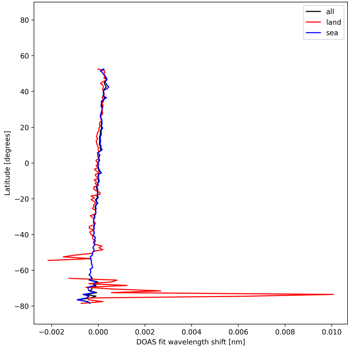
Figure 29: Zonal average of “DOAS fit wavelength shift” for 2025-12-07 to 2025-12-07.
