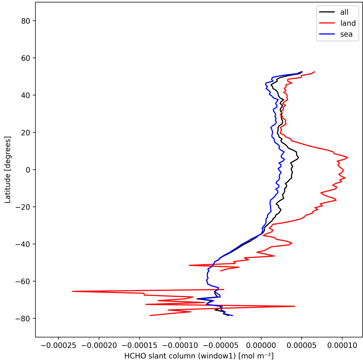
Figure 23: Zonal average of “HCHO slant column (window1)” for 2025-12-07 to 2025-12-07.
