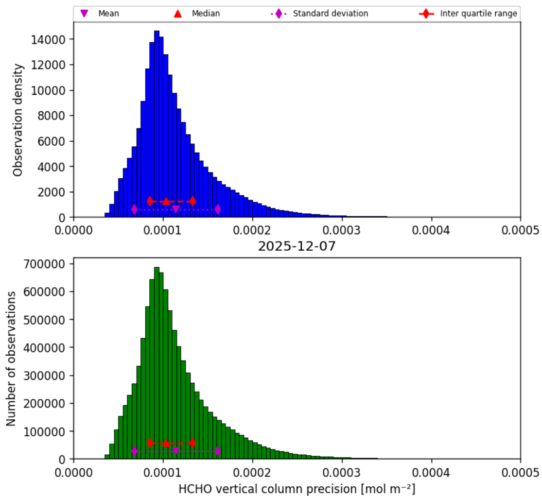
Figure 36: Histogram of “HCHO vertical column precision” for 2025-12-07 to 2025-12-07
