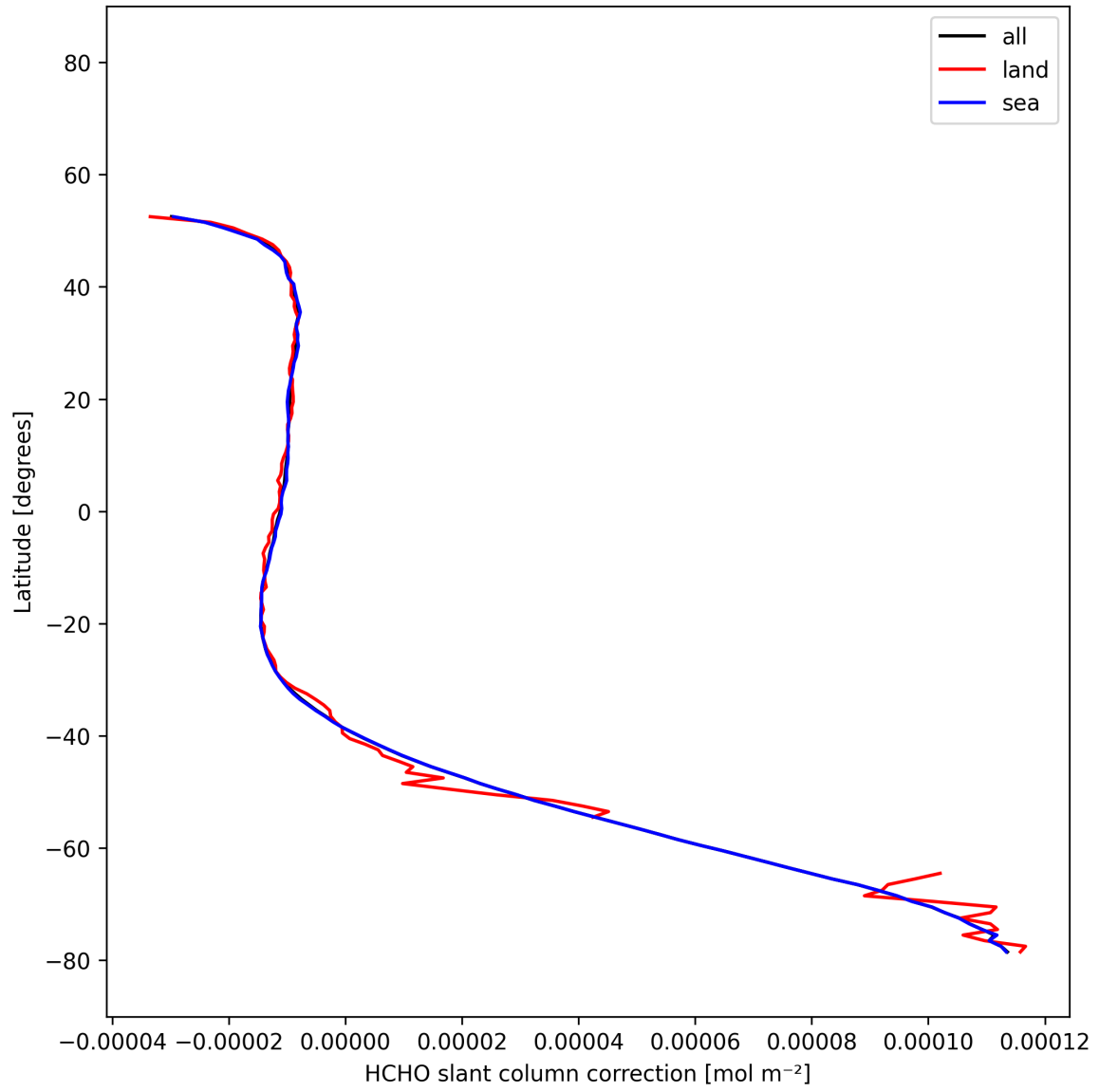
Figure 32: Zonal average of “HCHO slant column correction” for 2025-12-07 to 2025-12-07.
