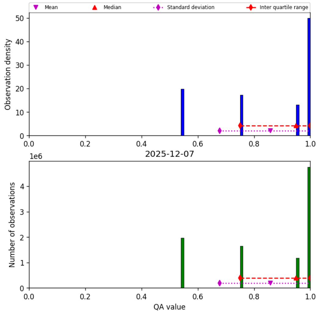
Figure 34: Histogram of “QA value” for 2025-12-07 to 2025-12-07
