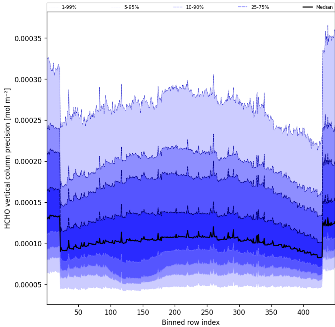
Figure 51: Along track statistics of “HCHO vertical column precision” for 2025-12-07 to 2025-12-07
