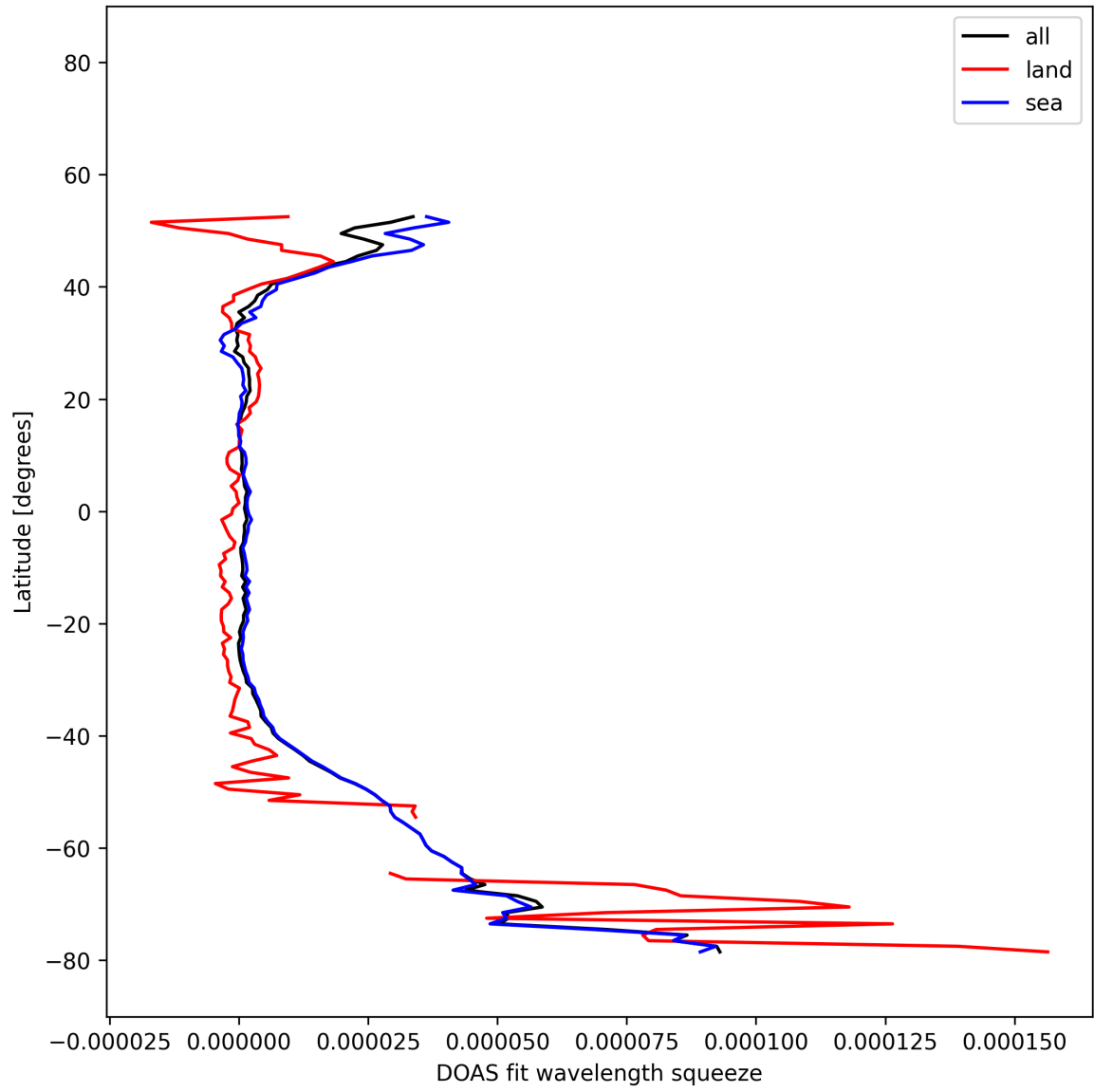
Figure 30: Zonal average of “DOAS fit wavelength squeeze” for 2025-12-07 to 2025-12-07.
