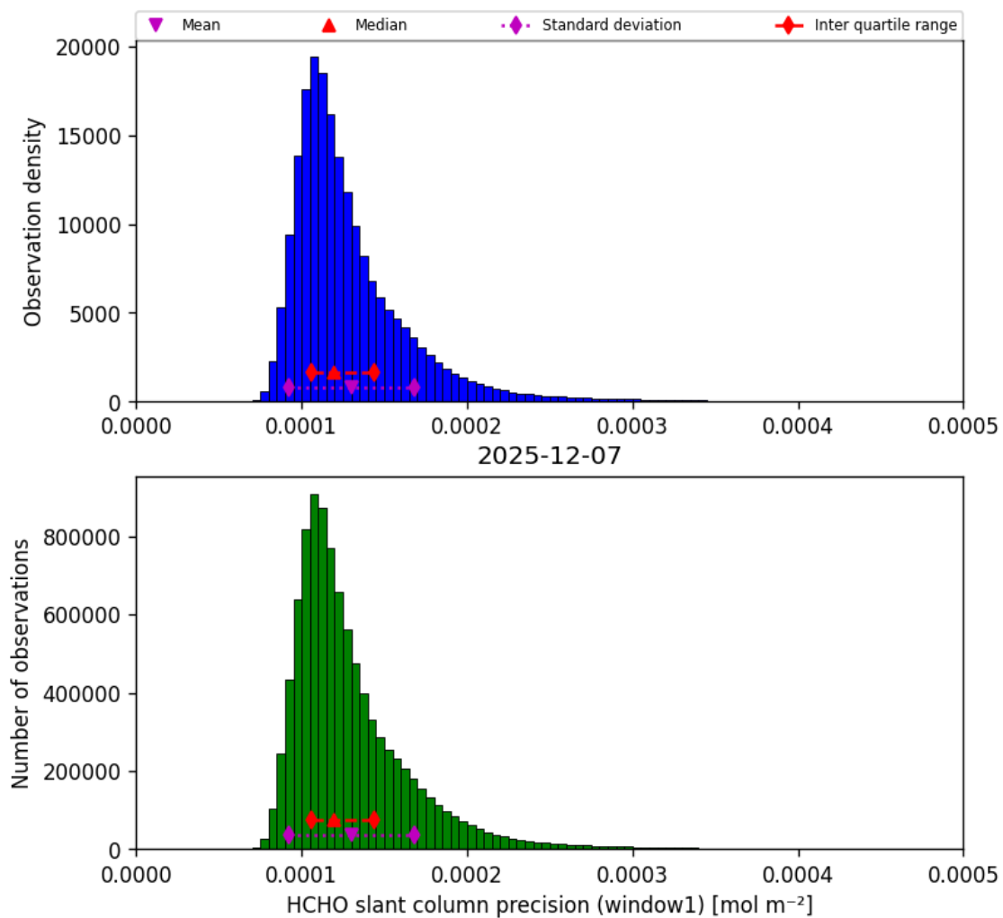
Figure 39: Histogram of “HCHO slant column precision (window1)” for 2025-12-07 to 2025-12-07
