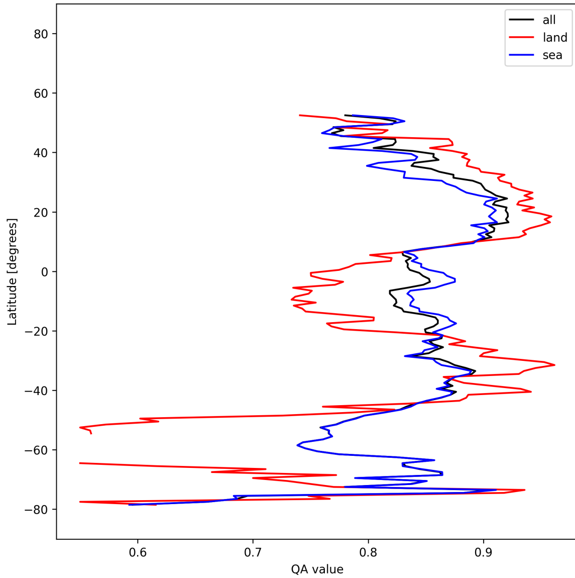
Figure 19: Zonal average of “QA value” for 2025-12-07 to 2025-12-07.
