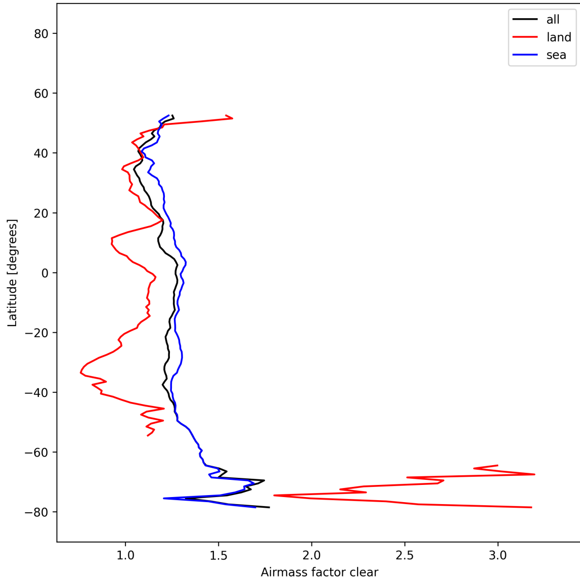
Figure 27: Zonal average of “Airmass factor clear” for 2025-12-07 to 2025-12-07.
