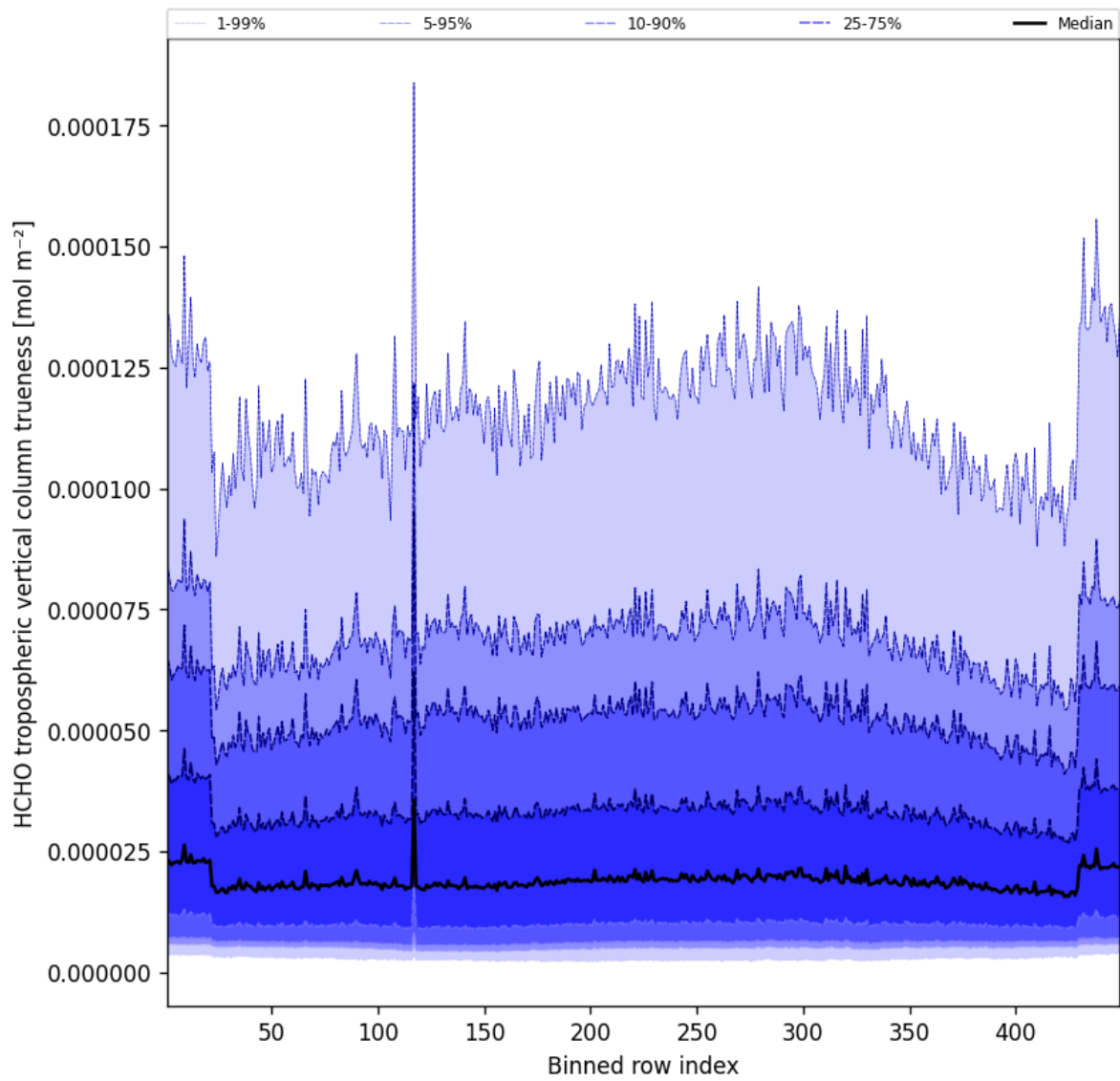
Figure 63: Along track statistics of “HCHO tropospheric vertical column trueness” for 2025-12-07 to 2025-12-07
