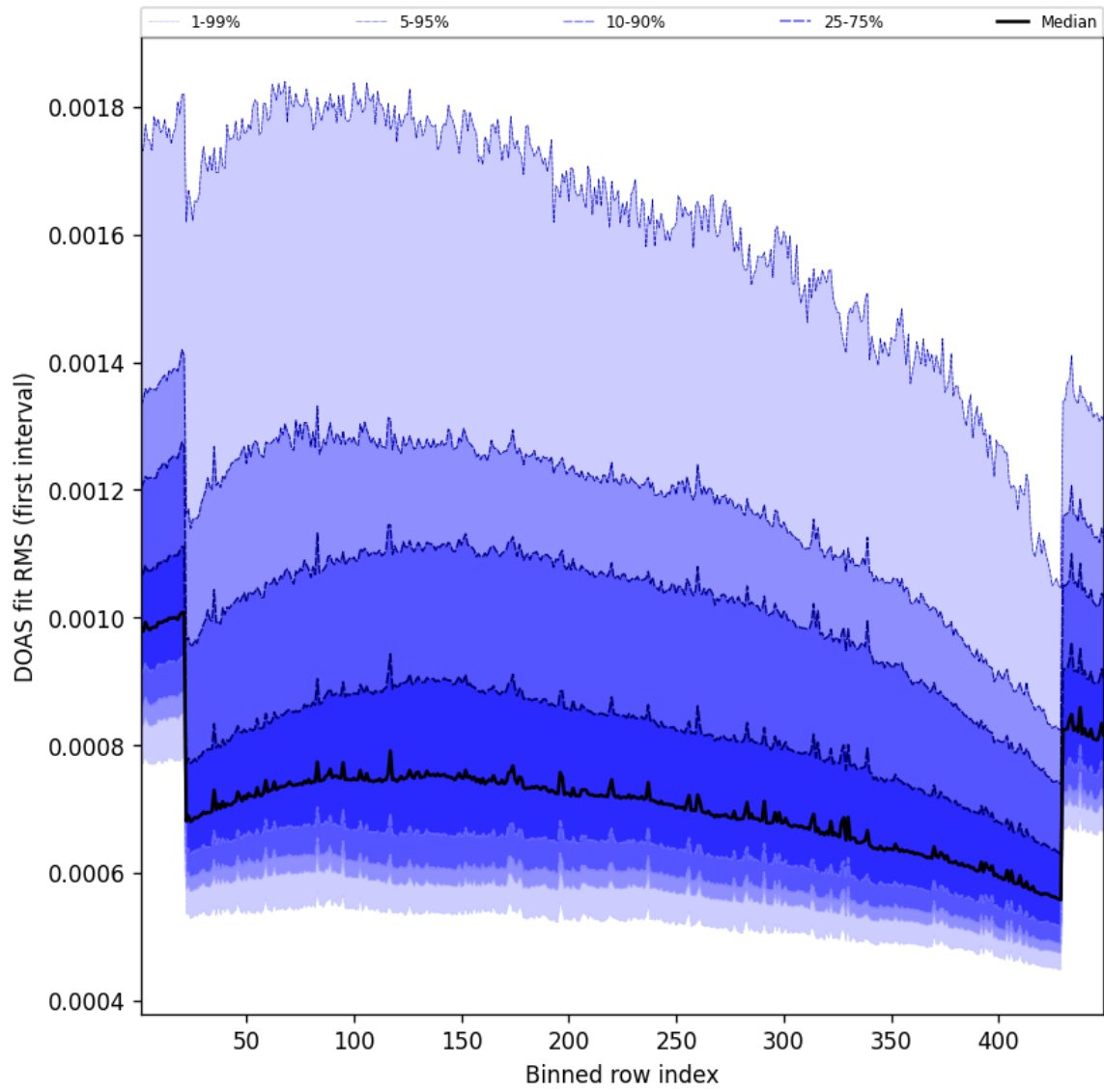
Figure 61: Along track statistics of “DOAS fit RMS (first interval)” for 2025-12-07 to 2025-12-07
