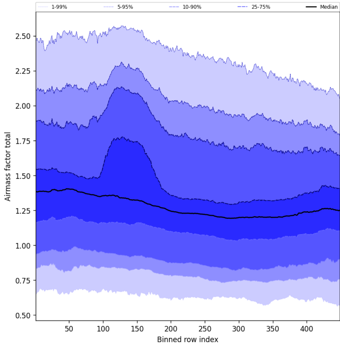
Figure 55: Along track statistics of “Airmass factor total” for 2025-12-07 to 2025-12-07
