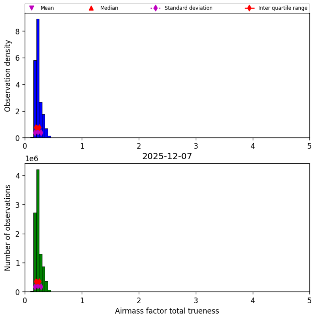
Figure 41: Histogram of “Airmass factor total trueness” for 2025-12-07 to 2025-12-07
