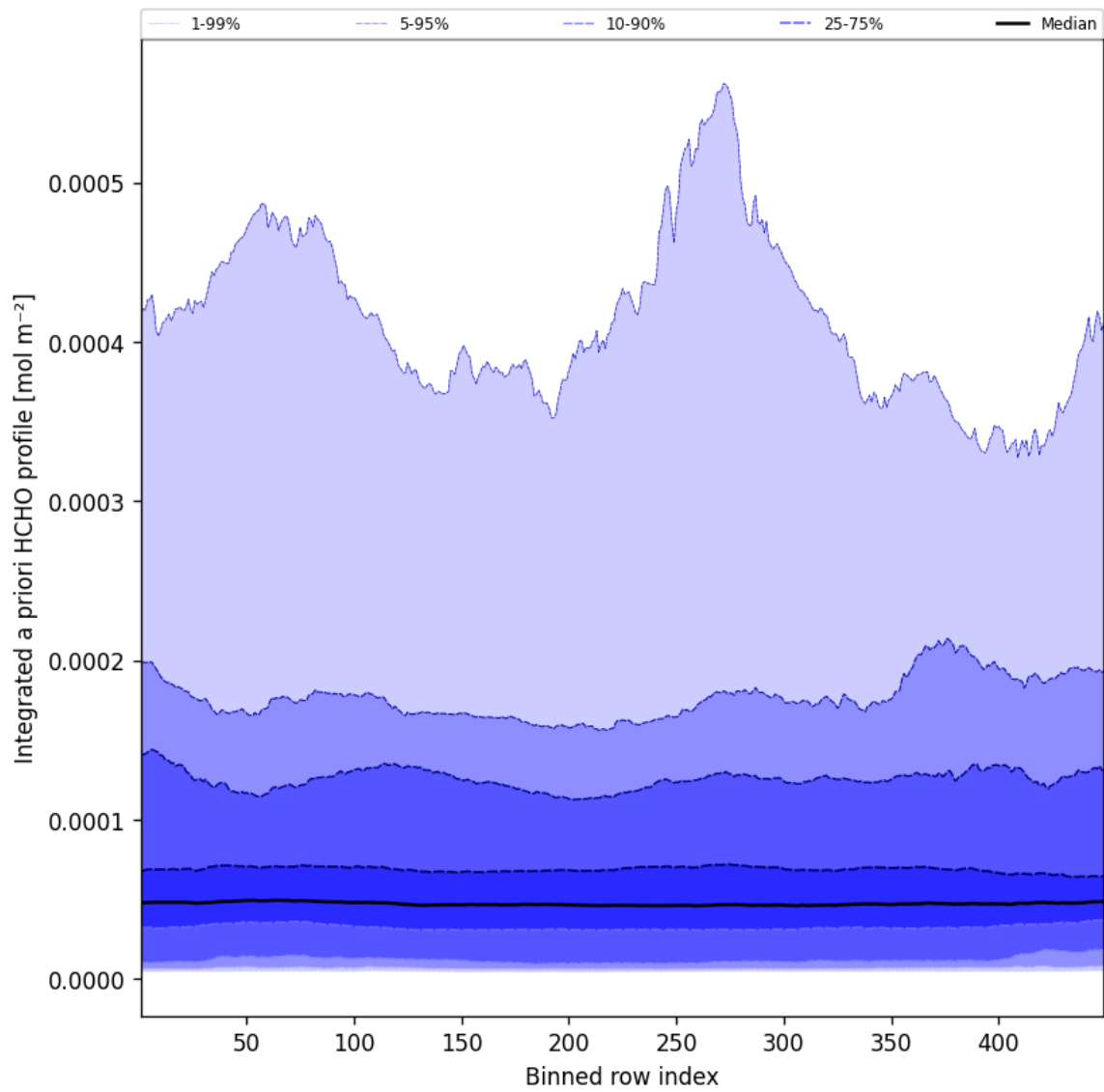
Figure 58: Along track statistics of "Integrated a priori HCHO profile" for 2025-12-07 to 2025-12-07
