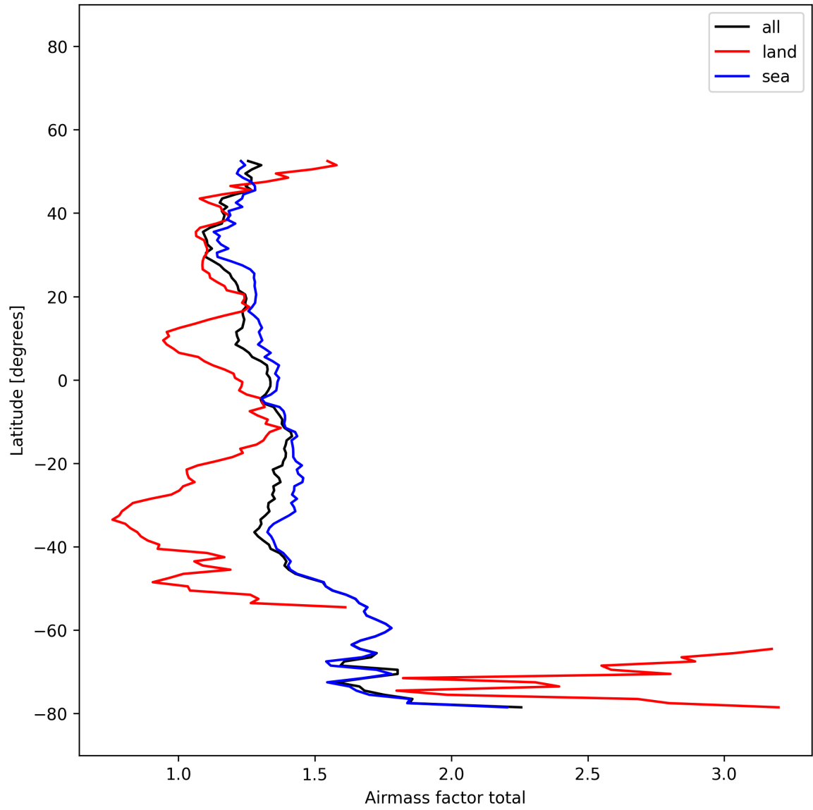
Figure 25: Zonal average of “Airmass factor total” for 2025-12-07 to 2025-12-07.
