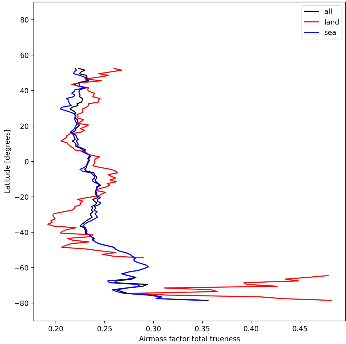
Figure 26: Zonal average of “Airmass factor total trueness” for 2025-12-07 to 2025-12-07.
