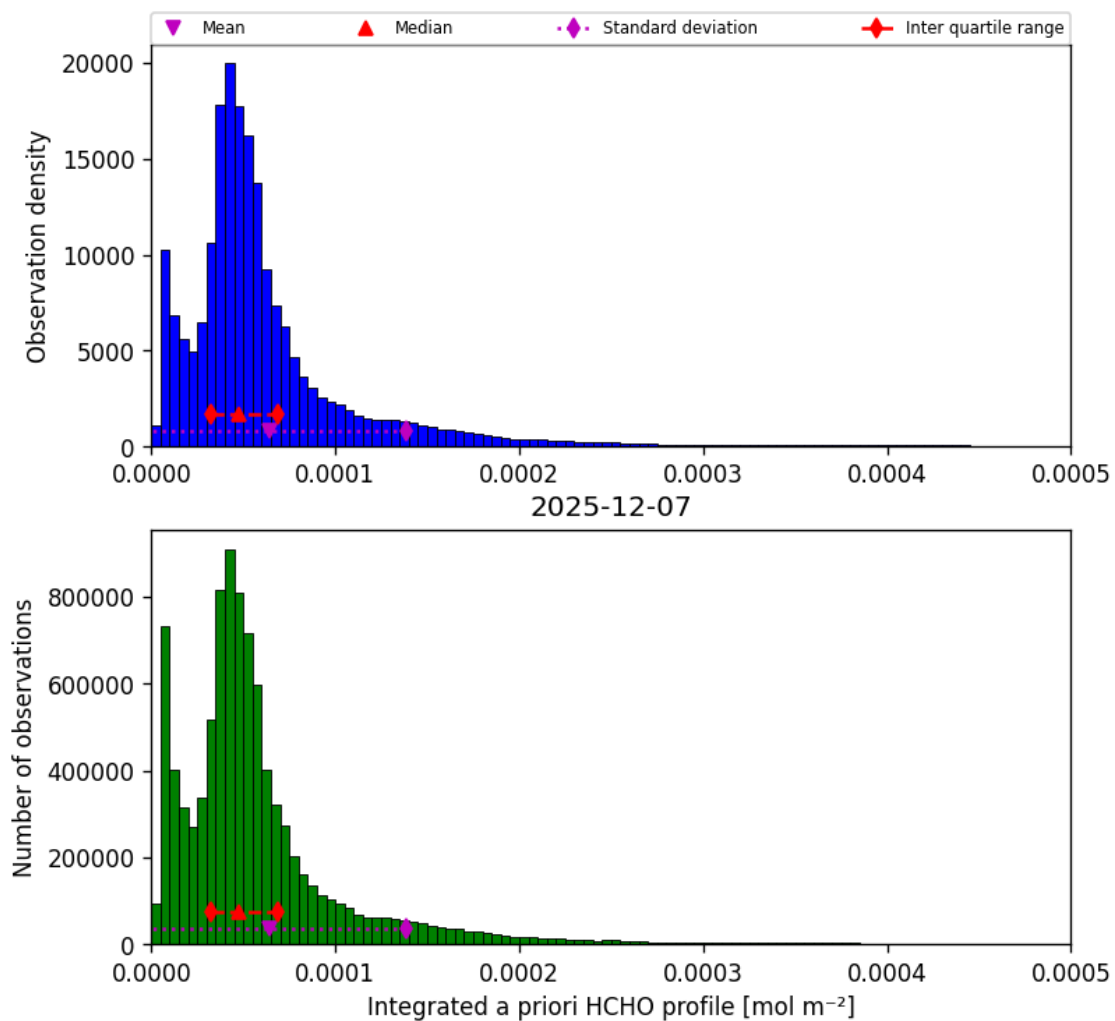
Figure 43: Histogram of “Integrated a priori HCHO profile” for 2025-12-07 to 2025-12-07
