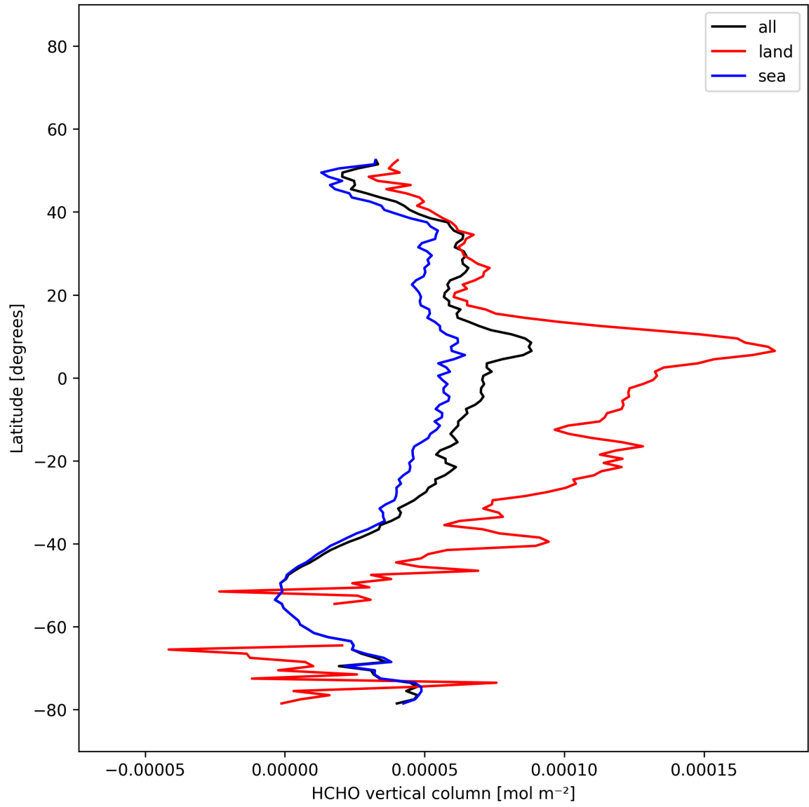
Figure 20: Zonal average of “HCHO vertical column” for 2025-12-07 to 2025-12-07.
