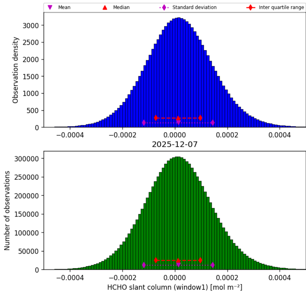
Figure 38: Histogram of “HCHO slant column (window1)” for 2025-12-07 to 2025-12-07
