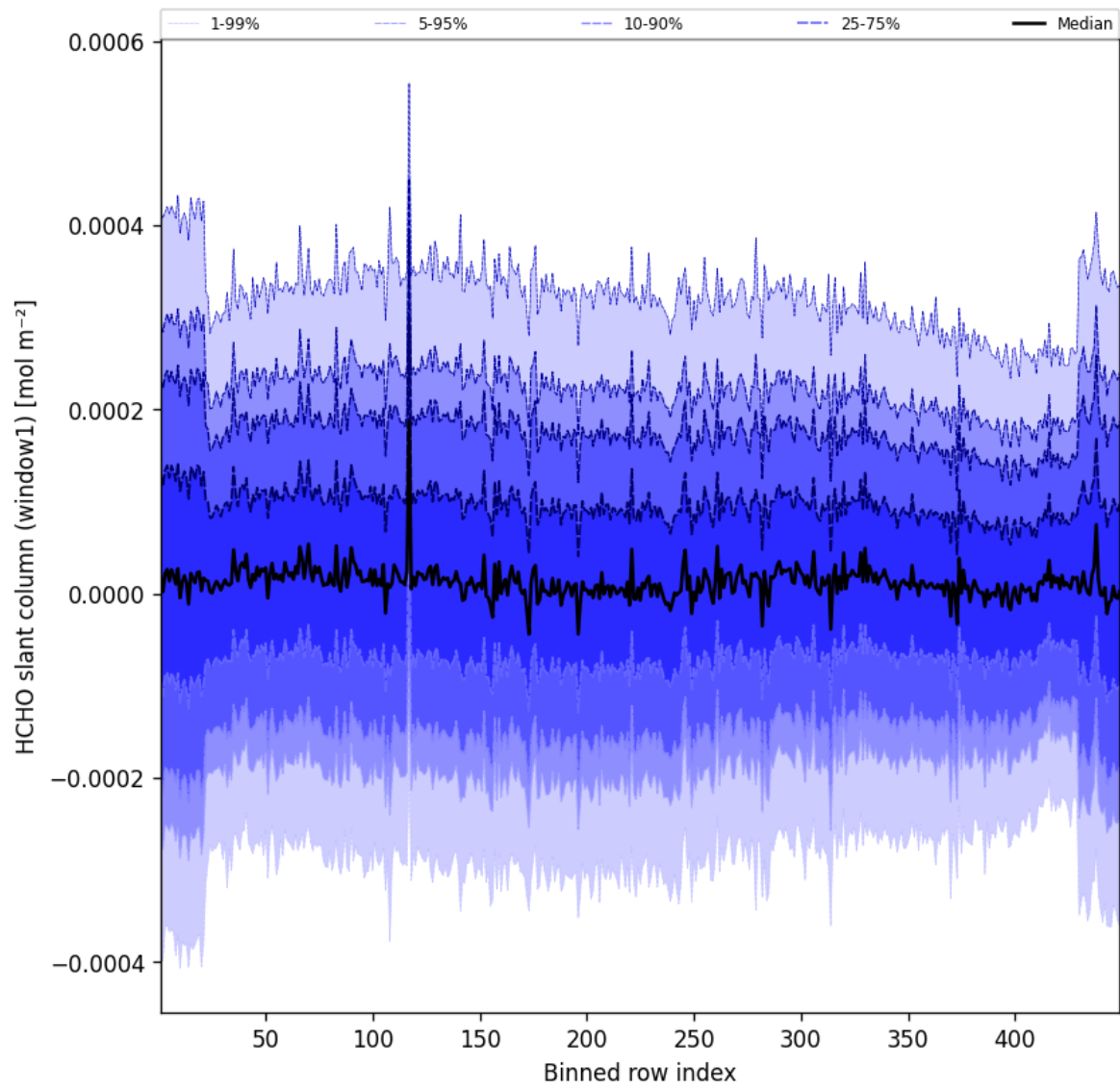
Figure 53: Along track statistics of “HCHO slant column (window1)” for 2025-12-07 to 2025-12-07
