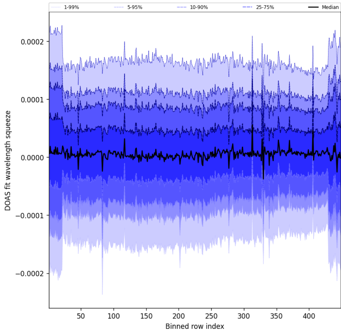
Figure 60: Along track statistics of “DOAS fit wavelength squeeze” for 2025-12-07 to 2025-12-07
