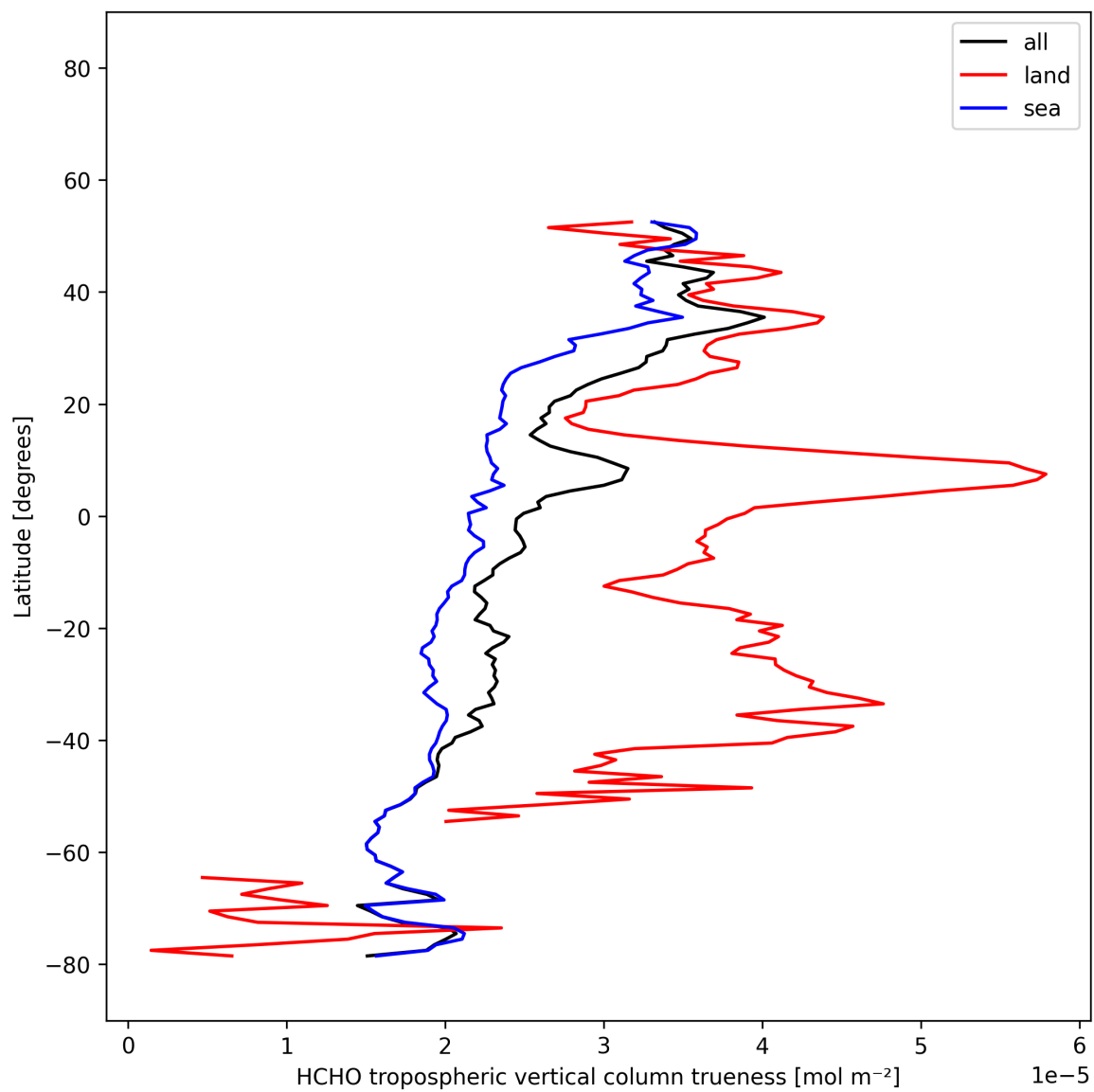
Figure 33: Zonal average of “HCHO tropospheric vertical column trueness” for 2025-12-07 to 2025-12-07.
