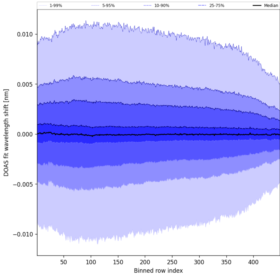
Figure 59: Along track statistics of “DOAS fit wavelength shift” for 2025-12-07 to 2025-12-07
