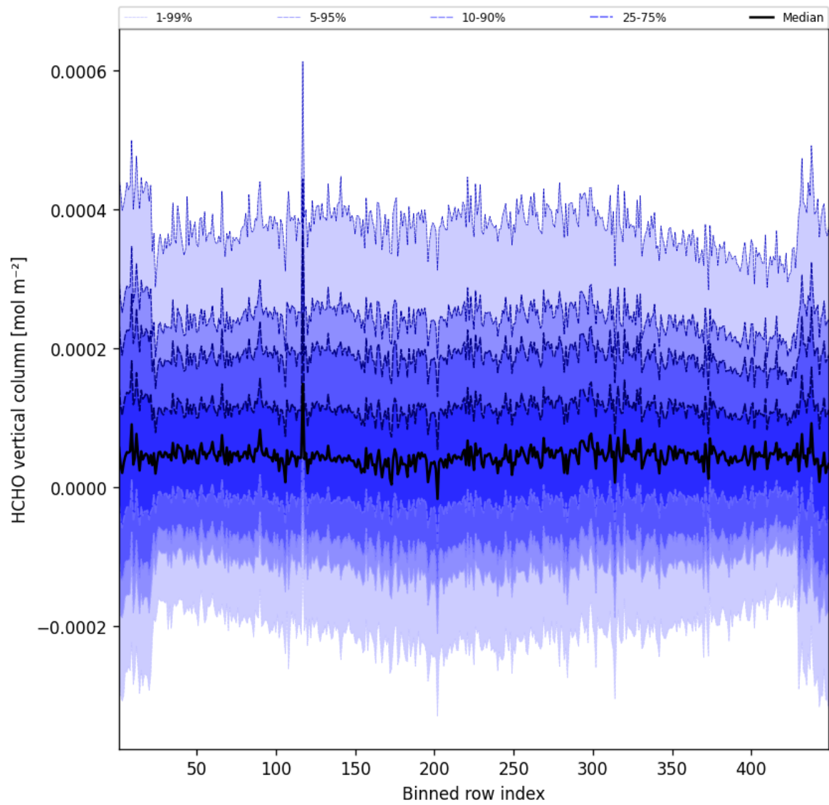
Figure 50: Along track statistics of “HCHO vertical column” for 2025-12-07 to 2025-12-07
