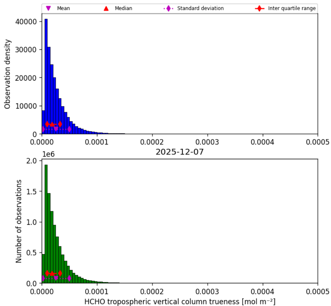
Figure 48: Histogram of “HCHO tropospheric vertical column trueness” for 2025-12-07 to 2025-12-07
