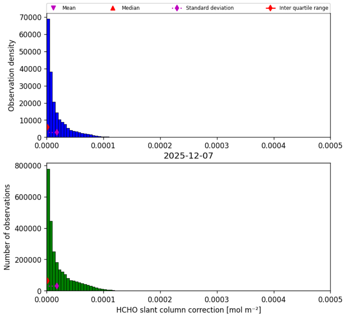
Figure 47: Histogram of “HCHO slant column correction” for 2025-12-07 to 2025-12-07
