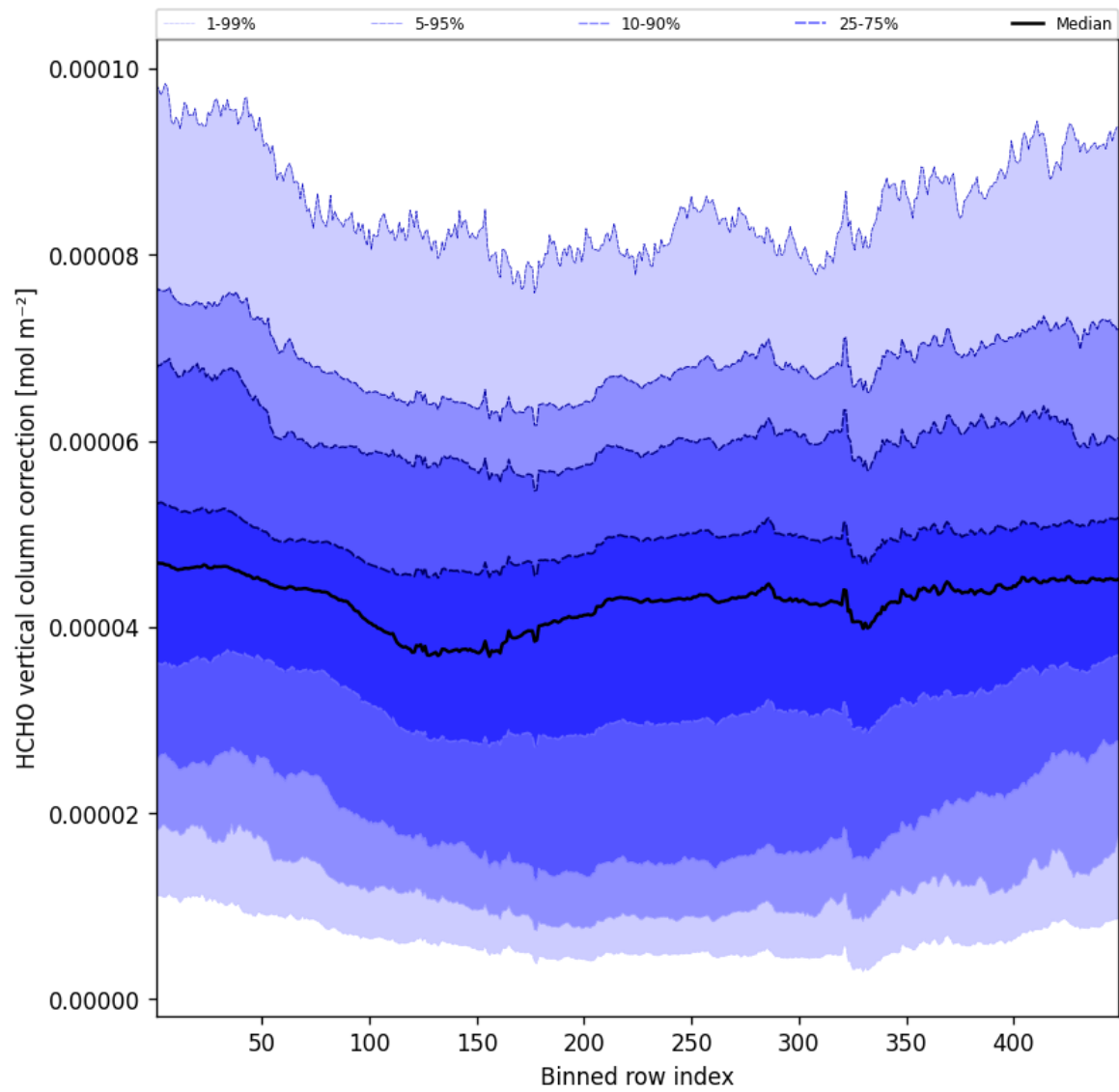
Figure 52: Along track statistics of “HCHO vertical column correction” for 2025-12-07 to 2025-12-07
