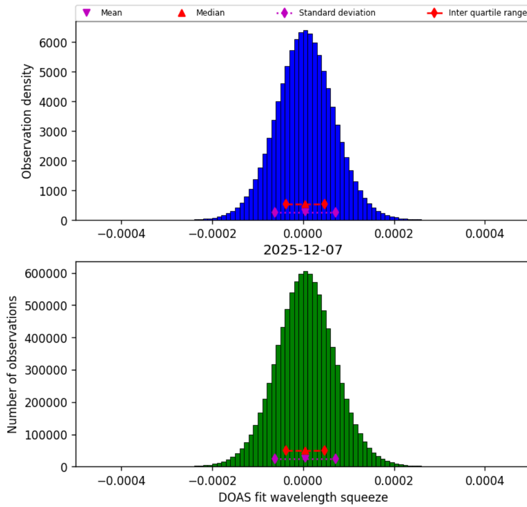
Figure 45: Histogram of “DOAS fit wavelength squeeze” for 2025-12-07 to 2025-12-07
