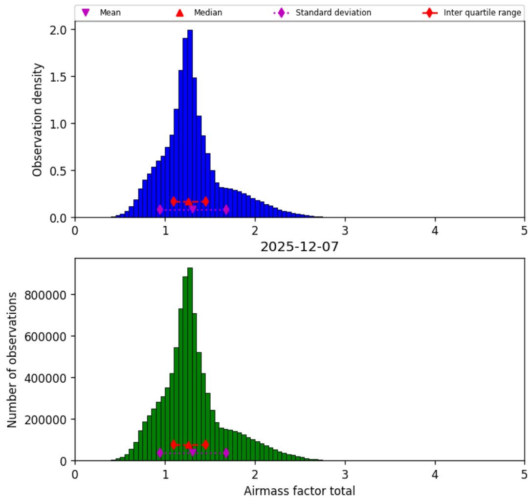
Figure 40: Histogram of “Airmass factor total” for 2025-12-07 to 2025-12-07
