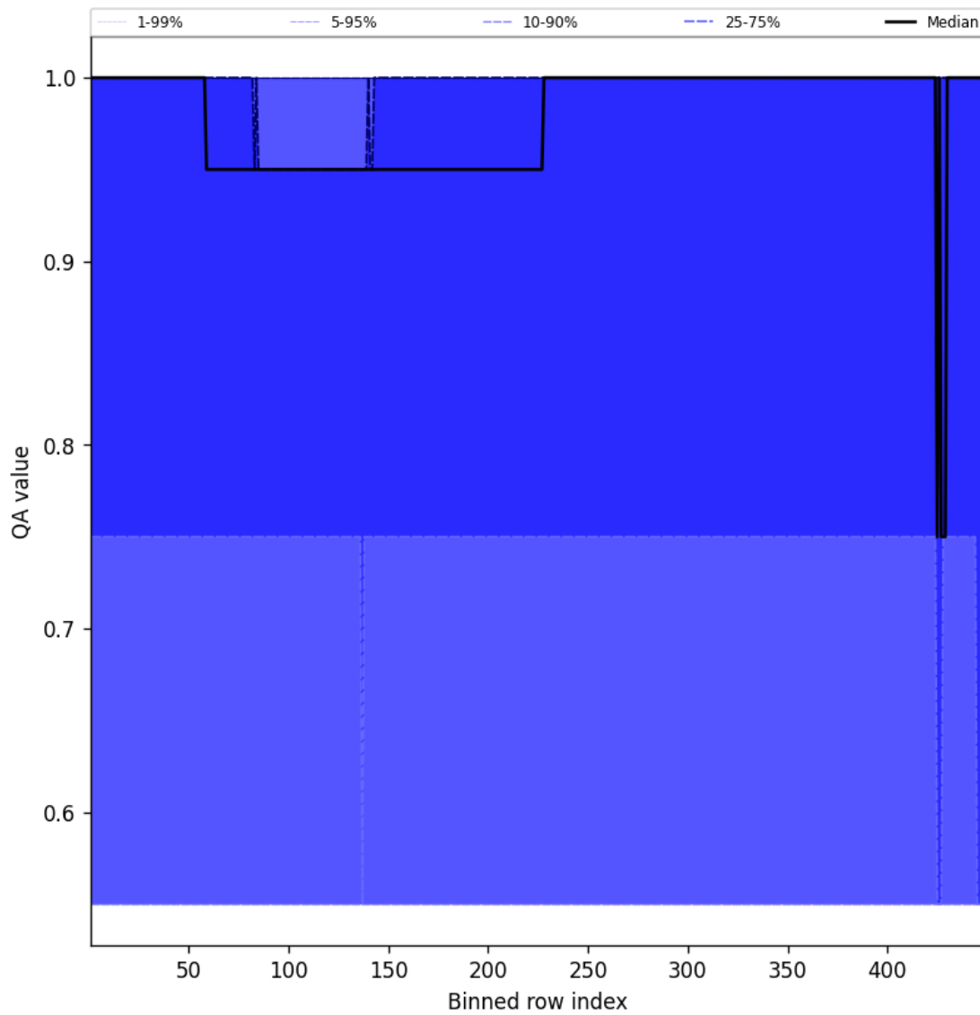
Figure 49: Along track statistics of “QA value” for 2025-12-07 to 2025-12-07
