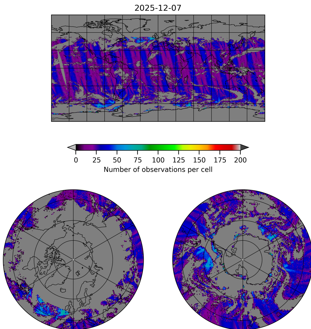
Figure 18: Map of the number of observations for 2025-12-07 to 2025-12-07
