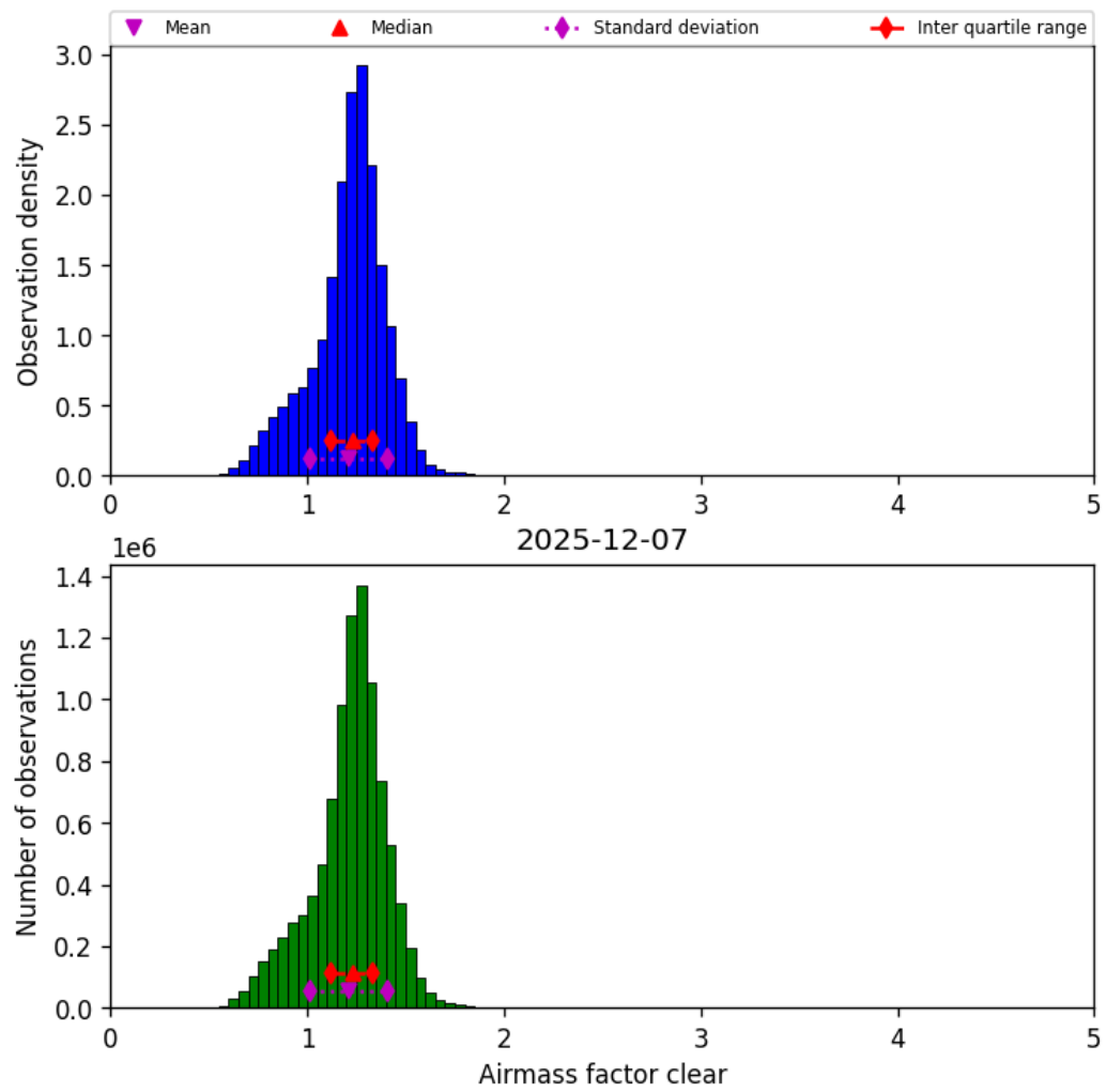
Figure 42: Histogram of “Airmass factor clear” for 2025-12-07 to 2025-12-07
