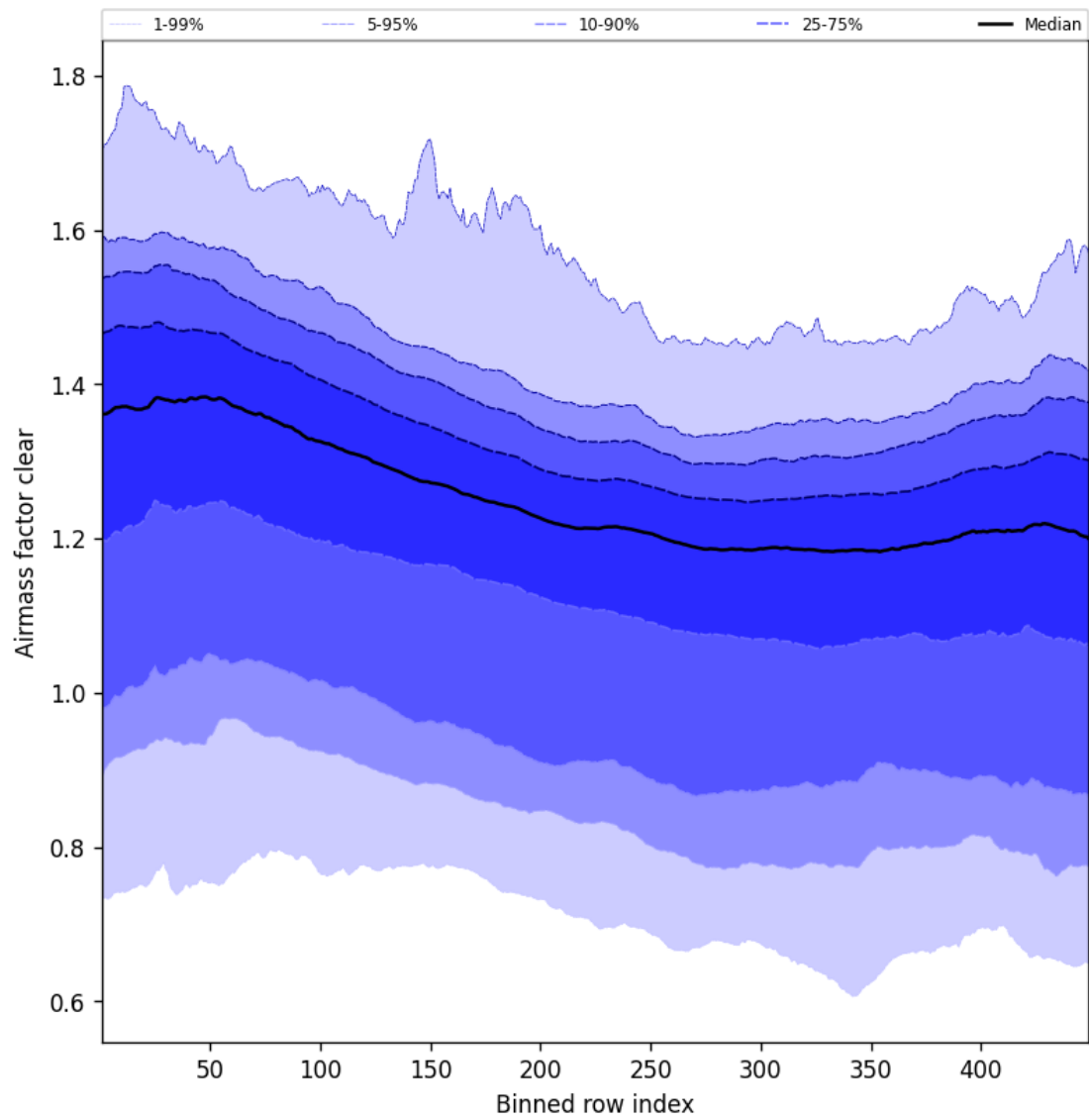
Figure 57: Along track statistics of “Airmass factor clear” for 2025-12-07 to 2025-12-07
