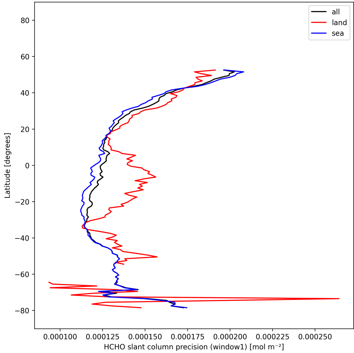
Figure 24: Zonal average of “HCHO slant column precision (window1)” for 2025-12-07 to 2025-12-07.
