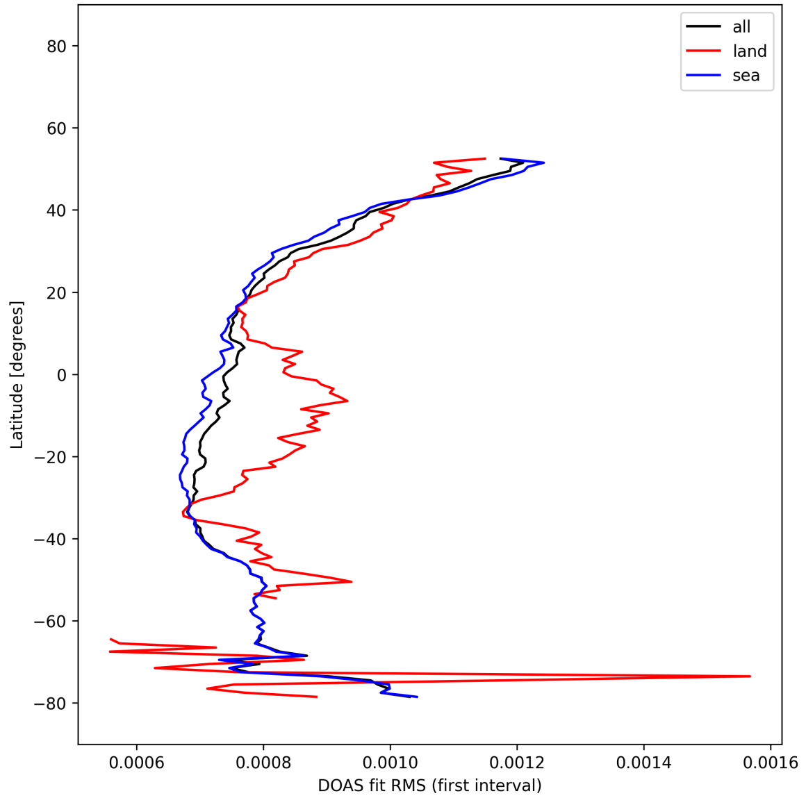
Figure 31: Zonal average of “DOAS fit RMS (first interval)” for 2025-12-07 to 2025-12-07.
