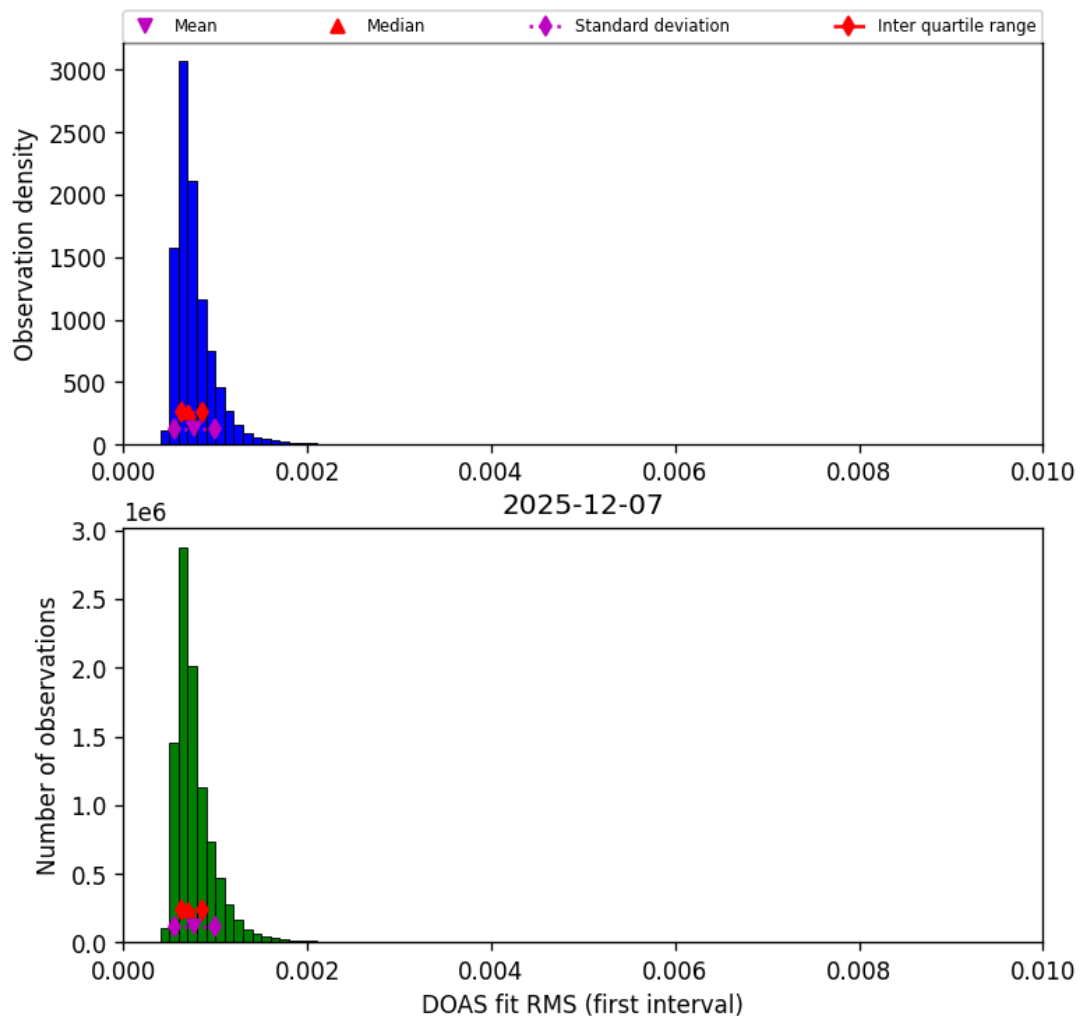
Figure 46: Histogram of “DOAS fit RMS (first interval)” for 2025-12-07 to 2025-12-07
