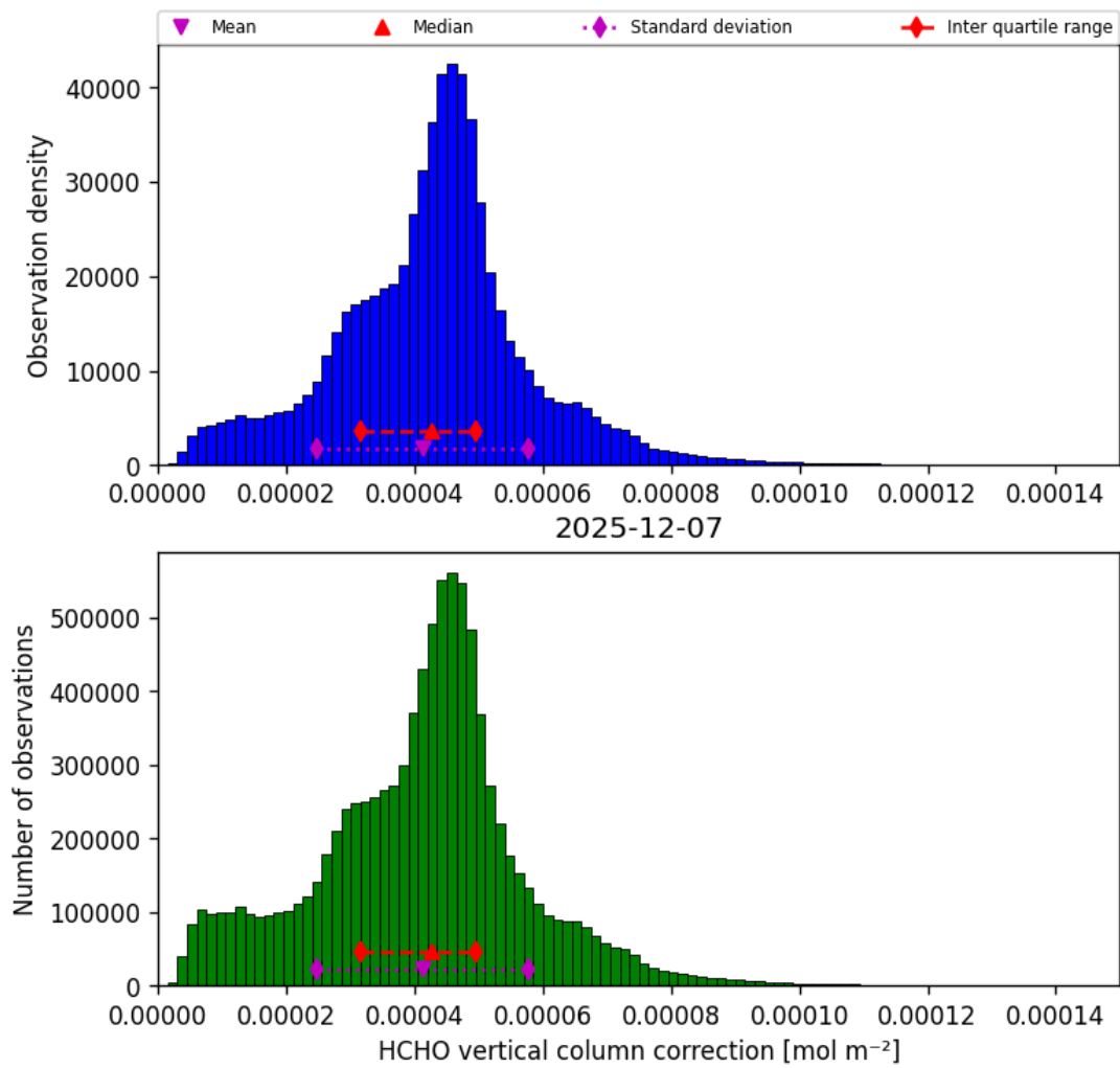
Figure 37: Histogram of “HCHO vertical column correction” for 2025-12-07 to 2025-12-07
