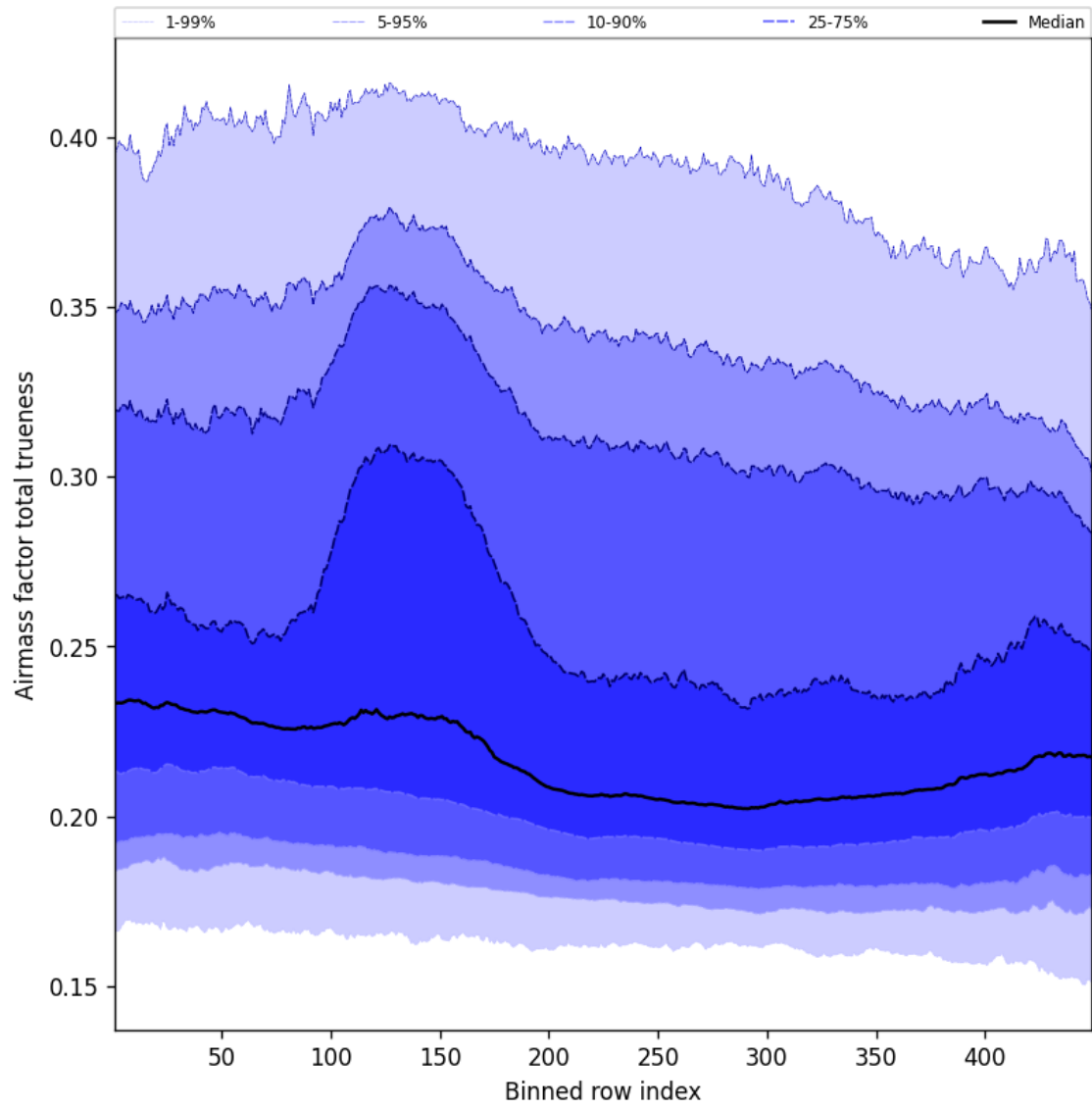
Figure 56: Along track statistics of “Airmass factor total trueness” for 2025-12-07 to 2025-12-07
