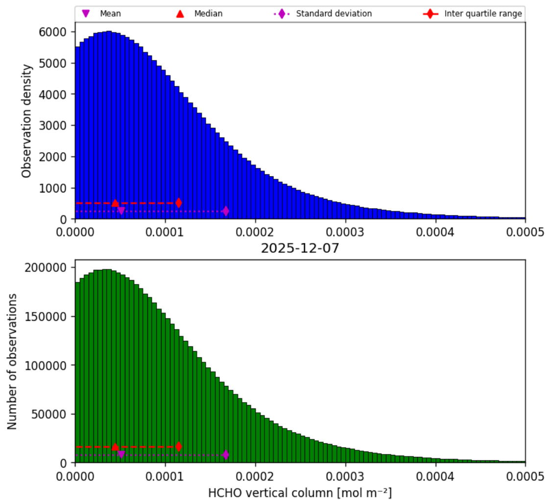
Figure 35: Histogram of “HCHO vertical column” for 2025-12-07 to 2025-12-07
