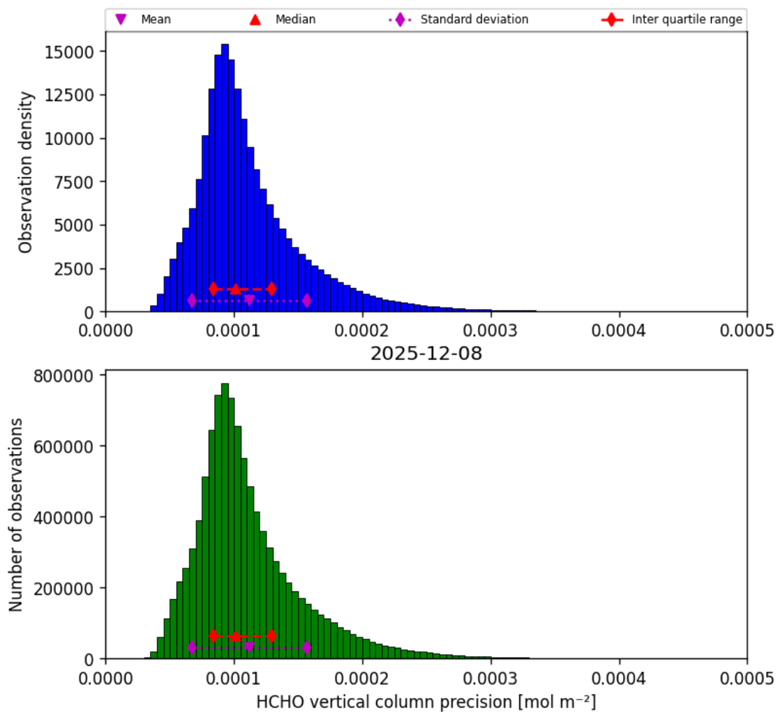
Figure 36: Histogram of “HCHO vertical column precision” for 2025-12-08 to 2025-12-09
