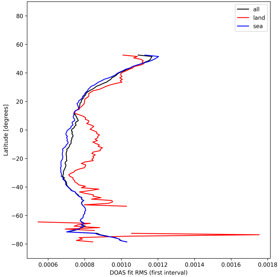
Figure 31: Zonal average of “DOAS fit RMS (first interval)” for 2025-12-08 to 2025-12-09.
