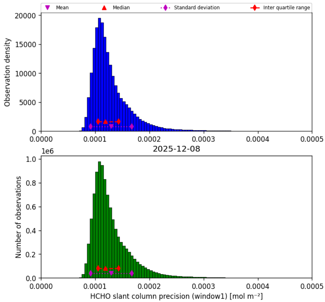
Figure 39: Histogram of “HCHO slant column precision (window1)” for 2025-12-08 to 2025-12-09
