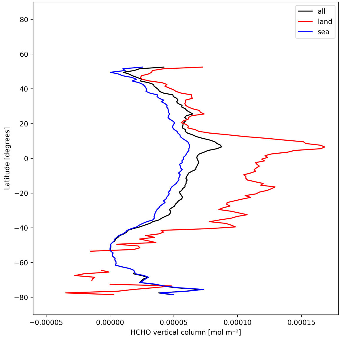
Figure 20: Zonal average of “HCHO vertical column” for 2025-12-08 to 2025-12-09.
