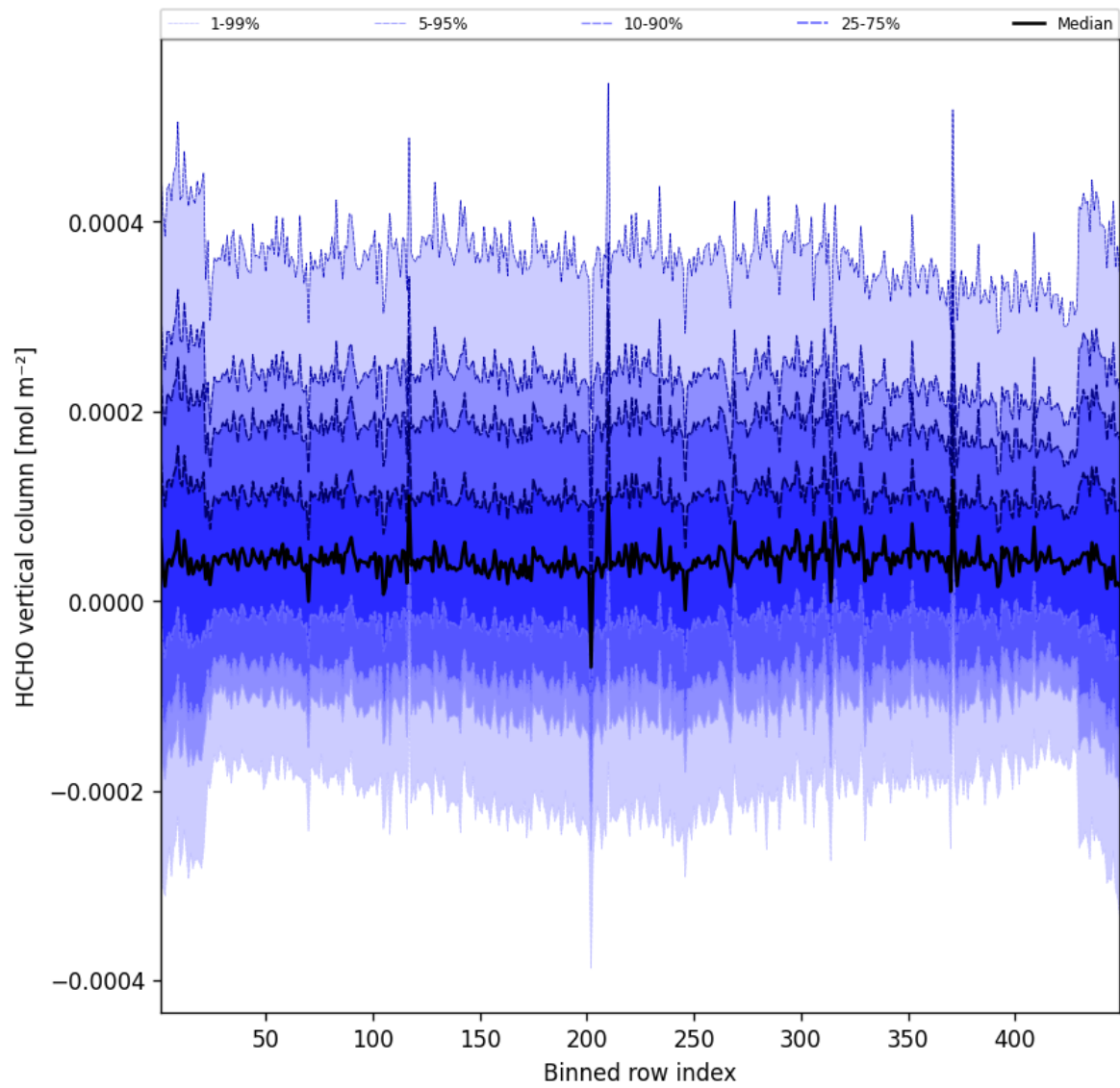
Figure 50: Along track statistics of “HCHO vertical column” for 2025-12-08 to 2025-12-09
