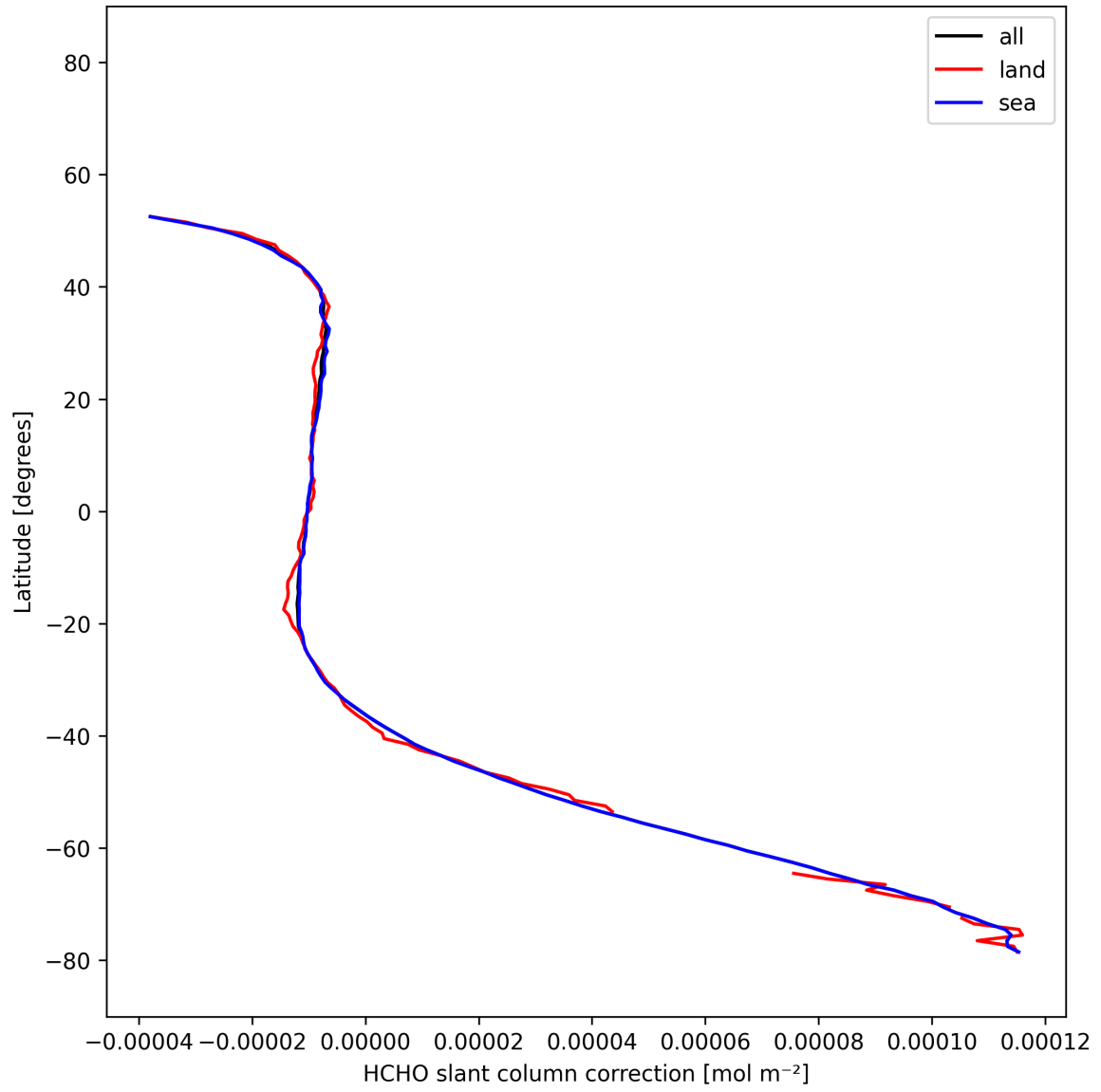
Figure 32: Zonal average of “HCHO slant column correction” for 2025-12-08 to 2025-12-09.
