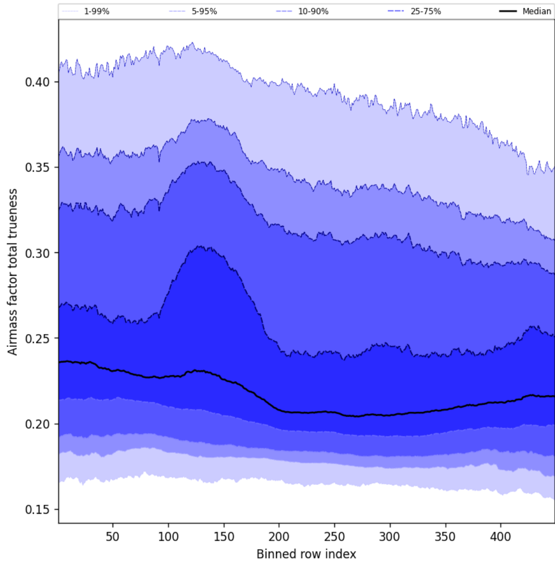
Figure 56: Along track statistics of “Airmass factor total trueness” for 2025-12-08 to 2025-12-09
