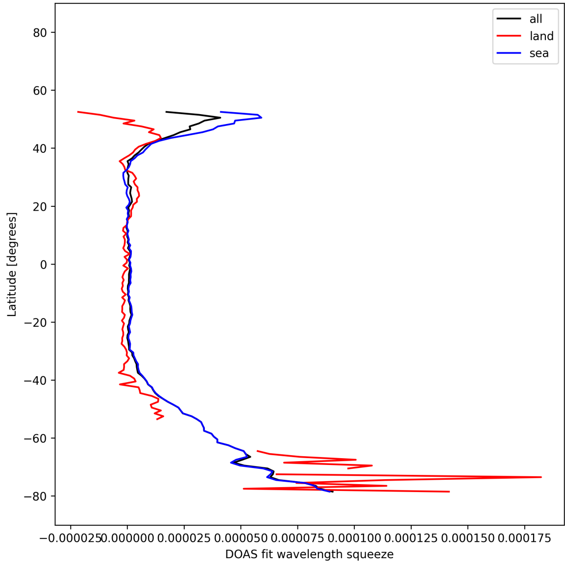
Figure 30: Zonal average of “DOAS fit wavelength squeeze” for 2025-12-08 to 2025-12-09.
