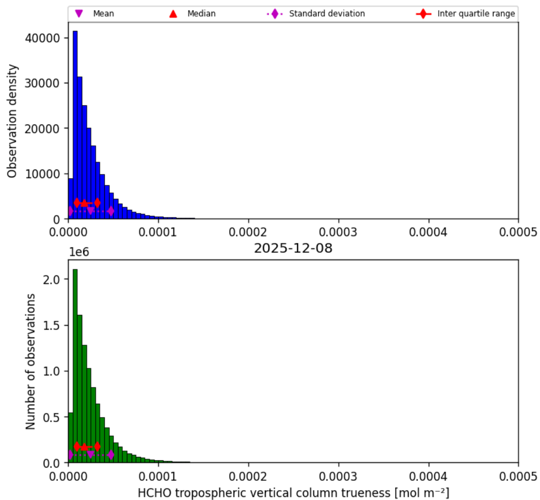
Figure 48: Histogram of “HCHO tropospheric vertical column trueness” for 2025-12-08 to 2025-12-09
