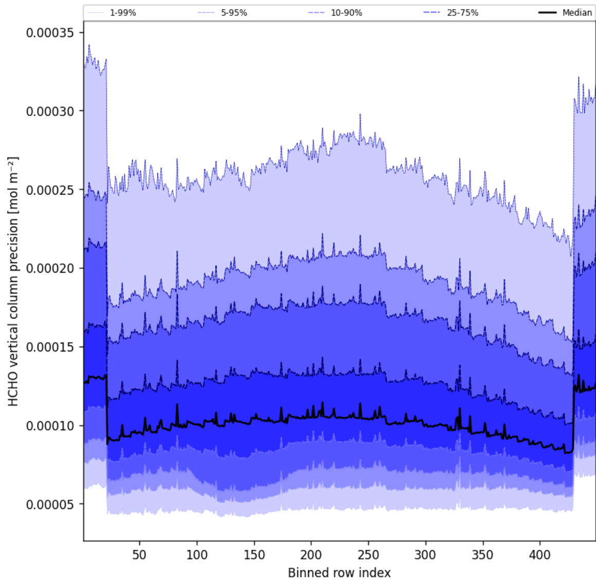
Figure 51: Along track statistics of “HCHO vertical column precision” for 2025-12-08 to 2025-12-09
