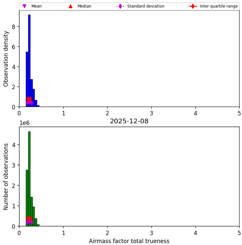
Figure 41: Histogram of “Airmass factor total trueness” for 2025-12-08 to 2025-12-09
