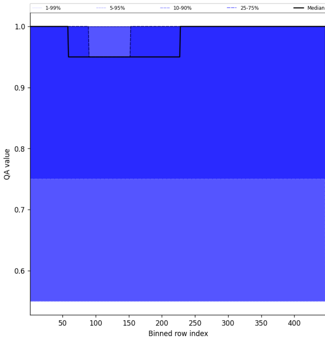
Figure 49: Along track statistics of “QA value” for 2025-12-08 to 2025-12-09
