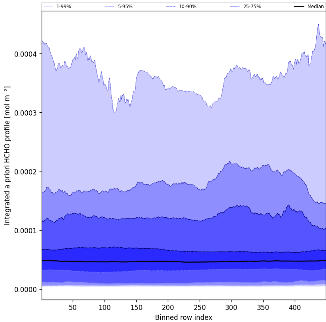
Figure 58: Along track statistics of “Integrated a priori HCHO profile” for 2025-12-08 to 2025-12-09
