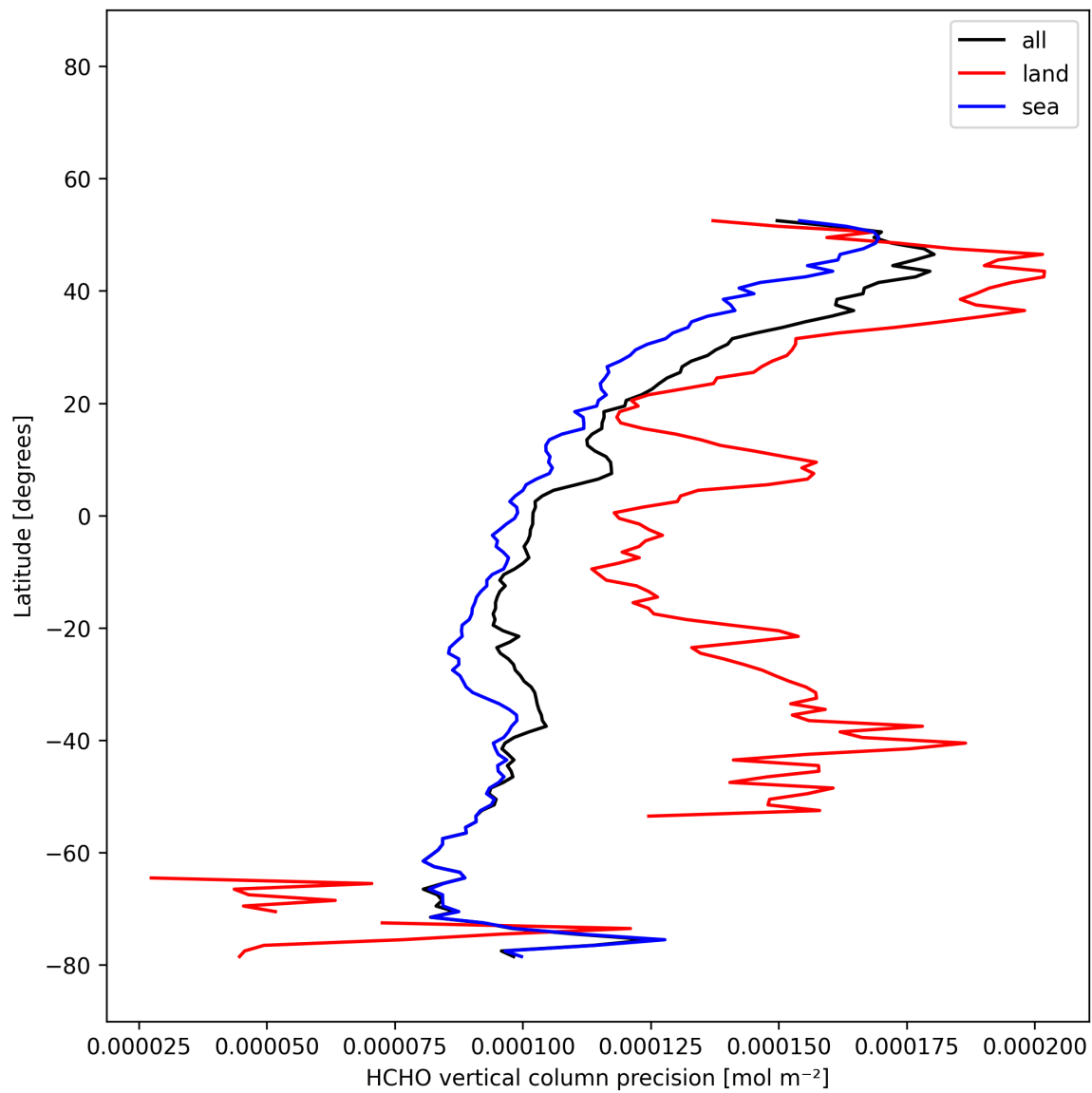
Figure 21: Zonal average of “HCHO vertical column precision” for 2025-12-08 to 2025-12-09.
