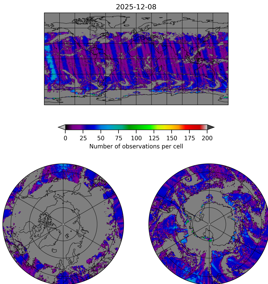
Figure 18: Map of the number of observations for 2025-12-08 to 2025-12-09
