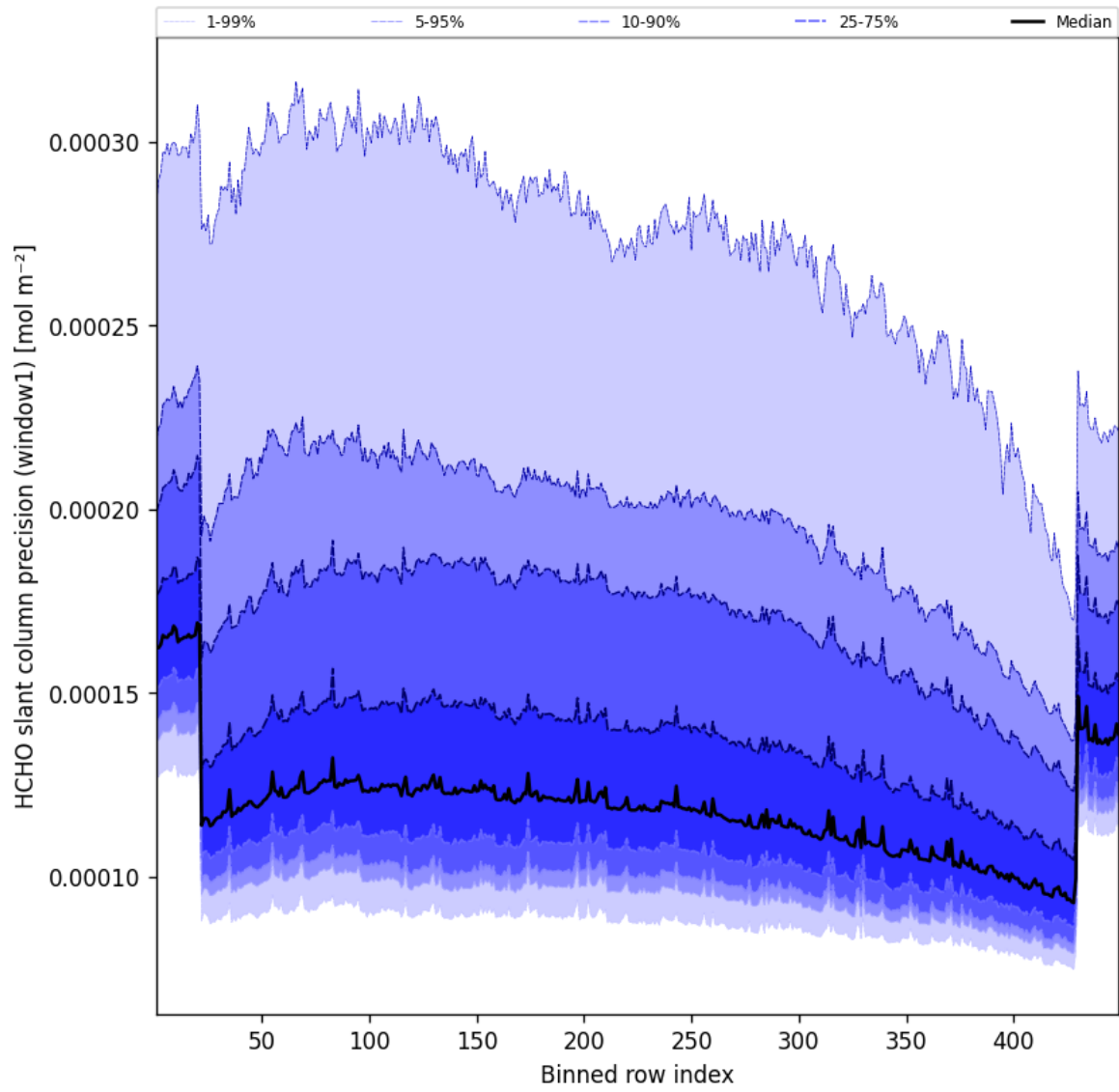
Figure 54: Along track statistics of “HCHO slant column precision (window1)” for 2025-12-08 to 2025-12-09
