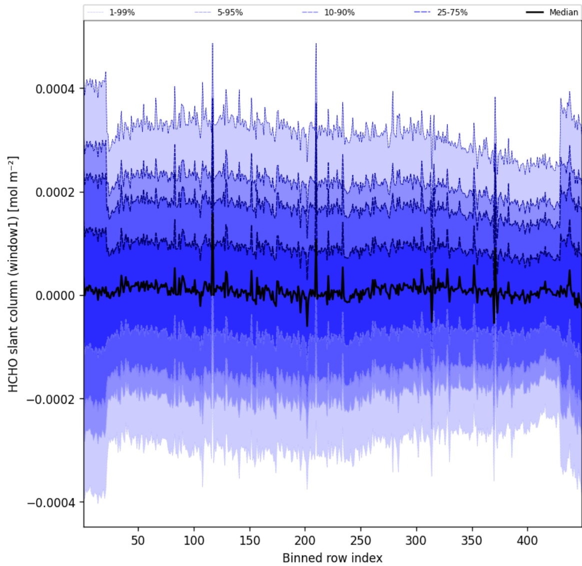
Figure 53: Along track statistics of “HCHO slant column (window1)” for 2025-12-08 to 2025-12-09
