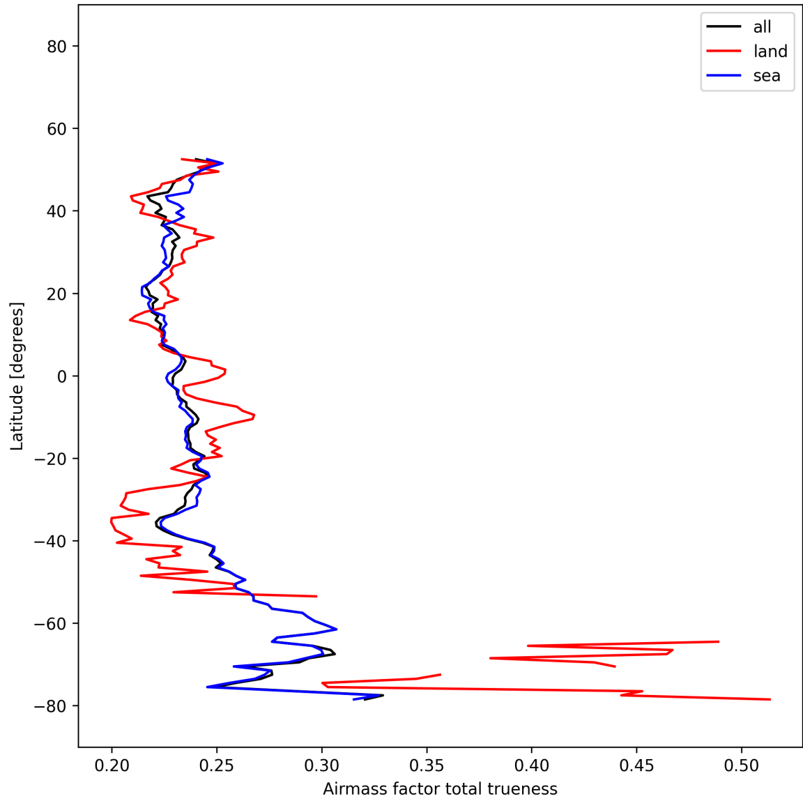
Figure 26: Zonal average of “Airmass factor total trueness” for 2025-12-08 to 2025-12-09.
