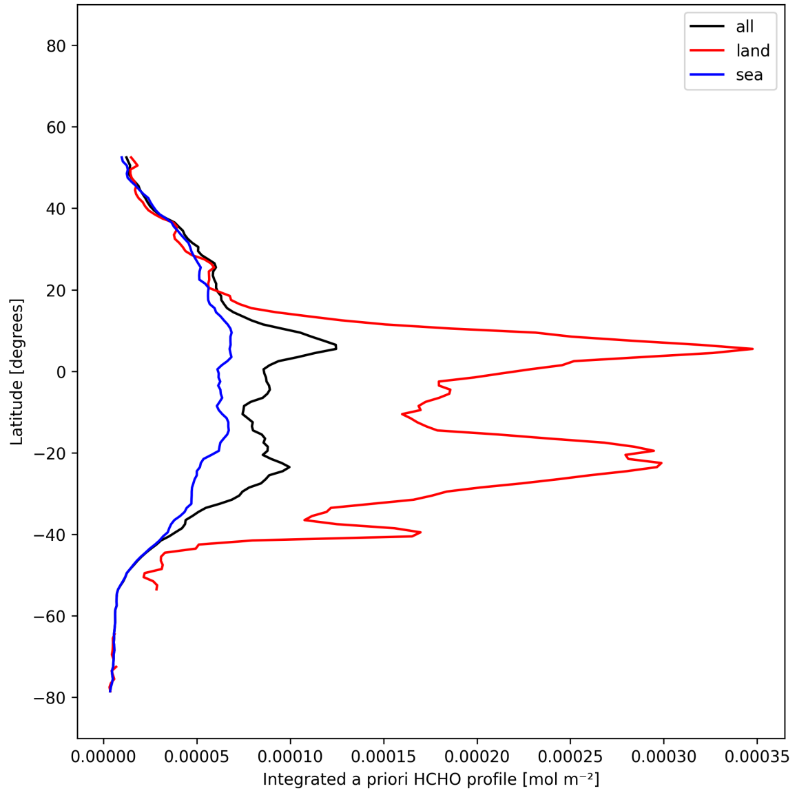
Figure 28: Zonal average of “Integrated a priori HCHO profile” for 2025-12-08 to 2025-12-09.
