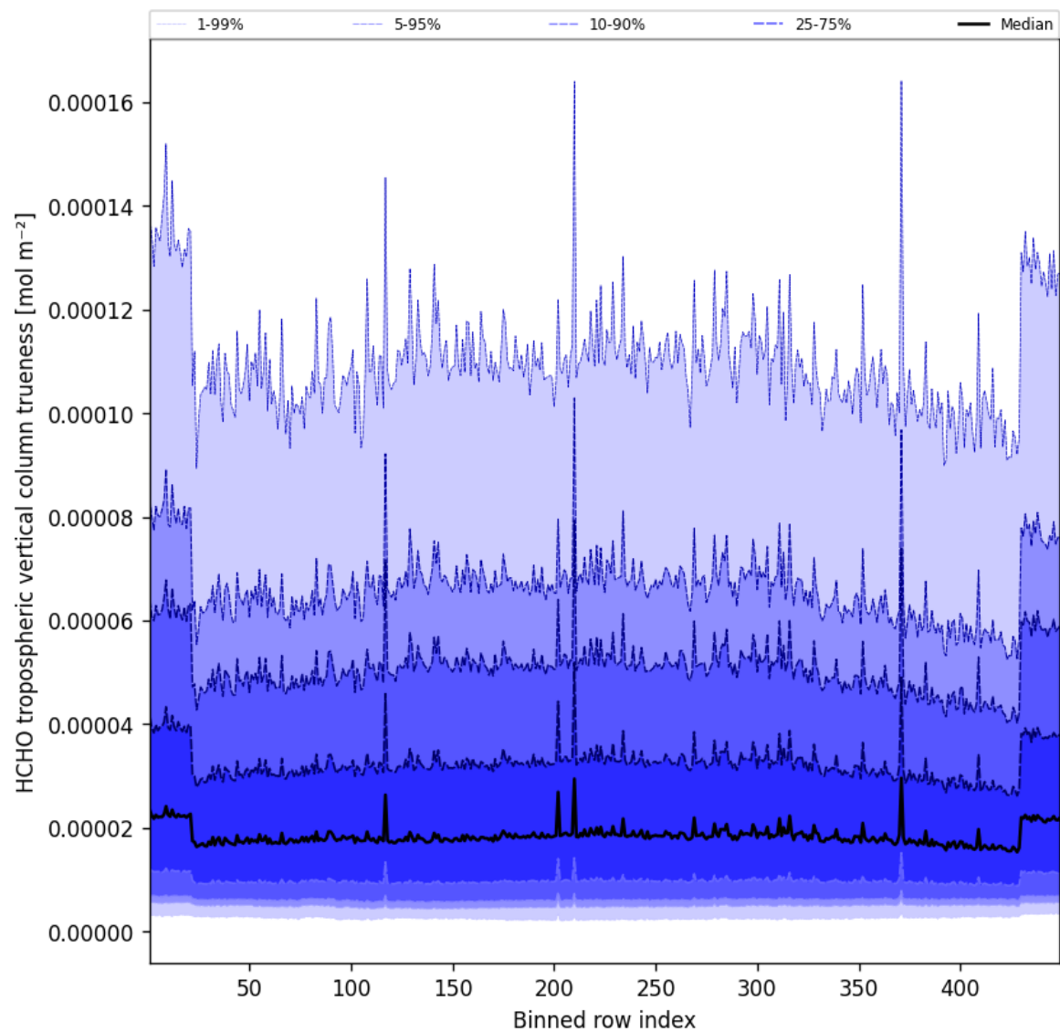
Figure 63: Along track statistics of “HCHO tropospheric vertical column trueness” for 2025-12-08 to 2025-12-09
