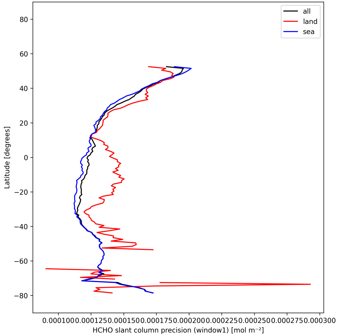
Figure 24: Zonal average of “HCHO slant column precision (window1)” for 2025-12-08 to 2025-12-09.
