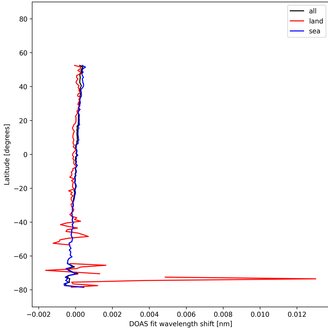
Figure 29: Zonal average of "DOAS fit wavelength shift" for 2025-12-08 to 2025-12-09.
