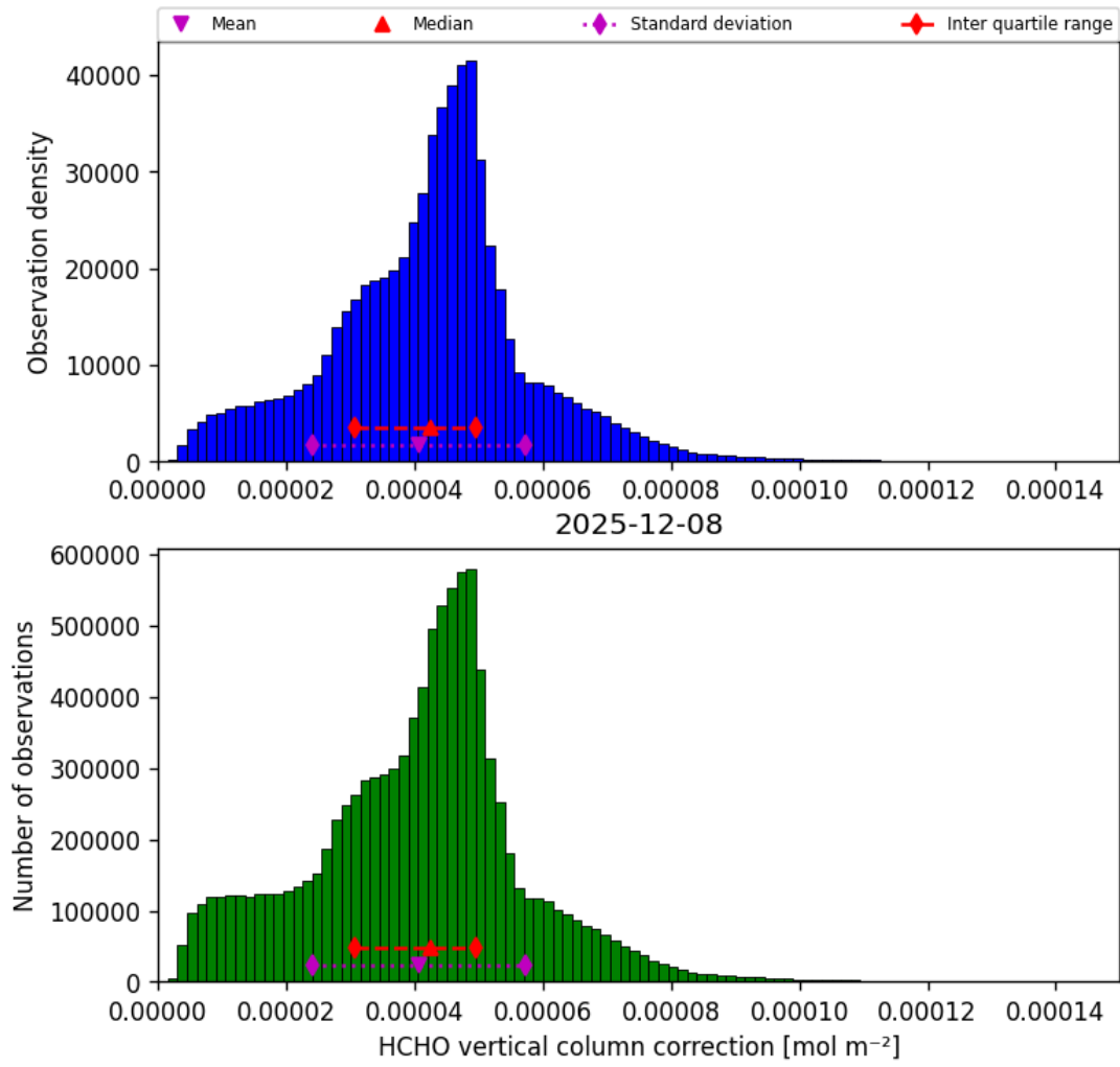
Figure 37: Histogram of “HCHO vertical column correction” for 2025-12-08 to 2025-12-09
