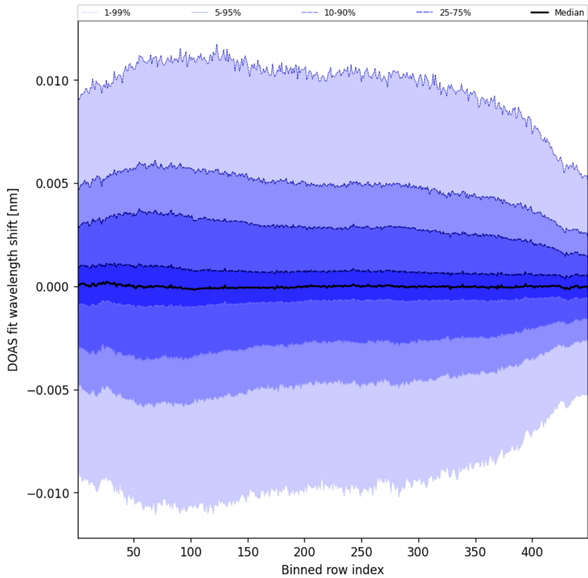
Figure 59: Along track statistics of “DOAS fit wavelength shift” for 2025-12-08 to 2025-12-09
