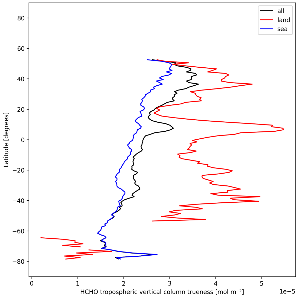
Figure 33: Zonal average of “HCHO tropospheric vertical column trueness” for 2025-12-08 to 2025-12-09.
