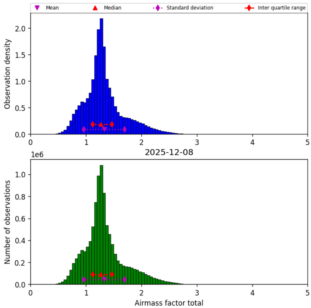
Figure 40: Histogram of “Airmass factor total” for 2025-12-08 to 2025-12-09
