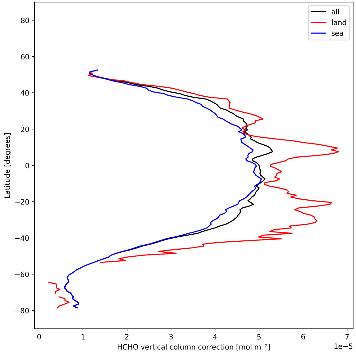
Figure 22: Zonal average of “HCHO vertical column correction” for 2025-12-08 to 2025-12-09.
