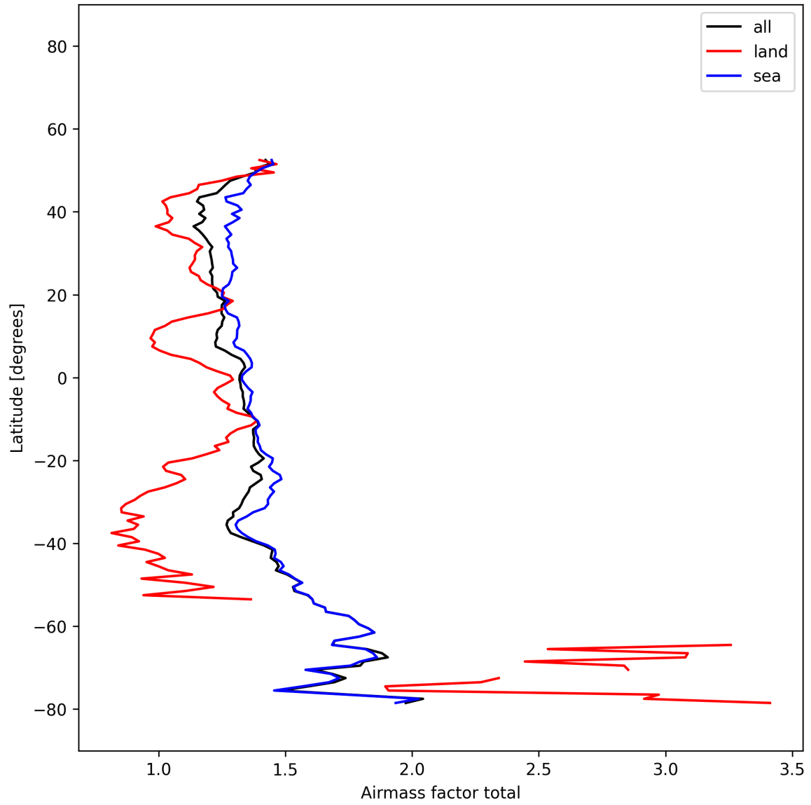
Figure 25: Zonal average of “Airmass factor total” for 2025-12-08 to 2025-12-09.
