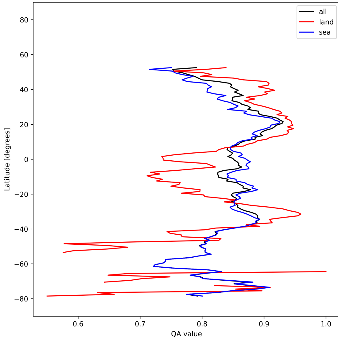
Figure 19: Zonal average of “QA value” for 2025-12-08 to 2025-12-09.
