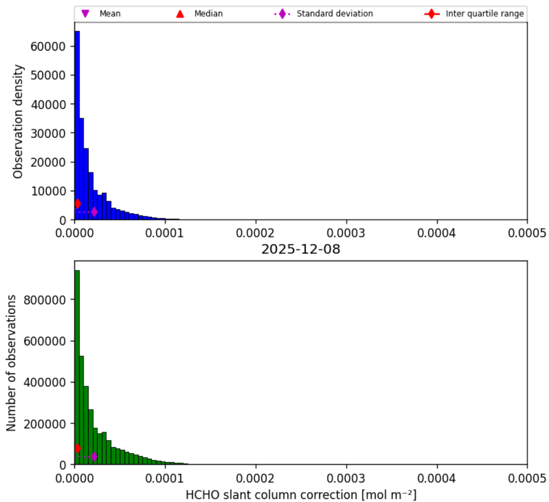
Figure 47: Histogram of “HCHO slant column correction” for 2025-12-08 to 2025-12-09
