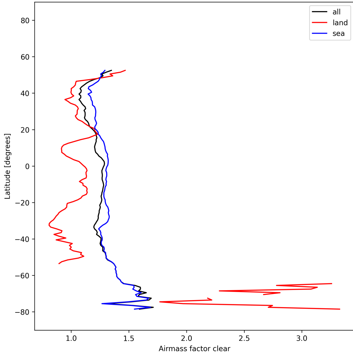
Figure 27: Zonal average of “Airmass factor clear” for 2025-12-08 to 2025-12-09.
