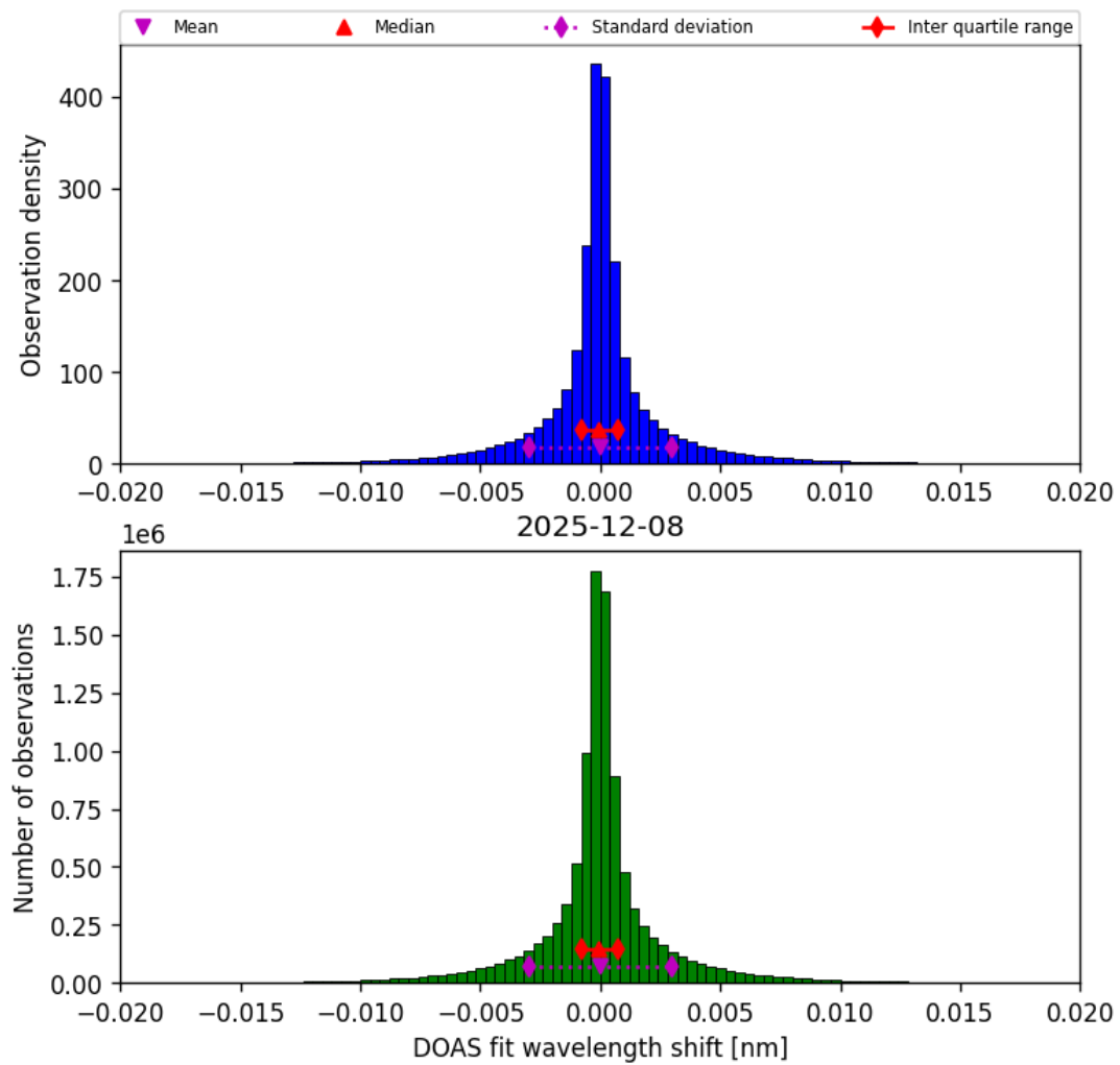
Figure 44: Histogram of “DOAS fit wavelength shift” for 2025-12-08 to 2025-12-09
