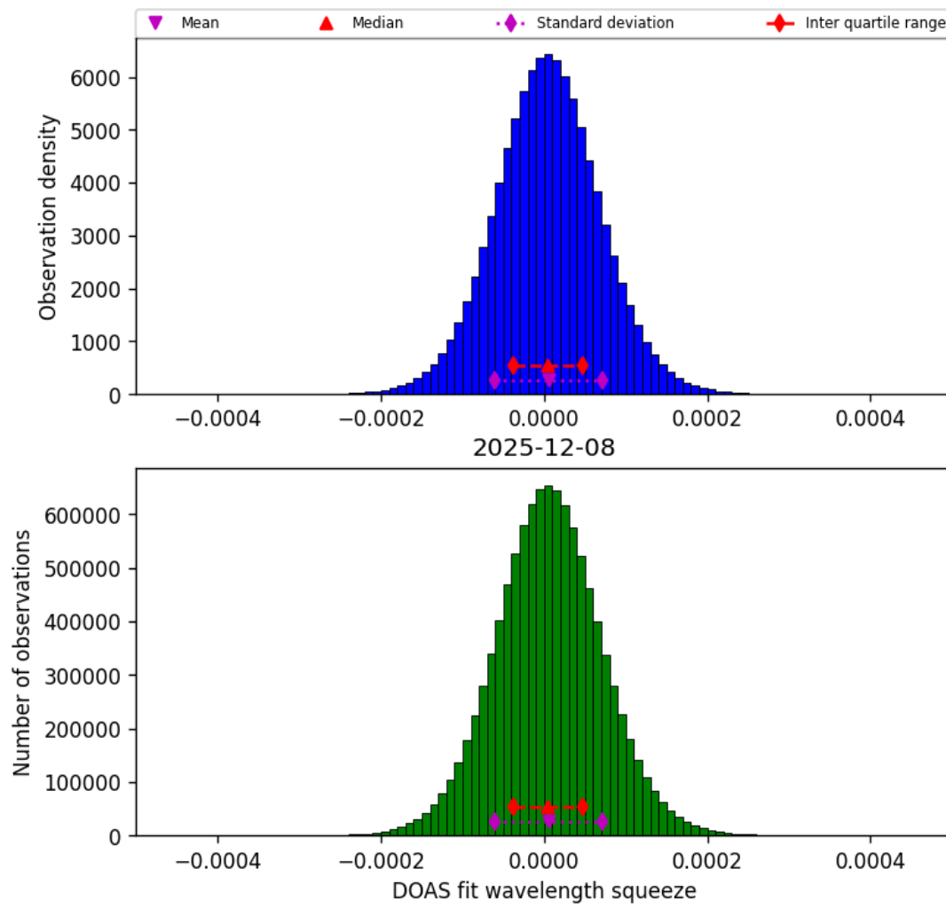
Figure 45: Histogram of “DOAS fit wavelength squeeze” for 2025-12-08 to 2025-12-09
