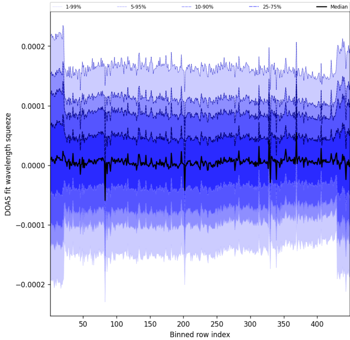
Figure 60: Along track statistics of “DOAS fit wavelength squeeze” for 2025-12-08 to 2025-12-09
