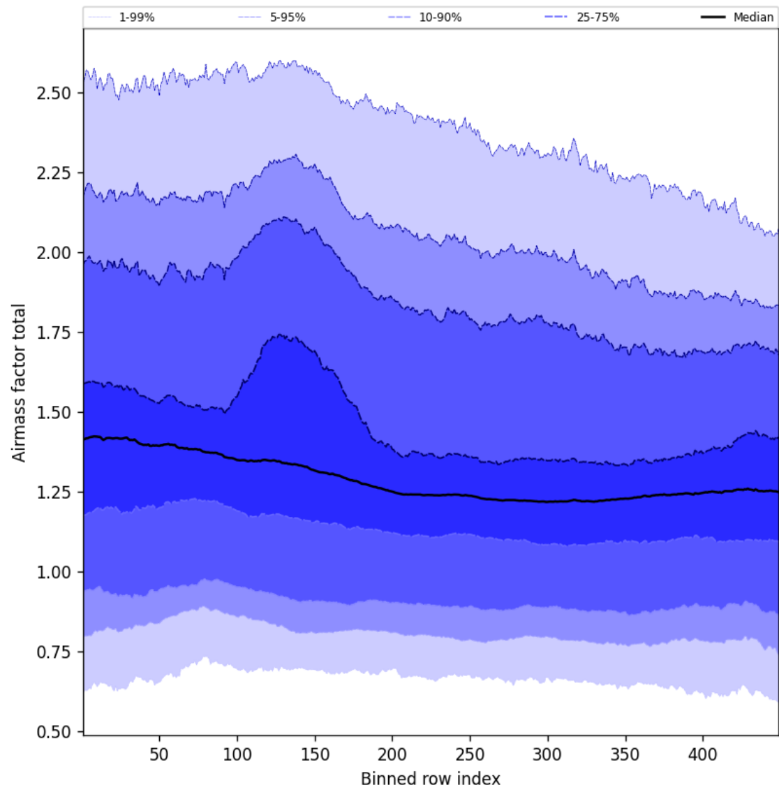
Figure 55: Along track statistics of “Airmass factor total” for 2025-12-08 to 2025-12-09
