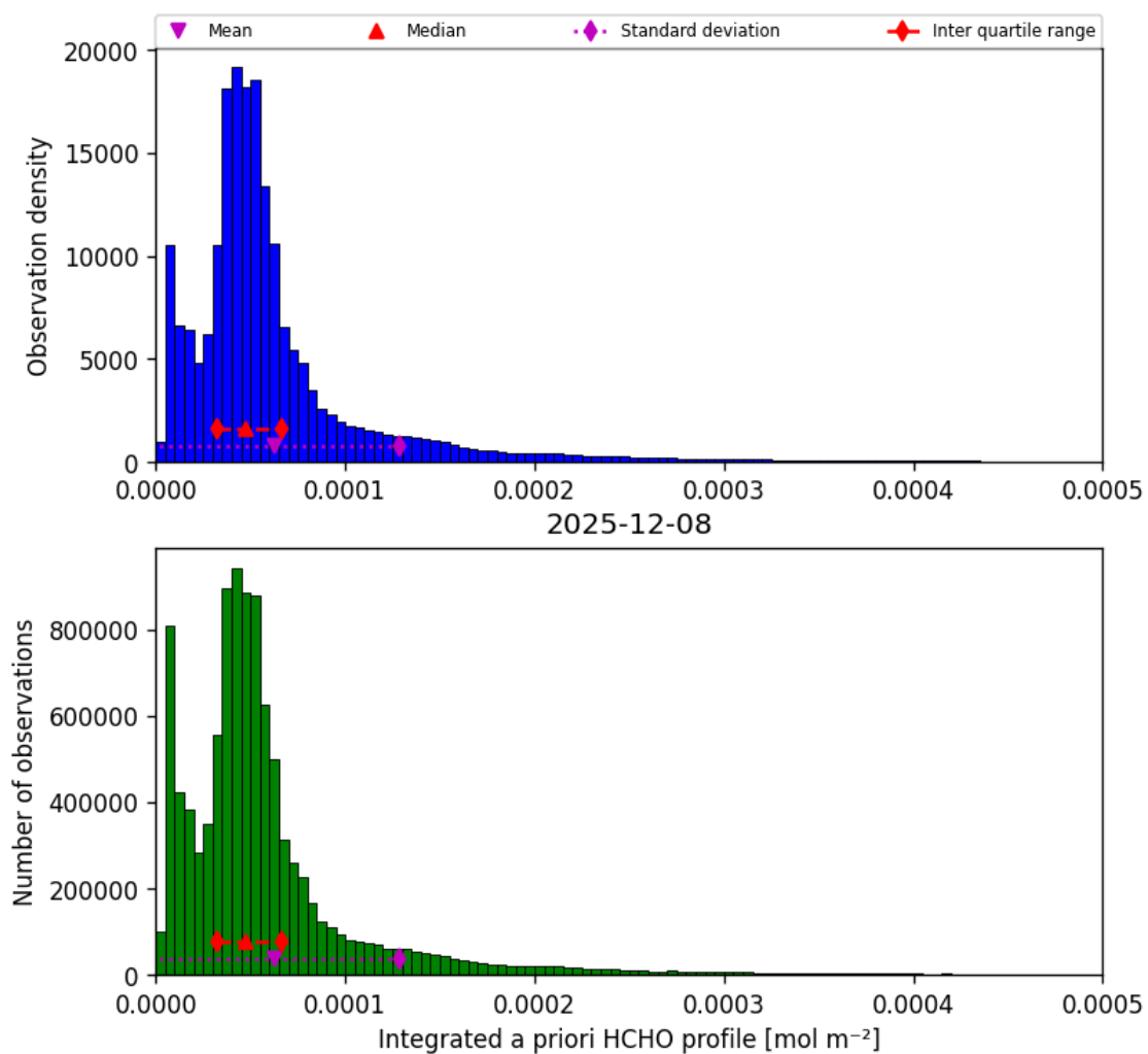
Figure 43: Histogram of “Integrated a priori HCHO profile” for 2025-12-08 to 2025-12-09
