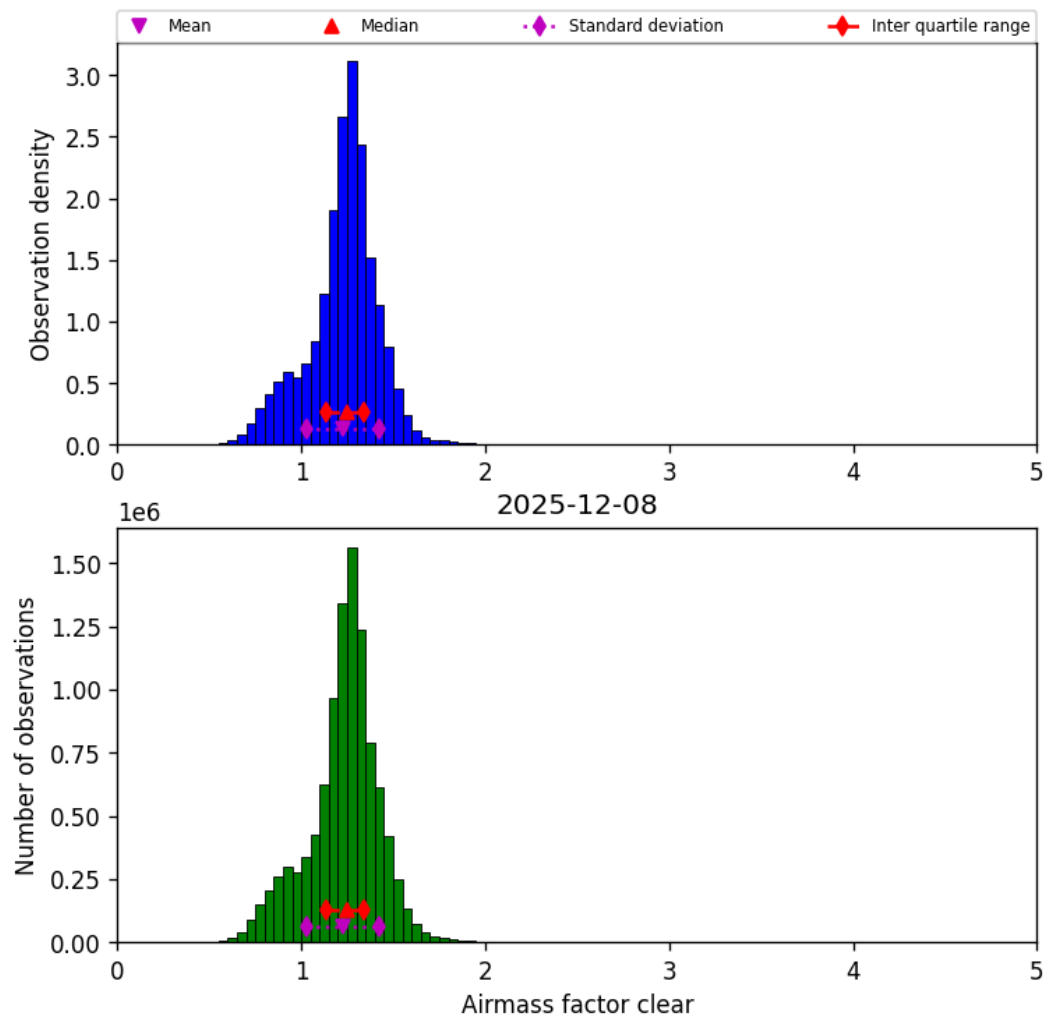
Figure 42: Histogram of “Airmass factor clear” for 2025-12-08 to 2025-12-09
