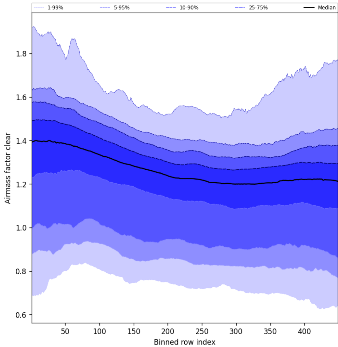
Figure 57: Along track statistics of “Airmass factor clear” for 2025-12-08 to 2025-12-09
