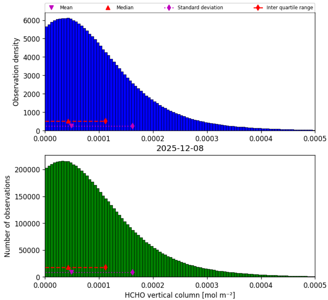
Figure 35: Histogram of “HCHO vertical column” for 2025-12-08 to 2025-12-09
