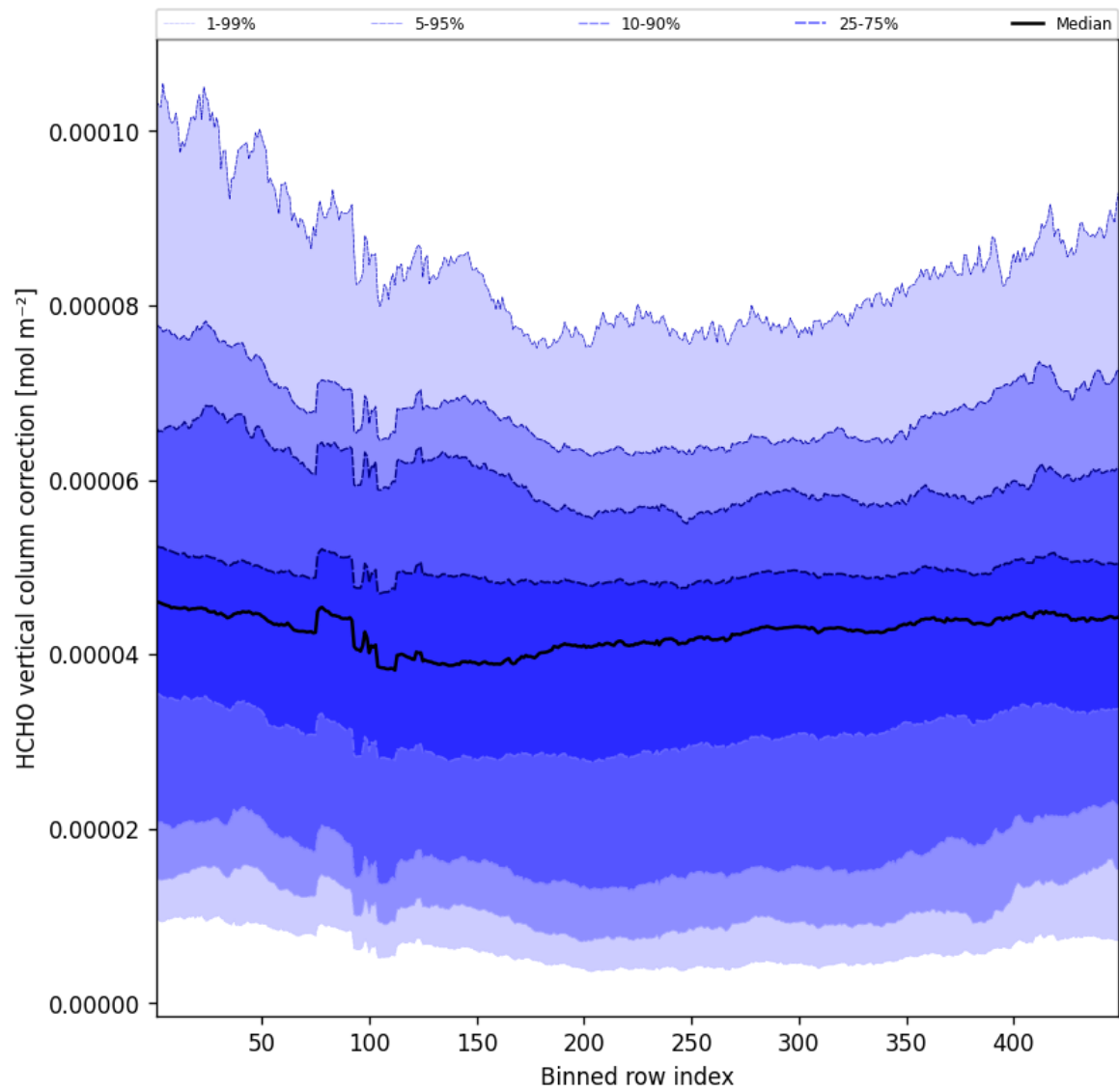
Figure 52: Along track statistics of “HCHO vertical column correction” for 2025-12-08 to 2025-12-09
