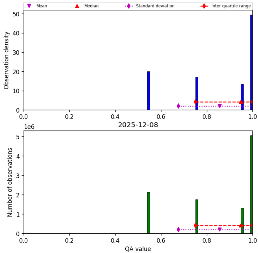
Figure 34: Histogram of “QA value” for 2025-12-08 to 2025-12-09
