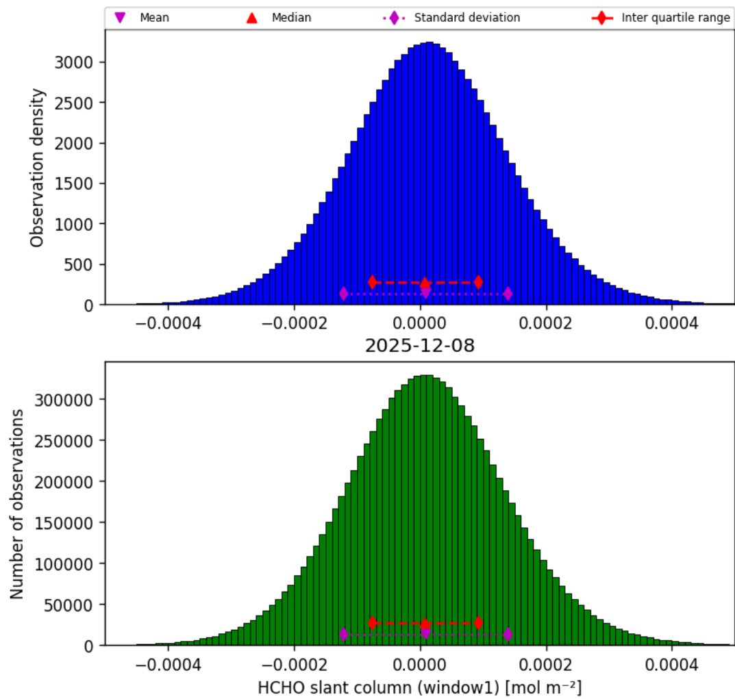
Figure 38: Histogram of “HCHO slant column (window1)” for 2025-12-08 to 2025-12-09
