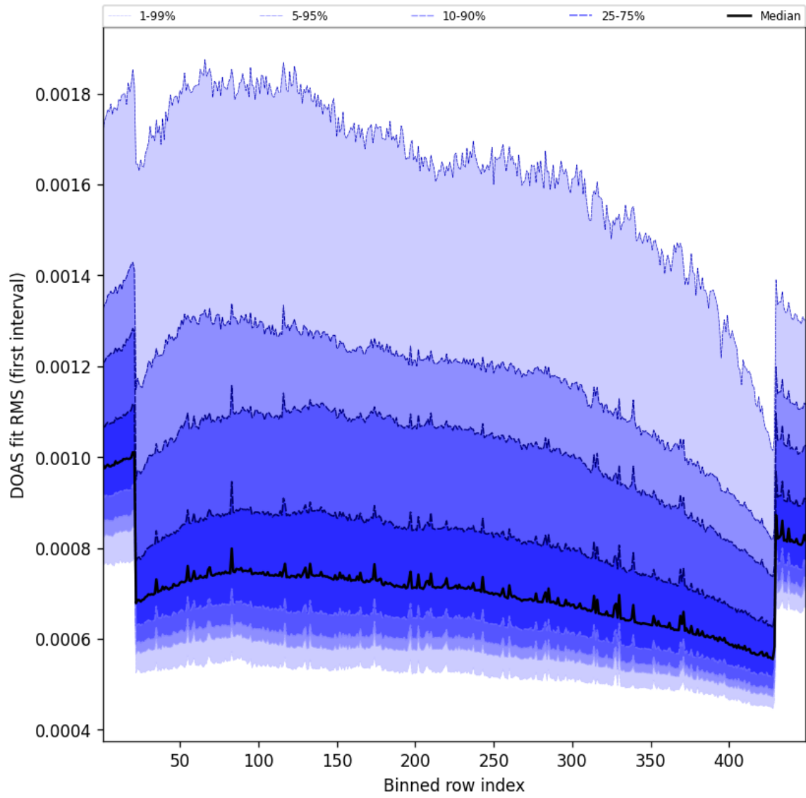
Figure 61: Along track statistics of “DOAS fit RMS (first interval)” for 2025-12-08 to 2025-12-09
