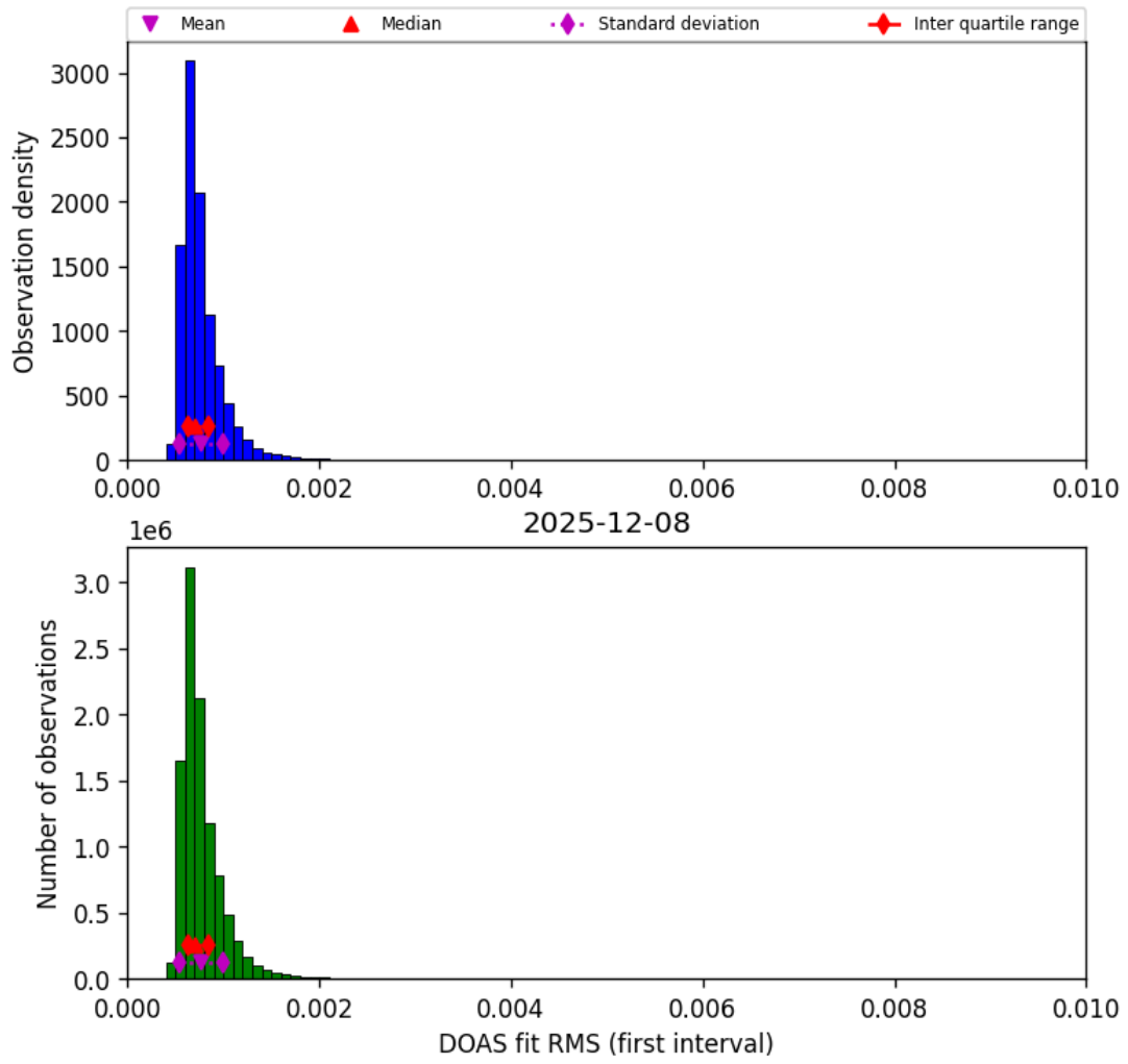
Figure 46: Histogram of “DOAS fit RMS (first interval)” for 2025-12-08 to 2025-12-09
