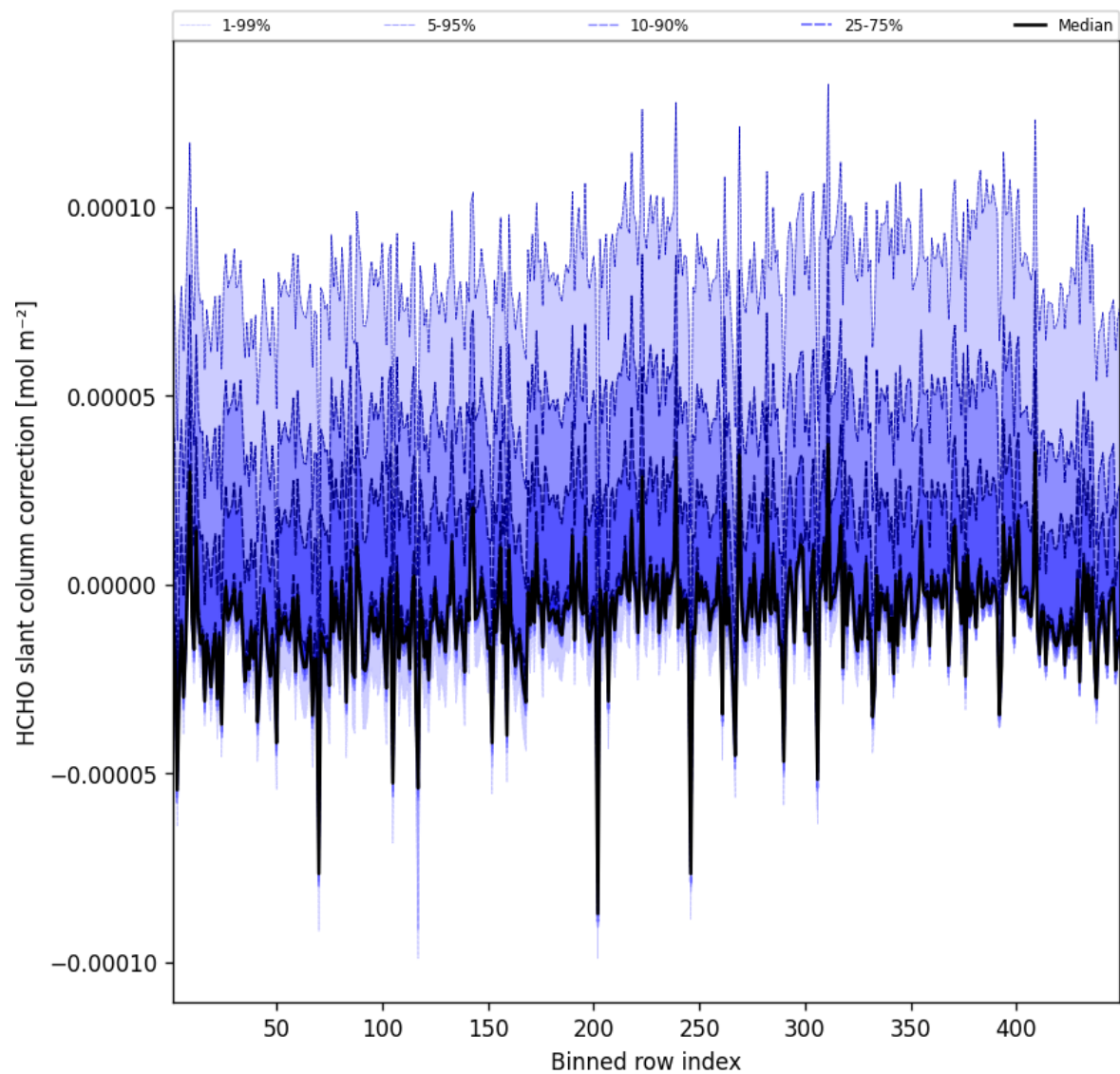
Figure 62: Along track statistics of “HCHO slant column correction” for 2025-12-08 to 2025-12-09
