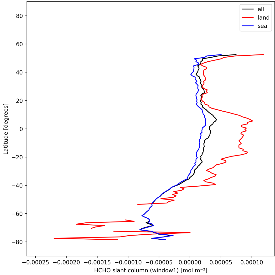
Figure 23: Zonal average of “HCHO slant column (window1)” for 2025-12-08 to 2025-12-09.
