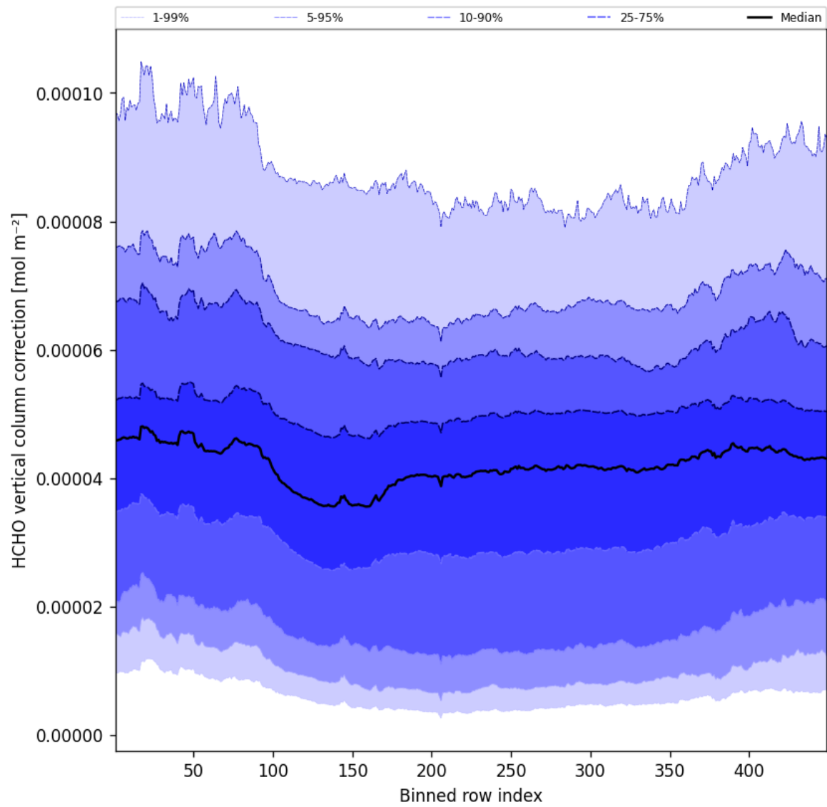
Figure 52: Along track statistics of “HCHO vertical column correction” for 2025-12-09 to 2025-12-10
