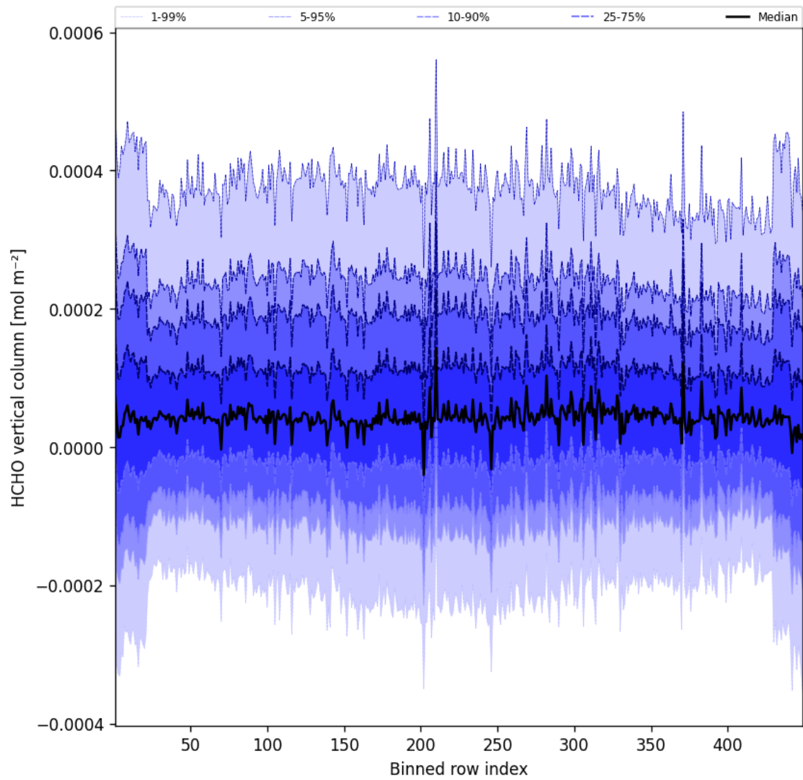
Figure 50: Along track statistics of “HCHO vertical column” for 2025-12-09 to 2025-12-10
