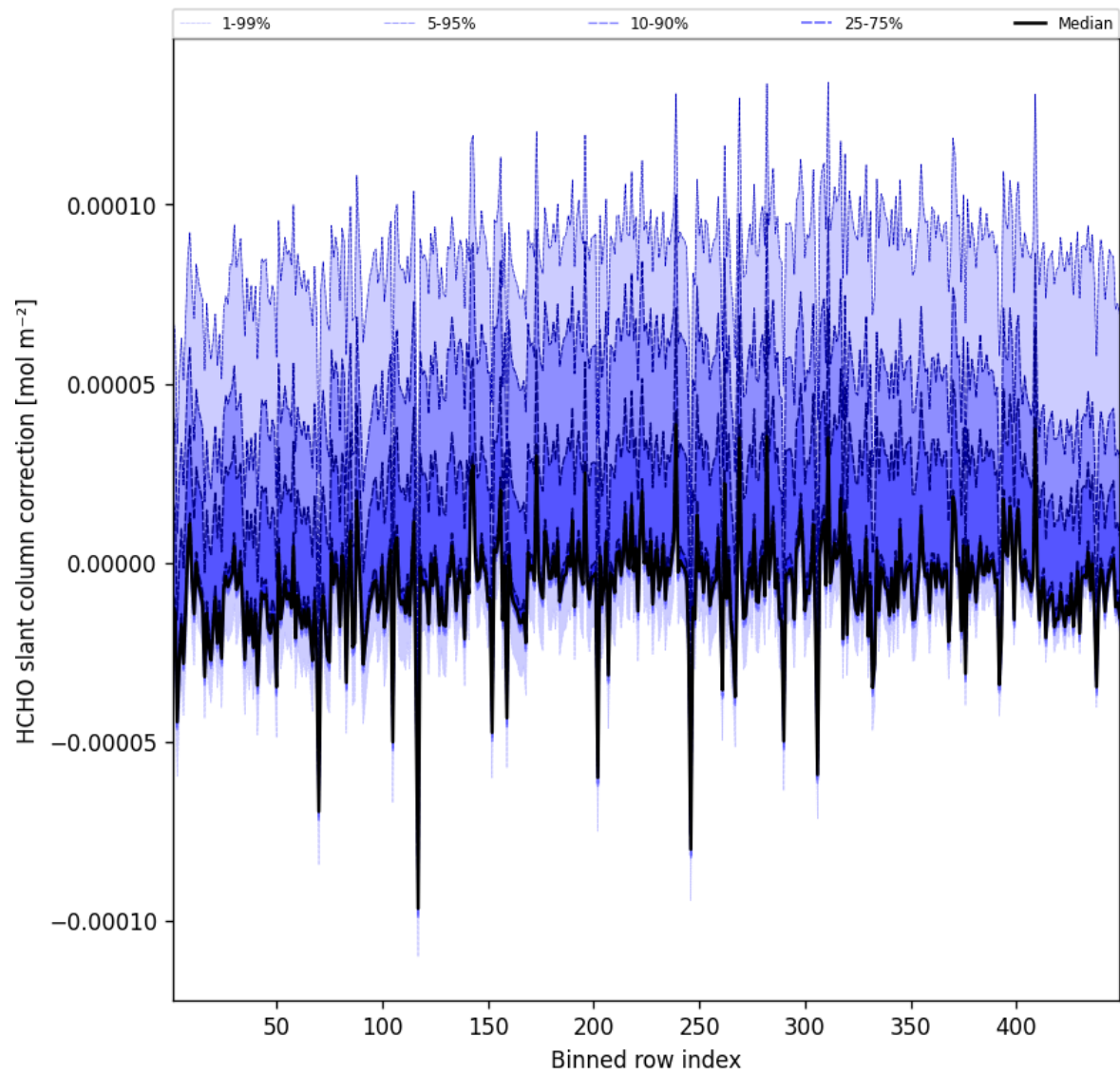
Figure 62: Along track statistics of “HCHO slant column correction” for 2025-12-09 to 2025-12-10
