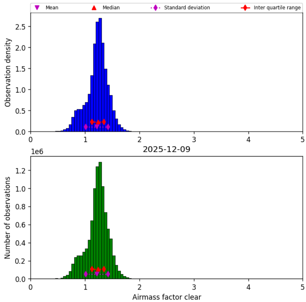
Figure 42: Histogram of “Airmass factor clear” for 2025-12-09 to 2025-12-10
