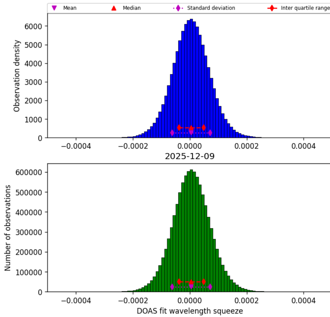
Figure 45: Histogram of “DOAS fit wavelength squeeze” for 2025-12-09 to 2025-12-10
