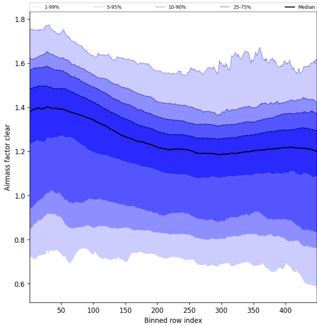
Figure 57: Along track statistics of “Airmass factor clear” for 2025-12-09 to 2025-12-10
