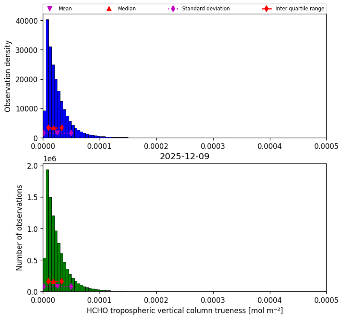
Figure 48: Histogram of “HCHO tropospheric vertical column trueness” for 2025-12-09 to 2025-12-10
