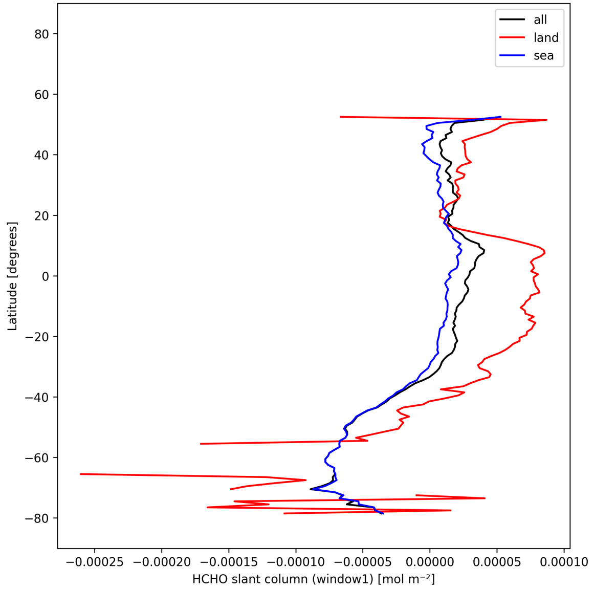
Figure 23: Zonal average of “HCHO slant column (window1)” for 2025-12-09 to 2025-12-10.
