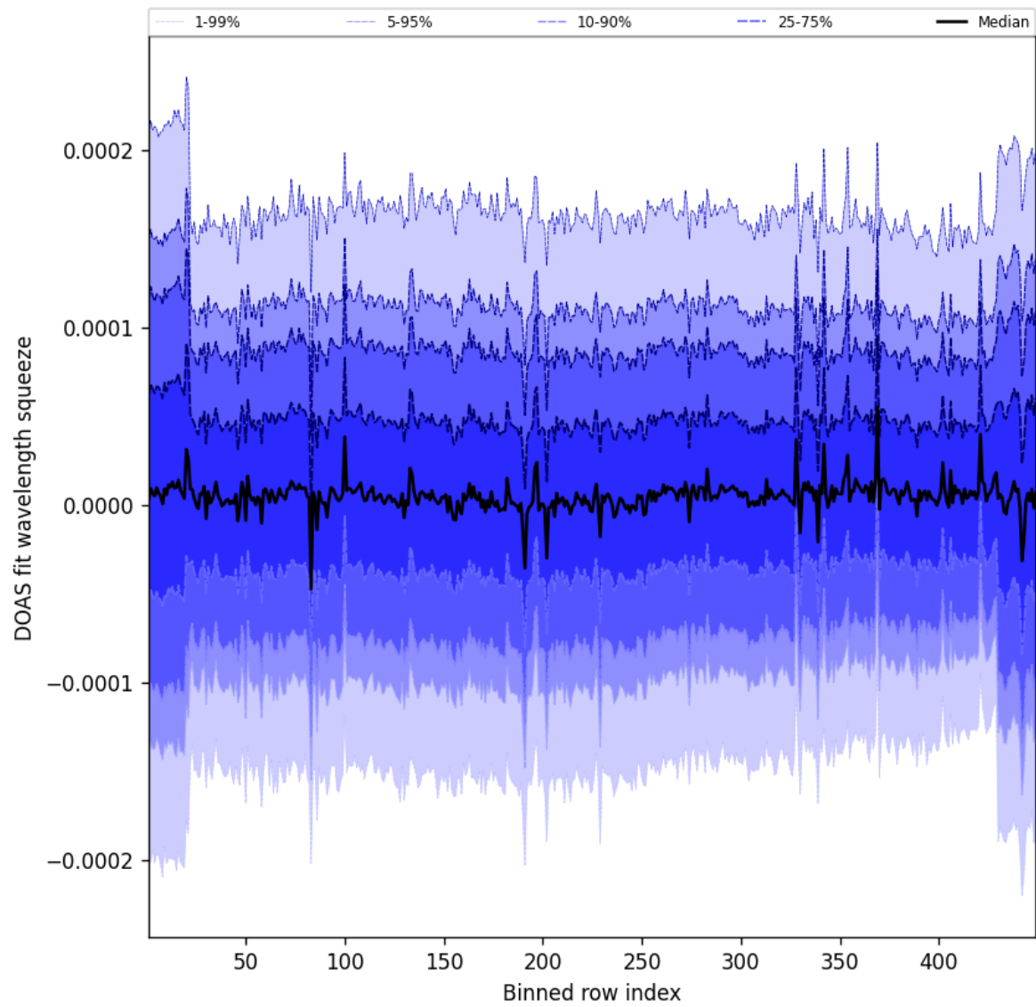
Figure 60: Along track statistics of “DOAS fit wavelength squeeze” for 2025-12-09 to 2025-12-10
