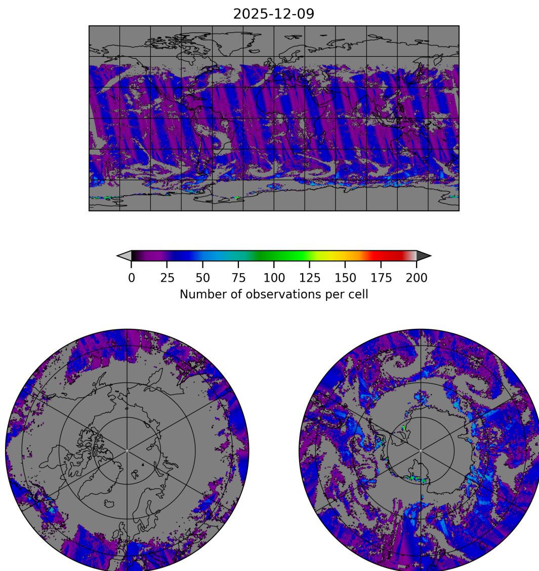
Figure 18: Map of the number of observations for 2025-12-09 to 2025-12-10
