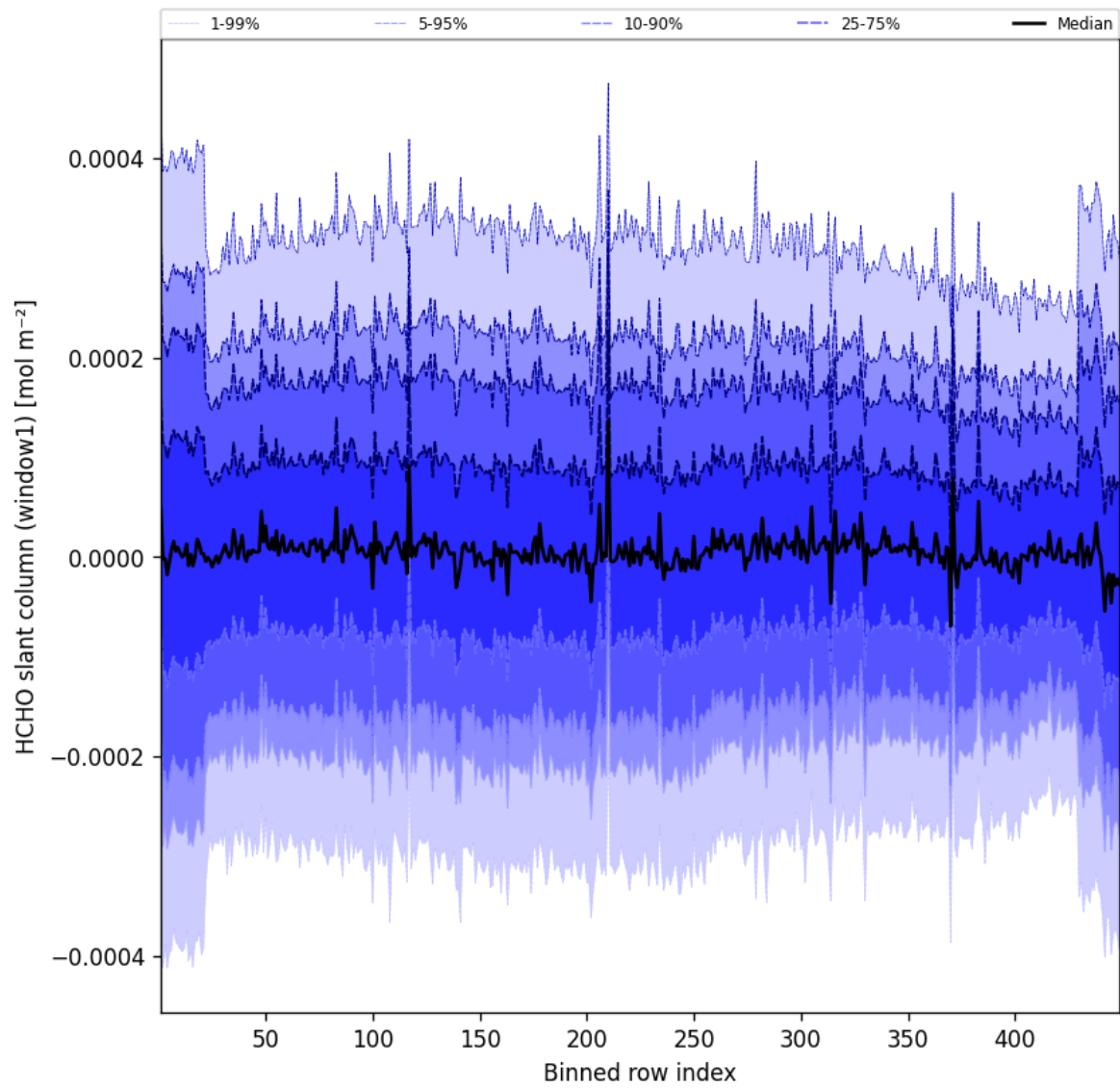
Figure 53: Along track statistics of “HCHO slant column (window1)” for 2025-12-09 to 2025-12-10
