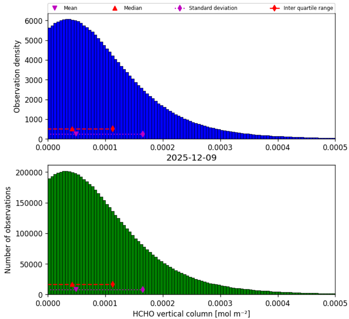
Figure 35: Histogram of “HCHO vertical column” for 2025-12-09 to 2025-12-10
