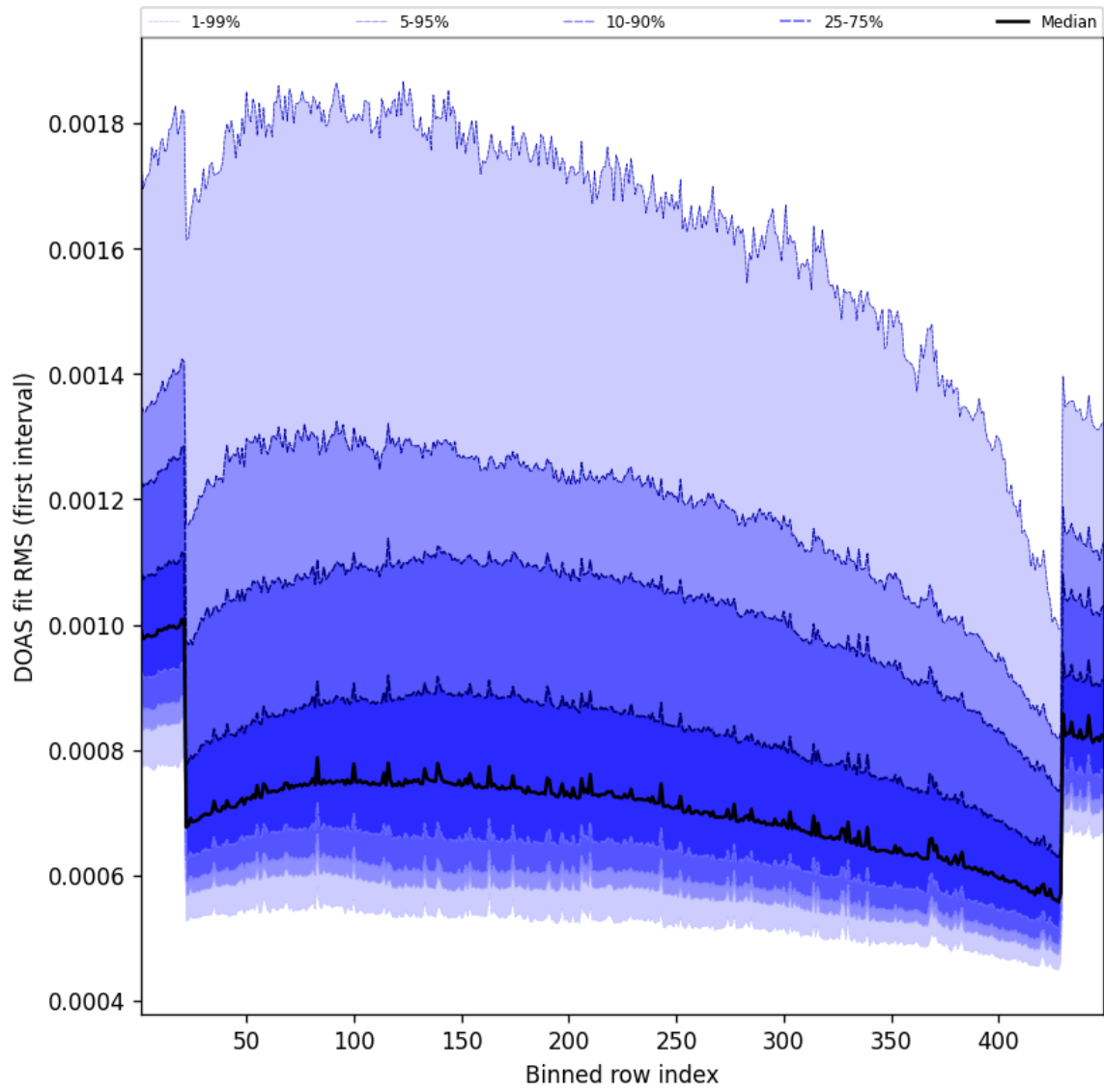
Figure 61: Along track statistics of “DOAS fit RMS (first interval)” for 2025-12-09 to 2025-12-10
