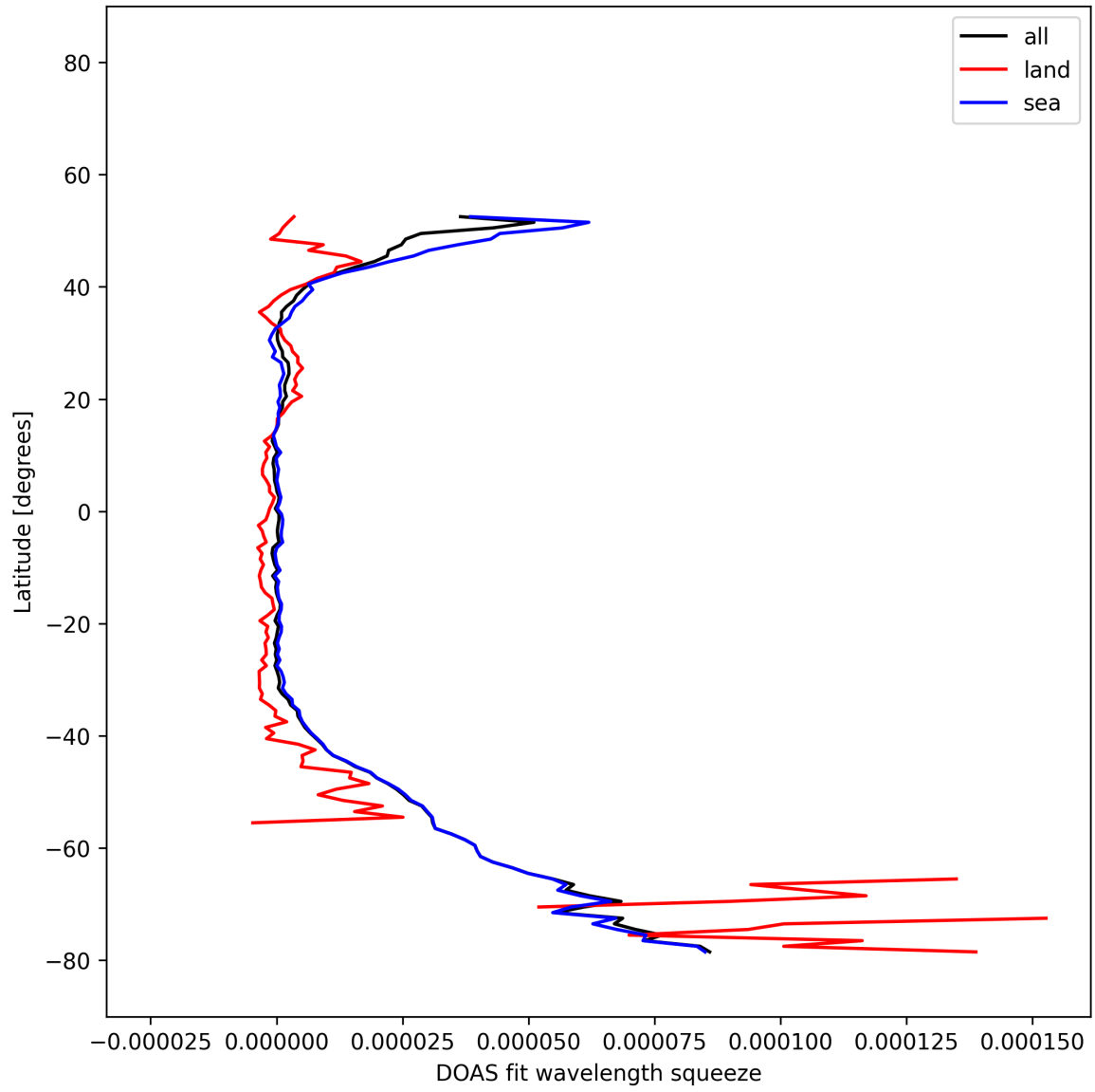
Figure 30: Zonal average of “DOAS fit wavelength squeeze” for 2025-12-09 to 2025-12-10.
