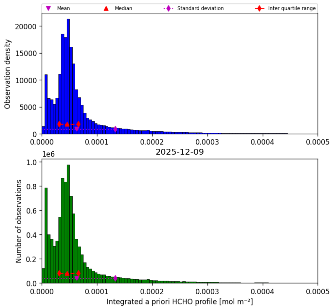
Figure 43: Histogram of “Integrated a priori HCHO profile” for 2025-12-09 to 2025-12-10
