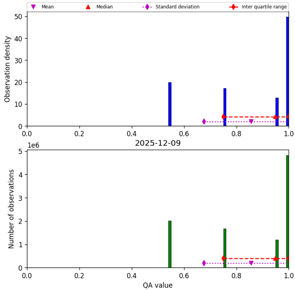
Figure 34: Histogram of “QA value” for 2025-12-09 to 2025-12-10
