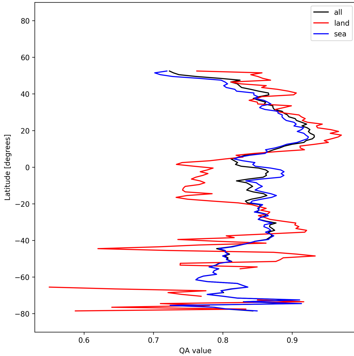
Figure 19: Zonal average of “QA value” for 2025-12-09 to 2025-12-10.
