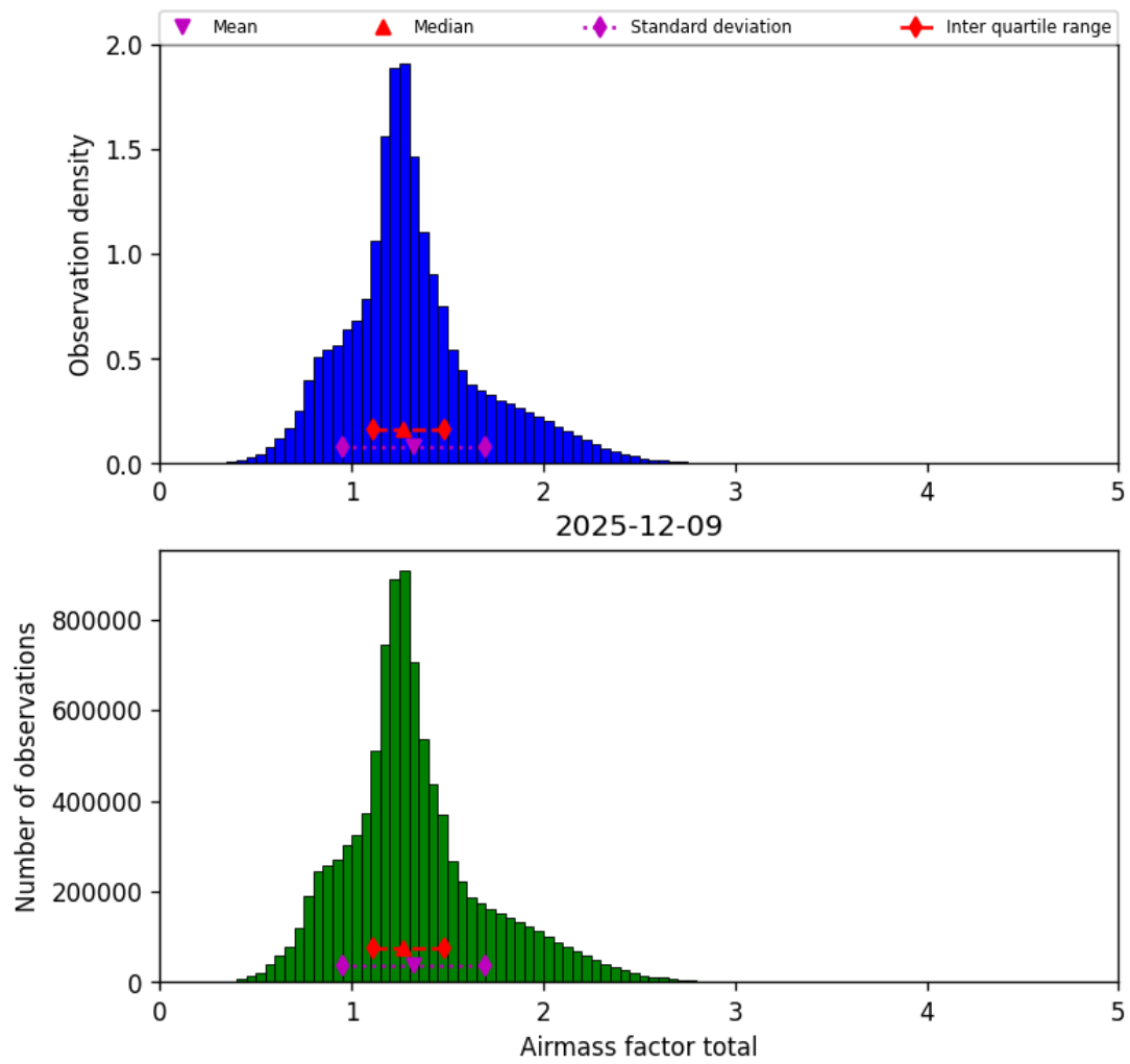
Figure 40: Histogram of “Airmass factor total” for 2025-12-09 to 2025-12-10
