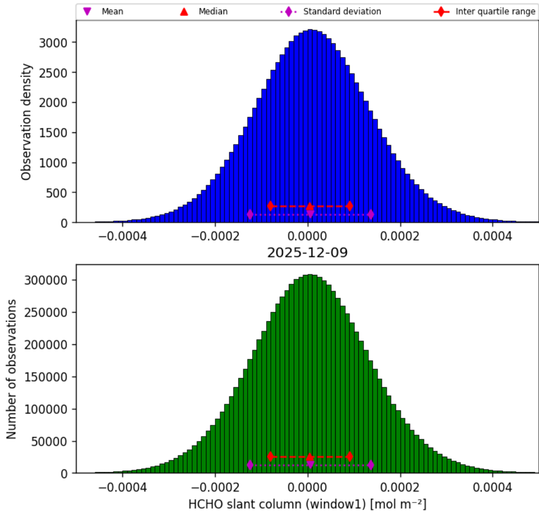
Figure 38: Histogram of “HCHO slant column (window1)” for 2025-12-09 to 2025-12-10
