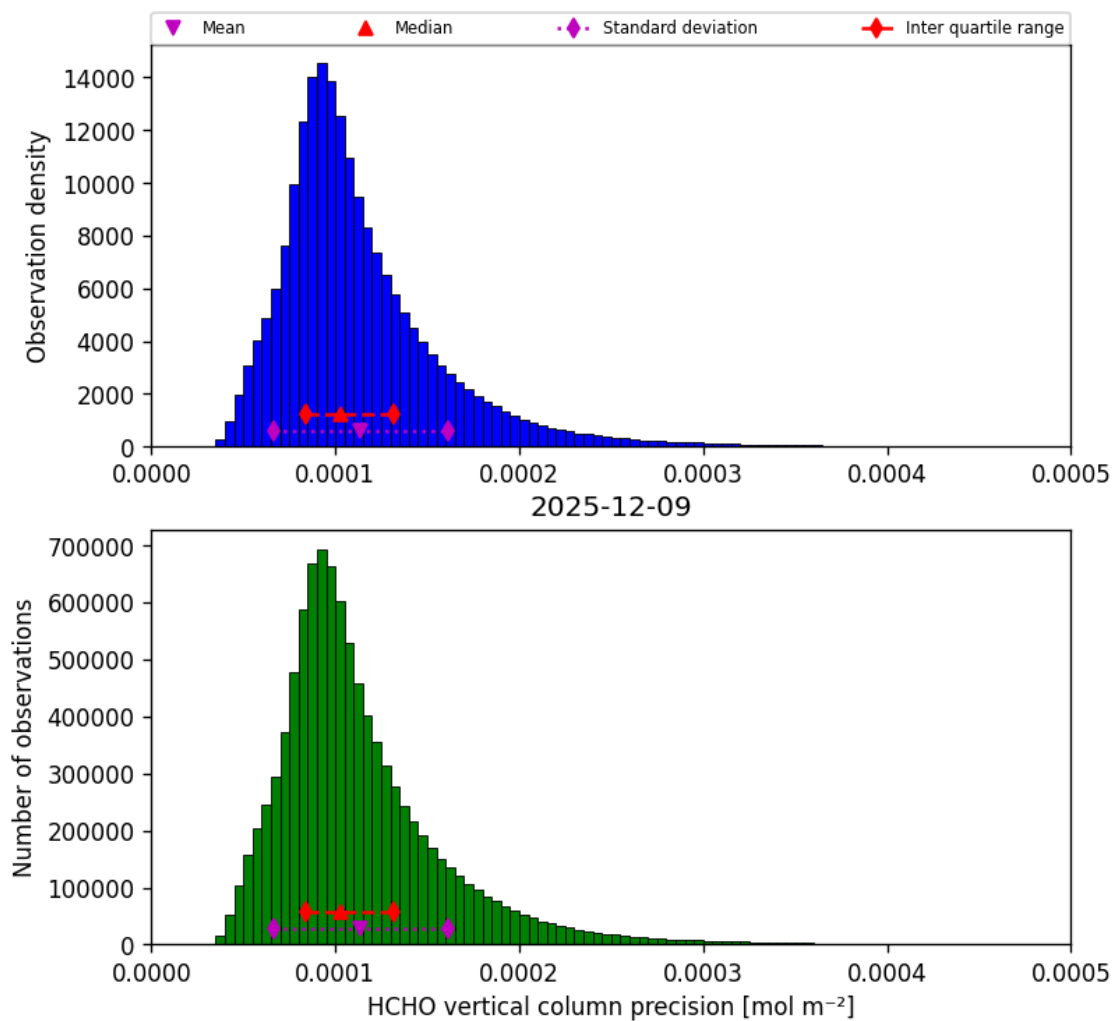
Figure 36: Histogram of “HCHO vertical column precision” for 2025-12-09 to 2025-12-10
