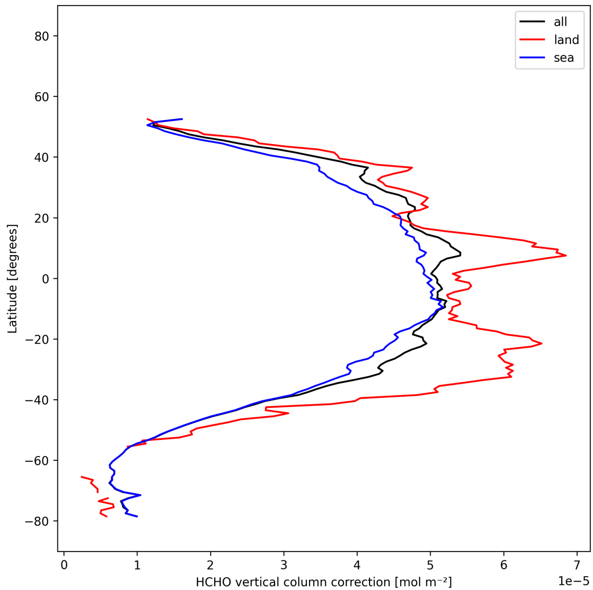
Figure 22: Zonal average of “HCHO vertical column correction” for 2025-12-09 to 2025-12-10.
