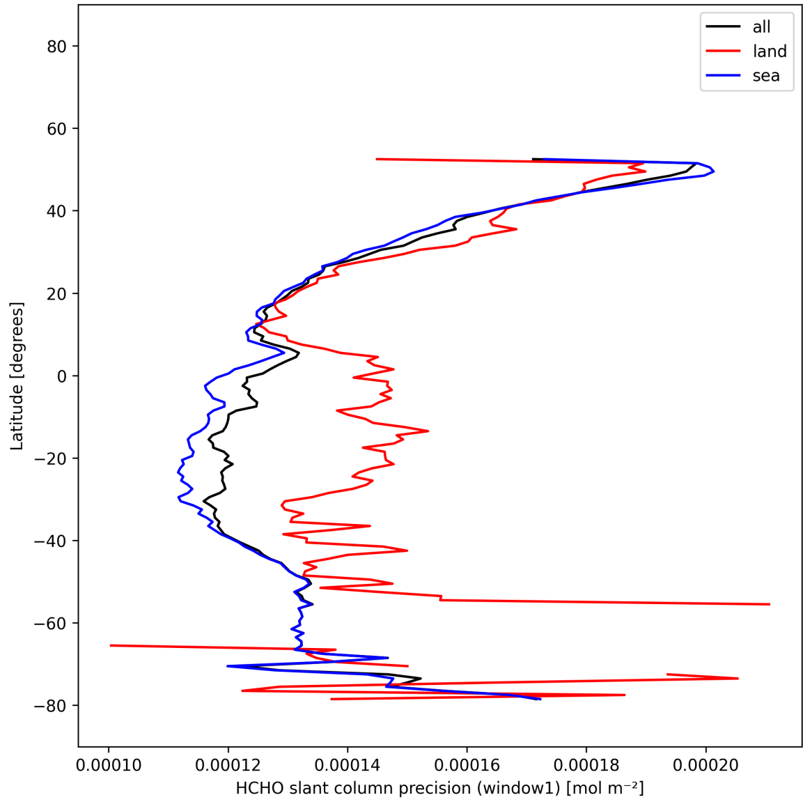
Figure 24: Zonal average of “HCHO slant column precision (window1)” for 2025-12-09 to 2025-12-10.
