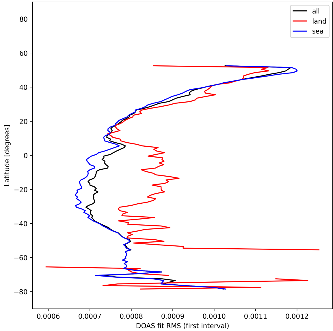
Figure 31: Zonal average of “DOAS fit RMS (first interval)” for 2025-12-09 to 2025-12-10.
