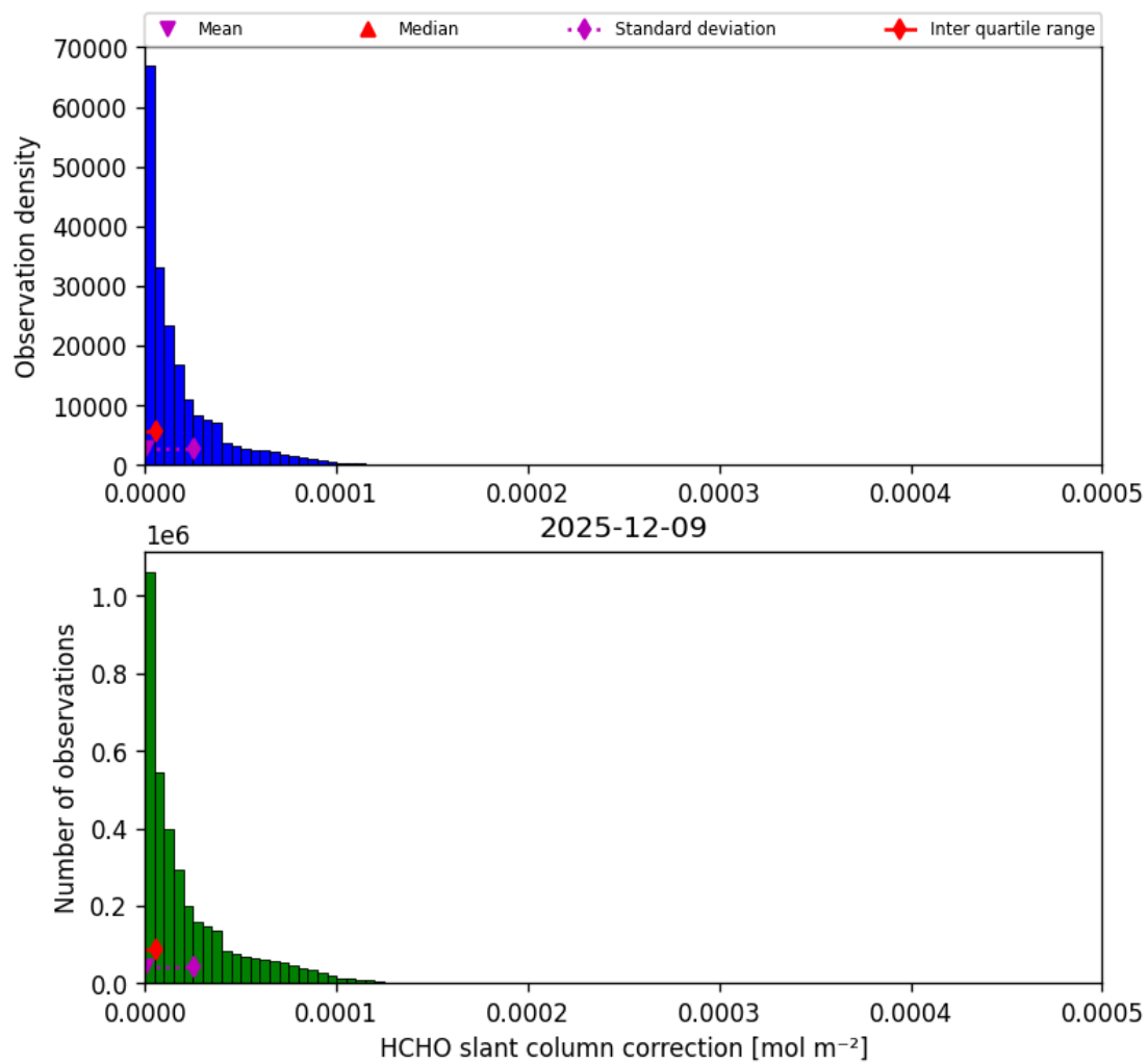
Figure 47: Histogram of “HCHO slant column correction” for 2025-12-09 to 2025-12-10
