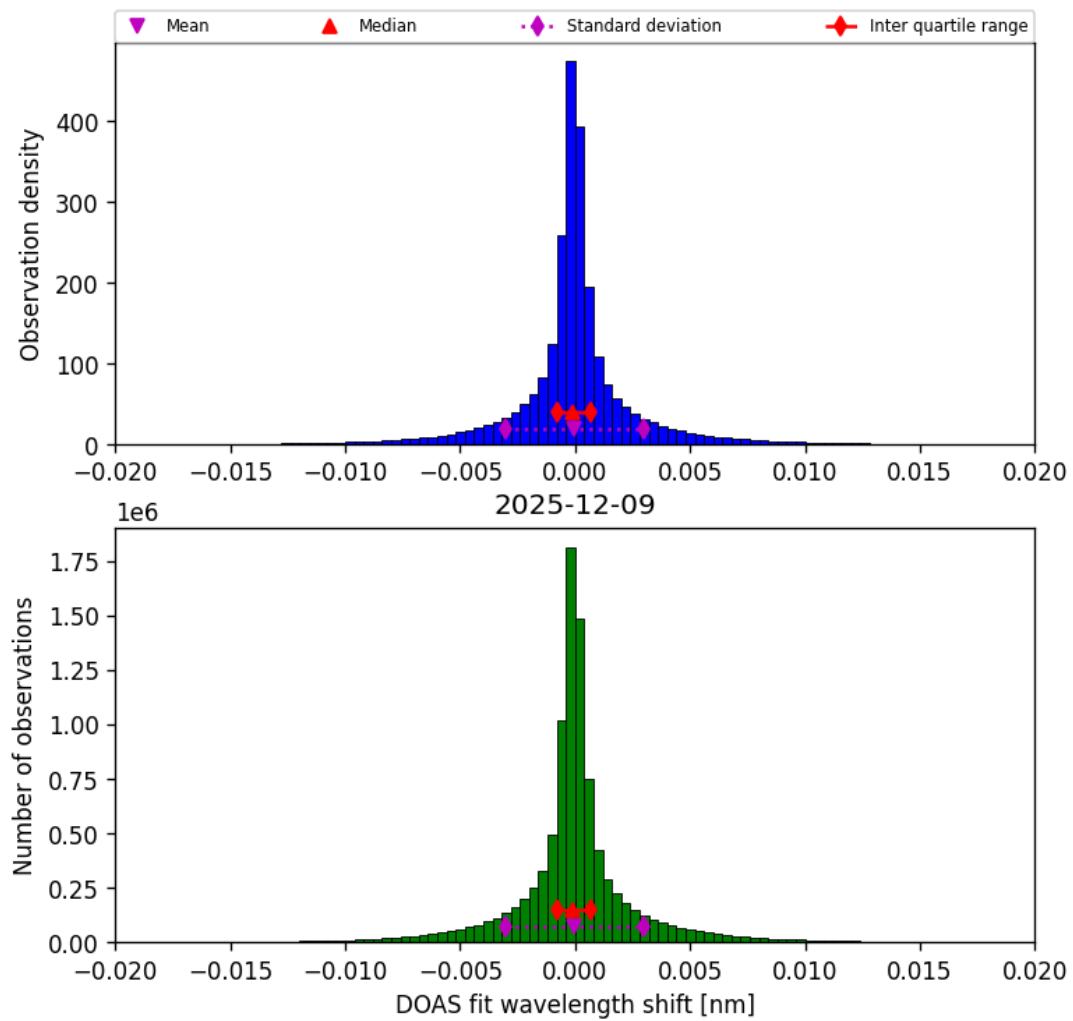
Figure 44: Histogram of “DOAS fit wavelength shift” for 2025-12-09 to 2025-12-10
