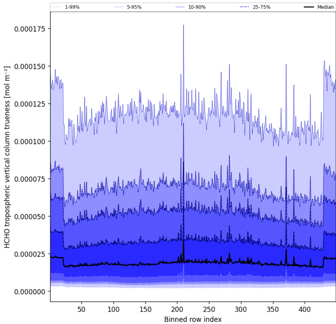
Figure 63: Along track statistics of “HCHO tropospheric vertical column trueness” for 2025-12-09 to 2025-12-10
