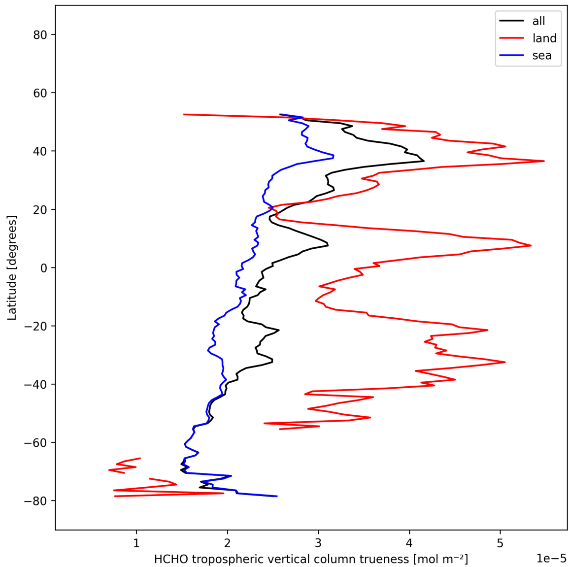
Figure 33: Zonal average of “HCHO tropospheric vertical column trueness” for 2025-12-09 to 2025-12-10.
