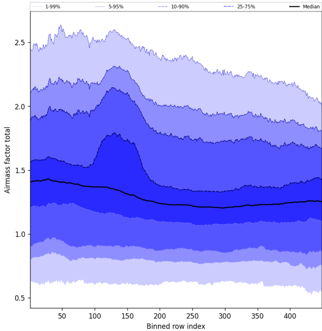
Figure 55: Along track statistics of “Airmass factor total” for 2025-12-09 to 2025-12-10
