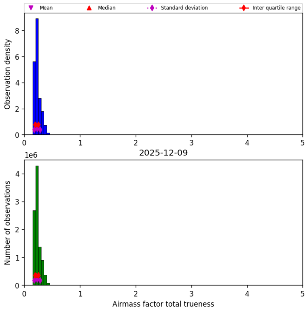
Figure 41: Histogram of “Airmass factor total trueness” for 2025-12-09 to 2025-12-10
