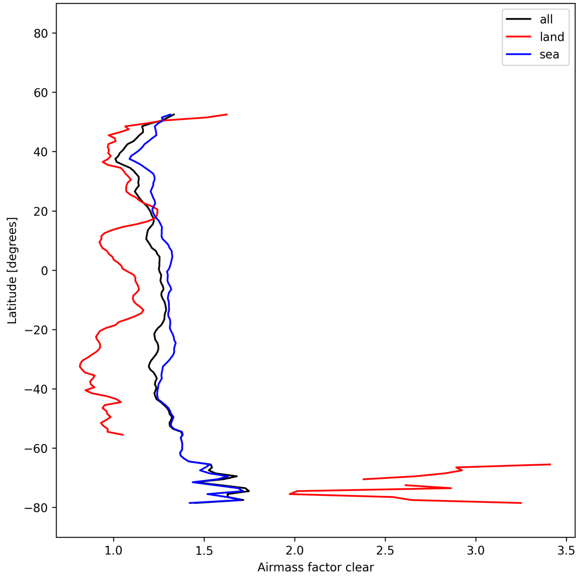
Figure 27: Zonal average of “Airmass factor clear” for 2025-12-09 to 2025-12-10.
