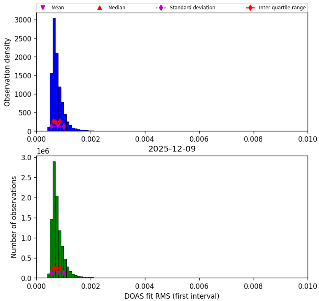
Figure 46: Histogram of “DOAS fit RMS (first interval)” for 2025-12-09 to 2025-12-10
