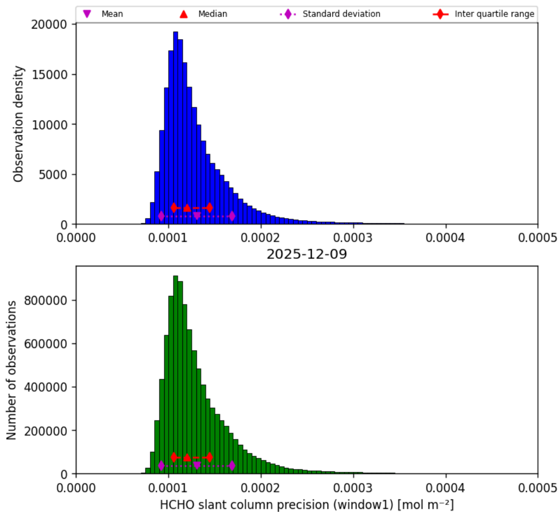
Figure 39: Histogram of “HCHO slant column precision (window1)” for 2025-12-09 to 2025-12-10
