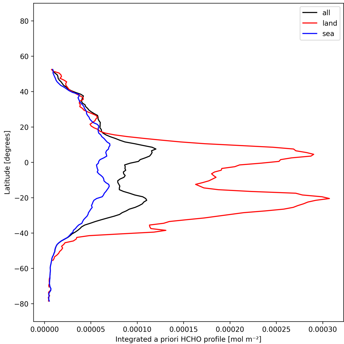
Figure 28: Zonal average of “Integrated a priori HCHO profile” for 2025-12-09 to 2025-12-10.
