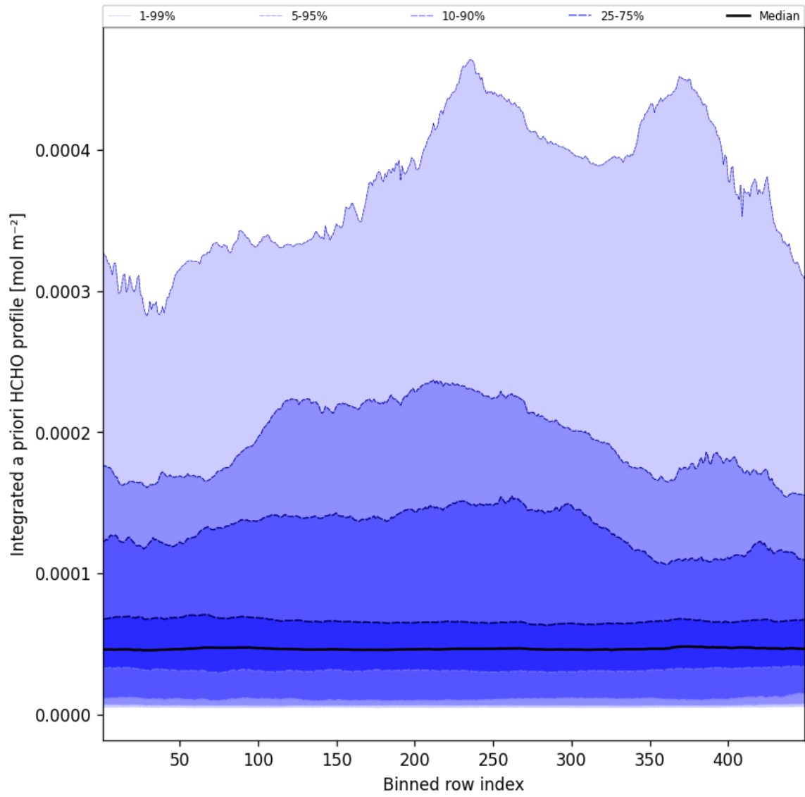
Figure 58: Along track statistics of “Integrated a priori HCHO profile” for 2025-12-09 to 2025-12-10
