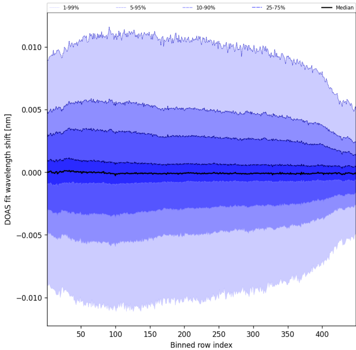
Figure 59: Along track statistics of “DOAS fit wavelength shift” for 2025-12-09 to 2025-12-10
