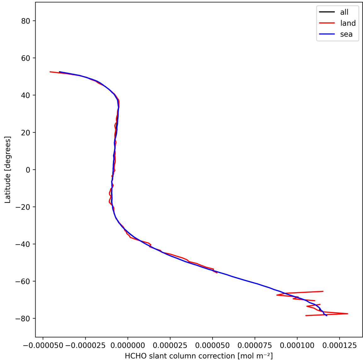
Figure 32: Zonal average of “HCHO slant column correction” for 2025-12-09 to 2025-12-10.
