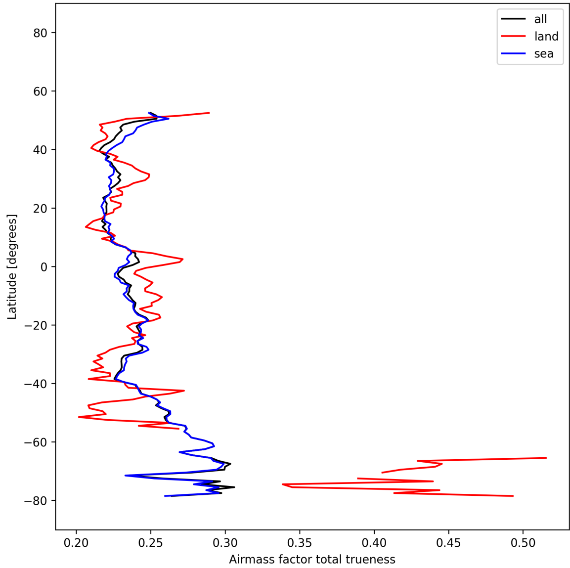
Figure 26: Zonal average of “Airmass factor total trueness” for 2025-12-09 to 2025-12-10.
