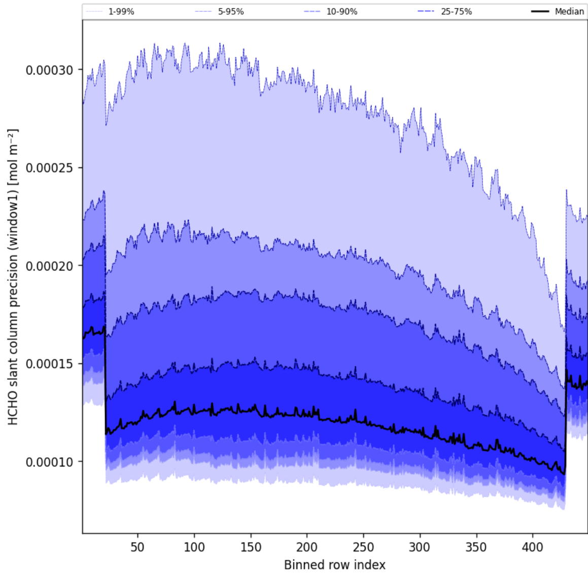
Figure 54: Along track statistics of “HCHO slant column precision (window1)” for 2025-12-09 to 2025-12-10
