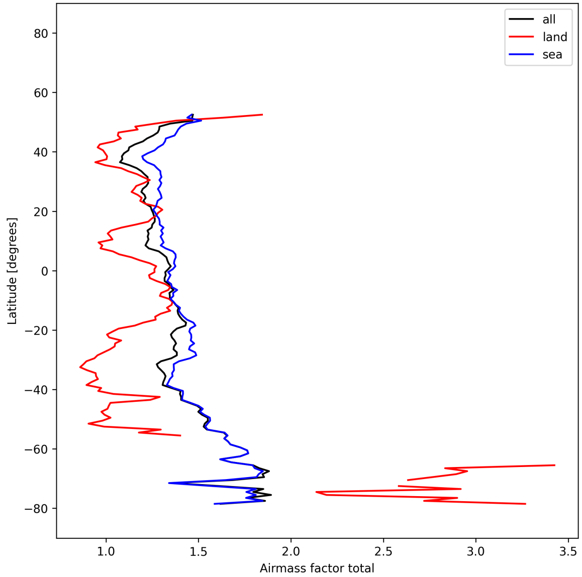
Figure 25: Zonal average of “Airmass factor total” for 2025-12-09 to 2025-12-10.
