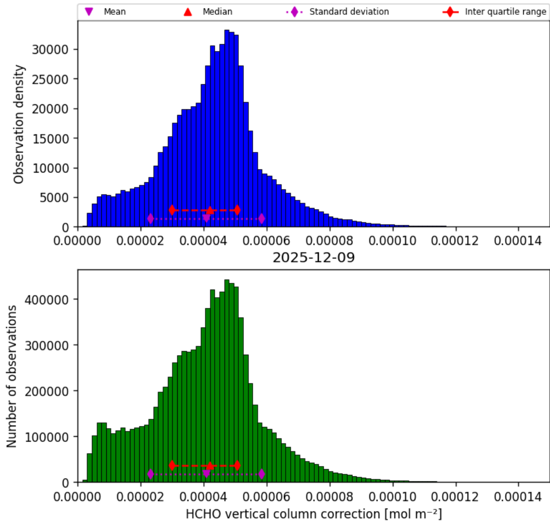
Figure 37: Histogram of “HCHO vertical column correction” for 2025-12-09 to 2025-12-10
