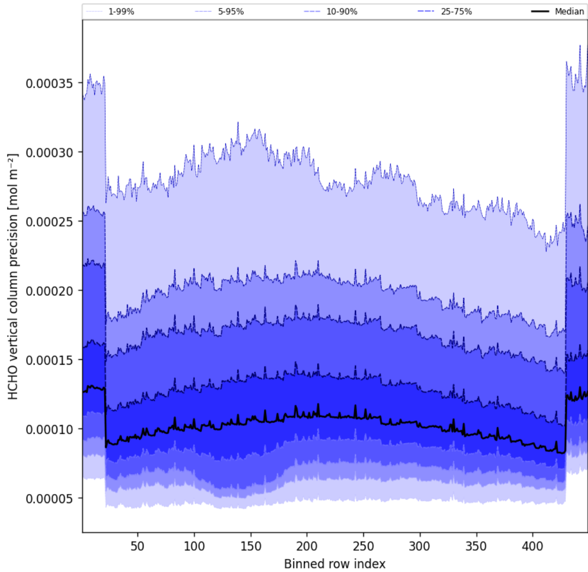
Figure 51: Along track statistics of “HCHO vertical column precision” for 2025-12-09 to 2025-12-10
