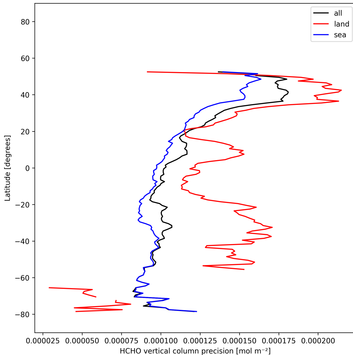
Figure 21: Zonal average of “HCHO vertical column precision” for 2025-12-09 to 2025-12-10.
