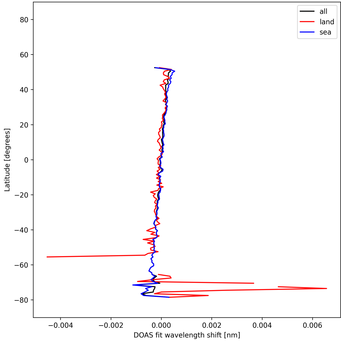
Figure 29: Zonal average of “DOAS fit wavelength shift” for 2025-12-09 to 2025-12-10.
