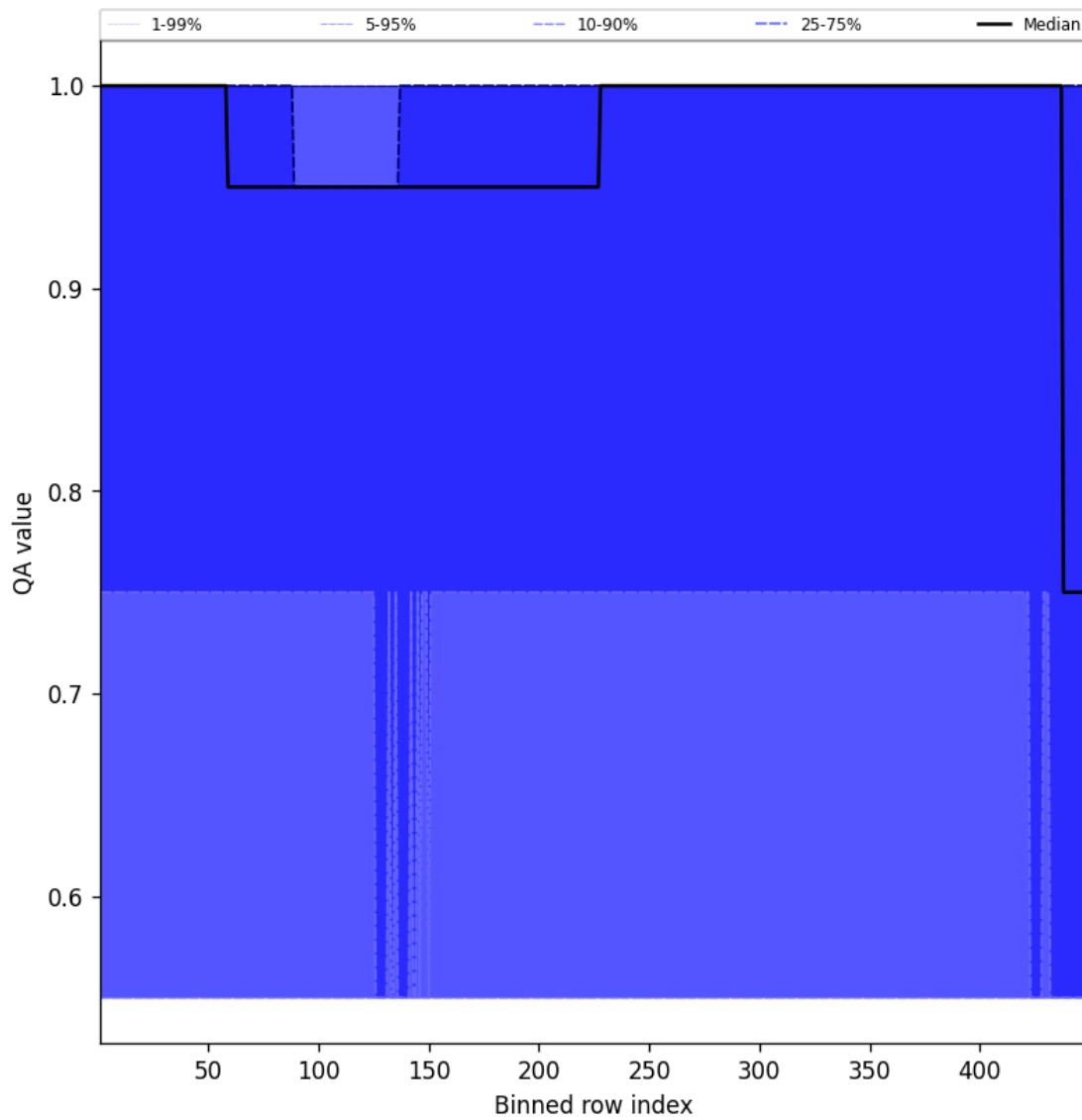
Figure 49: Along track statistics of “QA value” for 2025-12-09 to 2025-12-10
