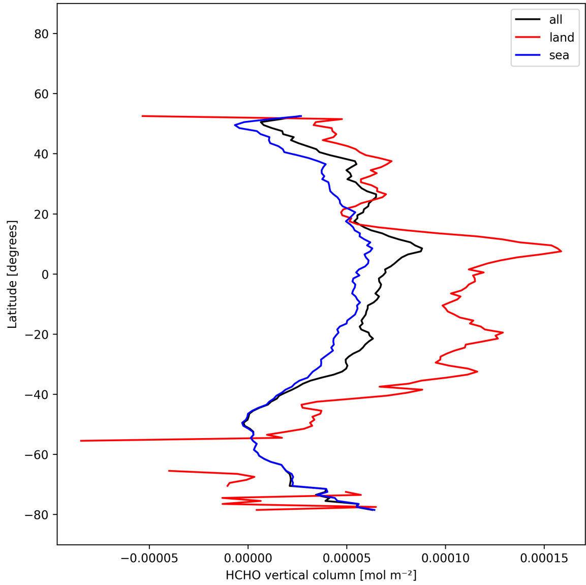
Figure 20: Zonal average of “HCHO vertical column” for 2025-12-09 to 2025-12-10.
