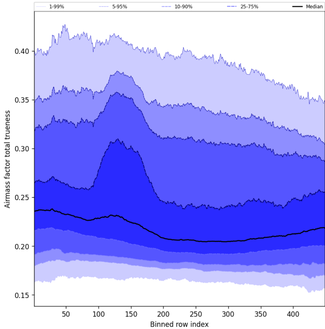
Figure 56: Along track statistics of “Airmass factor total trueness” for 2025-12-09 to 2025-12-10
