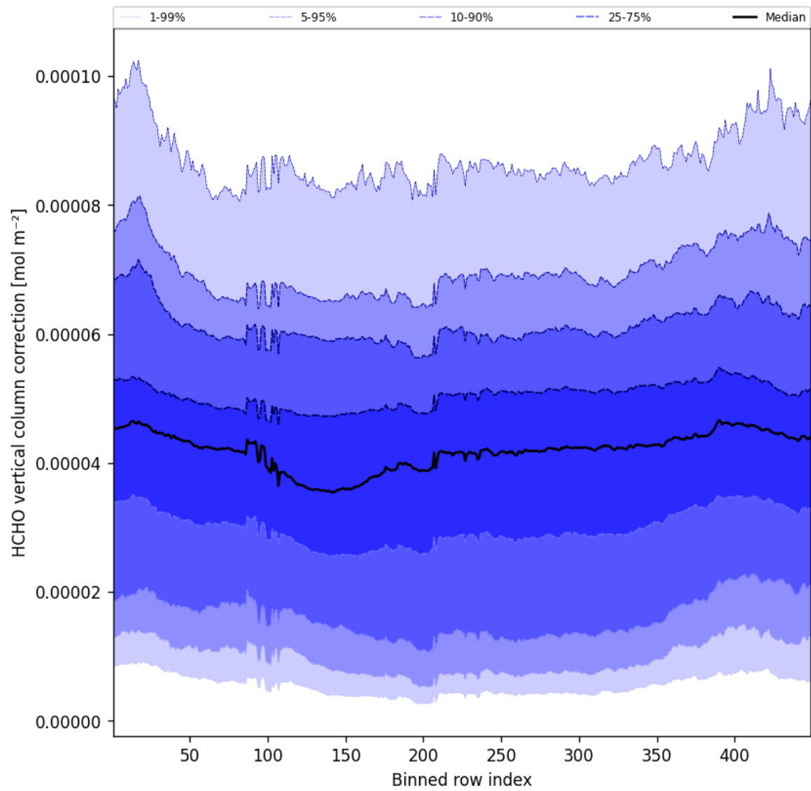
Figure 52: Along track statistics of “HCHO vertical column correction” for 2025-12-10 to 2025-12-11
