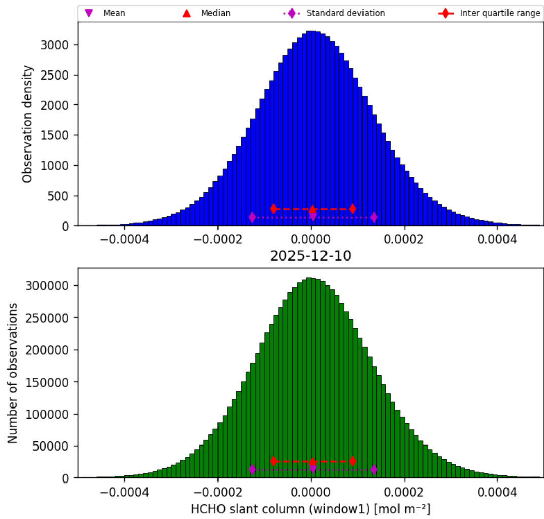
Figure 38: Histogram of “HCHO slant column (window1)” for 2025-12-10 to 2025-12-11
