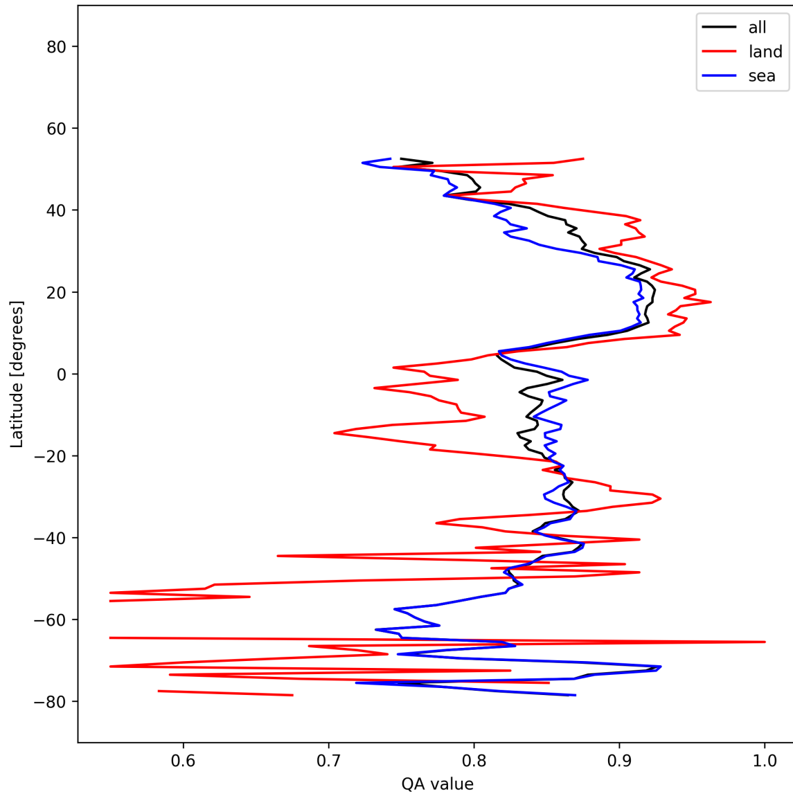
Figure 19: Zonal average of “QA value” for 2025-12-10 to 2025-12-11.
