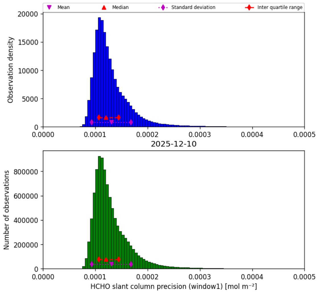
Figure 39: Histogram of “HCHO slant column precision (window1)” for 2025-12-10 to 2025-12-11
