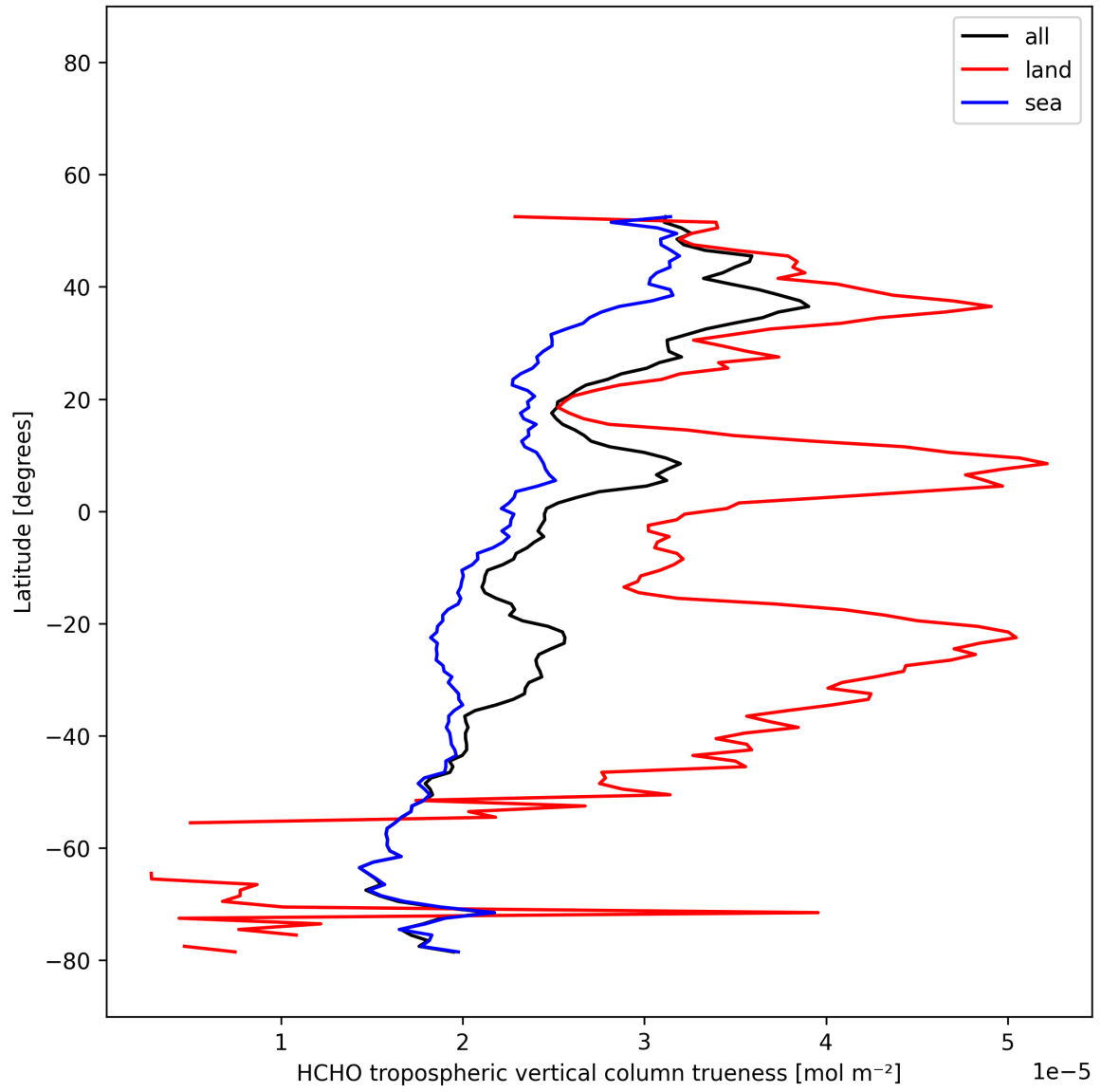
Figure 33: Zonal average of “HCHO tropospheric vertical column density” for 2025-12-10 to 2025-12-11.
