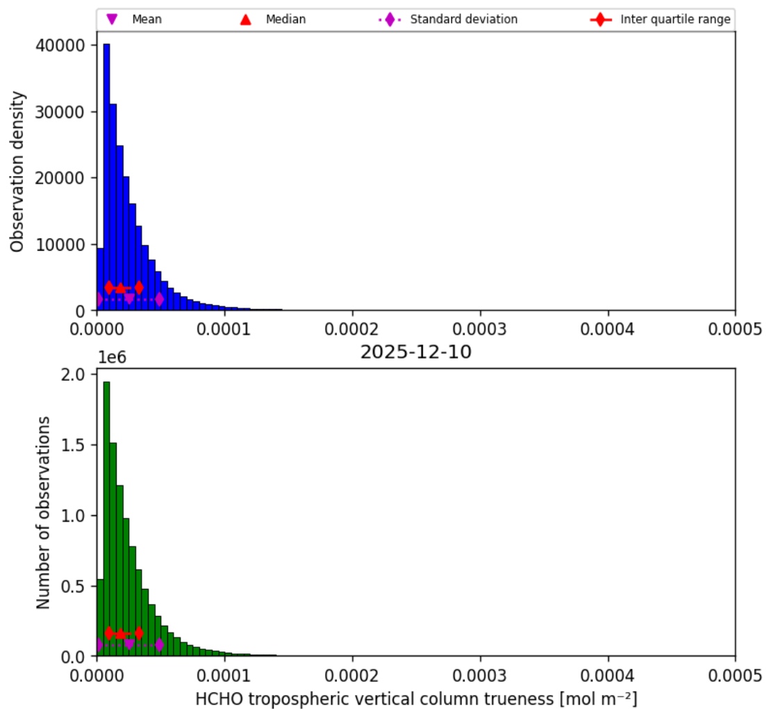
Figure 48: Histogram of “HCHO tropospheric vertical column trueness” for 2025-12-10 to 2025-12-11
