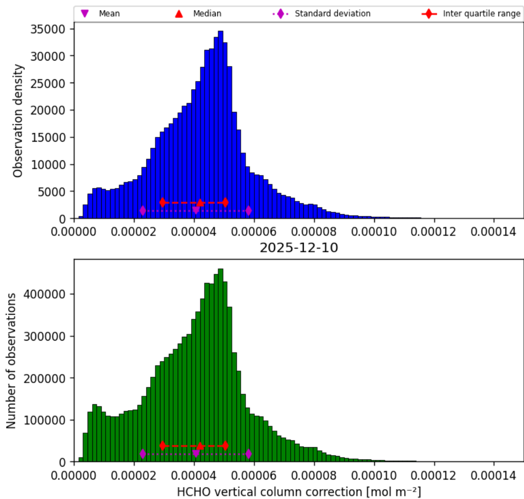
Figure 37: Histogram of “HCHO vertical column correction” for 2025-12-10 to 2025-12-11
