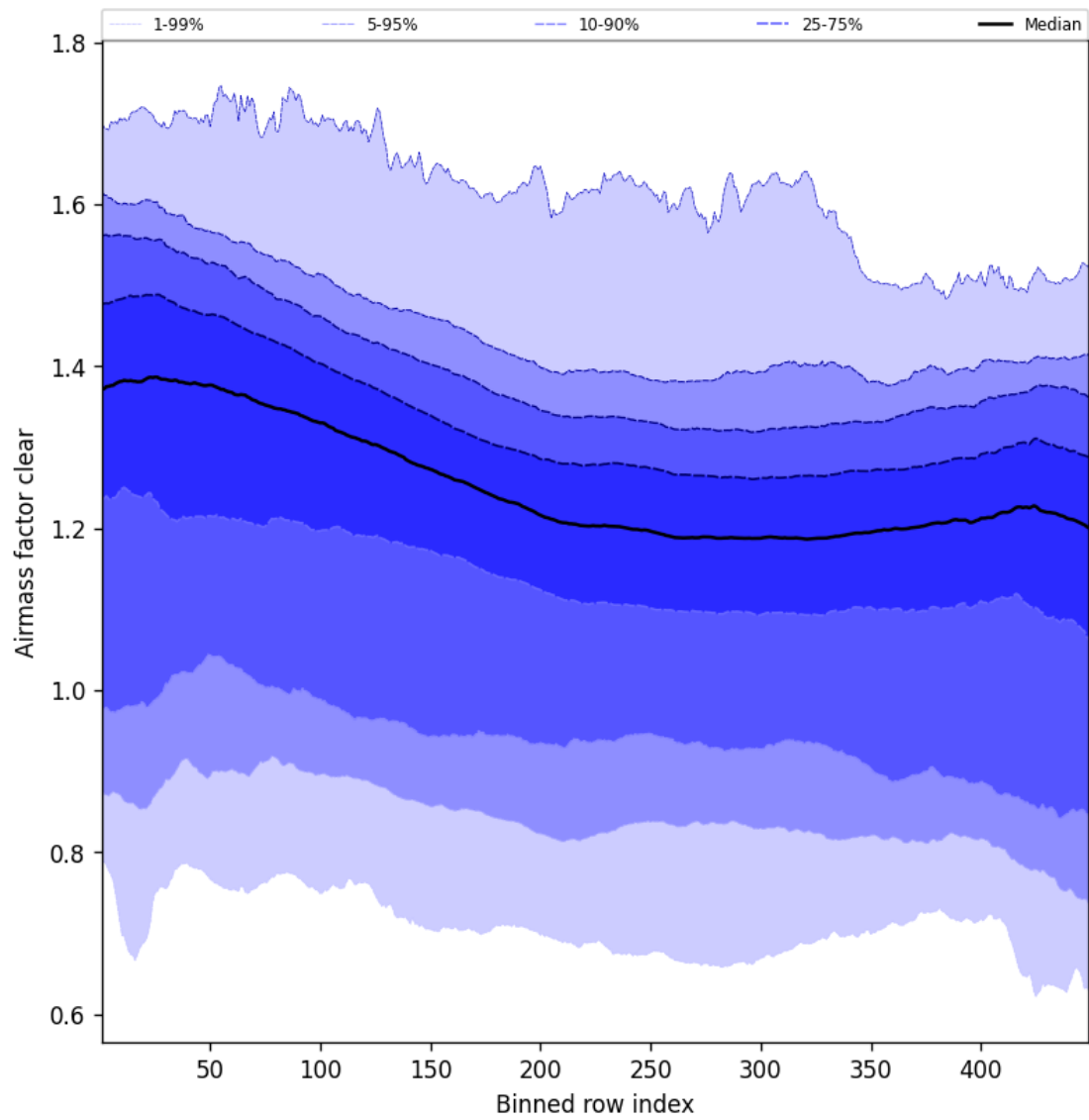
Figure 57: Along track statistics of “Airmass factor clear” for 2025-12-10 to 2025-12-11
