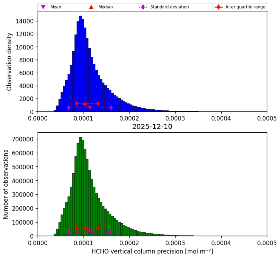
Figure 36: Histogram of “HCHO vertical column precision” for 2025-12-10 to 2025-12-11
