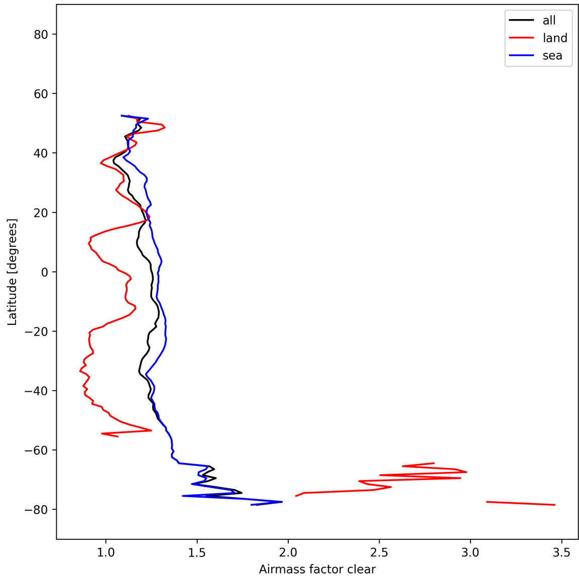
Figure 27: Zonal average of “Airmass factor clear” for 2025-12-10 to 2025-12-11.
