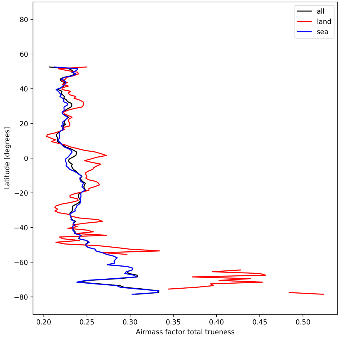
Figure 26: Zonal average of “Airmass factor total truiness” for 2025-12-10 to 2025-12-11.
