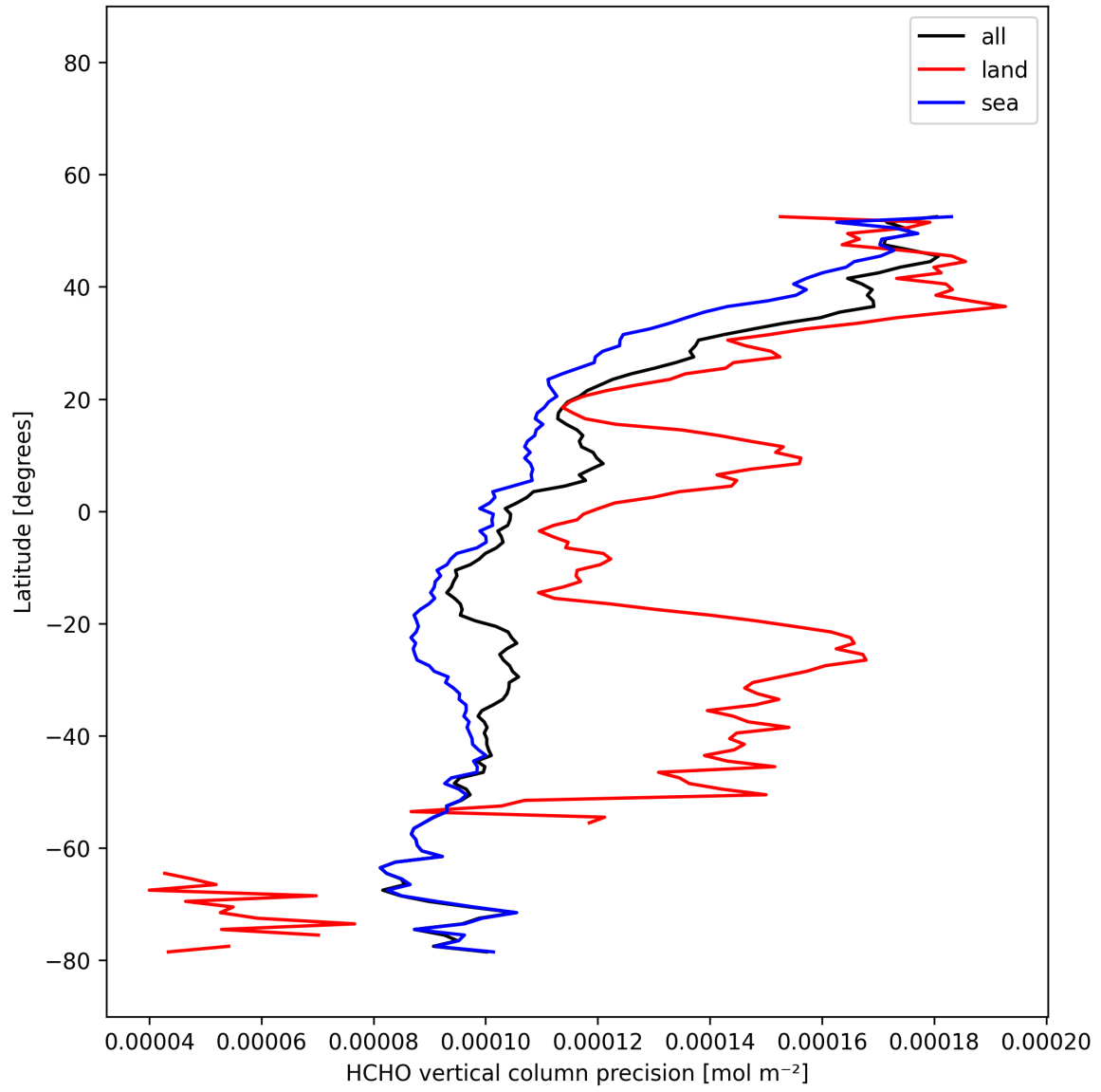
Figure 21: Zonal average of “HCHO vertical column precision” for 2025-12-10 to 2025-12-11.
