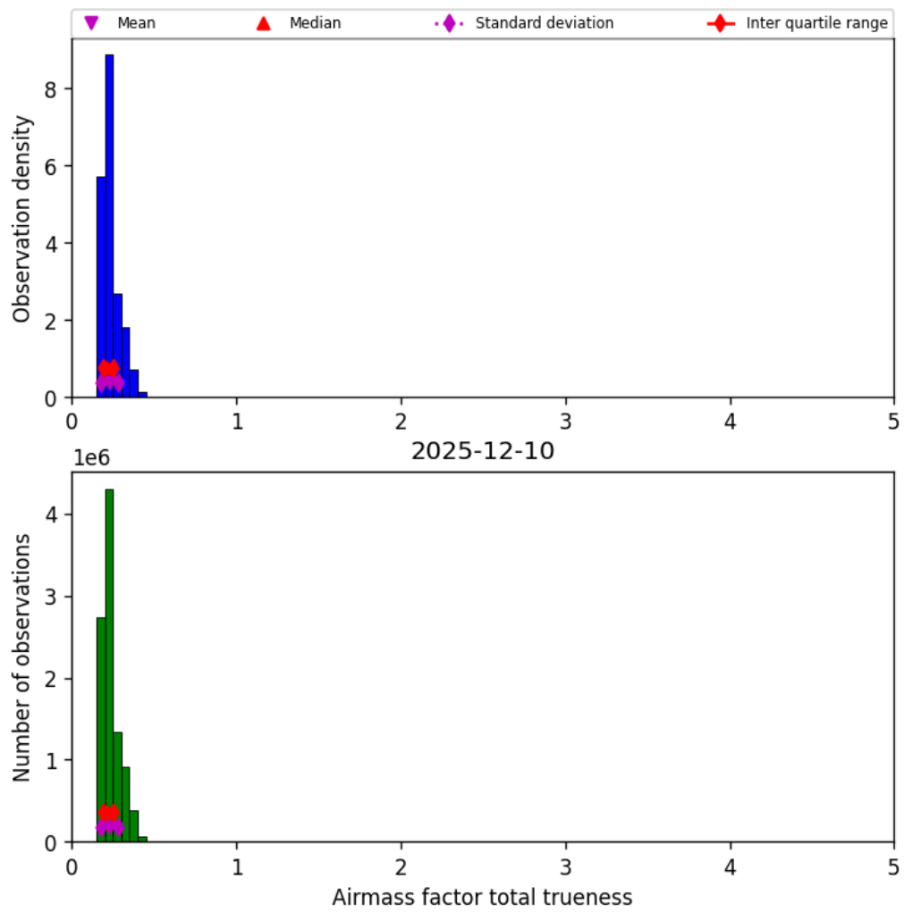
Figure 41: Histogram of “Airmass factor total trueness” for 2025-12-10 to 2025-12-11
