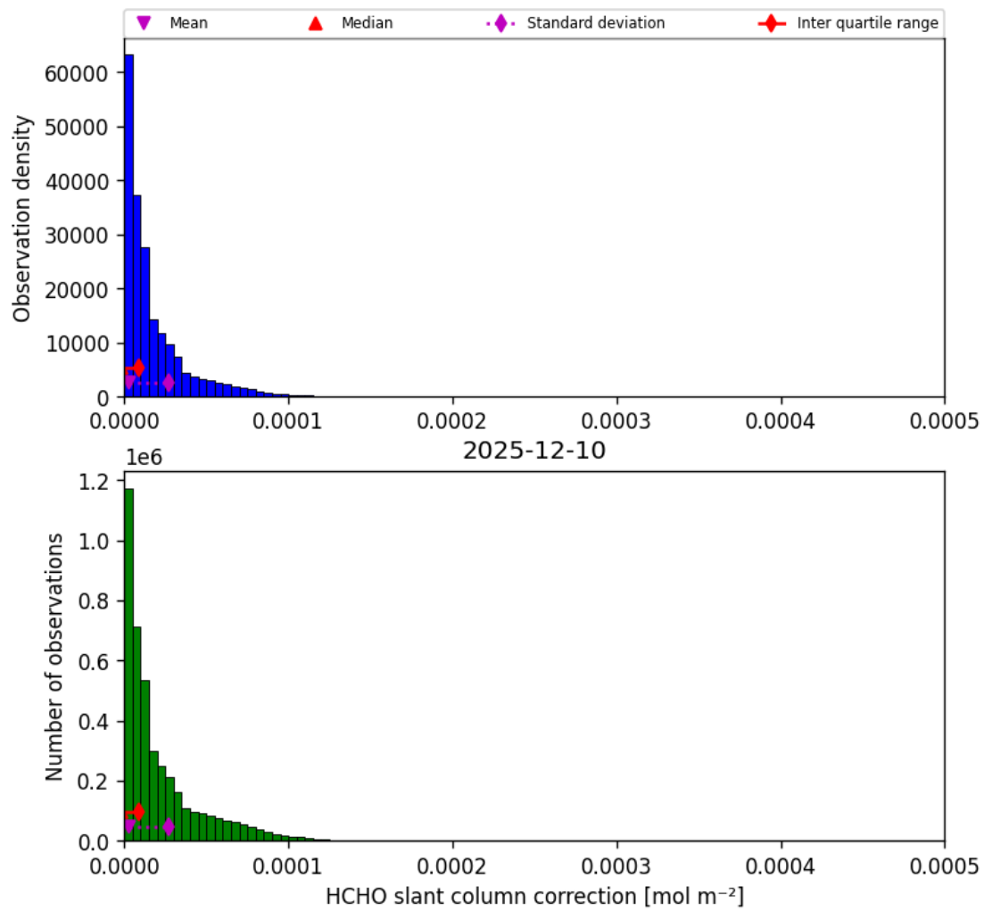
Figure 47: Histogram of “HCHO slant column correction” for 2025-12-10 to 2025-12-11
