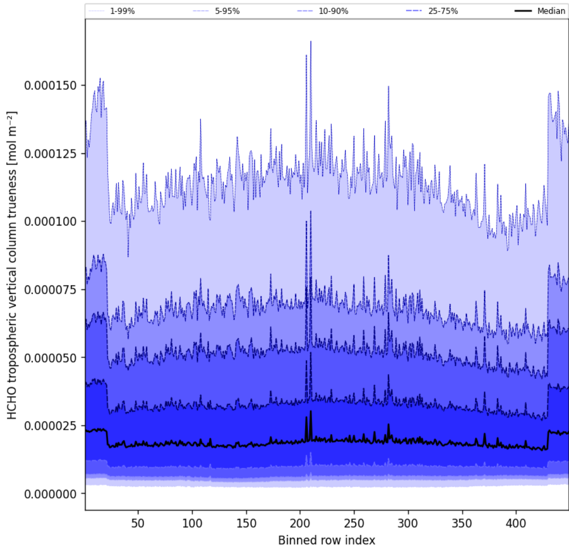
Figure 63: Along track statistics of “HCHO tropospheric vertical column trueness” for 2025-12-10 to 2025-12-11
