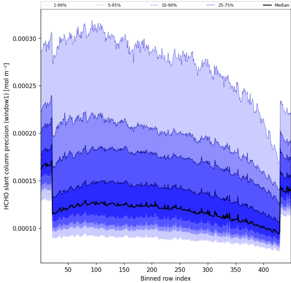
Figure 54: Along track statistics of “HCHO slant column precision (window1)” for 2025-12-10 to 2025-12-11
