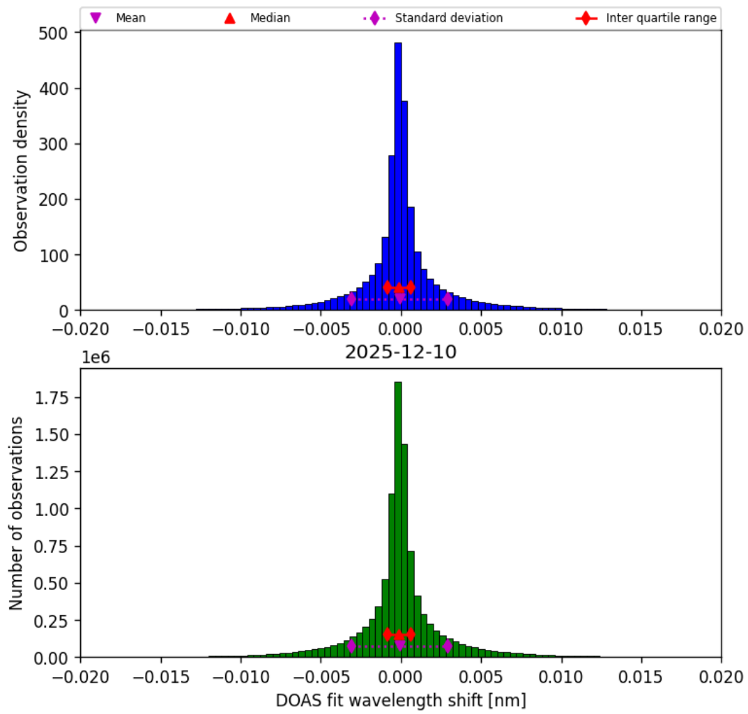
Figure 44: Histogram of “DOAS fit wavelength shift” for 2025-12-10 to 2025-12-11
