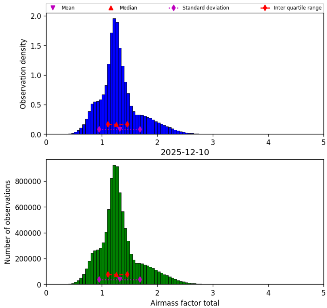
Figure 40: Histogram of “Airmass factor total” for 2025-12-10 to 2025-12-11
