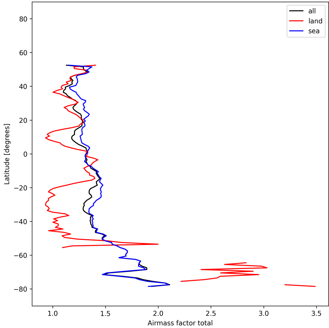
Figure 25: Zonal average of “Airmass factor total” for 2025-12-10 to 2025-12-11.
