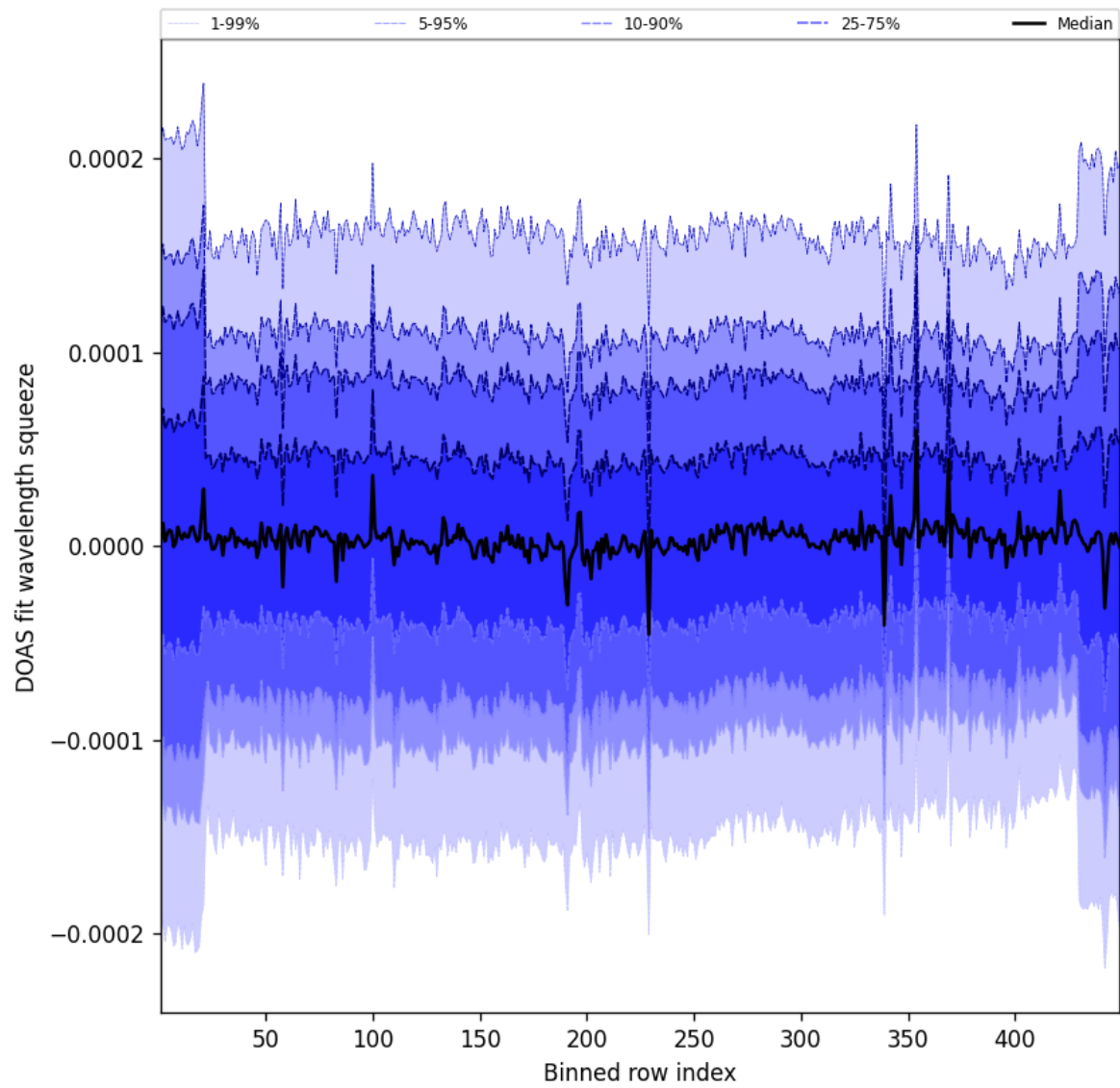
Figure 60: Along track statistics of “DOAS fit wavelength squeeze” for 2025-12-10 to 2025-12-11
