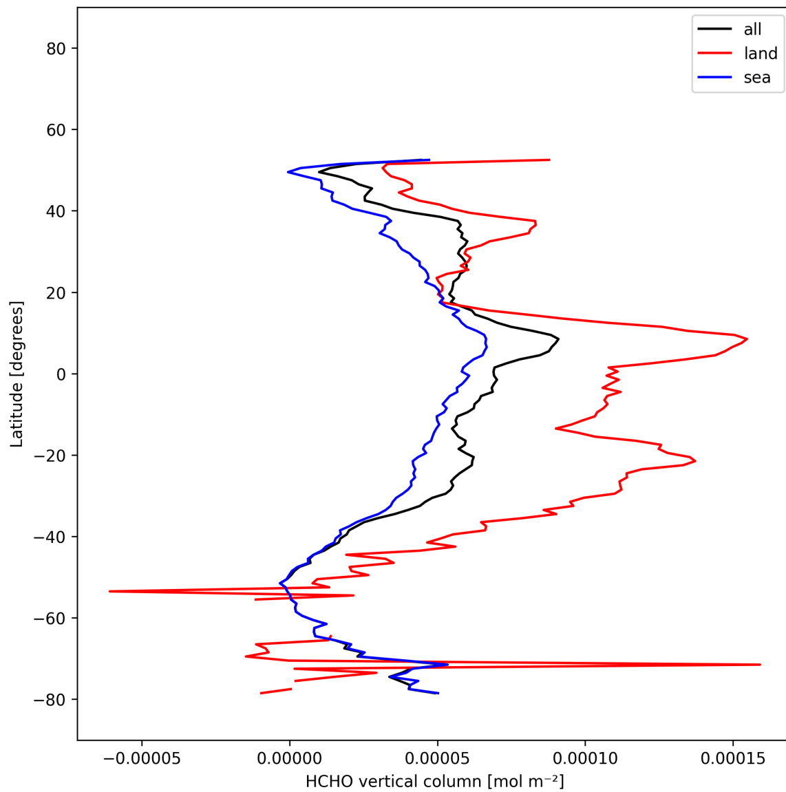
Figure 20: Zonal average of “HCHO vertical column” for 2025-12-10 to 2025-12-11.
