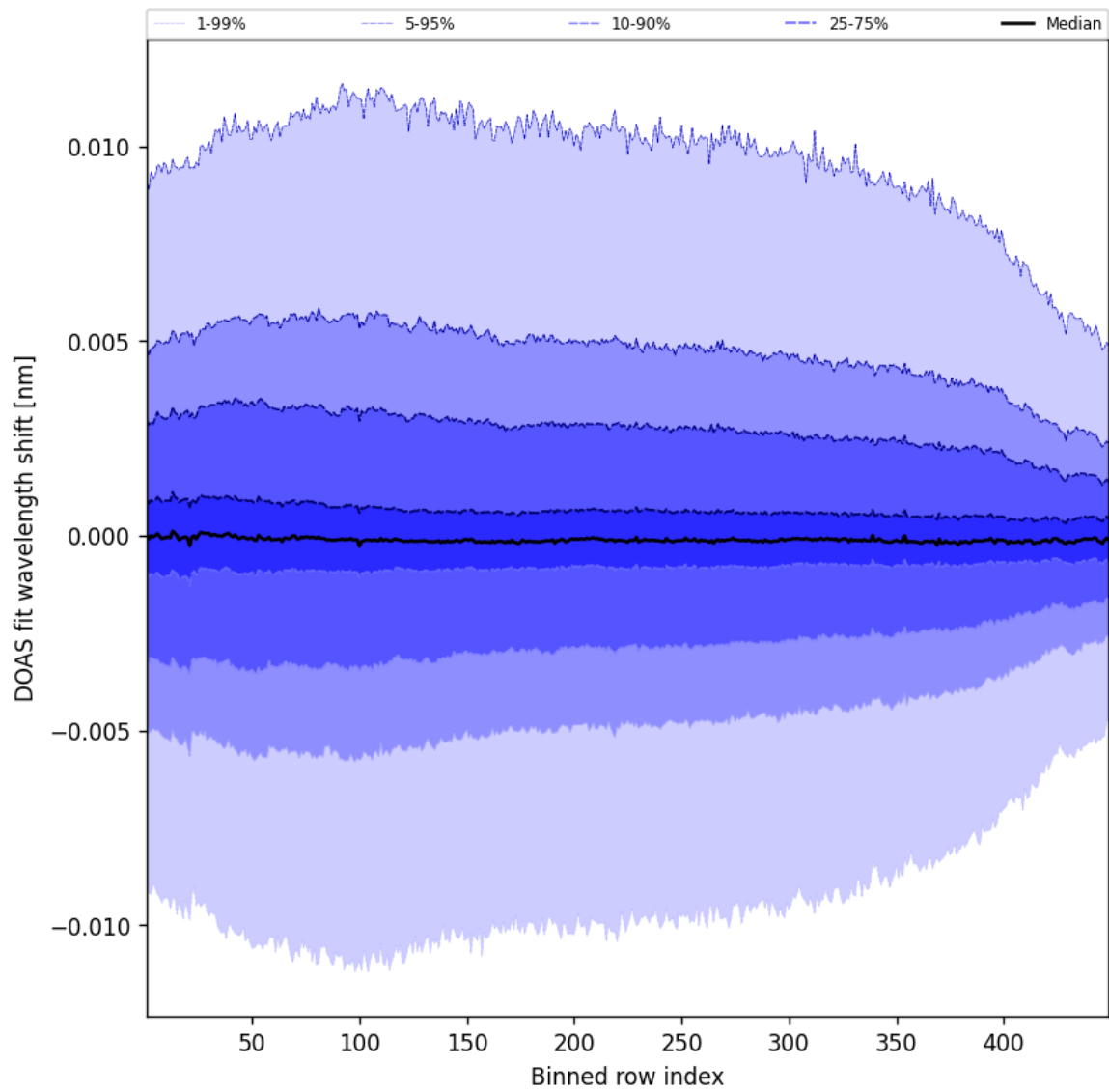
Figure 59: Along track statistics of “DOAS fit wavelength shift” for 2025-12-10 to 2025-12-11
