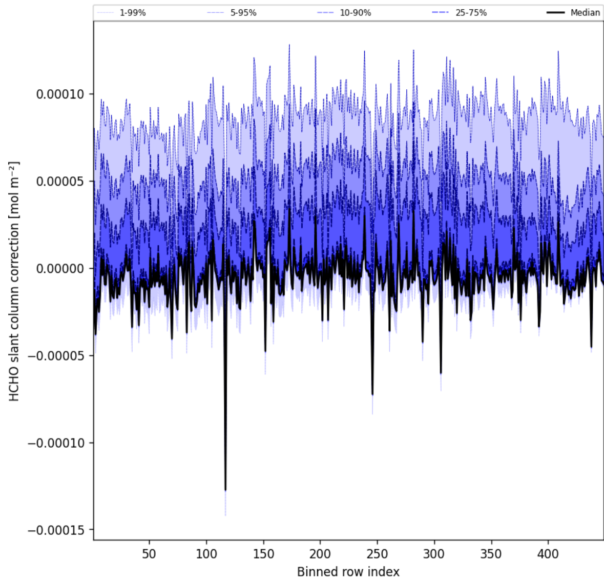
Figure 62: Along track statistics of “HCHO slant column correction” for 2025-12-10 to 2025-12-11
