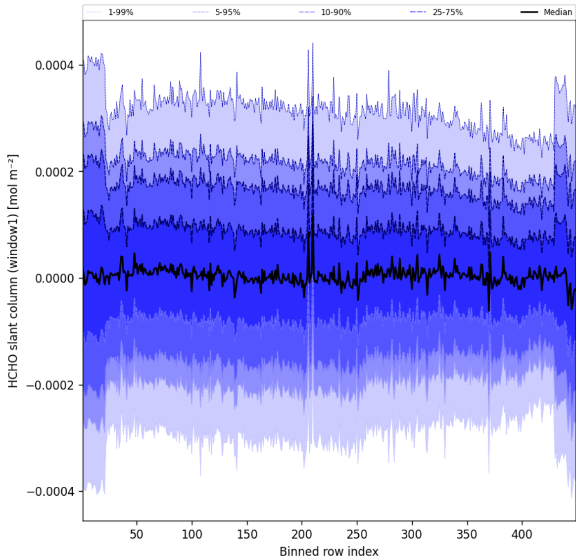
Figure 53: Along track statistics of “HCHO slant column (window1)” for 2025-12-10 to 2025-12-11
