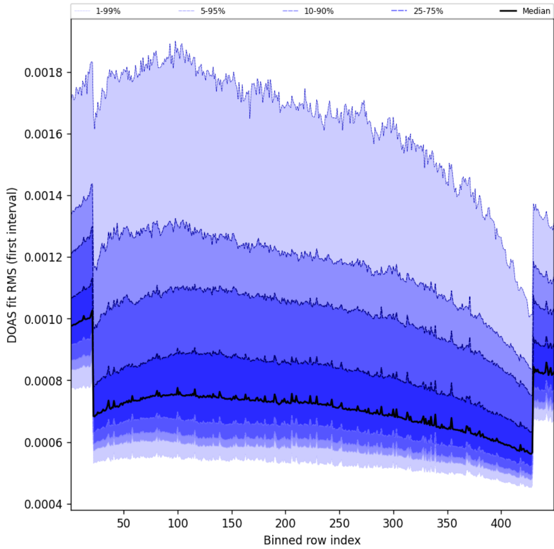
Figure 61: Along track statistics of “DOAS fit RMS (first interval)” for 2025-12-10 to 2025-12-11
