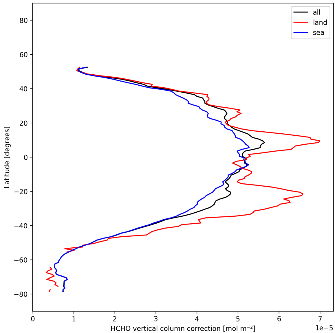
Figure 22: Zonal average of "HCHO vertical column correction" for 2025-12-10 to 2025-12-11.
