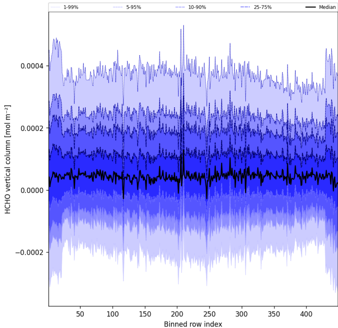
Figure 50: Along track statistics of “HCHO vertical column” for 2025-12-10 to 2025-12-11
