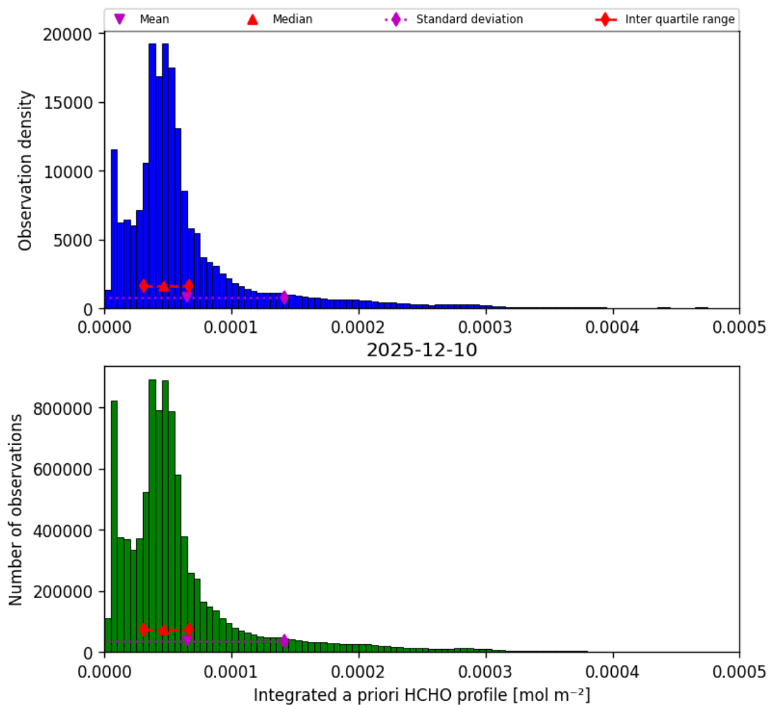
Figure 43: Histogram of “Integrated a priori HCHO profile” for 2025-12-10 to 2025-12-11
