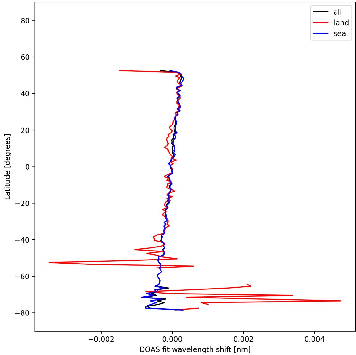
Figure 29: Zonal average of "DOAS fit wavelength shift" for 2025-12-10 to 2025-12-11.
