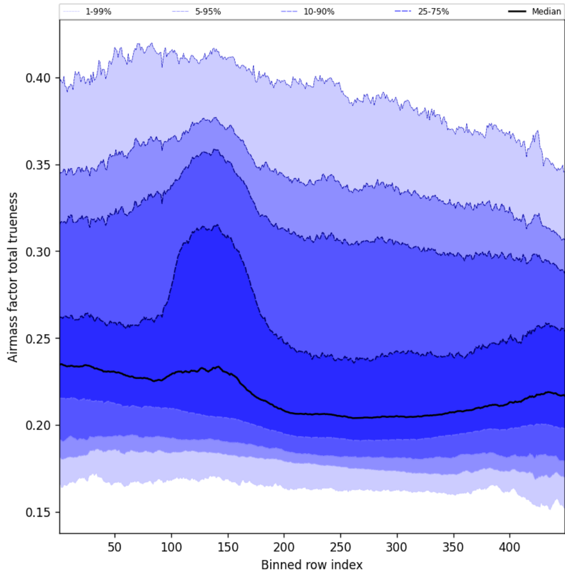
Figure 56: Along track statistics of “Airmass factor total trueness” for 2025-12-10 to 2025-12-11
