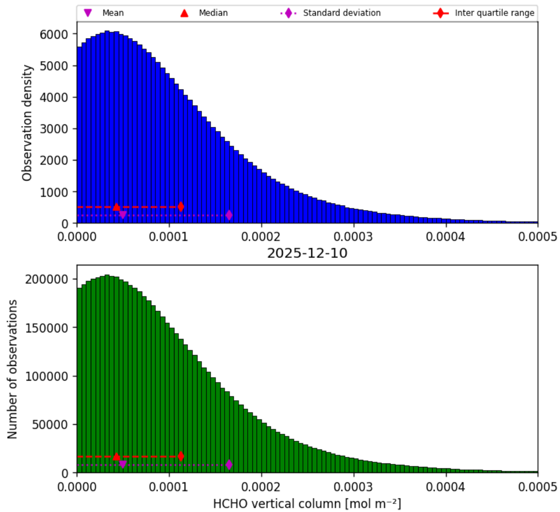
Figure 35: Histogram of “HCHO vertical column” for 2025-12-10 to 2025-12-11
