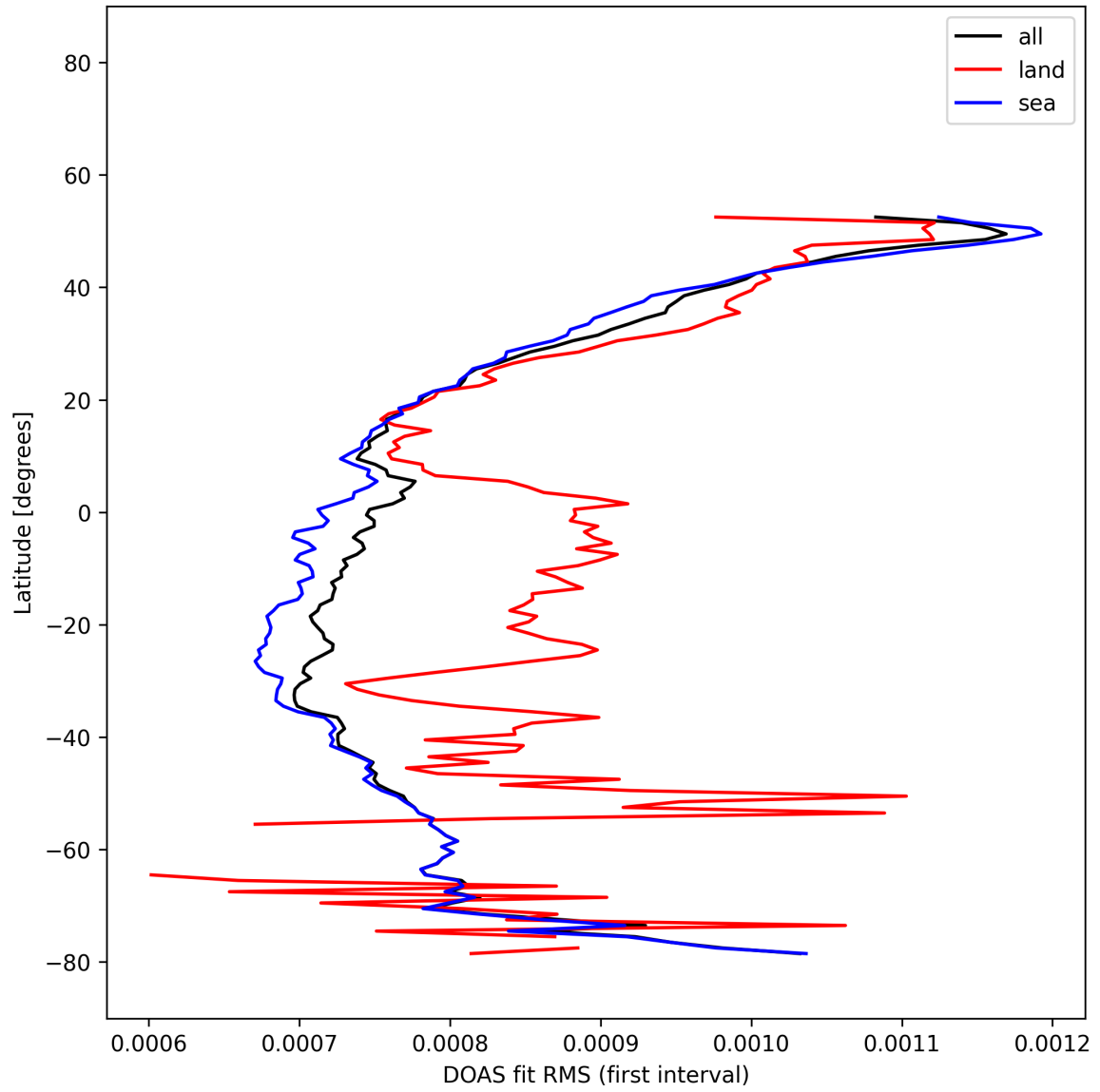
Figure 31: Zonal average of “DOAS fit RMS (first interval)” for 2025-12-10 to 2025-12-11.
