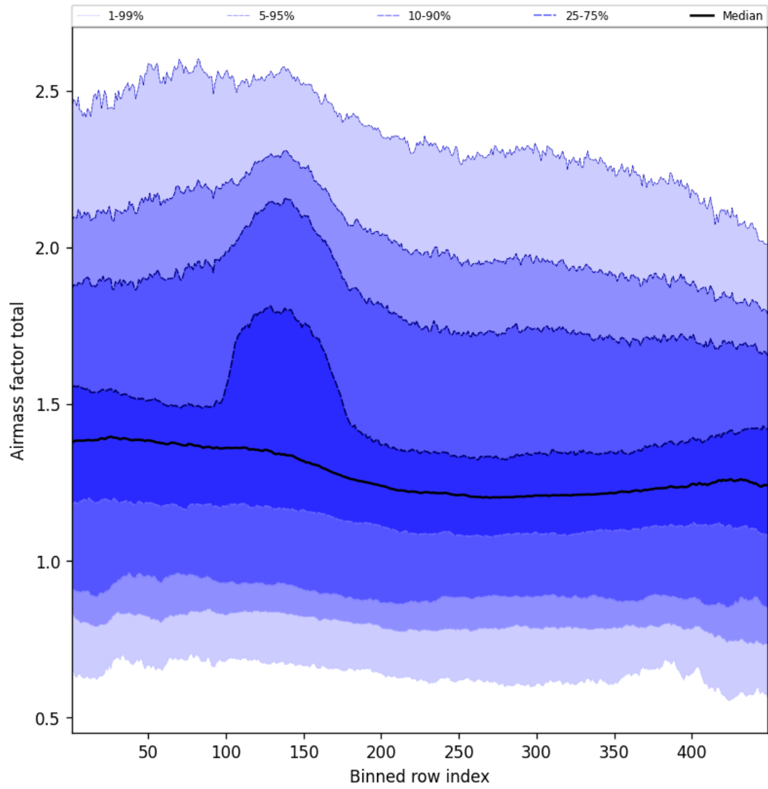
Figure 55: Along track statistics of “Airmass factor total” for 2025-12-10 to 2025-12-11
