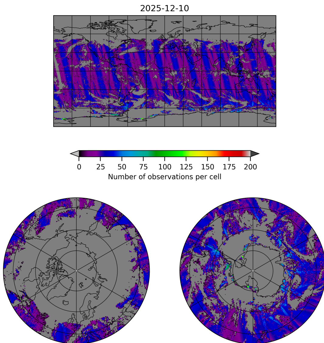
Figure 18: Map of the number of observations for 2025-12-10 to 2025-12-11
