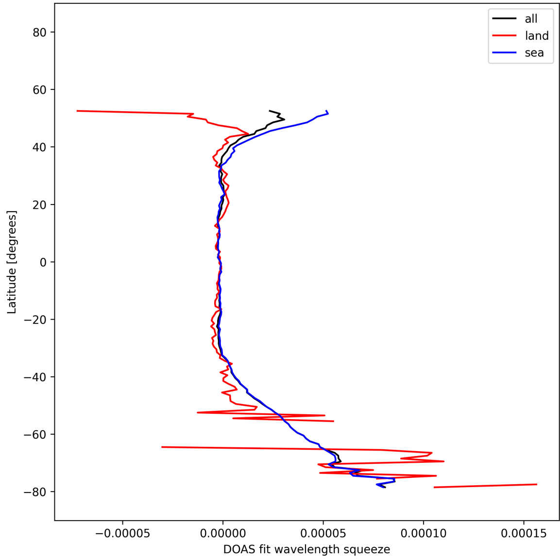
Figure 30: Zonal average of “DOAS fit wavelength squeeze” for 2025-12-10 to 2025-12-11.
