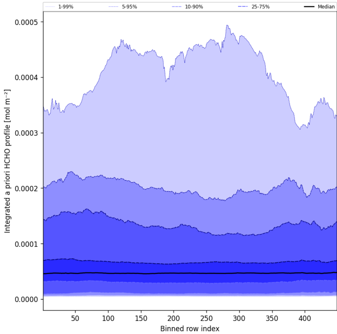
Figure 58: Along track statistics of “Integrated a priori HCHO profile” for 2025-12-10 to 2025-12-11
