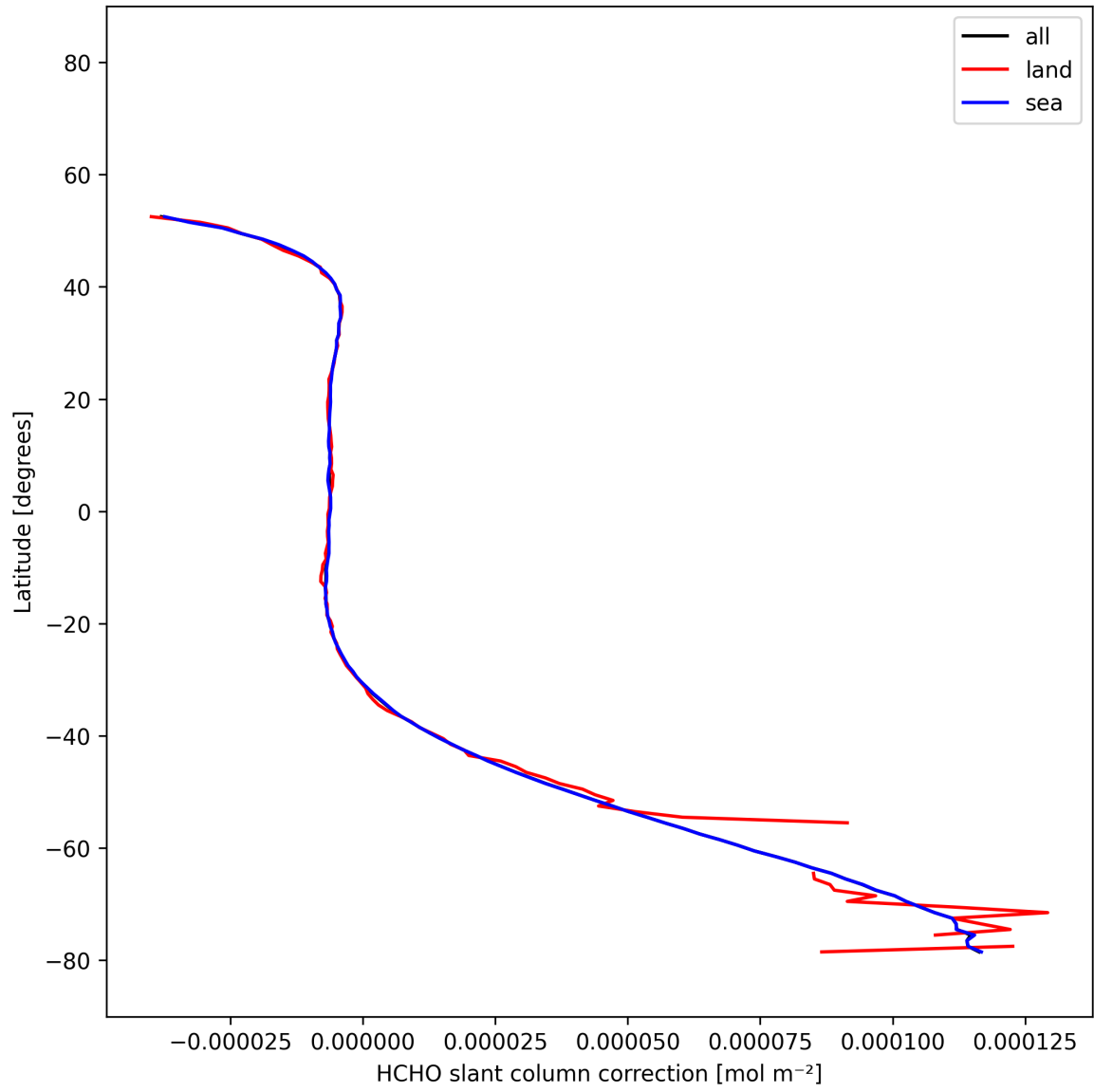
Figure 32: Zonal average of “HCHO slant column correction” for 2025-12-10 to 2025-12-11.
