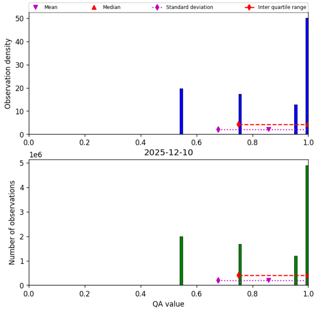
Figure 34: Histogram of “QA value” for 2025-12-10 to 2025-12-11
