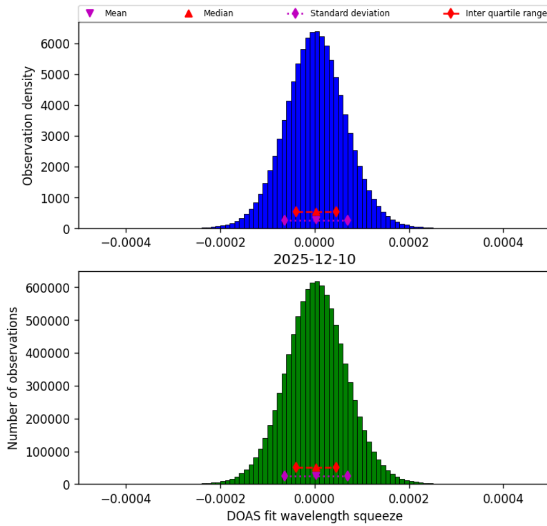
Figure 45: Histogram of “DOAS fit wavelength squeeze” for 2025-12-10 to 2025-12-11
