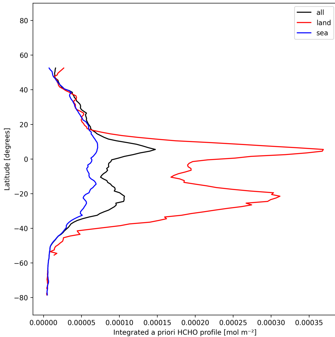
Figure 28: Zonal average of “Integrated a priori HCHO profile” for 2025-12-10 to 2025-12-11.
