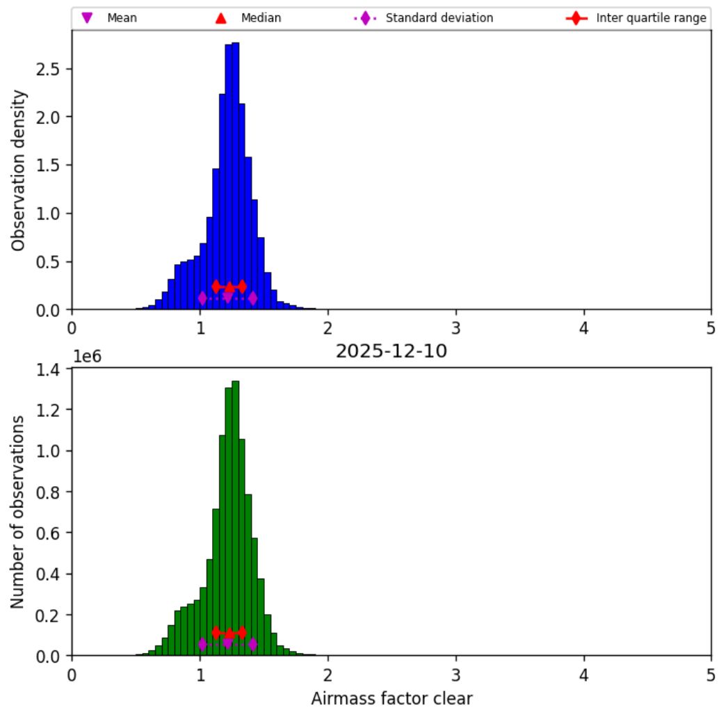
Figure 42: Histogram of “Airmass factor clear” for 2025-12-10 to 2025-12-11
