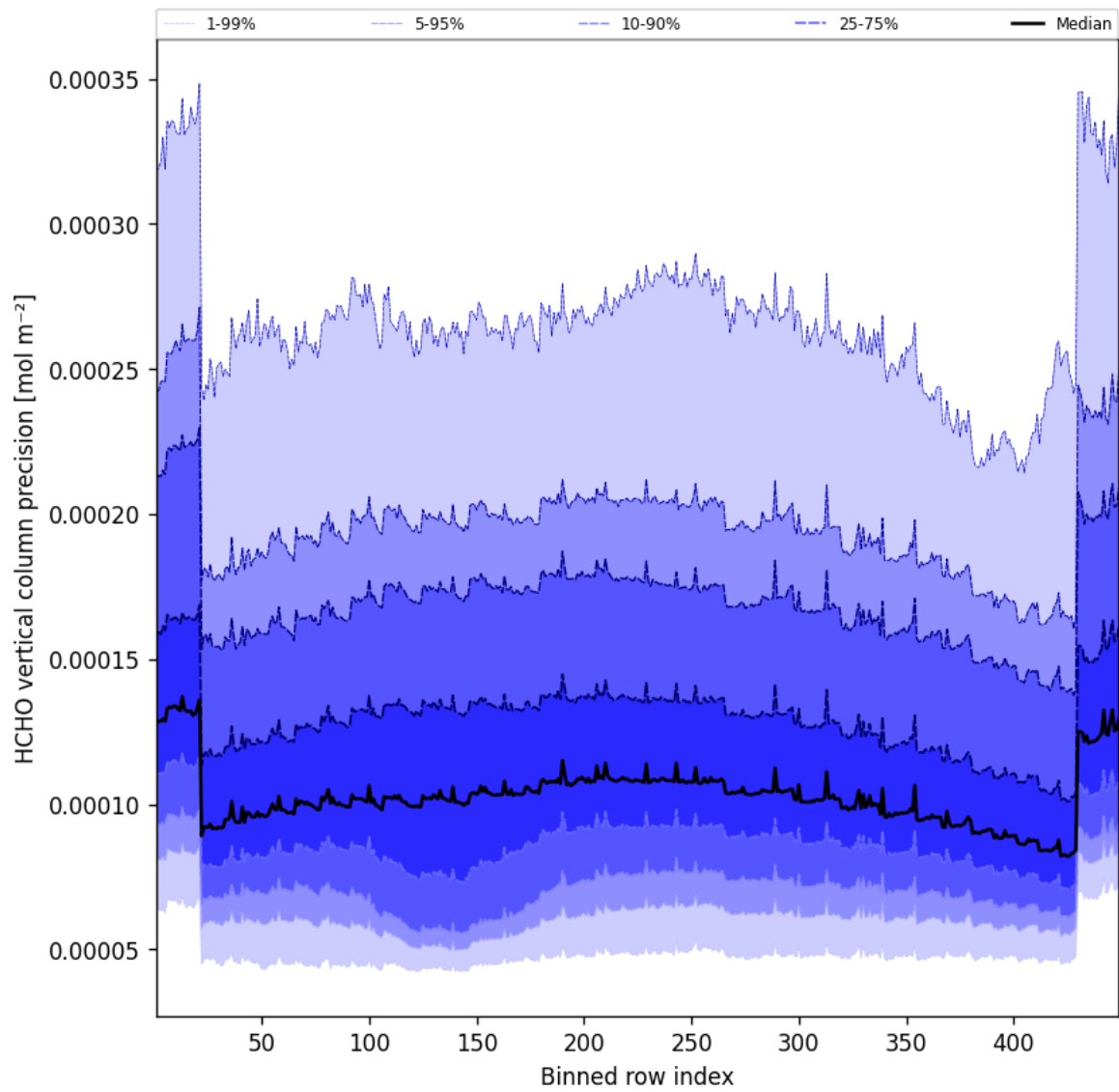
Figure 51: Along track statistics of “HCHO vertical column precision” for 2025-12-10 to 2025-12-11
