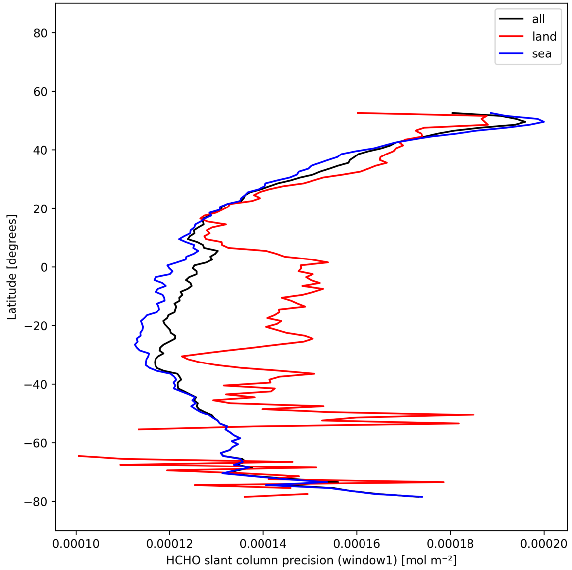
Figure 24: Zonal average of “HCHO slant column precision (window1)” for 2025-12-10 to 2025-12-11.
