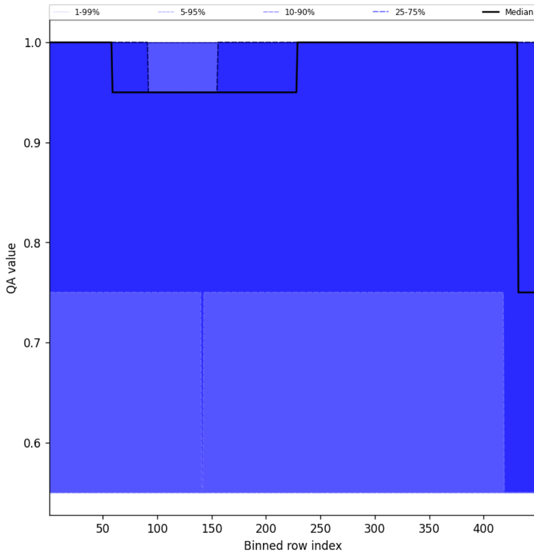
Figure 49: Along track statistics of “QA value” for 2025-12-10 to 2025-12-11
