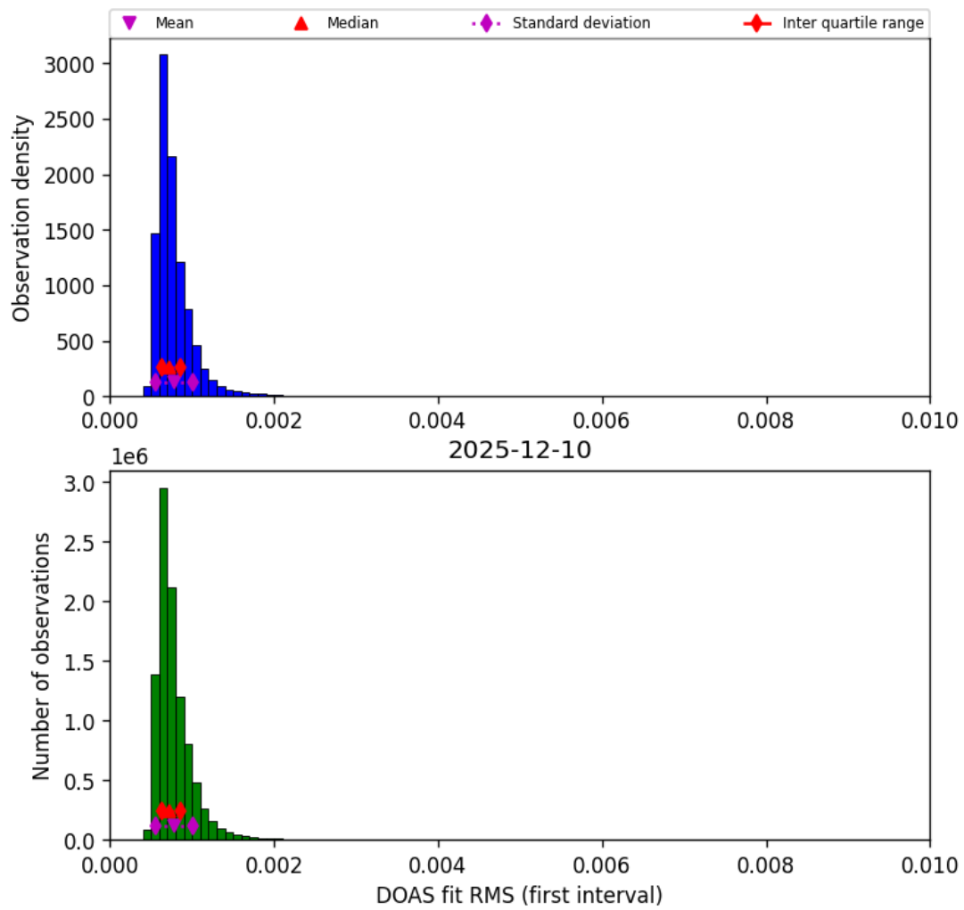
Figure 46: Histogram of “DOAS fit RMS (first interval)” for 2025-12-10 to 2025-12-11
