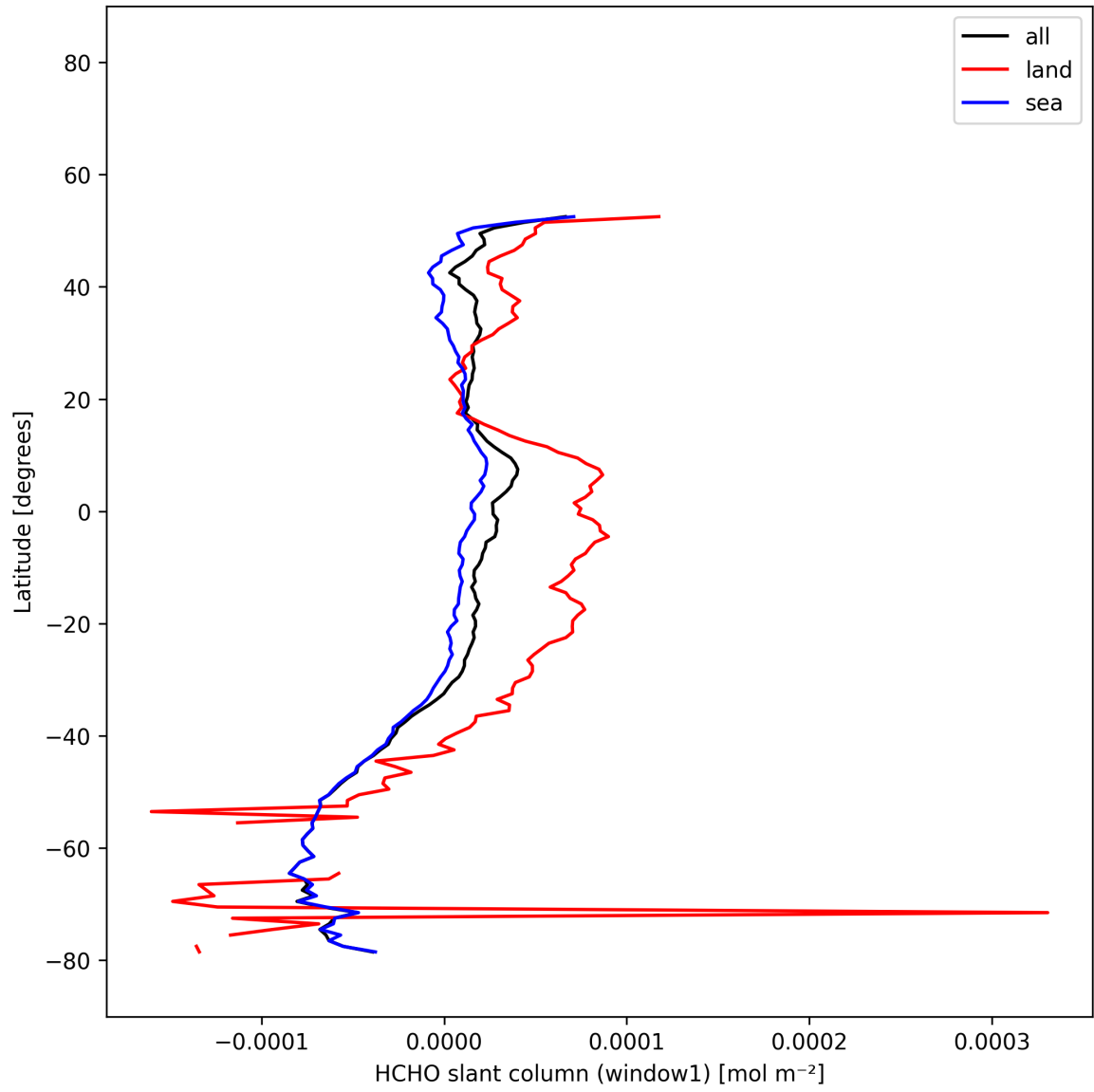
Figure 23: Zonal average of “HCHO slant column (window1)” for 2025-12-10 to 2025-12-11.
