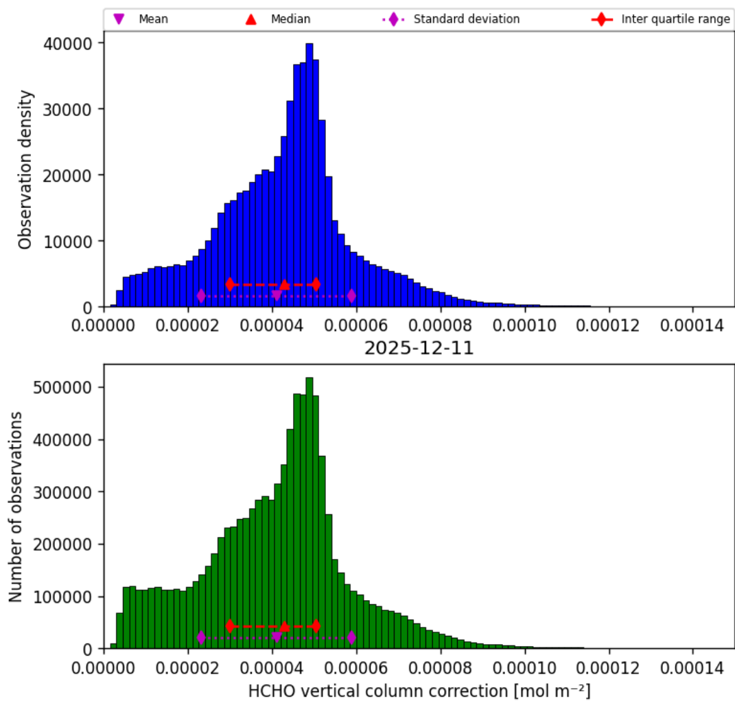
Figure 37: Histogram of “HCHO vertical column correction” for 2025-12-11 to 2025-12-12
