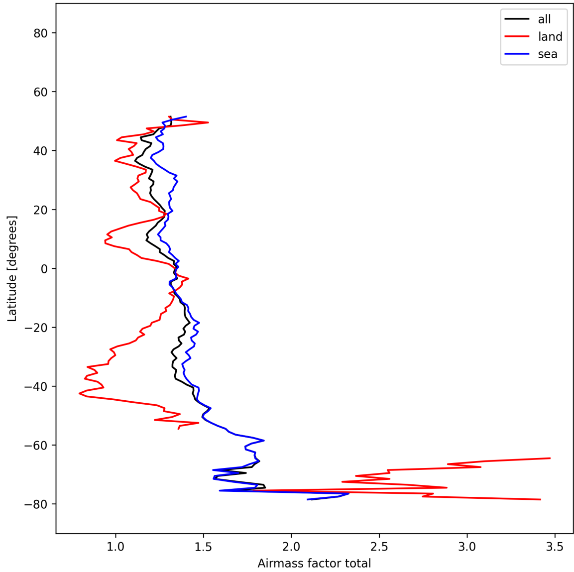
Figure 25: Zonal average of “Airmass factor total” for 2025-12-11 to 2025-12-12.
