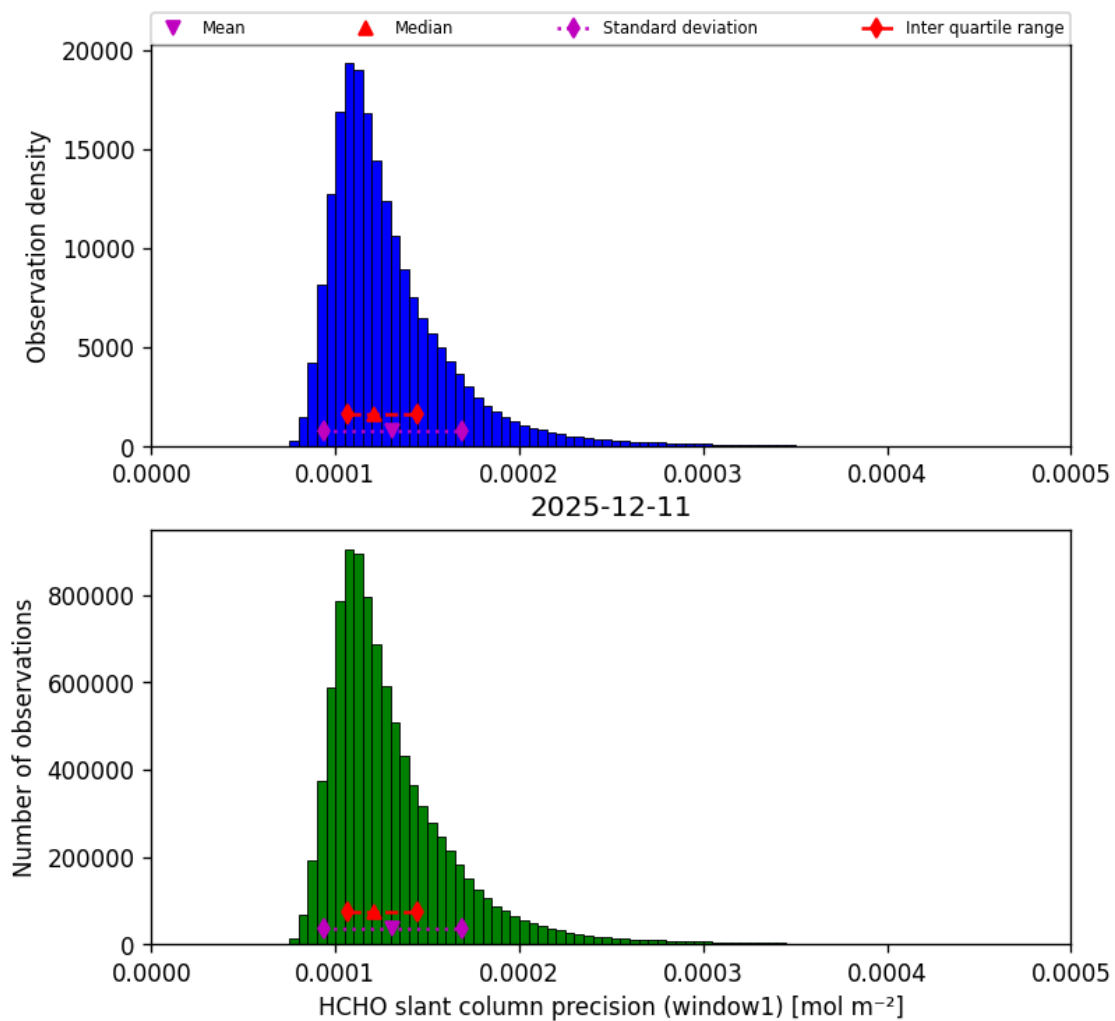
Figure 39: Histogram of “HCHO slant column precision (window1)” for 2025-12-11 to 2025-12-12
