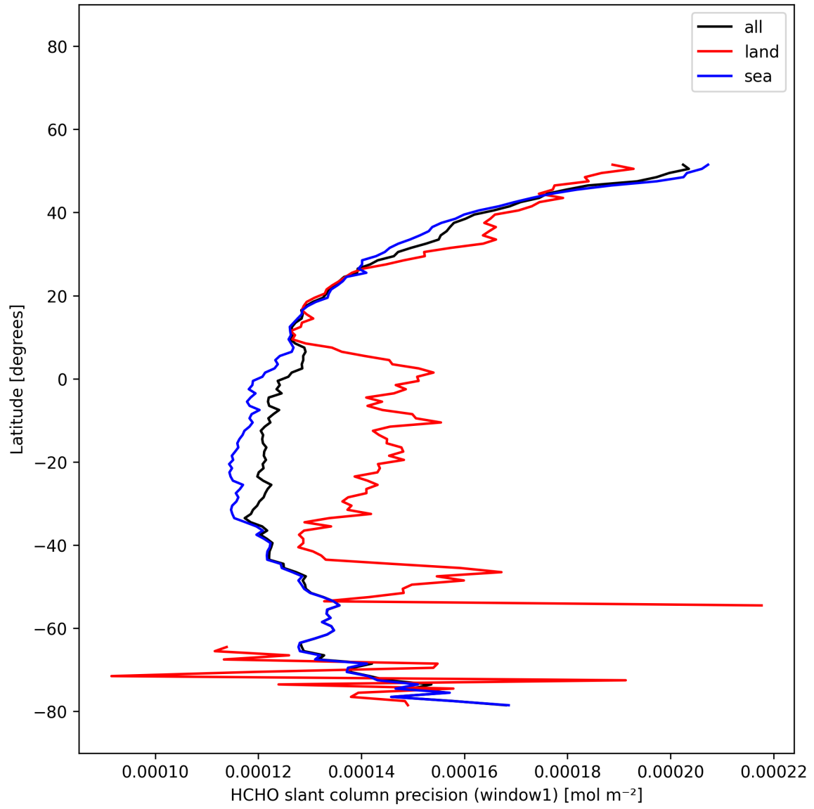
Figure 24: Zonal average of “HCHO slant column precision (window1)” for 2025-12-11 to 2025-12-12.
