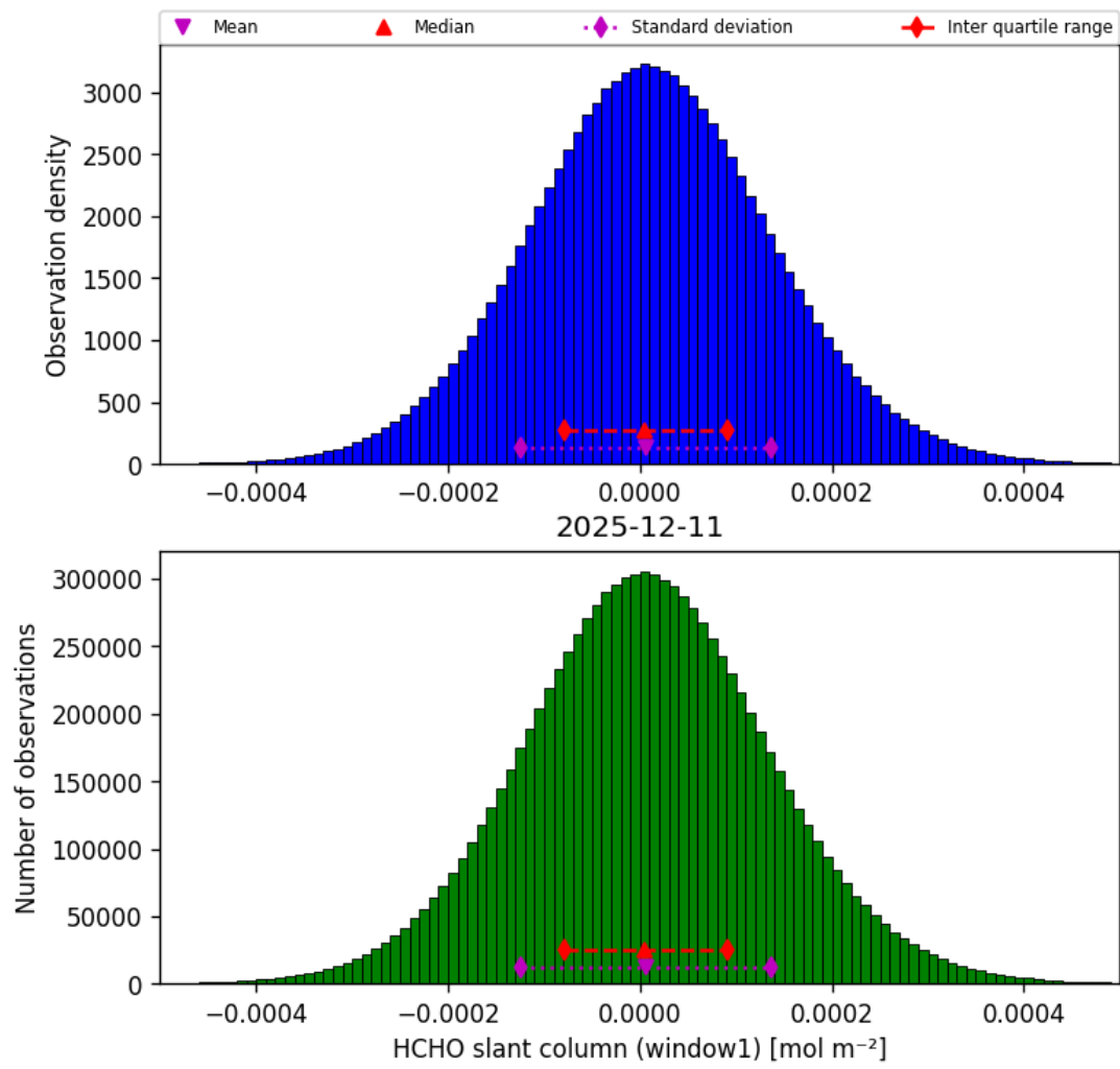
Figure 38: Histogram of “HCHO slant column (window1)” for 2025-12-11 to 2025-12-12
