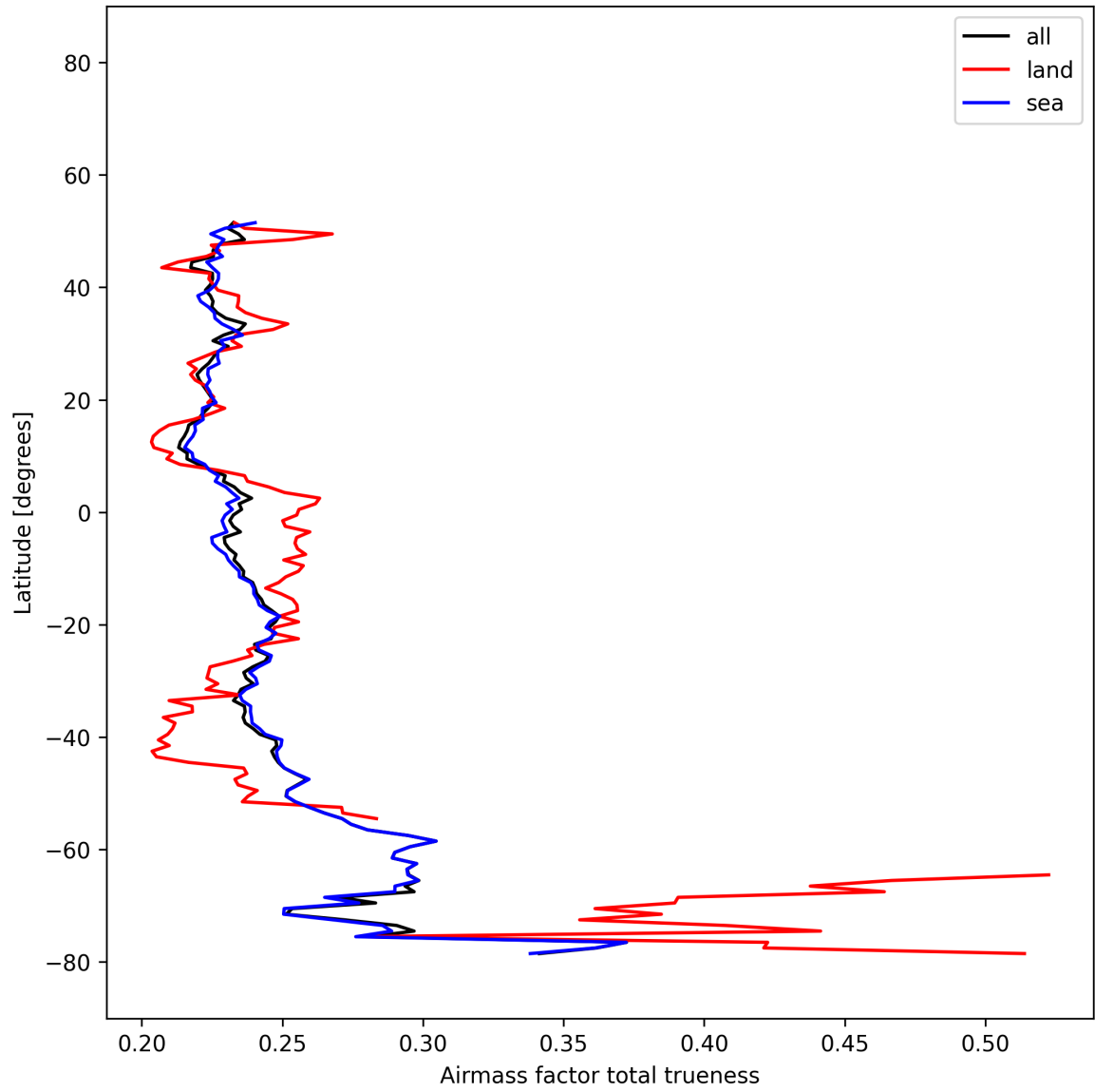
Figure 26: Zonal average of “Airmass factor total trueness” for 2025-12-11 to 2025-12-12.
