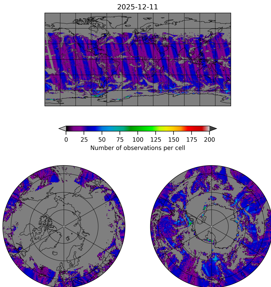
Figure 18: Map of the number of observations for 2025-12-11 to 2025-12-12
