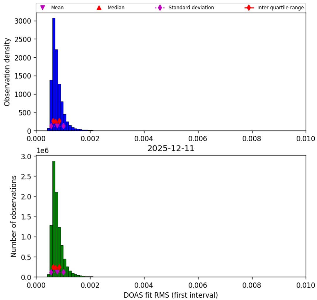
Figure 46: Histogram of “DOAS fit RMS (first interval)” for 2025-12-11 to 2025-12-12
