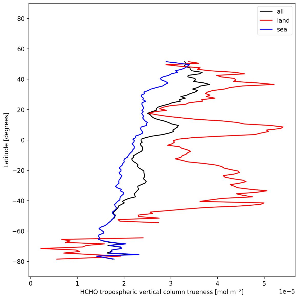
Figure 33: Zonal average of “HCHO tropospheric vertical column trueness” for 2025-12-11 to 2025-12-12.
