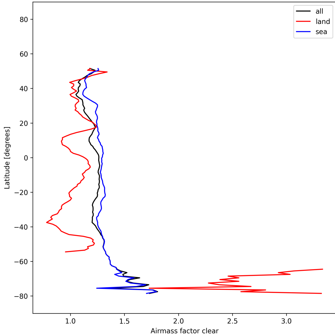
Figure 27: Zonal average of “Airmass factor clear” for 2025-12-11 to 2025-12-12.
