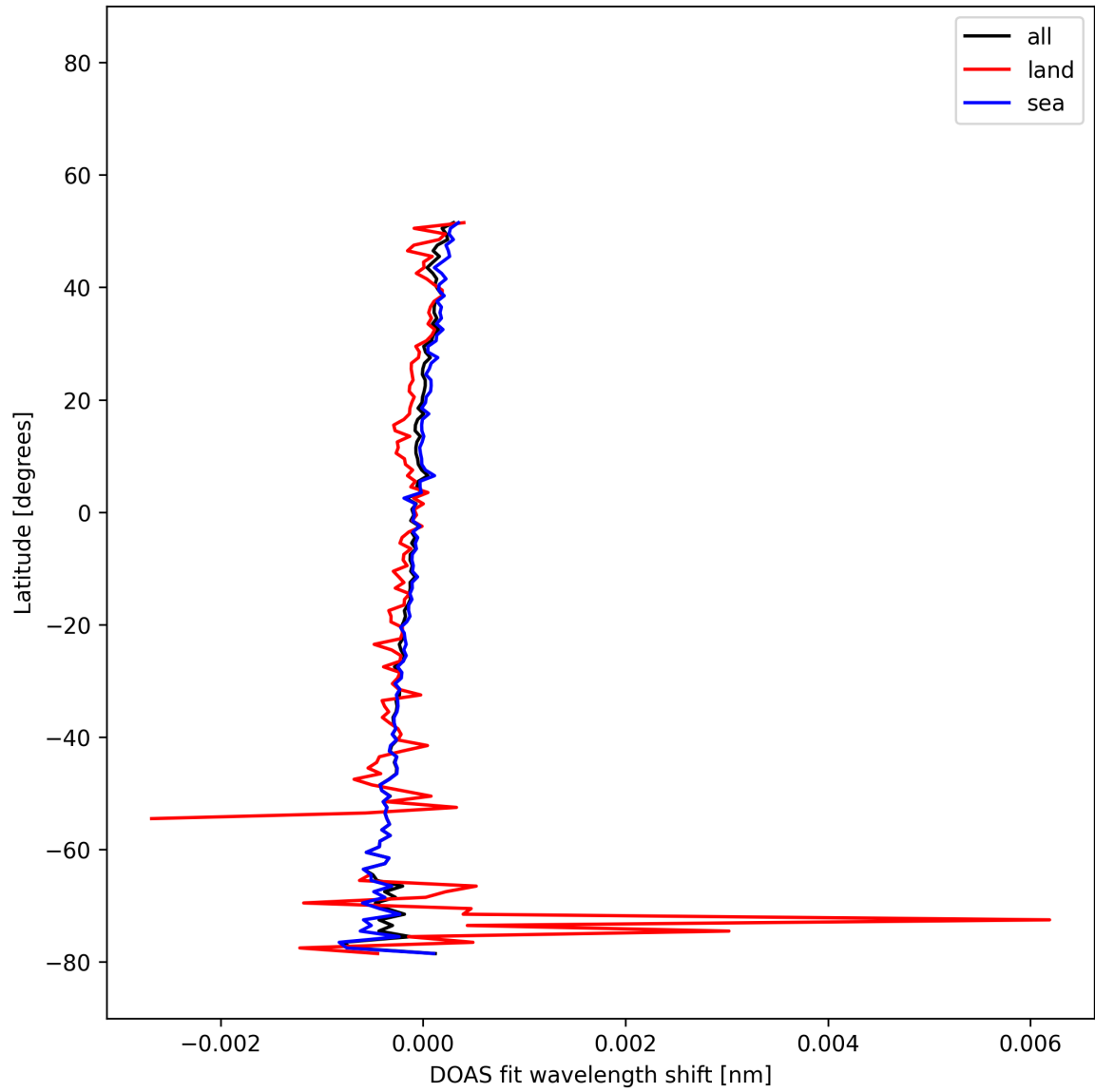
Figure 29: Zonal average of “DOAS fit wavelength shift” for 2025-12-11 to 2025-12-12.
