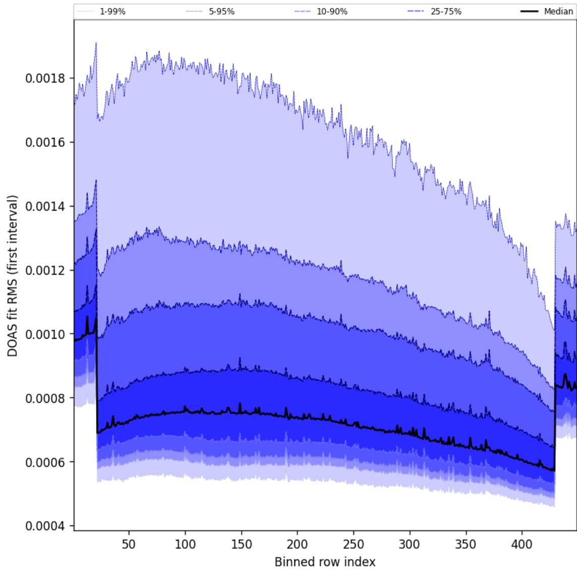
Figure 61: Along track statistics of “DOAS fit RMS (first interval)” for 2025-12-11 to 2025-12-12
