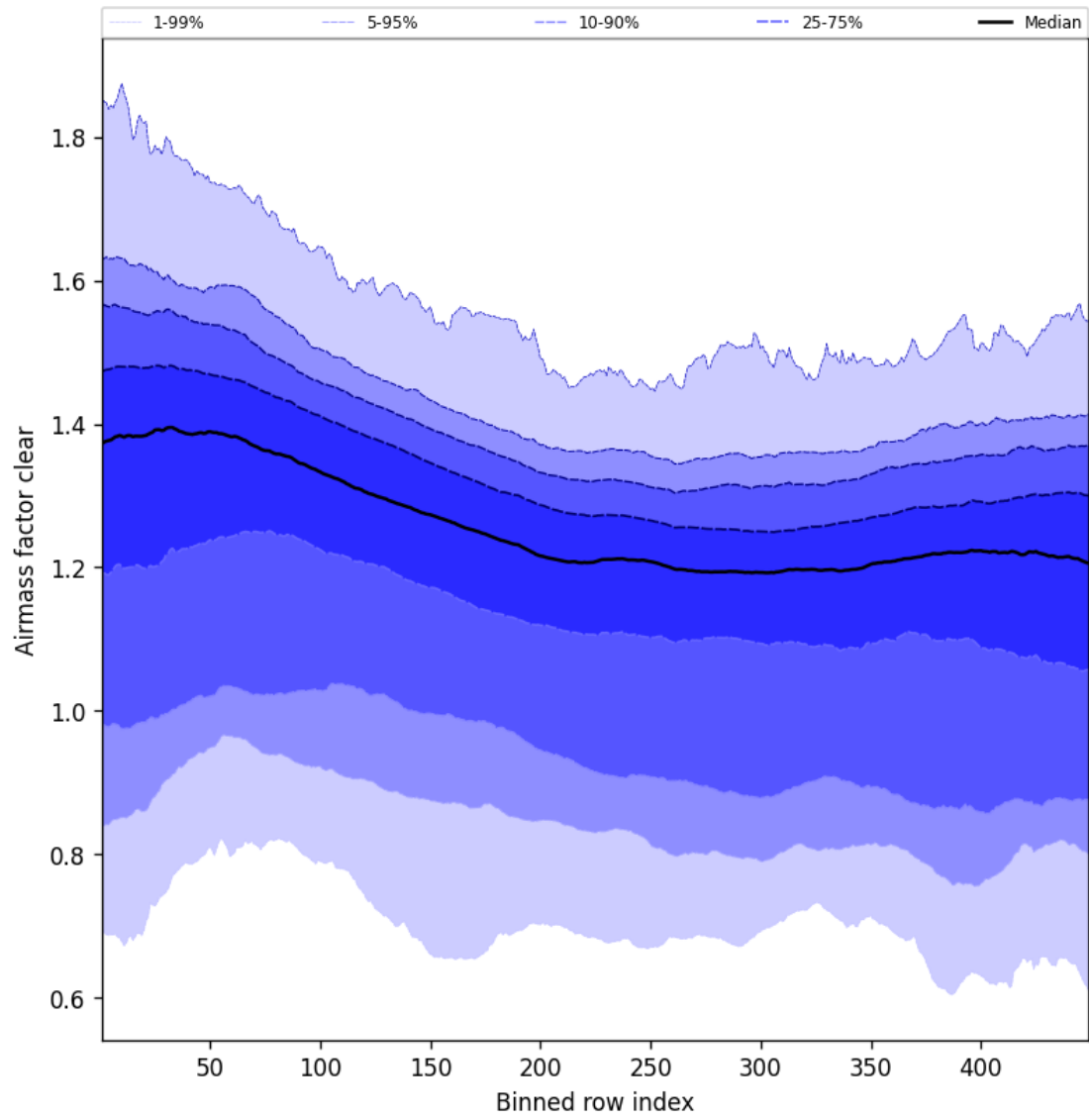
Figure 57: Along track statistics of “Airmass factor clear” for 2025-12-11 to 2025-12-12
