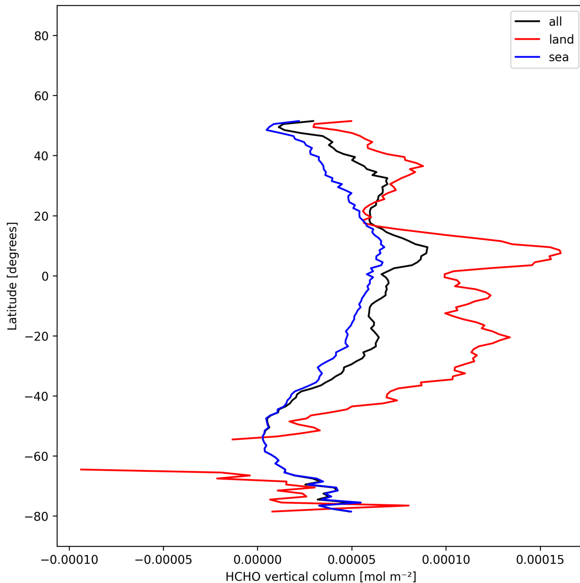
Figure 20: Zonal average of “HCHO vertical column” for 2025-12-11 to 2025-12-12.
