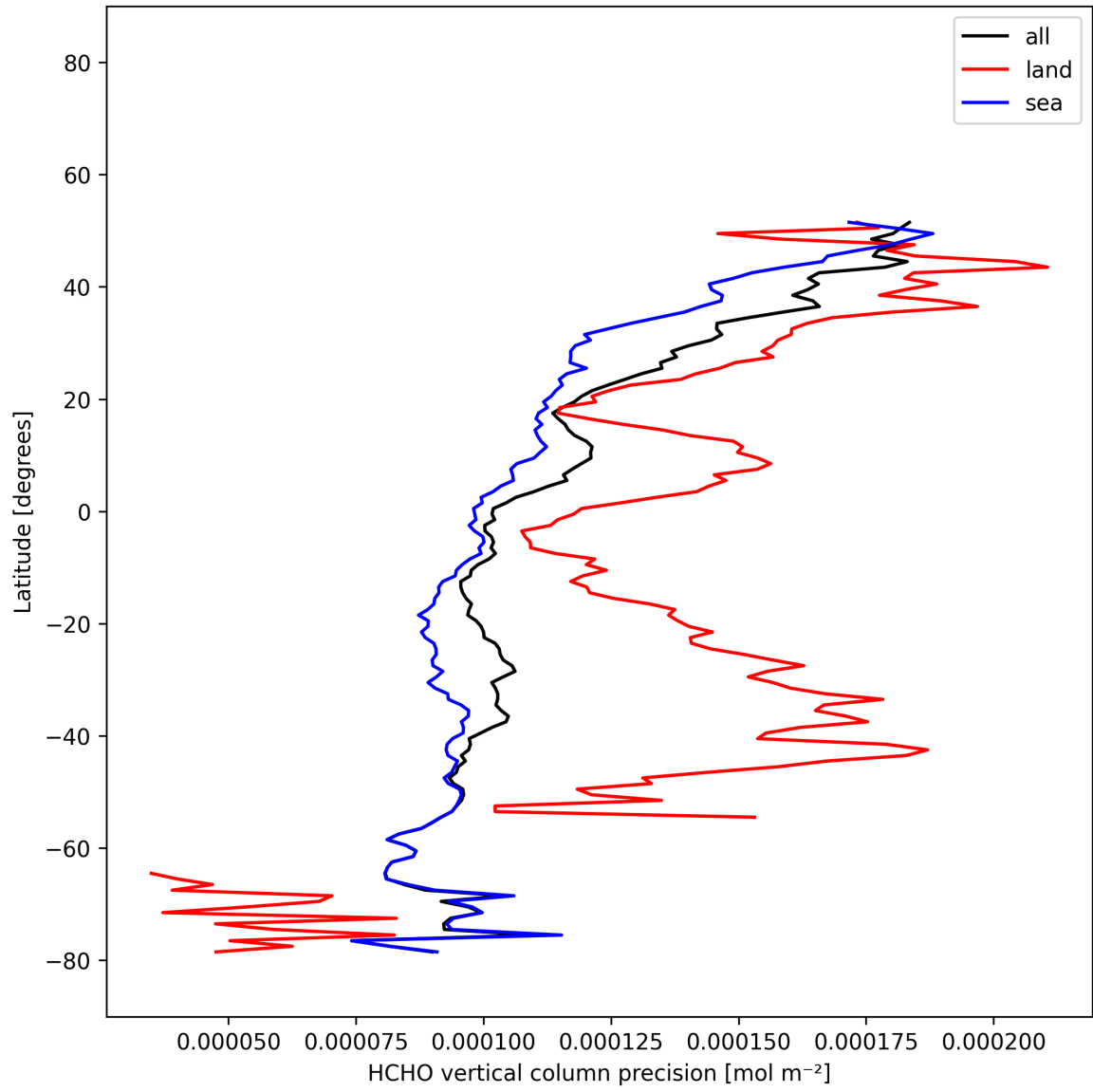
Figure 21: Zonal average of “HCHO vertical column precision” for 2025-12-11 to 2025-12-12.
