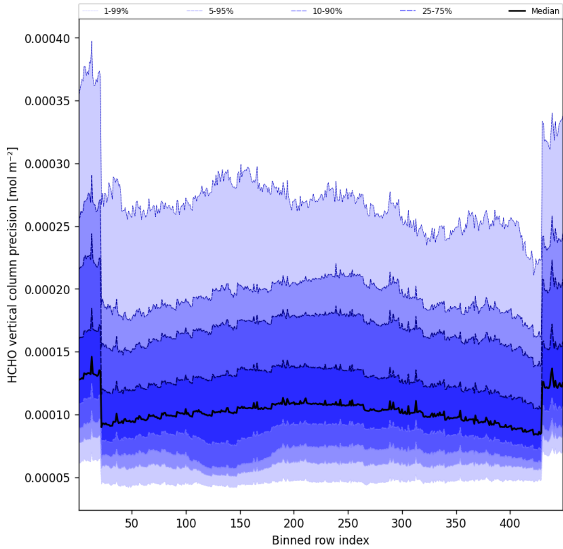
Figure 51: Along track statistics of “HCHO vertical column precision” for 2025-12-11 to 2025-12-12
