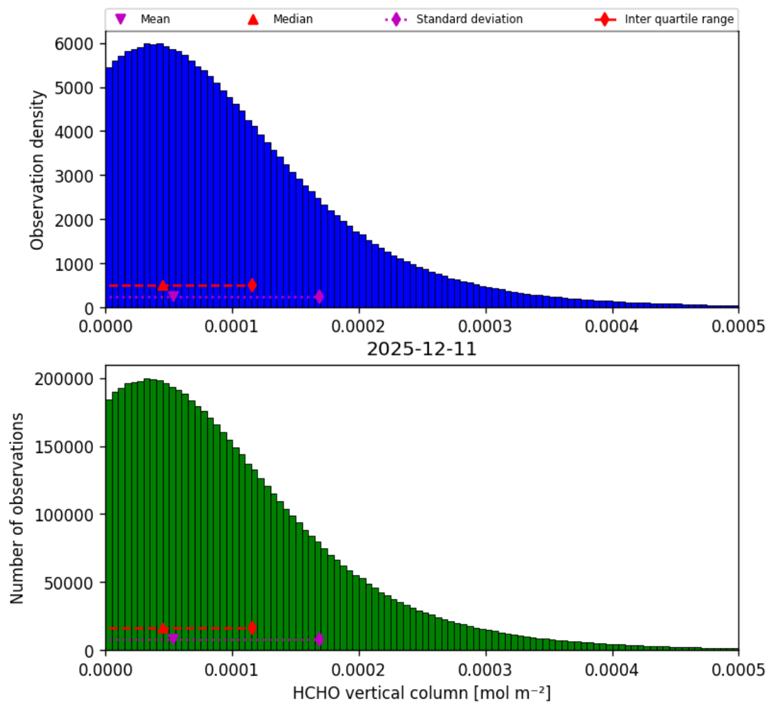
Figure 35: Histogram of “HCHO vertical column” for 2025-12-11 to 2025-12-12
