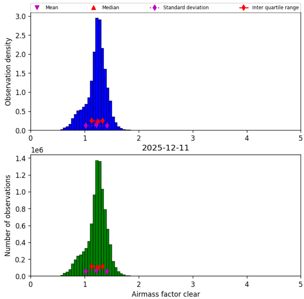
Figure 42: Histogram of “Airmass factor clear” for 2025-12-11 to 2025-12-12
