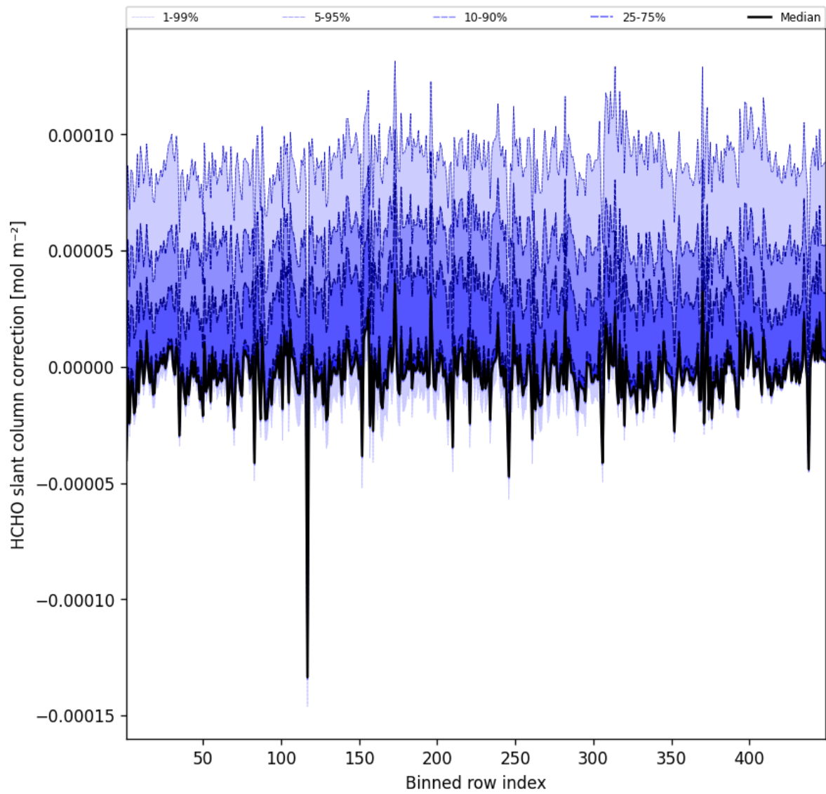
Figure 62: Along track statistics of “HCHO slant column correction” for 2025-12-11 to 2025-12-12
