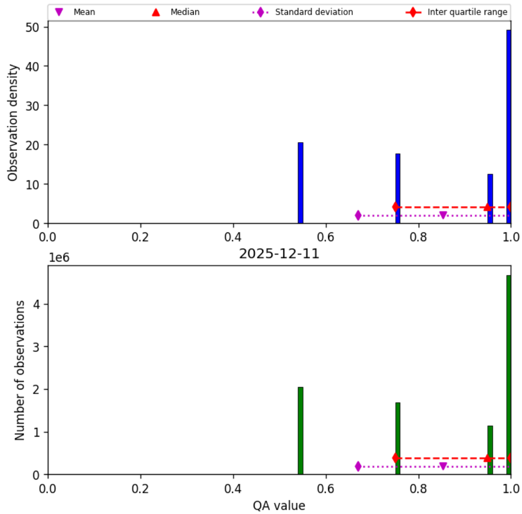
Figure 34: Histogram of “QA value” for 2025-12-11 to 2025-12-12
