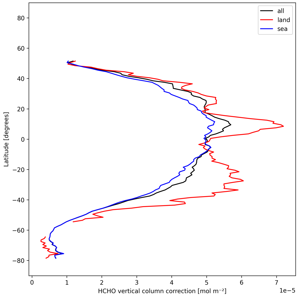
Figure 22: Zonal average of “HCHO vertical column correction” for 2025-12-11 to 2025-12-12.
