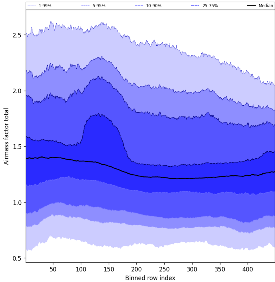
Figure 55: Along track statistics of “Airmass factor total” for 2025-12-11 to 2025-12-12
