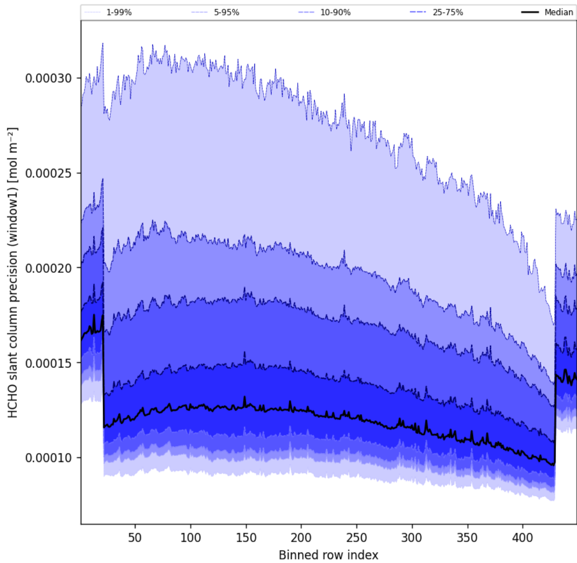
Figure 54: Along track statistics of “HCHO slant column precision (window1)” for 2025-12-11 to 2025-12-12
