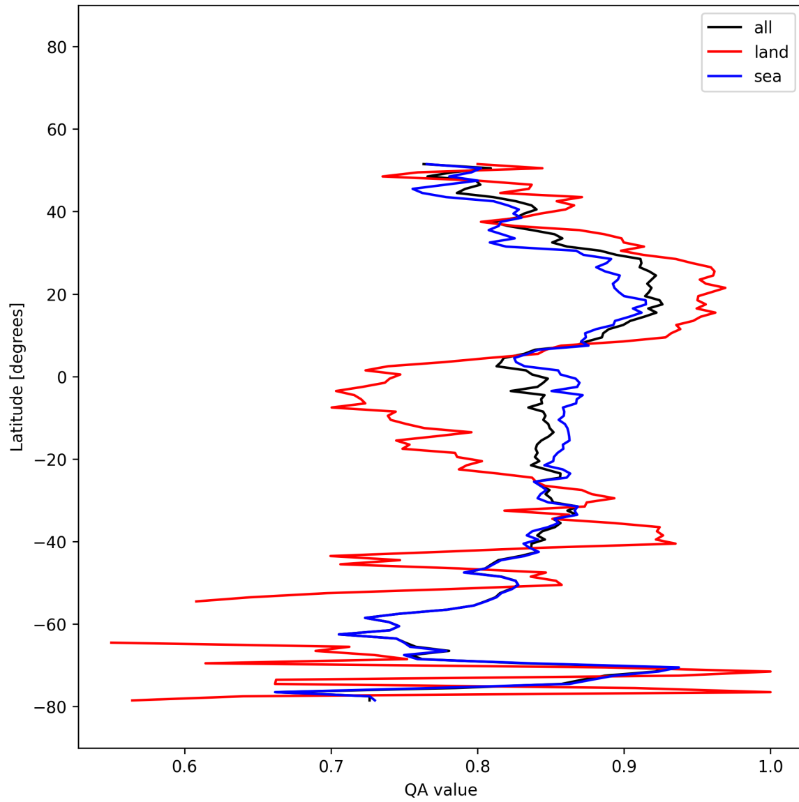
Figure 19: Zonal average of “QA value” for 2025-12-11 to 2025-12-12.
