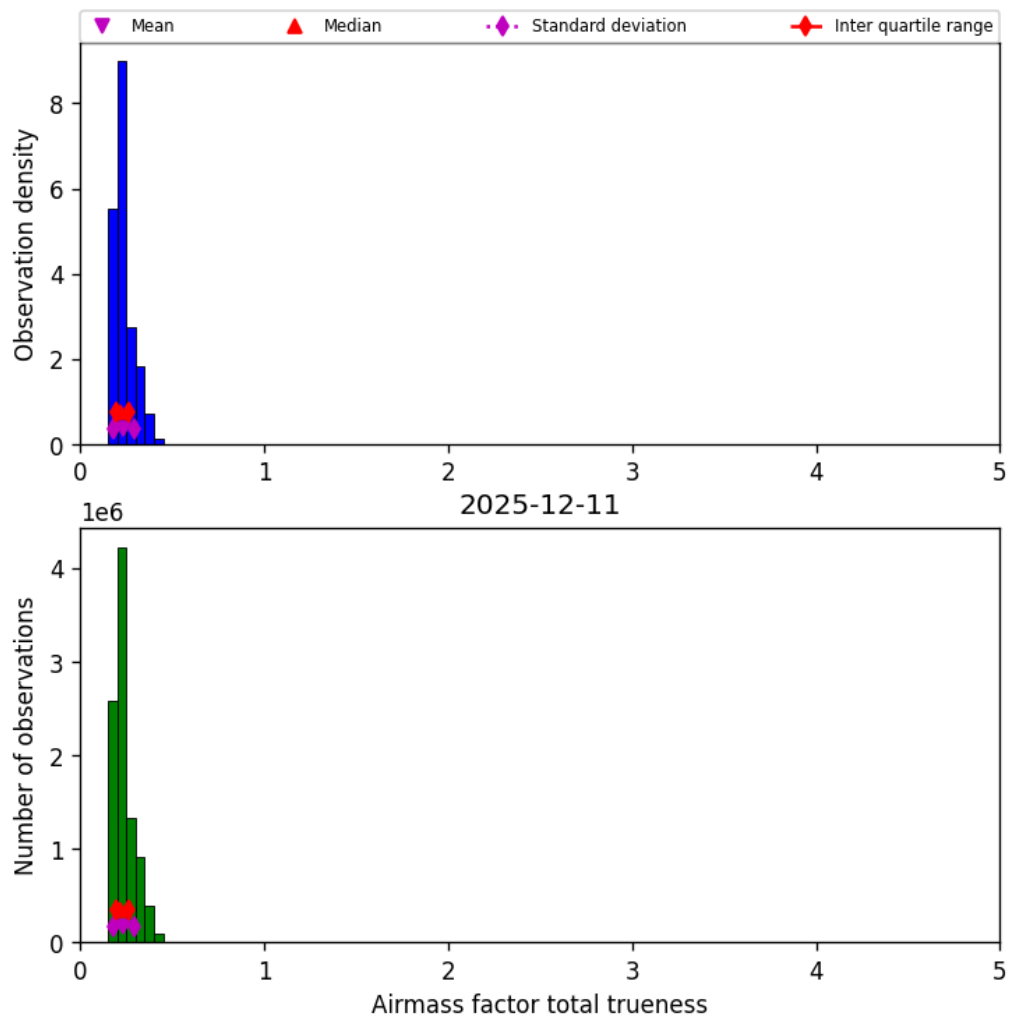
Figure 41: Histogram of “Airmass factor total trueness” for 2025-12-11 to 2025-12-12
