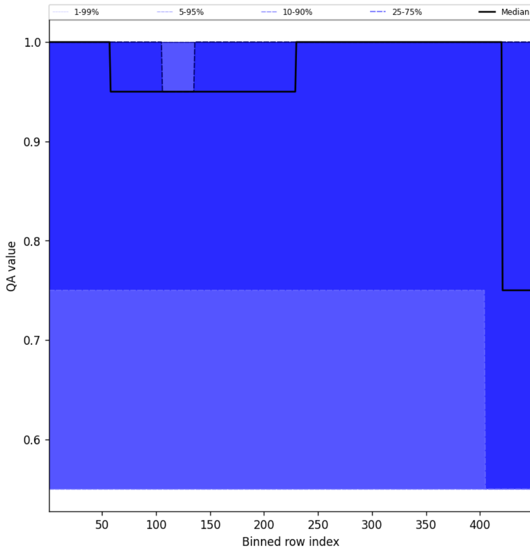
Figure 49: Along track statistics of “QA value” for 2025-12-11 to 2025-12-12
