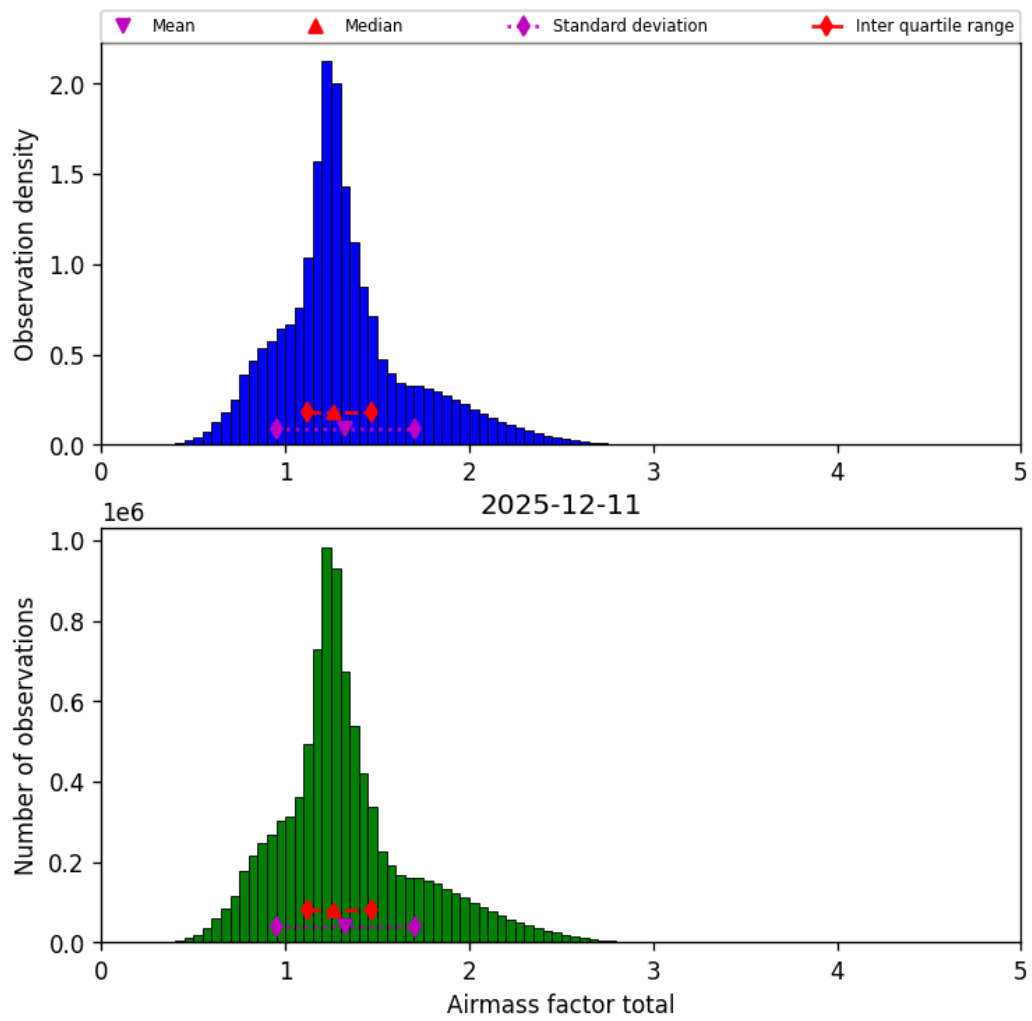
Figure 40: Histogram of “Airmass factor total” for 2025-12-11 to 2025-12-12
