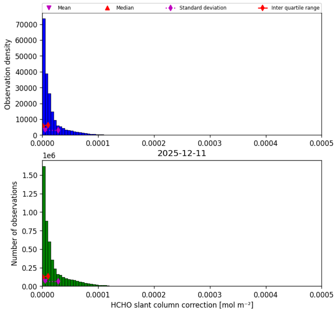
Figure 47: Histogram of “HCHO slant column correction” for 2025-12-11 to 2025-12-12
