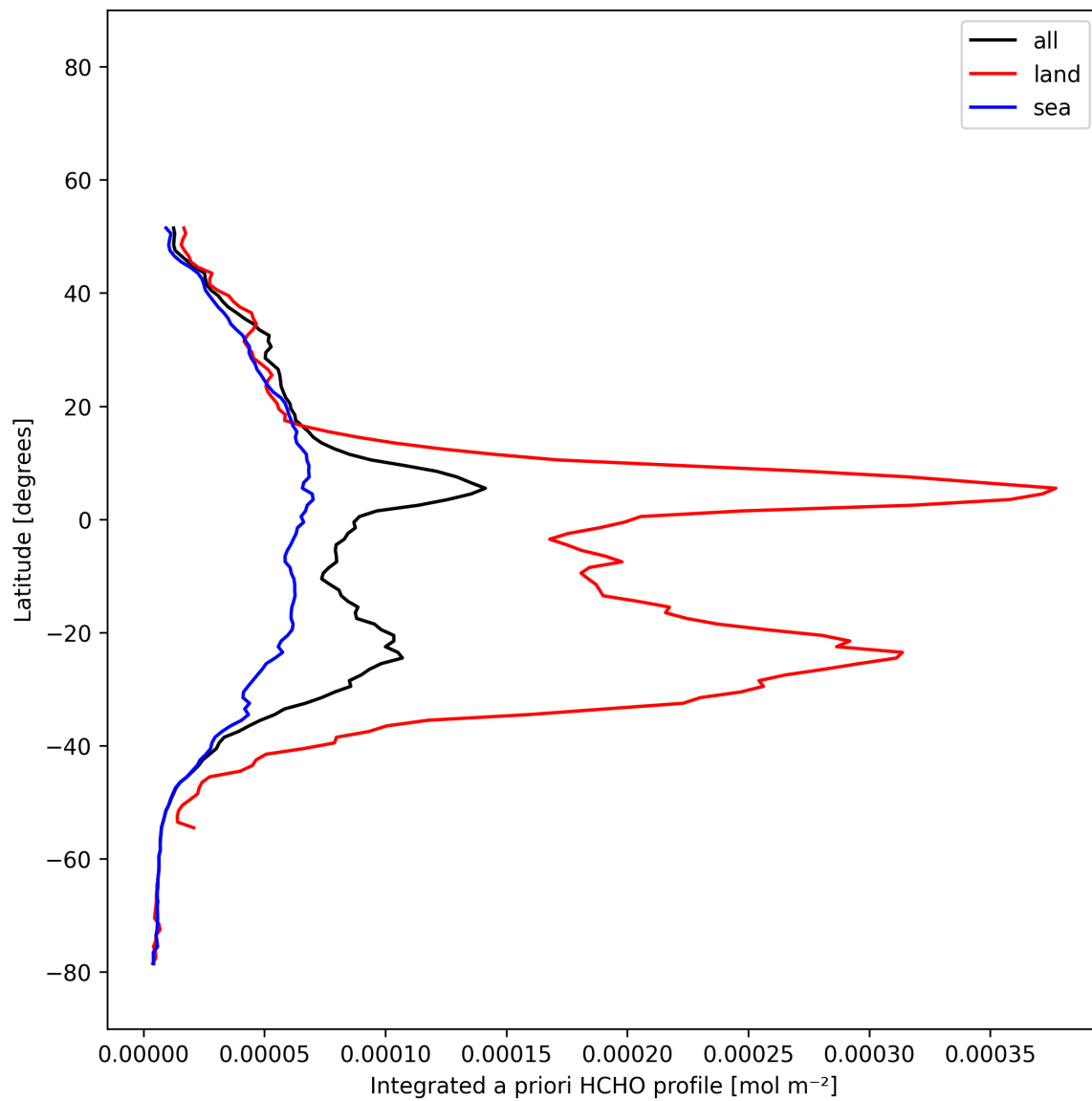
Figure 28: Zonal average of “Integrated a priori HCHO profile” for 2025-12-11 to 2025-12-12.
