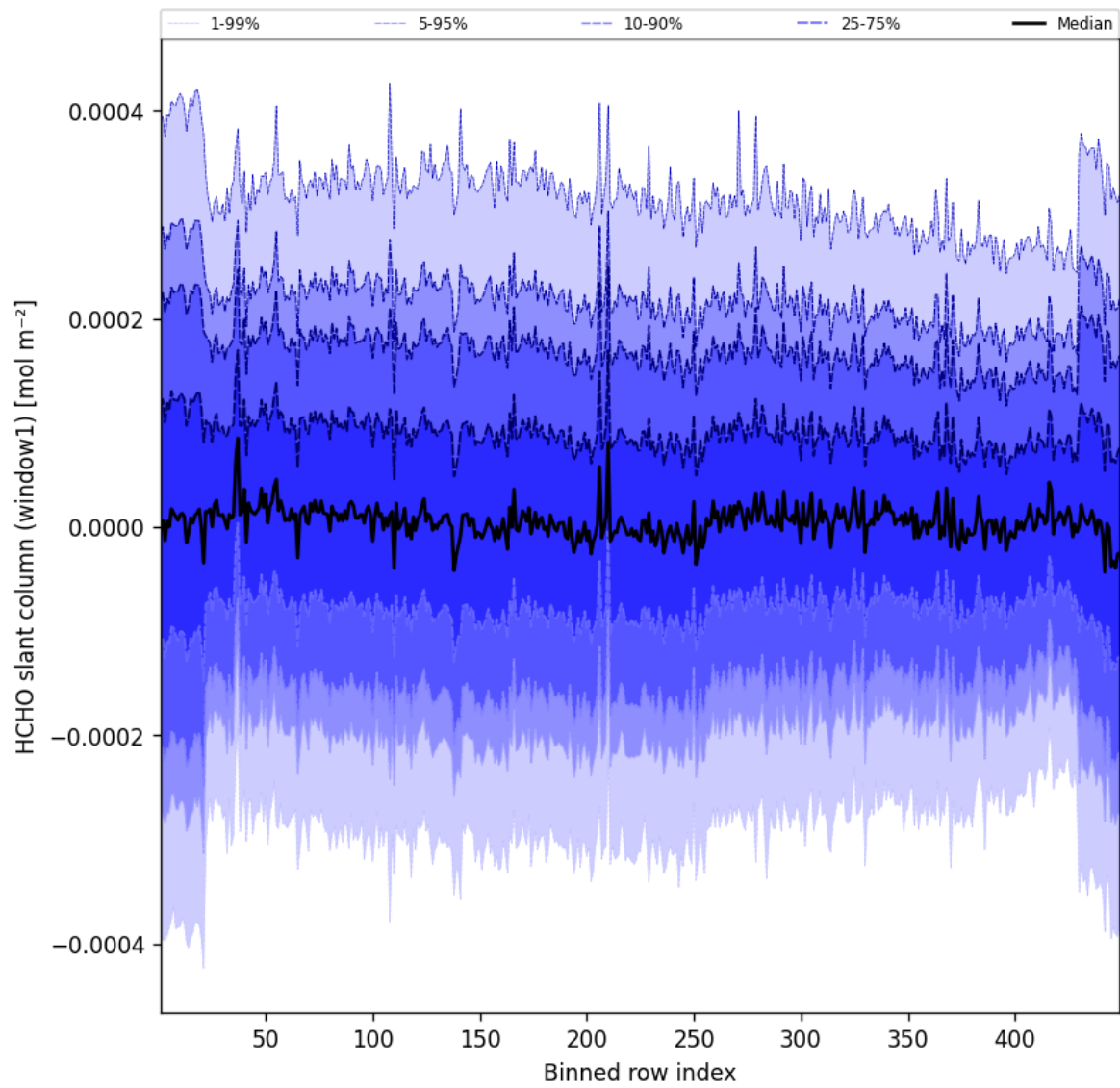
Figure 53: Along track statistics of “HCHO slant column (window1)” for 2025-12-11 to 2025-12-12
