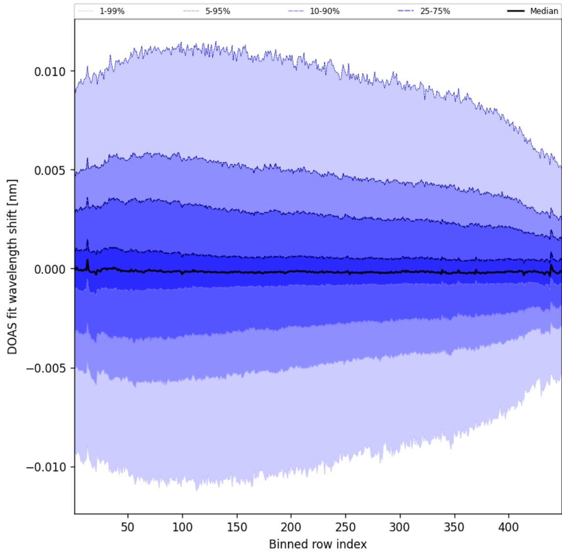
Figure 59: Along track statistics of “DOAS fit wavelength shift” for 2025-12-11 to 2025-12-12
