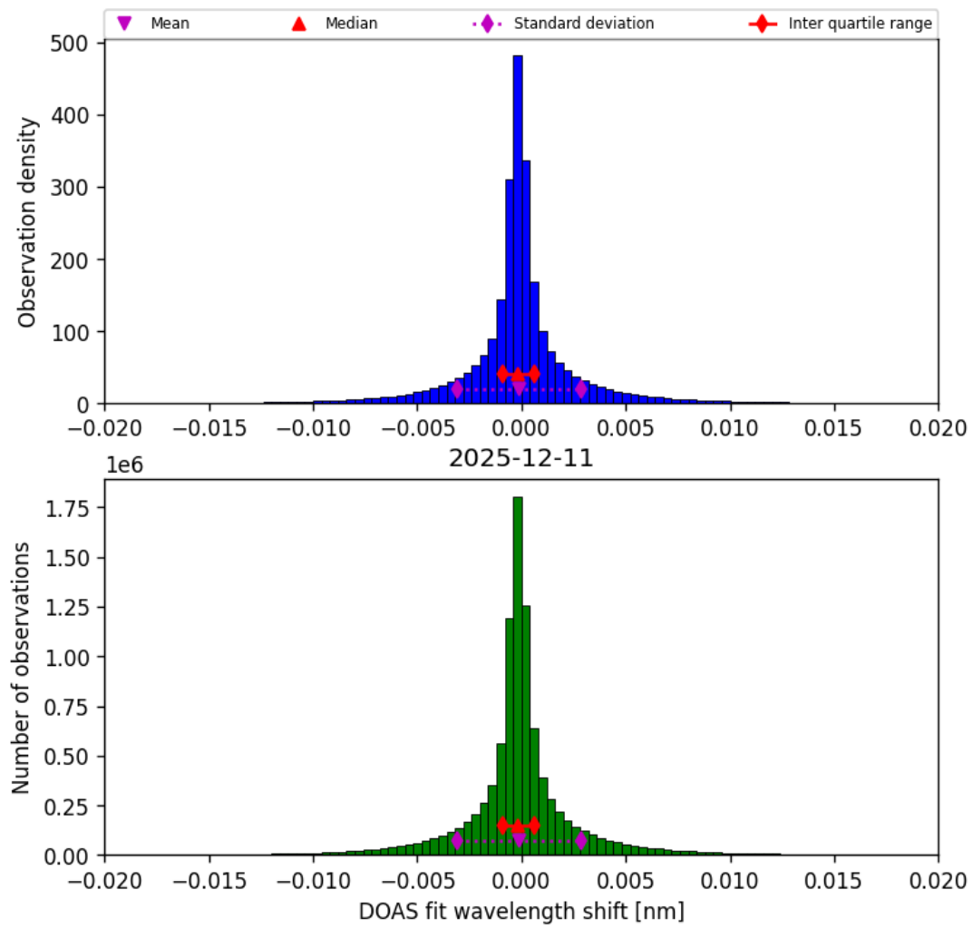
Figure 44: Histogram of “DOAS fit wavelength shift” for 2025-12-11 to 2025-12-12
