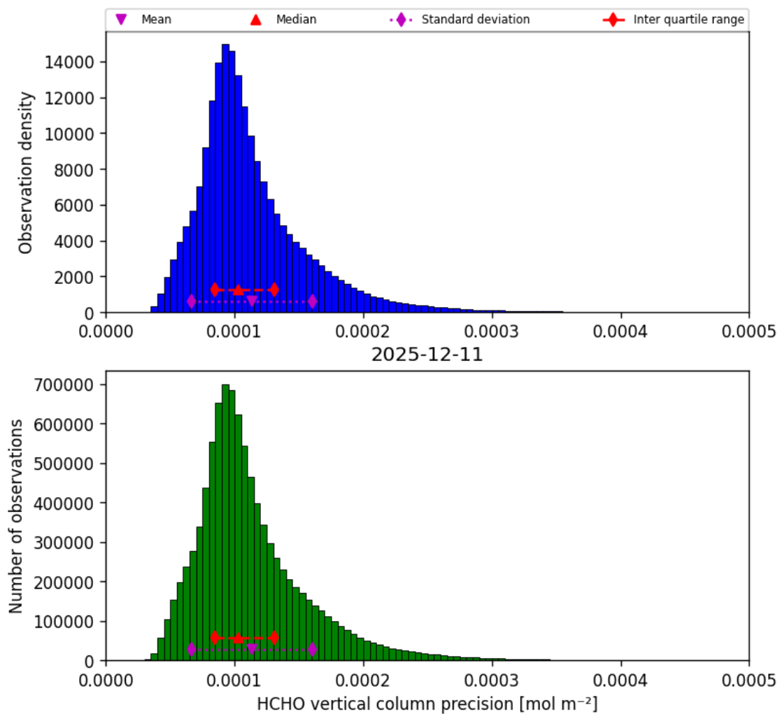
Figure 36: Histogram of “HCHO vertical column precision” for 2025-12-11 to 2025-12-12
