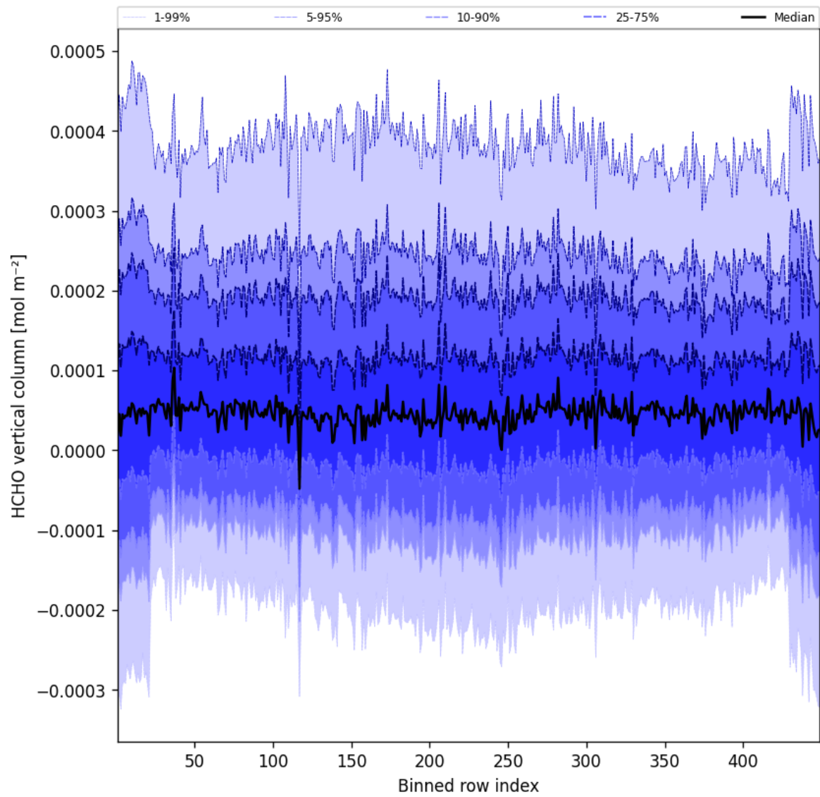
Figure 50: Along track statistics of “HCHO vertical column” for 2025-12-11 to 2025-12-12
