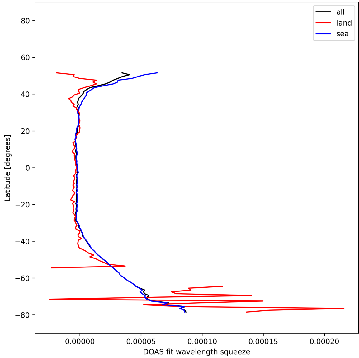
Figure 30: Zonal average of “DOAS fit wavelength squeeze” for 2025-12-11 to 2025-12-12.
