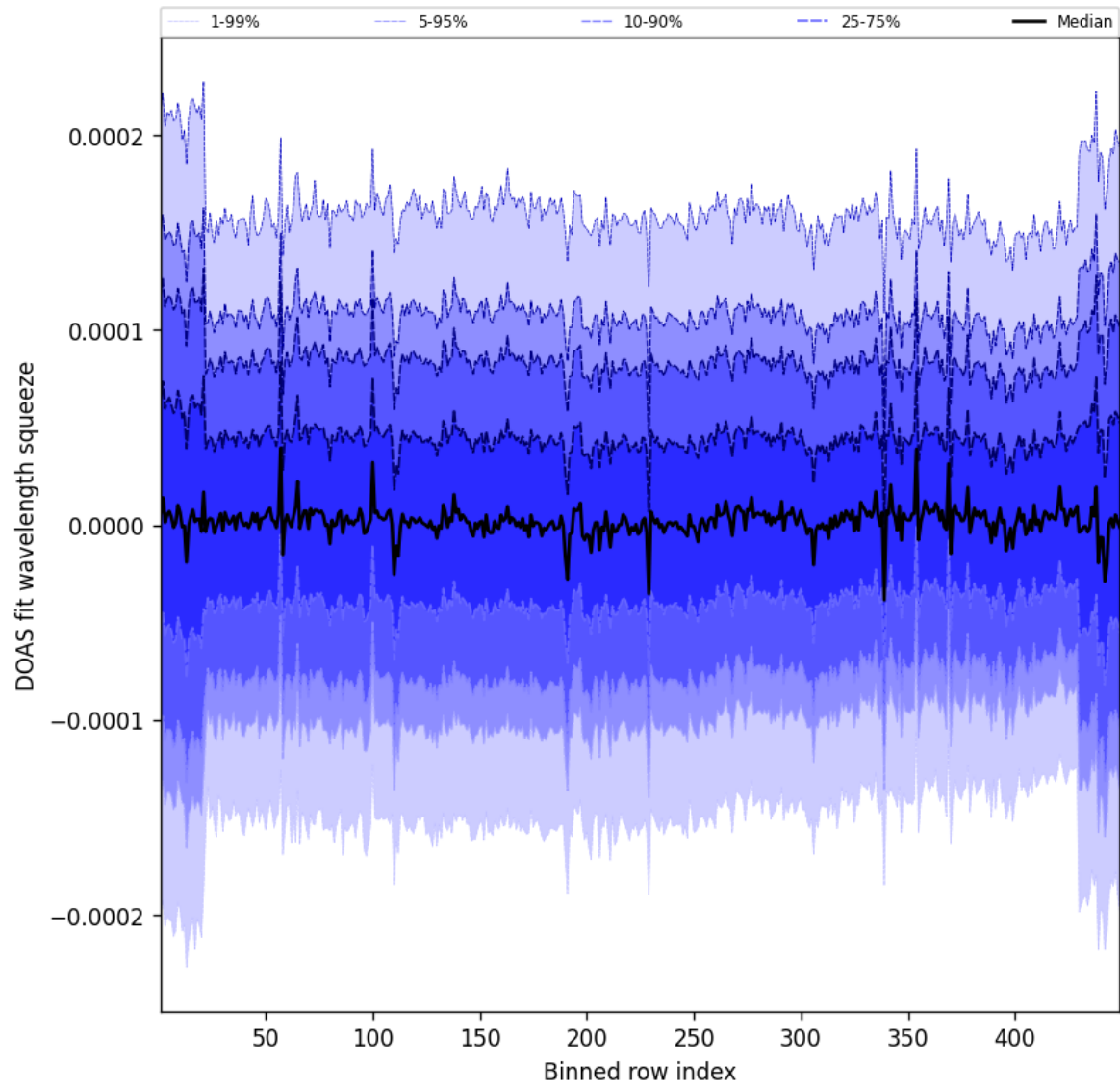
Figure 60: Along track statistics of “DOAS fit wavelength squeeze” for 2025-12-11 to 2025-12-12
