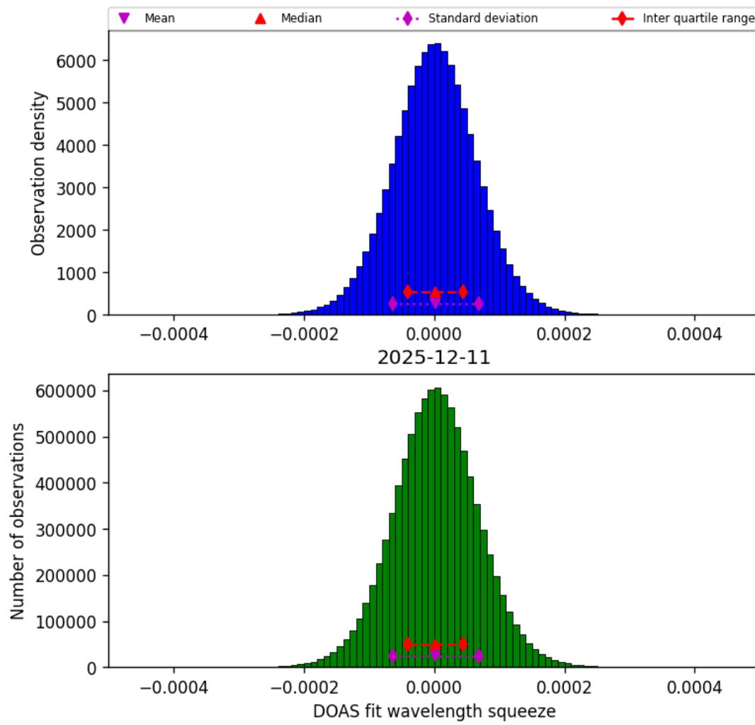
Figure 45: Histogram of “DOAS fit wavelength squeeze” for 2025-12-11 to 2025-12-12
