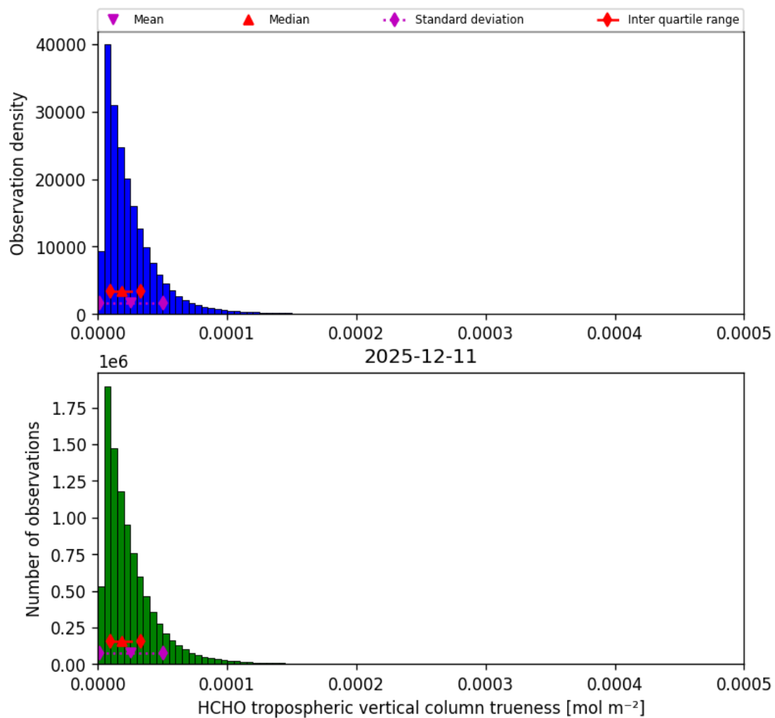
Figure 48: Histogram of “HCHO tropospheric vertical column trueness” for 2025-12-11 to 2025-12-12
