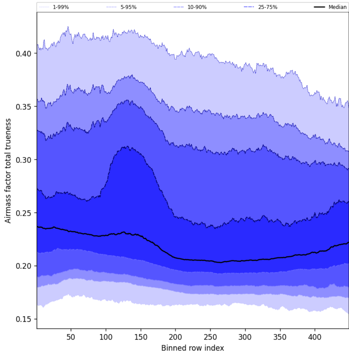
Figure 56: Along track statistics of “Airmass factor total trueness” for 2025-12-11 to 2025-12-12
