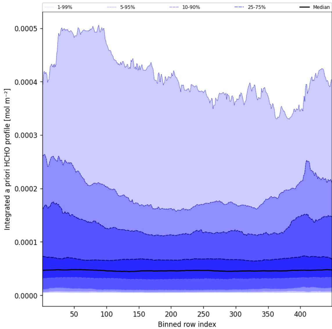
Figure 58: Along track statistics of “Integrated a priori HCHO profile” for 2025-12-11 to 2025-12-12
