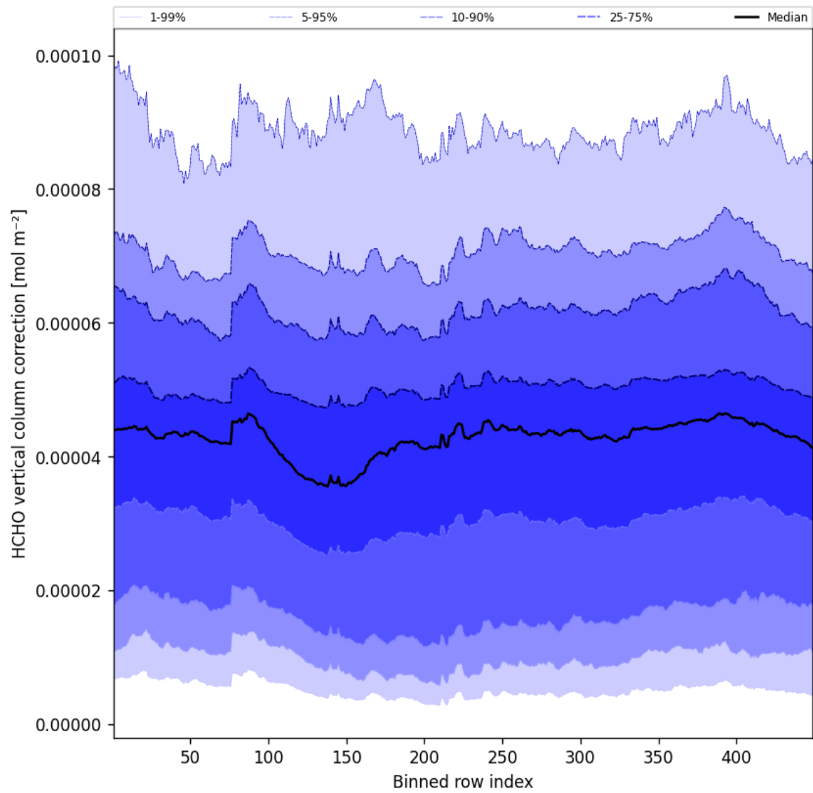
Figure 52: Along track statistics of “HCHO vertical column correction” for 2025-12-11 to 2025-12-12
