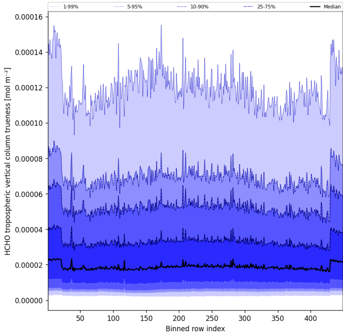
Figure 63: Along track statistics of “HCHO tropospheric vertical column trueness” for 2025-12-11 to 2025-12-12
