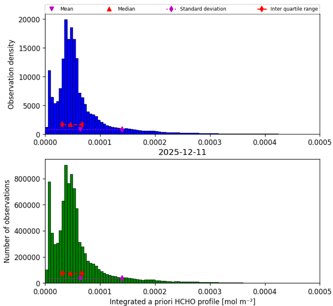
Figure 43: Histogram of “Integrated a priori HCHO profile” for 2025-12-11 to 2025-12-12
