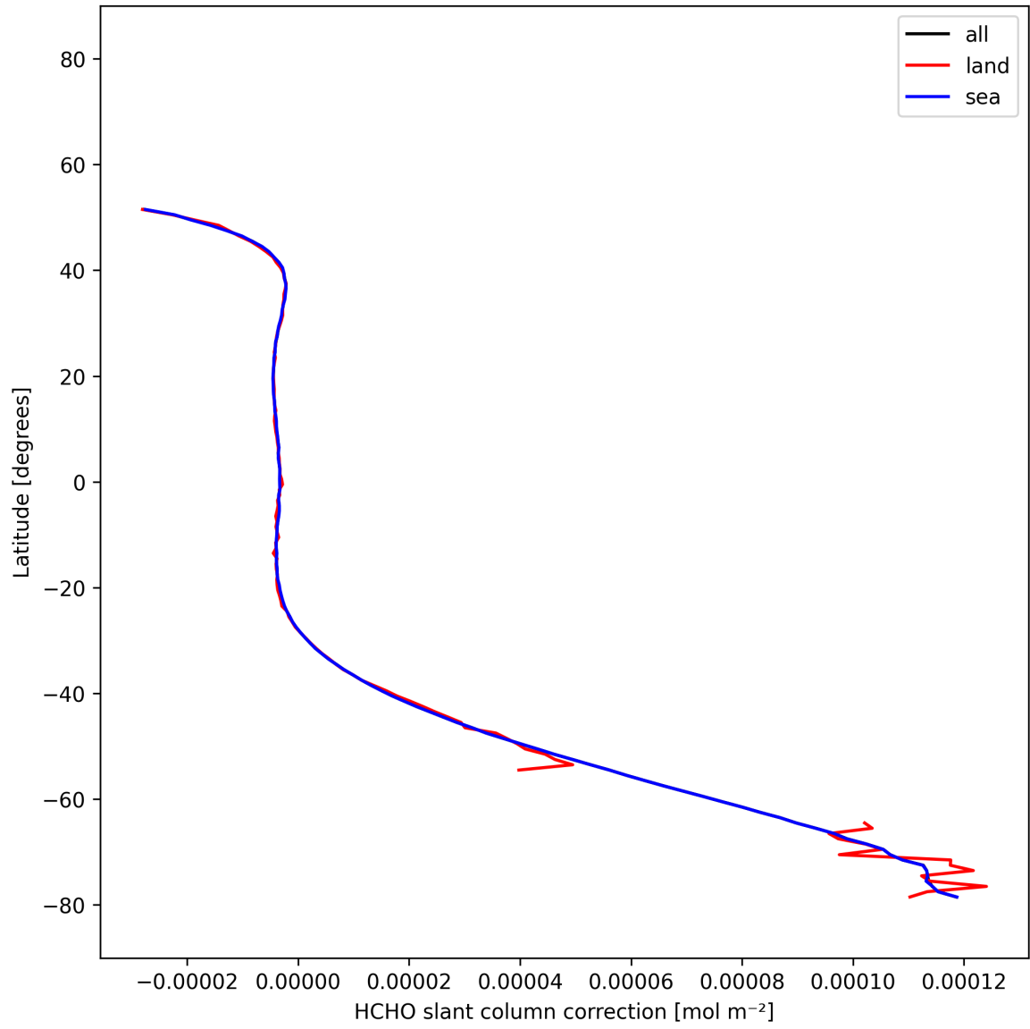
Figure 32: Zonal average of “HCHO slant column correction” for 2025-12-11 to 2025-12-12.
