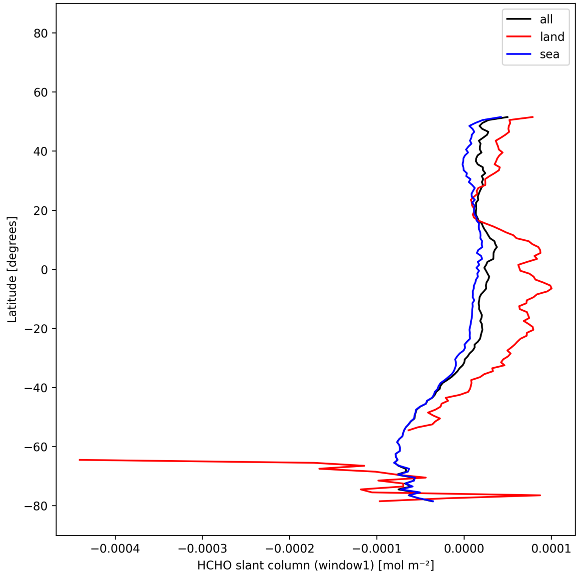
Figure 23: Zonal average of “HCHO slant column (window1)” for 2025-12-11 to 2025-12-12.
