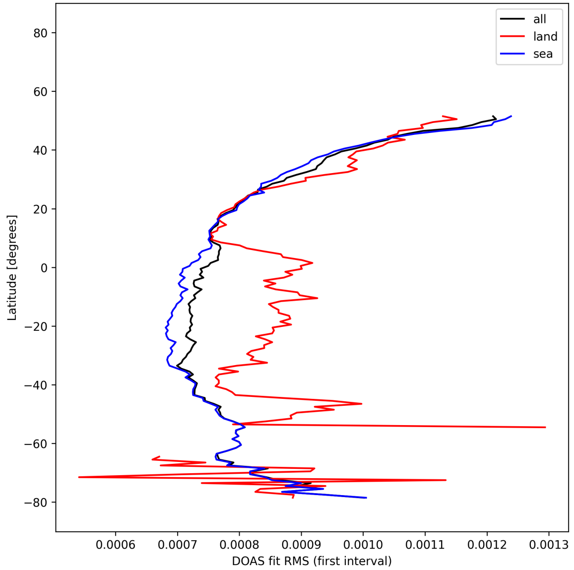
Figure 31: Zonal average of “DOAS fit RMS (first interval)” for 2025-12-11 to 2025-12-12.
