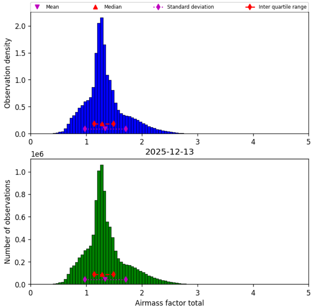
Figure 40: Histogram of “Airmass factor total” for 2025-12-13 to 2025-12-14
