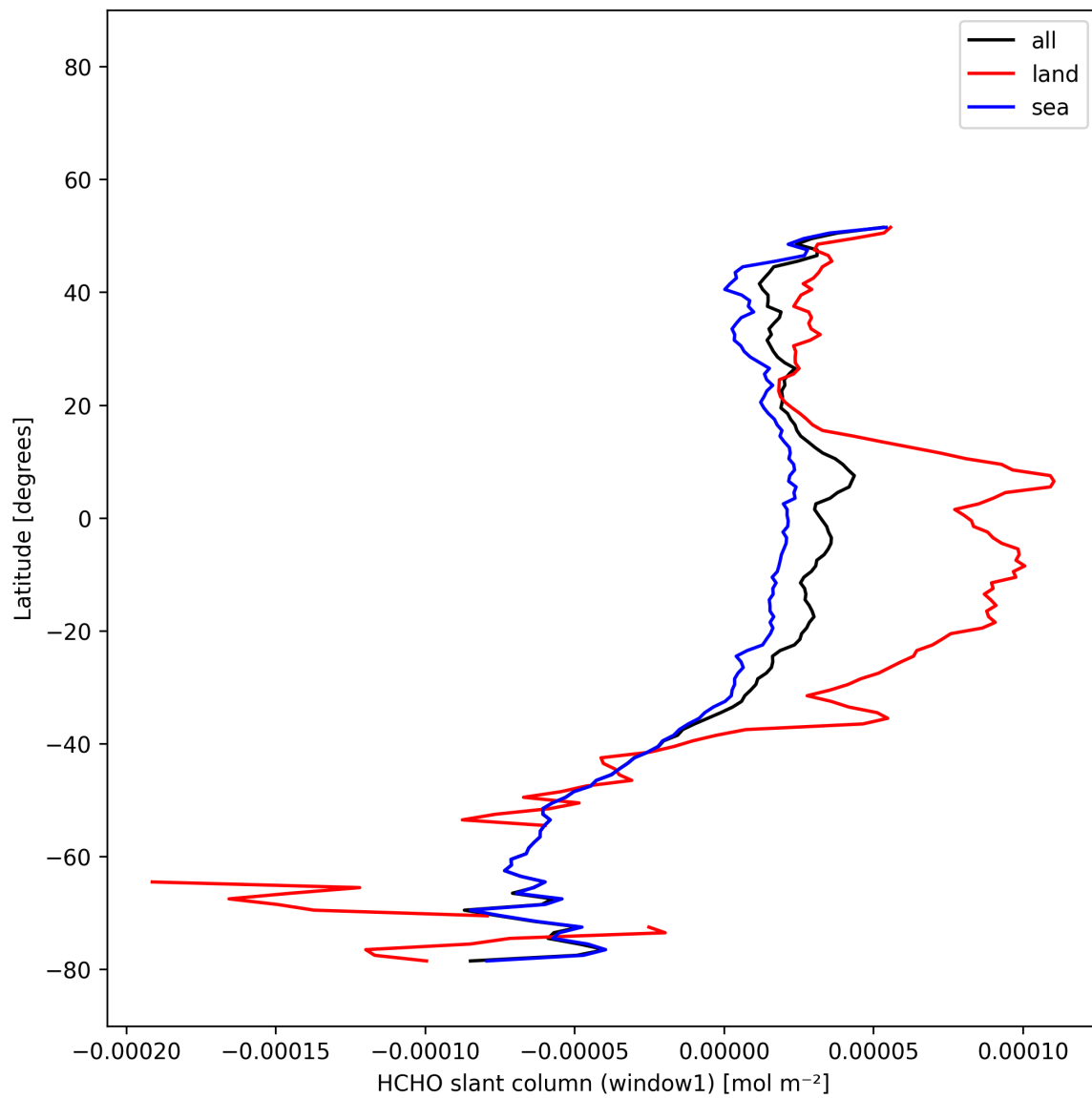
Figure 23: Zonal average of “HCHO slant column (window1)” for 2025-12-13 to 2025-12-14.
