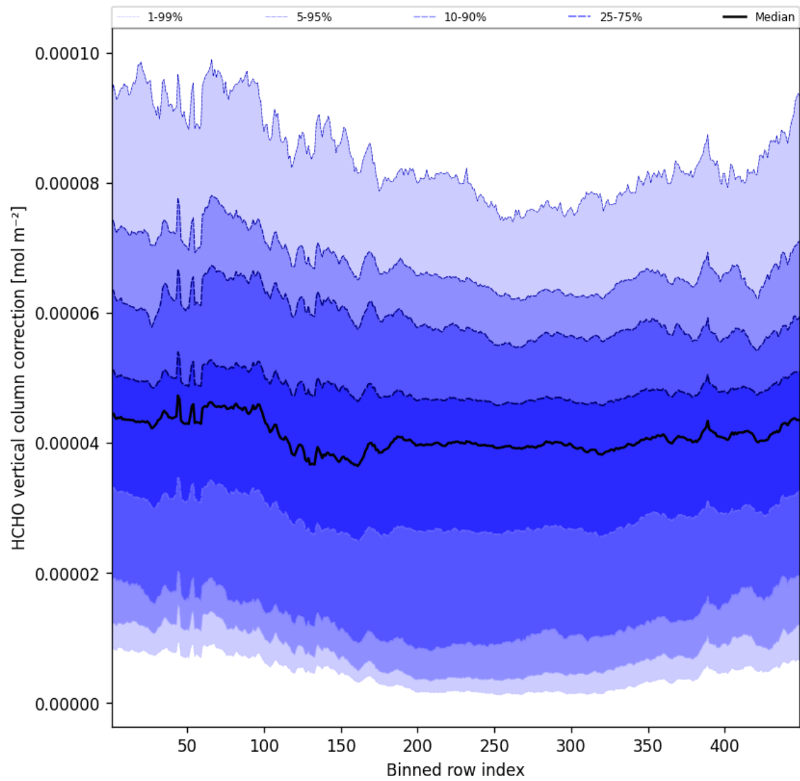
Figure 52: Along track statistics of “HCHO vertical column correction” for 2025-12-13 to 2025-12-14
