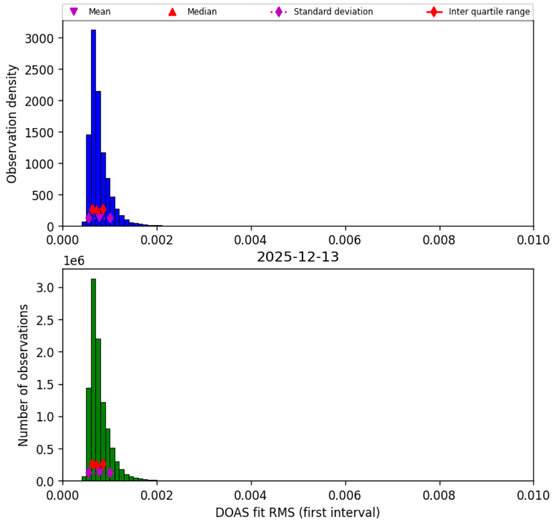
Figure 46: Histogram of “DOAS fit RMS (first interval)” for 2025-12-13 to 2025-12-14
