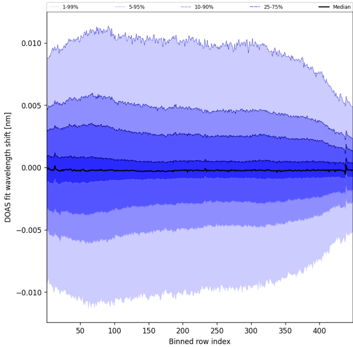
Figure 59: Along track statistics of “DOAS fit wavelength shift” for 2025-12-13 to 2025-12-14
