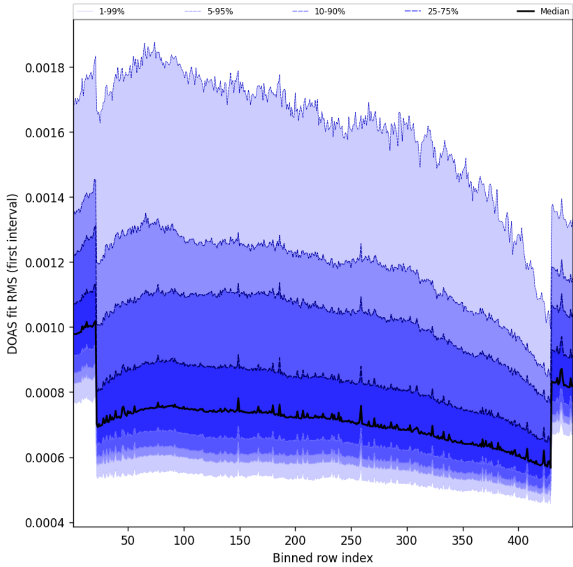
Figure 61: Along track statistics of “DOAS fit RMS (first interval)” for 2025-12-13 to 2025-12-14
