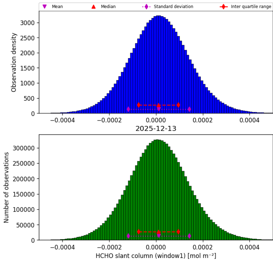
Figure 38: Histogram of “HCHO slant column (window1)” for 2025-12-13 to 2025-12-14
