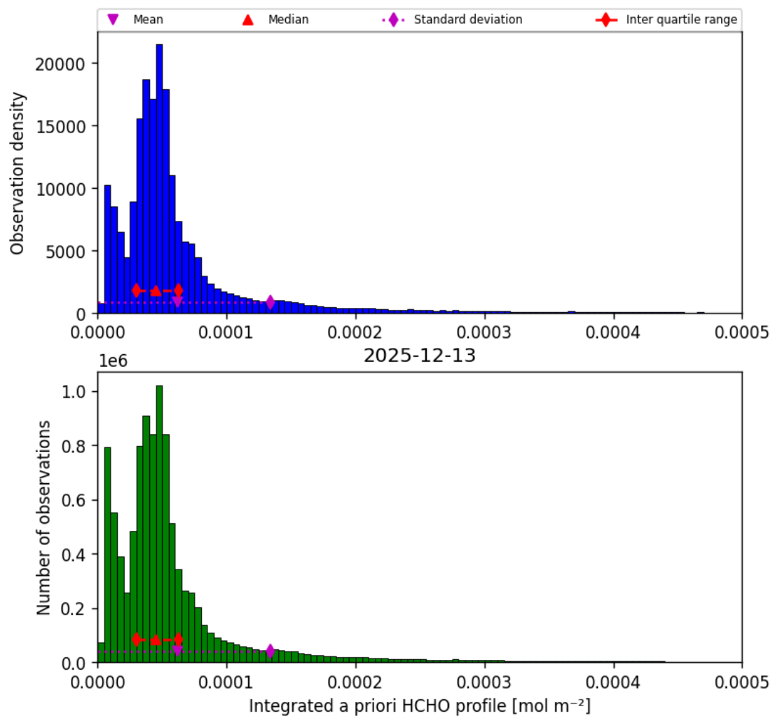
Figure 43: Histogram of “Integrated a priori HCHO profile” for 2025-12-13 to 2025-12-14
