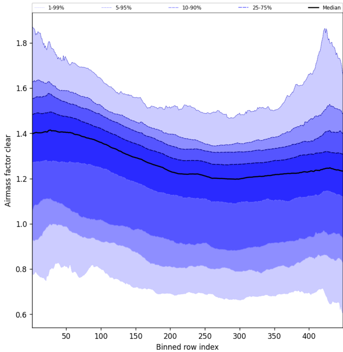
Figure 57: Along track statistics of “Airmass factor clear” for 2025-12-13 to 2025-12-14
