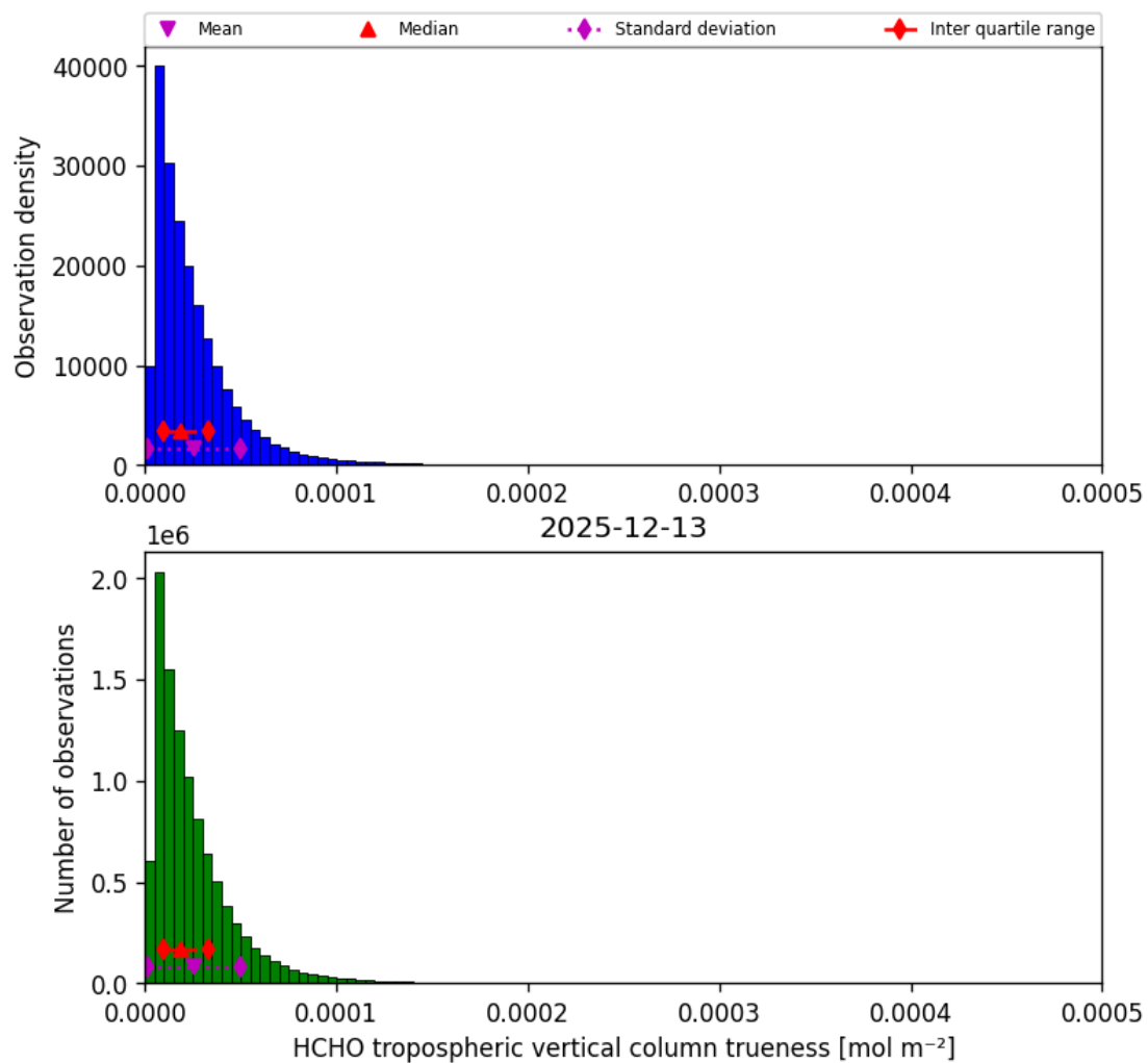
Figure 48: Histogram of “HCHO tropospheric vertical column trueness” for 2025-12-13 to 2025-12-14
