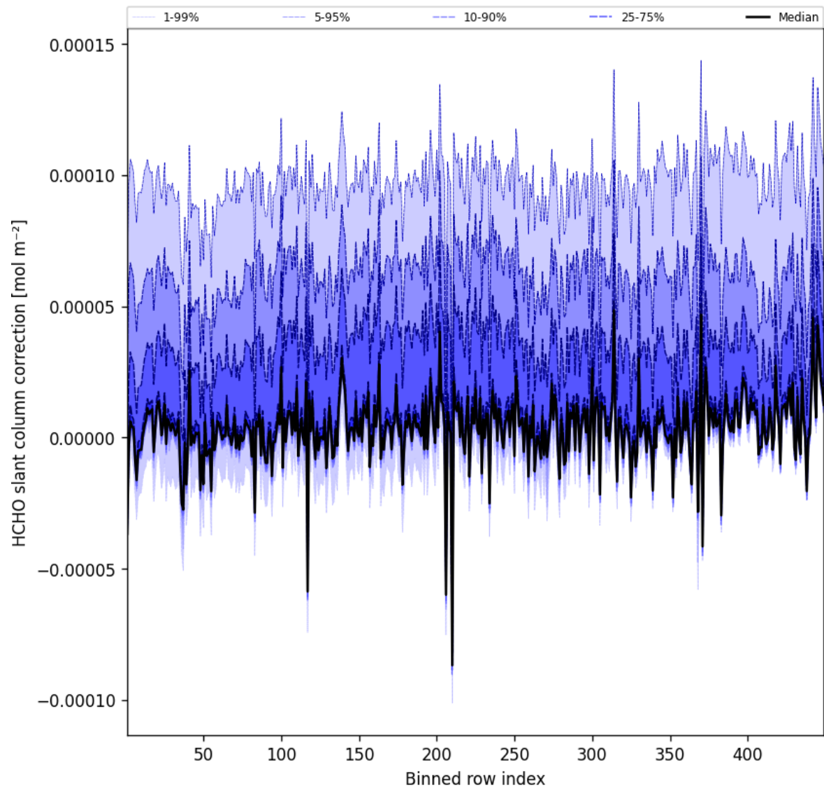
Figure 62: Along track statistics of “HCHO slant column correction” for 2025-12-13 to 2025-12-14
