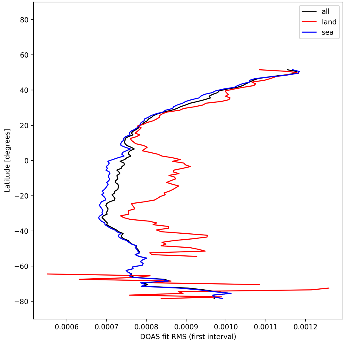
Figure 31: Zonal average of “DOAS fit RMS (first interval)” for 2025-12-13 to 2025-12-14.
