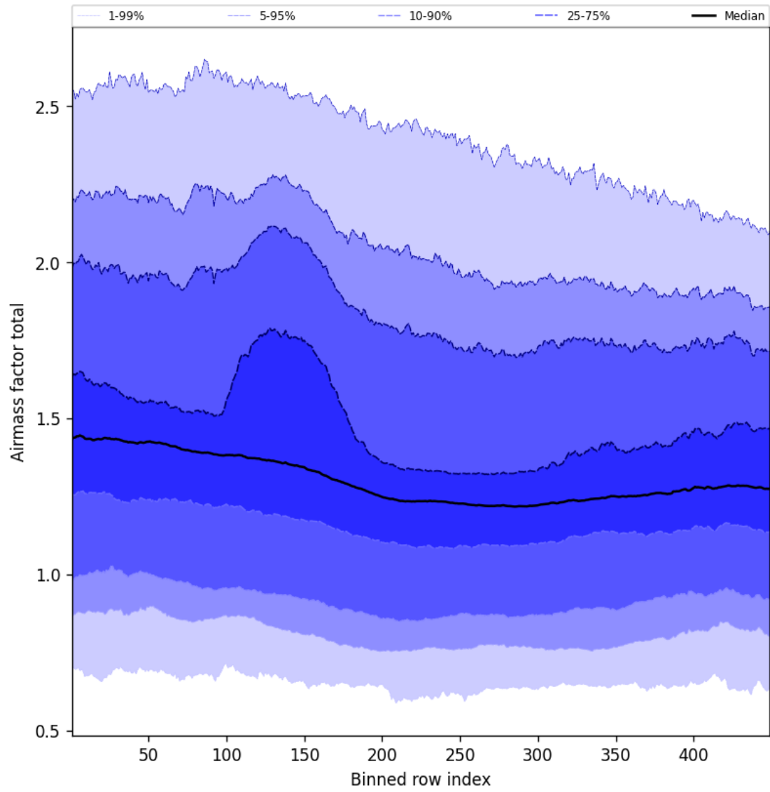
Figure 55: Along track statistics of “Airmass factor total” for 2025-12-13 to 2025-12-14
