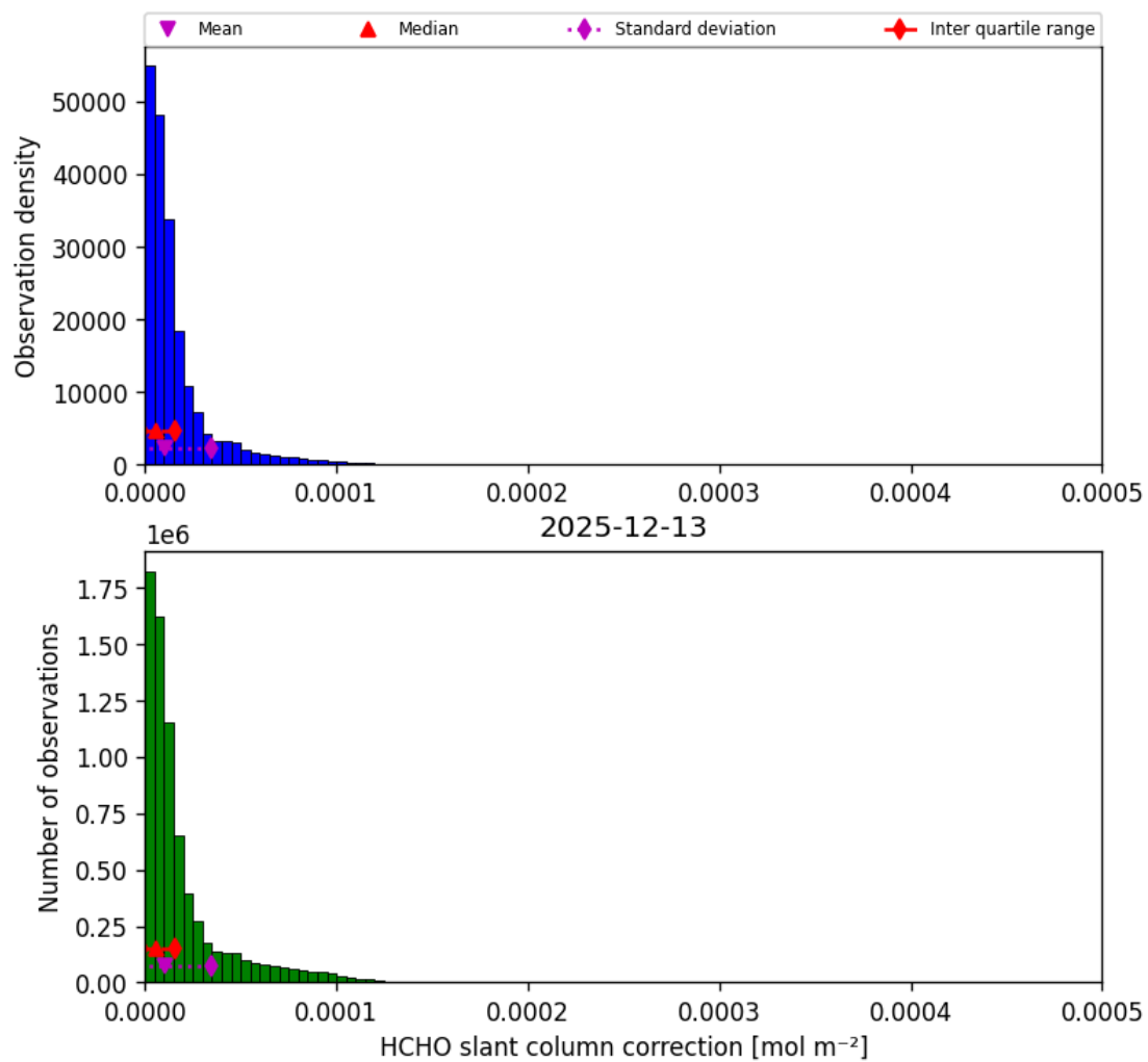
Figure 47: Histogram of “HCHO slant column correction” for 2025-12-13 to 2025-12-14
