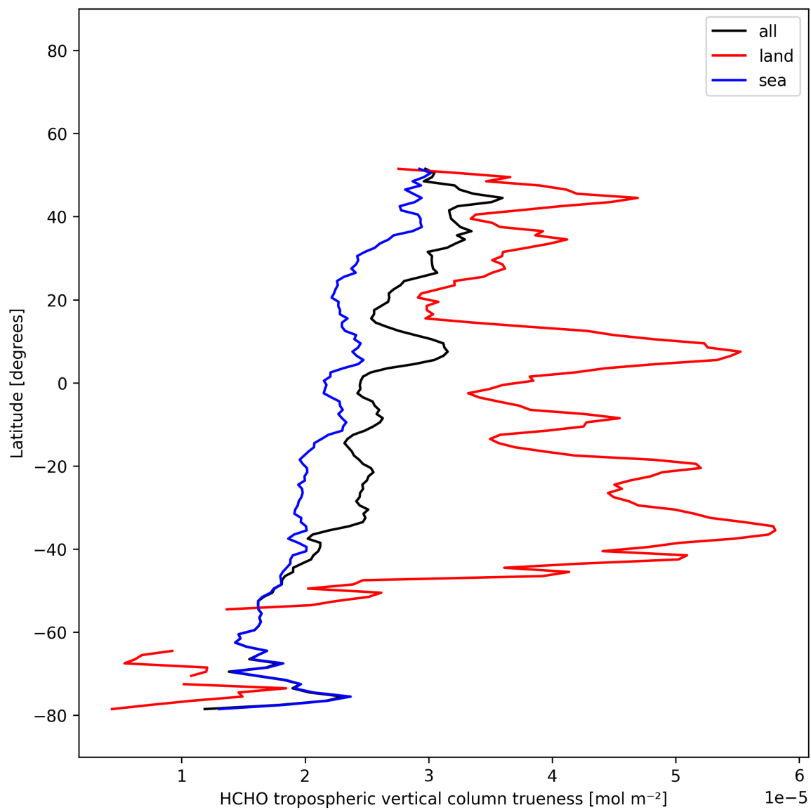
Figure 33: Zonal average of “HCHO tropospheric vertical column trueness” for 2025-12-13 to 2025-12-14.
