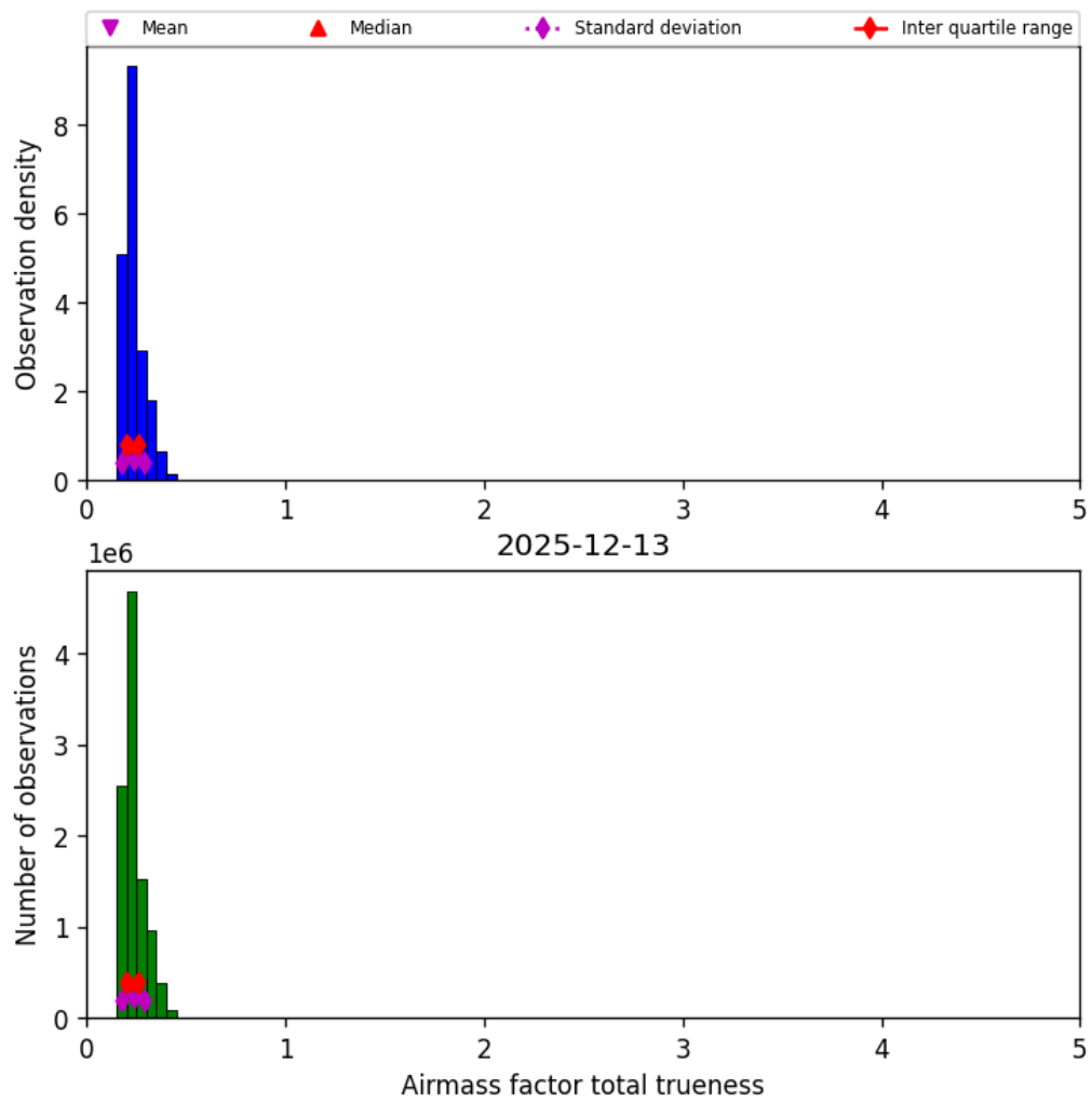
Figure 41: Histogram of “Airmass factor total trueness” for 2025-12-13 to 2025-12-14
