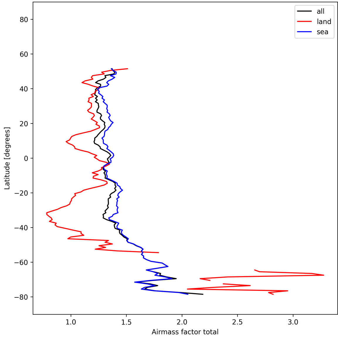
Figure 25: Zonal average of “Airmass factor total” for 2025-12-13 to 2025-12-14.
