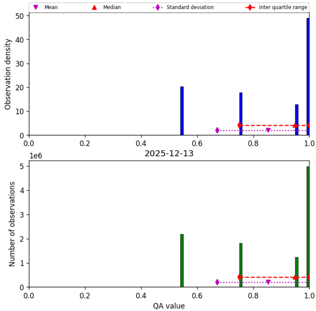
Figure 34: Histogram of “QA value” for 2025-12-13 to 2025-12-14
