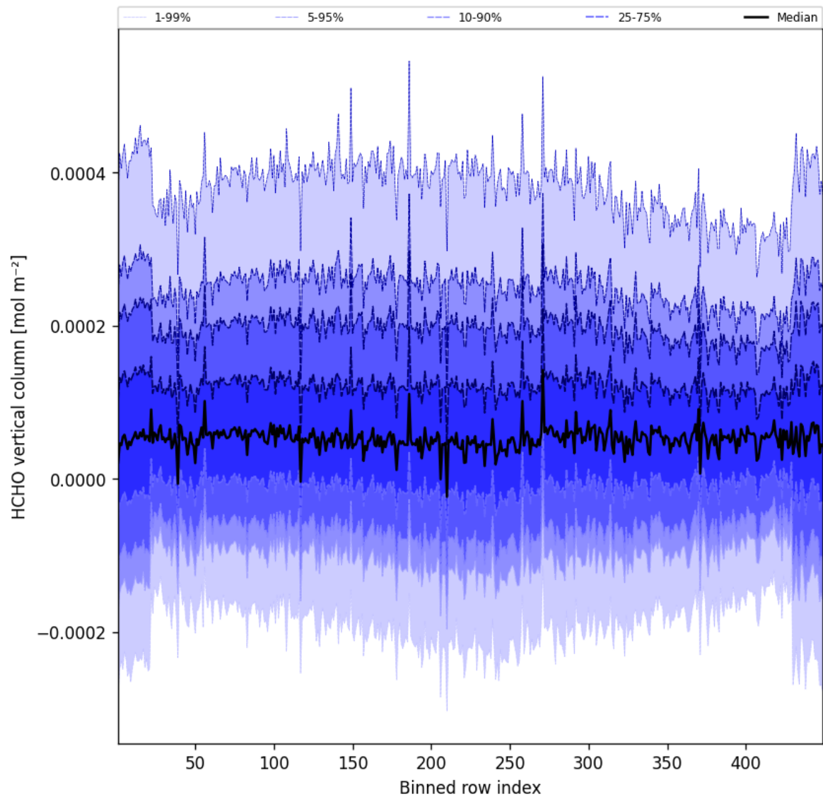
Figure 50: Along track statistics of “HCHO vertical column” for 2025-12-13 to 2025-12-14
