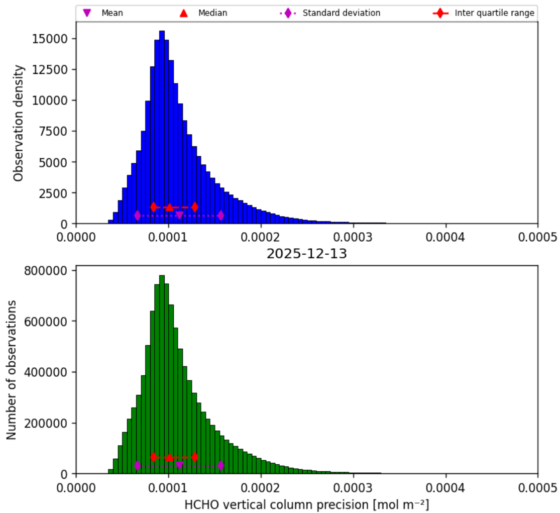
Figure 36: Histogram of “HCHO vertical column precision” for 2025-12-13 to 2025-12-14
