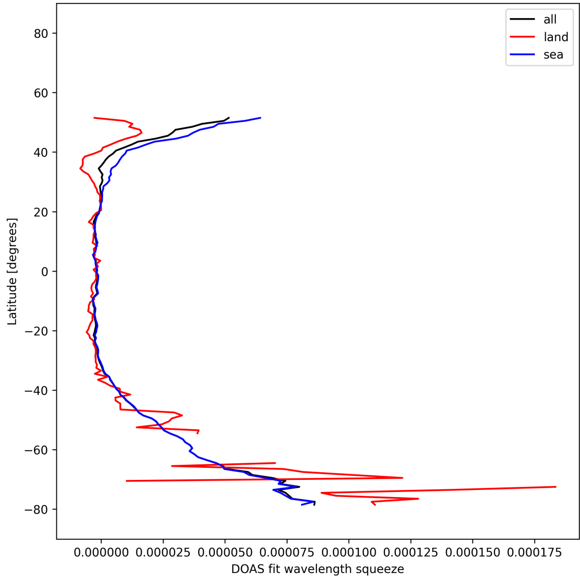
Figure 30: Zonal average of “DOAS fit wavelength squeeze” for 2025-12-13 to 2025-12-14.
