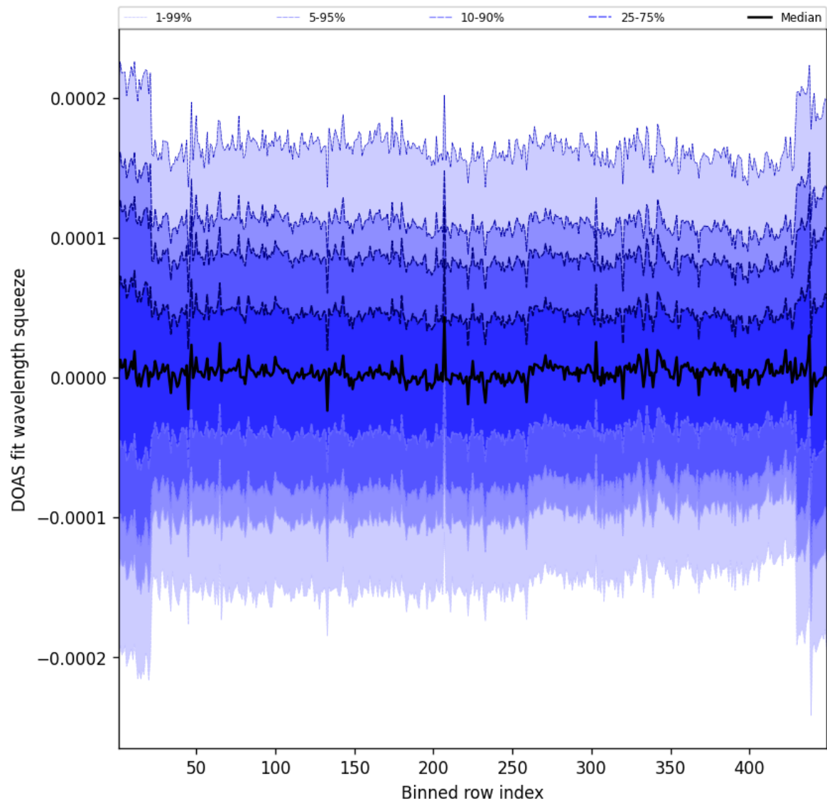
Figure 60: Along track statistics of “DOAS fit wavelength squeeze” for 2025-12-13 to 2025-12-14
