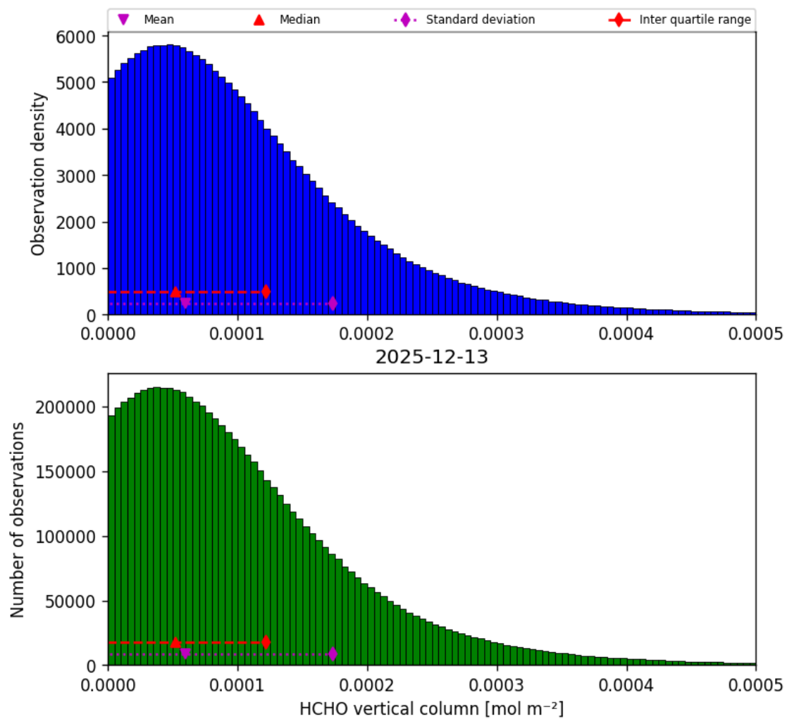
Figure 35: Histogram of “HCHO vertical column” for 2025-12-13 to 2025-12-14
