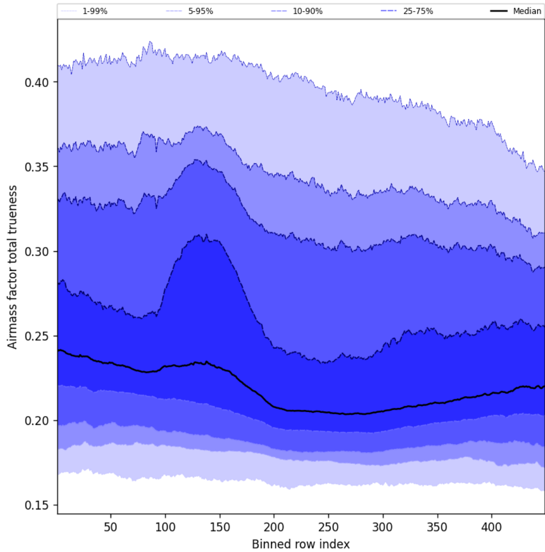
Figure 56: Along track statistics of “Airmass factor total trueness” for 2025-12-13 to 2025-12-14
