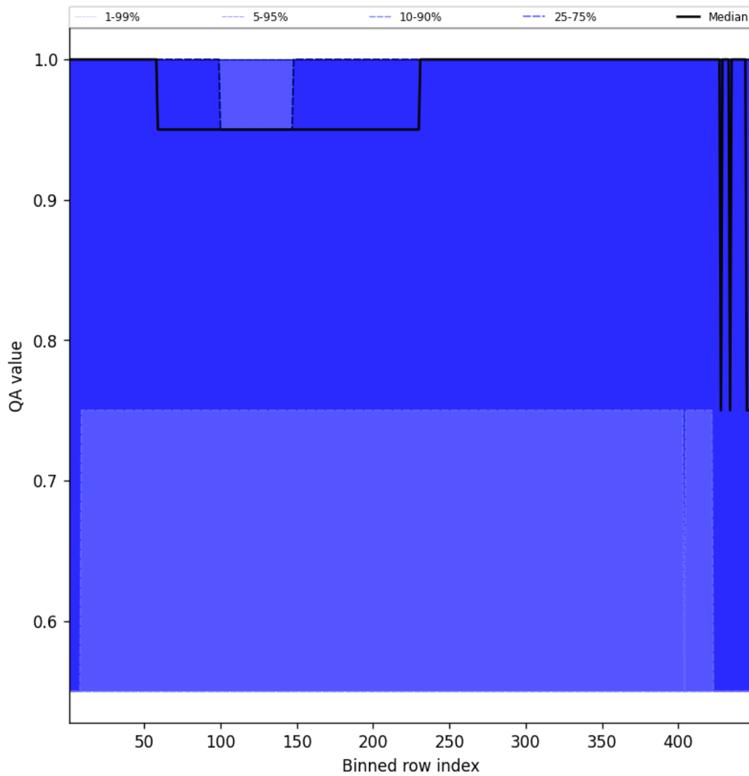
Figure 49: Along track statistics of “QA value” for 2025-12-13 to 2025-12-14
