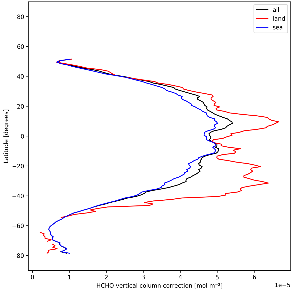
Figure 22: Zonal average of "HCHO vertical column correction" for 2025-12-13 to 2025-12-14.
