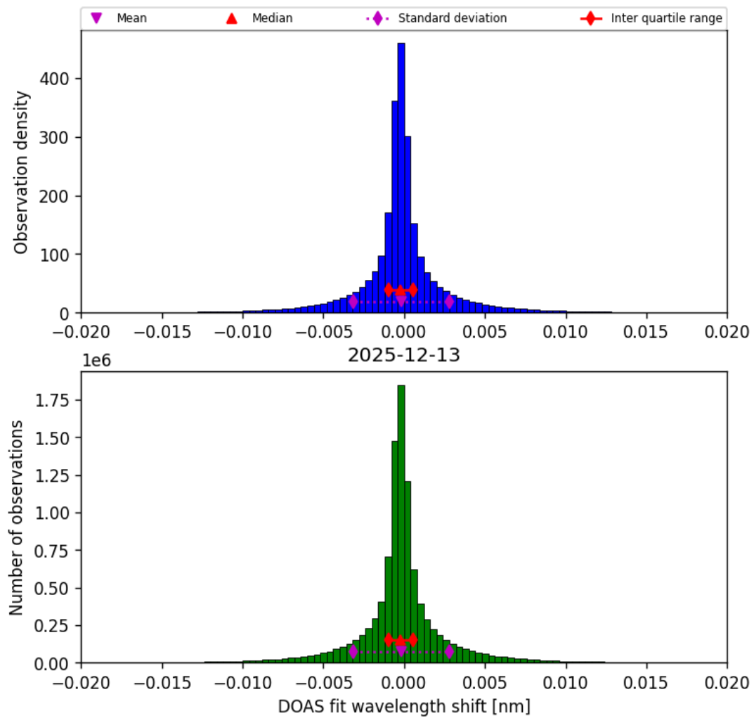
Figure 44: Histogram of “DOAS fit wavelength shift” for 2025-12-13 to 2025-12-14
