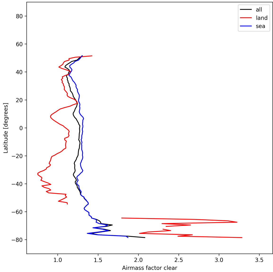
Figure 27: Zonal average of “Airmass factor clear” for 2025-12-13 to 2025-12-14.
