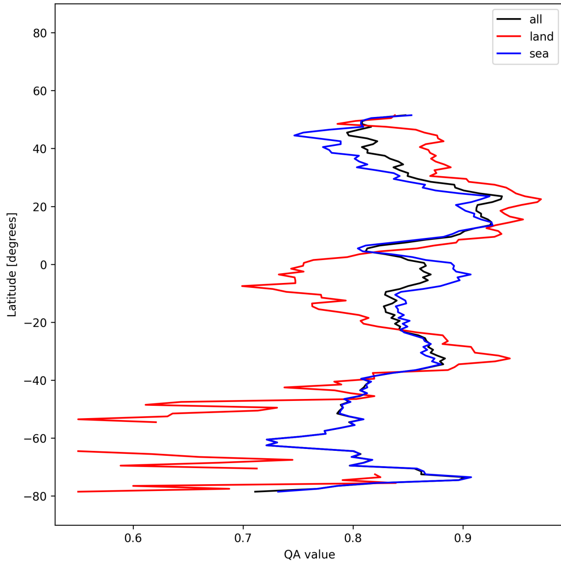
Figure 19: Zonal average of “QA value” for 2025-12-13 to 2025-12-14.
