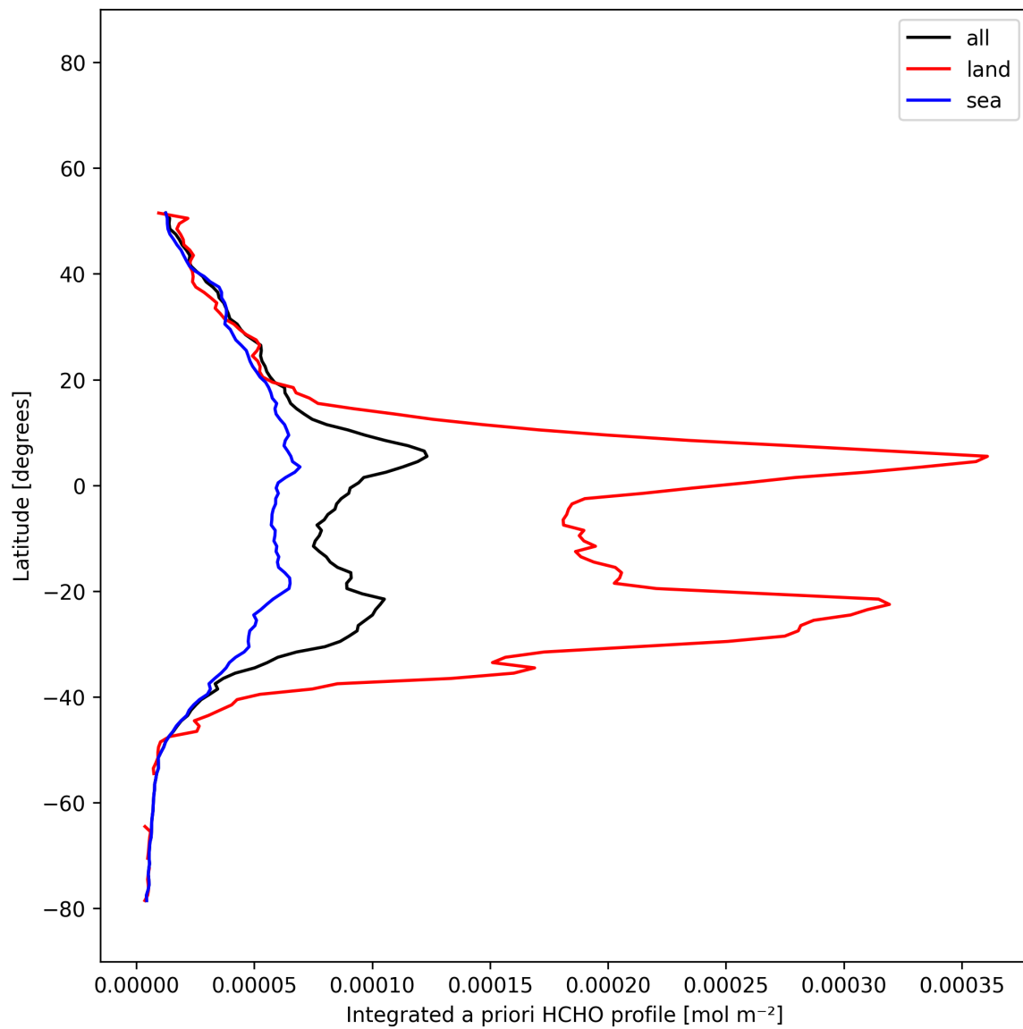
Figure 28: Zonal average of “Integrated a priori HCHO profile” for 2025-12-13 to 2025-12-14.
