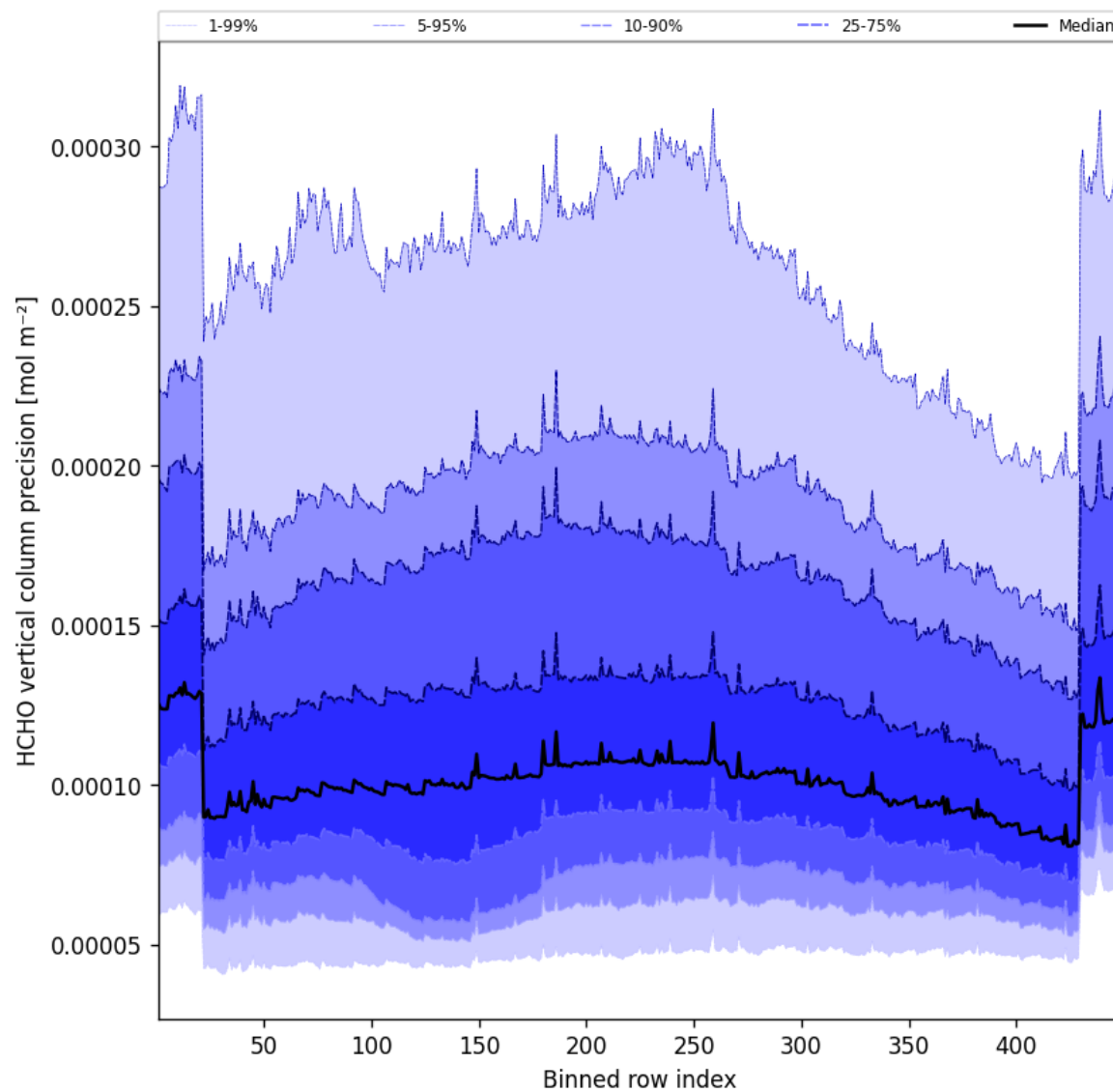
Figure 51: Along track statistics of “HCHO vertical column precision” for 2025-12-13 to 2025-12-14
