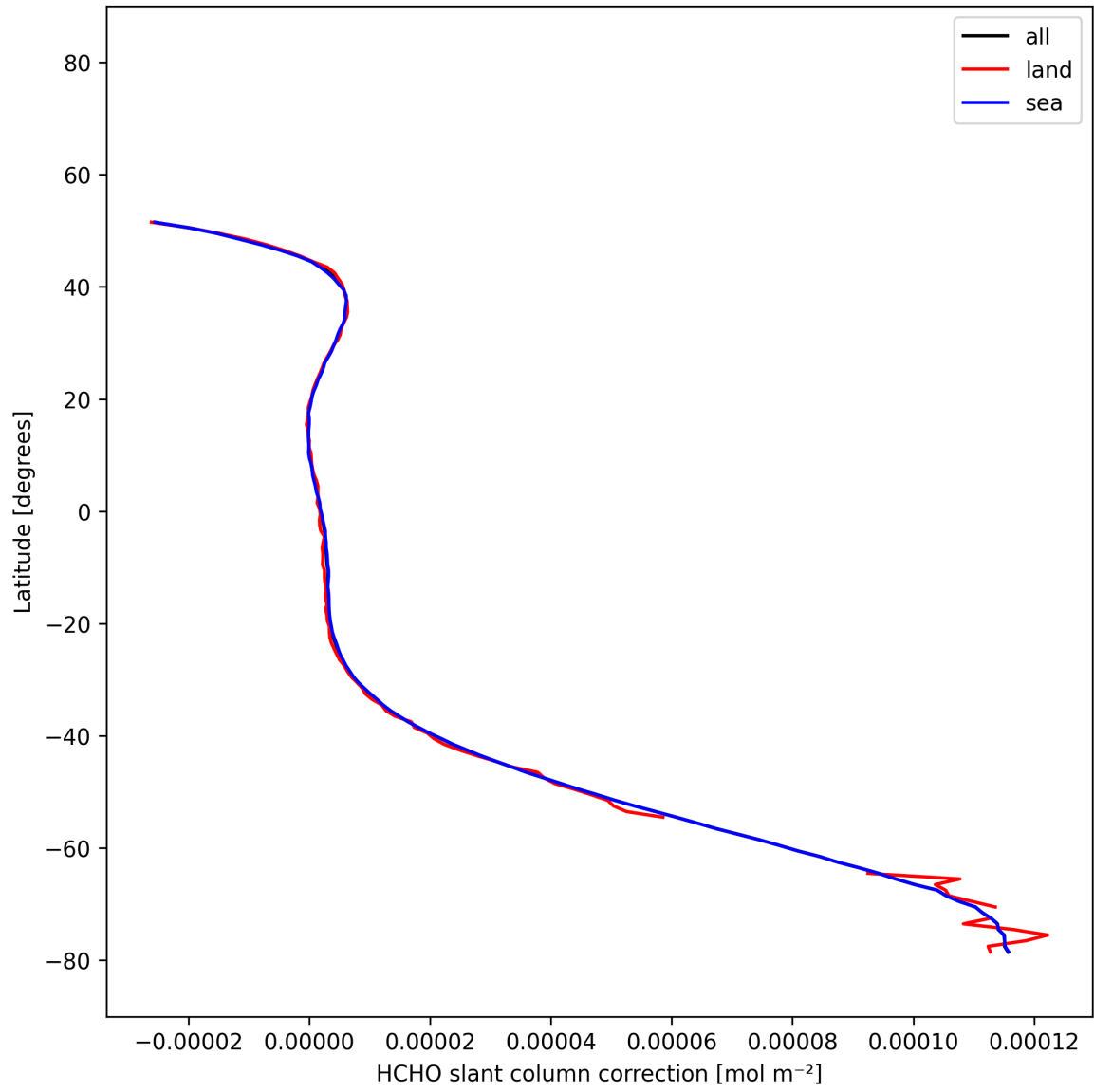
Figure 32: Zonal average of “HCHO slant column correction” for 2025-12-13 to 2025-12-14.
