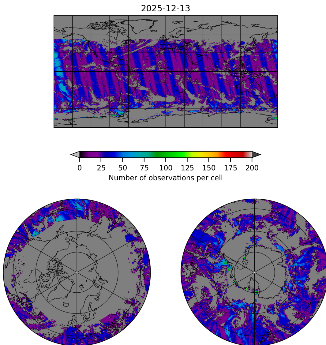
Figure 18: Map of the number of observations for 2025-12-13 to 2025-12-14
