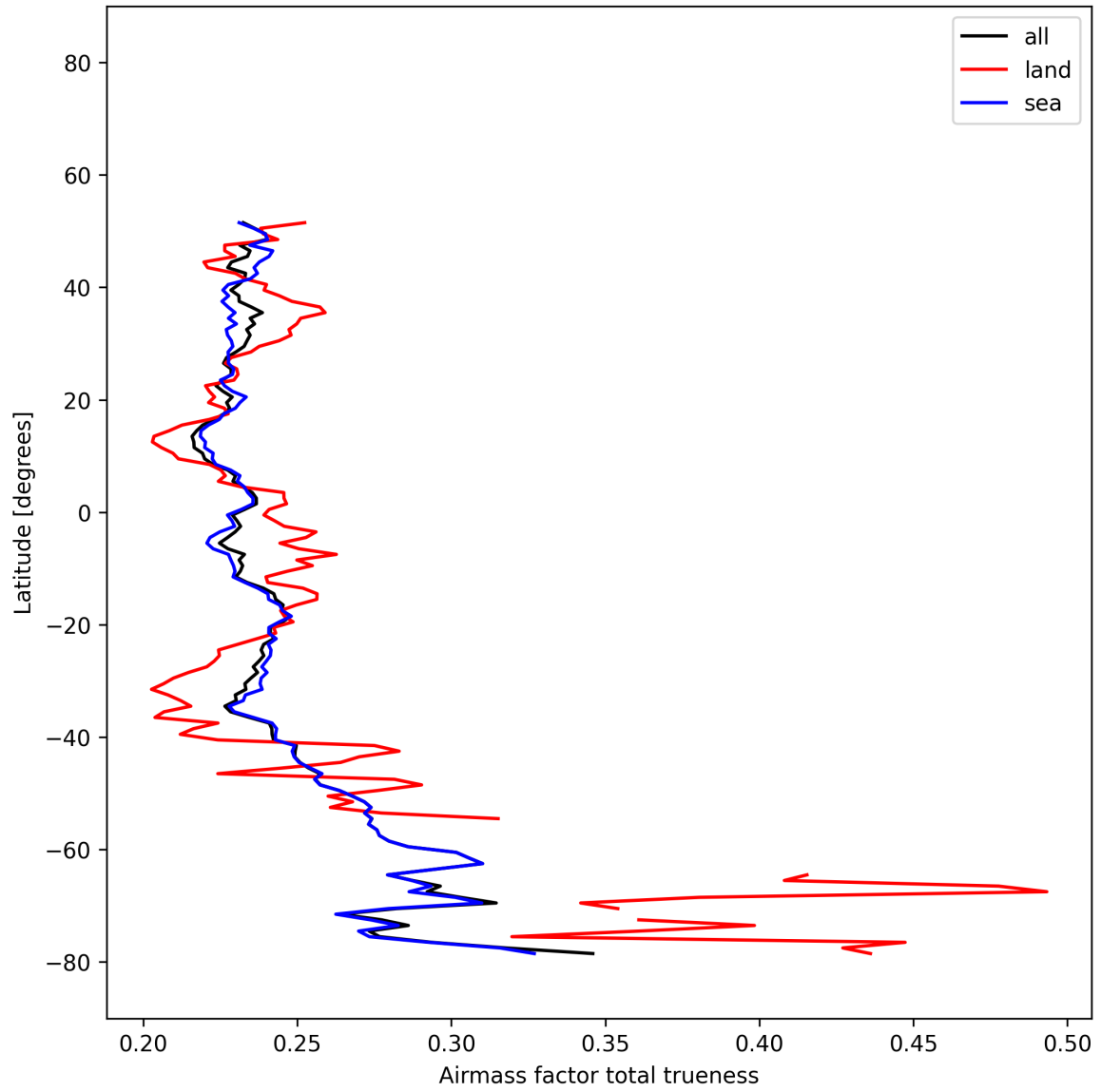
Figure 26: Zonal average of “Airmass factor total trueness” for 2025-12-13 to 2025-12-14.
