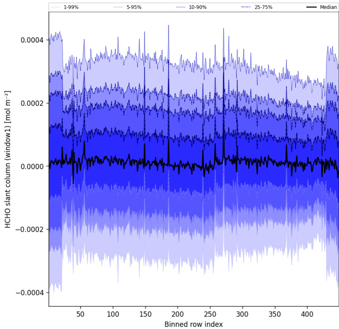
Figure 53: Along track statistics of “HCHO slant column (window1)” for 2025-12-13 to 2025-12-14
