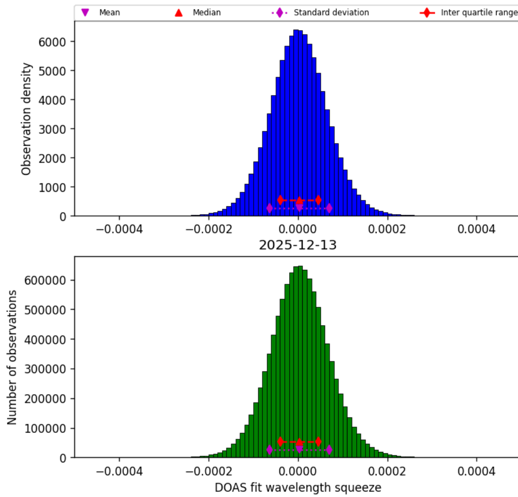
Figure 45: Histogram of “DOAS fit wavelength squeeze” for 2025-12-13 to 2025-12-14
