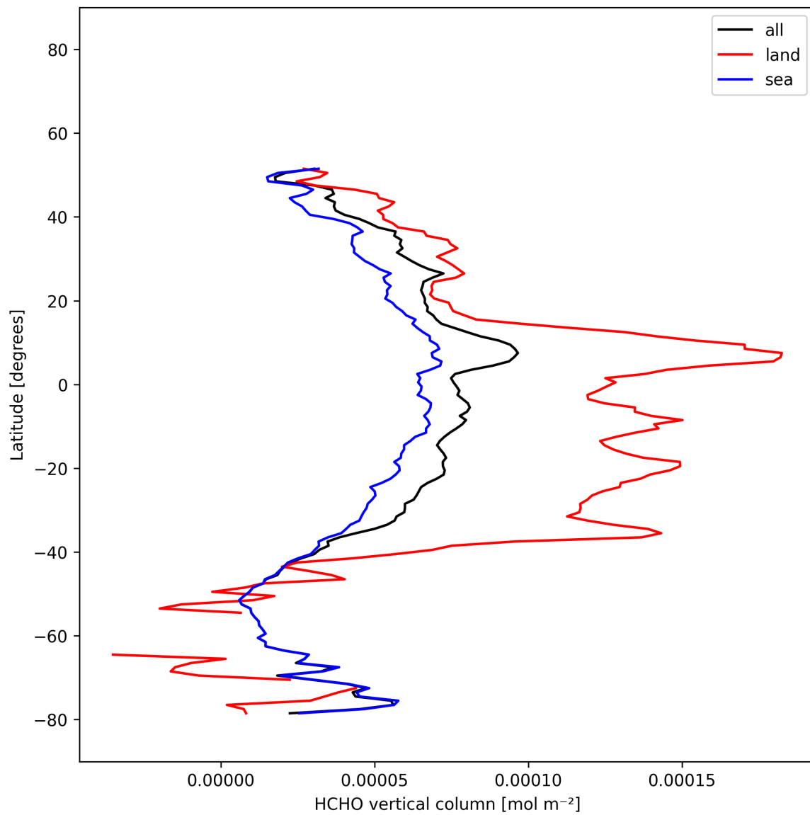
Figure 20: Zonal average of “HCHO vertical column” for 2025-12-13 to 2025-12-14.
