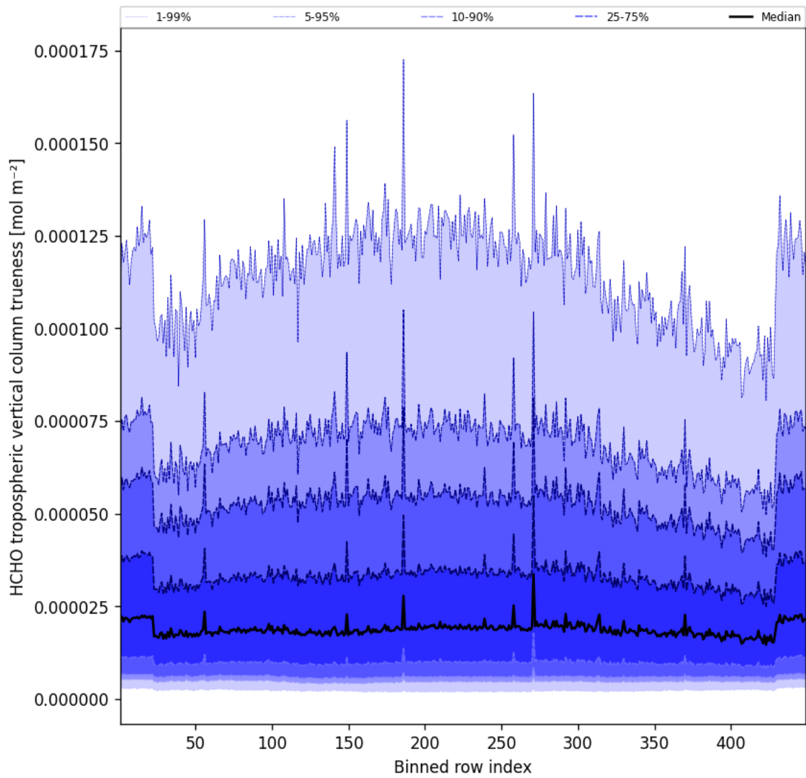
Figure 63: Along track statistics of “HCHO tropospheric vertical column trueness” for 2025-12-13 to 2025-12-14
