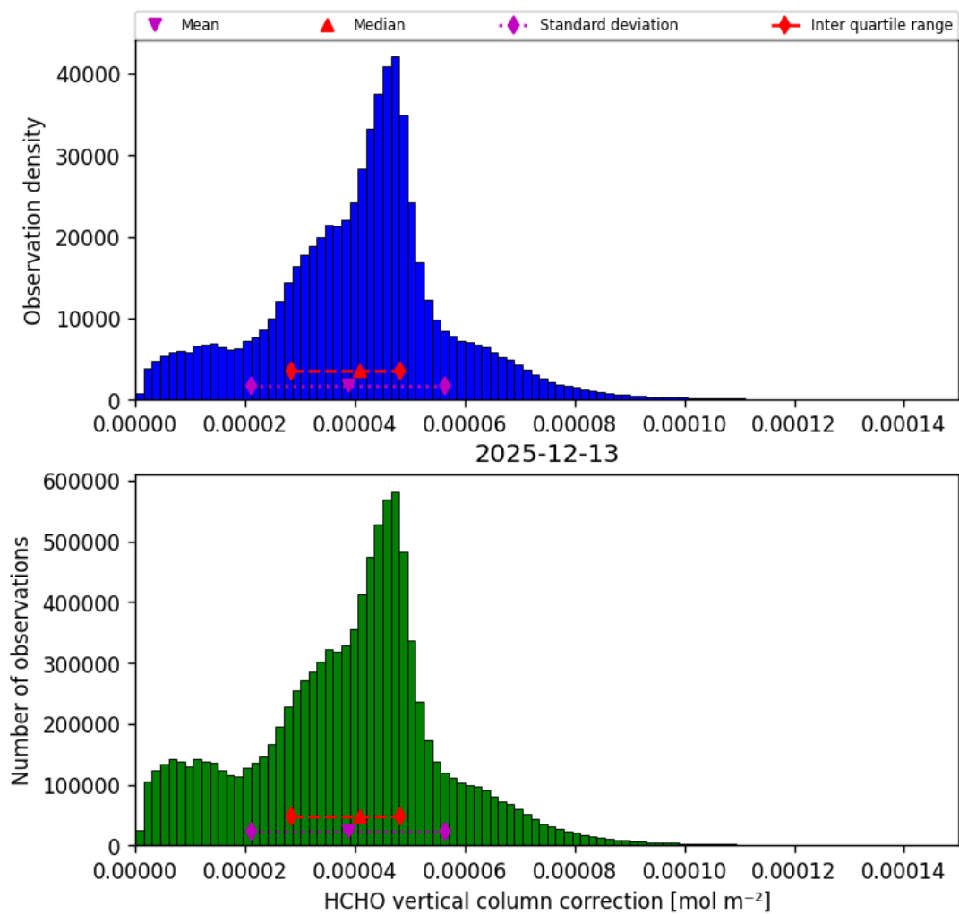
Figure 37: Histogram of “HCHO vertical column correction” for 2025-12-13 to 2025-12-14
