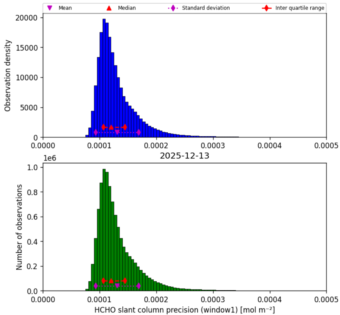
Figure 39: Histogram of “HCHO slant column precision (window1)” for 2025-12-13 to 2025-12-14
