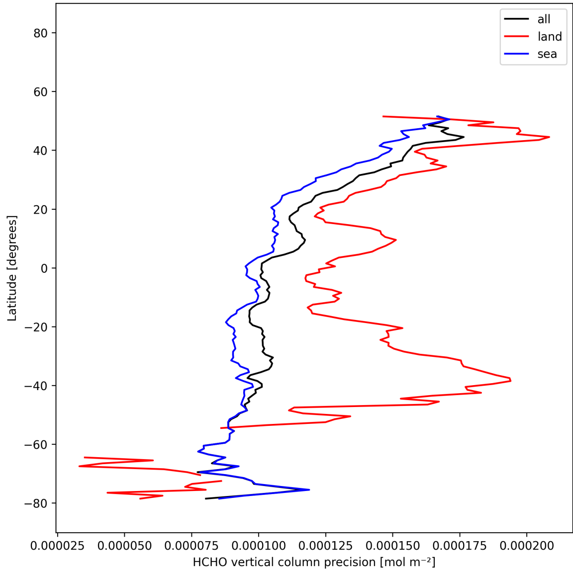
Figure 21: Zonal average of “HCHO vertical column precision” for 2025-12-13 to 2025-12-14.
