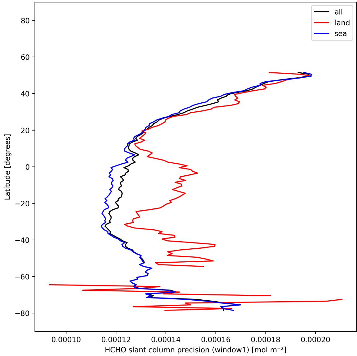
Figure 24: Zonal average of “HCHO slant column precision (window1)” for 2025-12-13 to 2025-12-14.
