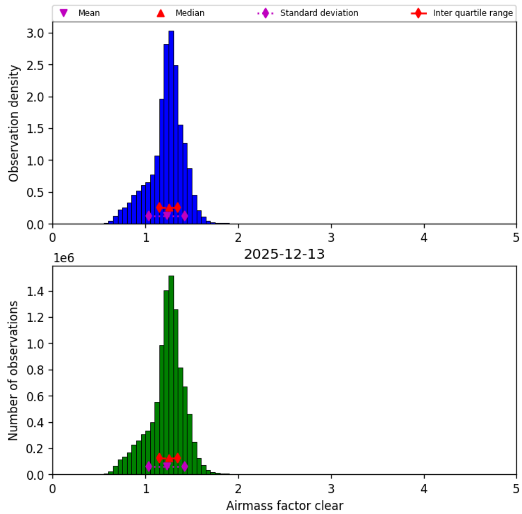
Figure 42: Histogram of “Airmass factor clear” for 2025-12-13 to 2025-12-14
