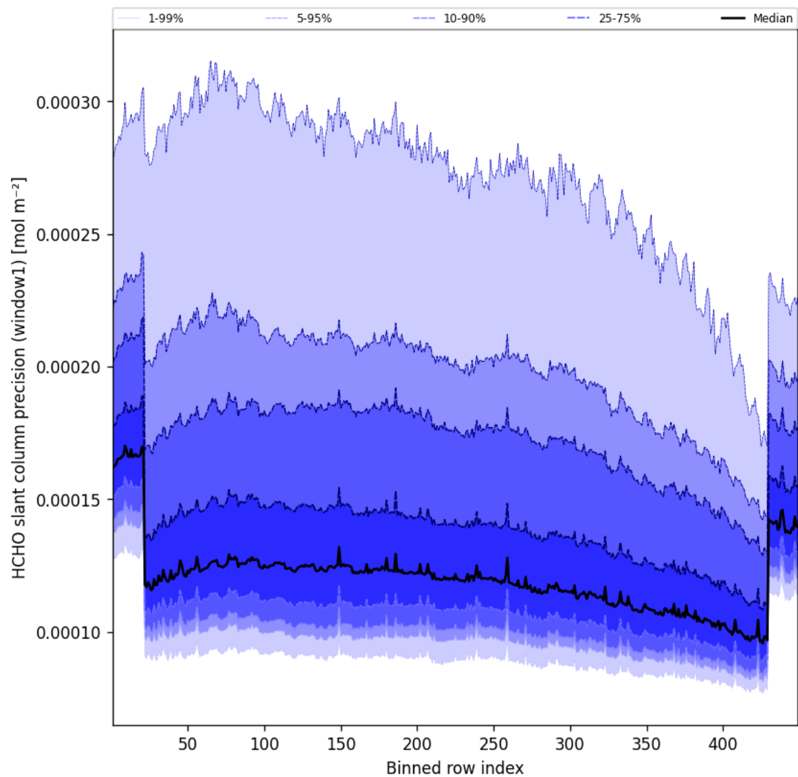
Figure 54: Along track statistics of “HCHO slant column precision (window1)” for 2025-12-13 to 2025-12-14
