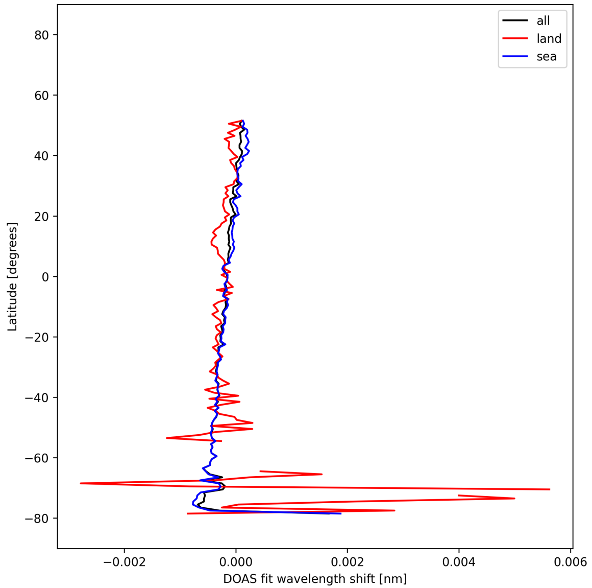
Figure 29: Zonal average of “DOAS fit wavelength shift” for 2025-12-13 to 2025-12-14.
