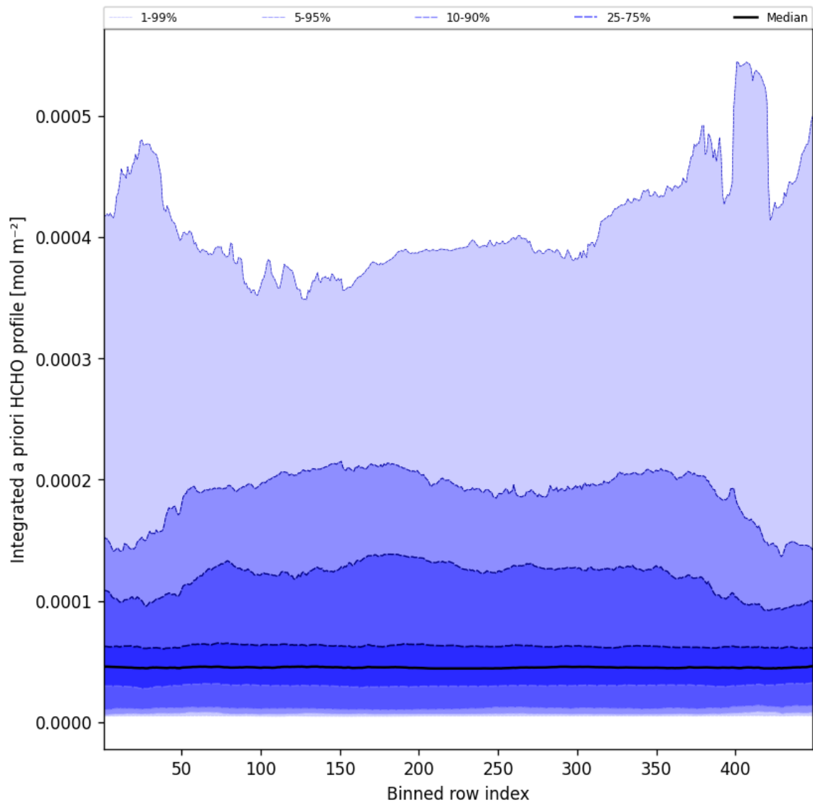
Figure 58: Along track statistics of “Integrated a priori HCHO profile” for 2025-12-13 to 2025-12-14
