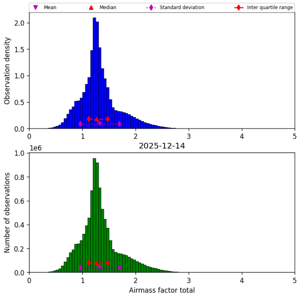
Figure 40: Histogram of “Airmass factor total” for 2025-12-14 to 2025-12-15
