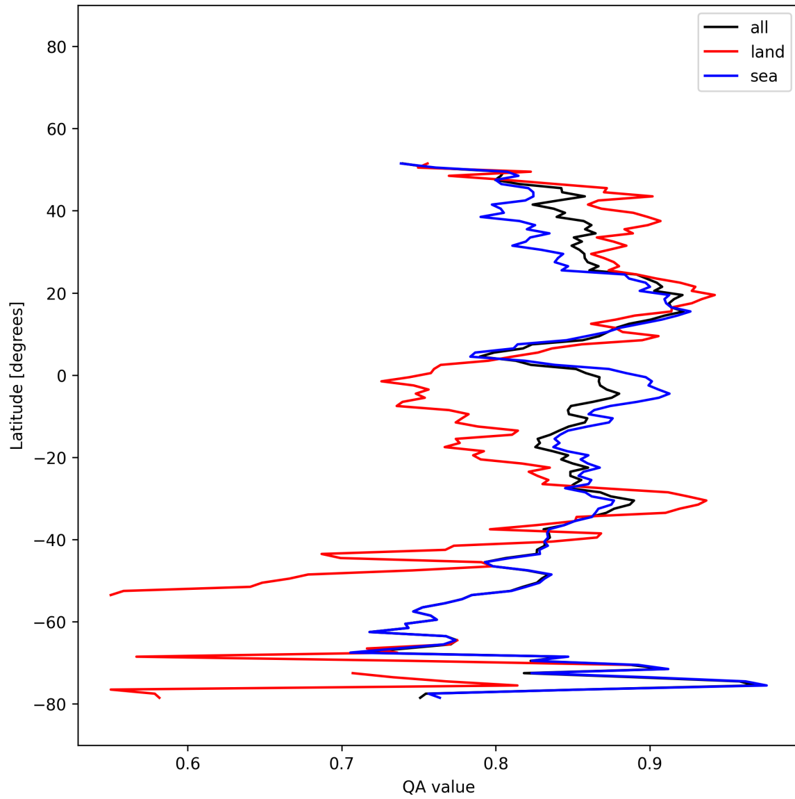
Figure 19: Zonal average of “QA value” for 2025-12-14 to 2025-12-15.
