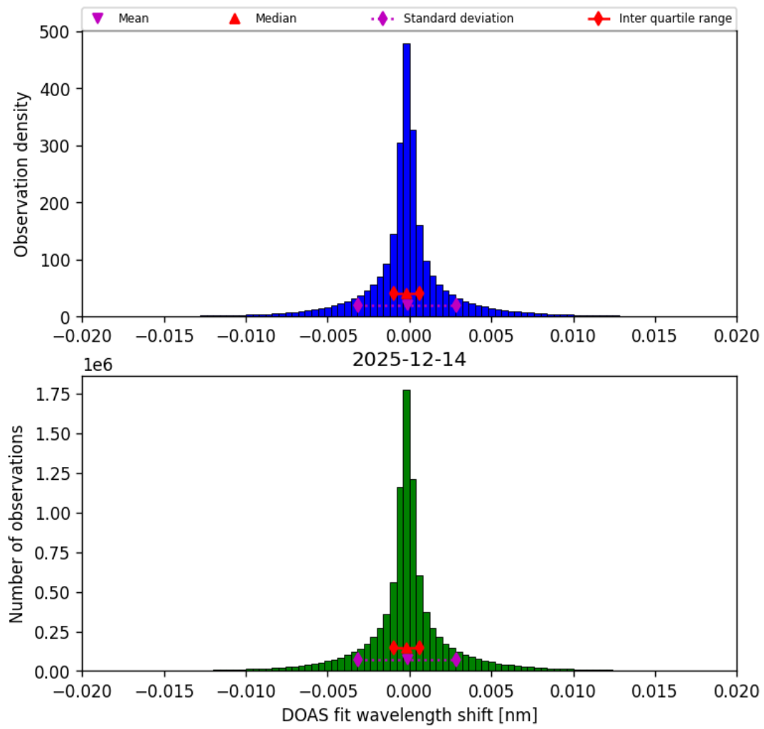
Figure 44: Histogram of “DOAS fit wavelength shift” for 2025-12-14 to 2025-12-15
