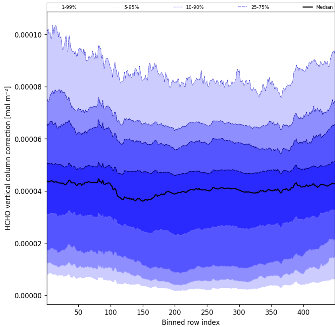
Figure 52: Along track statistics of “HCHO vertical column correction” for 2025-12-14 to 2025-12-15
