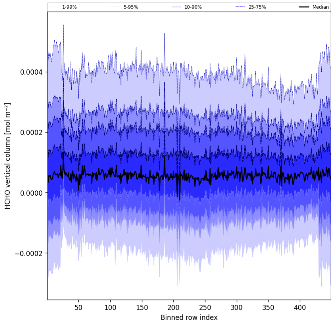
Figure 50: Along track statistics of “HCHO vertical column” for 2025-12-14 to 2025-12-15
