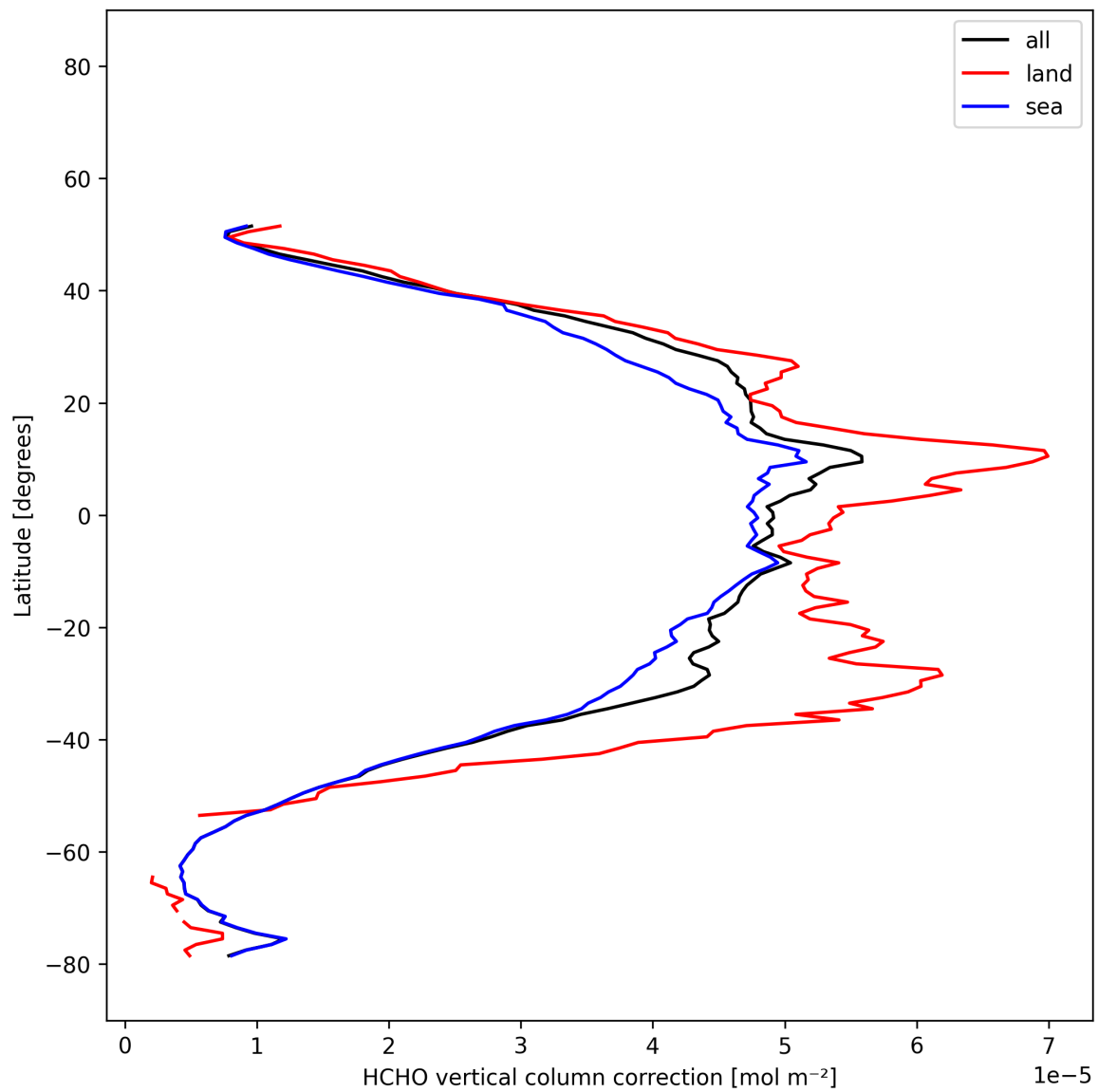
Figure 22: Zonal average of “HCHO vertical column correction” for 2025-12-14 to 2025-12-15.
