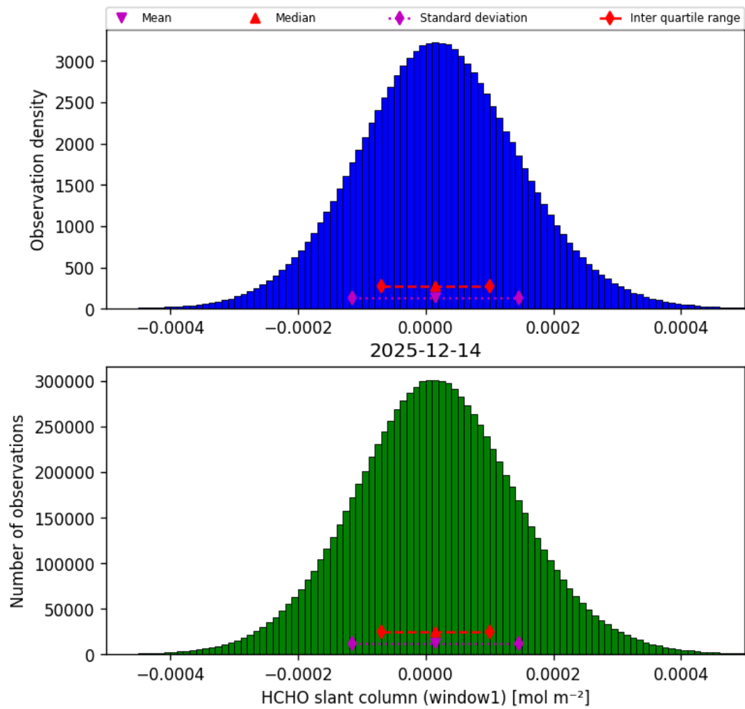
Figure 38: Histogram of “HCHO slant column (window1)” for 2025-12-14 to 2025-12-15
