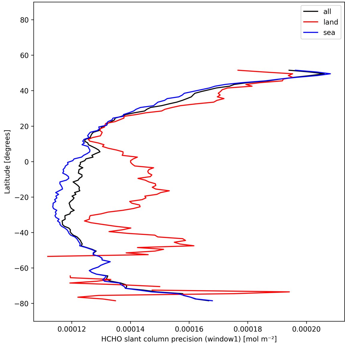
Figure 24: Zonal average of “HCHO slant column precision (window1)” for 2025-12-14 to 2025-12-15.
