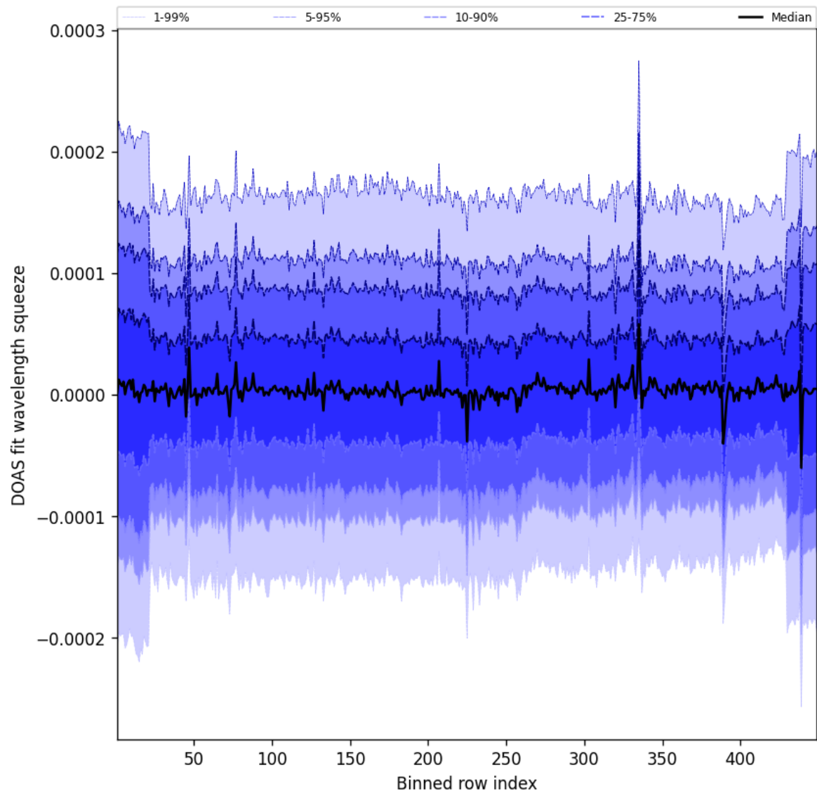
Figure 60: Along track statistics of “DOAS fit wavelength squeeze” for 2025-12-14 to 2025-12-15
