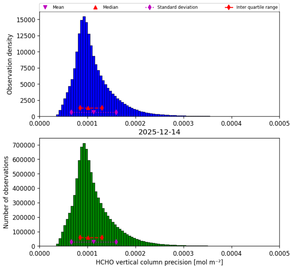
Figure 36: Histogram of “HCHO vertical column precision” for 2025-12-14 to 2025-12-15
