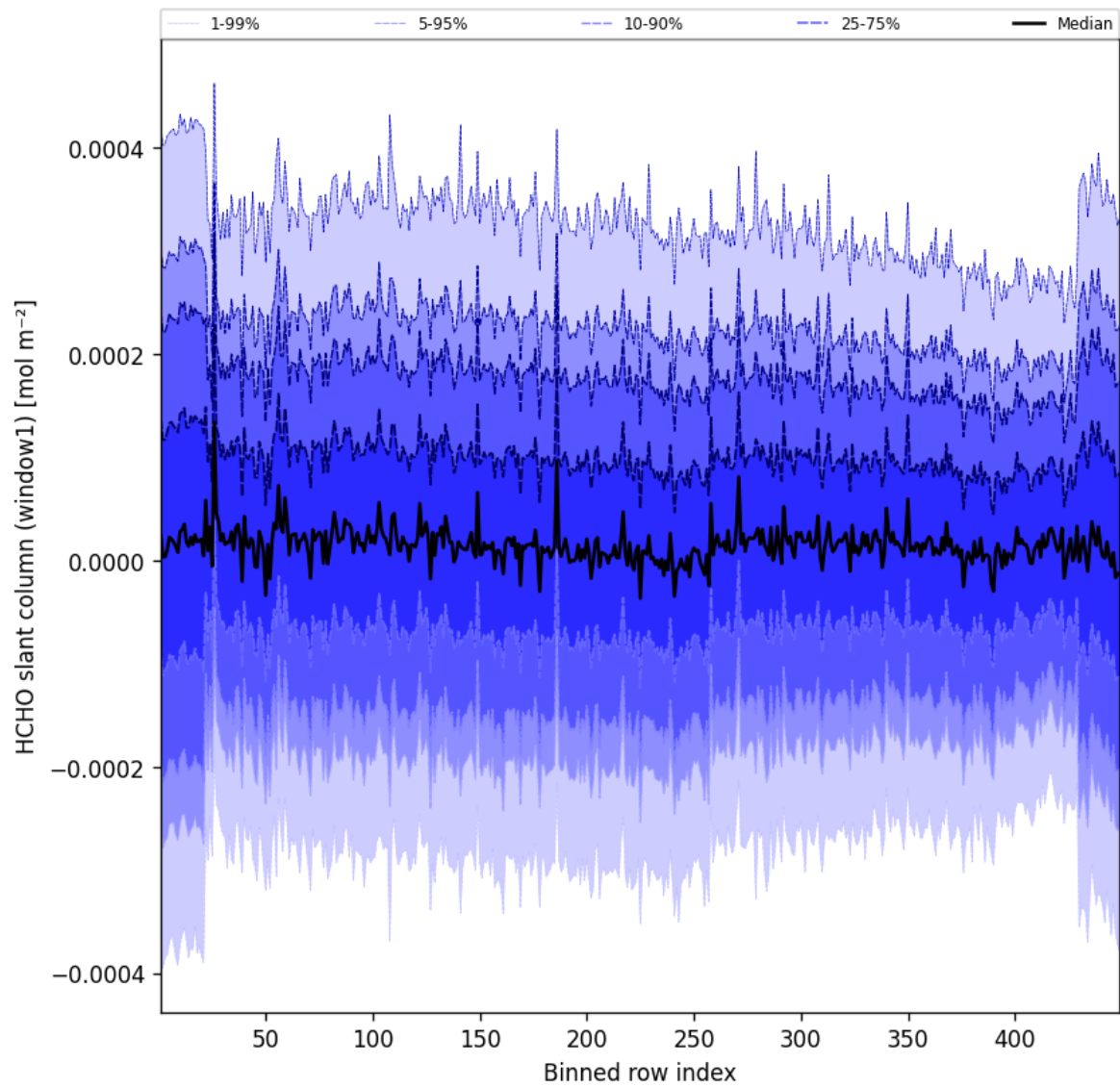
Figure 53: Along track statistics of “HCHO slant column (window1)” for 2025-12-14 to 2025-12-15
