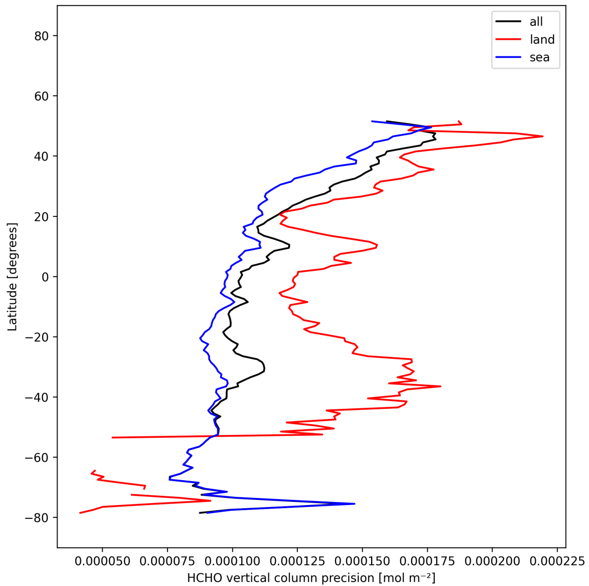
Figure 21: Zonal average of “HCHO vertical column precision” for 2025-12-14 to 2025-12-15.
