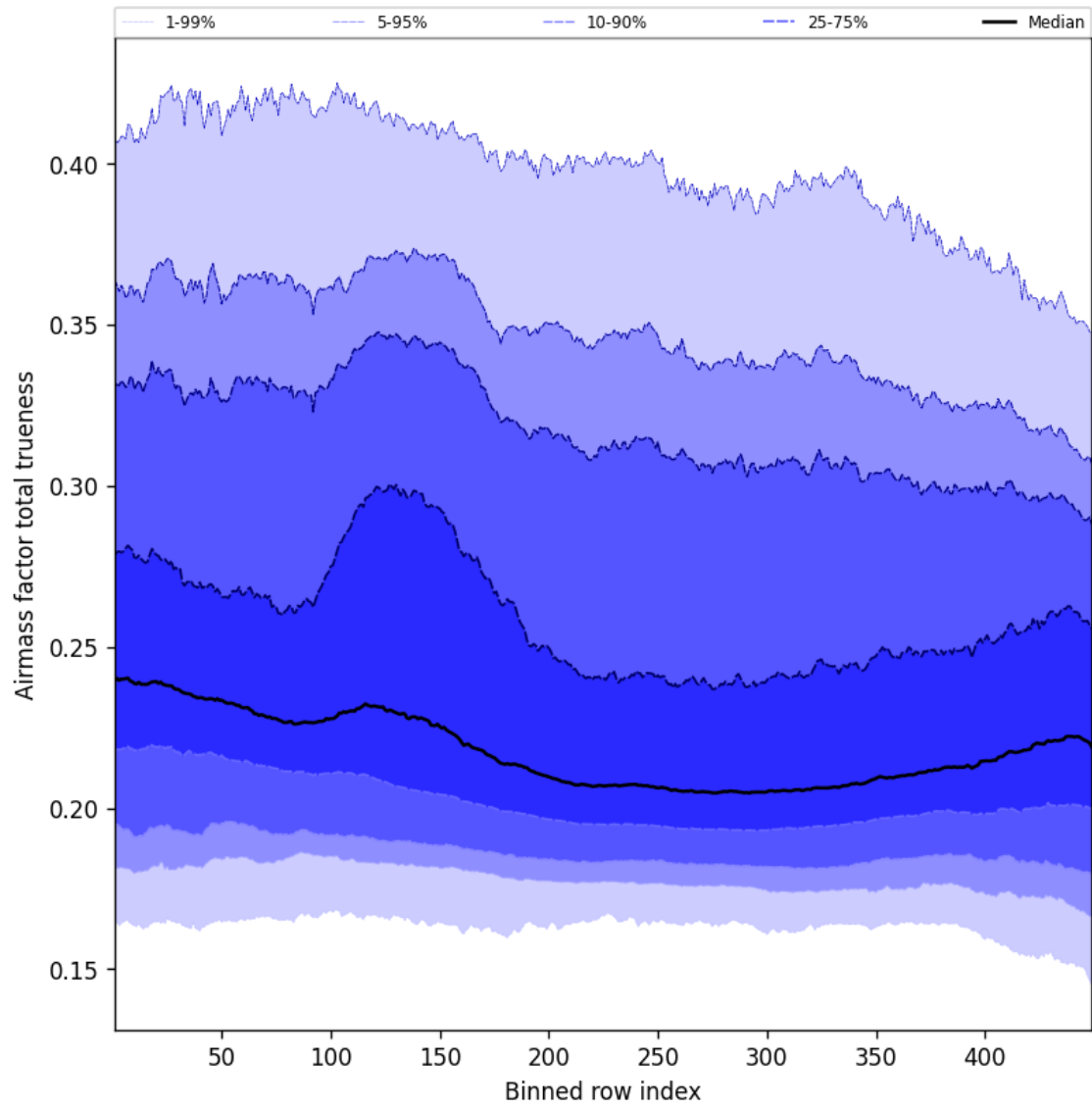
Figure 56: Along track statistics of “Airmass factor total trueness” for 2025-12-14 to 2025-12-15
