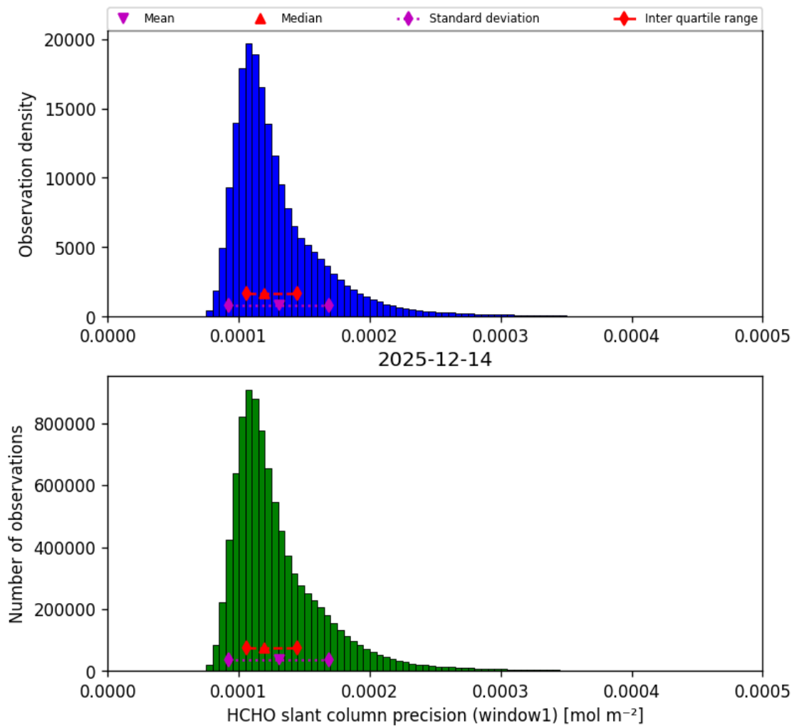
Figure 39: Histogram of “HCHO slant column precision (window1)” for 2025-12-14 to 2025-12-15
