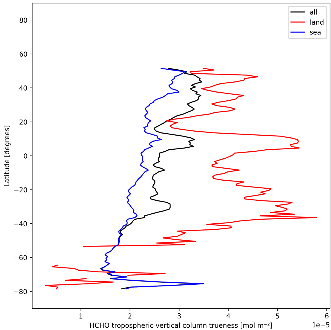
Figure 33: Zonal average of “HCHO tropospheric vertical column trueness” for 2025-12-14 to 2025-12-15.
