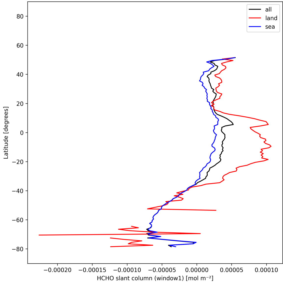
Figure 23: Zonal average of “HCHO slant column (window1)” for 2025-12-14 to 2025-12-15.
