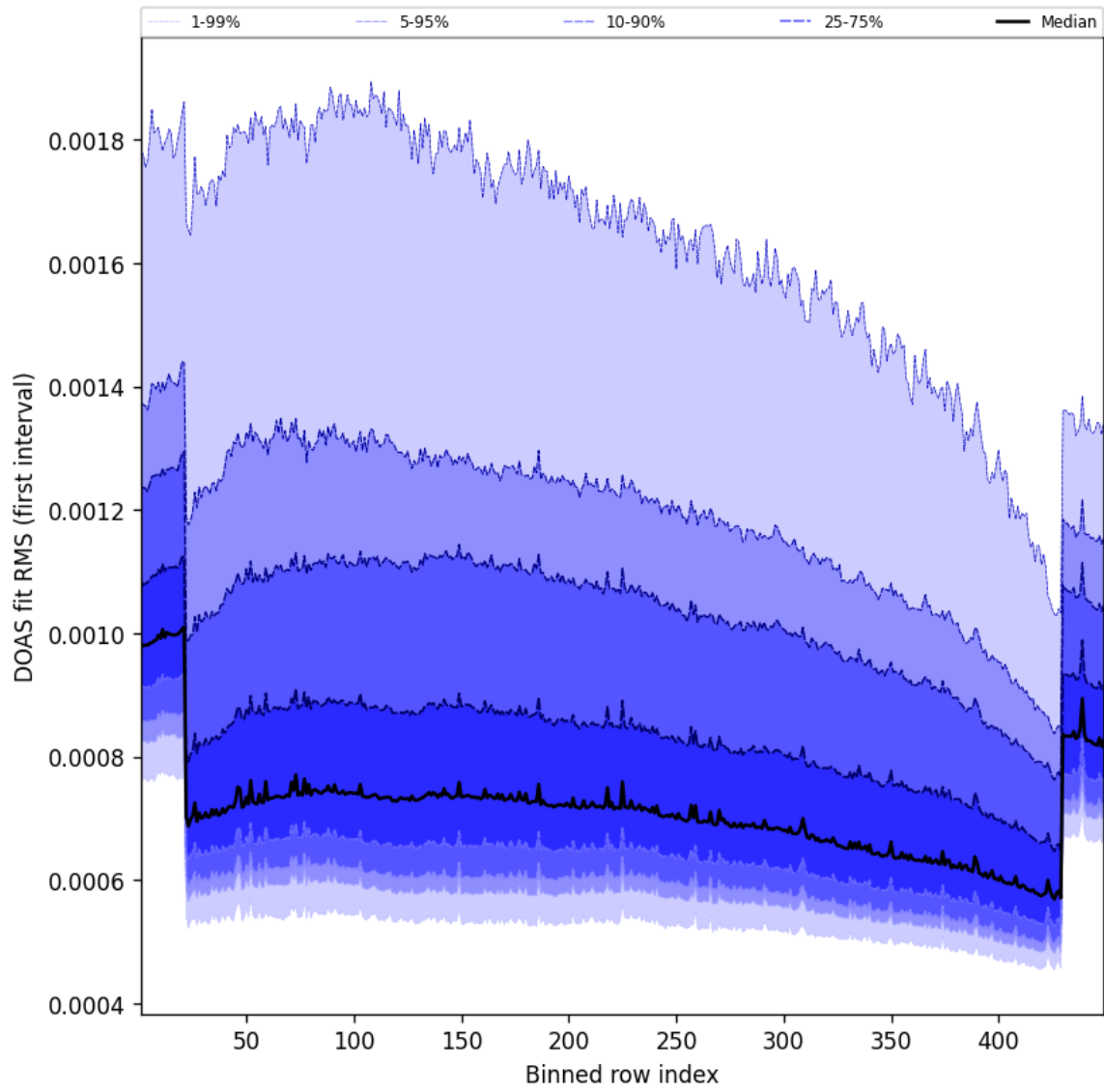
Figure 61: Along track statistics of “DOAS fit RMS (first interval)” for 2025-12-14 to 2025-12-15
