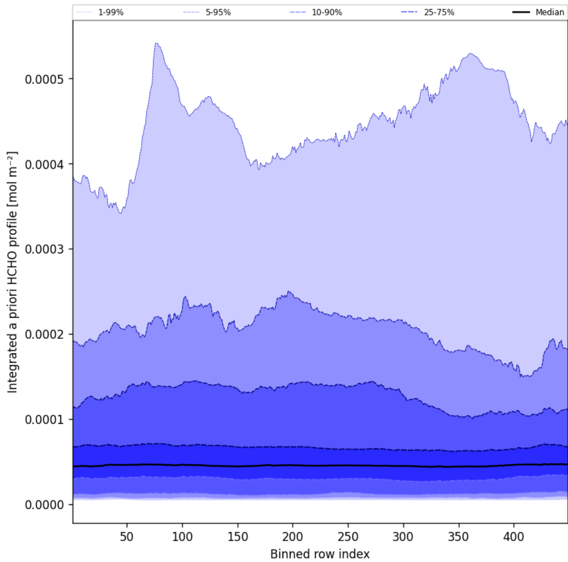
Figure 58: Along track statistics of “Integrated a priori HCHO profile” for 2025-12-14 to 2025-12-15
