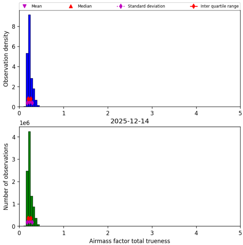
Figure 41: Histogram of “Airmass factor total trueness” for 2025-12-14 to 2025-12-15
