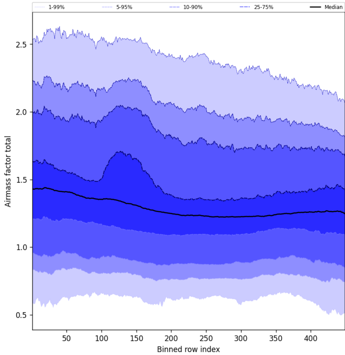
Figure 55: Along track statistics of “Airmass factor total” for 2025-12-14 to 2025-12-15
