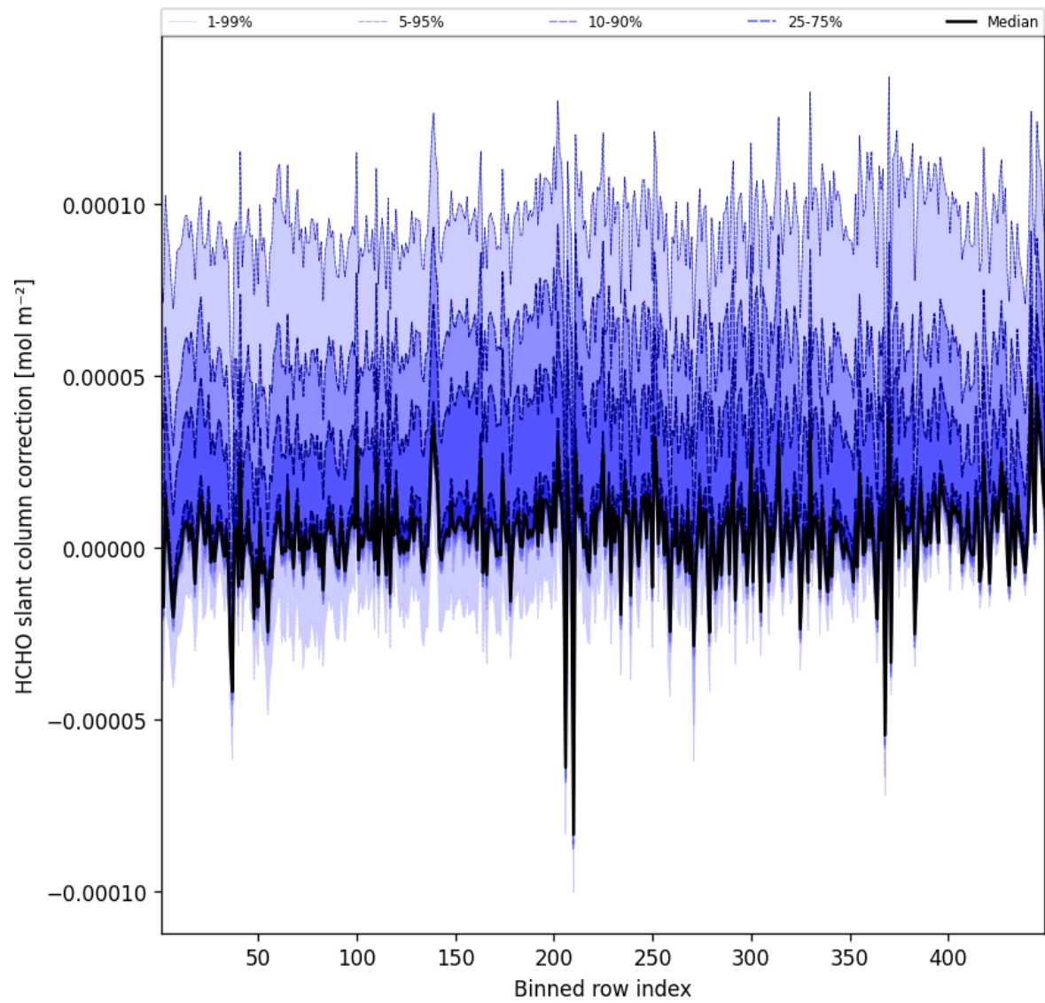
Figure 62: Along track statistics of “HCHO slant column correction” for 2025-12-14 to 2025-12-15
