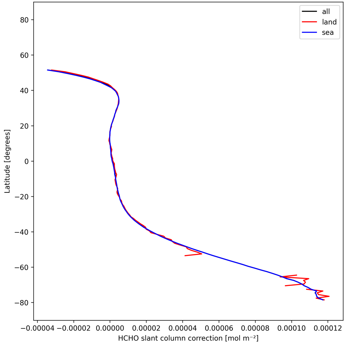
Figure 32: Zonal average of “HCHO slant column correction” for 2025-12-14 to 2025-12-15.
