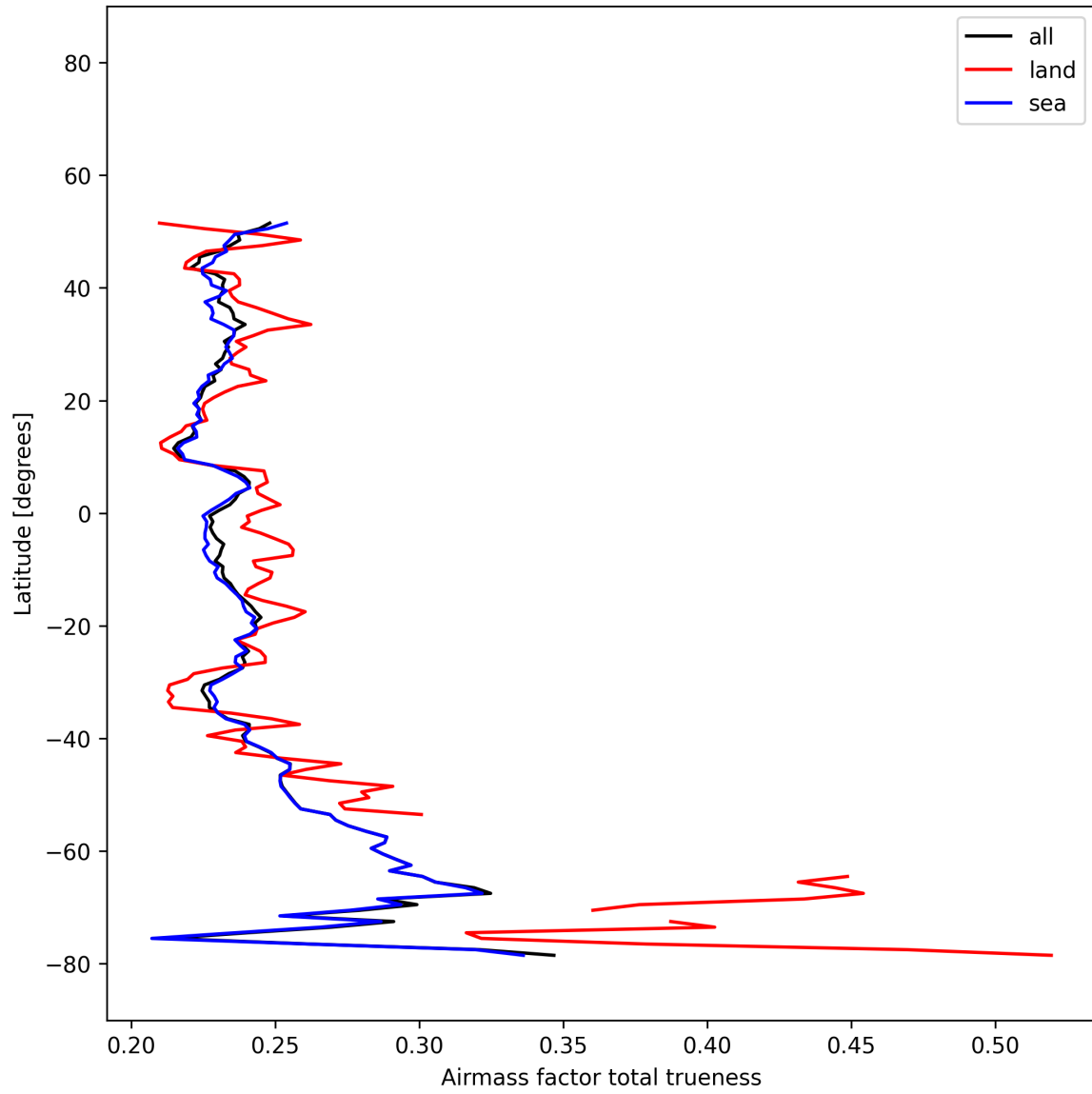
Figure 26: Zonal average of “Airmass factor total trueness” for 2025-12-14 to 2025-12-15.
