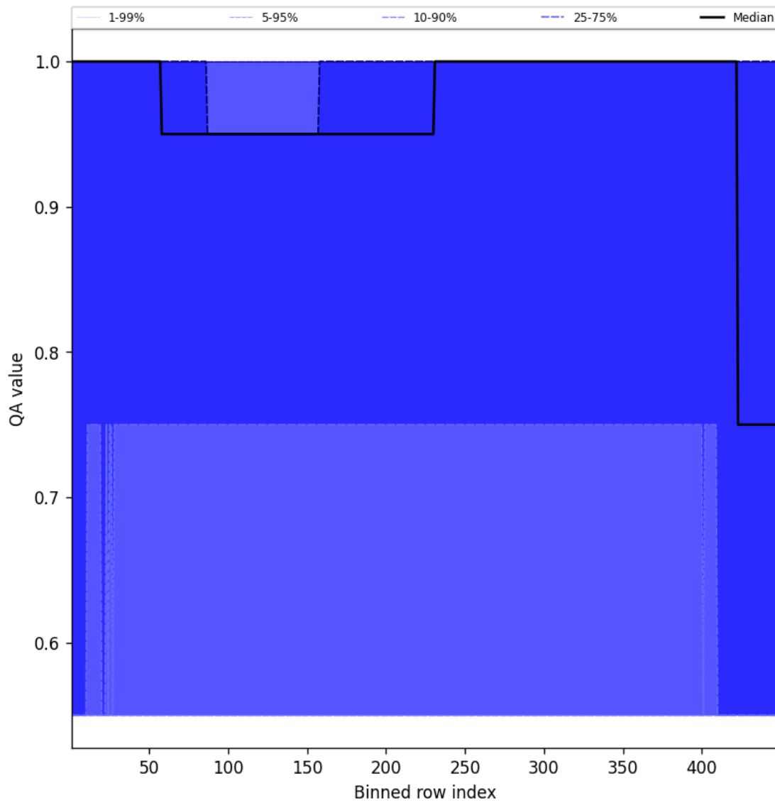
Figure 49: Along track statistics of “QA value” for 2025-12-14 to 2025-12-15
