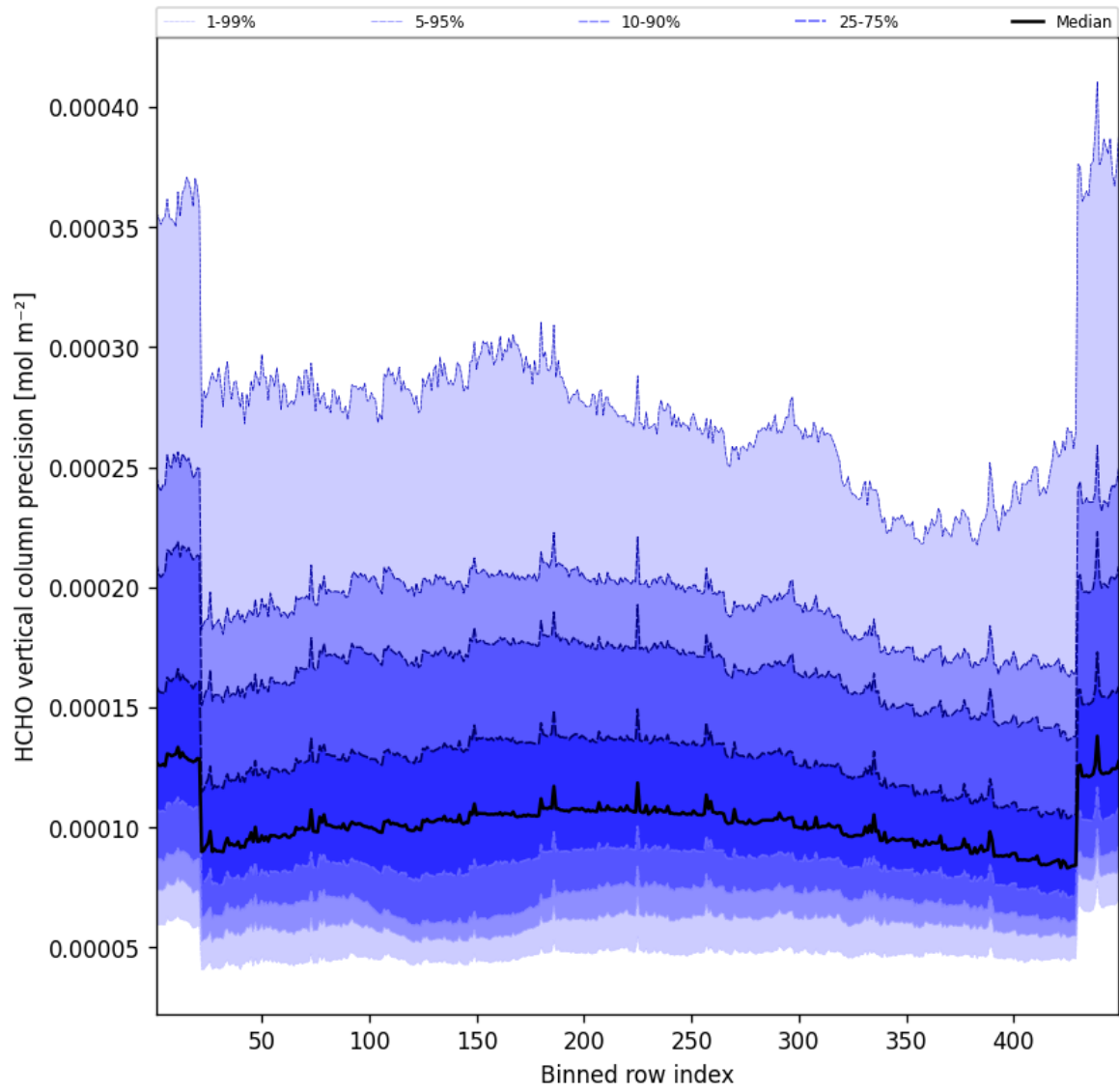
Figure 51: Along track statistics of “HCHO vertical column precision” for 2025-12-14 to 2025-12-15
