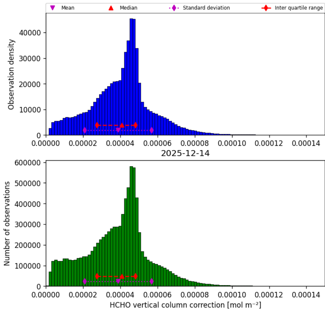
Figure 37: Histogram of “HCHO vertical column correction” for 2025-12-14 to 2025-12-15
