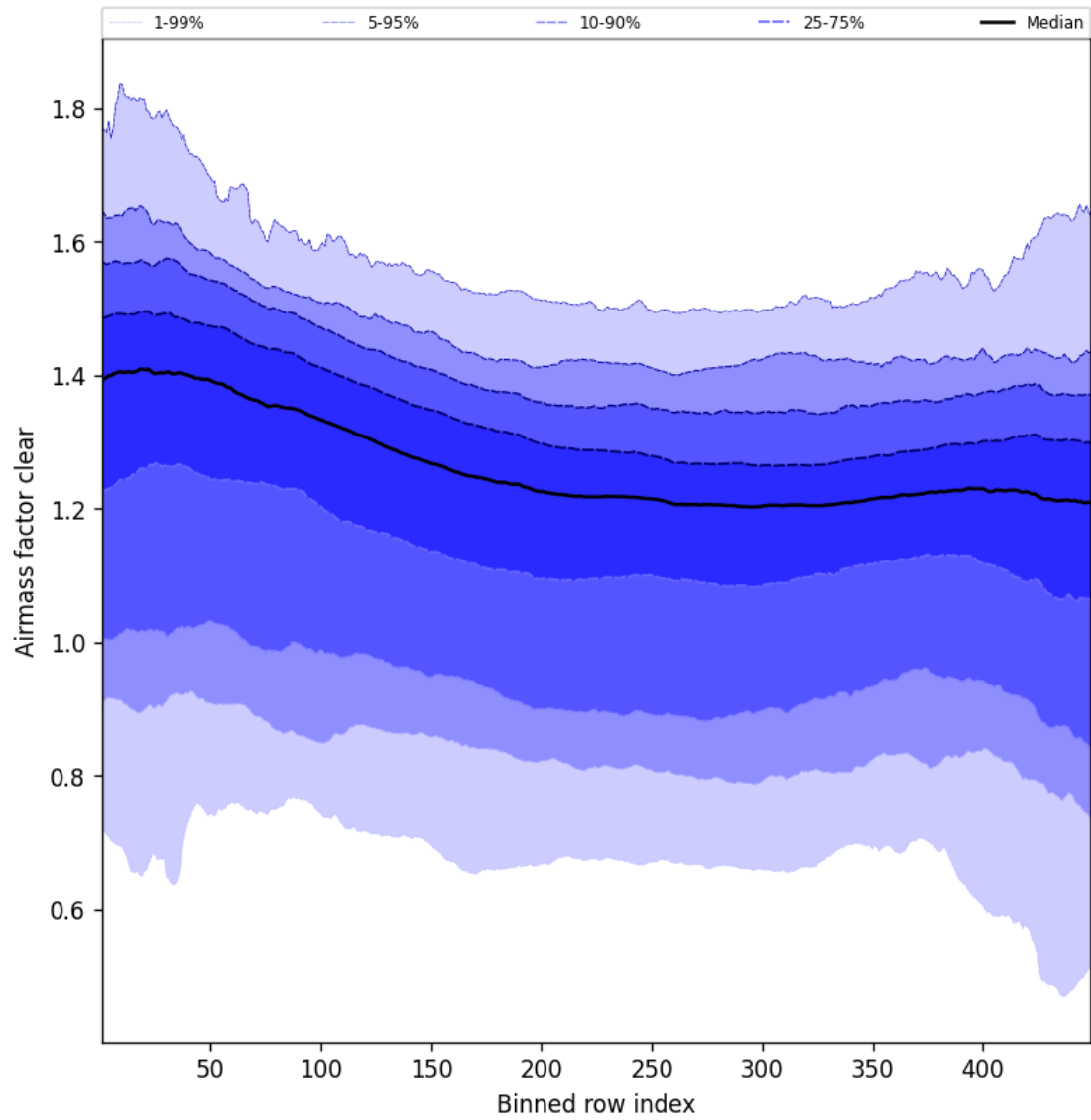
Figure 57: Along track statistics of “Airmass factor clear” for 2025-12-14 to 2025-12-15
