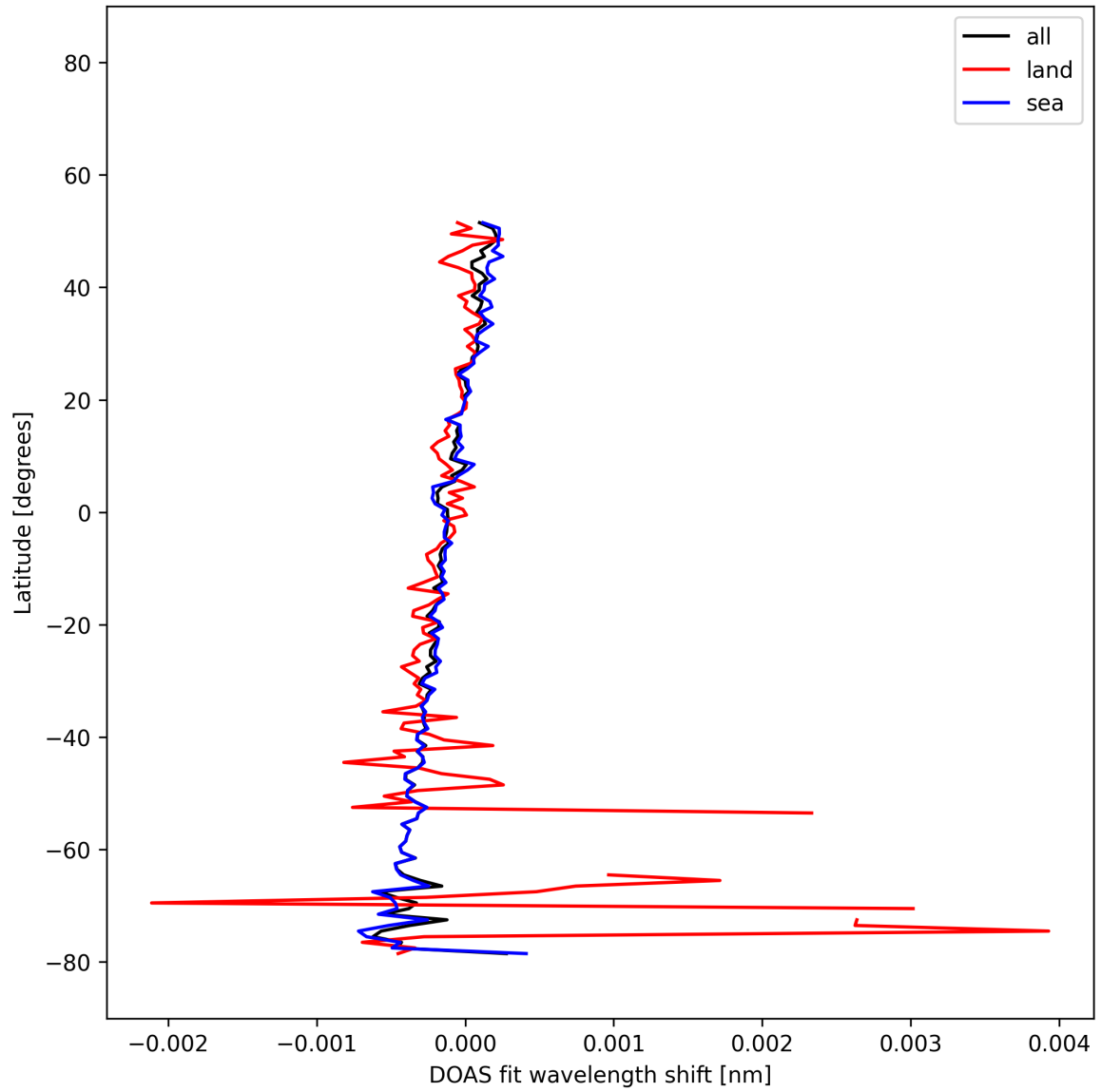
Figure 29: Zonal average of "DOAS fit wavelength shift" for 2025-12-14 to 2025-12-15.
