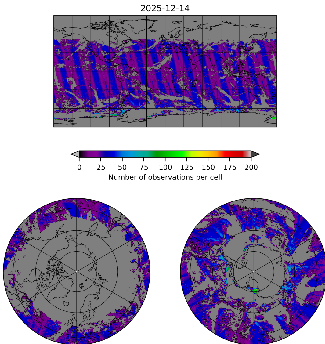
Figure 18: Map of the number of observations for 2025-12-14 to 2025-12-15
