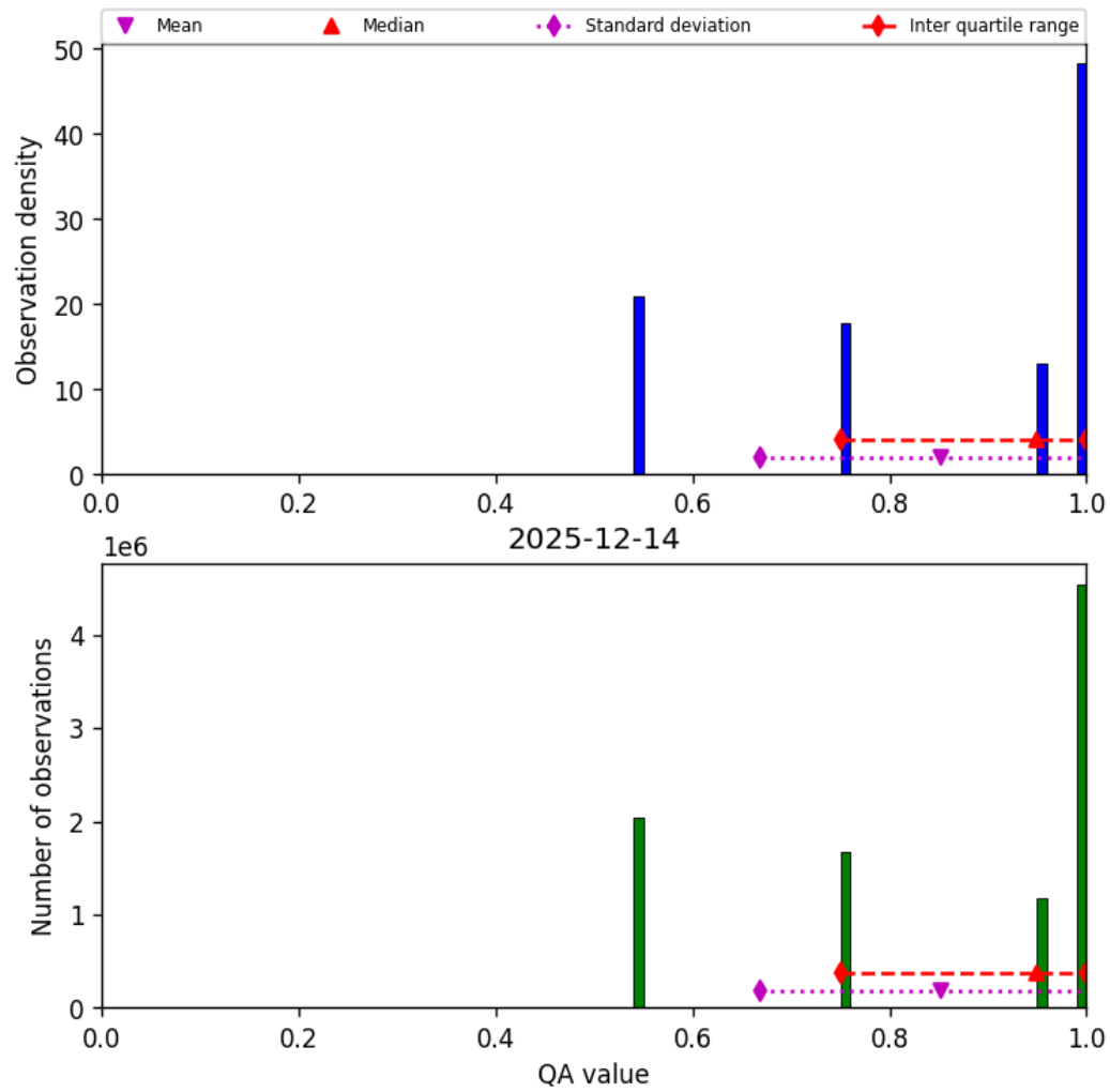
Figure 34: Histogram of “QA value” for 2025-12-14 to 2025-12-15
