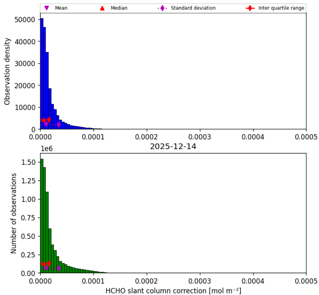
Figure 47: Histogram of “HCHO slant column correction” for 2025-12-14 to 2025-12-15
