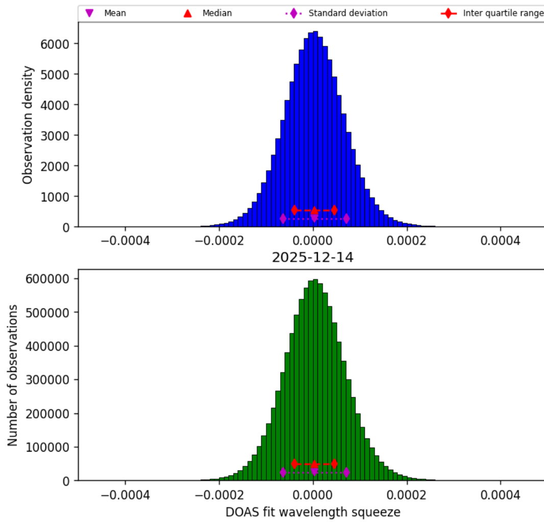
Figure 45: Histogram of “DOAS fit wavelength squeeze” for 2025-12-14 to 2025-12-15
