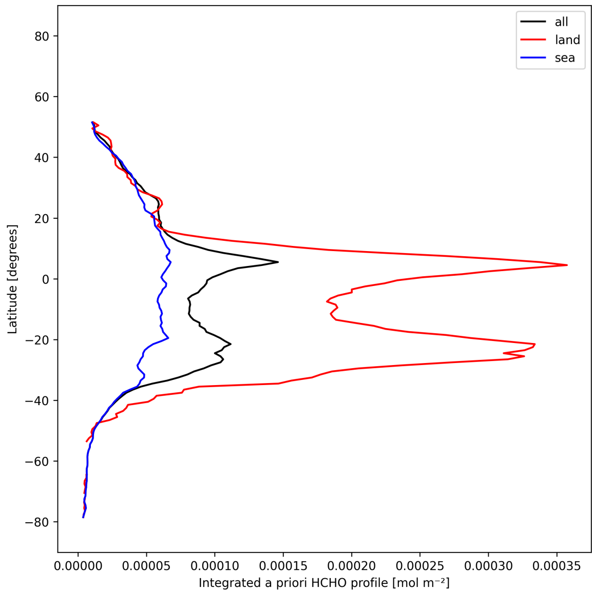
Figure 28: Zonal average of “Integrated a priori HCHO profile” for 2025-12-14 to 2025-12-15.
