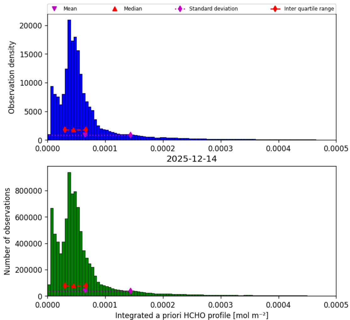
Figure 43: Histogram of “Integrated a priori HCHO profile” for 2025-12-14 to 2025-12-15
