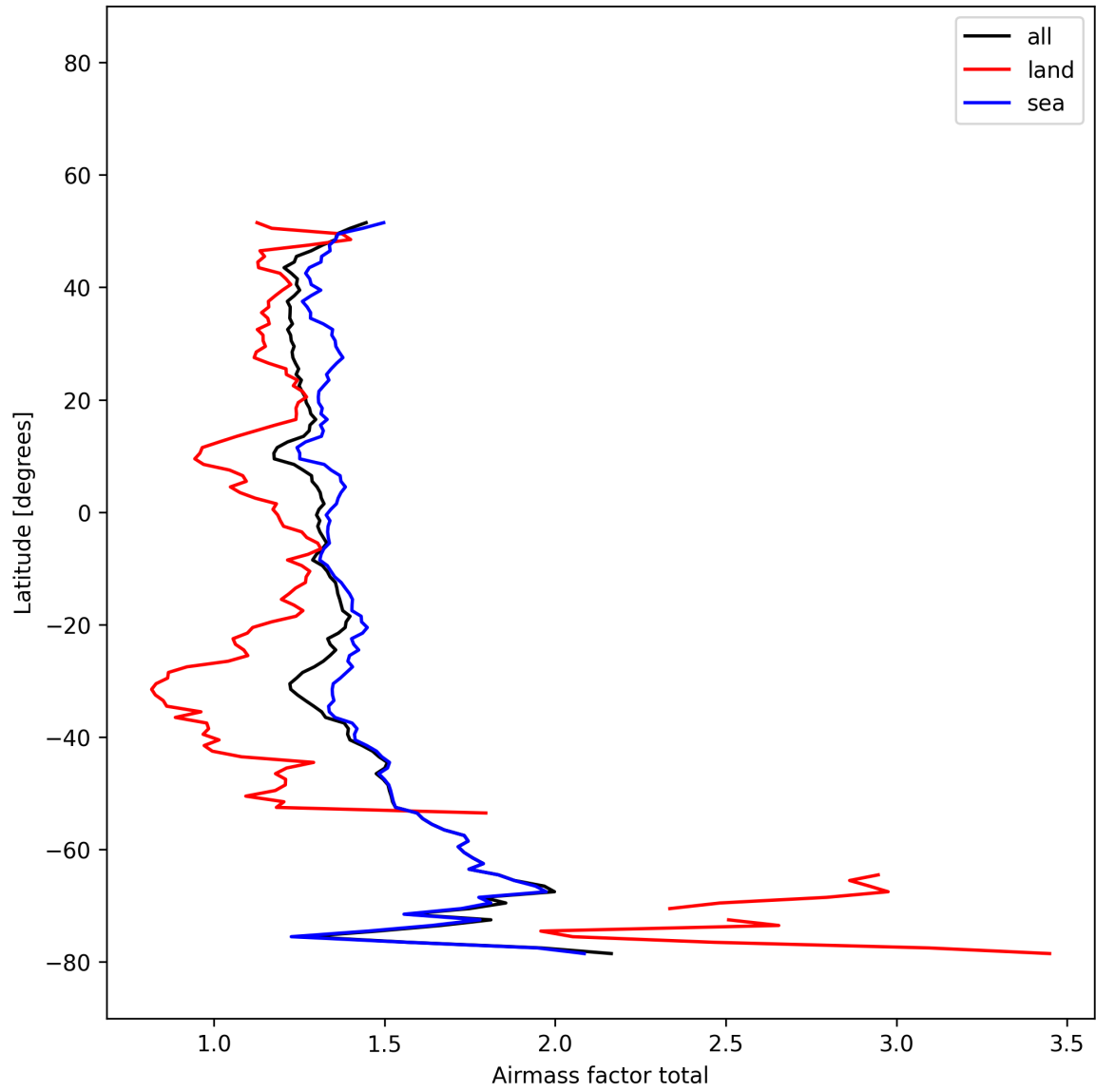
Figure 25: Zonal average of “Airmass factor total” for 2025-12-14 to 2025-12-15.
