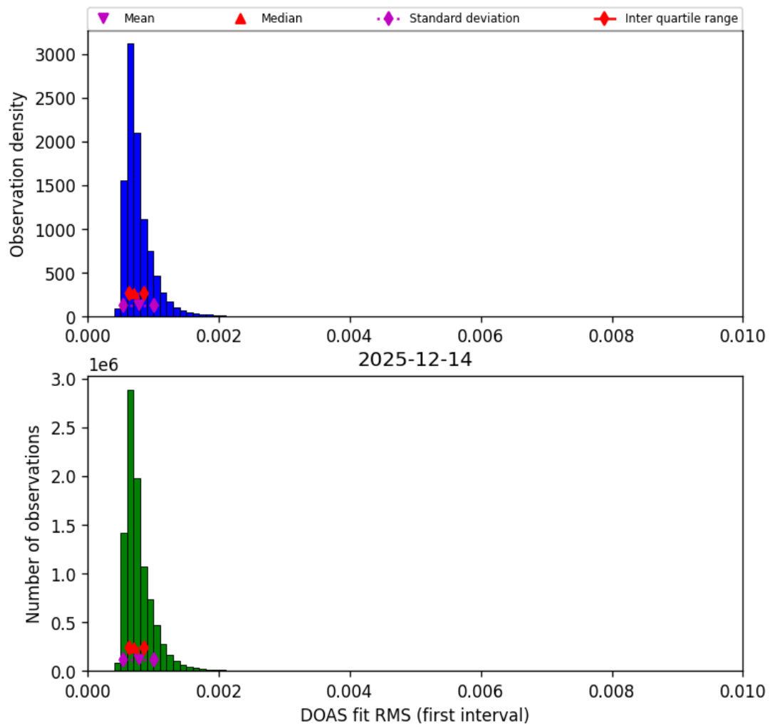
Figure 46: Histogram of “DOAS fit RMS (first interval)” for 2025-12-14 to 2025-12-15
