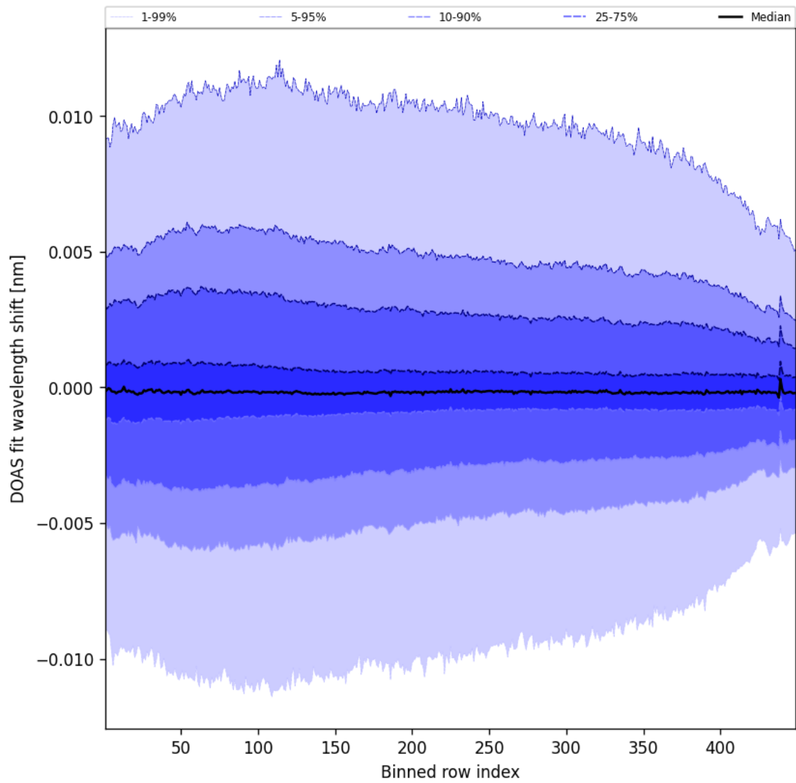
Figure 59: Along track statistics of “DOAS fit wavelength shift” for 2025-12-14 to 2025-12-15
