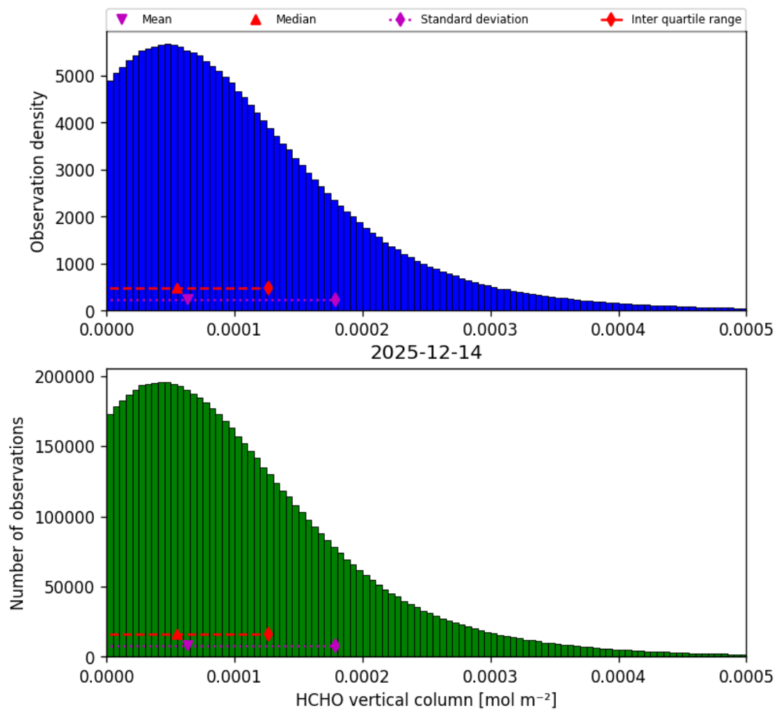
Figure 35: Histogram of “HCHO vertical column” for 2025-12-14 to 2025-12-15
