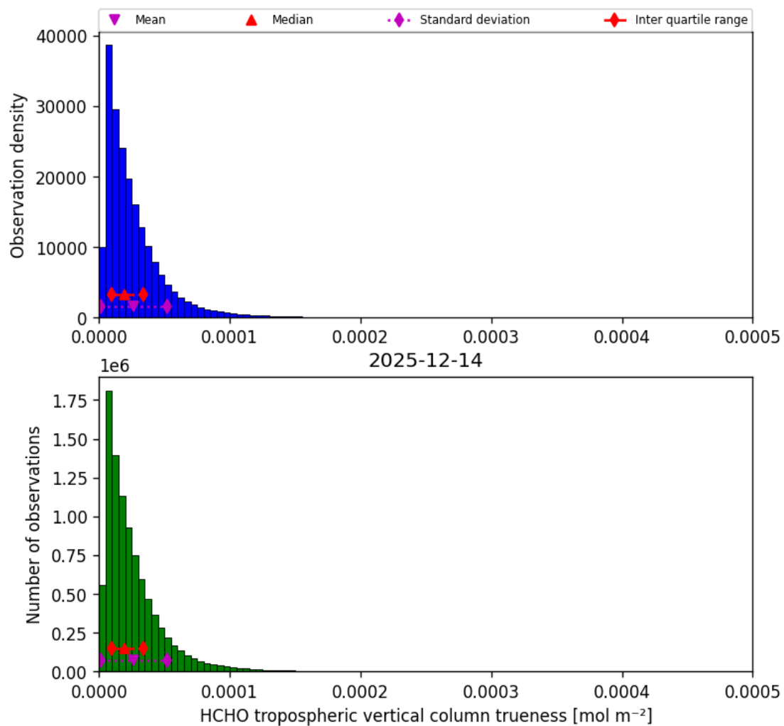
Figure 48: Histogram of “HCHO tropospheric vertical column trueness” for 2025-12-14 to 2025-12-15
