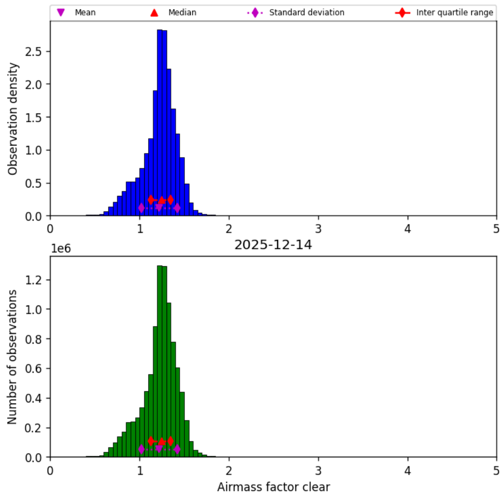
Figure 42: Histogram of “Airmass factor clear” for 2025-12-14 to 2025-12-15
