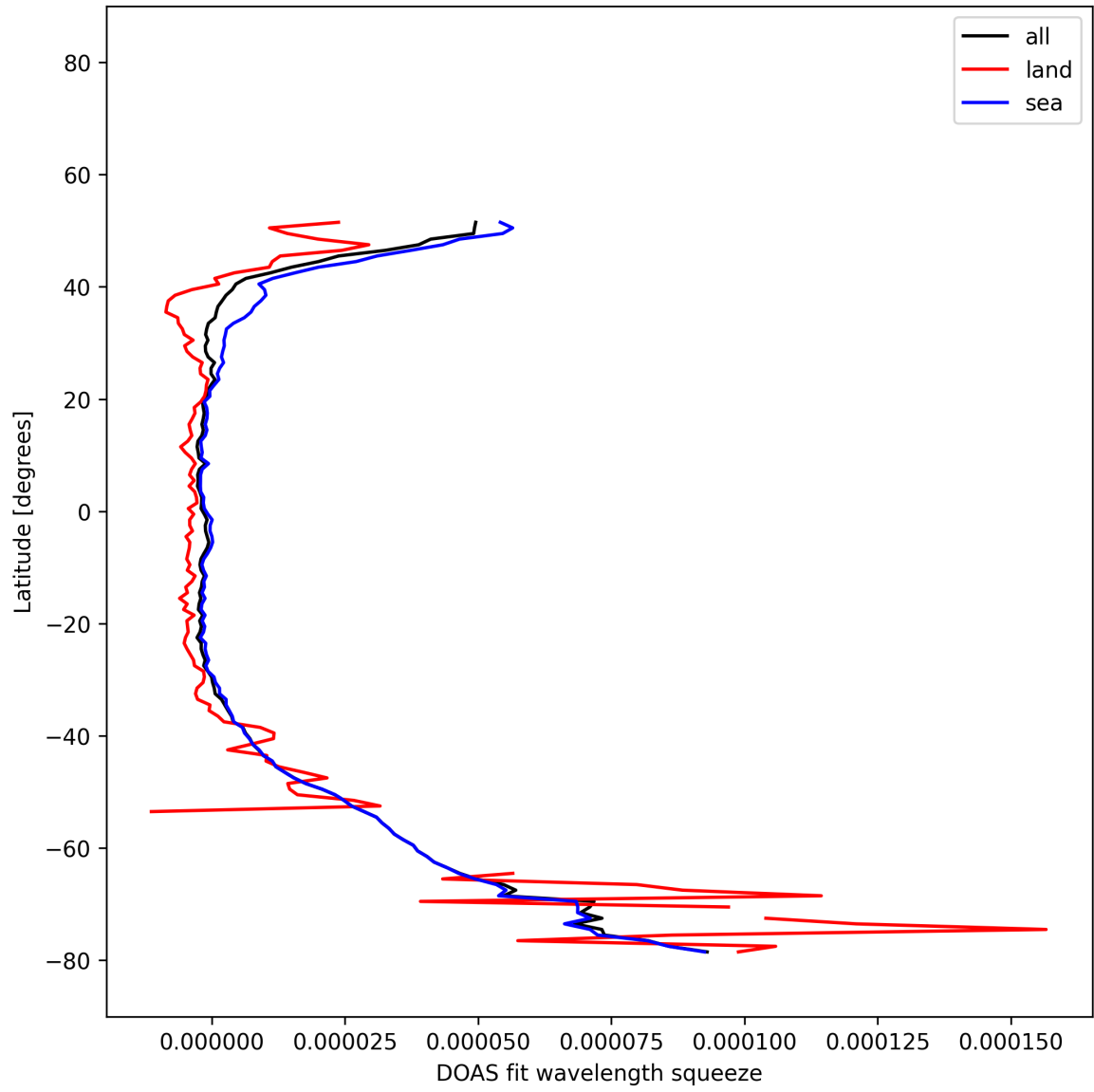
Figure 30: Zonal average of “DOAS fit wavelength squeeze” for 2025-12-14 to 2025-12-15.
