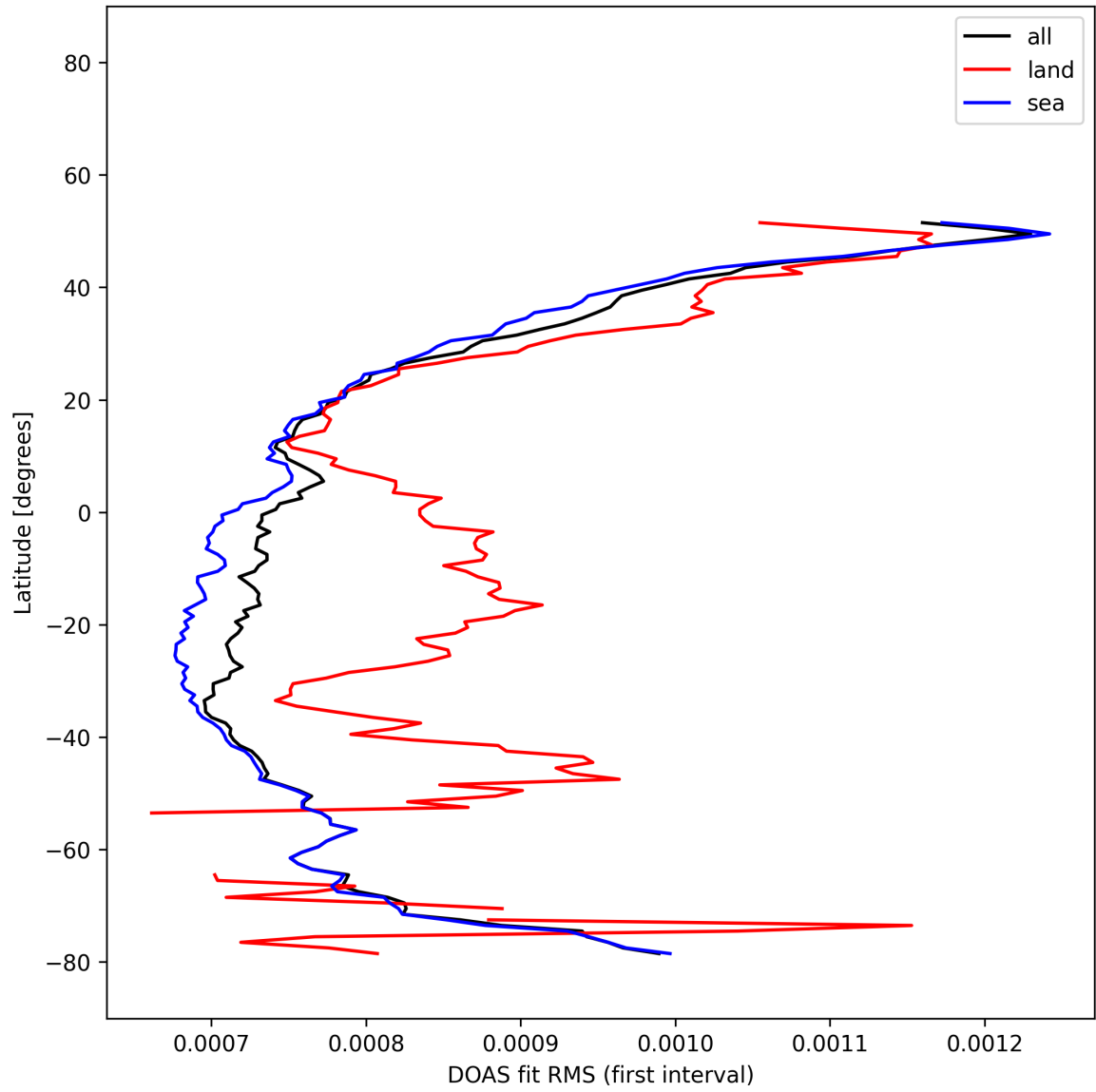
Figure 31: Zonal average of “DOAS fit RMS (first interval)” for 2025-12-14 to 2025-12-15.
