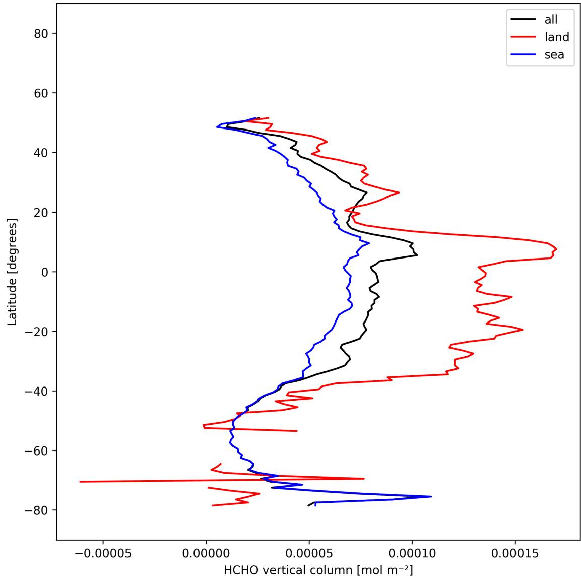
Figure 20: Zonal average of “HCHO vertical column” for 2025-12-14 to 2025-12-15.
