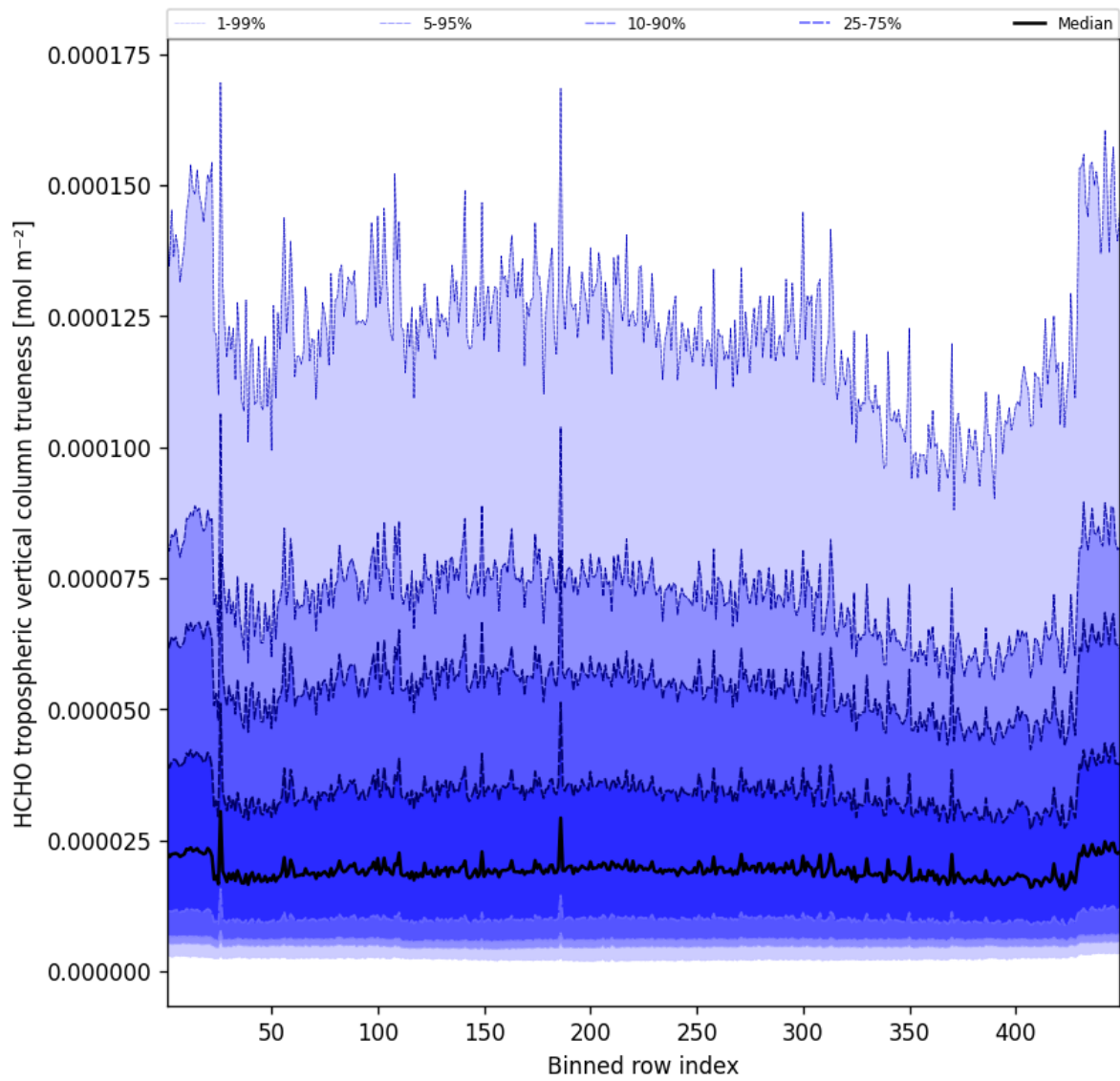
Figure 63: Along track statistics of “HCHO tropospheric vertical column trueness” for 2025-12-14 to 2025-12-15
