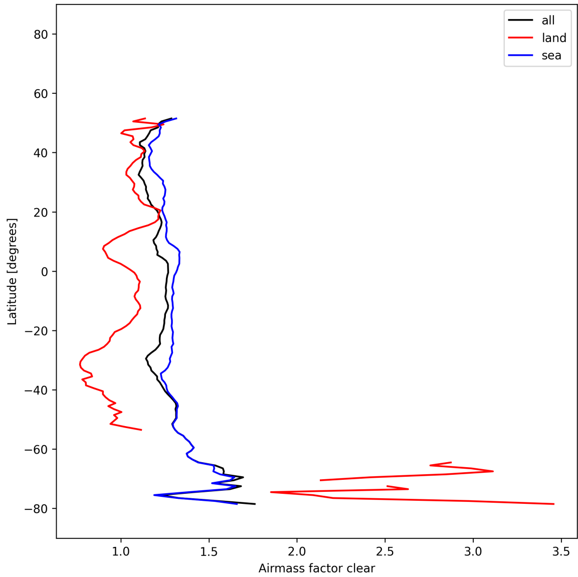
Figure 27: Zonal average of “Airmass factor clear” for 2025-12-14 to 2025-12-15.
