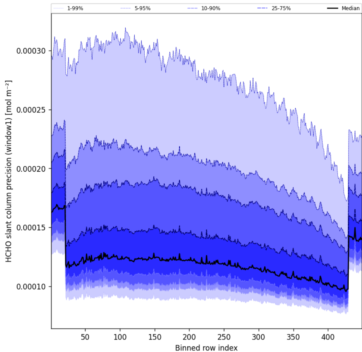
Figure 54: Along track statistics of “HCHO slant column precision (window1)” for 2025-12-14 to 2025-12-15
