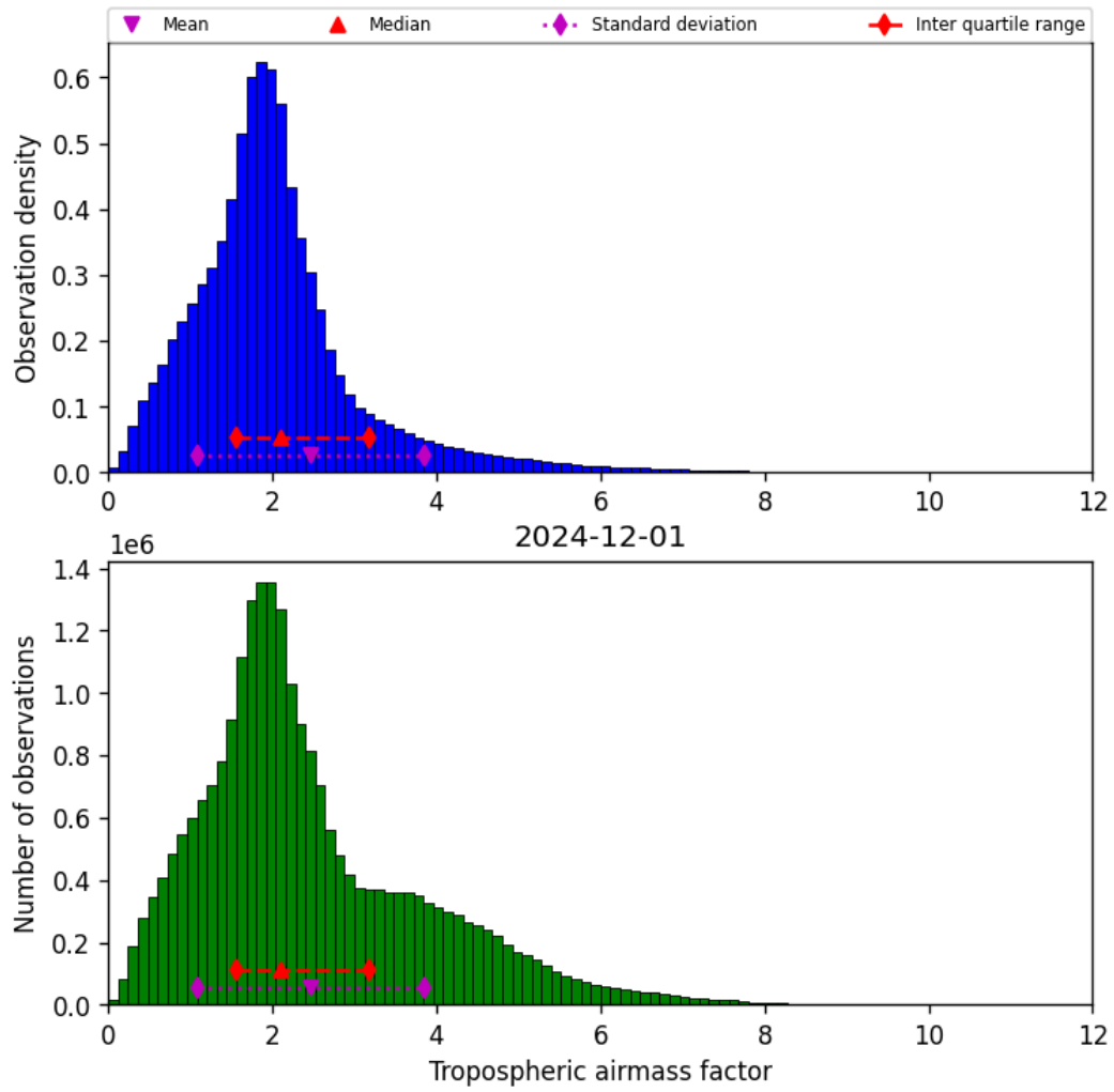
Figure 29: Histogram of “Tropospheric airmass factor” for 2024-12-01 to 2024-12-02
