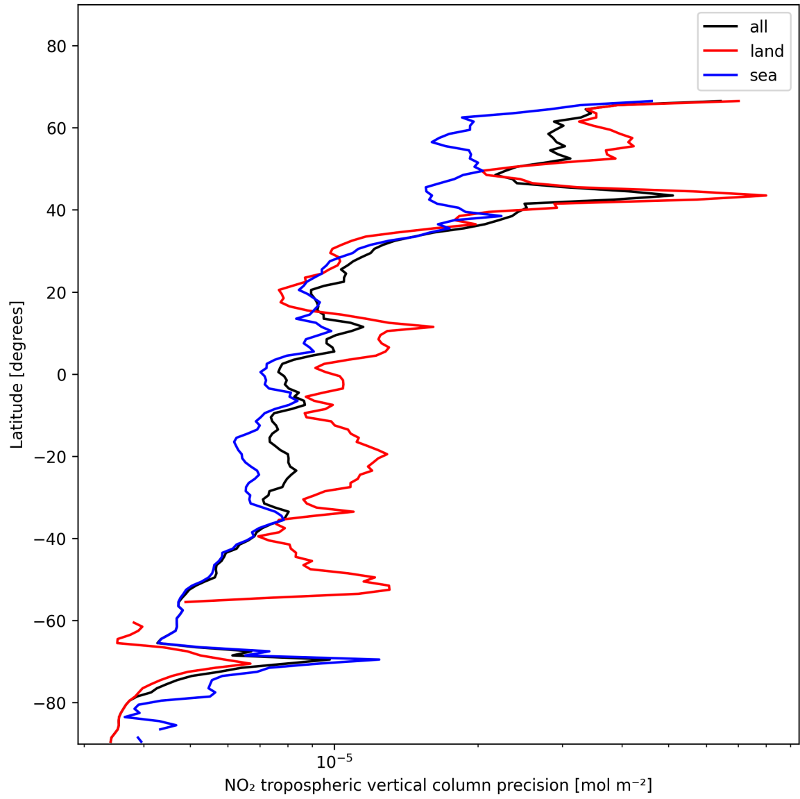
Figure 11: Zonal average of “NO 2 tropospheric vertical column precision” for 2024-12-01 to 2024-12-02.
