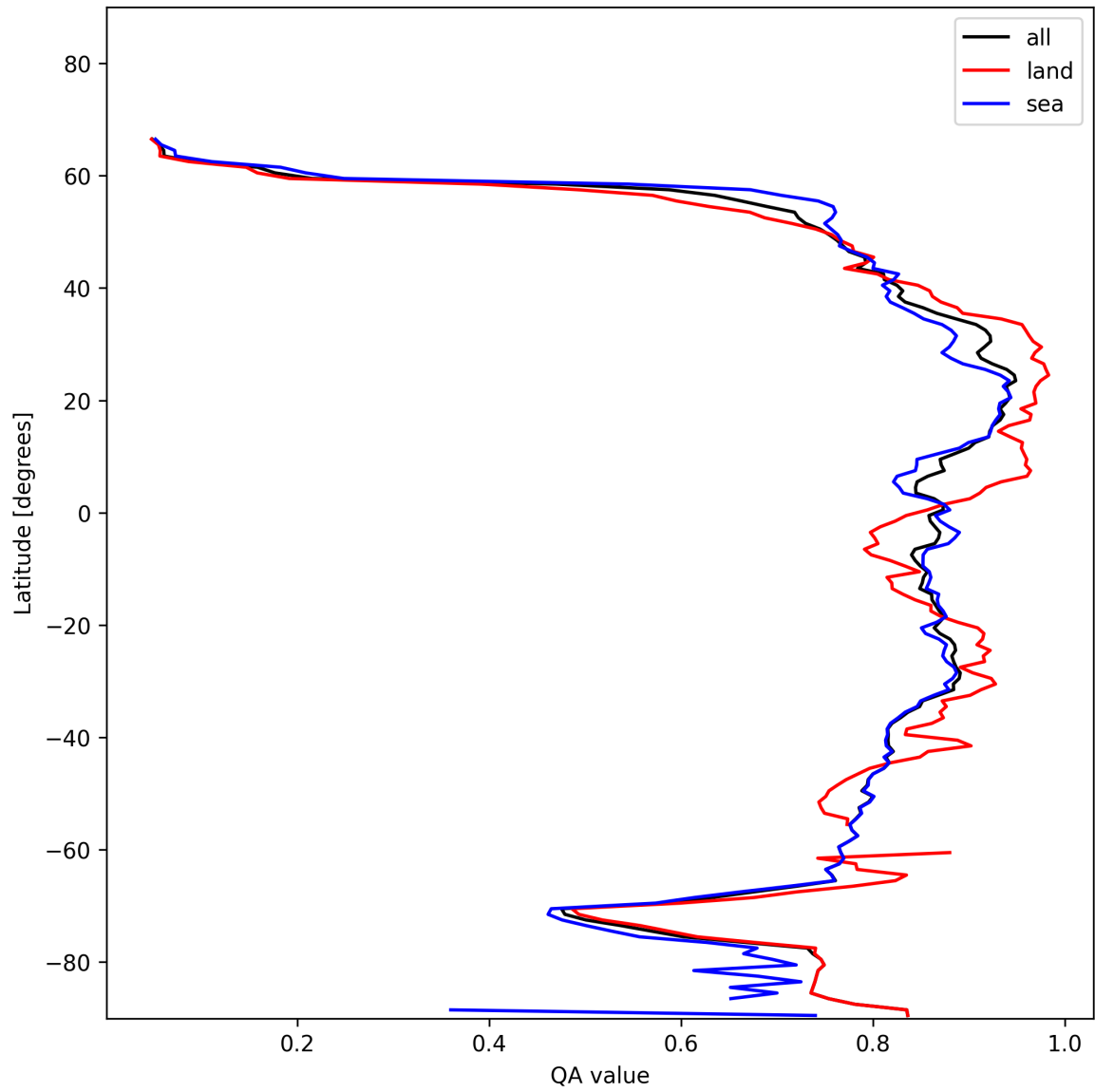
Figure 9: Zonal average of “QA value” for 2024-12-01 to 2024-12-02.
