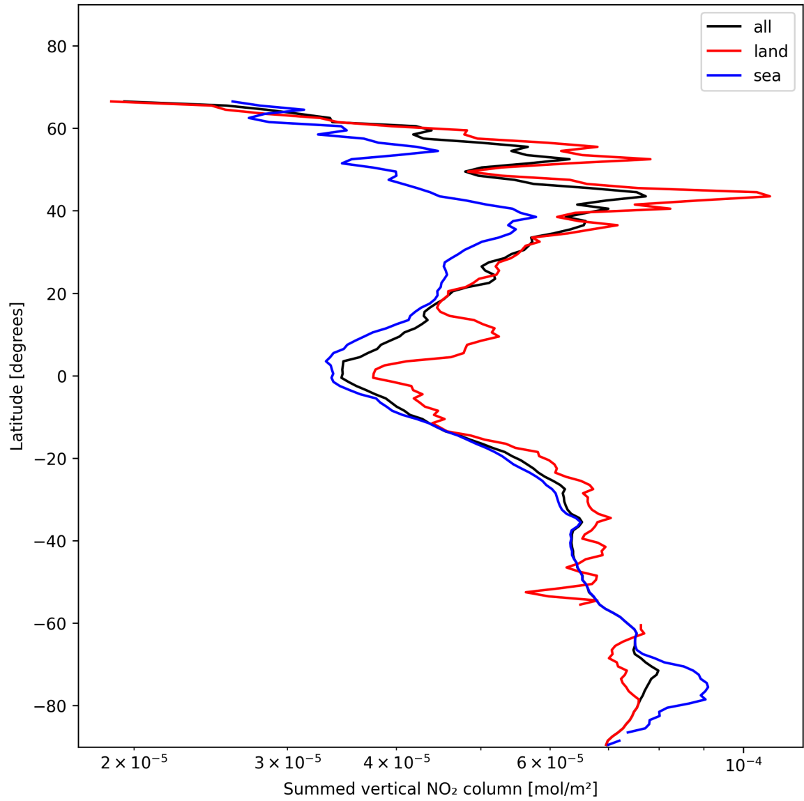
Figure 21: Zonal average of “Summed vertical NO 2 column” for 2024-12-01 to 2024-12-02.
