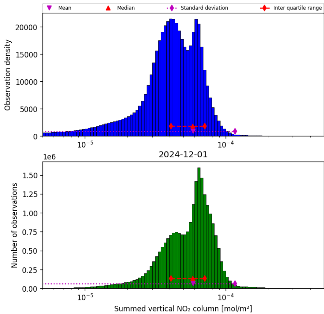
Figure 38: Histogram of “Summed vertical NO 2 column” for 2024-12-01 to 2024-12-02
