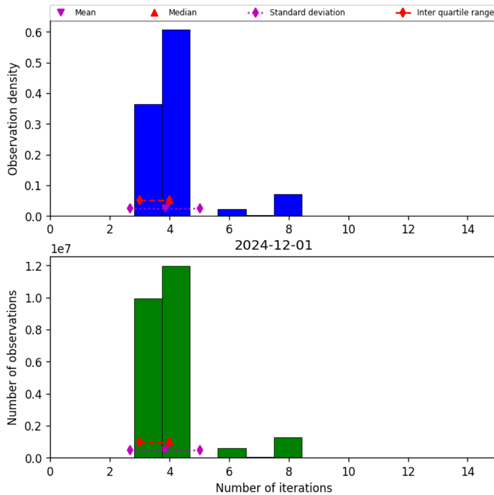
Figure 32: Histogram of “Number of iterations” for 2024-12-01 to 2024-12-02
