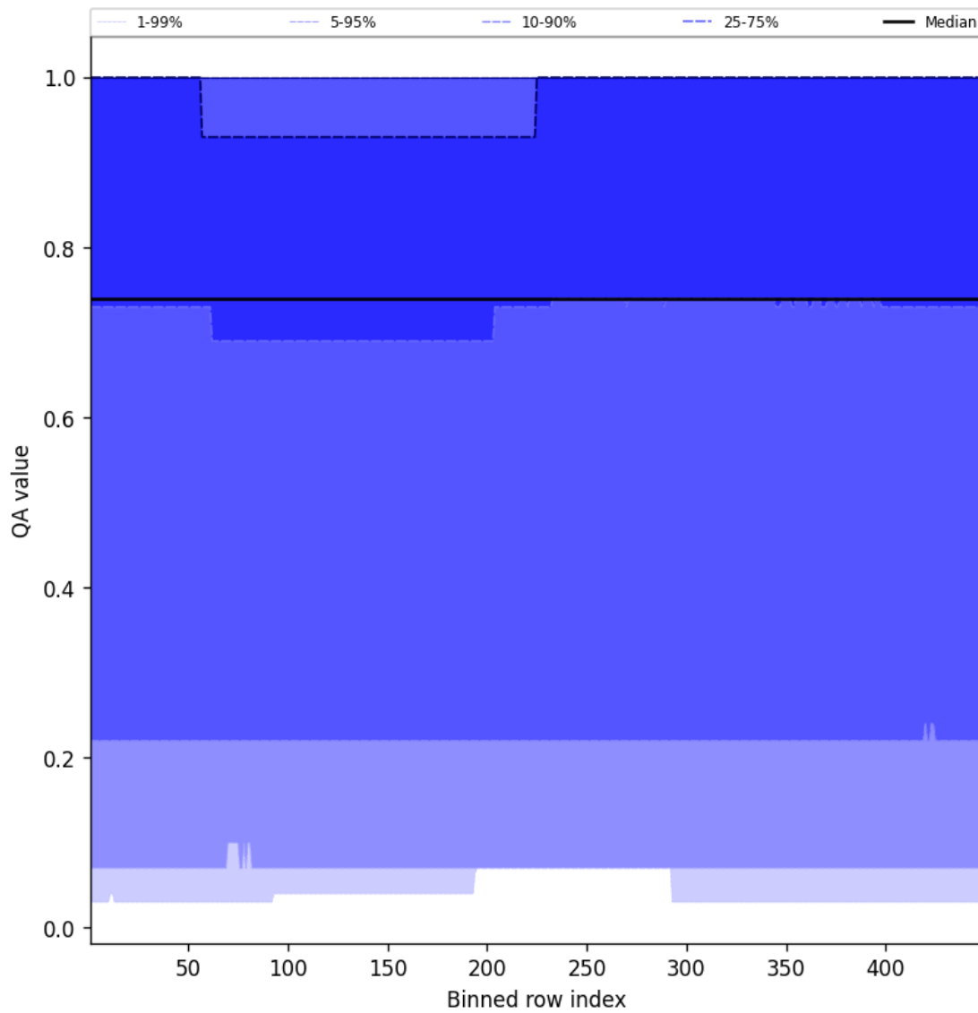
Figure 43: Along track statistics of “QA value” for 2024-12-01 to 2024-12-02
