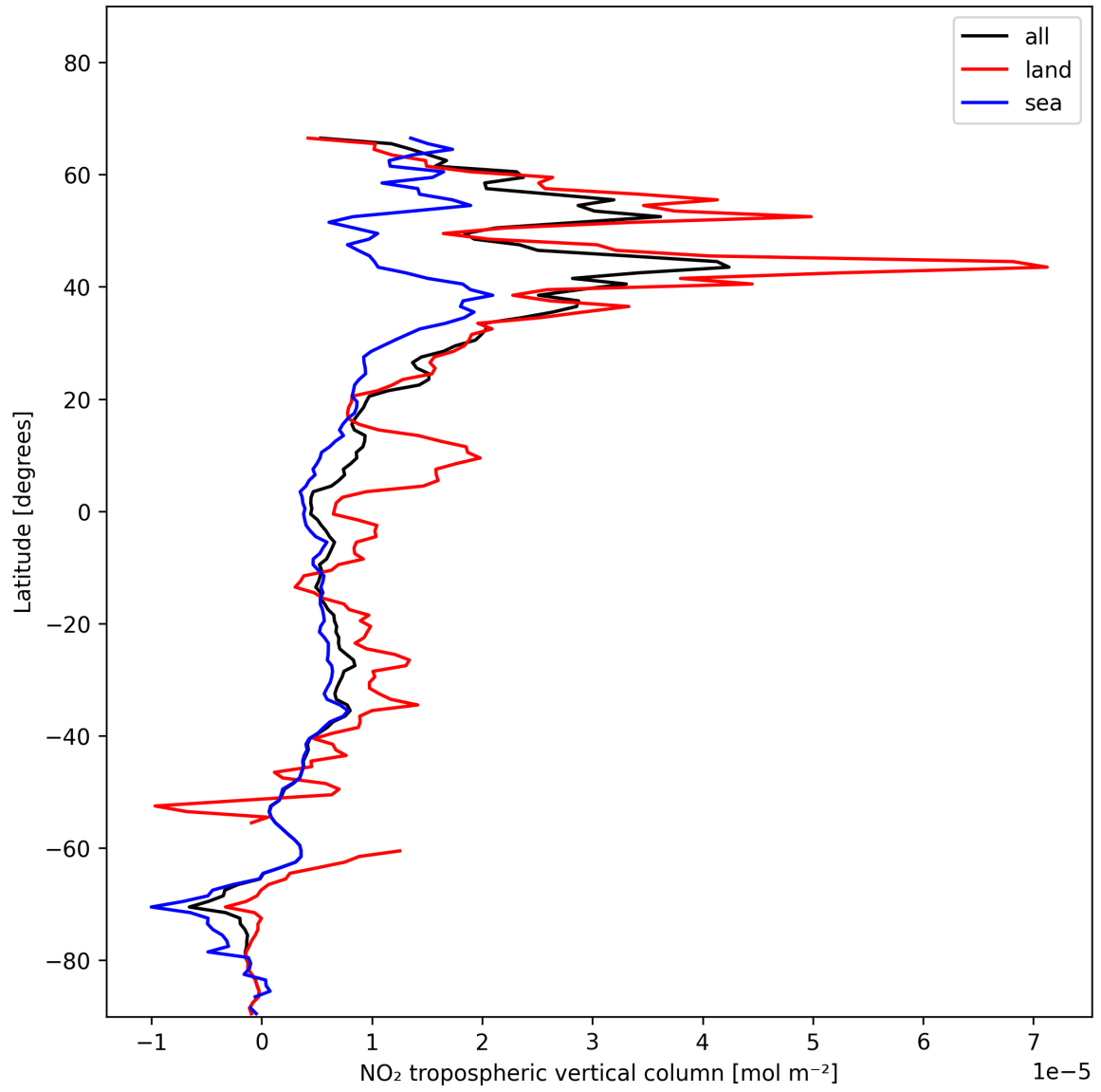
Figure 10: Zonal average of “NO 2 tropospheric vertical column” for 2024-12-01 to 2024-12-02.
