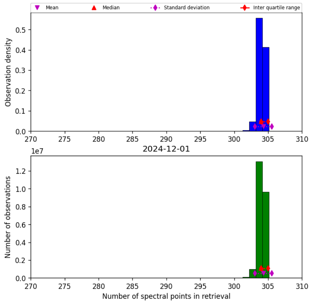
Figure 31: Histogram of “Number of spectral points in retrieval” for 2024-12-01 to 2024-12-02
