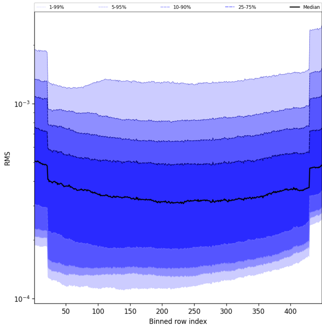
Figure 58: Along track statistics of “RMS” for 2024-12-01 to 2024-12-02
