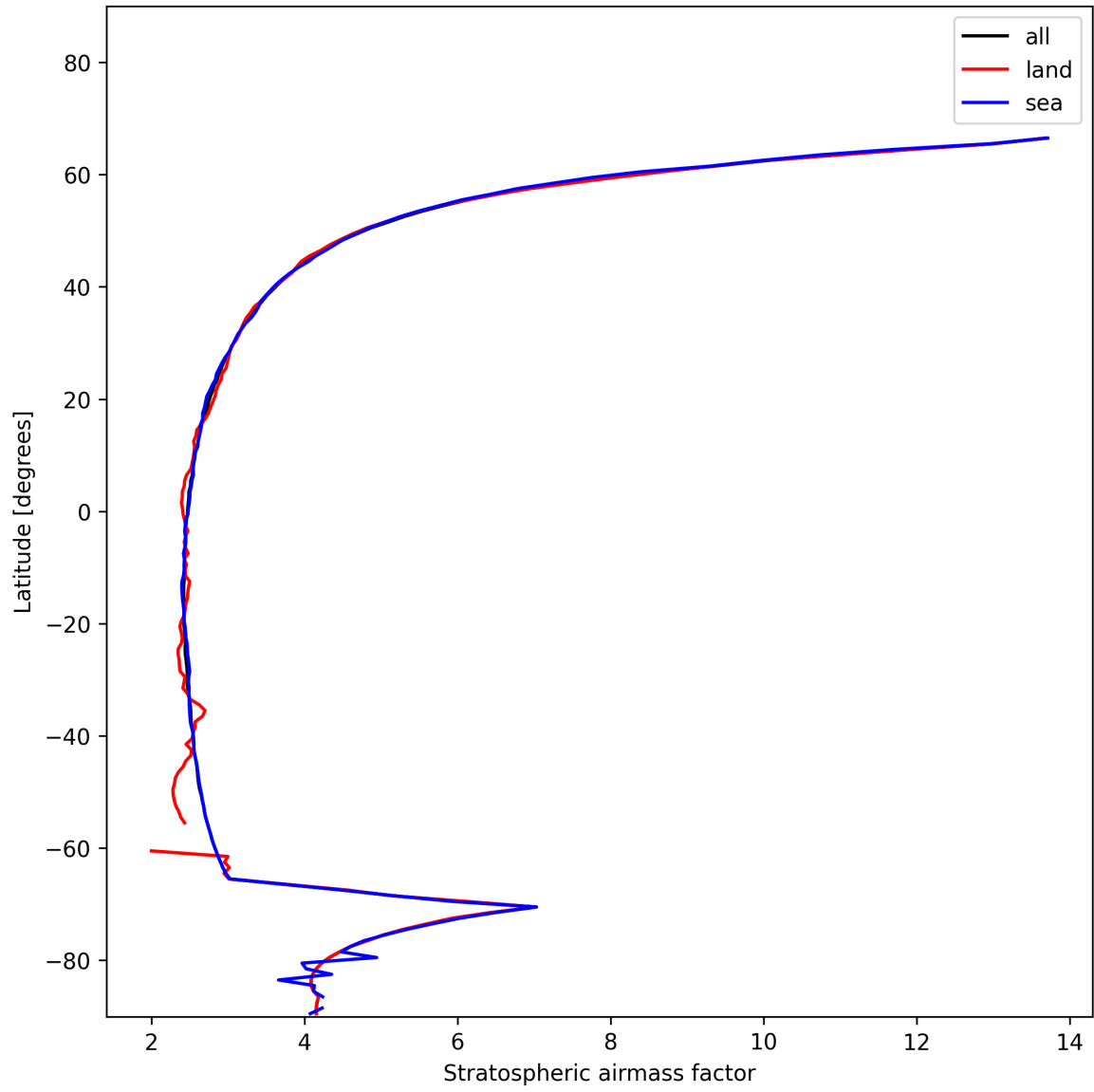
Figure 25: Zonal average of “Stratospheric air mass factor” for 2024-12-01 to 2024-12-02.
