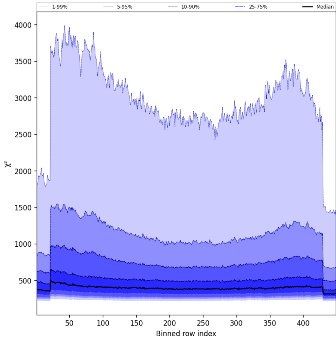
Figure 57: Along track statistics of “ \chi^2 ” for 2024-12-01 to 2024-12-02
