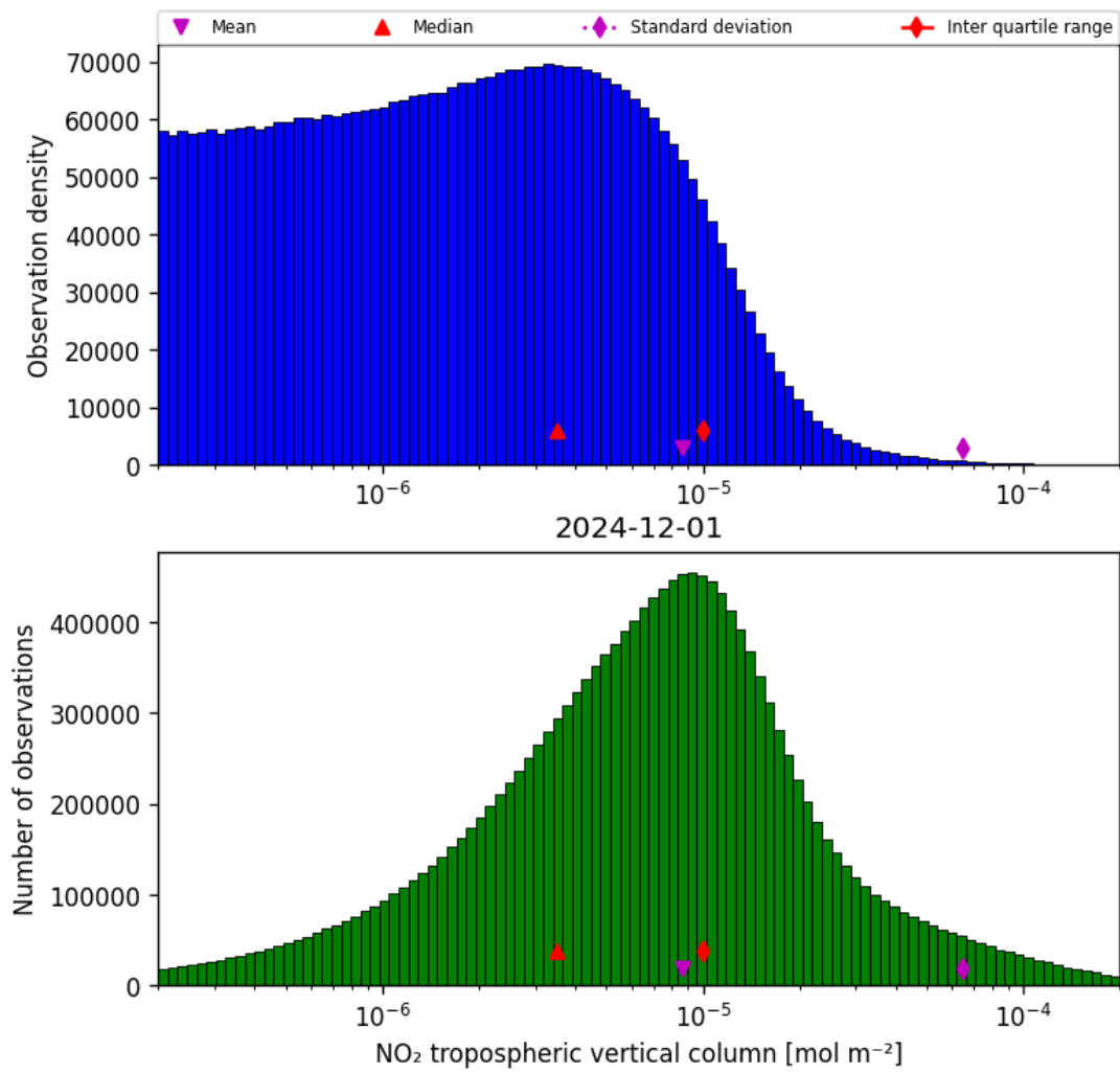
Figure 27: Histogram of “NO 2 tropospheric vertical column” for 2024-12-01 to 2024-12-02
