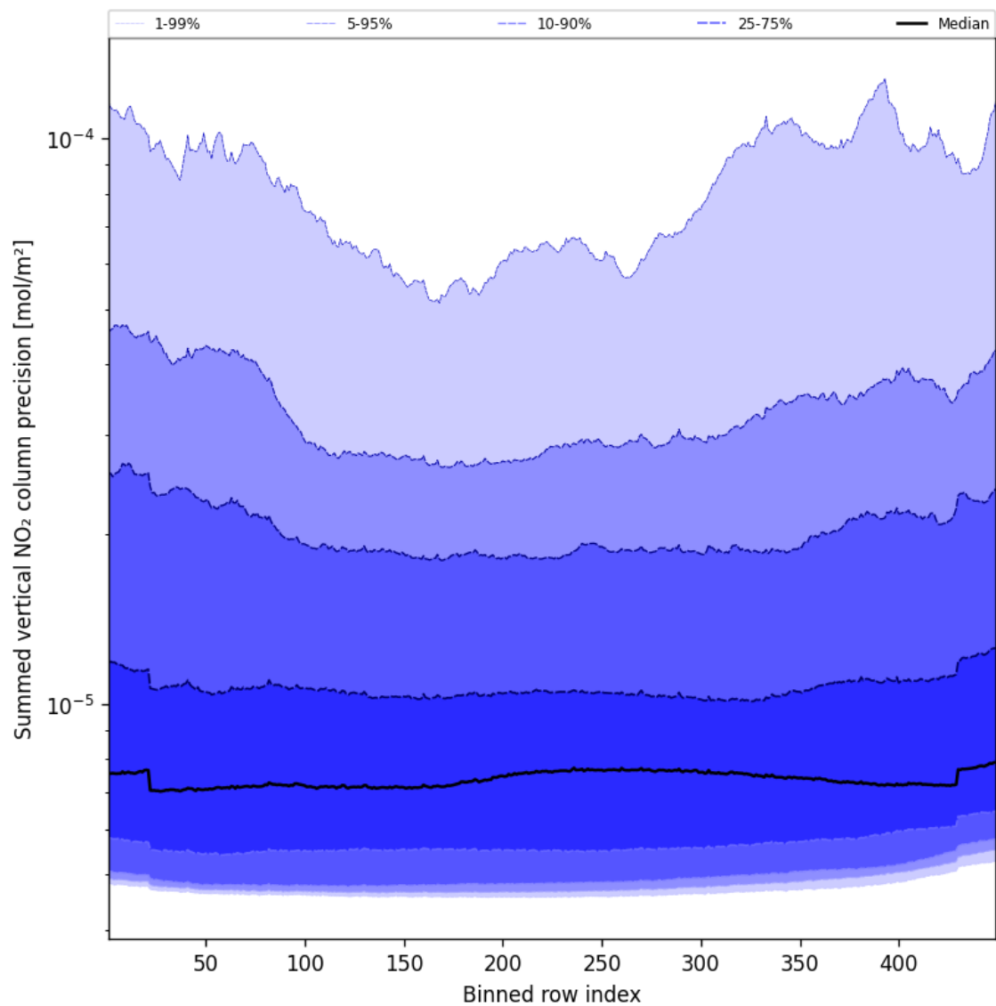
Figure 56: Along track statistics of “Summed vertical NO 2 column precision” for 2024-12-01 to 2024-12-02
