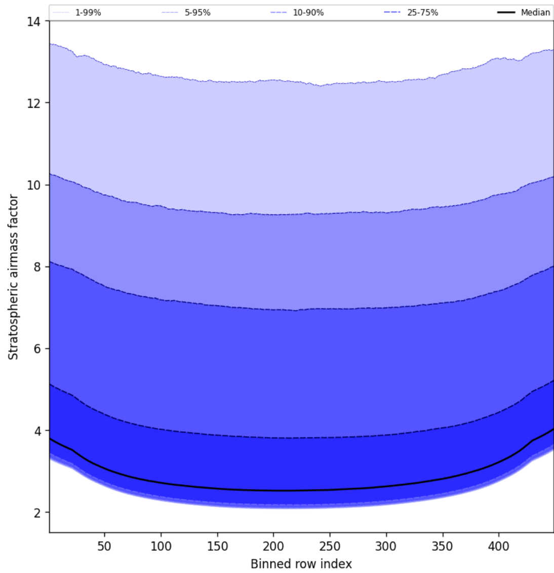
Figure 59: Along track statistics of “Stratospheric airmass factor” for 2024-12-01 to 2024-12-02
