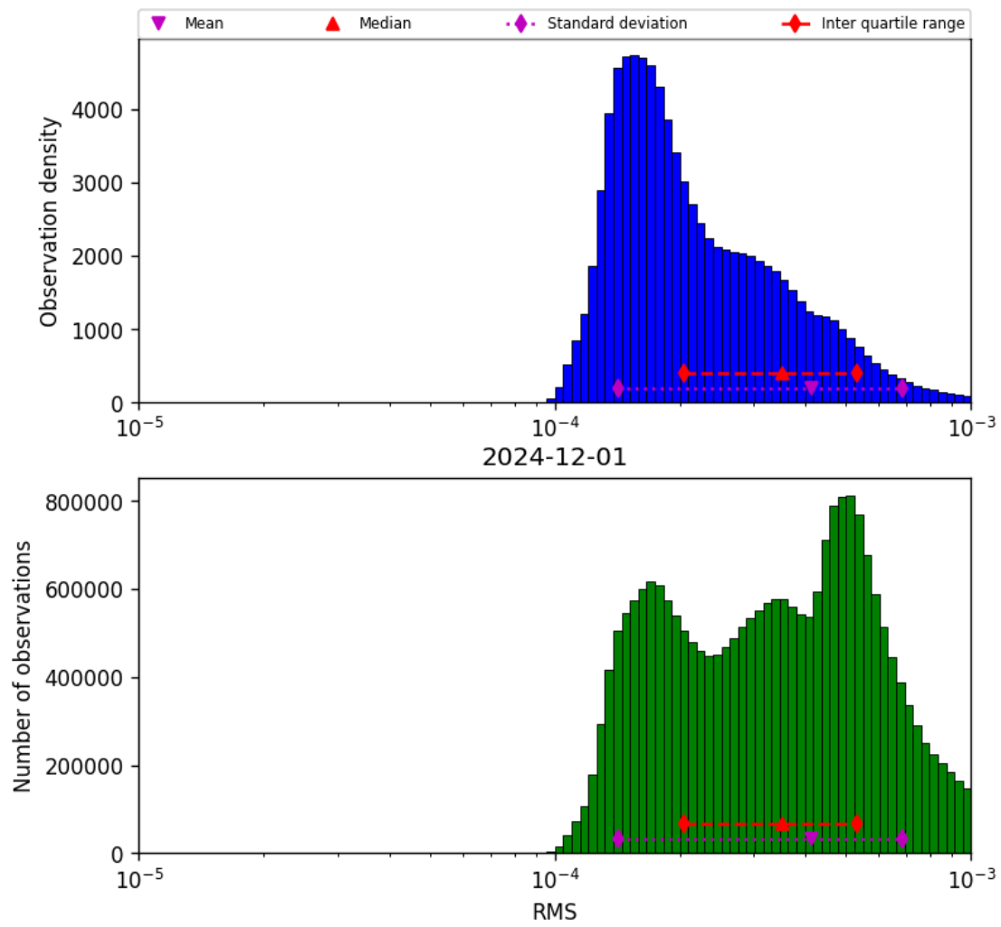
Figure 41: Histogram of “RMS” for 2024-12-01 to 2024-12-02
