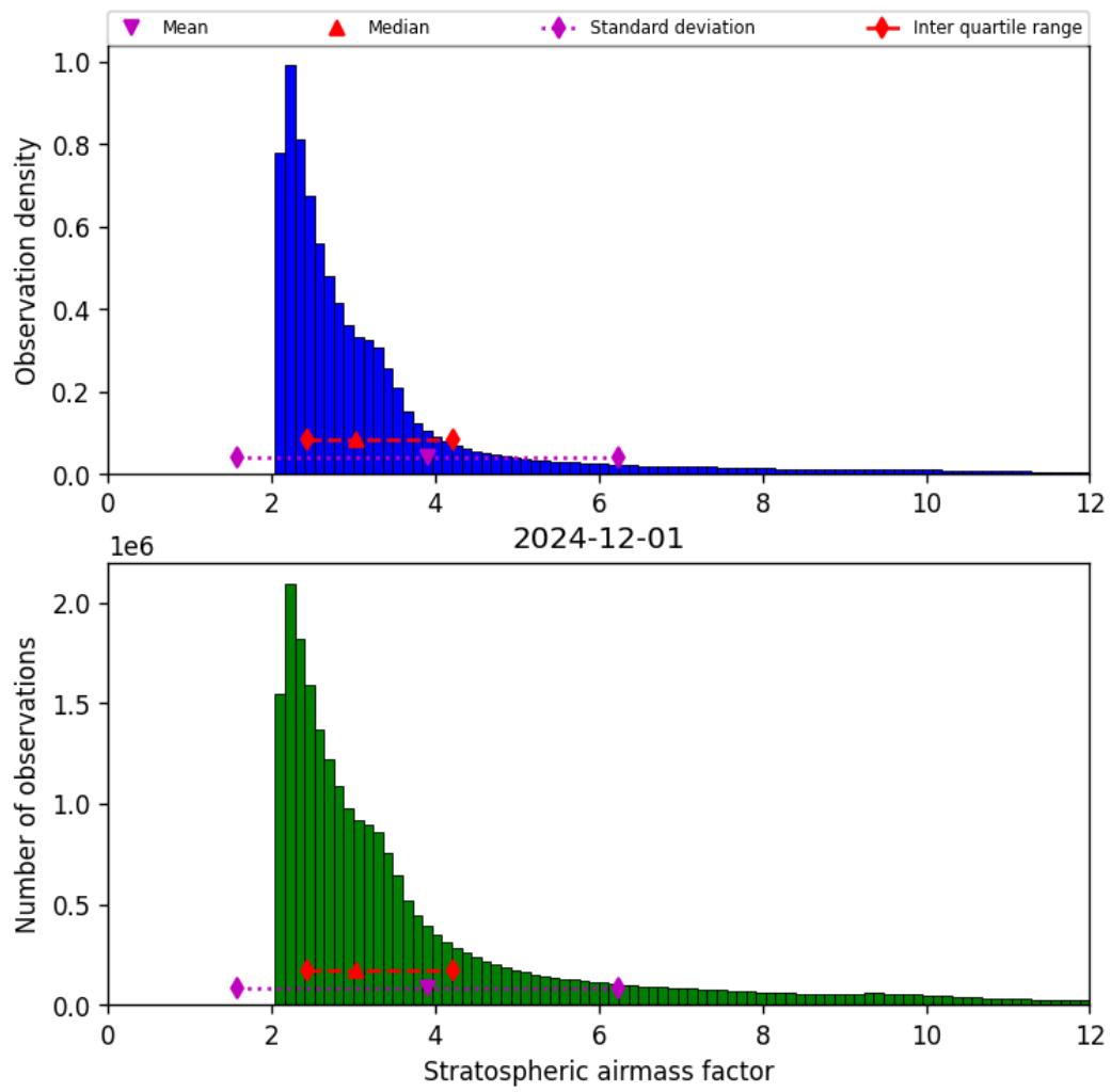
Figure 42: Histogram of “Stratospheric airmass factor” for 2024-12-01 to 2024-12-02
