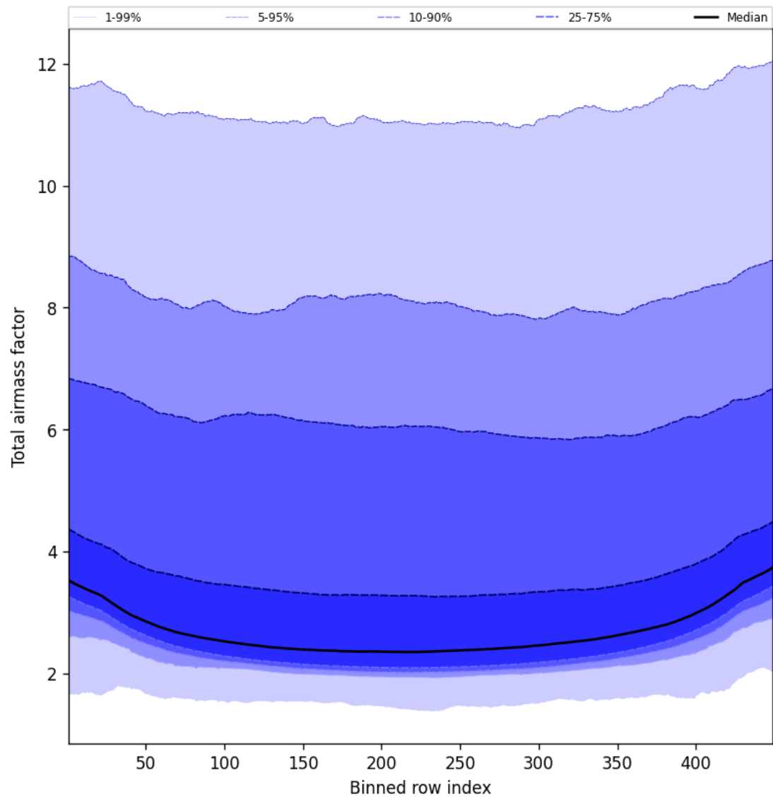
Figure 47: Along track statistics of “Total airmass factor” for 2024-12-01 to 2024-12-02
