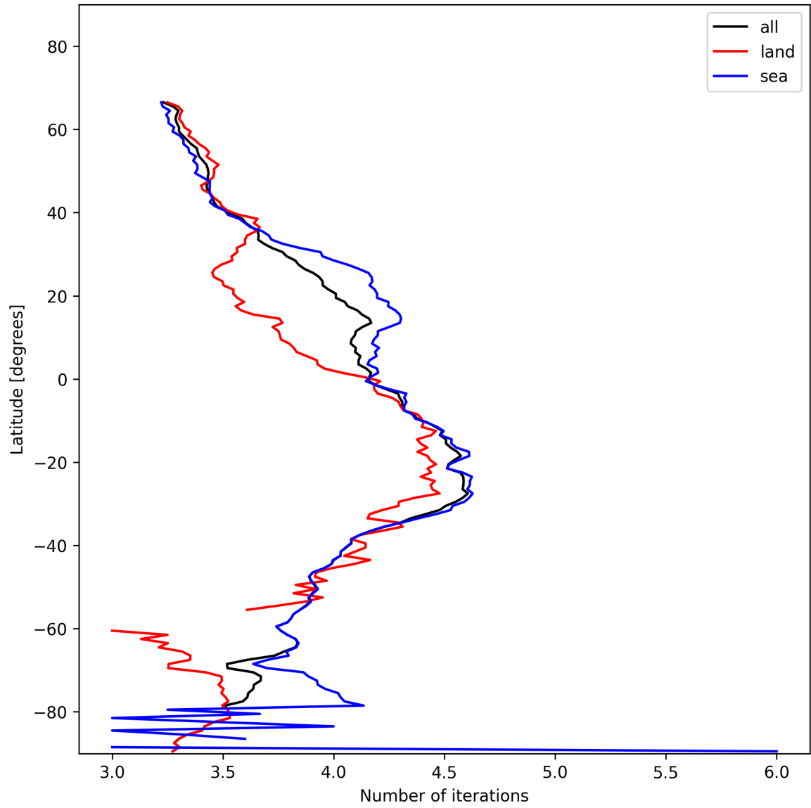
Figure 15: Zonal average of “Number of iterations” for 2024-12-01 to 2024-12-02.
