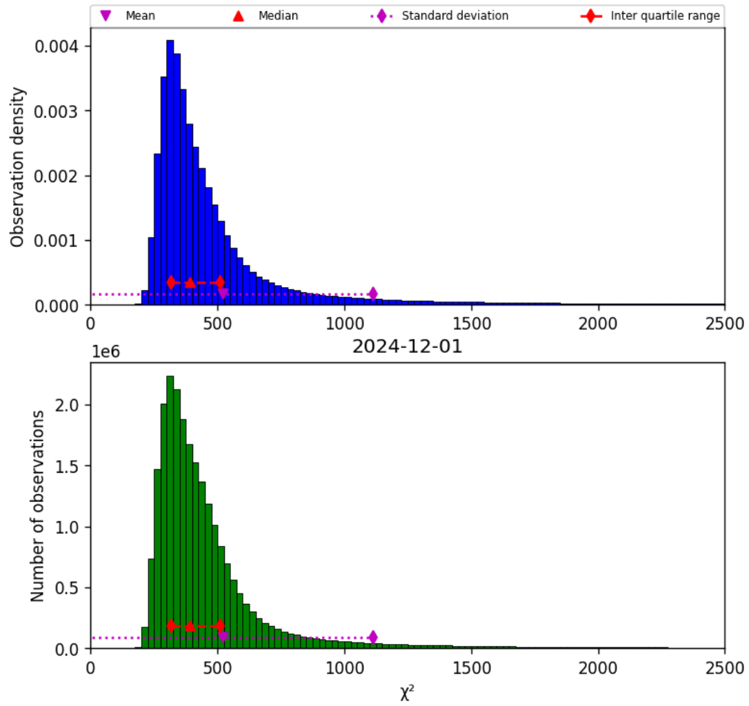
Figure 40: Histogram of “ \chi^2 ” for 2024-12-01 to 2024-12-02
