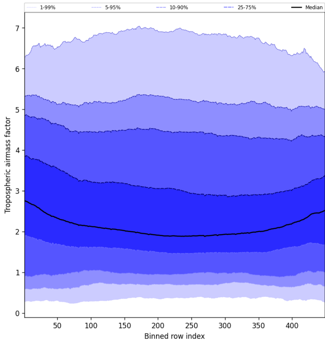
Figure 46: Along track statistics of “Tropospheric air mass factor” for 2024-12-01 to 2024-12-02
