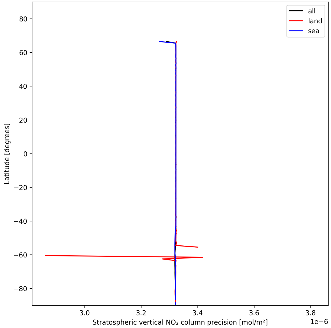
Figure 18: Zonal average of “Stratospheric vertical NO 2 column precision” for 2024-12-01 to 2024-12-02.
