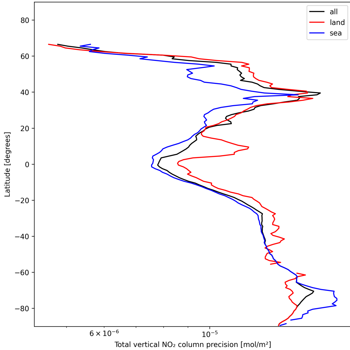
Figure 20: Zonal average of “Total vertical NO 2 column precision” for 2024-12-01 to 2024-12-02.
