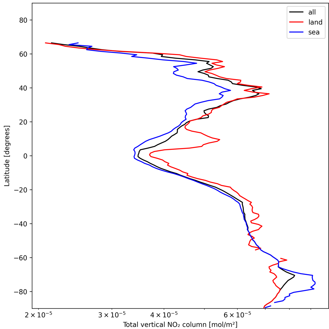
Figure 19: Zonal average of “Total vertical NO 2 column” for 2024-12-01 to 2024-12-02.
