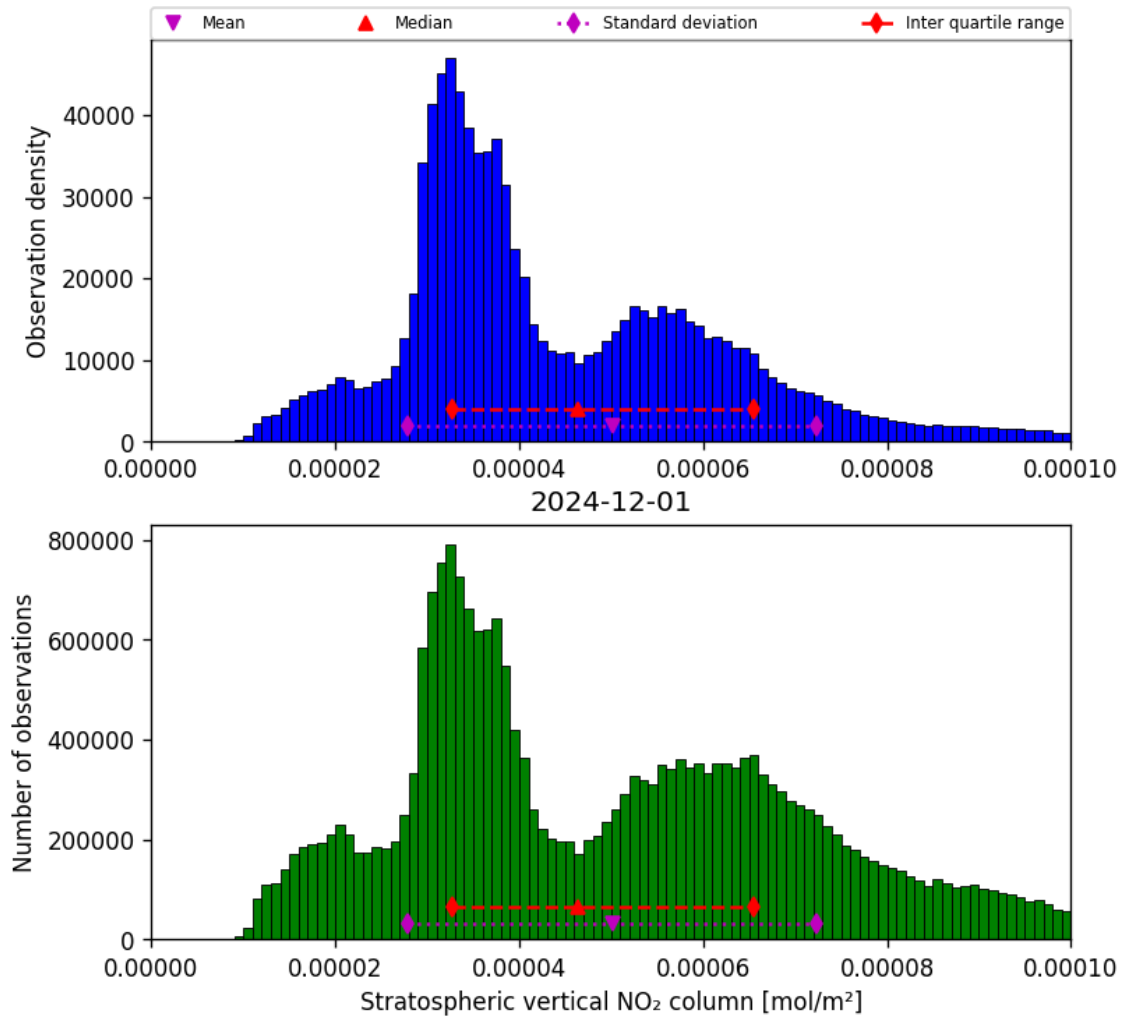
Figure 34: Histogram of “Stratospheric vertical NO 2 column” for 2024-12-01 to 2024-12-02
