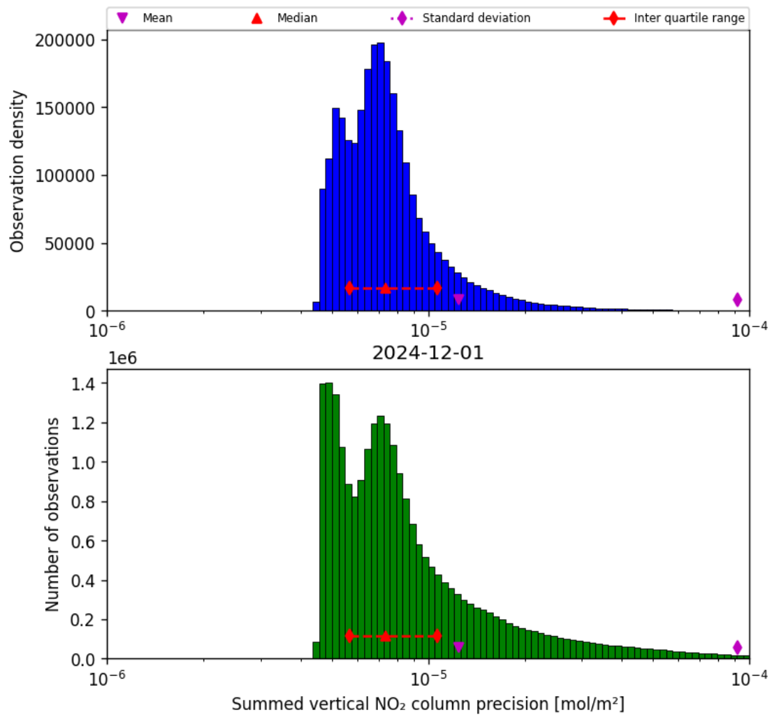
Figure 39: Histogram of “Summed vertical NO 2 column precision” for 2024-12-01 to 2024-12-02
