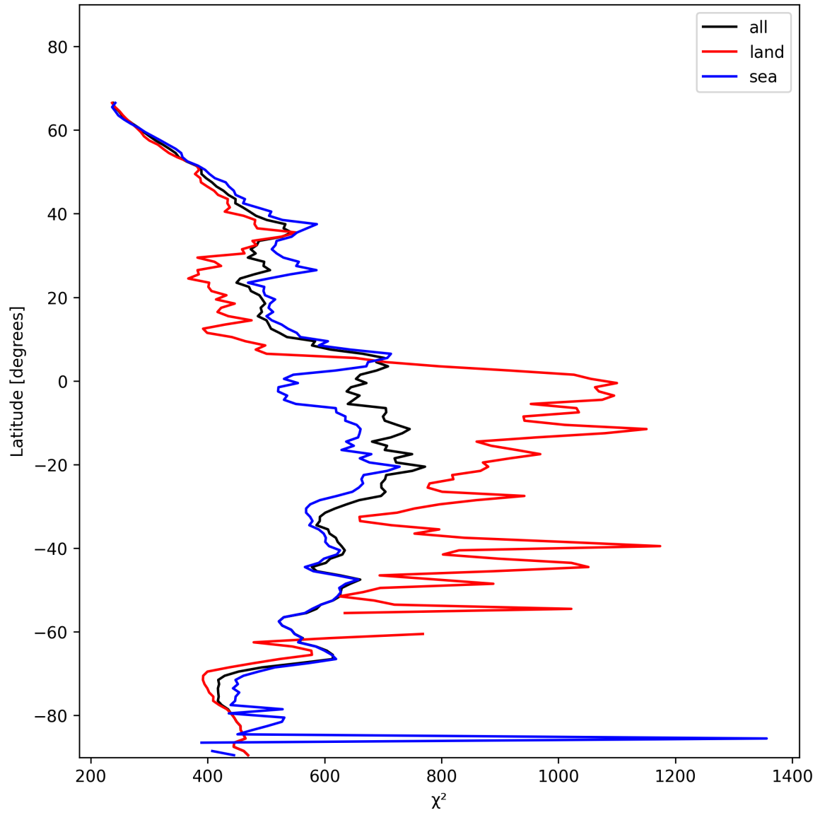
Figure 23: Zonal average of “ \chi^2 ” for 2024-12-01 to 2024-12-02.
