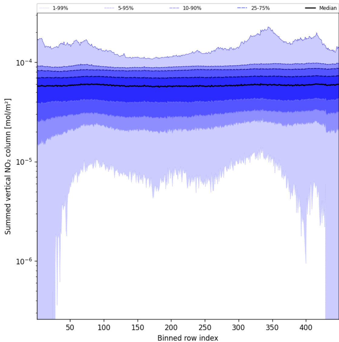
Figure 55: Along track statistics of “Summed vertical NO 2 column” for 2024-12-01 to 2024-12-02
