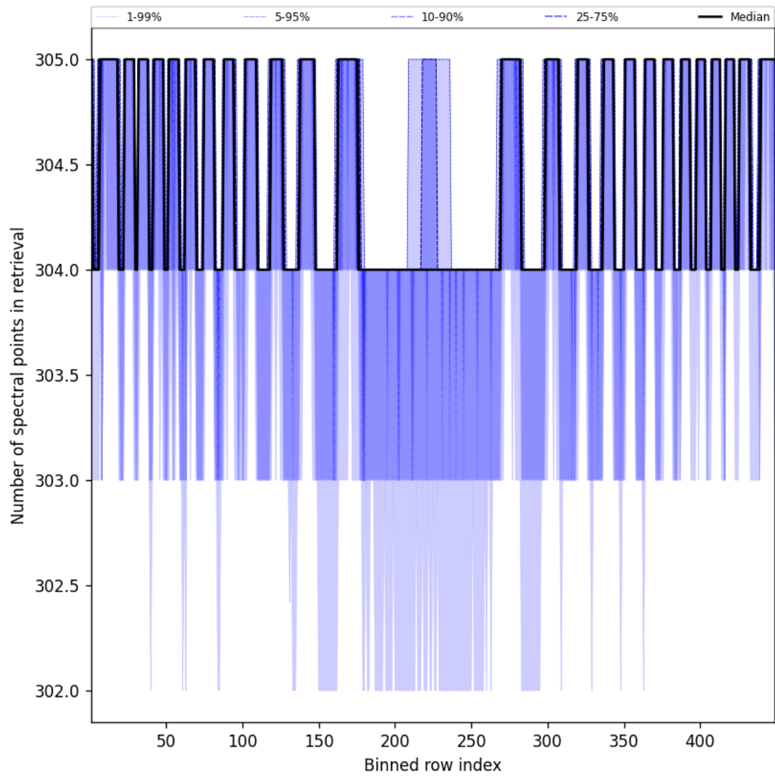
Figure 48: Along track statistics of “Number of spectral points in retrieval” for 2024-12-01 to 2024-12-02
