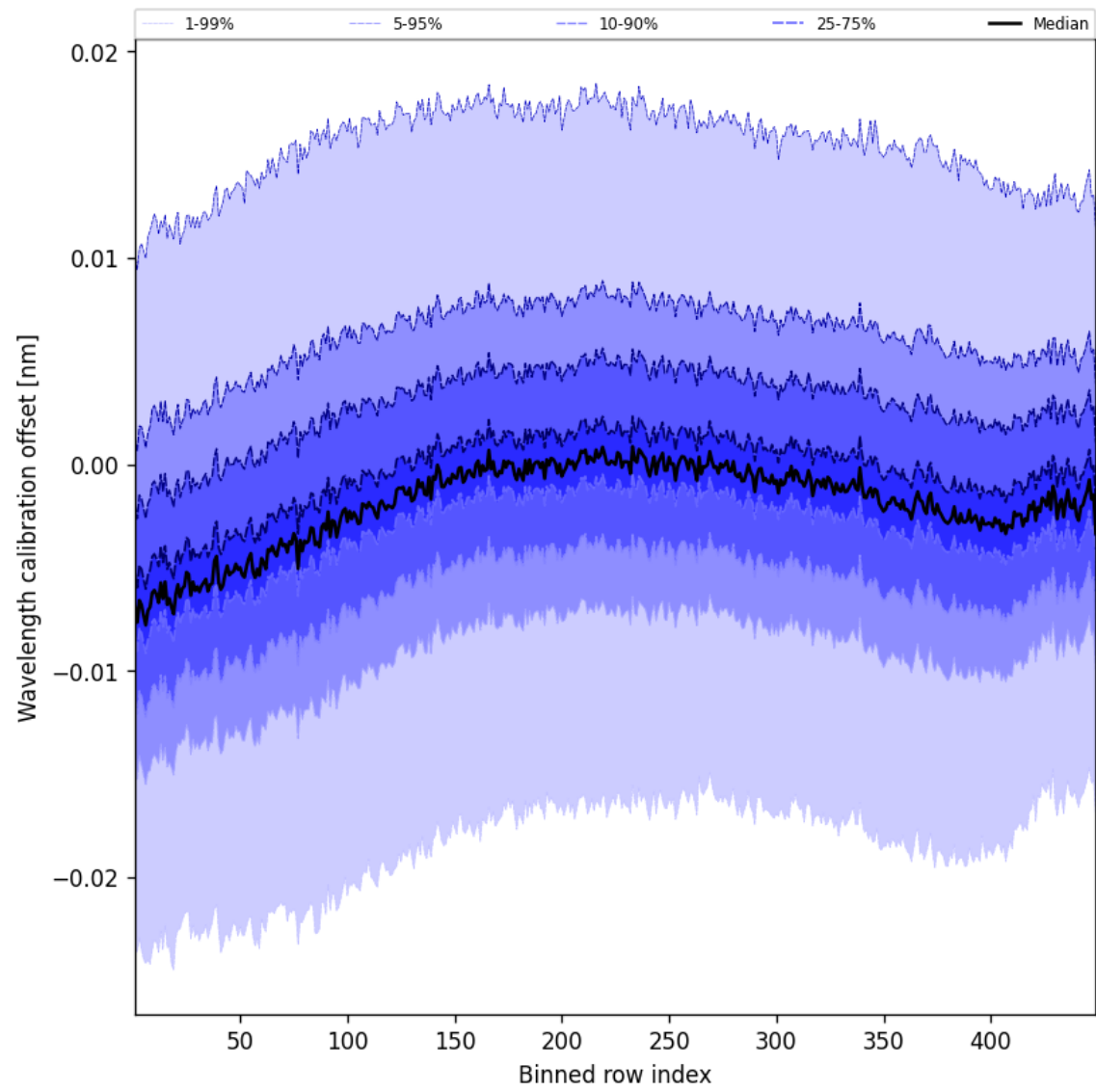
Figure 50: Along track statistics of “Wavelength calibration offset” for 2024-12-01 to 2024-12-02
