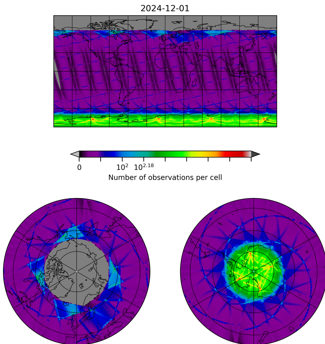
Figure 8: Map of the number of observations for 2024-12-01 to 2024-12-02
