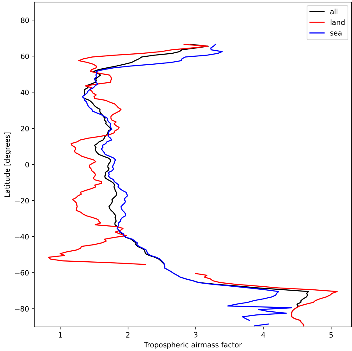
Figure 12: Zonal average of “Tropospheric airmass factor” for 2024-12-01 to 2024-12-02.
