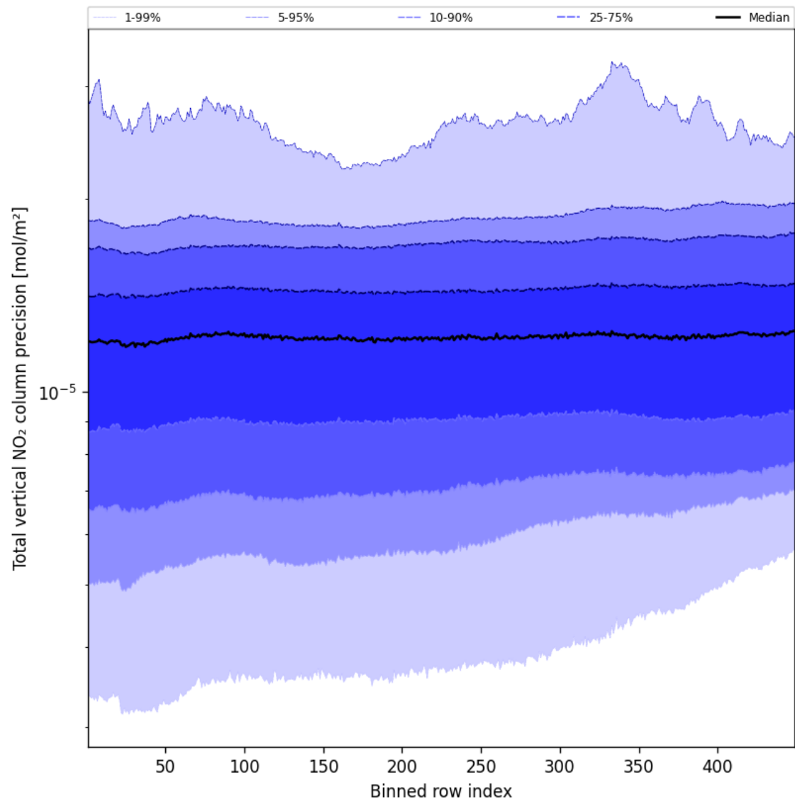
Figure 54: Along track statistics of “Total vertical NO 2 column precision” for 2024-12-01 to 2024-12-02
