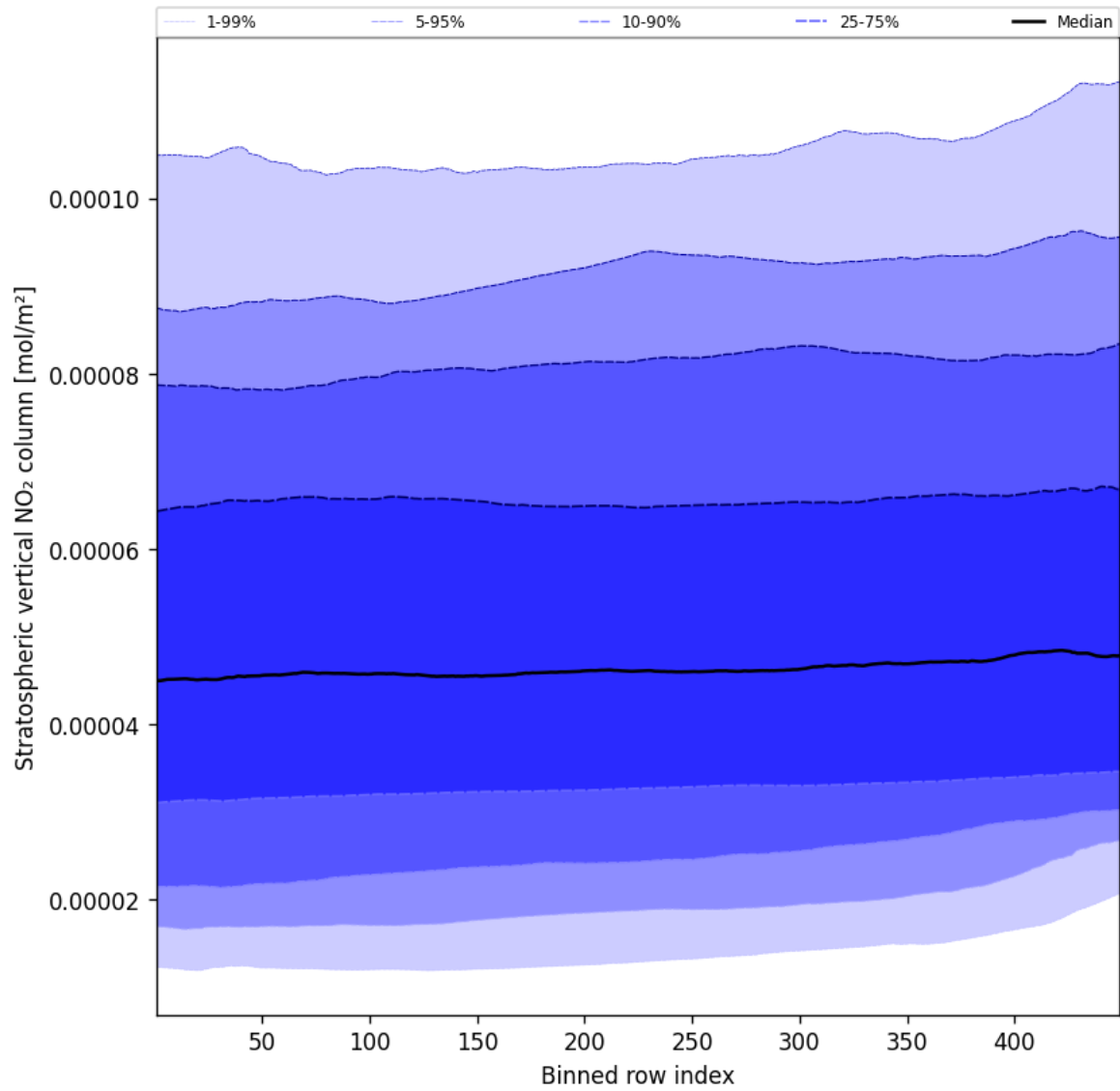
Figure 51: Along track statistics of “Stratospheric vertical NO 2 column” for 2024-12-01 to 2024-12-02
