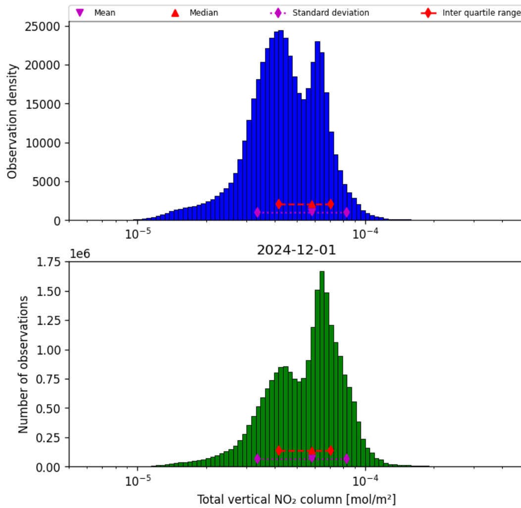
Figure 36: Histogram of “Total vertical NO 2 column” for 2024-12-01 to 2024-12-02
