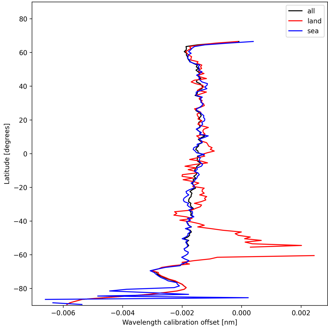
Figure 16: Zonal average of “Wavelength calibration offset” for 2024-12-01 to 2024-12-02.
