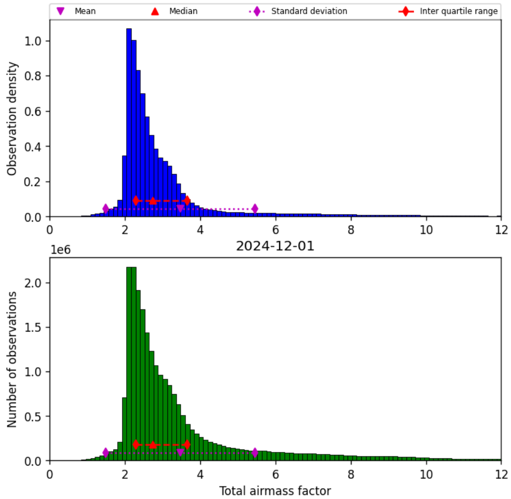
Figure 30: Histogram of “Total airmass factor” for 2024-12-01 to 2024-12-02
