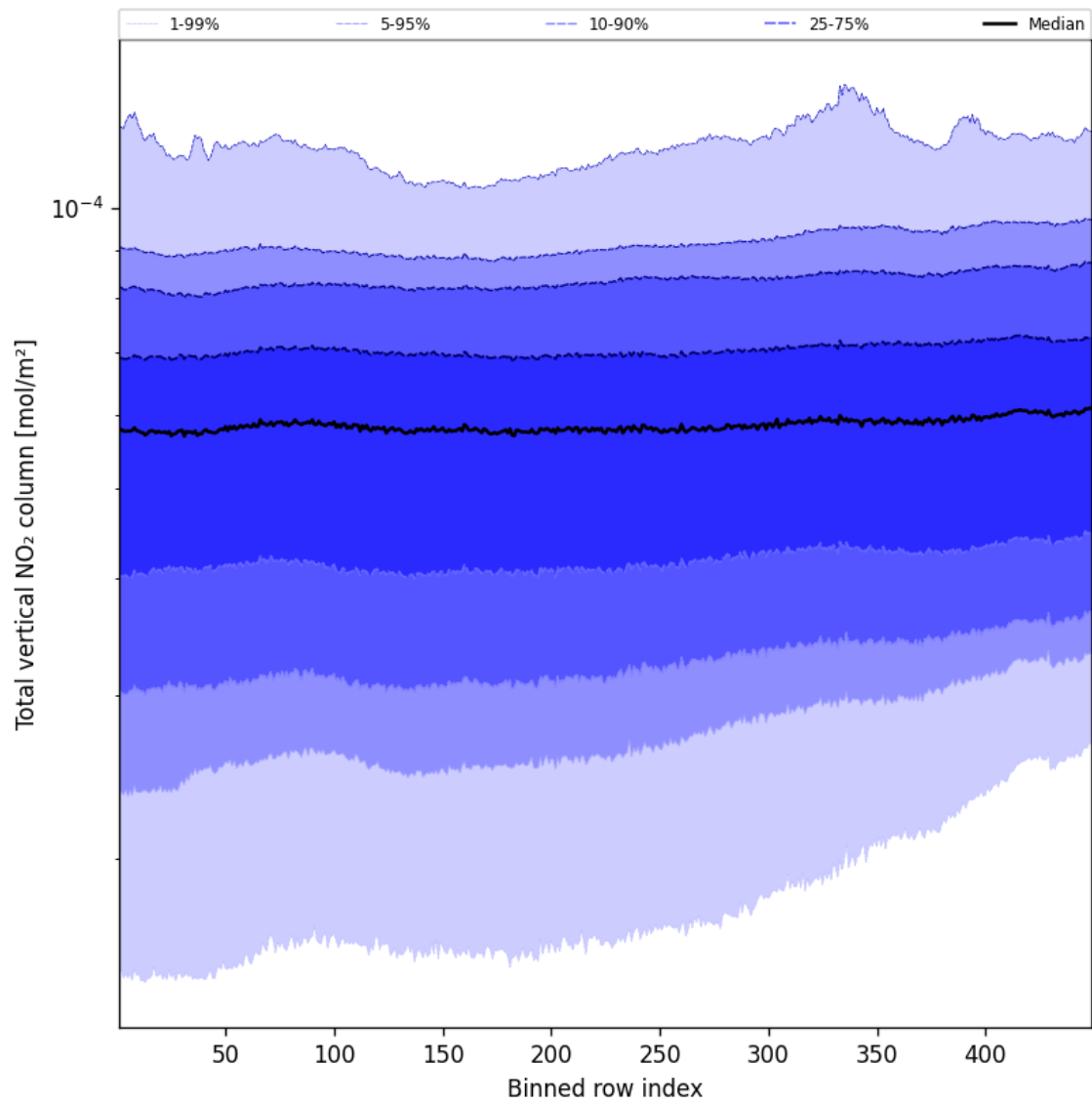
Figure 53: Along track statistics of “Total vertical NO 2 column” for 2024-12-01 to 2024-12-02
