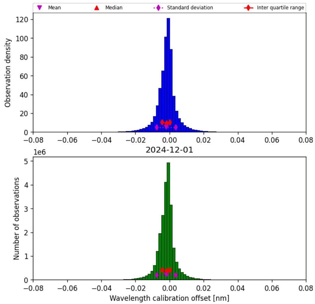
Figure 33: Histogram of “Wavelength calibration offset” for 2024-12-01 to 2024-12-02
