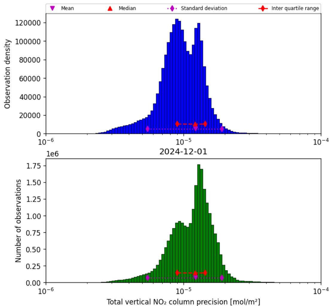
Figure 37: Histogram of “Total vertical NO 2 column precision” for 2024-12-01 to 2024-12-02
