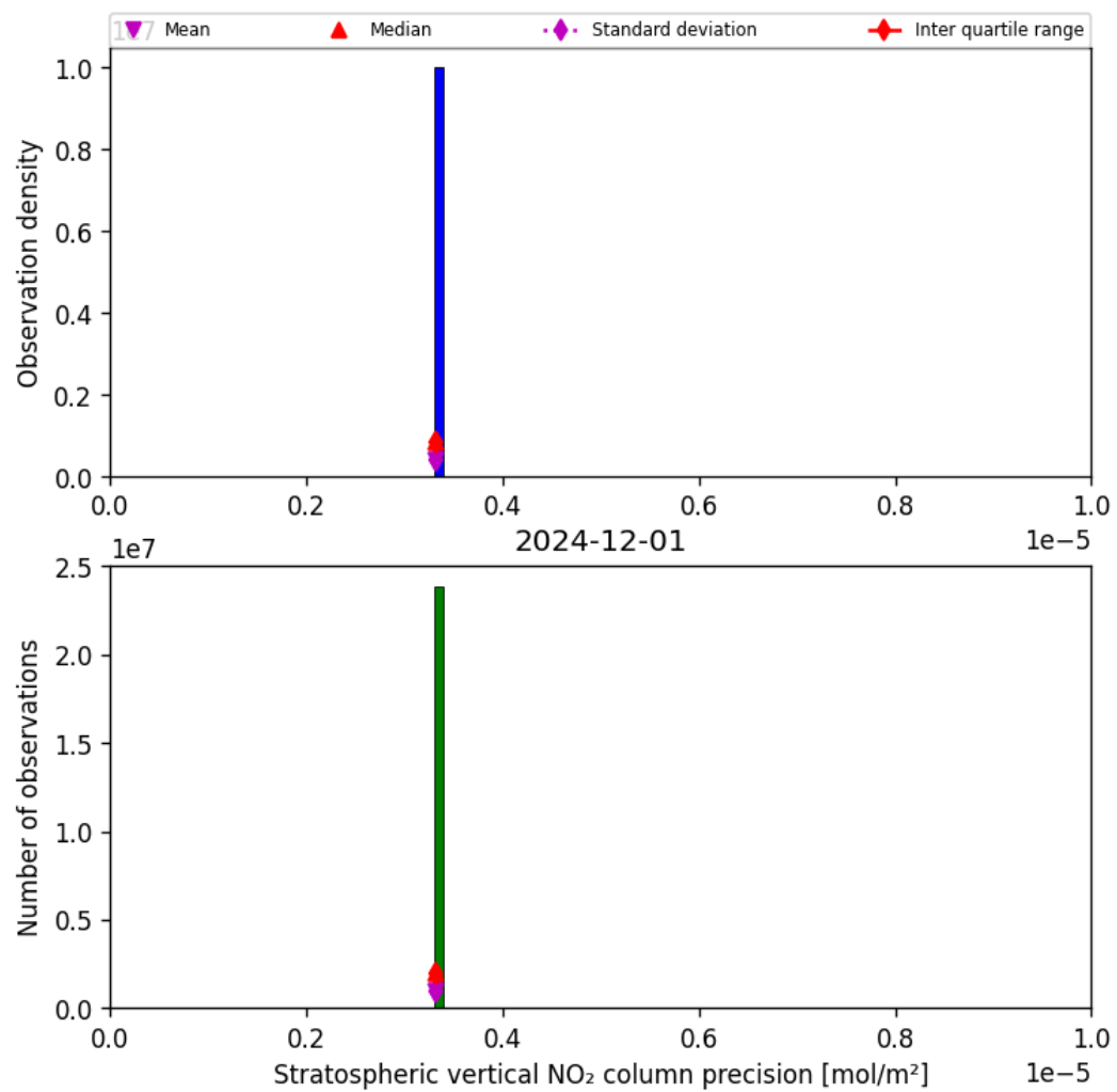
Figure 35: Histogram of “Stratospheric vertical NO 2 column precision” for 2024-12-01 to 2024-12-02
