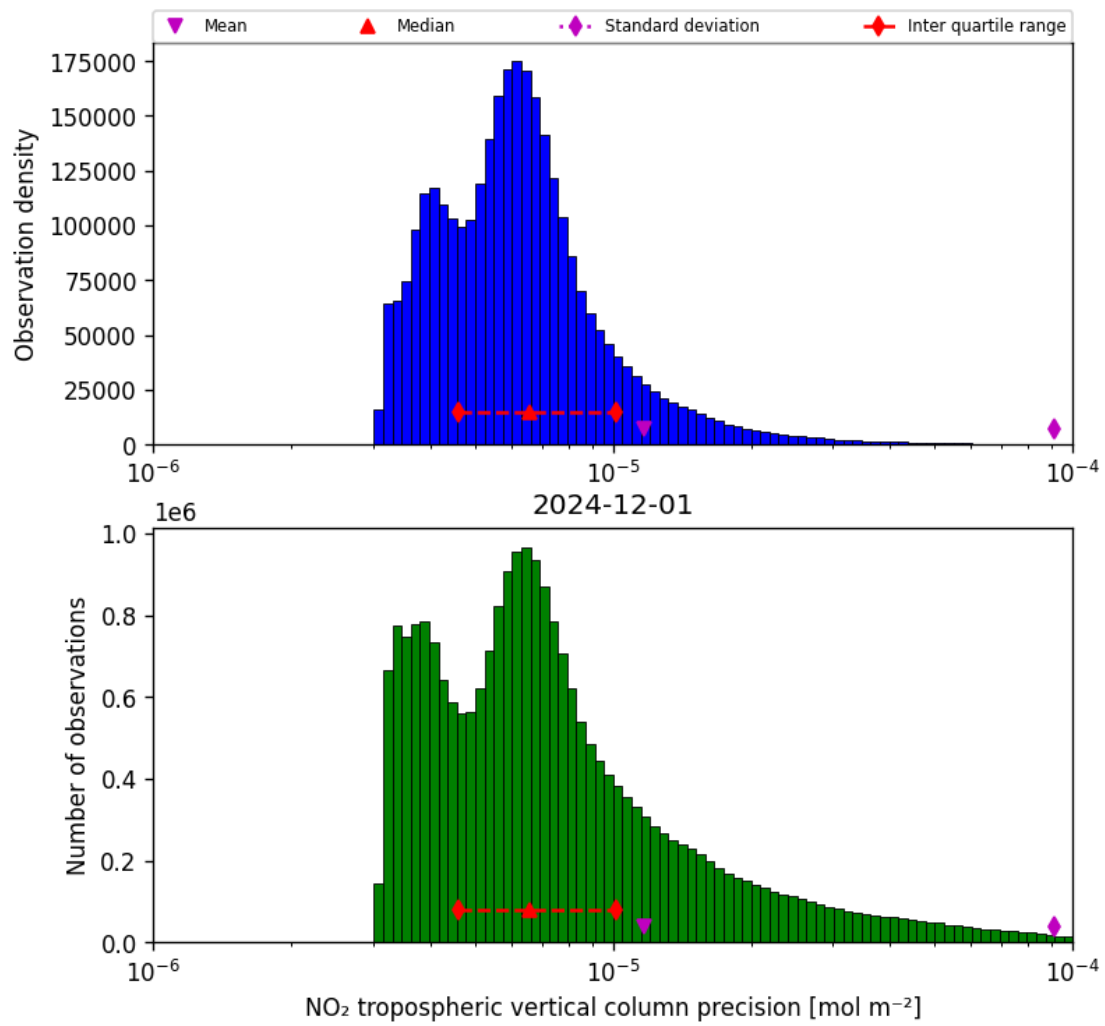
Figure 28: Histogram of “NO 2 tropospheric vertical column precision” for 2024-12-01 to 2024-12-02
