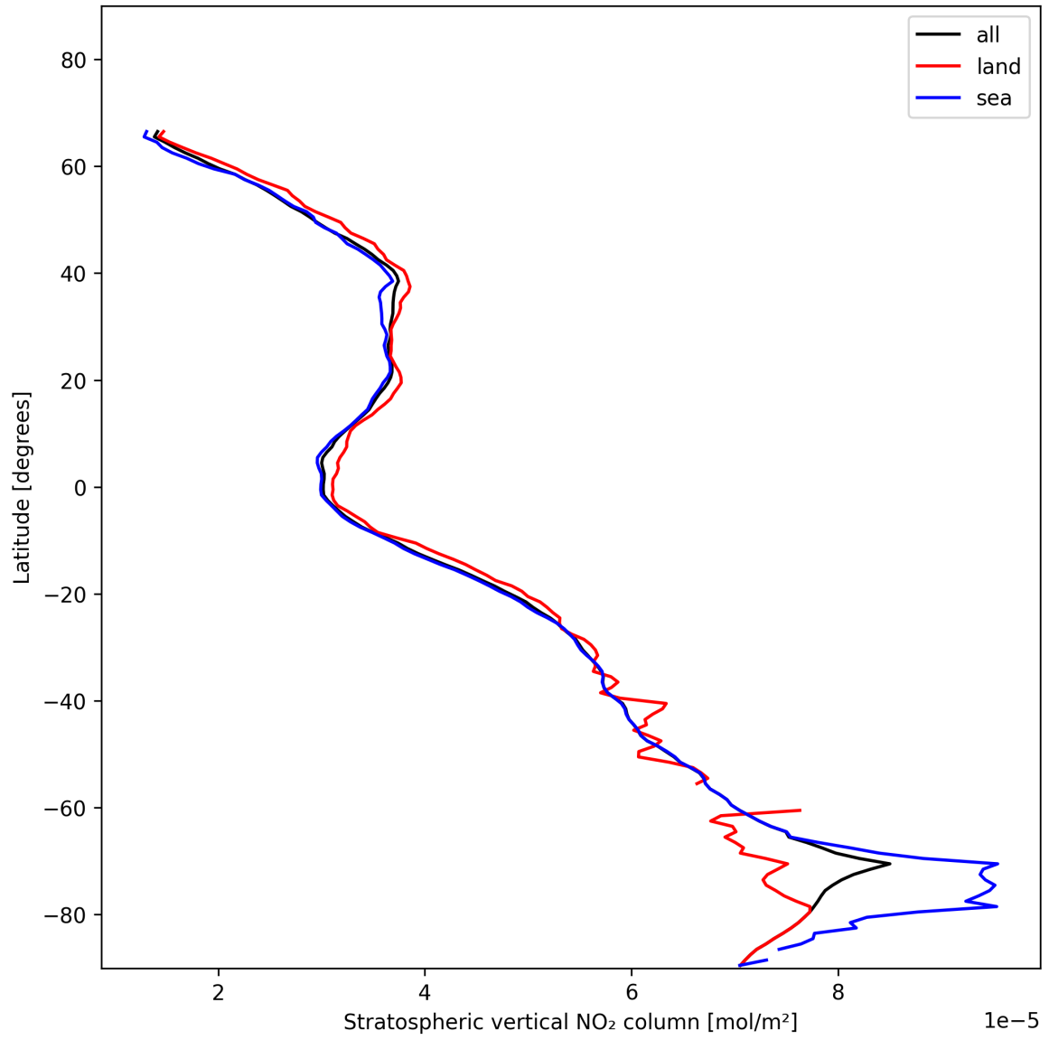
Figure 17: Zonal average of “Stratospheric vertical NO 2 column” for 2024-12-01 to 2024-12-02.
