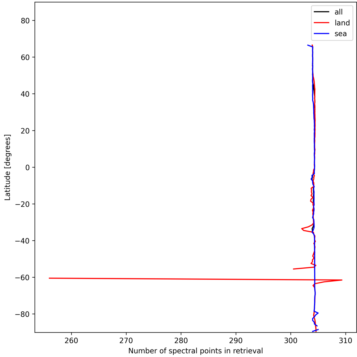
Figure 14: Zonal average of “Number of spectral points in retrieval” for 2024-12-01 to 2024-12-02.
