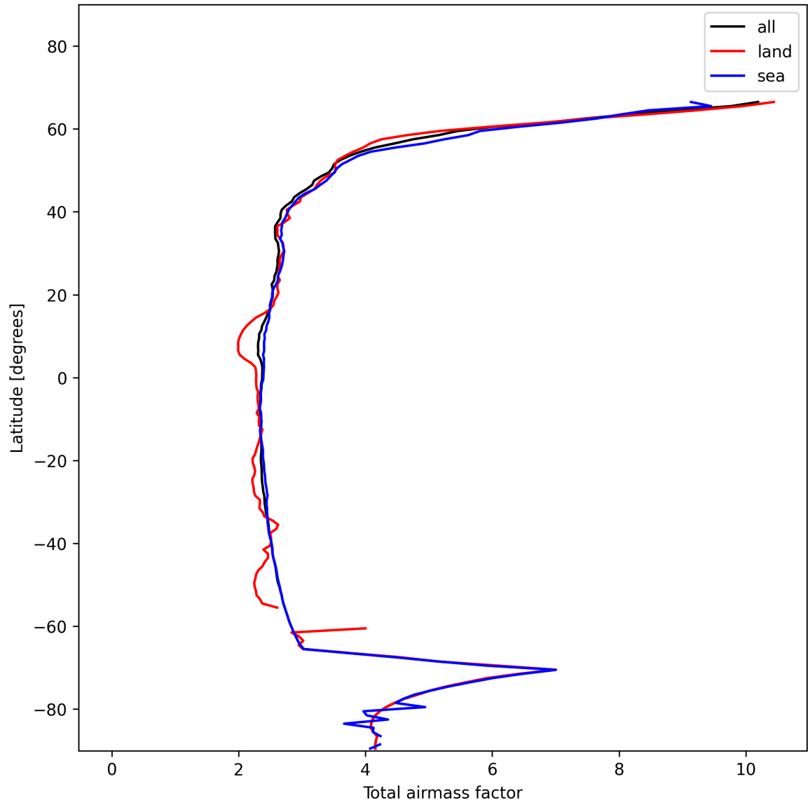
Figure 13: Zonal average of “Total airmass factor” for 2024-12-01 to 2024-12-02.
