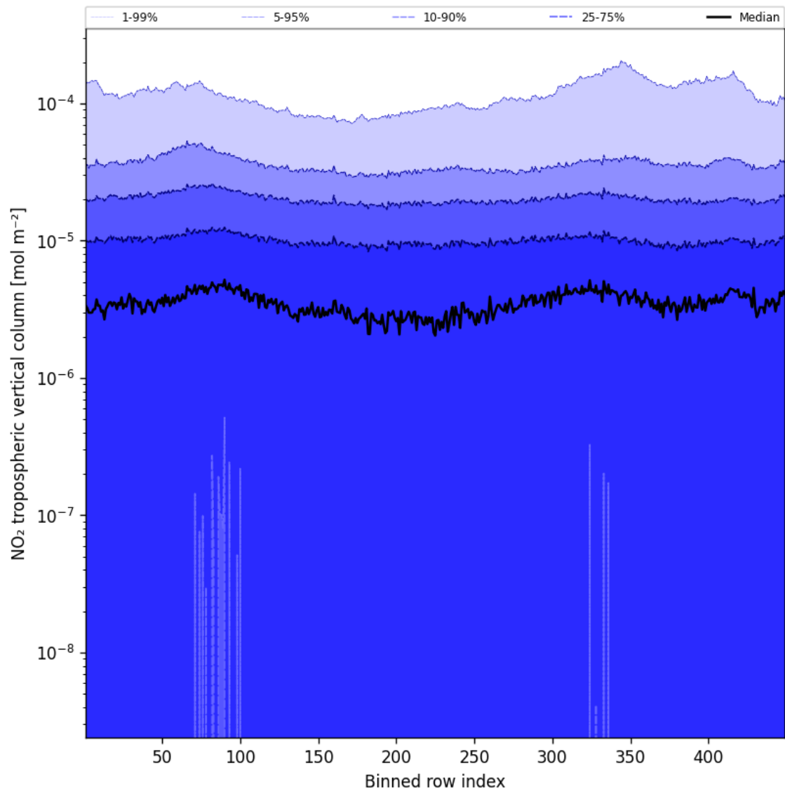
Figure 44: Along track statistics of “NO 2 tropospheric vertical column” for 2024-12-01 to 2024-12-02
