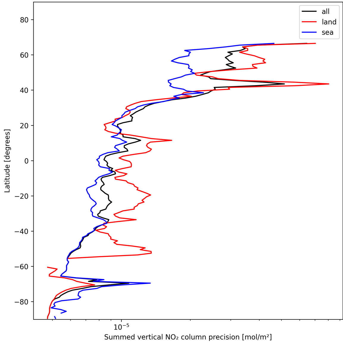
Figure 22: Zonal average of “Summed vertical NO 2 column precision” for 2024-12-01 to 2024-12-02.
