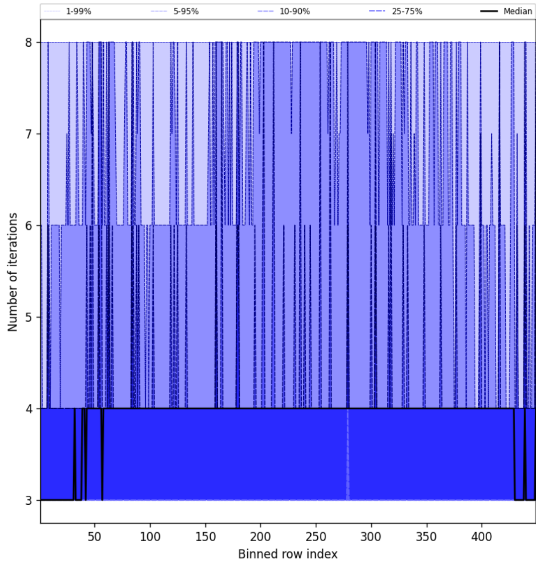
Figure 49: Along track statistics of “Number of iterations” for 2024-12-01 to 2024-12-02
