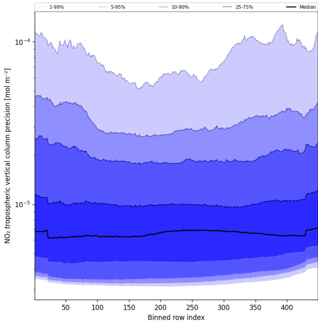
Figure 45: Along track statistics of “NO 2 tropospheric vertical column precision” for 2024-12-01 to 2024-12-02
