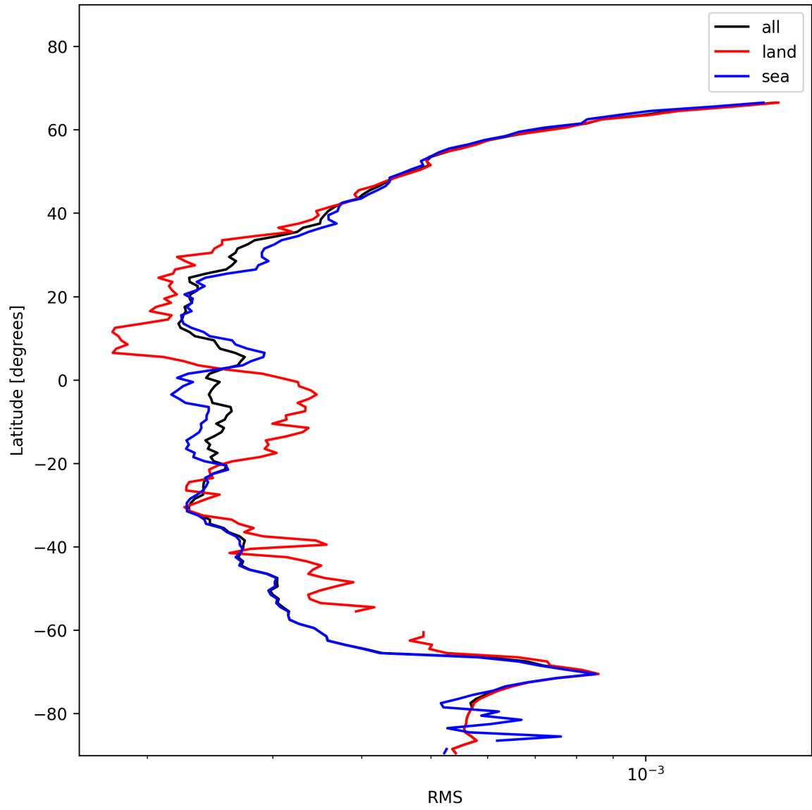
Figure 24: Zonal average of “RMS” for 2024-12-01 to 2024-12-02.
