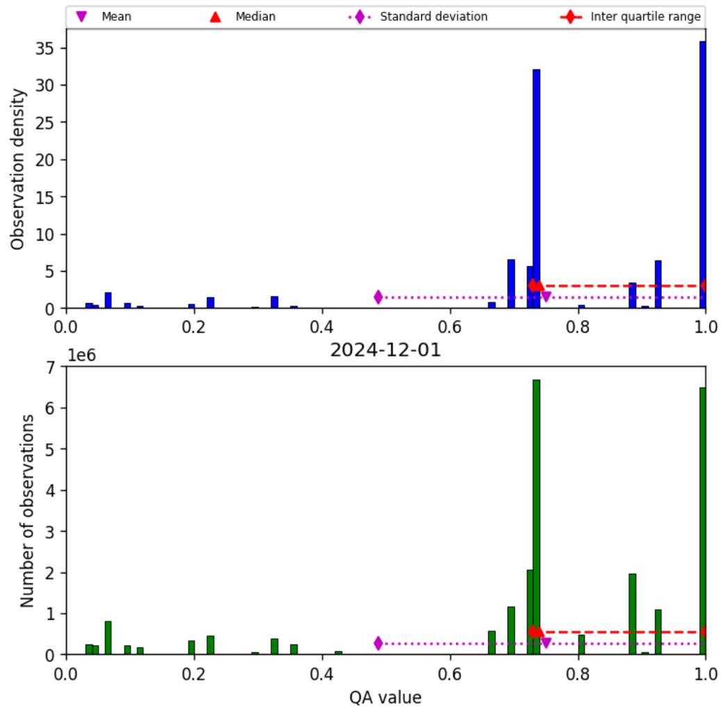
Figure 26: Histogram of “QA value” for 2024-12-01 to 2024-12-02
