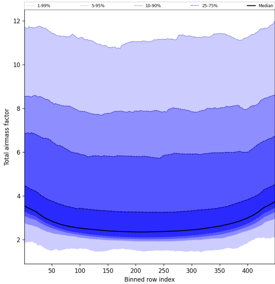
Figure 47: Along track statistics of “Total airmass factor” for 2024-12-02 to 2024-12-03
