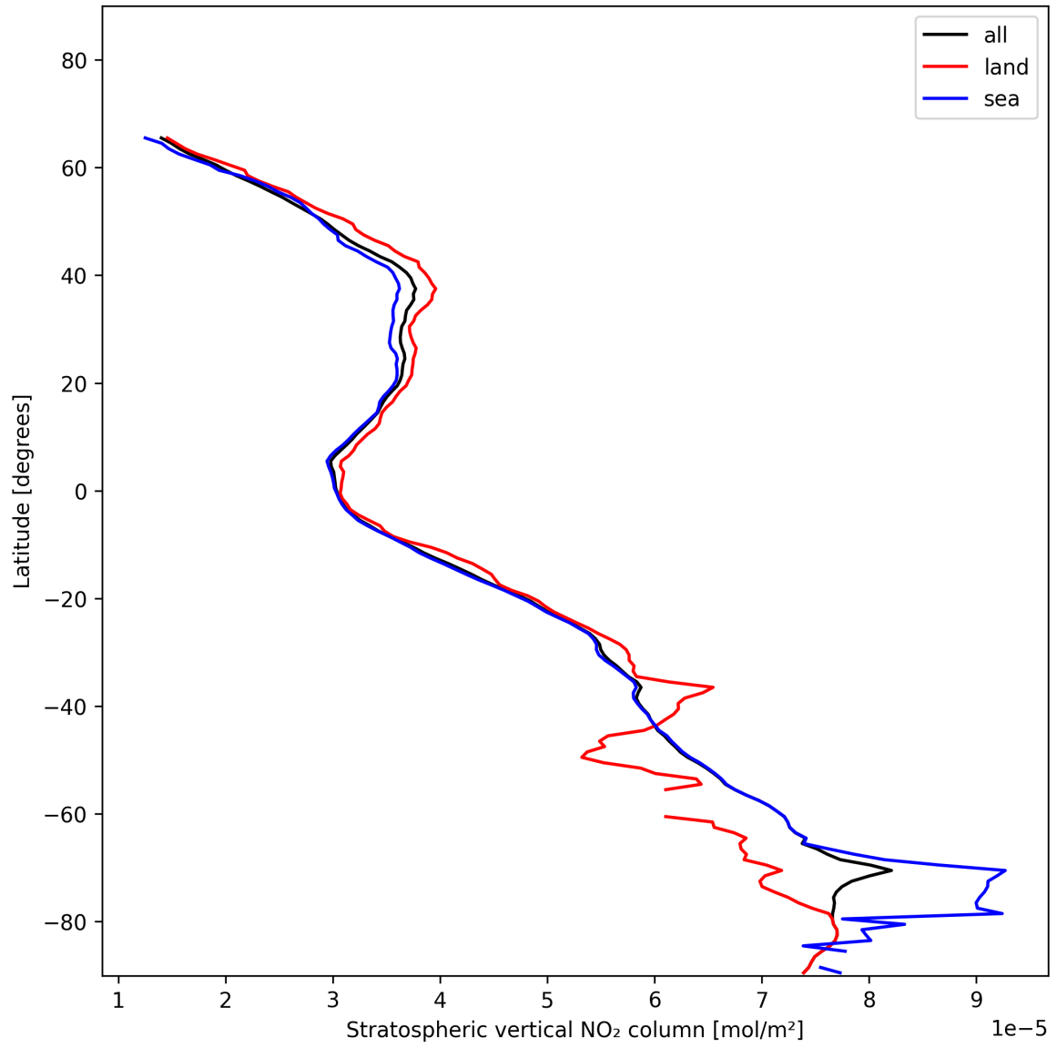
Figure 17: Zonal average of “Stratospheric vertical NO 2 column” for 2024-12-02 to 2024-12-03.
