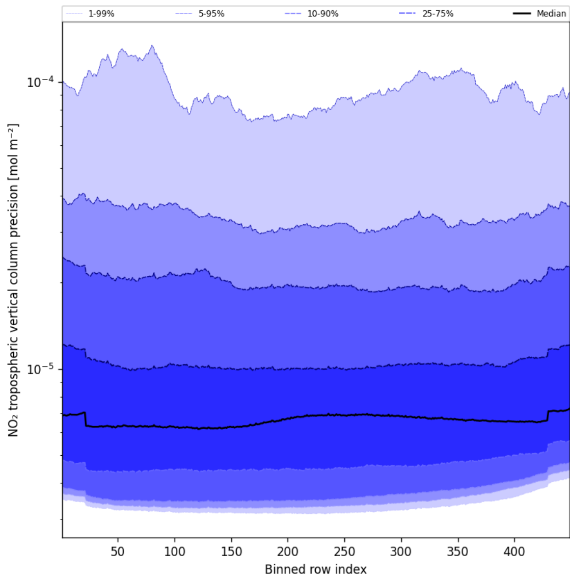
Figure 45: Along track statistics of “NO 2 tropospheric vertical column precision” for 2024-12-02 to 2024-12-03
