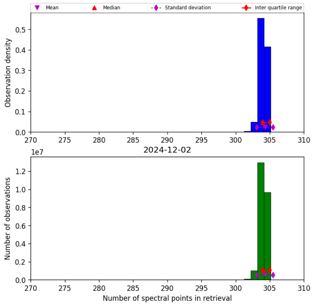
Figure 31: Histogram of “Number of spectral points in retrieval” for 2024-12-02 to 2024-12-03
