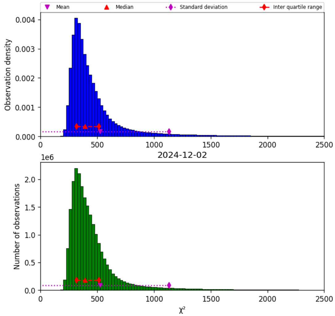
Figure 40: Histogram of “ \chi^2 ” for 2024-12-02 to 2024-12-03
