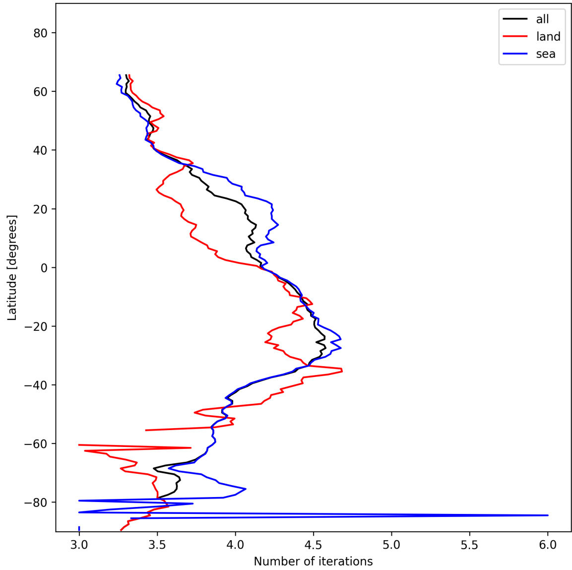
Figure 15: Zonal average of “Number of iterations” for 2024-12-02 to 2024-12-03.
