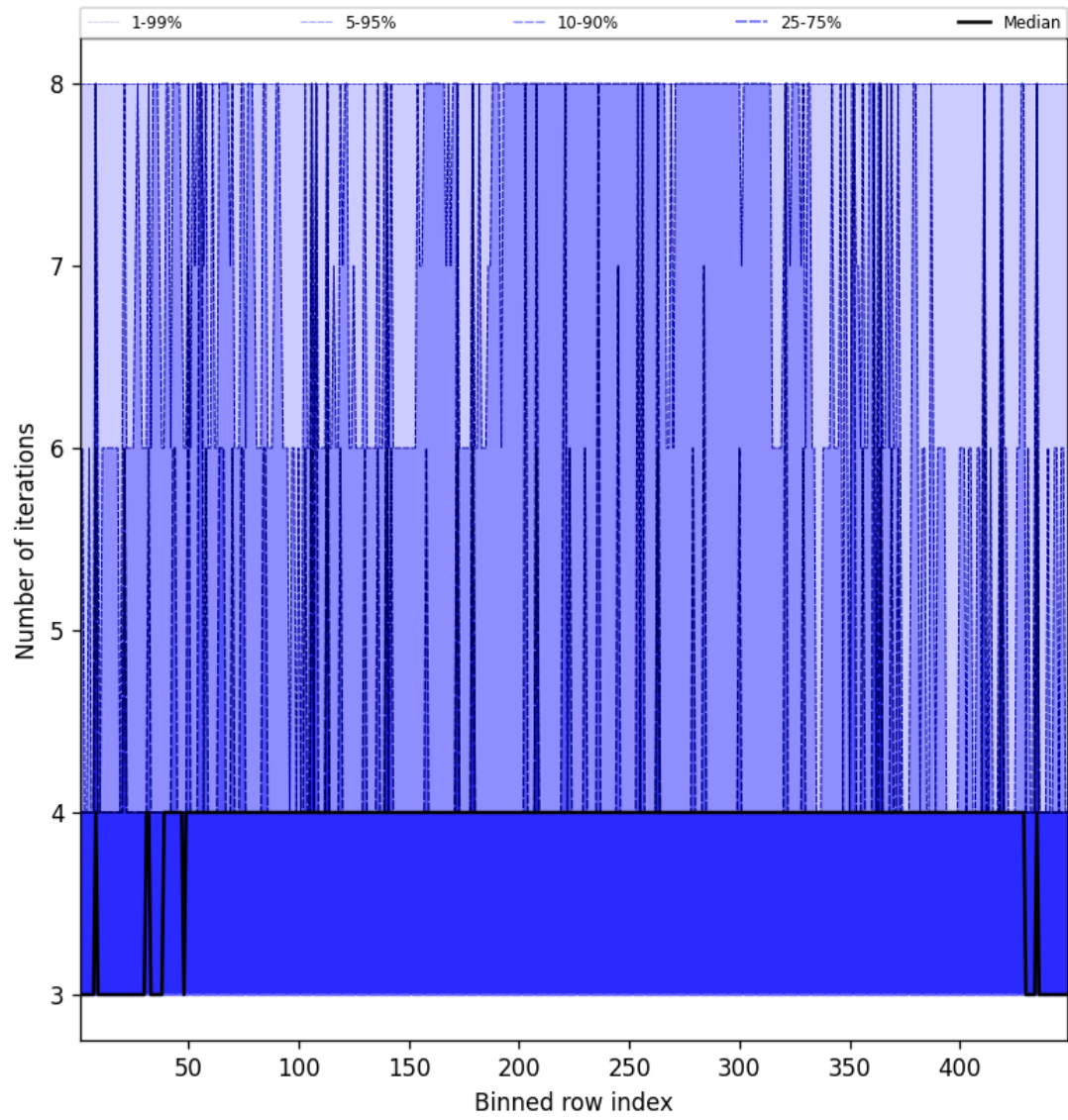
Figure 49: Along track statistics of “Number of iterations” for 2024-12-02 to 2024-12-03
