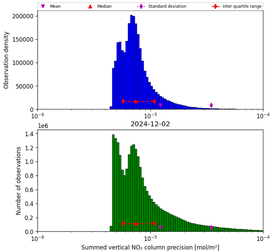
Figure 39: Histogram of “Summed vertical NO 2 column precision” for 2024-12-02 to 2024-12-03
