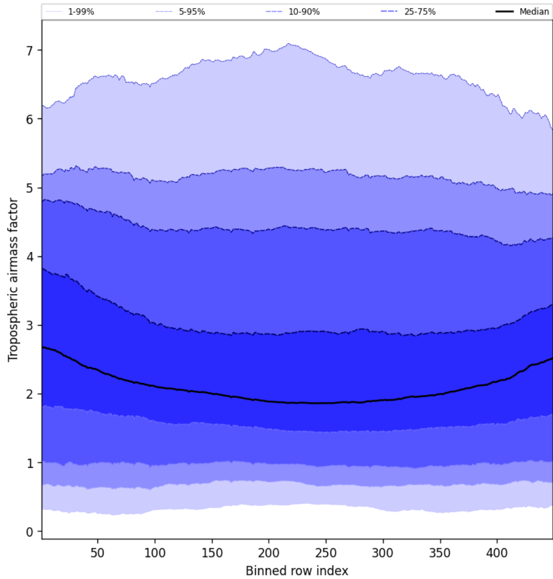
Figure 46: Along track statistics of “Tropospheric airmass factor” for 2024-12-02 to 2024-12-03
