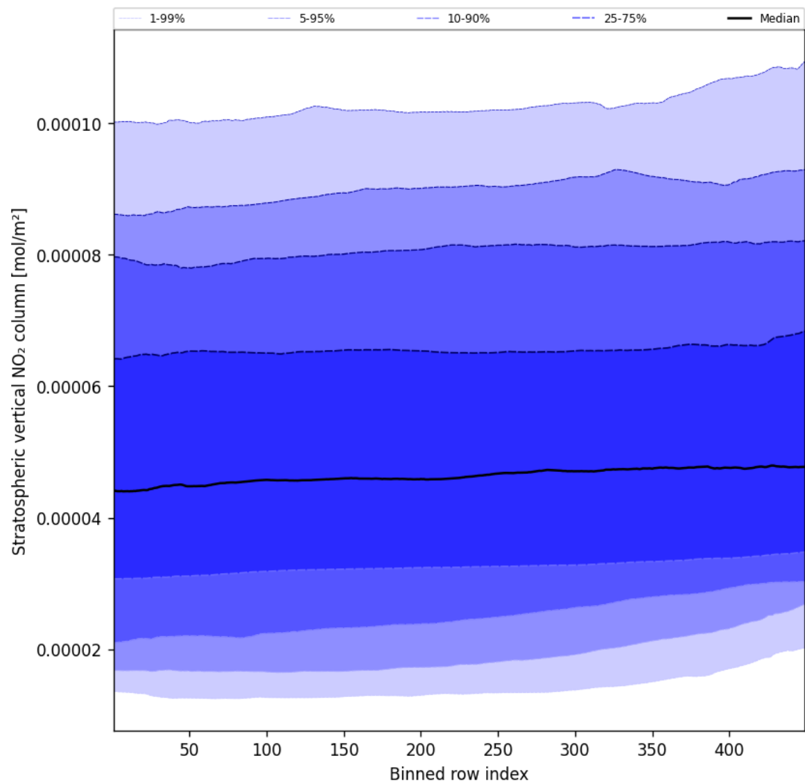
Figure 51: Along track statistics of “Stratospheric vertical NO 2 column” for 2024-12-02 to 2024-12-03
