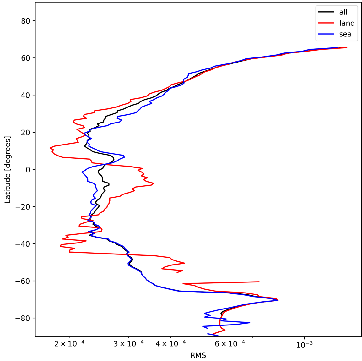
Figure 24: Zonal average of “RMS” for 2024-12-02 to 2024-12-03.
