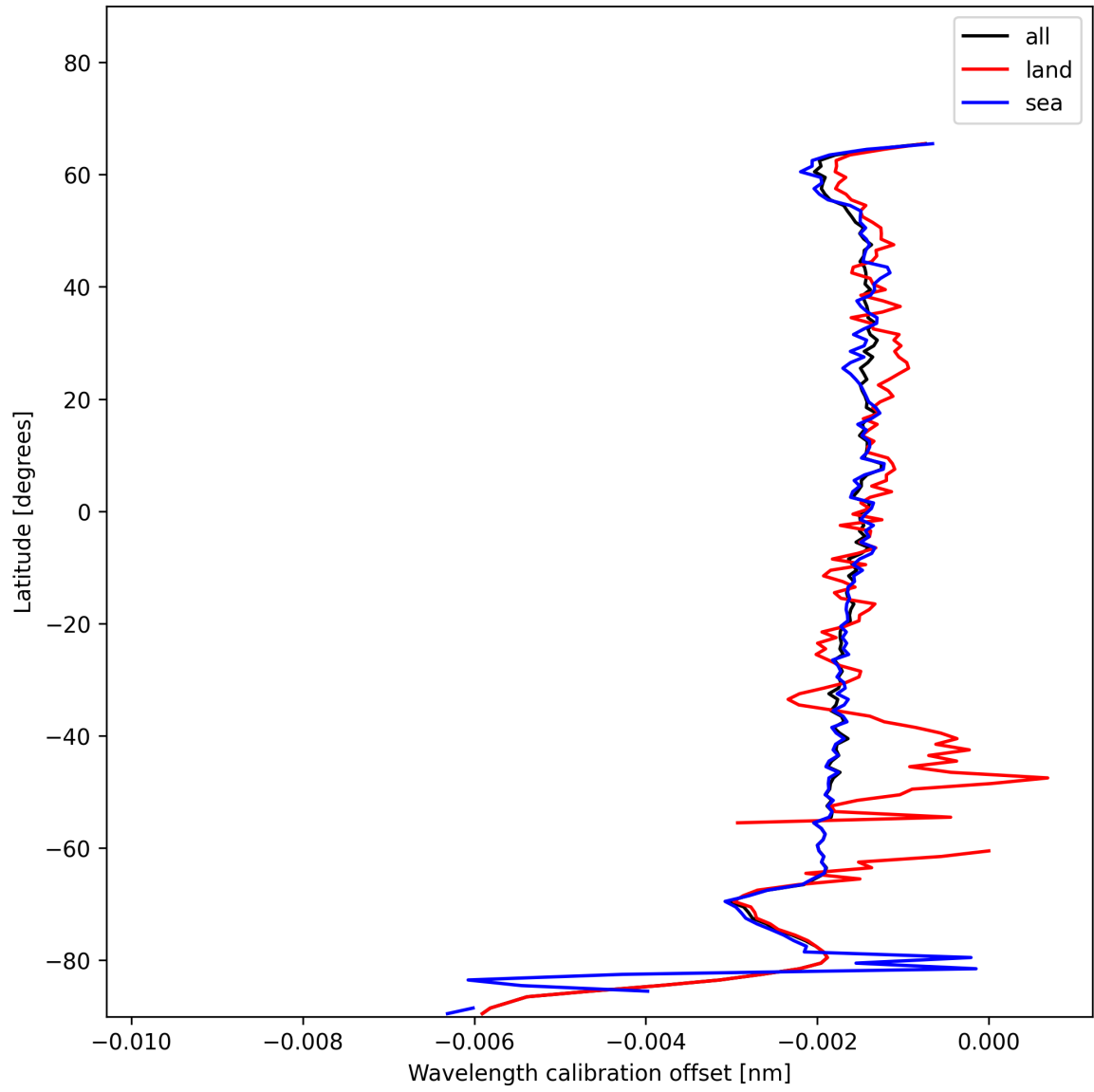
Figure 16: Zonal average of “Wavelength calibration offset” for 2024-12-02 to 2024-12-03.
