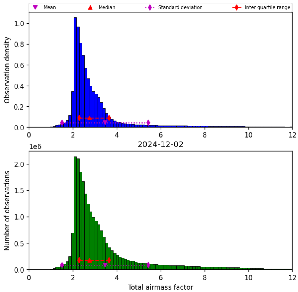
Figure 30: Histogram of “Total airmass factor” for 2024-12-02 to 2024-12-03
