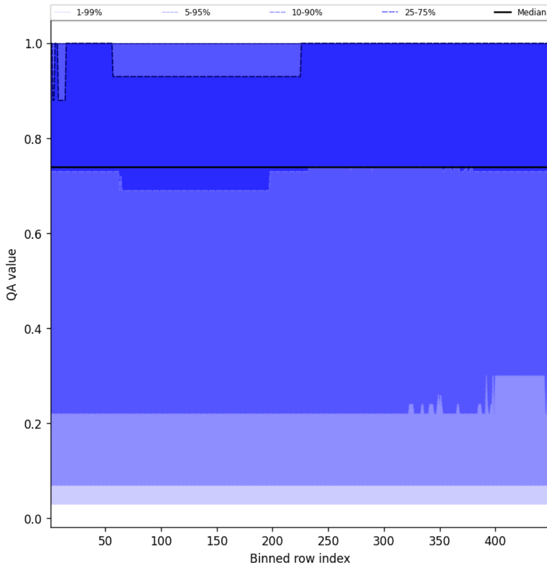
Figure 43: Along track statistics of “QA value” for 2024-12-02 to 2024-12-03
