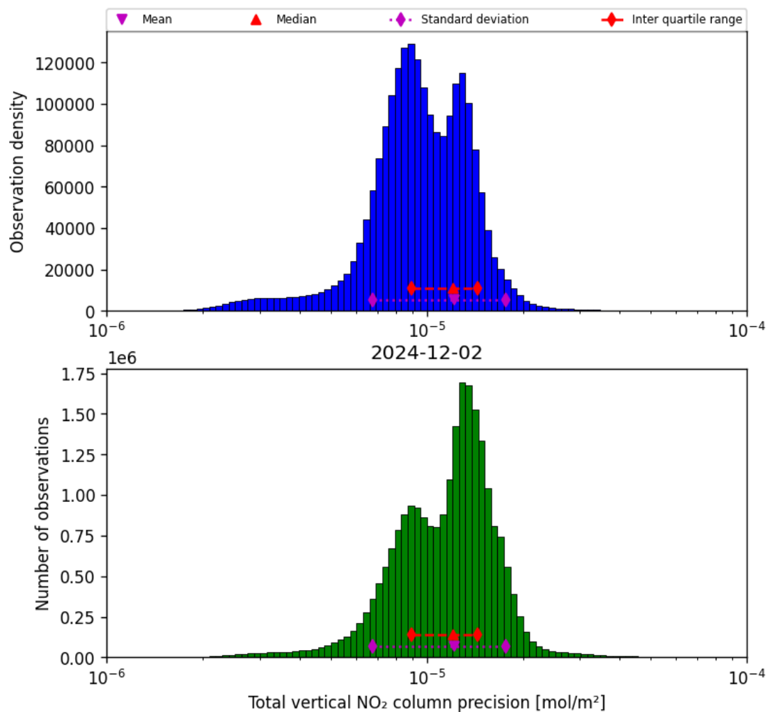
Figure 37: Histogram of “Total vertical NO 2 column precision” for 2024-12-02 to 2024-12-03
