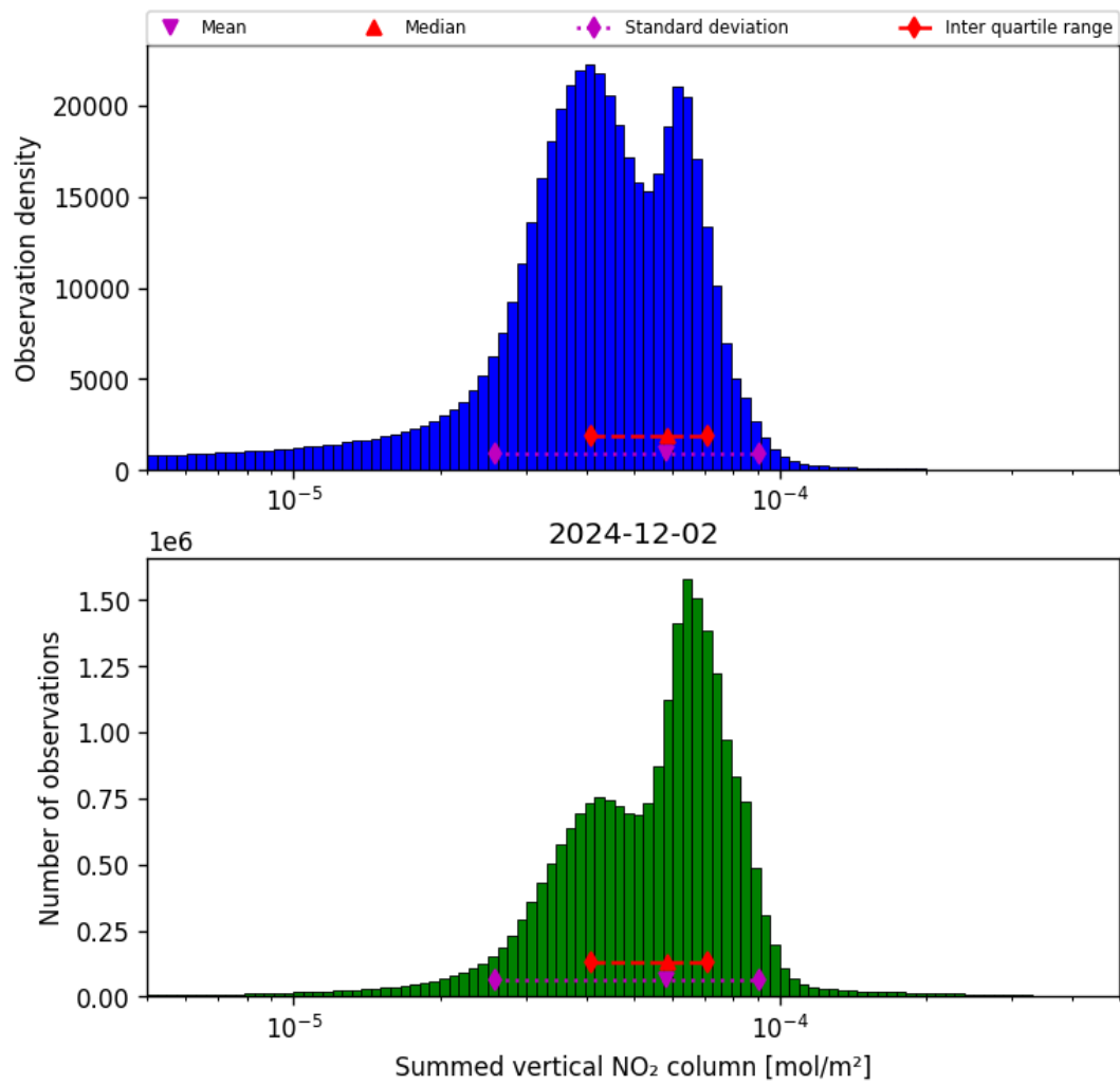
Figure 38: Histogram of “Summed vertical NO 2 column” for 2024-12-02 to 2024-12-03
