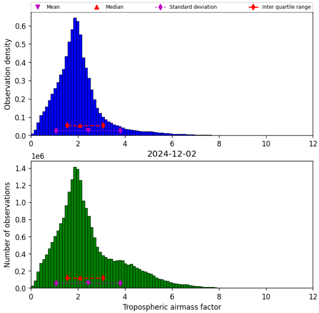
Figure 29: Histogram of “Tropospheric airmass factor” for 2024-12-02 to 2024-12-03
