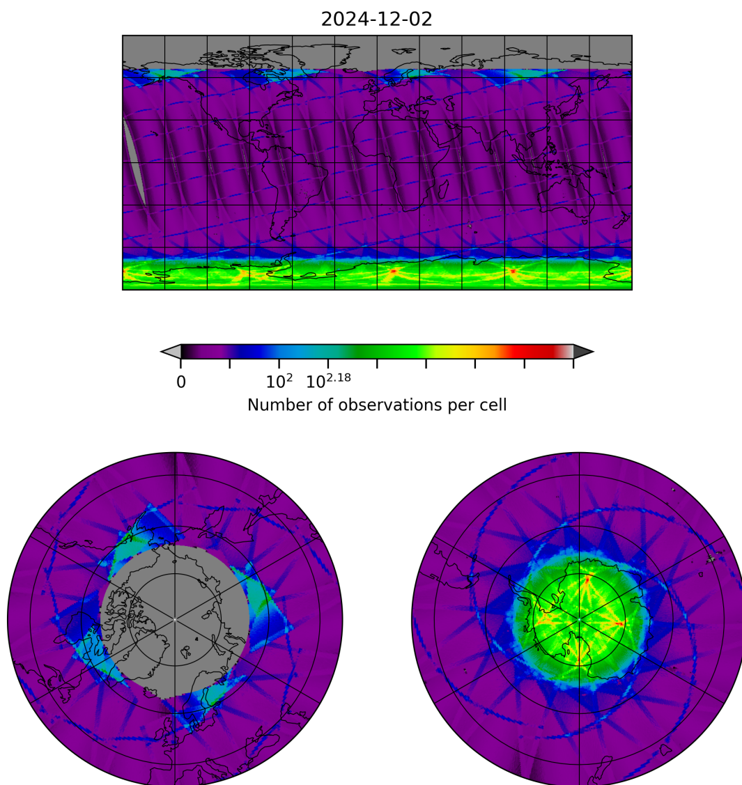
Figure 8: Map of the number of observations for 2024-12-02 to 2024-12-03
