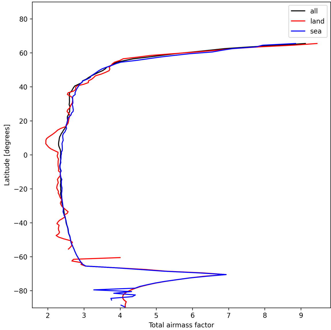
Figure 13: Zonal average of “Total airmass factor” for 2024-12-02 to 2024-12-03.
