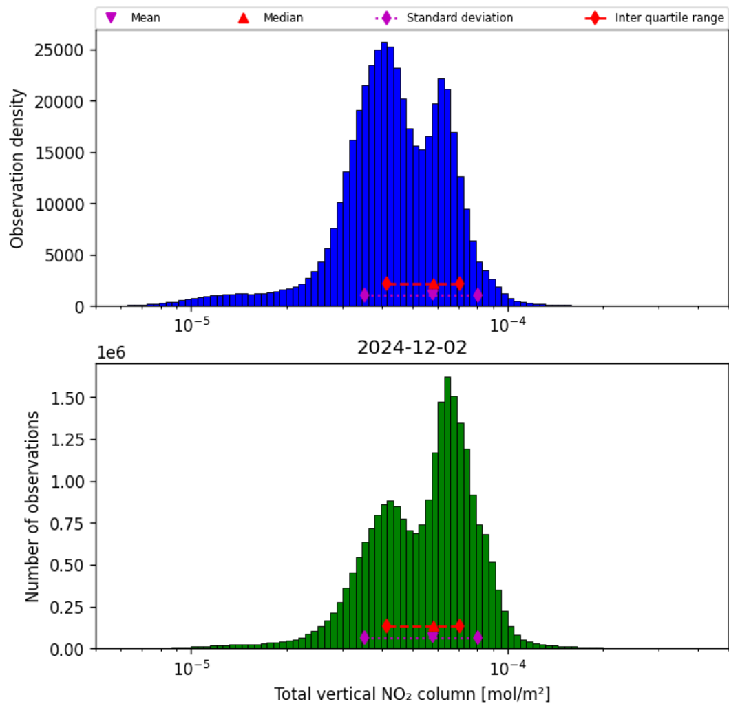
Figure 36: Histogram of “Total vertical NO 2 column” for 2024-12-02 to 2024-12-03
