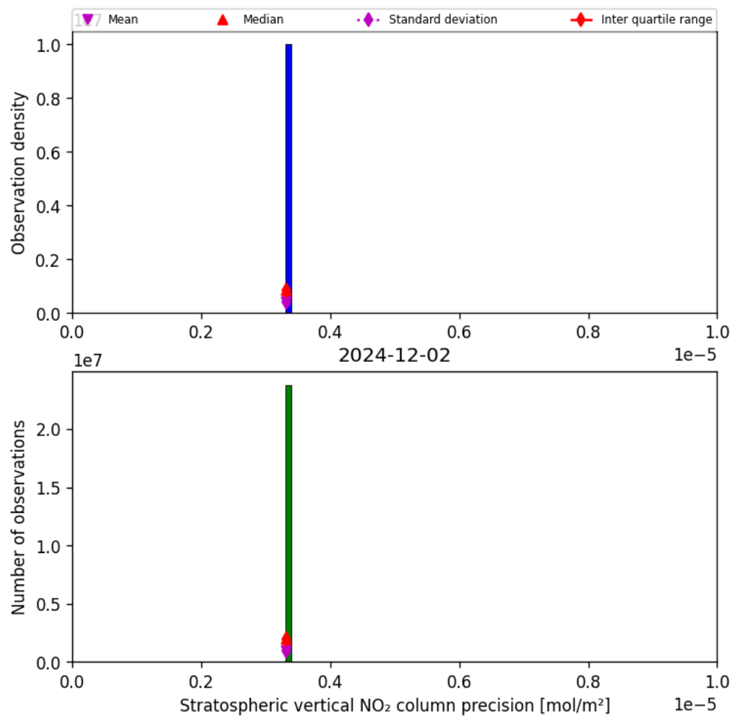
Figure 35: Histogram of “Stratospheric vertical NO 2 column precision” for 2024-12-02 to 2024-12-03
