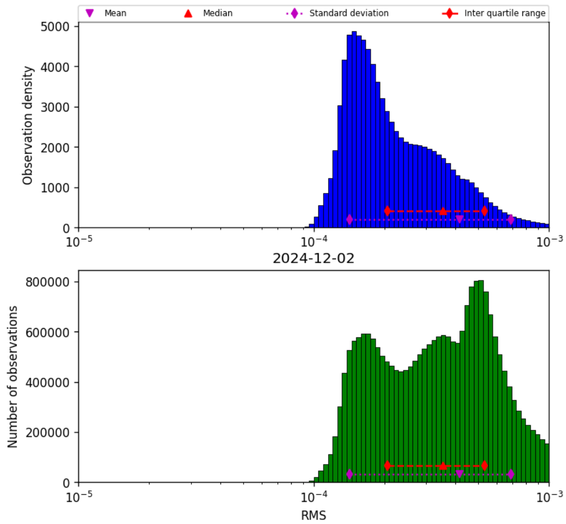
Figure 41: Histogram of “RMS” for 2024-12-02 to 2024-12-03
