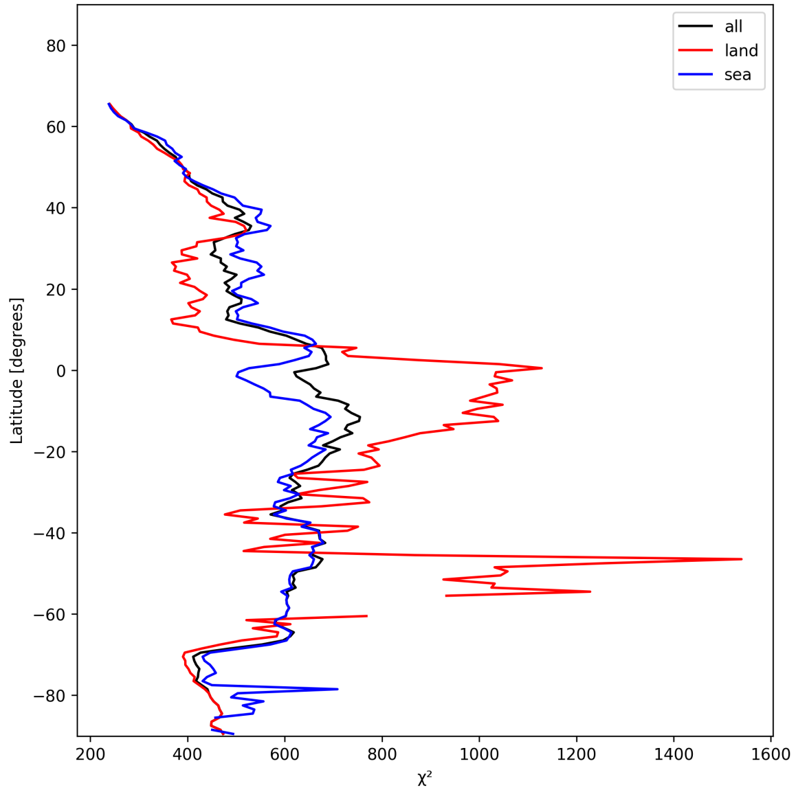
Figure 23: Zonal average of “ \chi^2 ” for 2024-12-02 to 2024-12-03.
