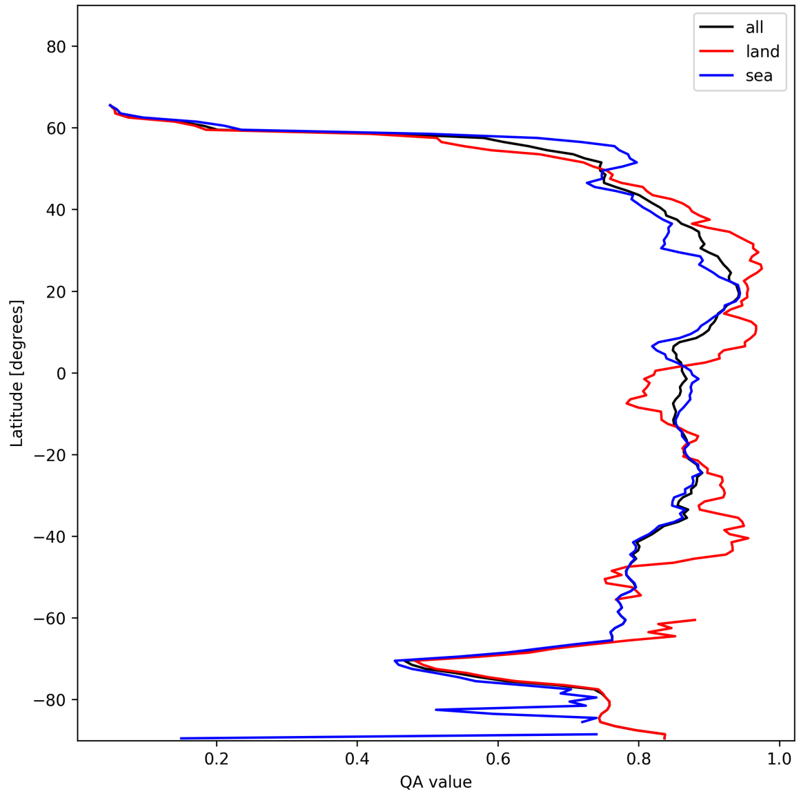
Figure 9: Zonal average of “QA value” for 2024-12-02 to 2024-12-03.
