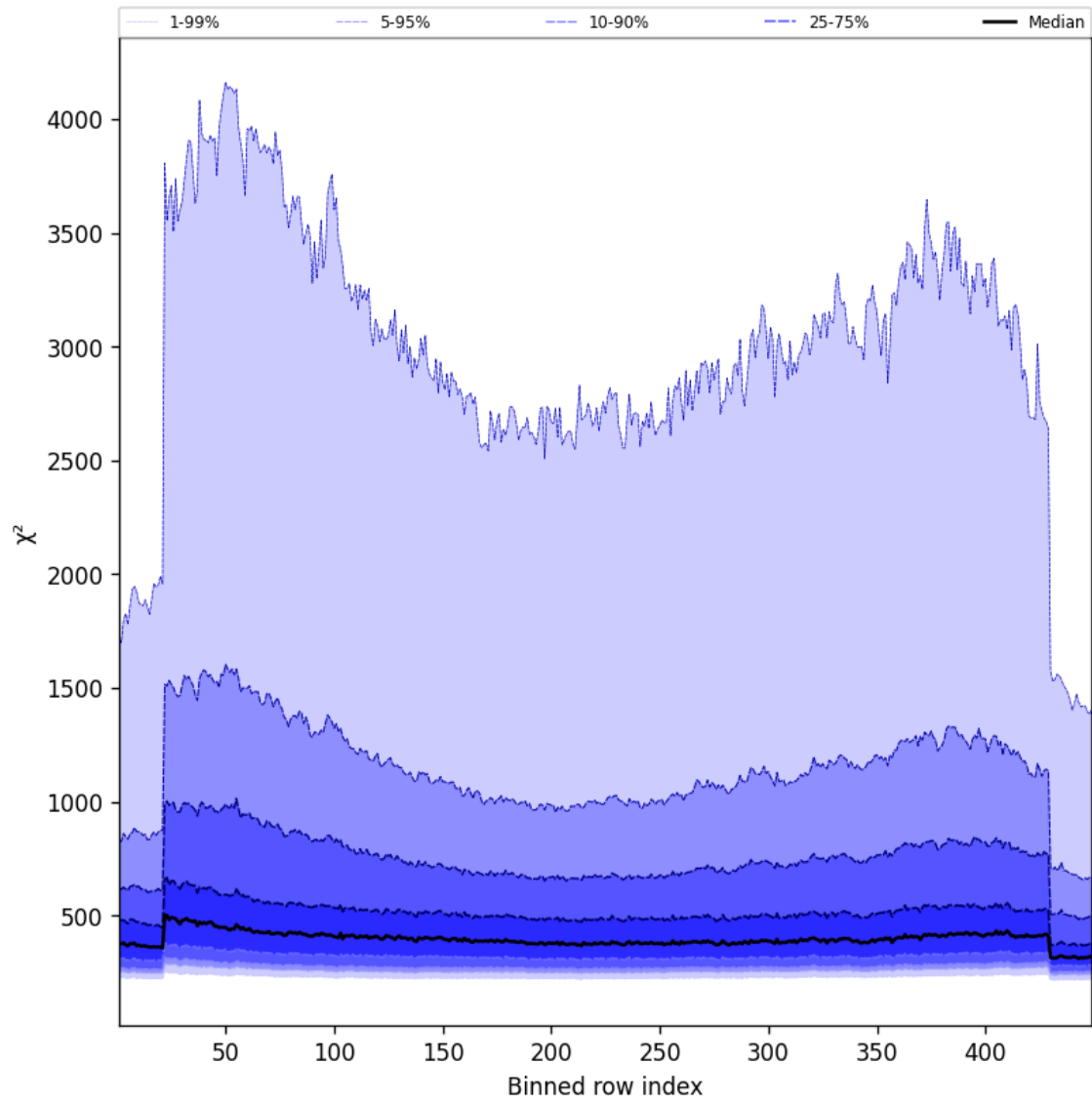
Figure 57: Along track statistics of “ \chi^2 ” for 2024-12-02 to 2024-12-03
