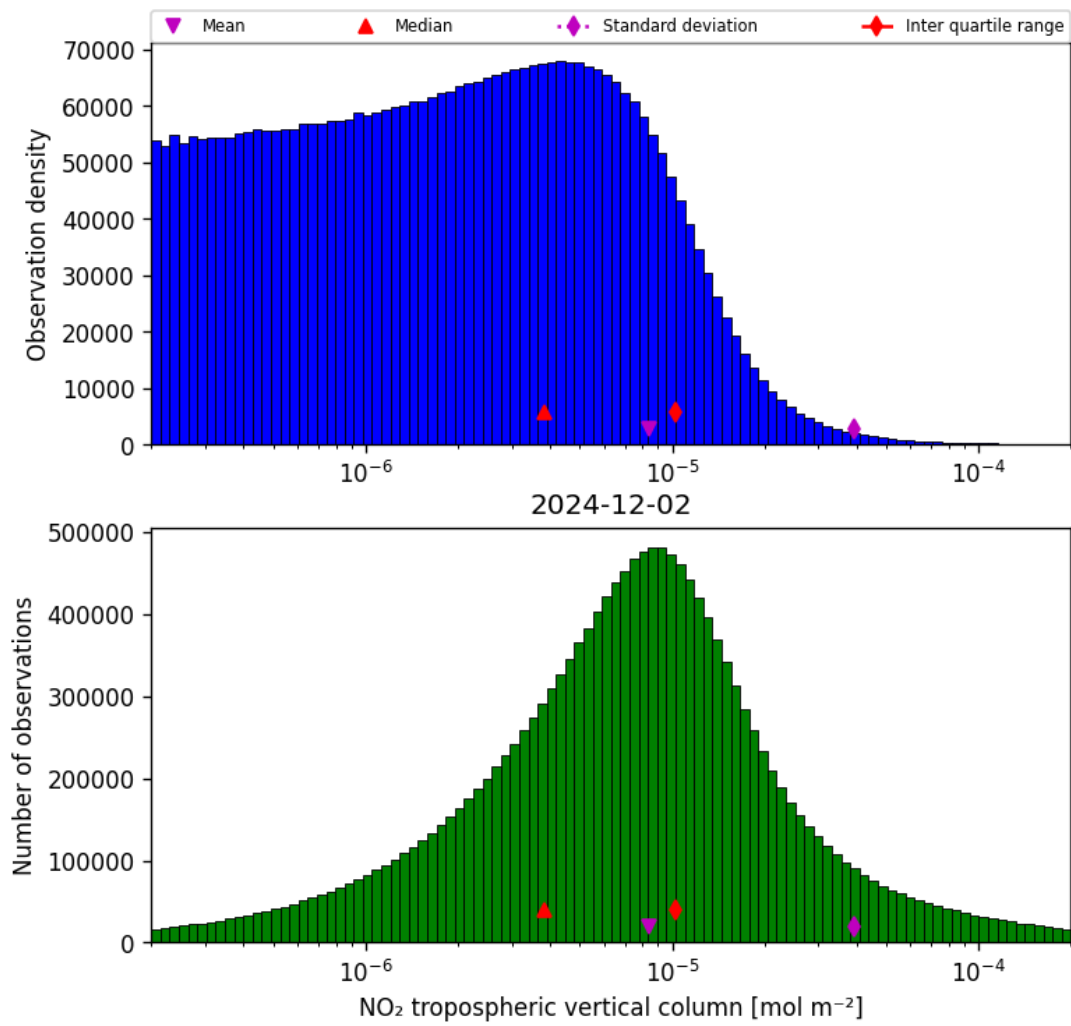
Figure 27: Histogram of “NO 2 tropospheric vertical column” for 2024-12-02 to 2024-12-03
