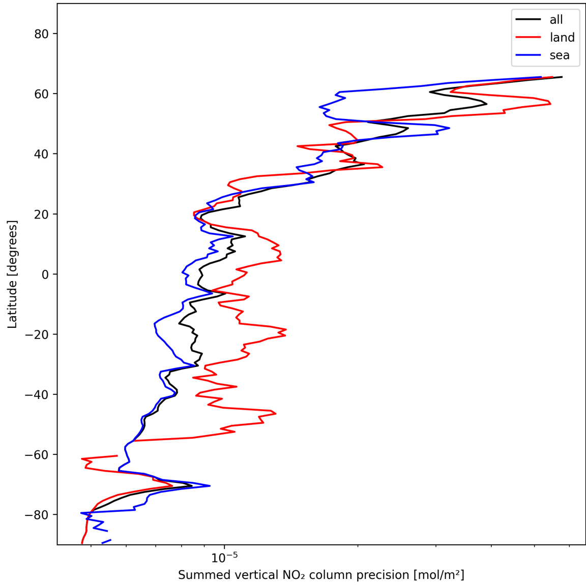
Figure 22: Zonal average of “Summed vertical NO 2 column precision” for 2024-12-02 to 2024-12-03.
