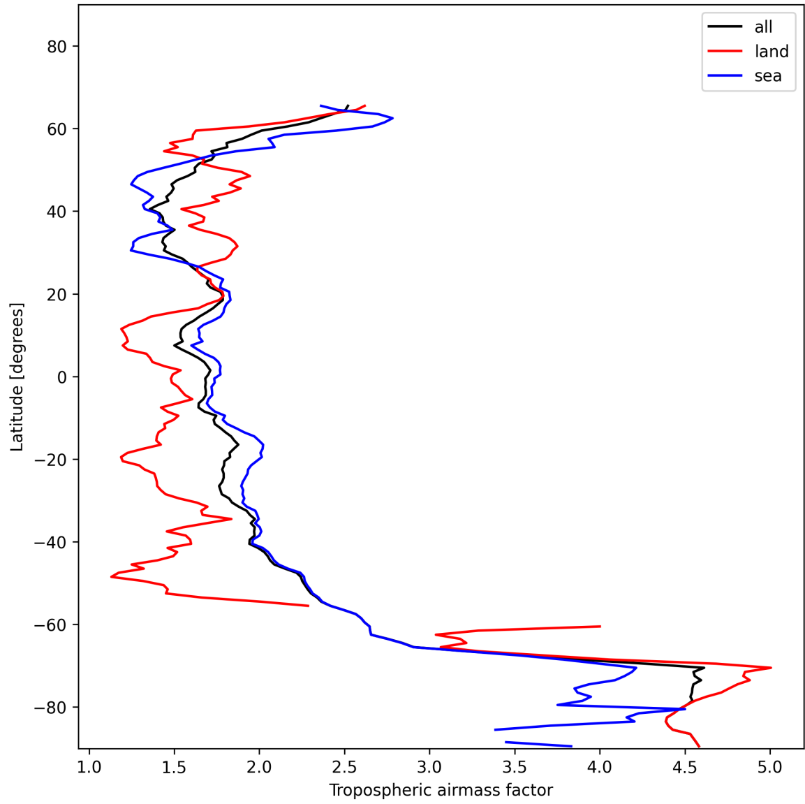
Figure 12: Zonal average of “Tropospheric airmass factor” for 2024-12-02 to 2024-12-03.
