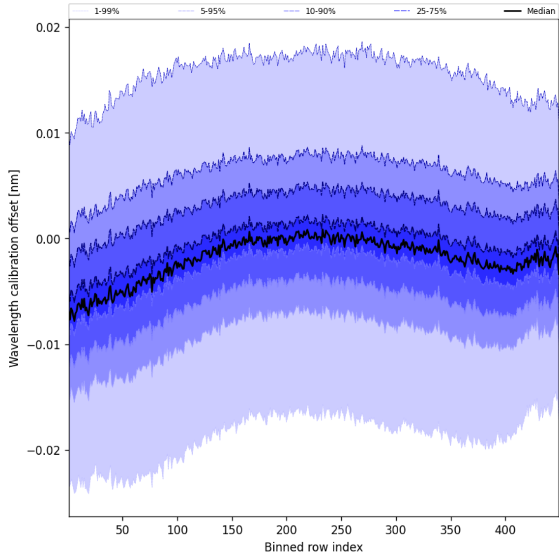
Figure 50: Along track statistics of “Wavelength calibration offset” for 2024-12-02 to 2024-12-03
