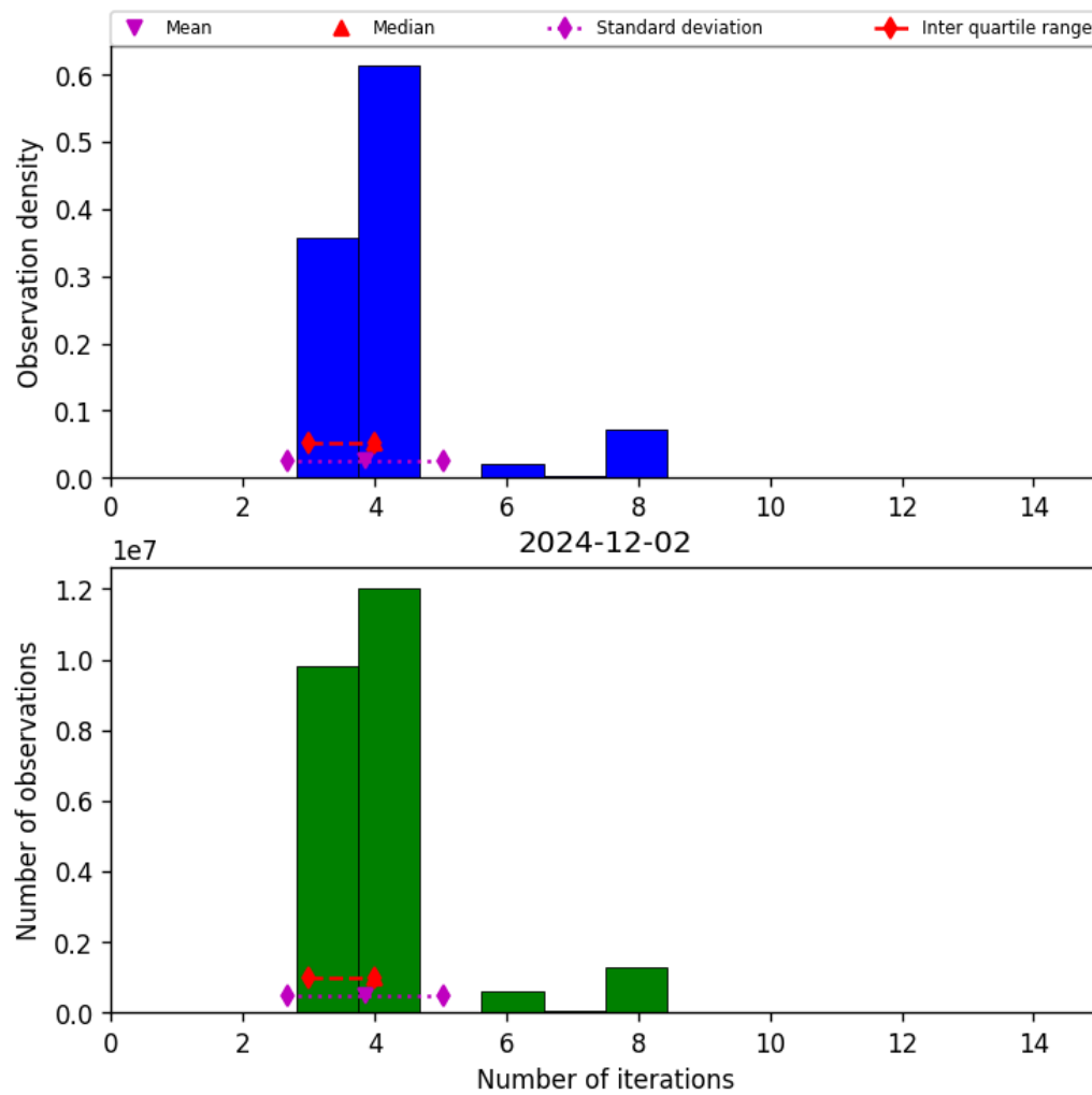
Figure 32: Histogram of “Number of iterations” for 2024-12-02 to 2024-12-03
