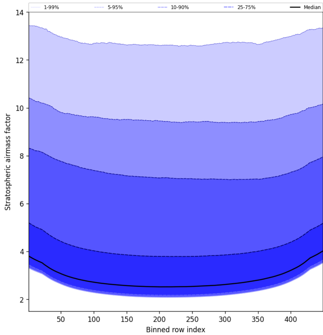
Figure 59: Along track statistics of “Stratospheric airmass factor” for 2024-12-02 to 2024-12-03
