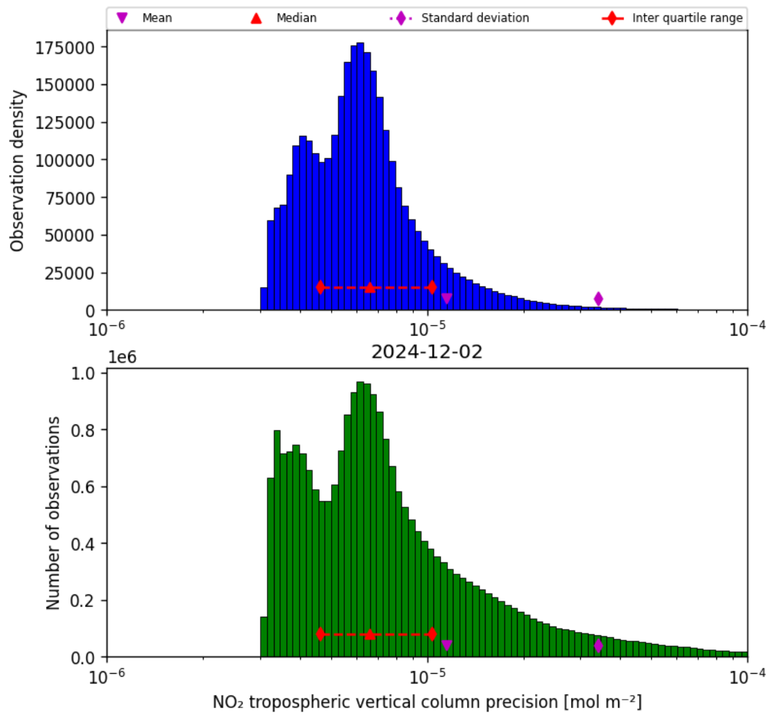
Figure 28: Histogram of “NO 2 tropospheric vertical column precision” for 2024-12-02 to 2024-12-03
