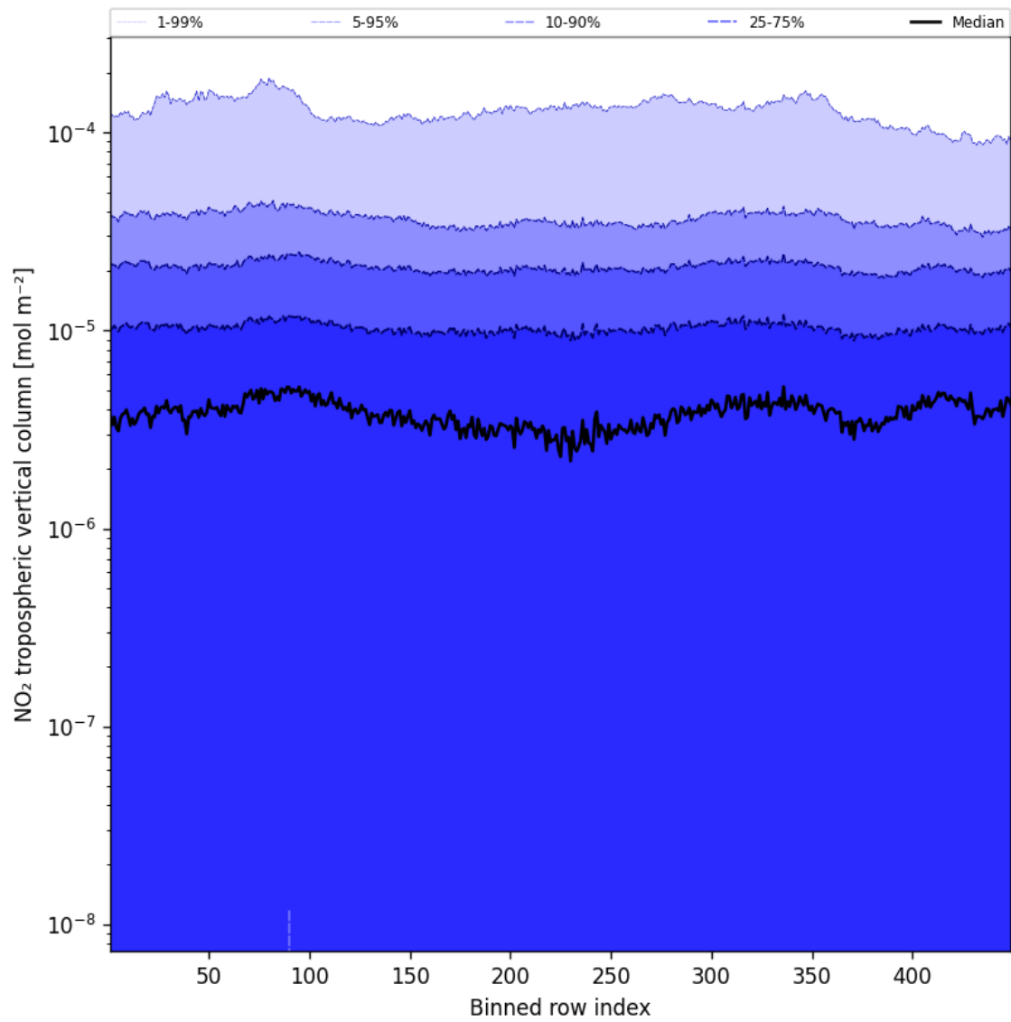
Figure 44: Along track statistics of “ \text{NO}_2 tropospheric vertical column” for 2024-12-02 to 2024-12-03
