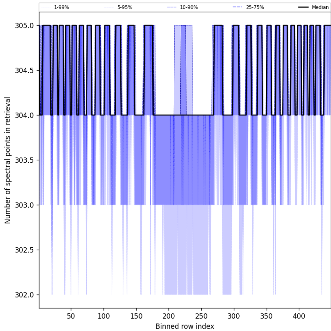
Figure 48: Along track statistics of “Number of spectral points in retrieval” for 2024-12-02 to 2024-12-03
