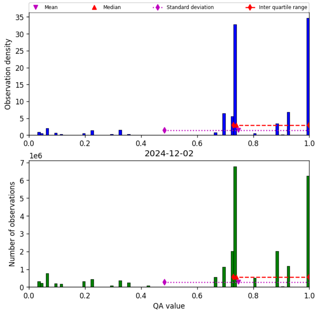
Figure 26: Histogram of “QA value” for 2024-12-02 to 2024-12-03
