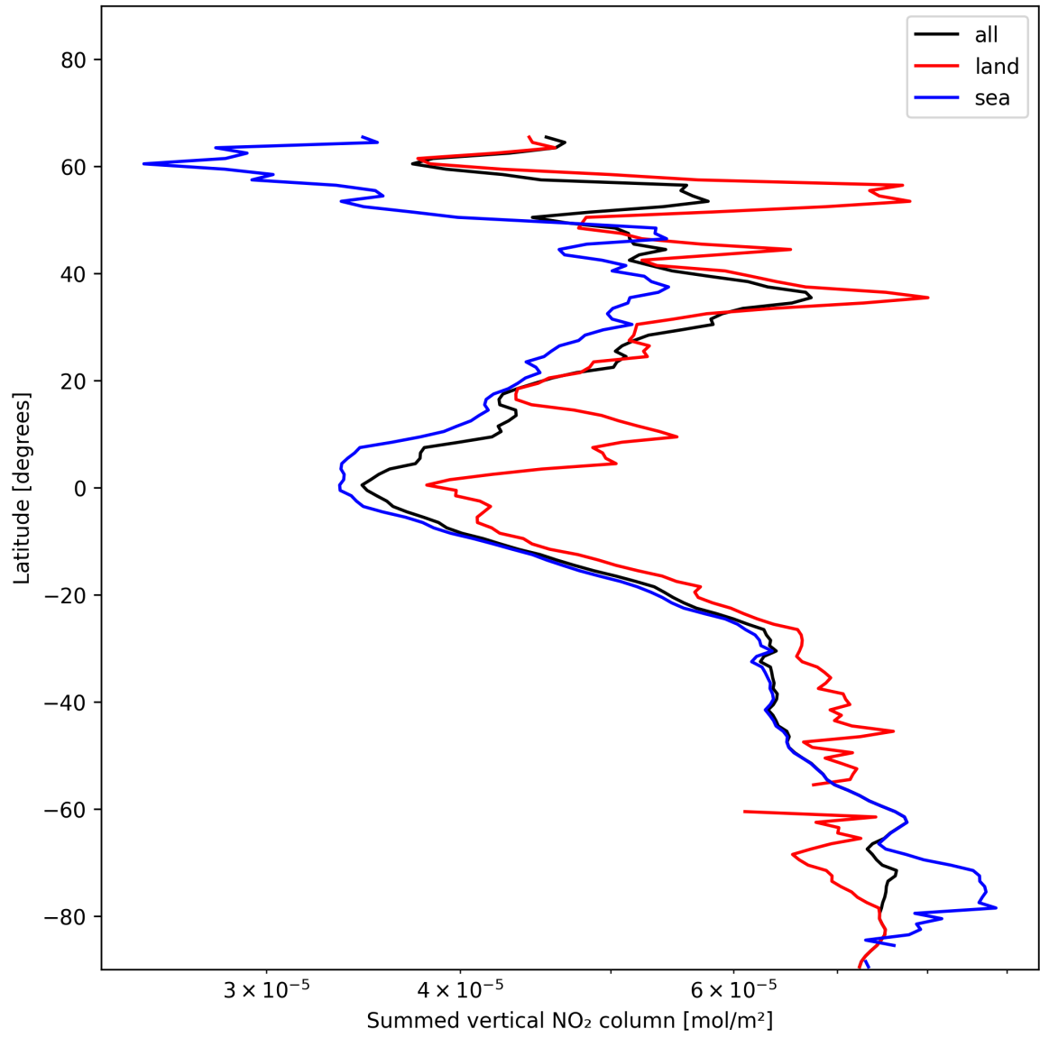
Figure 21: Zonal average of “Summed vertical NO 2 column” for 2024-12-02 to 2024-12-03.
