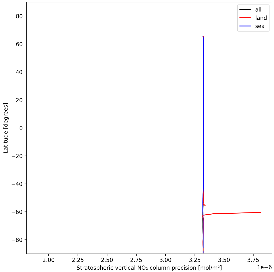
Figure 18: Zonal average of “Stratospheric vertical NO 2 column precision” for 2024-12-02 to 2024-12-03.
