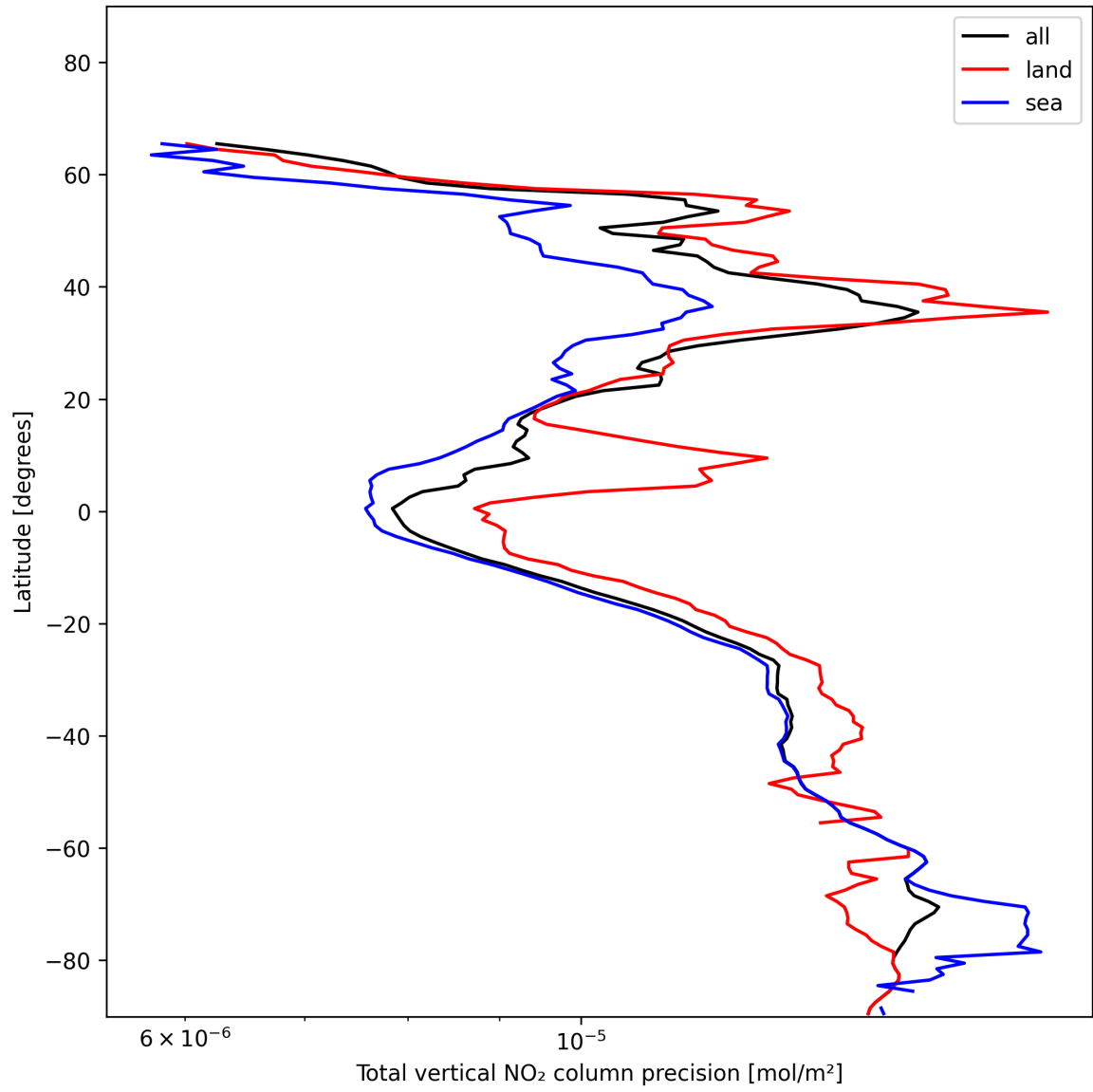
Figure 20: Zonal average of “Total vertical NO 2 column precision” for 2024-12-02 to 2024-12-03.
