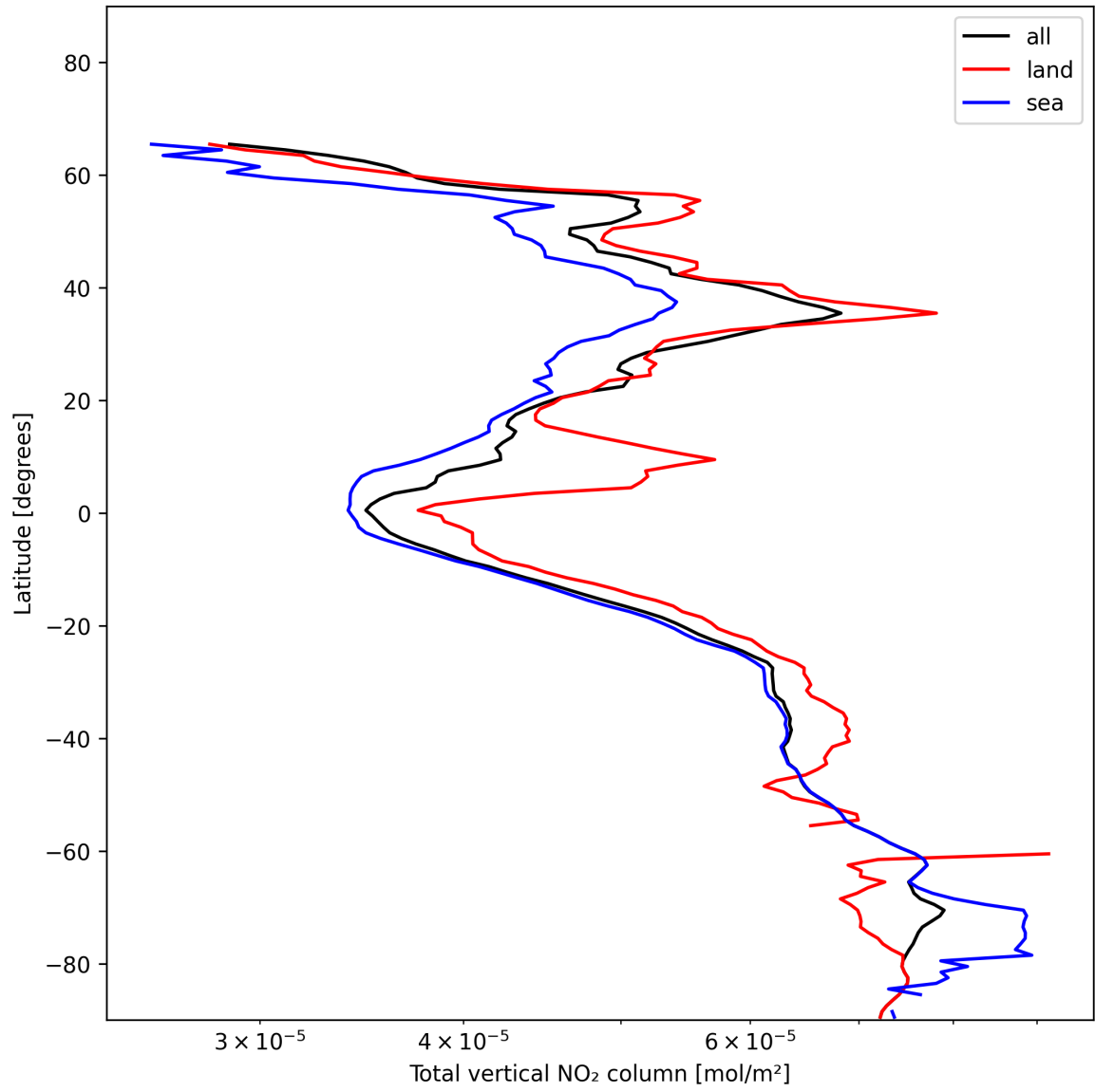
Figure 19: Zonal average of “Total vertical NO 2 column” for 2024-12-02 to 2024-12-03.
