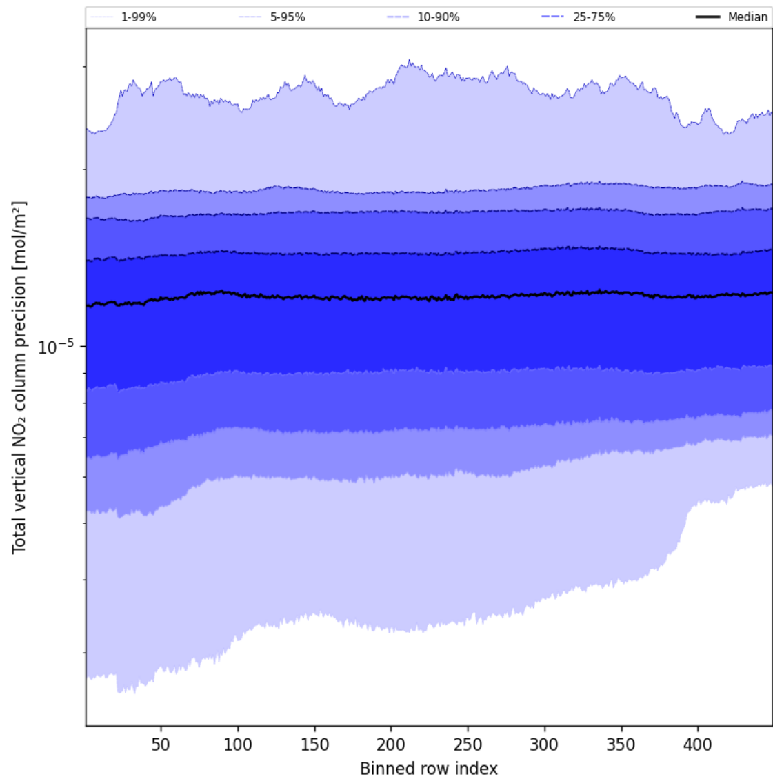
Figure 54: Along track statistics of “Total vertical NO 2 column precision” for 2024-12-02 to 2024-12-03
