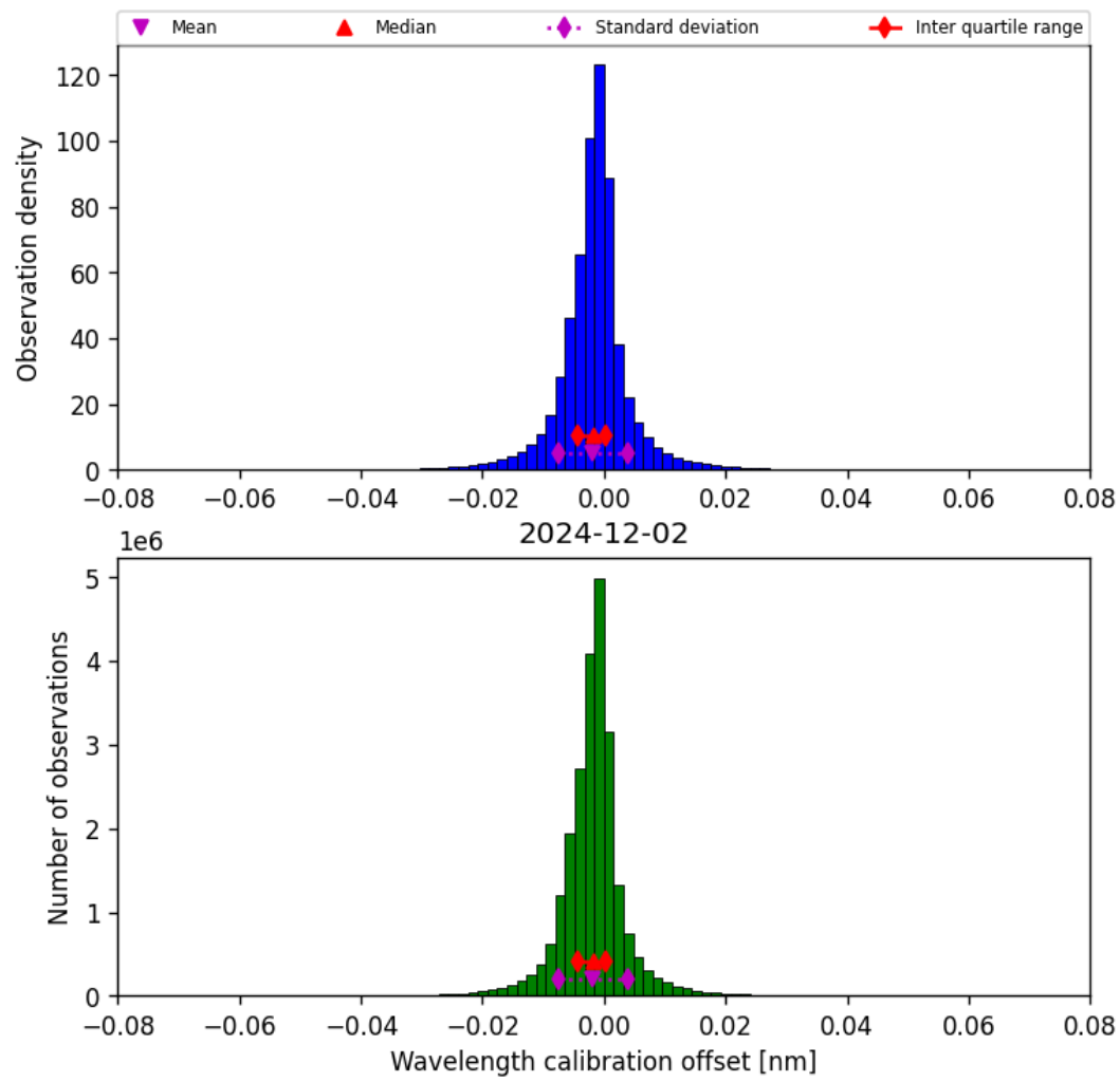
Figure 33: Histogram of “Wavelength calibration offset” for 2024-12-02 to 2024-12-03
