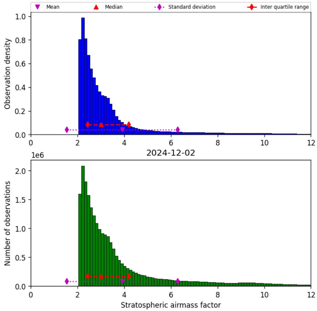
Figure 42: Histogram of “Stratospheric airmass factor” for 2024-12-02 to 2024-12-03
