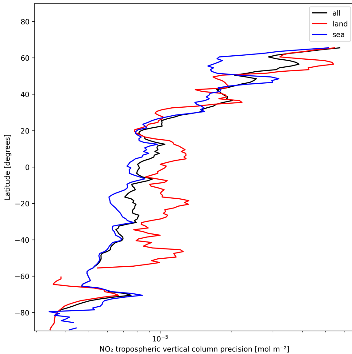
Figure 11: Zonal average of “NO 2 tropospheric vertical column precision” for 2024-12-02 to 2024-12-03.
