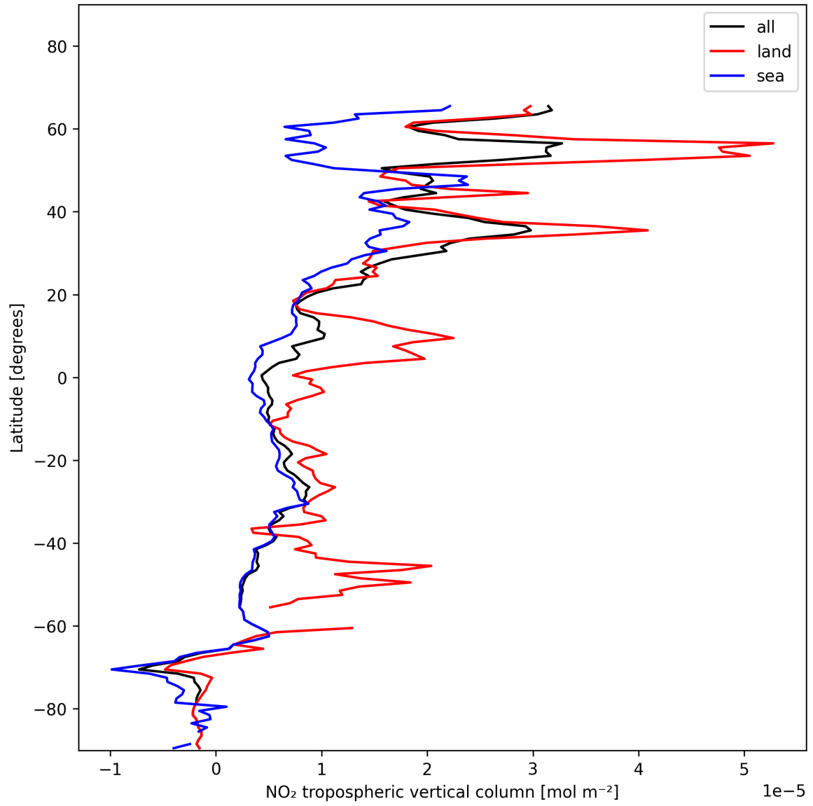
Figure 10: Zonal average of “NO 2 tropospheric vertical column” for 2024-12-02 to 2024-12-03.
