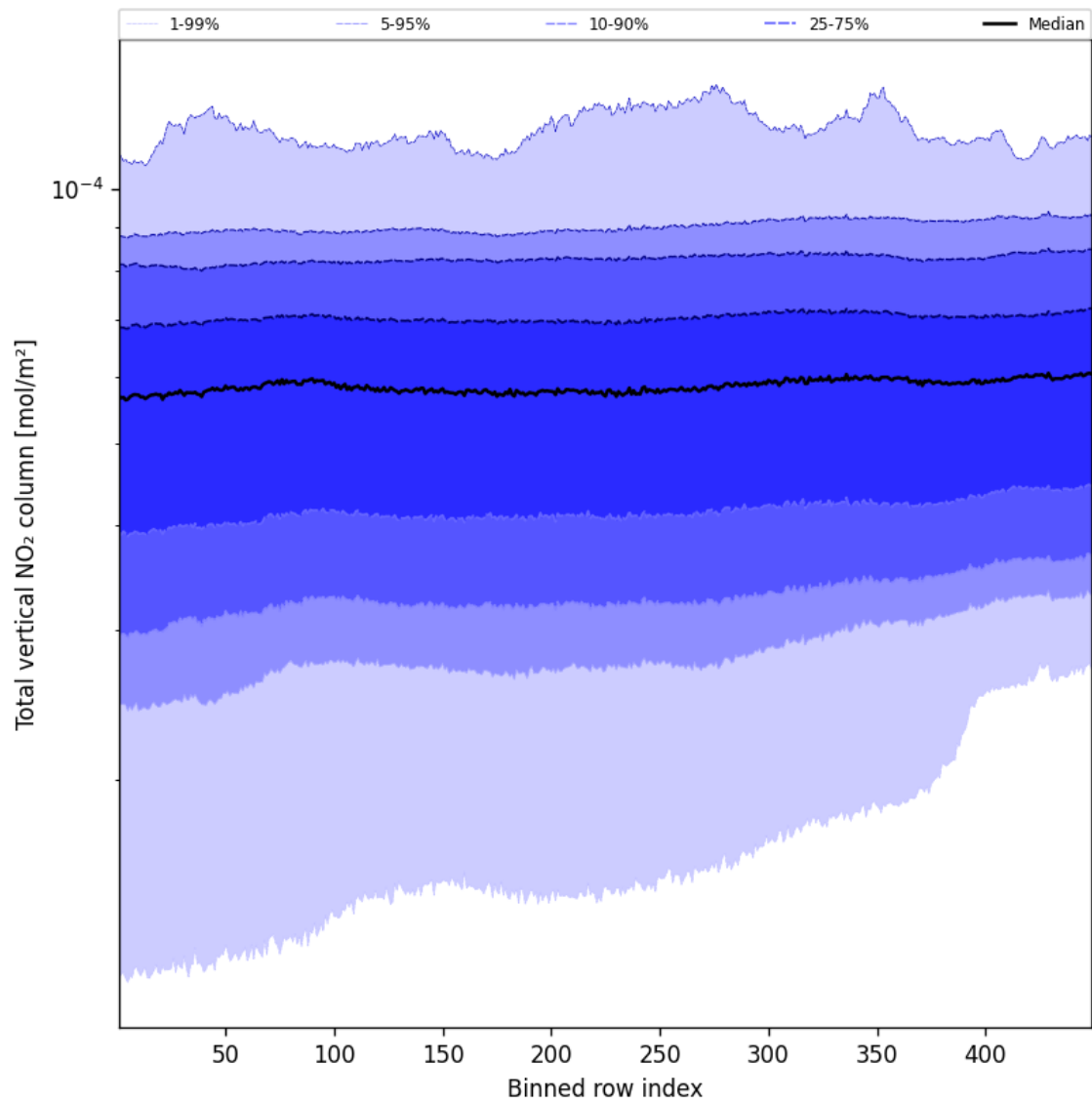
Figure 53: Along track statistics of “Total vertical NO 2 column” for 2024-12-02 to 2024-12-03
