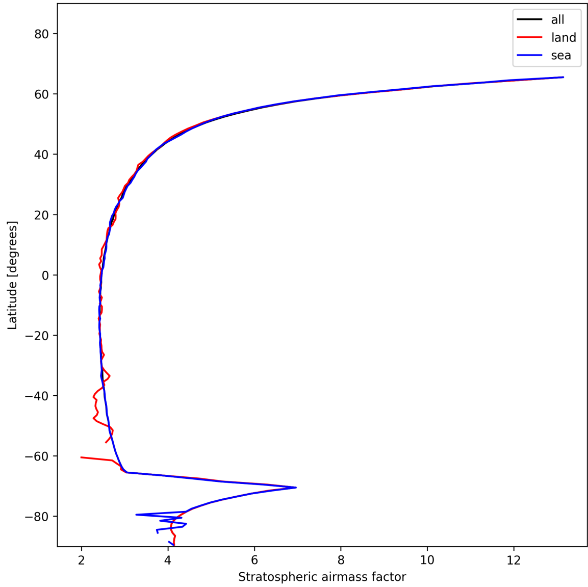
Figure 25: Zonal average of “Stratospheric airmass factor” for 2024-12-02 to 2024-12-03.
