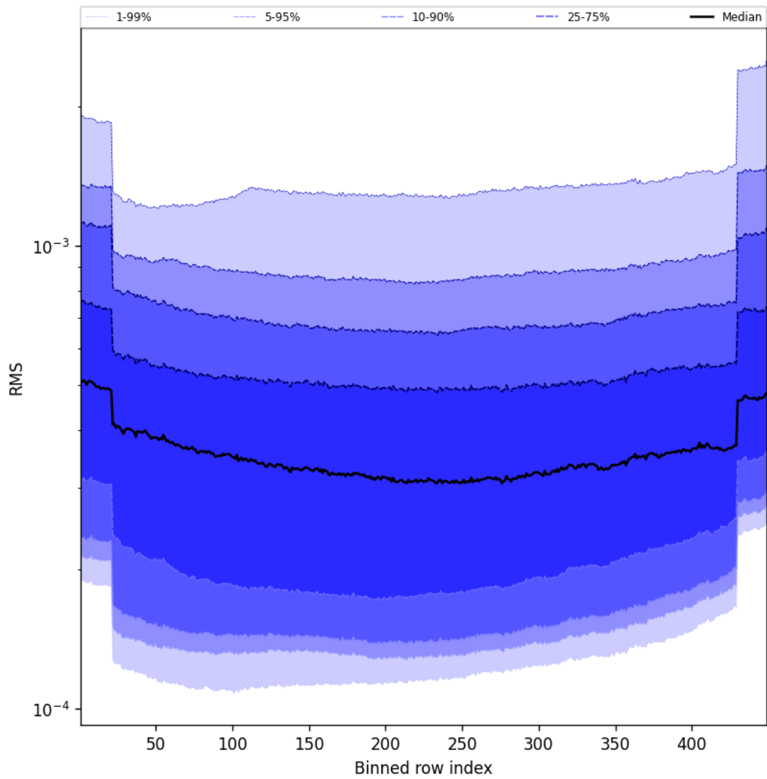
Figure 58: Along track statistics of “RMS” for 2024-12-02 to 2024-12-03
