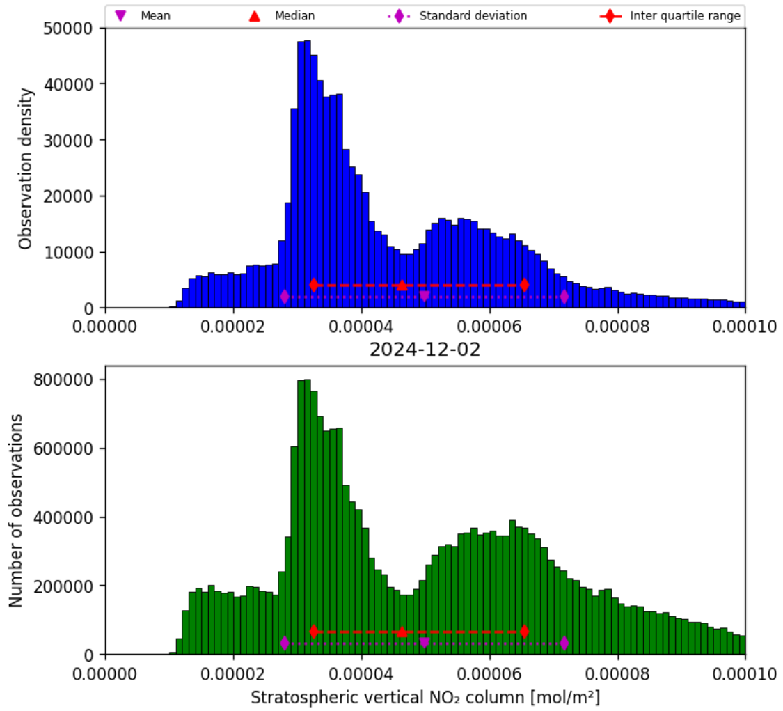
Figure 34: Histogram of “Stratospheric vertical NO 2 column” for 2024-12-02 to 2024-12-03
