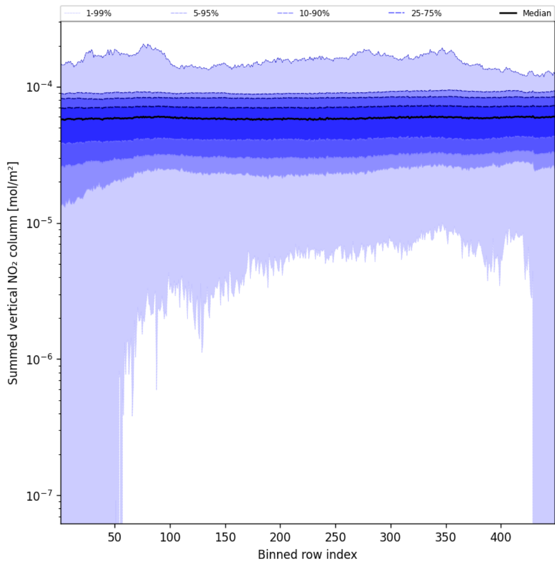
Figure 55: Along track statistics of “Summed vertical NO 2 column” for 2024-12-02 to 2024-12-03
