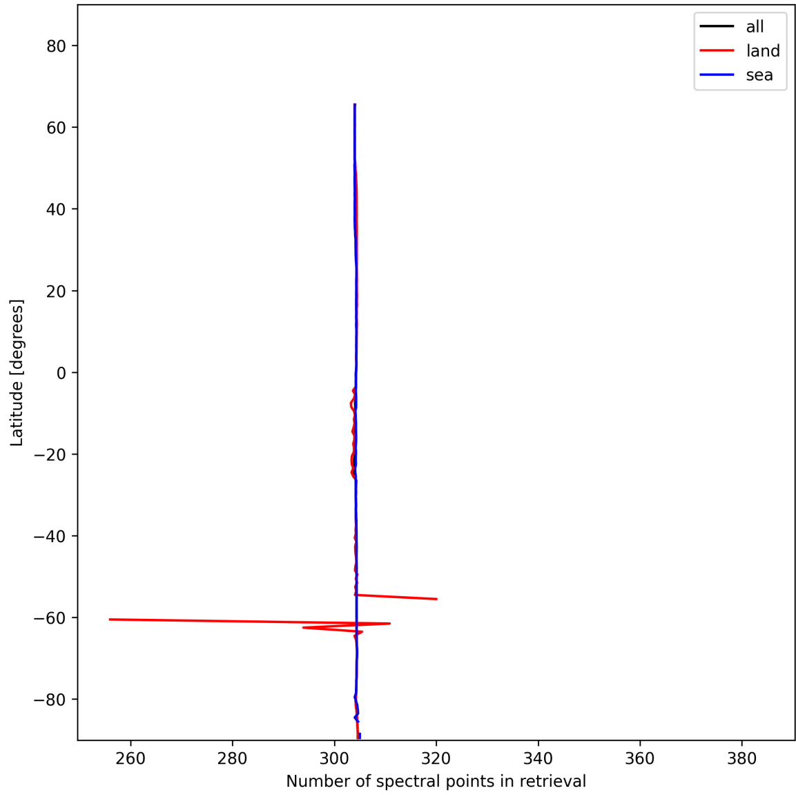
Figure 14: Zonal average of “Number of spectral points in retrieval” for 2024-12-02 to 2024-12-03.
