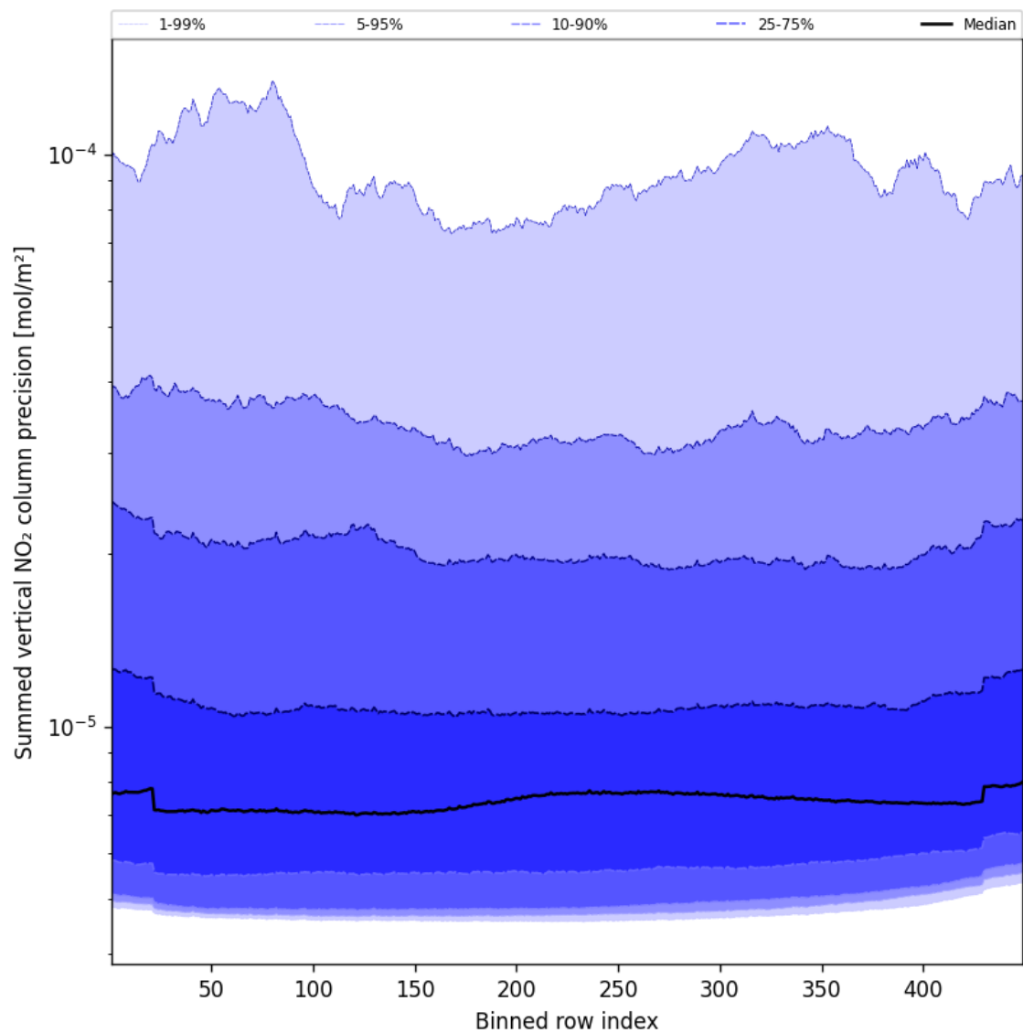
Figure 56: Along track statistics of “Summed vertical NO 2 column precision” for 2024-12-02 to 2024-12-03
