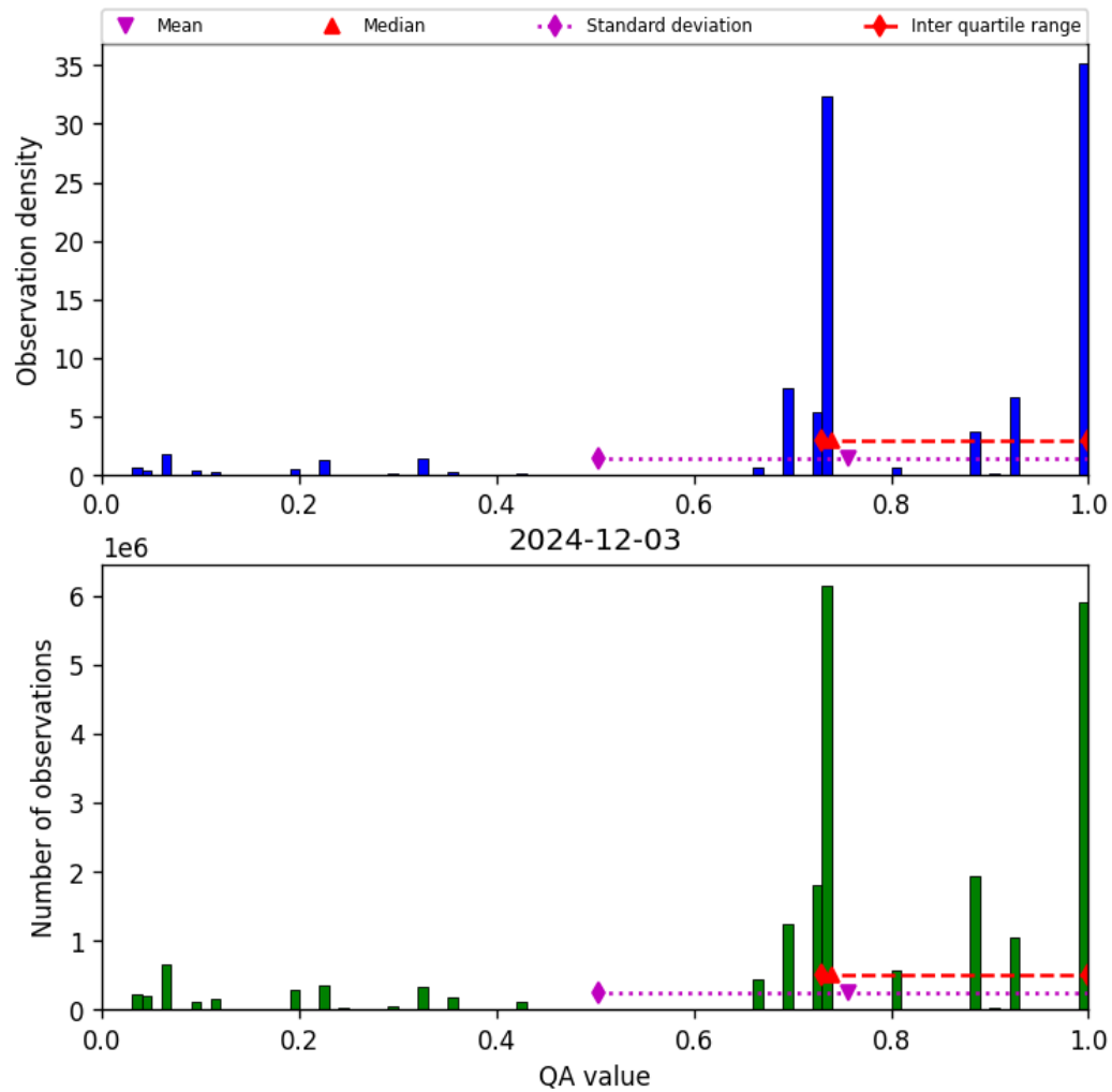
Figure 26: Histogram of “QA value” for 2024-12-03 to 2024-12-03
