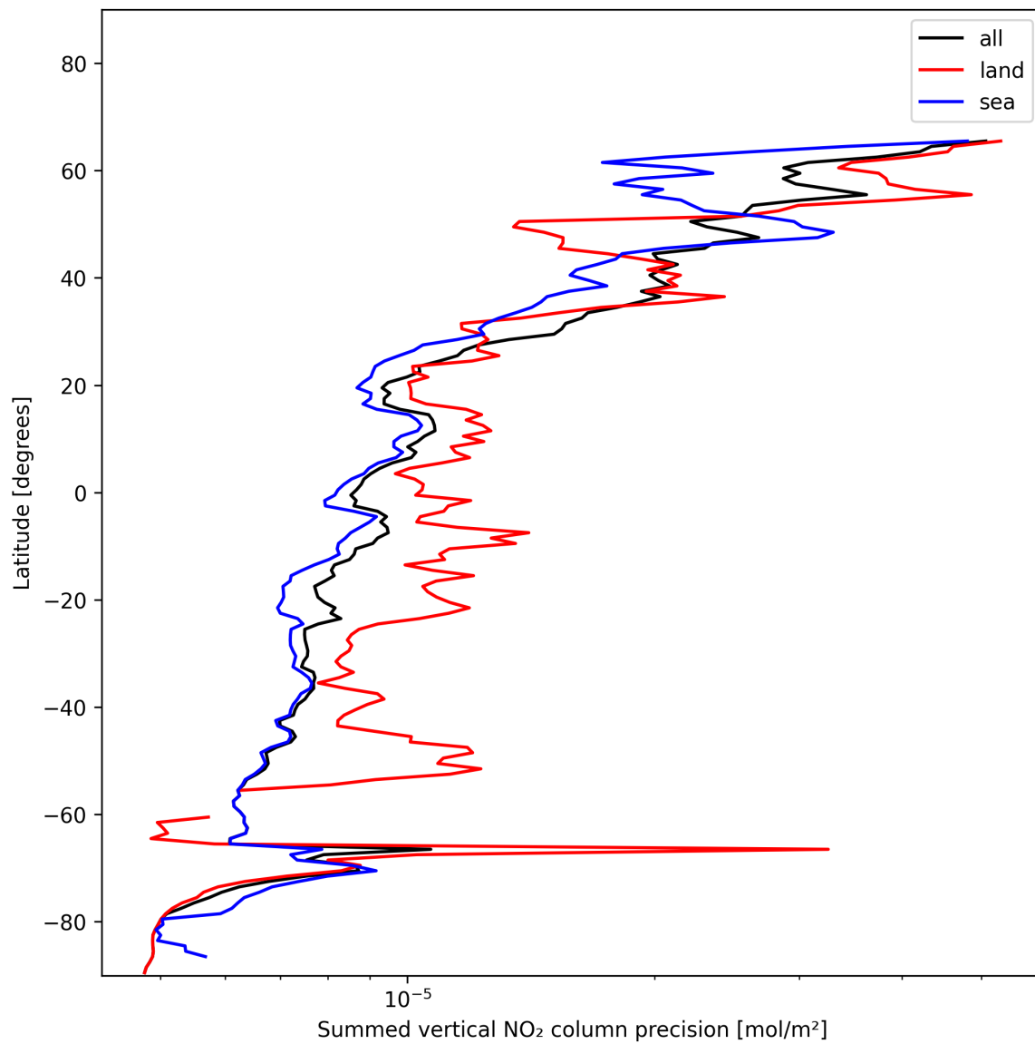
Figure 22: Zonal average of “Summed vertical NO 2 column precision” for 2024-12-03 to 2024-12-03.
