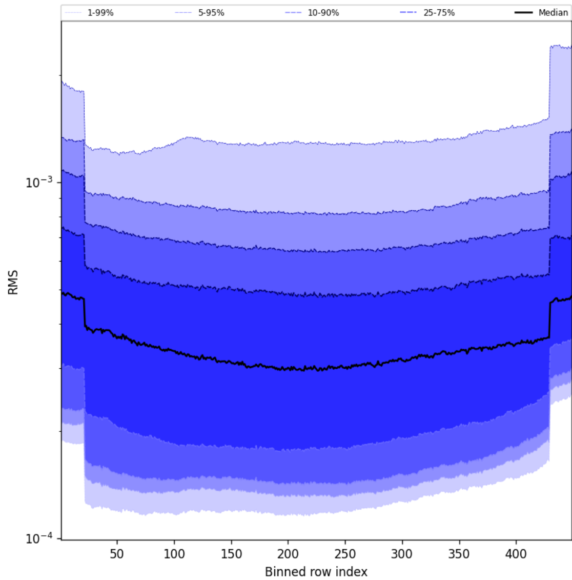
Figure 58: Along track statistics of “RMS” for 2024-12-03 to 2024-12-03
