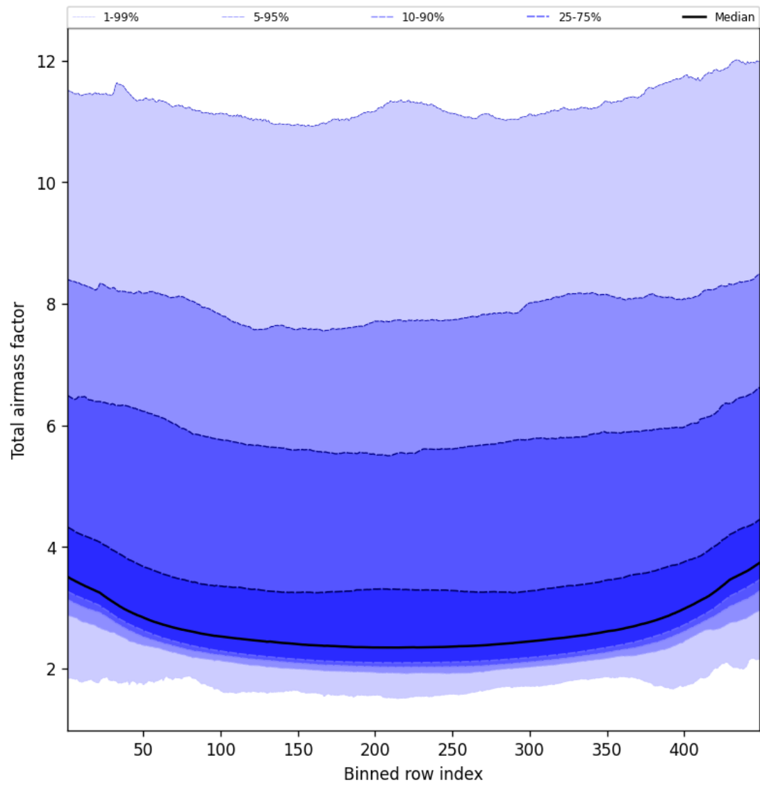
Figure 47: Along track statistics of “Total airmass factor” for 2024-12-03 to 2024-12-03
