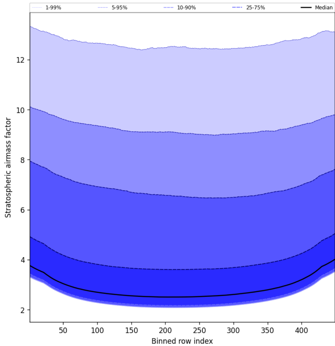
Figure 59: Along track statistics of “Stratospheric airmass factor” for 2024-12-03 to 2024-12-03
