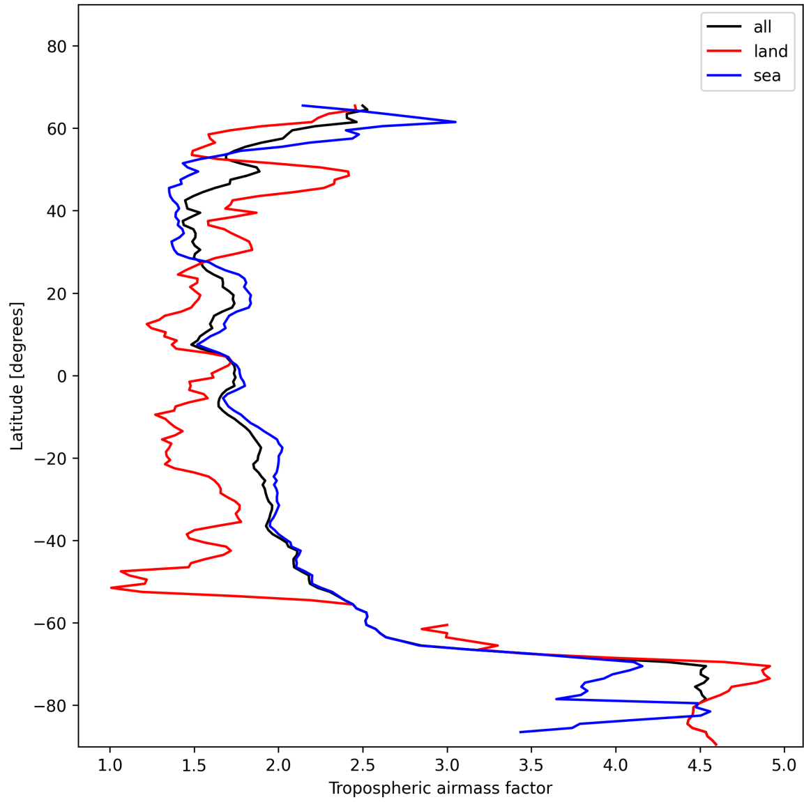
Figure 12: Zonal average of “Tropospheric airmass factor” for 2024-12-03 to 2024-12-03.
