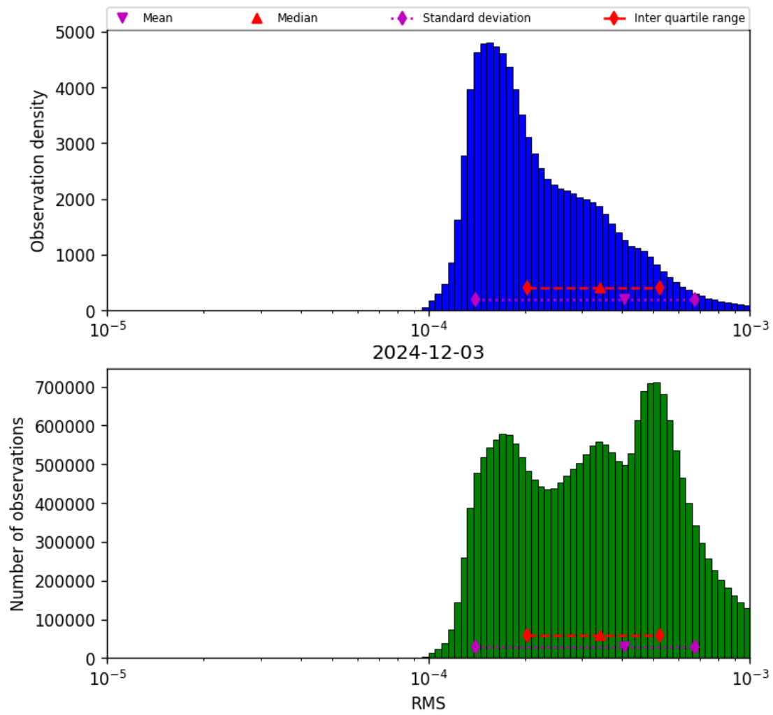
Figure 41: Histogram of “RMS” for 2024-12-03 to 2024-12-03
