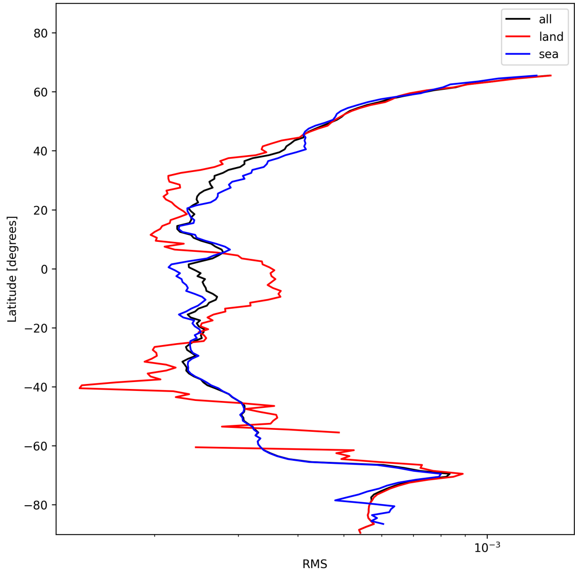
Figure 24: Zonal average of “RMS” for 2024-12-03 to 2024-12-03.
