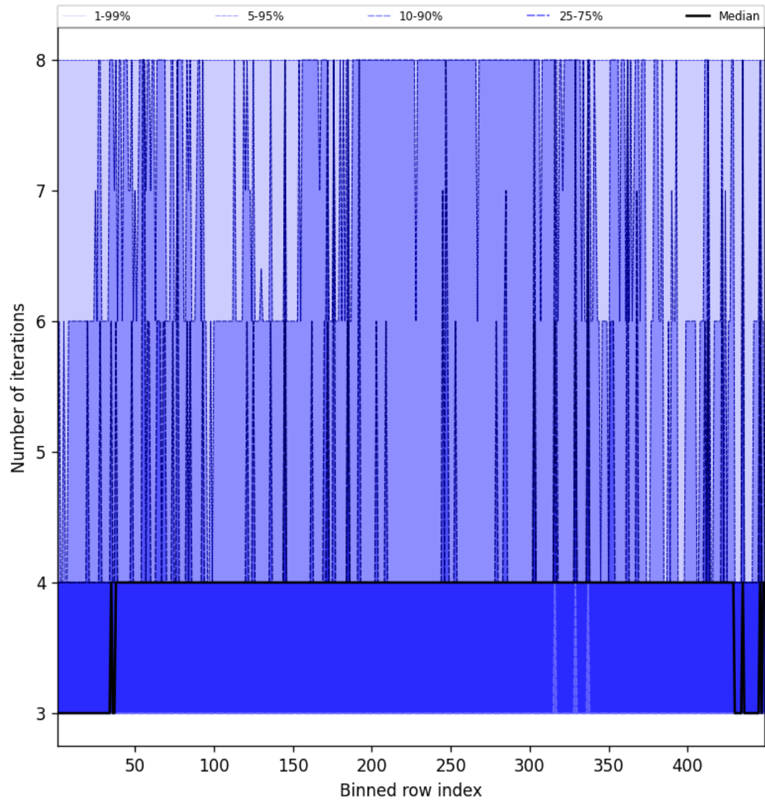
Figure 49: Along track statistics of “Number of iterations” for 2024-12-03 to 2024-12-03
