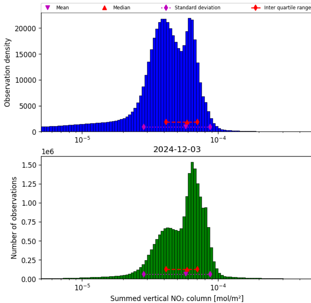
Figure 38: Histogram of "Summed vertical NO 2 column" for 2024-12-03 to 2024-12-03
