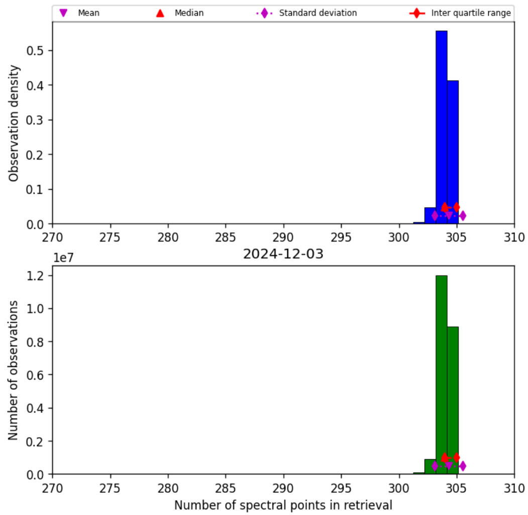
Figure 31: Histogram of “Number of spectral points in retrieval” for 2024-12-03 to 2024-12-03
