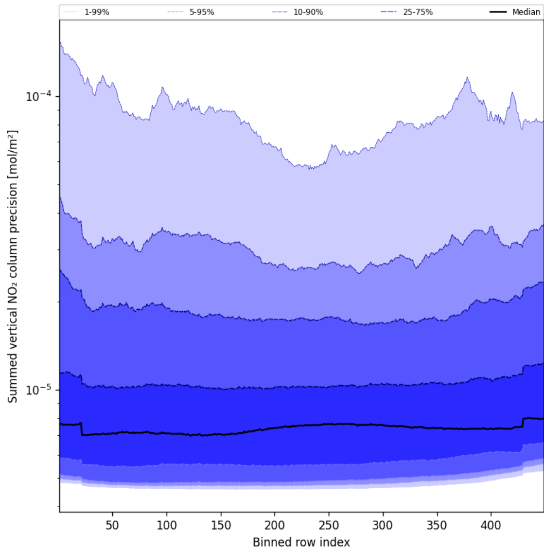
Figure 56: Along track statistics of “Summed vertical NO 2 column precision” for 2024-12-03 to 2024-12-03
