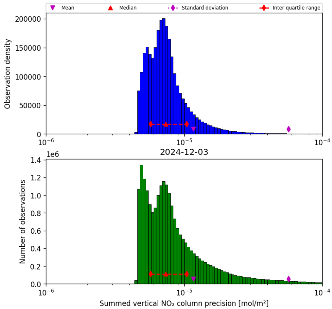
Figure 39: Histogram of "Summed vertical NO 2 column precision" for 2024-12-03 to 2024-12-03
