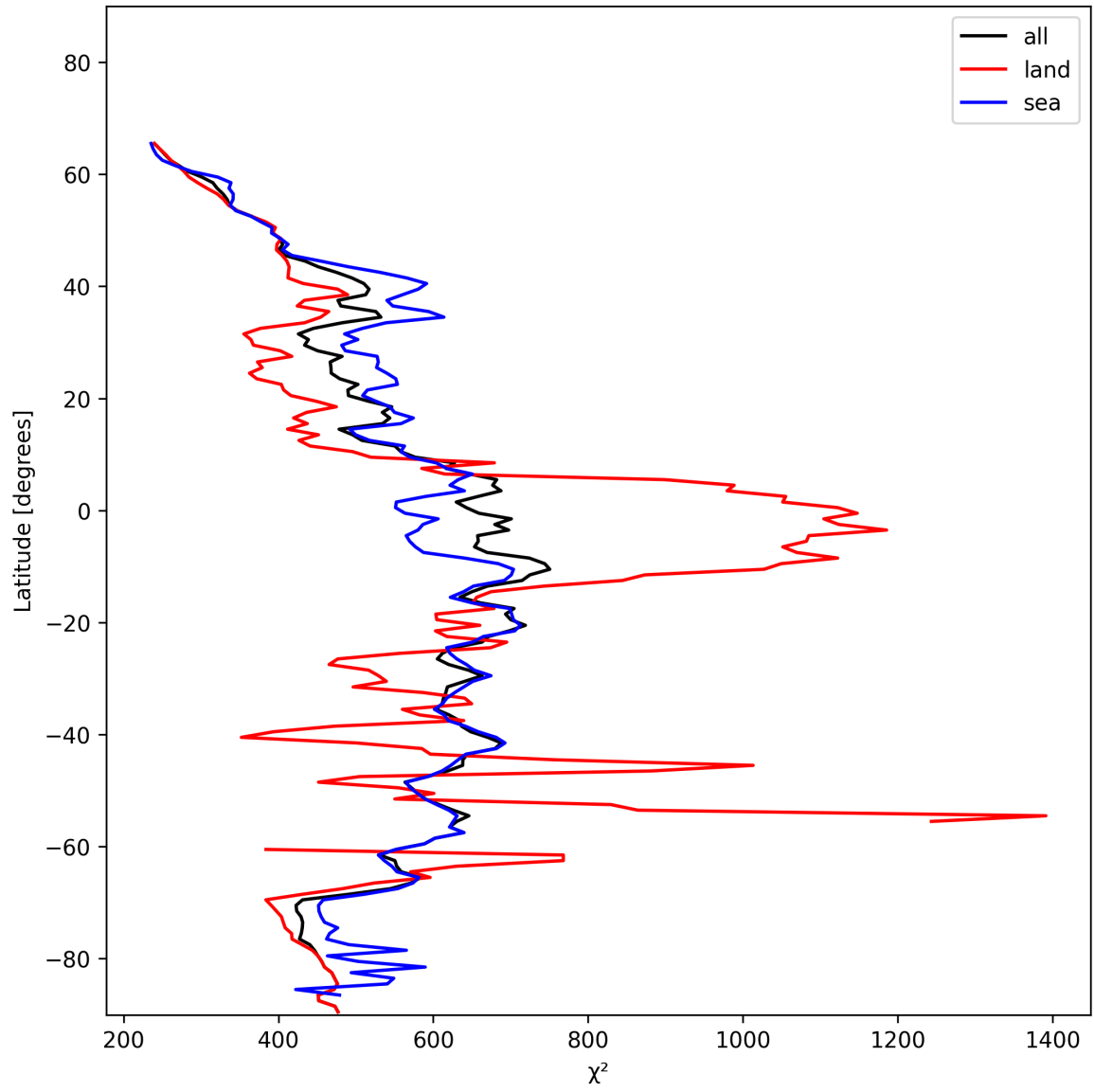
Figure 23: Zonal average of “ \chi^2 ” for 2024-12-03 to 2024-12-03.
