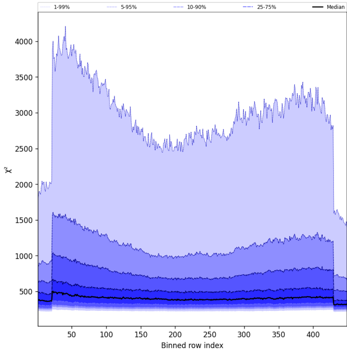
Figure 57: Along track statistics of “ \chi^2 ” for 2024-12-03 to 2024-12-03
