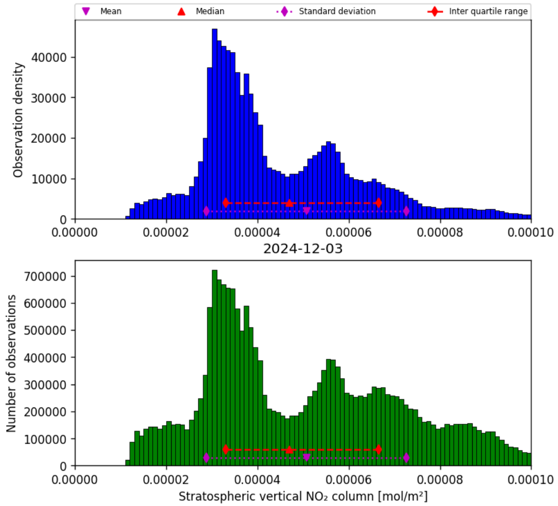
Figure 34: Histogram of “Stratospheric vertical NO 2 column” for 2024-12-03 to 2024-12-03
