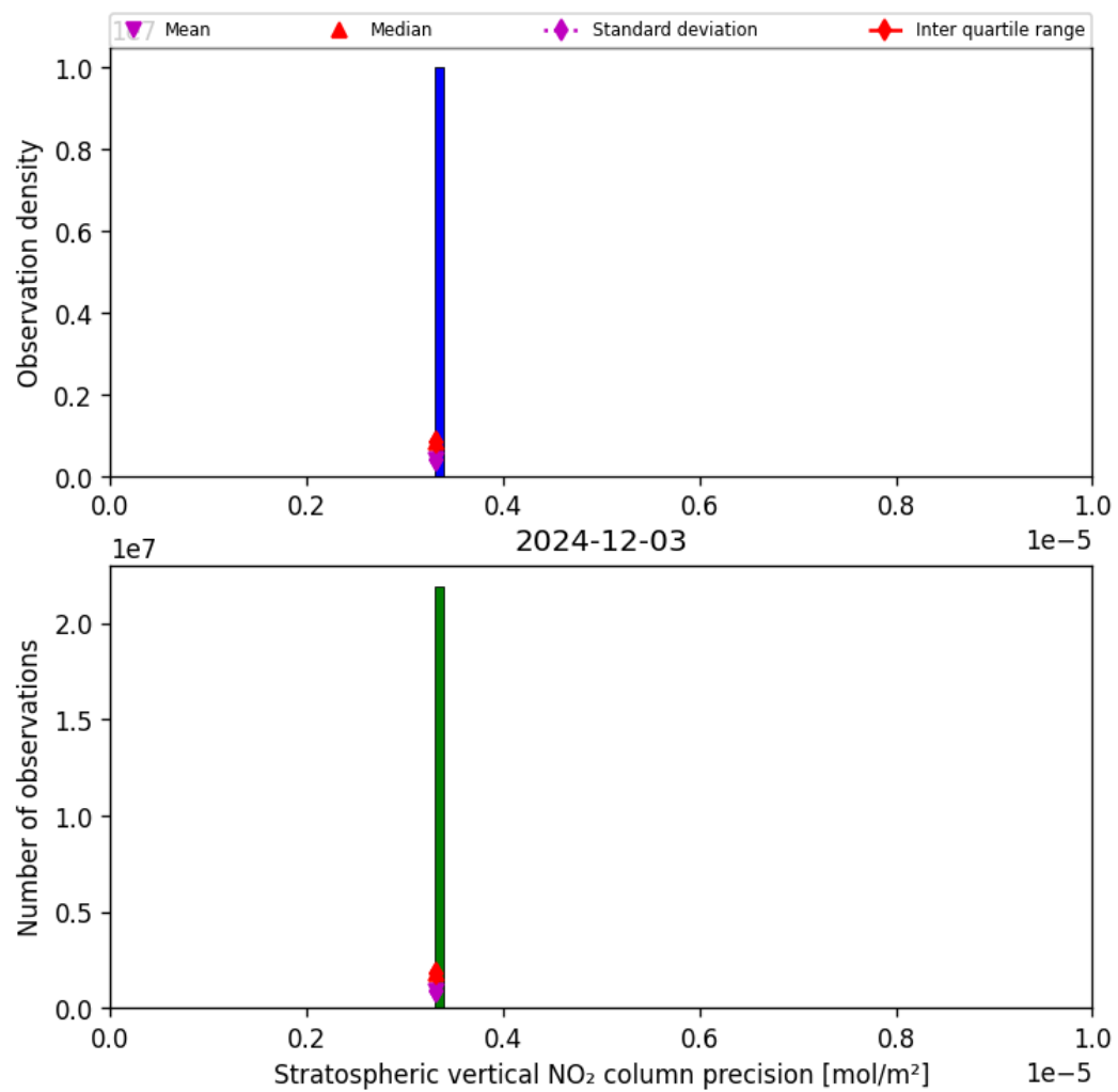
Figure 35: Histogram of “Stratospheric vertical NO 2 column precision” for 2024-12-03 to 2024-12-03
