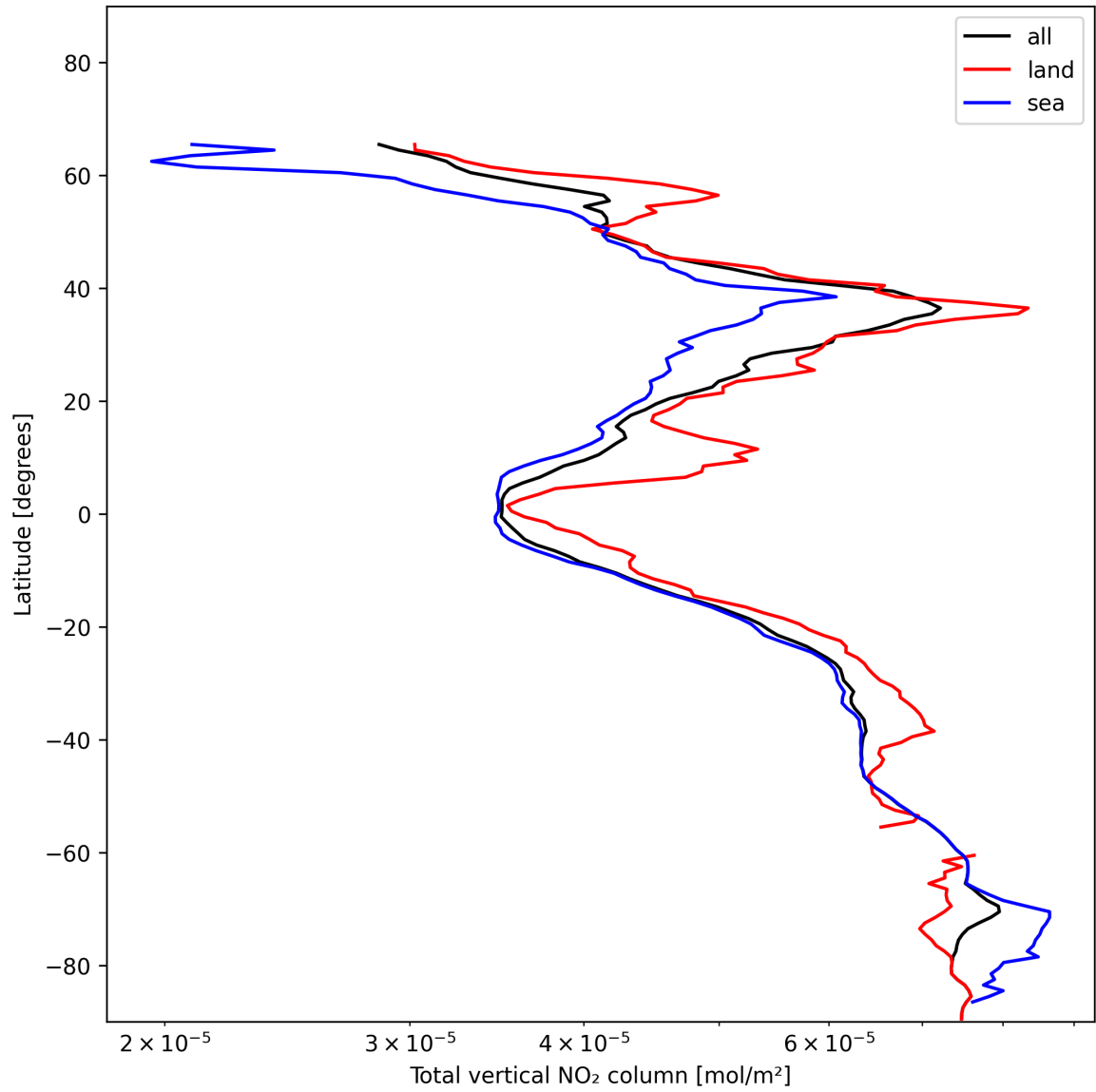
Figure 19: Zonal average of “Total vertical NO 2 column” for 2024-12-03 to 2024-12-03.
