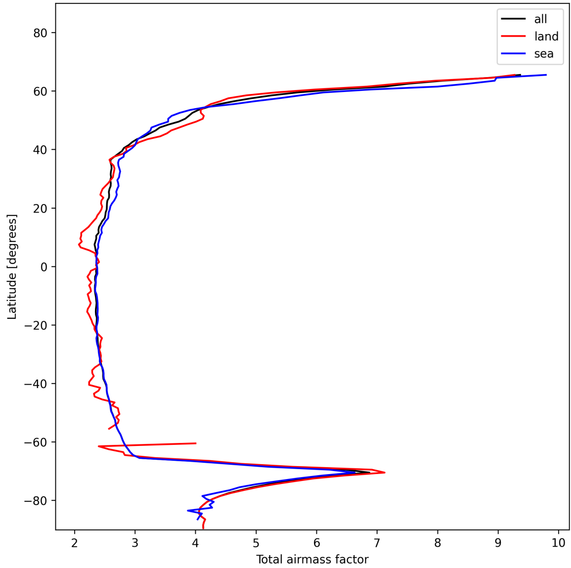
Figure 13: Zonal average of “Total airmass factor” for 2024-12-03 to 2024-12-03.
