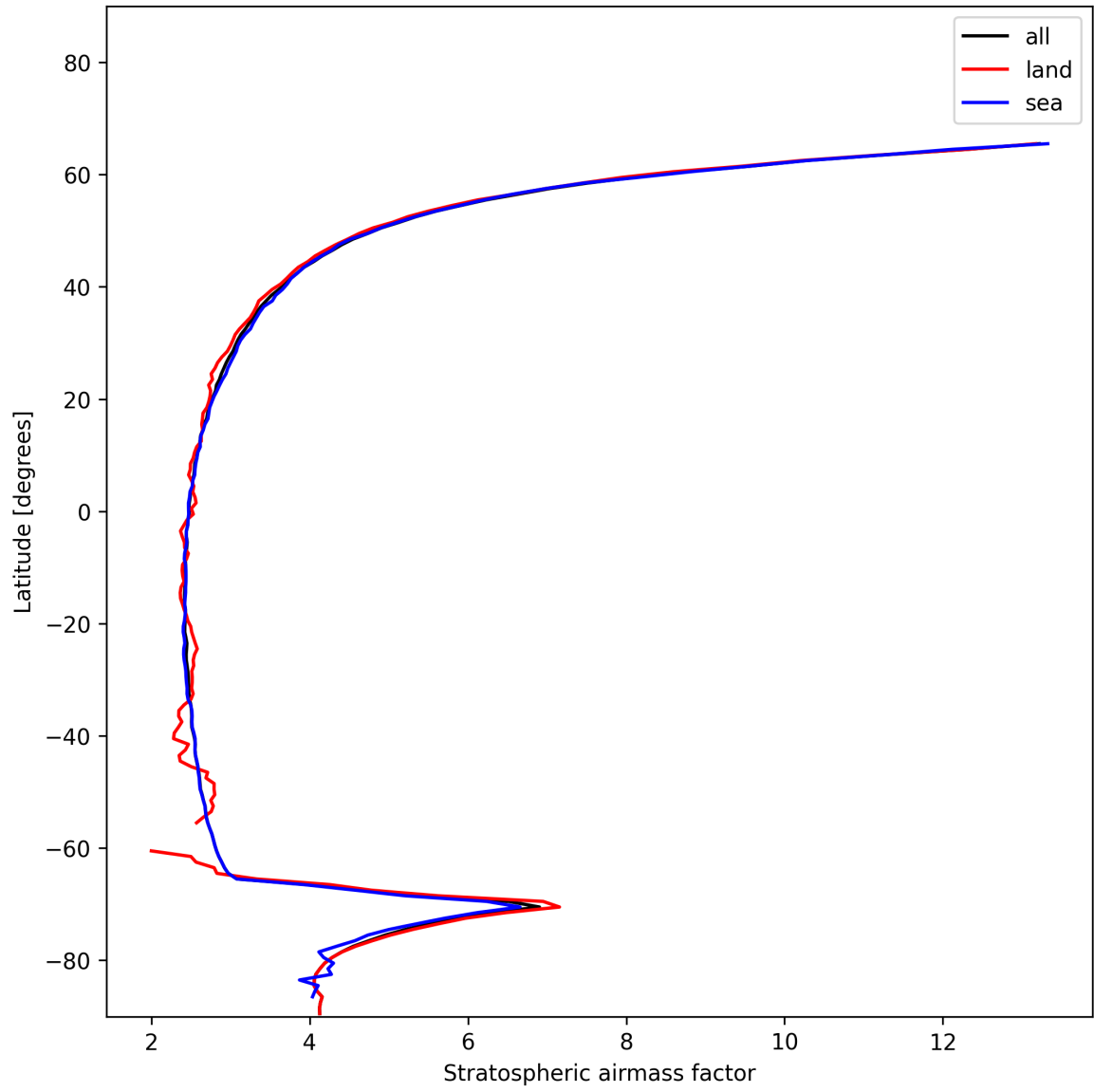
Figure 25: Zonal average of “Stratospheric air mass factor” for 2024-12-03 to 2024-12-03.
