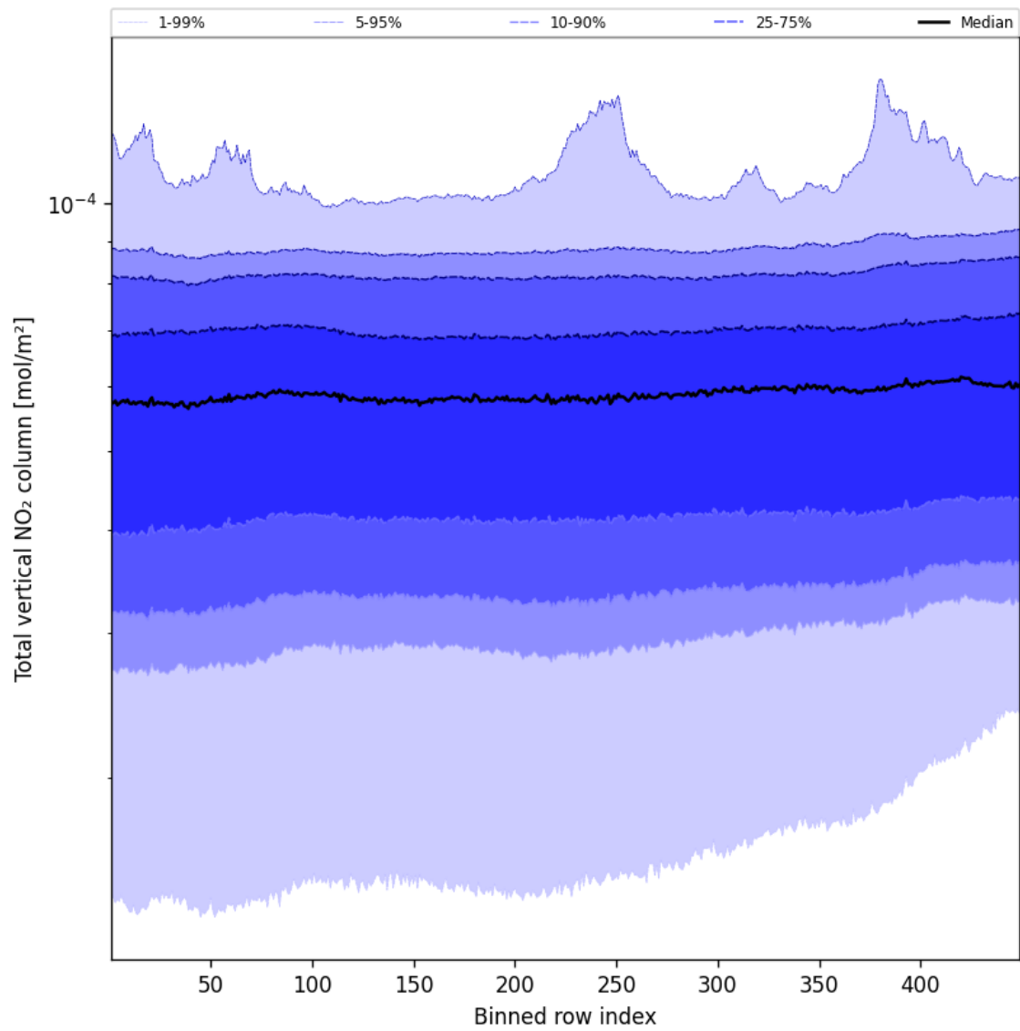
Figure 53: Along track statistics of “Total vertical NO 2 column” for 2024-12-03 to 2024-12-03
