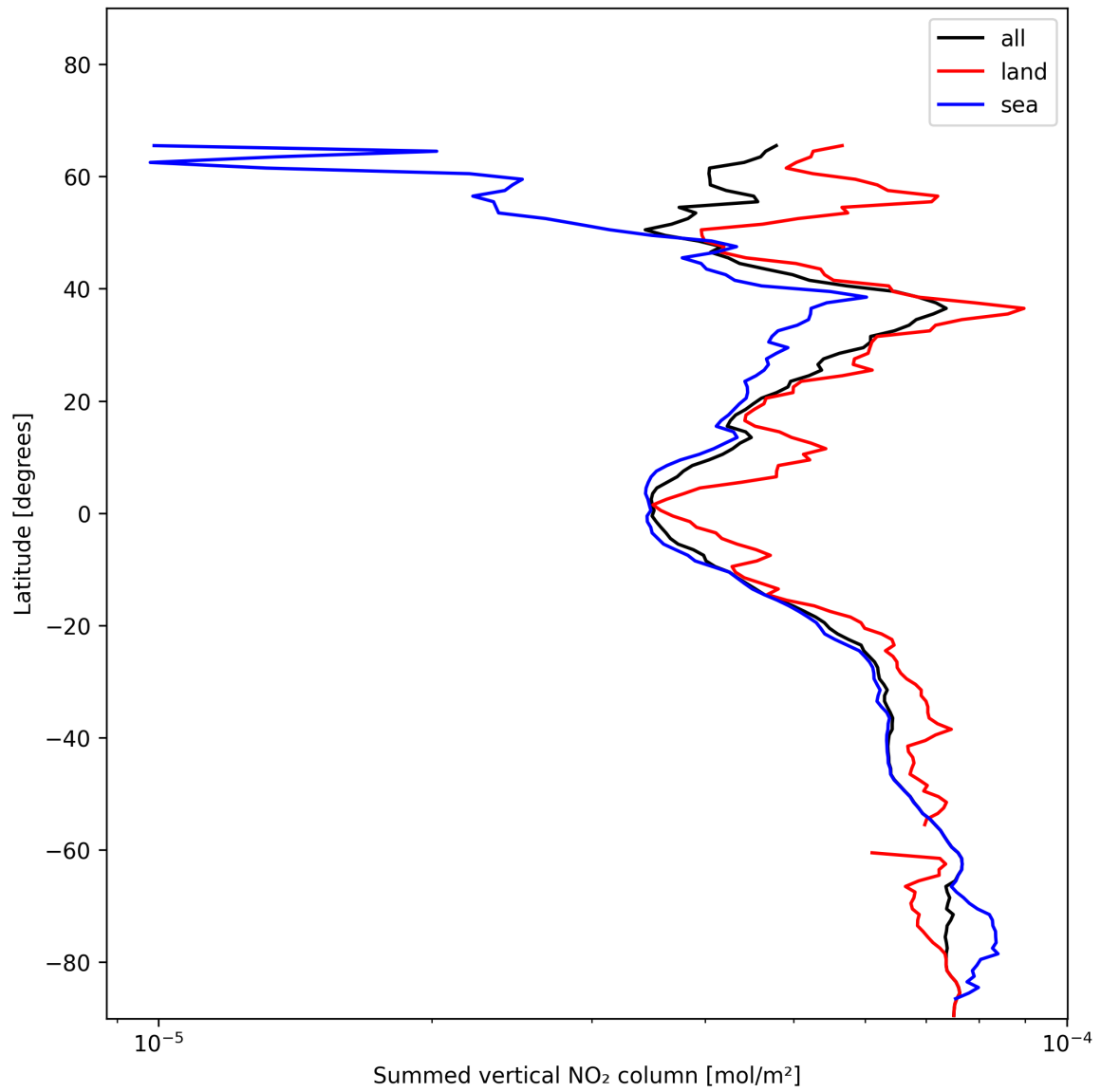
Figure 21: Zonal average of “Summed vertical NO 2 column” for 2024-12-03 to 2024-12-03.
