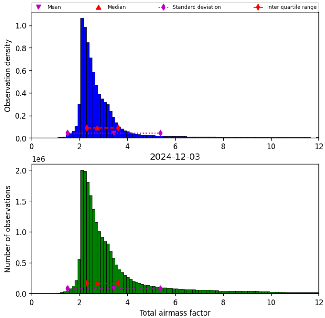
Figure 30: Histogram of “Total airmass factor” for 2024-12-03 to 2024-12-03
