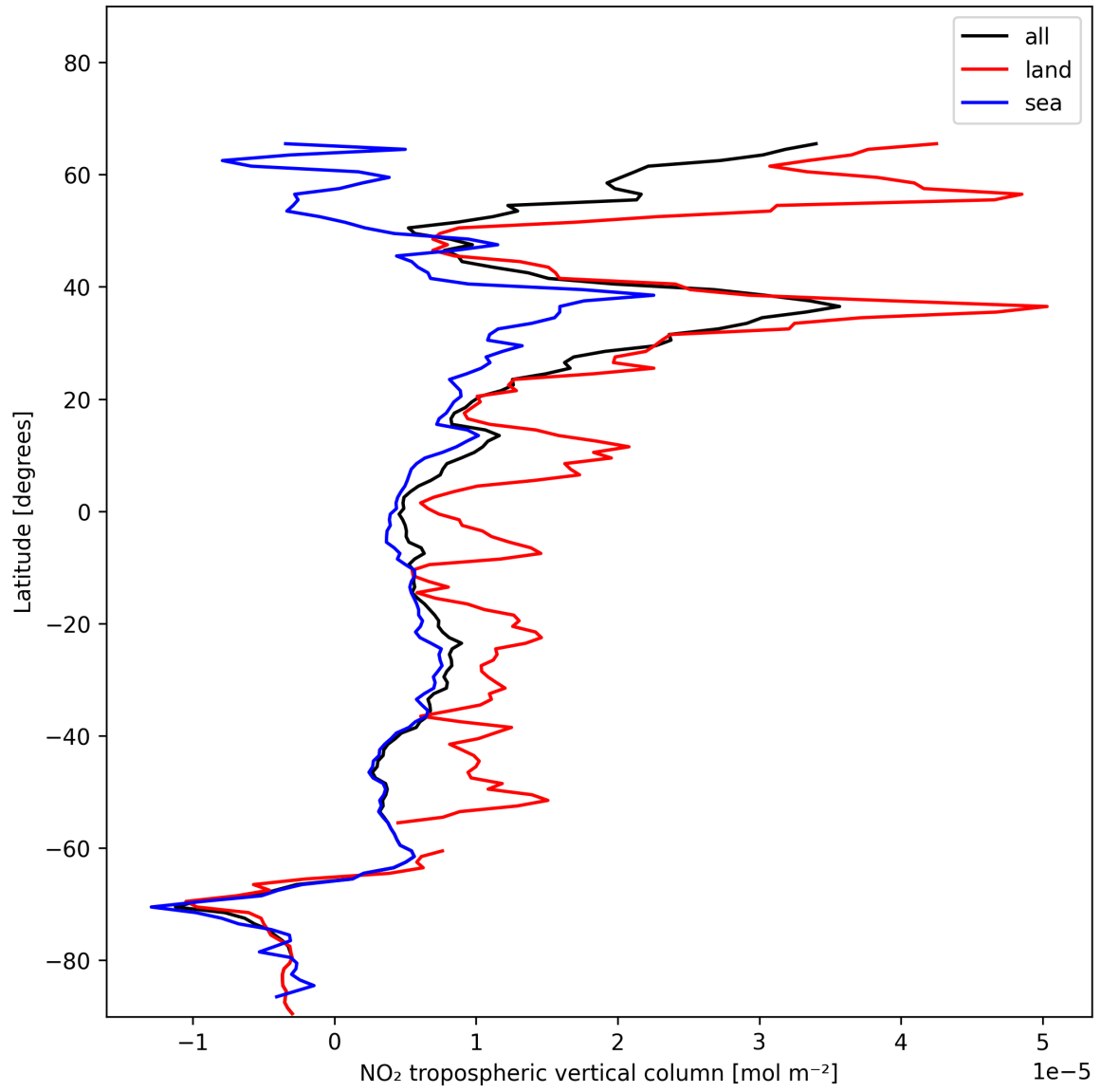
Figure 10: Zonal average of “NO 2 tropospheric vertical column” for 2024-12-03 to 2024-12-03.
