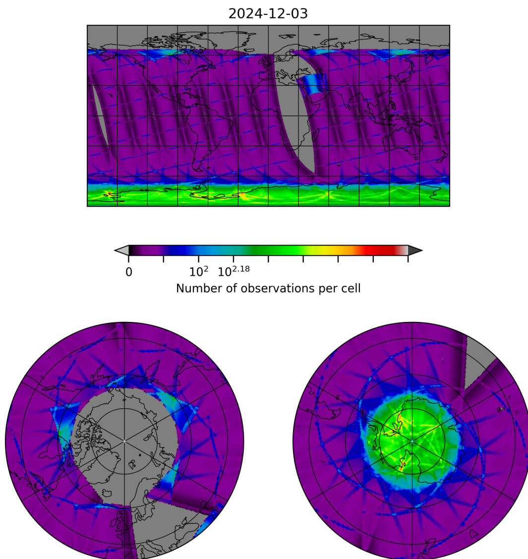
Figure 8: Map of the number of observations for 2024-12-03 to 2024-12-03
