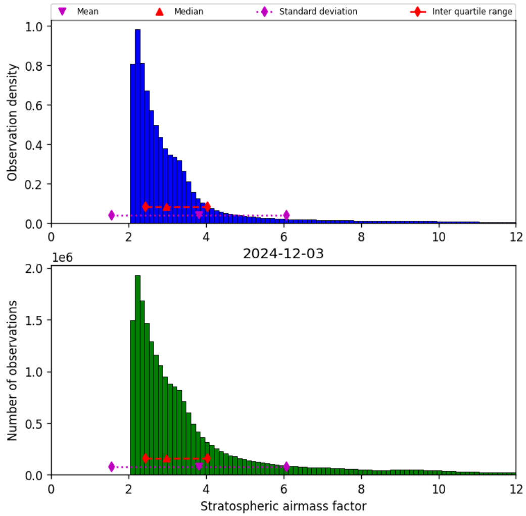
Figure 42: Histogram of “Stratospheric airmass factor” for 2024-12-03 to 2024-12-03
