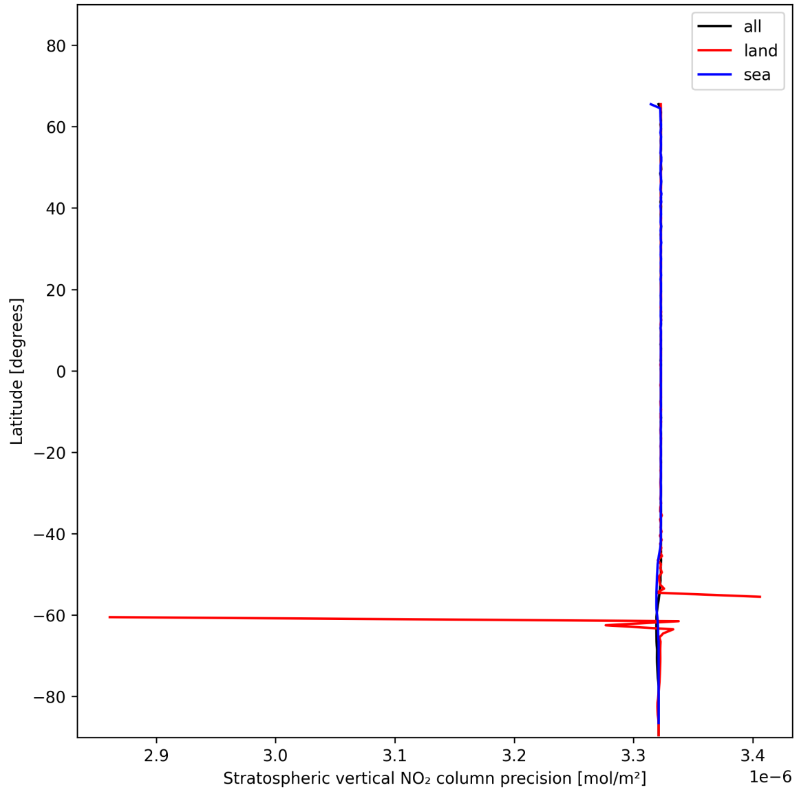
Figure 18: Zonal average of “Stratospheric vertical NO 2 column precision” for 2024-12-03 to 2024-12-03.
