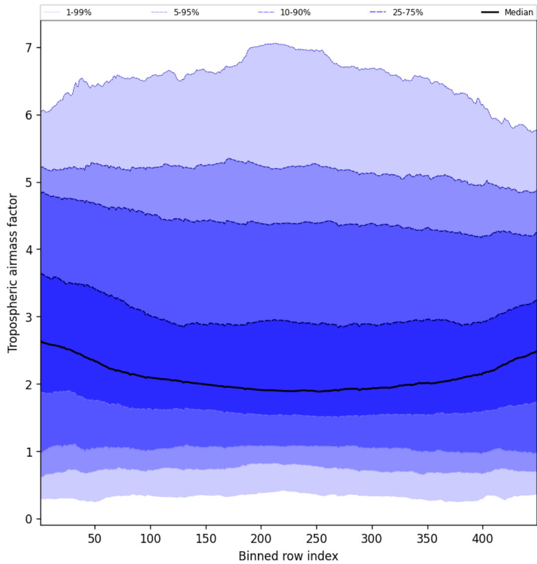
Figure 46: Along track statistics of “Tropospheric air mass factor” for 2024-12-03 to 2024-12-03
