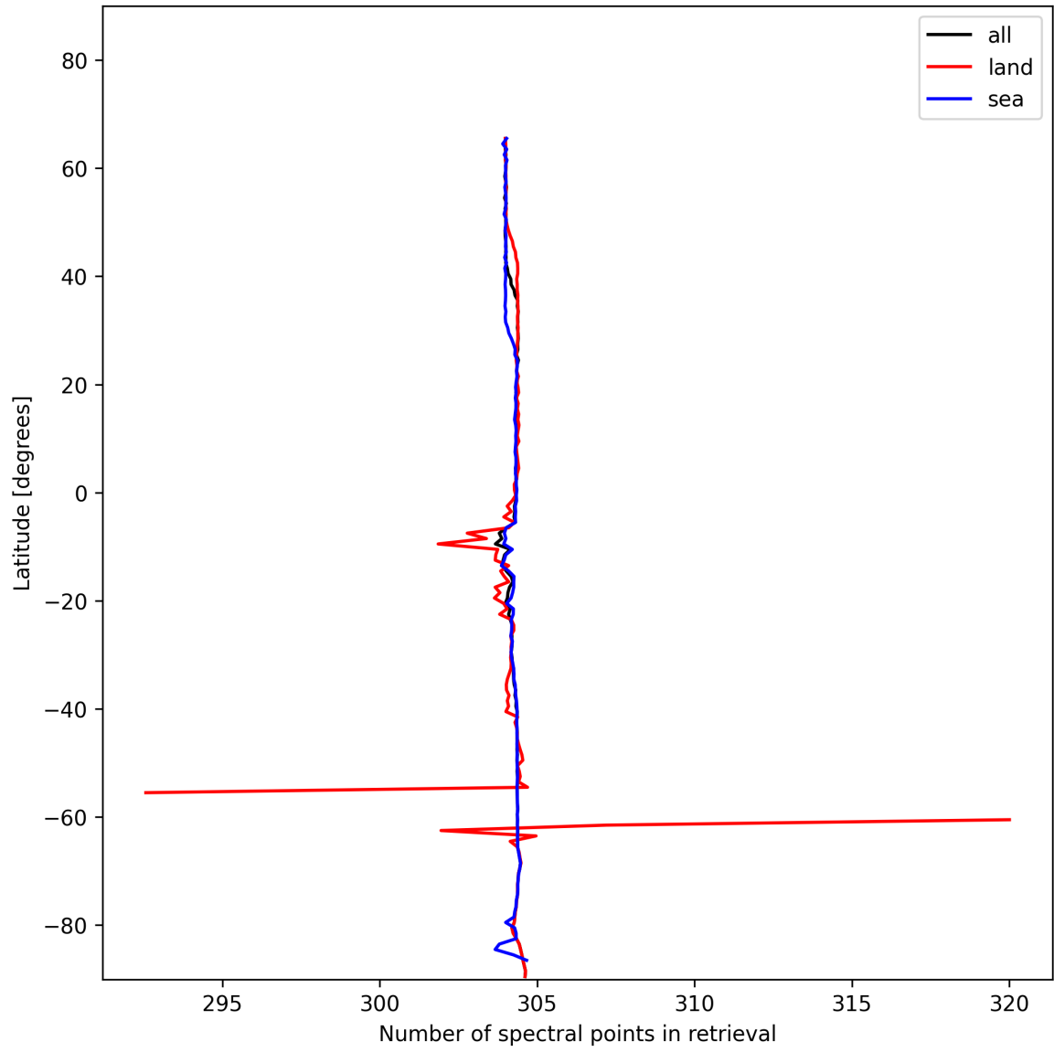
Figure 14: Zonal average of “Number of spectral points in retrieval” for 2024-12-03 to 2024-12-03.
