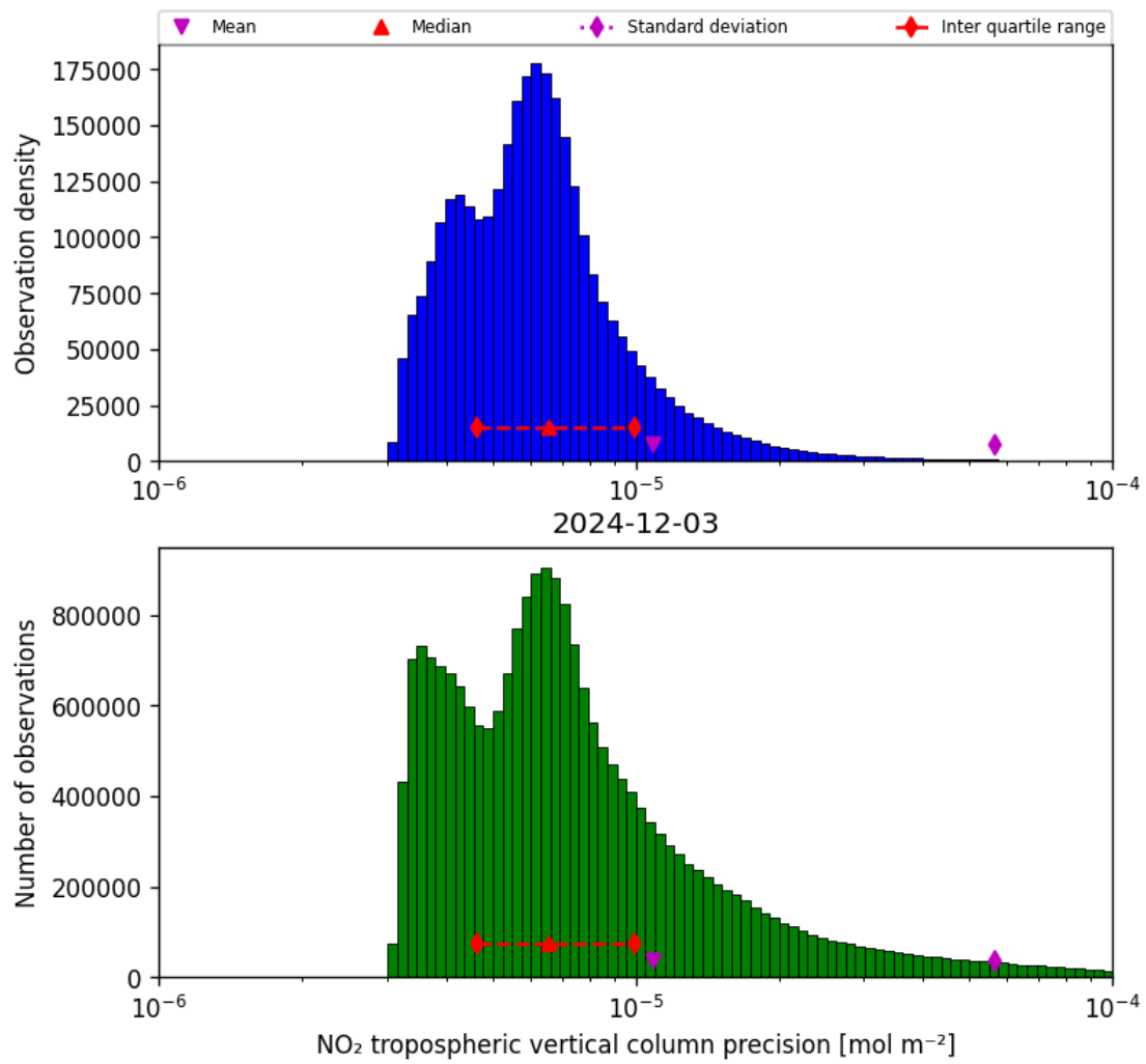
Figure 28: Histogram of “NO 2 tropospheric vertical column precision” for 2024-12-03 to 2024-12-03
