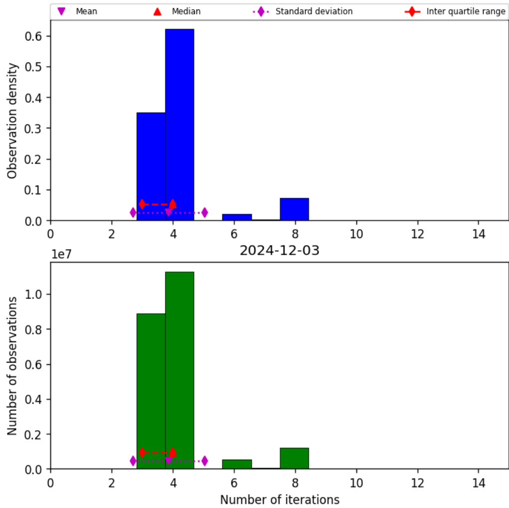
Figure 32: Histogram of “Number of iterations” for 2024-12-03 to 2024-12-03
