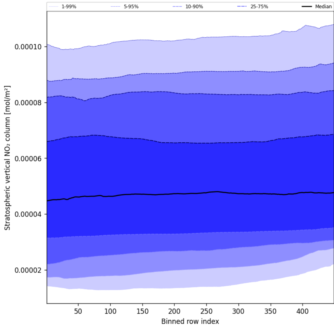
Figure 51: Along track statistics of “Stratospheric vertical NO 2 column” for 2024-12-03 to 2024-12-03
