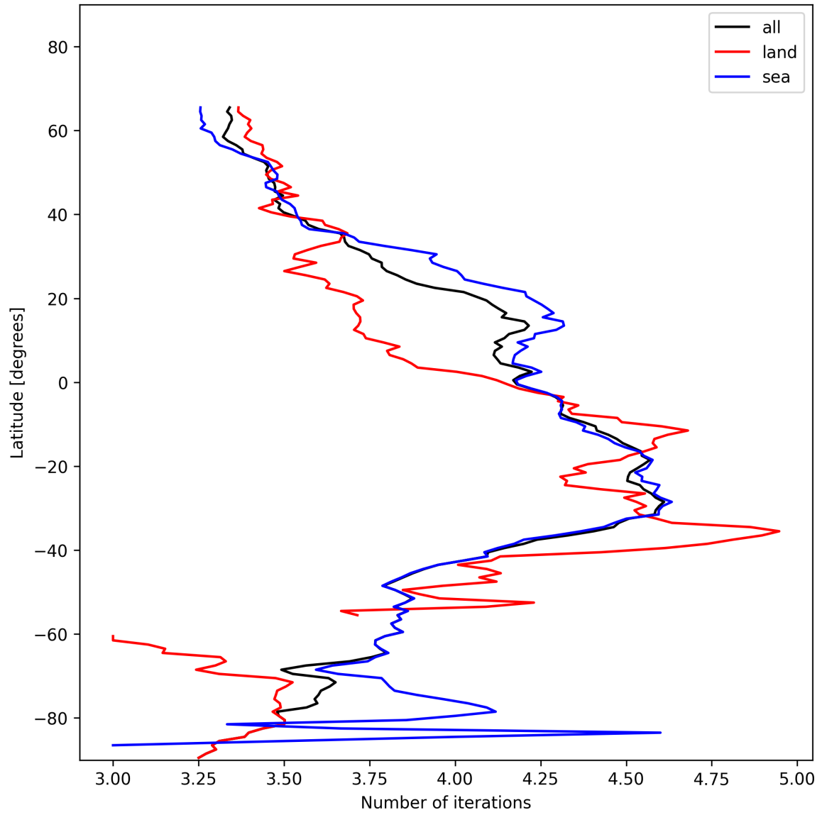
Figure 15: Zonal average of “Number of iterations” for 2024-12-03 to 2024-12-03.
