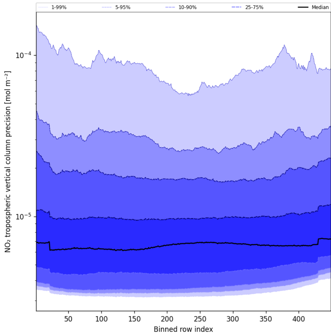
Figure 45: Along track statistics of “NO 2 tropospheric vertical column precision” for 2024-12-03 to 2024-12-03
