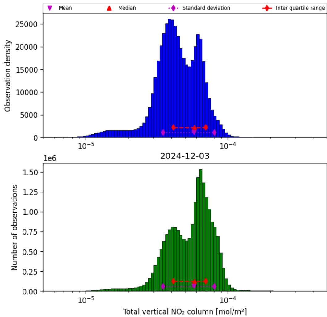
Figure 36: Histogram of "Total vertical NO 2 column" for 2024-12-03 to 2024-12-03
