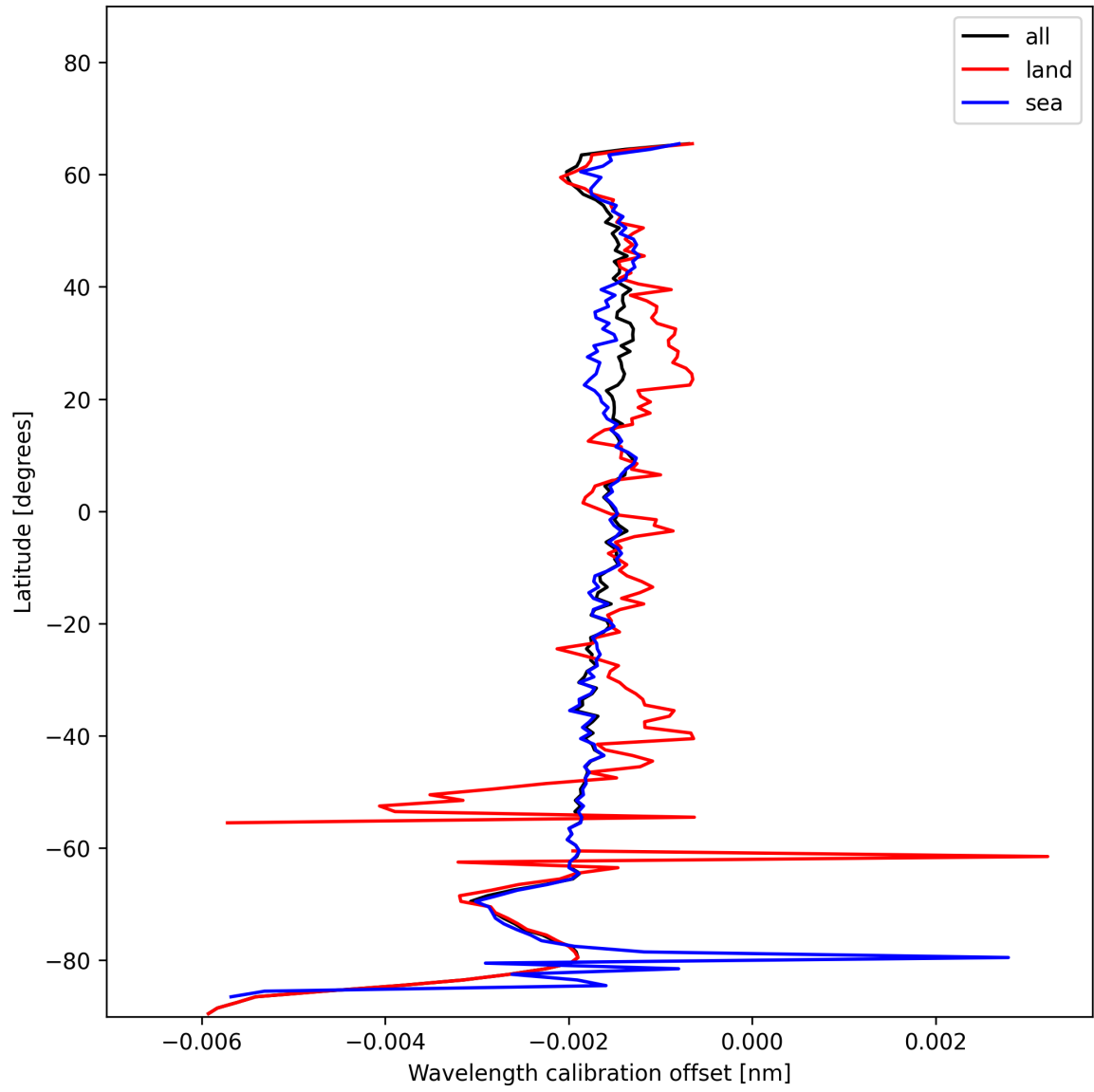
Figure 16: Zonal average of “Wavelength calibration offset” for 2024-12-03 to 2024-12-03.
