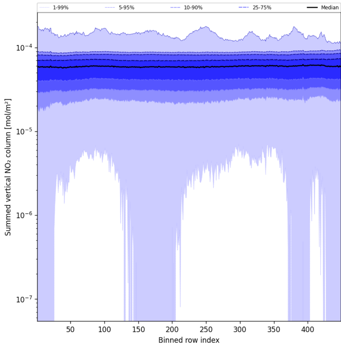
Figure 55: Along track statistics of “Summed vertical NO 2 column” for 2024-12-03 to 2024-12-03
