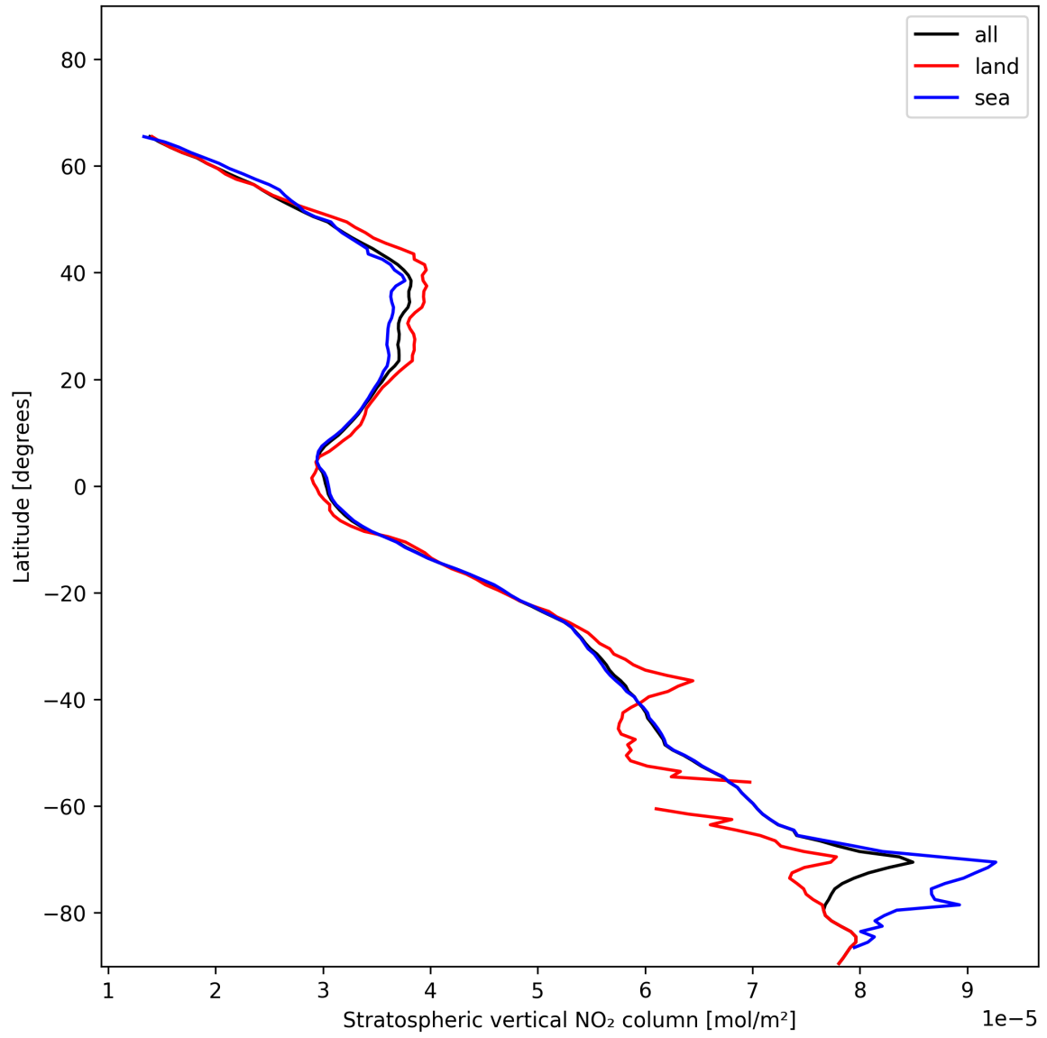
Figure 17: Zonal average of “Stratospheric vertical NO 2 column” for 2024-12-03 to 2024-12-03.
