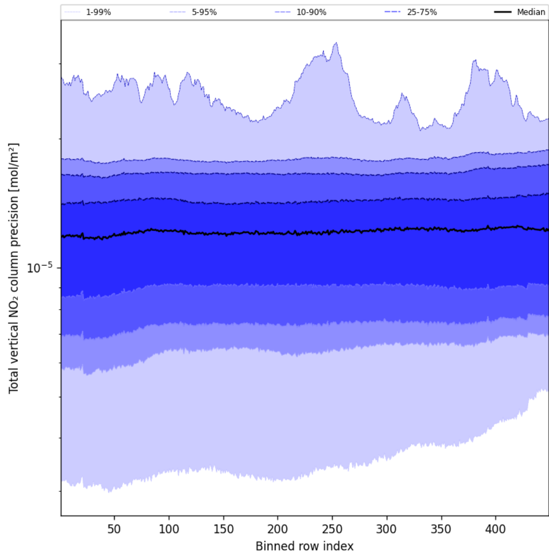
Figure 54: Along track statistics of “Total vertical NO 2 column precision” for 2024-12-03 to 2024-12-03
