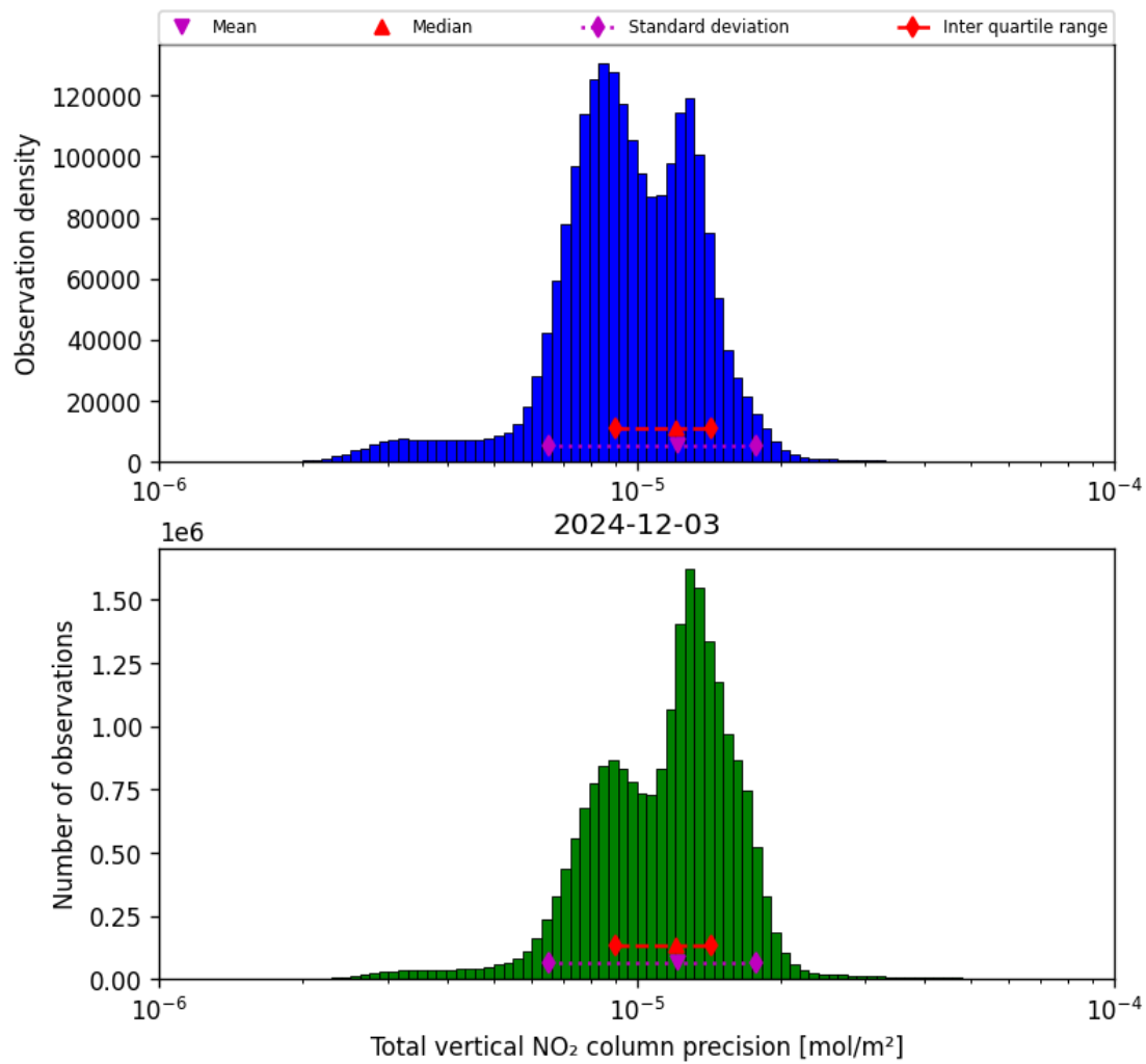
Figure 37: Histogram of “Total vertical NO 2 column precision” for 2024-12-03 to 2024-12-03
