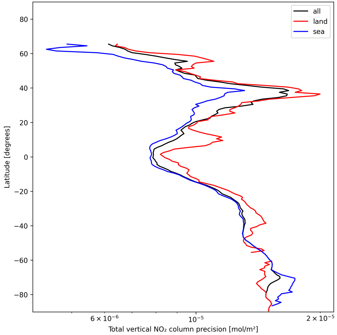
Figure 20: Zonal average of “Total vertical NO 2 column precision” for 2024-12-03 to 2024-12-03.
