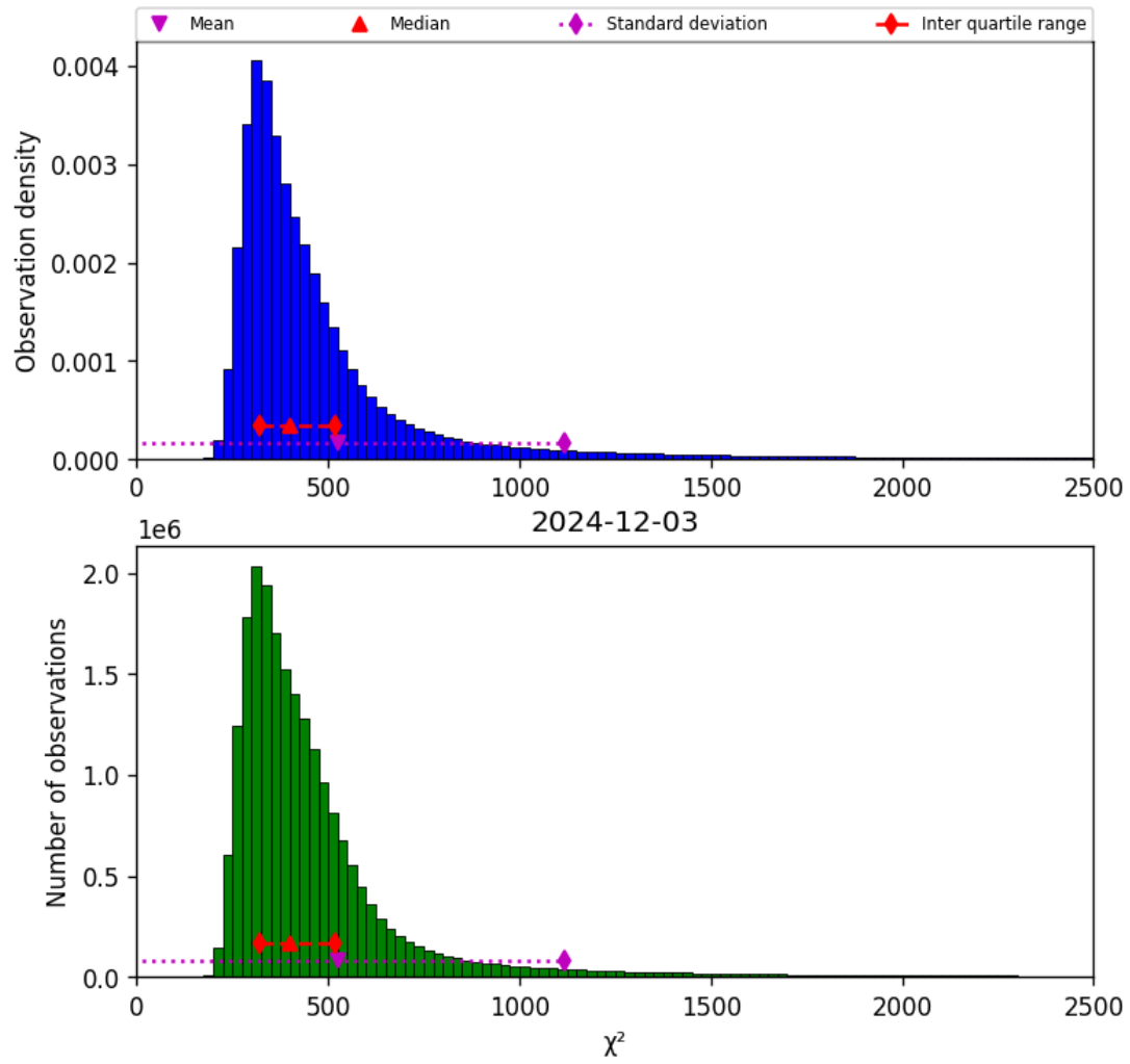
Figure 40: Histogram of “ \chi^2 ” for 2024-12-03 to 2024-12-03
