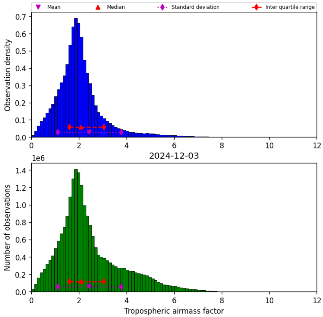
Figure 29: Histogram of “Tropospheric airmass factor” for 2024-12-03 to 2024-12-03
