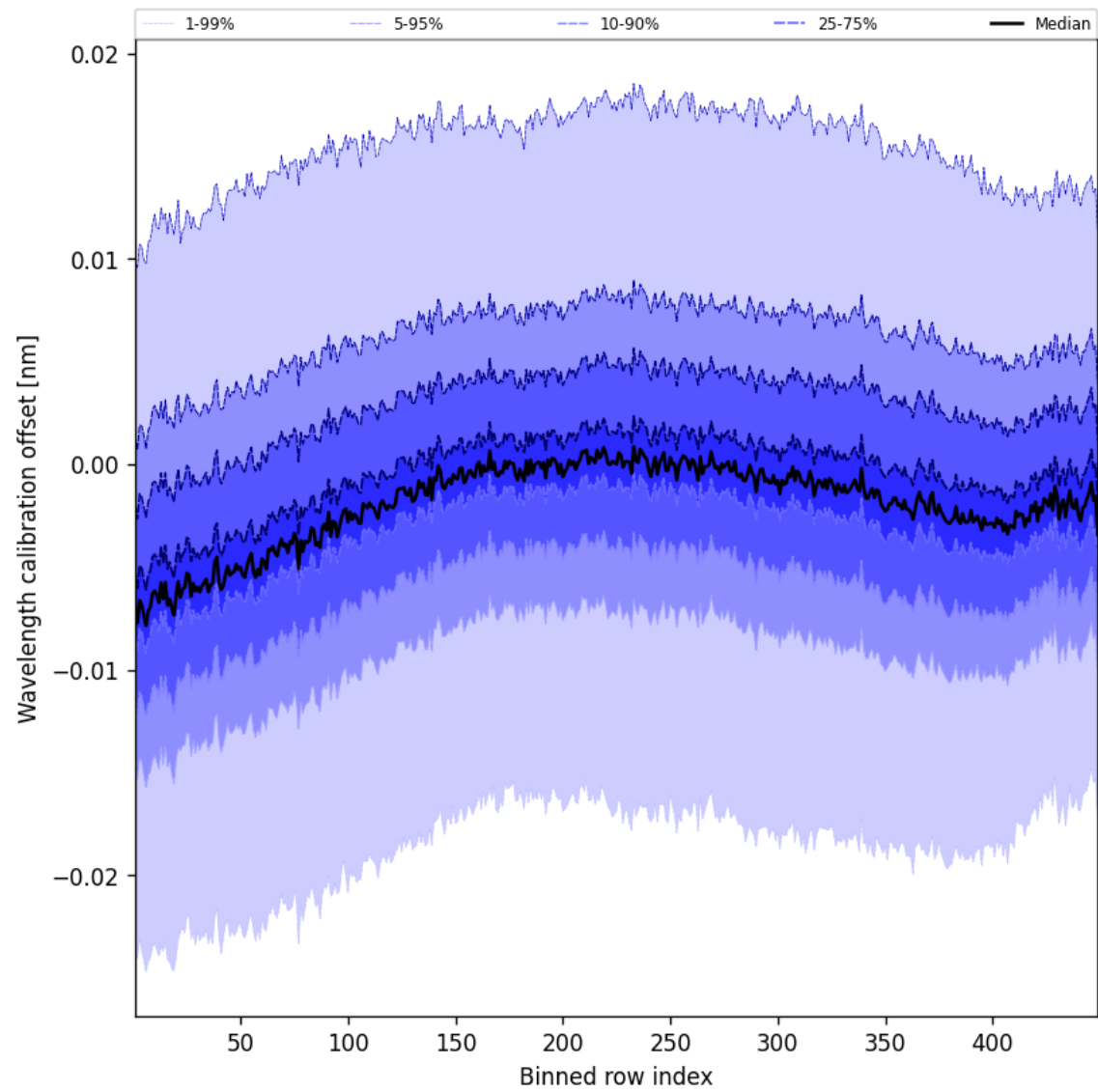
Figure 50: Along track statistics of “Wavelength calibration offset” for 2024-12-03 to 2024-12-03
