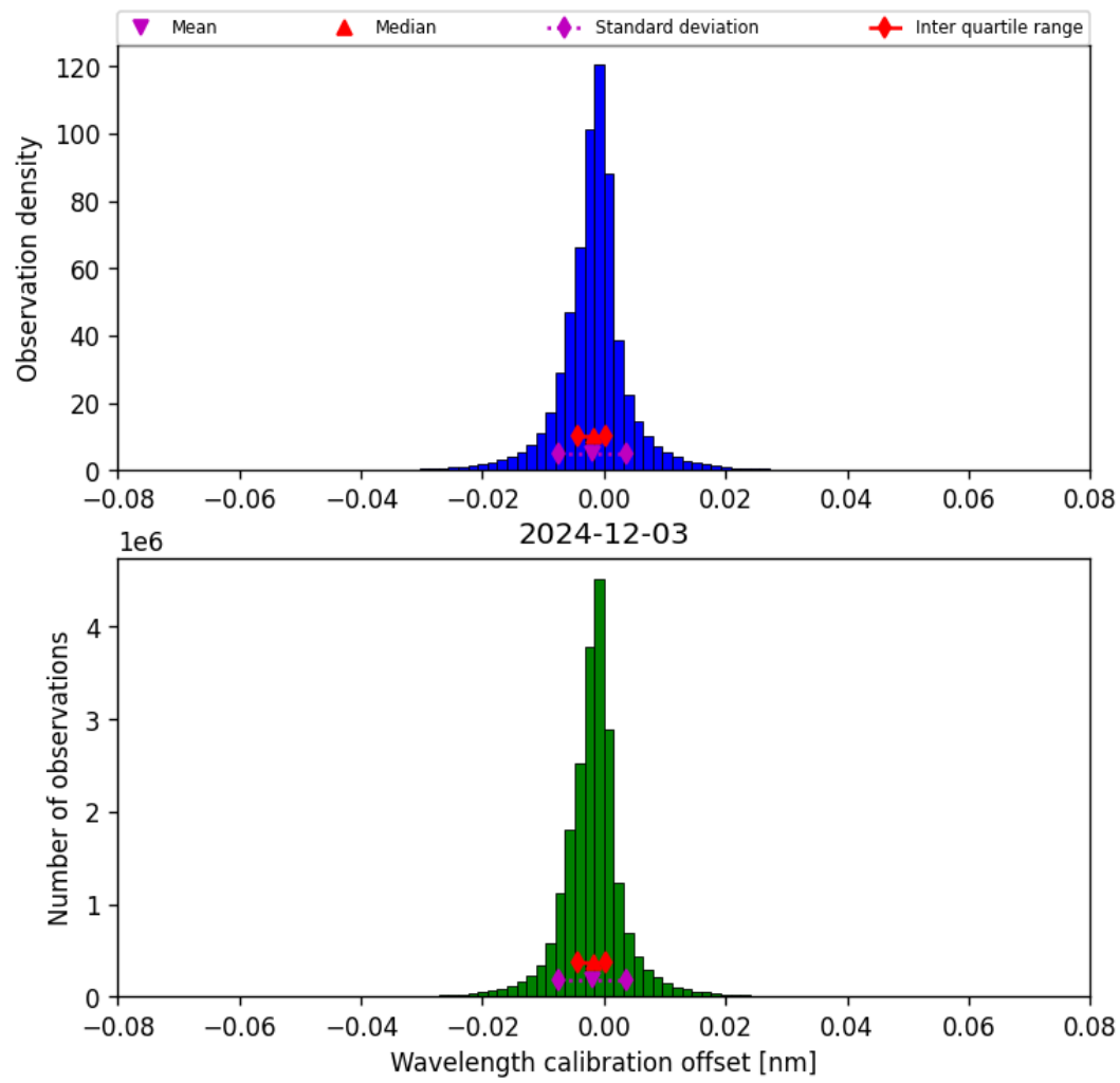
Figure 33: Histogram of “Wavelength calibration offset” for 2024-12-03 to 2024-12-03
