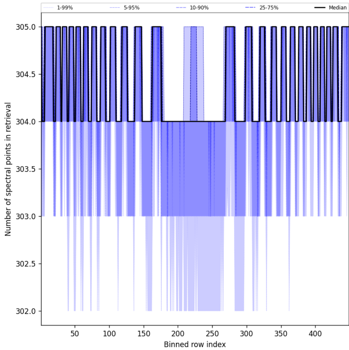
Figure 48: Along track statistics of “Number of spectral points in retrieval” for 2024-12-03 to 2024-12-03
