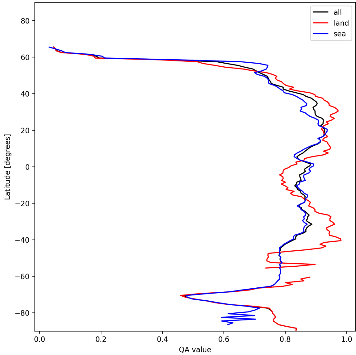
Figure 9: Zonal average of “QA value” for 2024-12-03 to 2024-12-03.
