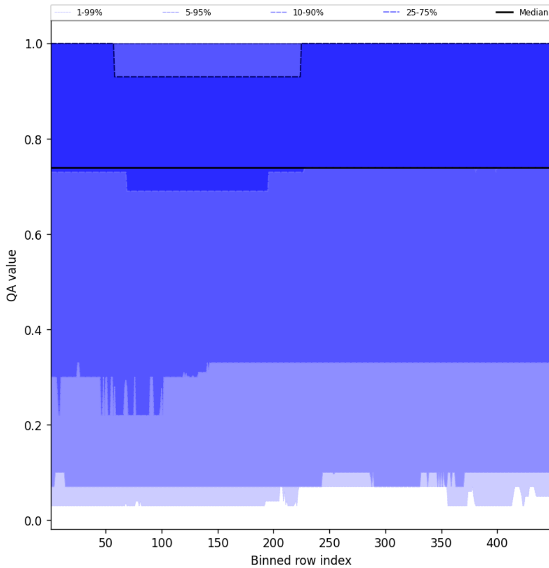
Figure 43: Along track statistics of "QA value" for 2024-12-03 to 2024-12-03
