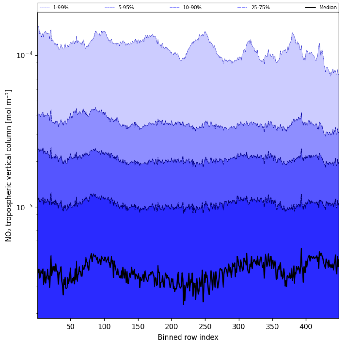
Figure 44: Along track statistics of “NO 2 tropospheric vertical column” for 2024-12-03 to 2024-12-03
