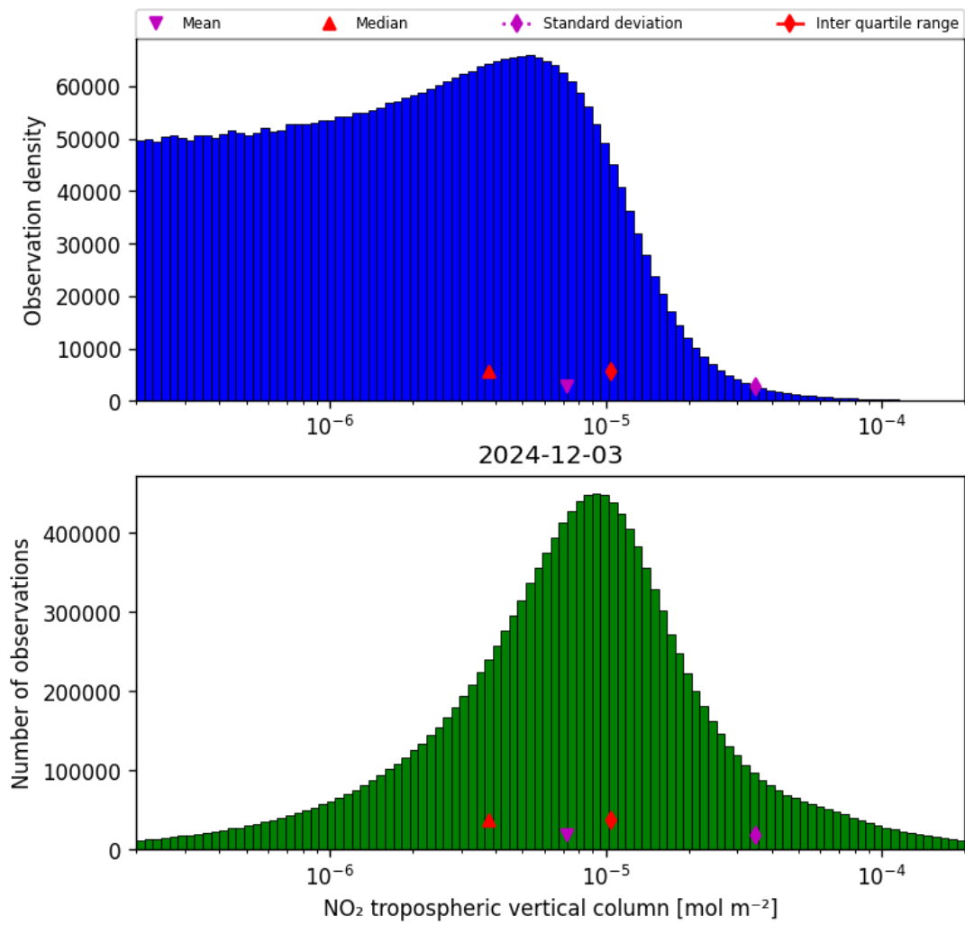
Figure 27: Histogram of “ \text{NO}_2 tropospheric vertical column” for 2024-12-03 to 2024-12-03
