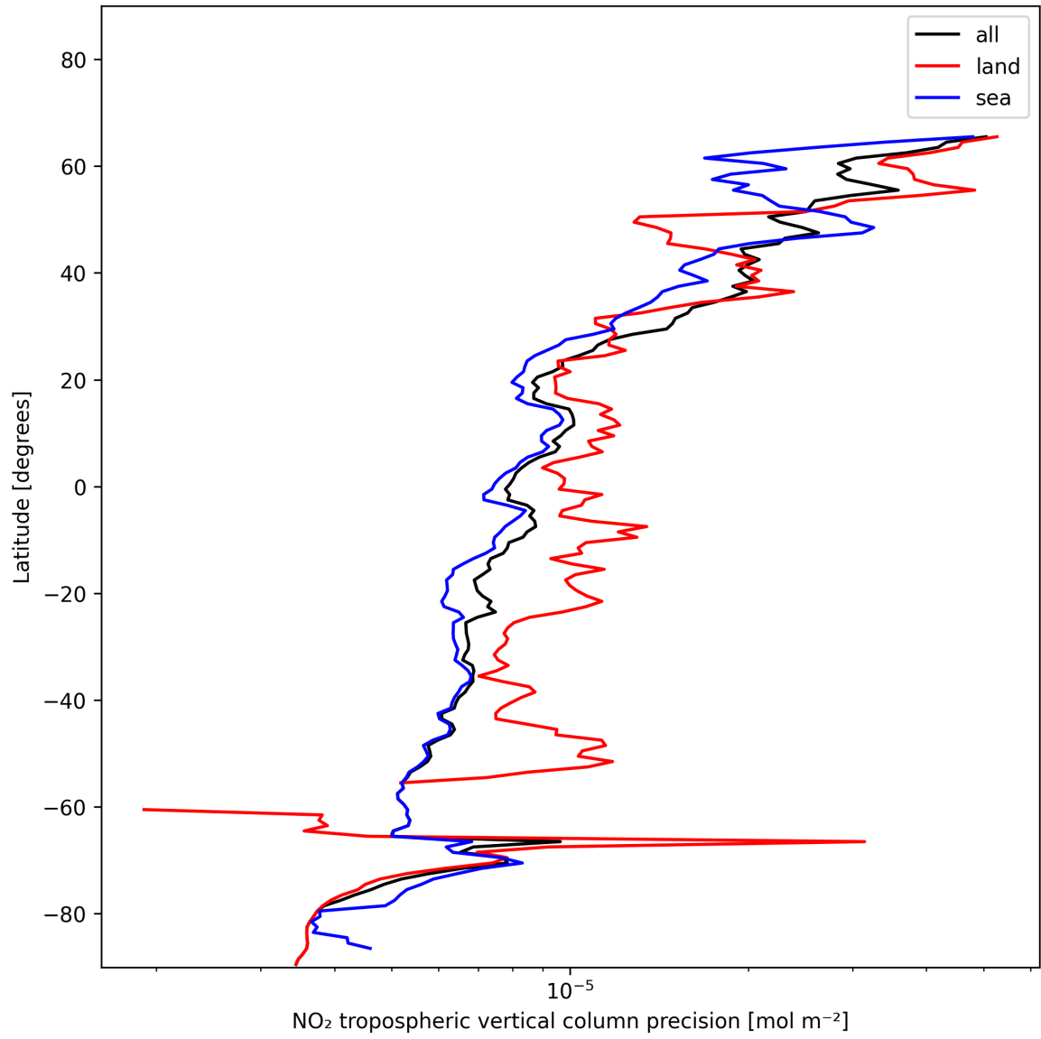
Figure 11: Zonal average of “NO 2 tropospheric vertical column precision” for 2024-12-03 to 2024-12-03.
