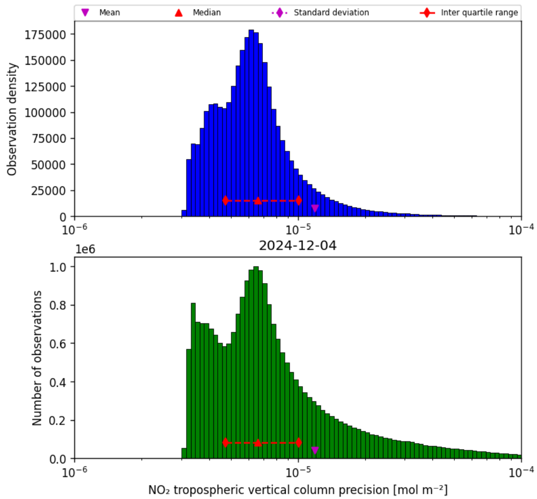
Figure 28: Histogram of “NO 2 tropospheric vertical column precision” for 2024-12-04 to 2024-12-04
