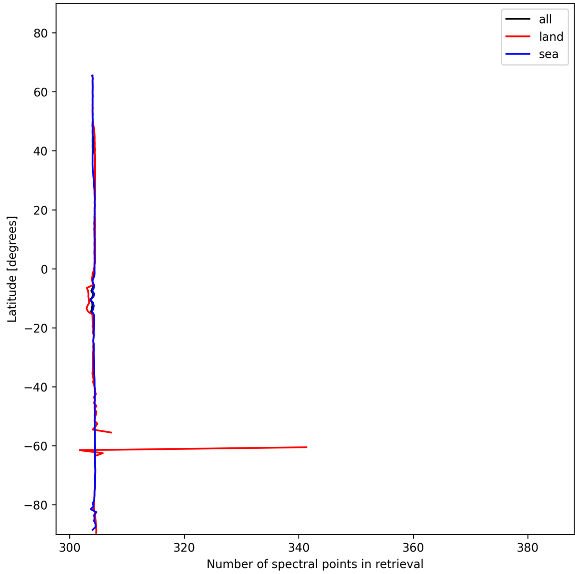
Figure 14: Zonal average of “Number of spectral points in retrieval” for 2024-12-04 to 2024-12-04.
