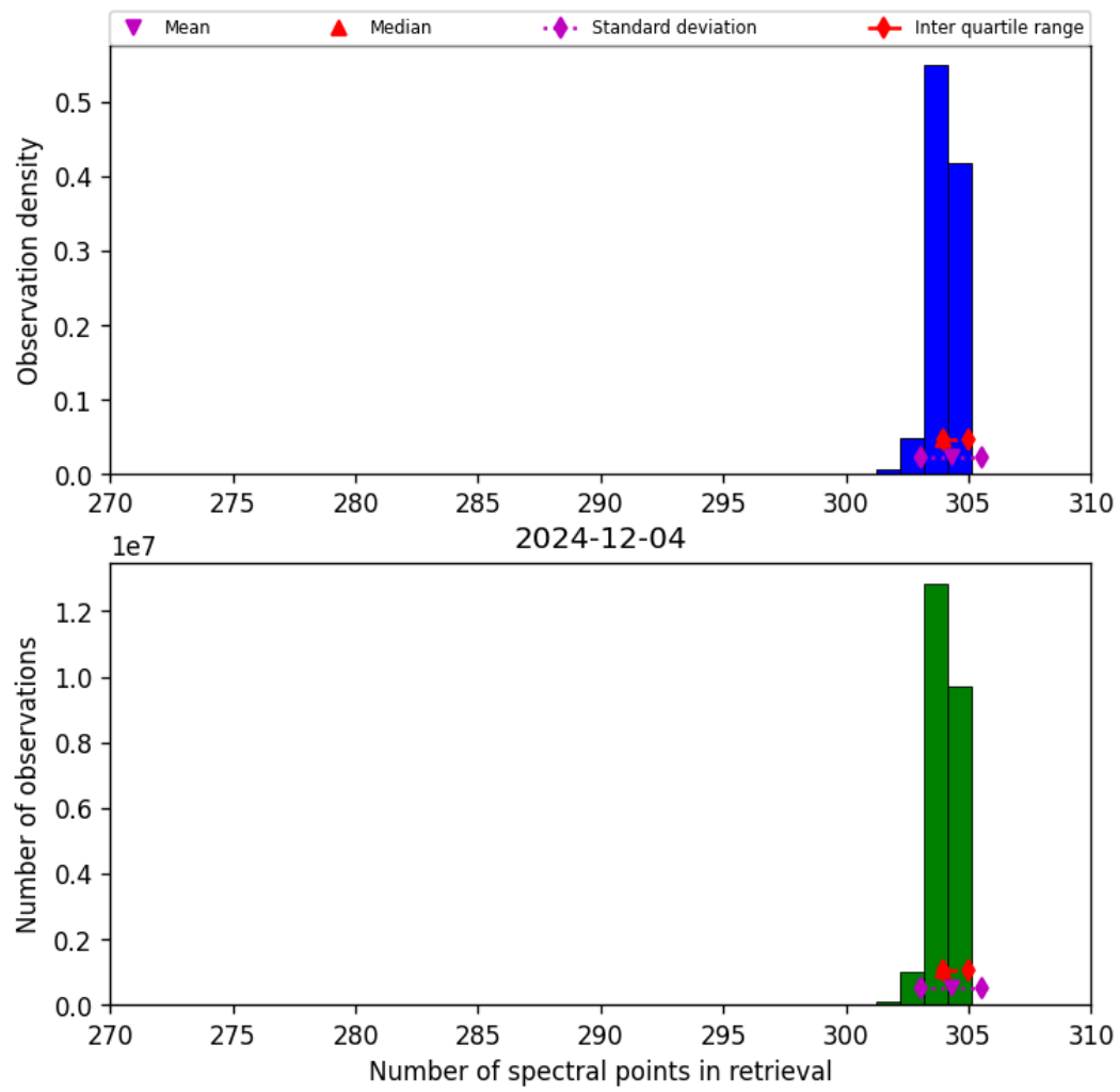
Figure 31: Histogram of “Number of spectral points in retrieval” for 2024-12-04 to 2024-12-04
