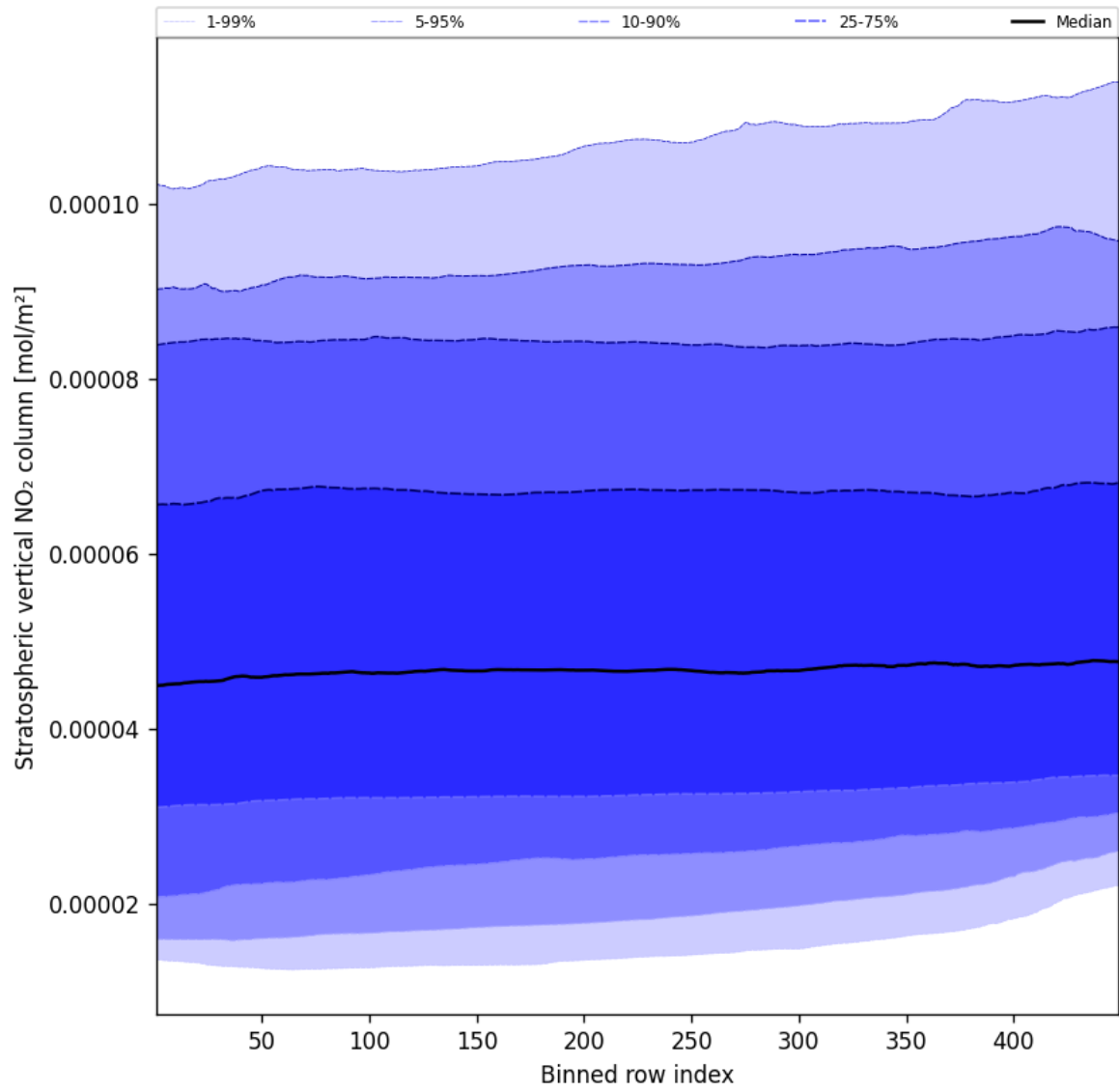
Figure 51: Along track statistics of “Stratospheric vertical NO 2 column” for 2024-12-04 to 2024-12-04
