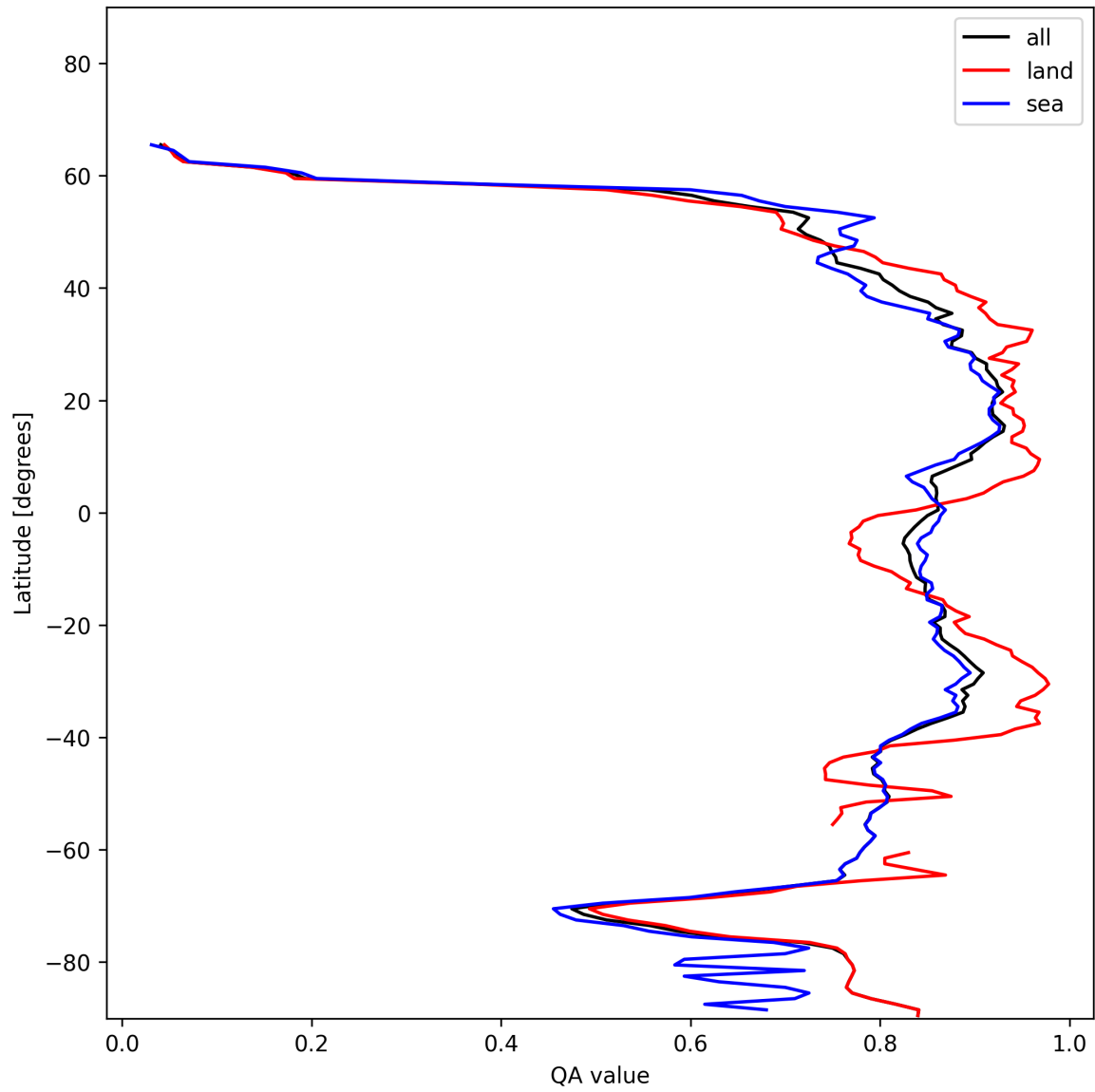
Figure 9: Zonal average of “QA value” for 2024-12-04 to 2024-12-04.
