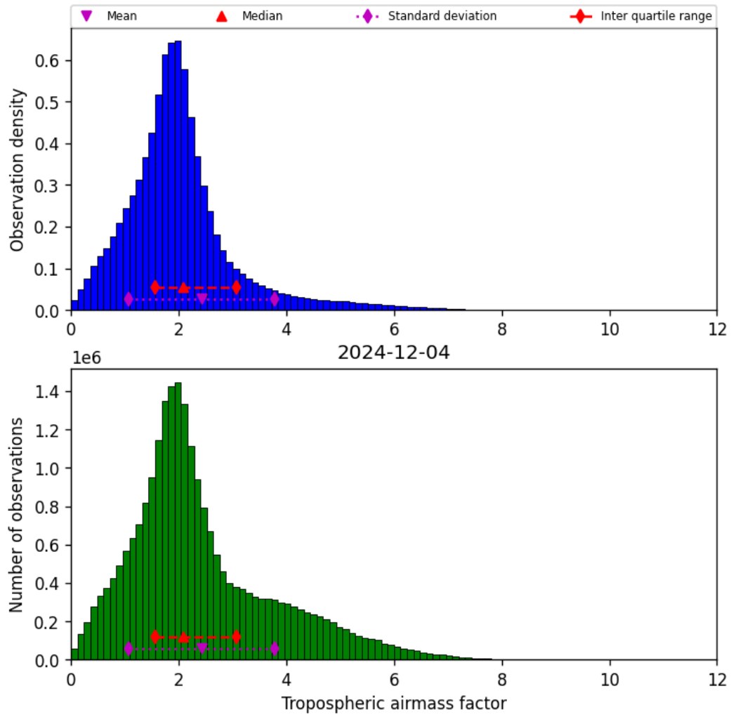
Figure 29: Histogram of “Tropospheric airmass factor” for 2024-12-04 to 2024-12-04
