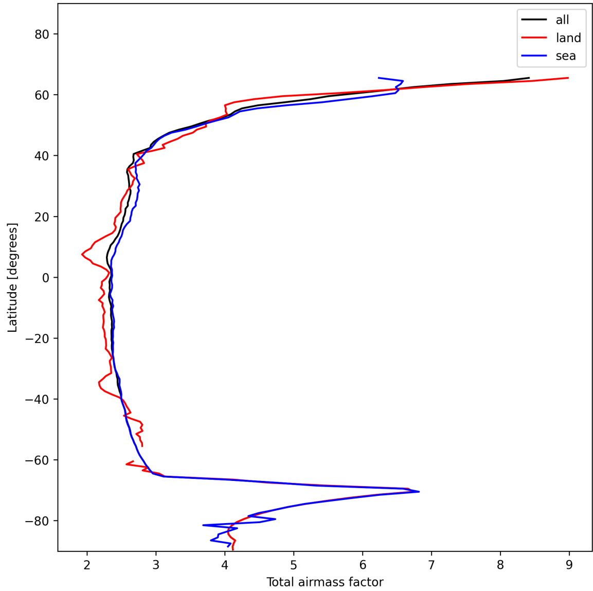
Figure 13: Zonal average of “Total airmass factor” for 2024-12-04 to 2024-12-04.
