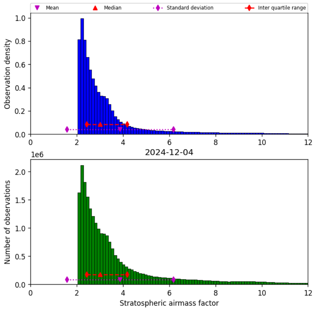
Figure 42: Histogram of “Stratospheric airmass factor” for 2024-12-04 to 2024-12-04
