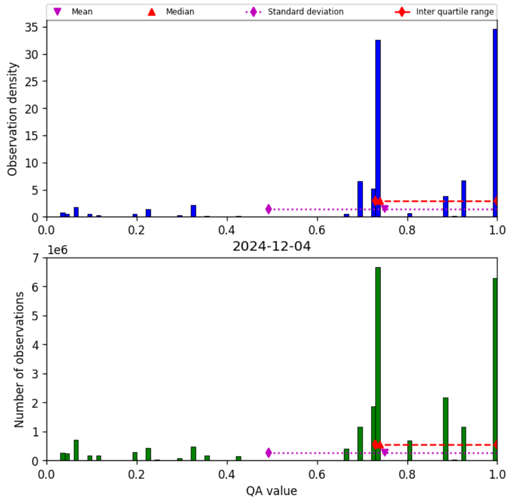
Figure 26: Histogram of “QA value” for 2024-12-04 to 2024-12-04
