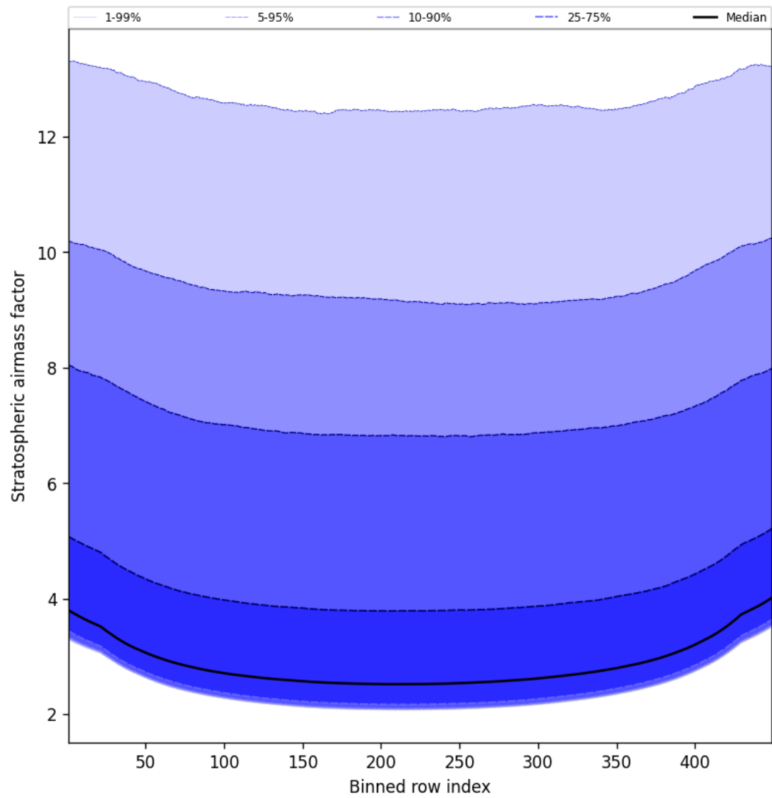
Figure 59: Along track statistics of “Stratospheric airmass factor” for 2024-12-04 to 2024-12-04
