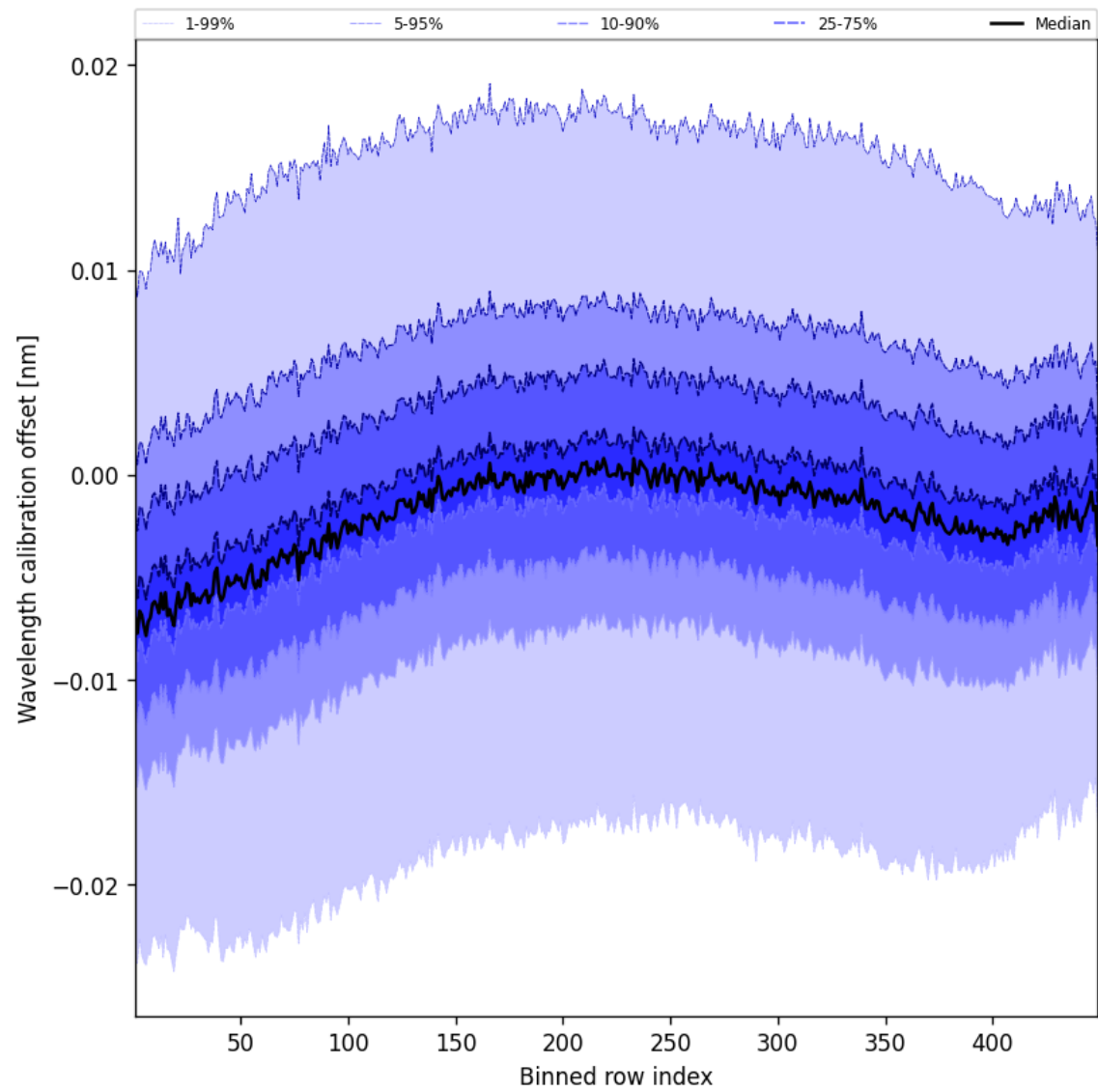
Figure 50: Along track statistics of “Wavelength calibration offset” for 2024-12-04 to 2024-12-04
