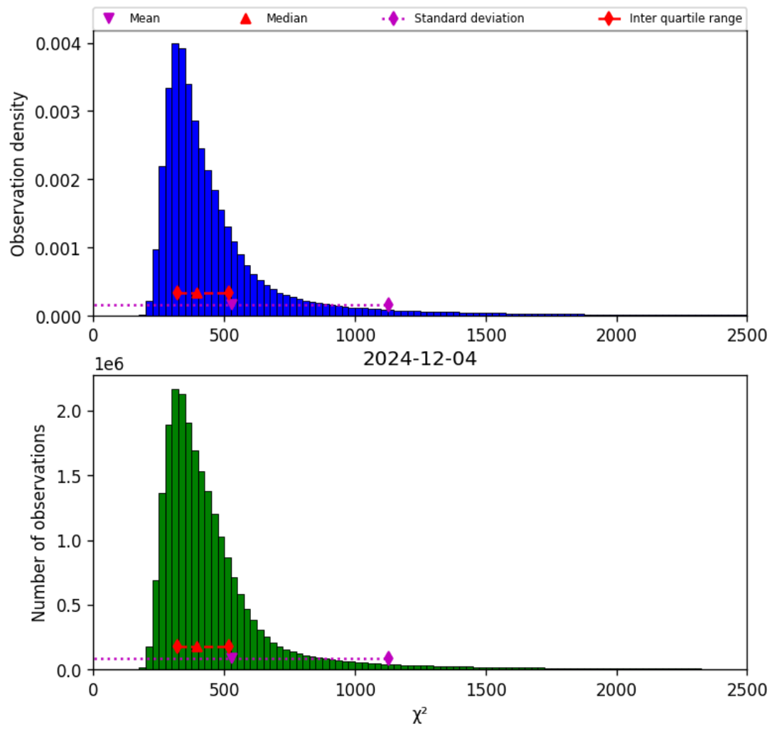
Figure 40: Histogram of " \chi^2 " for 2024-12-04 to 2024-12-04
