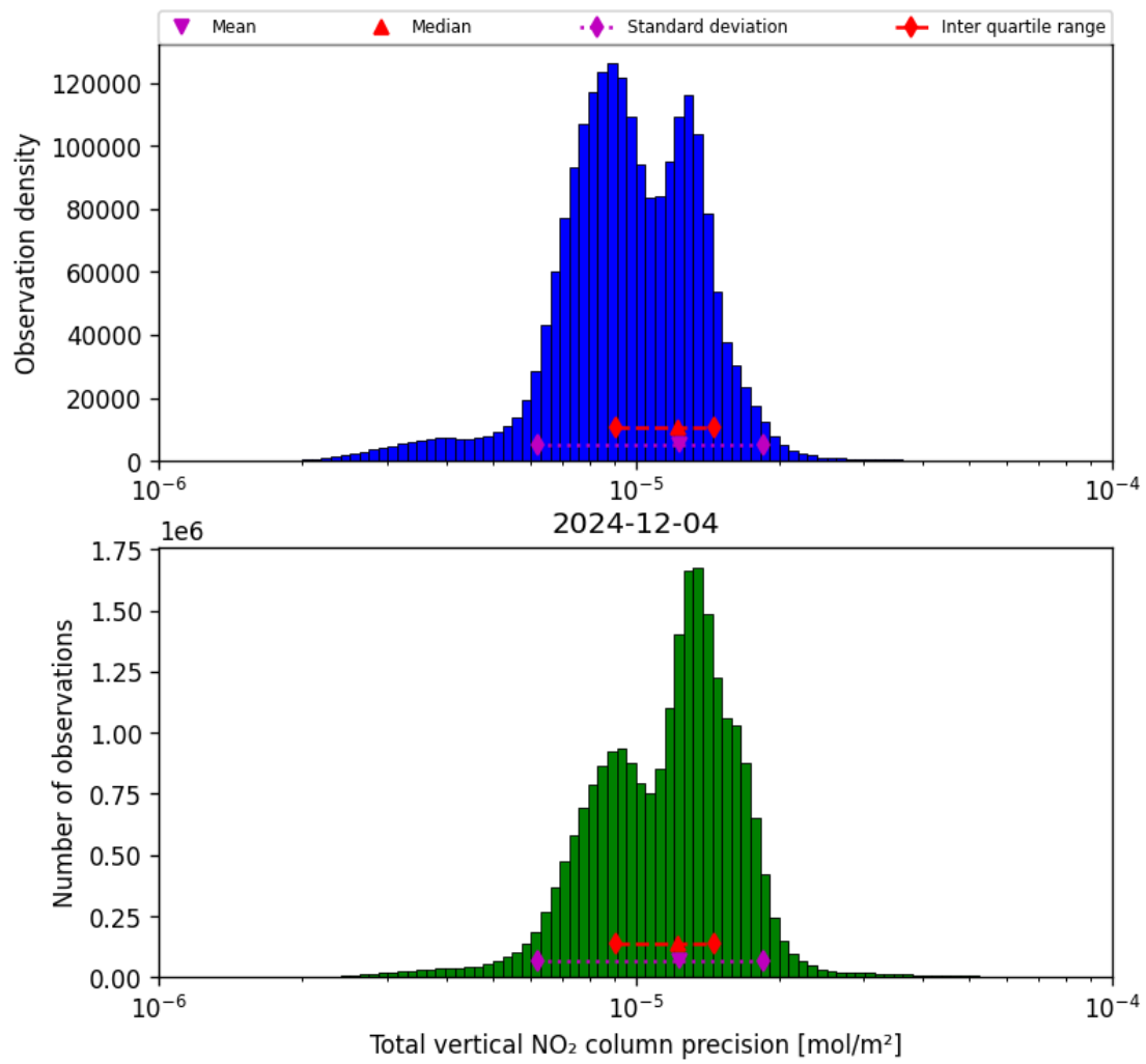
Figure 37: Histogram of “Total vertical NO 2 column precision” for 2024-12-04 to 2024-12-04
