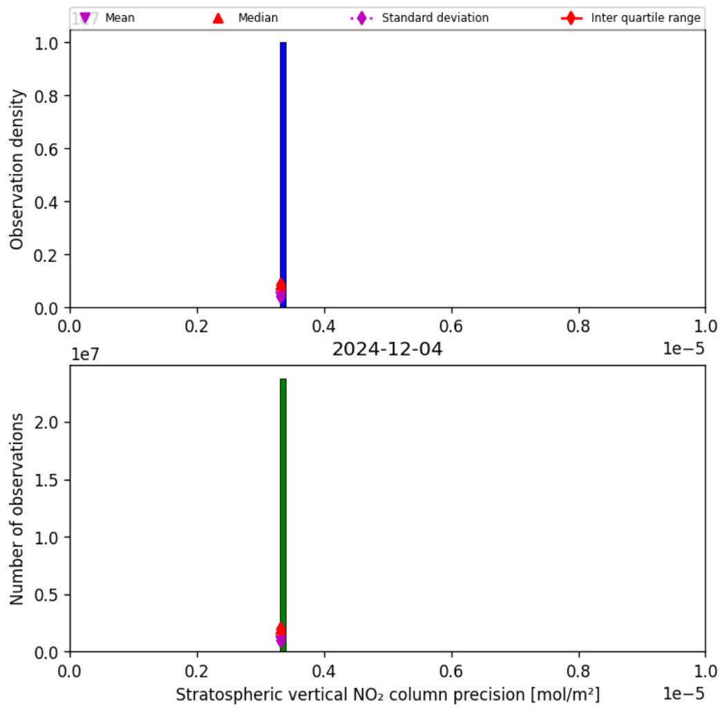
Figure 35: Histogram of “Stratospheric vertical NO 2 column precision” for 2024-12-04 to 2024-12-04
