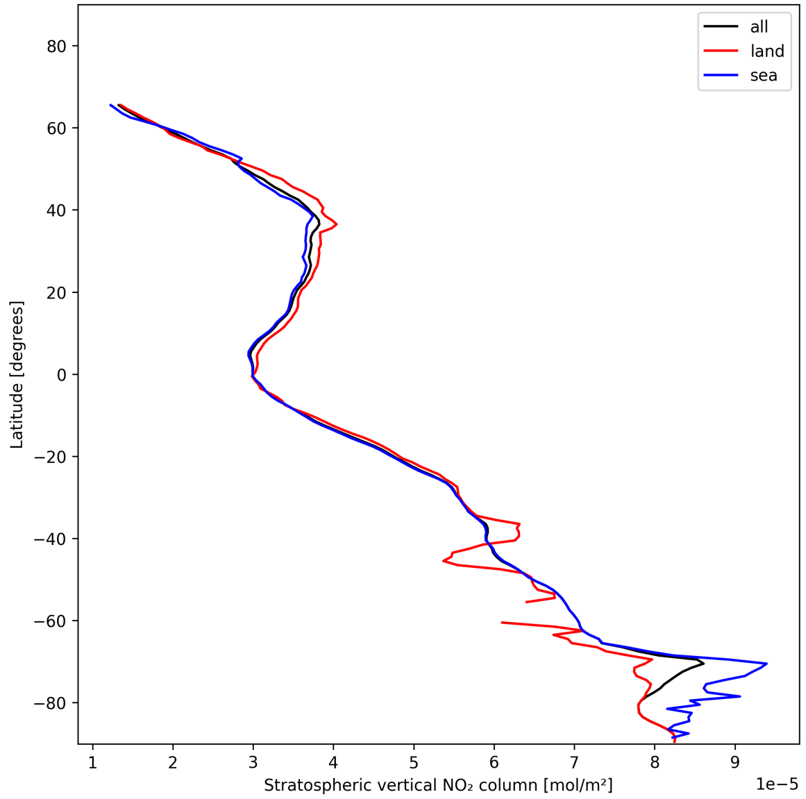
Figure 17: Zonal average of “Stratospheric vertical NO 2 column” for 2024-12-04 to 2024-12-04.
