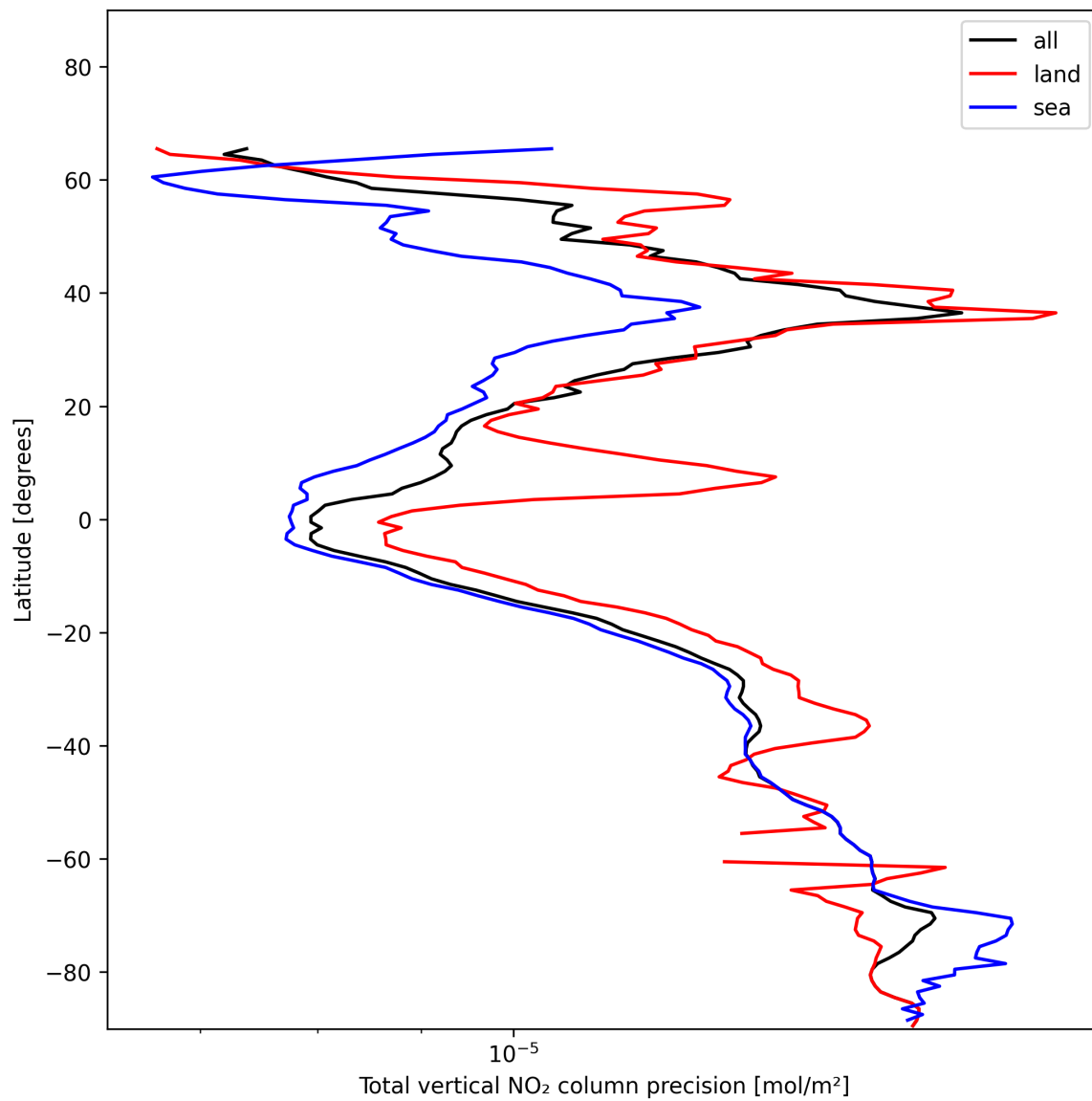
Figure 20: Zonal average of “Total vertical NO 2 column precision” for 2024-12-04 to 2024-12-04.
