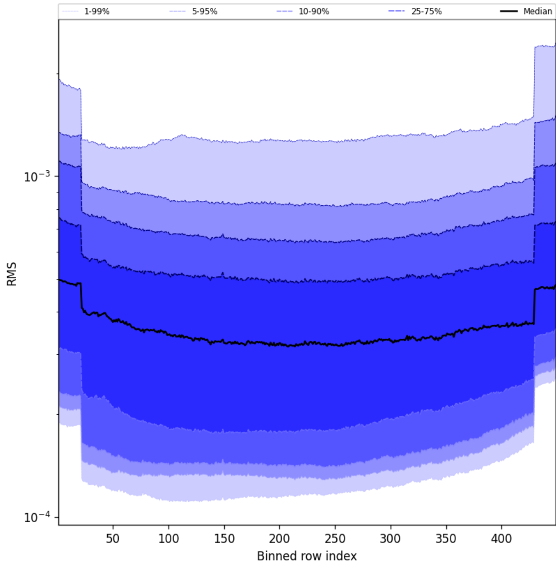
Figure 58: Along track statistics of “RMS” for 2024-12-04 to 2024-12-04
