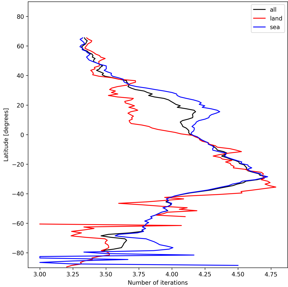
Figure 15: Zonal average of “Number of iterations” for 2024-12-04 to 2024-12-04.
