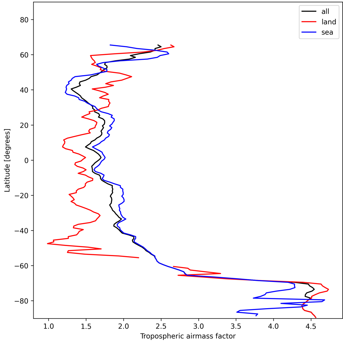
Figure 12: Zonal average of “Tropospheric air mass factor” for 2024-12-04 to 2024-12-04.
