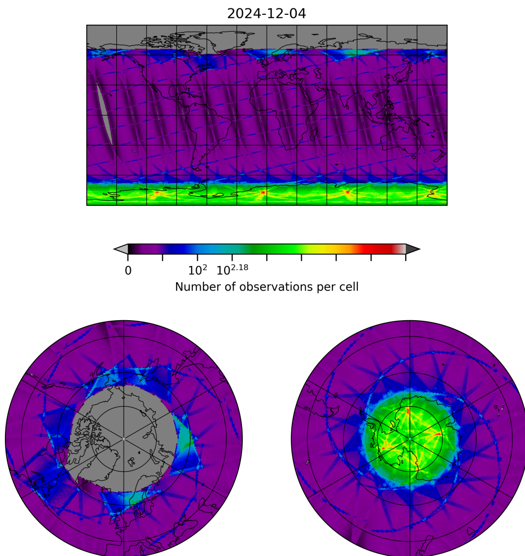
Figure 8: Map of the number of observations for 2024-12-04 to 2024-12-04
