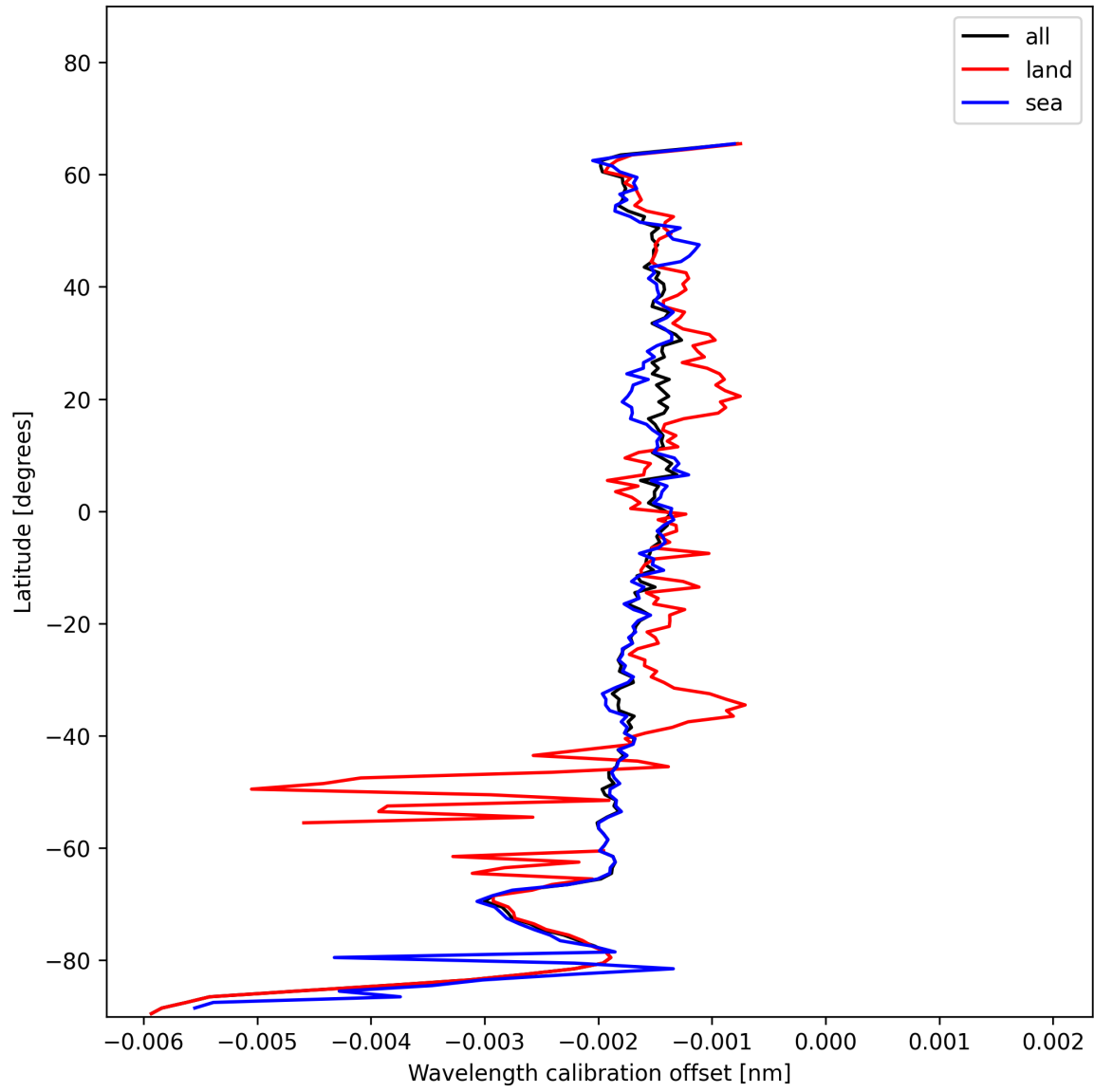
Figure 16: Zonal average of “Wavelength calibration offset” for 2024-12-04 to 2024-12-04.
