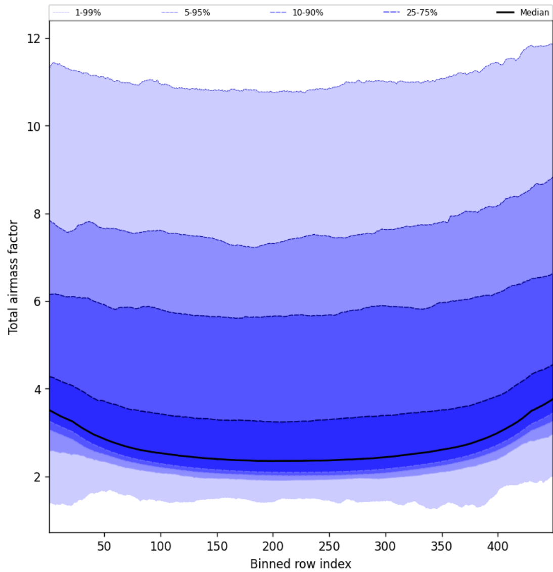
Figure 47: Along track statistics of “Total airmass factor” for 2024-12-04 to 2024-12-04
