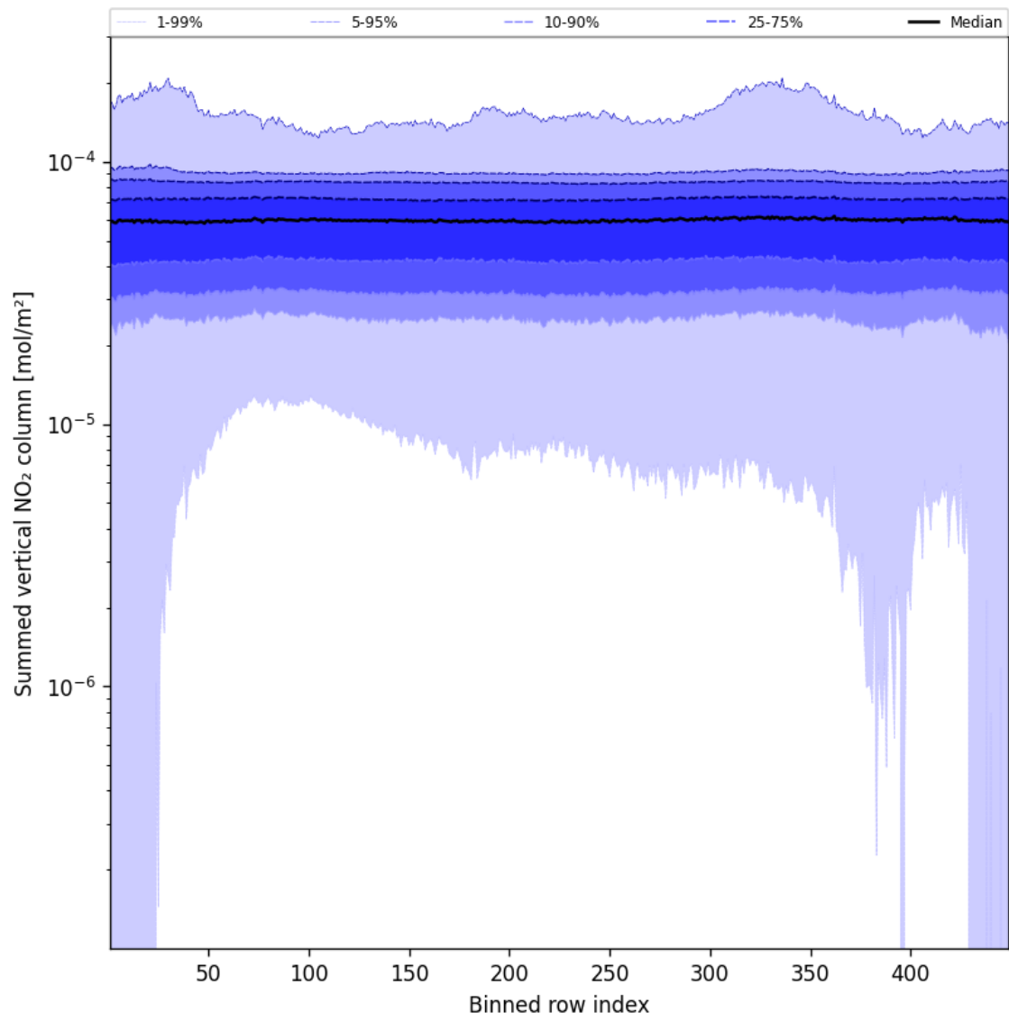
Figure 55: Along track statistics of “Summed vertical NO 2 column” for 2024-12-04 to 2024-12-04
