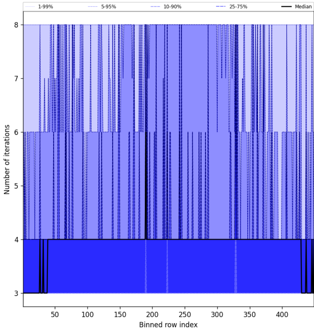
Figure 49: Along track statistics of “Number of iterations” for 2024-12-04 to 2024-12-04
