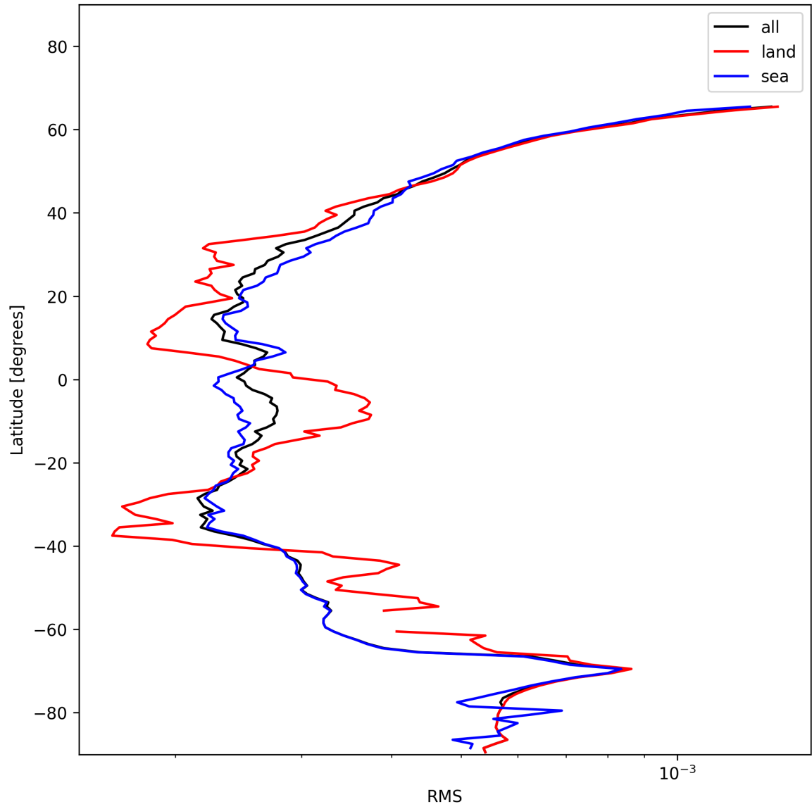
Figure 24: Zonal average of “RMS” for 2024-12-04 to 2024-12-04.
