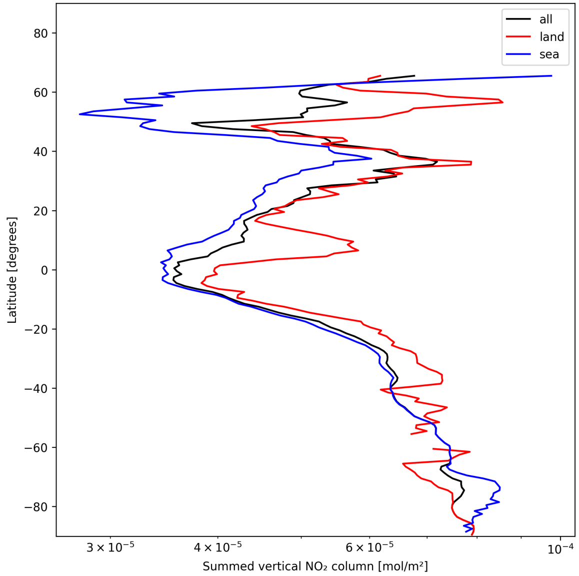
Figure 21: Zonal average of “Summed vertical NO 2 column” for 2024-12-04 to 2024-12-04.
