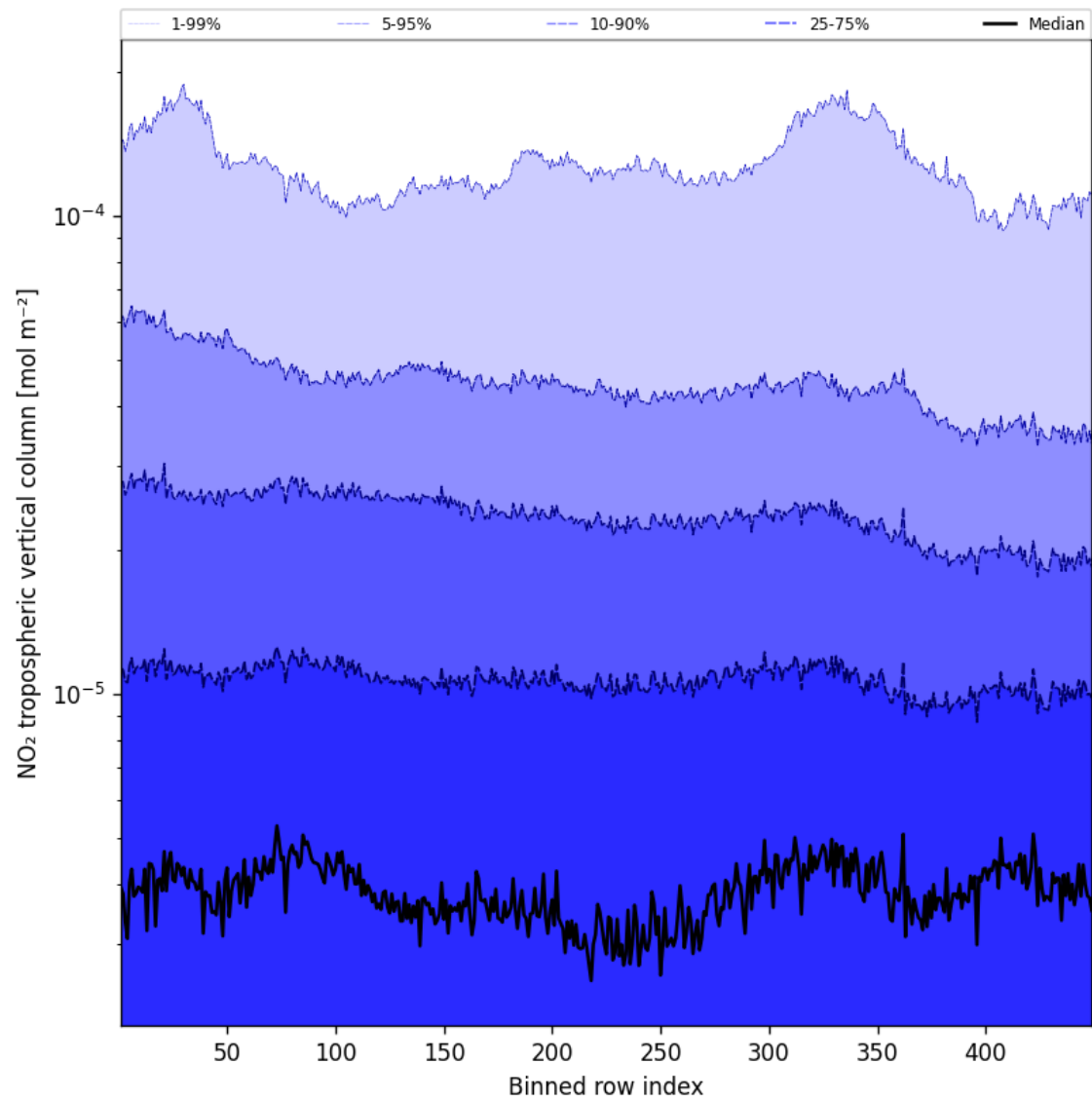
Figure 44: Along track statistics of “NO 2 tropospheric vertical column” for 2024-12-04 to 2024-12-04
