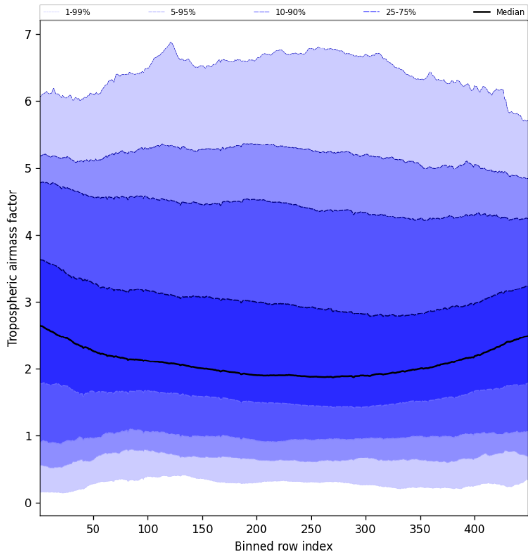
Figure 46: Along track statistics of “Tropospheric airmass factor” for 2024-12-04 to 2024-12-04
