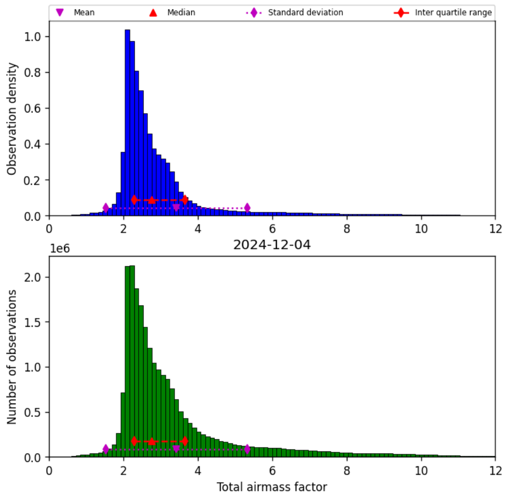
Figure 30: Histogram of “Total airmass factor” for 2024-12-04 to 2024-12-04
