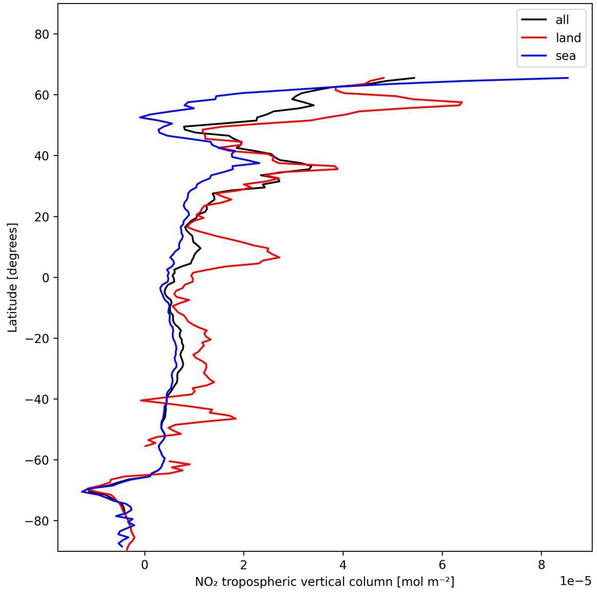
Figure 10: Zonal average of “NO 2 tropospheric vertical column” for 2024-12-04 to 2024-12-04.
