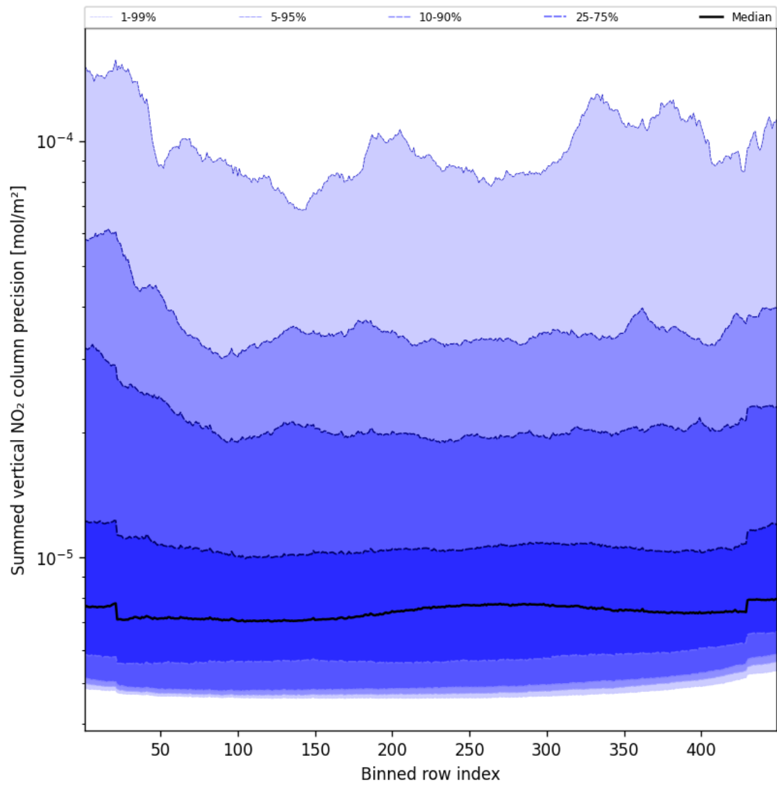
Figure 56: Along track statistics of “Summed vertical NO 2 column precision” for 2024-12-04 to 2024-12-04
