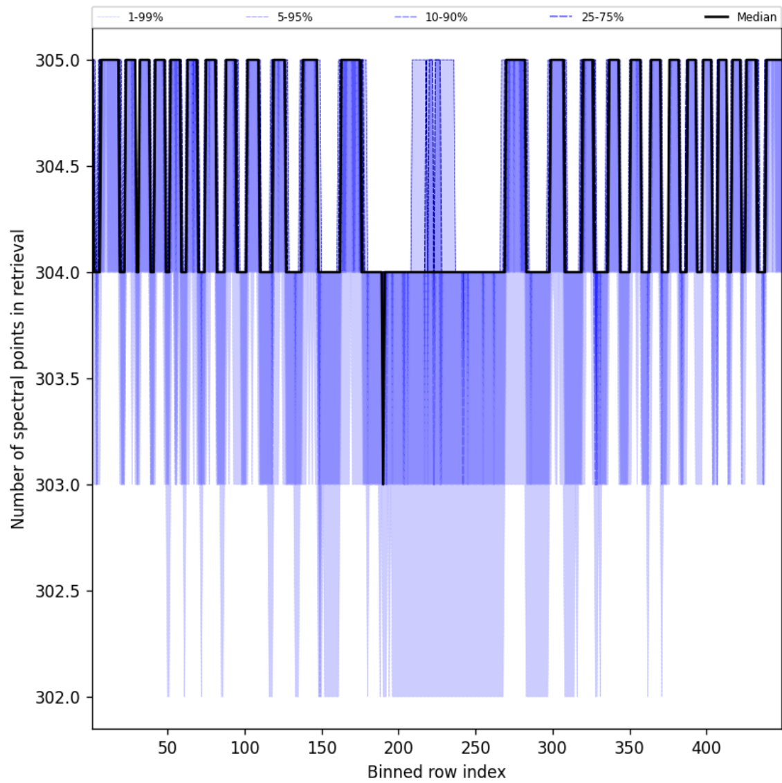
Figure 48: Along track statistics of “Number of spectral points in retrieval” for 2024-12-04 to 2024-12-04
