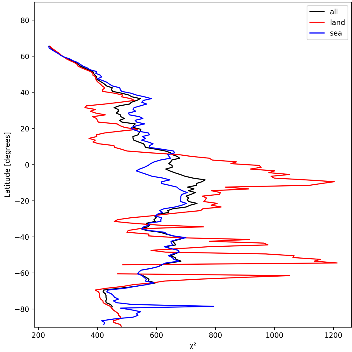
Figure 23: Zonal average of “ \chi^2 ” for 2024-12-04 to 2024-12-04.
