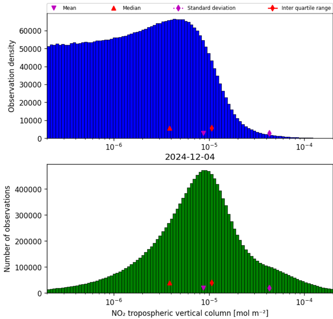
Figure 27: Histogram of “NO 2 tropospheric vertical column” for 2024-12-04 to 2024-12-04
