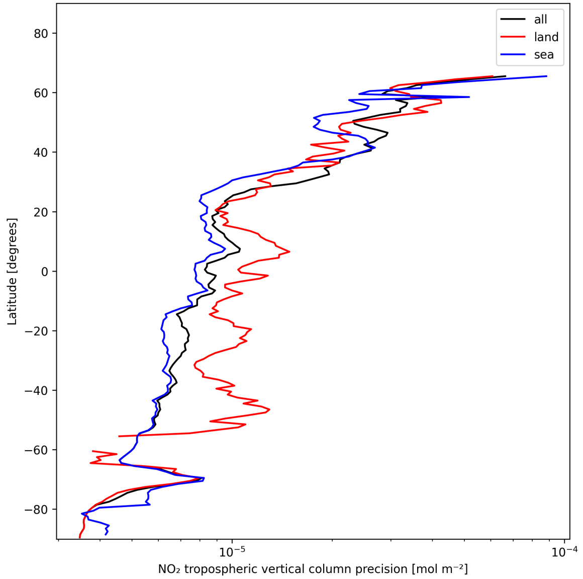
Figure 11: Zonal average of “NO 2 tropospheric vertical column precision” for 2024-12-04 to 2024-12-04.
