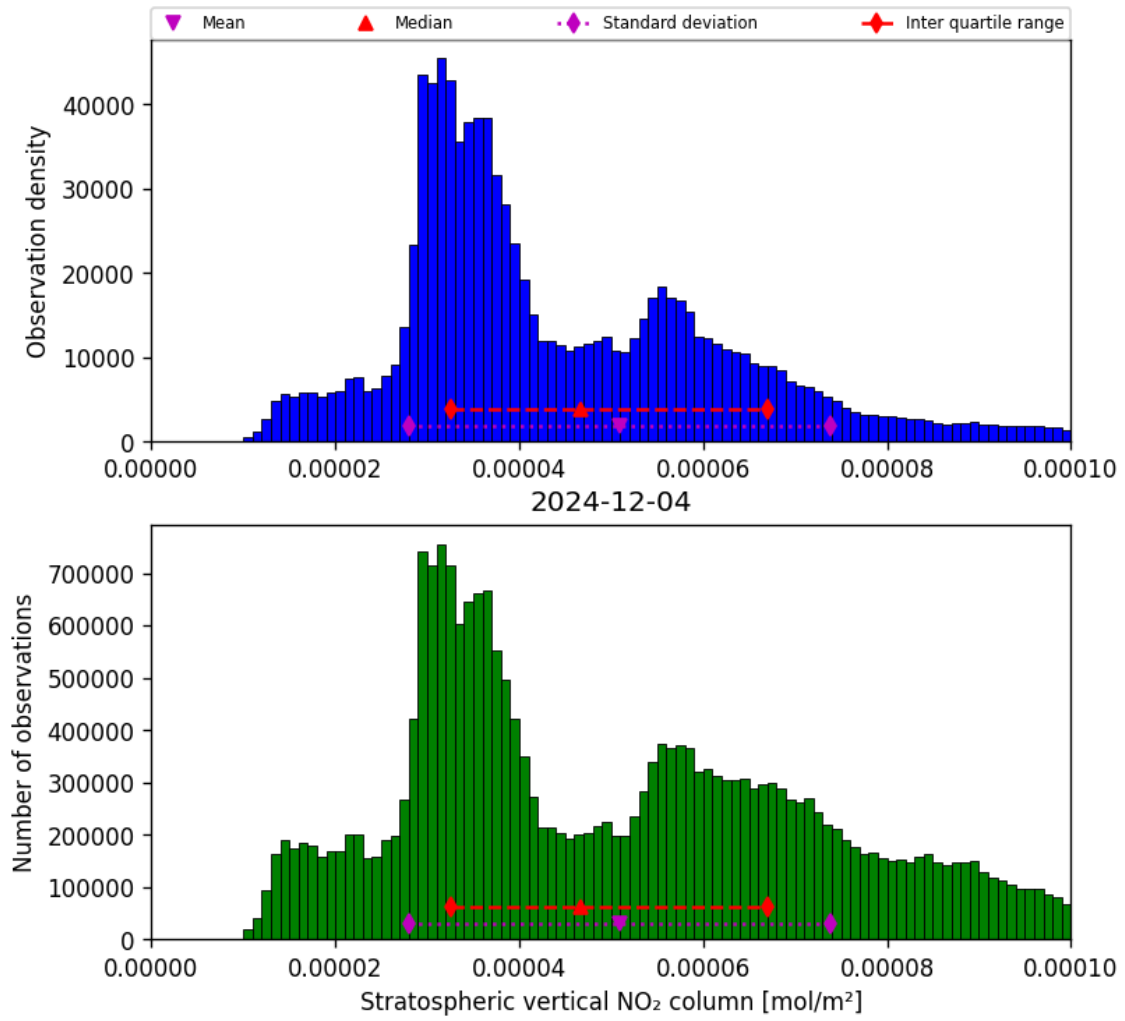
Figure 34: Histogram of “Stratospheric vertical NO 2 column” for 2024-12-04 to 2024-12-04
