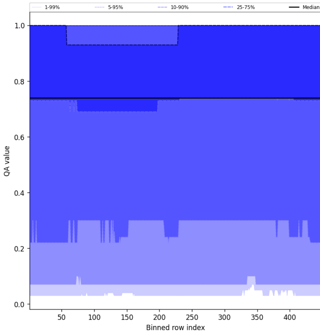
Figure 43: Along track statistics of “QA value” for 2024-12-04 to 2024-12-04
