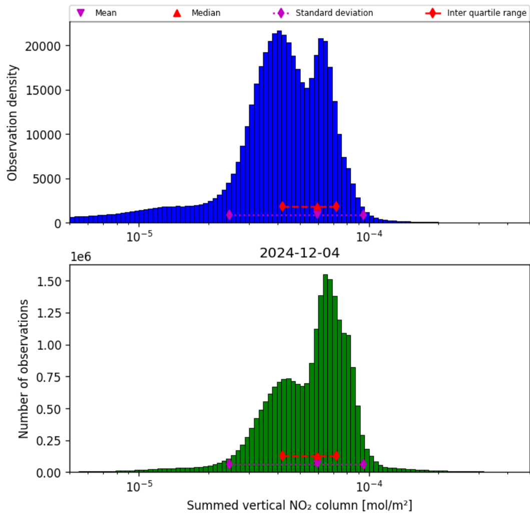
Figure 38: Histogram of “Summed vertical NO 2 column” for 2024-12-04 to 2024-12-04
