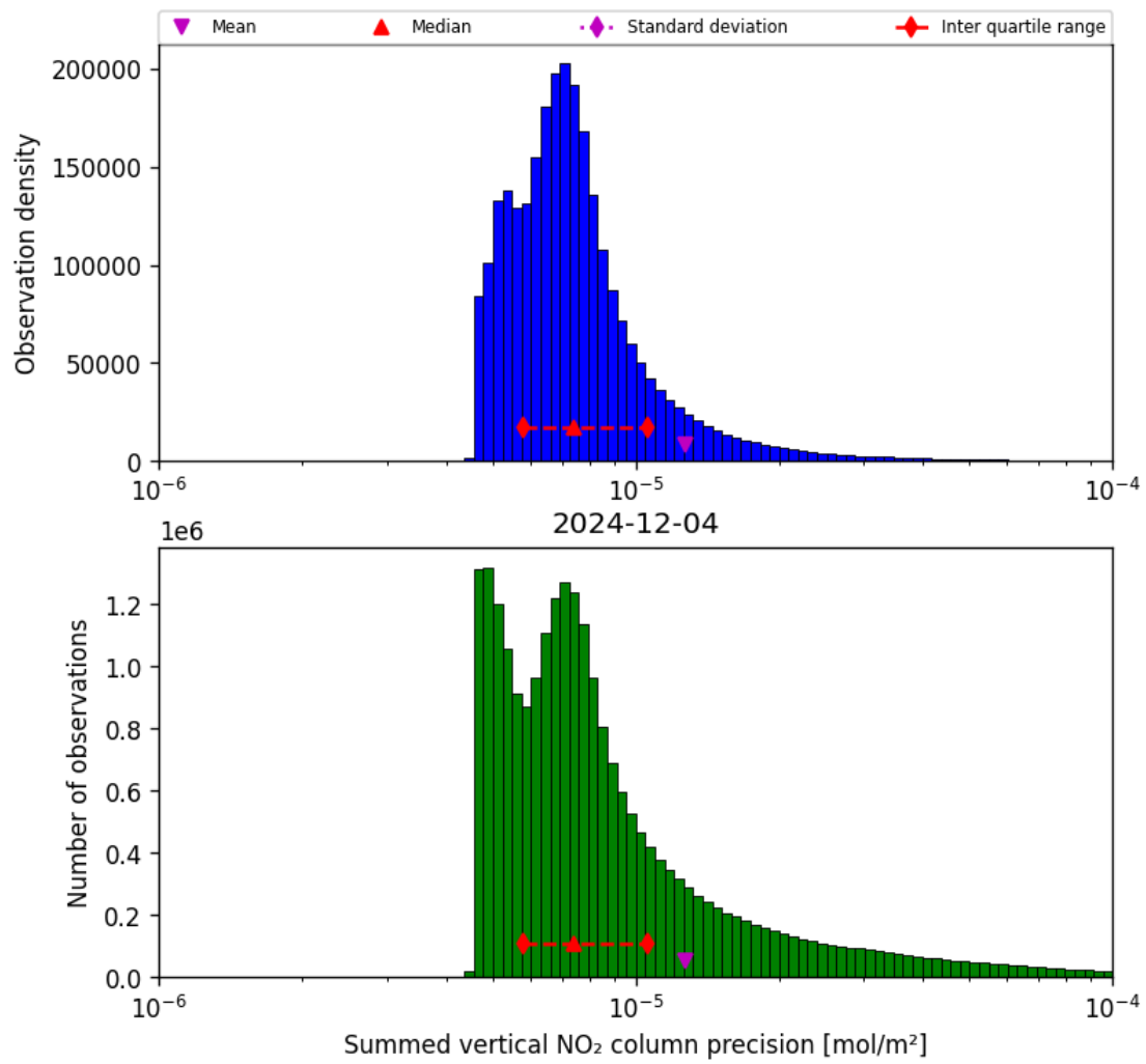
Figure 39: Histogram of "Summed vertical NO 2 column precision" for 2024-12-04 to 2024-12-04
