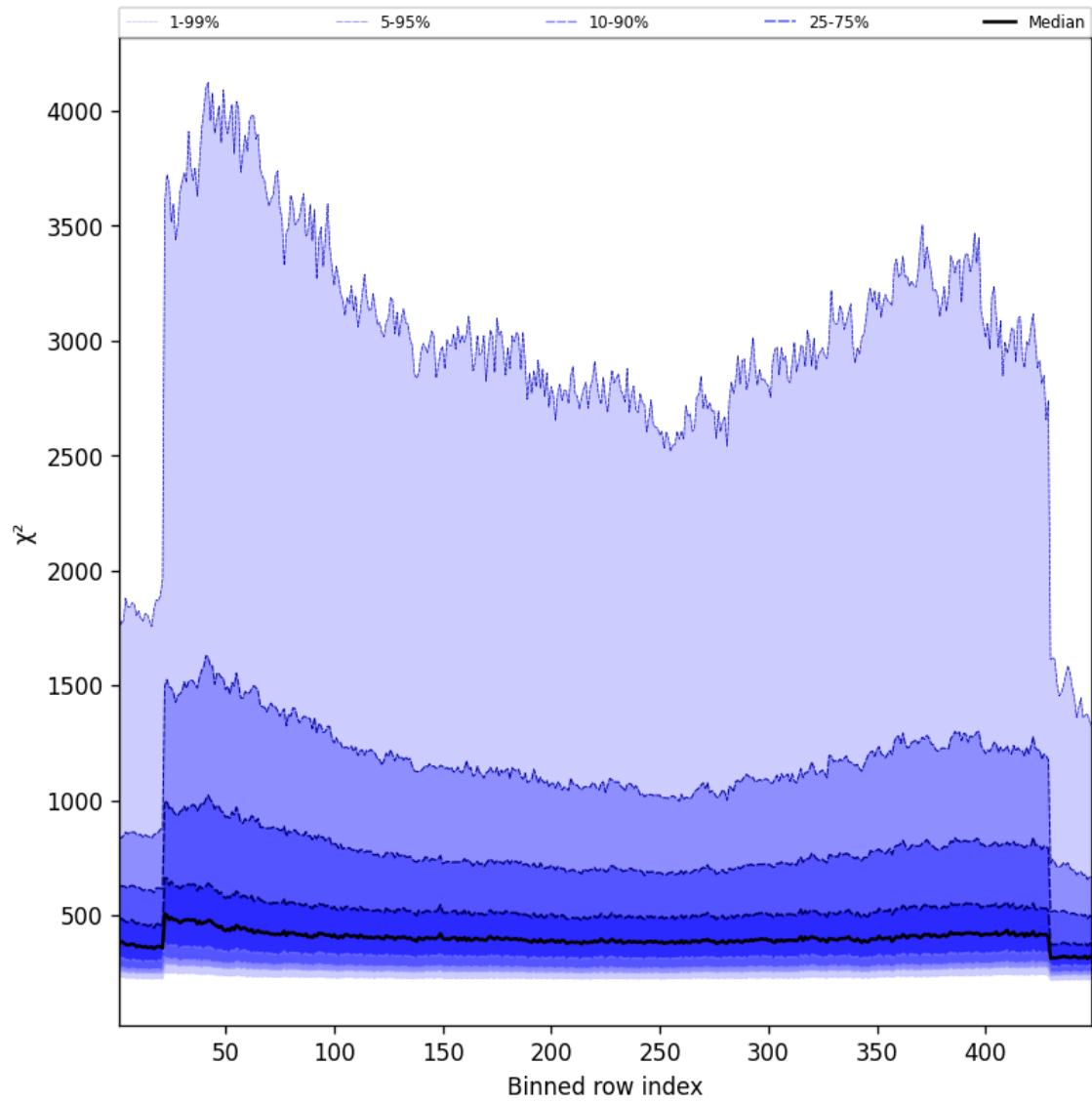
Figure 57: Along track statistics of “ \chi^2 ” for 2024-12-04 to 2024-12-04
