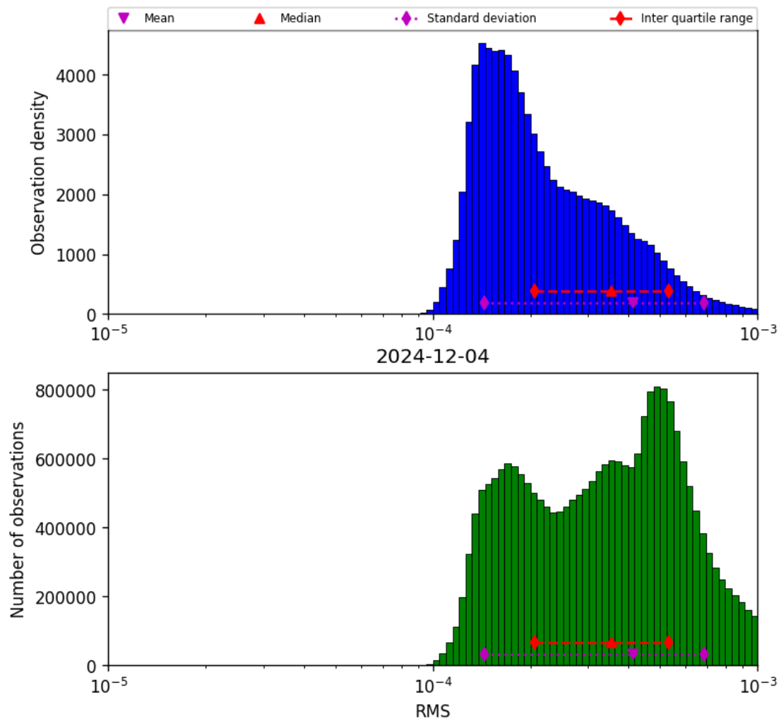
Figure 41: Histogram of “RMS” for 2024-12-04 to 2024-12-04
