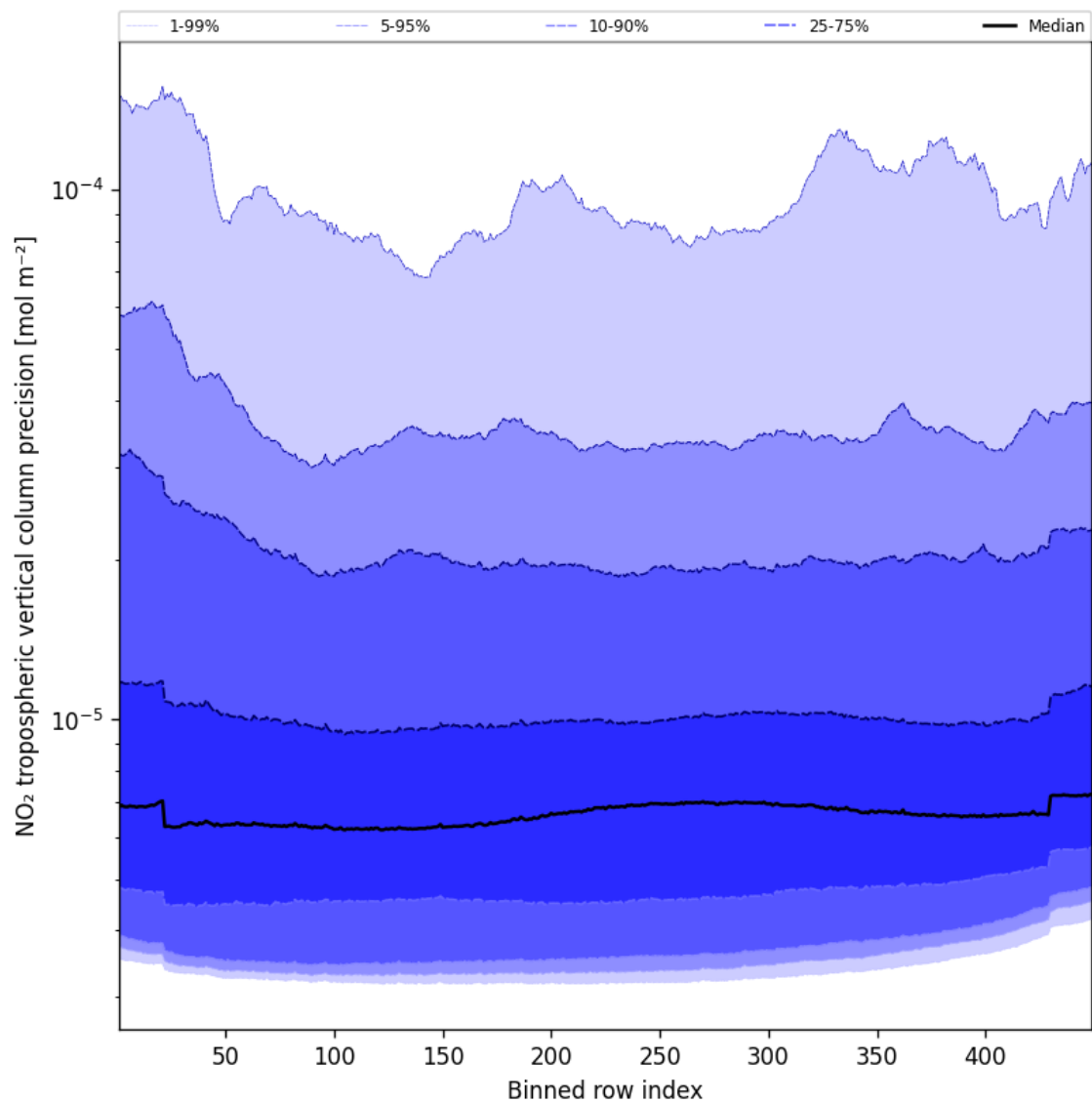
Figure 45: Along track statistics of “NO 2 tropospheric vertical column precision” for 2024-12-04 to 2024-12-04
