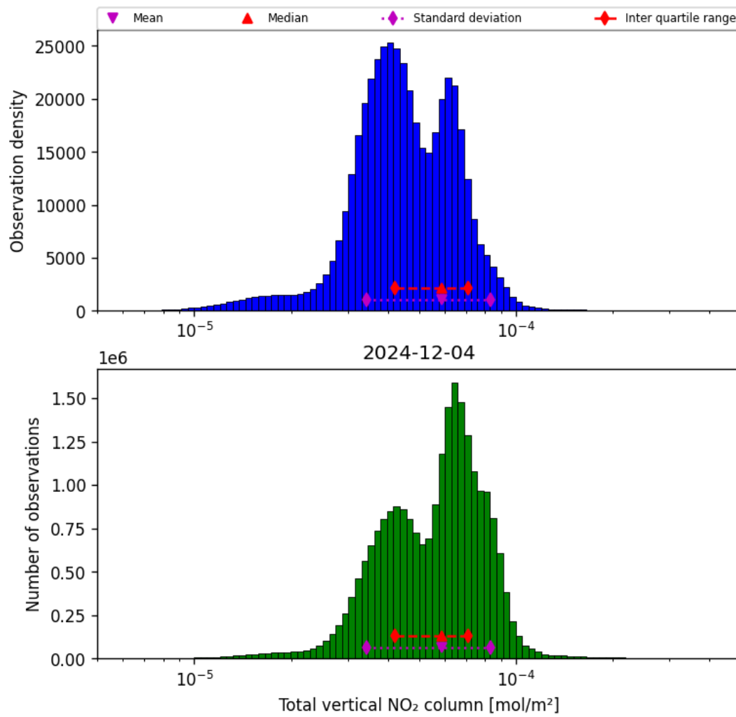
Figure 36: Histogram of “Total vertical NO 2 column” for 2024-12-04 to 2024-12-04
