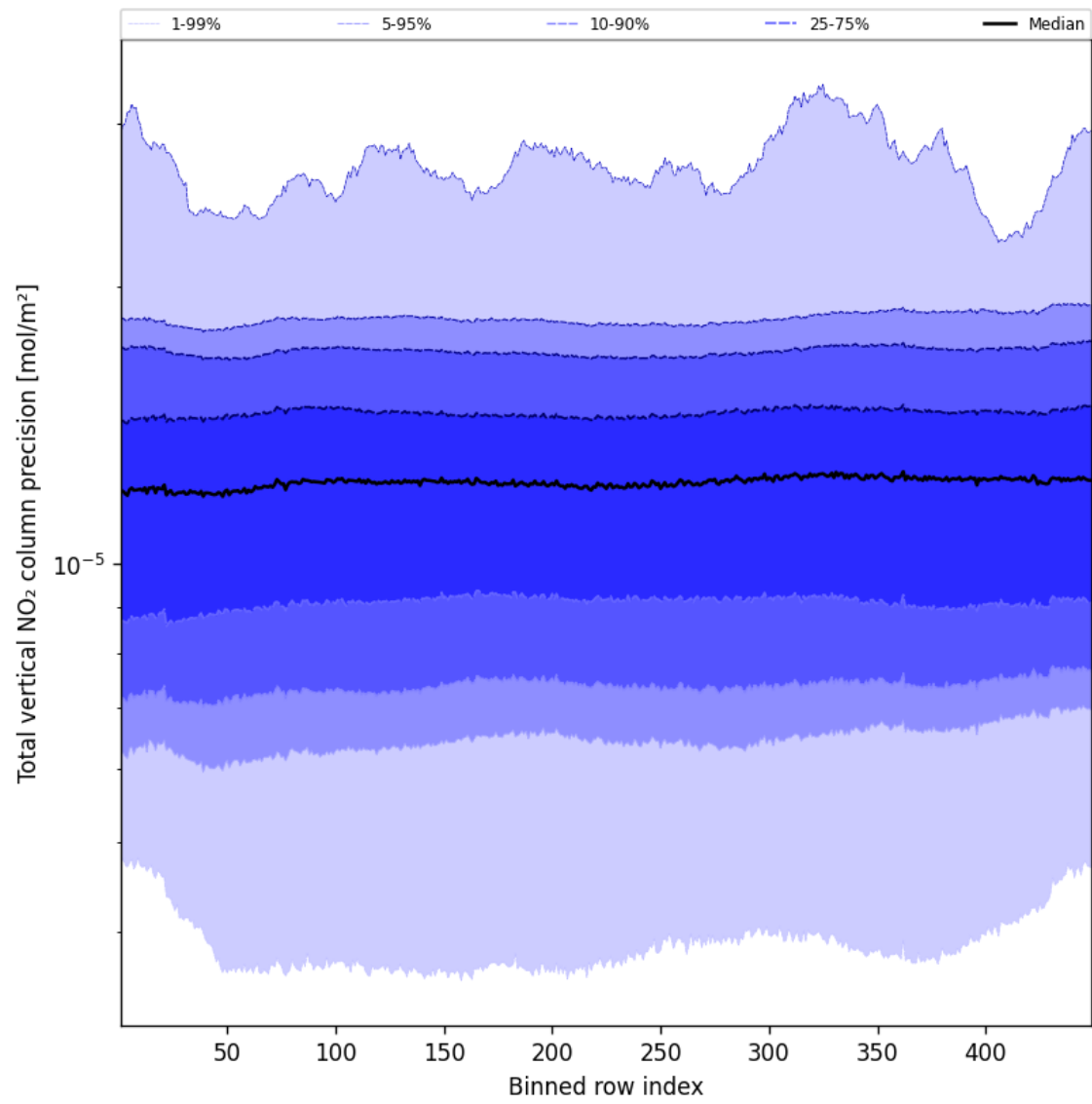
Figure 54: Along track statistics of “Total vertical NO 2 column precision” for 2024-12-04 to 2024-12-04
