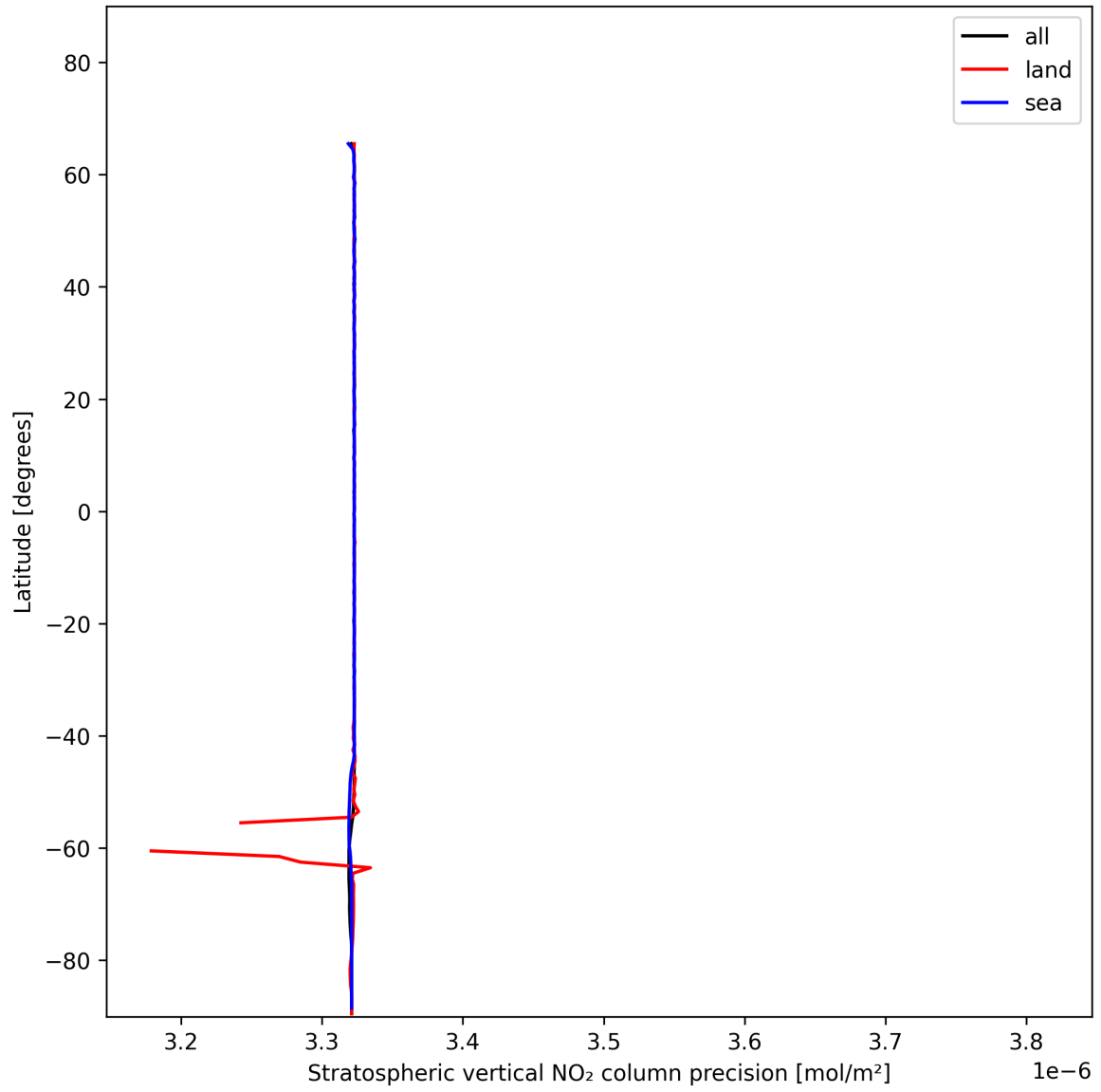
Figure 18: Zonal average of “Stratospheric vertical NO 2 column precision” for 2024-12-04 to 2024-12-04.
