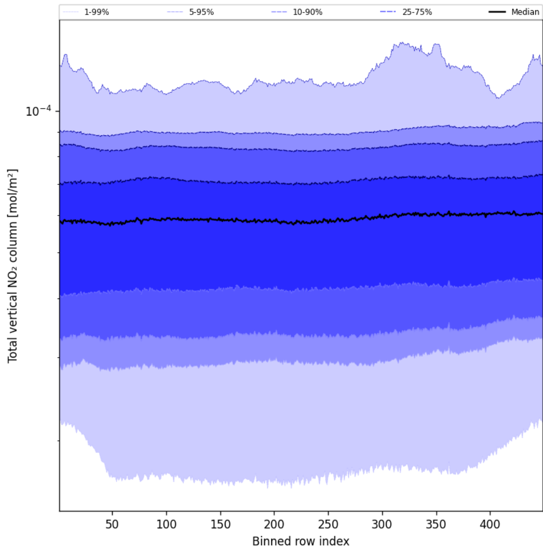
Figure 53: Along track statistics of “Total vertical NO 2 column” for 2024-12-04 to 2024-12-04
