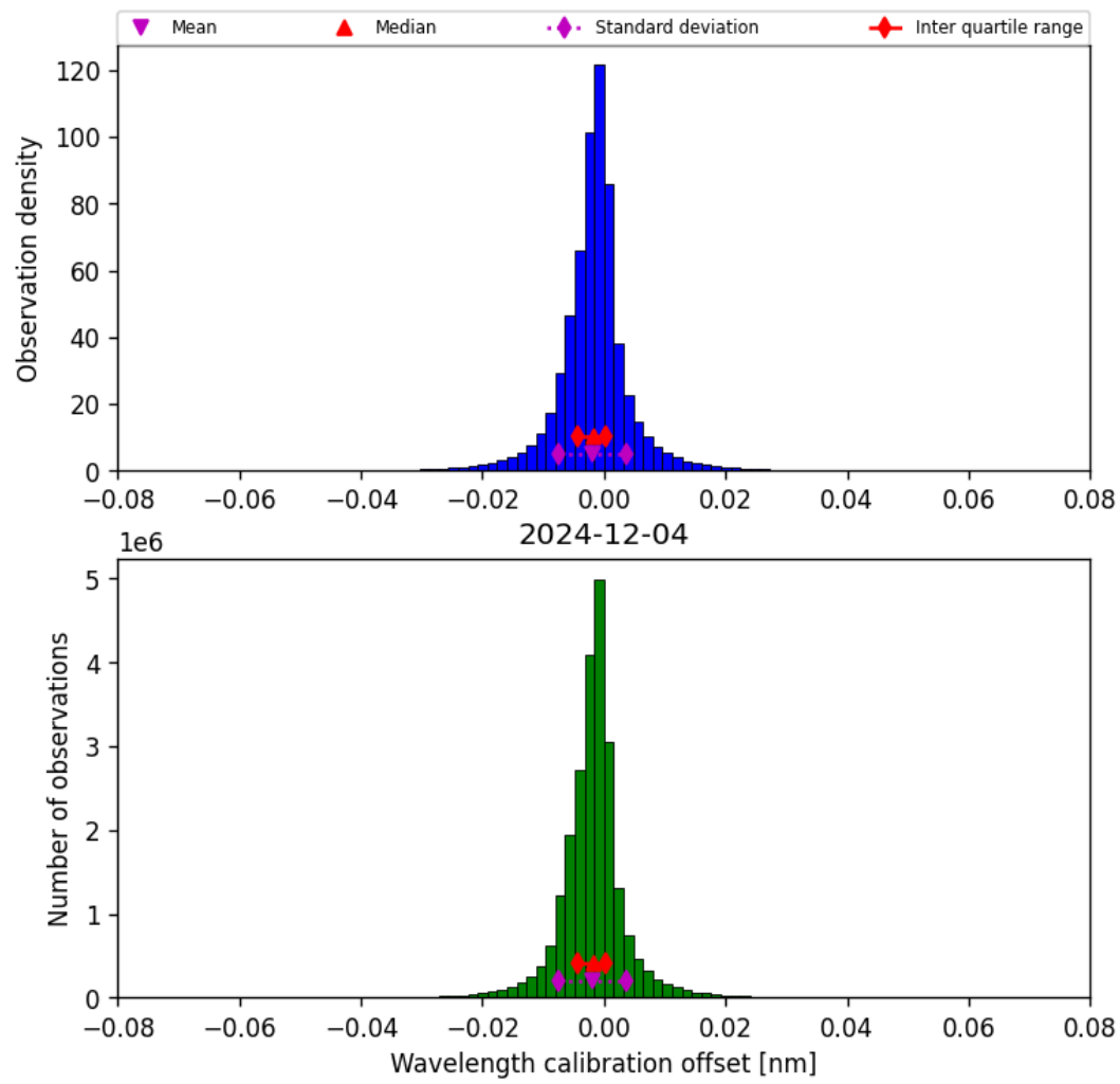
Figure 33: Histogram of “Wavelength calibration offset” for 2024-12-04 to 2024-12-04
