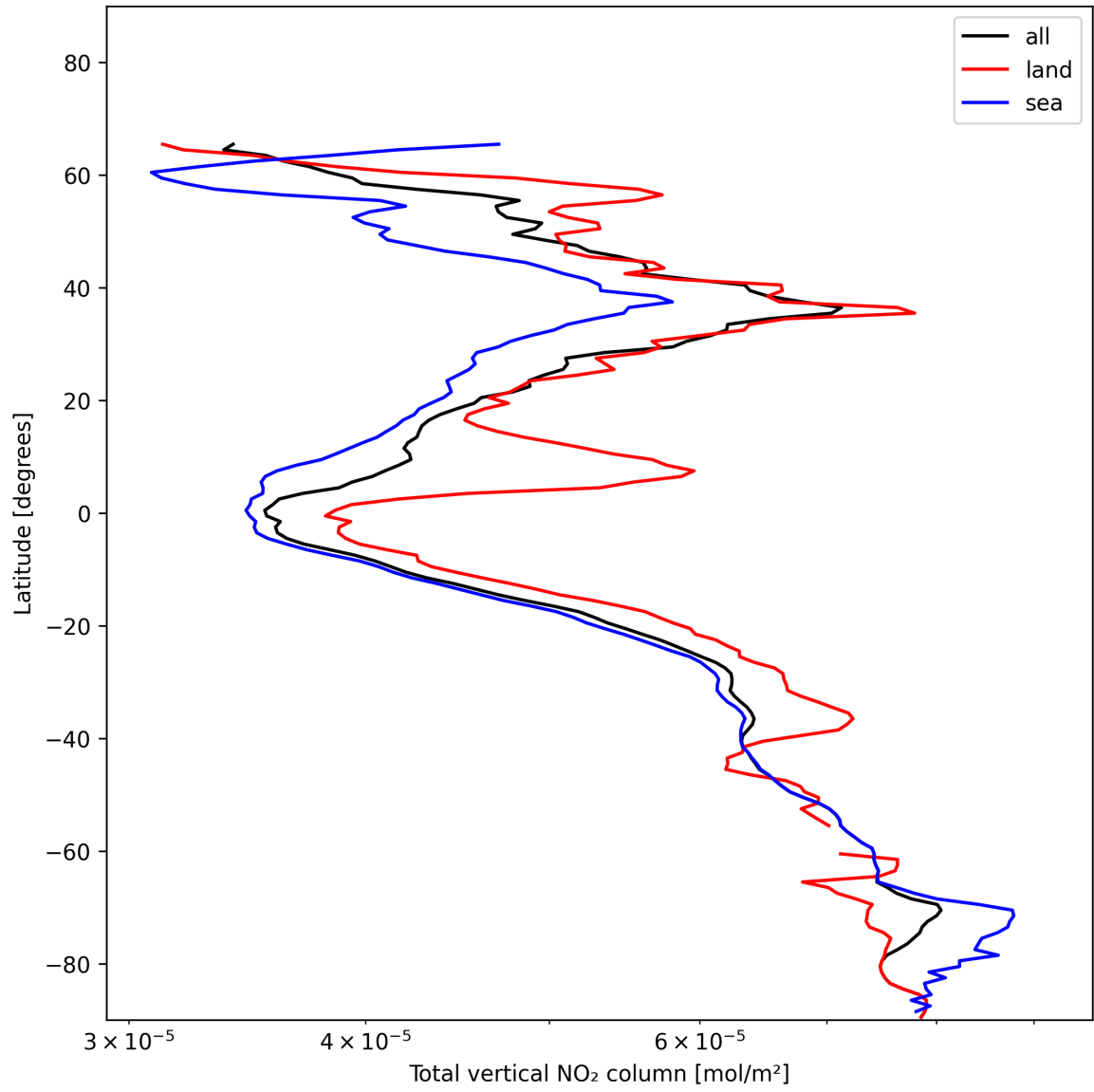
Figure 19: Zonal average of “Total vertical NO 2 column” for 2024-12-04 to 2024-12-04.
