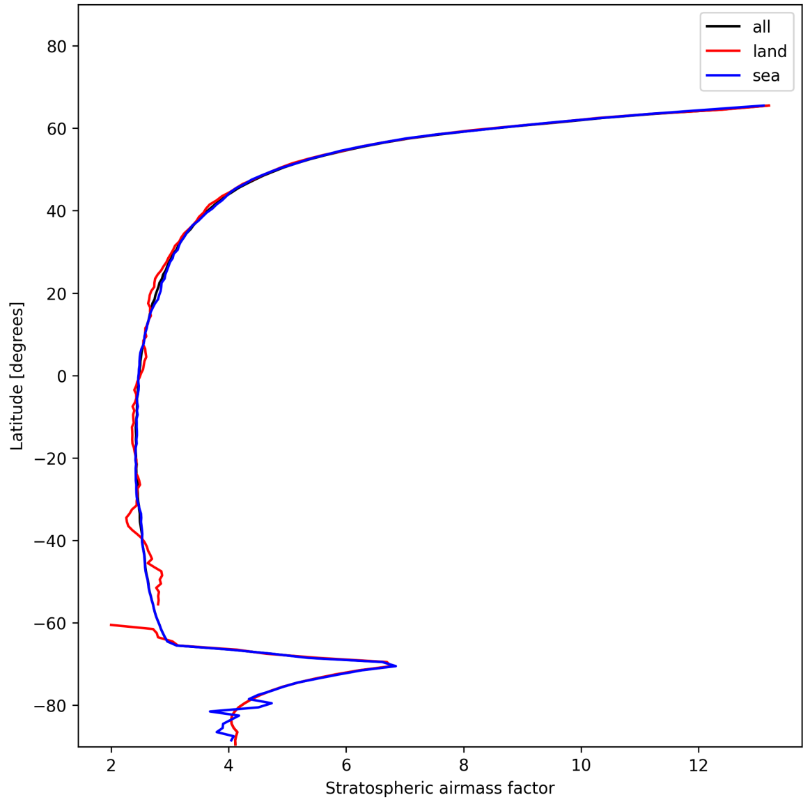
Figure 25: Zonal average of “Stratospheric airmass factor” for 2024-12-04 to 2024-12-04.
