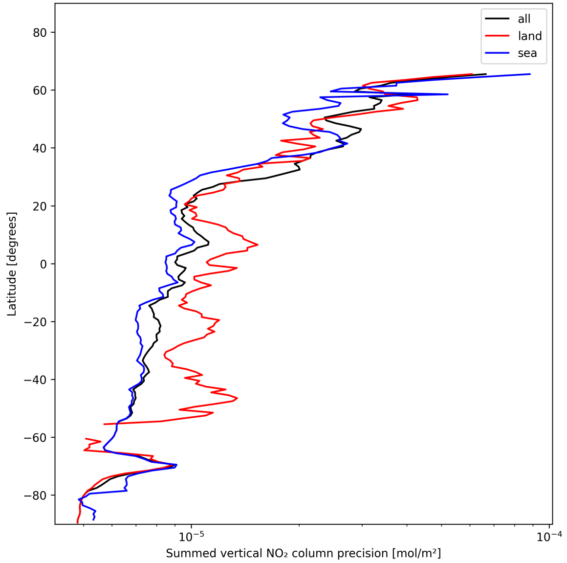
Figure 22: Zonal average of “Summed vertical NO 2 column precision” for 2024-12-04 to 2024-12-04.
