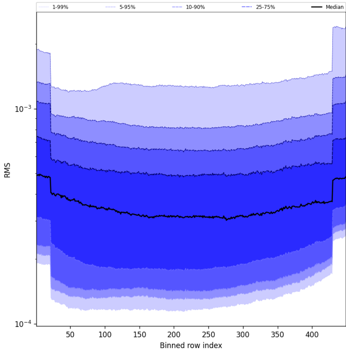
Figure 58: Along track statistics of “RMS” for 2024-12-05 to 2024-12-06
