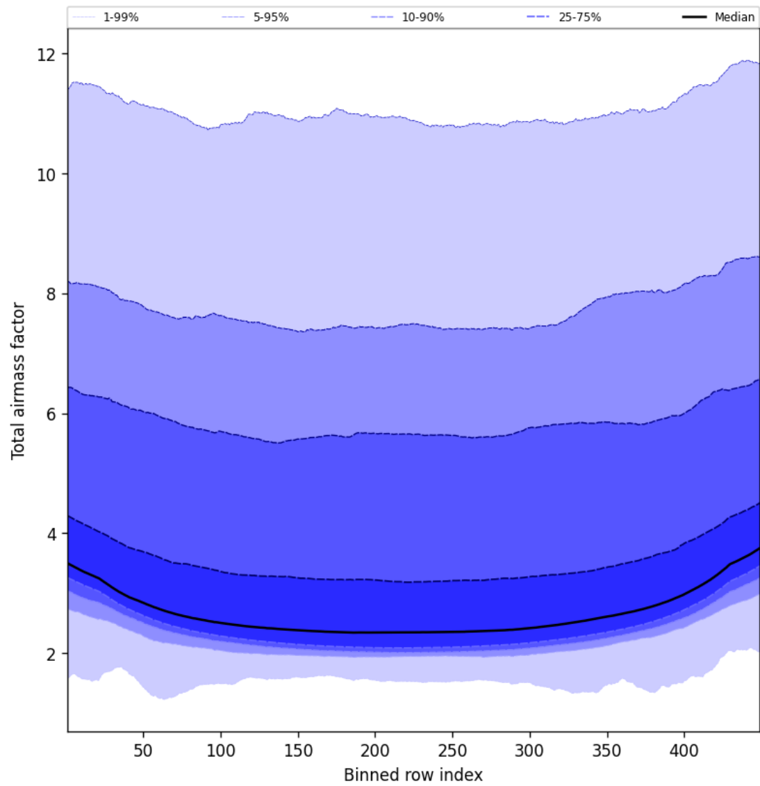
Figure 47: Along track statistics of “Total airmass factor” for 2024-12-05 to 2024-12-06
