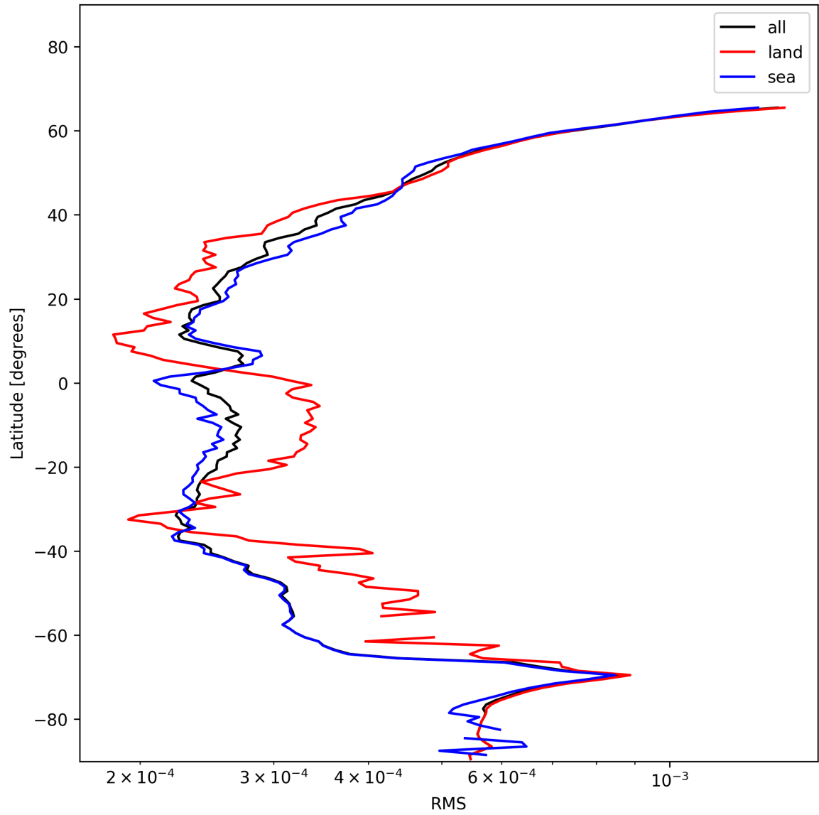
Figure 24: Zonal average of “RMS” for 2024-12-05 to 2024-12-06.
