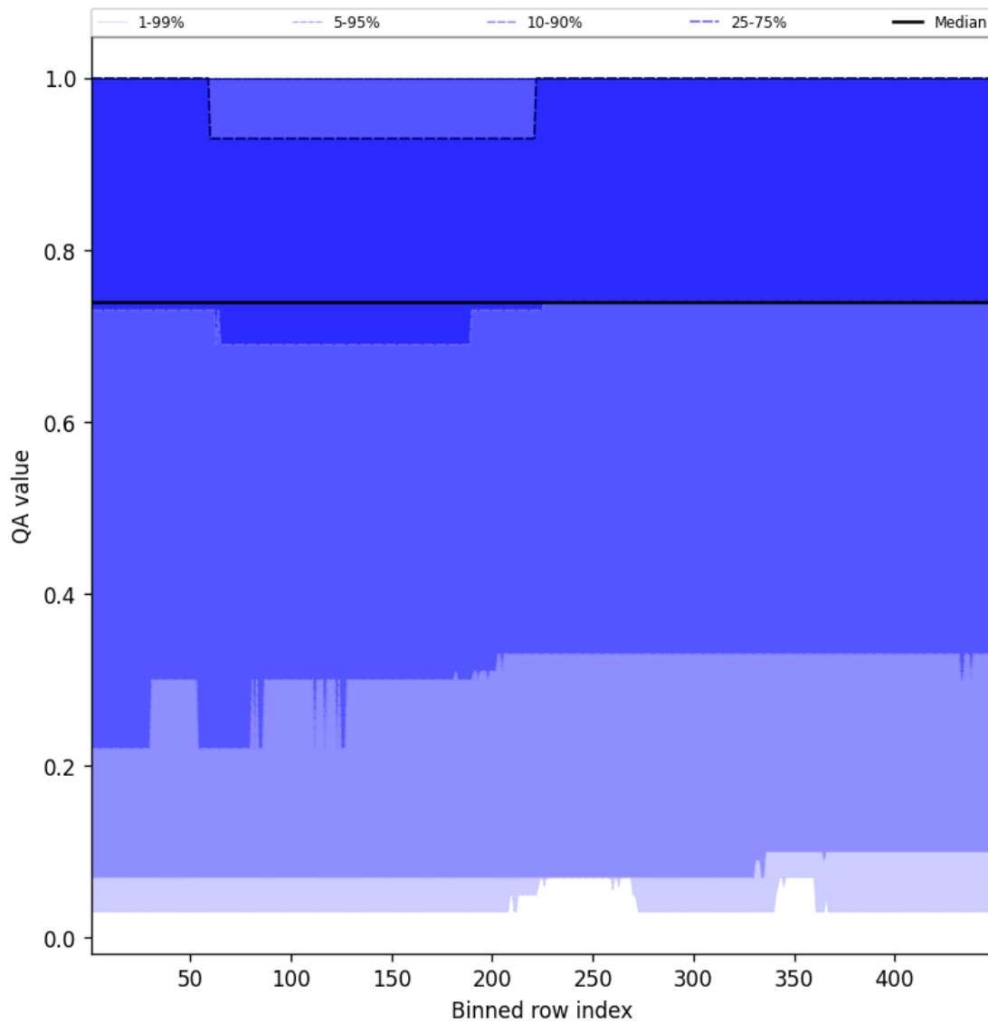
Figure 43: Along track statistics of “QA value” for 2024-12-05 to 2024-12-06
