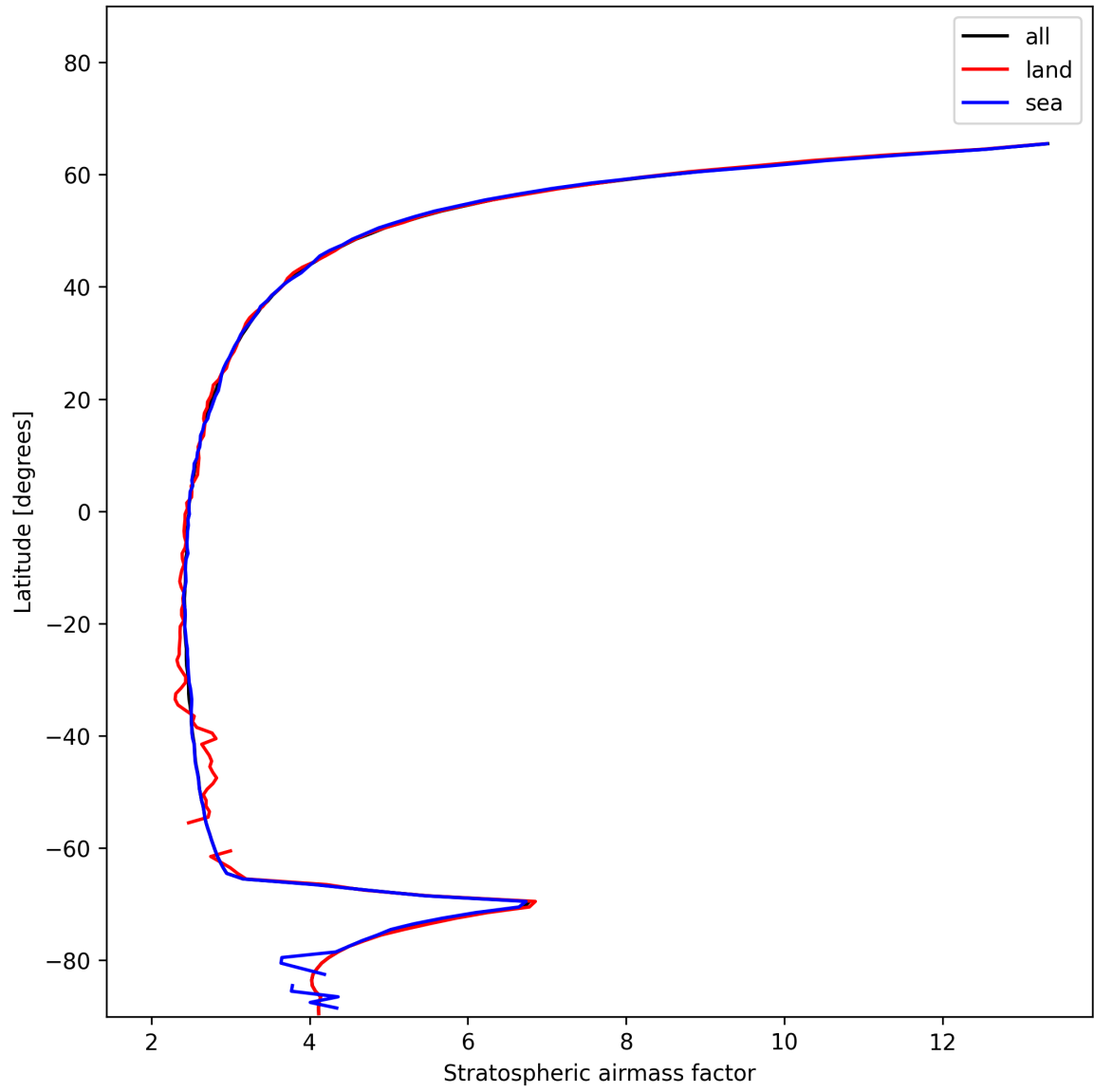
Figure 25: Zonal average of “Stratospheric air mass factor” for 2024-12-05 to 2024-12-06.
