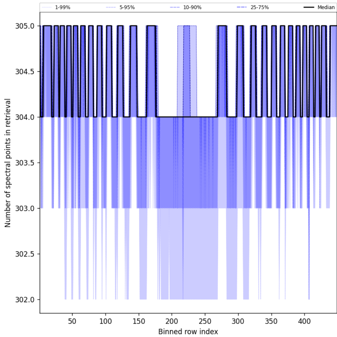
Figure 48: Along track statistics of “Number of spectral points in retrieval” for 2024-12-05 to 2024-12-06
