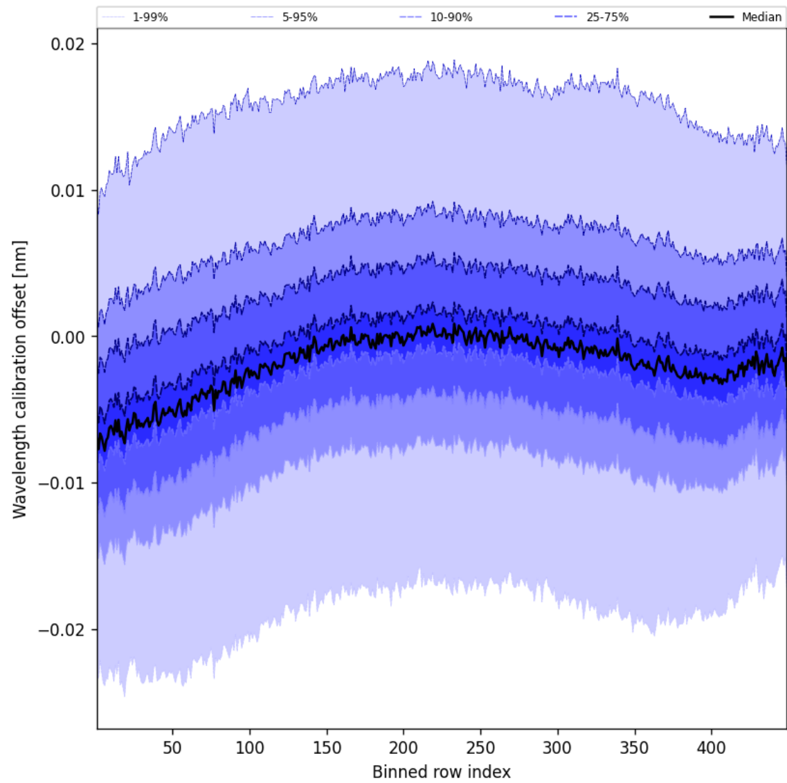
Figure 50: Along track statistics of “Wavelength calibration offset” for 2024-12-05 to 2024-12-06
