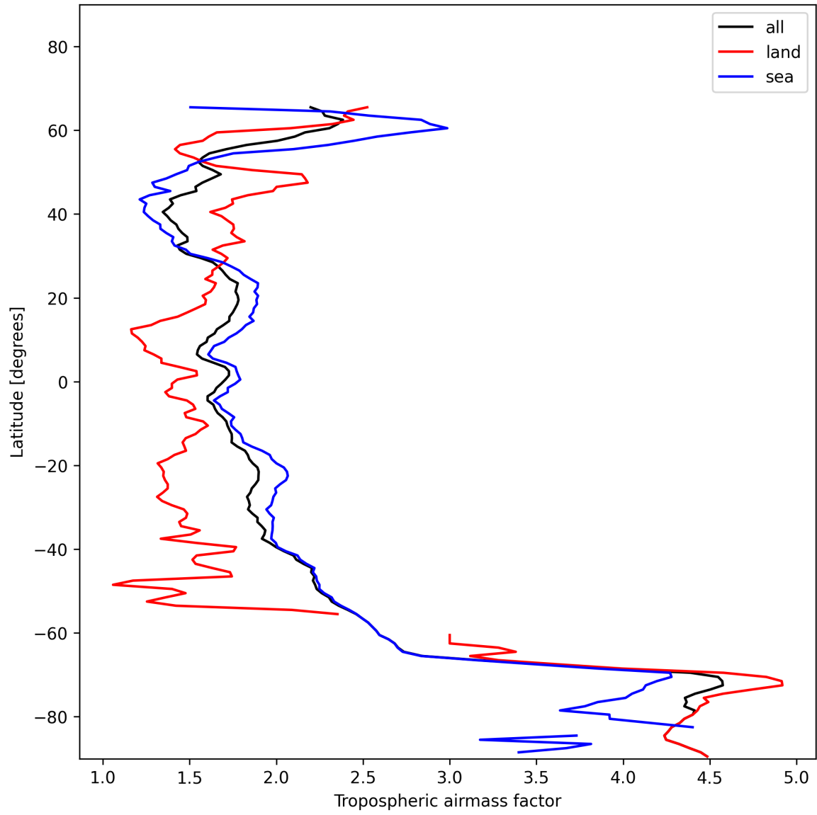
Figure 12: Zonal average of “Tropospheric air mass factor” for 2024-12-05 to 2024-12-06.
