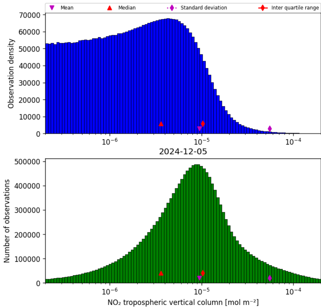
Figure 27: Histogram of “NO 2 tropospheric vertical column” for 2024-12-05 to 2024-12-06
