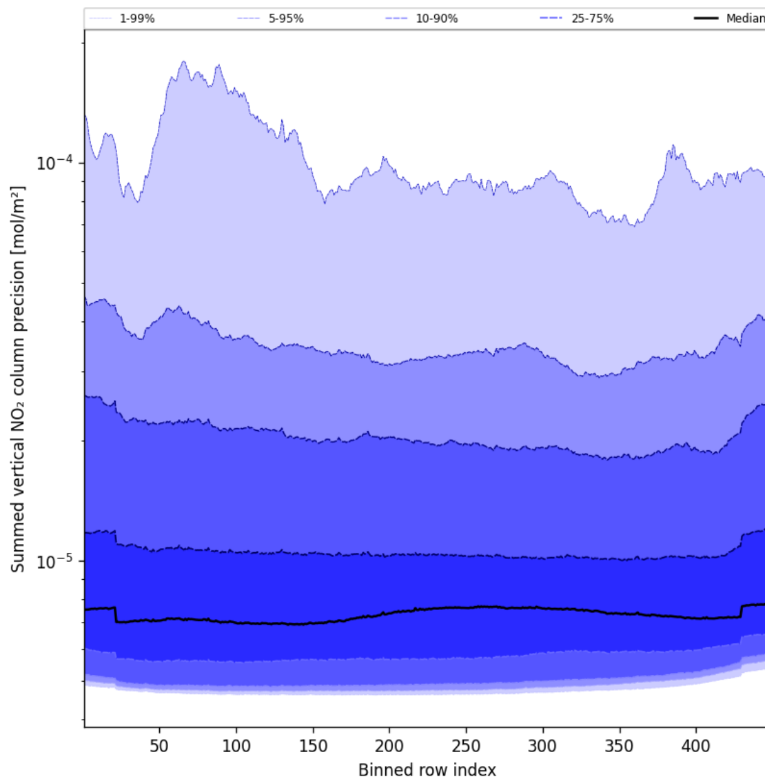
Figure 56: Along track statistics of “Summed vertical NO 2 column precision” for 2024-12-05 to 2024-12-06
