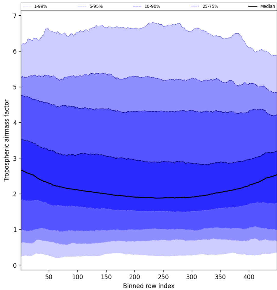
Figure 46: Along track statistics of “Tropospheric airmass factor” for 2024-12-05 to 2024-12-06
