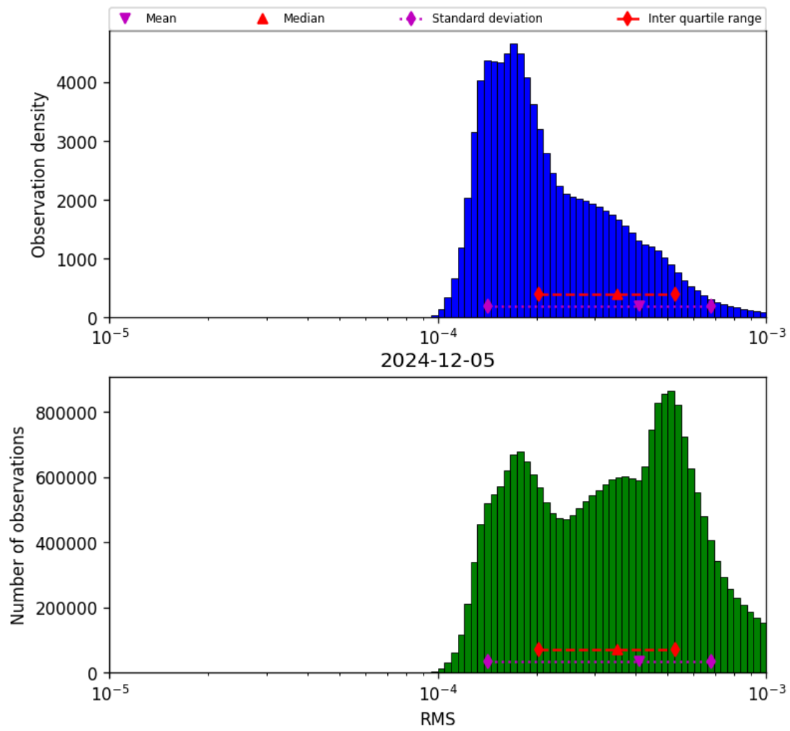
Figure 41: Histogram of “RMS” for 2024-12-05 to 2024-12-06
