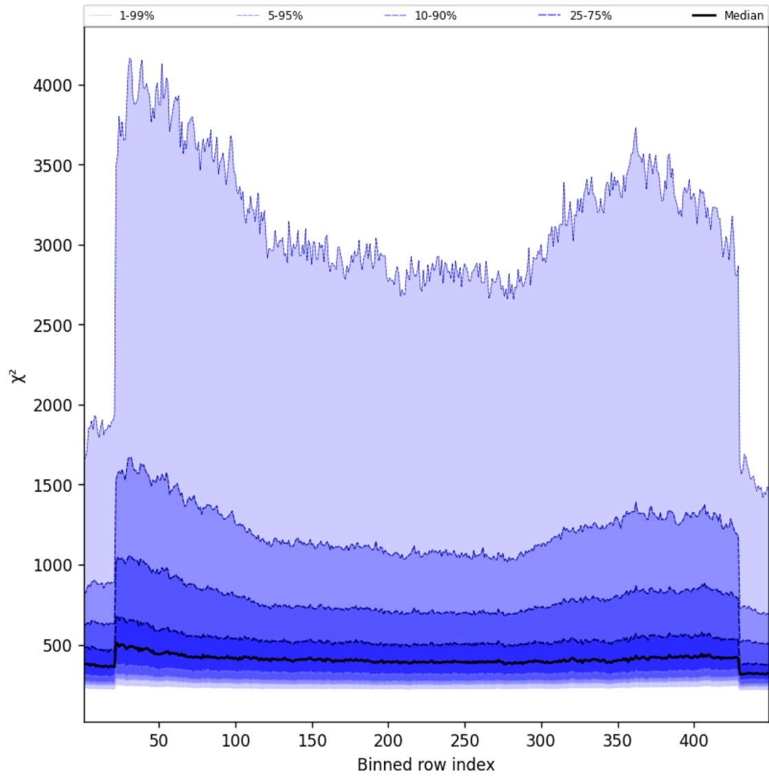
Figure 57: Along track statistics of “ \chi^2 ” for 2024-12-05 to 2024-12-06
