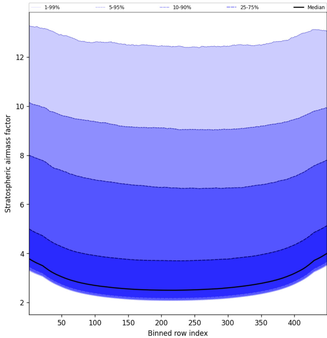
Figure 59: Along track statistics of “Stratospheric airmass factor” for 2024-12-05 to 2024-12-06
