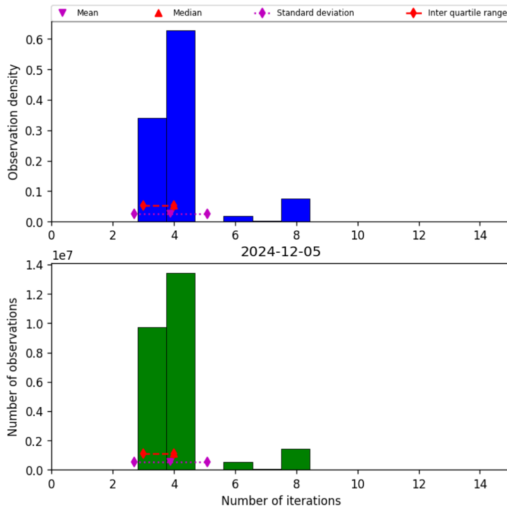
Figure 32: Histogram of “Number of iterations” for 2024-12-05 to 2024-12-06
