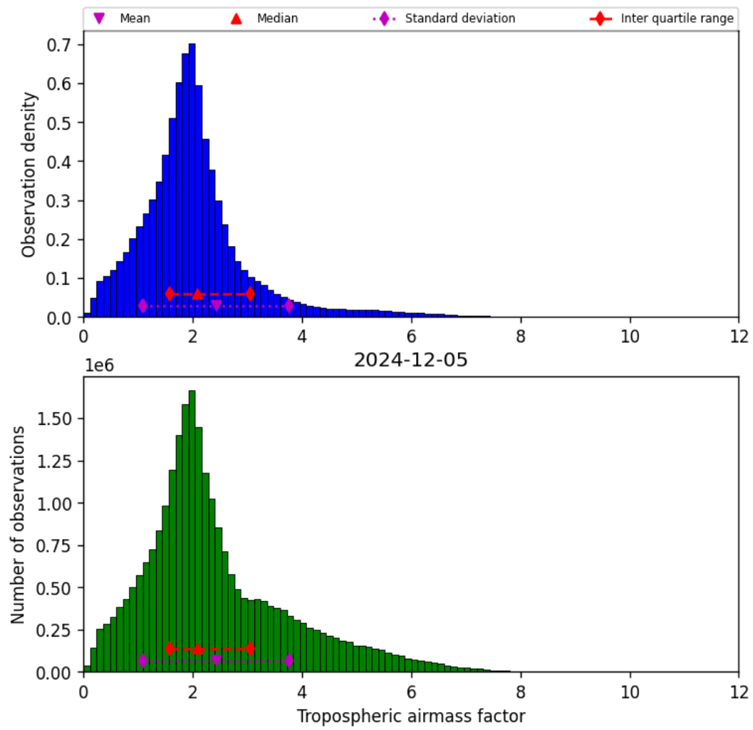
Figure 29: Histogram of “Tropospheric airmass factor” for 2024-12-05 to 2024-12-06
