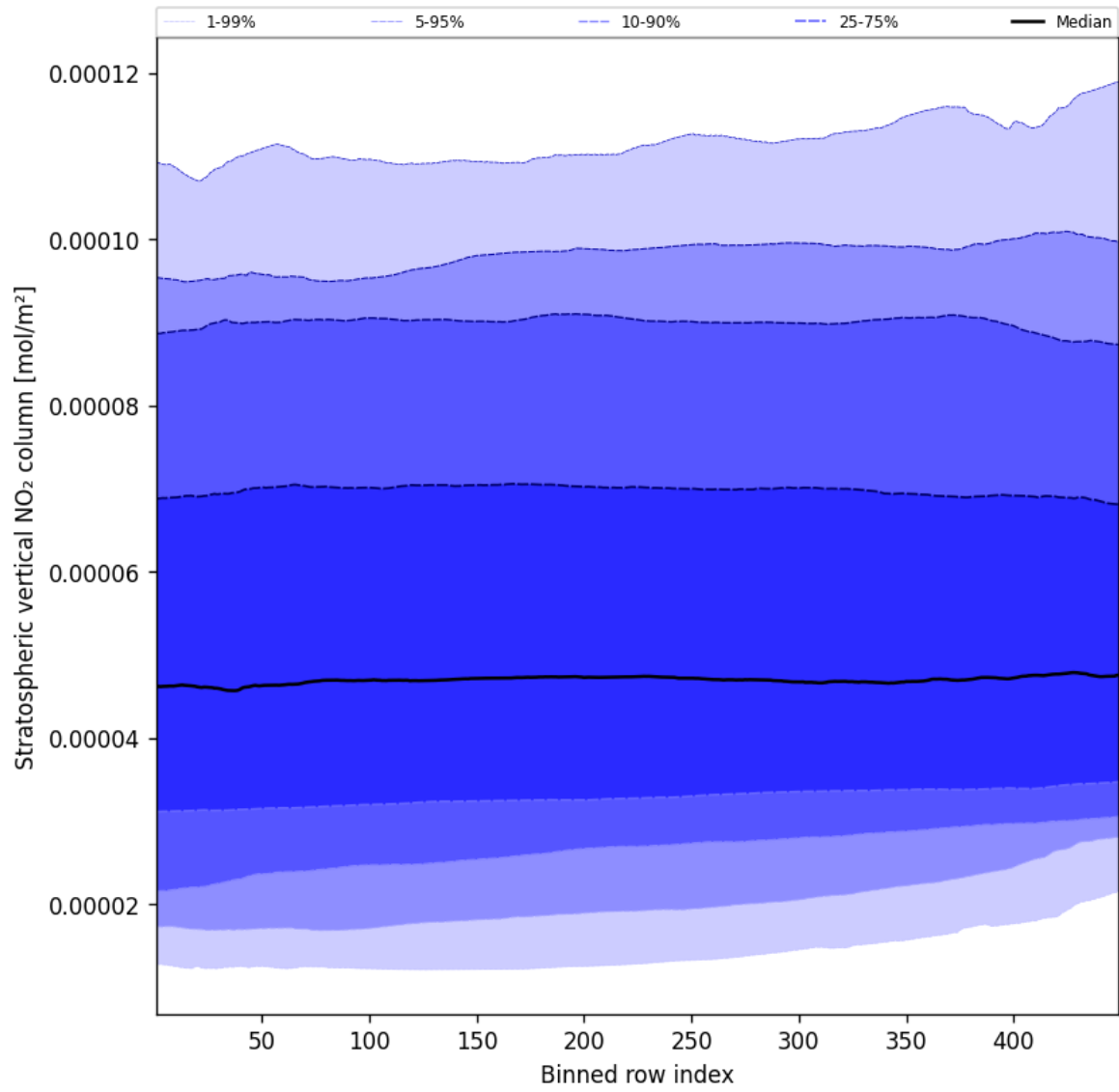
Figure 51: Along track statistics of “Stratospheric vertical NO 2 column” for 2024-12-05 to 2024-12-06
