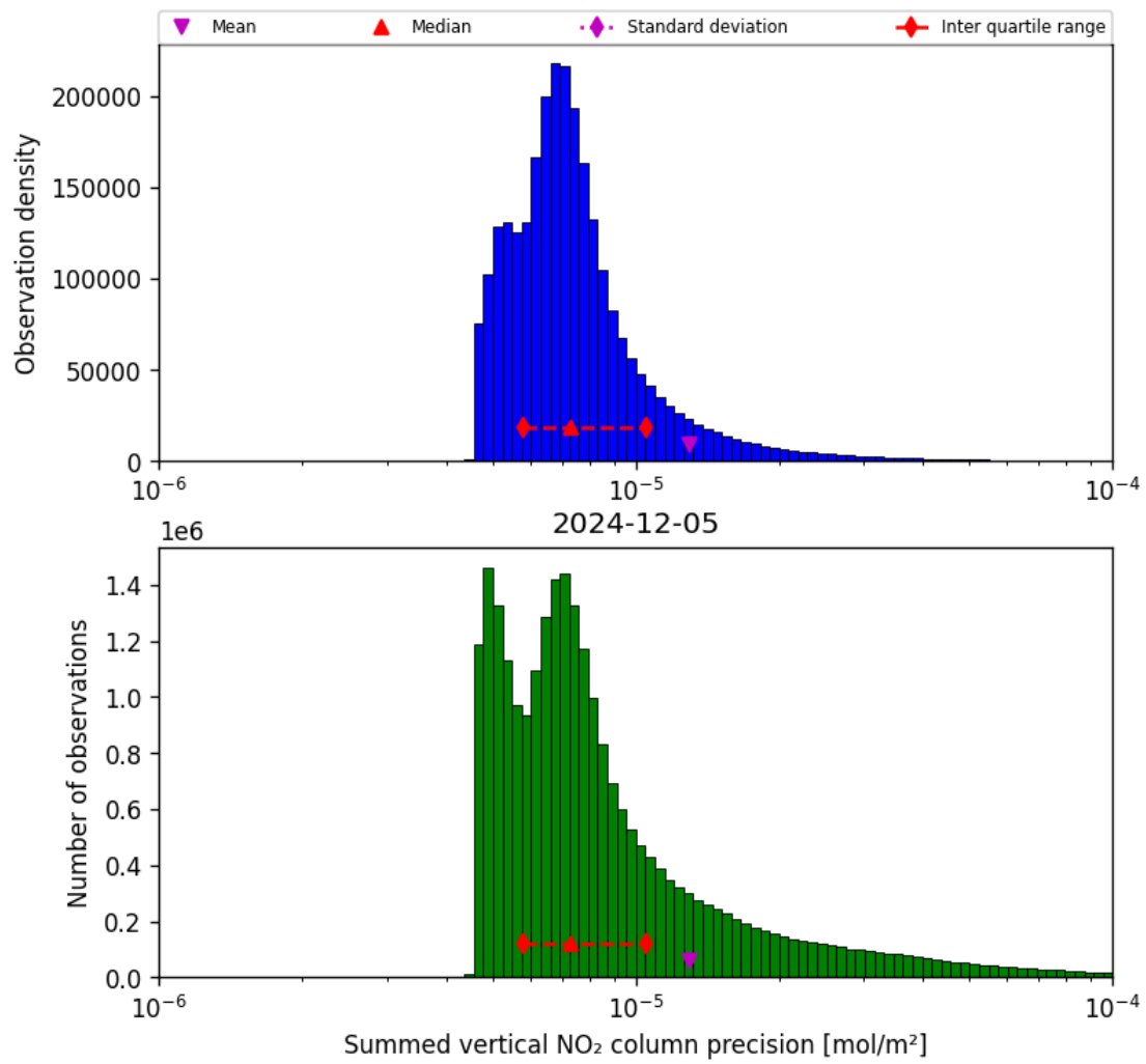
Figure 39: Histogram of “Summed vertical NO 2 column precision” for 2024-12-05 to 2024-12-06
