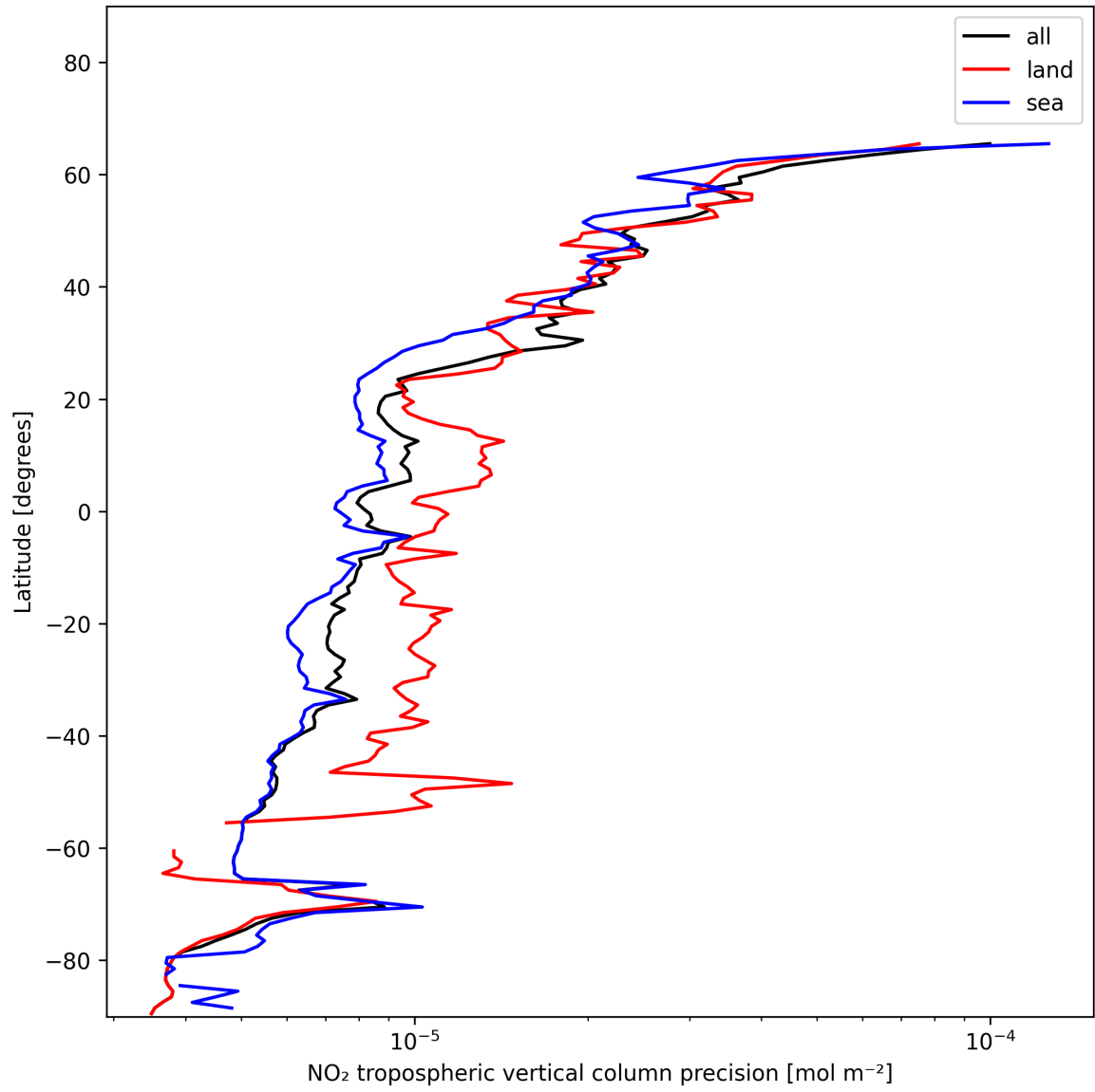
Figure 11: Zonal average of “NO 2 tropospheric vertical column precision” for 2024-12-05 to 2024-12-06.
