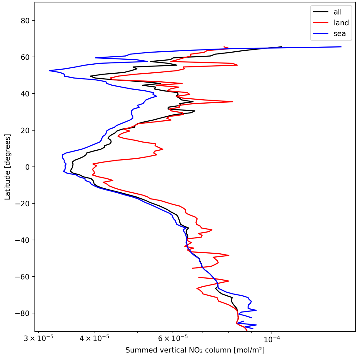
Figure 21: Zonal average of “Summed vertical NO 2 column” for 2024-12-05 to 2024-12-06.
