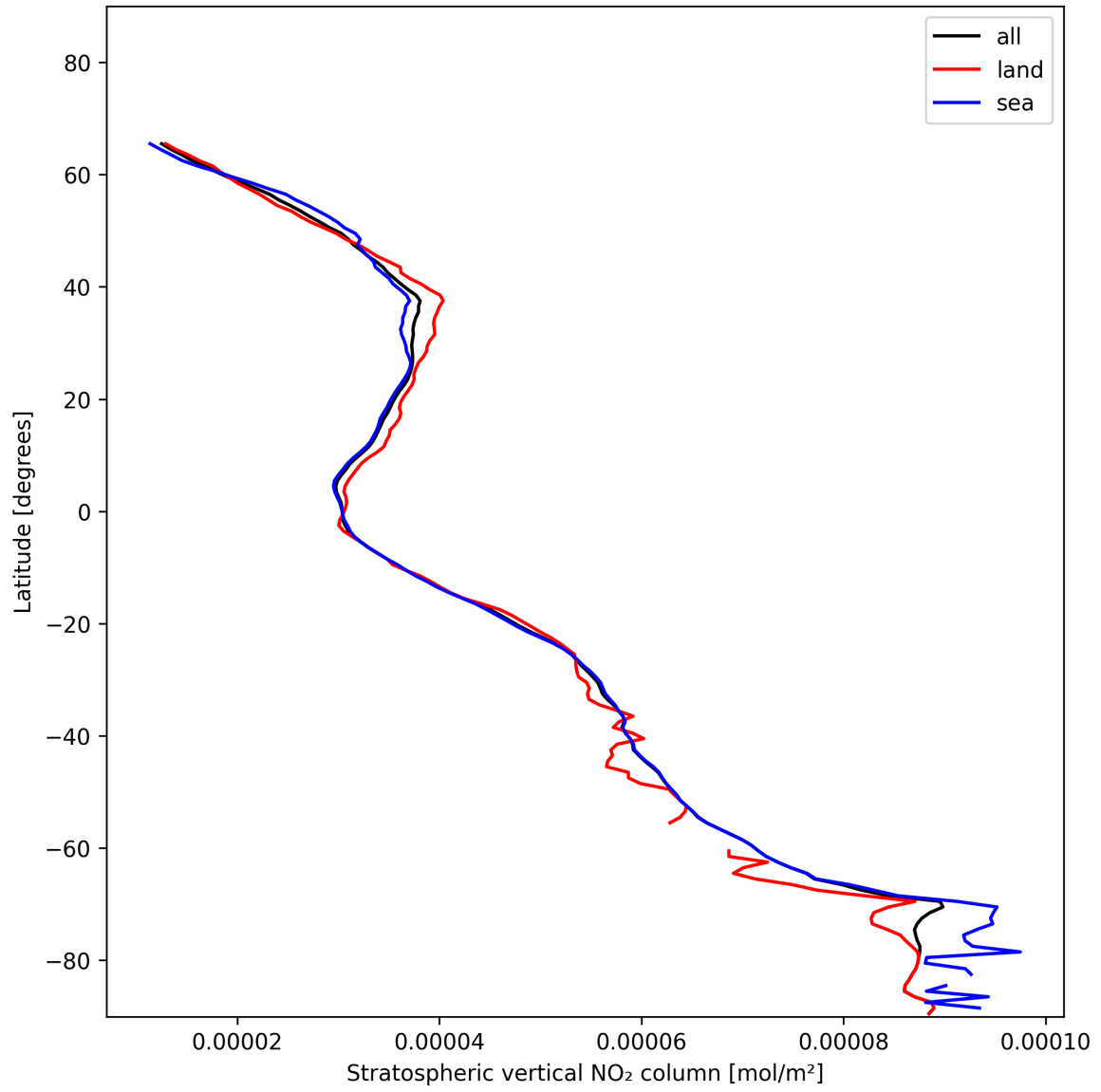
Figure 17: Zonal average of “Stratospheric vertical NO 2 column” for 2024-12-05 to 2024-12-06.
