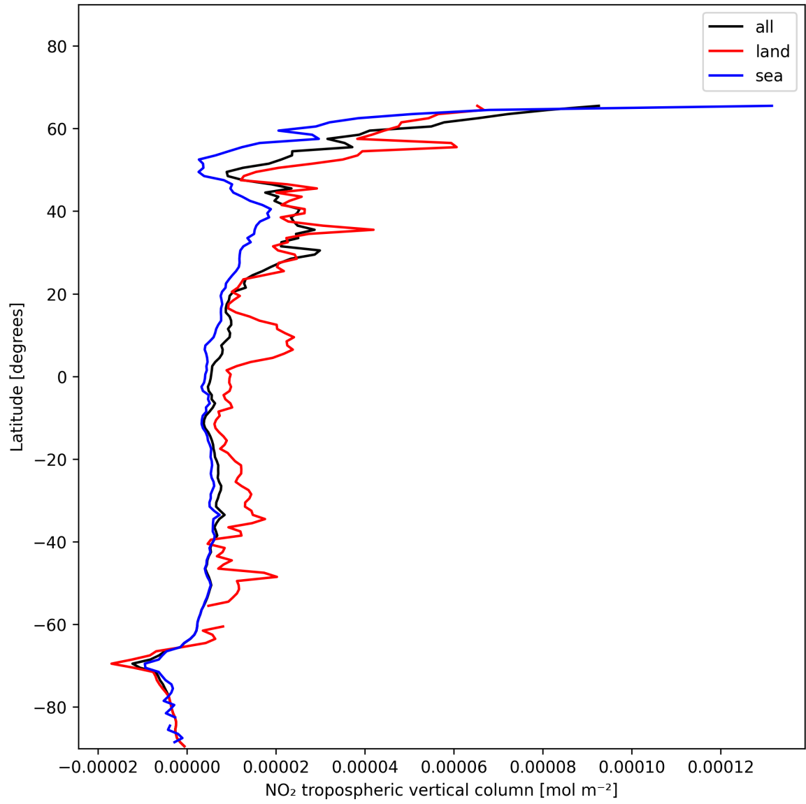
Figure 10: Zonal average of “NO 2 tropospheric vertical column” for 2024-12-05 to 2024-12-06.
