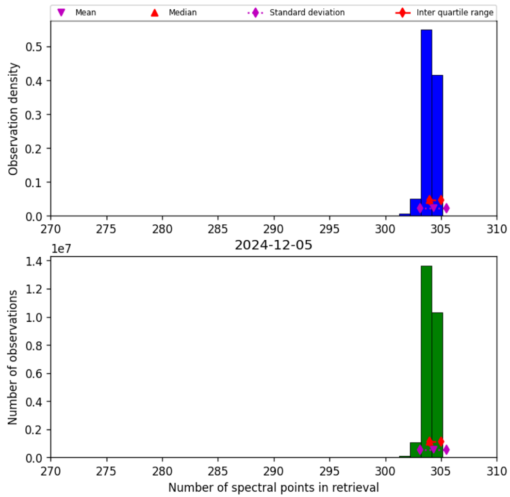
Figure 31: Histogram of “Number of spectral points in retrieval” for 2024-12-05 to 2024-12-06
