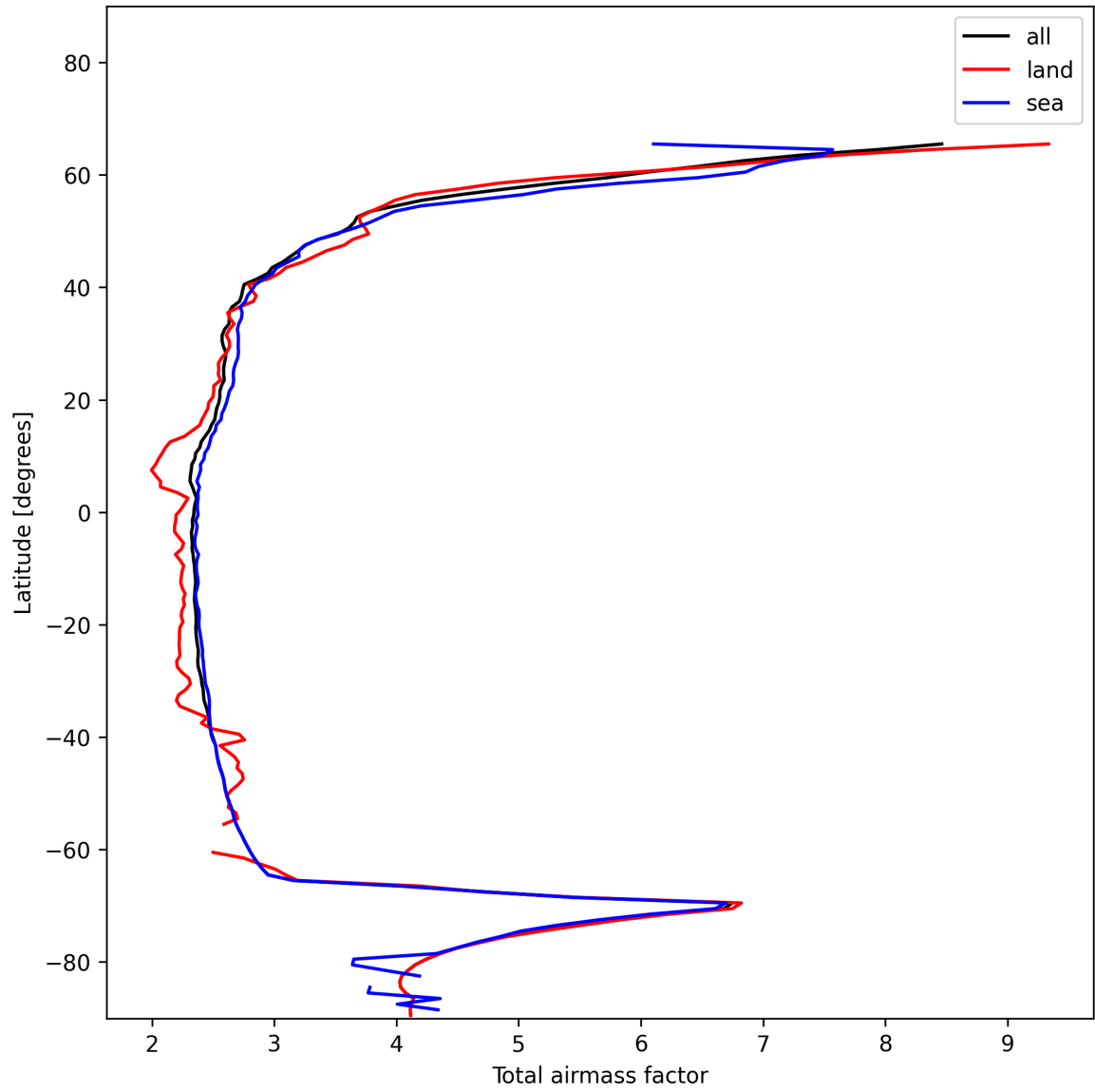
Figure 13: Zonal average of “Total airmass factor” for 2024-12-05 to 2024-12-06.
