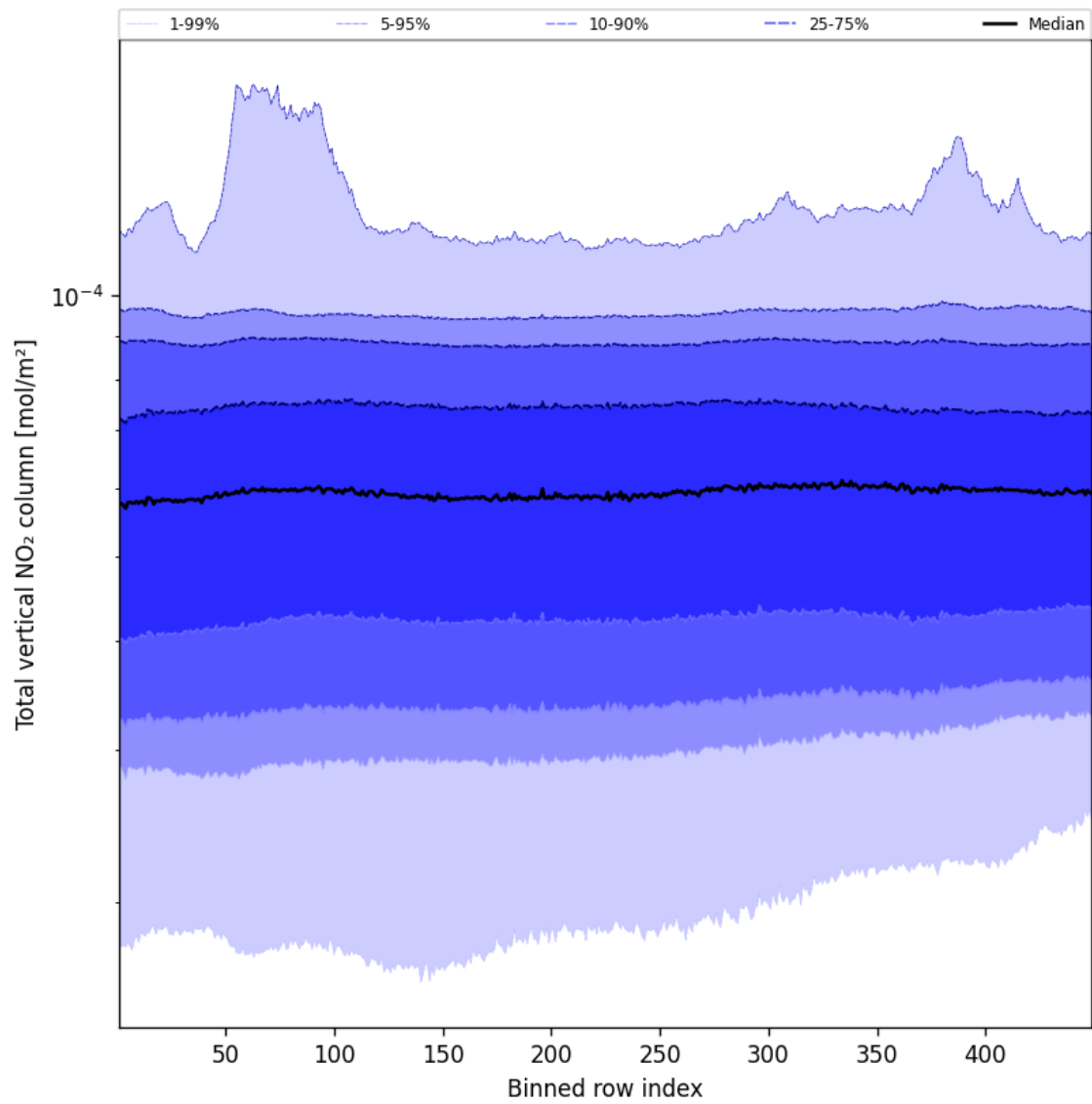
Figure 53: Along track statistics of “Total vertical NO 2 column” for 2024-12-05 to 2024-12-06
