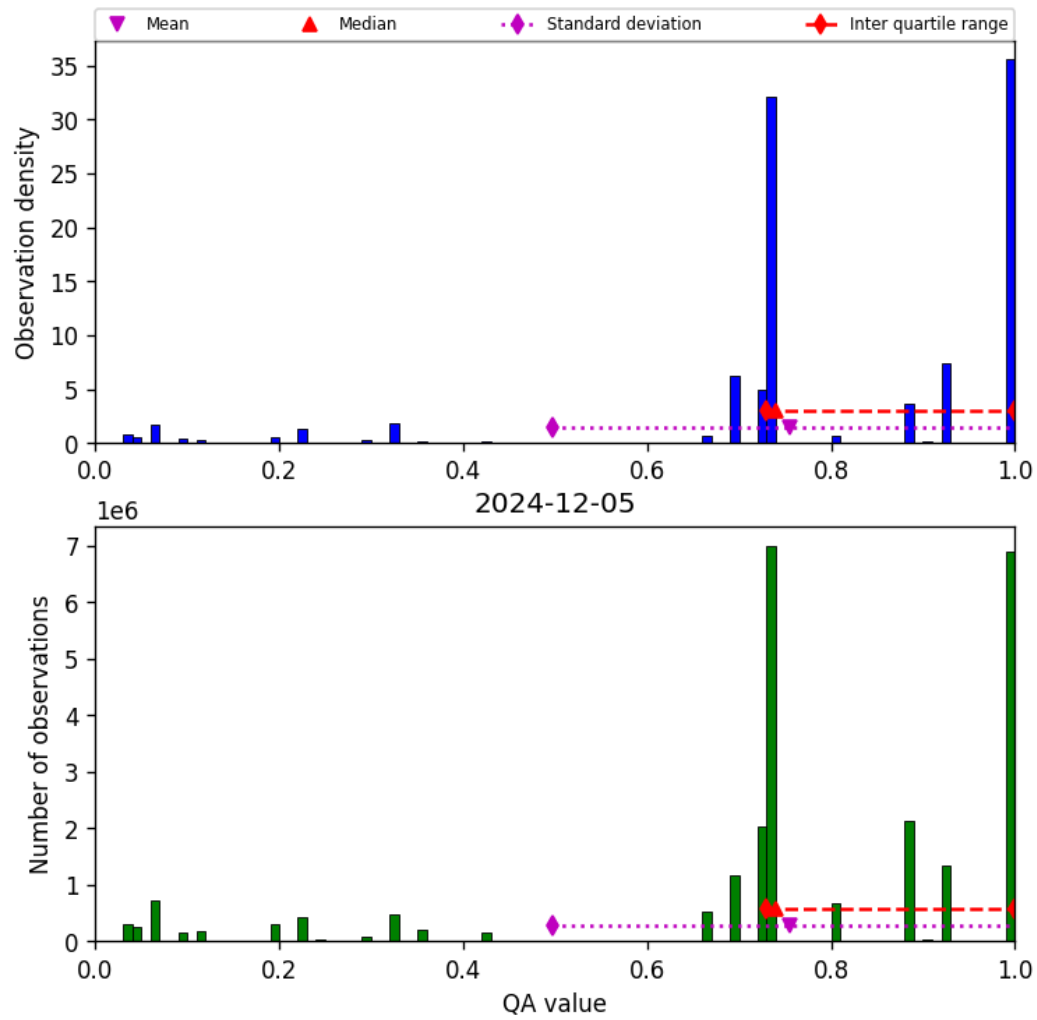
Figure 26: Histogram of “QA value” for 2024-12-05 to 2024-12-06
