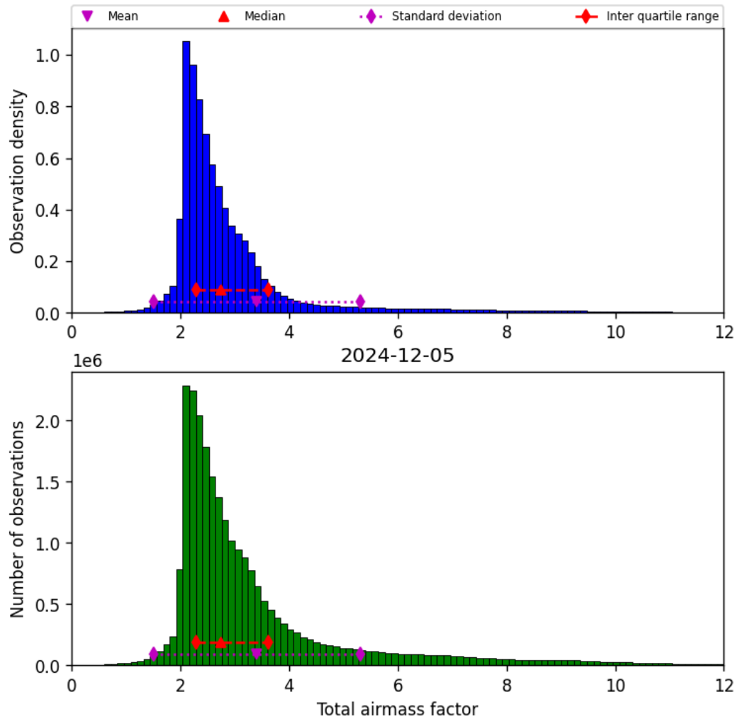
Figure 30: Histogram of “Total airmass factor” for 2024-12-05 to 2024-12-06
