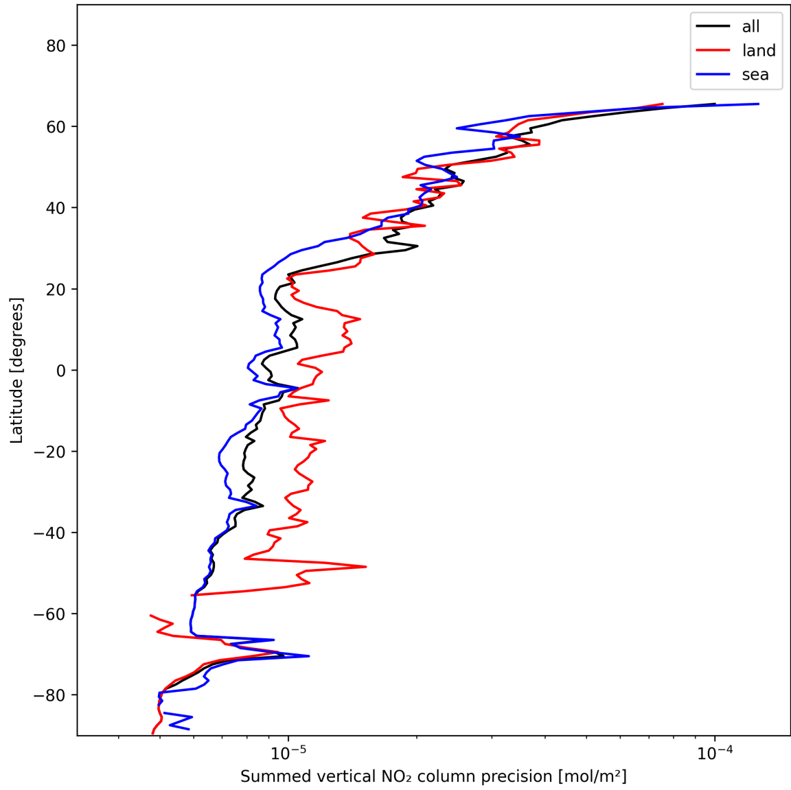
Figure 22: Zonal average of “Summed vertical NO 2 column precision” for 2024-12-05 to 2024-12-06.
