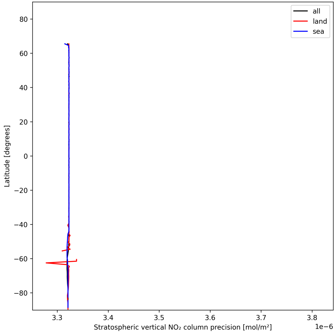
Figure 18: Zonal average of “Stratospheric vertical NO 2 column precision” for 2024-12-05 to 2024-12-06.
