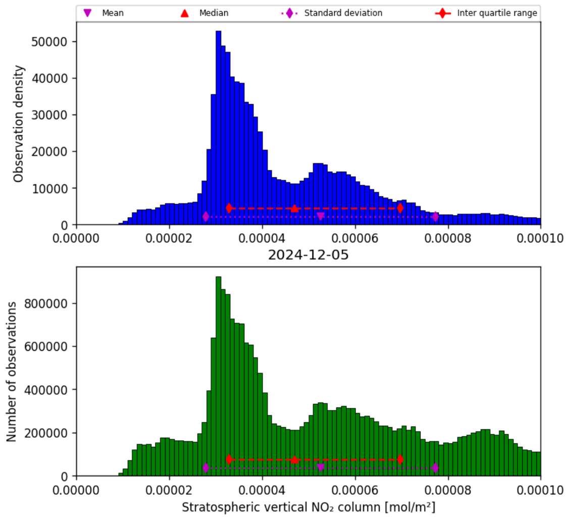
Figure 34: Histogram of “Stratospheric vertical NO 2 column” for 2024-12-05 to 2024-12-06
