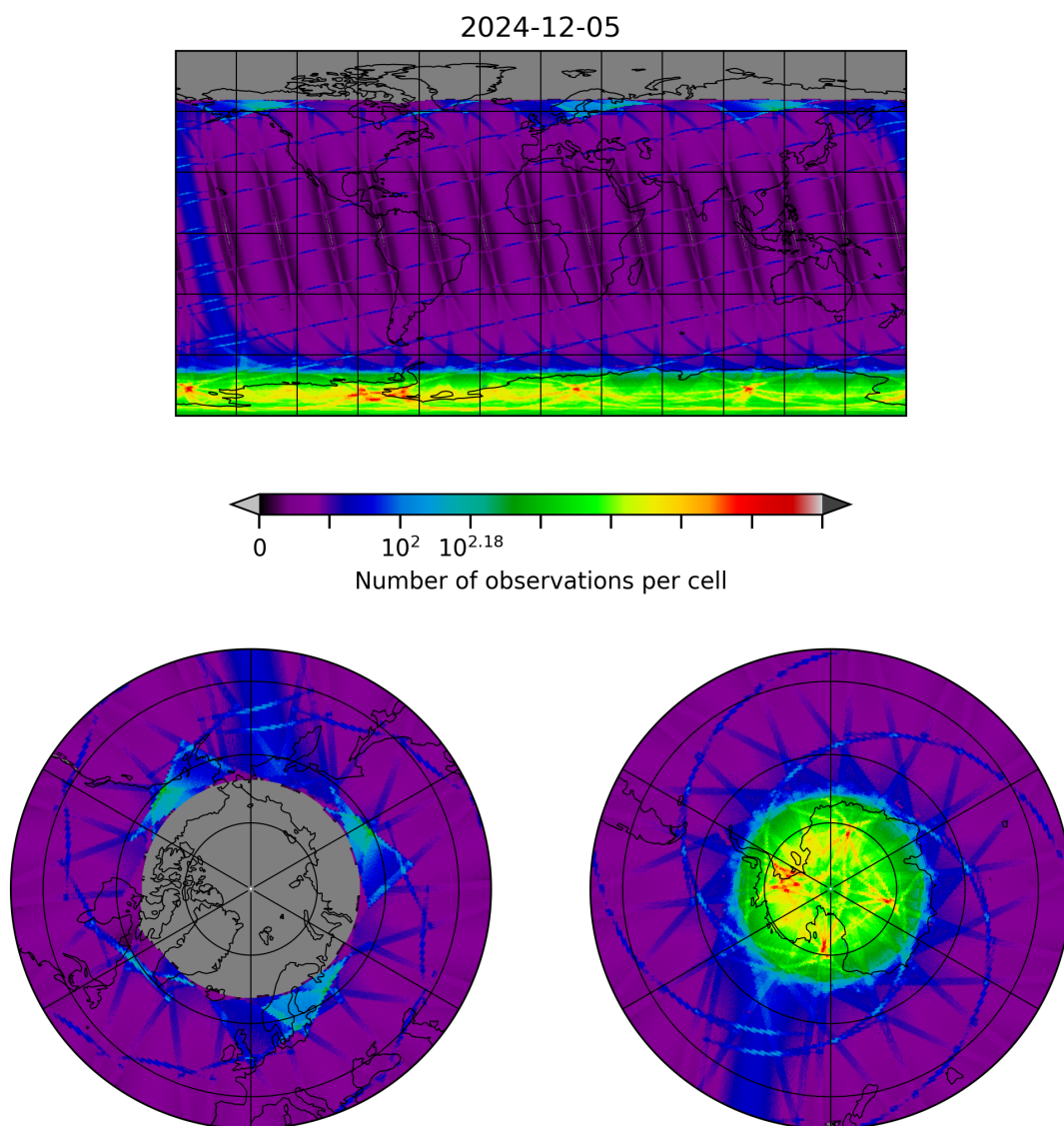
Figure 8: Map of the number of observations for 2024-12-05 to 2024-12-06
