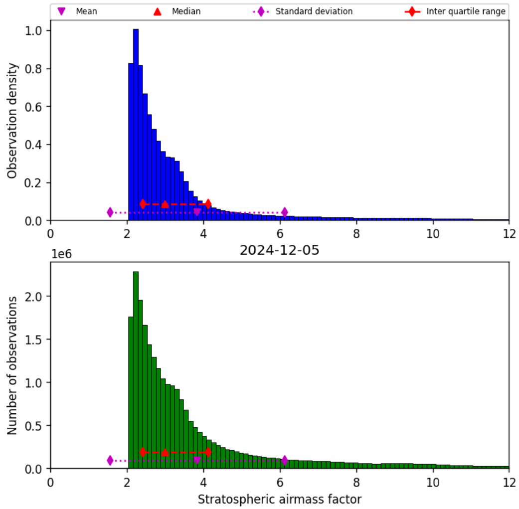
Figure 42: Histogram of “Stratospheric airmass factor” for 2024-12-05 to 2024-12-06
