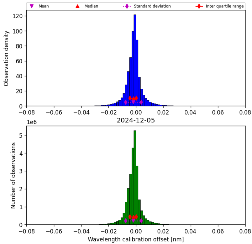
Figure 33: Histogram of “Wavelength calibration offset” for 2024-12-05 to 2024-12-06
