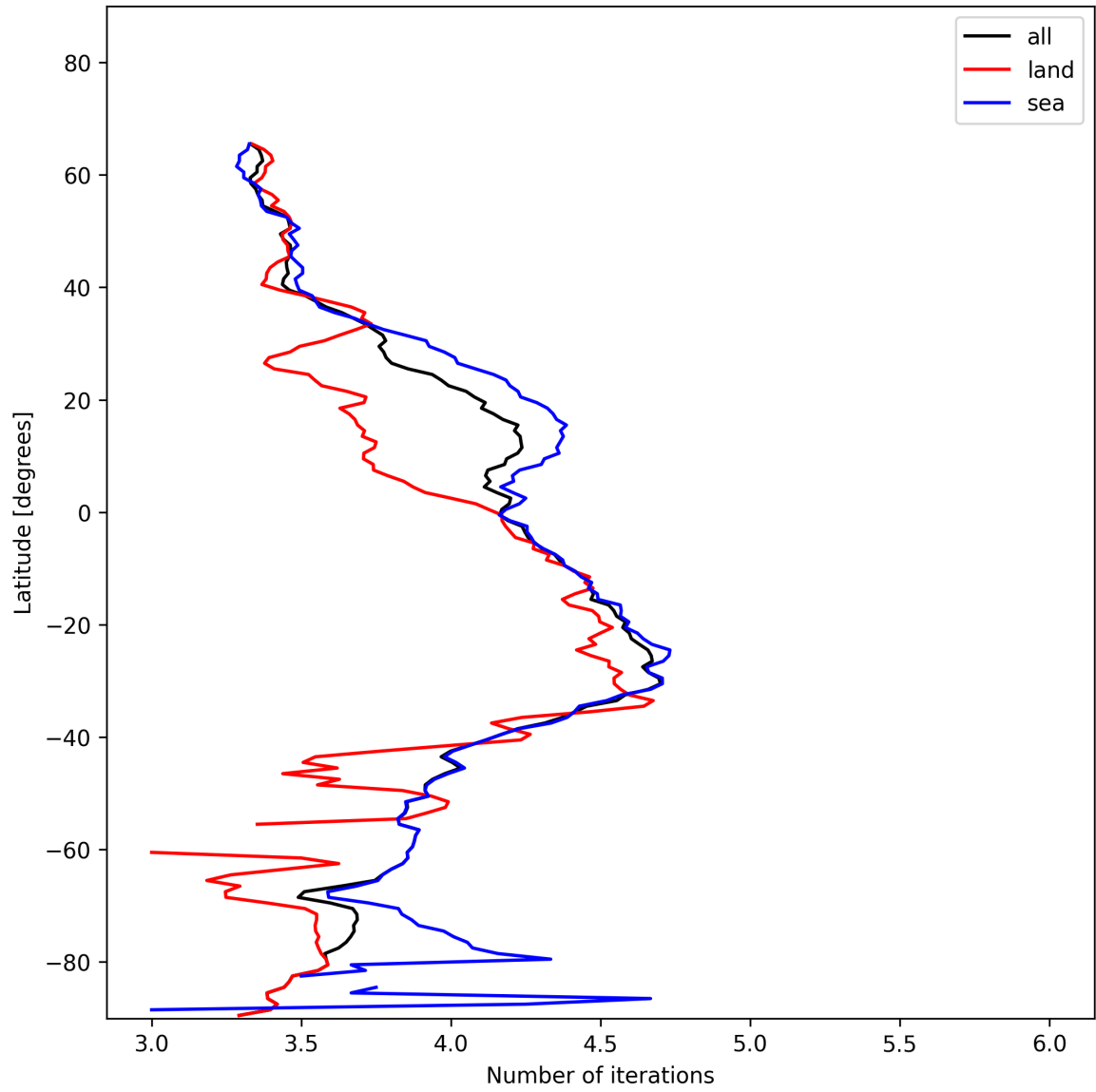
Figure 15: Zonal average of “Number of iterations” for 2024-12-05 to 2024-12-06.
