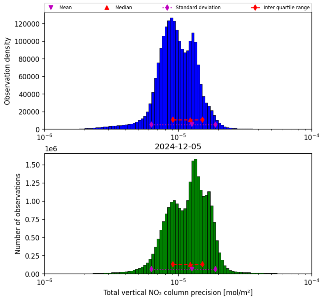
Figure 37: Histogram of “Total vertical NO 2 column precision” for 2024-12-05 to 2024-12-06
