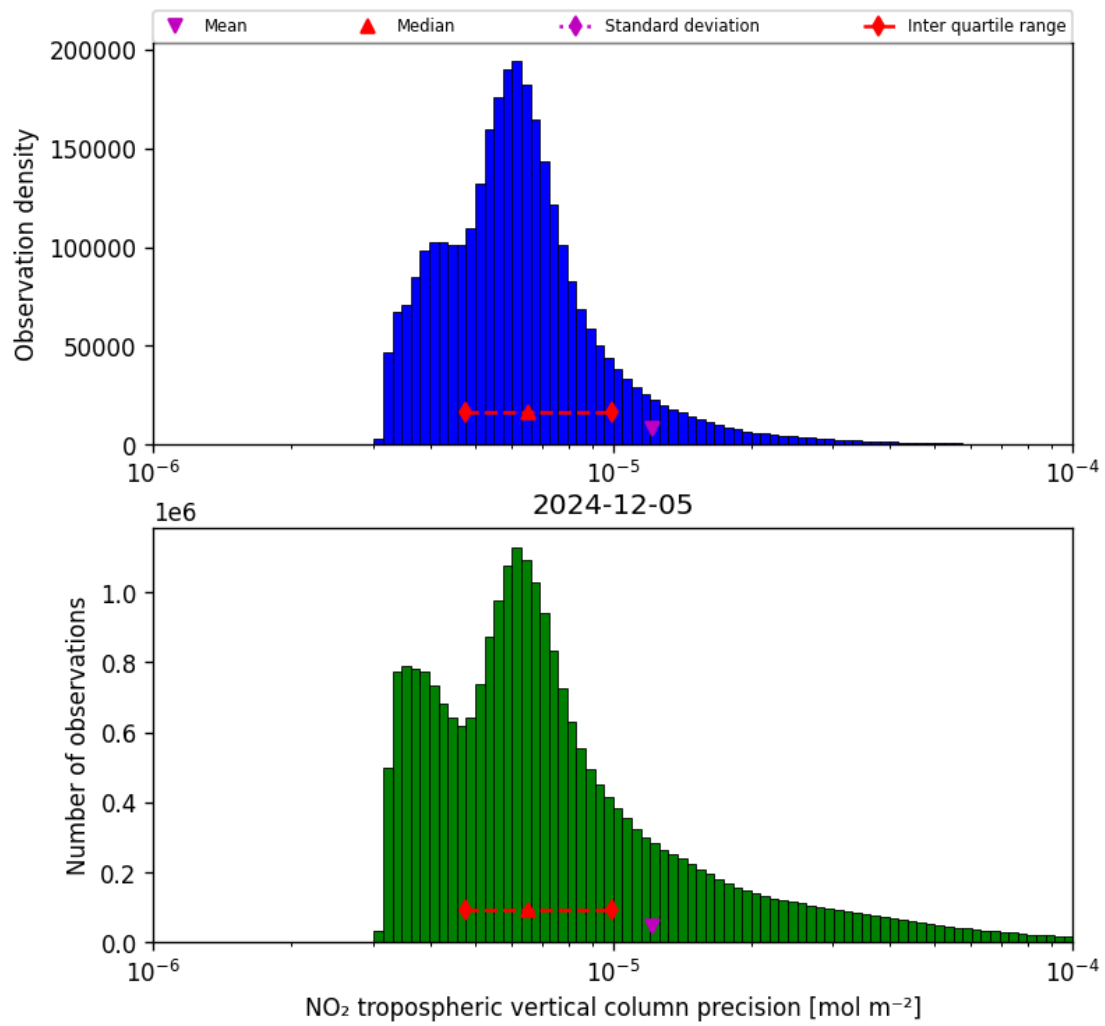
Figure 28: Histogram of “NO 2 tropospheric vertical column precision” for 2024-12-05 to 2024-12-06
