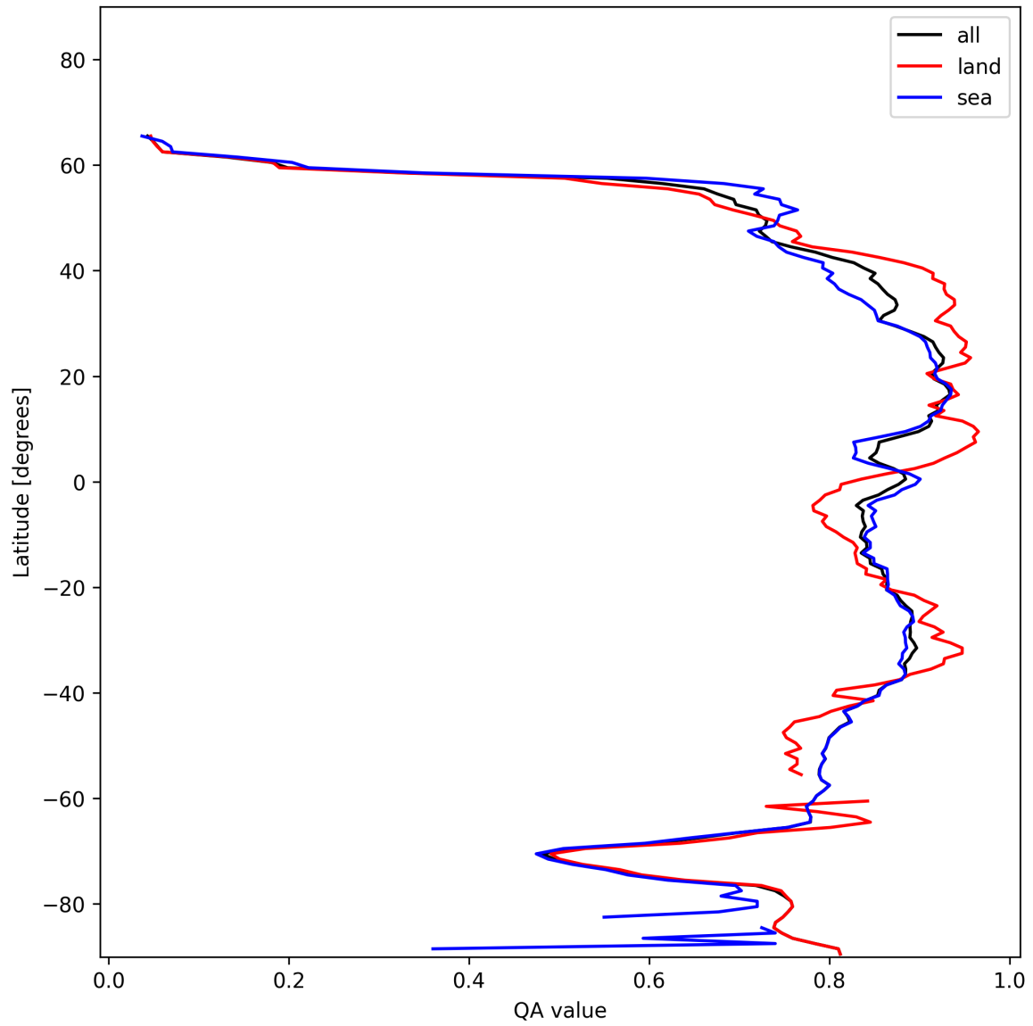
Figure 9: Zonal average of “QA value” for 2024-12-05 to 2024-12-06.
