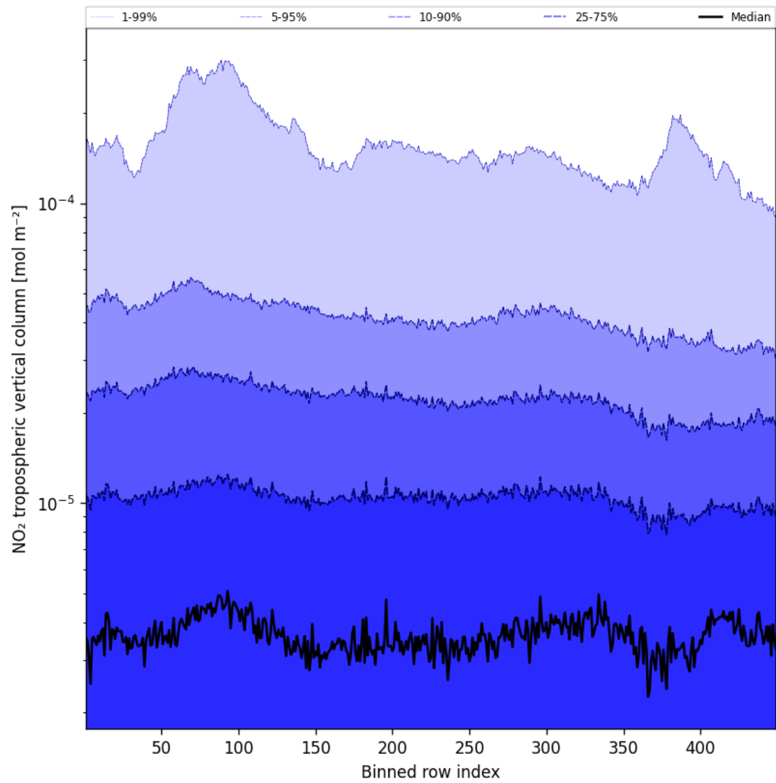
Figure 44: Along track statistics of “NO 2 tropospheric vertical column” for 2024-12-05 to 2024-12-06
