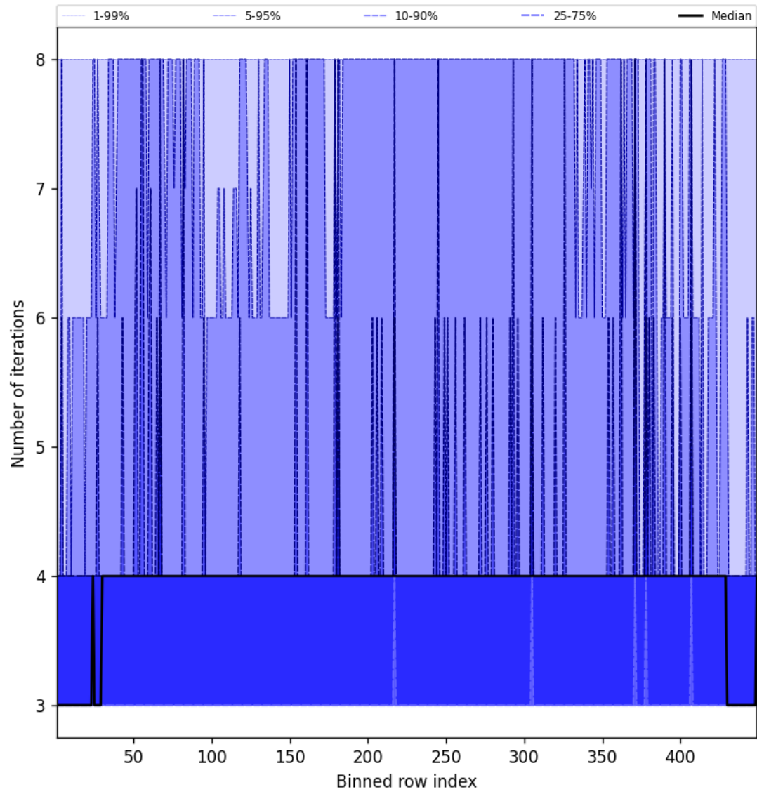
Figure 49: Along track statistics of “Number of iterations” for 2024-12-05 to 2024-12-06
