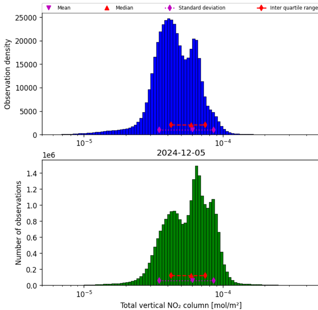
Figure 36: Histogram of “Total vertical NO 2 column” for 2024-12-05 to 2024-12-06
