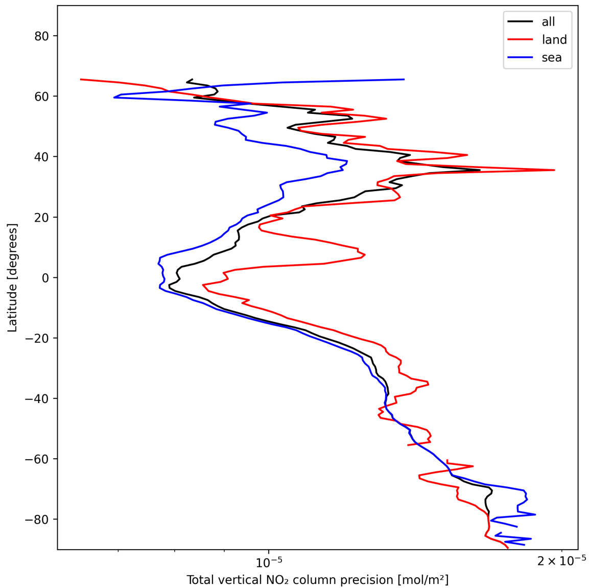
Figure 20: Zonal average of “Total vertical NO 2 column precision” for 2024-12-05 to 2024-12-06.
