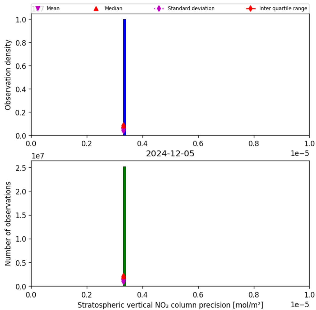
Figure 35: Histogram of “Stratospheric vertical NO 2 column precision” for 2024-12-05 to 2024-12-06
