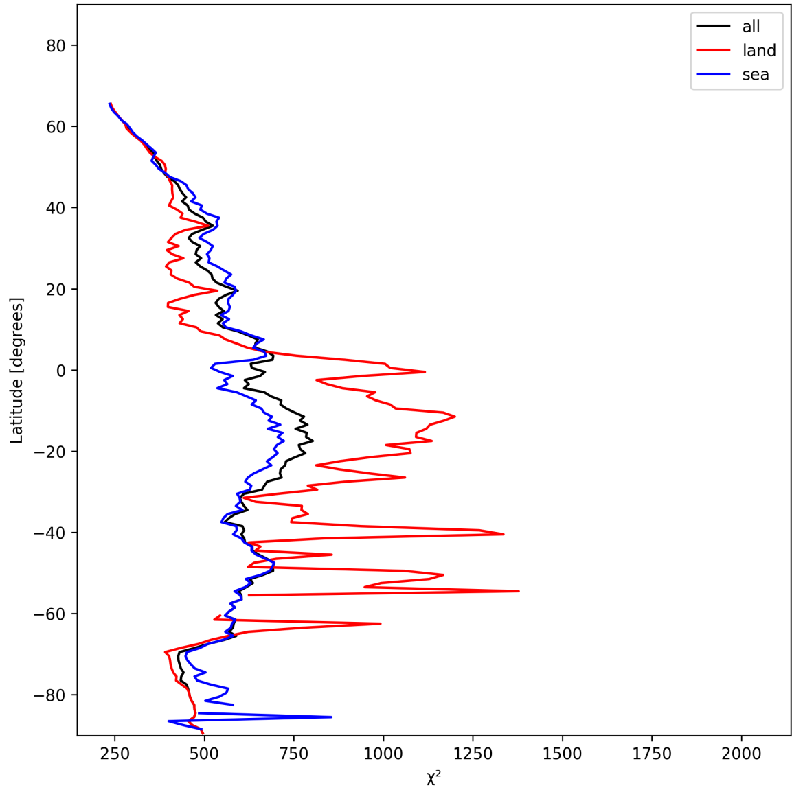
Figure 23: Zonal average of “ \chi^2 ” for 2024-12-05 to 2024-12-06.
