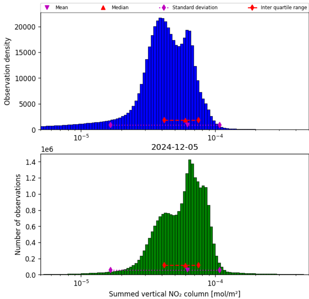
Figure 38: Histogram of “Summed vertical NO 2 column” for 2024-12-05 to 2024-12-06
