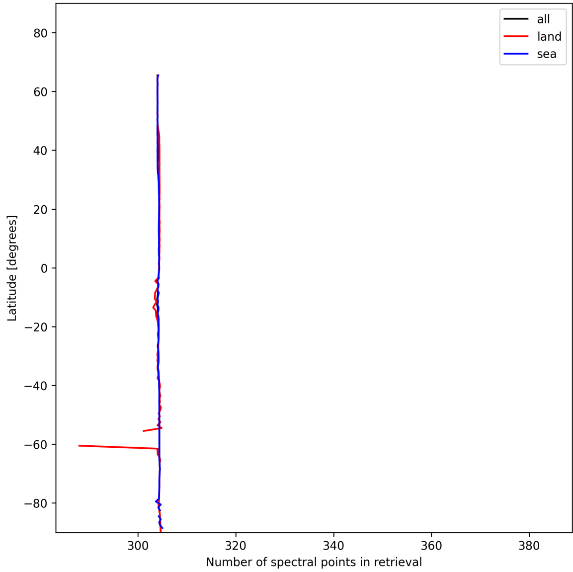
Figure 14: Zonal average of “Number of spectral points in retrieval” for 2024-12-05 to 2024-12-06.
