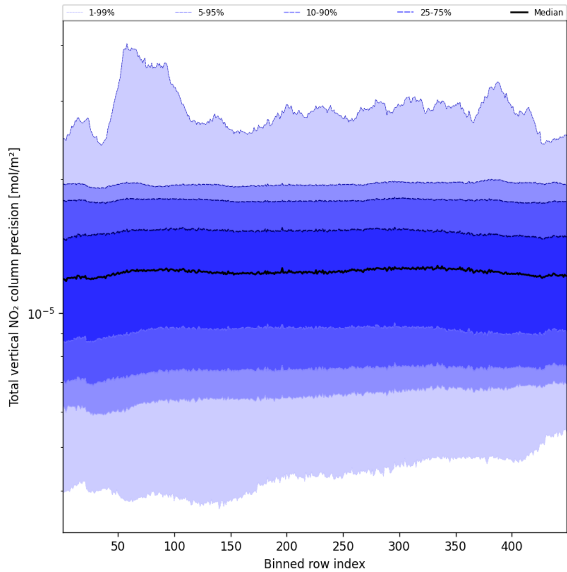
Figure 54: Along track statistics of “Total vertical NO 2 column precision” for 2024-12-05 to 2024-12-06
