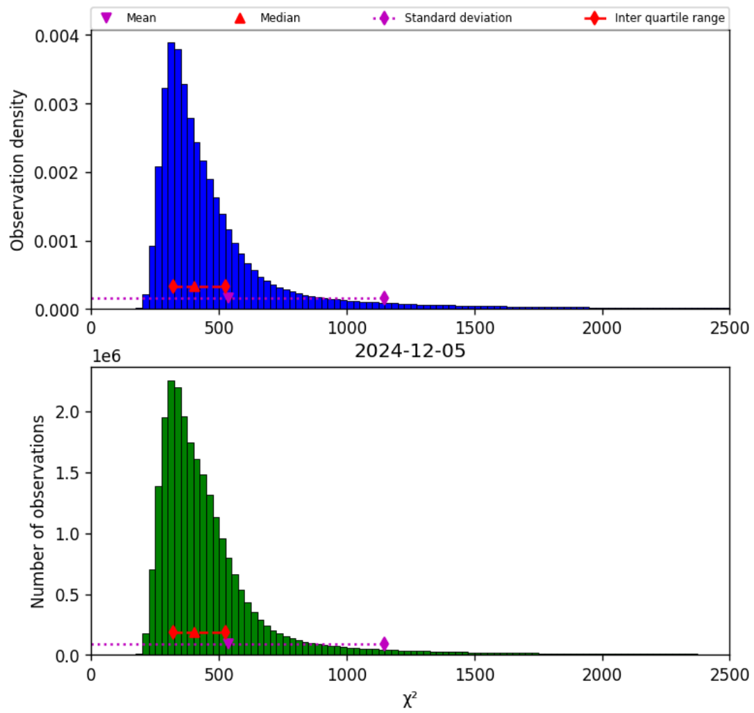
Figure 40: Histogram of “ \chi^2 ” for 2024-12-05 to 2024-12-06
