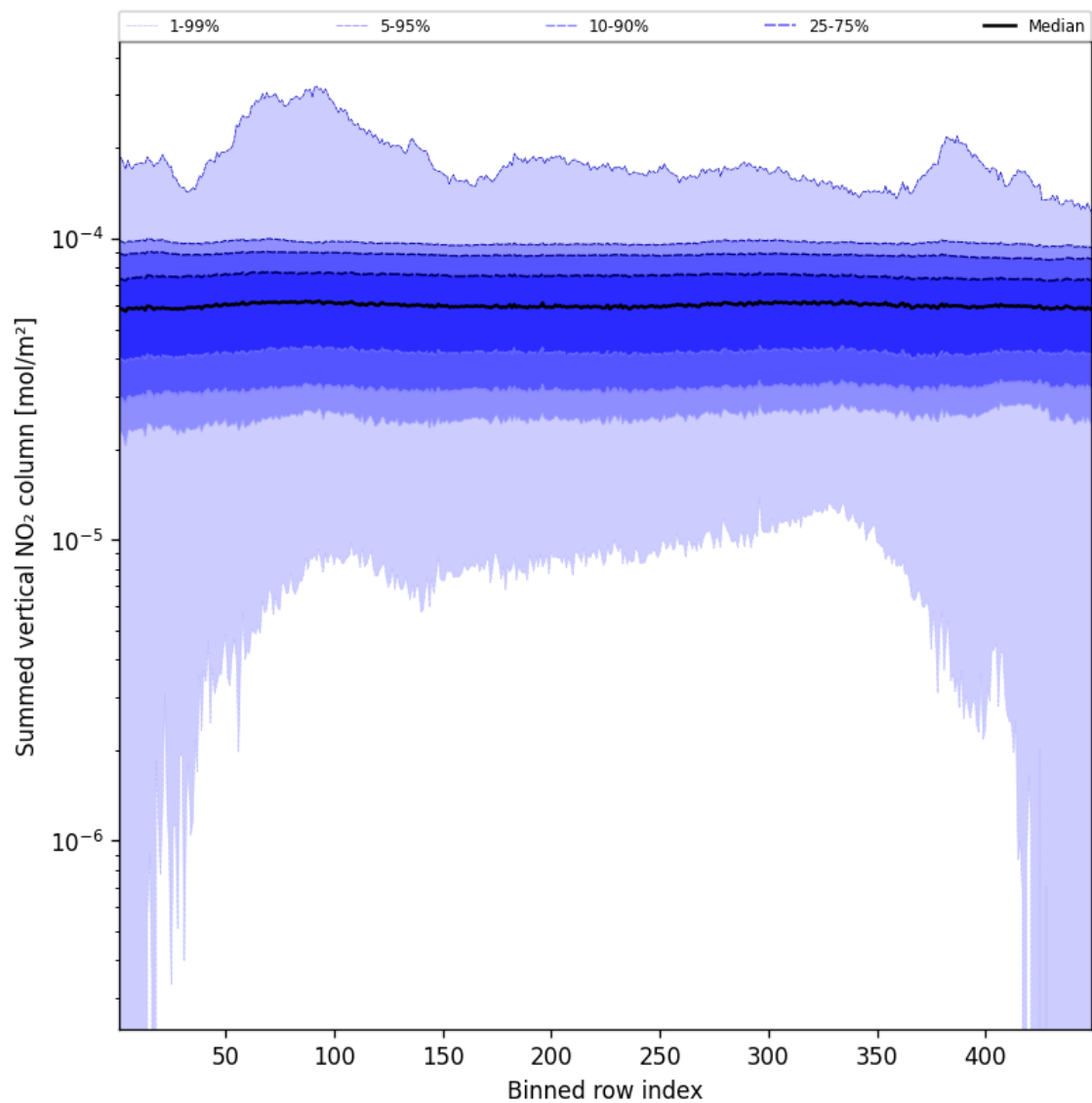
Figure 55: Along track statistics of “Summed vertical NO 2 column” for 2024-12-05 to 2024-12-06
