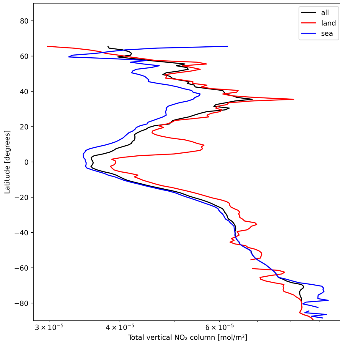
Figure 19: Zonal average of “Total vertical NO 2 column” for 2024-12-05 to 2024-12-06.
