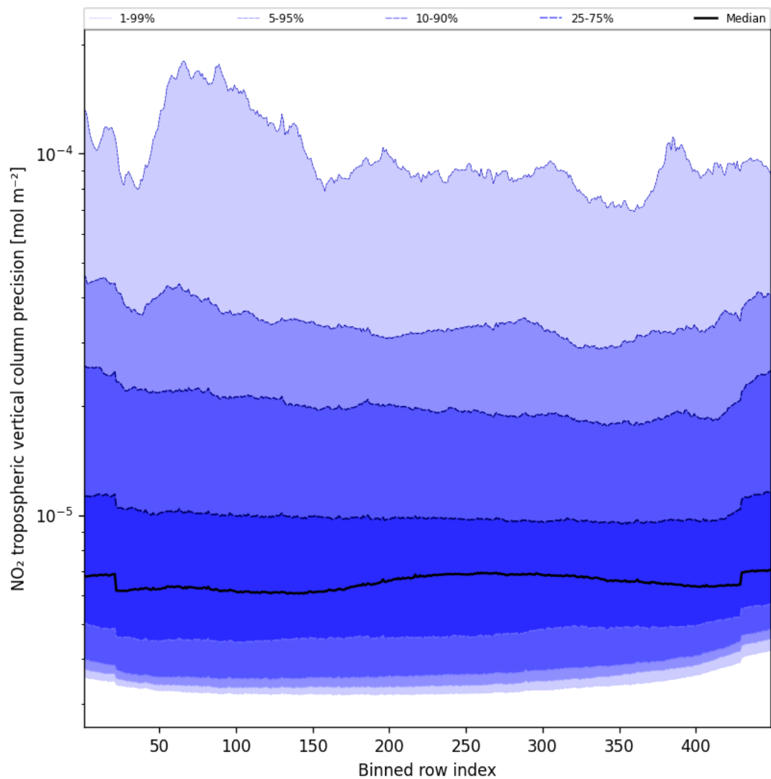
Figure 45: Along track statistics of “NO 2 tropospheric vertical column precision” for 2024-12-05 to 2024-12-06
