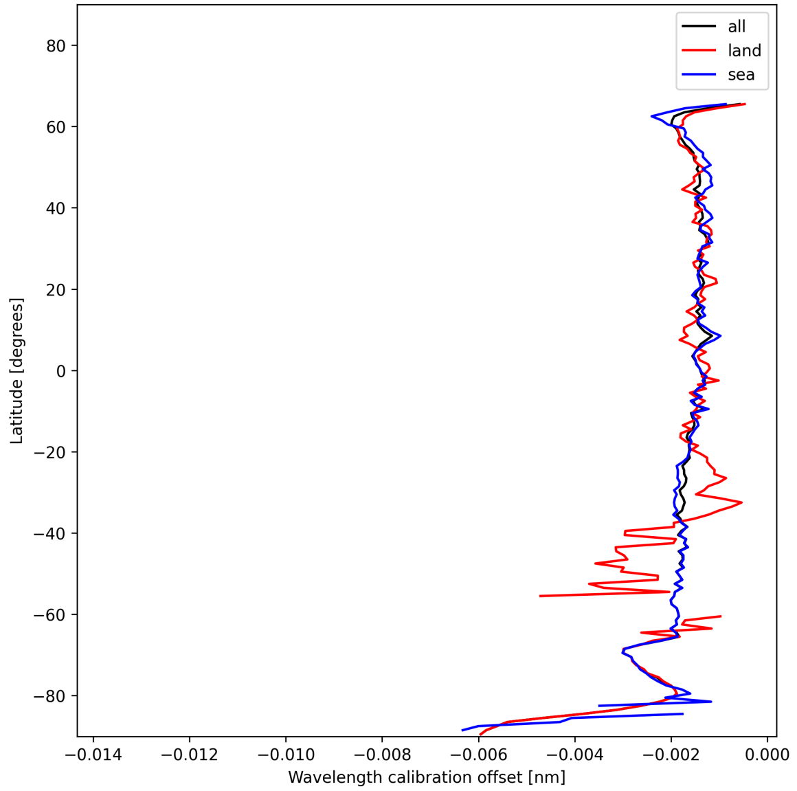
Figure 16: Zonal average of “Wavelength calibration offset” for 2024-12-05 to 2024-12-06.
