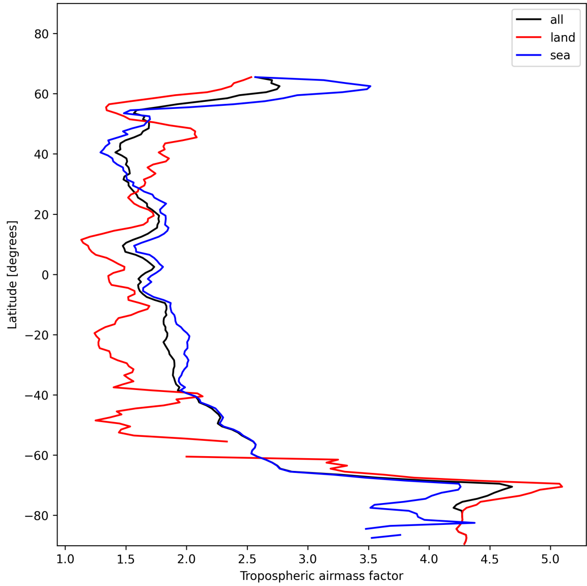
Figure 12: Zonal average of “Tropospheric airmass factor” for 2024-12-06 to 2024-12-07.
