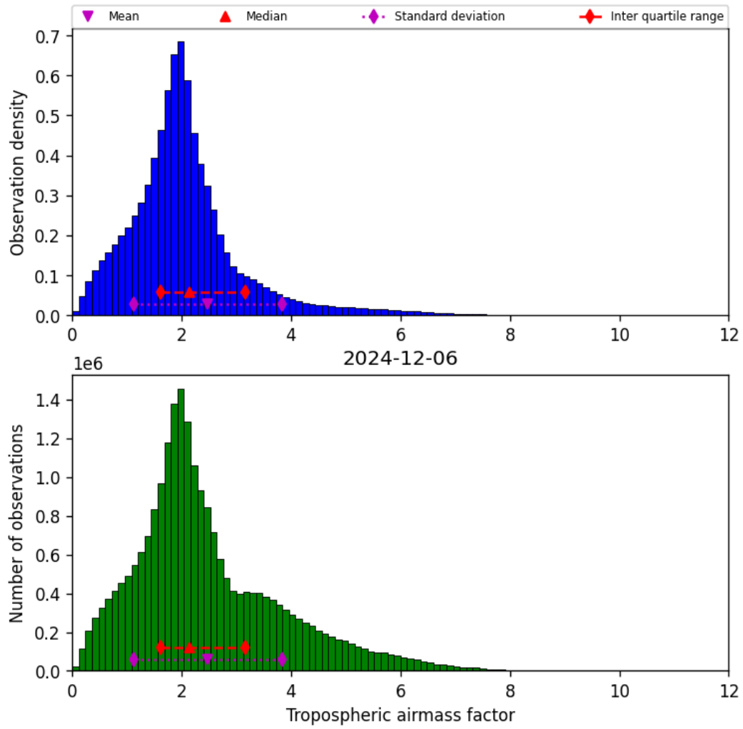
Figure 29: Histogram of “Tropospheric airmass factor” for 2024-12-06 to 2024-12-07
