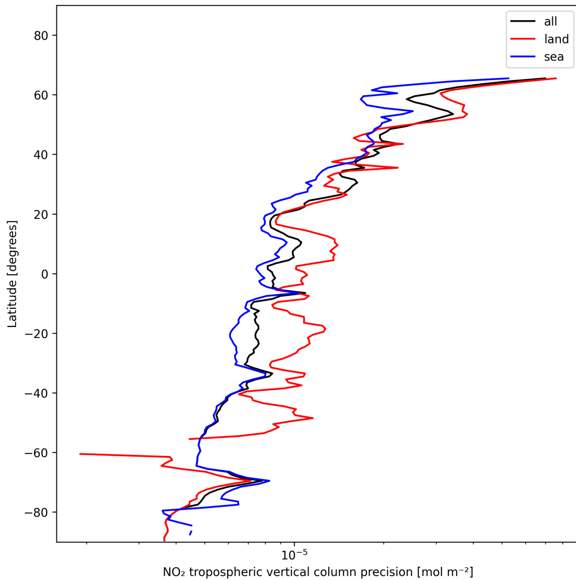
Figure 11: Zonal average of “NO 2 tropospheric vertical column precision” for 2024-12-06 to 2024-12-07.
