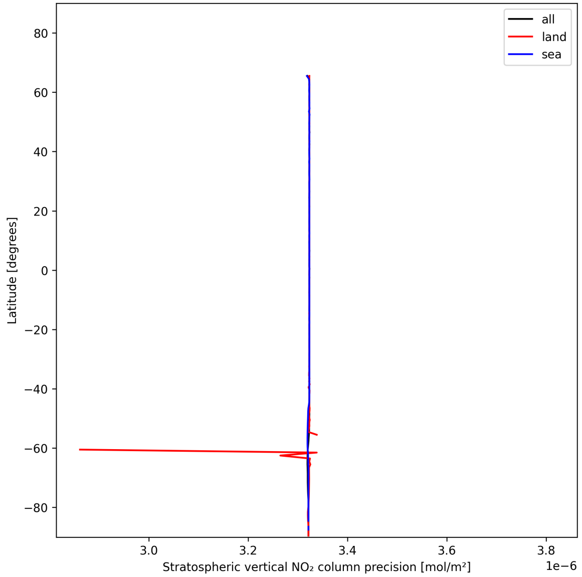
Figure 18: Zonal average of “Stratospheric vertical NO 2 column precision” for 2024-12-06 to 2024-12-07.
