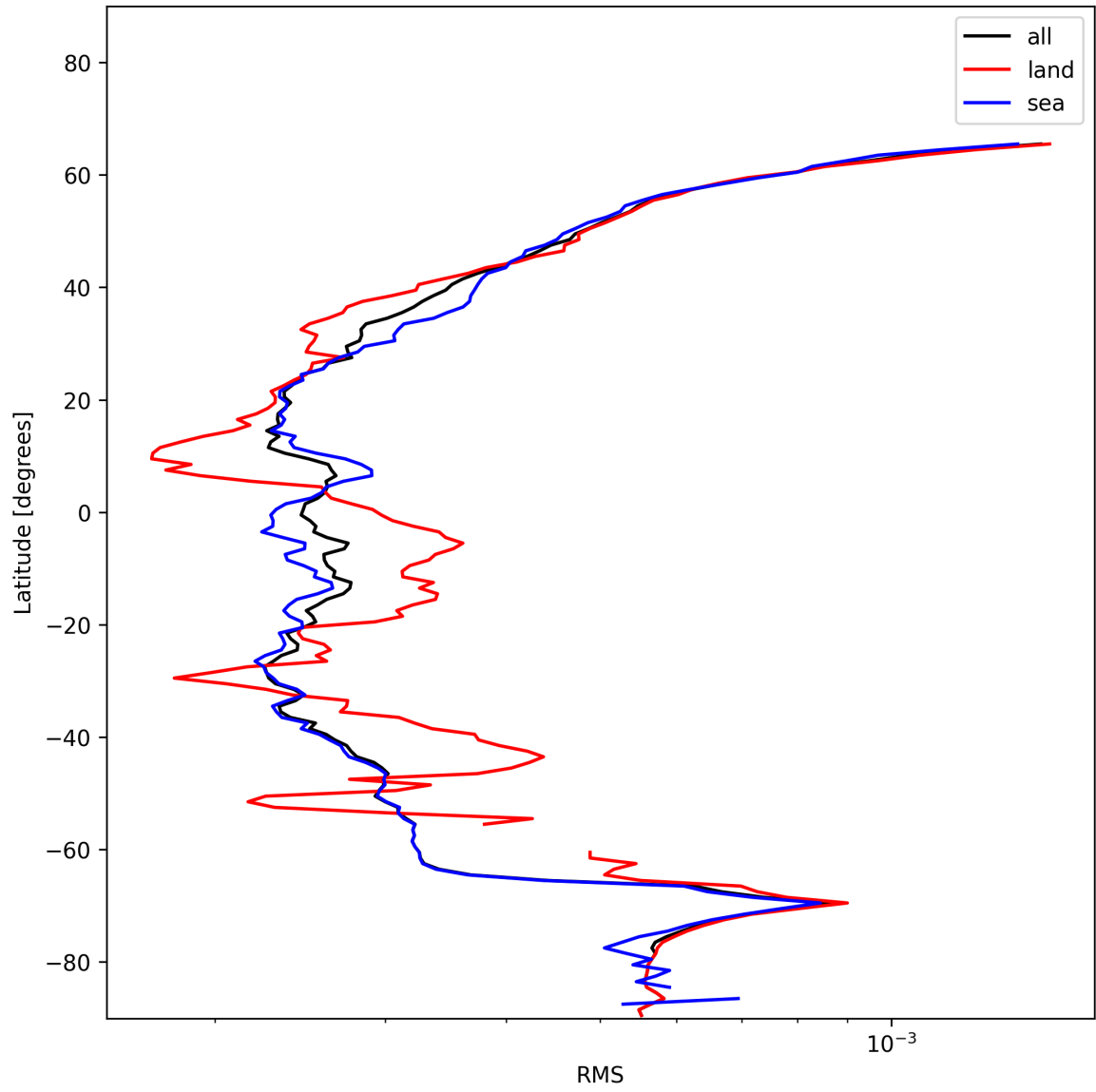
Figure 24: Zonal average of “RMS” for 2024-12-06 to 2024-12-07.
