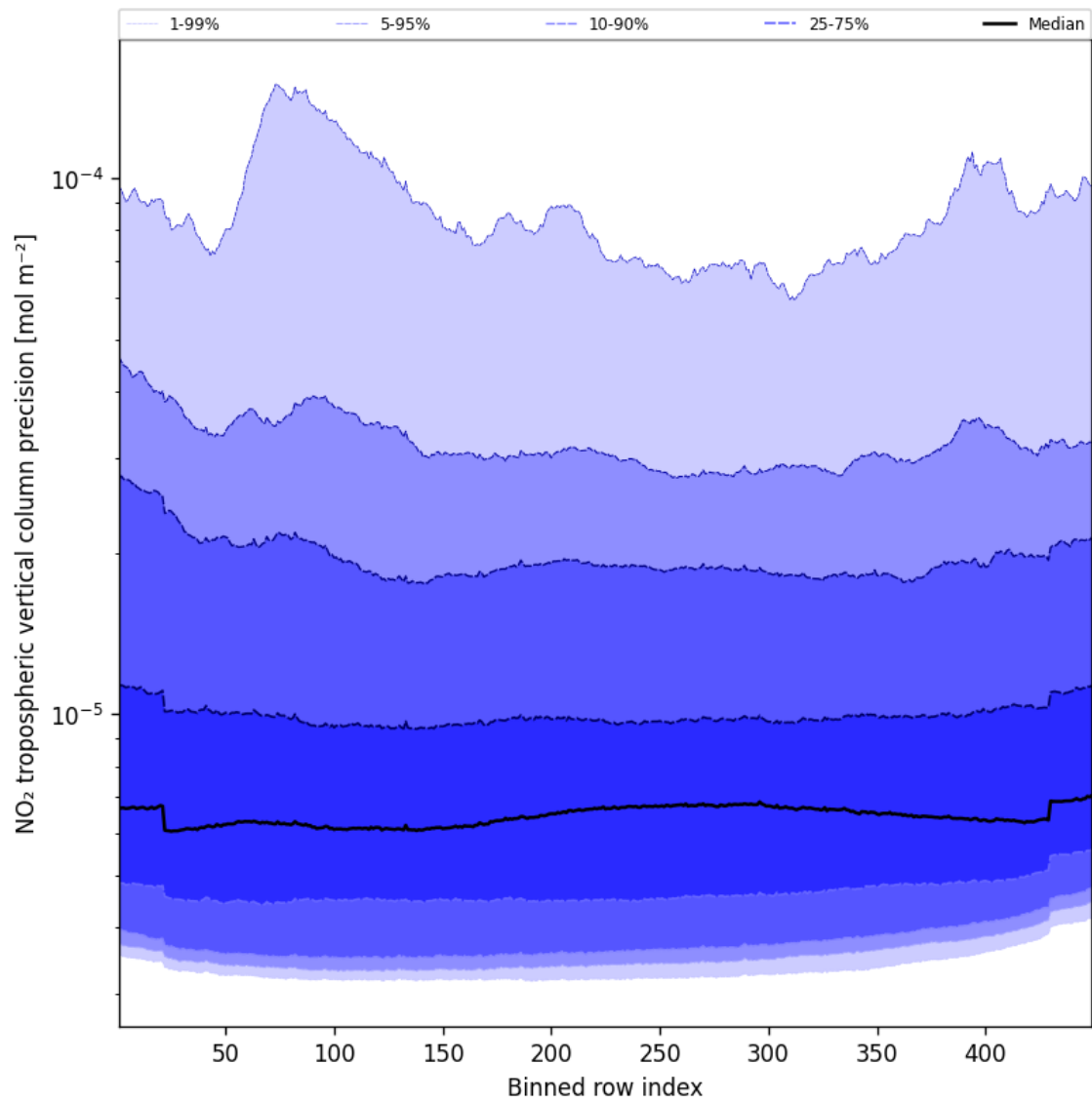
Figure 45: Along track statistics of “NO 2 tropospheric vertical column precision” for 2024-12-06 to 2024-12-07
