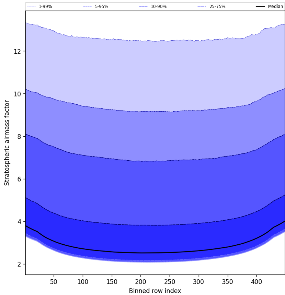
Figure 59: Along track statistics of “Stratospheric airmass factor” for 2024-12-06 to 2024-12-07
