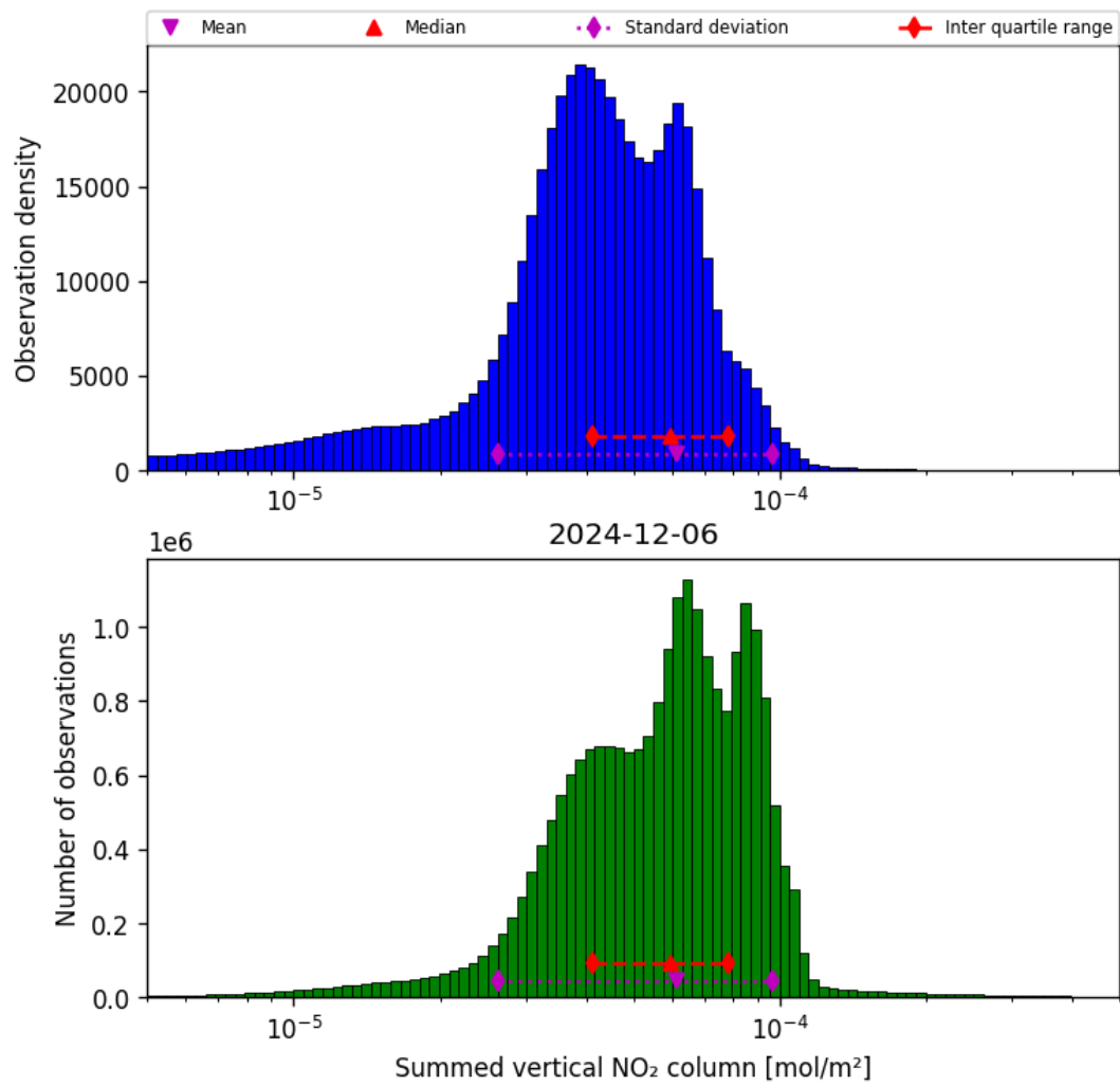
Figure 38: Histogram of “Summed vertical NO 2 column” for 2024-12-06 to 2024-12-07
