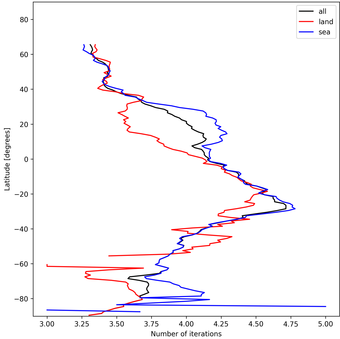
Figure 15: Zonal average of “Number of iterations” for 2024-12-06 to 2024-12-07.
