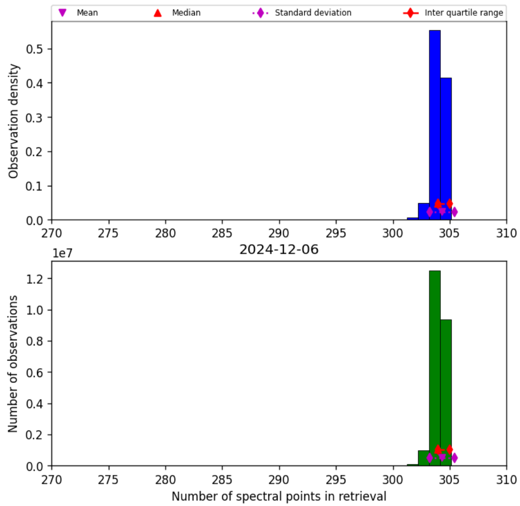
Figure 31: Histogram of “Number of spectral points in retrieval” for 2024-12-06 to 2024-12-07
