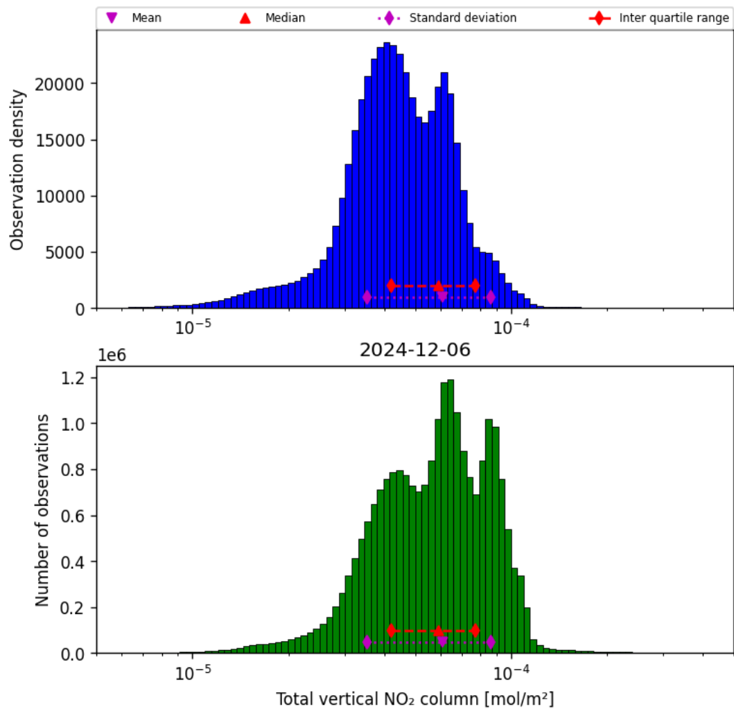
Figure 36: Histogram of “Total vertical NO 2 column” for 2024-12-06 to 2024-12-07
