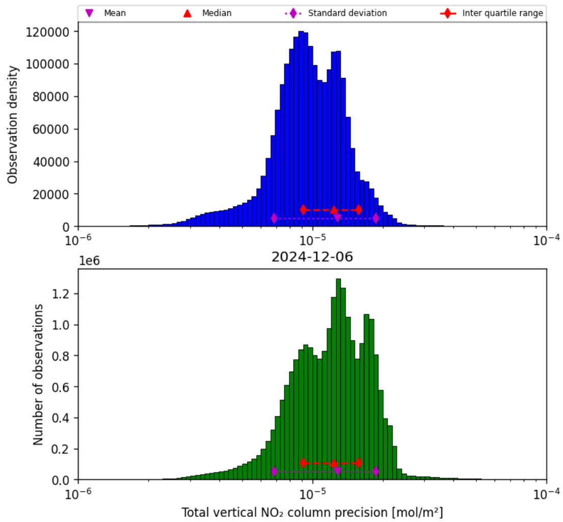
Figure 37: Histogram of “Total vertical NO 2 column precision” for 2024-12-06 to 2024-12-07
