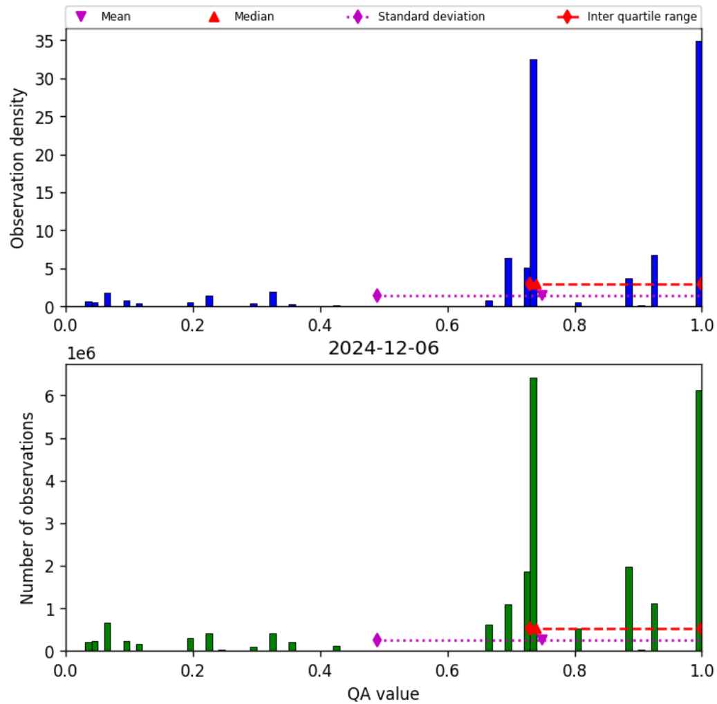
Figure 26: Histogram of “QA value” for 2024-12-06 to 2024-12-07
