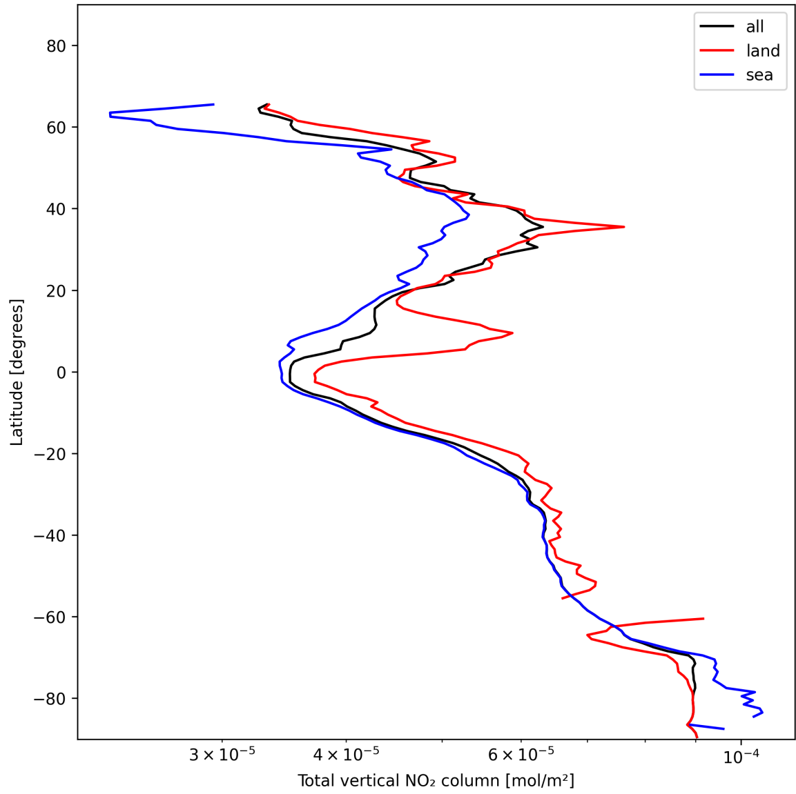
Figure 19: Zonal average of “Total vertical NO 2 column” for 2024-12-06 to 2024-12-07.
