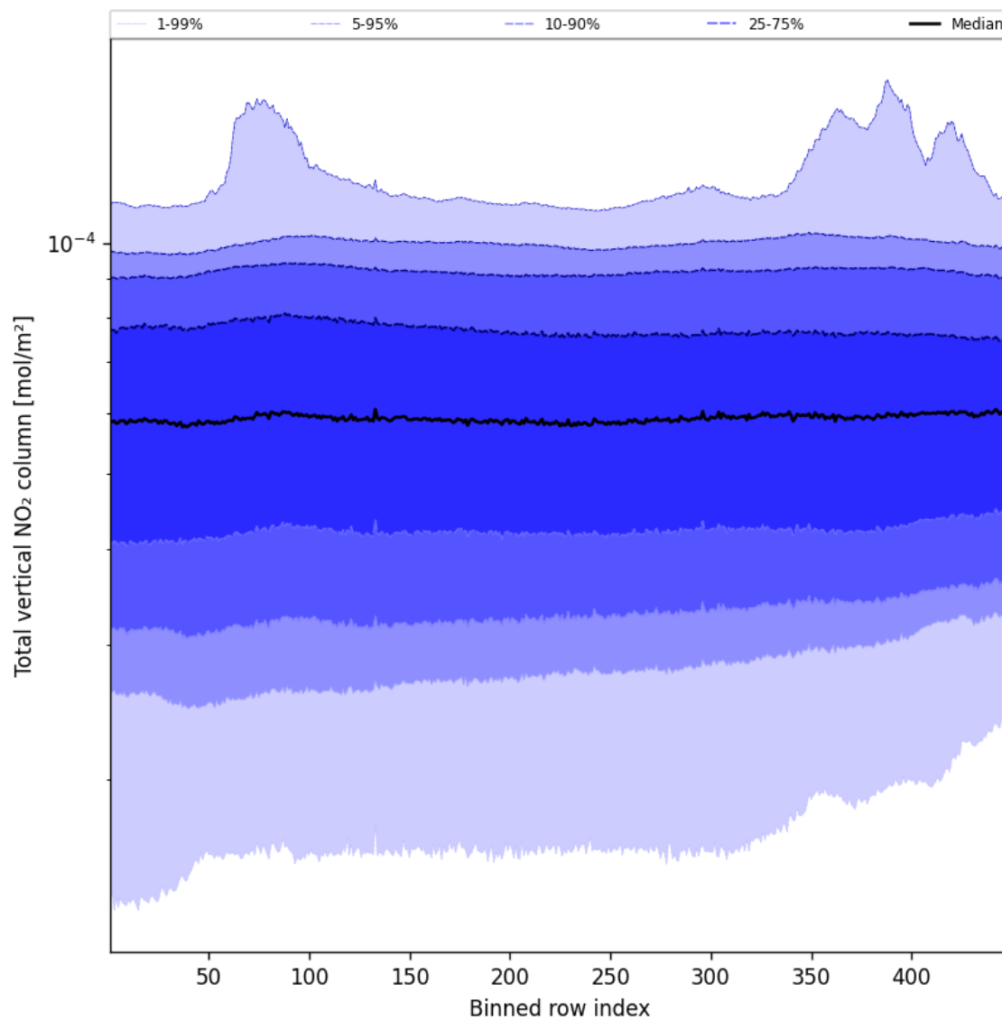
Figure 53: Along track statistics of "Total vertical NO 2 column" for 2024-12-06 to 2024-12-07
