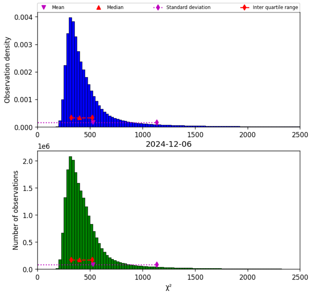
Figure 40: Histogram of “ \chi^2 ” for 2024-12-06 to 2024-12-07
