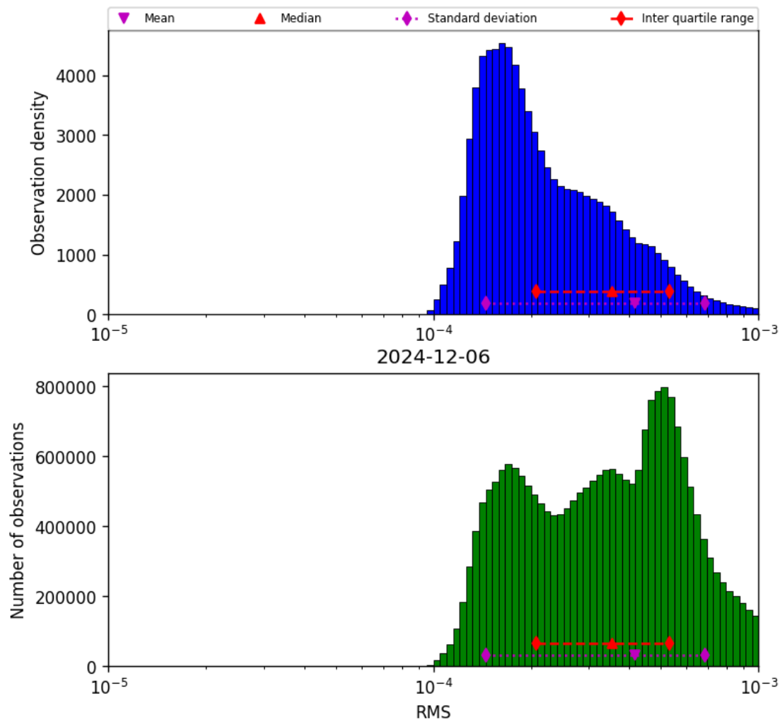
Figure 41: Histogram of “RMS” for 2024-12-06 to 2024-12-07
