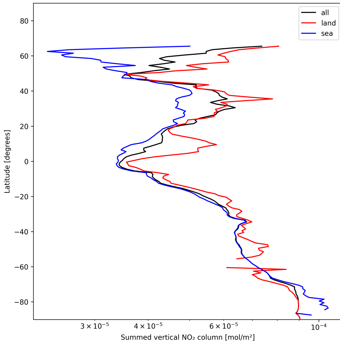
Figure 21: Zonal average of “Summed vertical NO 2 column” for 2024-12-06 to 2024-12-07.
