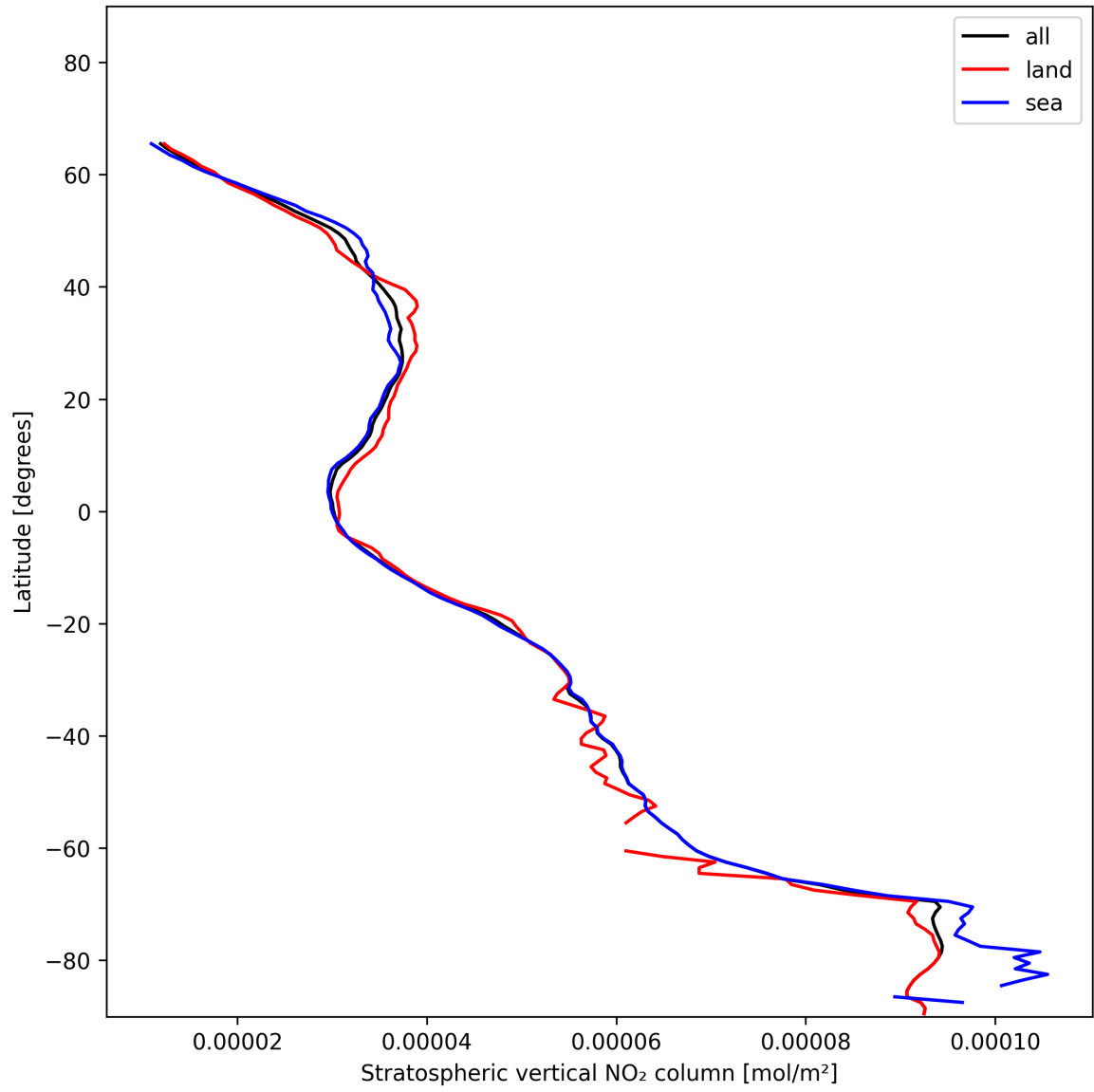
Figure 17: Zonal average of “Stratospheric vertical NO 2 column” for 2024-12-06 to 2024-12-07.
