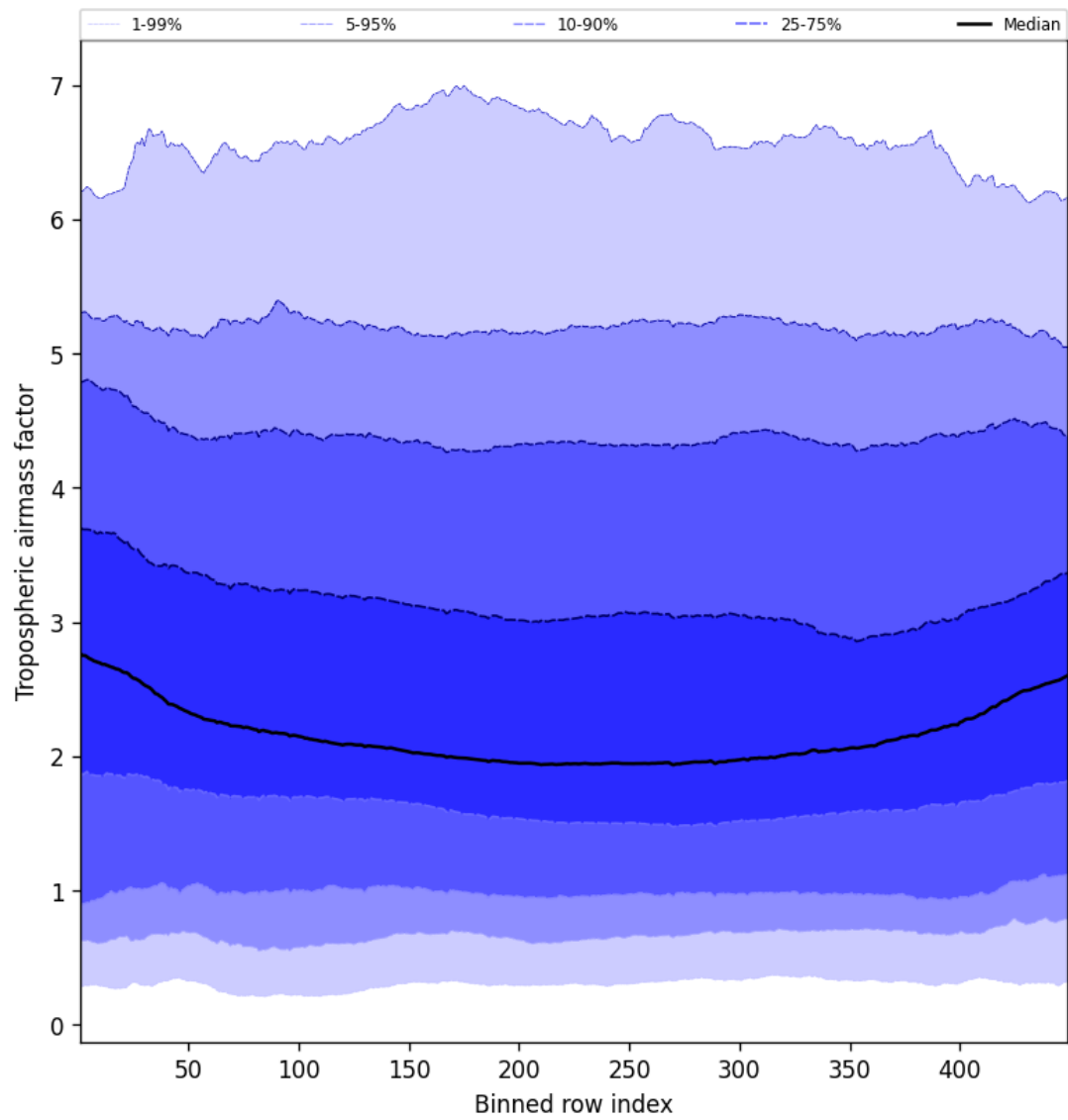
Figure 46: Along track statistics of “Tropospheric air mass factor” for 2024-12-06 to 2024-12-07
