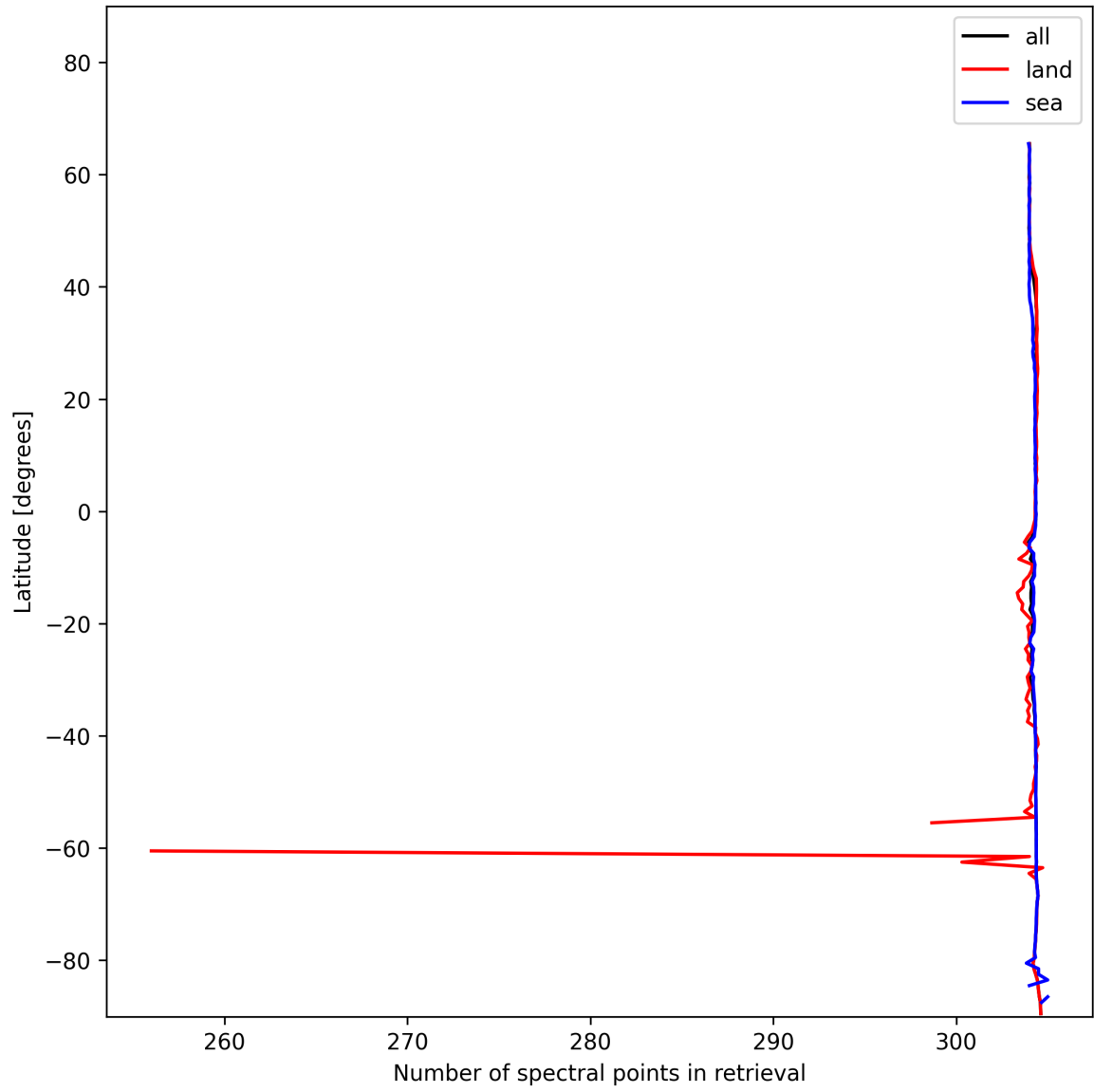
Figure 14: Zonal average of “Number of spectral points in retrieval” for 2024-12-06 to 2024-12-07.
