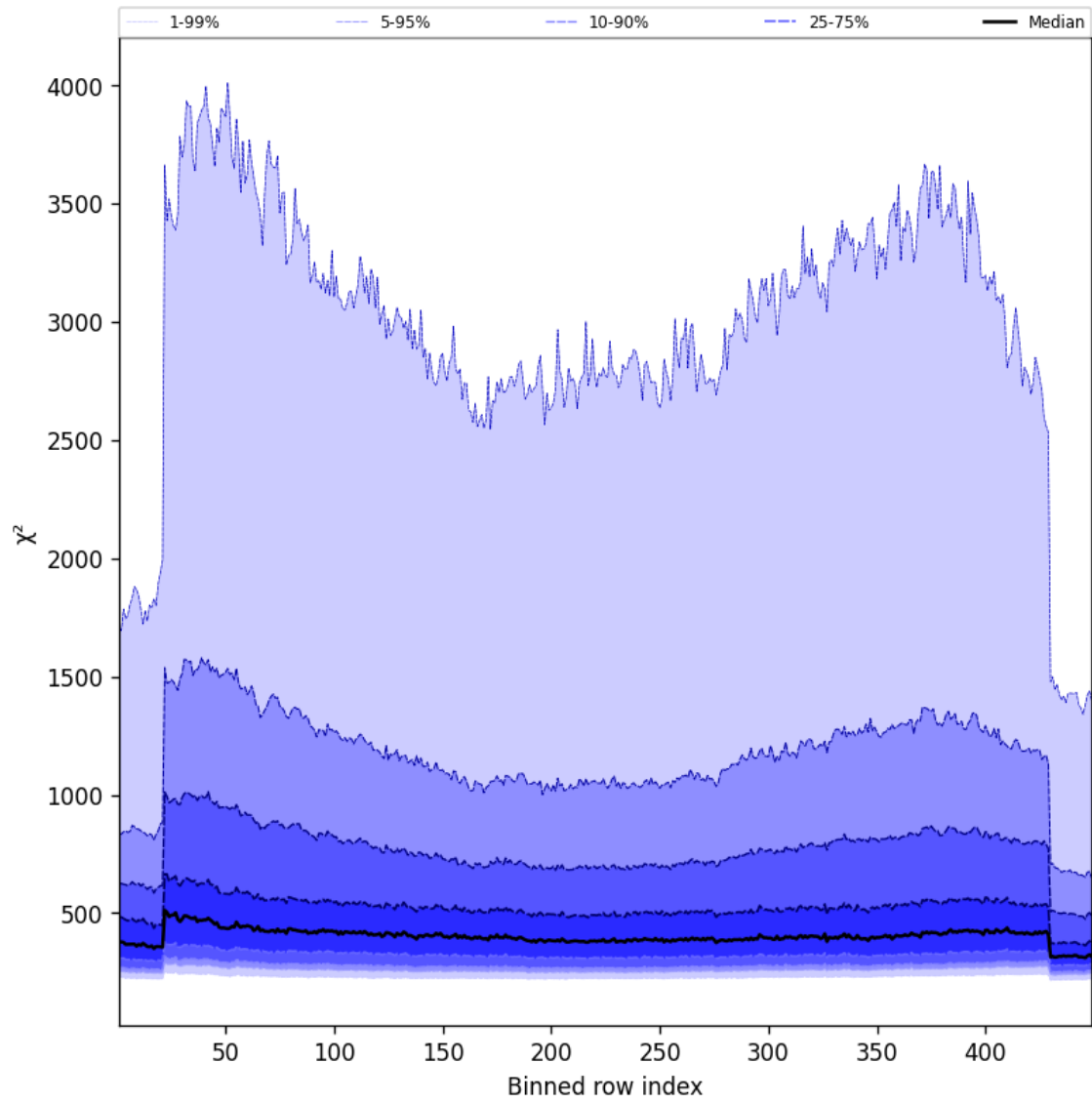
Figure 57: Along track statistics of “ \chi^2 ” for 2024-12-06 to 2024-12-07
