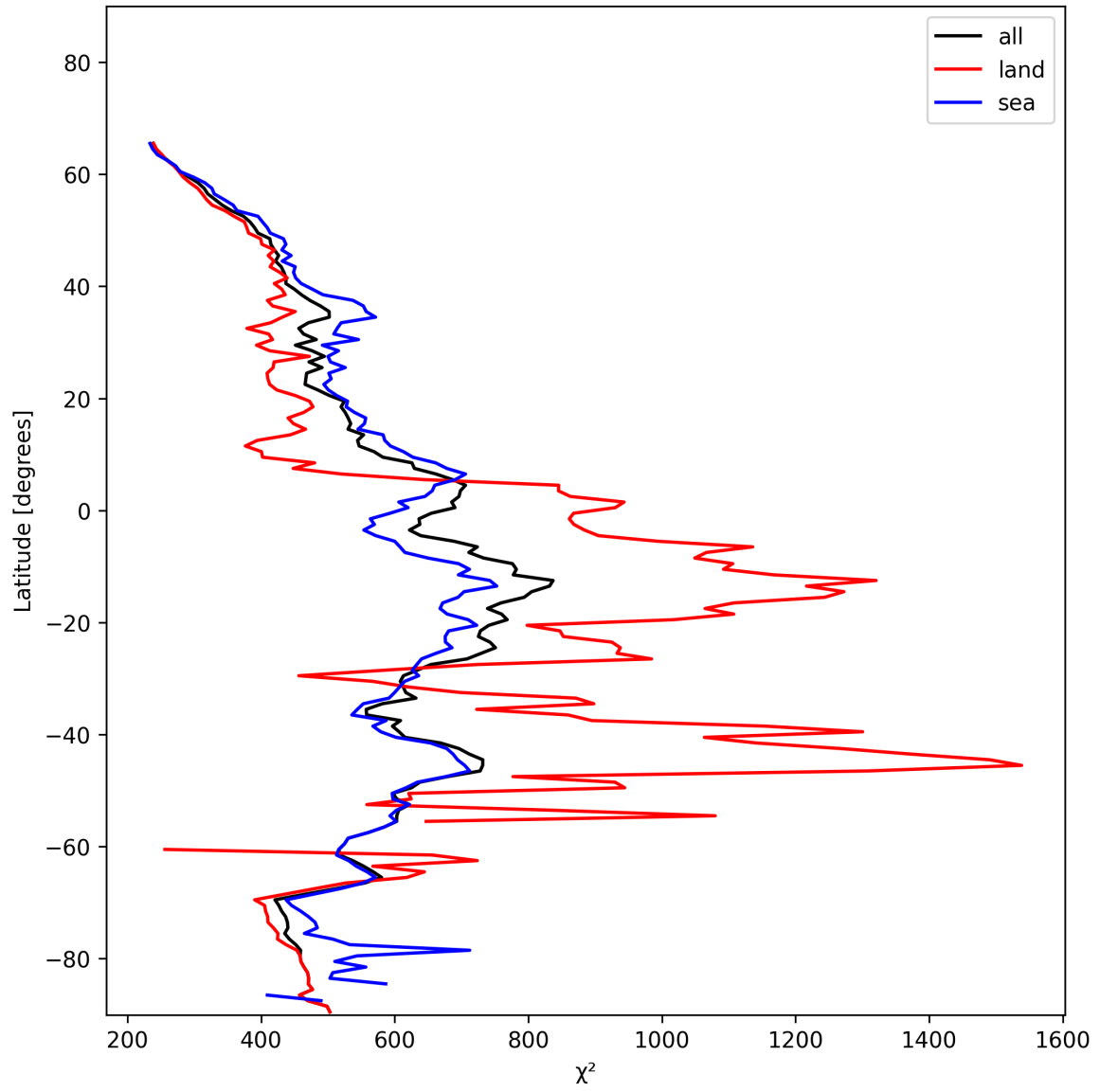
Figure 23: Zonal average of “ \chi^2 ” for 2024-12-06 to 2024-12-07.
