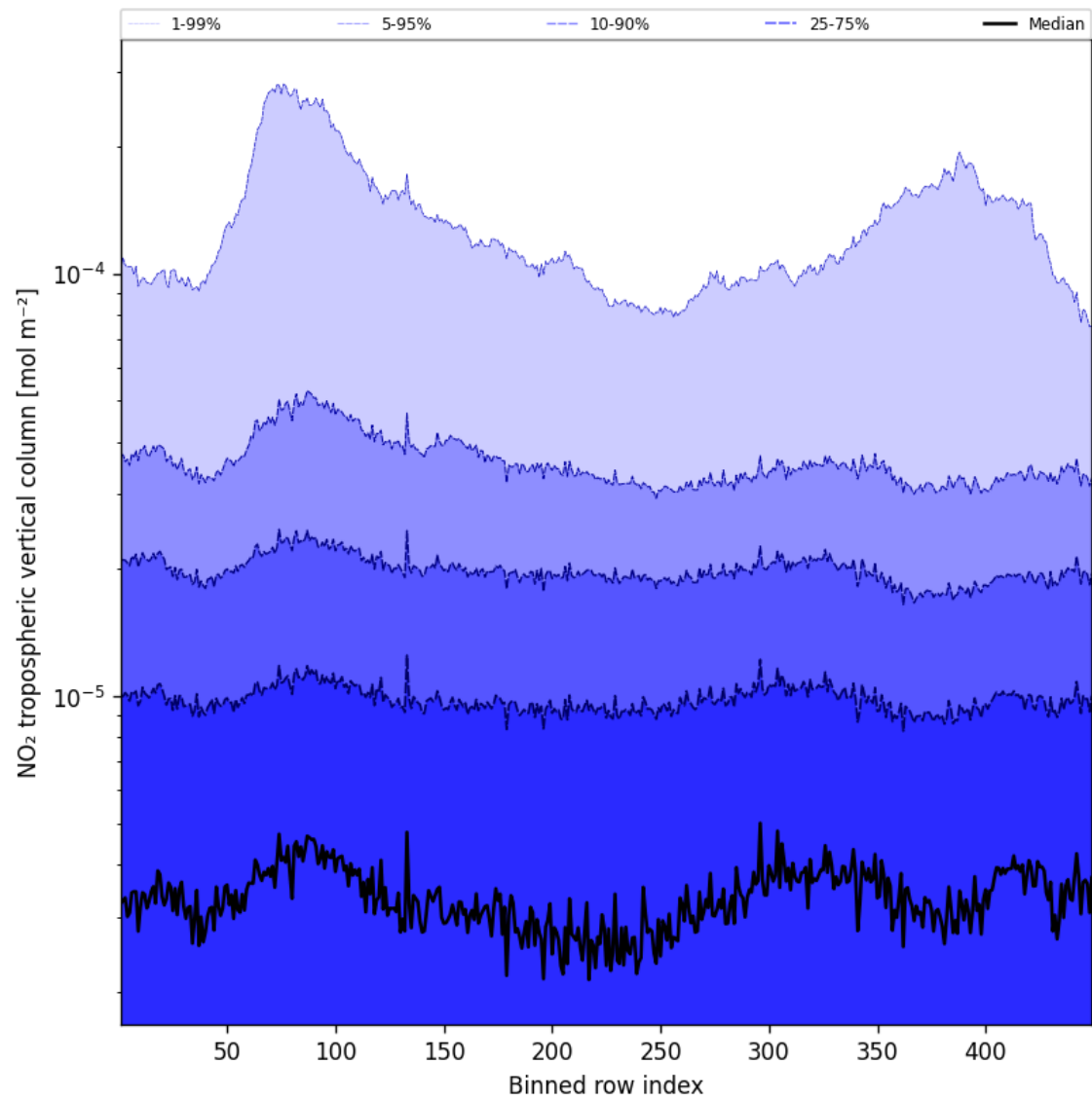
Figure 44: Along track statistics of “NO 2 tropospheric vertical column” for 2024-12-06 to 2024-12-07
