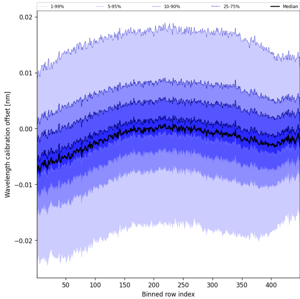
Figure 50: Along track statistics of “Wavelength calibration offset” for 2024-12-06 to 2024-12-07
