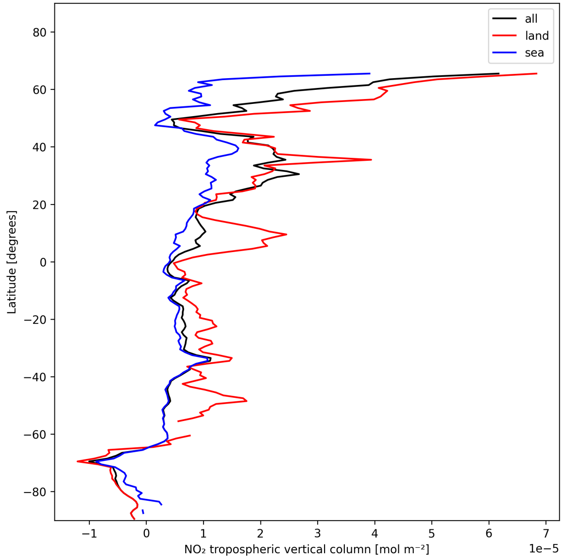
Figure 10: Zonal average of “NO 2 tropospheric vertical column” for 2024-12-06 to 2024-12-07.
