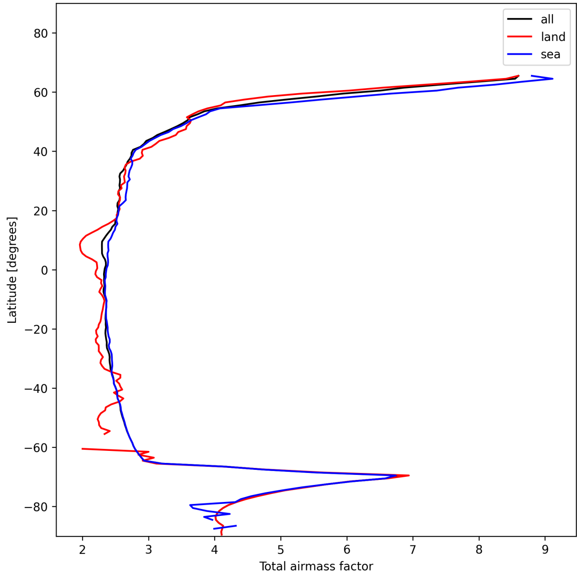
Figure 13: Zonal average of “Total airmass factor” for 2024-12-06 to 2024-12-07.
