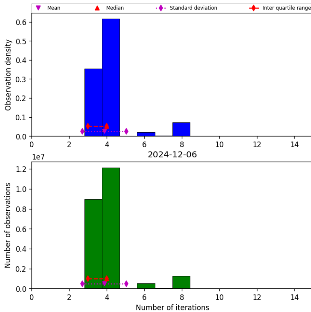
Figure 32: Histogram of “Number of iterations” for 2024-12-06 to 2024-12-07
