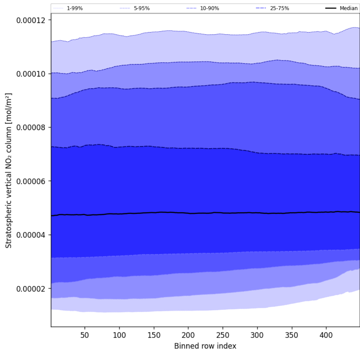
Figure 51: Along track statistics of “Stratospheric vertical NO 2 column” for 2024-12-06 to 2024-12-07
