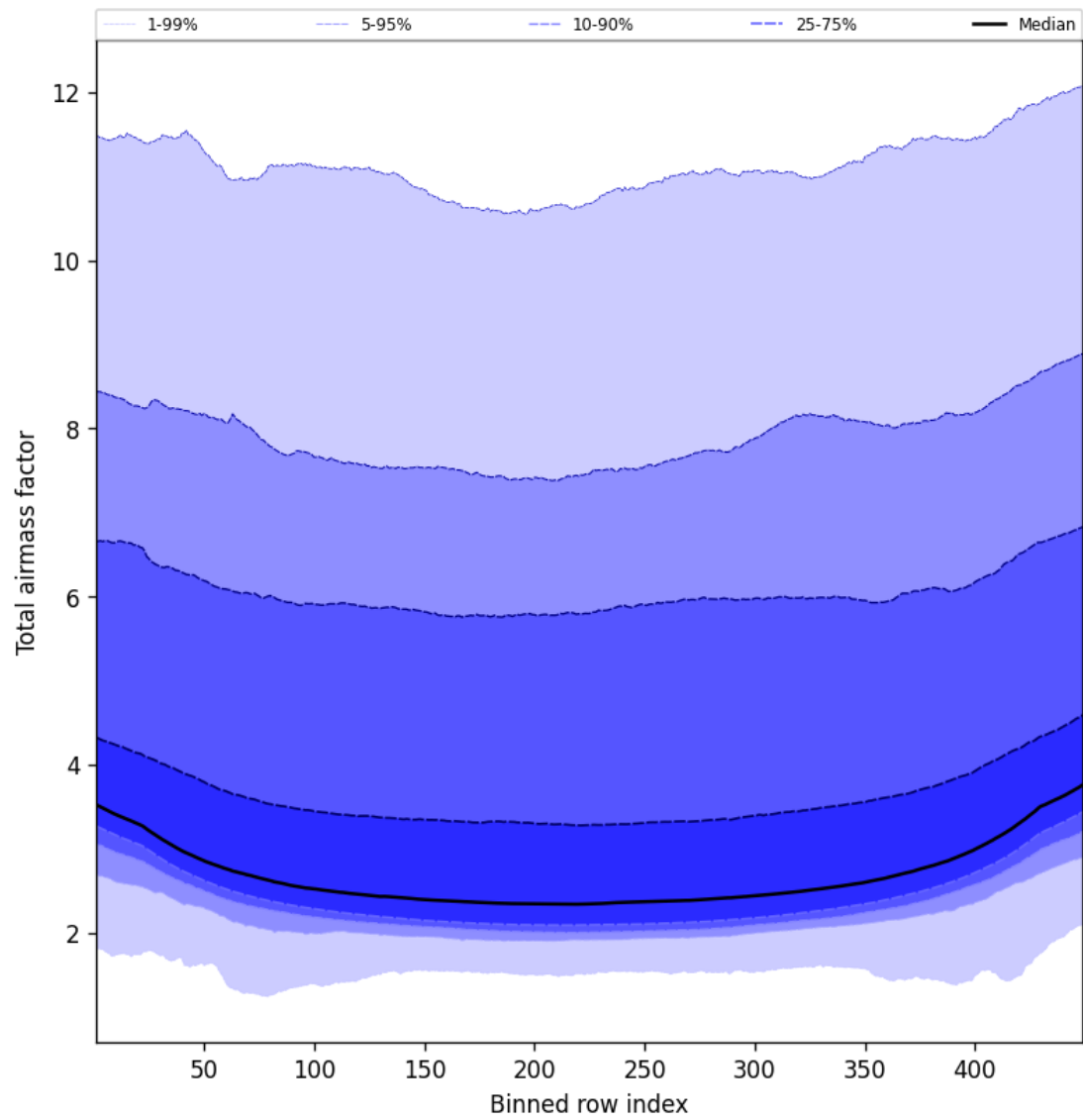
Figure 47: Along track statistics of “Total airmass factor” for 2024-12-06 to 2024-12-07
