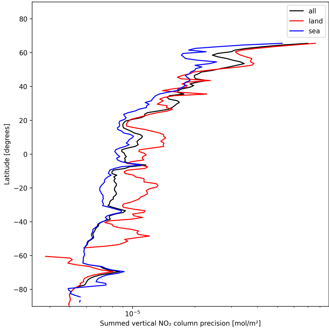
Figure 22: Zonal average of “Summed vertical NO 2 column precision” for 2024-12-06 to 2024-12-07.
