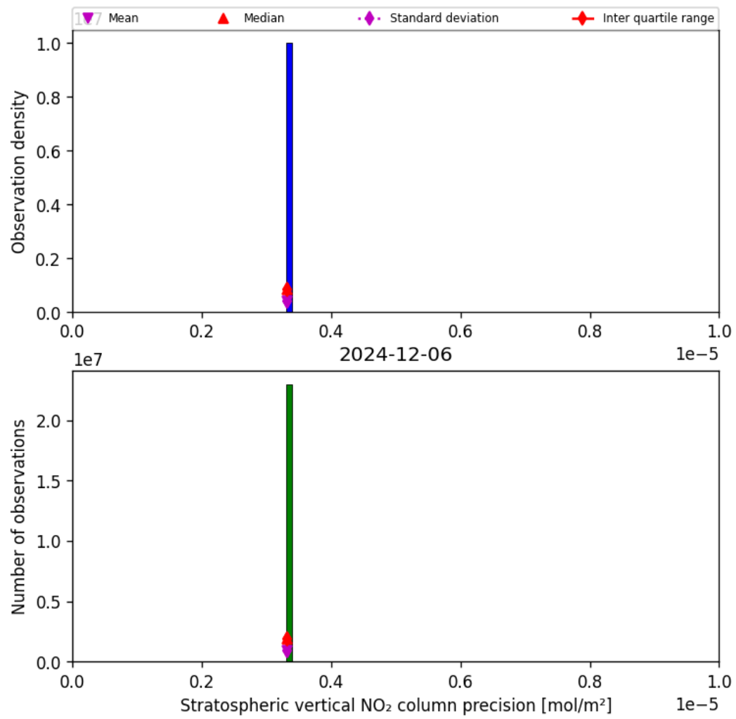
Figure 35: Histogram of “Stratospheric vertical NO 2 column precision” for 2024-12-06 to 2024-12-07
