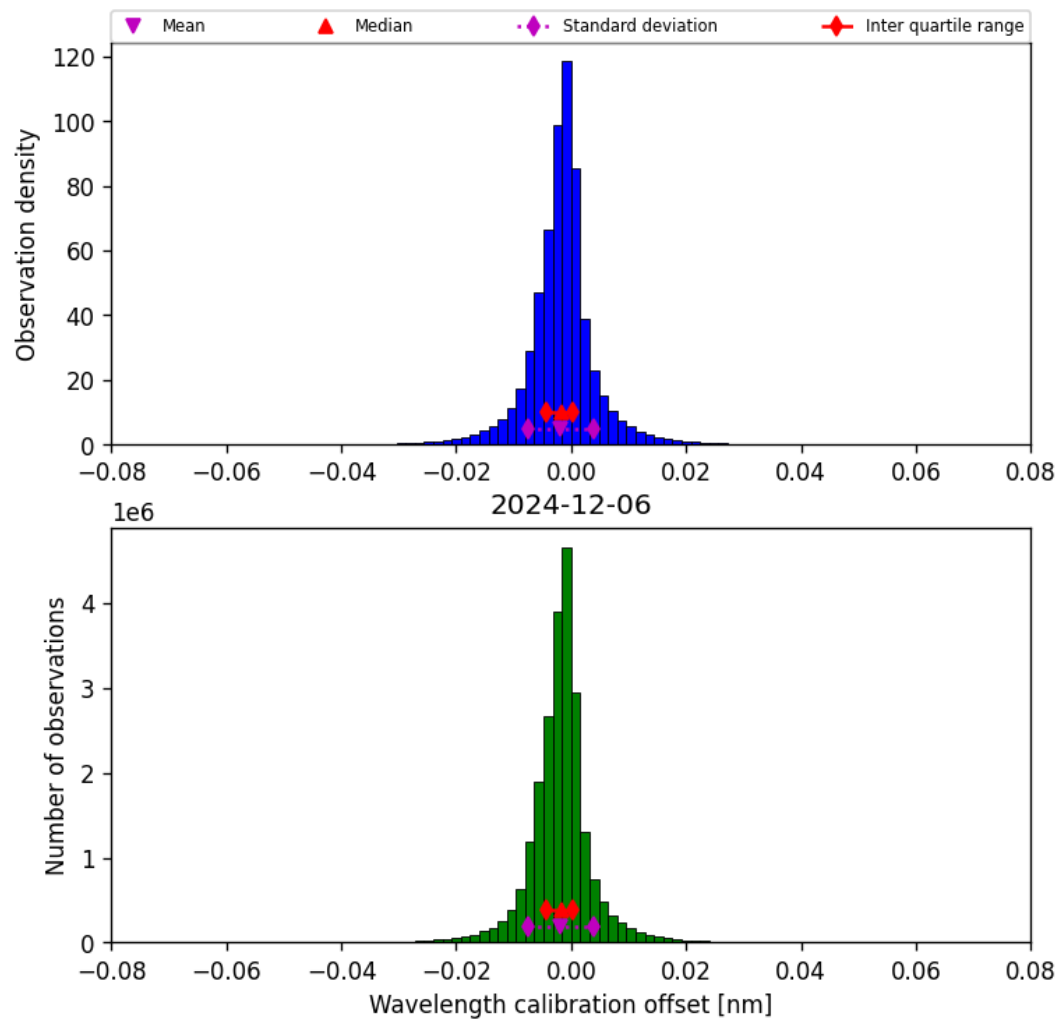
Figure 33: Histogram of “Wavelength calibration offset” for 2024-12-06 to 2024-12-07
