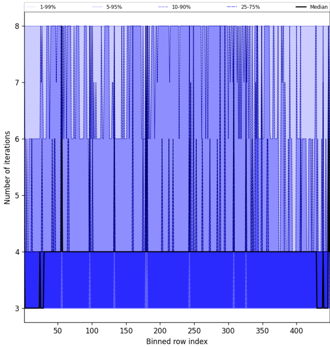
Figure 49: Along track statistics of “Number of iterations” for 2024-12-06 to 2024-12-07
