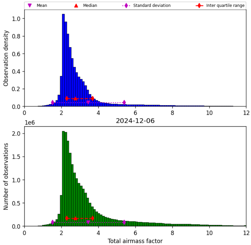
Figure 30: Histogram of “Total airmass factor” for 2024-12-06 to 2024-12-07
