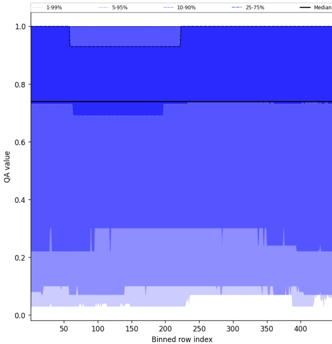
Figure 43: Along track statistics of “QA value” for 2024-12-06 to 2024-12-07
