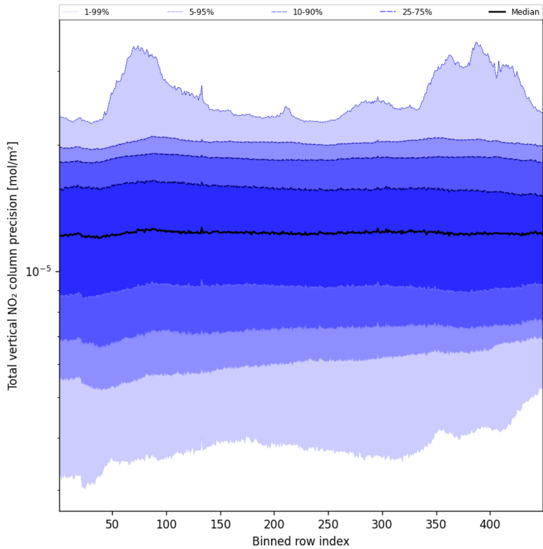
Figure 54: Along track statistics of “Total vertical NO 2 column precision” for 2024-12-06 to 2024-12-07
