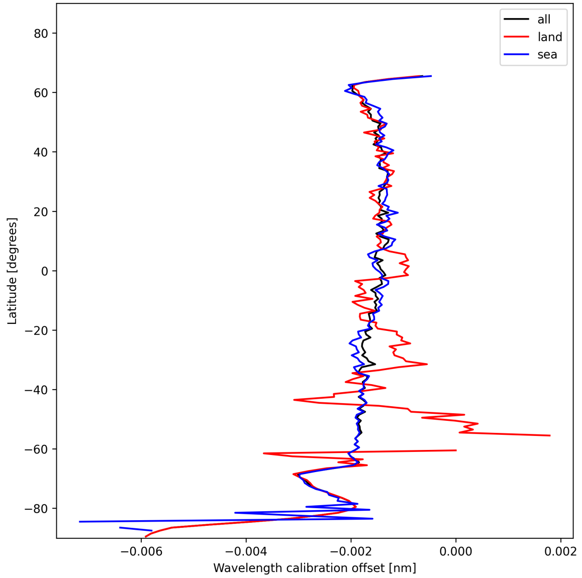
Figure 16: Zonal average of “Wavelength calibration offset” for 2024-12-06 to 2024-12-07.
