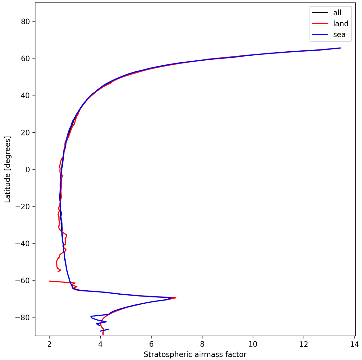
Figure 25: Zonal average of “Stratospheric airmass factor” for 2024-12-06 to 2024-12-07.
