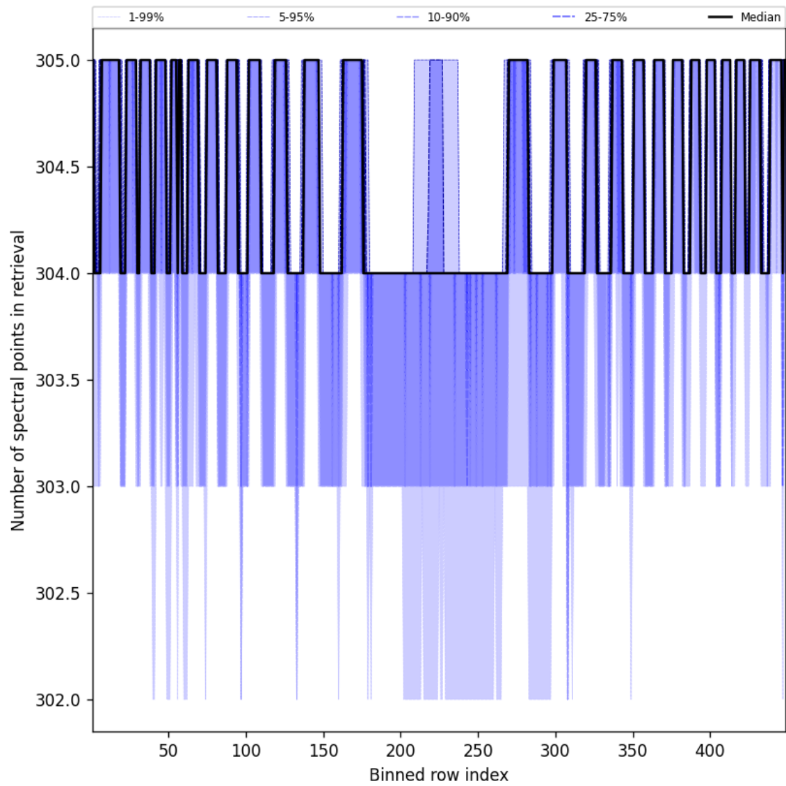
Figure 48: Along track statistics of “Number of spectral points in retrieval” for 2024-12-06 to 2024-12-07
