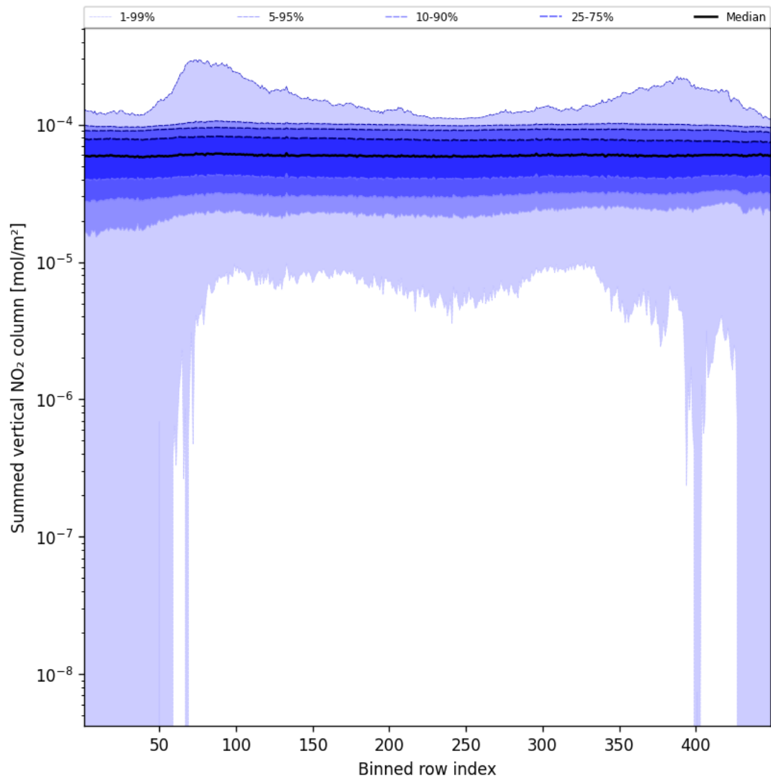
Figure 55: Along track statistics of "Summed vertical NO 2 column" for 2024-12-06 to 2024-12-07
