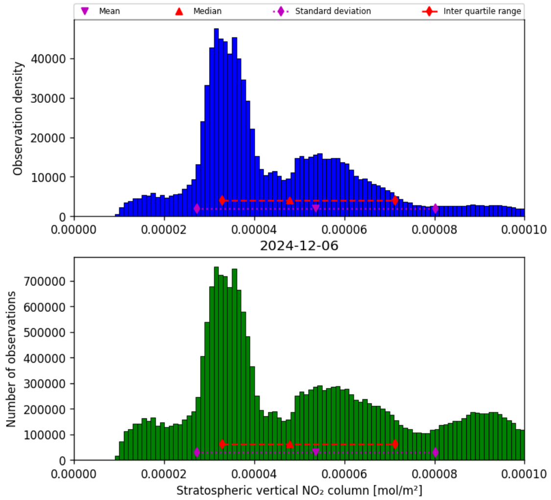
Figure 34: Histogram of “Stratospheric vertical NO 2 column” for 2024-12-06 to 2024-12-07
