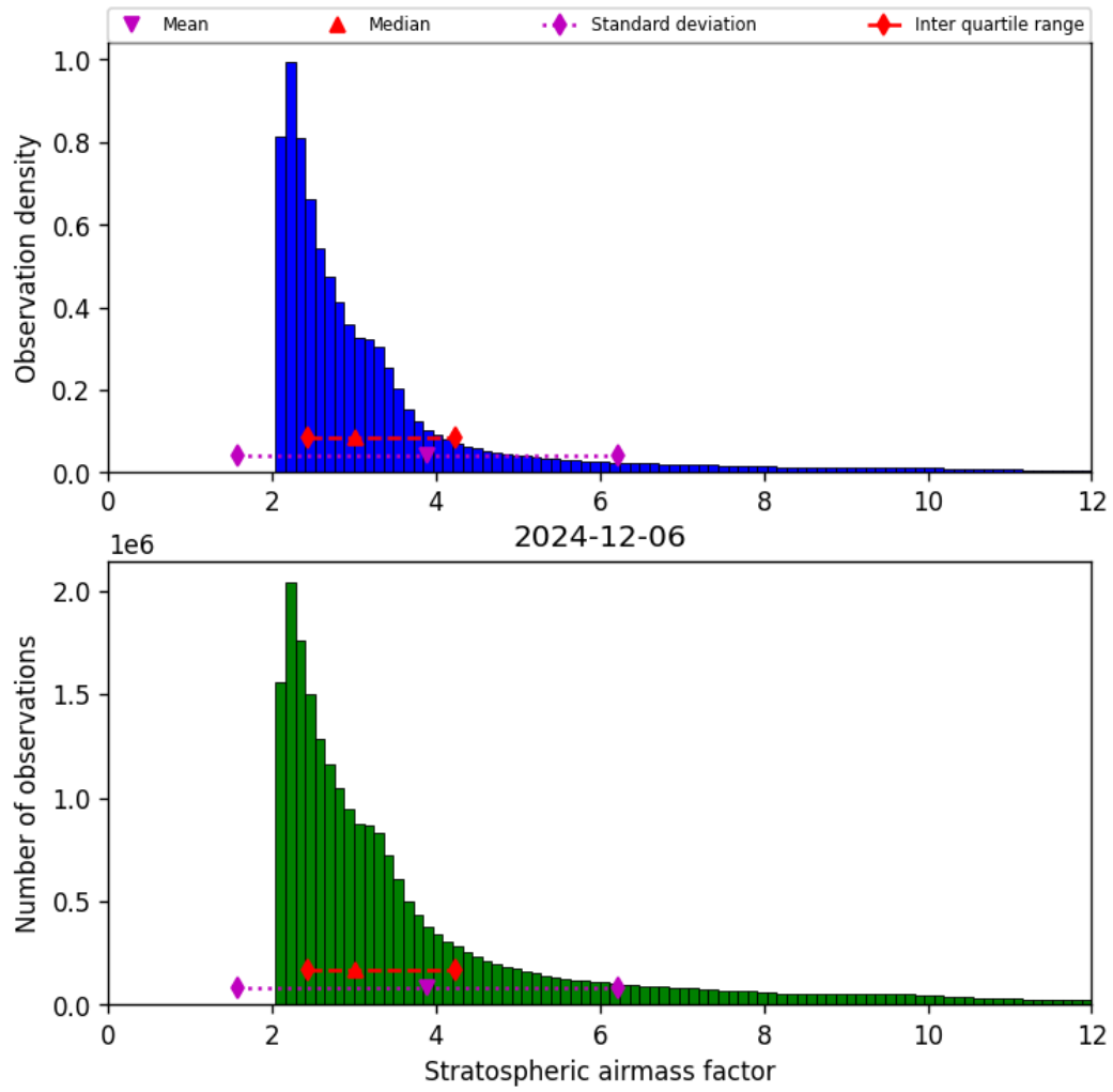
Figure 42: Histogram of “Stratospheric airmass factor” for 2024-12-06 to 2024-12-07
