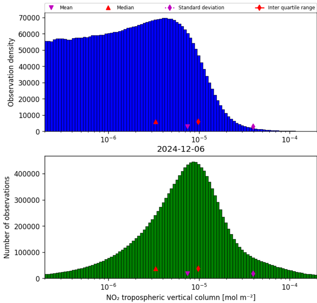
Figure 27: Histogram of “NO 2 tropospheric vertical column” for 2024-12-06 to 2024-12-07
