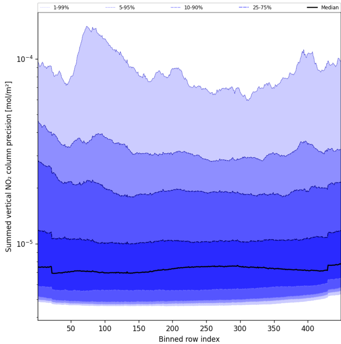
Figure 56: Along track statistics of “Summed vertical NO 2 column precision” for 2024-12-06 to 2024-12-07
