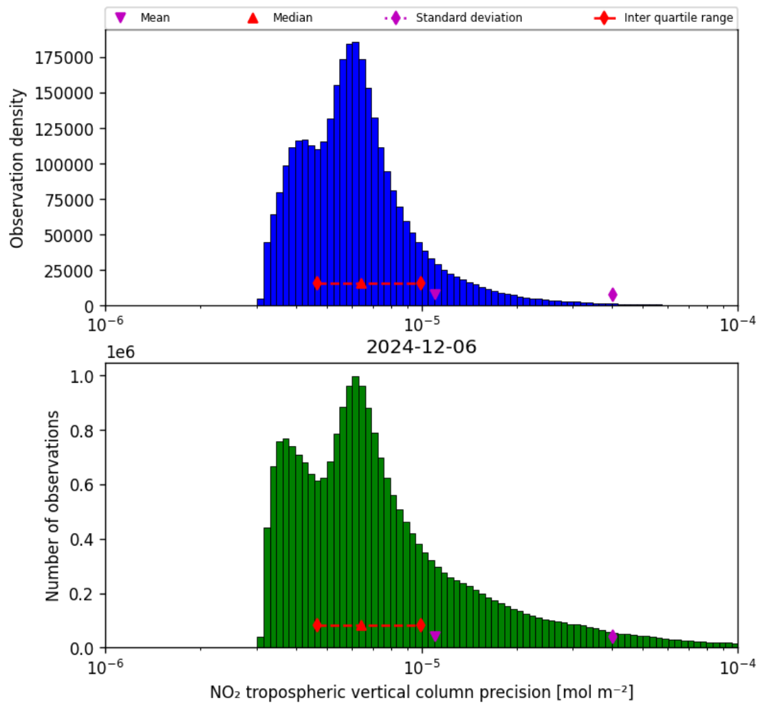
Figure 28: Histogram of “NO 2 tropospheric vertical column precision” for 2024-12-06 to 2024-12-07
