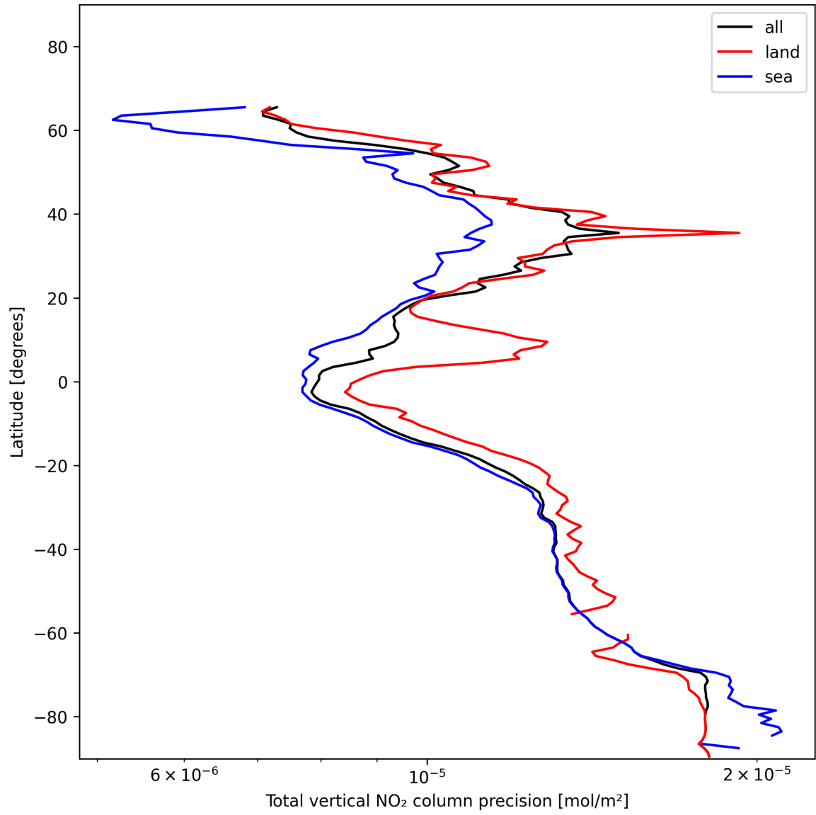
Figure 20: Zonal average of “Total vertical NO 2 column precision” for 2024-12-06 to 2024-12-07.
