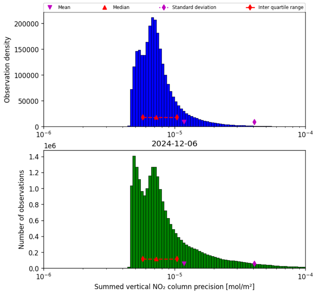
Figure 39: Histogram of “Summed vertical NO 2 column precision” for 2024-12-06 to 2024-12-07
