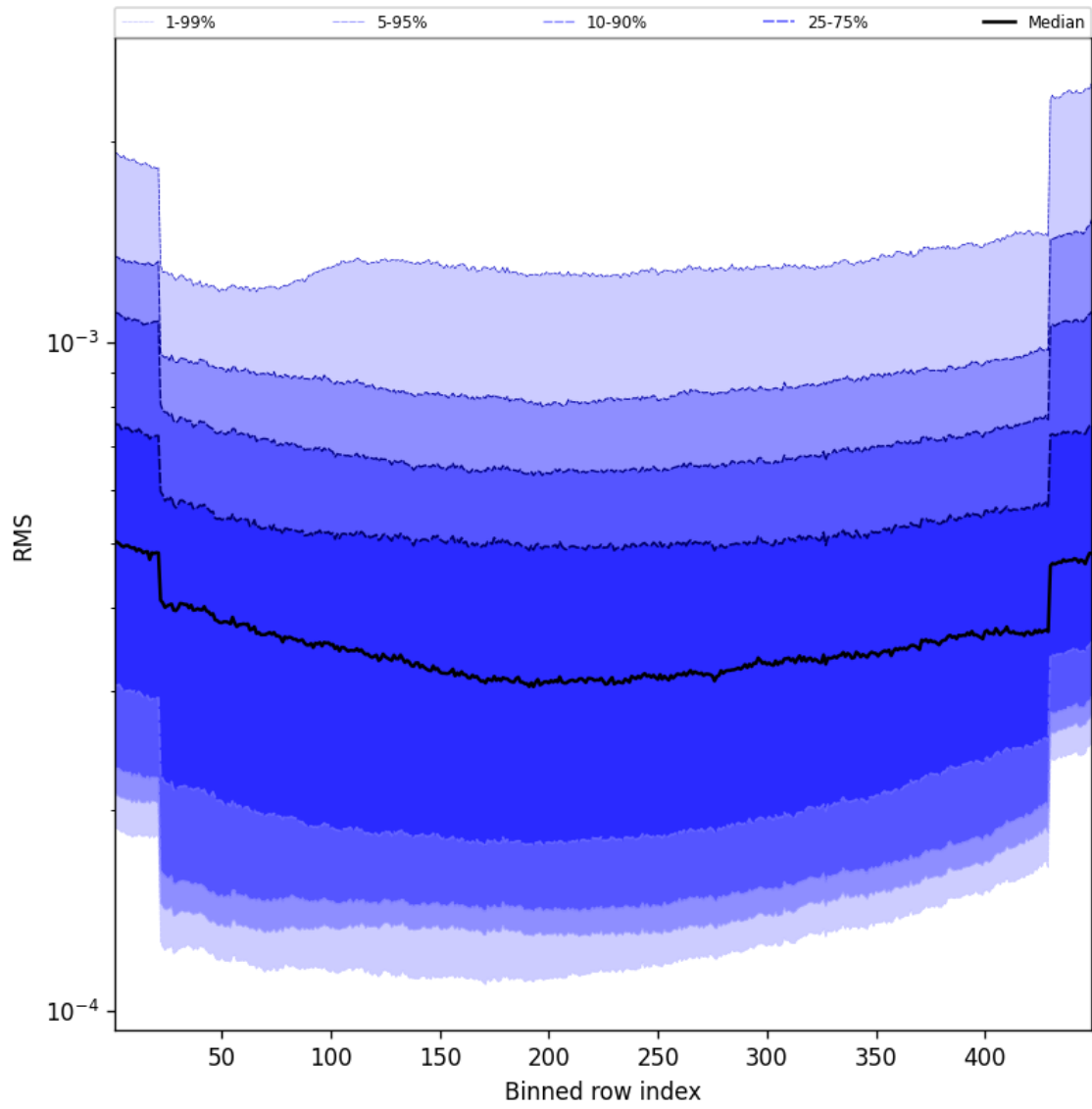
Figure 58: Along track statistics of “RMS” for 2024-12-06 to 2024-12-07
