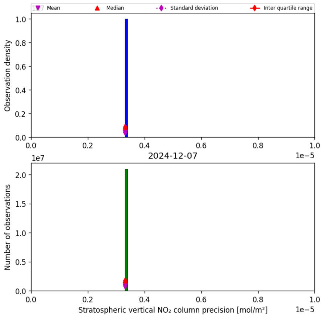
Figure 35: Histogram of “Stratospheric vertical NO 2 column precision” for 2024-12-07 to 2024-12-08
