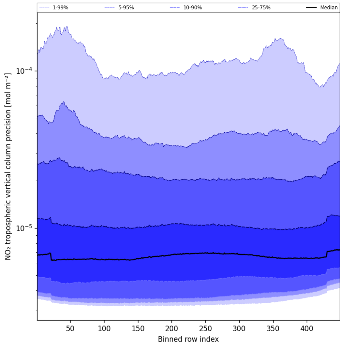
Figure 45: Along track statistics of “NO 2 tropospheric vertical column precision” for 2024-12-07 to 2024-12-08
