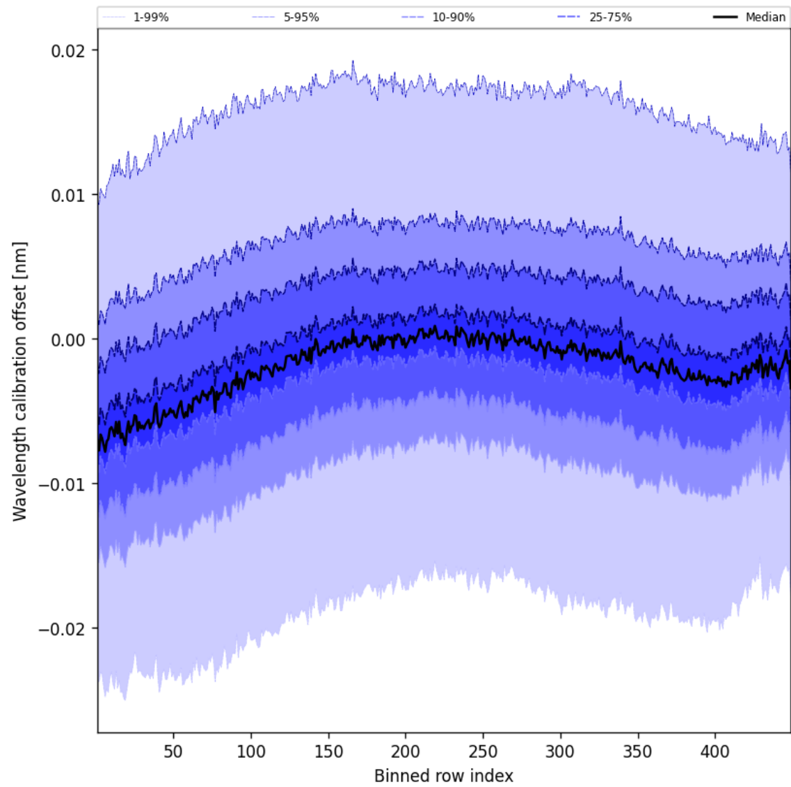
Figure 50: Along track statistics of “Wavelength calibration offset” for 2024-12-07 to 2024-12-08
