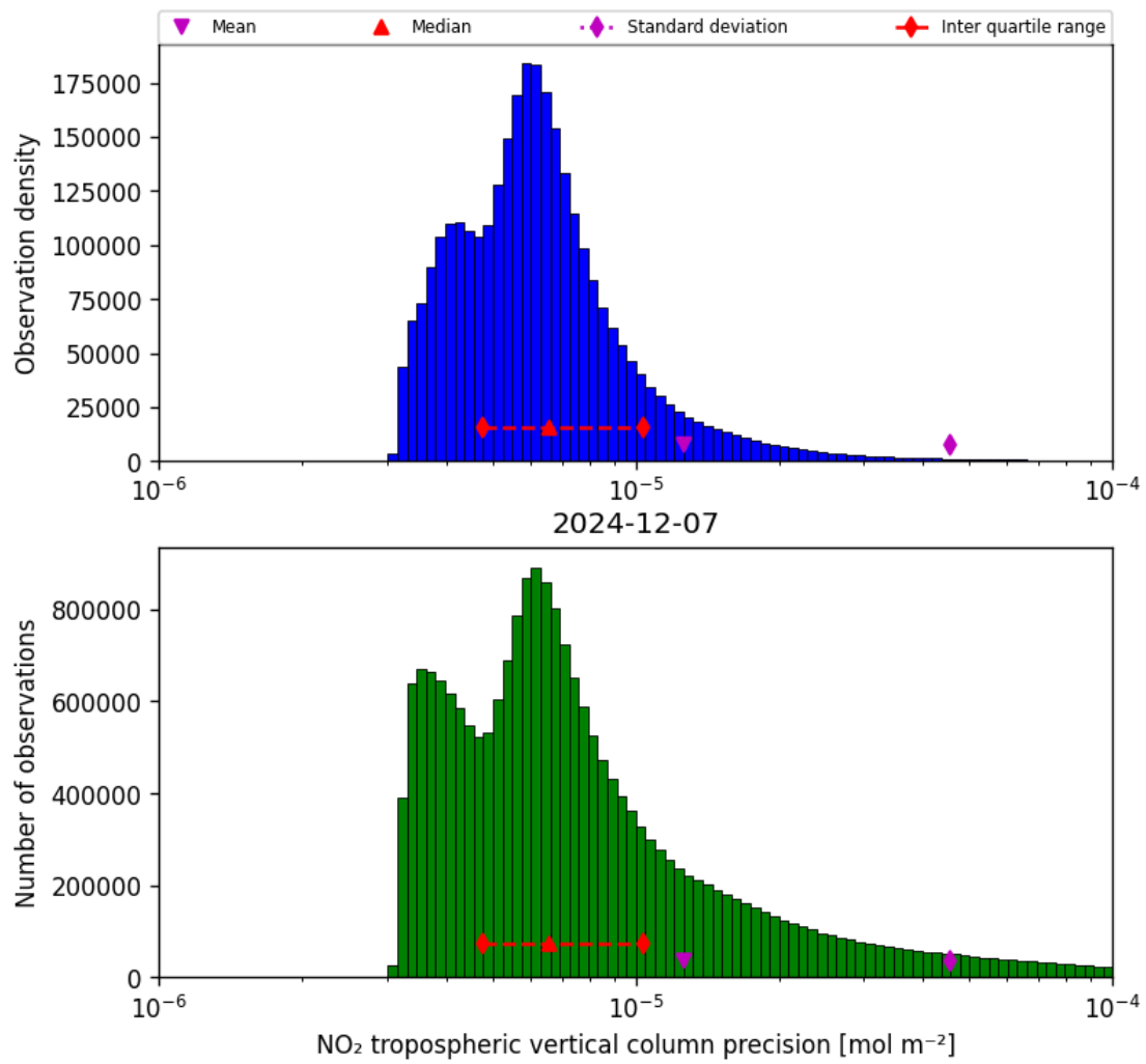
Figure 28: Histogram of “NO 2 tropospheric vertical column precision” for 2024-12-07 to 2024-12-08
