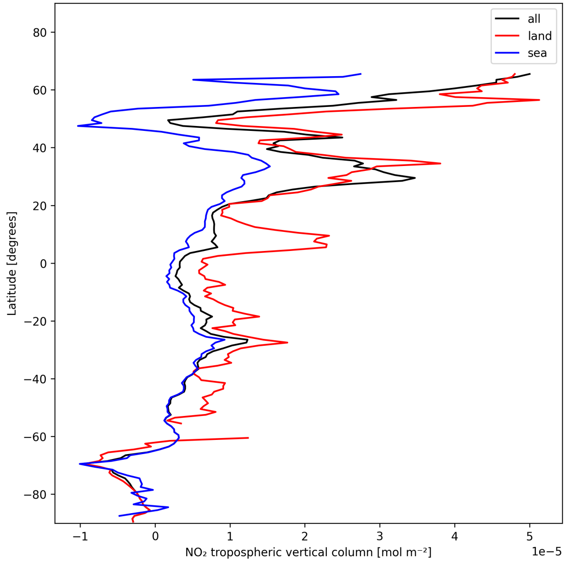
Figure 10: Zonal average of “NO 2 tropospheric vertical column” for 2024-12-07 to 2024-12-08.
