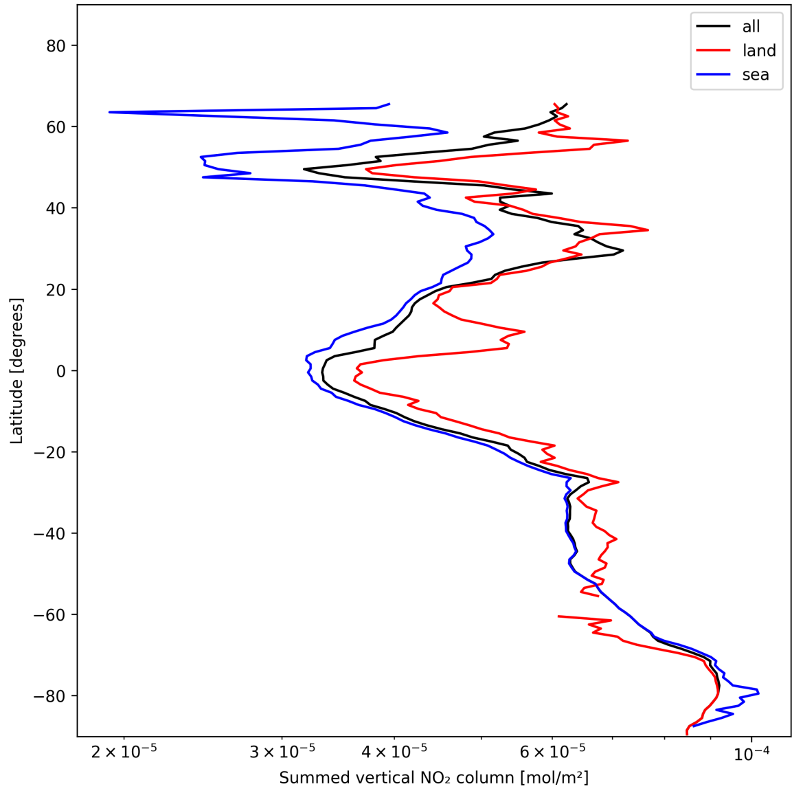
Figure 21: Zonal average of “Summed vertical NO 2 column” for 2024-12-07 to 2024-12-08.
