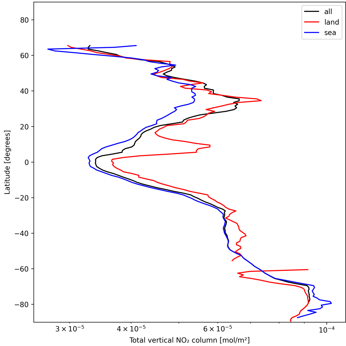
Figure 19: Zonal average of “Total vertical NO 2 column” for 2024-12-07 to 2024-12-08.
