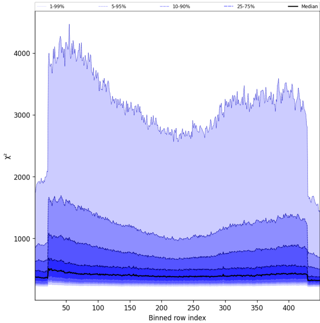
Figure 57: Along track statistics of “ \chi^2 ” for 2024-12-07 to 2024-12-08
