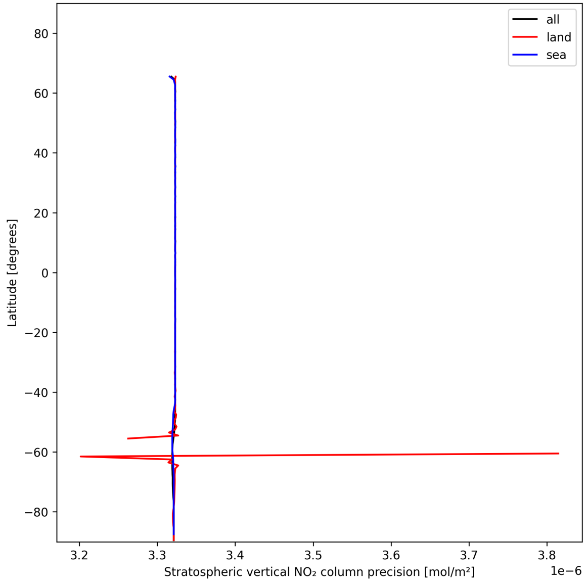
Figure 18: Zonal average of “Stratospheric vertical NO 2 column precision” for 2024-12-07 to 2024-12-08.
