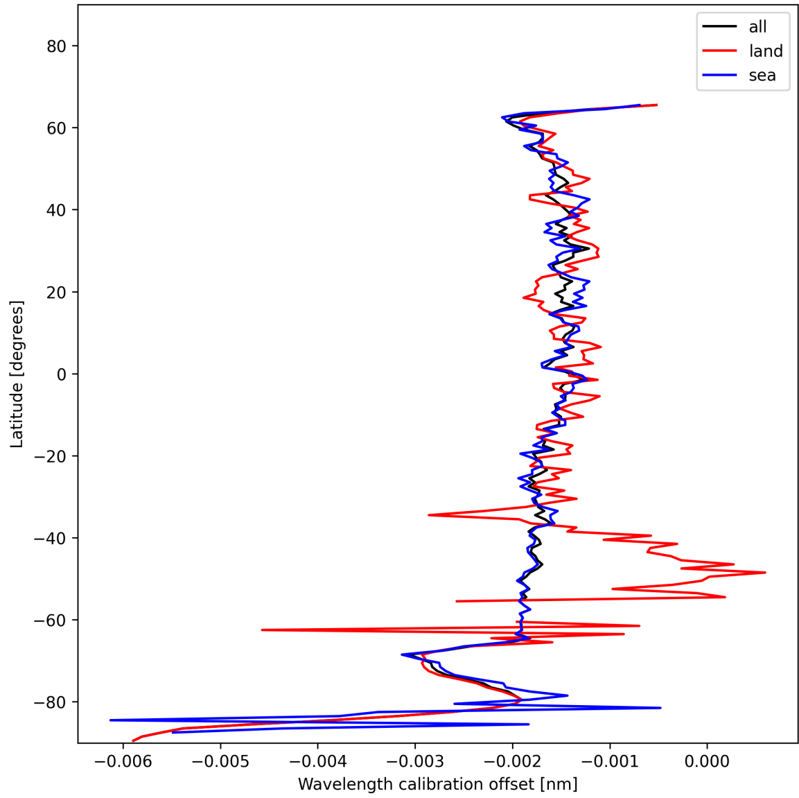
Figure 16: Zonal average of “Wavelength calibration offset” for 2024-12-07 to 2024-12-08.
