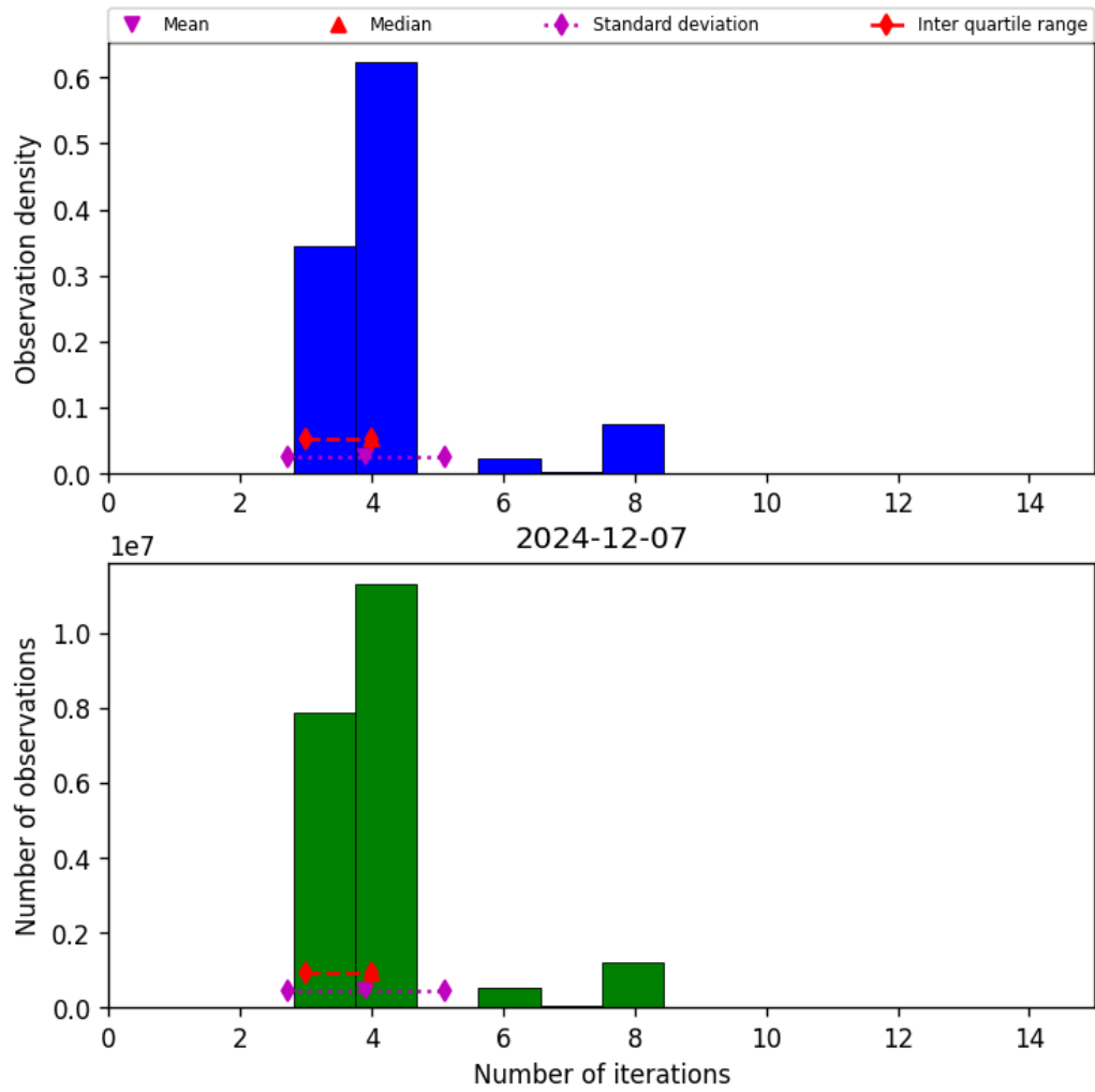
Figure 32: Histogram of “Number of iterations” for 2024-12-07 to 2024-12-08
