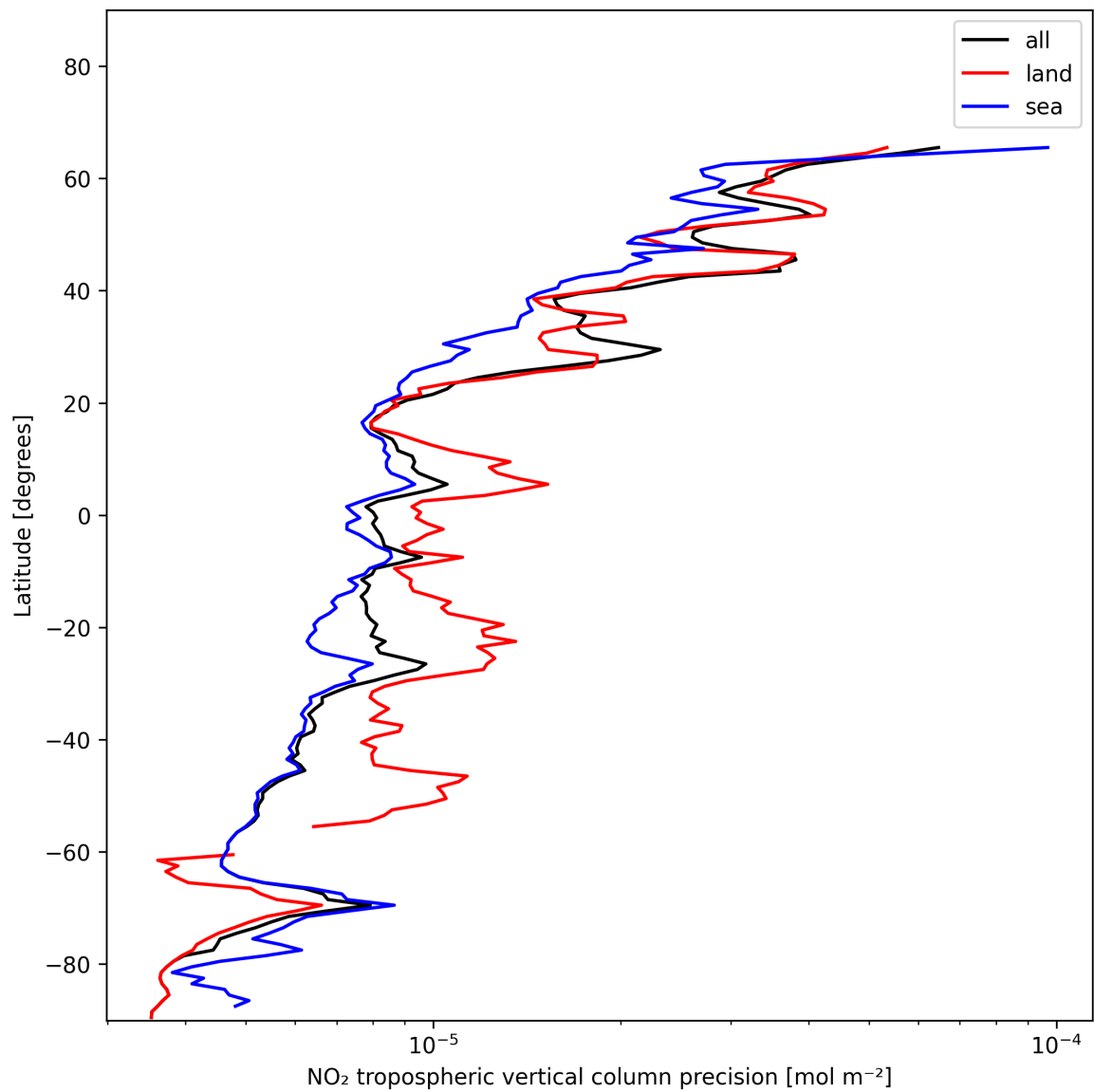
Figure 11: Zonal average of “NO 2 tropospheric vertical column precision” for 2024-12-07 to 2024-12-08.
