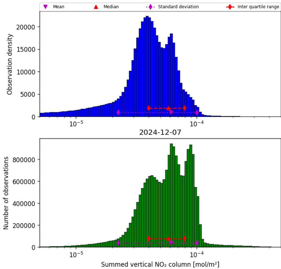
Figure 38: Histogram of “Summed vertical NO 2 column” for 2024-12-07 to 2024-12-08
