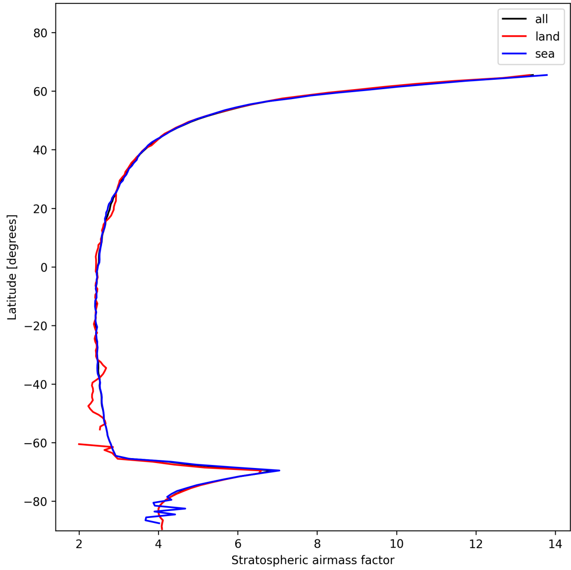
Figure 25: Zonal average of “Stratospheric airmass factor” for 2024-12-07 to 2024-12-08.
