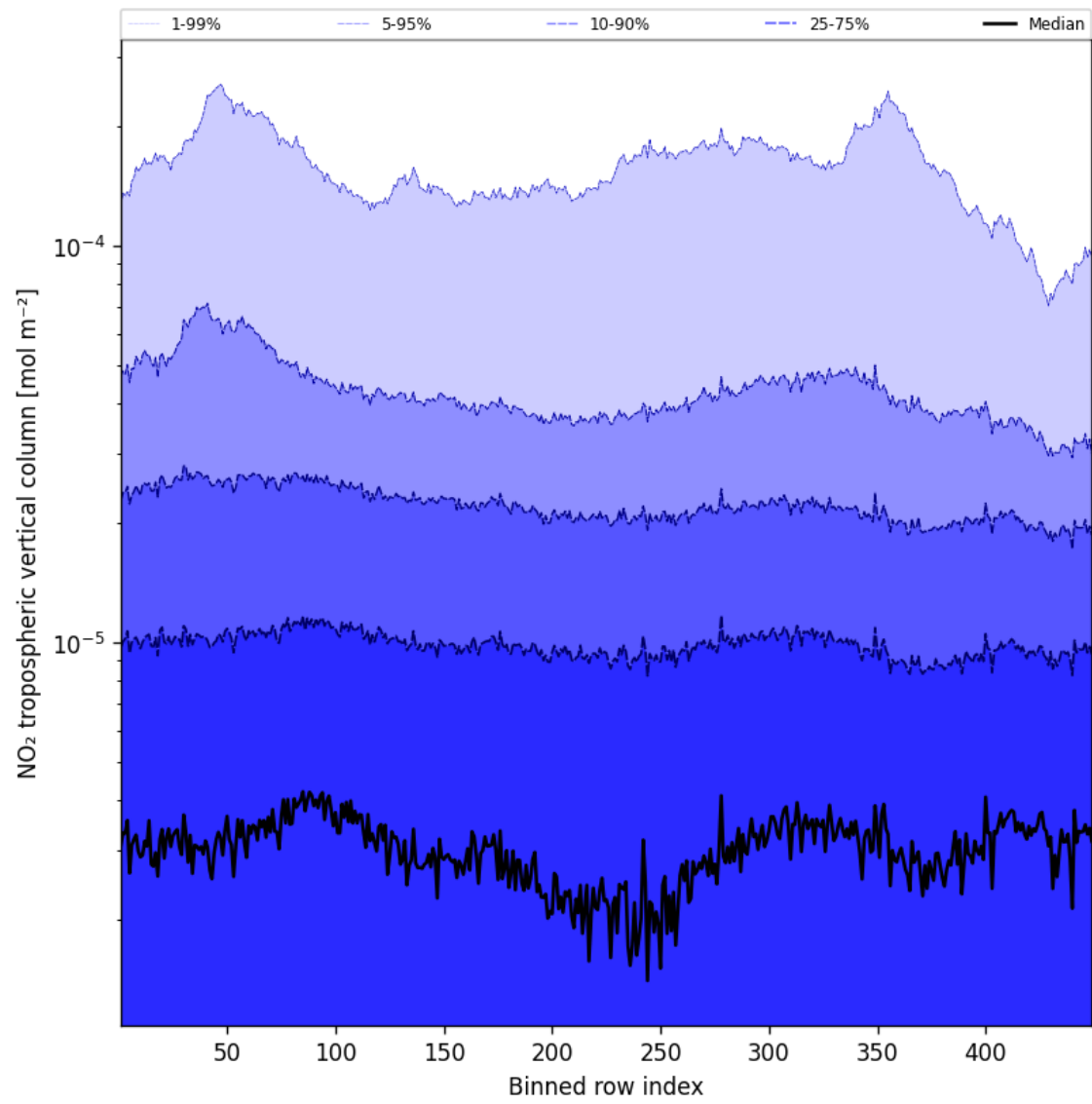
Figure 44: Along track statistics of “NO 2 tropospheric vertical column” for 2024-12-07 to 2024-12-08
