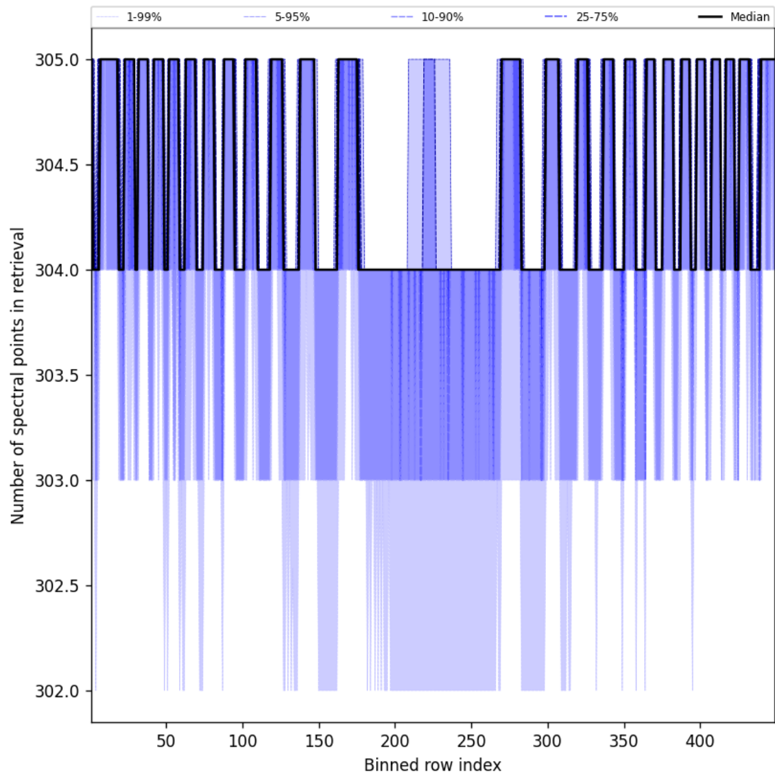
Figure 48: Along track statistics of “Number of spectral points in retrieval” for 2024-12-07 to 2024-12-08
