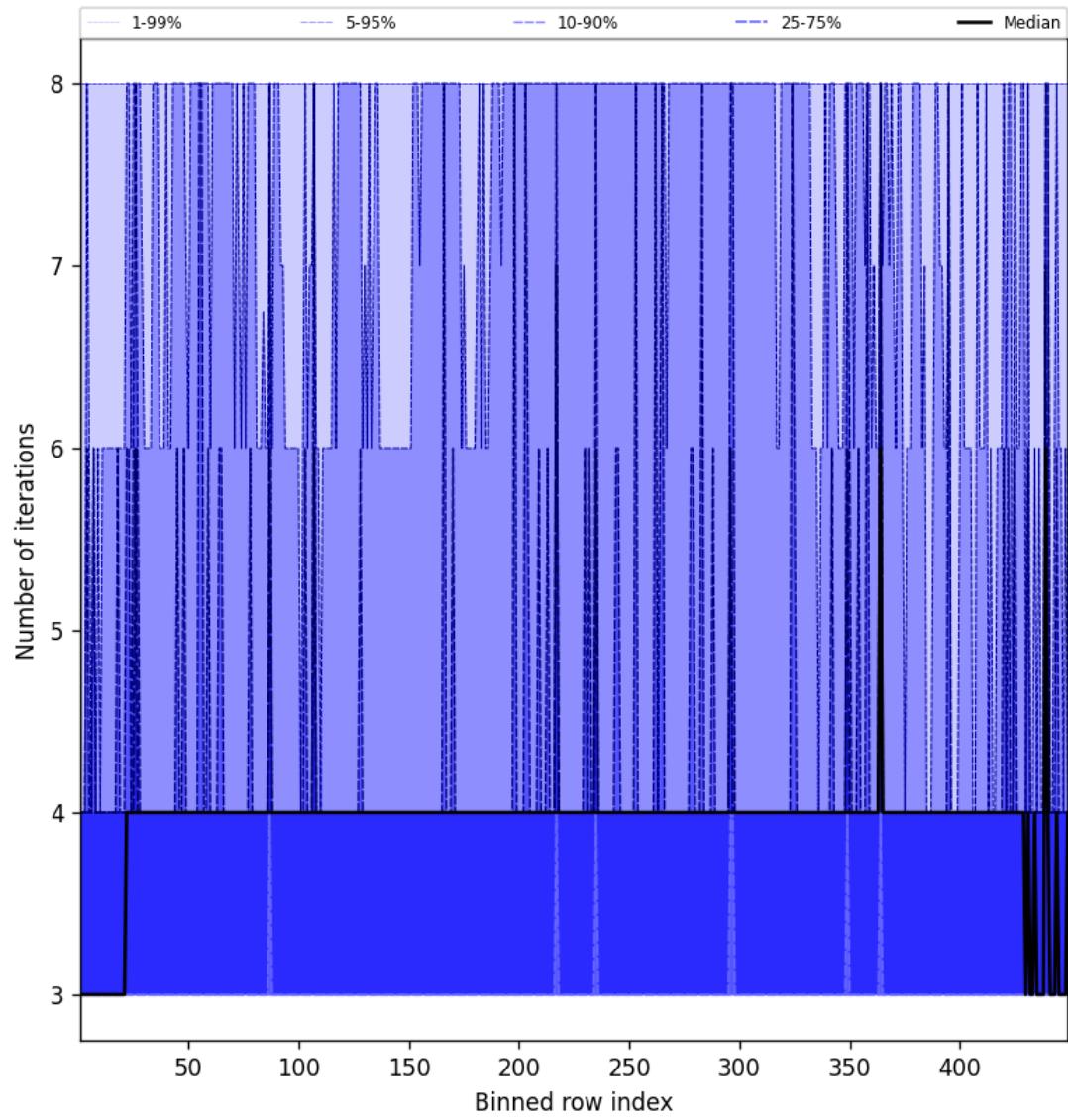
Figure 49: Along track statistics of “Number of iterations” for 2024-12-07 to 2024-12-08
