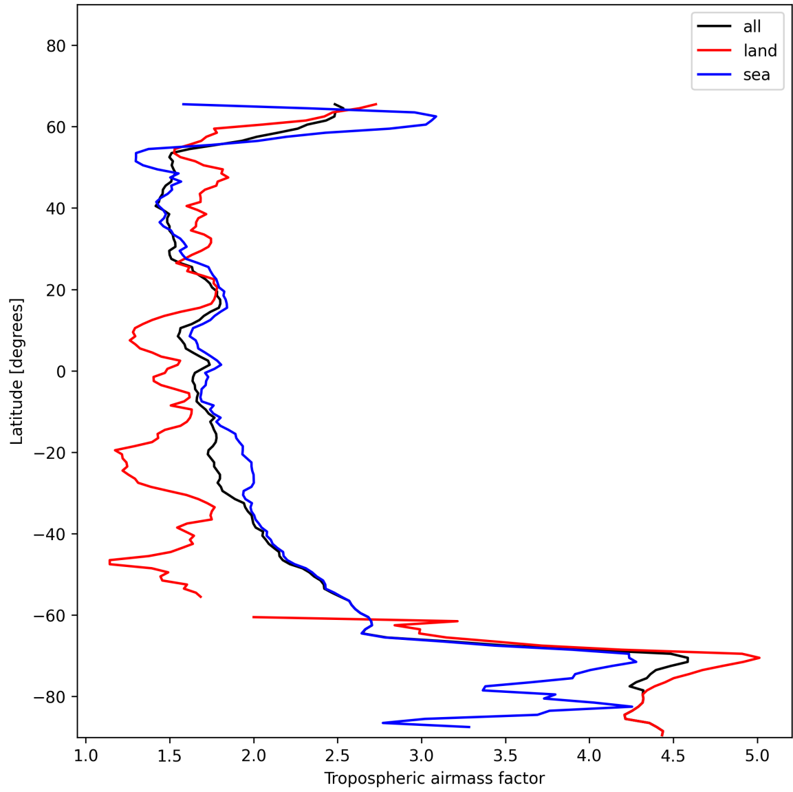
Figure 12: Zonal average of “Tropospheric airmass factor” for 2024-12-07 to 2024-12-08.
