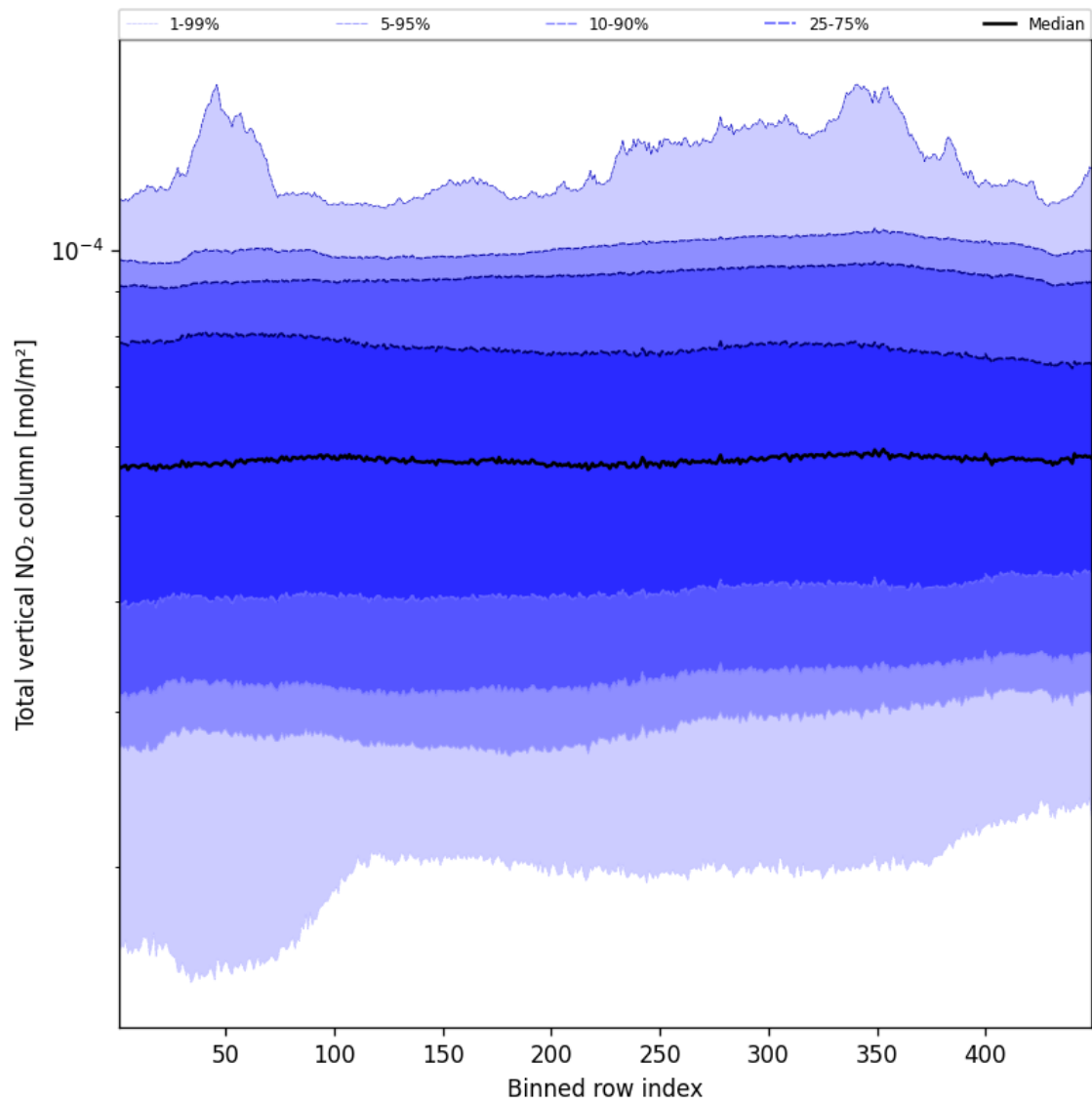
Figure 53: Along track statistics of "Total vertical NO 2 column" for 2024-12-07 to 2024-12-08
