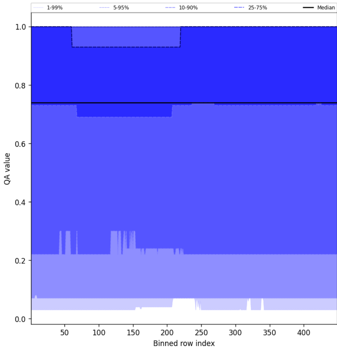
Figure 43: Along track statistics of “QA value” for 2024-12-07 to 2024-12-08
