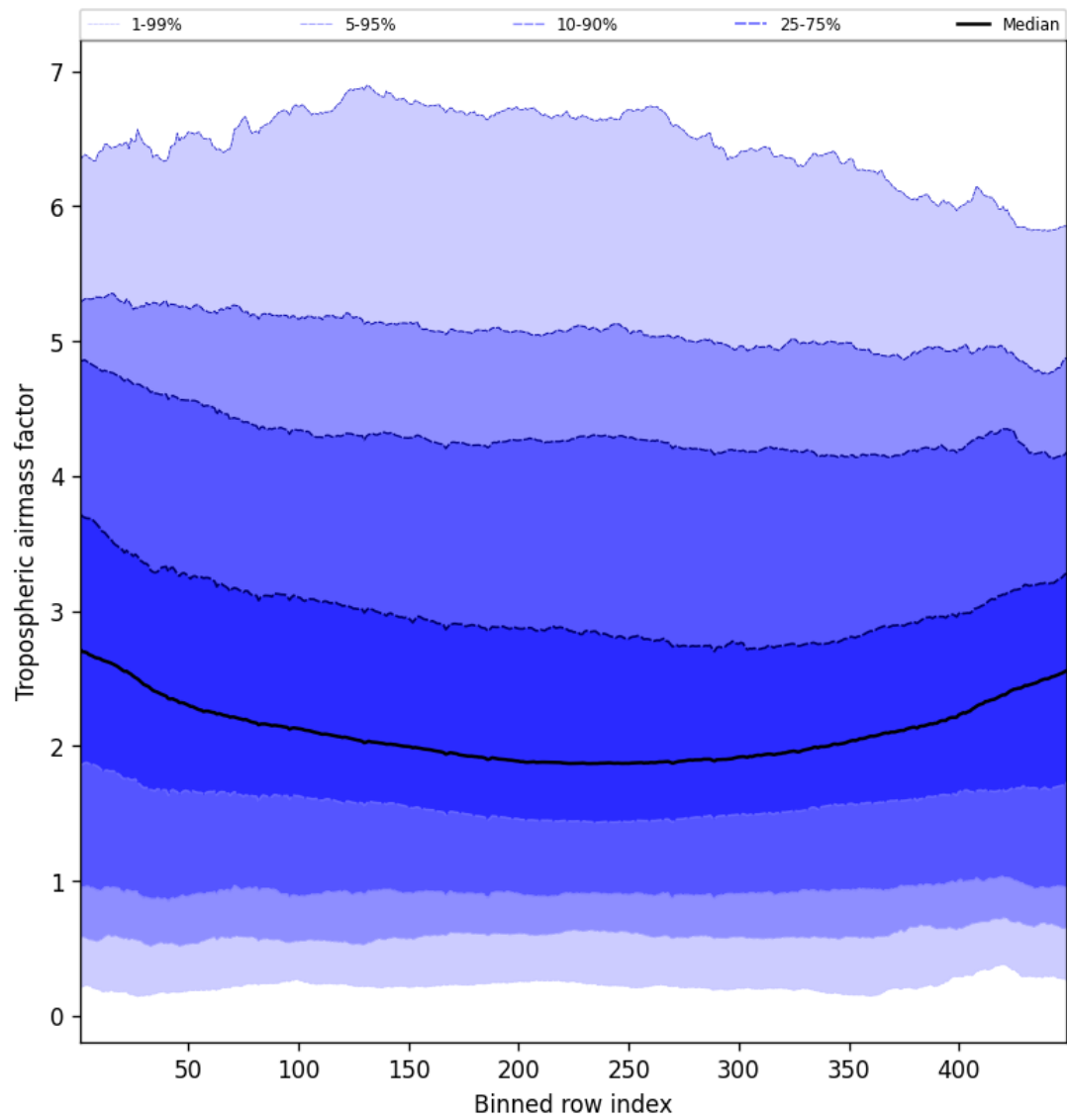
Figure 46: Along track statistics of “Tropospheric airmass factor” for 2024-12-07 to 2024-12-08
