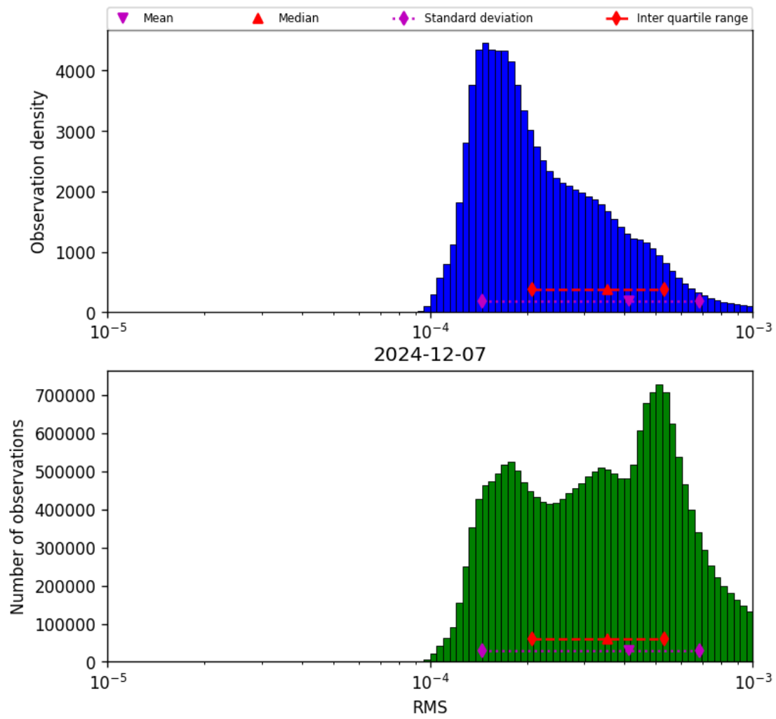
Figure 41: Histogram of “RMS” for 2024-12-07 to 2024-12-08
