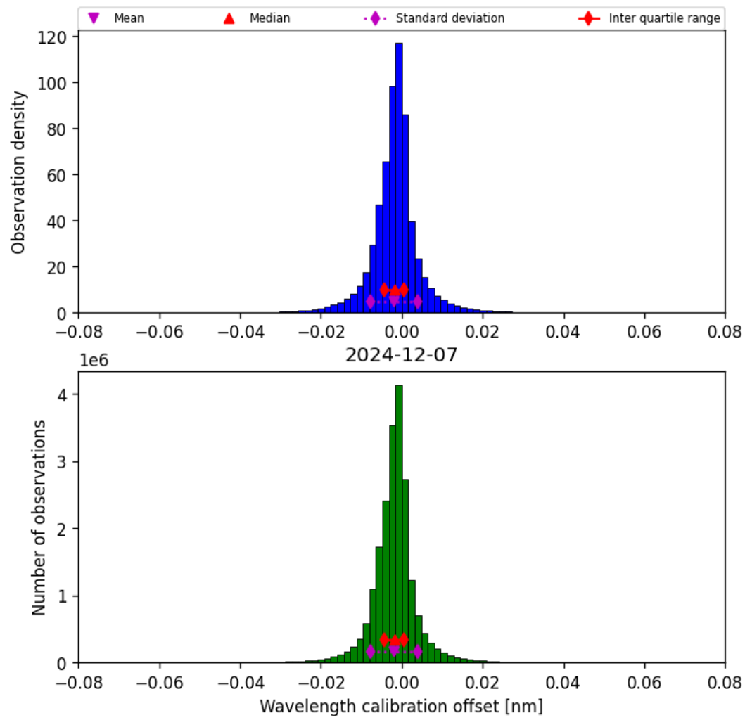
Figure 33: Histogram of “Wavelength calibration offset” for 2024-12-07 to 2024-12-08
