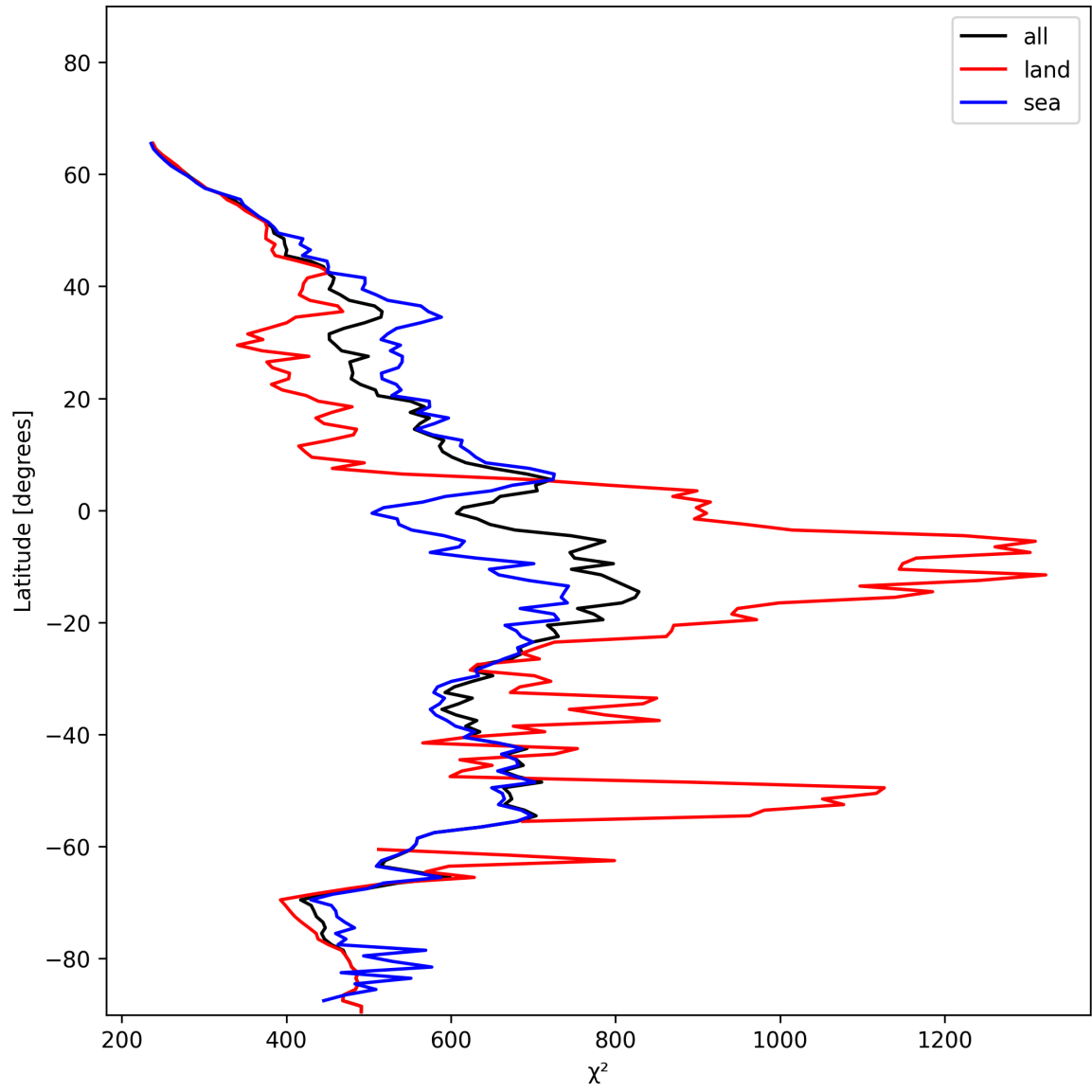
Figure 23: Zonal average of “ \chi^2 ” for 2024-12-07 to 2024-12-08.
