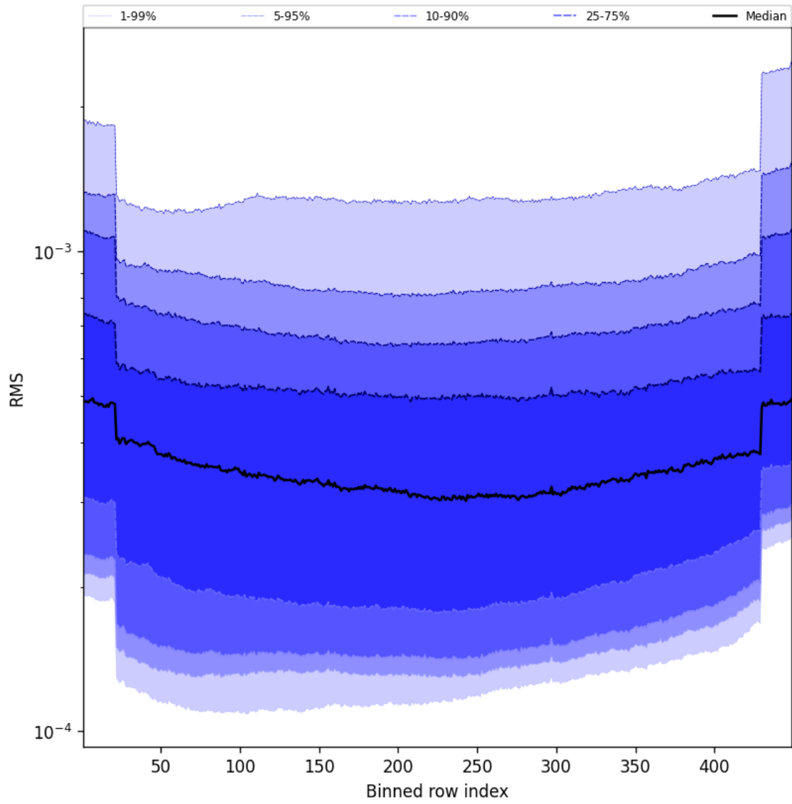
Figure 58: Along track statistics of “RMS” for 2024-12-07 to 2024-12-08
