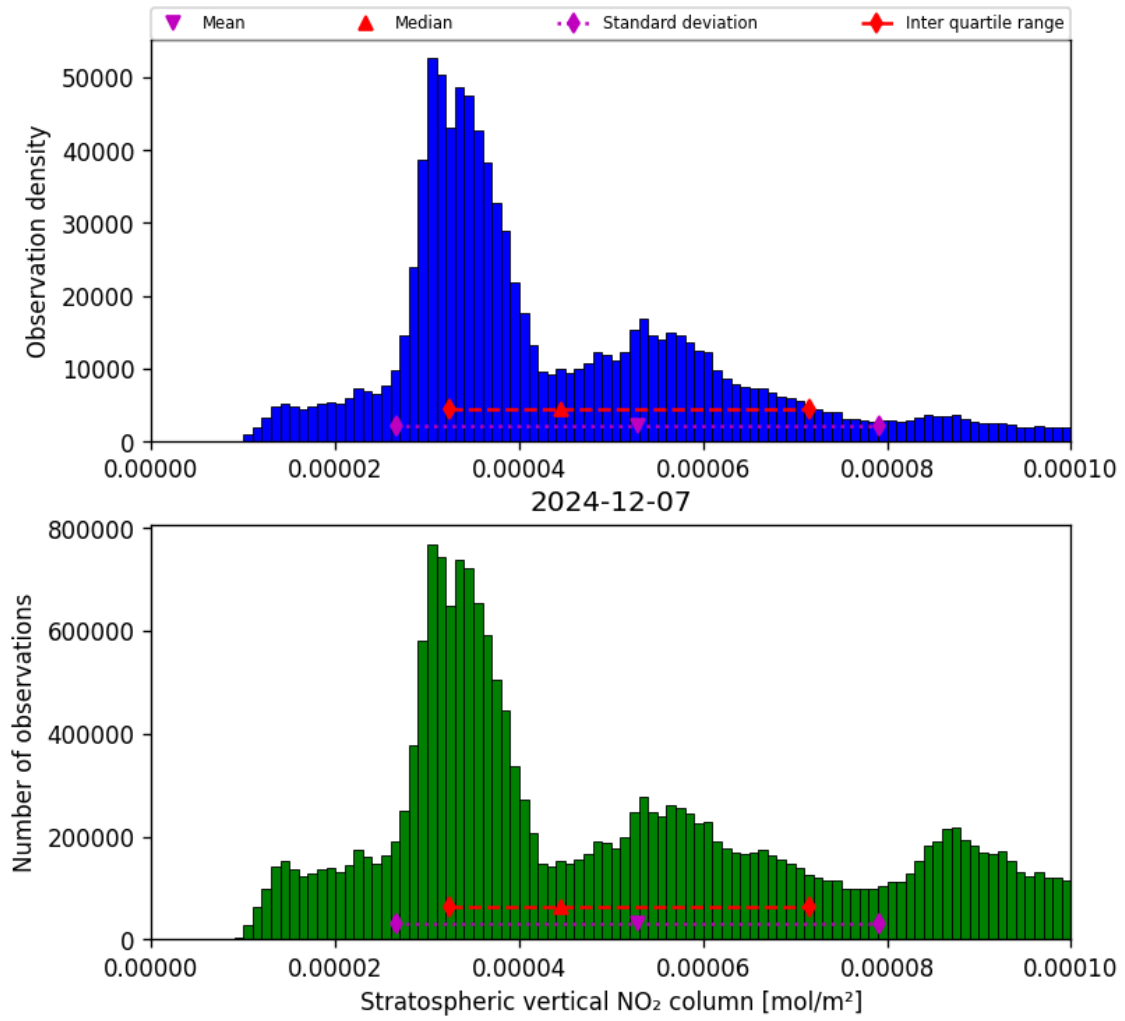
Figure 34: Histogram of “Stratospheric vertical NO 2 column” for 2024-12-07 to 2024-12-08
