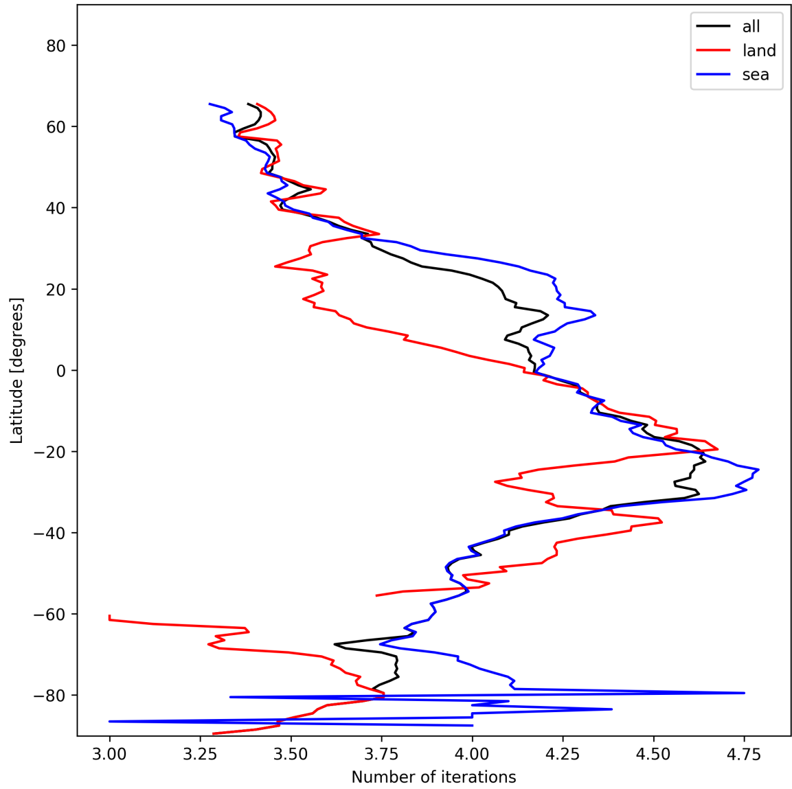
Figure 15: Zonal average of “Number of iterations” for 2024-12-07 to 2024-12-08.
