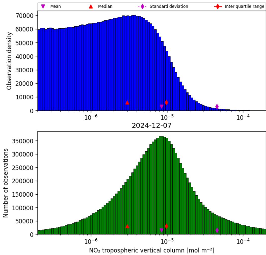
Figure 27: Histogram of “NO 2 tropospheric vertical column” for 2024-12-07 to 2024-12-08
