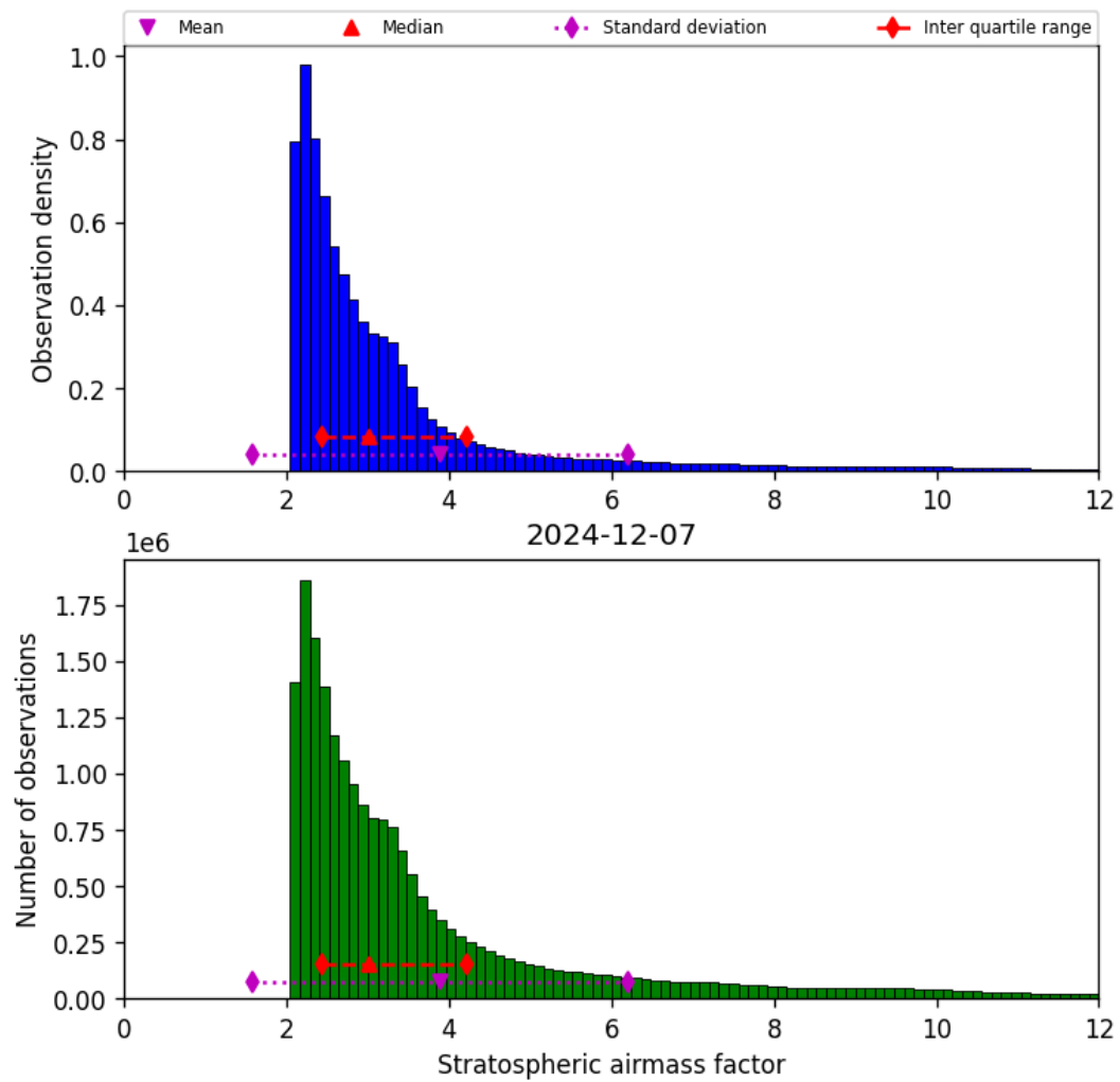
Figure 42: Histogram of “Stratospheric airmass factor” for 2024-12-07 to 2024-12-08
