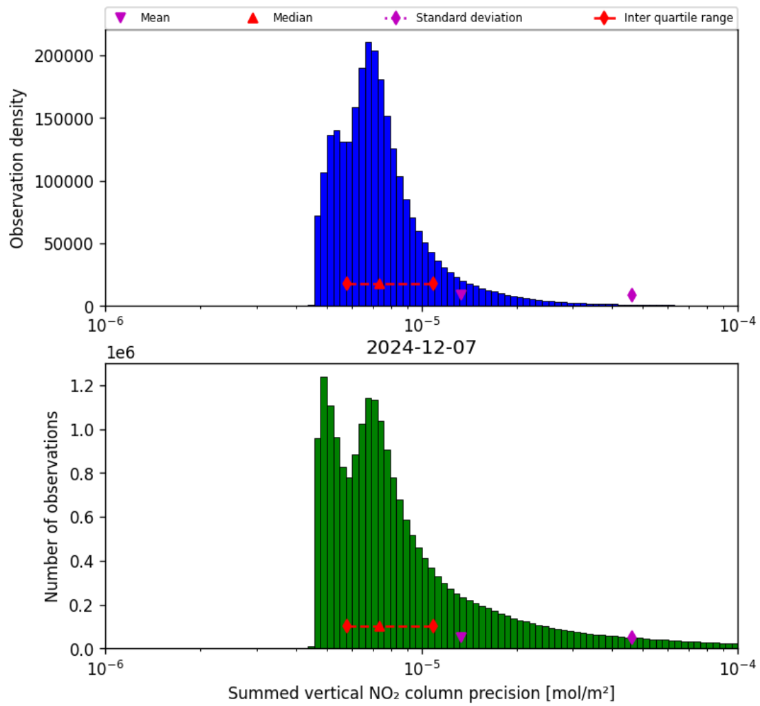
Figure 39: Histogram of “Summed vertical NO 2 column precision” for 2024-12-07 to 2024-12-08
