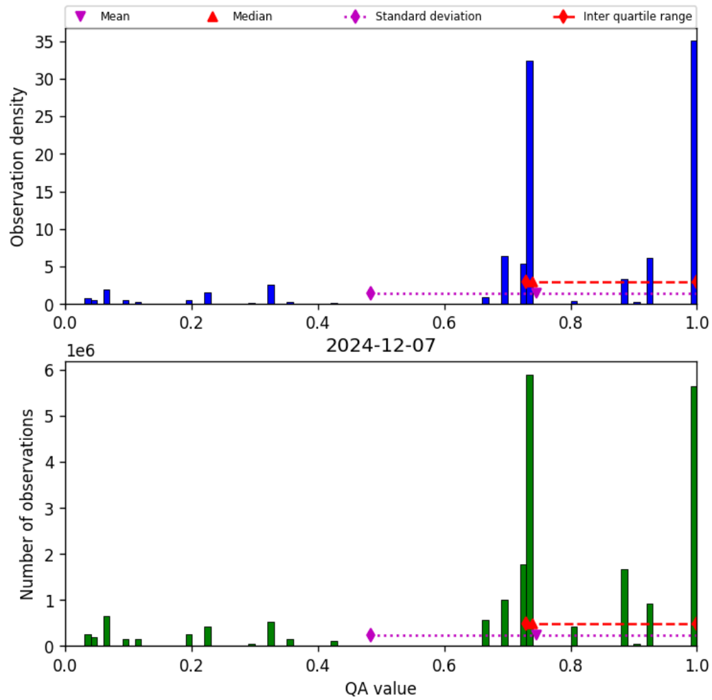
Figure 26: Histogram of “QA value” for 2024-12-07 to 2024-12-08
