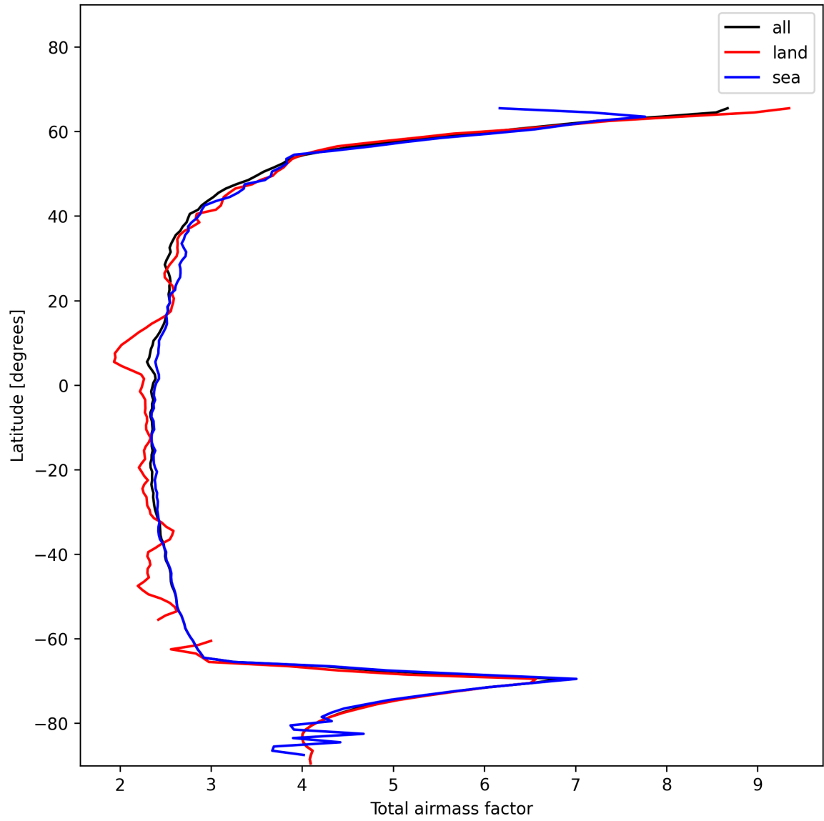
Figure 13: Zonal average of “Total airmass factor” for 2024-12-07 to 2024-12-08.
