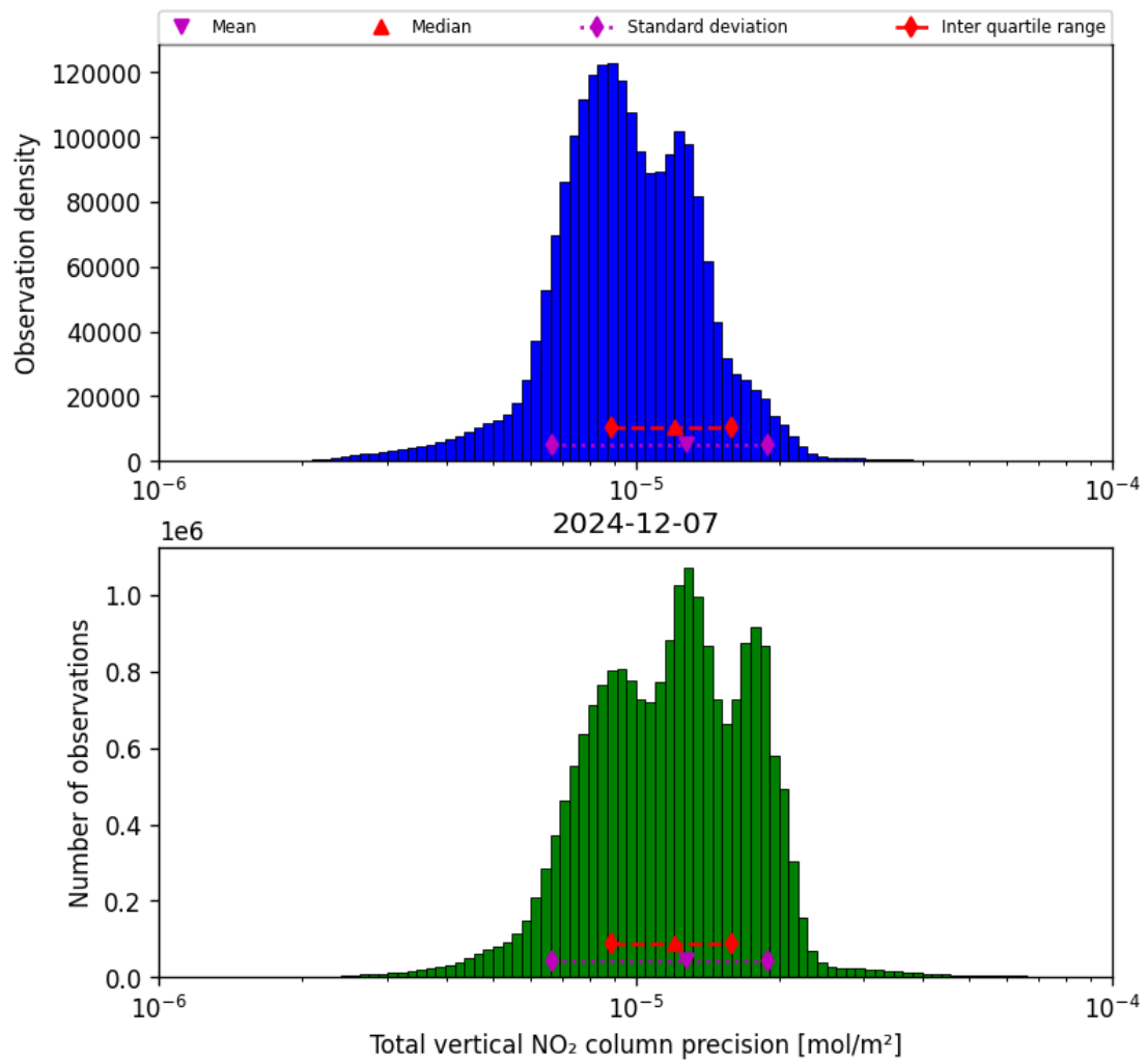
Figure 37: Histogram of “Total vertical NO 2 column precision” for 2024-12-07 to 2024-12-08
