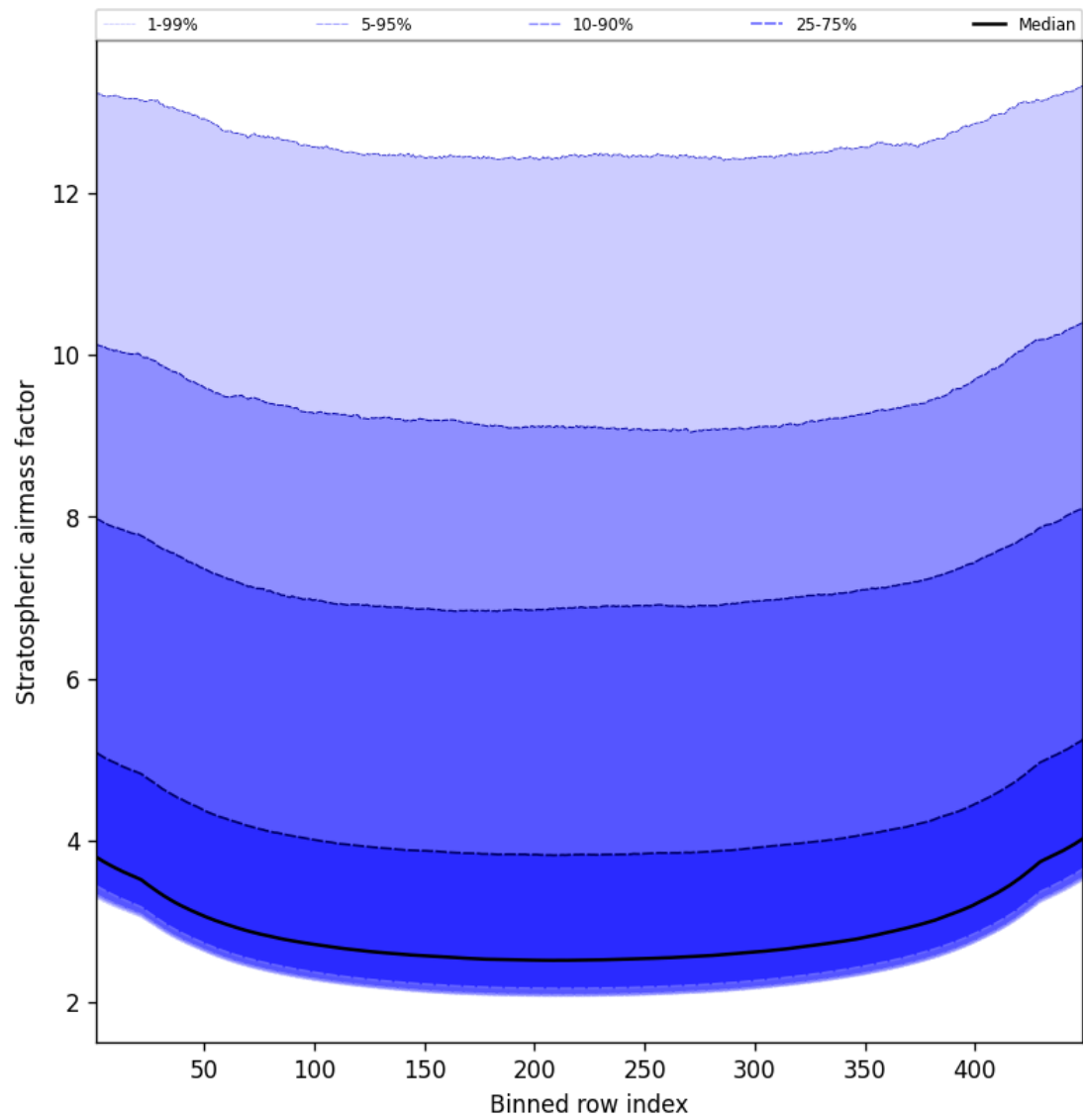
Figure 59: Along track statistics of “Stratospheric airmass factor” for 2024-12-07 to 2024-12-08
