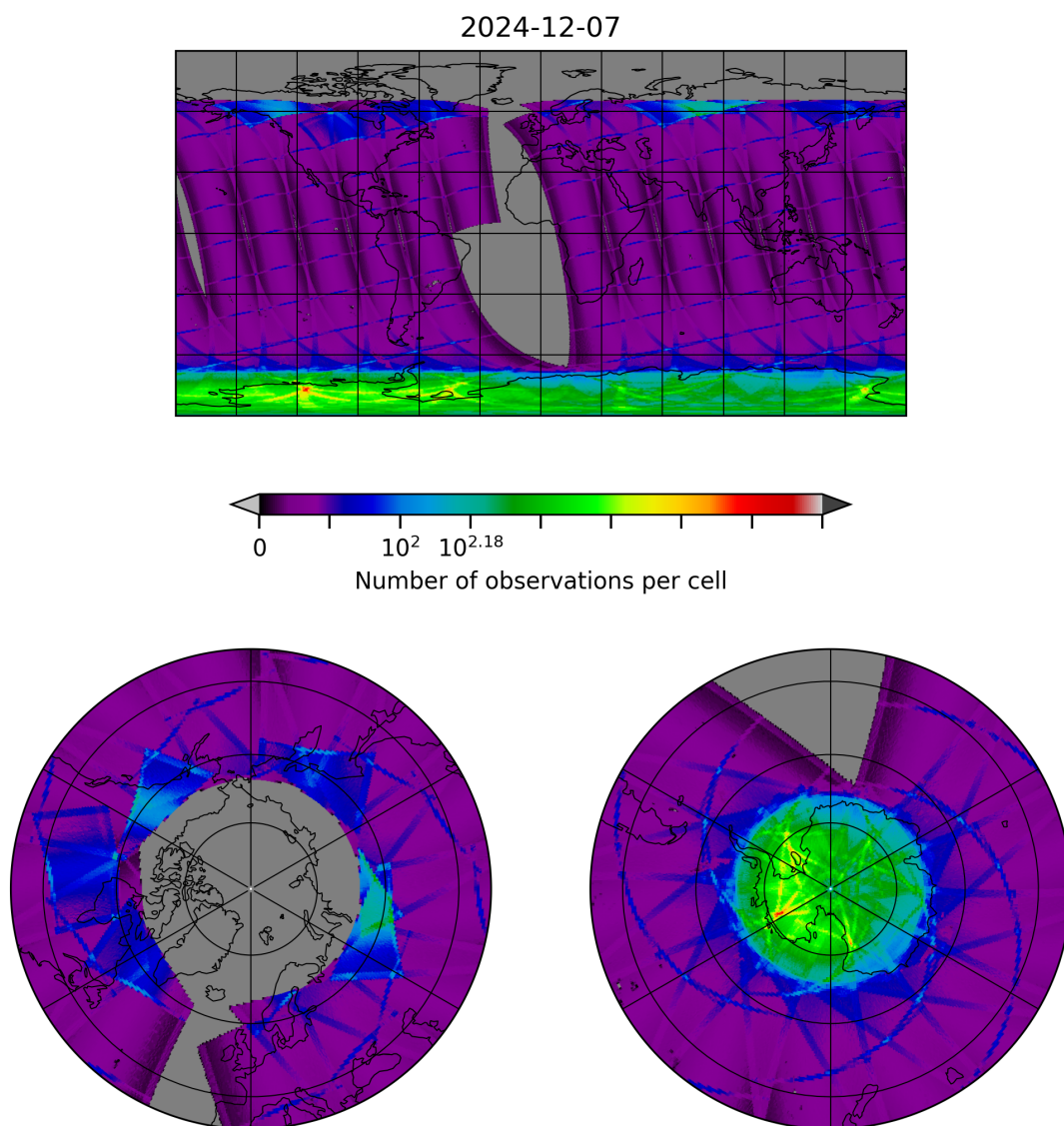
Figure 8: Map of the number of observations for 2024-12-07 to 2024-12-08
