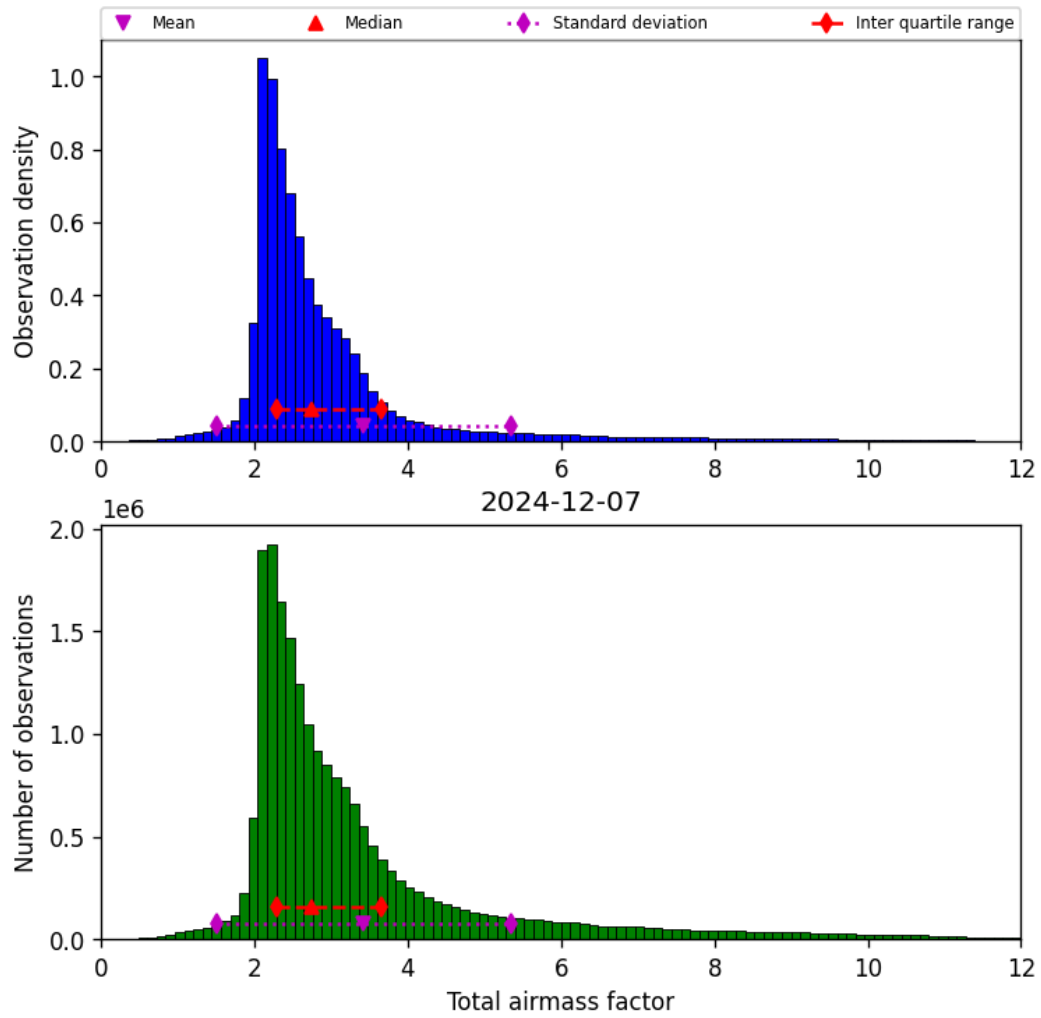
Figure 30: Histogram of “Total airmass factor” for 2024-12-07 to 2024-12-08
