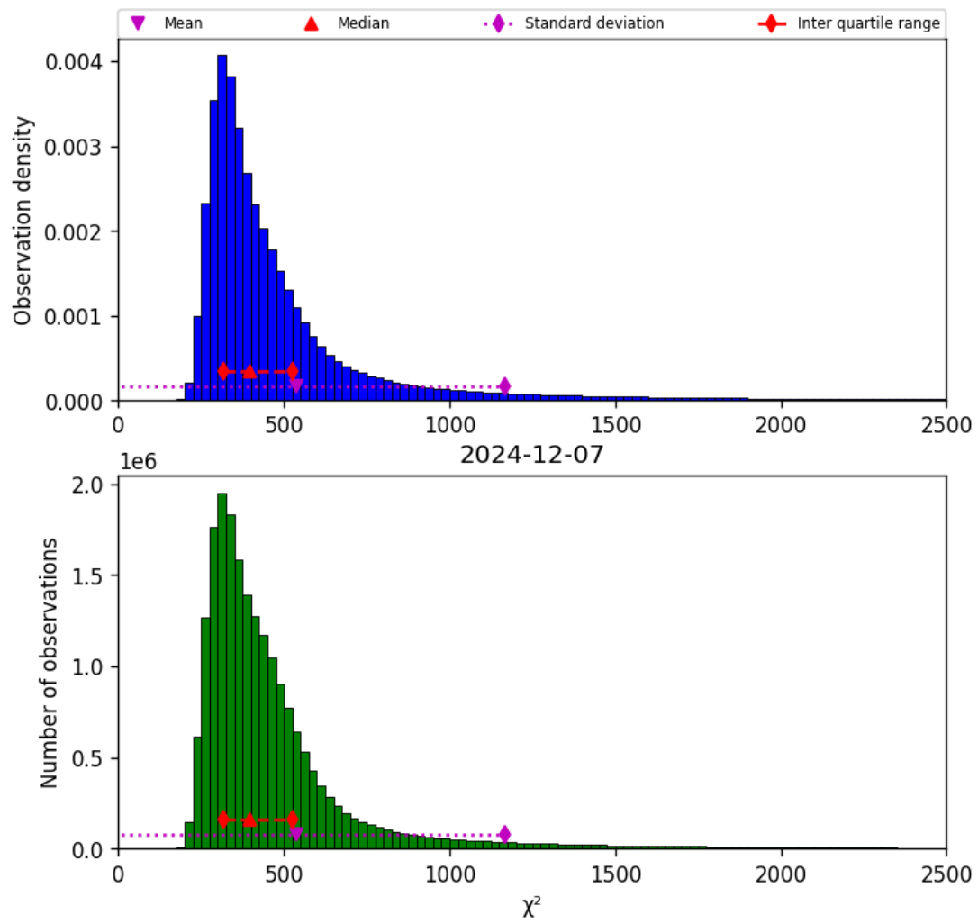
Figure 40: Histogram of " \chi^2 " for 2024-12-07 to 2024-12-08
