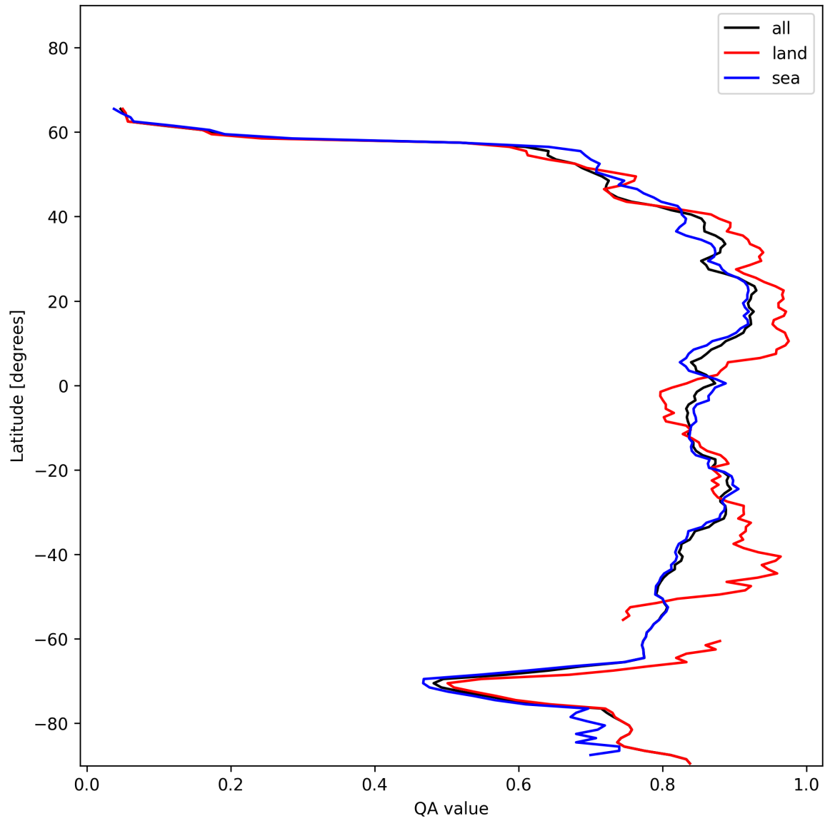
Figure 9: Zonal average of “QA value” for 2024-12-07 to 2024-12-08.
