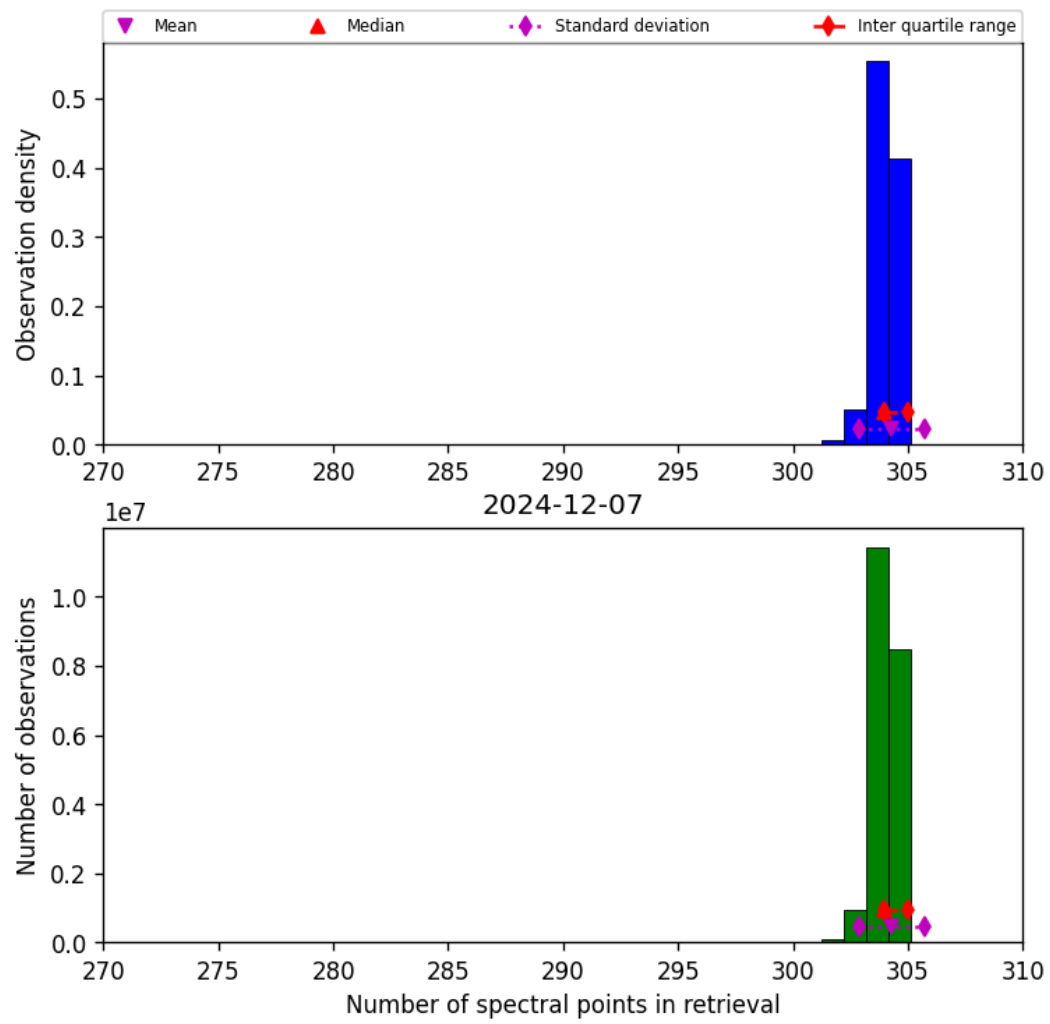
Figure 31: Histogram of “Number of spectral points in retrieval” for 2024-12-07 to 2024-12-08
