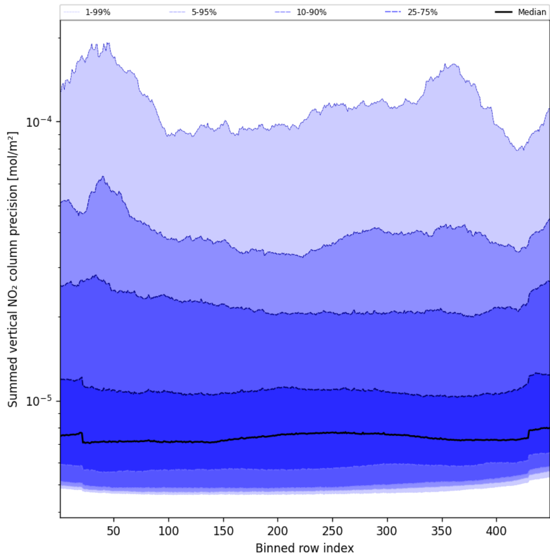
Figure 56: Along track statistics of “Summed vertical NO 2 column precision” for 2024-12-07 to 2024-12-08
