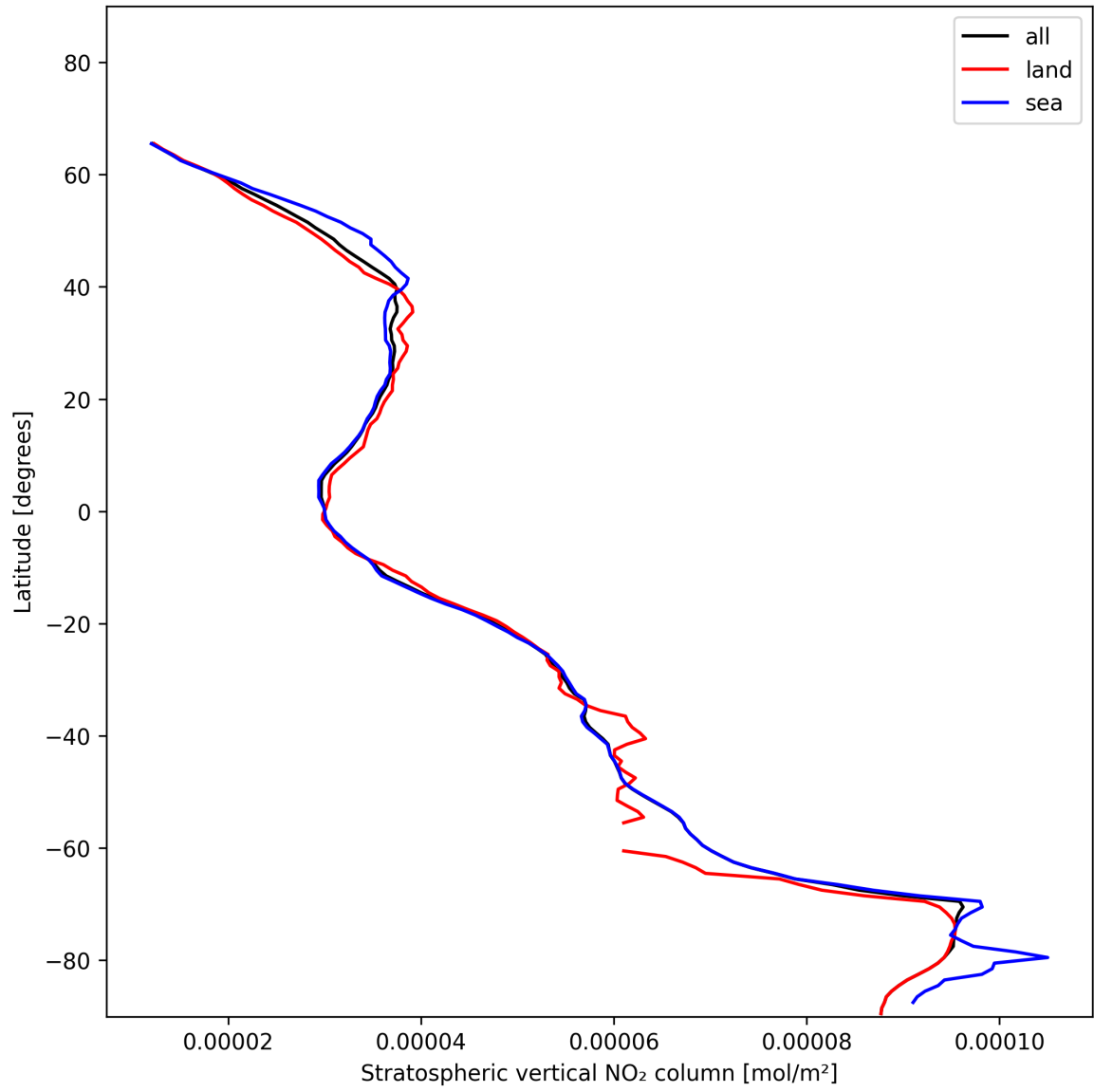
Figure 17: Zonal average of “Stratospheric vertical NO 2 column” for 2024-12-07 to 2024-12-08.
