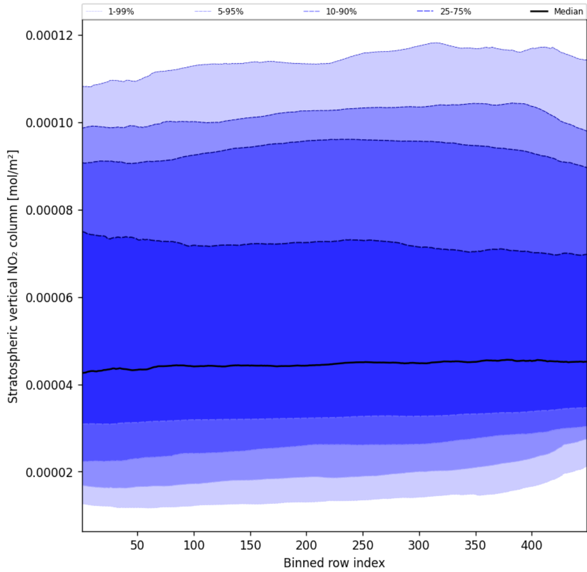
Figure 51: Along track statistics of “Stratospheric vertical NO 2 column” for 2024-12-07 to 2024-12-08
