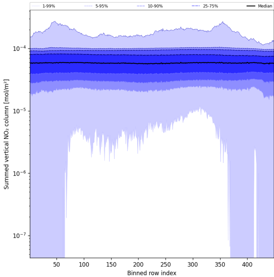
Figure 55: Along track statistics of “Summed vertical NO 2 column” for 2024-12-07 to 2024-12-08
