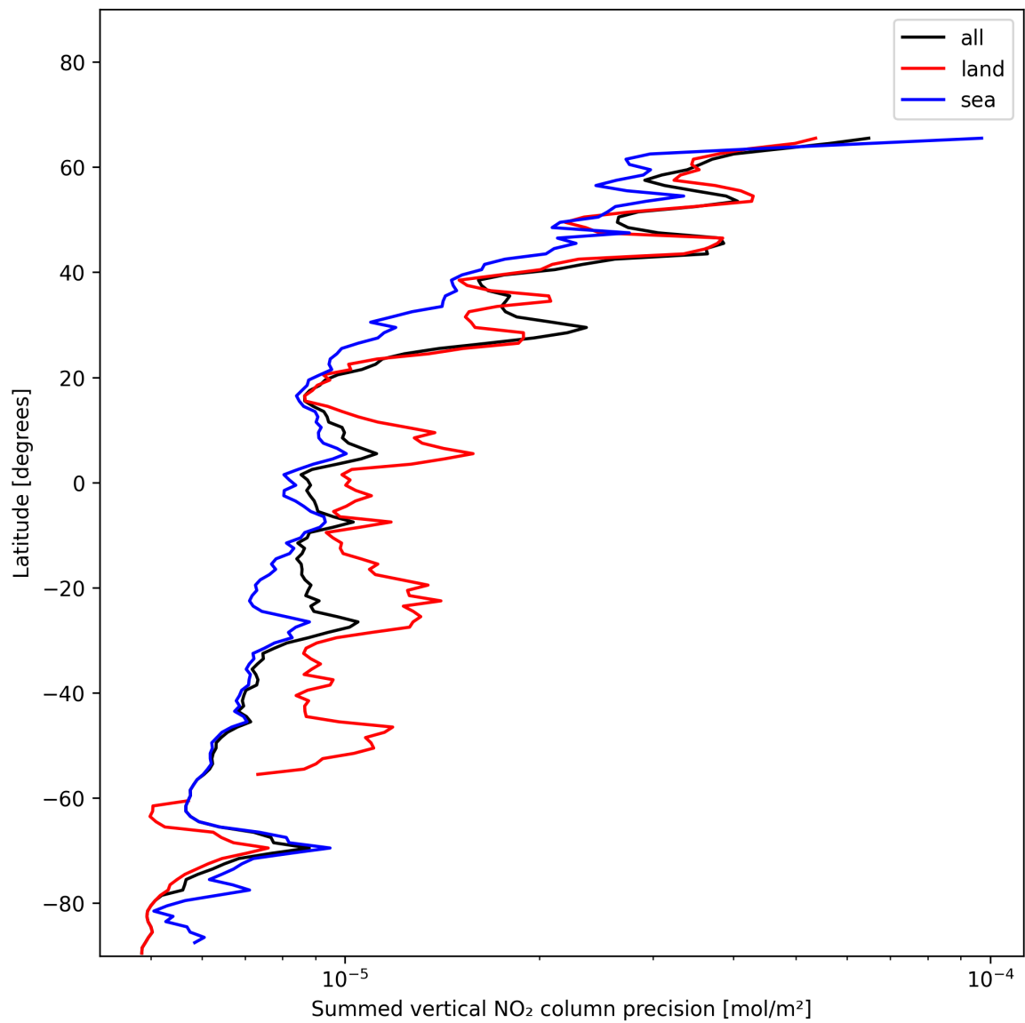
Figure 22: Zonal average of “Summed vertical NO 2 column precision” for 2024-12-07 to 2024-12-08.
