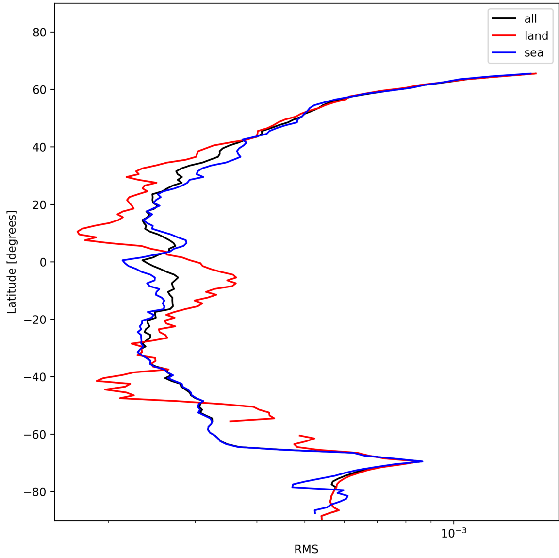
Figure 24: Zonal average of “RMS” for 2024-12-07 to 2024-12-08.
