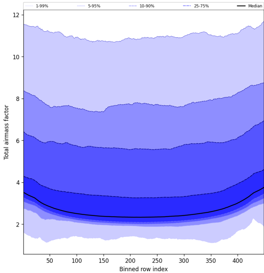
Figure 47: Along track statistics of “Total airmass factor” for 2024-12-07 to 2024-12-08
