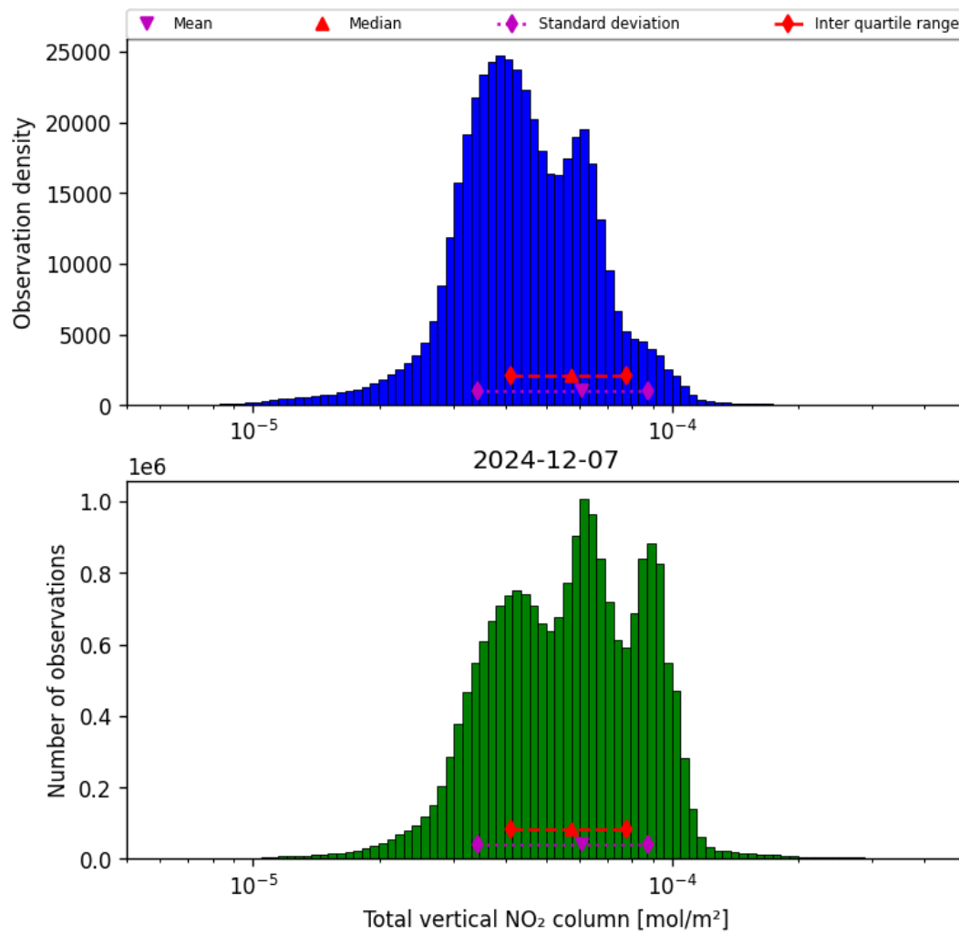
Figure 36: Histogram of “Total vertical NO 2 column” for 2024-12-07 to 2024-12-08
