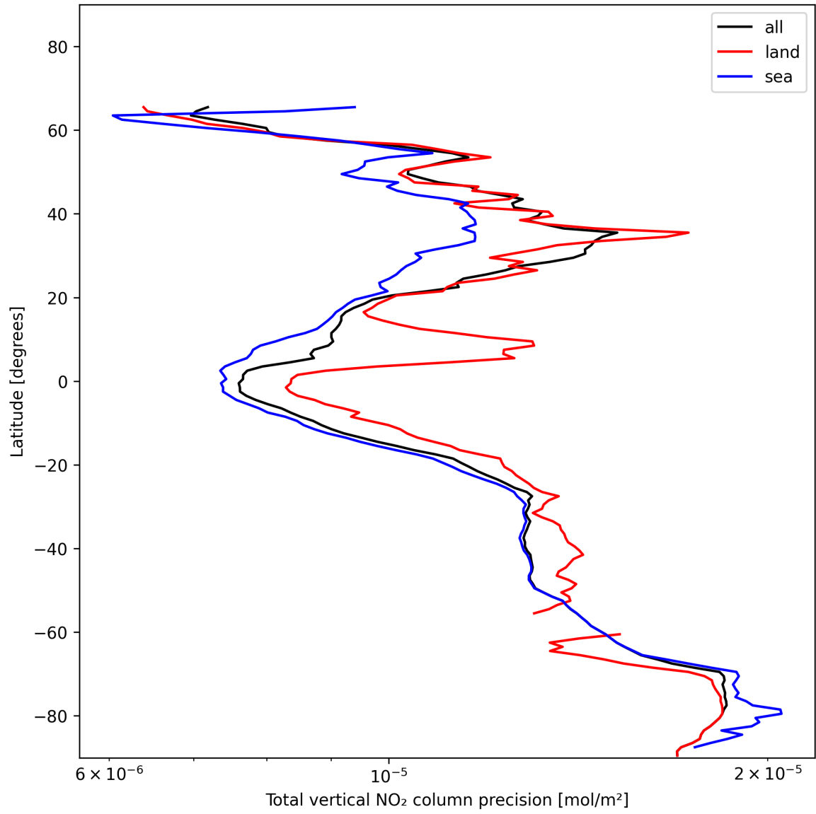
Figure 20: Zonal average of “Total vertical NO 2 column precision” for 2024-12-07 to 2024-12-08.
