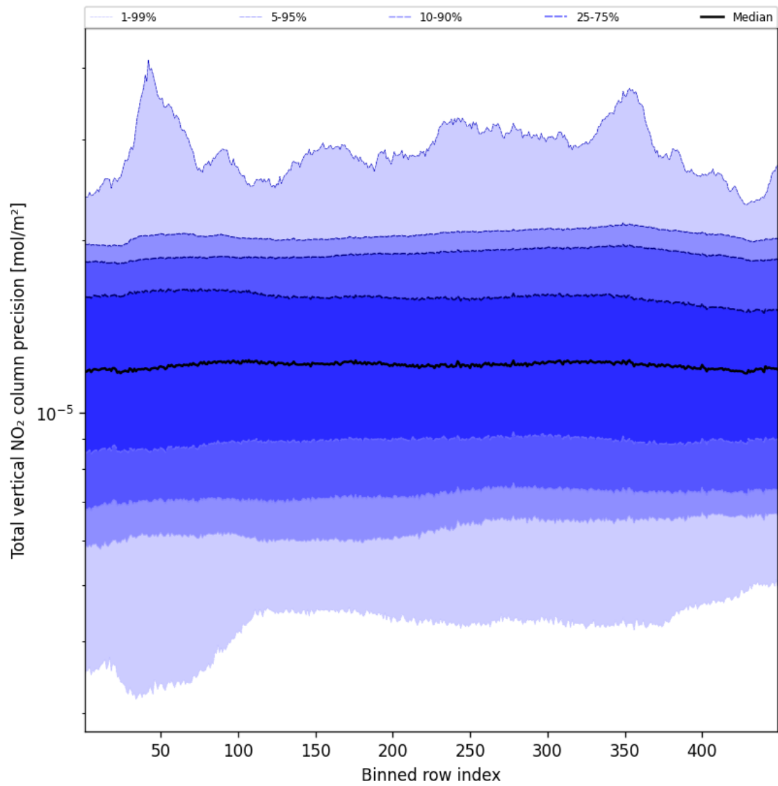
Figure 54: Along track statistics of “Total vertical NO 2 column precision” for 2024-12-07 to 2024-12-08
