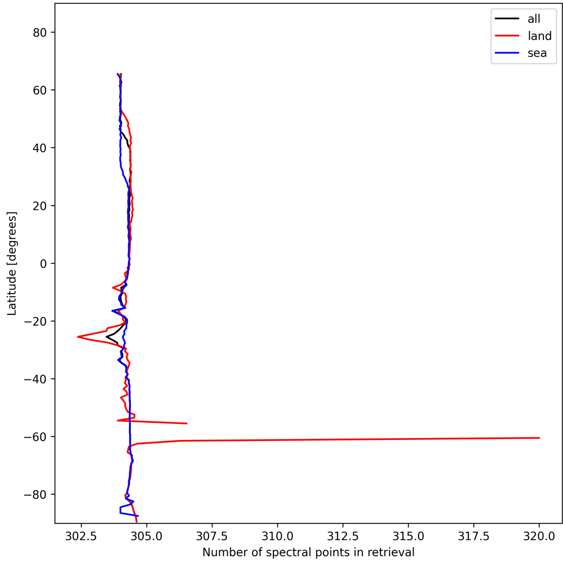
Figure 14: Zonal average of “Number of spectral points in retrieval” for 2024-12-07 to 2024-12-08.
