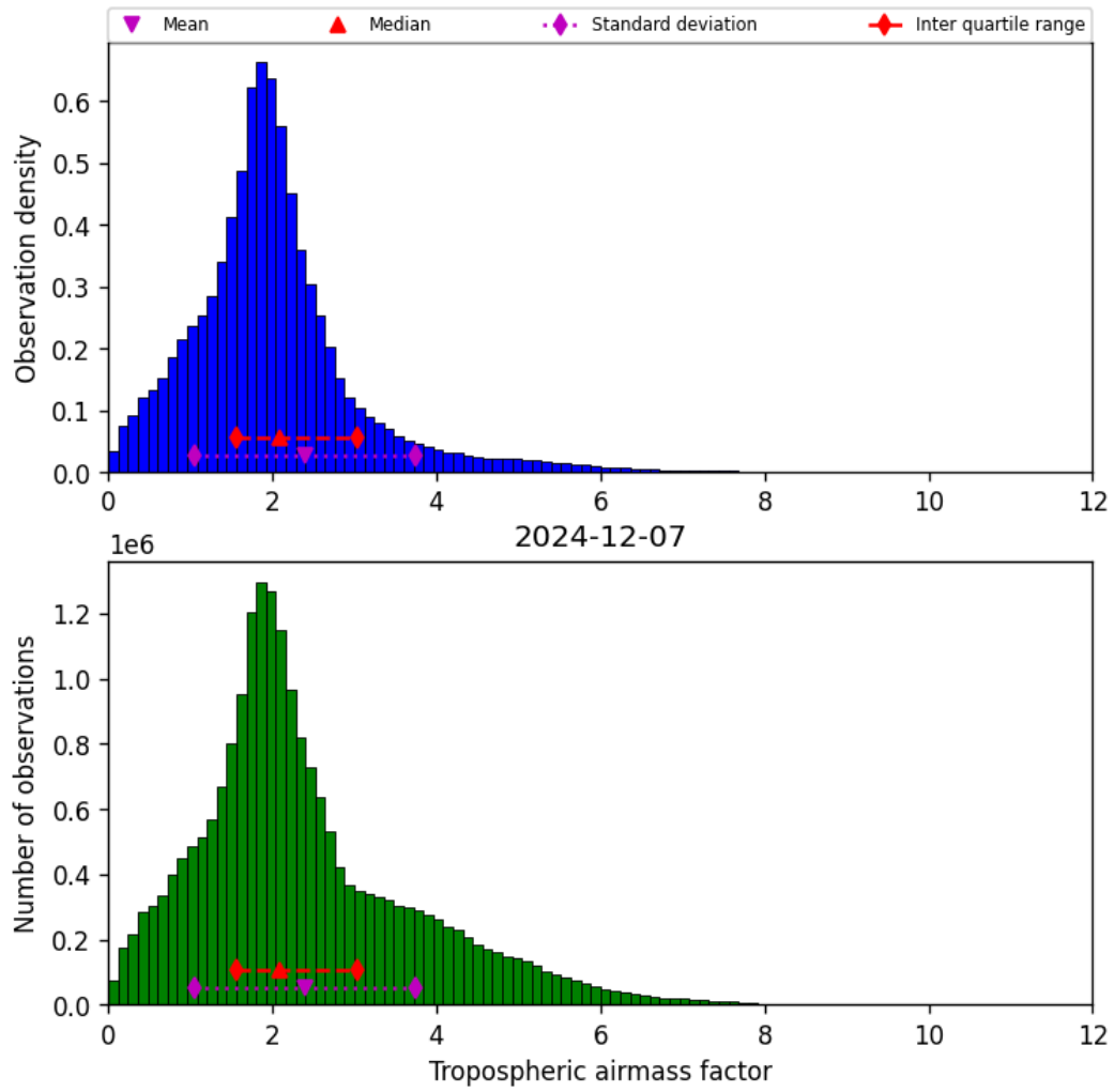
Figure 29: Histogram of “Tropospheric airmass factor” for 2024-12-07 to 2024-12-08
