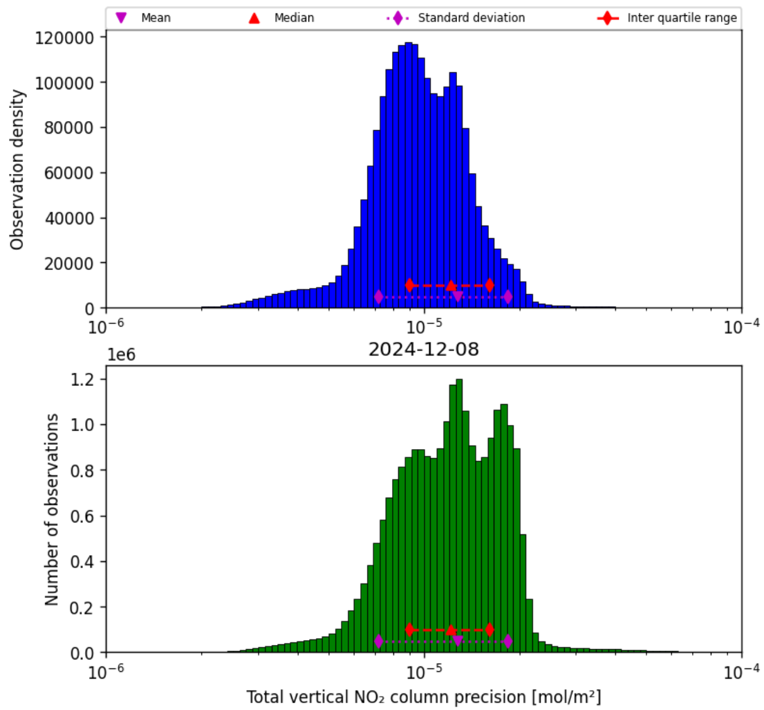
Figure 37: Histogram of “Total vertical NO 2 column precision” for 2024-12-08 to 2024-12-09
