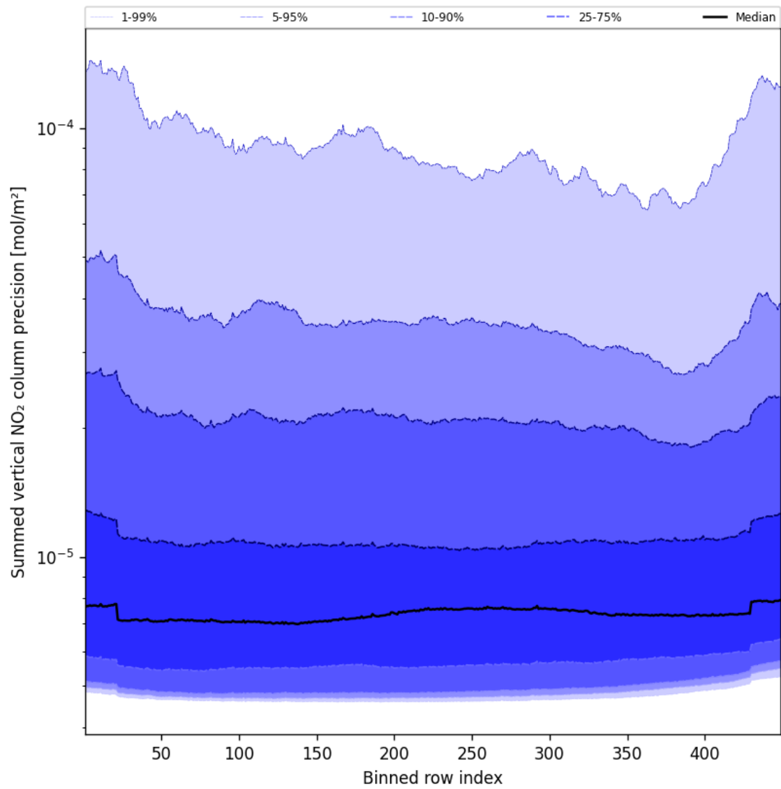
Figure 56: Along track statistics of “Summed vertical NO 2 column precision” for 2024-12-08 to 2024-12-09
