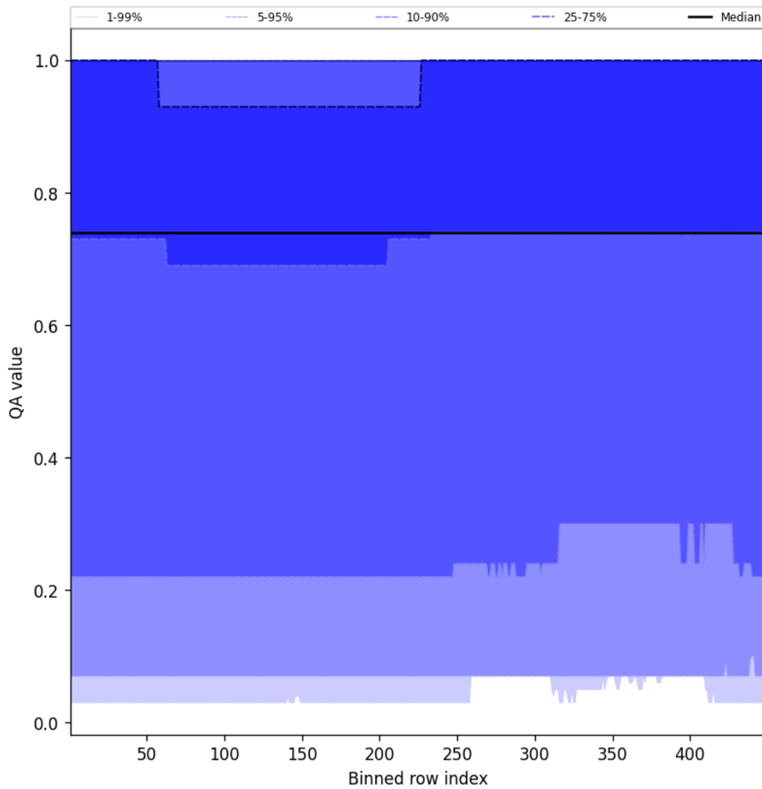
Figure 43: Along track statistics of “QA value” for 2024-12-08 to 2024-12-09
