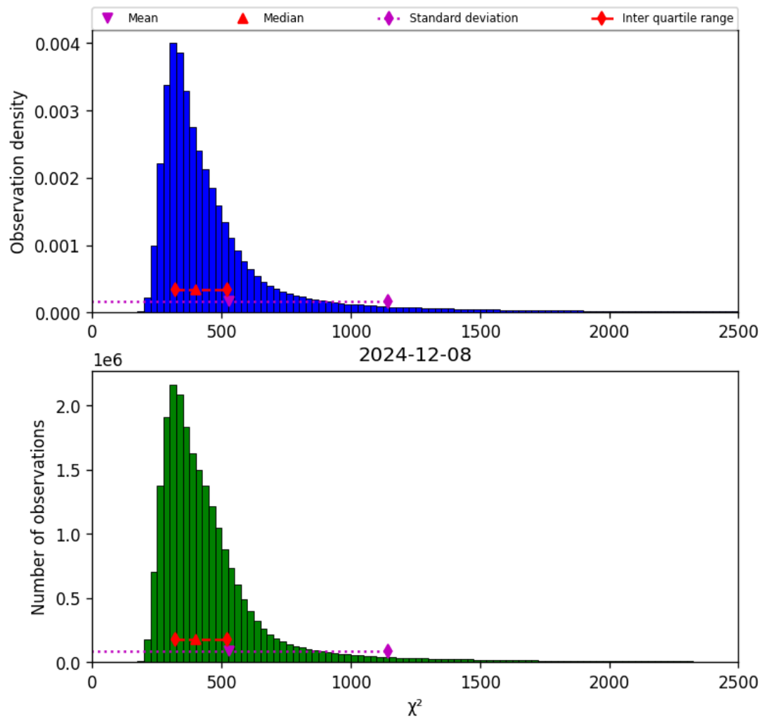
Figure 40: Histogram of “ \chi^2 ” for 2024-12-08 to 2024-12-09
