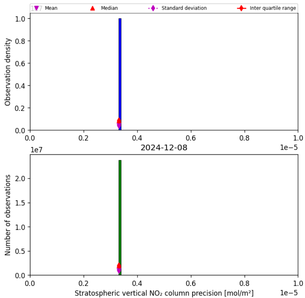
Figure 35: Histogram of “Stratospheric vertical NO 2 column precision” for 2024-12-08 to 2024-12-09
