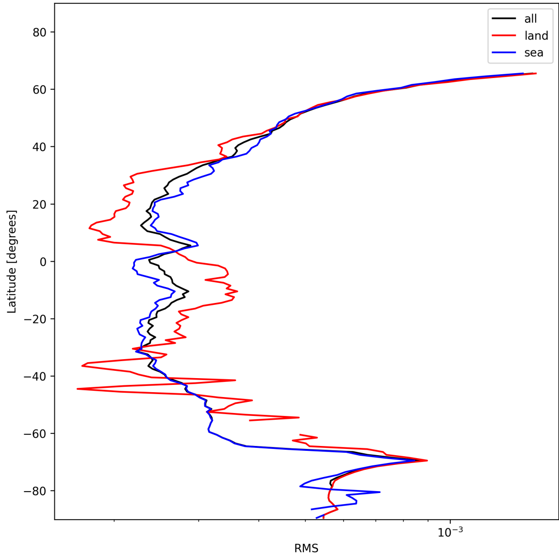
Figure 24: Zonal average of “RMS” for 2024-12-08 to 2024-12-09.
