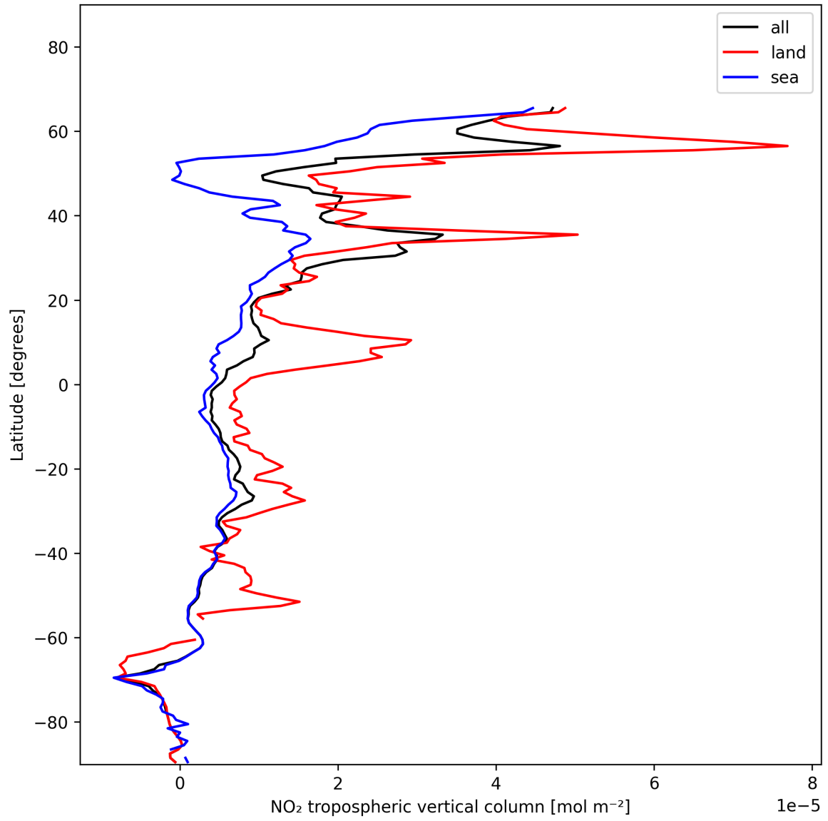
Figure 10: Zonal average of “NO 2 tropospheric vertical column” for 2024-12-08 to 2024-12-09.
