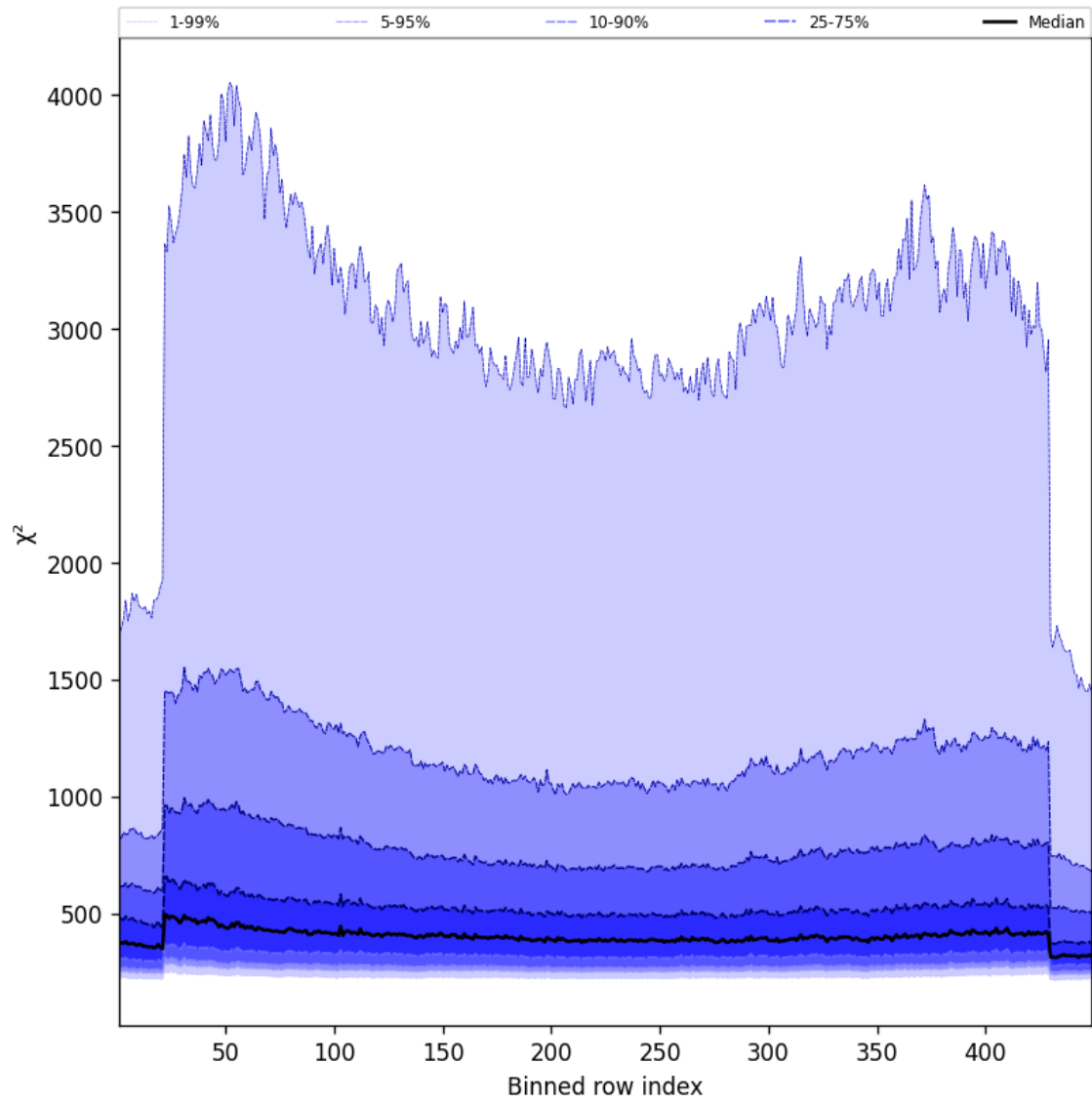
Figure 57: Along track statistics of “ \chi^2 ” for 2024-12-08 to 2024-12-09
