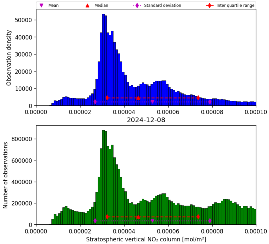
Figure 34: Histogram of “Stratospheric vertical NO 2 column” for 2024-12-08 to 2024-12-09
