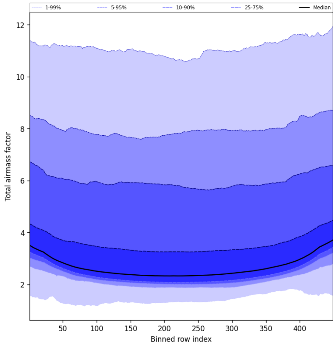
Figure 47: Along track statistics of “Total airmass factor” for 2024-12-08 to 2024-12-09
