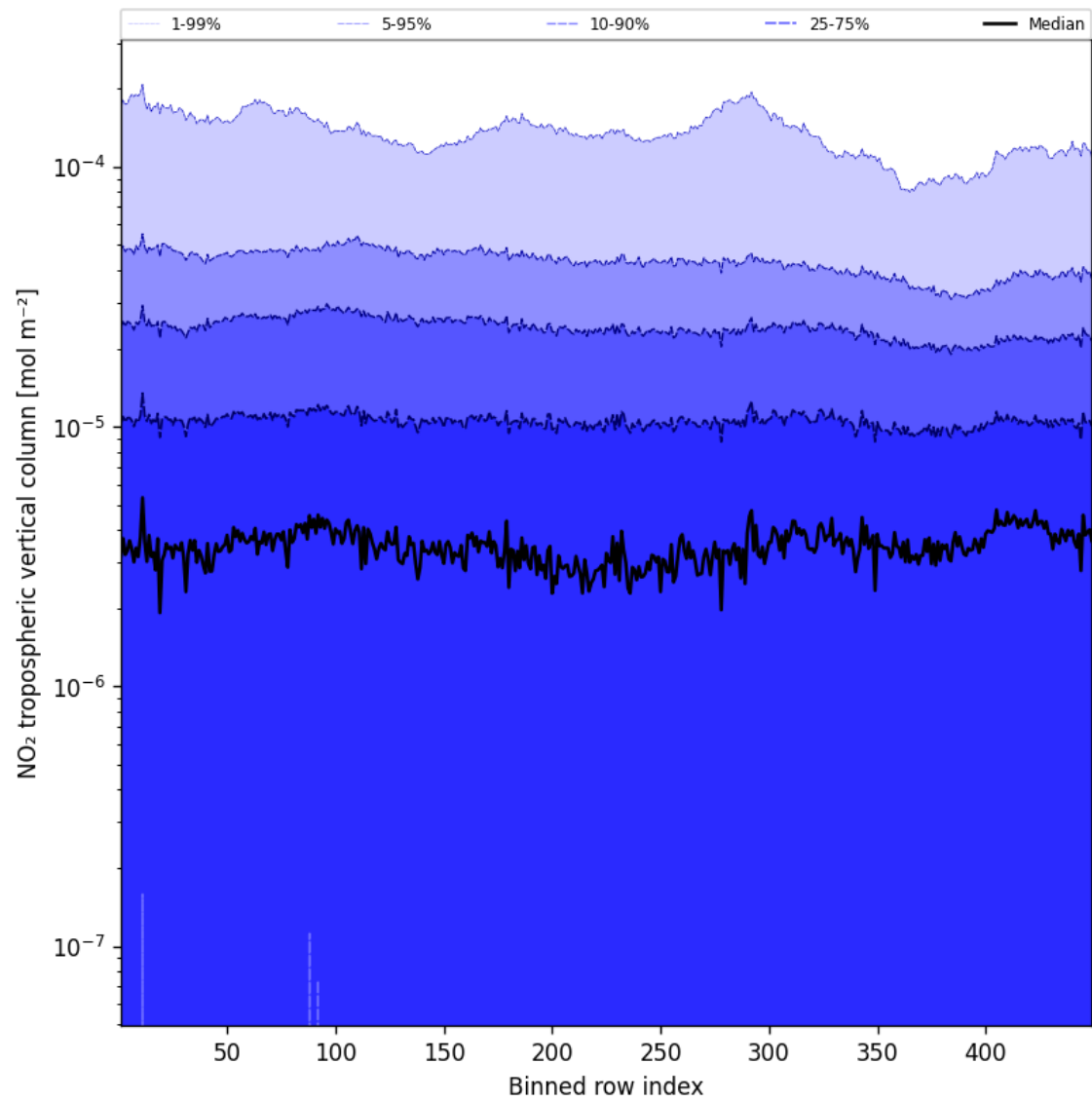
Figure 44: Along track statistics of “NO 2 tropospheric vertical column” for 2024-12-08 to 2024-12-09
