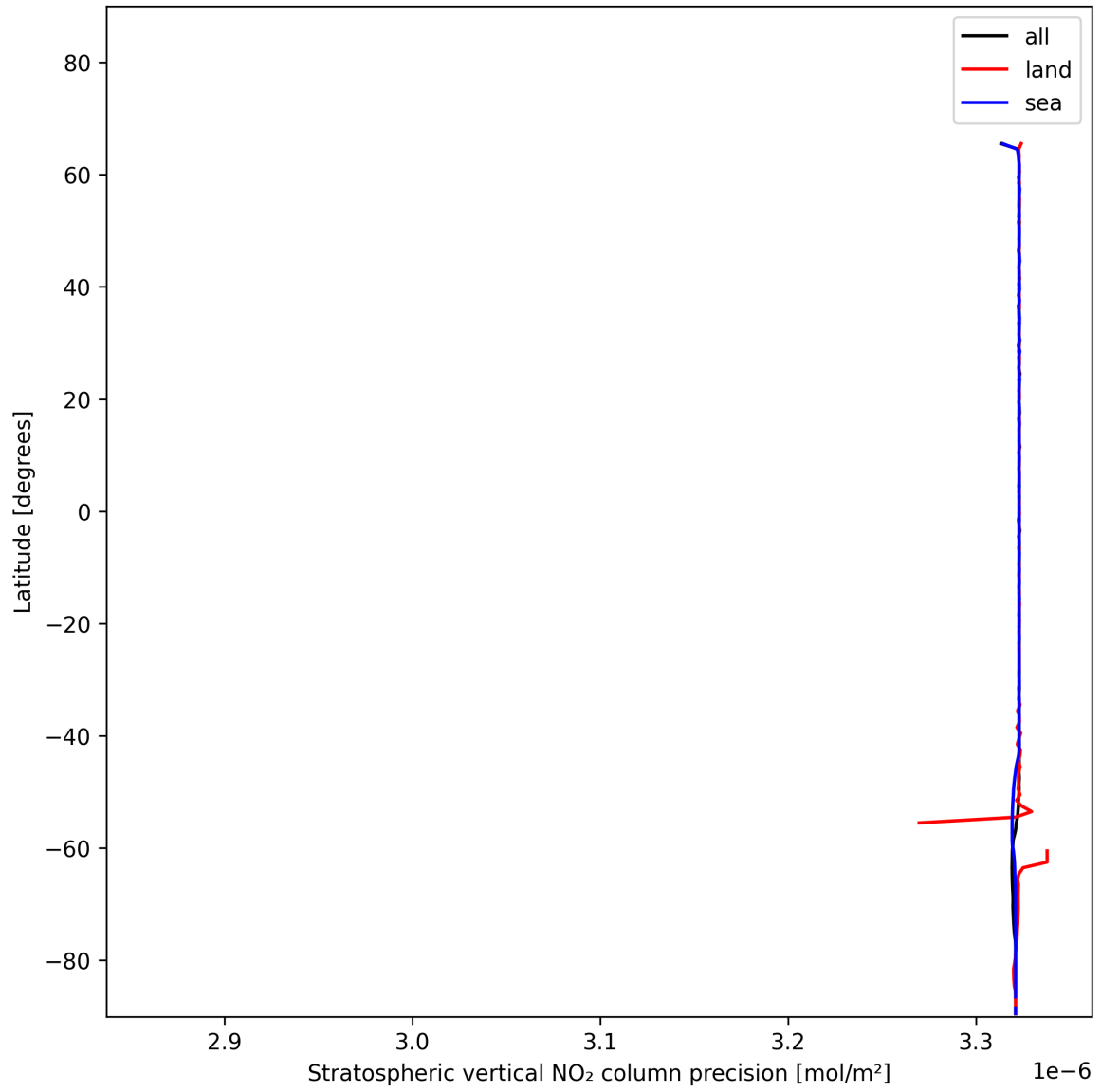
Figure 18: Zonal average of "Stratospheric vertical NO 2 column precision" for 2024-12-08 to 2024-12-09.
