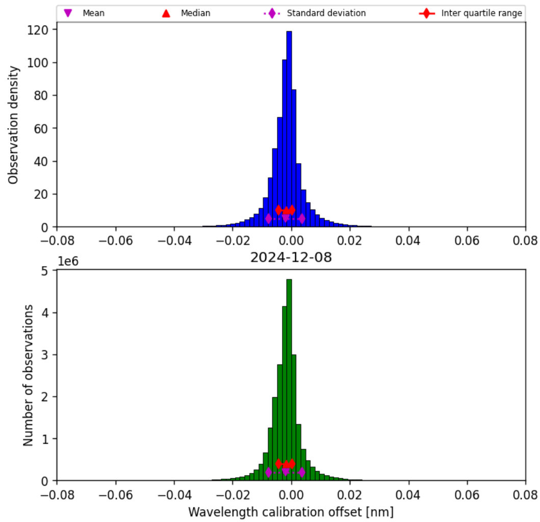
Figure 33: Histogram of “Wavelength calibration offset” for 2024-12-08 to 2024-12-09
