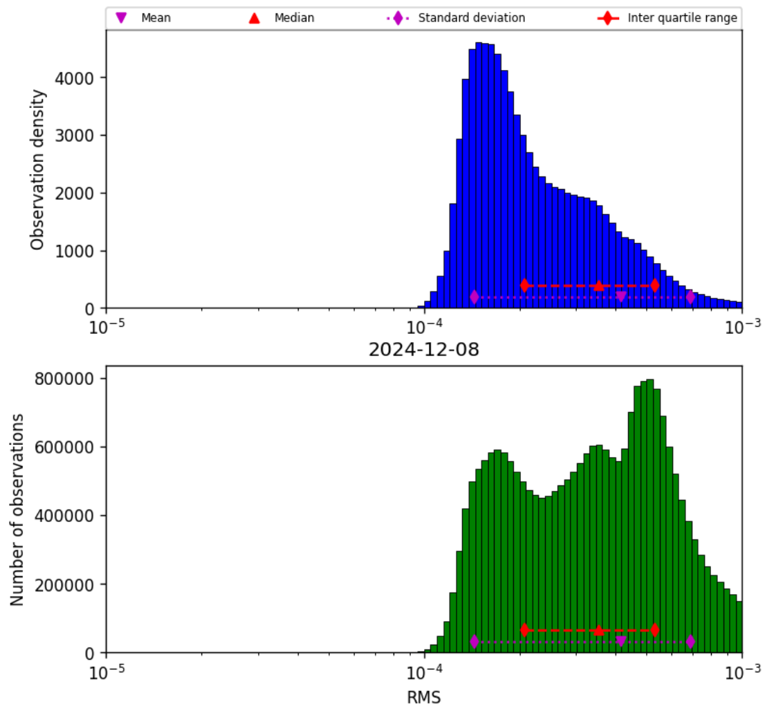
Figure 41: Histogram of “RMS” for 2024-12-08 to 2024-12-09
