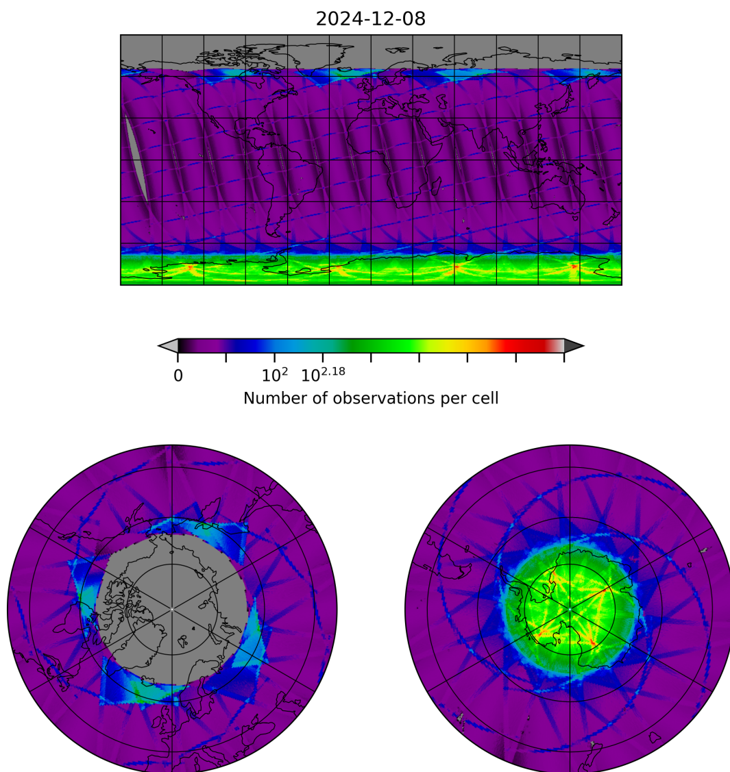
Figure 8: Map of the number of observations for 2024-12-08 to 2024-12-09
