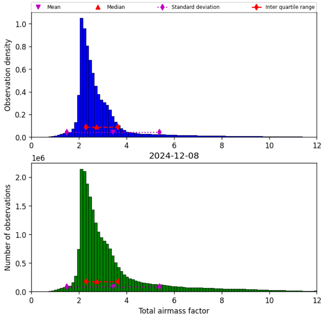
Figure 30: Histogram of “Total airmass factor” for 2024-12-08 to 2024-12-09
