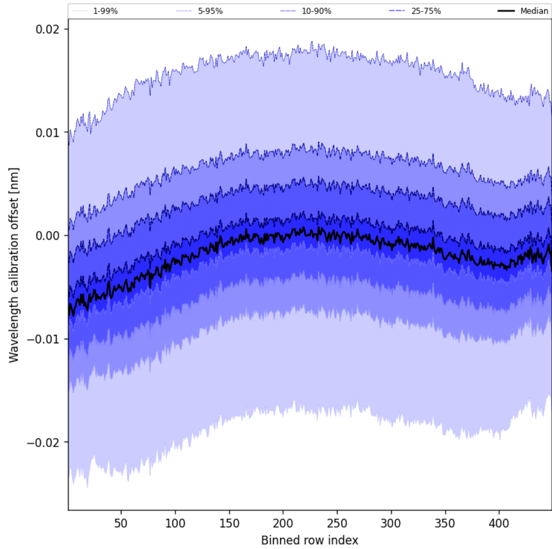
Figure 50: Along track statistics of “Wavelength calibration offset” for 2024-12-08 to 2024-12-09
