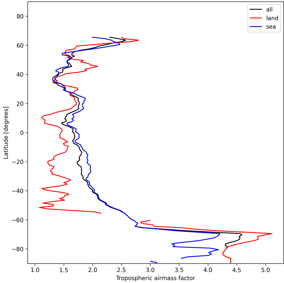
Figure 12: Zonal average of “Tropospheric airmass factor” for 2024-12-08 to 2024-12-09.
