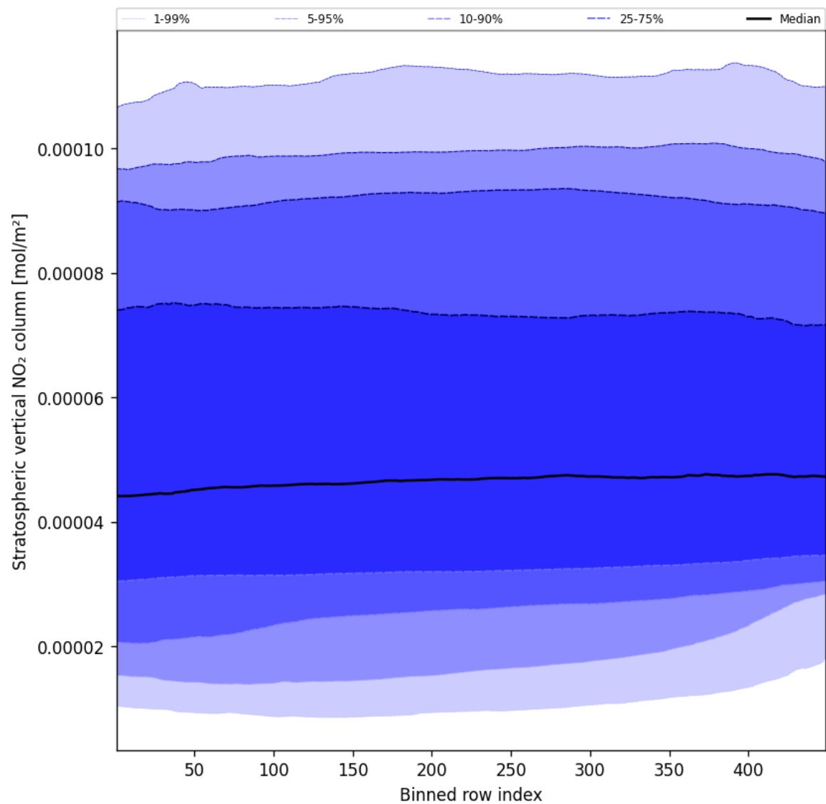
Figure 51: Along track statistics of “Stratospheric vertical NO 2 column” for 2024-12-08 to 2024-12-09
