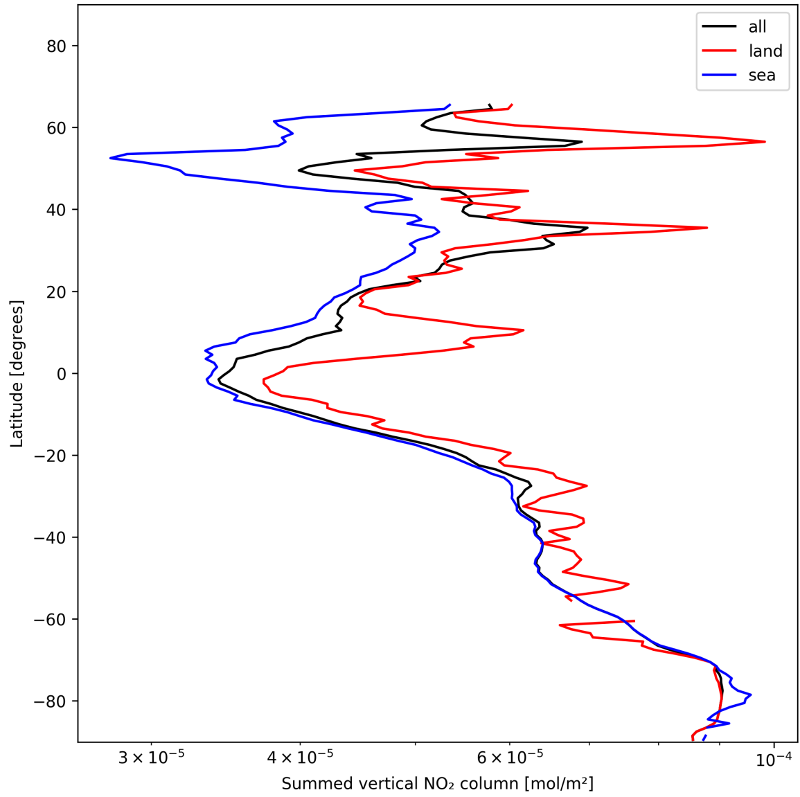
Figure 21: Zonal average of “Summed vertical NO 2 column” for 2024-12-08 to 2024-12-09.
