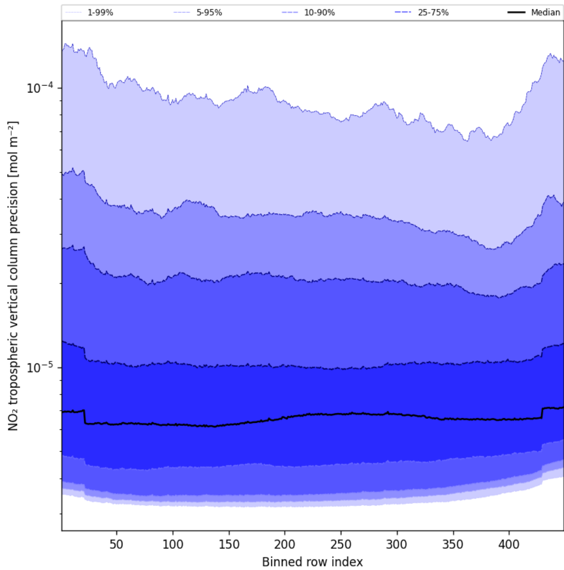
Figure 45: Along track statistics of “NO 2 tropospheric vertical column precision” for 2024-12-08 to 2024-12-09
