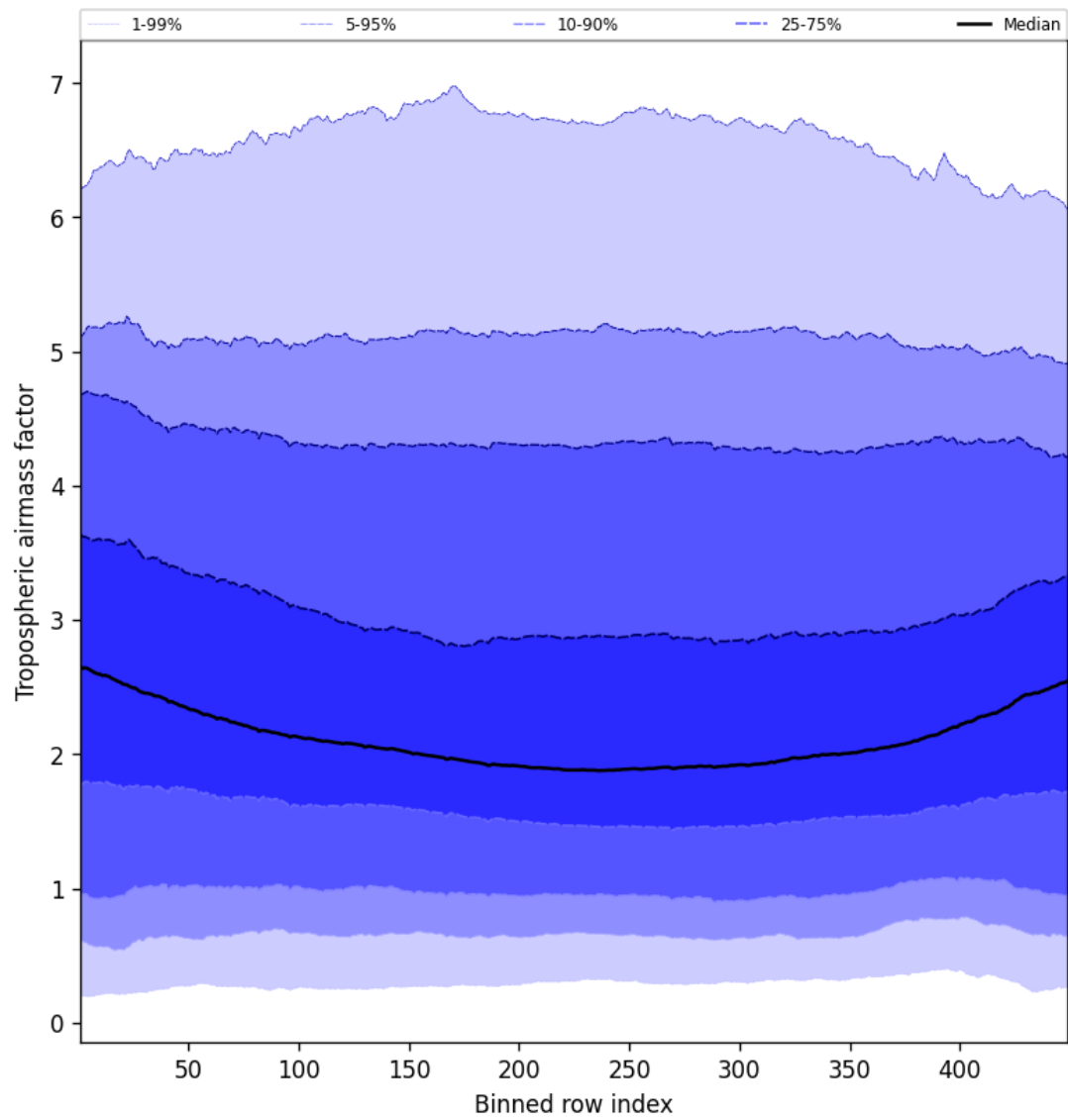
Figure 46: Along track statistics of “Tropospheric air mass factor” for 2024-12-08 to 2024-12-09
