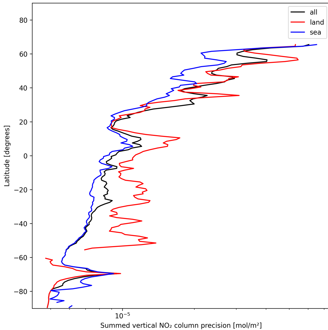
Figure 22: Zonal average of “Summed vertical NO 2 column precision” for 2024-12-08 to 2024-12-09.
