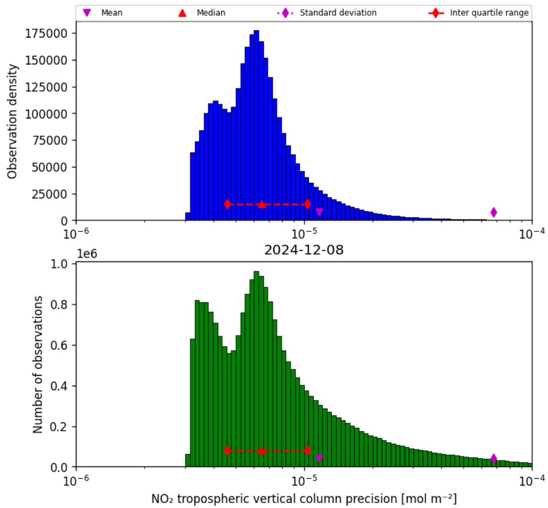
Figure 28: Histogram of “NO 2 tropospheric vertical column precision” for 2024-12-08 to 2024-12-09
