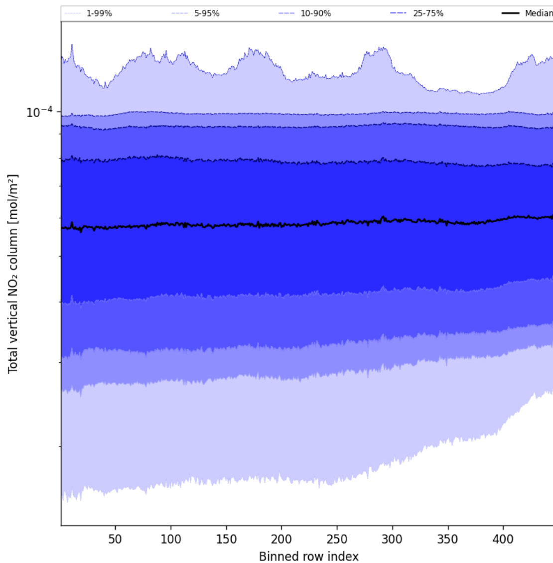
Figure 53: Along track statistics of “Total vertical NO 2 column” for 2024-12-08 to 2024-12-09
