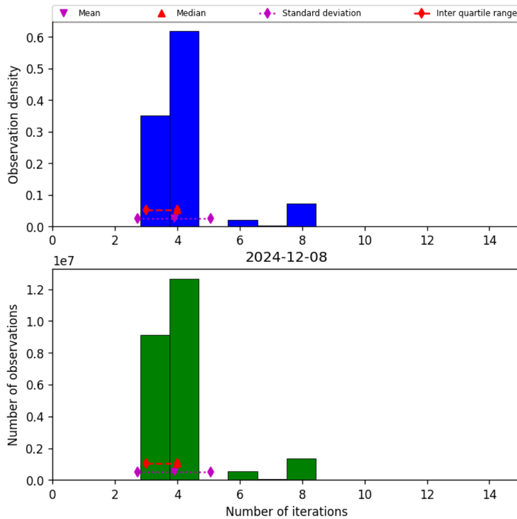
Figure 32: Histogram of “Number of iterations” for 2024-12-08 to 2024-12-09
