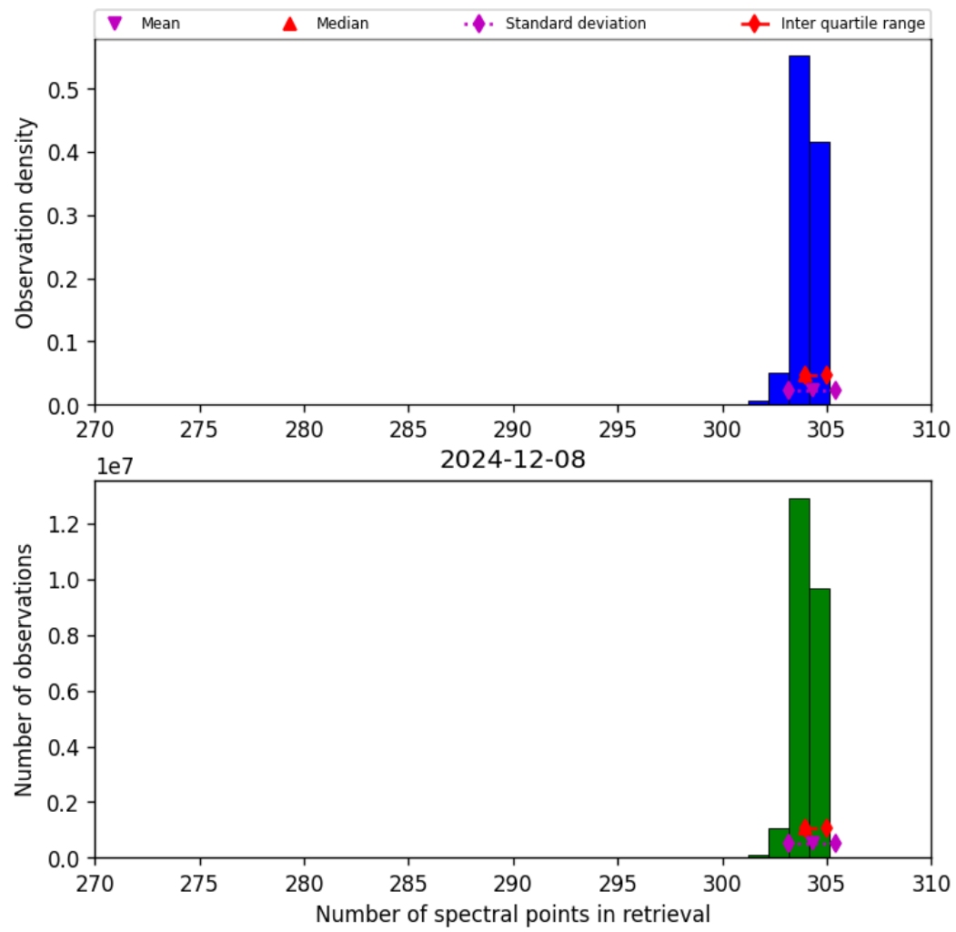
Figure 31: Histogram of “Number of spectral points in retrieval” for 2024-12-08 to 2024-12-09
