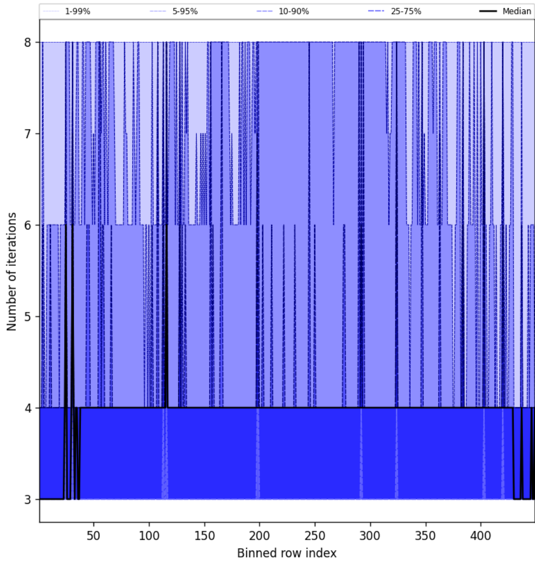
Figure 49: Along track statistics of “Number of iterations” for 2024-12-08 to 2024-12-09
