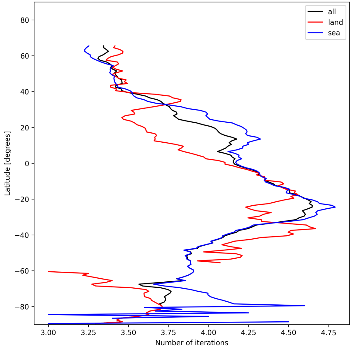
Figure 15: Zonal average of “Number of iterations” for 2024-12-08 to 2024-12-09.
