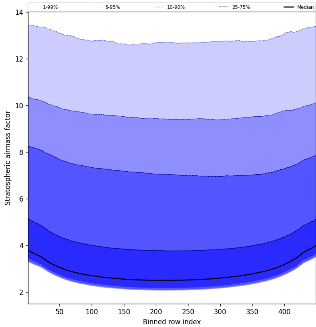
Figure 59: Along track statistics of “Stratospheric airmass factor” for 2024-12-08 to 2024-12-09
