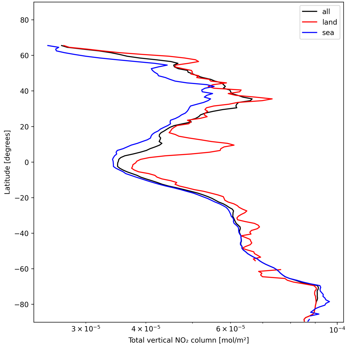
Figure 19: Zonal average of “Total vertical NO 2 column” for 2024-12-08 to 2024-12-09.
