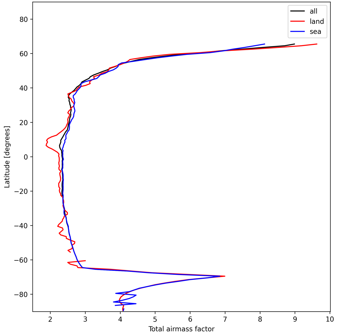
Figure 13: Zonal average of “Total airmass factor” for 2024-12-08 to 2024-12-09.
