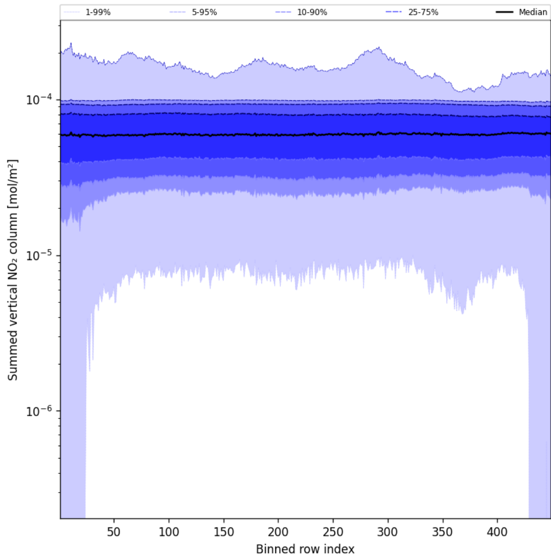
Figure 55: Along track statistics of “Summed vertical NO 2 column” for 2024-12-08 to 2024-12-09
