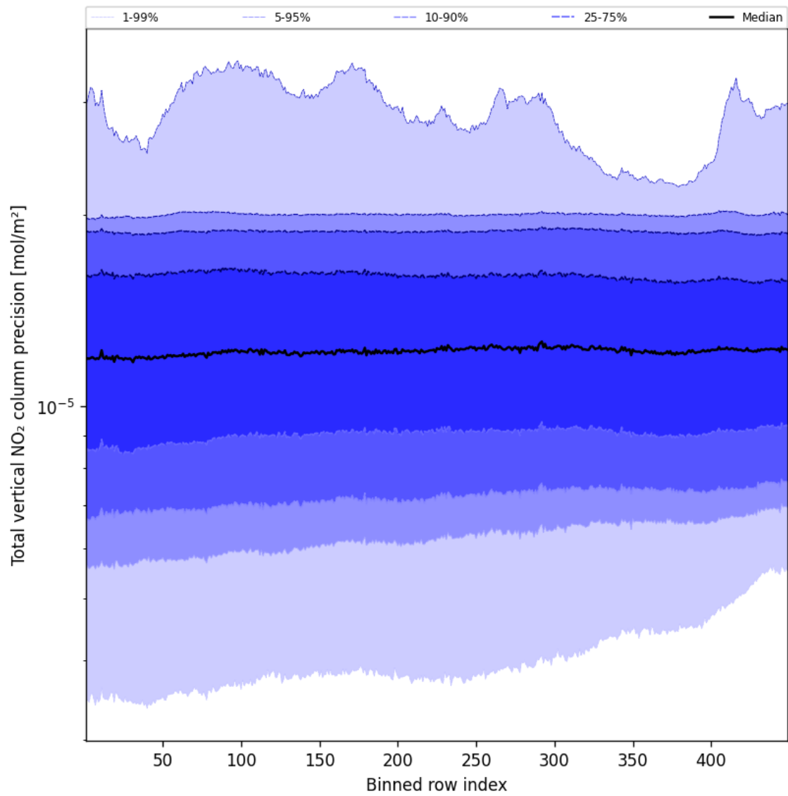
Figure 54: Along track statistics of “Total vertical NO 2 column precision” for 2024-12-08 to 2024-12-09
