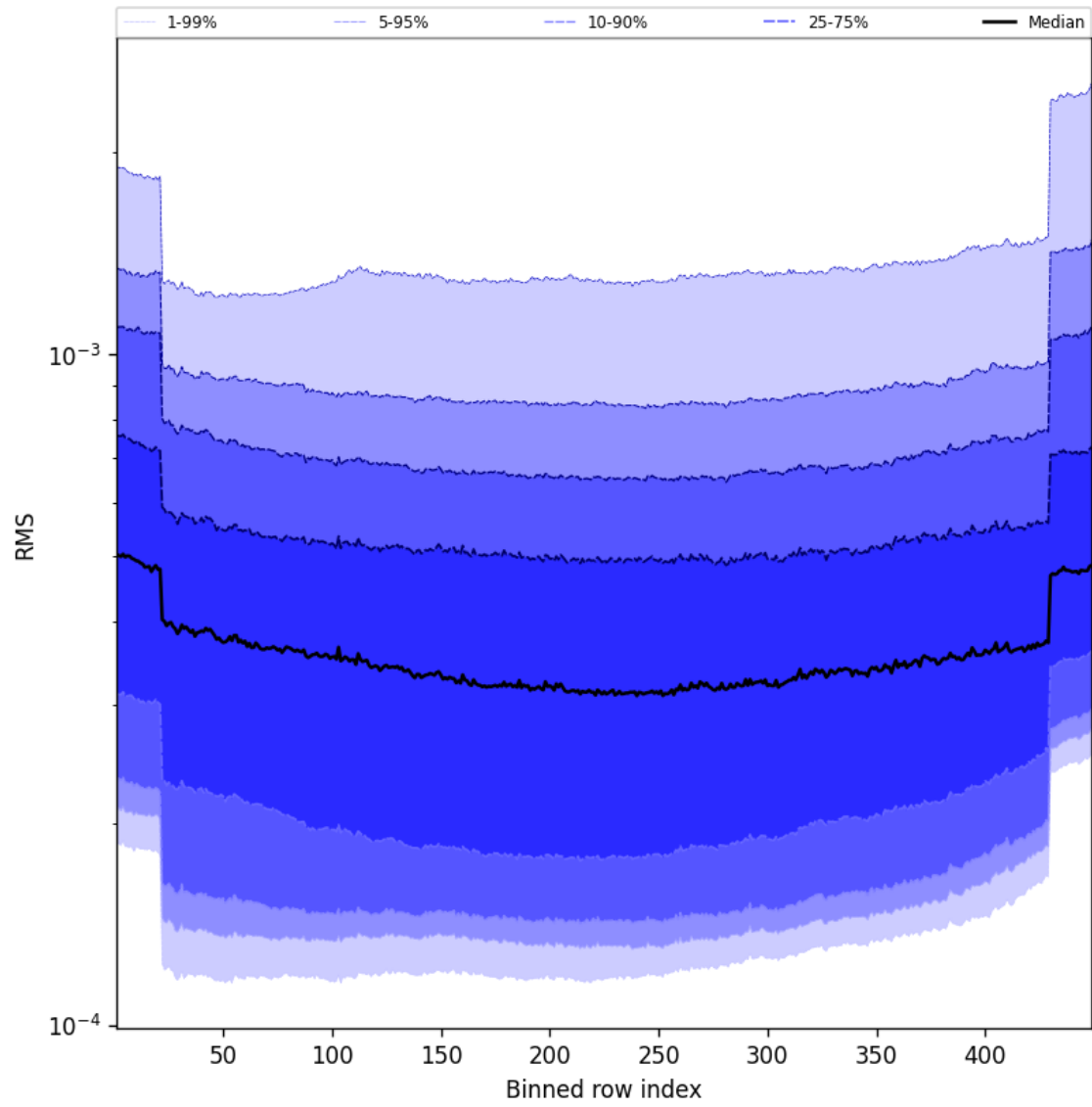
Figure 58: Along track statistics of “RMS” for 2024-12-08 to 2024-12-09
