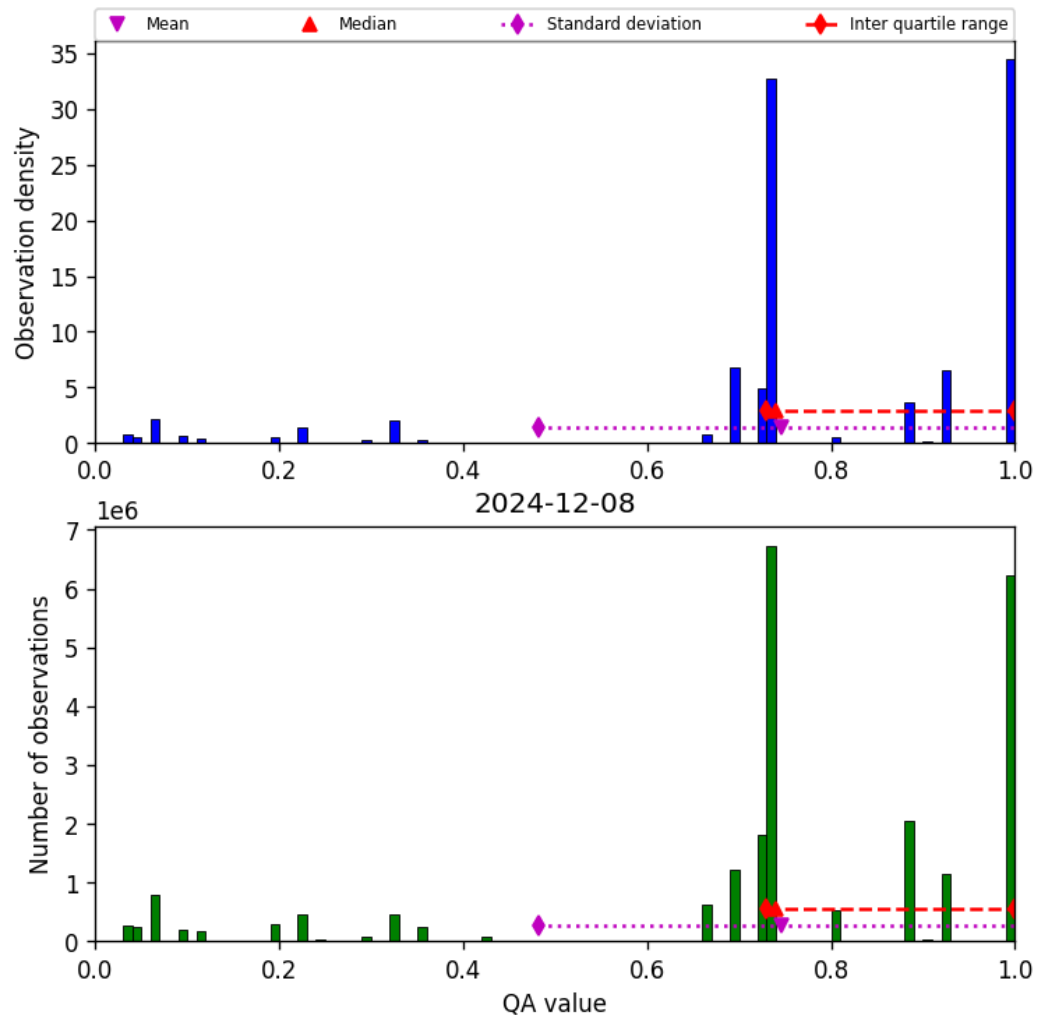
Figure 26: Histogram of “QA value” for 2024-12-08 to 2024-12-09
