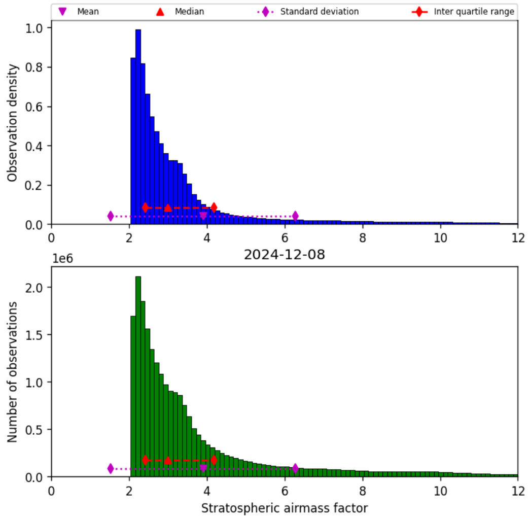
Figure 42: Histogram of “Stratospheric airmass factor” for 2024-12-08 to 2024-12-09
