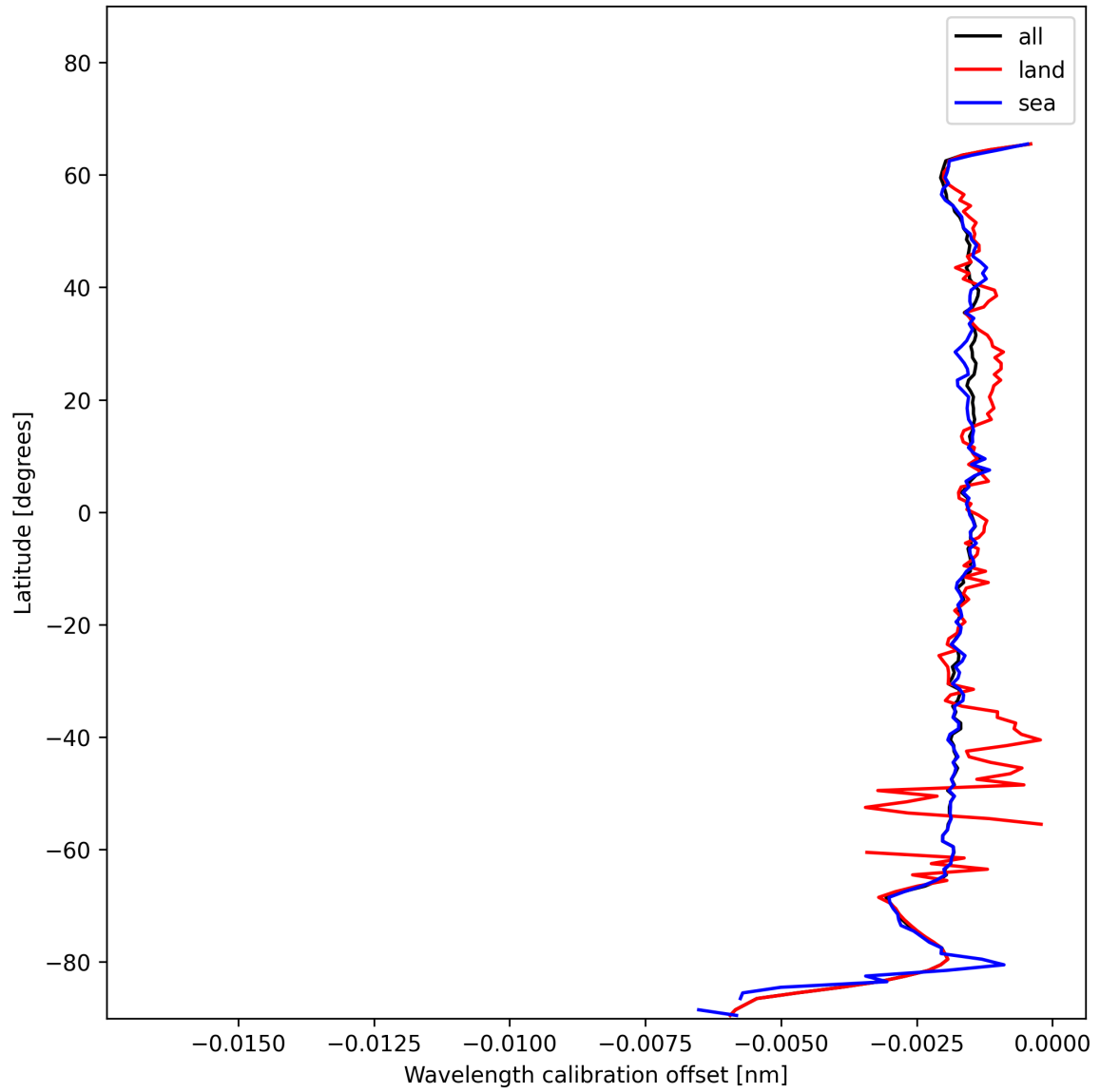
Figure 16: Zonal average of “Wavelength calibration offset” for 2024-12-08 to 2024-12-09.
