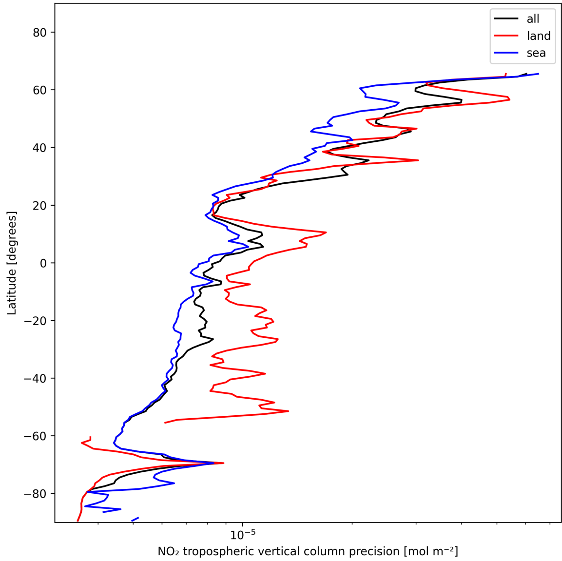
Figure 11: Zonal average of “NO 2 tropospheric vertical column precision” for 2024-12-08 to 2024-12-09.
