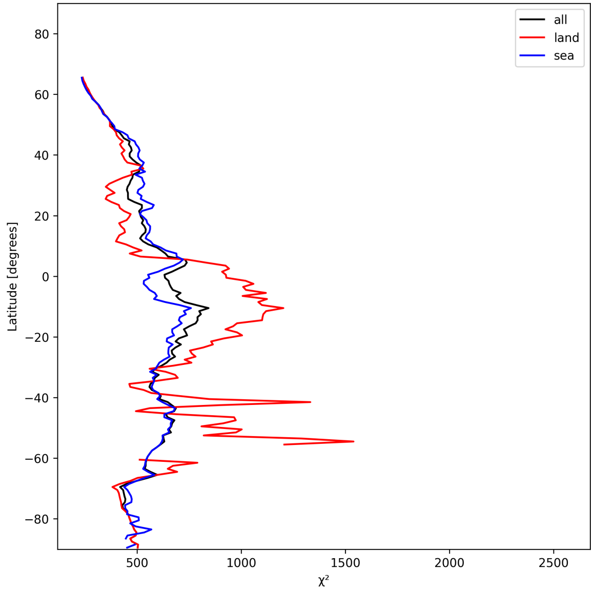
Figure 23: Zonal average of “ \chi^2 ” for 2024-12-08 to 2024-12-09.
