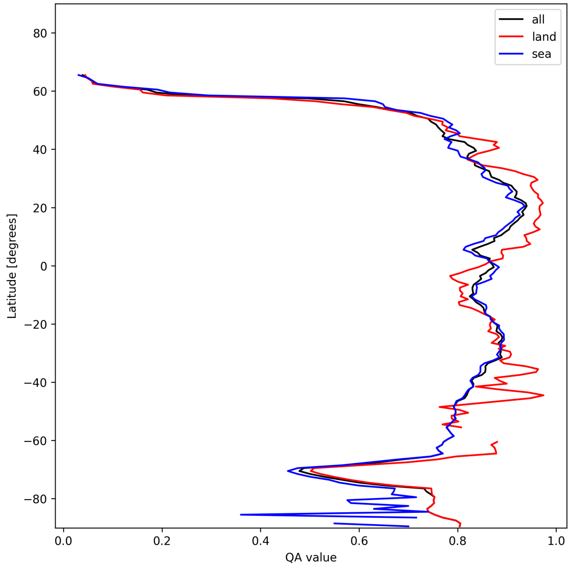
Figure 9: Zonal average of “QA value” for 2024-12-08 to 2024-12-09.
