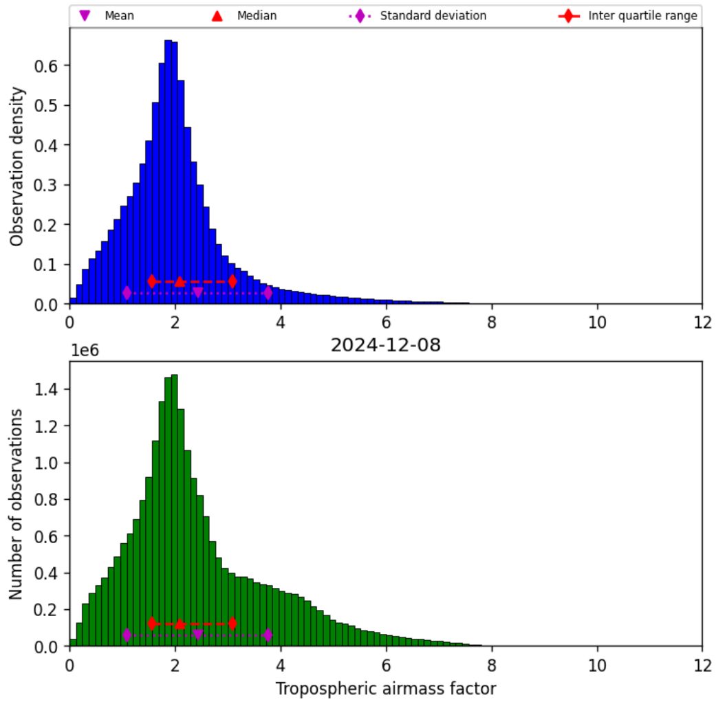
Figure 29: Histogram of “Tropospheric airmass factor” for 2024-12-08 to 2024-12-09
