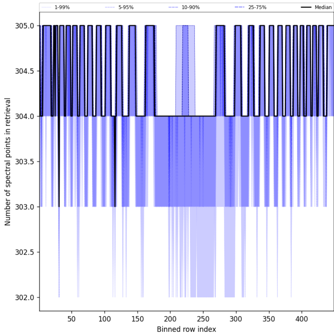
Figure 48: Along track statistics of “Number of spectral points in retrieval” for 2024-12-08 to 2024-12-09
