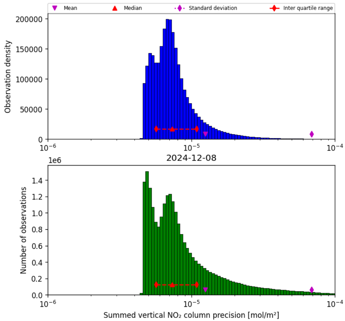
Figure 39: Histogram of “Summed vertical NO 2 column precision” for 2024-12-08 to 2024-12-09
