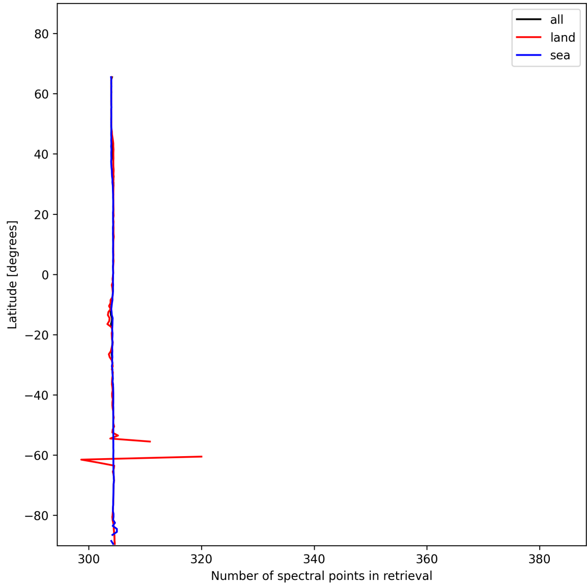
Figure 14: Zonal average of “Number of spectral points in retrieval” for 2024-12-08 to 2024-12-09.
