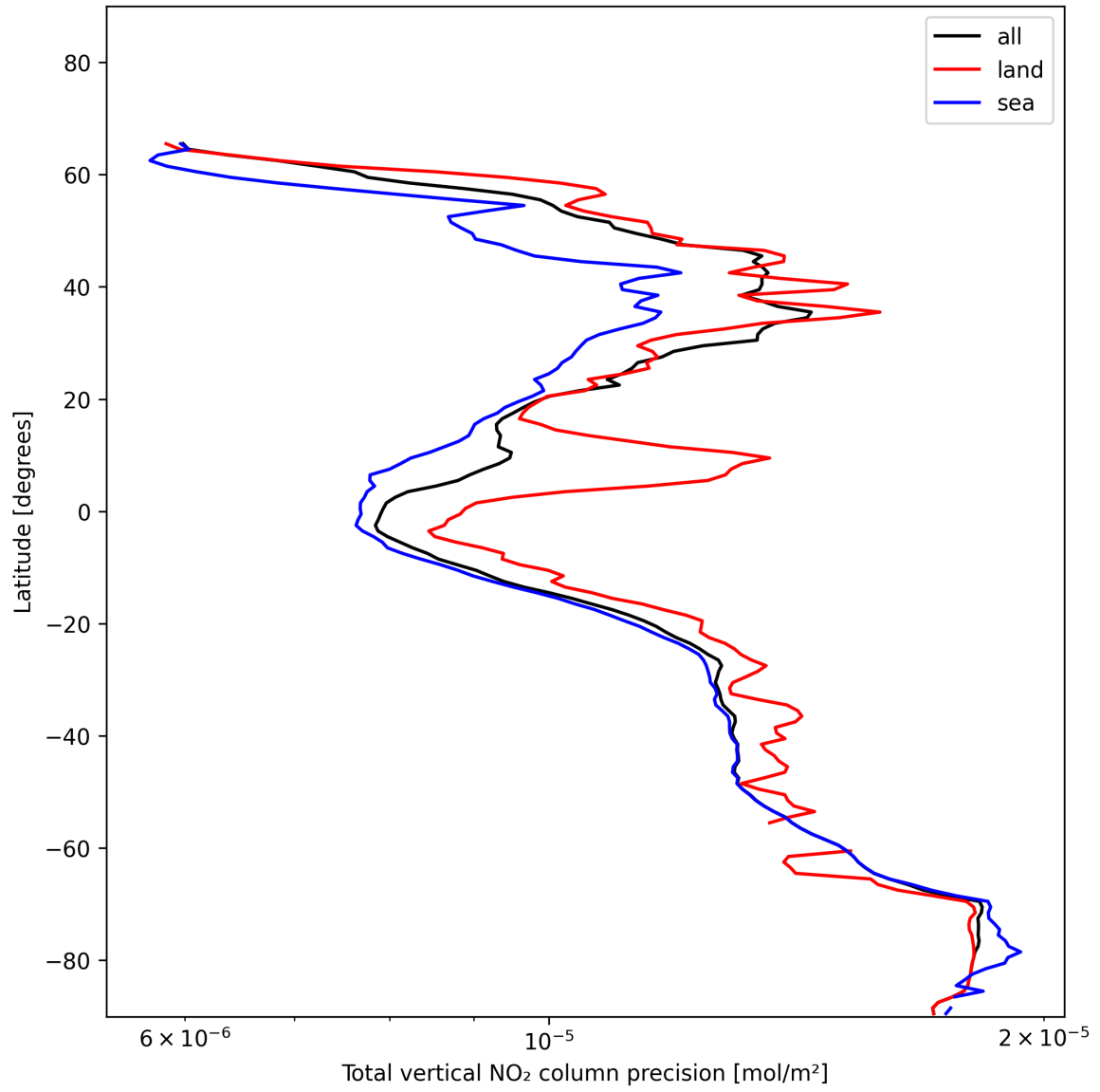
Figure 20: Zonal average of “Total vertical NO 2 column precision” for 2024-12-08 to 2024-12-09.
