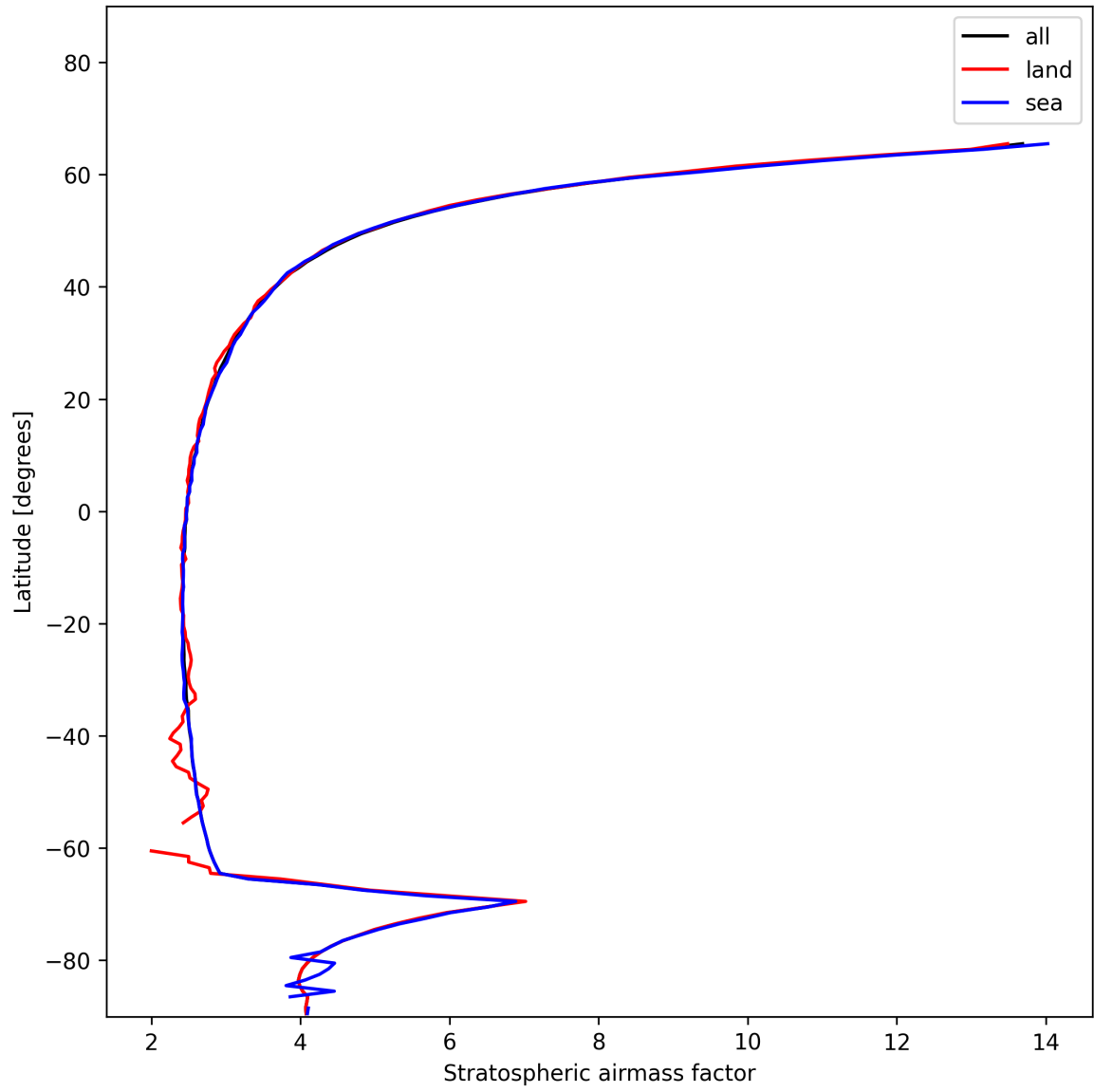
Figure 25: Zonal average of “Stratospheric air mass factor” for 2024-12-08 to 2024-12-09.
