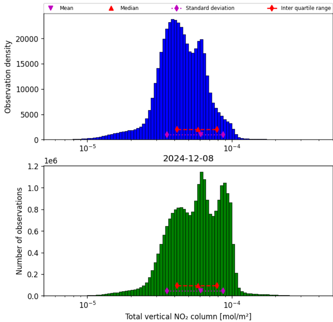
Figure 36: Histogram of “Total vertical NO 2 column” for 2024-12-08 to 2024-12-09
