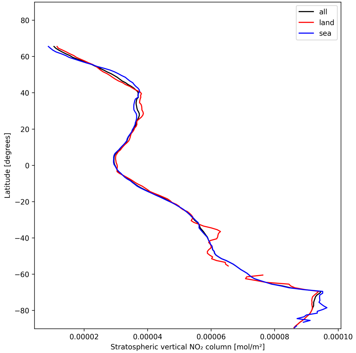
Figure 17: Zonal average of “Stratospheric vertical NO 2 column” for 2024-12-08 to 2024-12-09.
