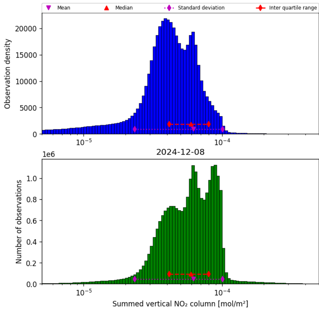
Figure 38: Histogram of “Summed vertical NO 2 column” for 2024-12-08 to 2024-12-09
