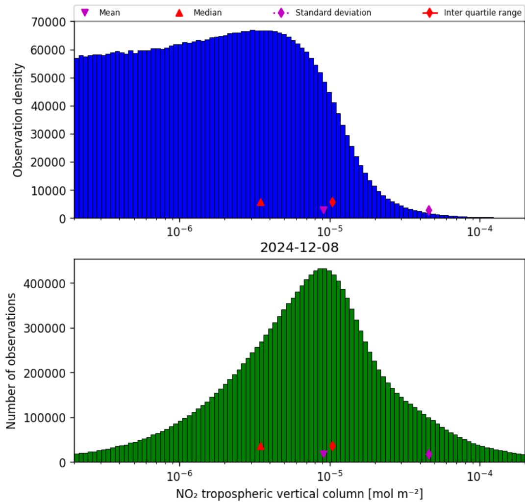
Figure 27: Histogram of “NO 2 tropospheric vertical column” for 2024-12-08 to 2024-12-09
