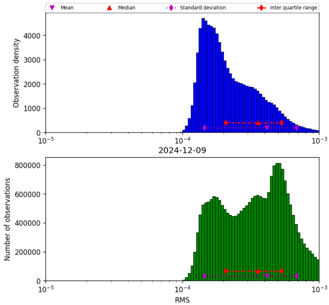
Figure 41: Histogram of “RMS” for 2024-12-09 to 2024-12-09
