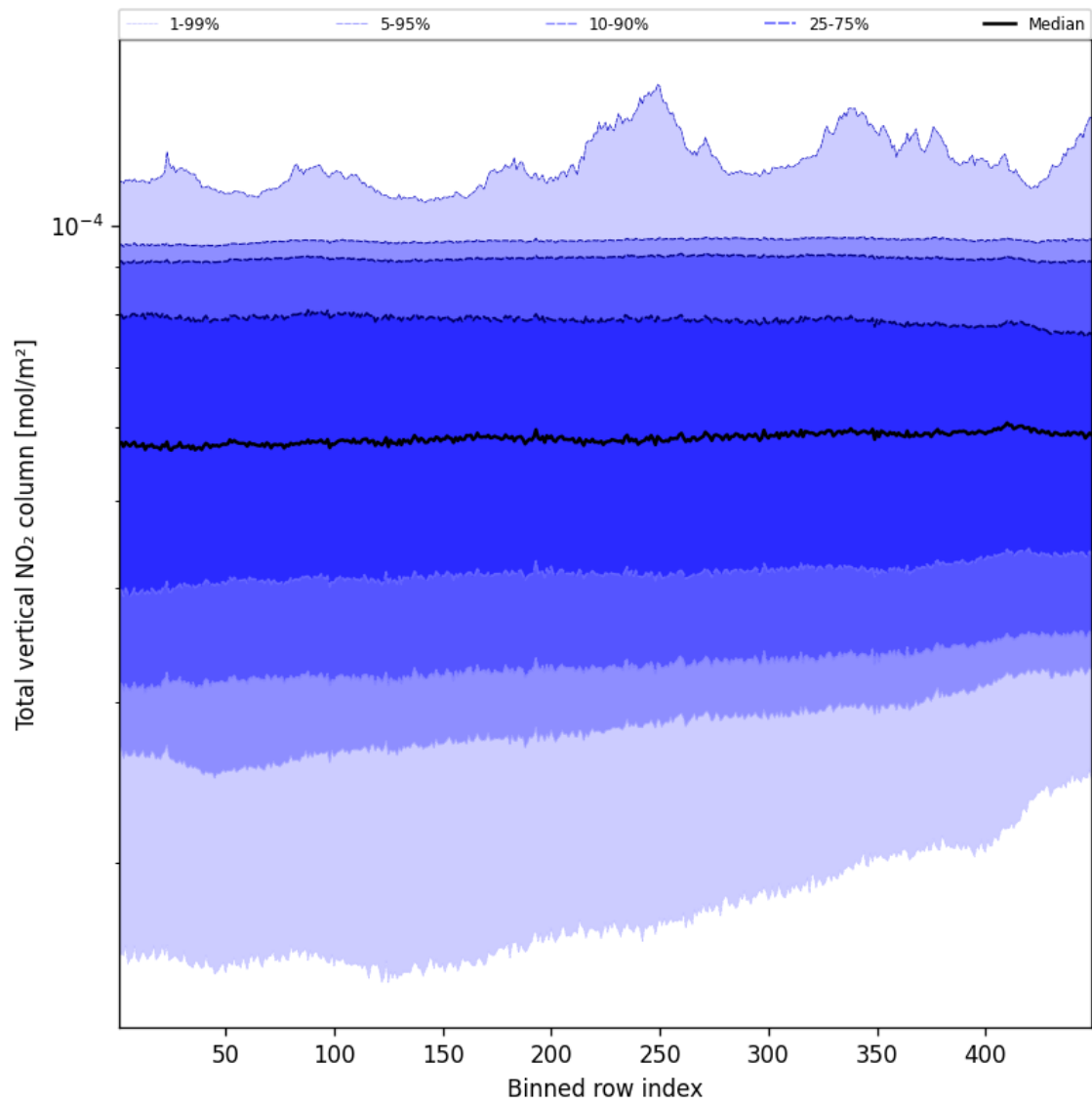
Figure 53: Along track statistics of “Total vertical NO 2 column” for 2024-12-09 to 2024-12-09
