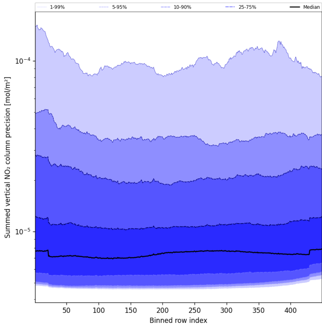
Figure 56: Along track statistics of “Summed vertical NO 2 column precision” for 2024-12-09 to 2024-12-09
