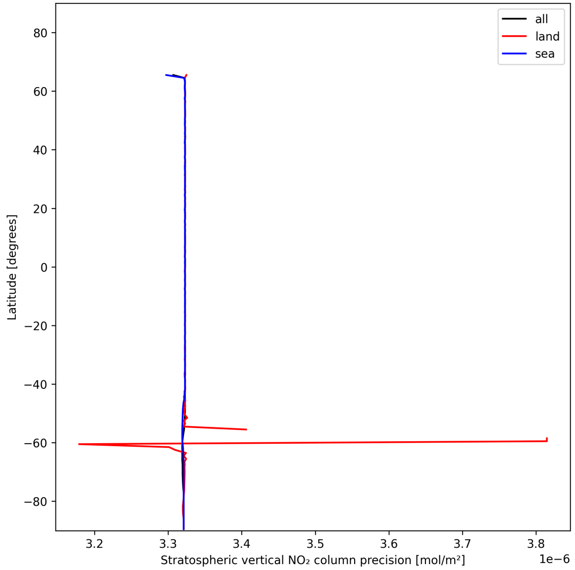
Figure 18: Zonal average of “Stratospheric vertical NO 2 column precision” for 2024-12-09 to 2024-12-09.
