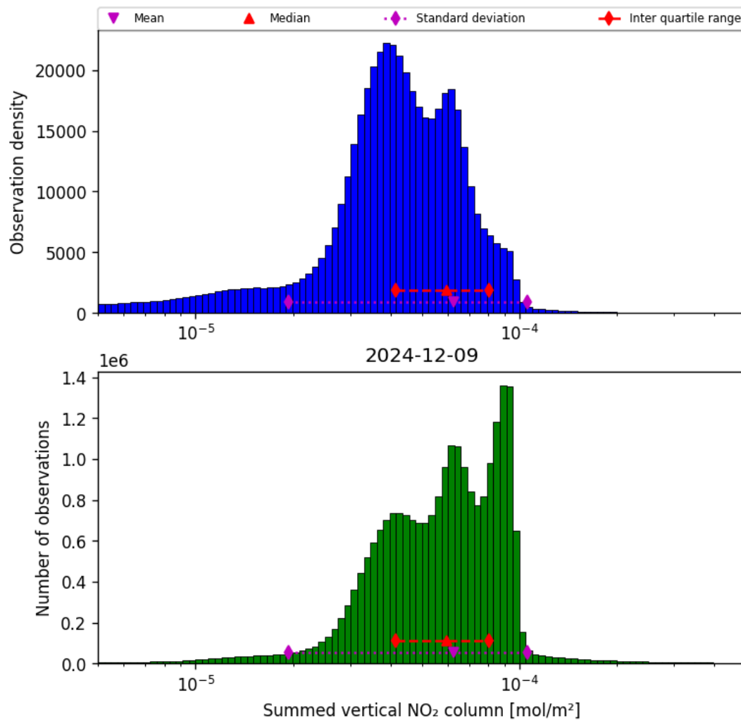
Figure 38: Histogram of “Summed vertical NO 2 column” for 2024-12-09 to 2024-12-09
