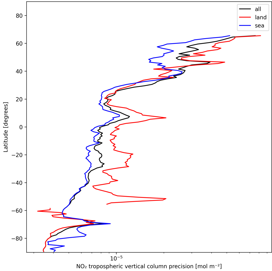
Figure 11: Zonal average of “NO 2 tropospheric vertical column precision” for 2024-12-09 to 2024-12-09.
