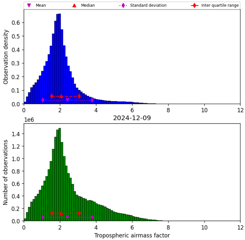
Figure 29: Histogram of “Tropospheric airmass factor” for 2024-12-09 to 2024-12-09
