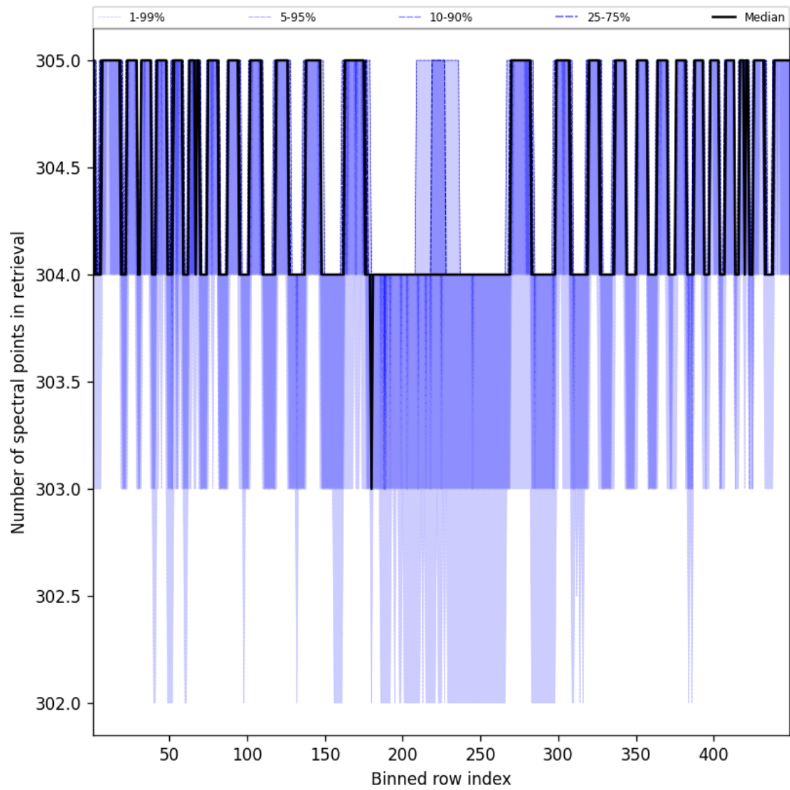
Figure 48: Along track statistics of “Number of spectral points in retrieval” for 2024-12-09 to 2024-12-09
