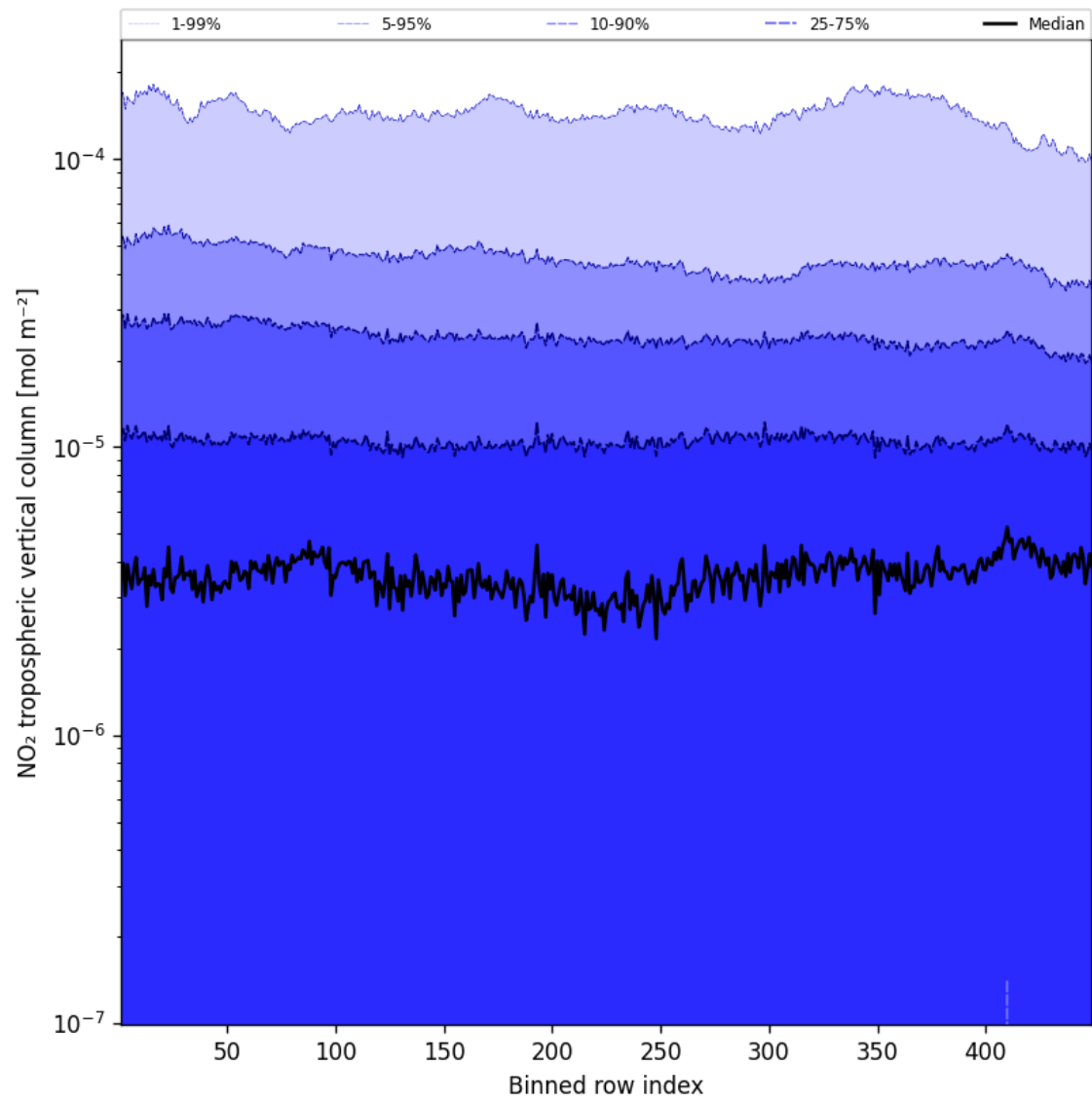
Figure 44: Along track statistics of “NO 2 tropospheric vertical column” for 2024-12-09 to 2024-12-09
