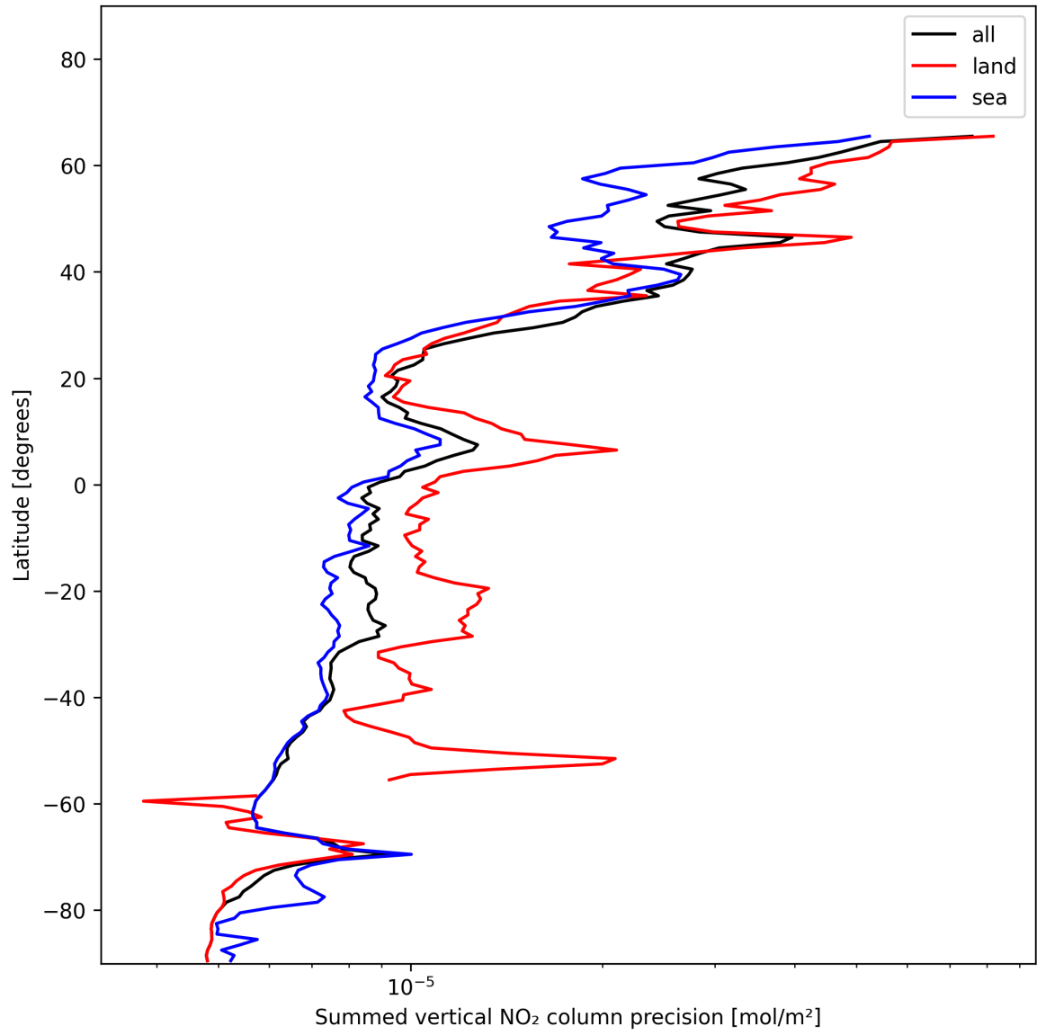
Figure 22: Zonal average of “Summed vertical NO 2 column precision” for 2024-12-09 to 2024-12-09.
