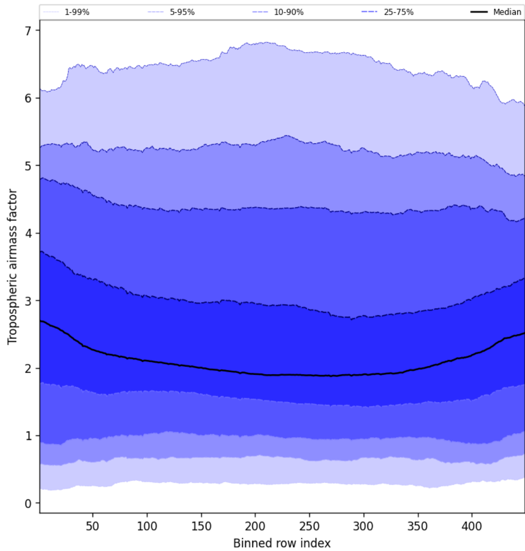
Figure 46: Along track statistics of “Tropospheric airmass factor” for 2024-12-09 to 2024-12-09
