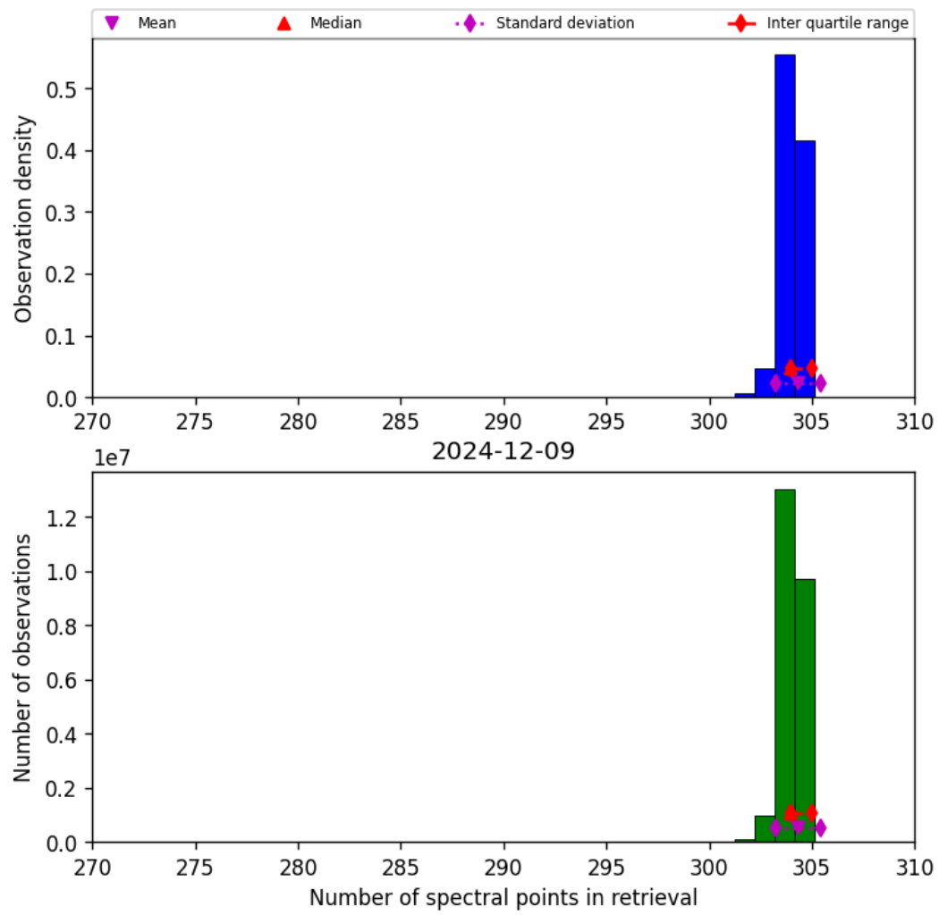
Figure 31: Histogram of “Number of spectral points in retrieval” for 2024-12-09 to 2024-12-09
