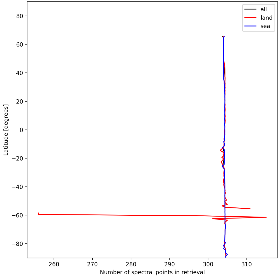
Figure 14: Zonal average of “Number of spectral points in retrieval” for 2024-12-09 to 2024-12-09.
