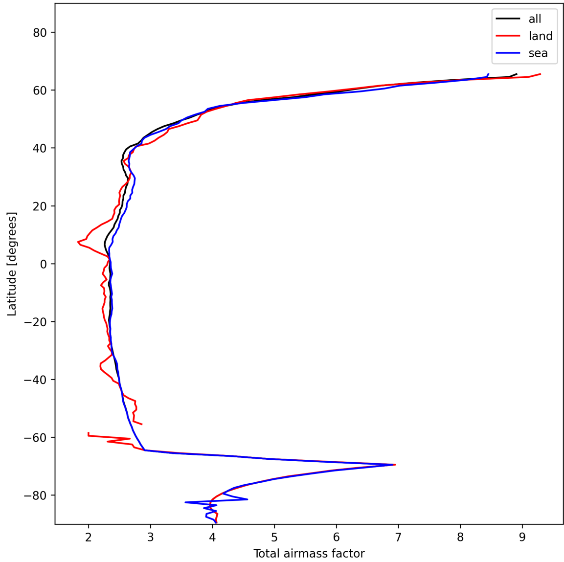
Figure 13: Zonal average of “Total airmass factor” for 2024-12-09 to 2024-12-09.
