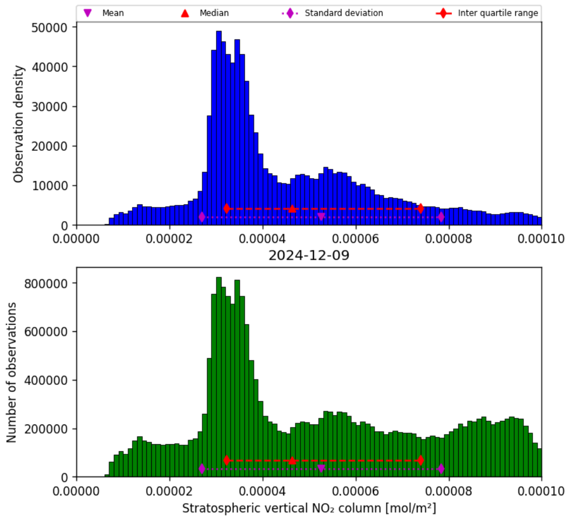
Figure 34: Histogram of “Stratospheric vertical NO 2 column” for 2024-12-09 to 2024-12-09
