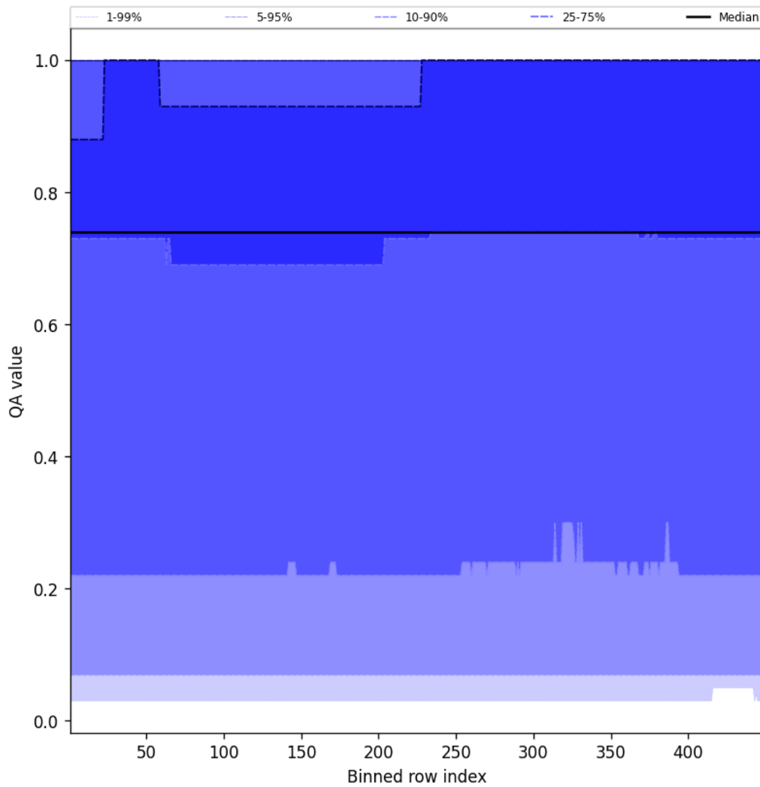
Figure 43: Along track statistics of “QA value” for 2024-12-09 to 2024-12-09
