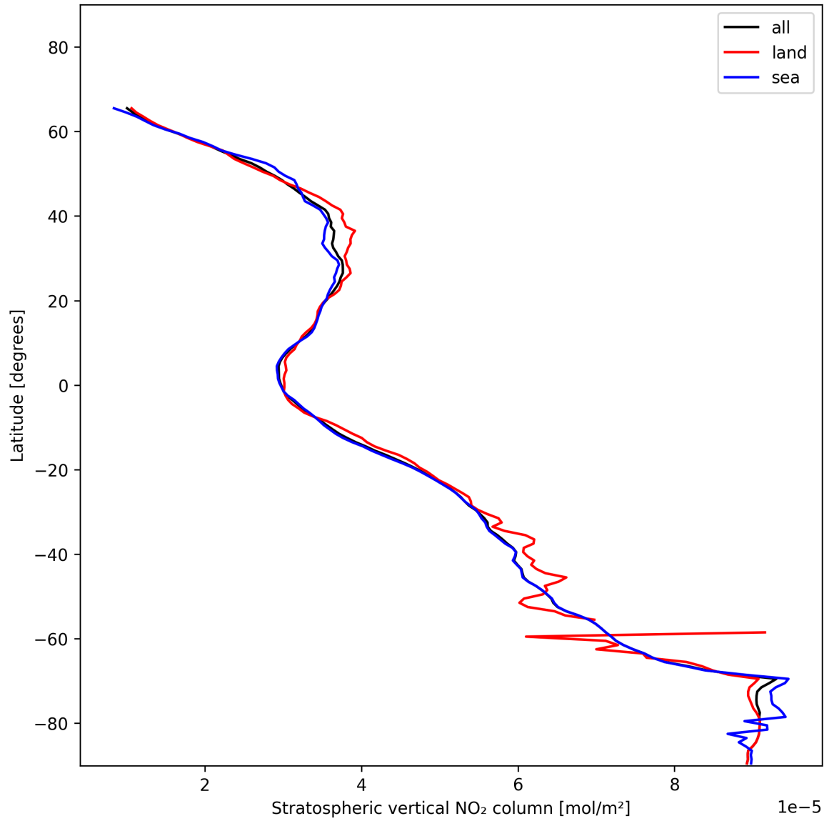
Figure 17: Zonal average of “Stratospheric vertical NO 2 column” for 2024-12-09 to 2024-12-09.
