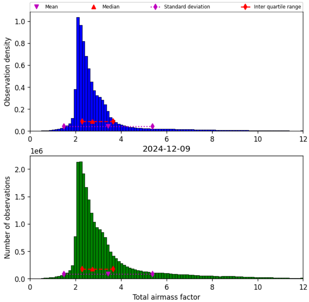
Figure 30: Histogram of “Total airmass factor” for 2024-12-09 to 2024-12-09
