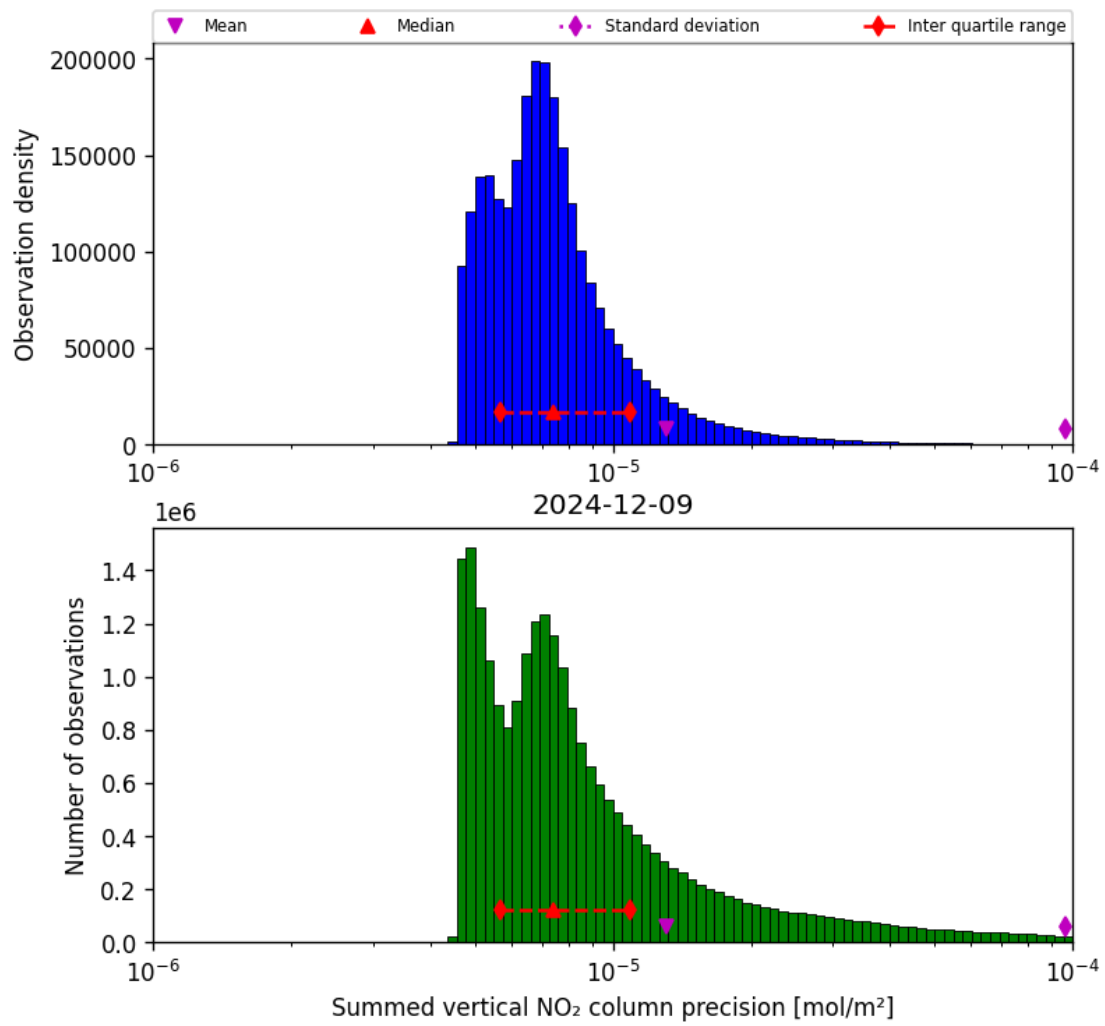
Figure 39: Histogram of "Summed vertical NO 2 column precision" for 2024-12-09 to 2024-12-09
