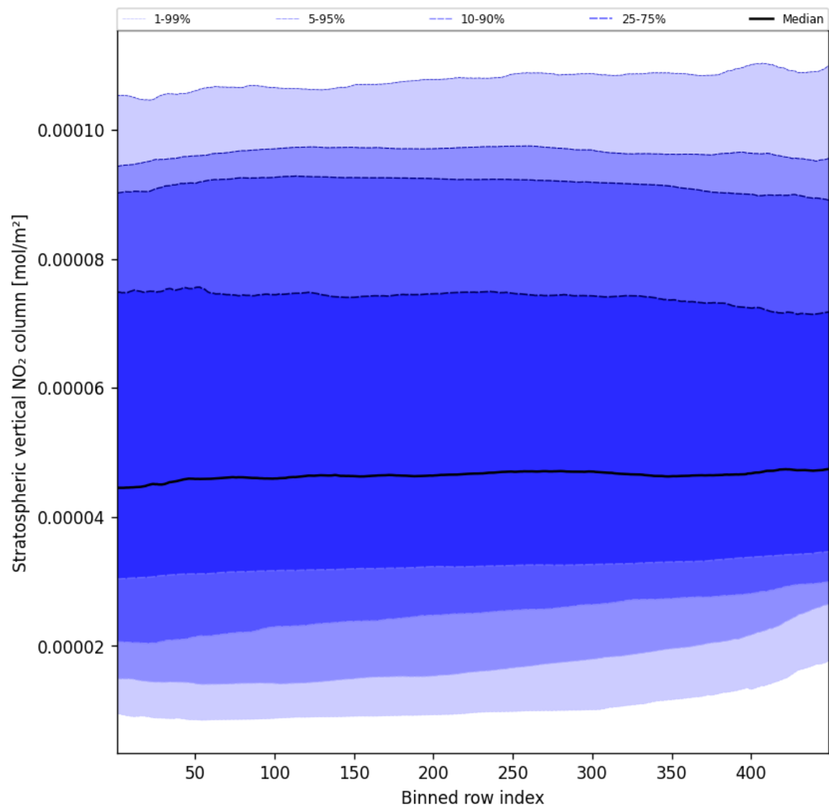
Figure 51: Along track statistics of “Stratospheric vertical NO 2 column” for 2024-12-09 to 2024-12-09
