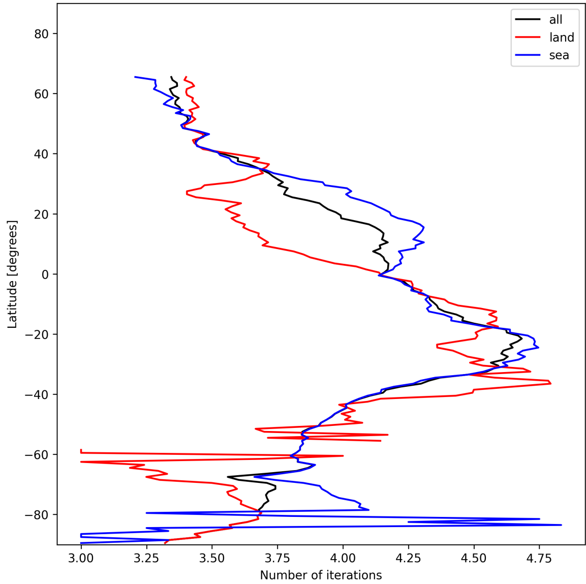
Figure 15: Zonal average of “Number of iterations” for 2024-12-09 to 2024-12-09.
