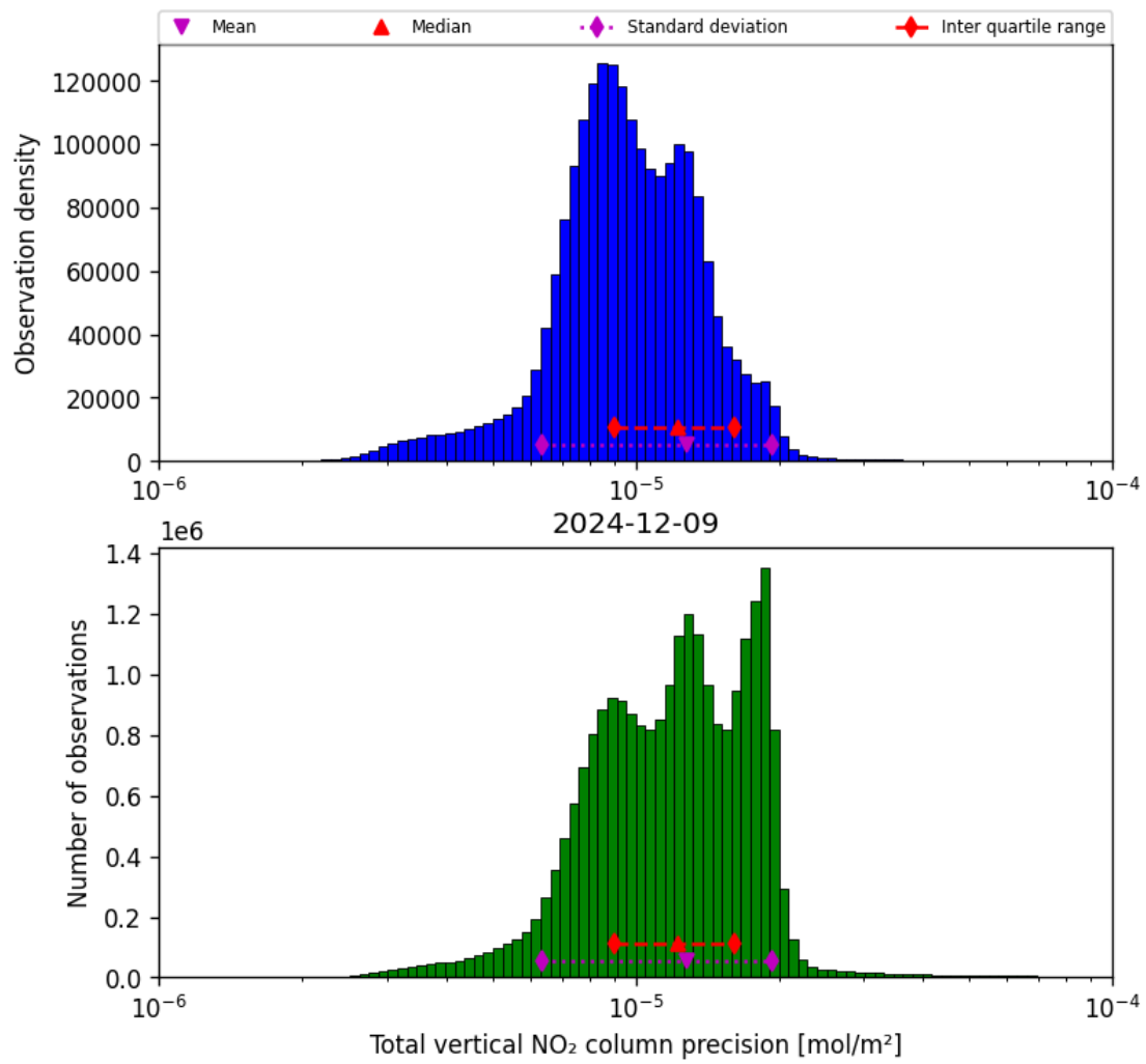
Figure 37: Histogram of "Total vertical NO 2 column precision" for 2024-12-09 to 2024-12-09
