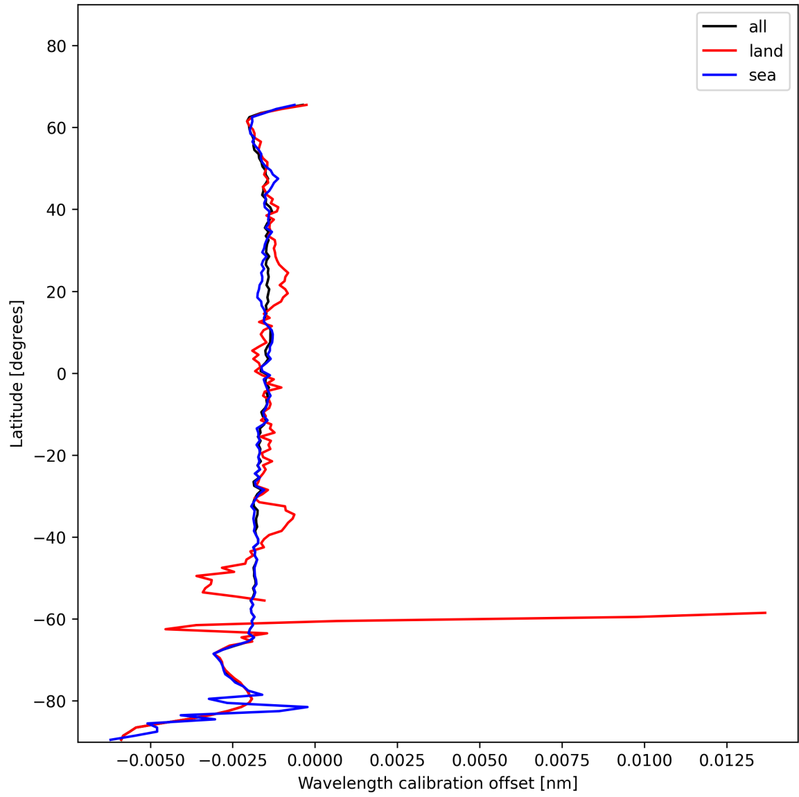
Figure 16: Zonal average of “Wavelength calibration offset” for 2024-12-09 to 2024-12-09.
