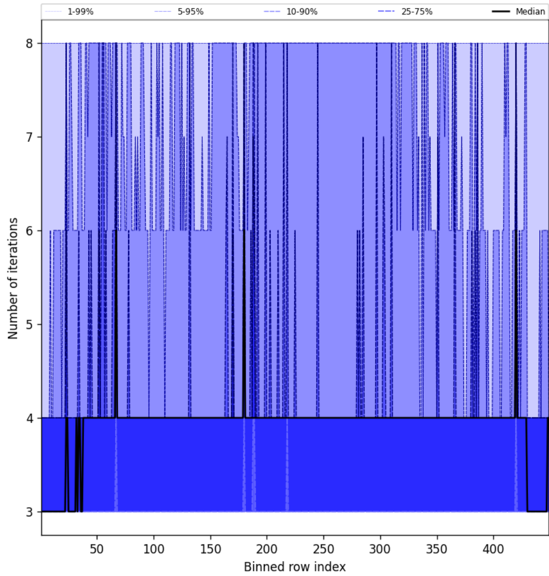
Figure 49: Along track statistics of “Number of iterations” for 2024-12-09 to 2024-12-09
