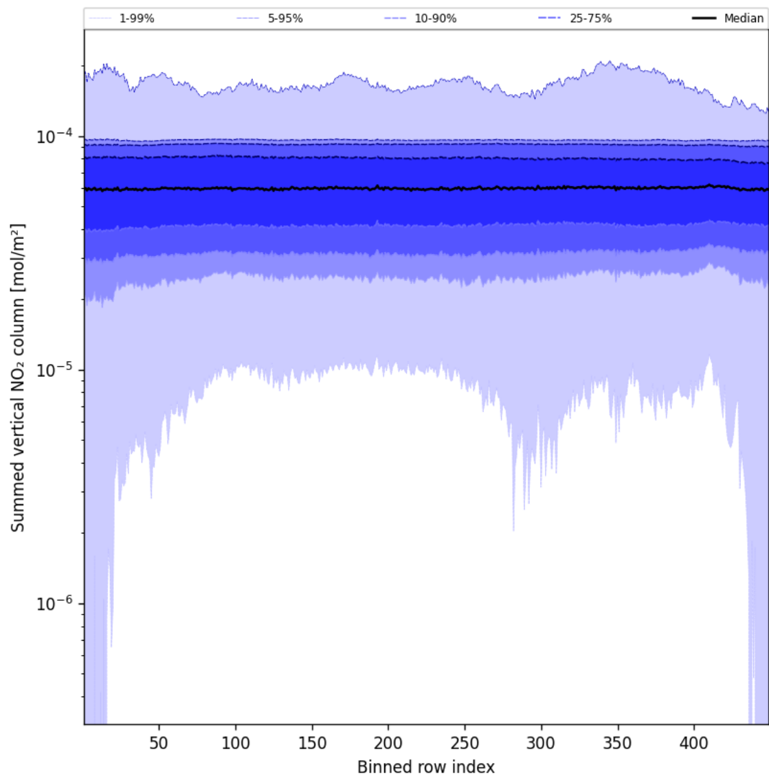
Figure 55: Along track statistics of “Summed vertical NO 2 column” for 2024-12-09 to 2024-12-09
