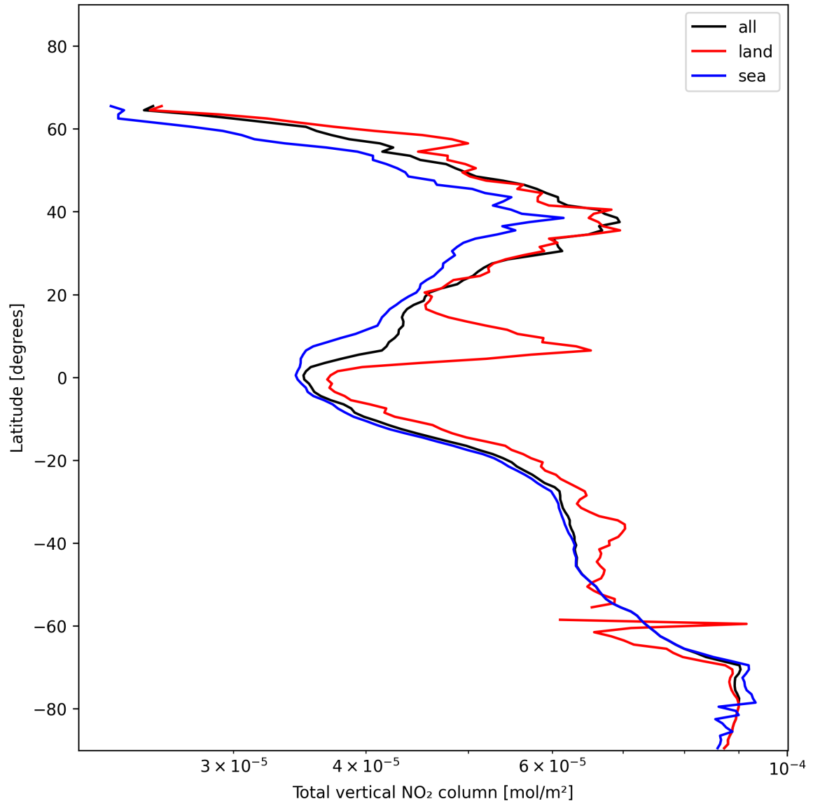
Figure 19: Zonal average of “Total vertical NO 2 column” for 2024-12-09 to 2024-12-09.
