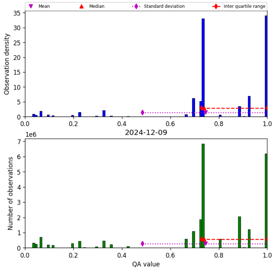
Figure 26: Histogram of “QA value” for 2024-12-09 to 2024-12-09
