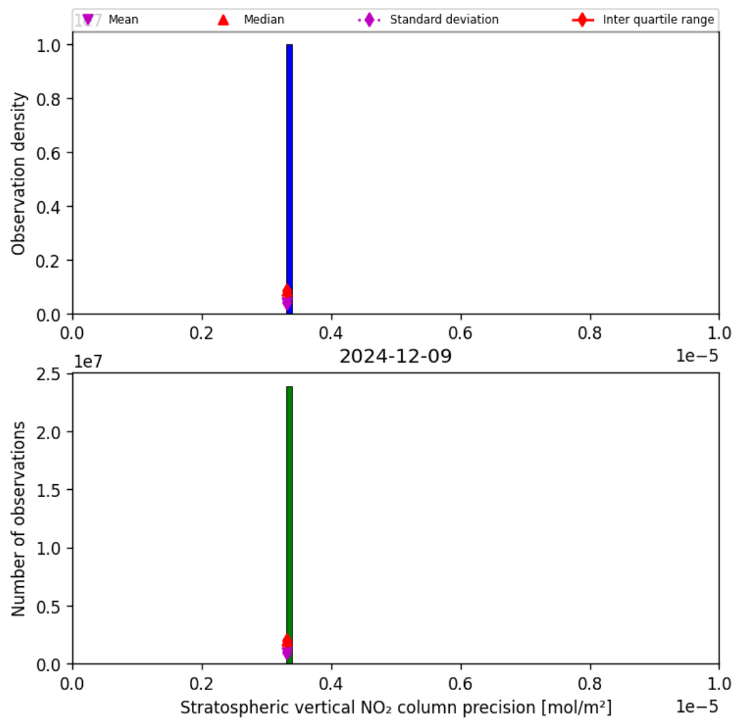
Figure 35: Histogram of “Stratospheric vertical NO 2 column precision” for 2024-12-09 to 2024-12-09
