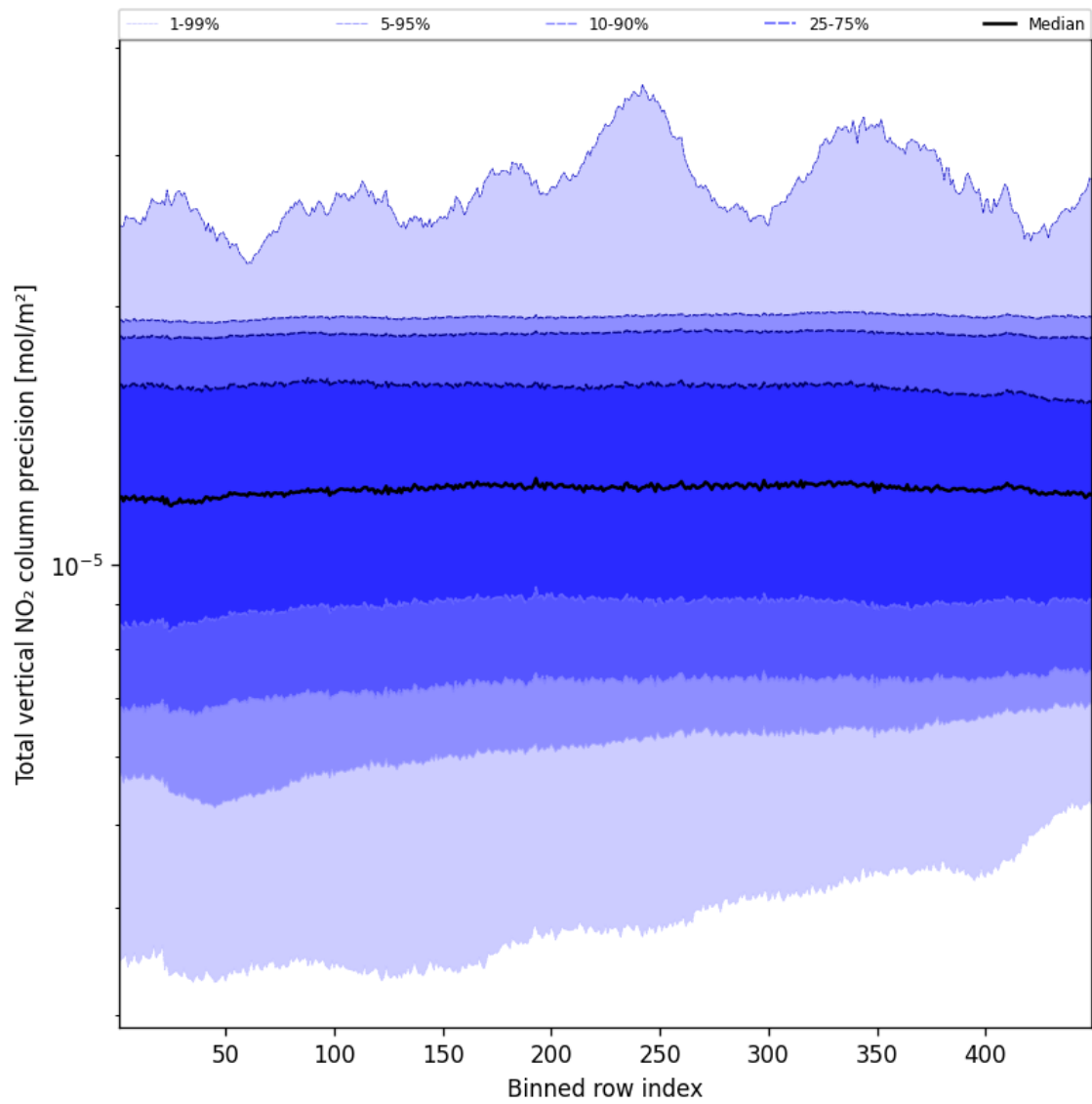
Figure 54: Along track statistics of “Total vertical NO 2 column precision” for 2024-12-09 to 2024-12-09
