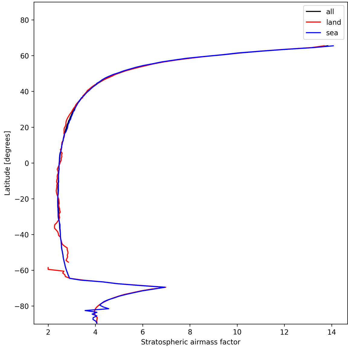
Figure 25: Zonal average of “Stratospheric airmass factor” for 2024-12-09 to 2024-12-09.
