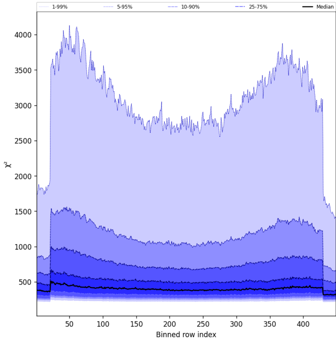
Figure 57: Along track statistics of “ \chi^2 ” for 2024-12-09 to 2024-12-09
