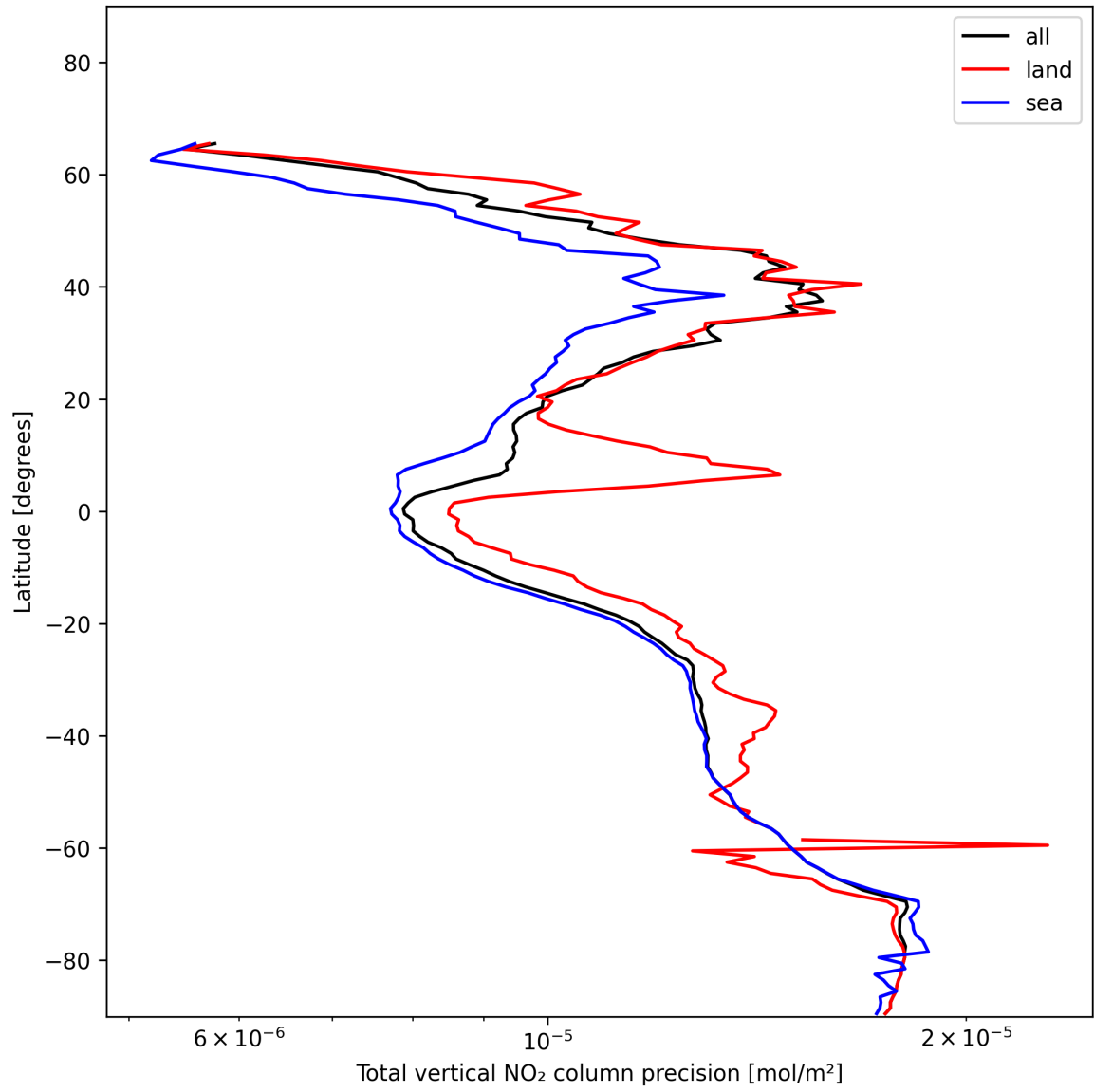
Figure 20: Zonal average of “Total vertical NO 2 column precision” for 2024-12-09 to 2024-12-09.
