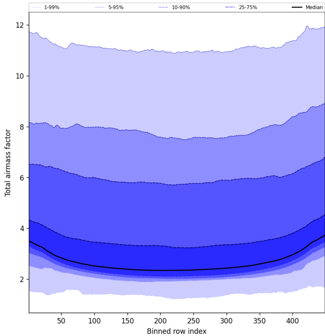
Figure 47: Along track statistics of “Total airmass factor” for 2024-12-09 to 2024-12-09
