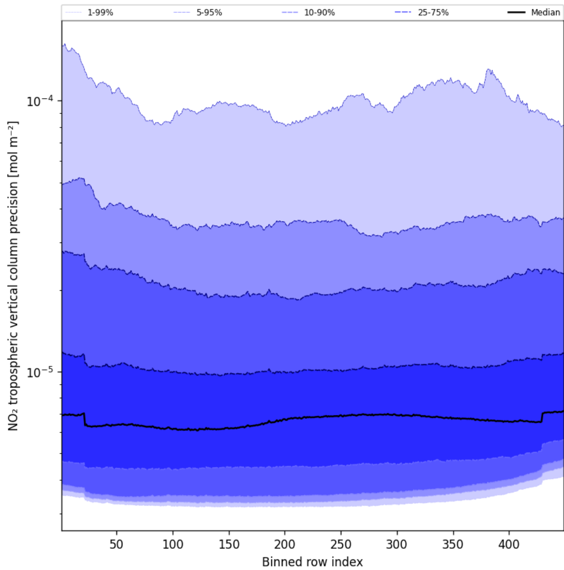
Figure 45: Along track statistics of “NO 2 tropospheric vertical column precision” for 2024-12-09 to 2024-12-09
