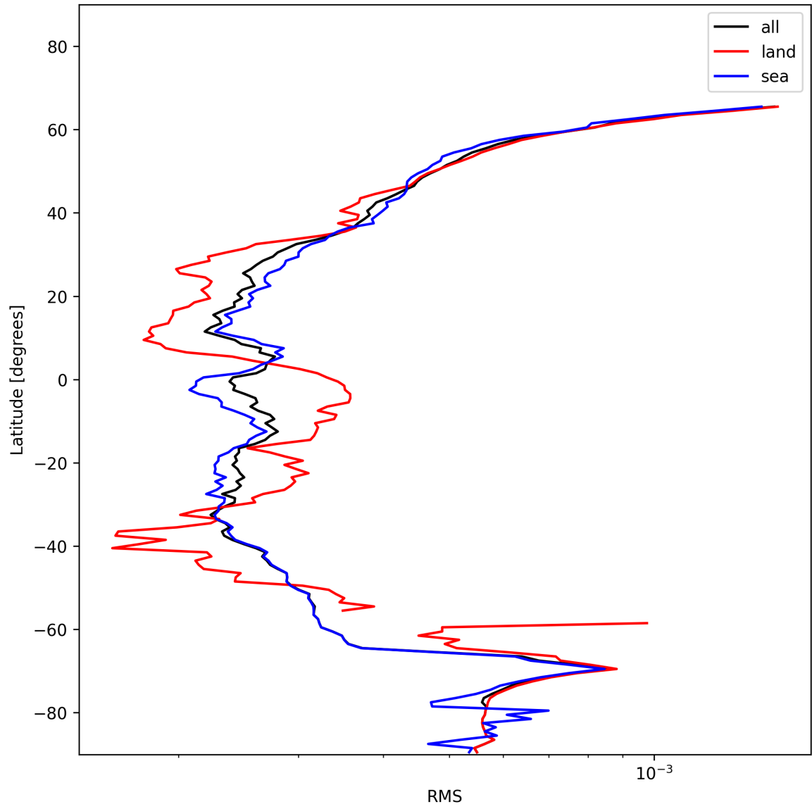
Figure 24: Zonal average of “RMS” for 2024-12-09 to 2024-12-09.
