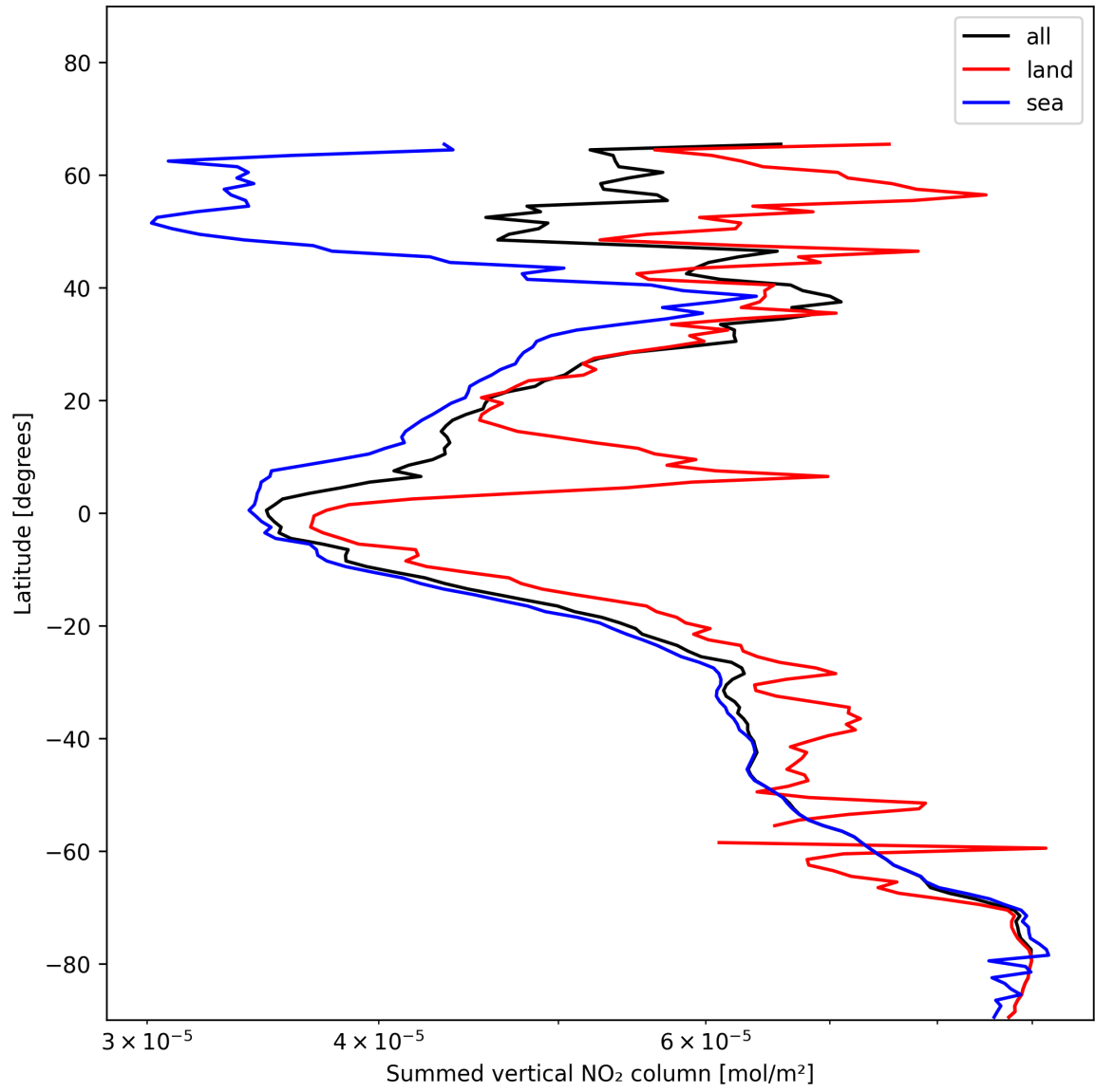
Figure 21: Zonal average of “Summed vertical NO 2 column” for 2024-12-09 to 2024-12-09.
