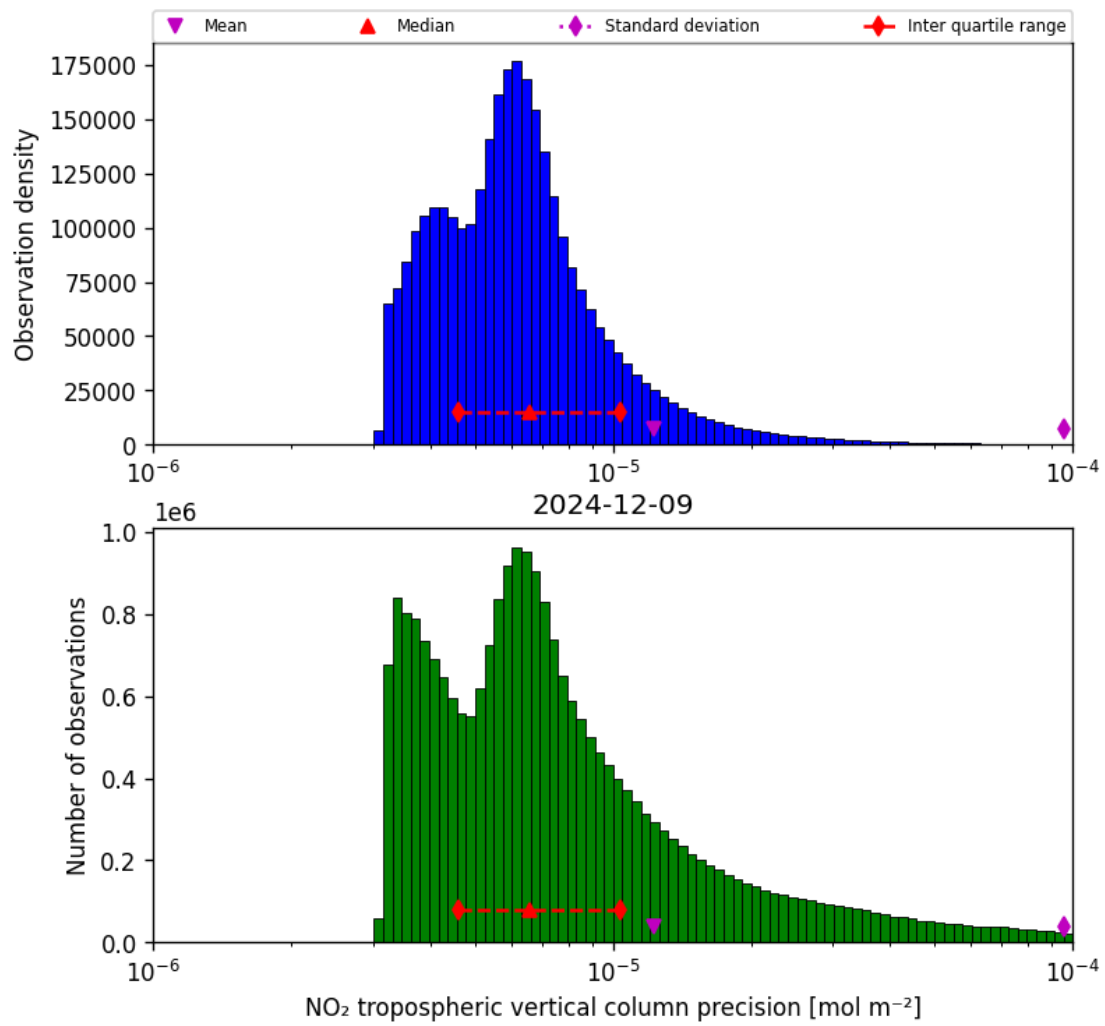
Figure 28: Histogram of "NO 2 tropospheric vertical column precision" for 2024-12-09 to 2024-12-09
