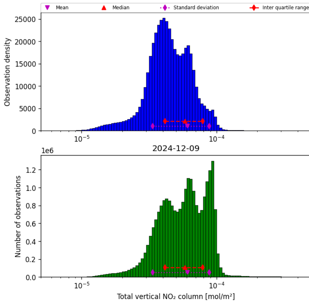
Figure 36: Histogram of “Total vertical NO 2 column” for 2024-12-09 to 2024-12-09
