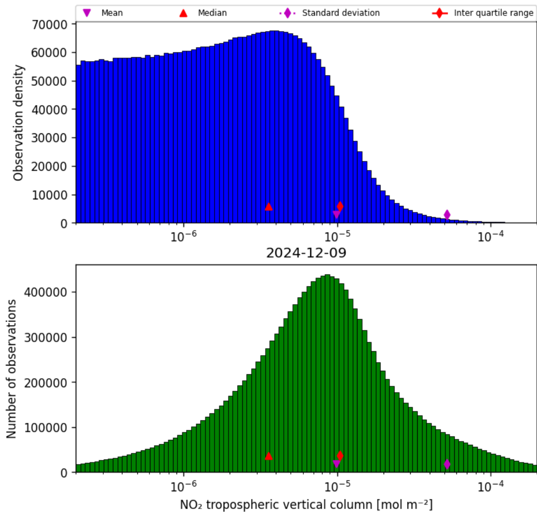
Figure 27: Histogram of “NO 2 tropospheric vertical column” for 2024-12-09 to 2024-12-09
