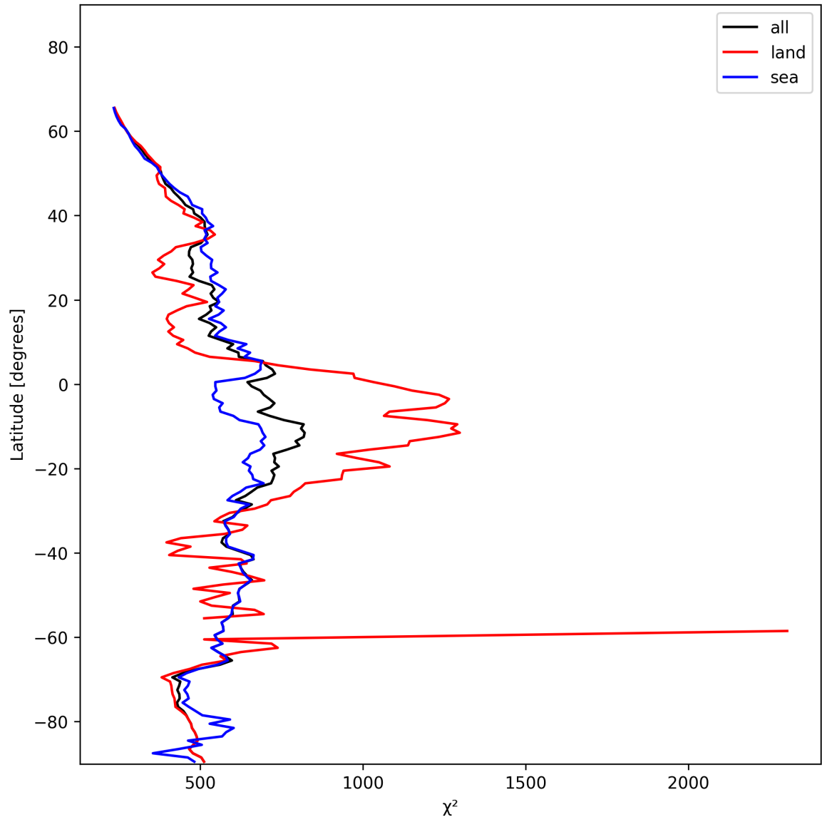
Figure 23: Zonal average of “ \chi^2 ” for 2024-12-09 to 2024-12-09.
