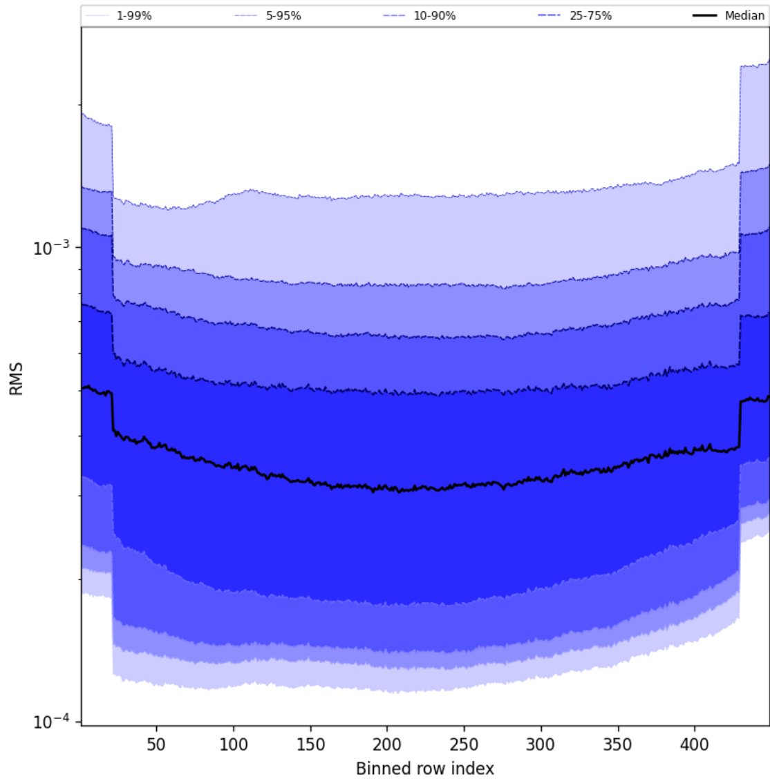
Figure 58: Along track statistics of “RMS” for 2024-12-09 to 2024-12-09
