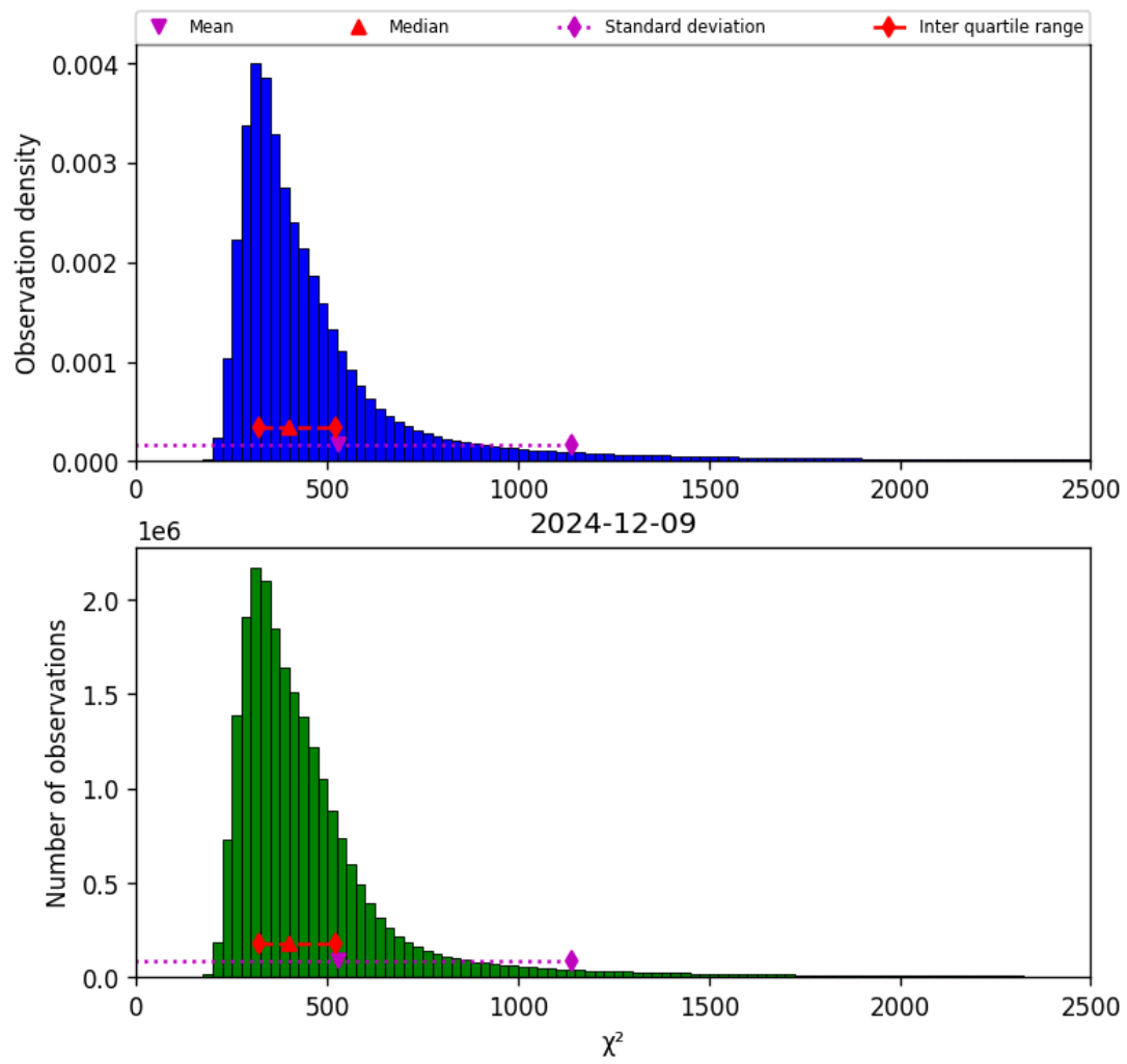
Figure 40: Histogram of “ \chi^2 ” for 2024-12-09 to 2024-12-09
