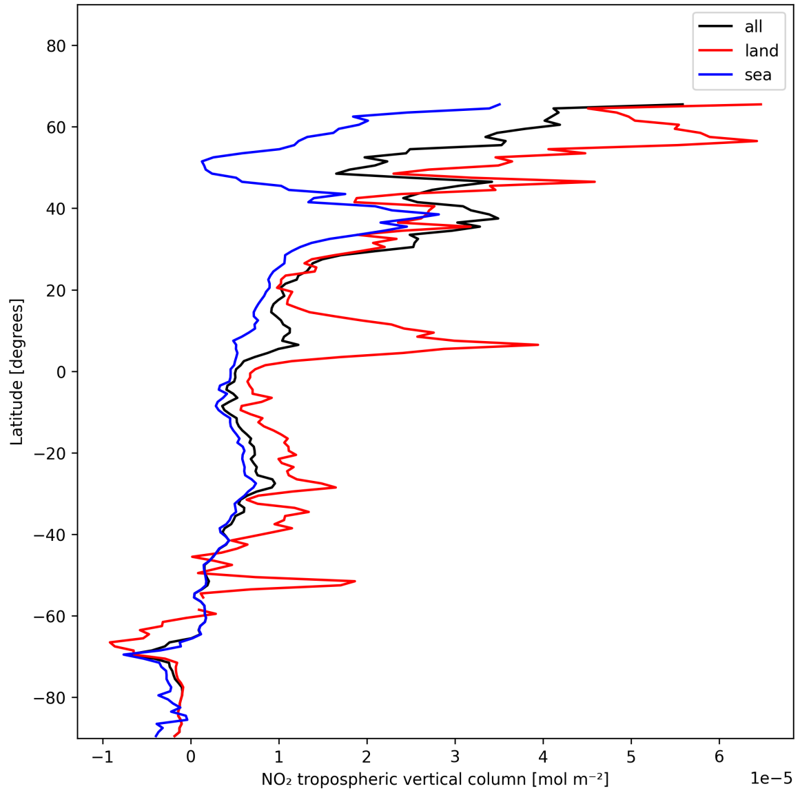
Figure 10: Zonal average of “NO 2 tropospheric vertical column” for 2024-12-09 to 2024-12-09.
