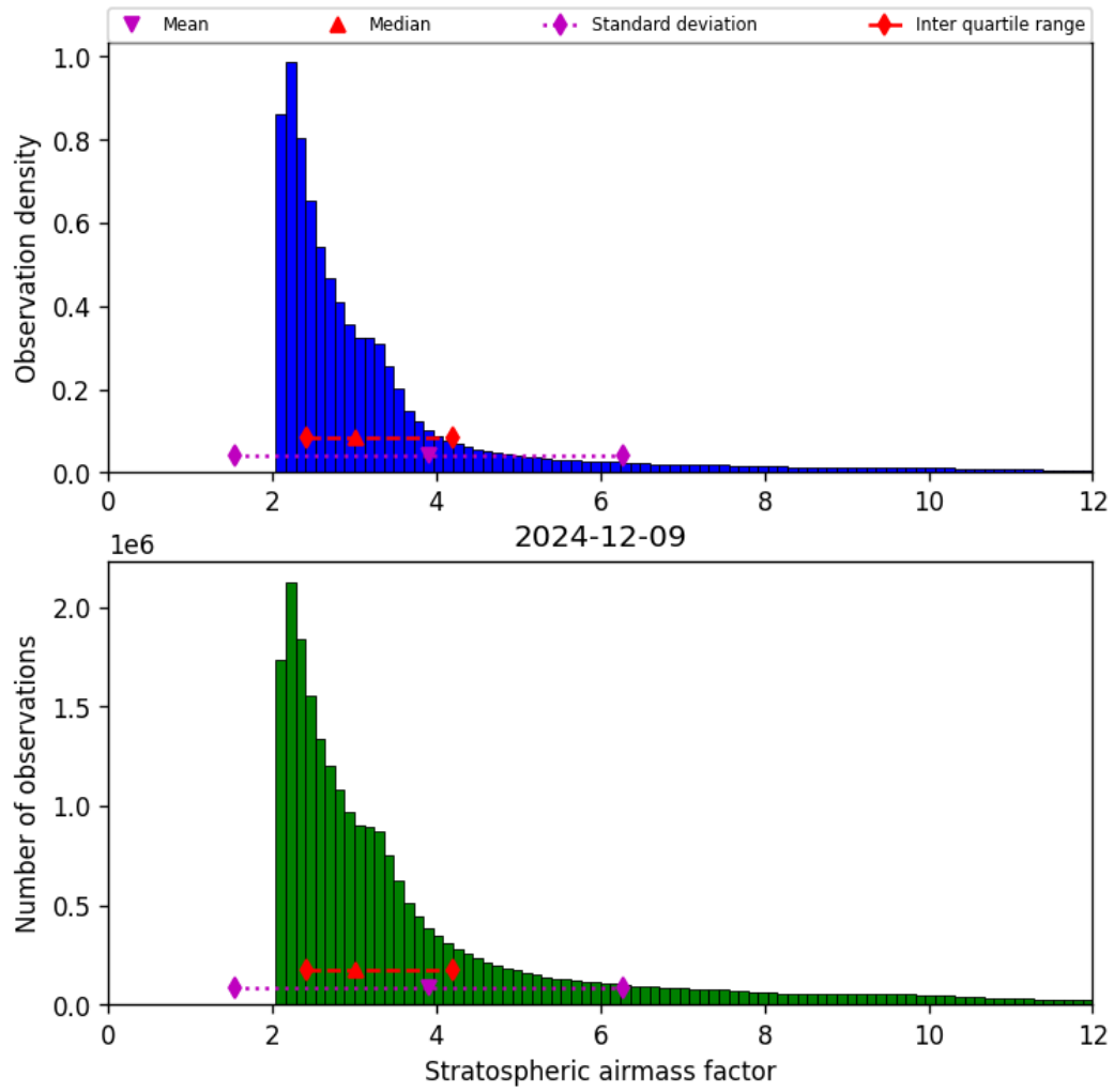
Figure 42: Histogram of “Stratospheric airmass factor” for 2024-12-09 to 2024-12-09
