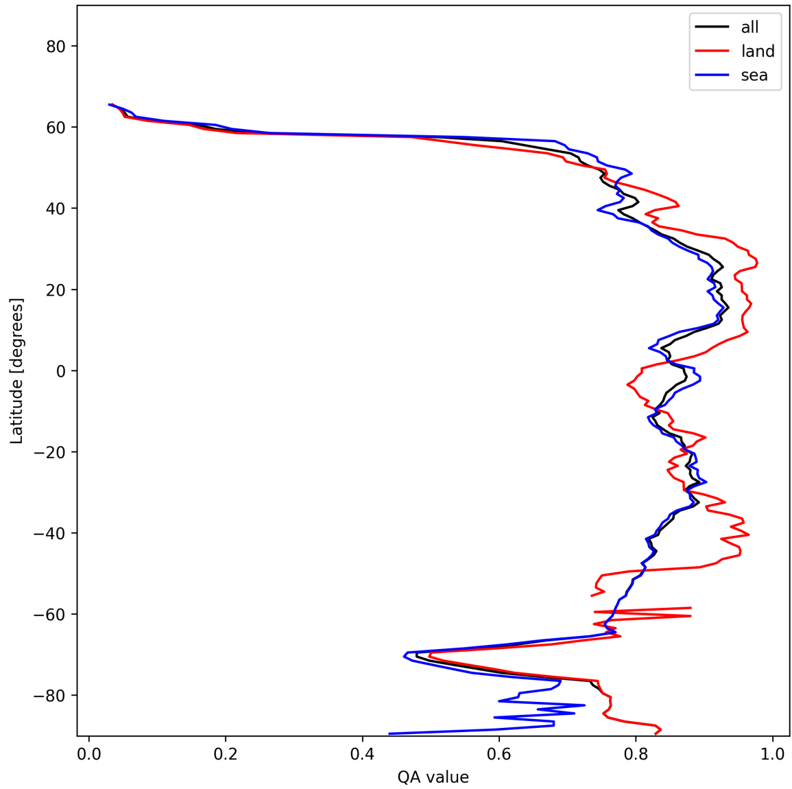
Figure 9: Zonal average of “QA value” for 2024-12-09 to 2024-12-09.
