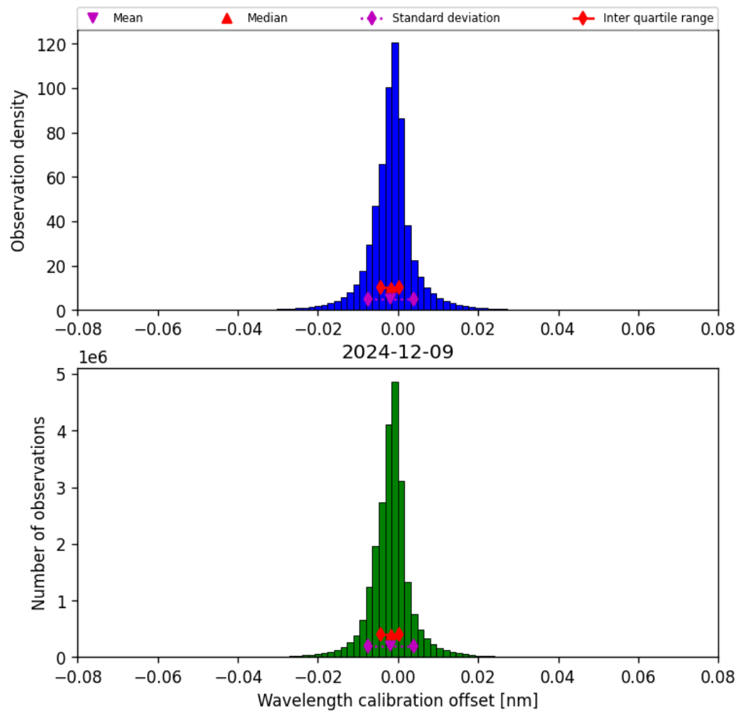
Figure 33: Histogram of “Wavelength calibration offset” for 2024-12-09 to 2024-12-09
