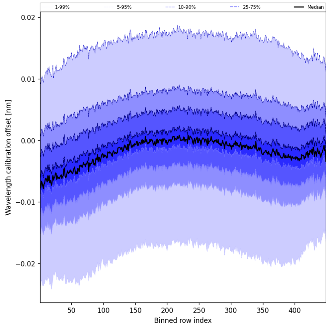
Figure 50: Along track statistics of “Wavelength calibration offset” for 2024-12-09 to 2024-12-09
