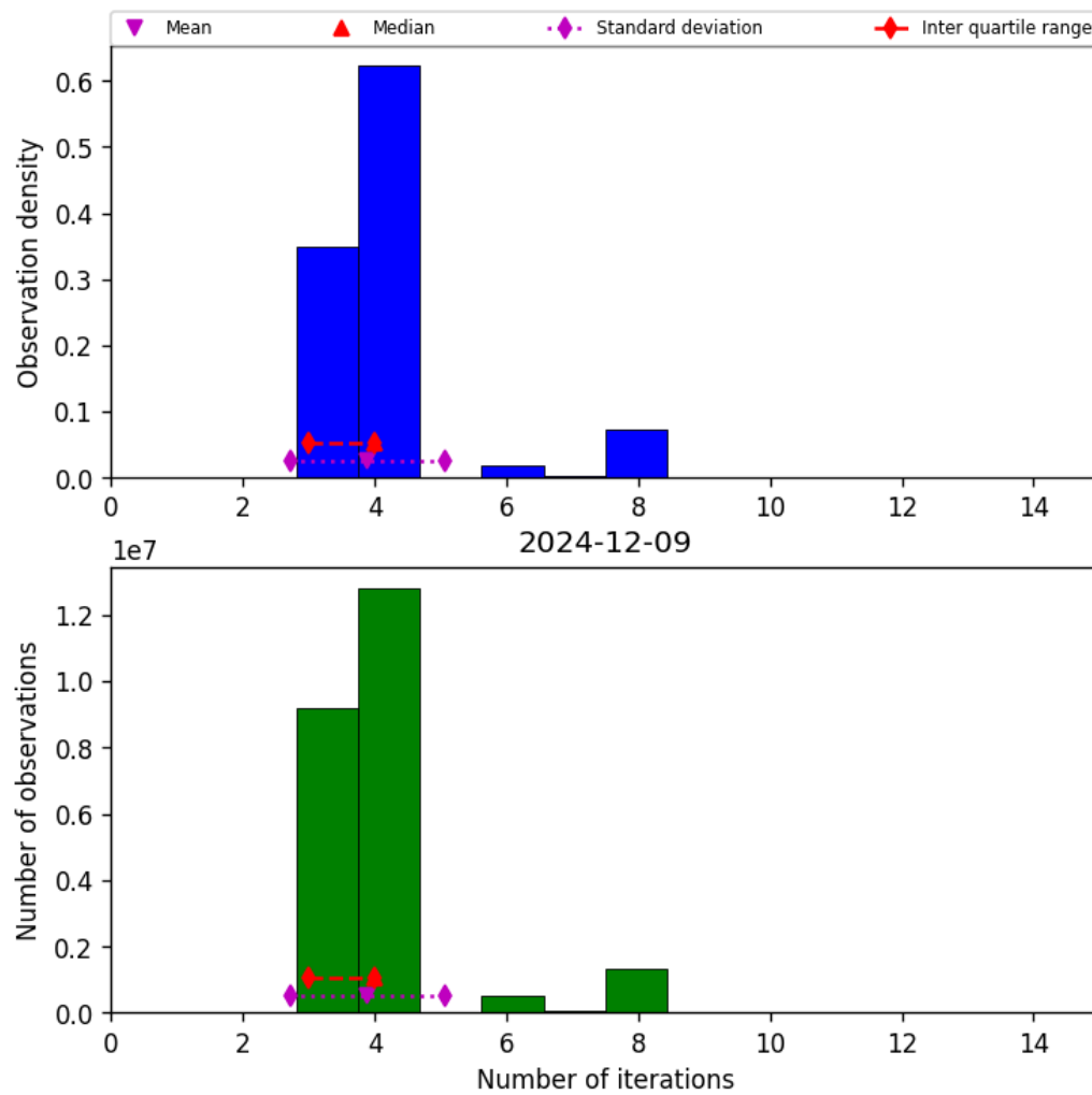
Figure 32: Histogram of “Number of iterations” for 2024-12-09 to 2024-12-09
