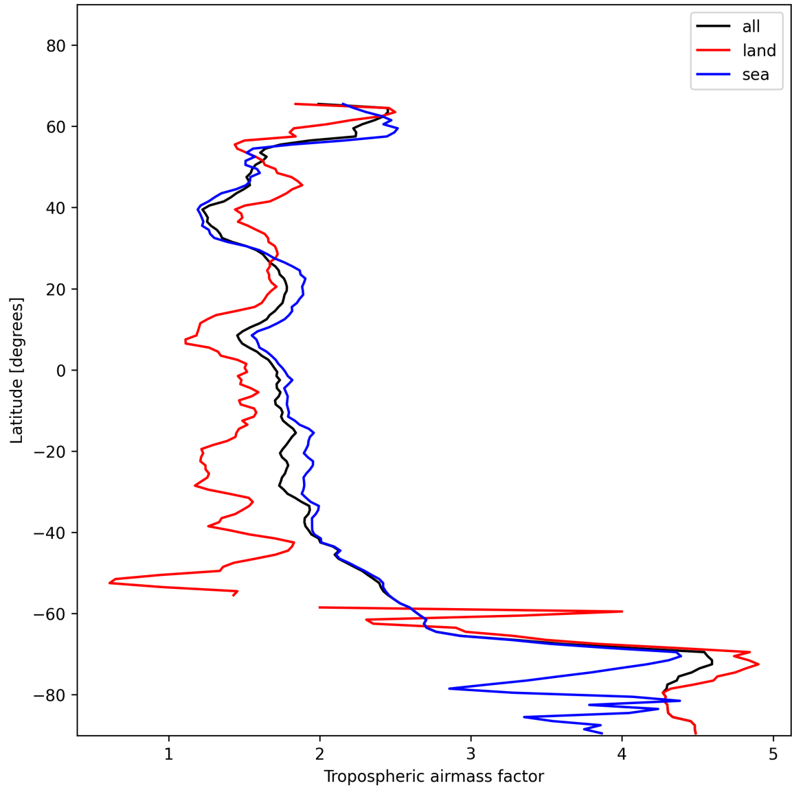
Figure 12: Zonal average of “Tropospheric airmass factor” for 2024-12-09 to 2024-12-09.
