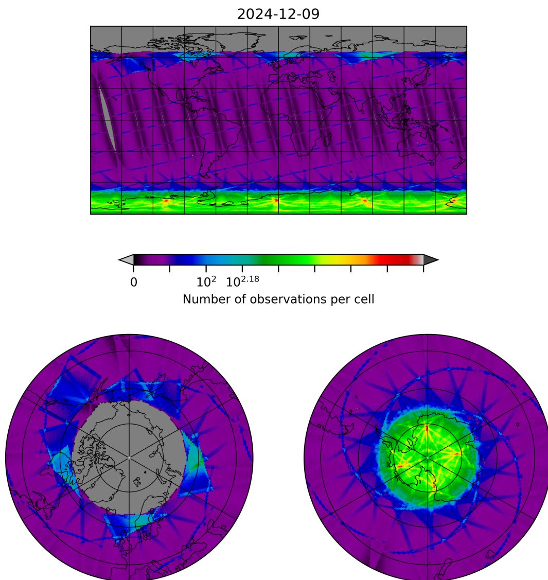
Figure 8: Map of the number of observations for 2024-12-09 to 2024-12-09
