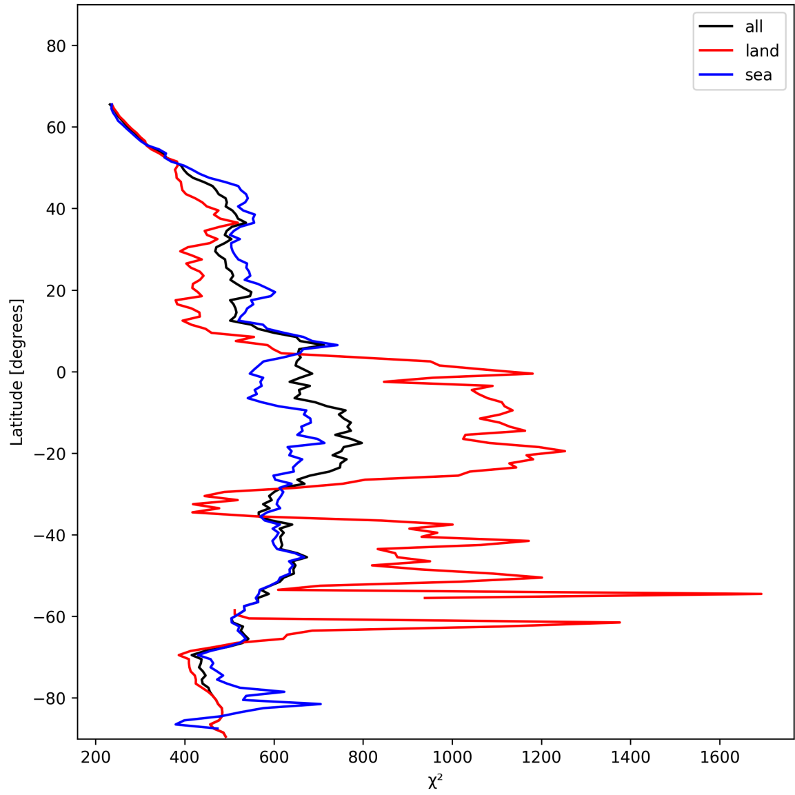
Figure 23: Zonal average of “ \chi^2 ” for 2024-12-10 to 2024-12-11.
