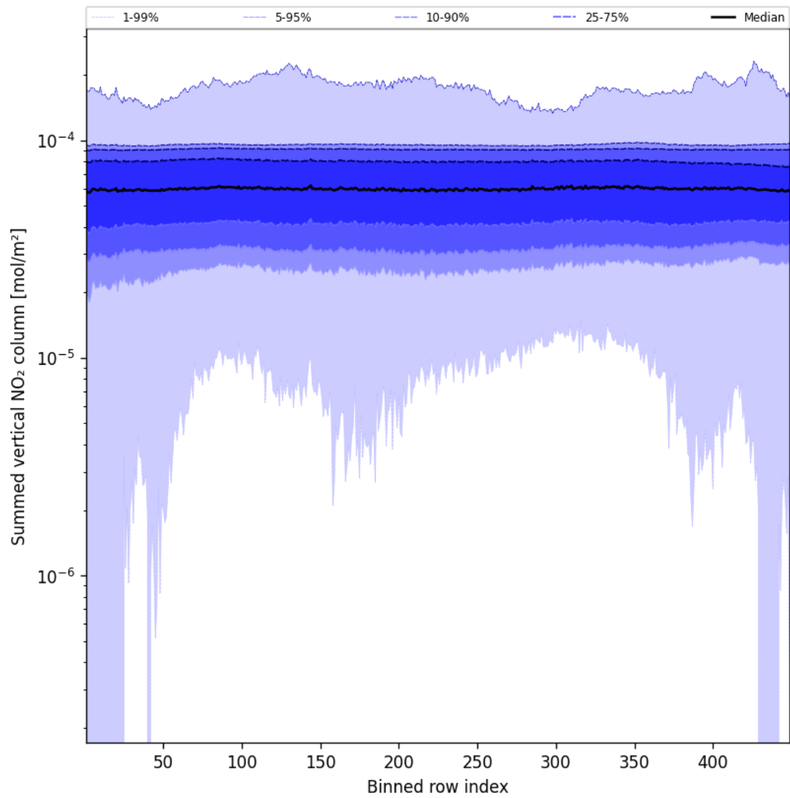
Figure 55: Along track statistics of “Summed vertical NO 2 column” for 2024-12-10 to 2024-12-11
