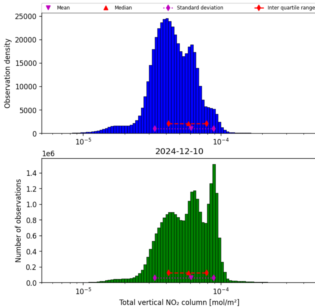
Figure 36: Histogram of “Total vertical NO 2 column” for 2024-12-10 to 2024-12-11
