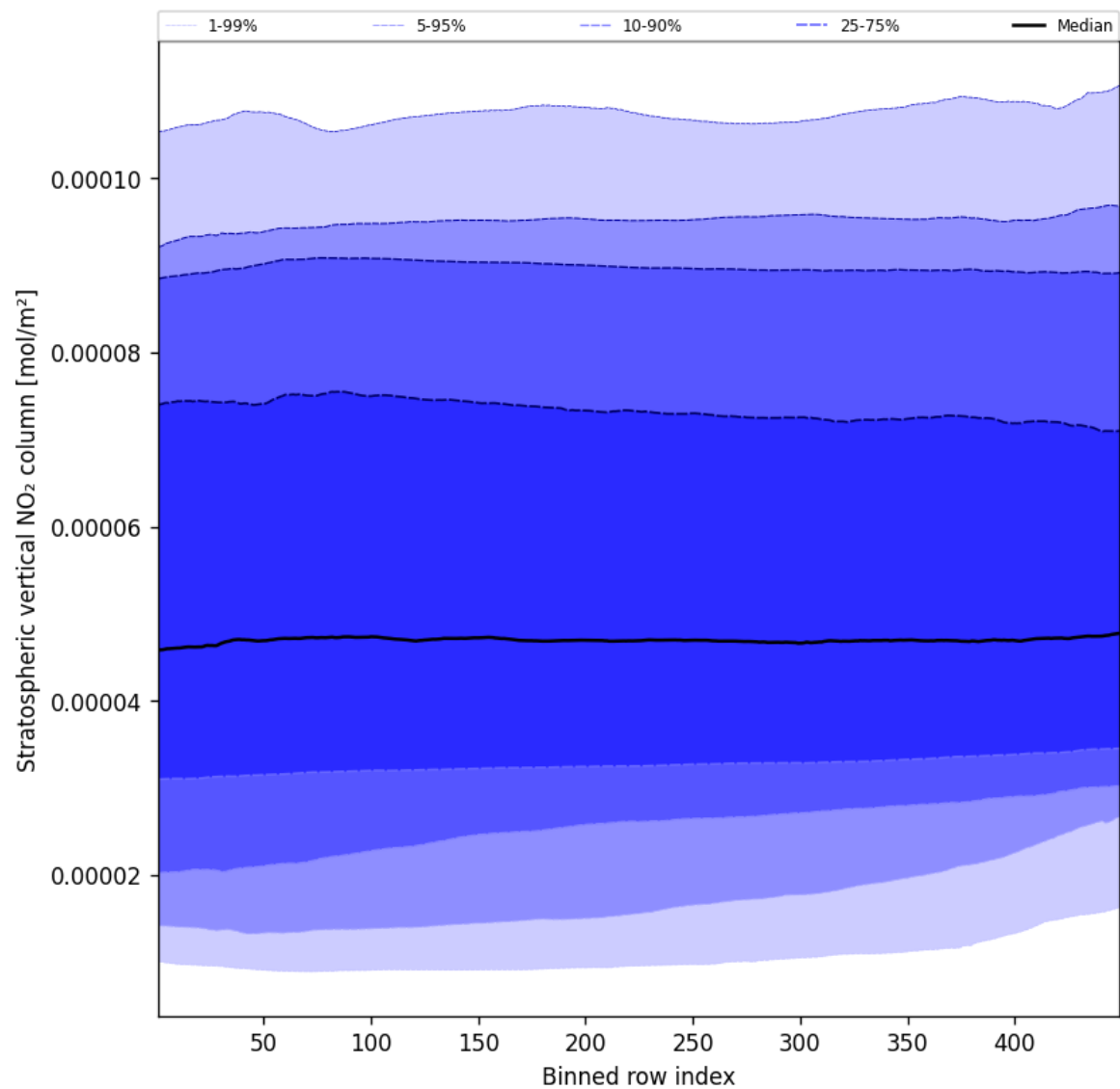
Figure 51: Along track statistics of “Stratospheric vertical NO 2 column” for 2024-12-10 to 2024-12-11
