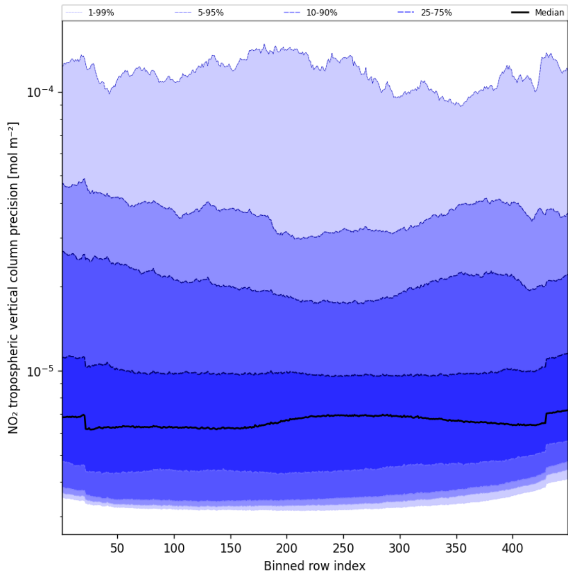
Figure 45: Along track statistics of “NO 2 tropospheric vertical column precision” for 2024-12-10 to 2024-12-11
