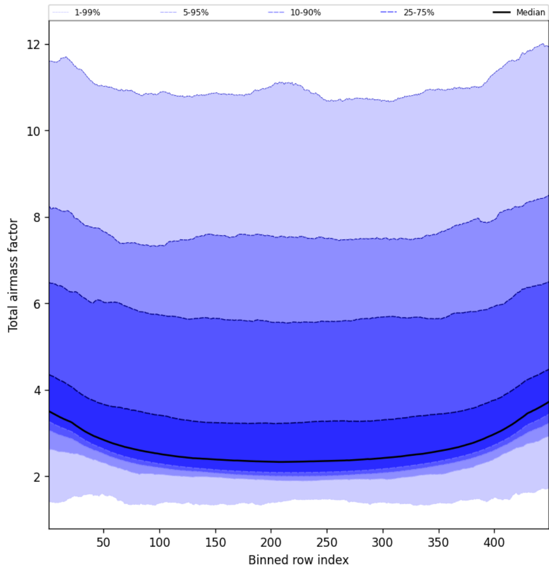
Figure 47: Along track statistics of “Total airmass factor” for 2024-12-10 to 2024-12-11
