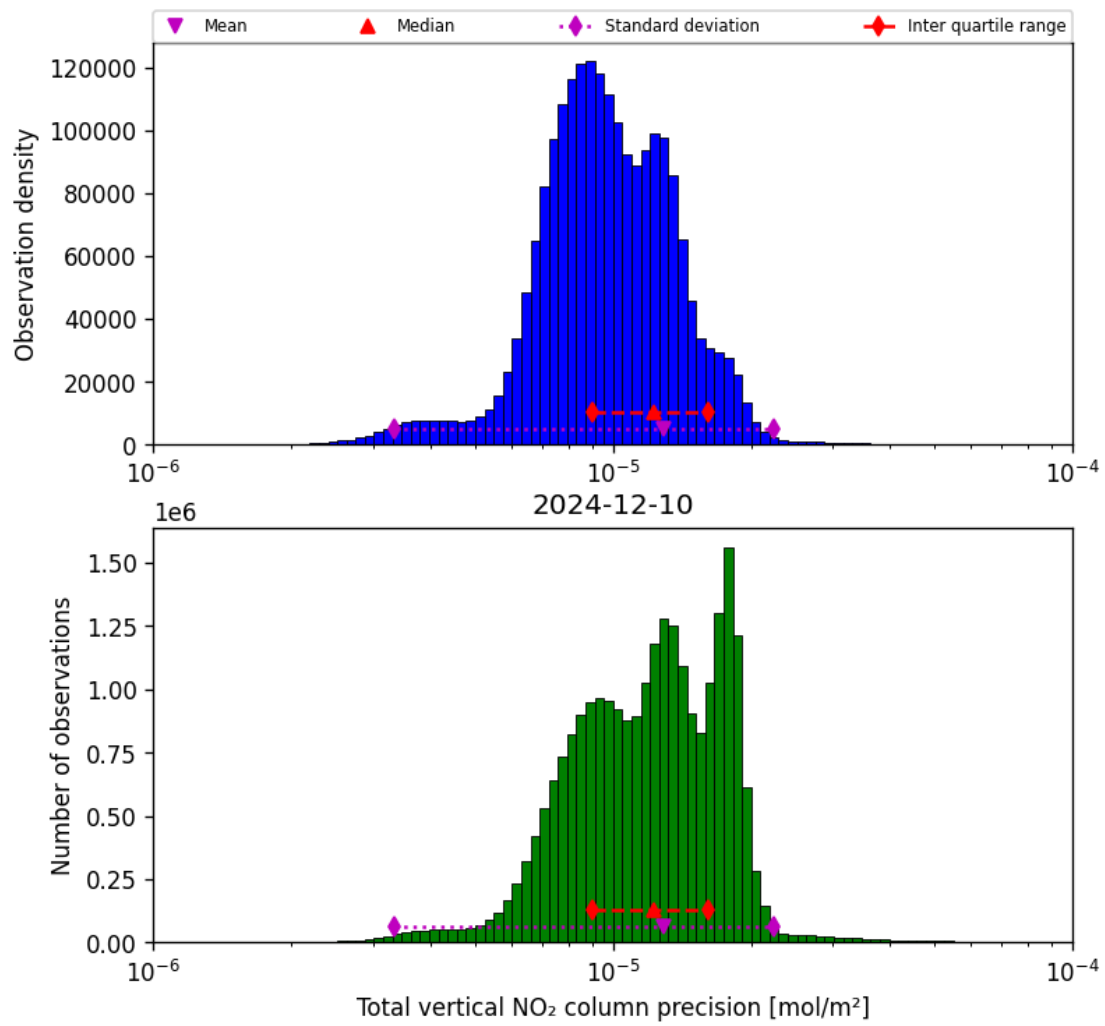
Figure 37: Histogram of “Total vertical NO 2 column precision” for 2024-12-10 to 2024-12-11
