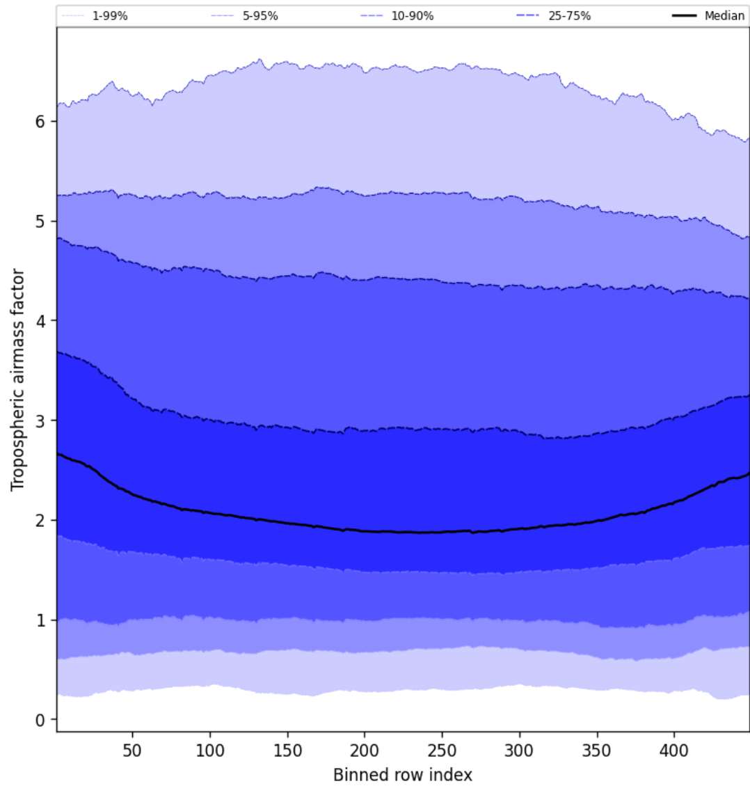
Figure 46: Along track statistics of “Tropospheric airmass factor” for 2024-12-10 to 2024-12-11
