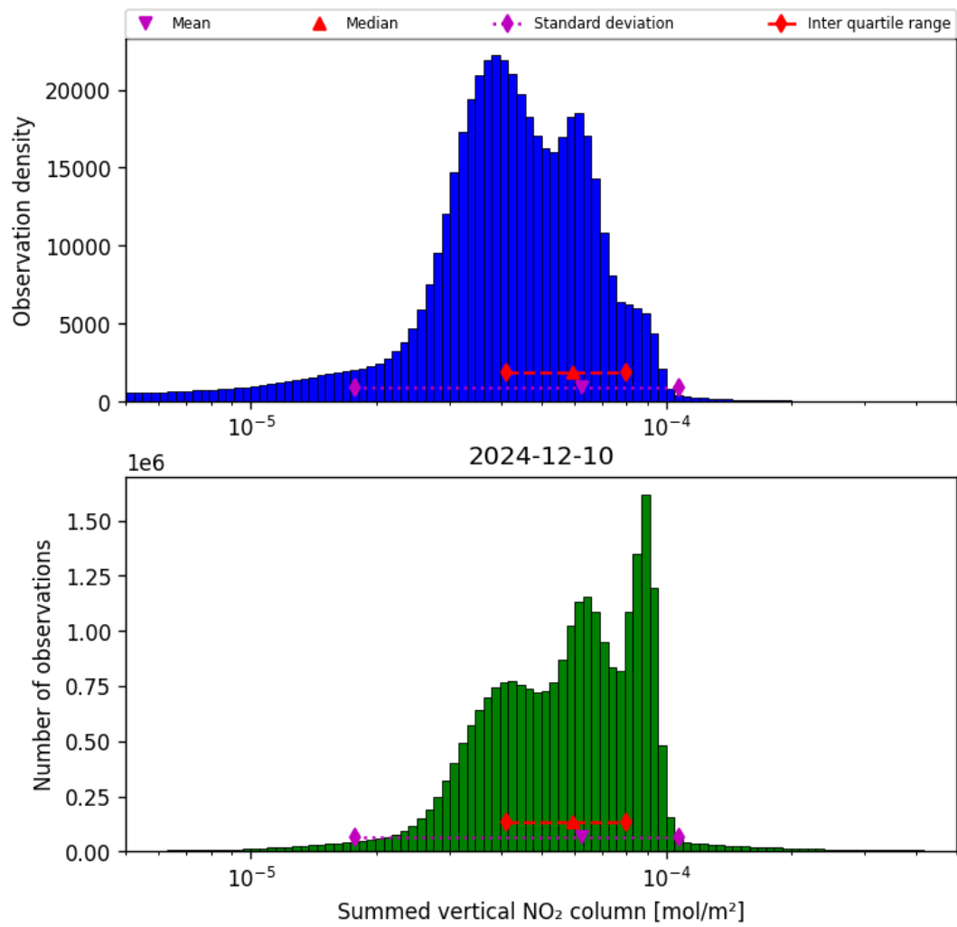
Figure 38: Histogram of “Summed vertical NO 2 column” for 2024-12-10 to 2024-12-11
