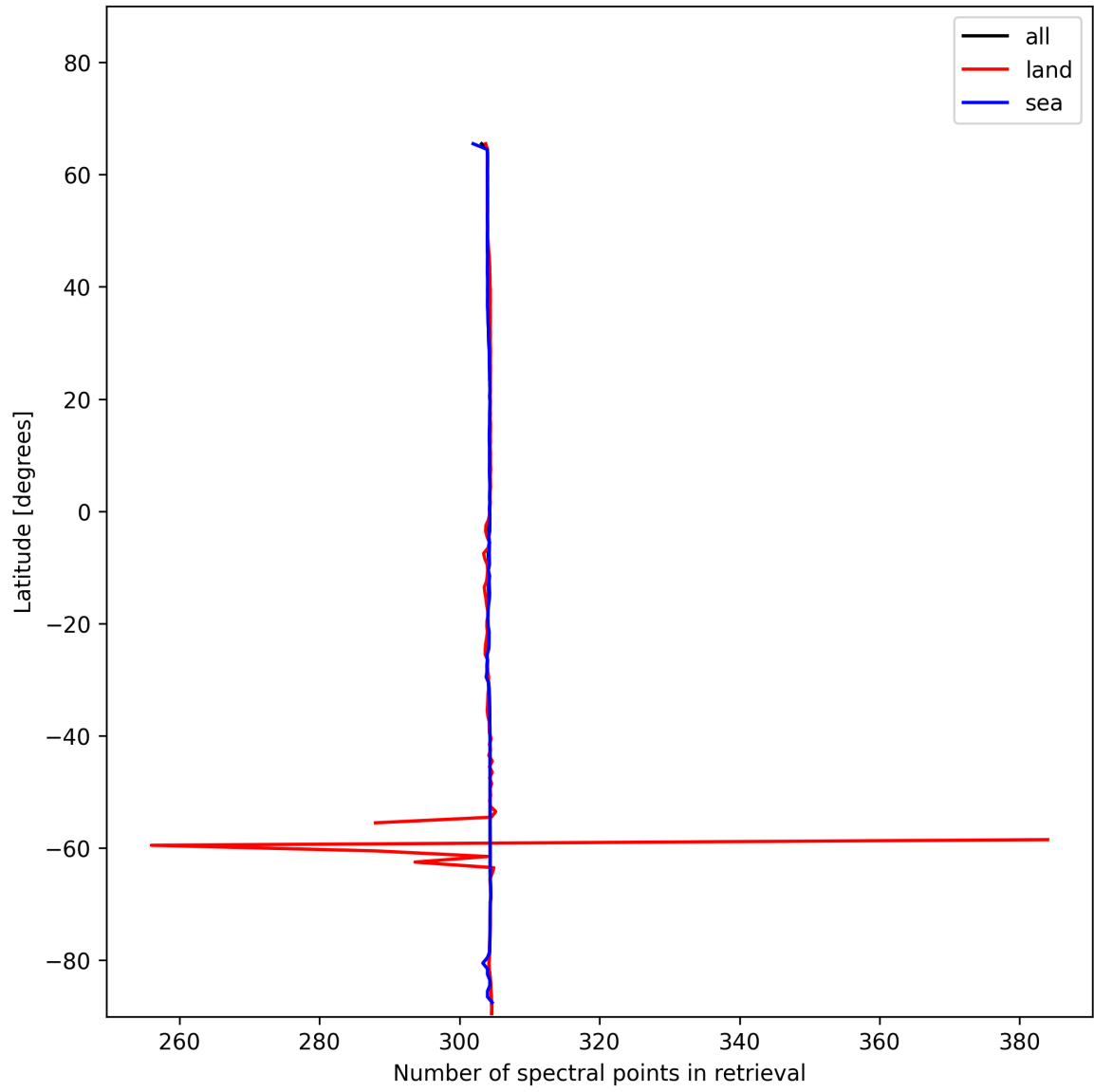
Figure 14: Zonal average of “Number of spectral points in retrieval” for 2024-12-10 to 2024-12-11.
