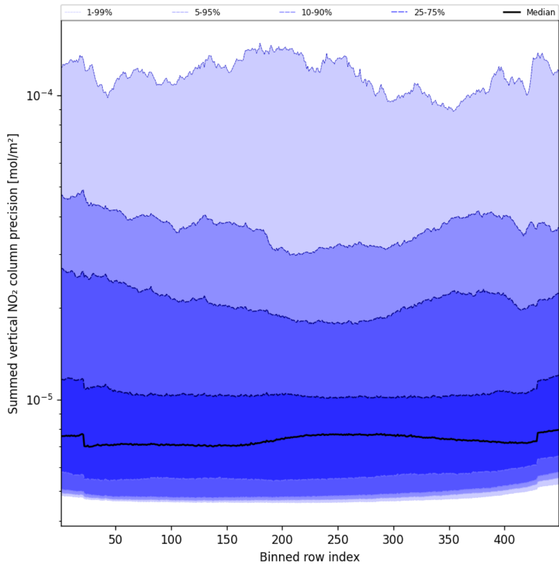
Figure 56: Along track statistics of “Summed vertical NO 2 column precision” for 2024-12-10 to 2024-12-11
