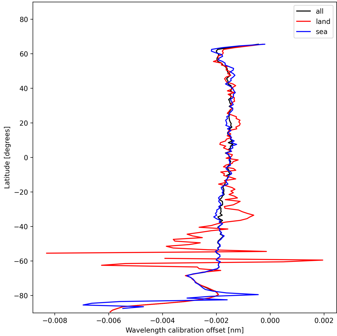
Figure 16: Zonal average of “Wavelength calibration offset” for 2024-12-10 to 2024-12-11.
