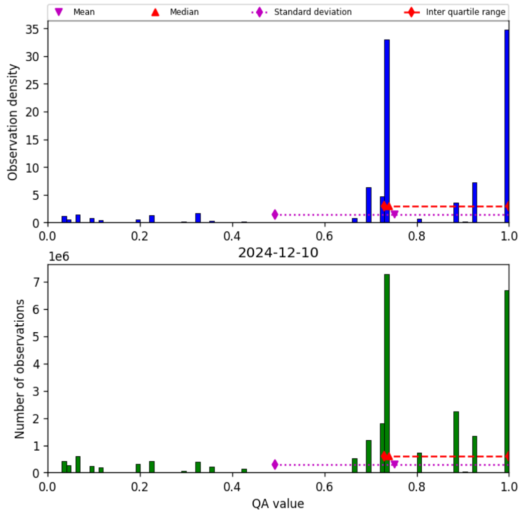
Figure 26: Histogram of “QA value” for 2024-12-10 to 2024-12-11
