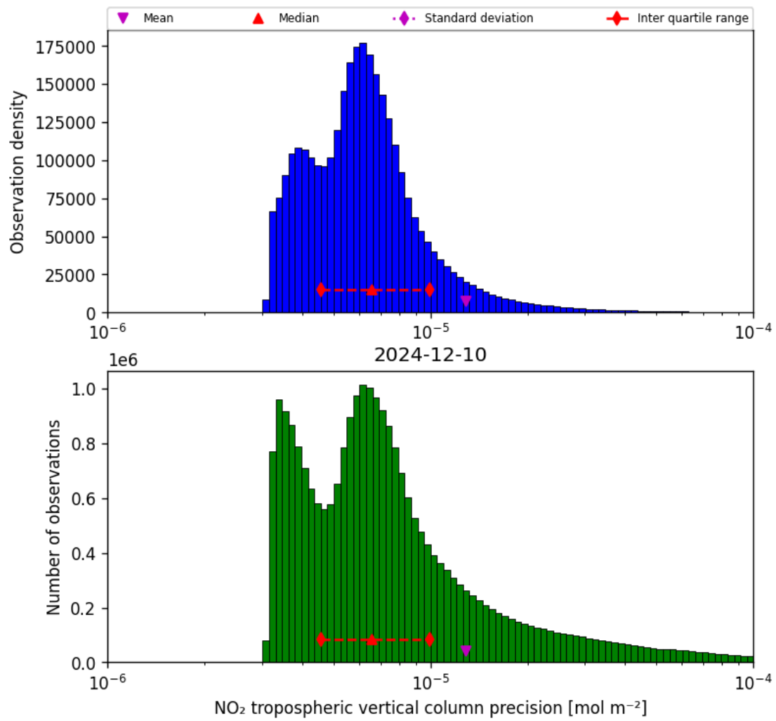
Figure 28: Histogram of “NO 2 tropospheric vertical column precision” for 2024-12-10 to 2024-12-11
