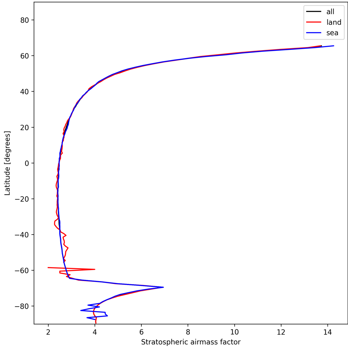
Figure 25: Zonal average of “Stratospheric airmass factor” for 2024-12-10 to 2024-12-11.
