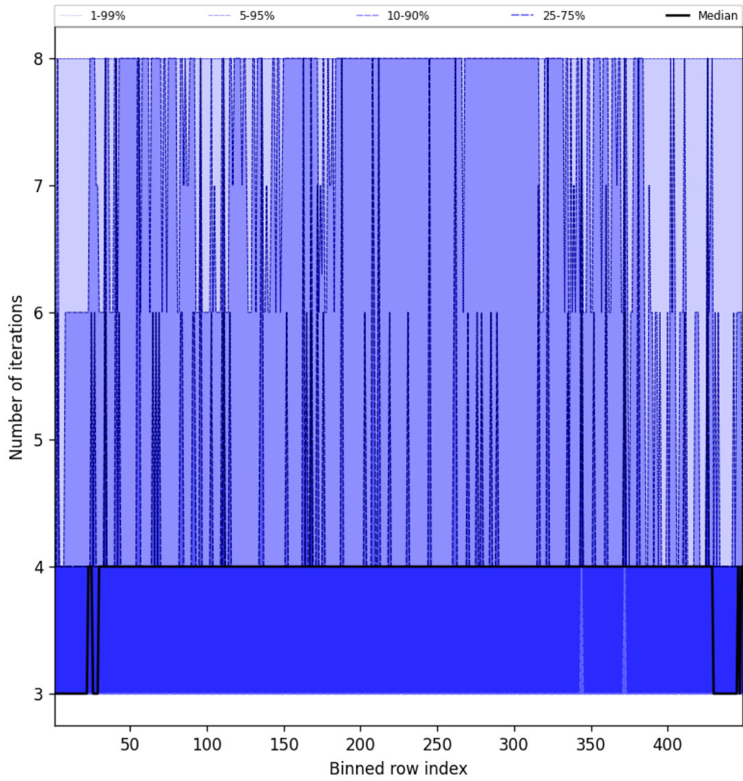
Figure 49: Along track statistics of “Number of iterations” for 2024-12-10 to 2024-12-11
