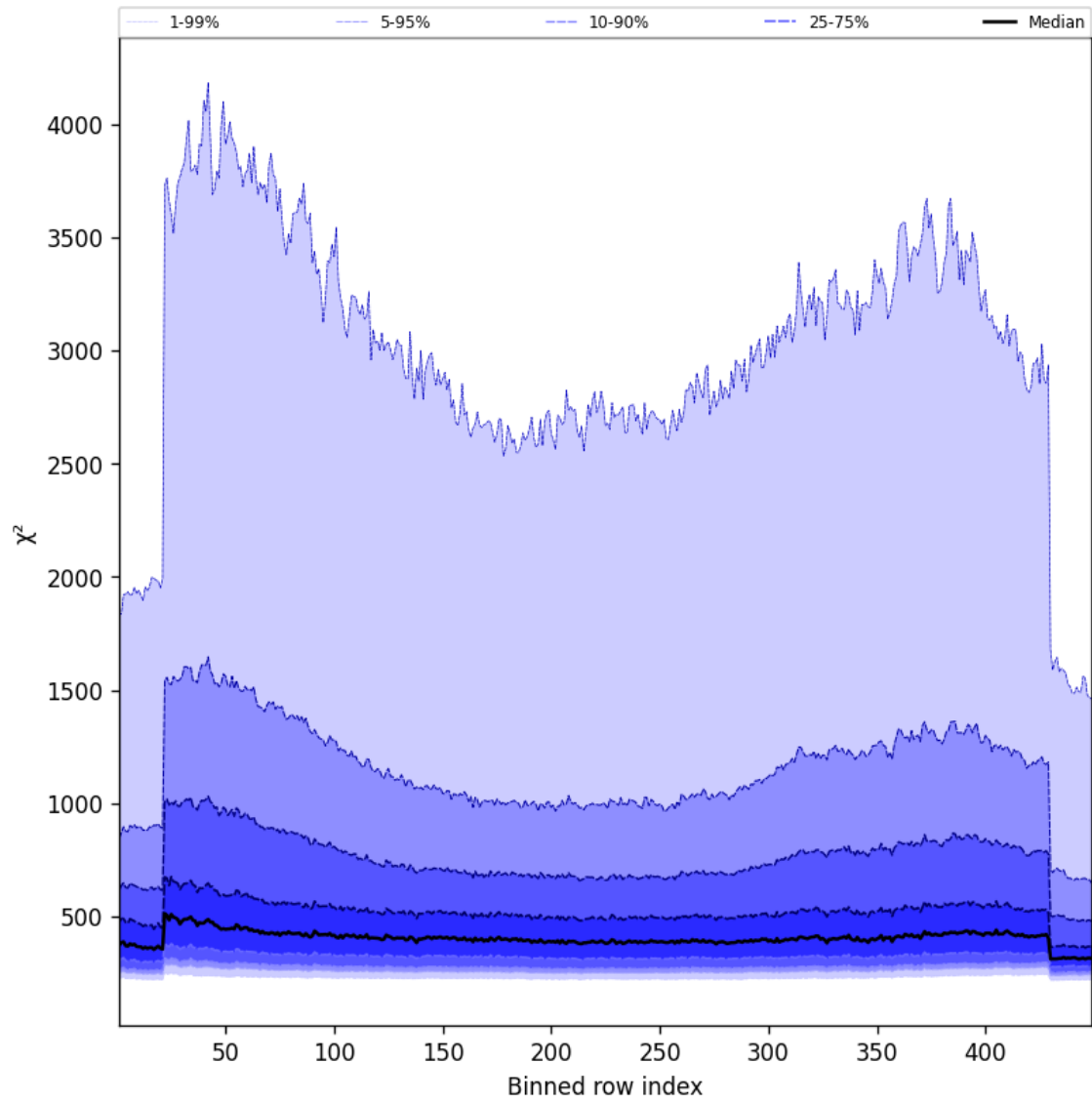
Figure 57: Along track statistics of “ \chi^2 ” for 2024-12-10 to 2024-12-11
