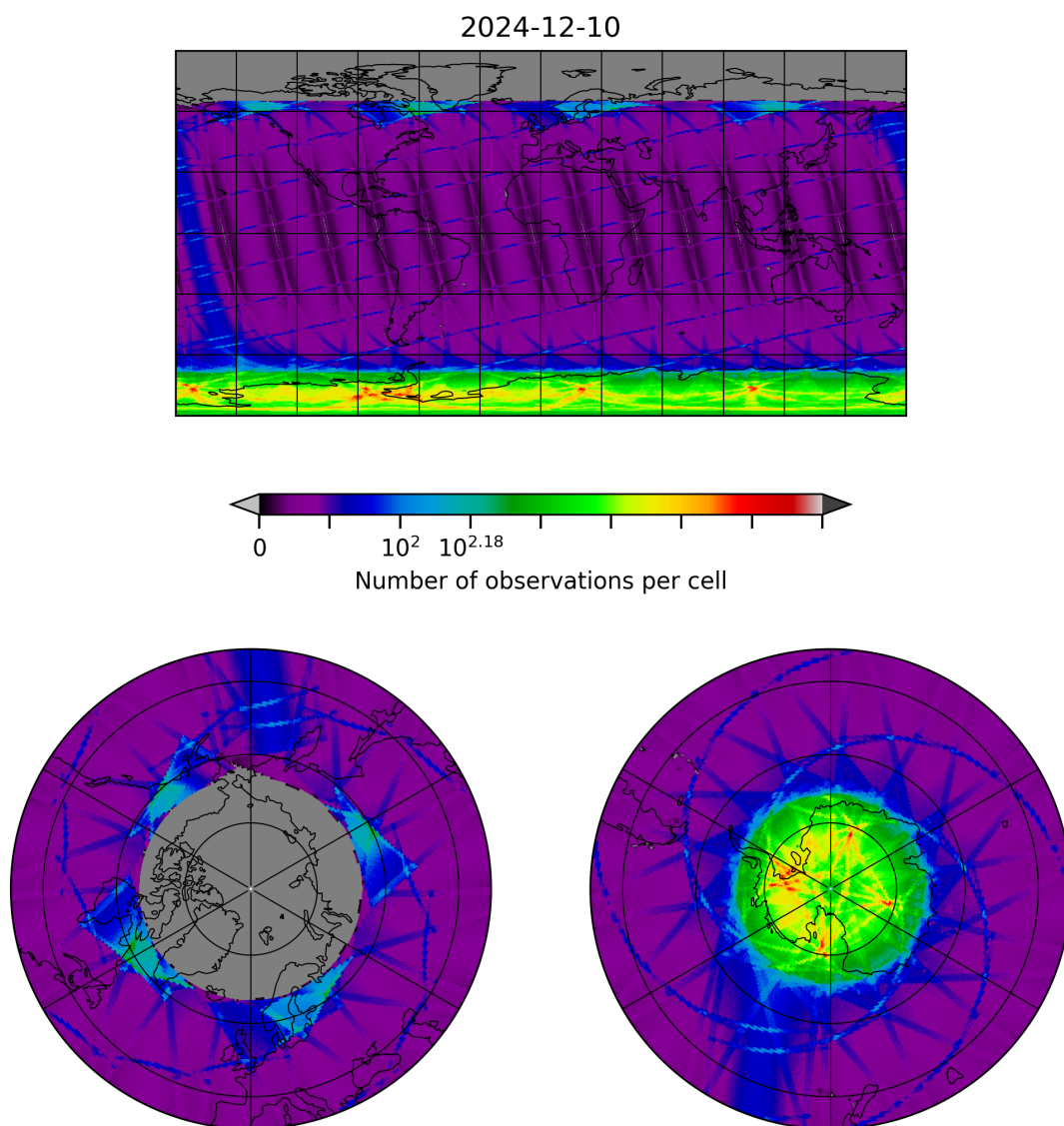
Figure 8: Map of the number of observations for 2024-12-10 to 2024-12-11
