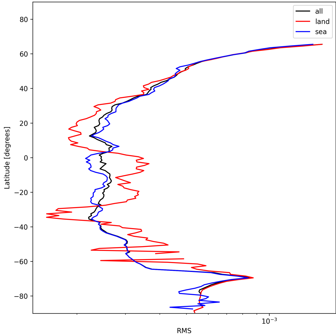
Figure 24: Zonal average of “RMS” for 2024-12-10 to 2024-12-11.
