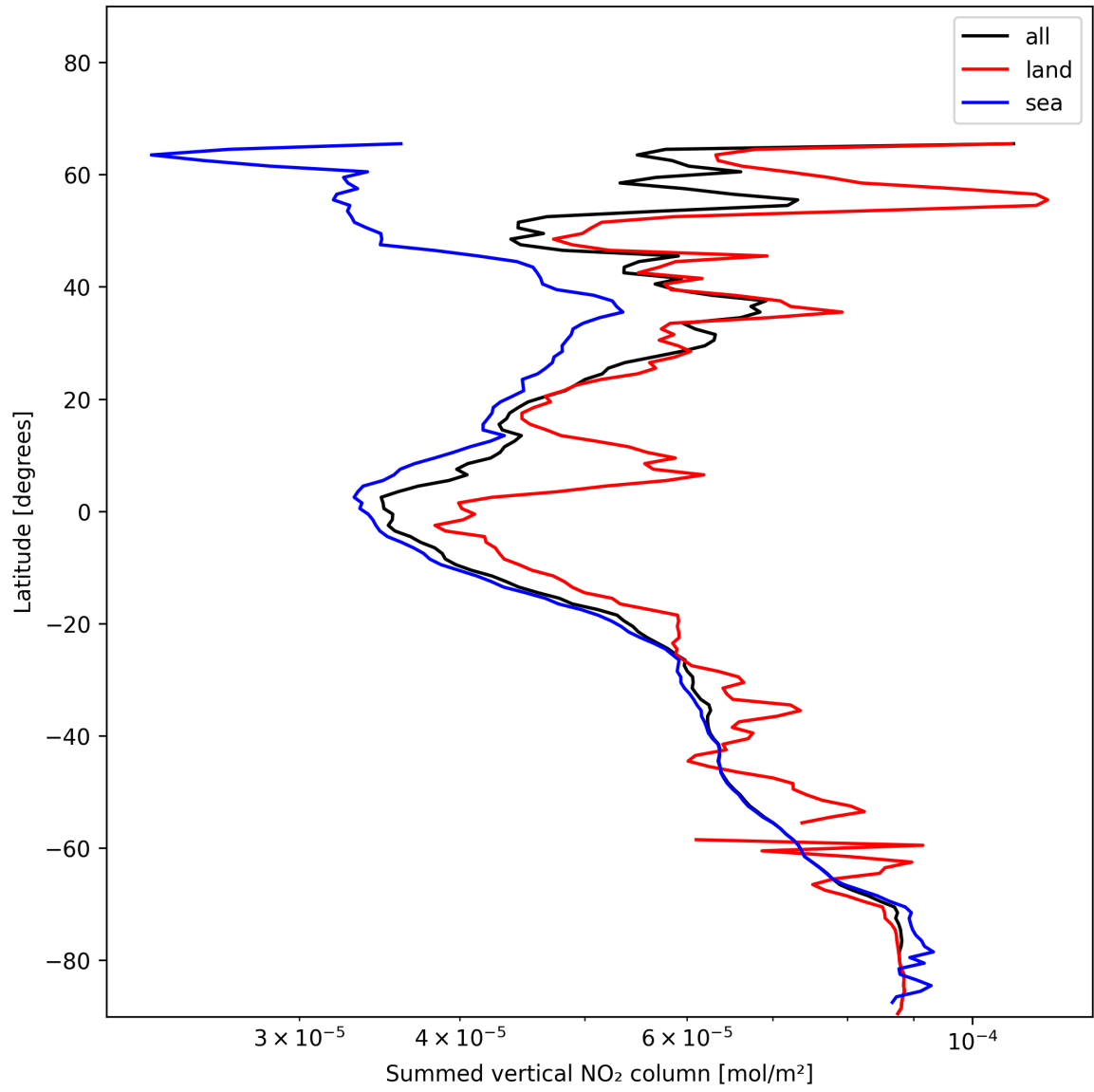
Figure 21: Zonal average of “Summed vertical NO 2 column” for 2024-12-10 to 2024-12-11.
