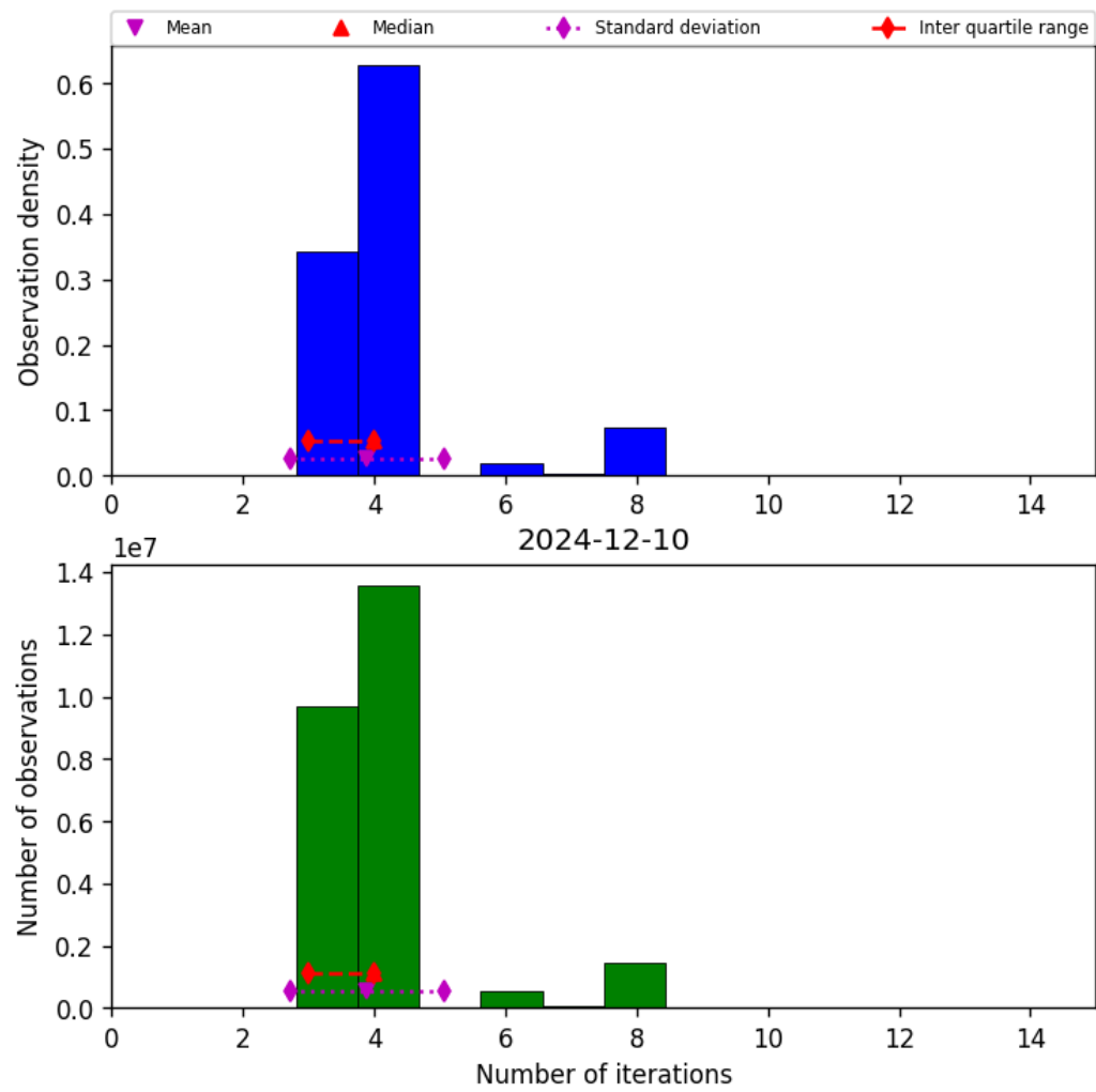
Figure 32: Histogram of “Number of iterations” for 2024-12-10 to 2024-12-11
