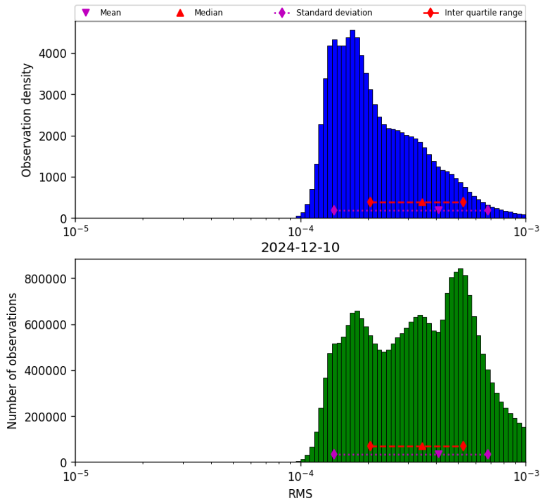
Figure 41: Histogram of “RMS” for 2024-12-10 to 2024-12-11
