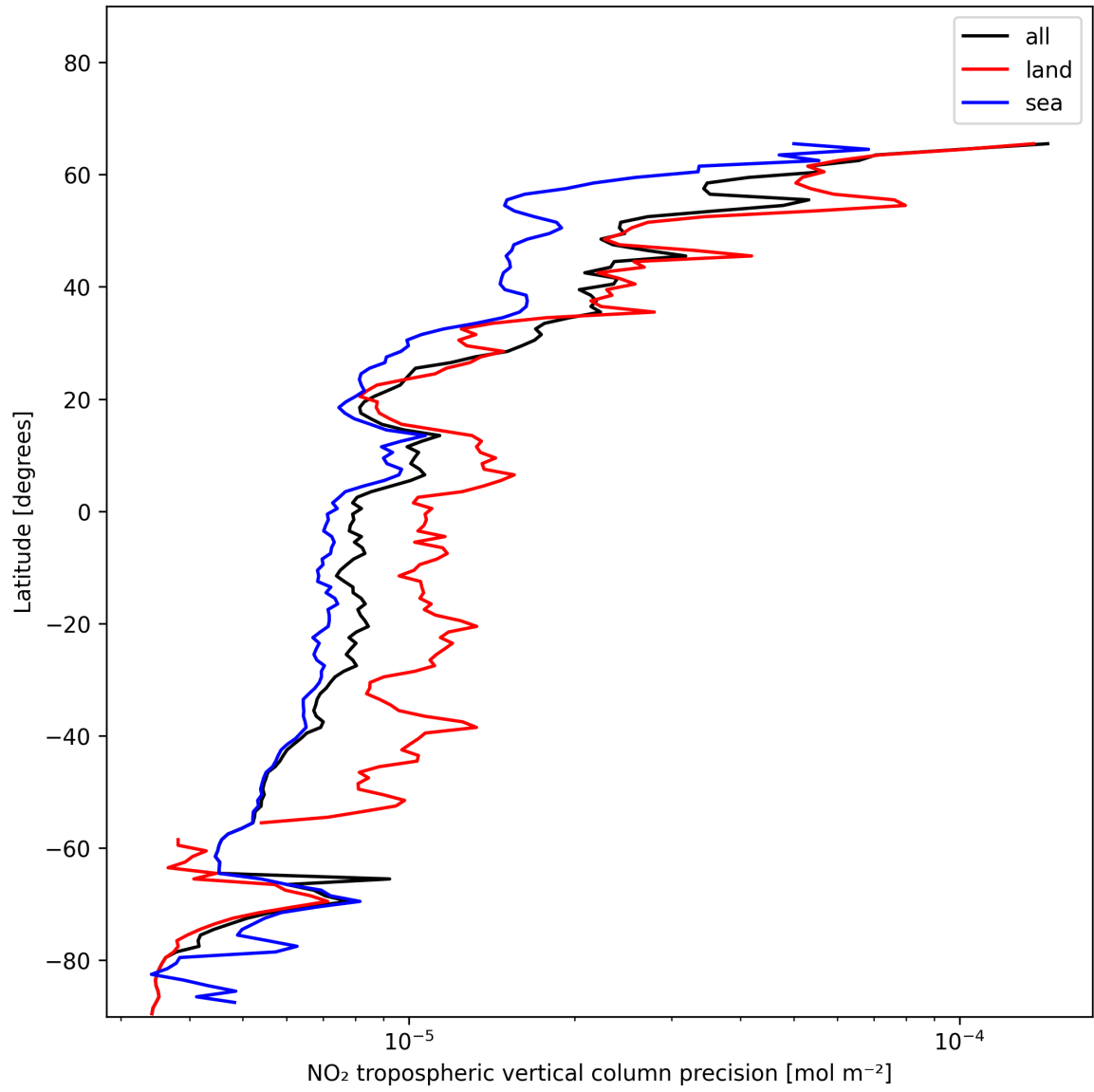
Figure 11: Zonal average of “NO 2 tropospheric vertical column precision” for 2024-12-10 to 2024-12-11.
