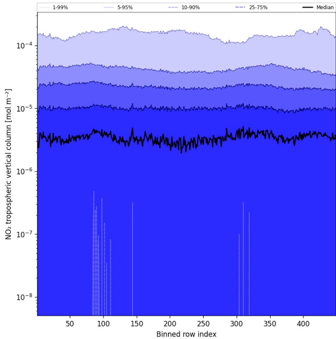
Figure 44: Along track statistics of “NO 2 tropospheric vertical column” for 2024-12-10 to 2024-12-11
