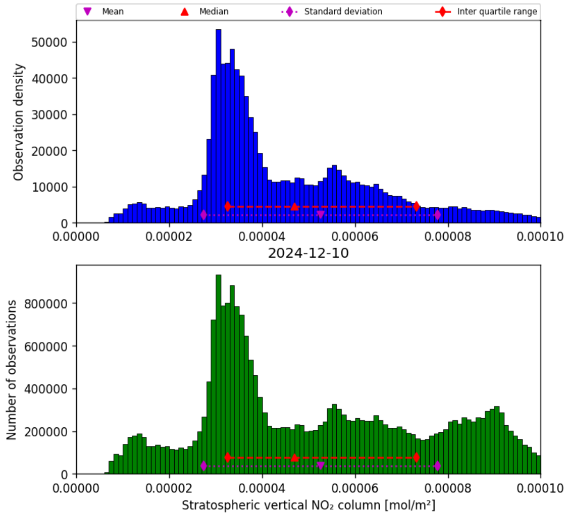
Figure 34: Histogram of “Stratospheric vertical NO 2 column” for 2024-12-10 to 2024-12-11
