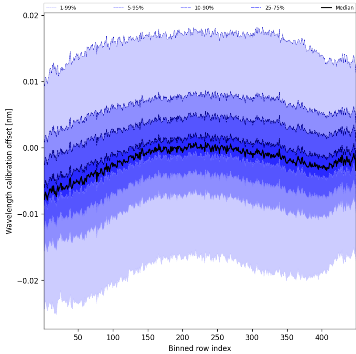
Figure 50: Along track statistics of “Wavelength calibration offset” for 2024-12-10 to 2024-12-11
