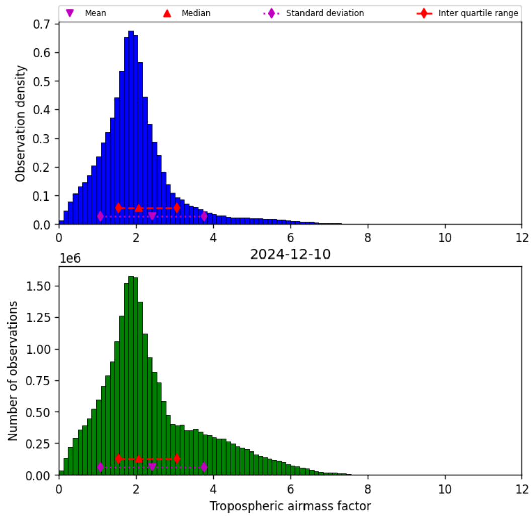
Figure 29: Histogram of “Tropospheric airmass factor” for 2024-12-10 to 2024-12-11
