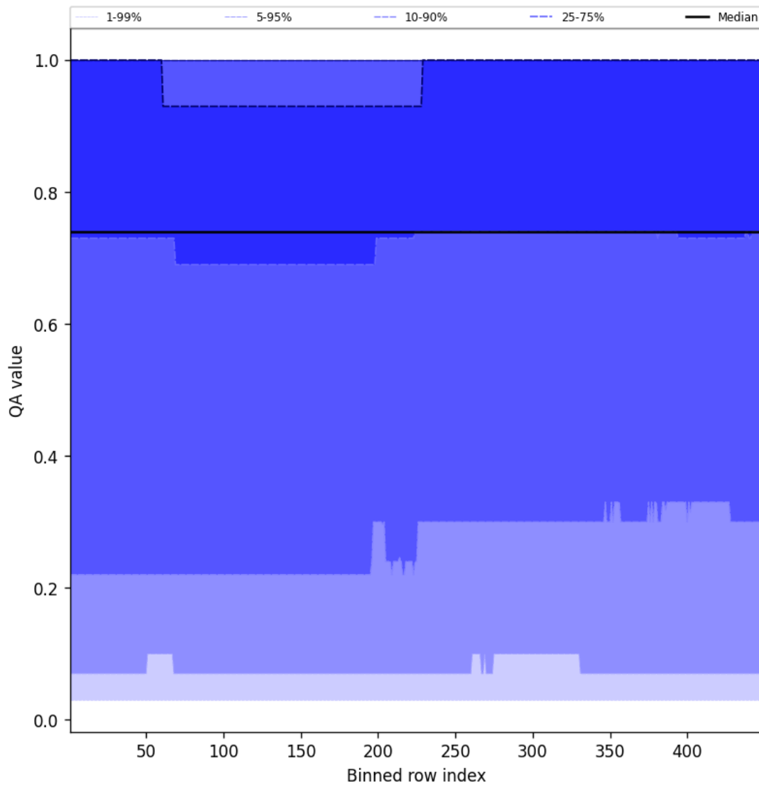
Figure 43: Along track statistics of “QA value” for 2024-12-10 to 2024-12-11
