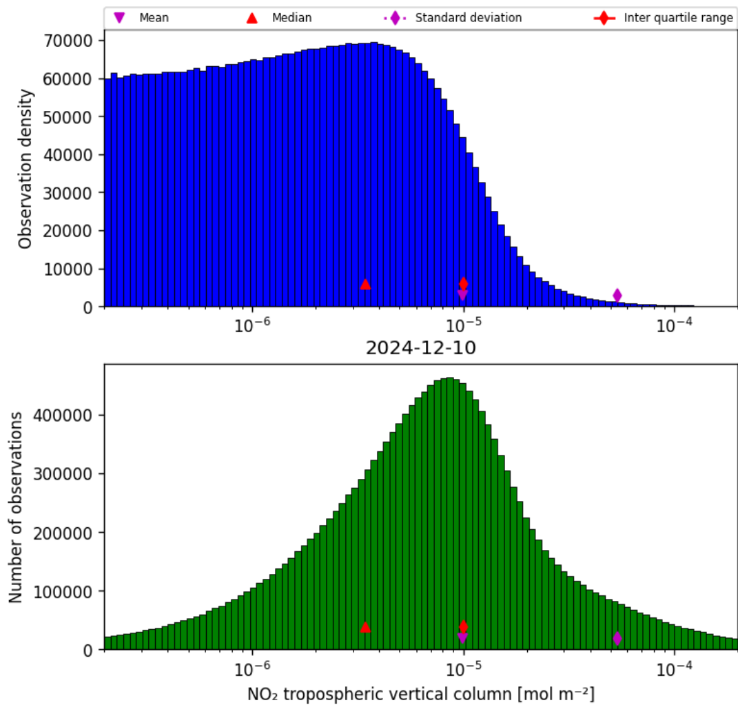
Figure 27: Histogram of “NO 2 tropospheric vertical column” for 2024-12-10 to 2024-12-11
