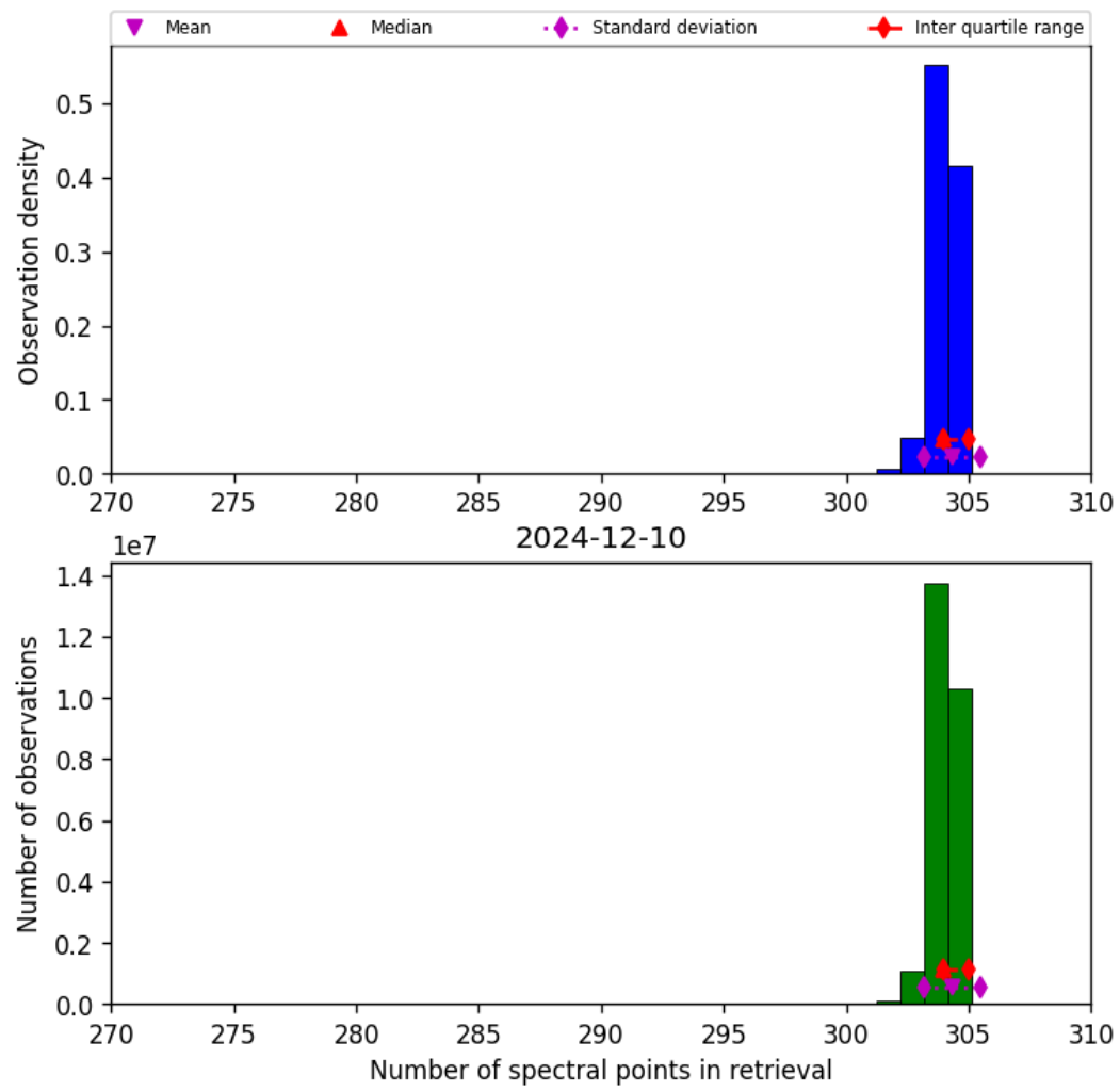
Figure 31: Histogram of “Number of spectral points in retrieval” for 2024-12-10 to 2024-12-11
