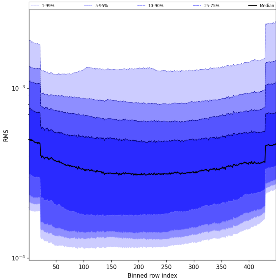
Figure 58: Along track statistics of “RMS” for 2024-12-10 to 2024-12-11
