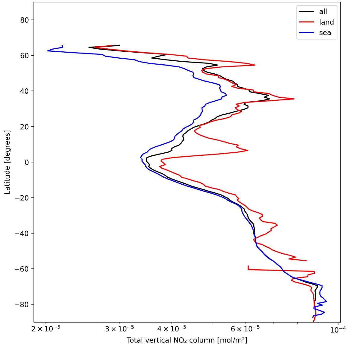
Figure 19: Zonal average of “Total vertical NO 2 column” for 2024-12-10 to 2024-12-11.
