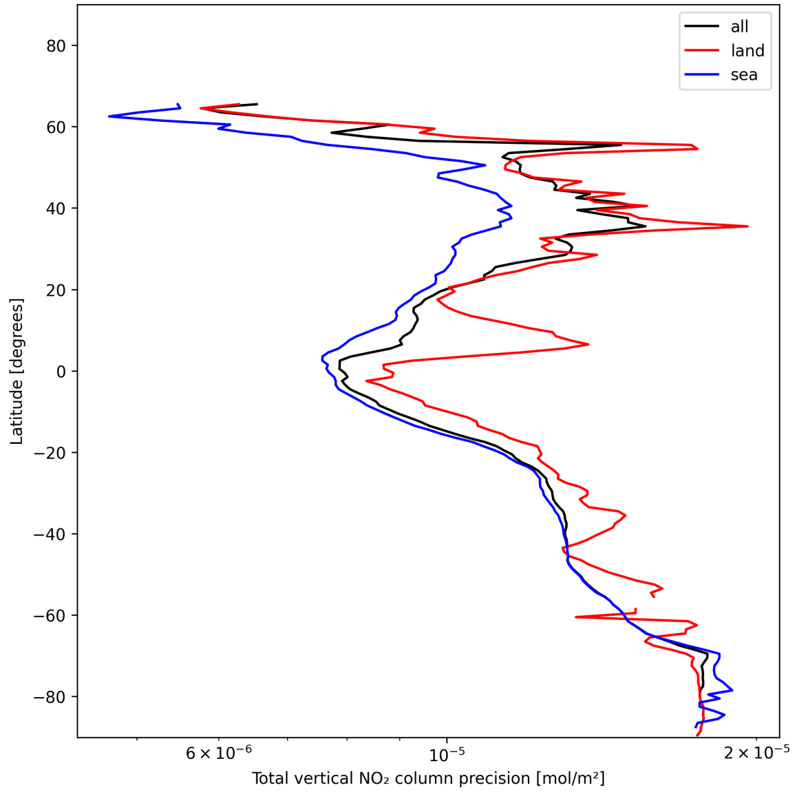
Figure 20: Zonal average of “Total vertical NO 2 column precision” for 2024-12-10 to 2024-12-11.
