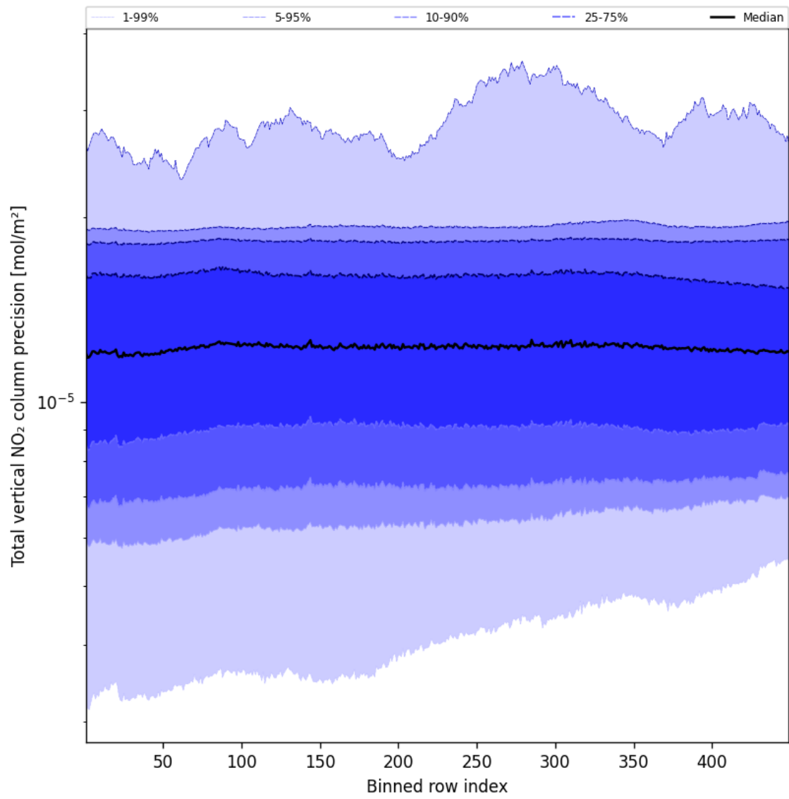
Figure 54: Along track statistics of “Total vertical NO 2 column precision” for 2024-12-10 to 2024-12-11
