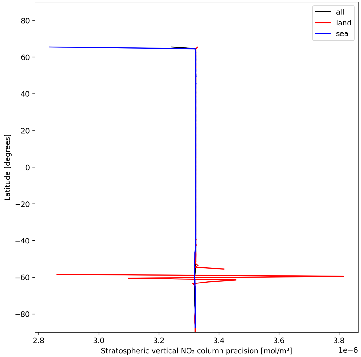
Figure 18: Zonal average of “Stratospheric vertical NO 2 column precision” for 2024-12-10 to 2024-12-11.
