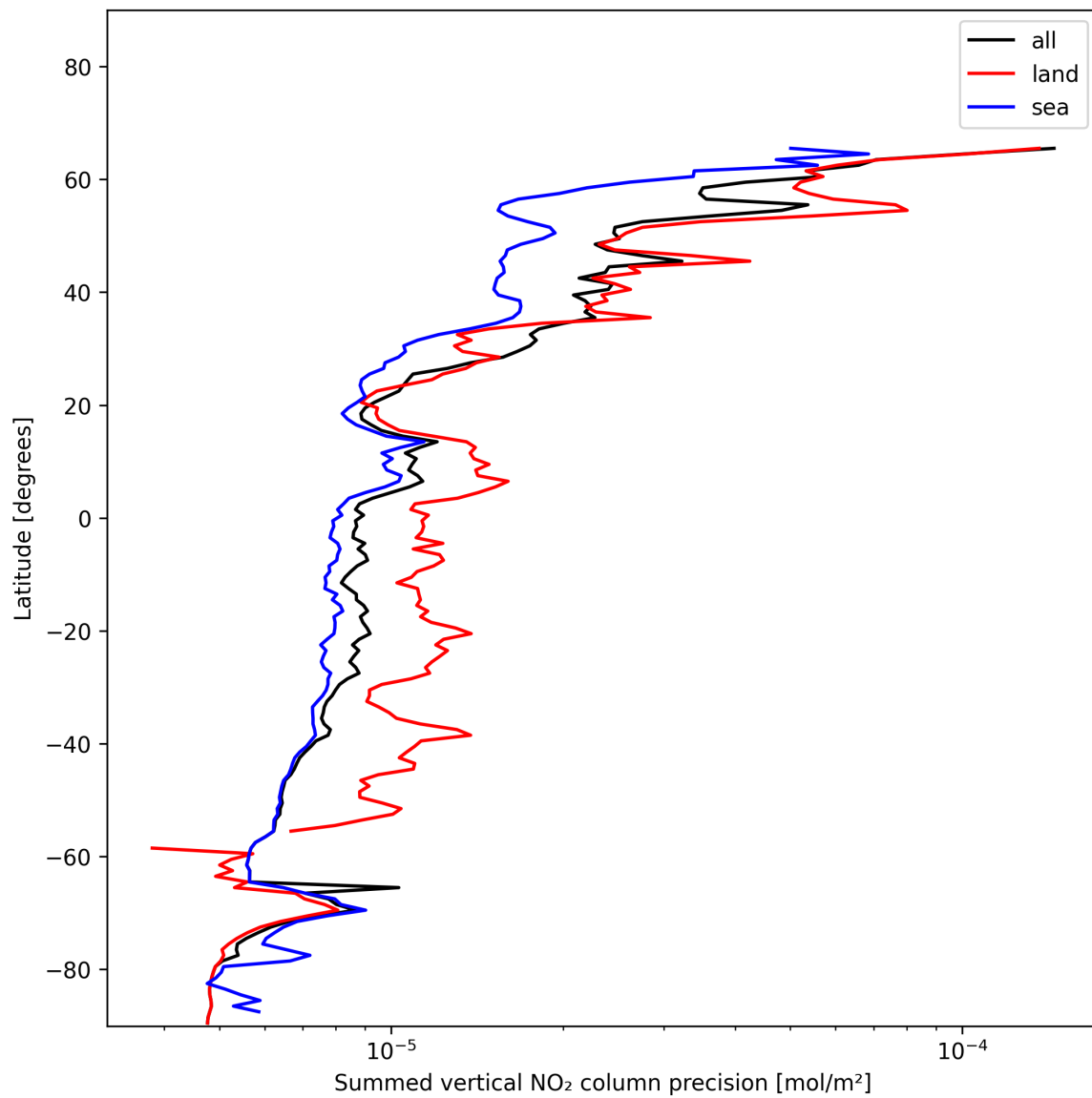
Figure 22: Zonal average of “Summed vertical NO 2 column precision” for 2024-12-10 to 2024-12-11.
