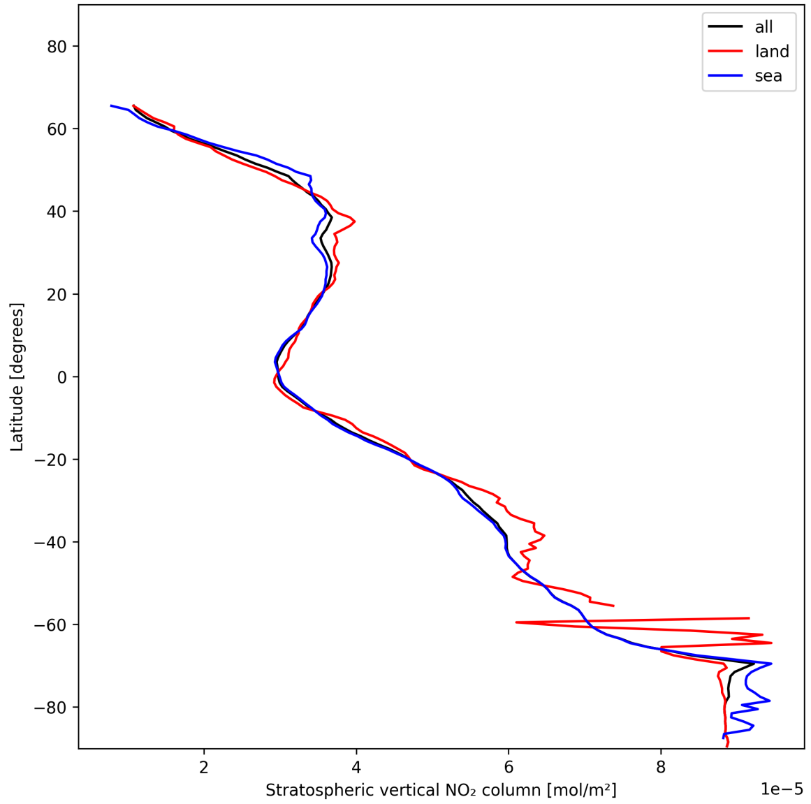
Figure 17: Zonal average of “Stratospheric vertical NO 2 column” for 2024-12-10 to 2024-12-11.
