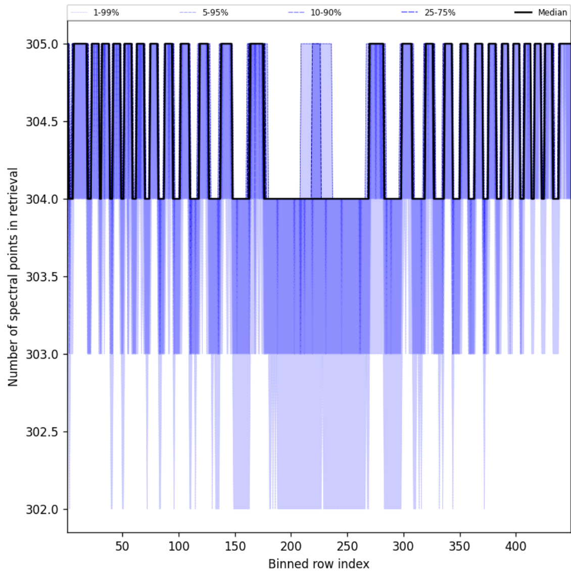
Figure 48: Along track statistics of “Number of spectral points in retrieval” for 2024-12-10 to 2024-12-11
