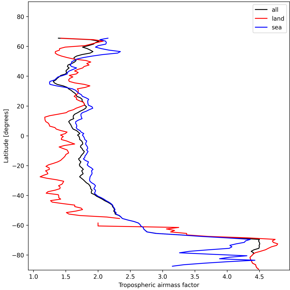
Figure 12: Zonal average of “Tropospheric airmass factor” for 2024-12-10 to 2024-12-11.
