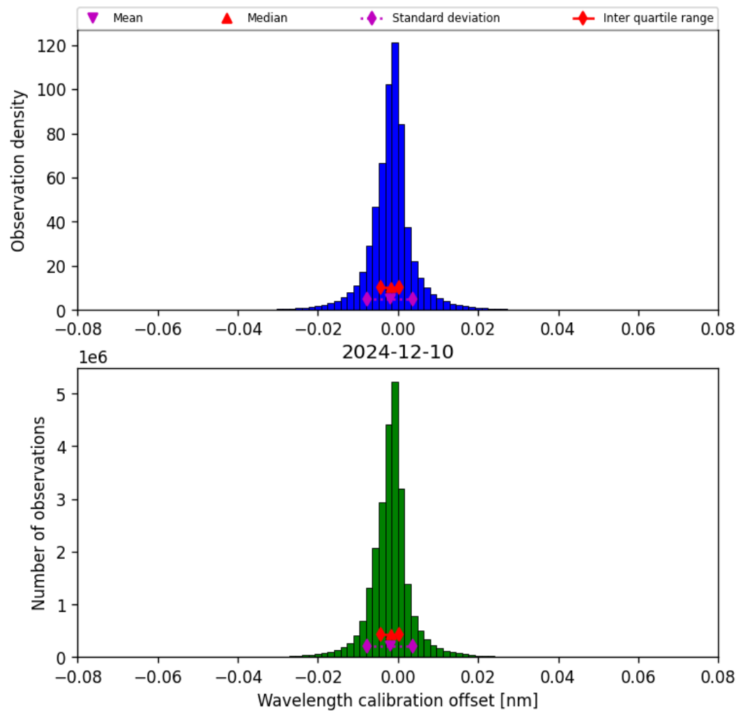
Figure 33: Histogram of “Wavelength calibration offset” for 2024-12-10 to 2024-12-11
