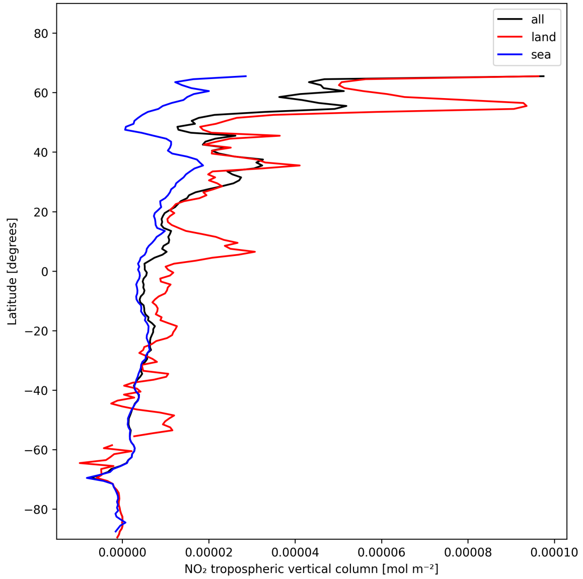
Figure 10: Zonal average of “NO 2 tropospheric vertical column” for 2024-12-10 to 2024-12-11.
