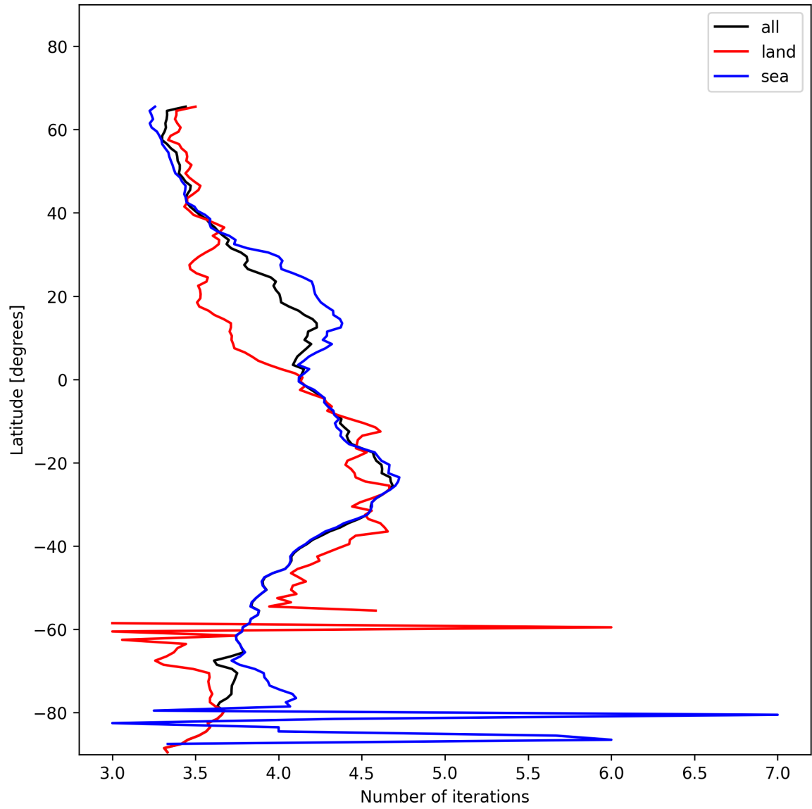
Figure 15: Zonal average of “Number of iterations” for 2024-12-10 to 2024-12-11.
