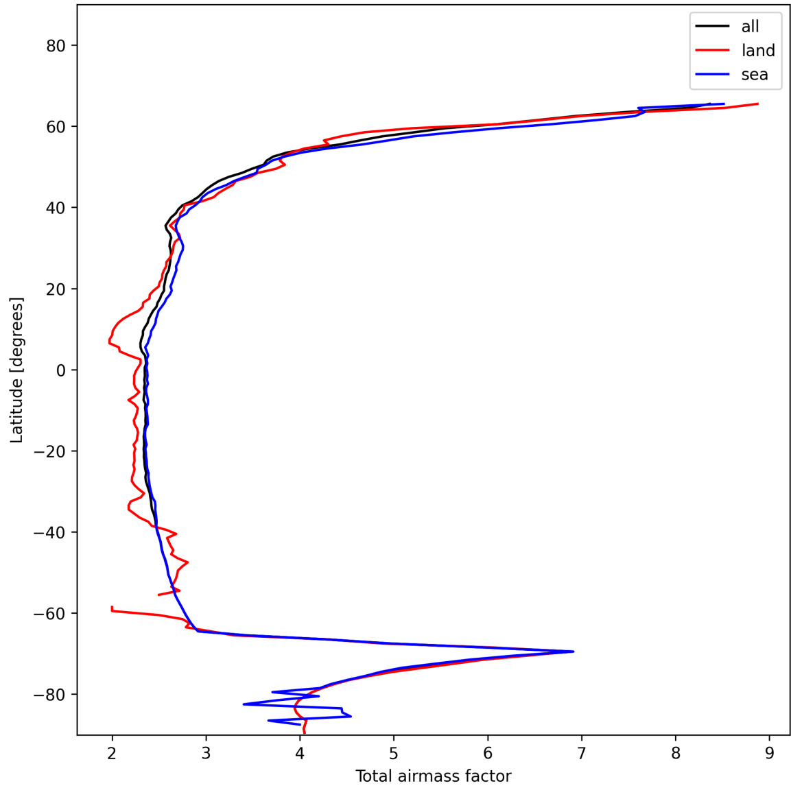
Figure 13: Zonal average of “Total airmass factor” for 2024-12-10 to 2024-12-11.
