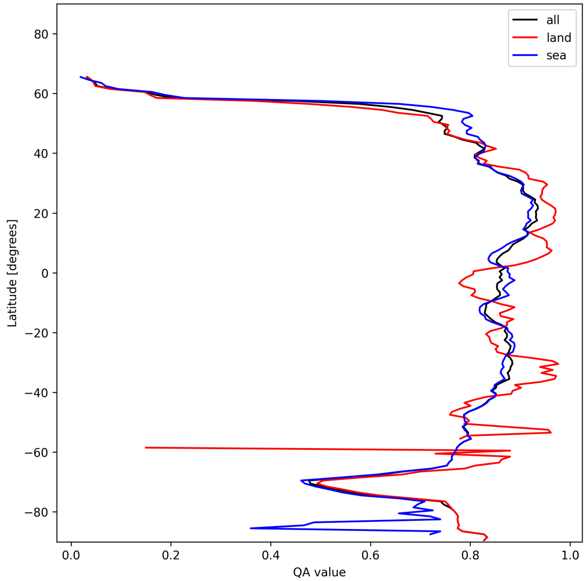
Figure 9: Zonal average of “QA value” for 2024-12-10 to 2024-12-11.
