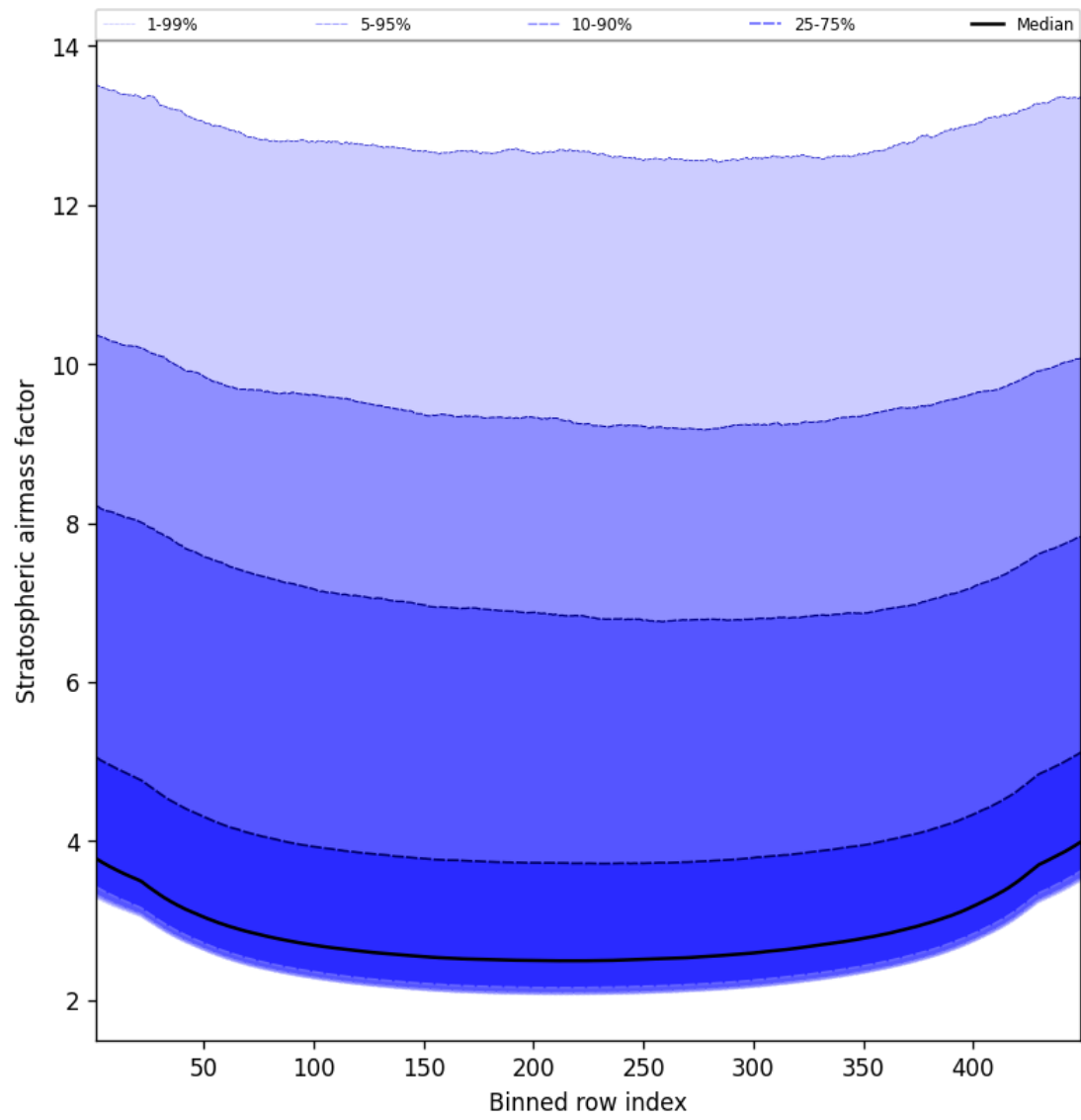
Figure 59: Along track statistics of “Stratospheric airmass factor” for 2024-12-10 to 2024-12-11
