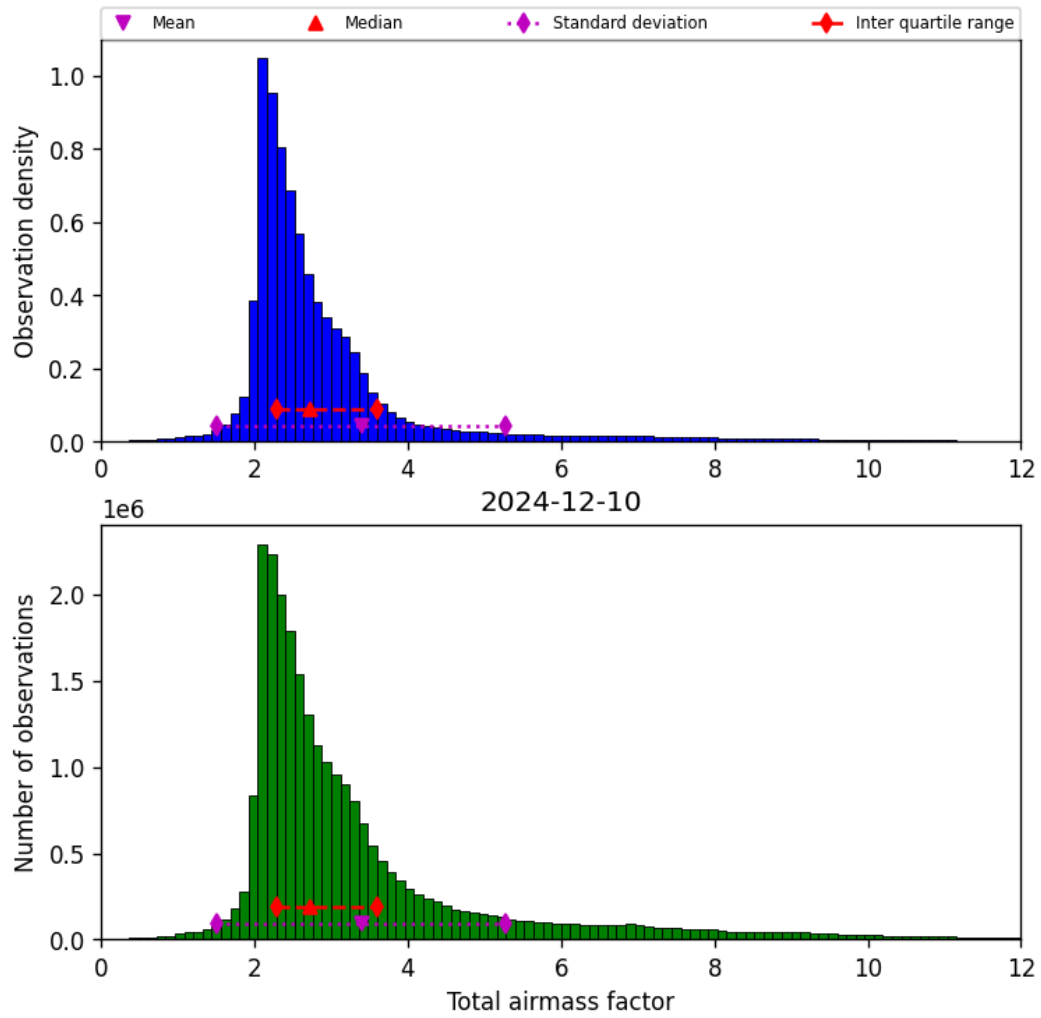
Figure 30: Histogram of “Total airmass factor” for 2024-12-10 to 2024-12-11
