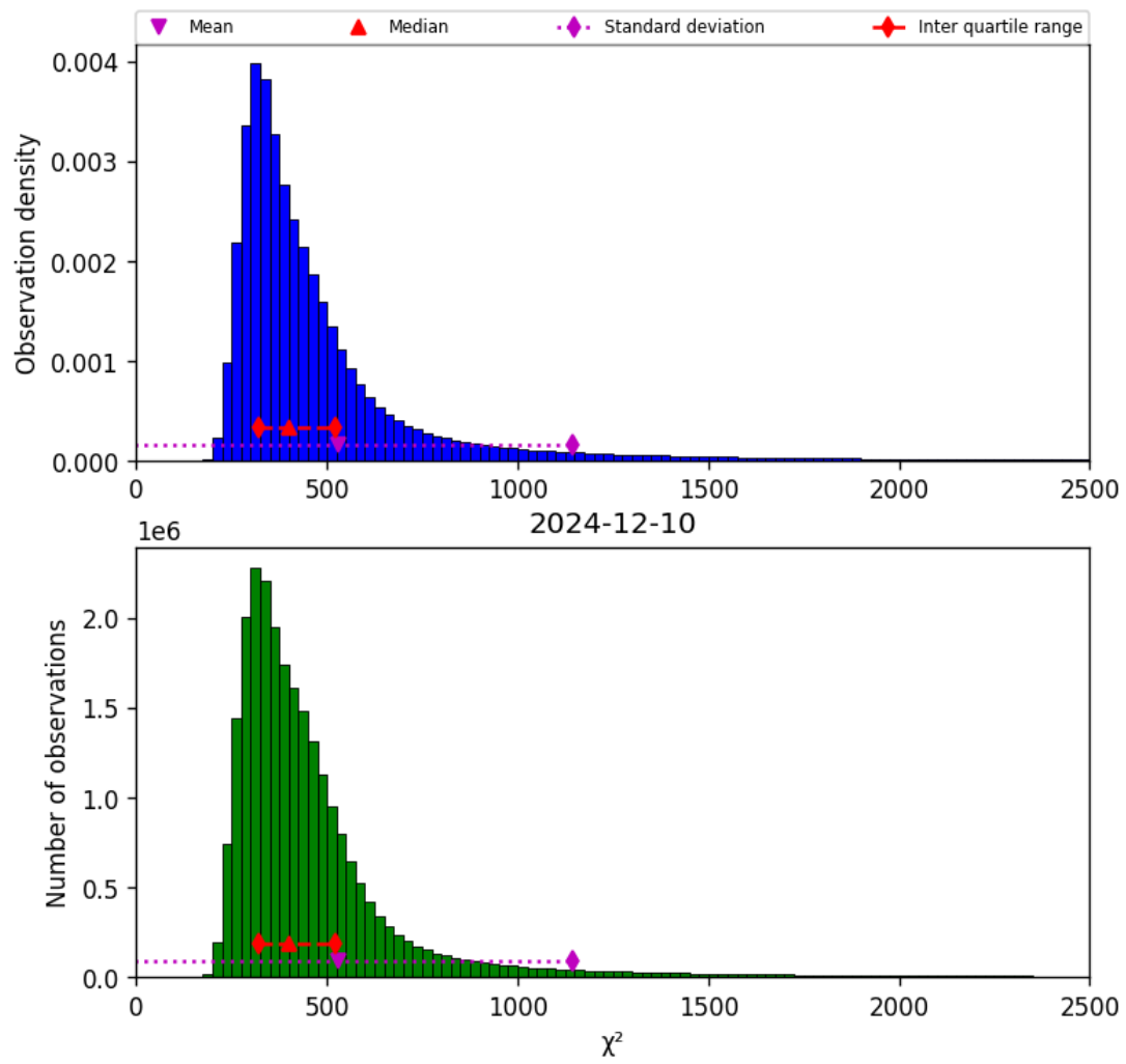
Figure 40: Histogram of “ \chi^2 ” for 2024-12-10 to 2024-12-11
