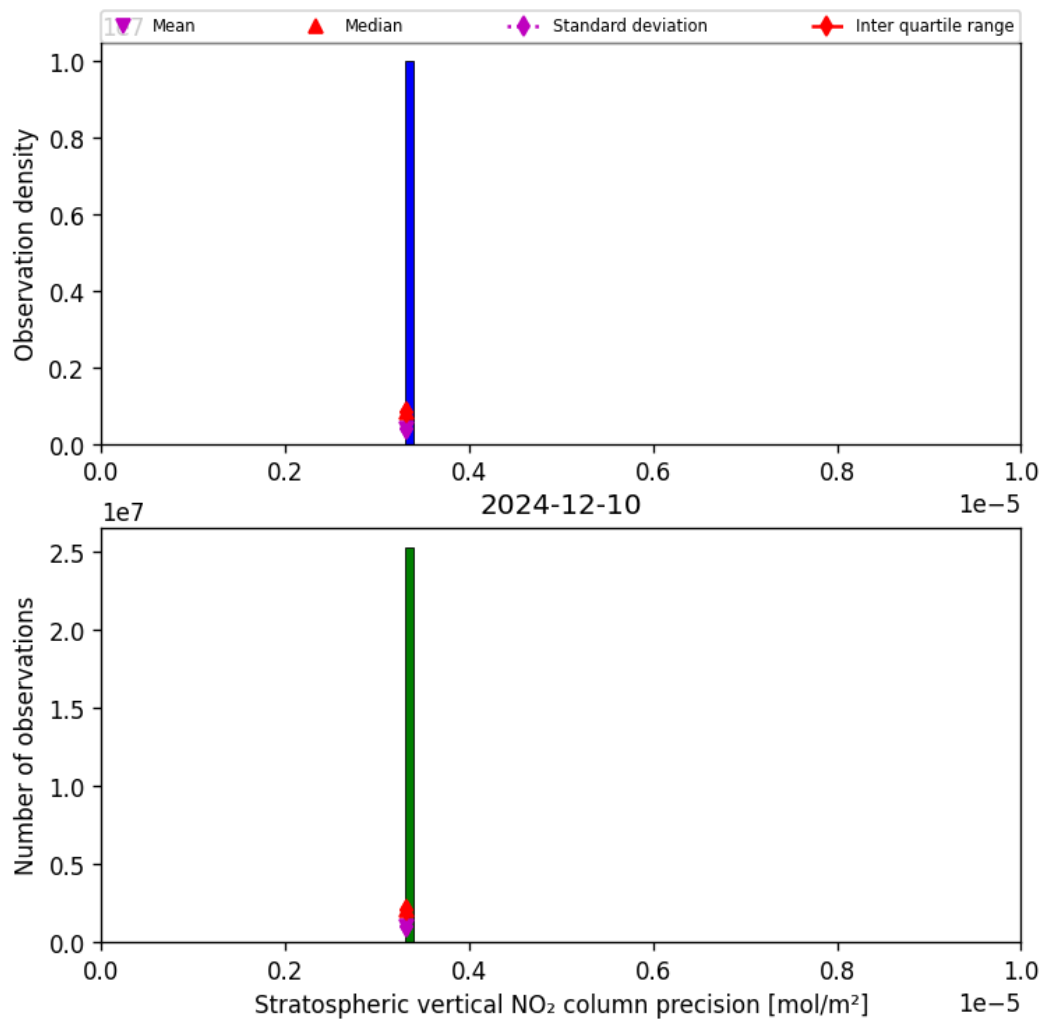
Figure 35: Histogram of “Stratospheric vertical NO 2 column precision” for 2024-12-10 to 2024-12-11
