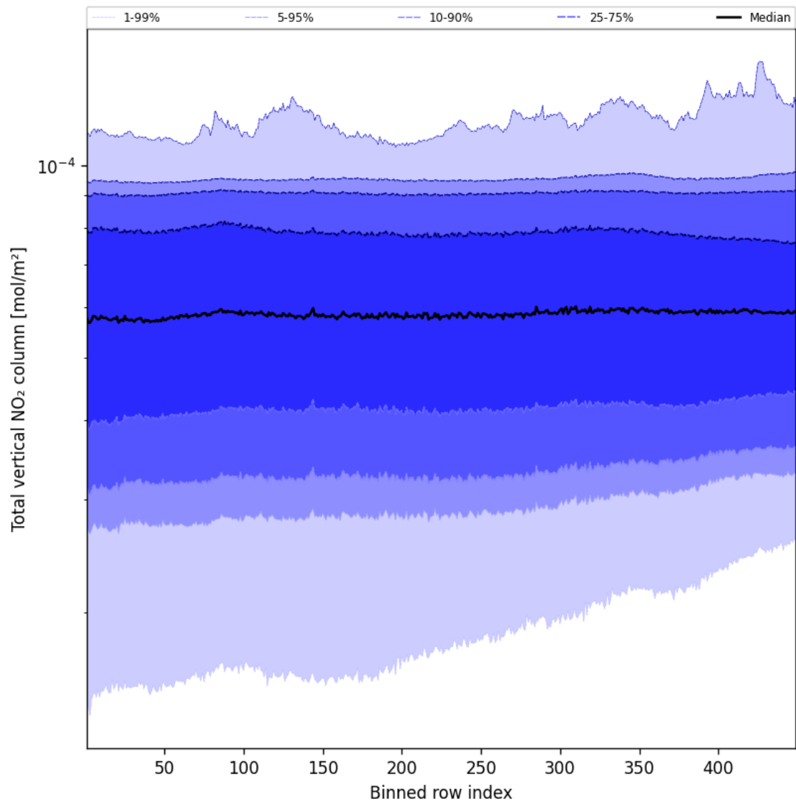
Figure 53: Along track statistics of “Total vertical NO 2 column” for 2024-12-10 to 2024-12-11
