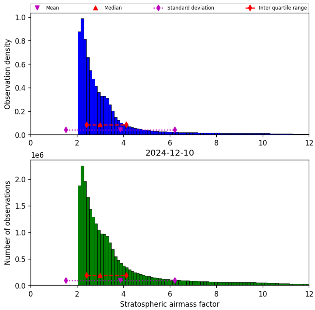
Figure 42: Histogram of “Stratospheric airmass factor” for 2024-12-10 to 2024-12-11
