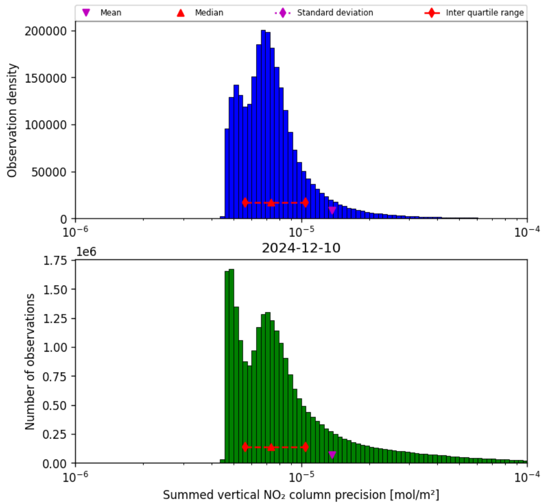
Figure 39: Histogram of “Summed vertical NO 2 column precision” for 2024-12-10 to 2024-12-11
