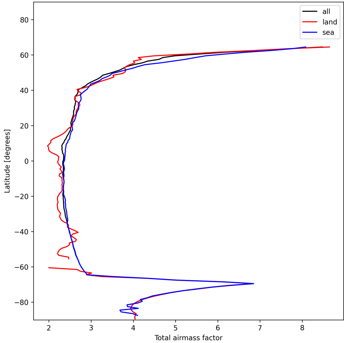
Figure 13: Zonal average of “Total airmass factor” for 2024-12-11 to 2024-12-12.
