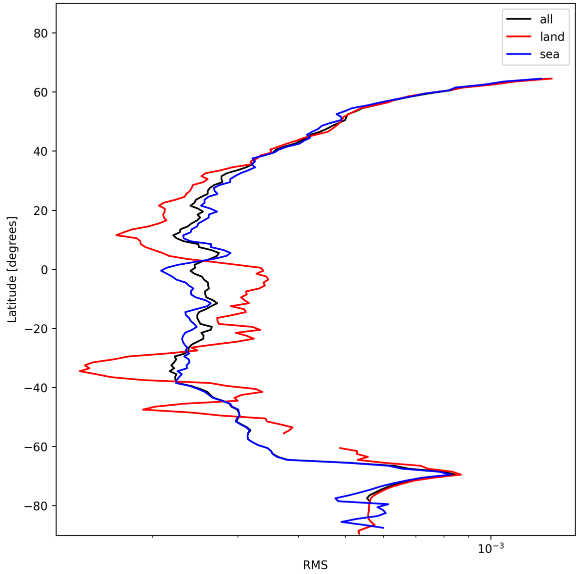
Figure 24: Zonal average of “RMS” for 2024-12-11 to 2024-12-12.
