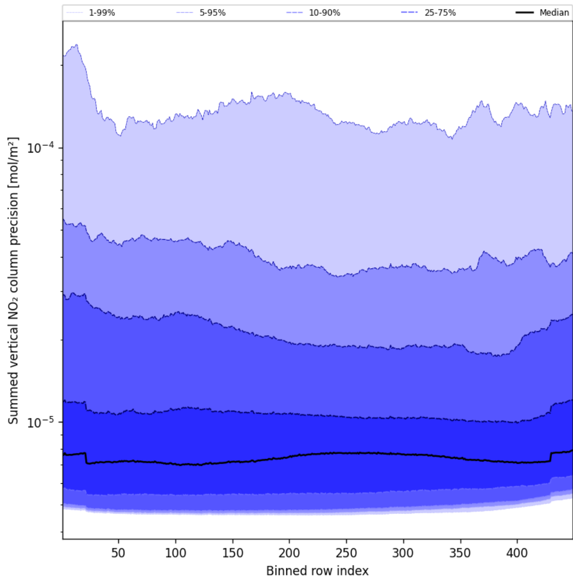
Figure 56: Along track statistics of “Summed vertical NO 2 column precision” for 2024-12-11 to 2024-12-12
