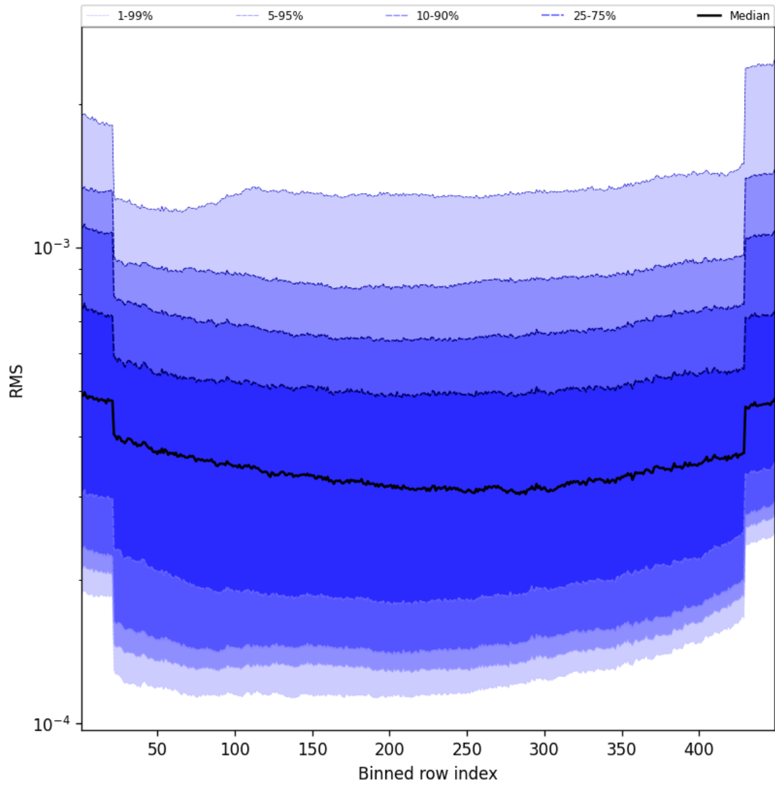
Figure 58: Along track statistics of “RMS” for 2024-12-11 to 2024-12-12
