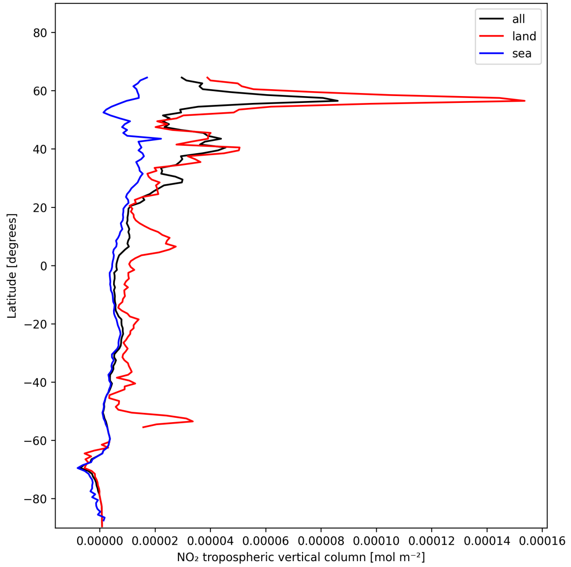
Figure 10: Zonal average of “NO 2 tropospheric vertical column” for 2024-12-11 to 2024-12-12.
