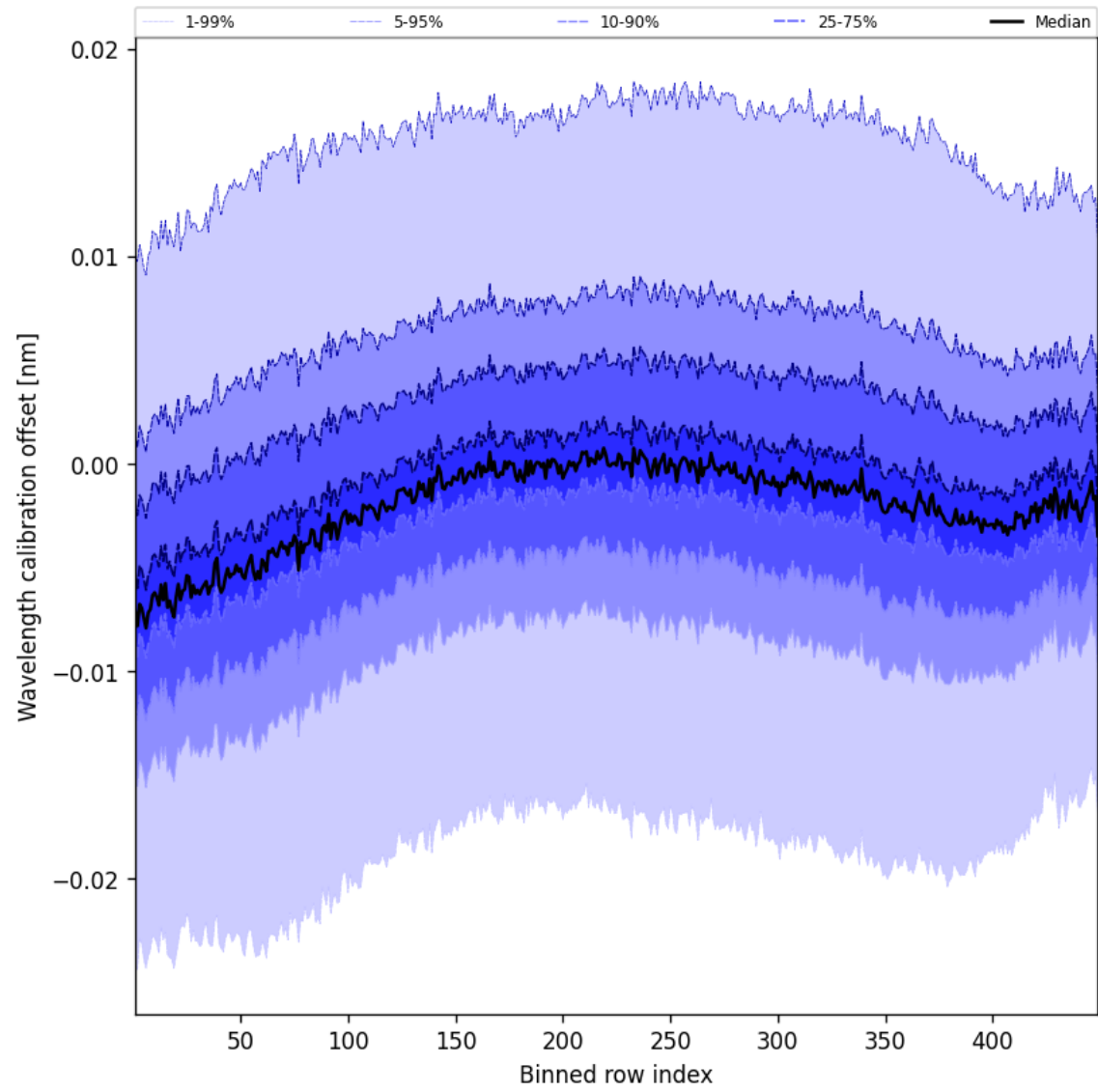
Figure 50: Along track statistics of “Wavelength calibration offset” for 2024-12-11 to 2024-12-12
