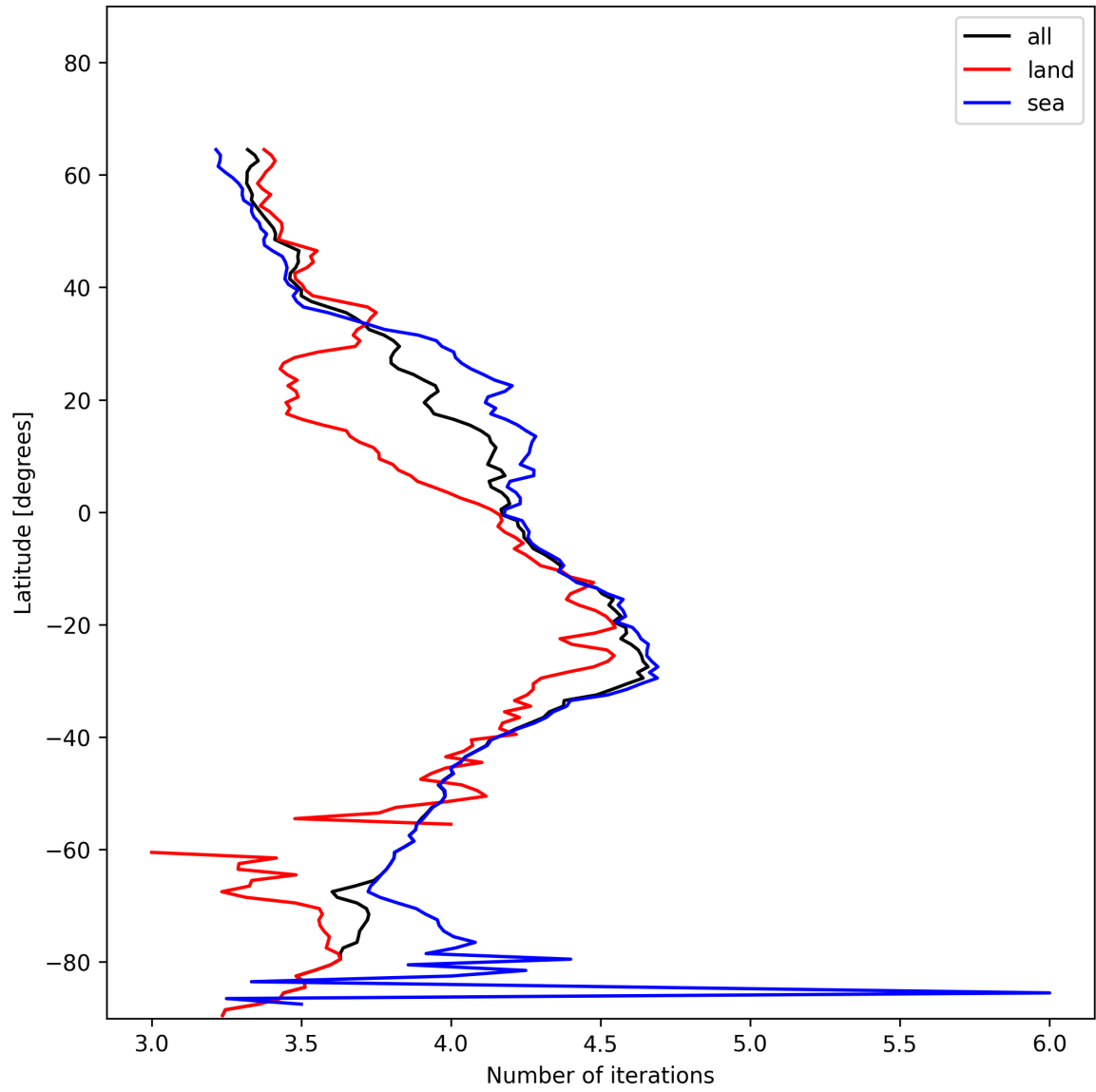
Figure 15: Zonal average of “Number of iterations” for 2024-12-11 to 2024-12-12.
