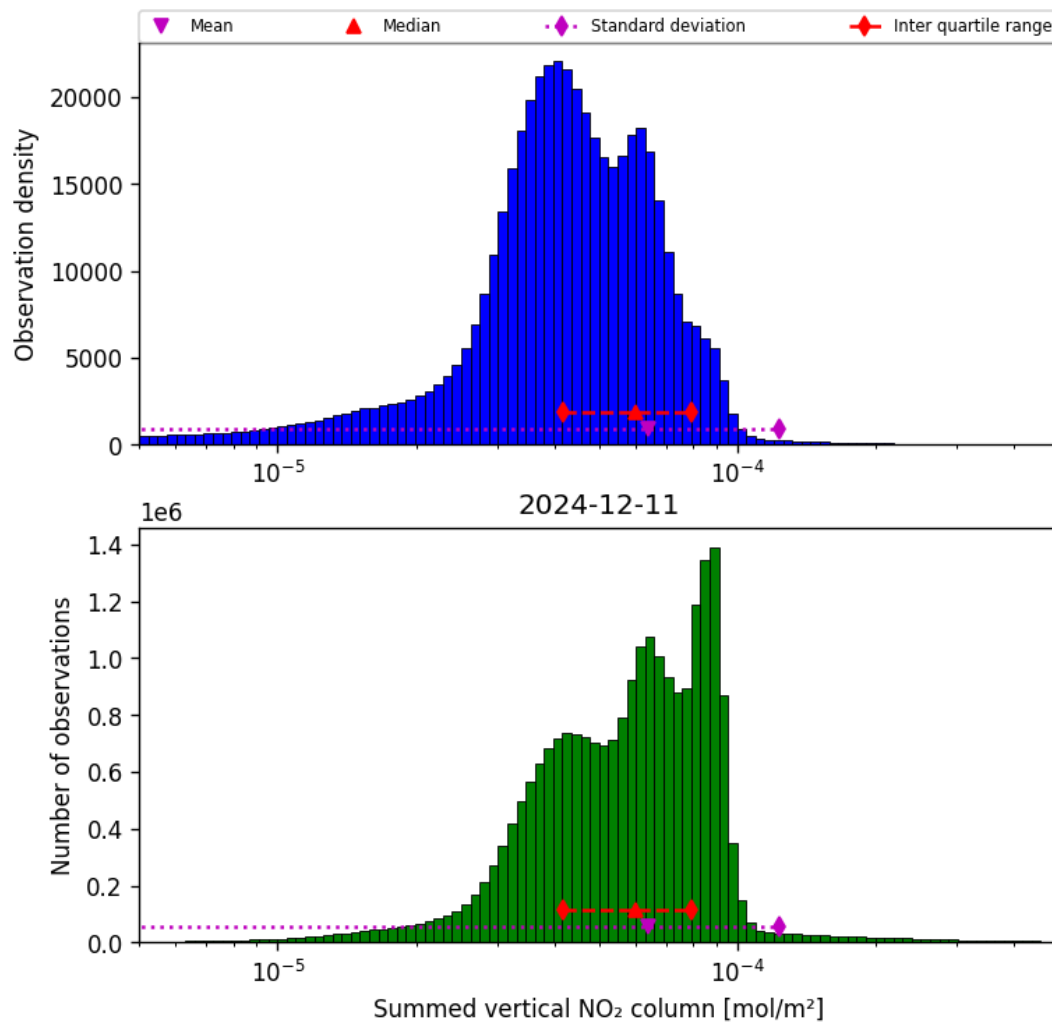
Figure 38: Histogram of “Summed vertical NO 2 column” for 2024-12-11 to 2024-12-12
