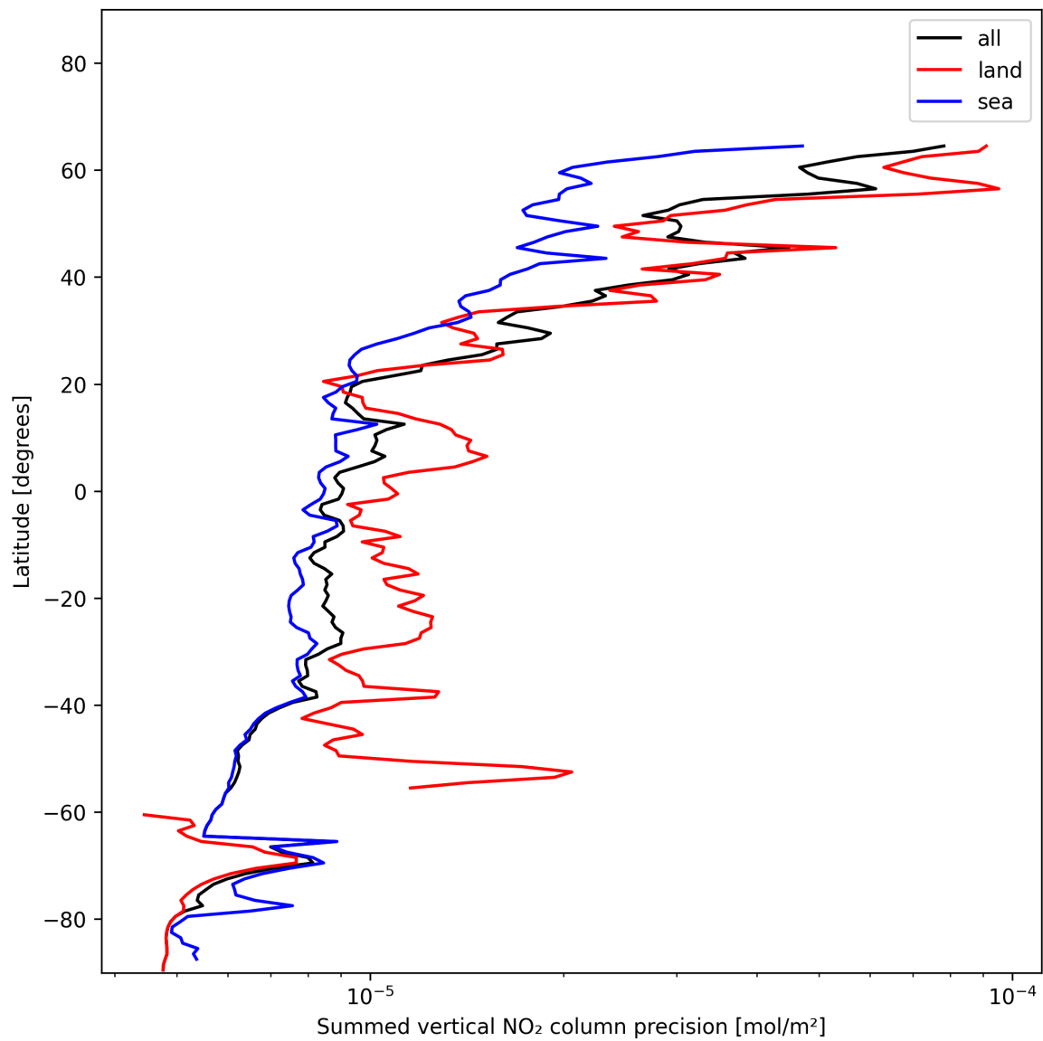
Figure 22: Zonal average of “Summed vertical NO 2 column precision” for 2024-12-11 to 2024-12-12.
