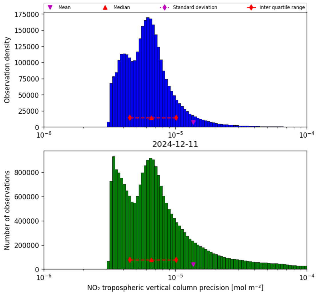
Figure 28: Histogram of “NO 2 tropospheric vertical column precision” for 2024-12-11 to 2024-12-12
