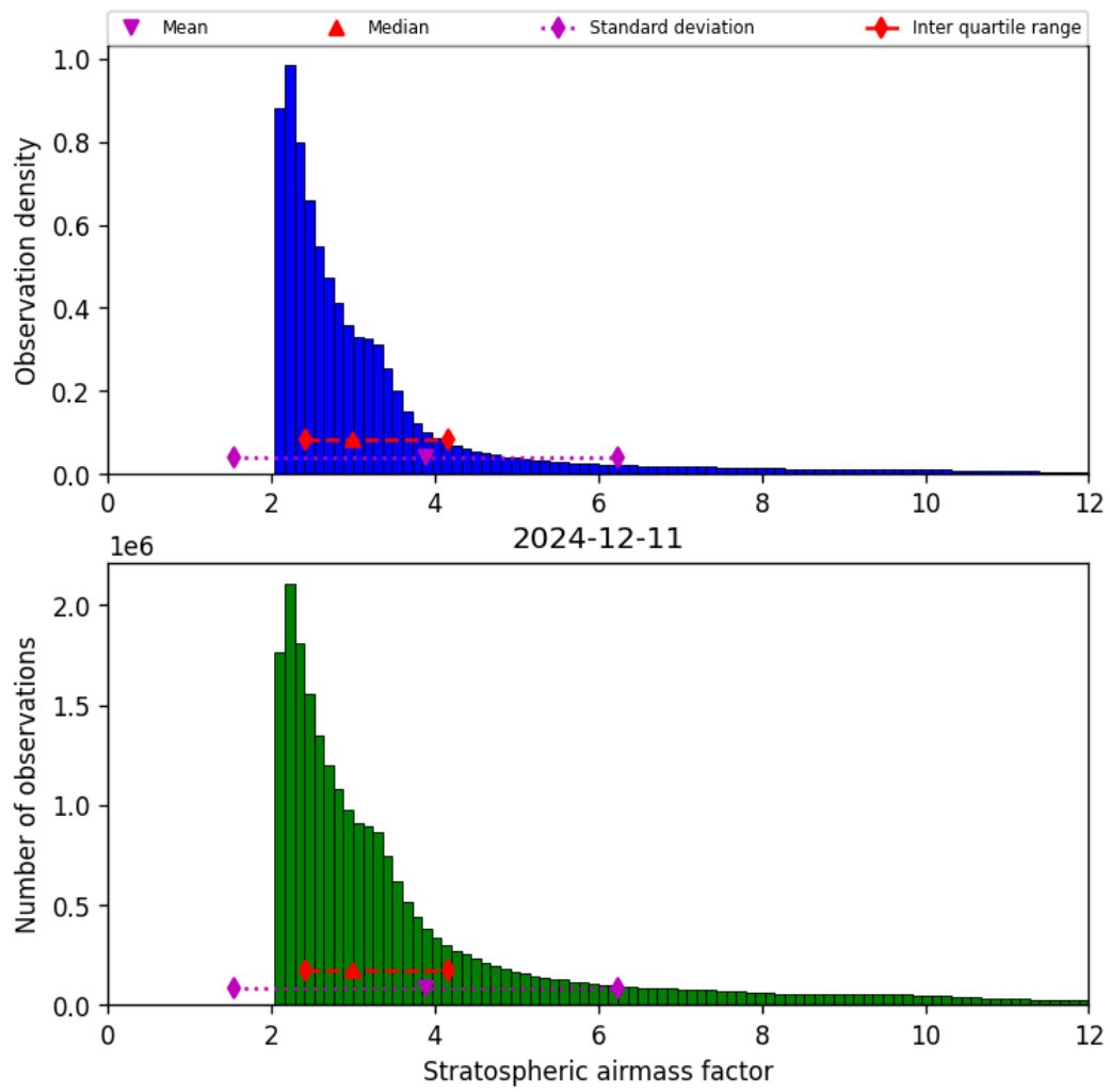
Figure 42: Histogram of “Stratospheric airmass factor” for 2024-12-11 to 2024-12-12
