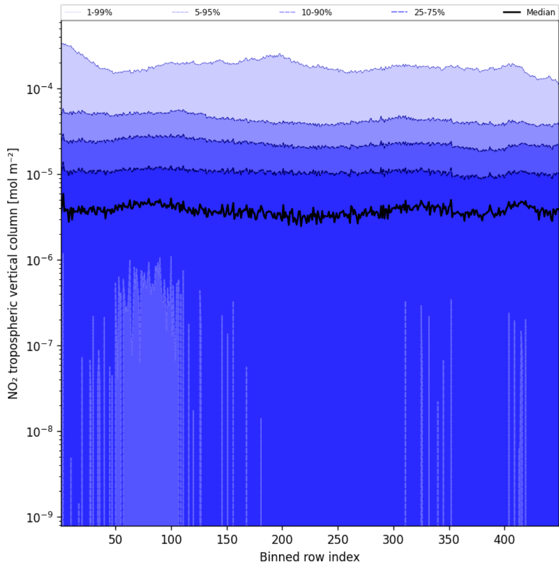
Figure 44: Along track statistics of “NO 2 tropospheric vertical column” for 2024-12-11 to 2024-12-12
