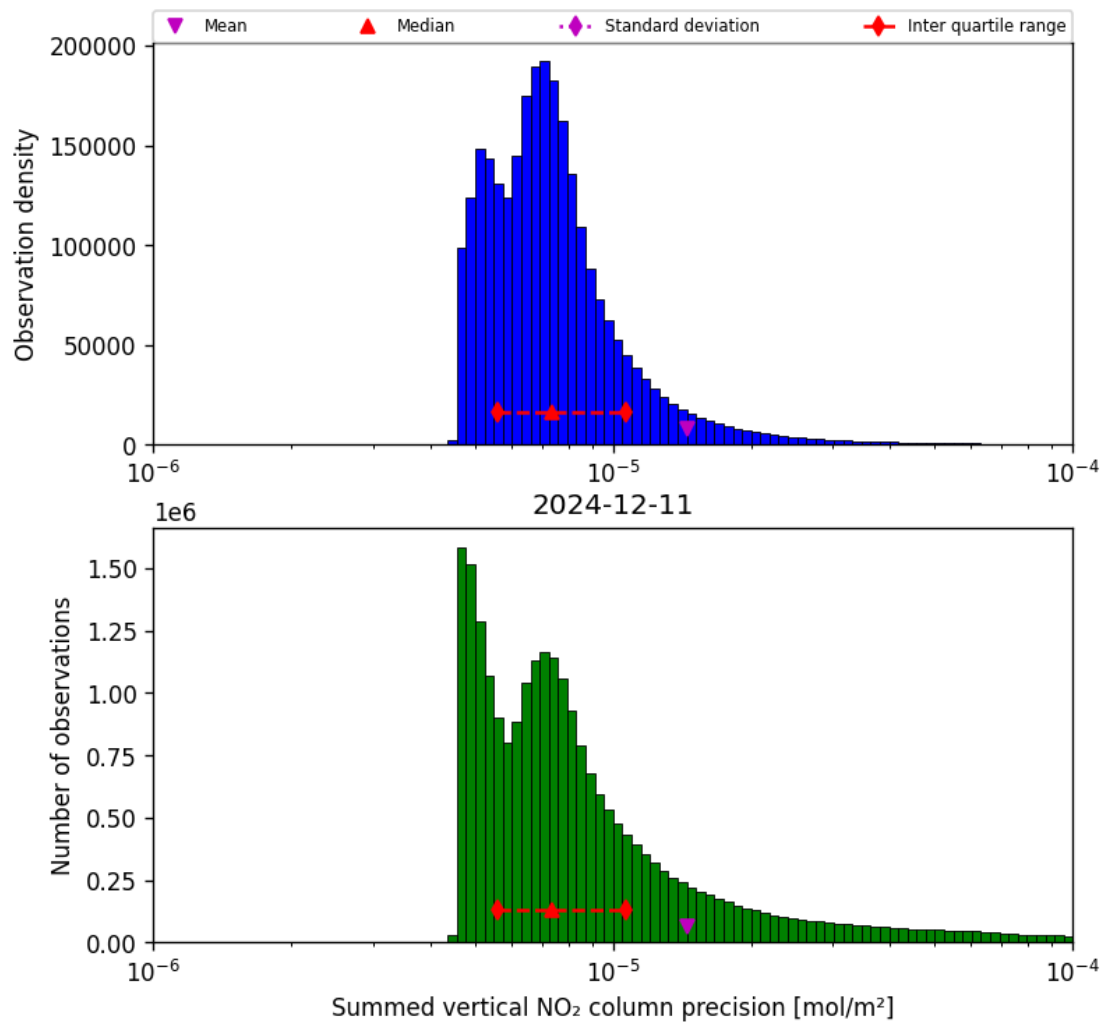
Figure 39: Histogram of “Summed vertical NO 2 column precision” for 2024-12-11 to 2024-12-12
