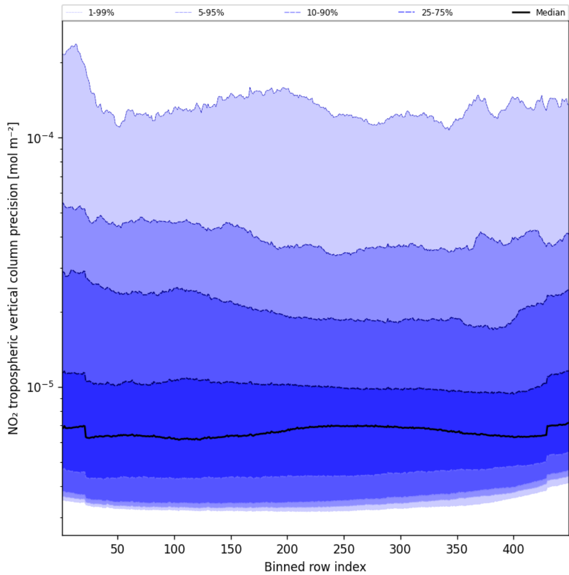
Figure 45: Along track statistics of “NO 2 tropospheric vertical column precision” for 2024-12-11 to 2024-12-12
