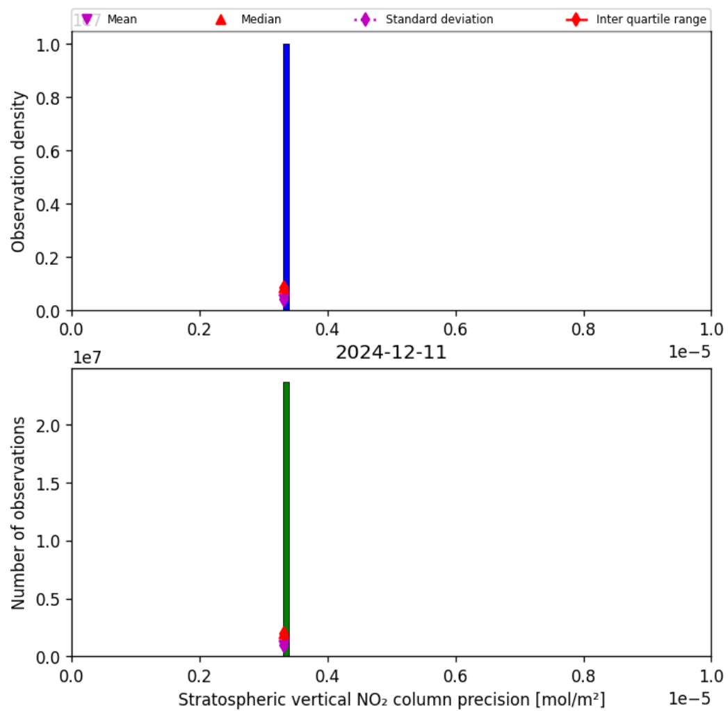
Figure 35: Histogram of “Stratospheric vertical NO 2 column precision” for 2024-12-11 to 2024-12-12
