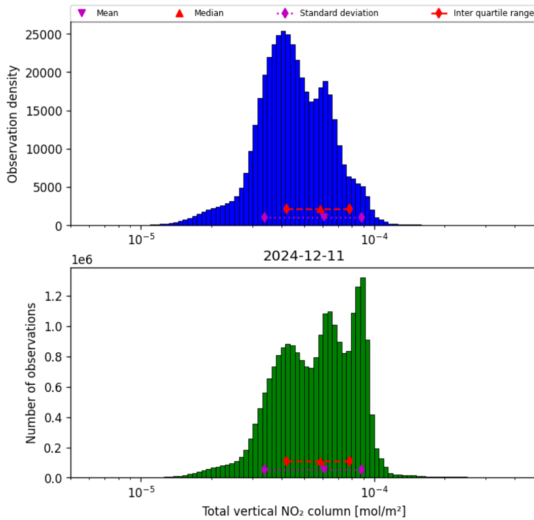
Figure 36: Histogram of “Total vertical NO 2 column” for 2024-12-11 to 2024-12-12
