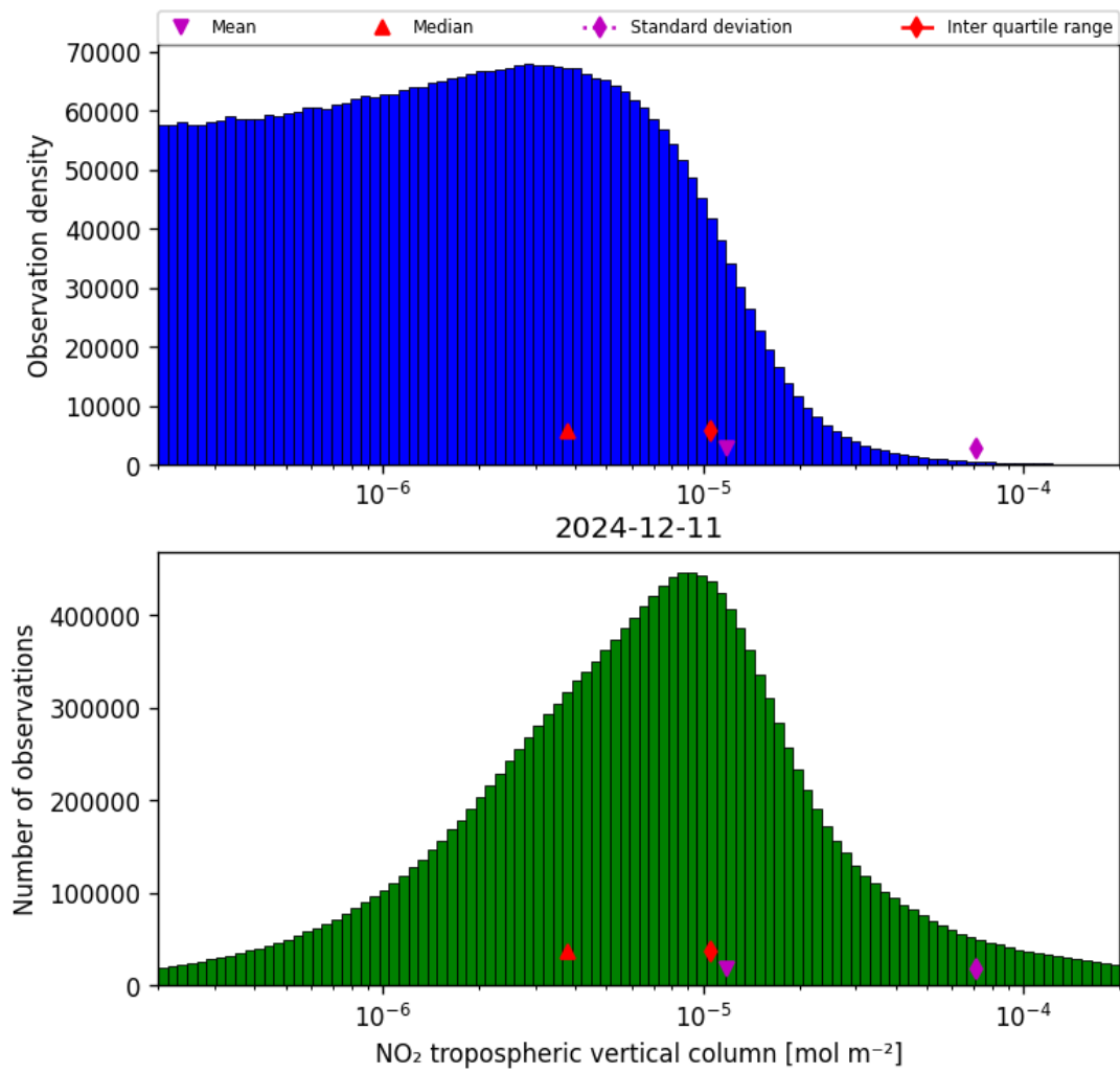
Figure 27: Histogram of “NO 2 tropospheric vertical column” for 2024-12-11 to 2024-12-12
