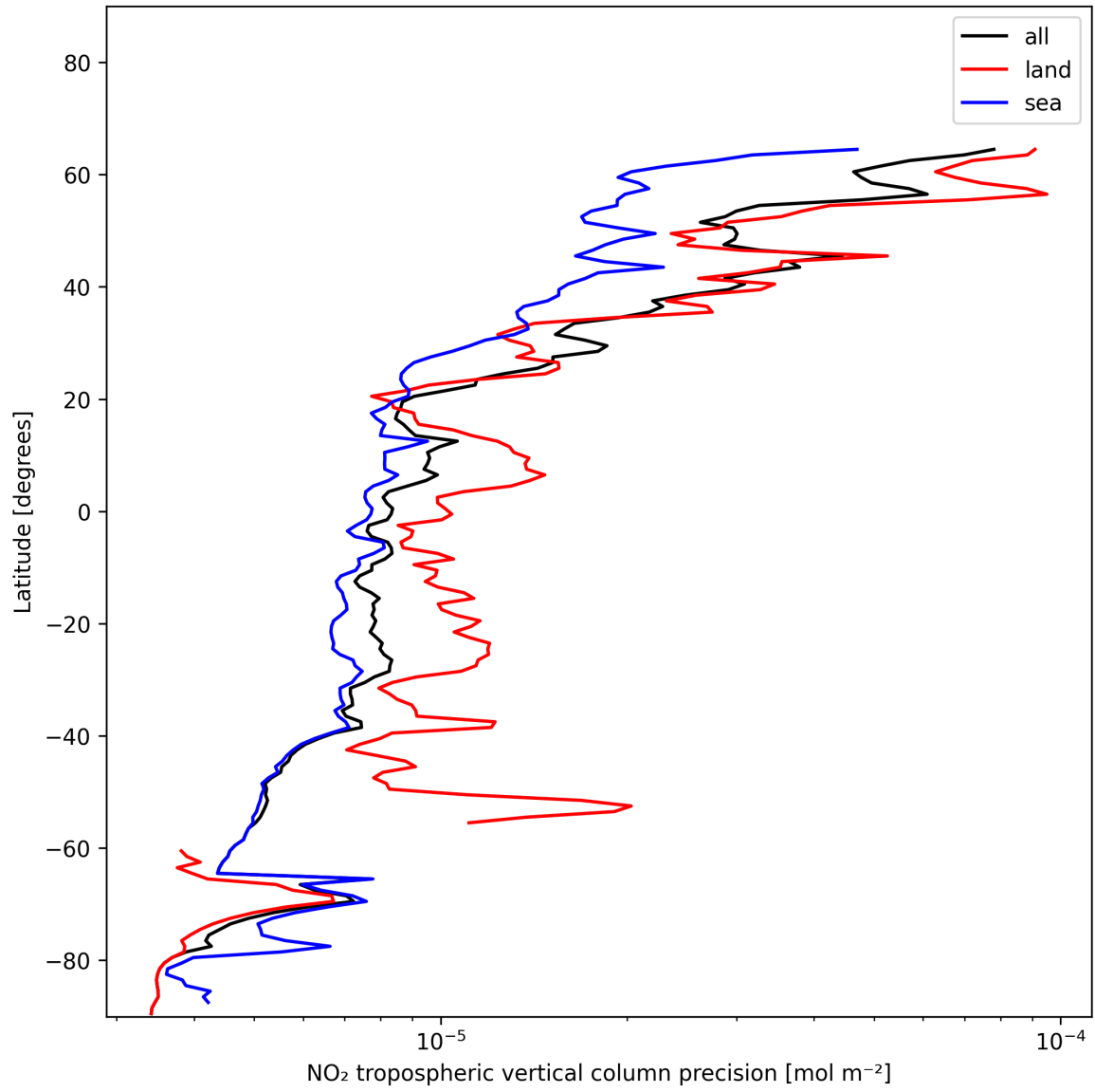
Figure 11: Zonal average of “NO 2 tropospheric vertical column precision” for 2024-12-11 to 2024-12-12.
