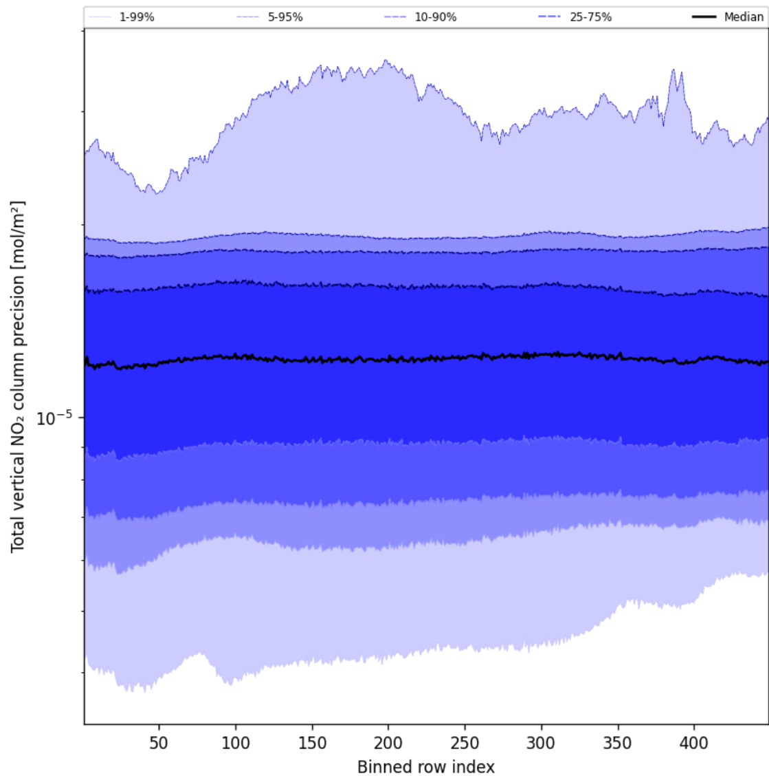
Figure 54: Along track statistics of “Total vertical NO 2 column precision” for 2024-12-11 to 2024-12-12
