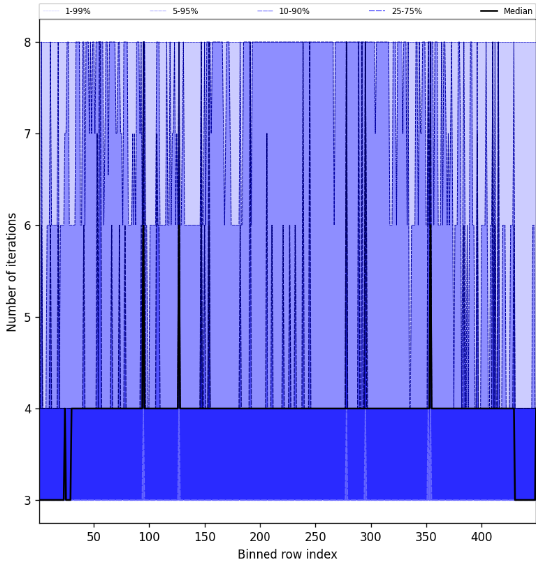
Figure 49: Along track statistics of “Number of iterations” for 2024-12-11 to 2024-12-12
