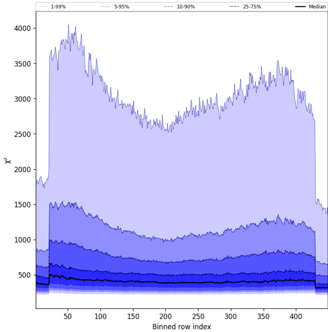
Figure 57: Along track statistics of “ \chi^2 ” for 2024-12-11 to 2024-12-12
