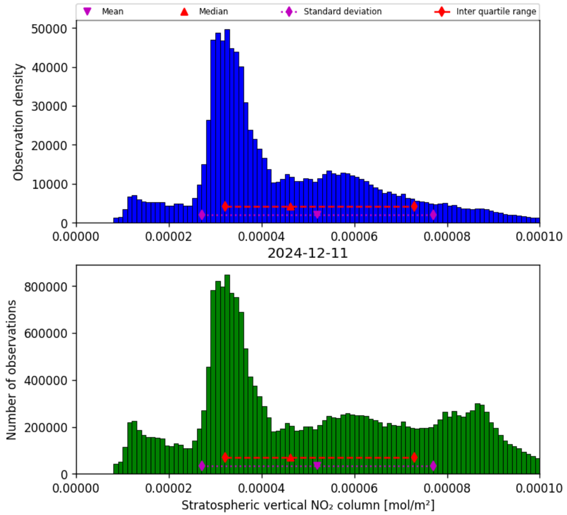
Figure 34: Histogram of “Stratospheric vertical NO 2 column” for 2024-12-11 to 2024-12-12
