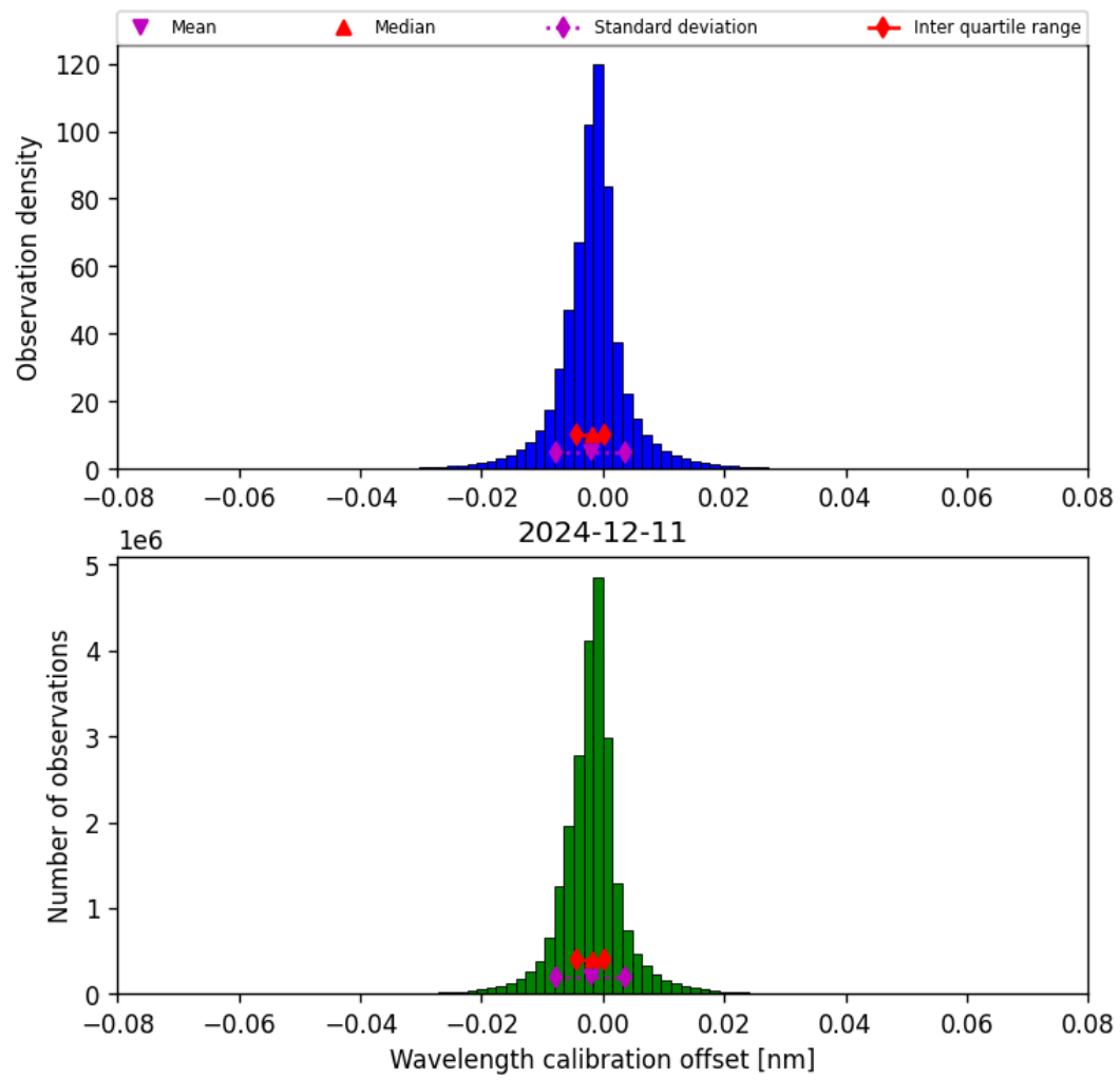
Figure 33: Histogram of “Wavelength calibration offset” for 2024-12-11 to 2024-12-12
