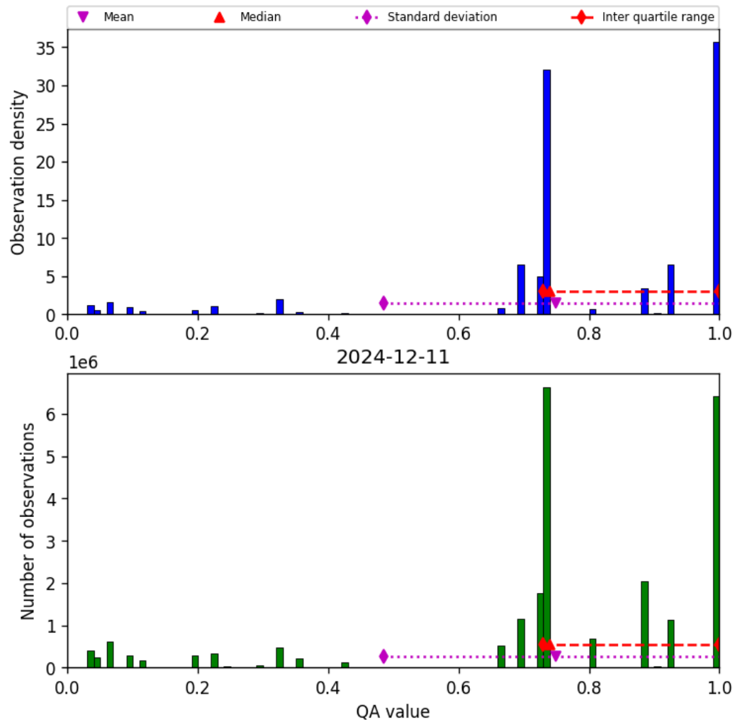
Figure 26: Histogram of “QA value” for 2024-12-11 to 2024-12-12
