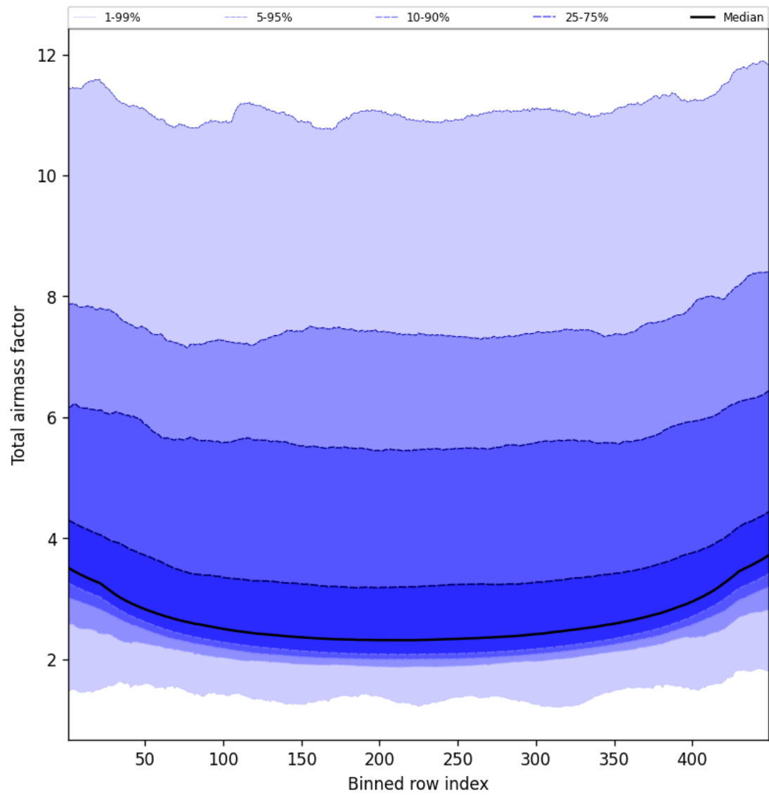
Figure 47: Along track statistics of “Total airmass factor” for 2024-12-11 to 2024-12-12
