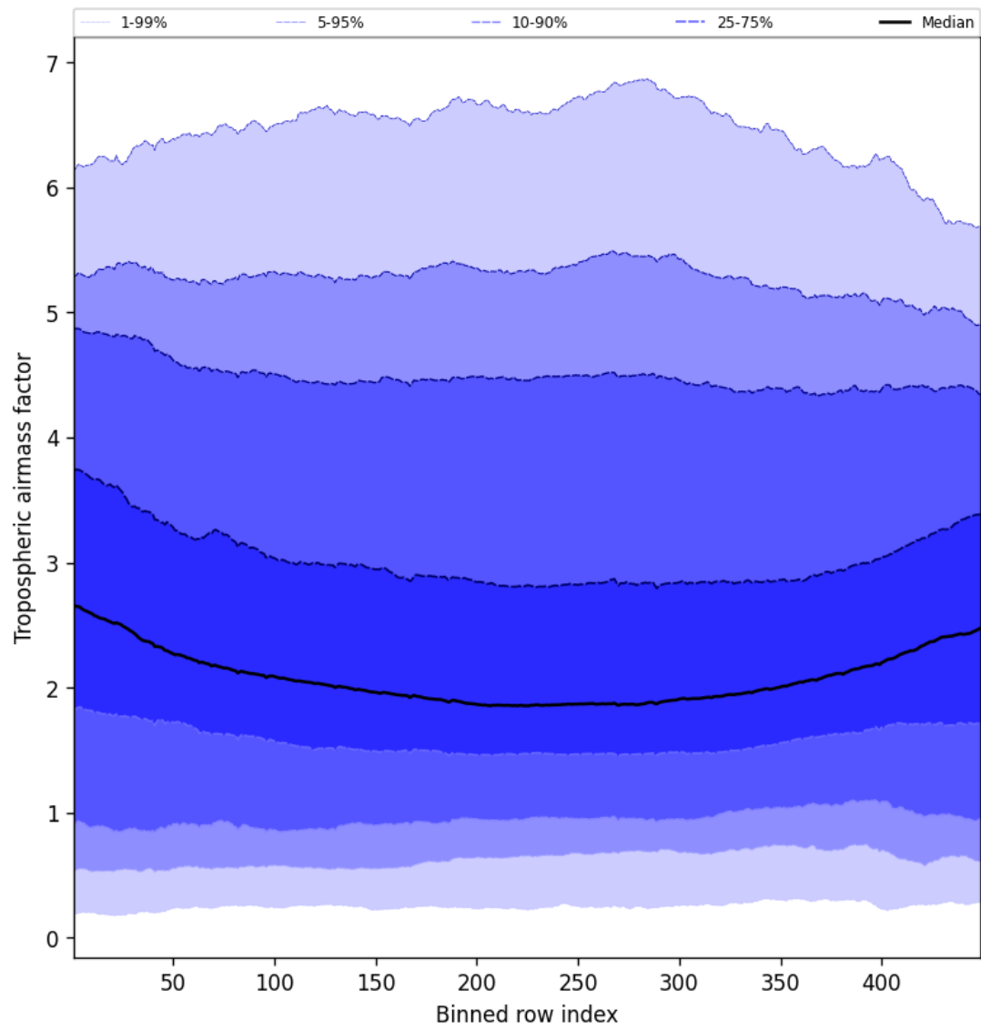
Figure 46: Along track statistics of “Tropospheric airmass factor” for 2024-12-11 to 2024-12-12
