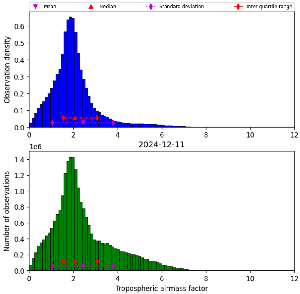
Figure 29: Histogram of “Tropospheric airmass factor” for 2024-12-11 to 2024-12-12
