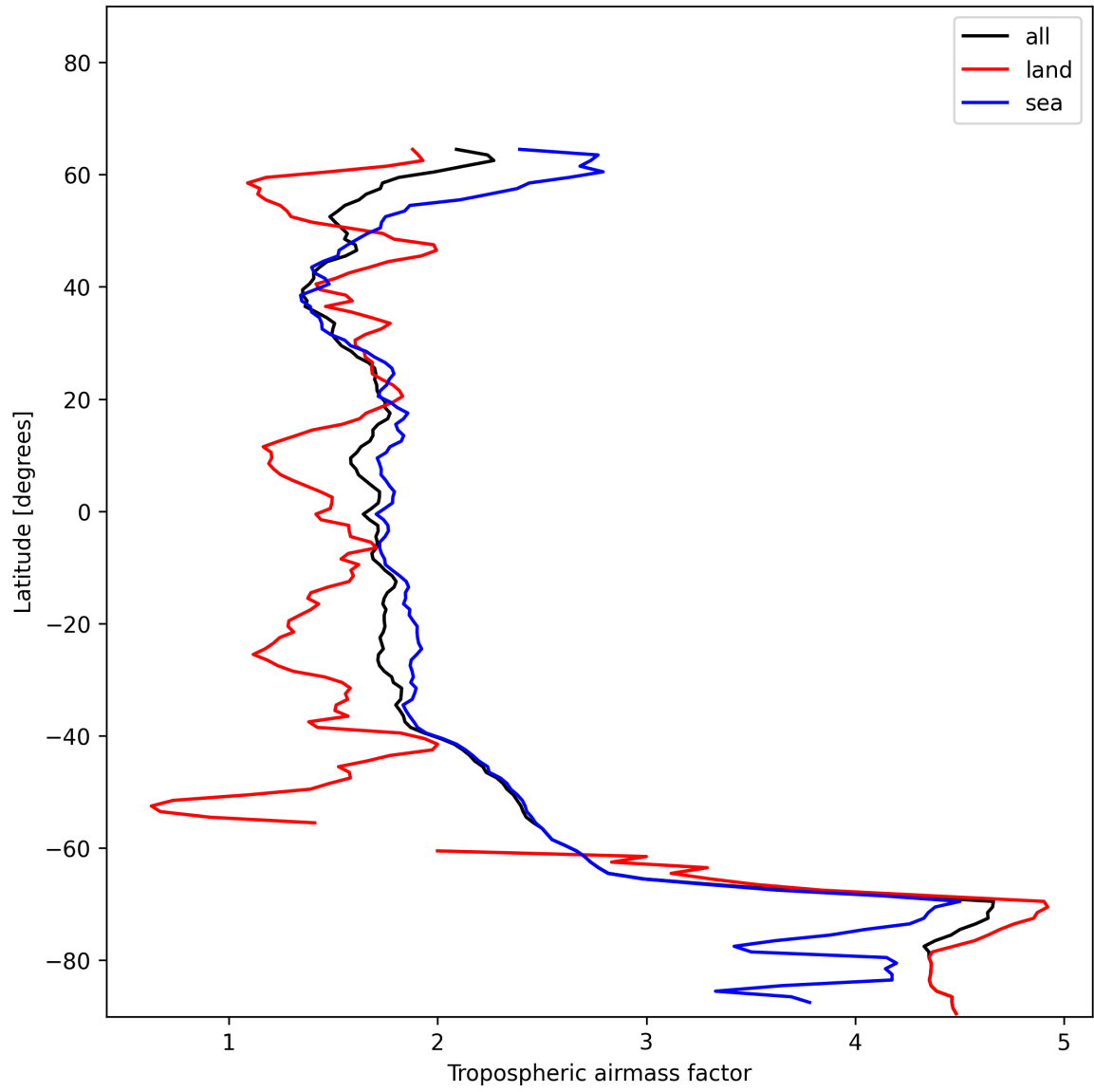
Figure 12: Zonal average of “Tropospheric airmass factor” for 2024-12-11 to 2024-12-12.
