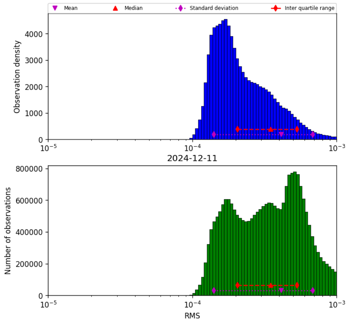
Figure 41: Histogram of “RMS” for 2024-12-11 to 2024-12-12
