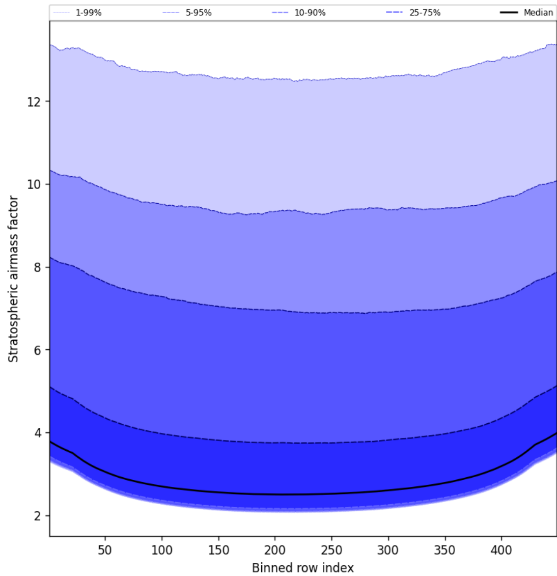
Figure 59: Along track statistics of “Stratospheric airmass factor” for 2024-12-11 to 2024-12-12
