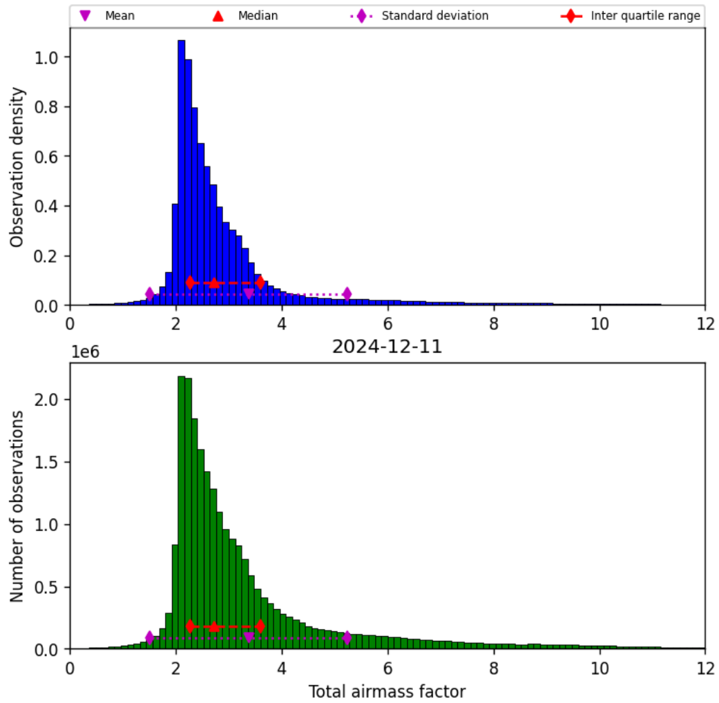
Figure 30: Histogram of “Total airmass factor” for 2024-12-11 to 2024-12-12
