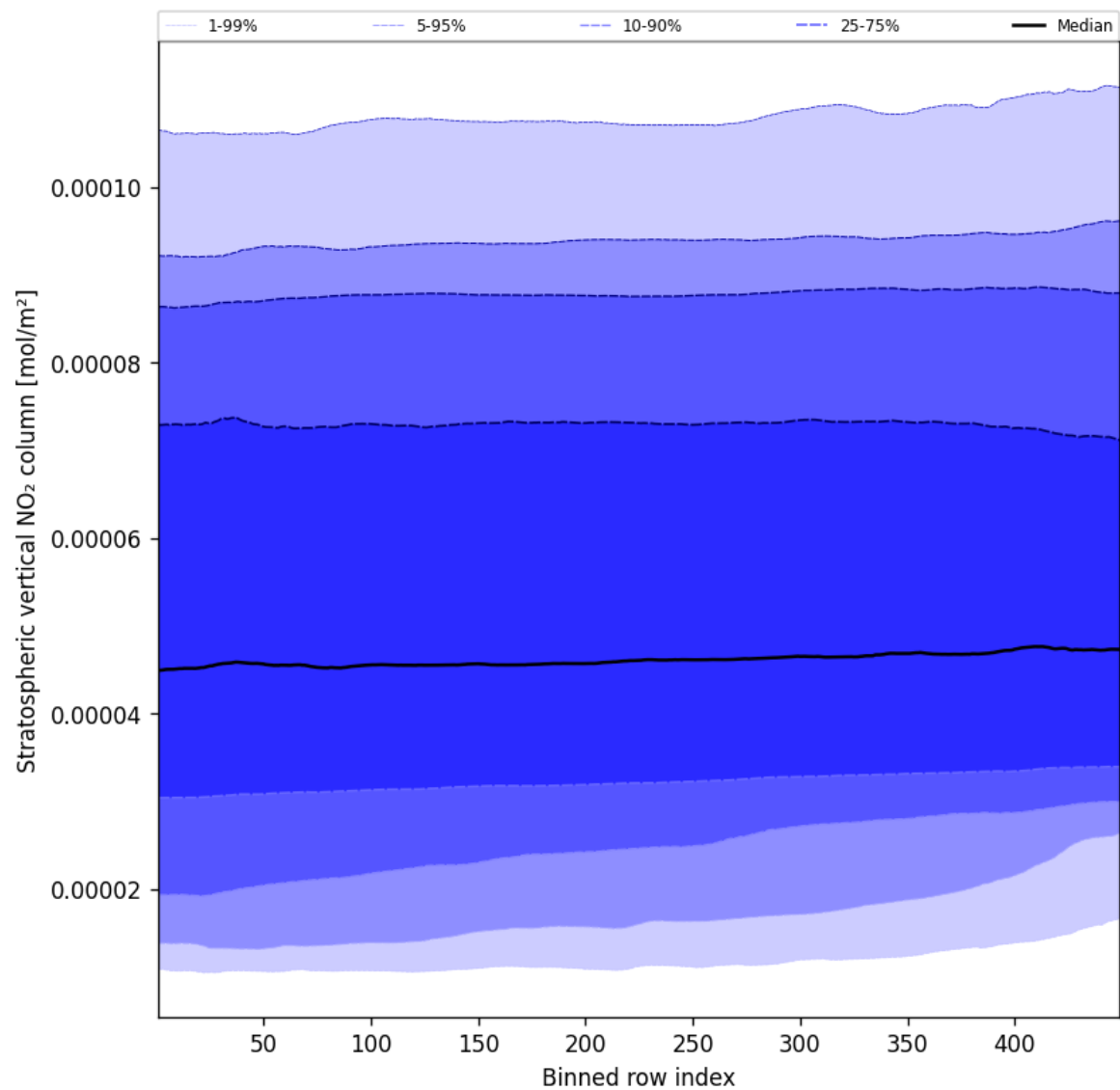
Figure 51: Along track statistics of “Stratospheric vertical NO 2 column” for 2024-12-11 to 2024-12-12
