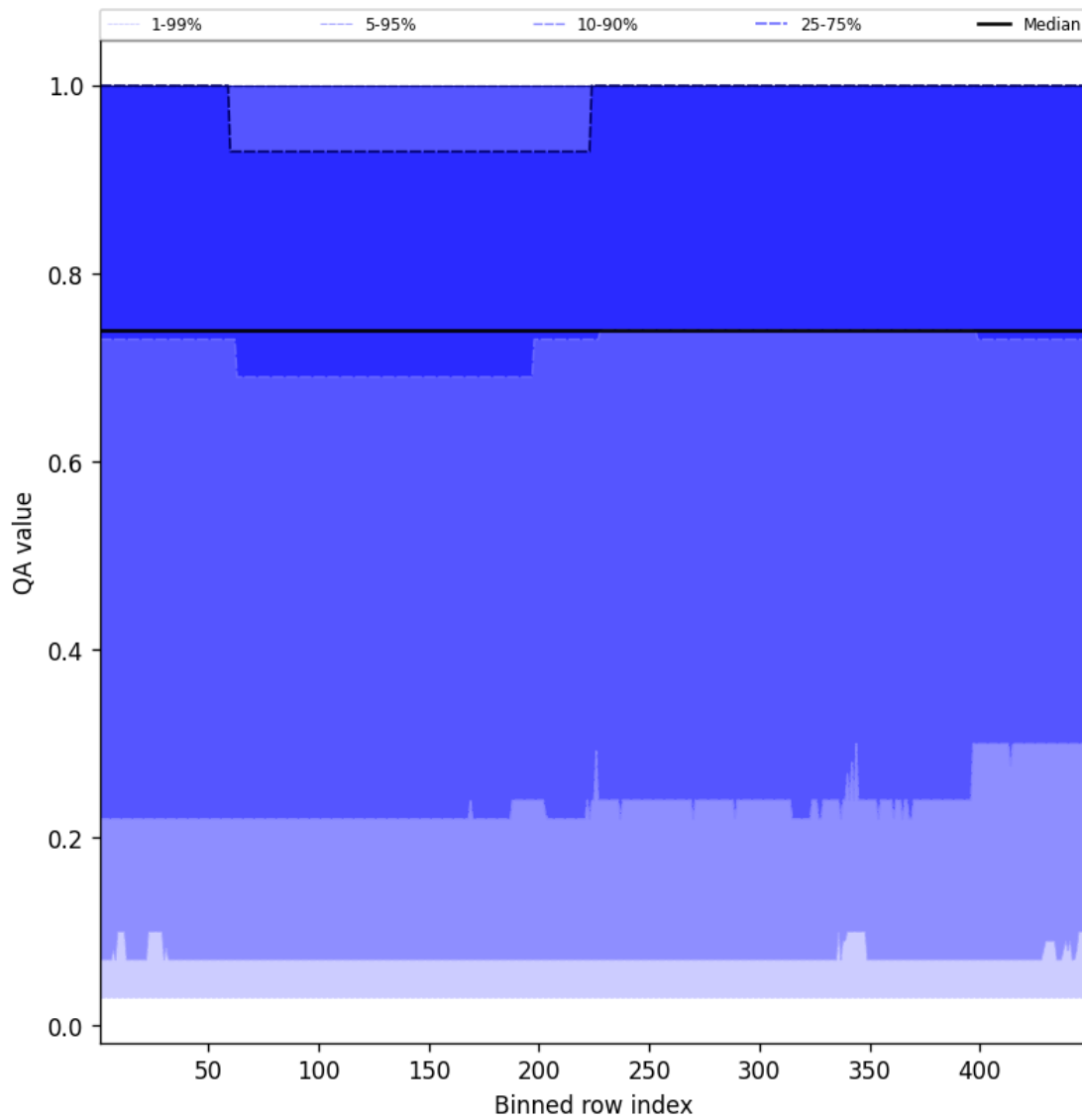
Figure 43: Along track statistics of “QA value” for 2024-12-11 to 2024-12-12
