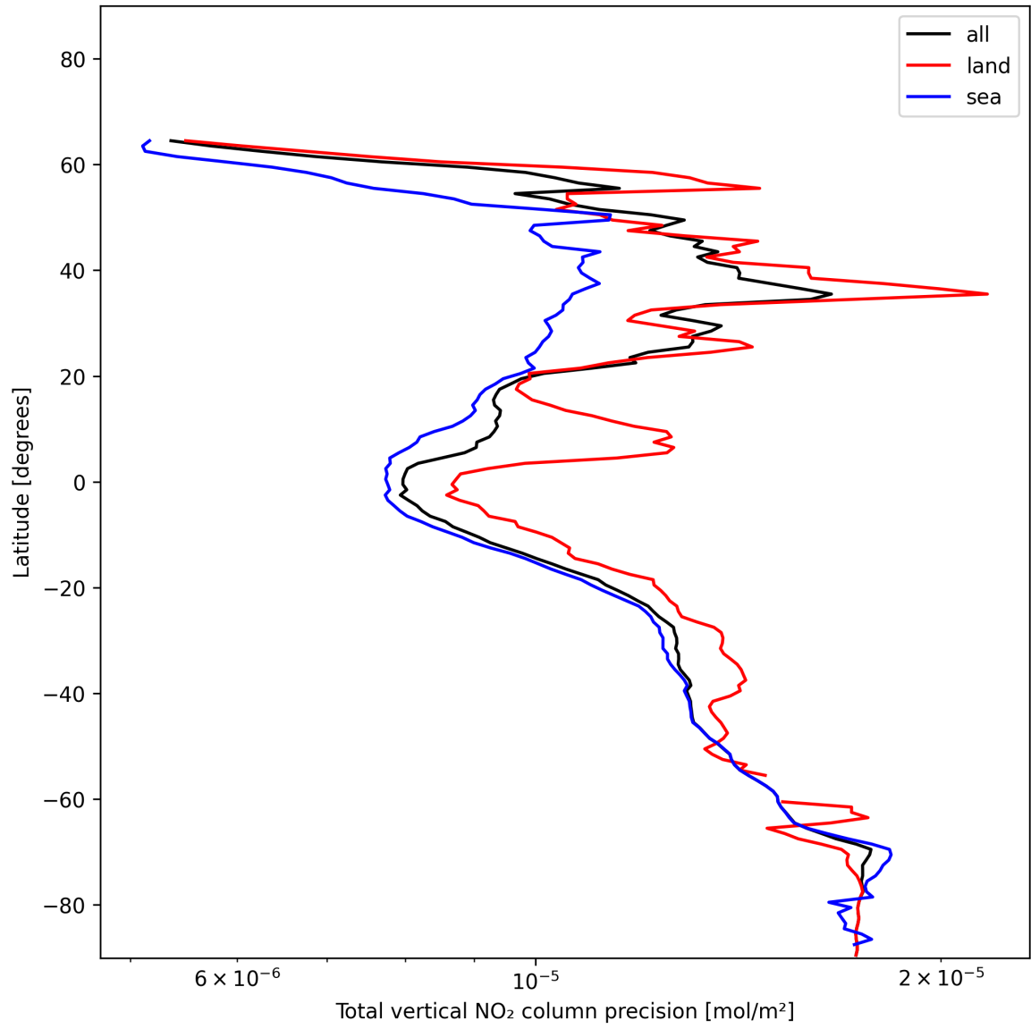
Figure 20: Zonal average of “Total vertical NO 2 column precision” for 2024-12-11 to 2024-12-12.
