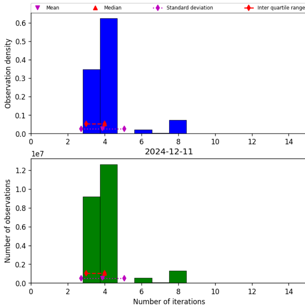
Figure 32: Histogram of “Number of iterations” for 2024-12-11 to 2024-12-12
