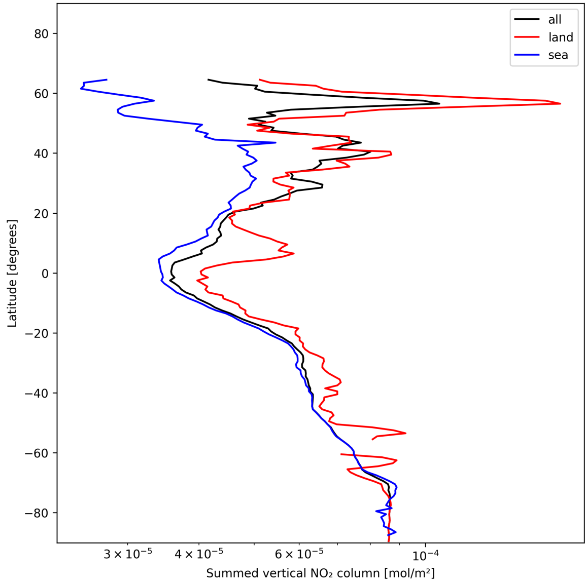
Figure 21: Zonal average of “Summed vertical NO 2 column” for 2024-12-11 to 2024-12-12.
