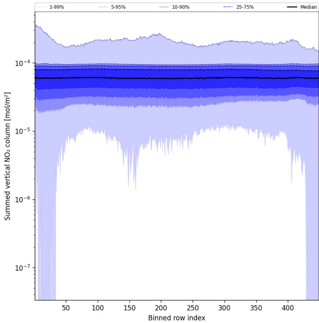
Figure 55: Along track statistics of “Summed vertical NO 2 column” for 2024-12-11 to 2024-12-12
