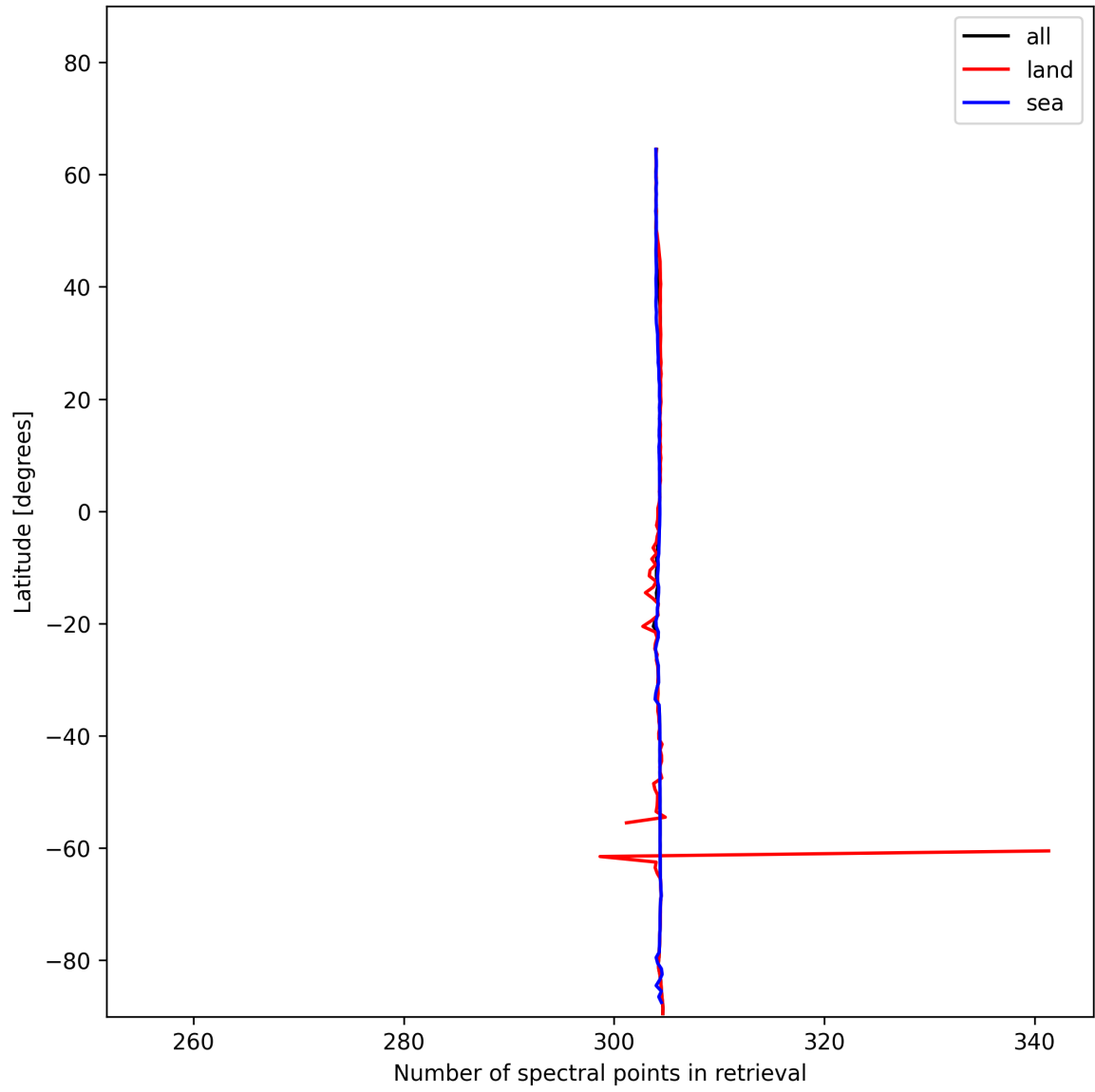
Figure 14: Zonal average of “Number of spectral points in retrieval” for 2024-12-11 to 2024-12-12.
