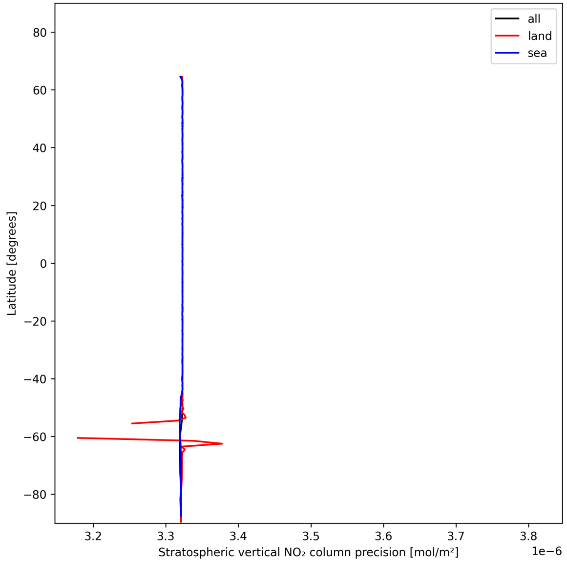
Figure 18: Zonal average of “Stratospheric vertical NO 2 column precision” for 2024-12-11 to 2024-12-12.
