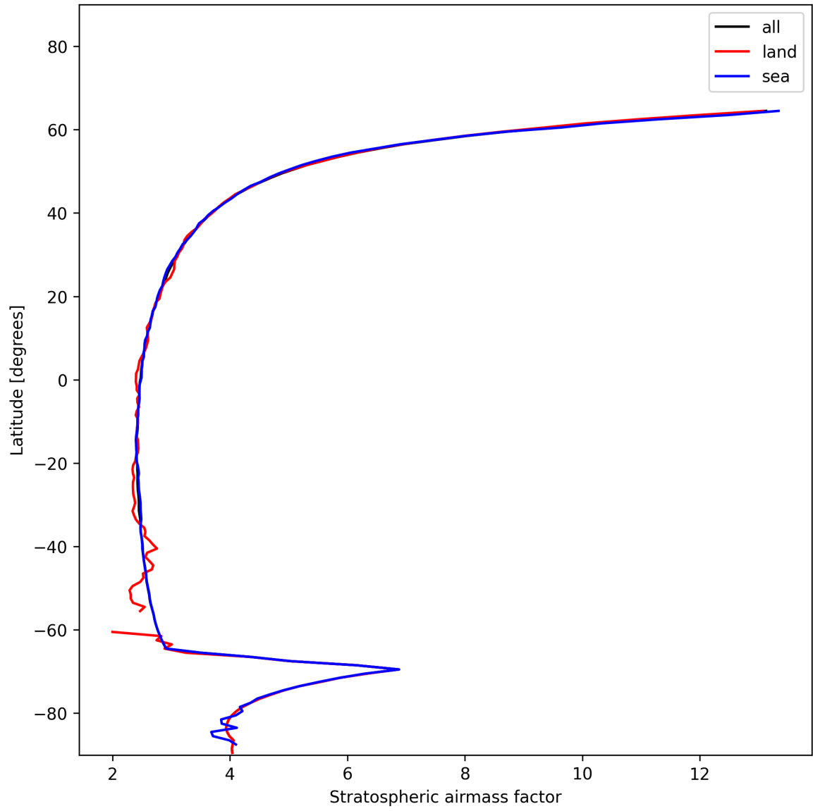
Figure 25: Zonal average of “Stratospheric airmass factor” for 2024-12-11 to 2024-12-12.
