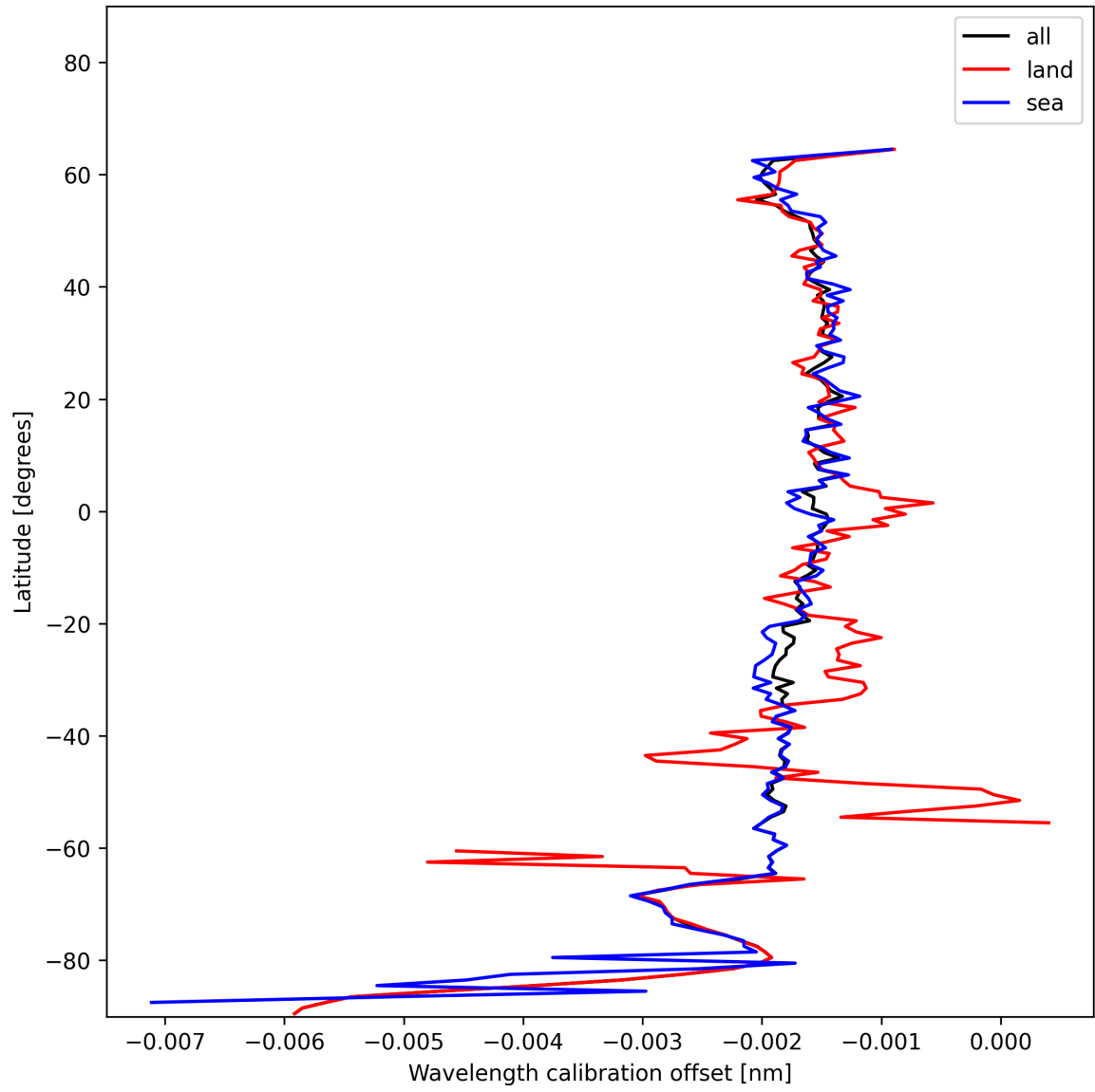
Figure 16: Zonal average of “Wavelength calibration offset” for 2024-12-11 to 2024-12-12.
