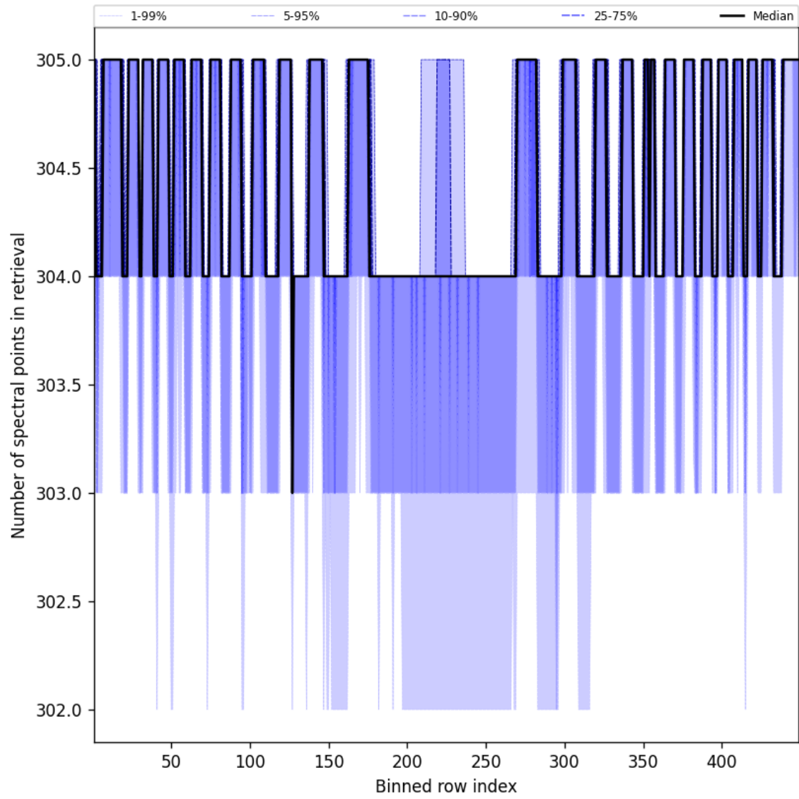
Figure 48: Along track statistics of “Number of spectral points in retrieval” for 2024-12-11 to 2024-12-12
