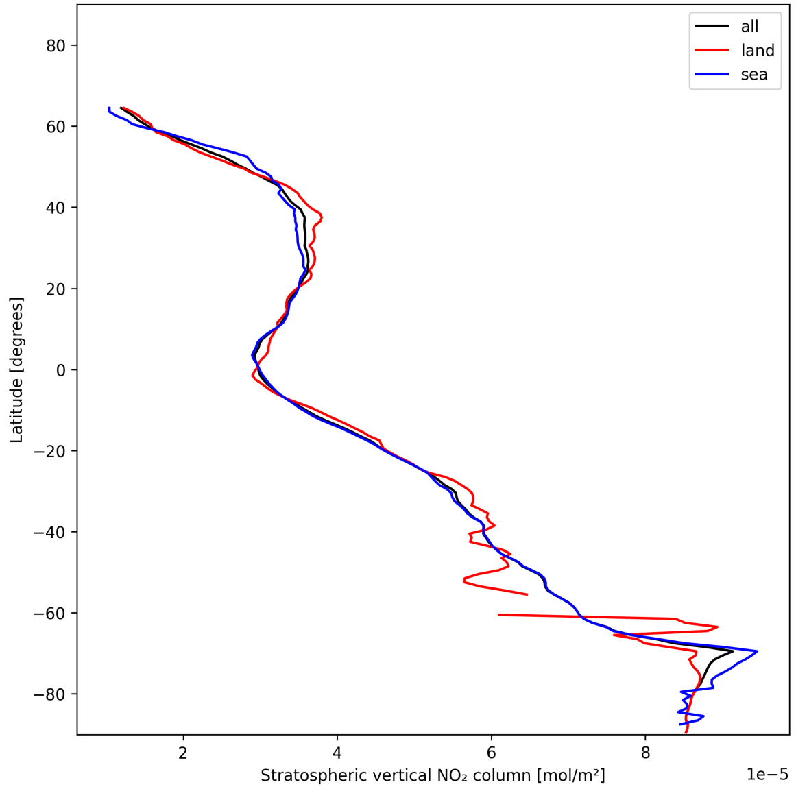
Figure 17: Zonal average of “Stratospheric vertical NO 2 column” for 2024-12-11 to 2024-12-12.
