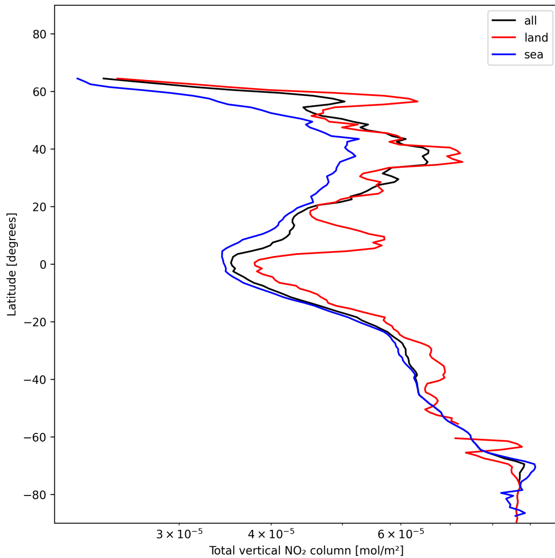
Figure 19: Zonal average of “Total vertical NO 2 column” for 2024-12-11 to 2024-12-12.
