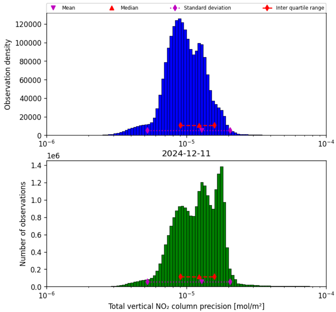
Figure 37: Histogram of “Total vertical NO 2 column precision” for 2024-12-11 to 2024-12-12
