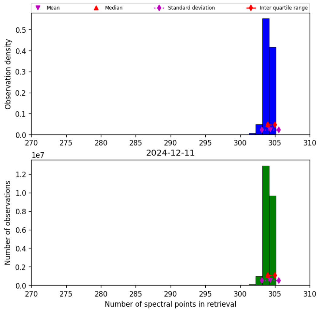
Figure 31: Histogram of “Number of spectral points in retrieval” for 2024-12-11 to 2024-12-12
