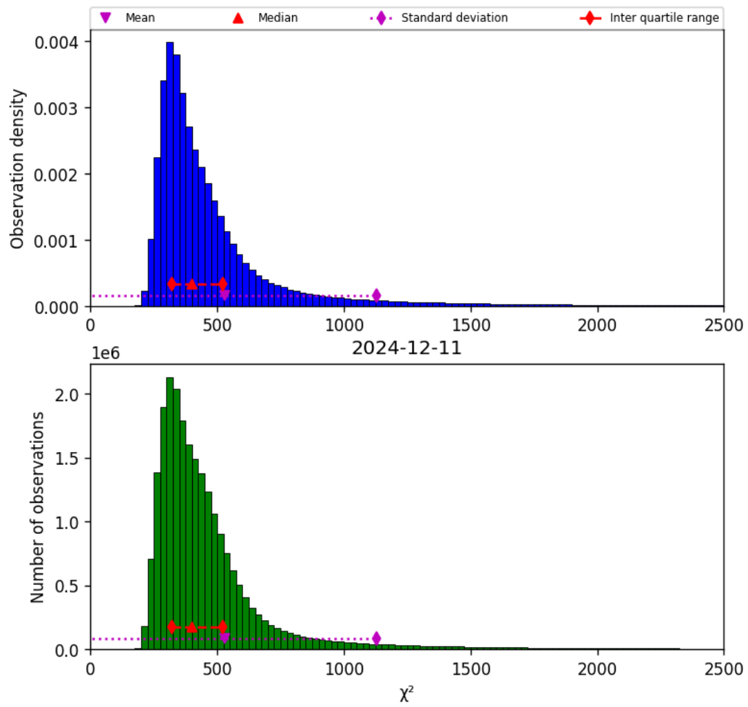
Figure 40: Histogram of “ \chi^2 ” for 2024-12-11 to 2024-12-12
