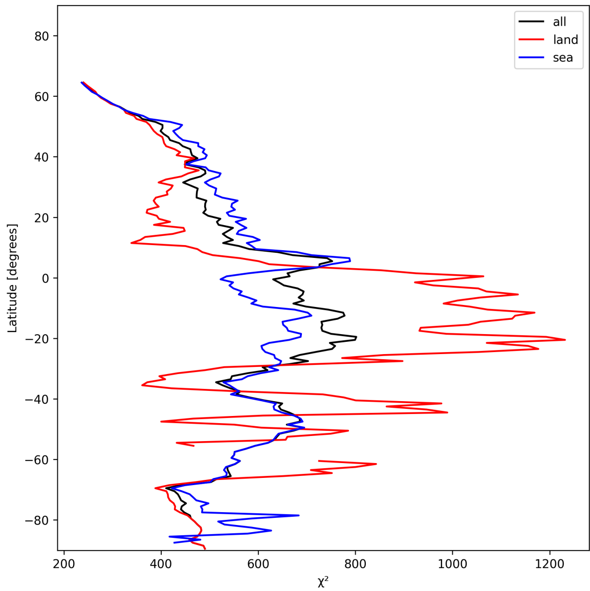
Figure 23: Zonal average of “ \chi^2 ” for 2024-12-11 to 2024-12-12.
