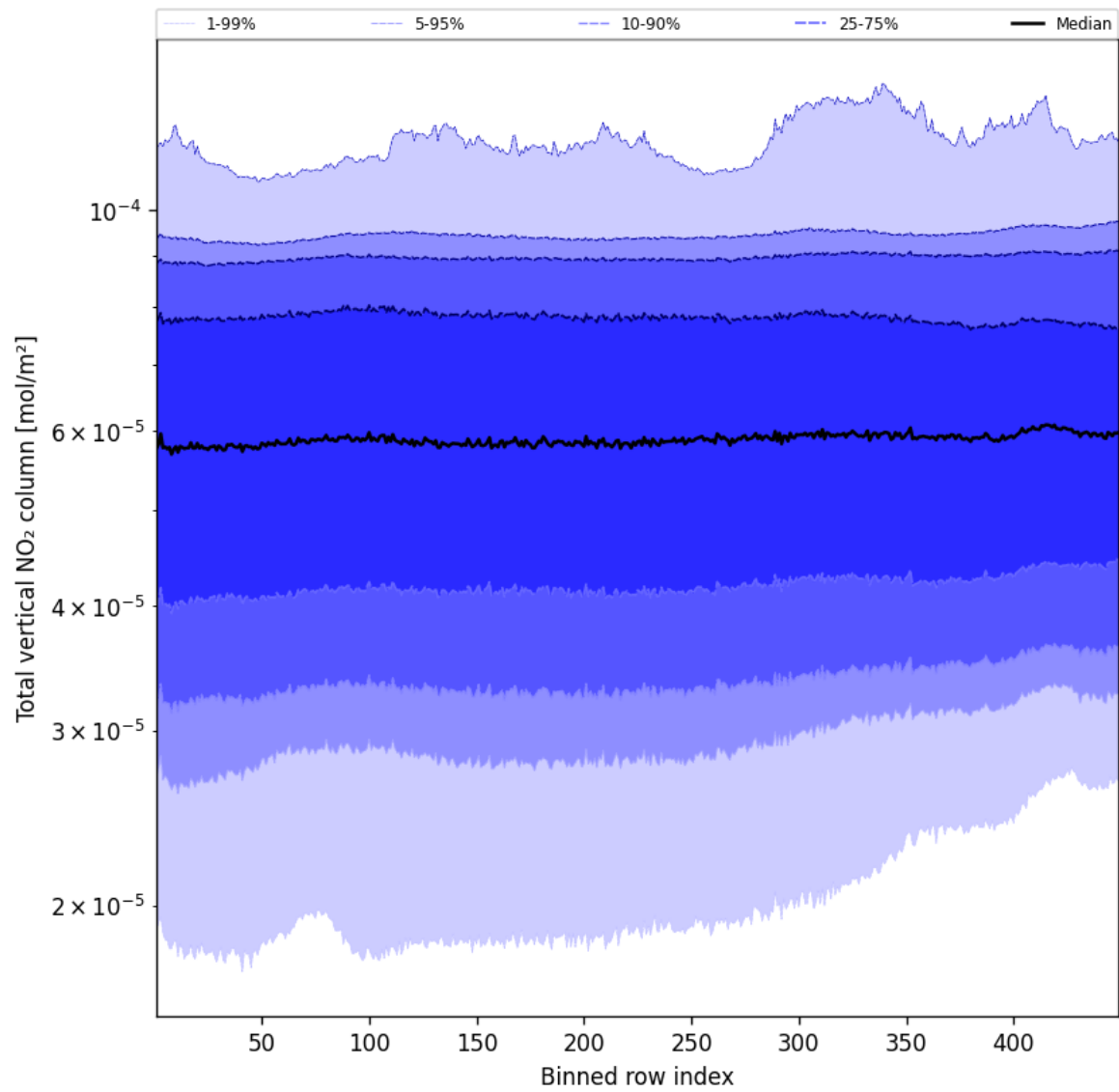
Figure 53: Along track statistics of “Total vertical NO 2 column” for 2024-12-11 to 2024-12-12
