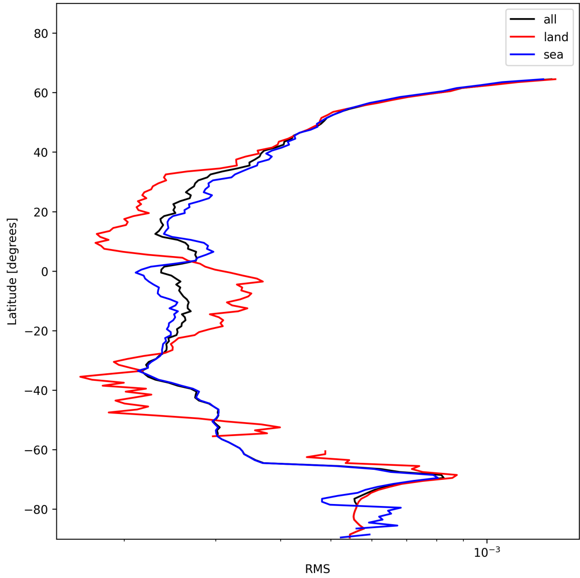
Figure 24: Zonal average of “RMS” for 2024-12-13 to 2024-12-14.
