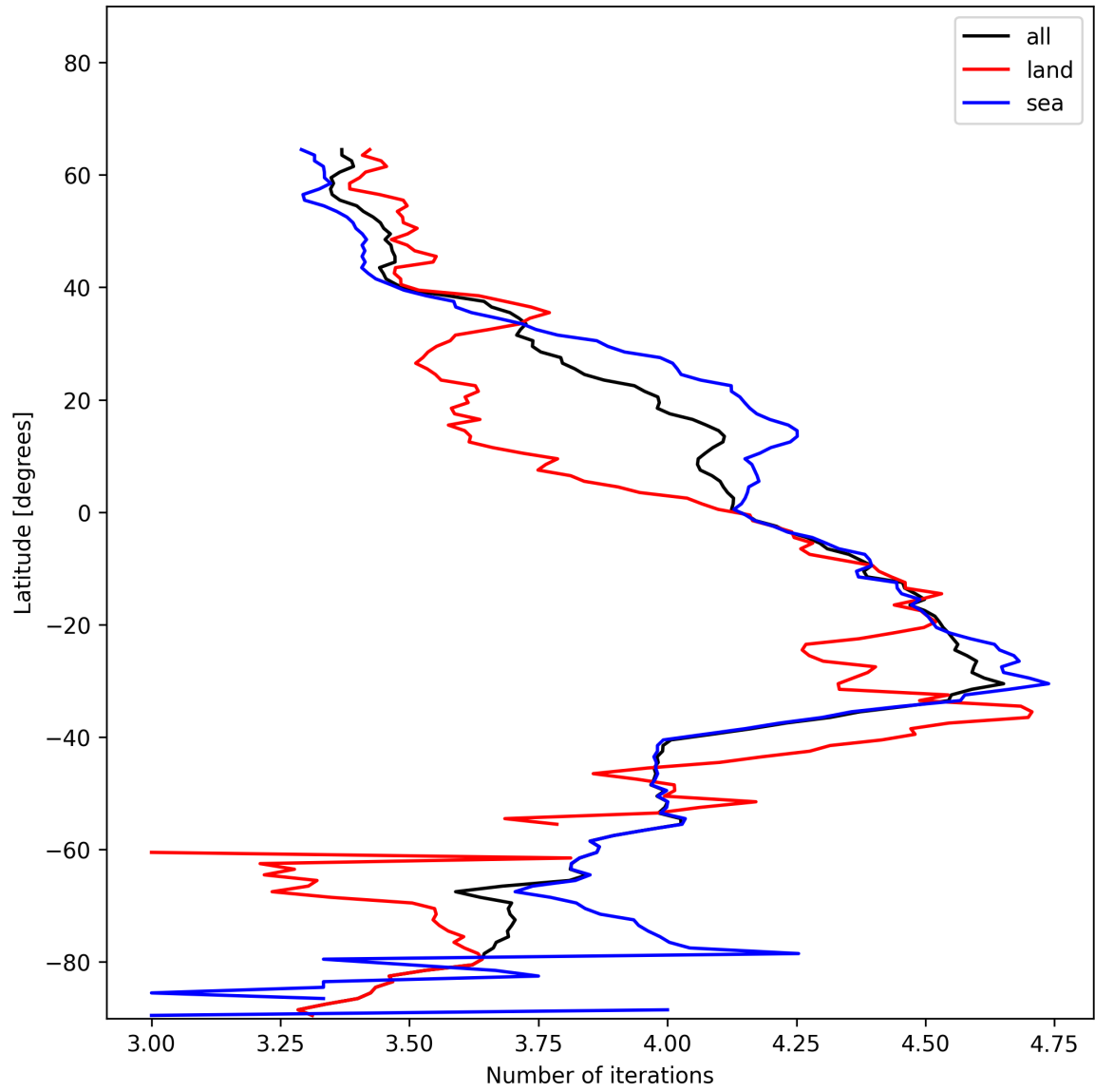
Figure 15: Zonal average of “Number of iterations” for 2024-12-13 to 2024-12-14.
