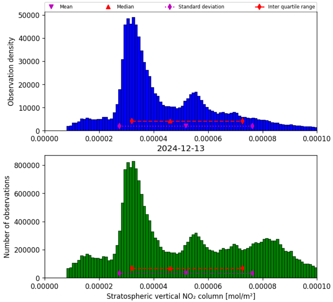
Figure 34: Histogram of “Stratospheric vertical NO 2 column” for 2024-12-13 to 2024-12-14
