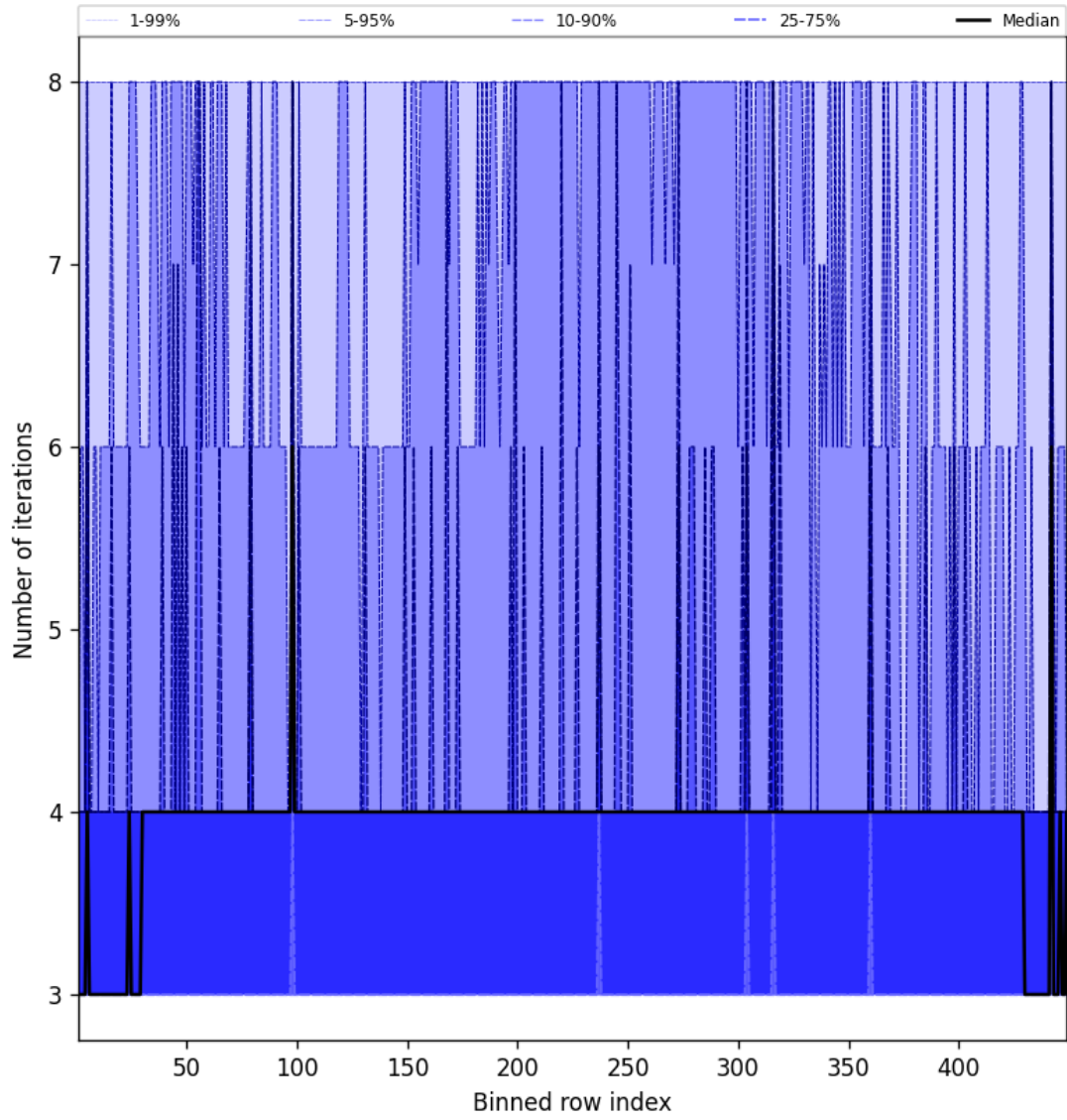
Figure 49: Along track statistics of "Number of iterations" for 2024-12-13 to 2024-12-14
