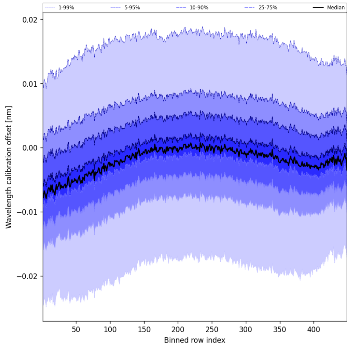
Figure 50: Along track statistics of “Wavelength calibration offset” for 2024-12-13 to 2024-12-14
