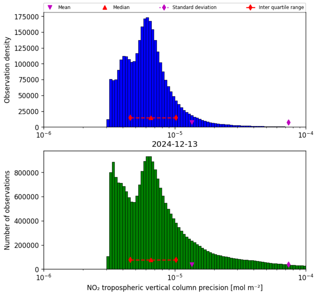
Figure 28: Histogram of “NO 2 tropospheric vertical column precision” for 2024-12-13 to 2024-12-14
