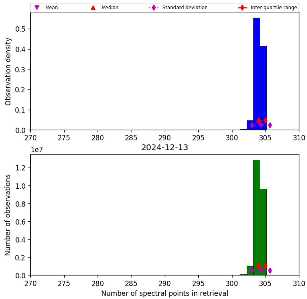
Figure 31: Histogram of “Number of spectral points in retrieval” for 2024-12-13 to 2024-12-14
