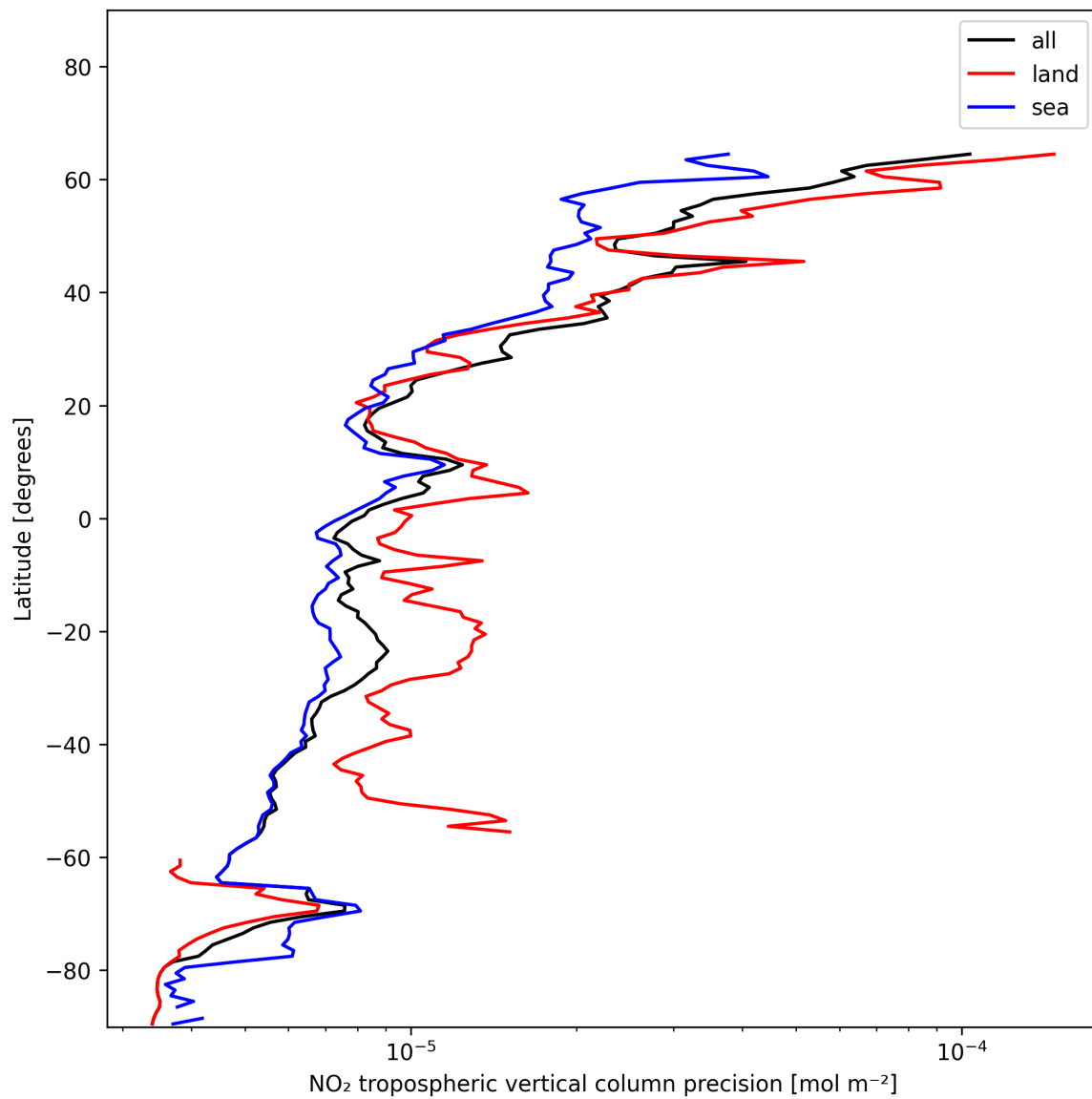
Figure 11: Zonal average of “NO 2 tropospheric vertical column precision” for 2024-12-13 to 2024-12-14.
