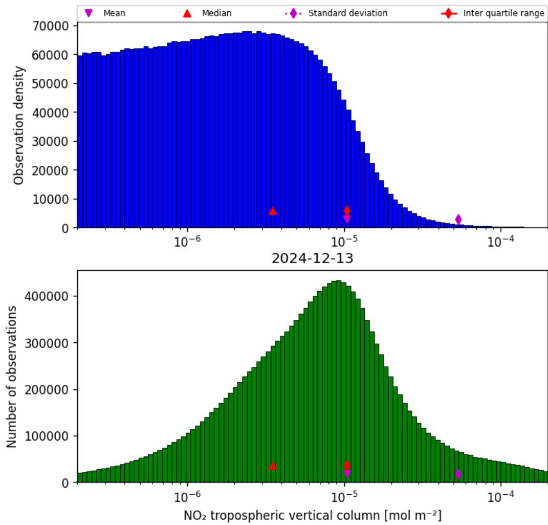
Figure 27: Histogram of “NO 2 tropospheric vertical column” for 2024-12-13 to 2024-12-14
