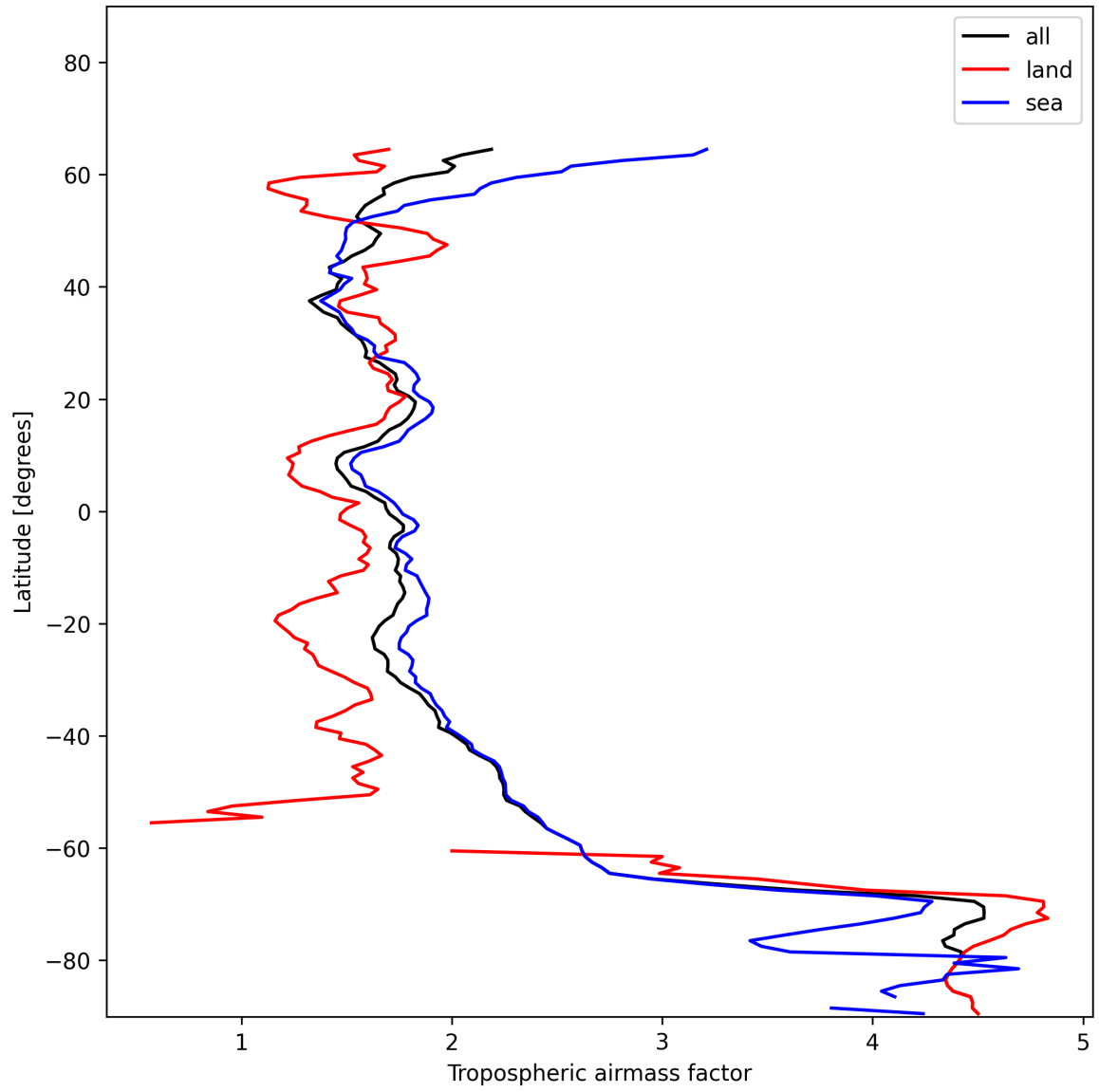
Figure 12: Zonal average of “Tropospheric air mass factor” for 2024-12-13 to 2024-12-14.
