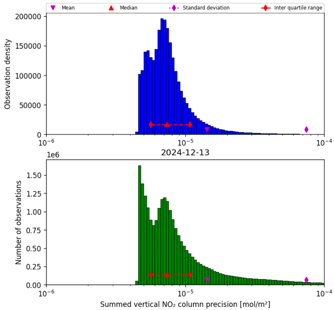
Figure 39: Histogram of “Summed vertical NO 2 column precision” for 2024-12-13 to 2024-12-14
