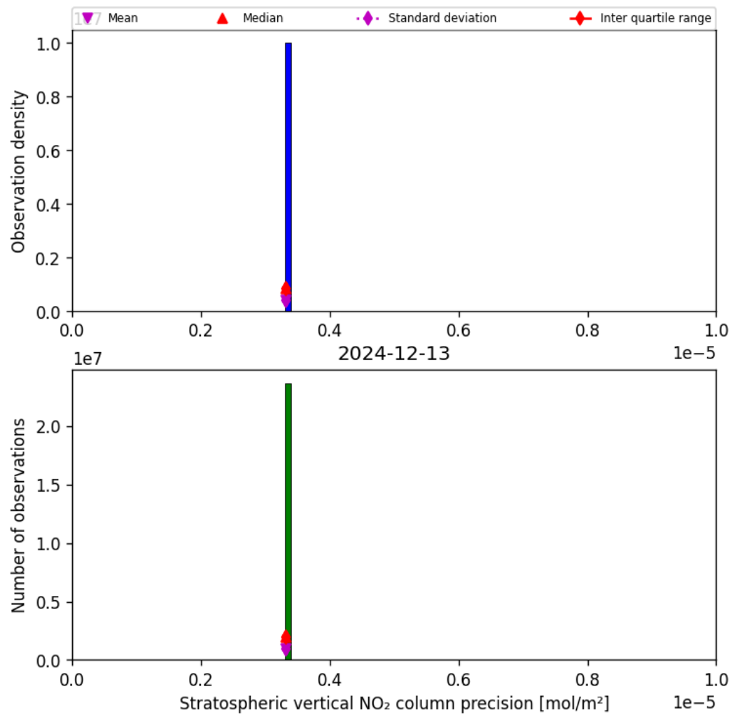
Figure 35: Histogram of “Stratospheric vertical NO 2 column precision” for 2024-12-13 to 2024-12-14
