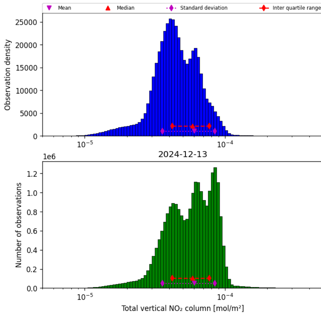
Figure 36: Histogram of “Total vertical NO 2 column” for 2024-12-13 to 2024-12-14
