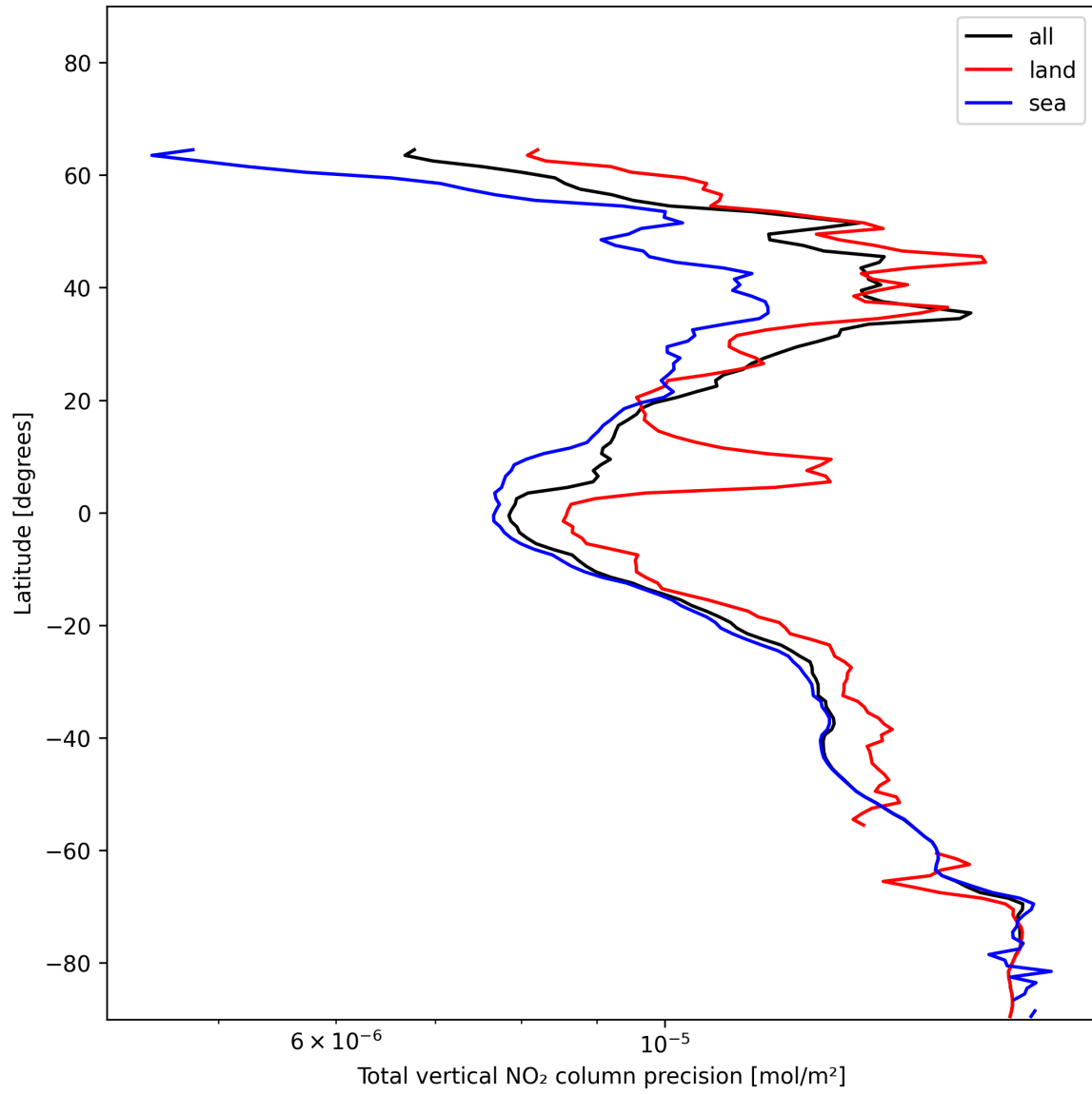
Figure 20: Zonal average of “Total vertical NO 2 column precision” for 2024-12-13 to 2024-12-14.
