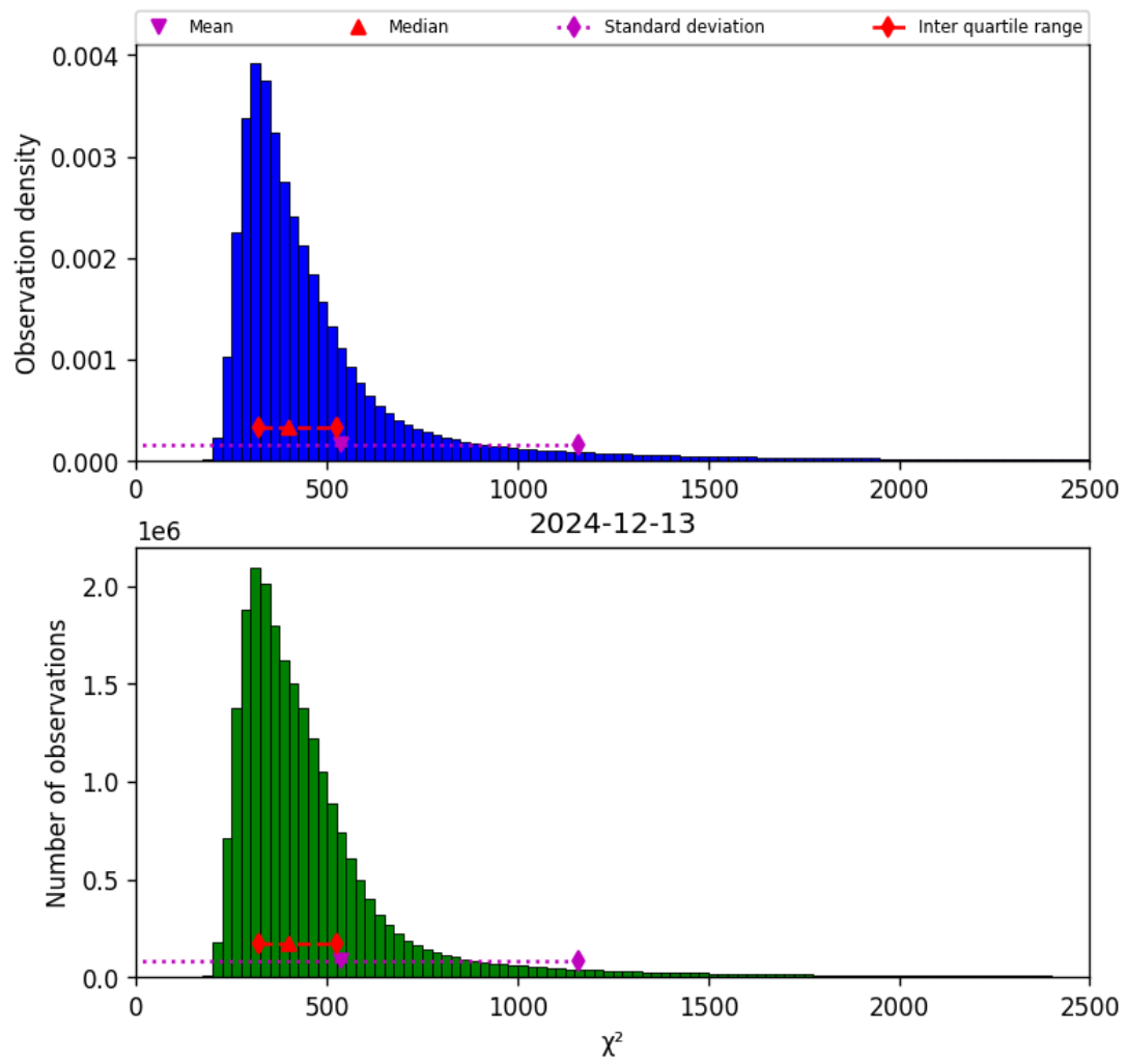
Figure 40: Histogram of “ \chi^2 ” for 2024-12-13 to 2024-12-14
