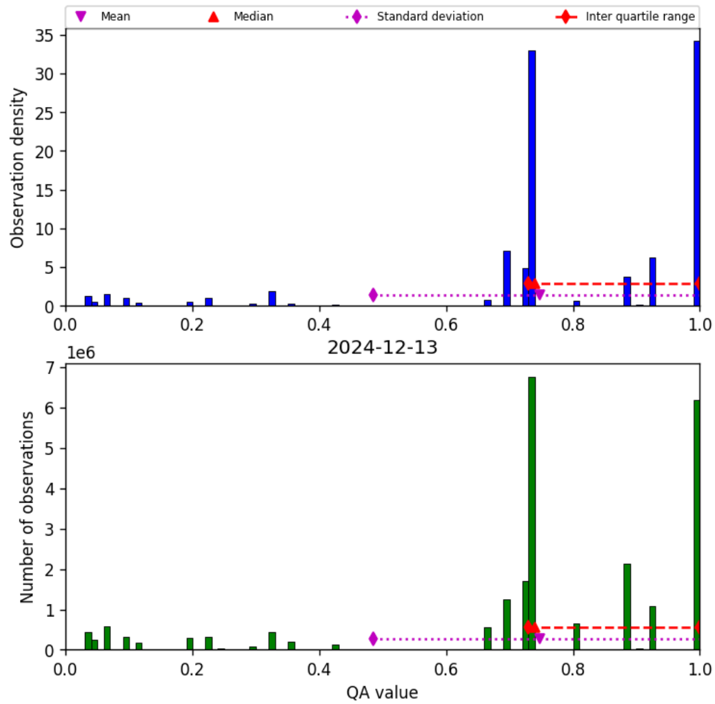
Figure 26: Histogram of “QA value” for 2024-12-13 to 2024-12-14
