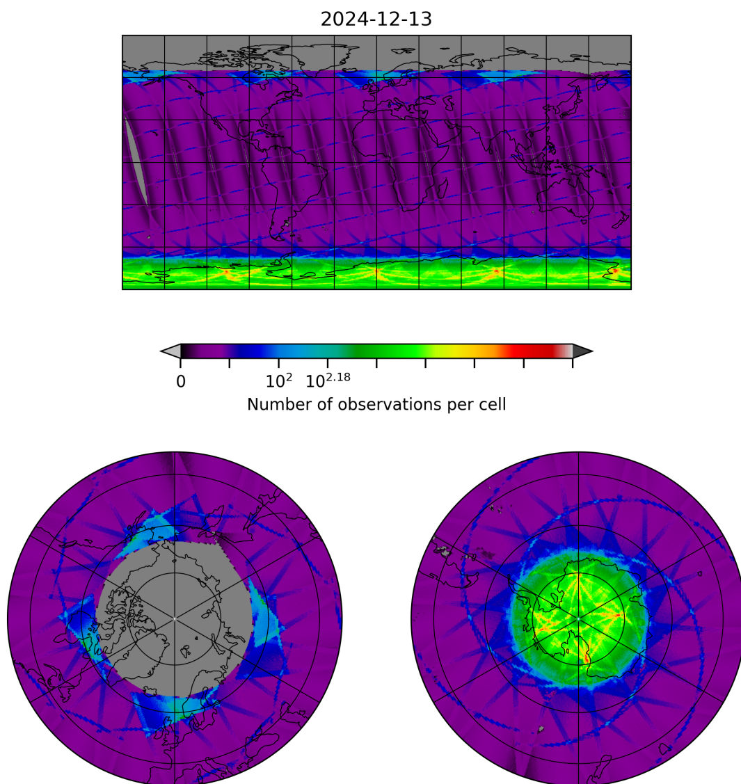
Figure 8: Map of the number of observations for 2024-12-13 to 2024-12-14
