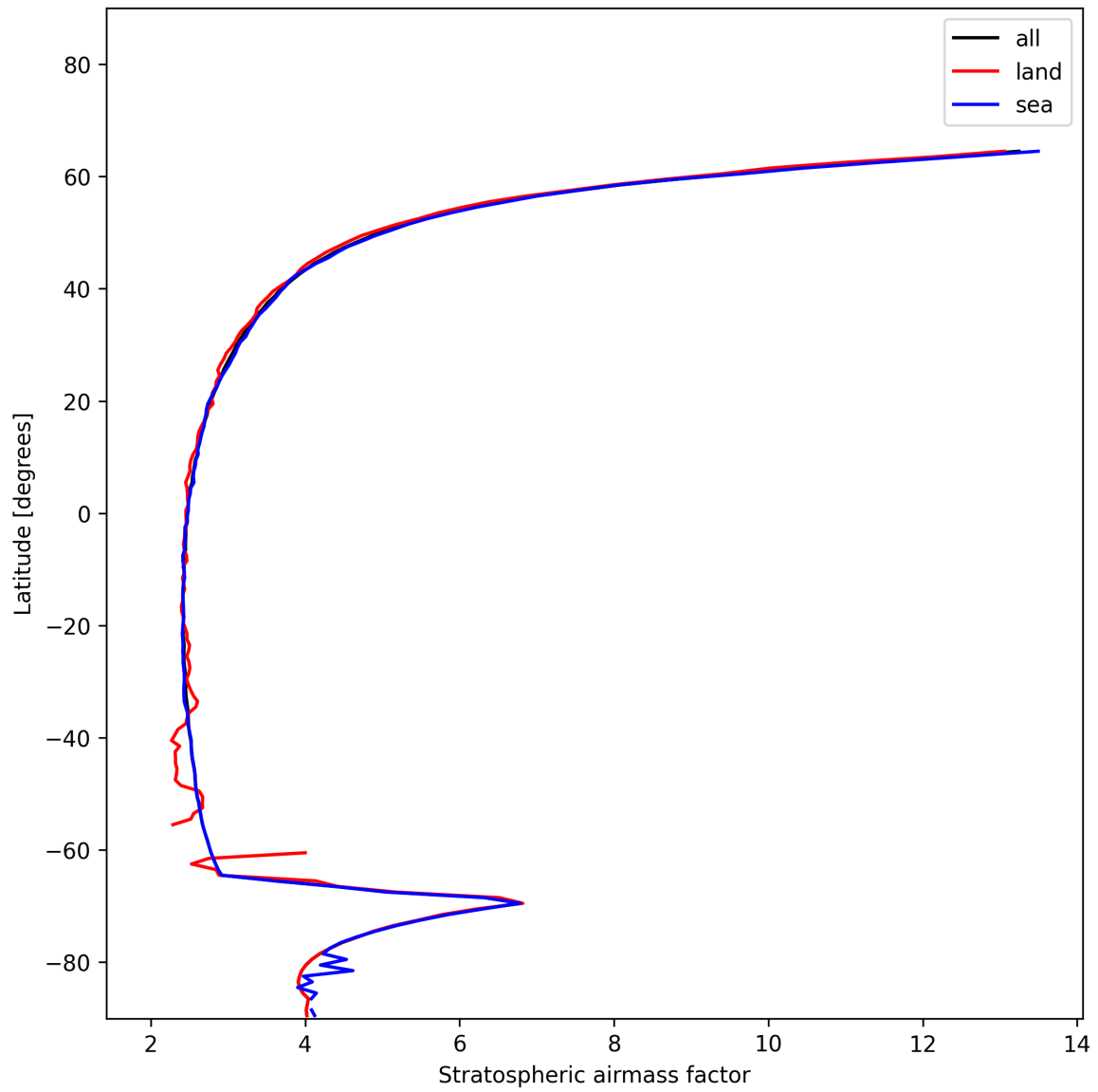
Figure 25: Zonal average of “Stratospheric airmass factor” for 2024-12-13 to 2024-12-14.
