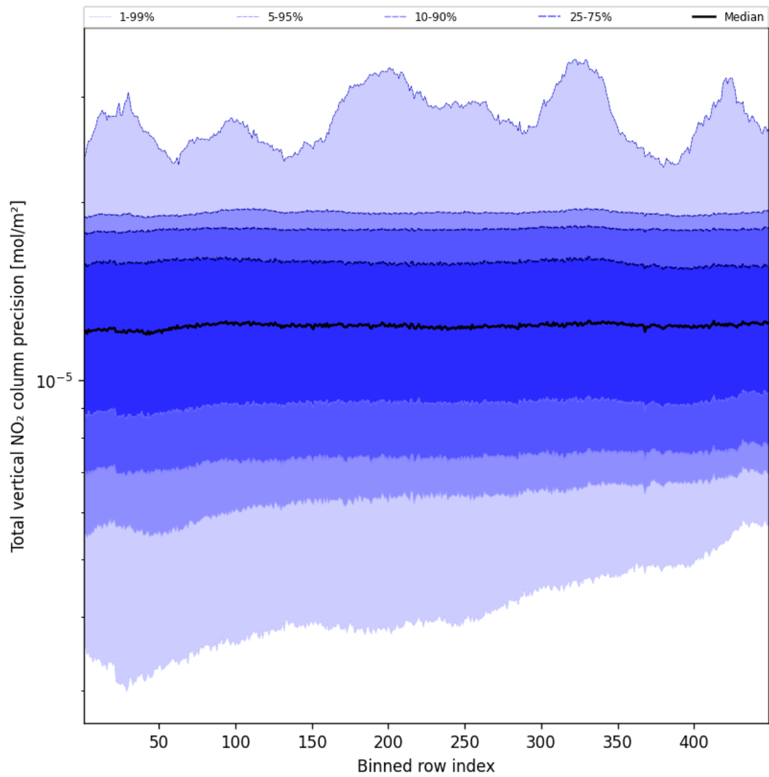
Figure 54: Along track statistics of “Total vertical NO 2 column precision” for 2024-12-13 to 2024-12-14
