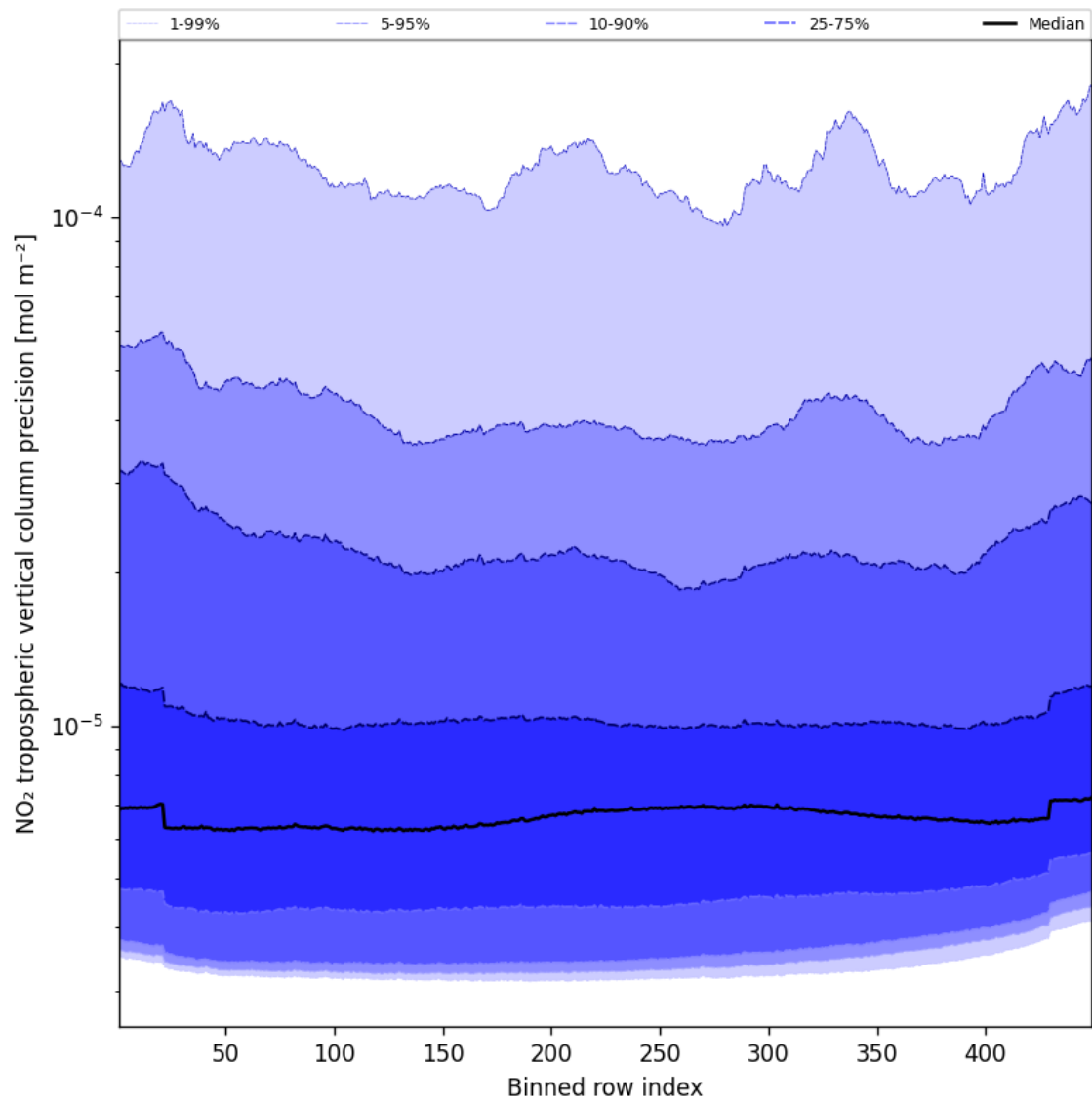
Figure 45: Along track statistics of “NO 2 tropospheric vertical column precision” for 2024-12-13 to 2024-12-14
