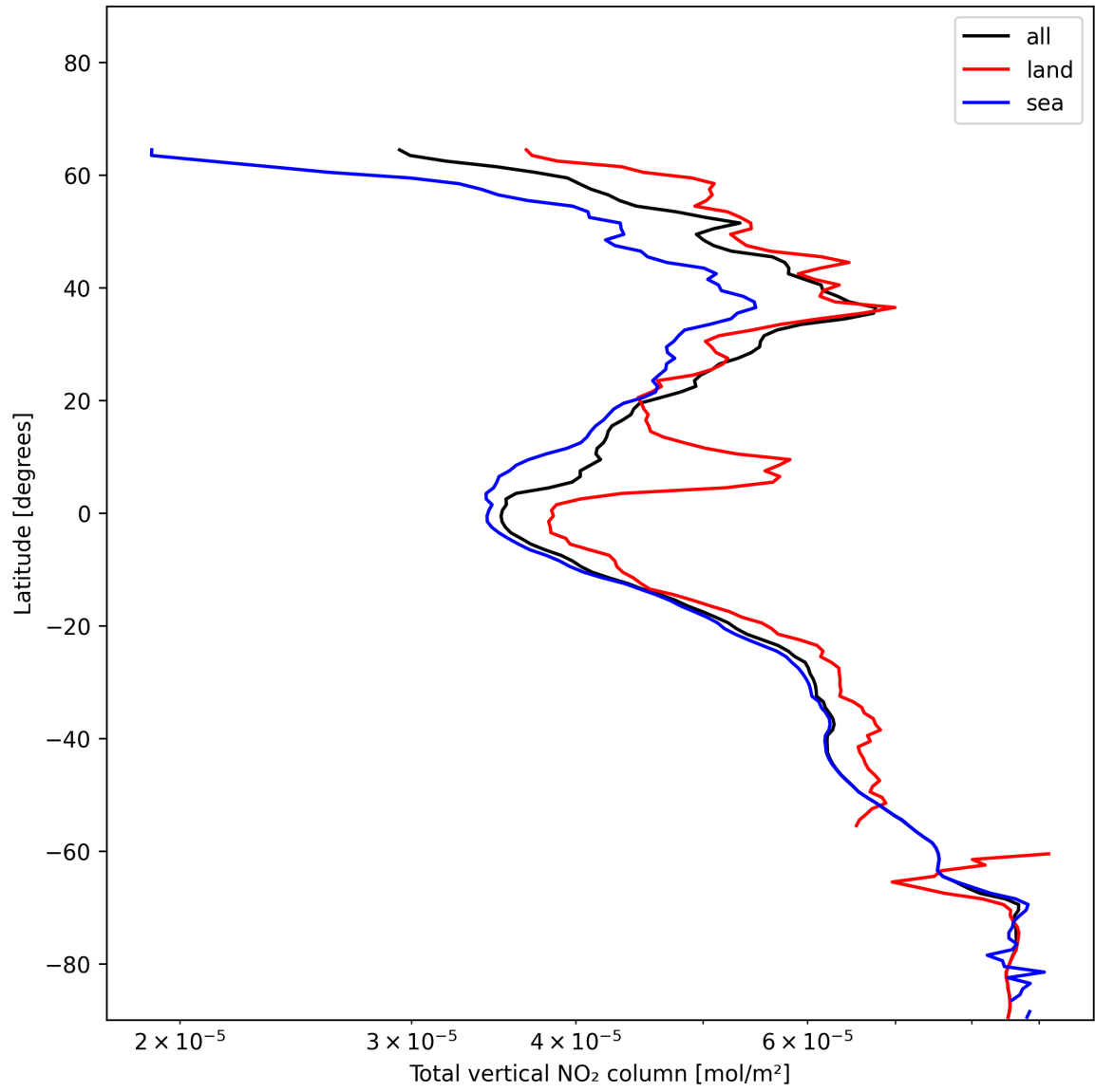
Figure 19: Zonal average of “Total vertical NO 2 column” for 2024-12-13 to 2024-12-14.
