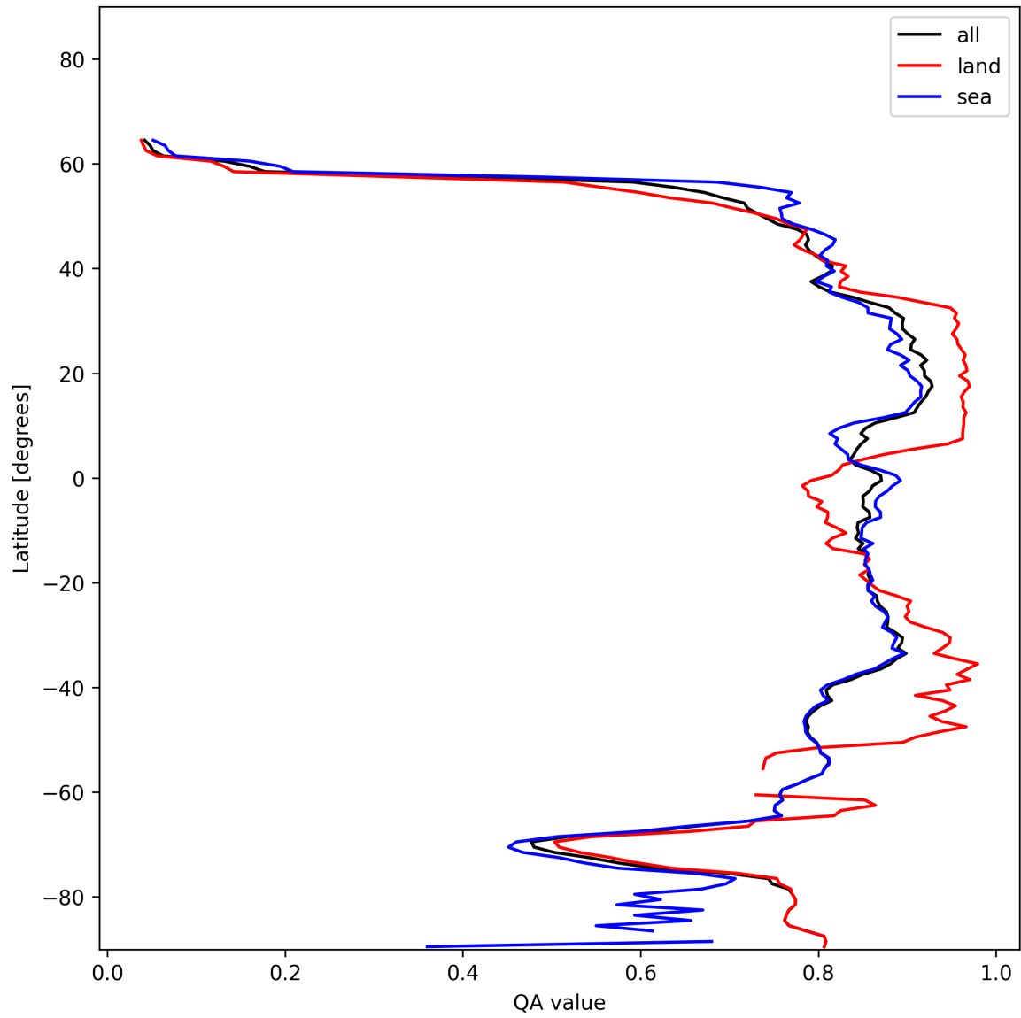
Figure 9: Zonal average of “QA value” for 2024-12-13 to 2024-12-14.
