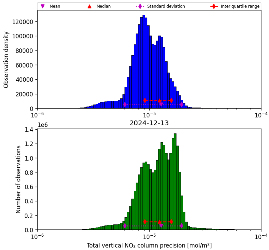
Figure 37: Histogram of “Total vertical NO 2 column precision” for 2024-12-13 to 2024-12-14
