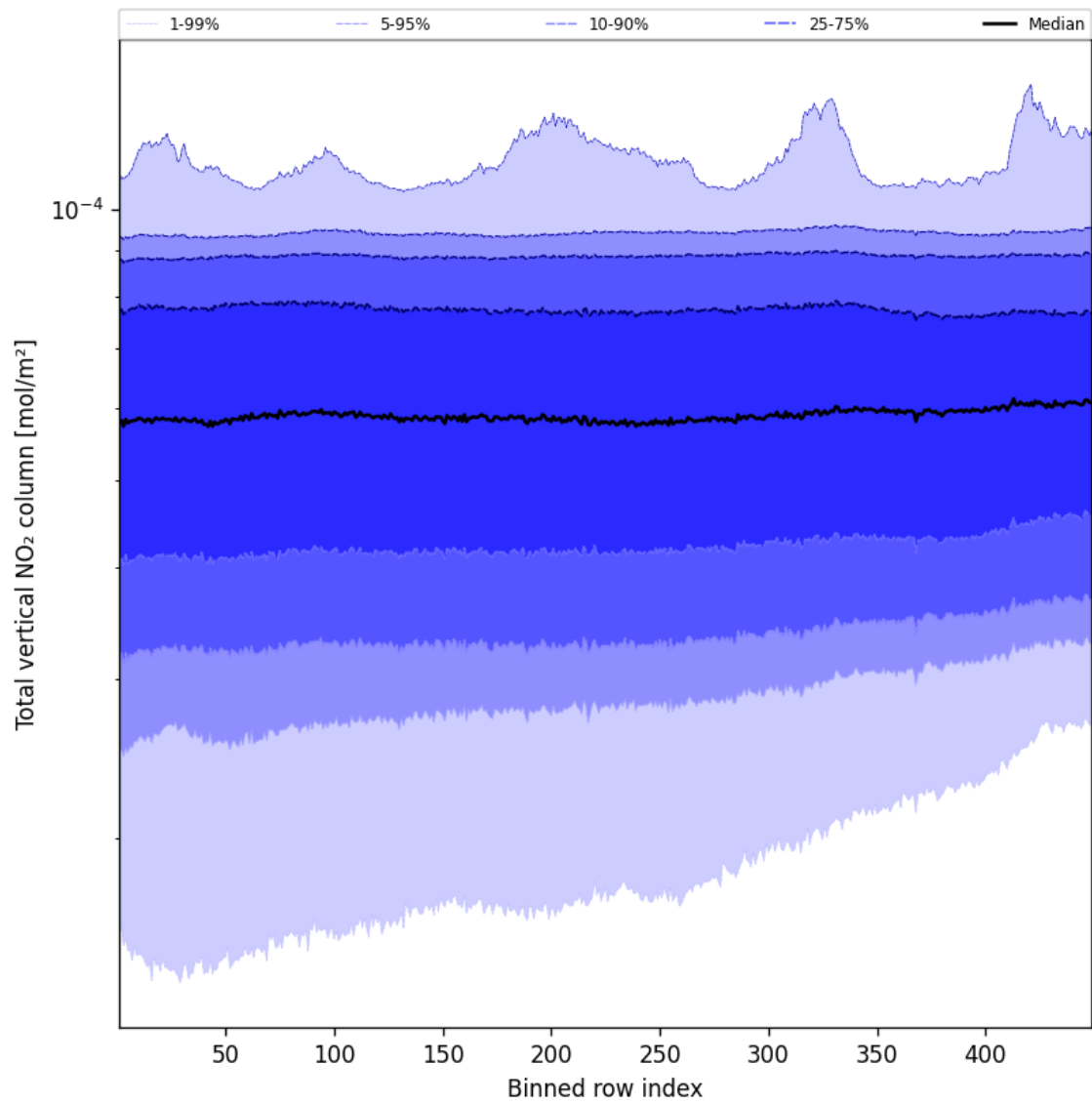
Figure 53: Along track statistics of “Total vertical NO 2 column” for 2024-12-13 to 2024-12-14
