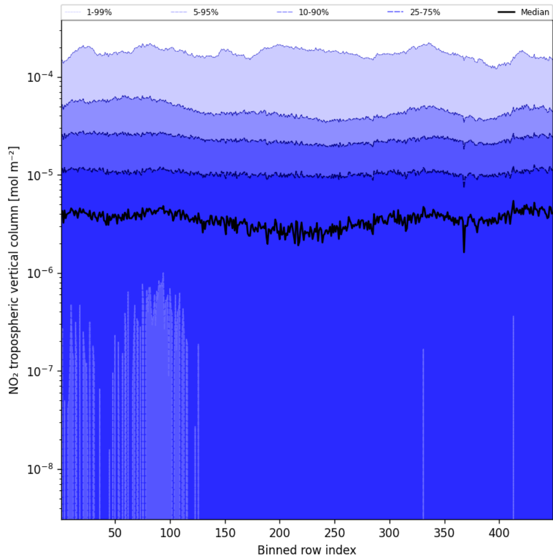
Figure 44: Along track statistics of “NO 2 tropospheric vertical column” for 2024-12-13 to 2024-12-14
