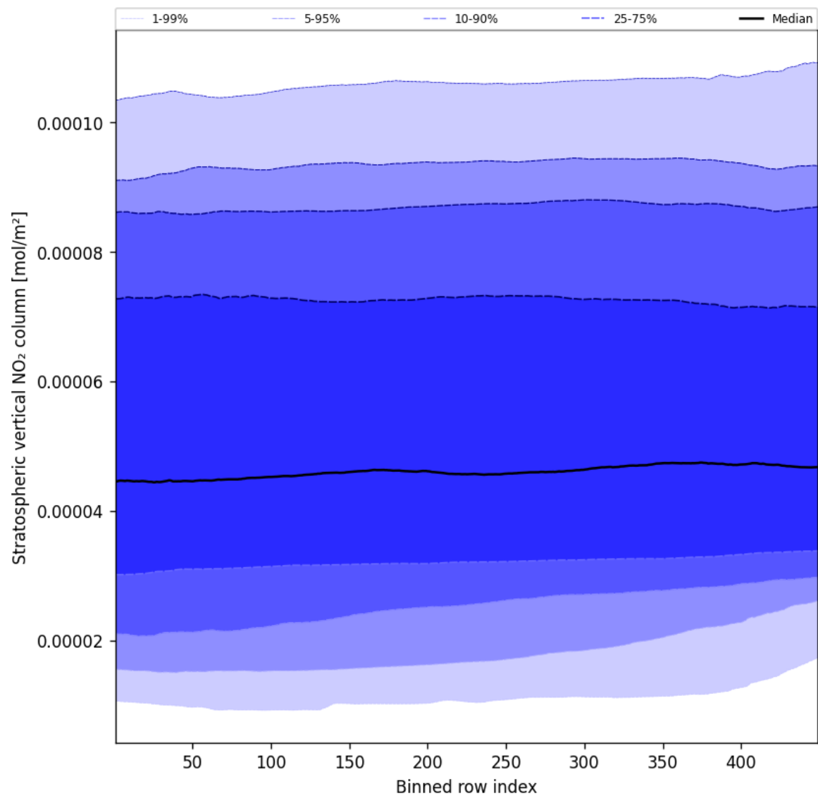
Figure 51: Along track statistics of “Stratospheric vertical NO 2 column” for 2024-12-13 to 2024-12-14
