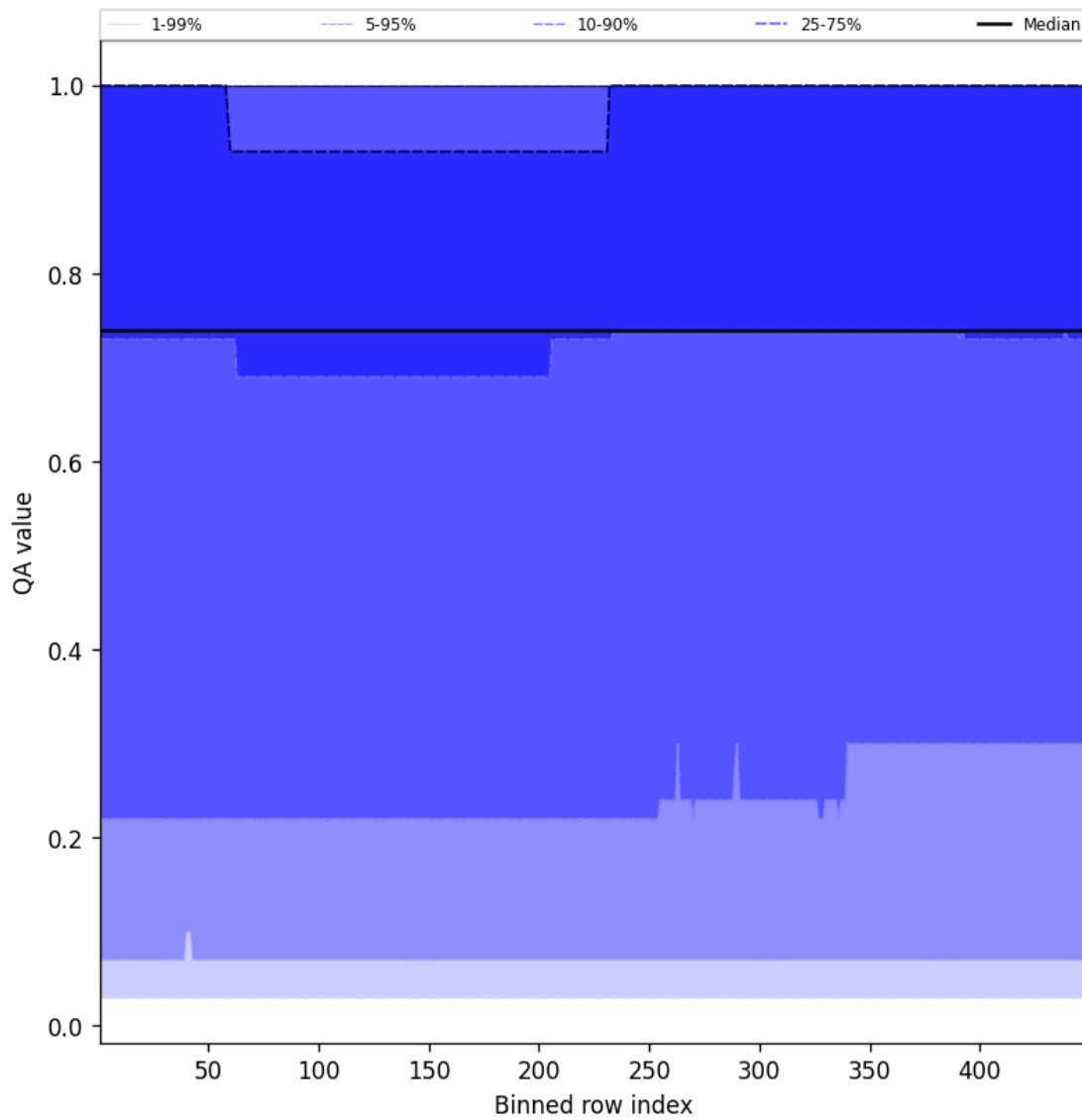
Figure 43: Along track statistics of "QA value" for 2024-12-13 to 2024-12-14
