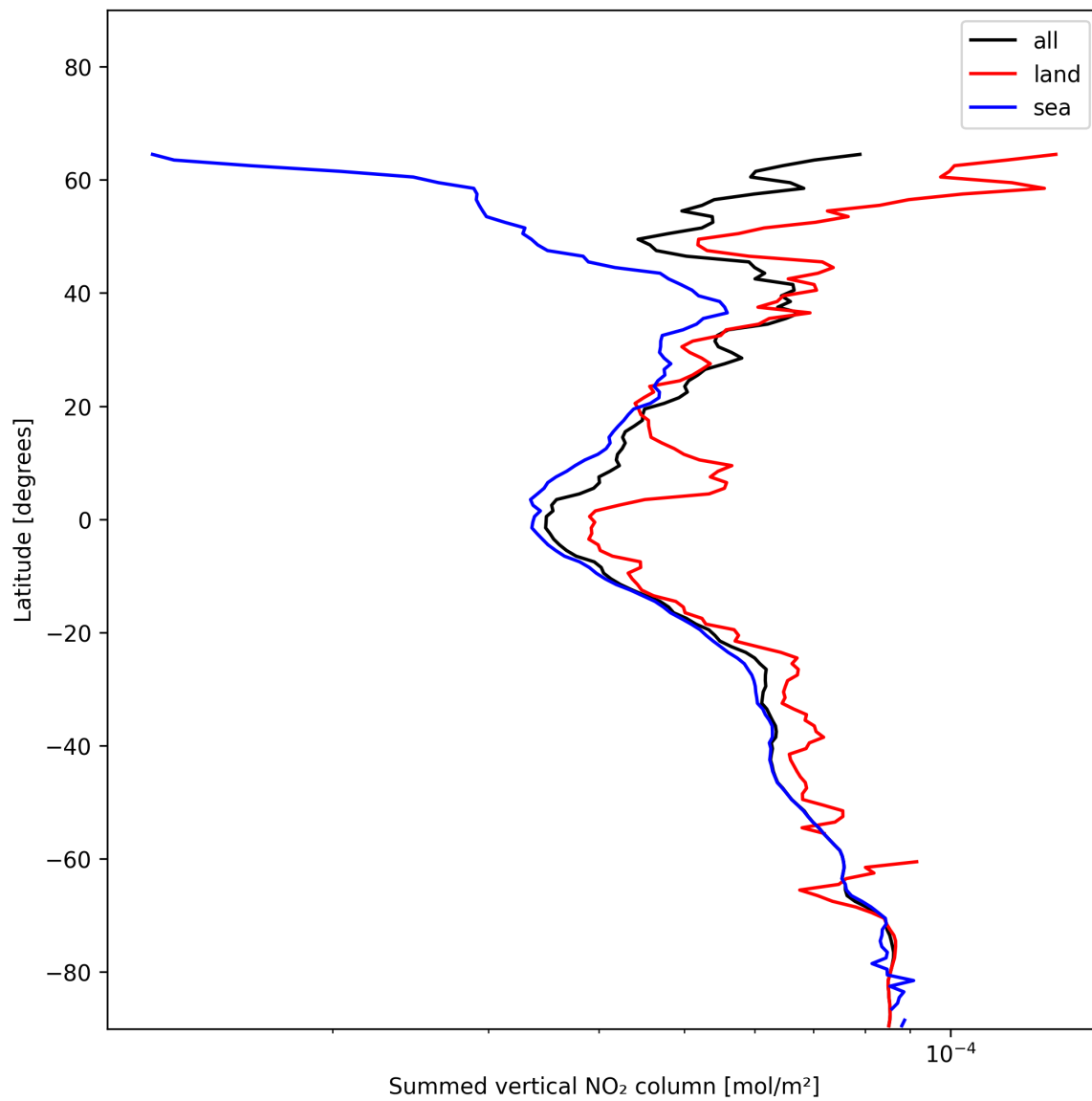
Figure 21: Zonal average of “Summed vertical NO 2 column” for 2024-12-13 to 2024-12-14.
