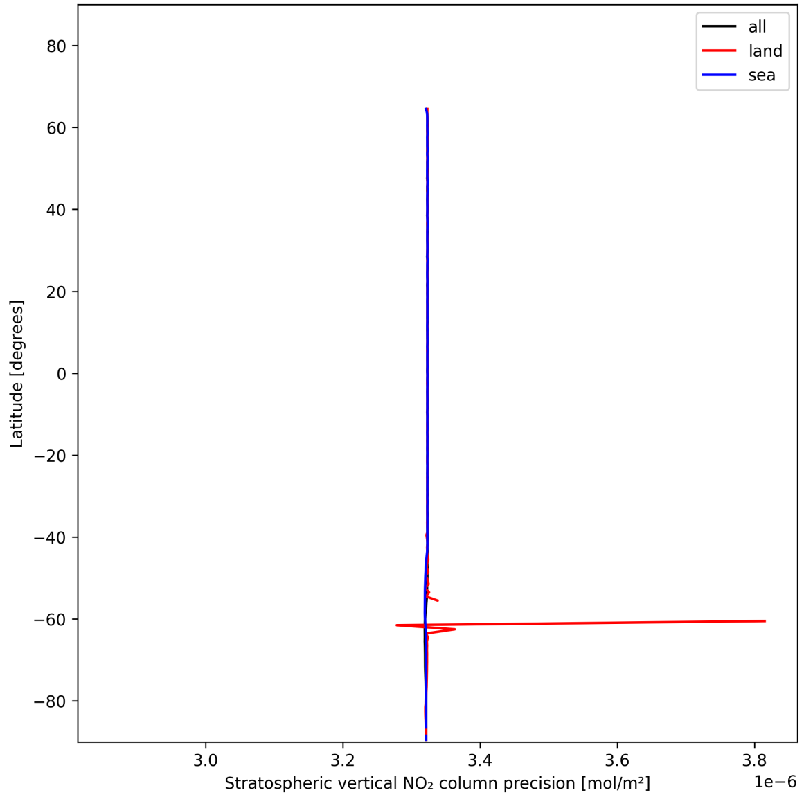
Figure 18: Zonal average of “Stratospheric vertical NO 2 column precision” for 2024-12-13 to 2024-12-14.
