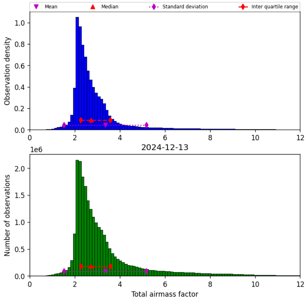
Figure 30: Histogram of “Total airmass factor” for 2024-12-13 to 2024-12-14
