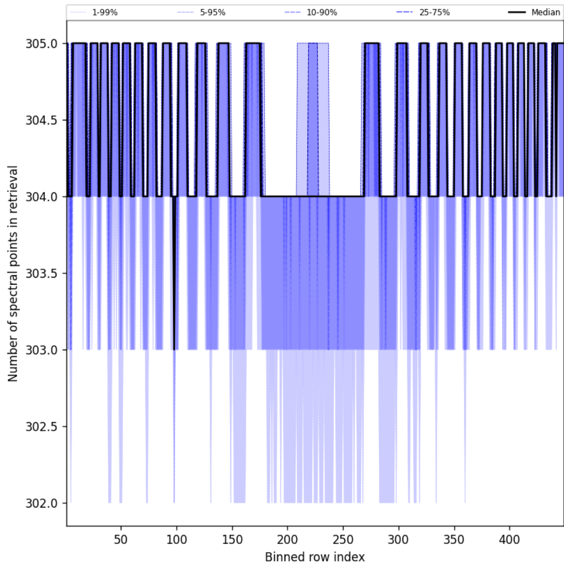
Figure 48: Along track statistics of “Number of spectral points in retrieval” for 2024-12-13 to 2024-12-14
