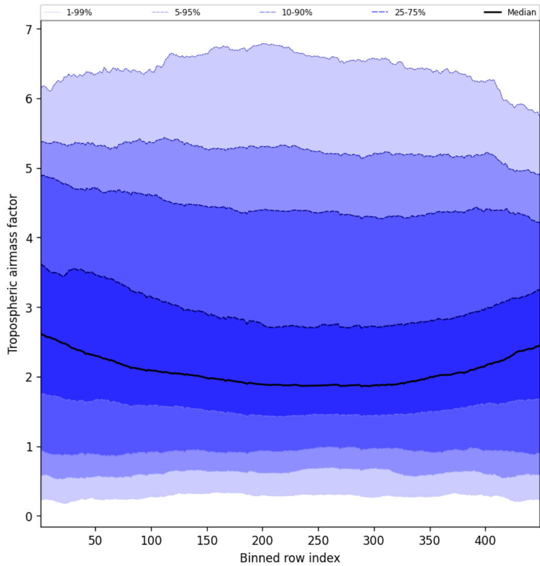
Figure 46: Along track statistics of “Tropospheric airmass factor” for 2024-12-13 to 2024-12-14
