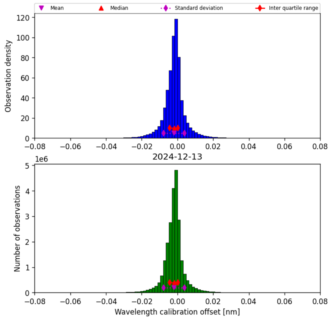
Figure 33: Histogram of “Wavelength calibration offset” for 2024-12-13 to 2024-12-14
