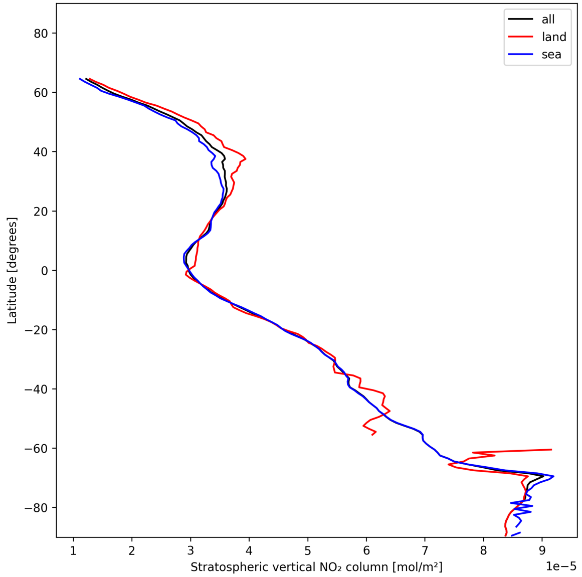
Figure 17: Zonal average of “Stratospheric vertical NO 2 column” for 2024-12-13 to 2024-12-14.
