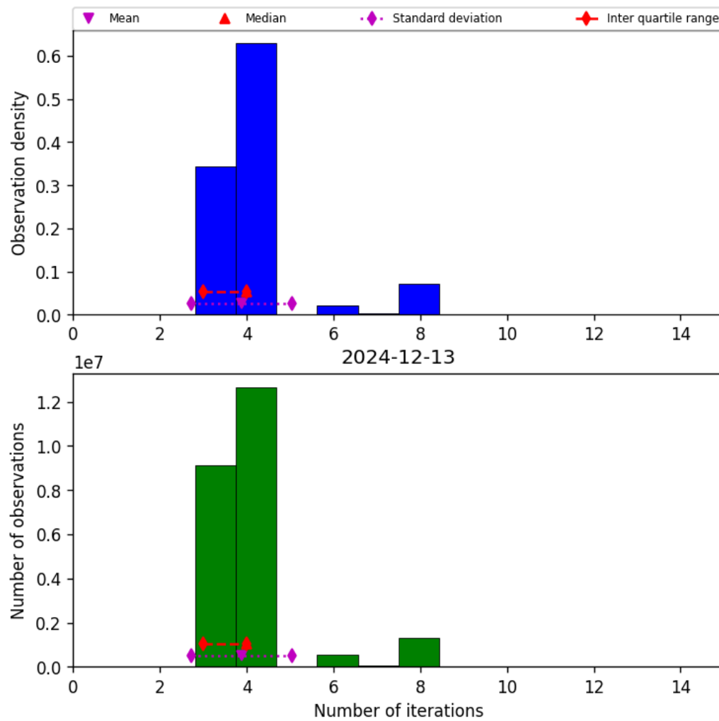
Figure 32: Histogram of “Number of iterations” for 2024-12-13 to 2024-12-14
