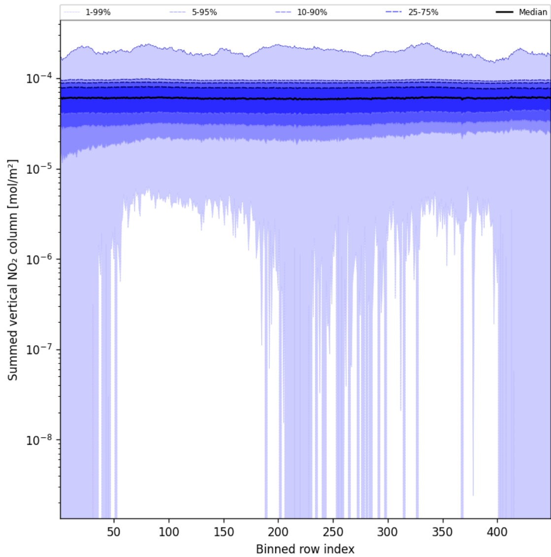
Figure 55: Along track statistics of “Summed vertical NO 2 column” for 2024-12-13 to 2024-12-14
