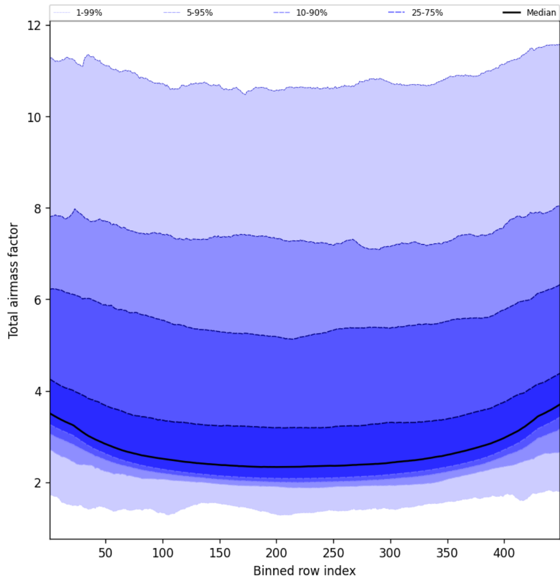
Figure 47: Along track statistics of “Total airmass factor” for 2024-12-13 to 2024-12-14
