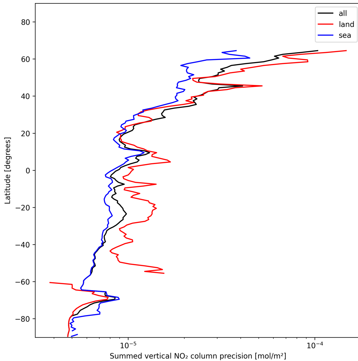
Figure 22: Zonal average of “Summed vertical NO 2 column precision” for 2024-12-13 to 2024-12-14.
