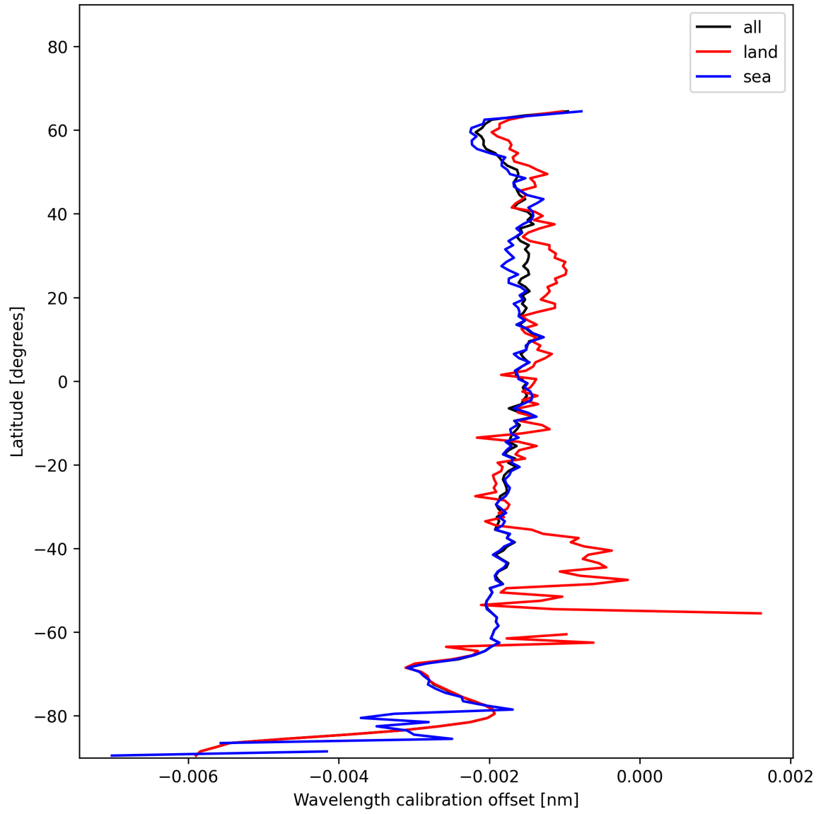
Figure 16: Zonal average of “Wavelength calibration offset” for 2024-12-13 to 2024-12-14.
