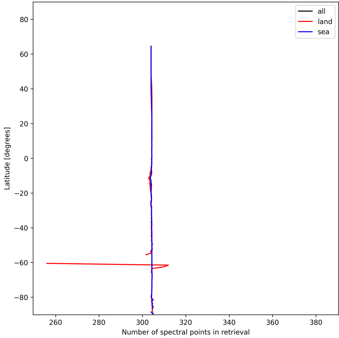
Figure 14: Zonal average of “Number of spectral points in retrieval” for 2024-12-13 to 2024-12-14.
