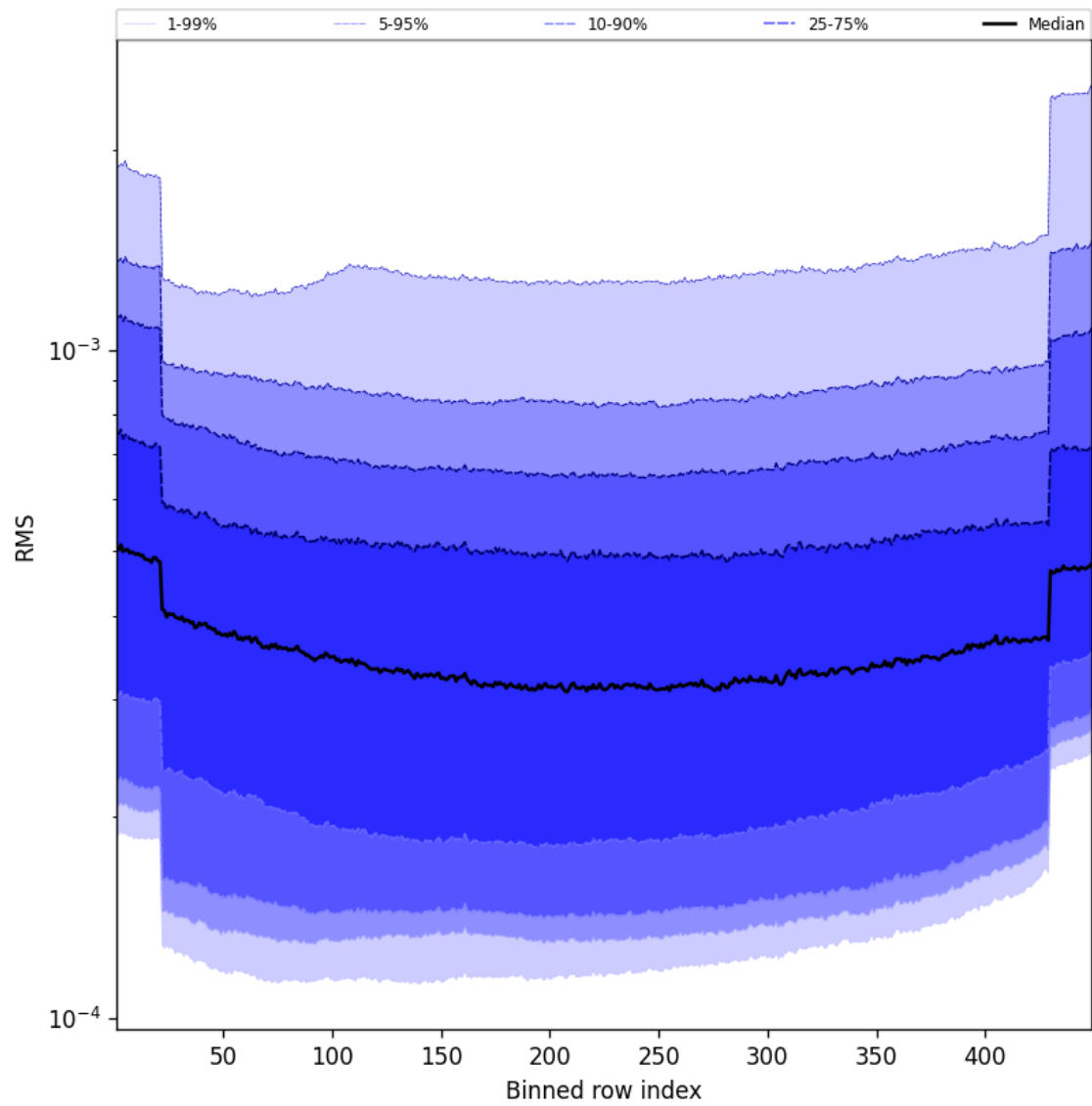
Figure 58: Along track statistics of “RMS” for 2024-12-13 to 2024-12-14
