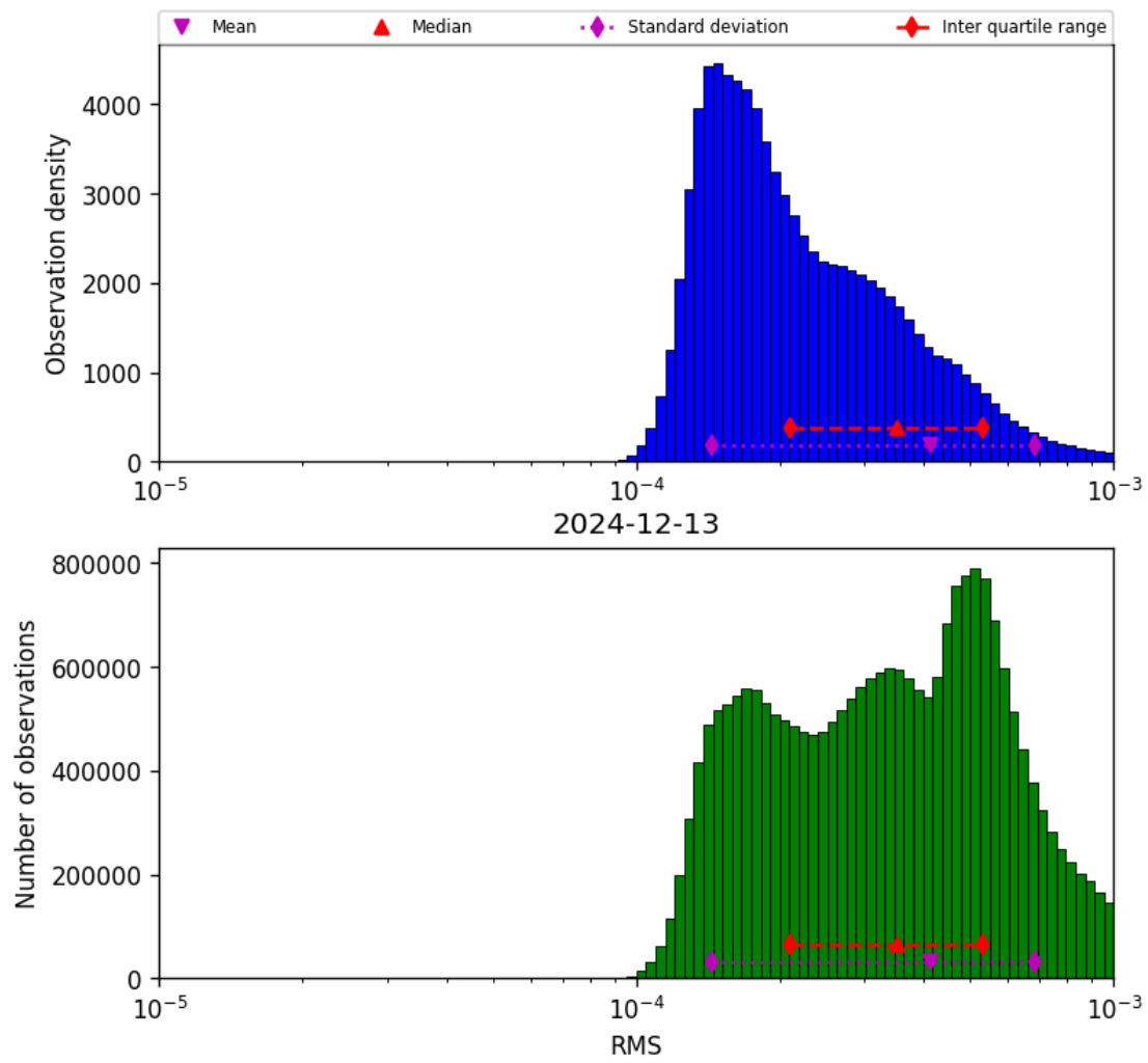
Figure 41: Histogram of “RMS” for 2024-12-13 to 2024-12-14
