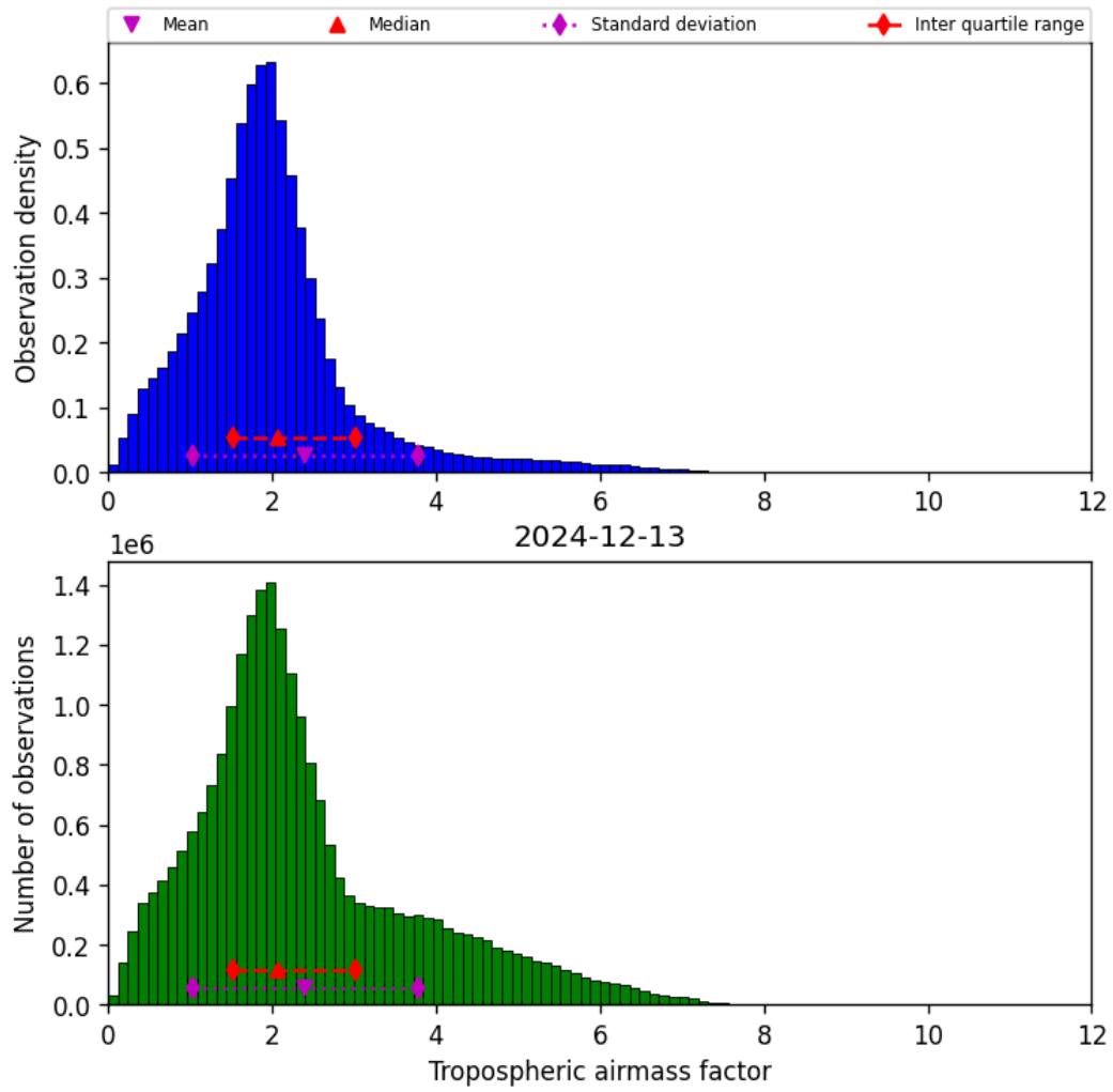
Figure 29: Histogram of “Tropospheric airmass factor” for 2024-12-13 to 2024-12-14
