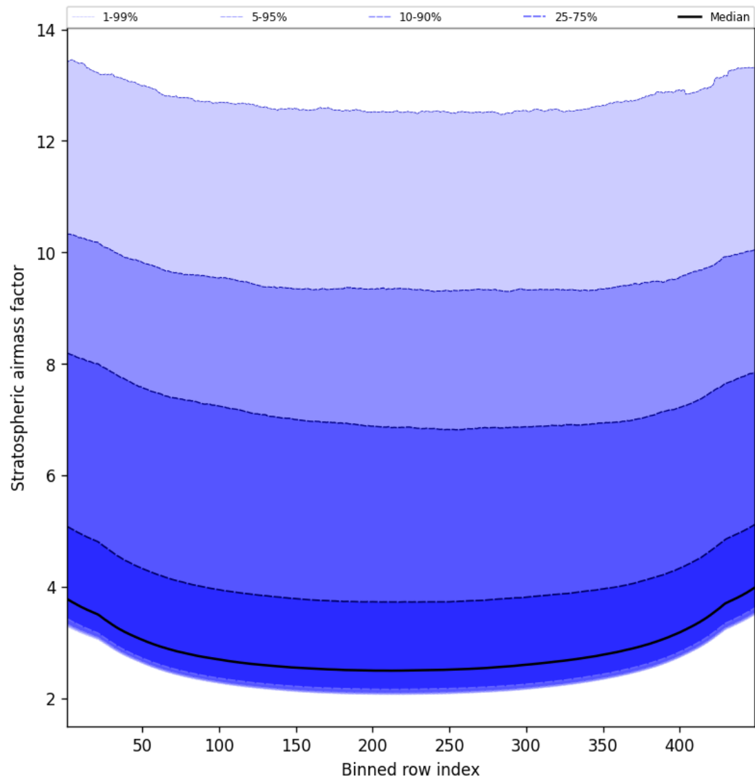
Figure 59: Along track statistics of “Stratospheric airmass factor” for 2024-12-13 to 2024-12-14
