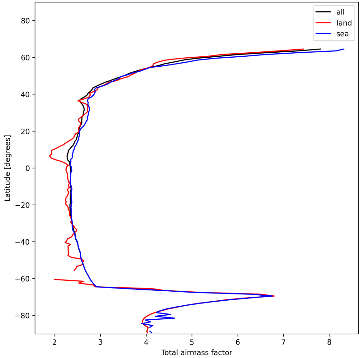
Figure 13: Zonal average of “Total airmass factor” for 2024-12-13 to 2024-12-14.
