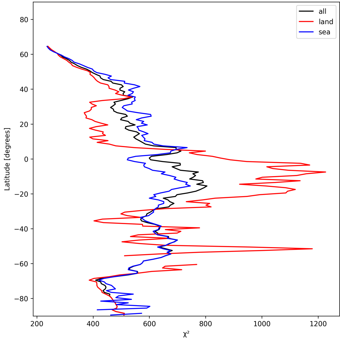
Figure 23: Zonal average of “ \chi^2 ” for 2024-12-13 to 2024-12-14.
