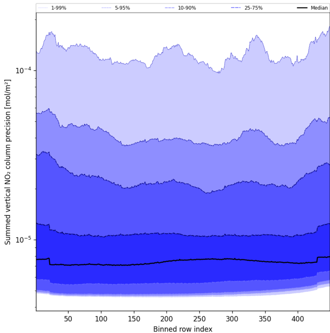
Figure 56: Along track statistics of “Summed vertical NO 2 column precision” for 2024-12-13 to 2024-12-14
