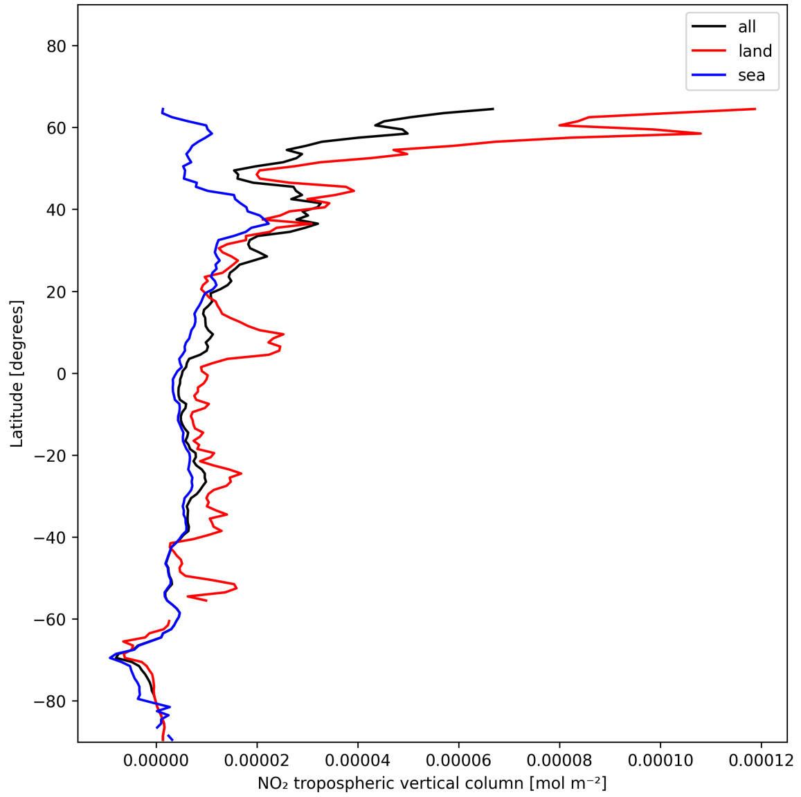
Figure 10: Zonal average of “NO 2 tropospheric vertical column” for 2024-12-13 to 2024-12-14.
