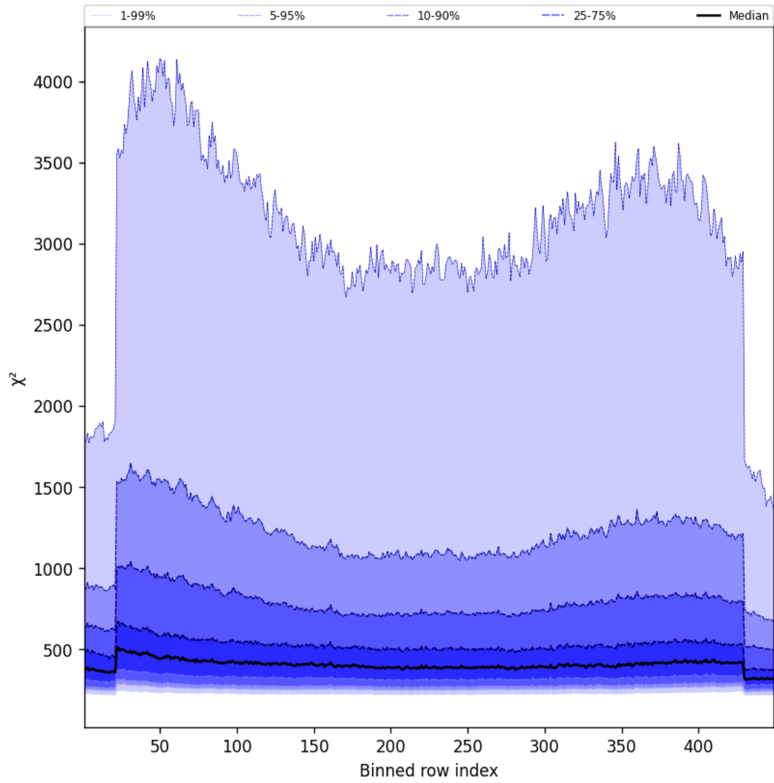
Figure 57: Along track statistics of “ \chi^2 ” for 2024-12-13 to 2024-12-14
