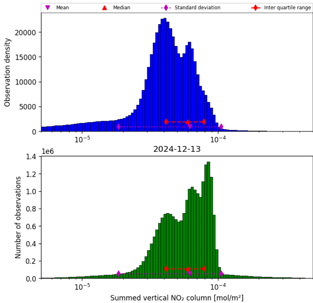
Figure 38: Histogram of “Summed vertical NO 2 column” for 2024-12-13 to 2024-12-14
