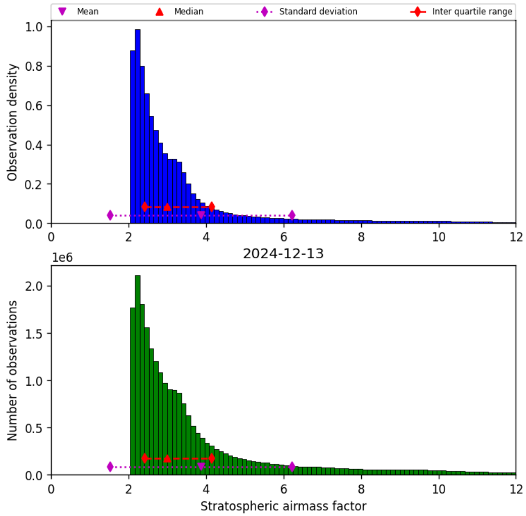
Figure 42: Histogram of “Stratospheric airmass factor” for 2024-12-13 to 2024-12-14
